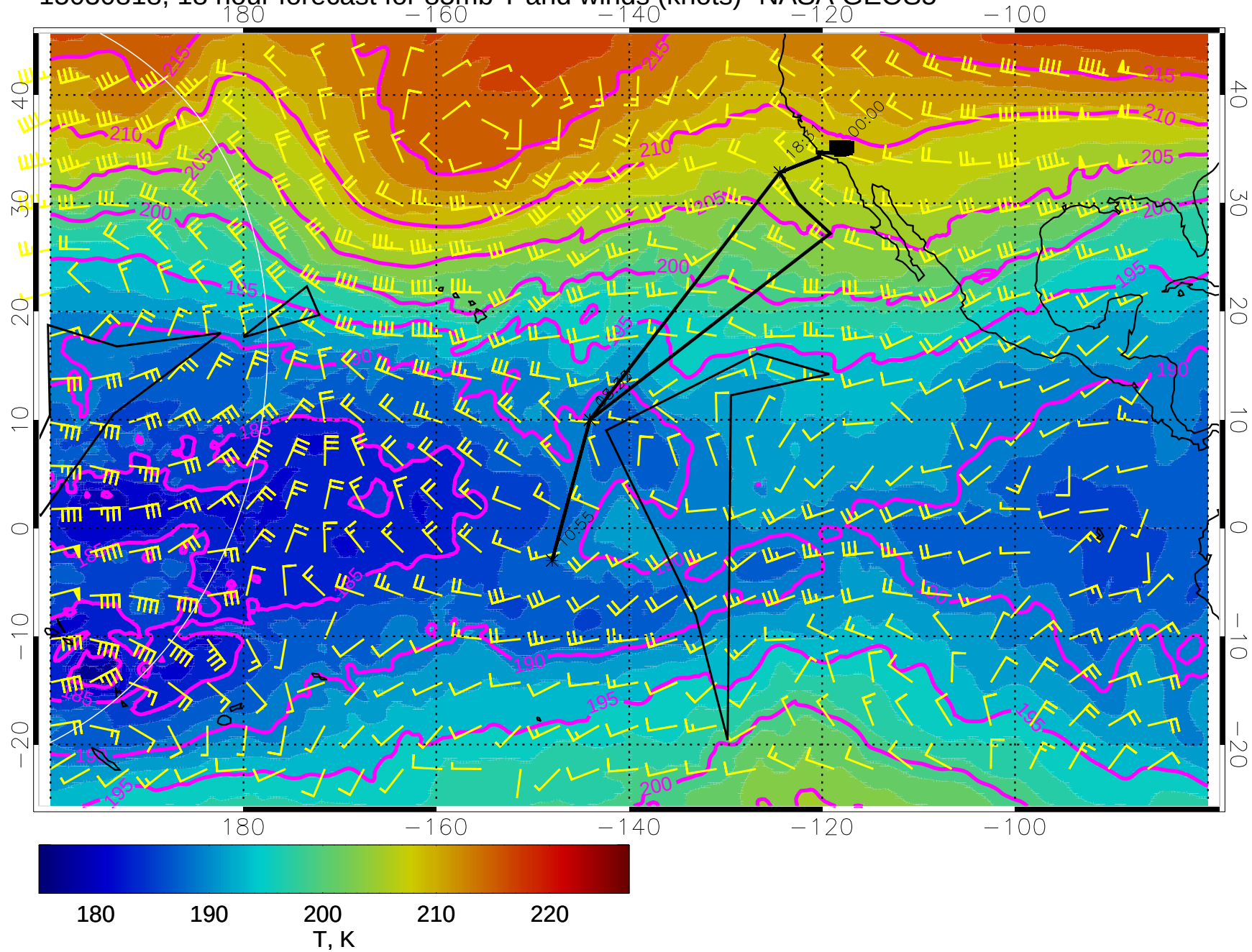
15030818, 18 hour forecast for 85mb T and winds (knots)- NASA GEOS5
