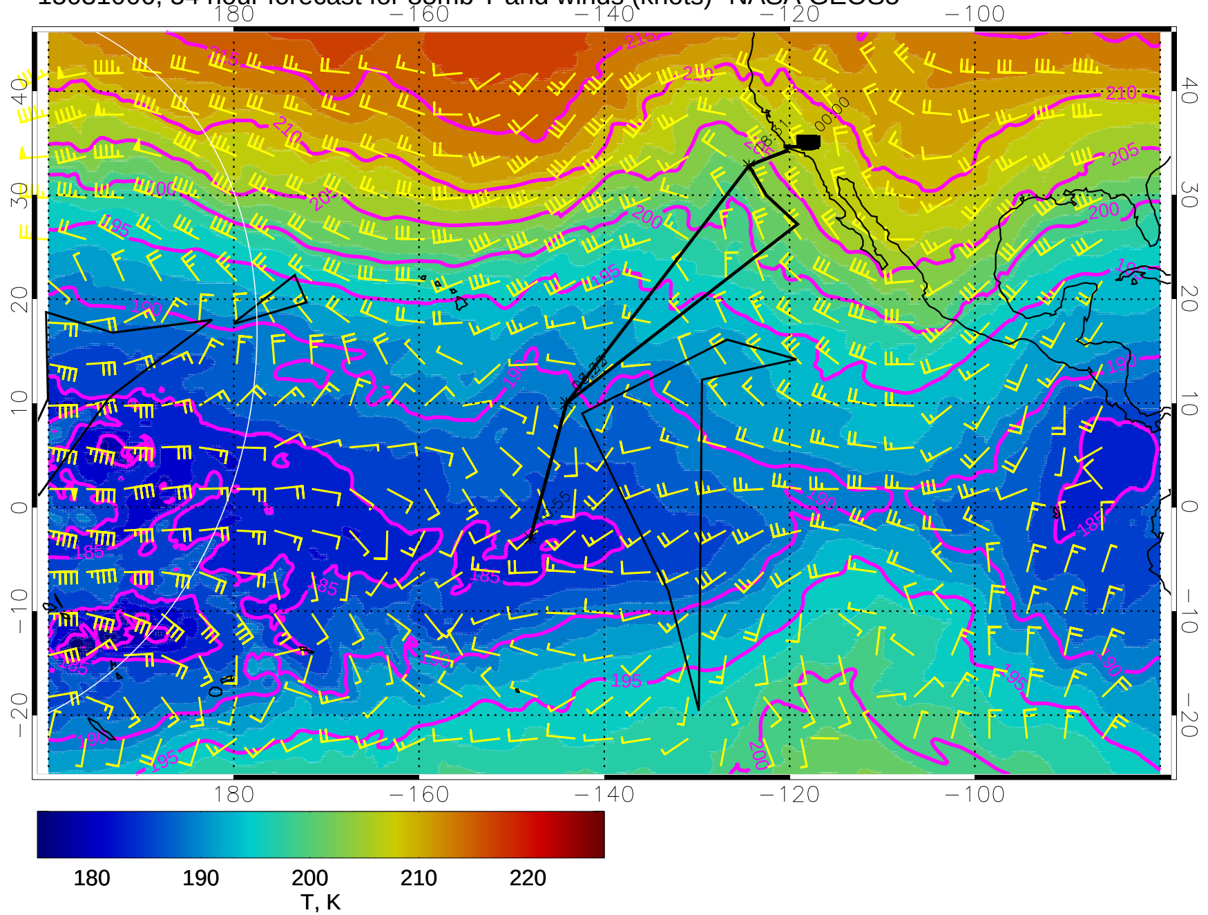
15031006, 54 hour forecast for 85mb T and winds (knots)- NASA GEOS5
