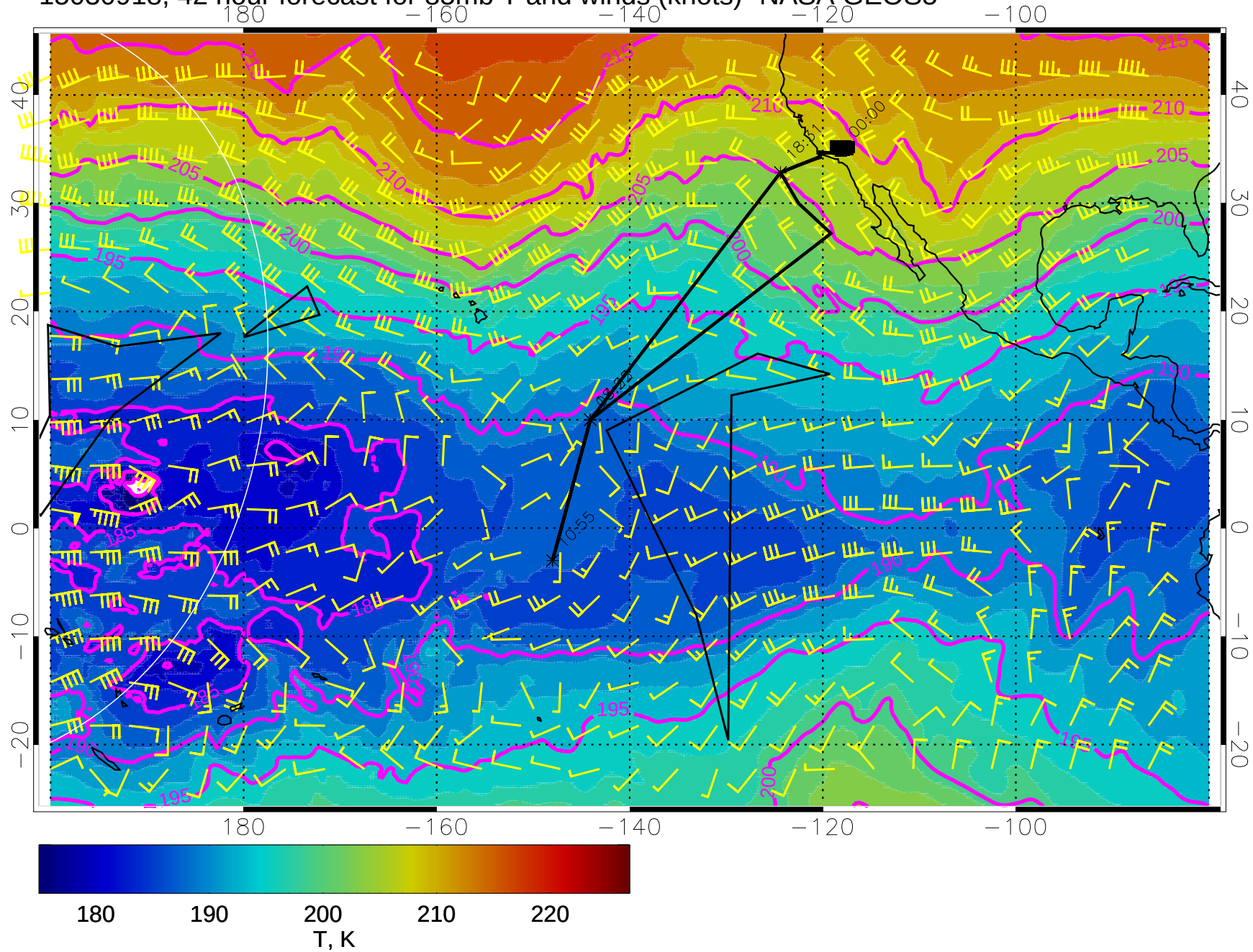
15030918, 42 hour forecast for 85mb T and winds (knots)- NASA GEOS5
