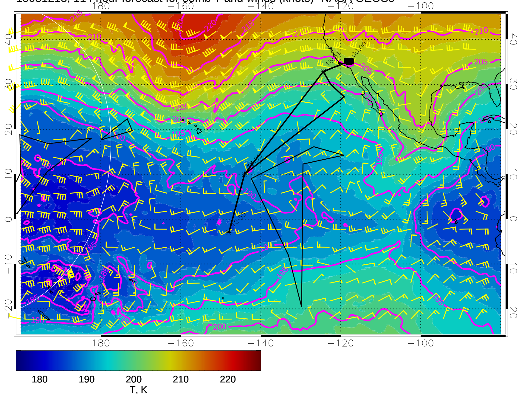
15031218, 114 hour forecast for 85mb T and winds (knots)- NASA GEOS5
