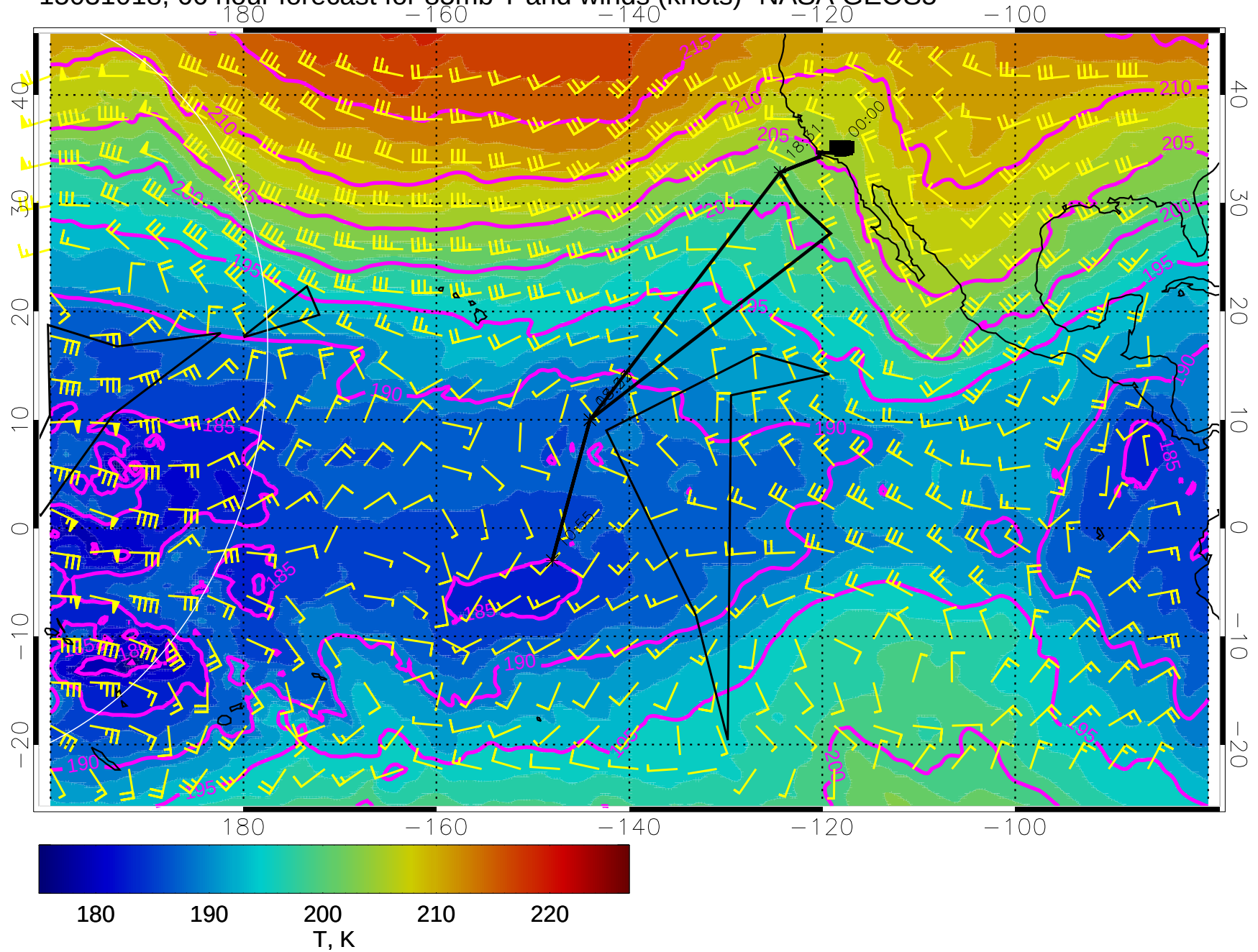
15031018, 66 hour forecast for 85mb T and winds (knots)- NASA GEOS5
