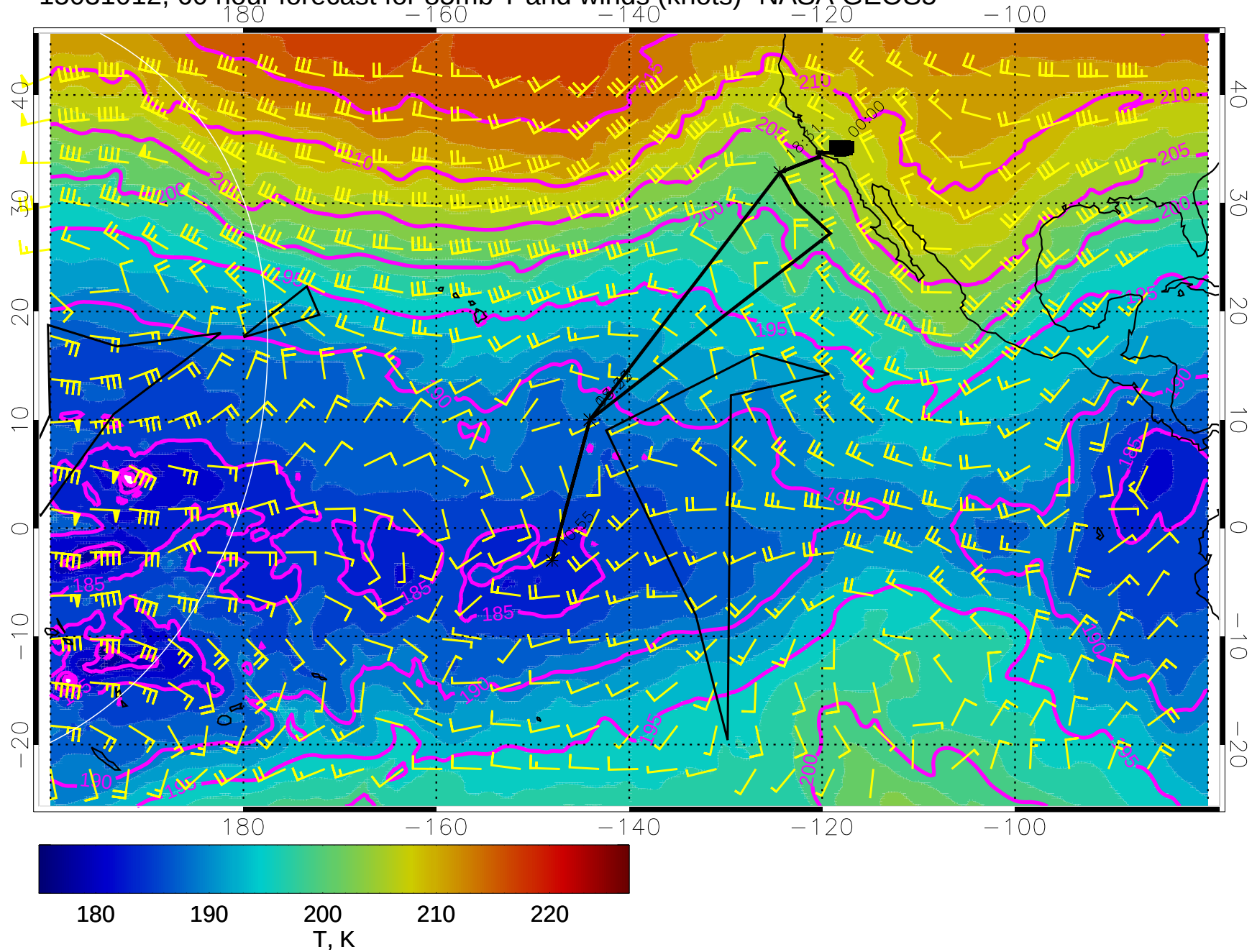
15031012, 60 hour forecast for 85mb T and winds (knots)- NASA GEOS5
