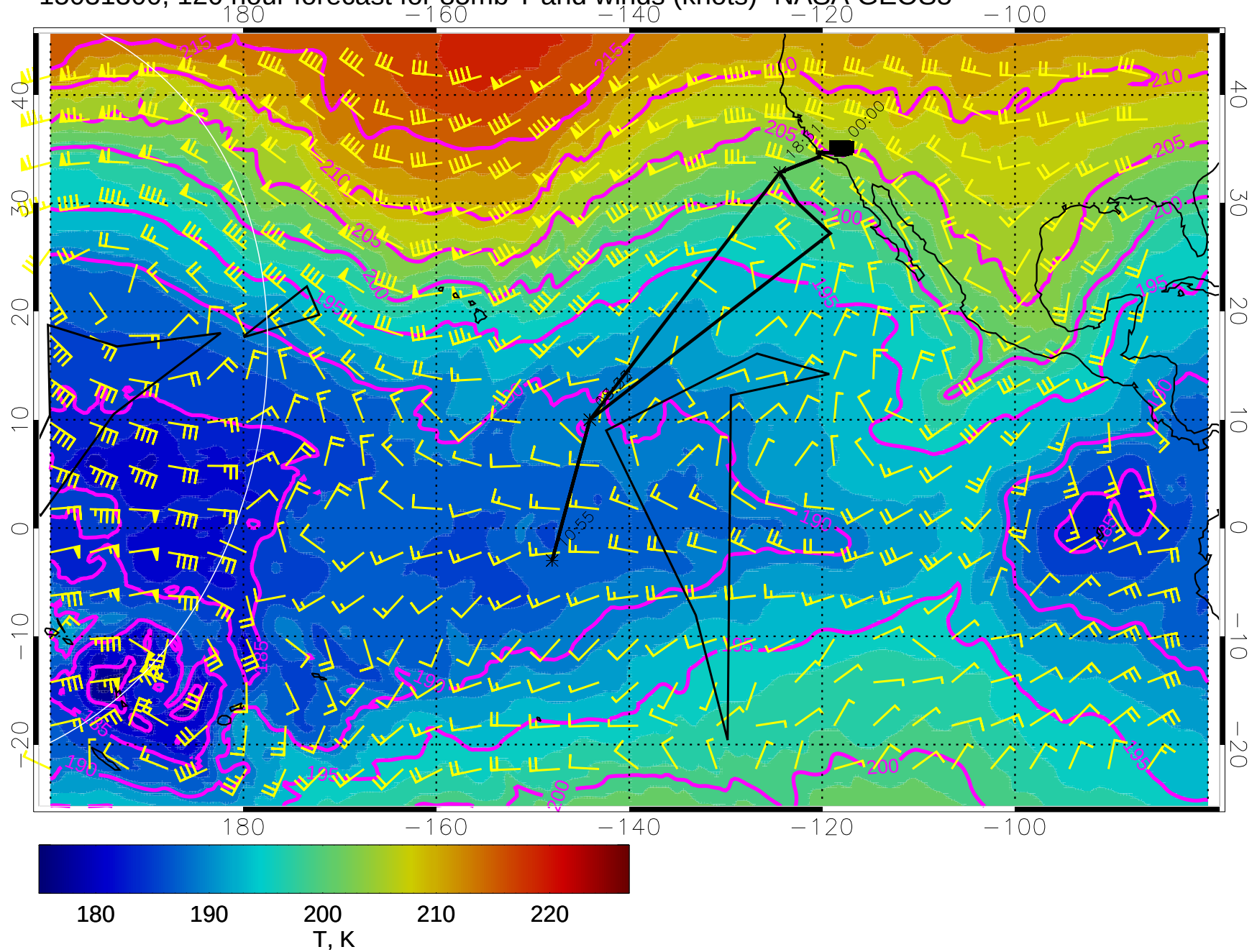
15031300, 120 hour forecast for 85mb T and winds (knots)- NASA GEOS5
