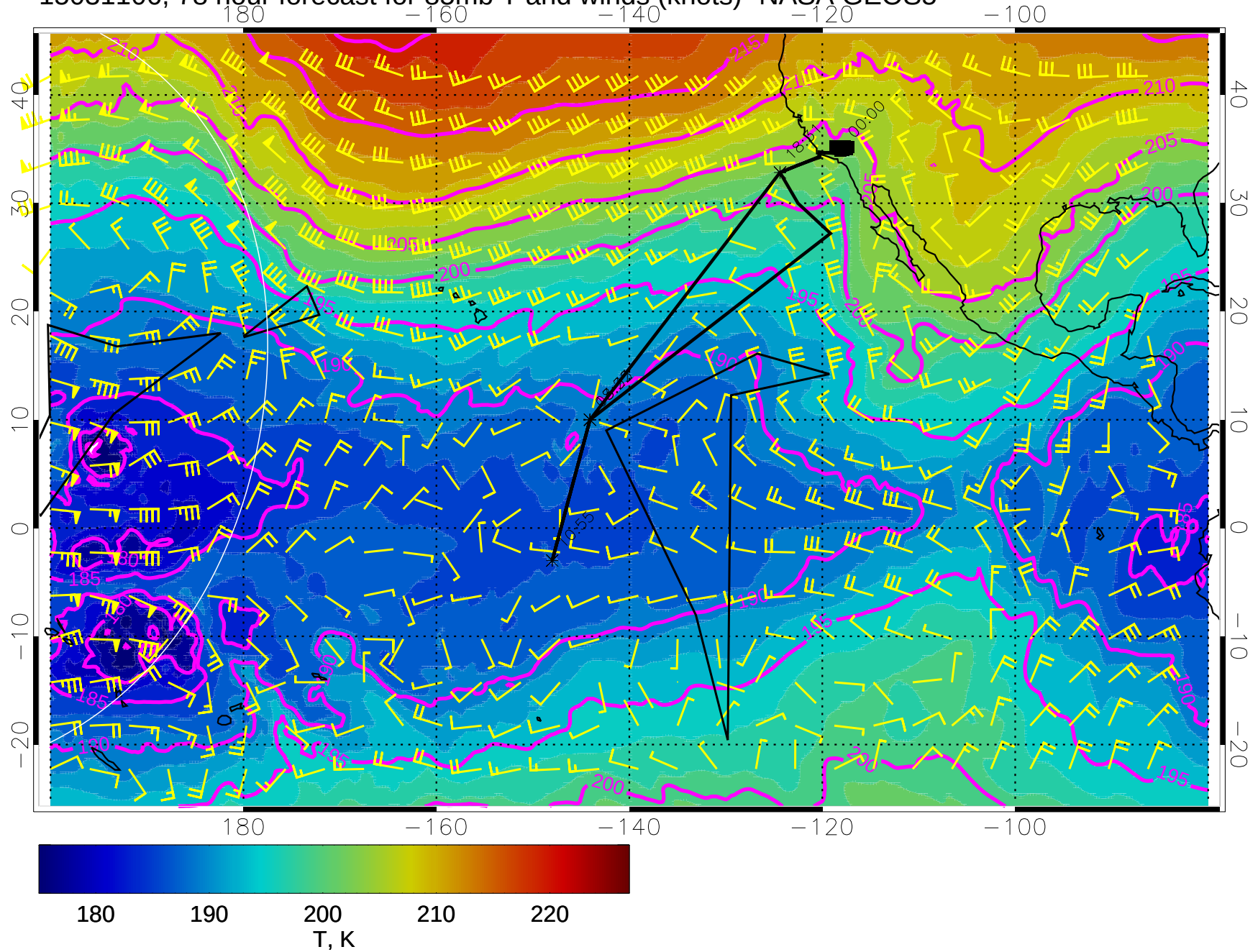
15031106, 78 hour forecast for 85mb T and winds (knots)- NASA GEOS5
