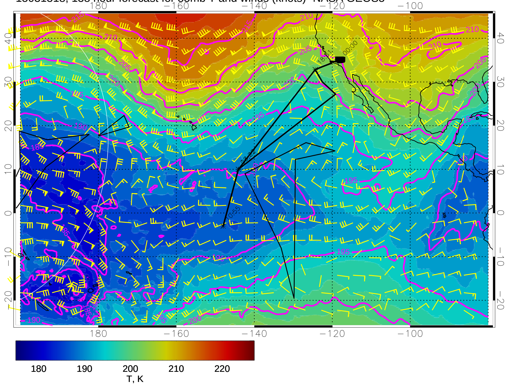
15031318, 138 hour forecast for 85mb T and winds (knots)- NASA GEOS5
