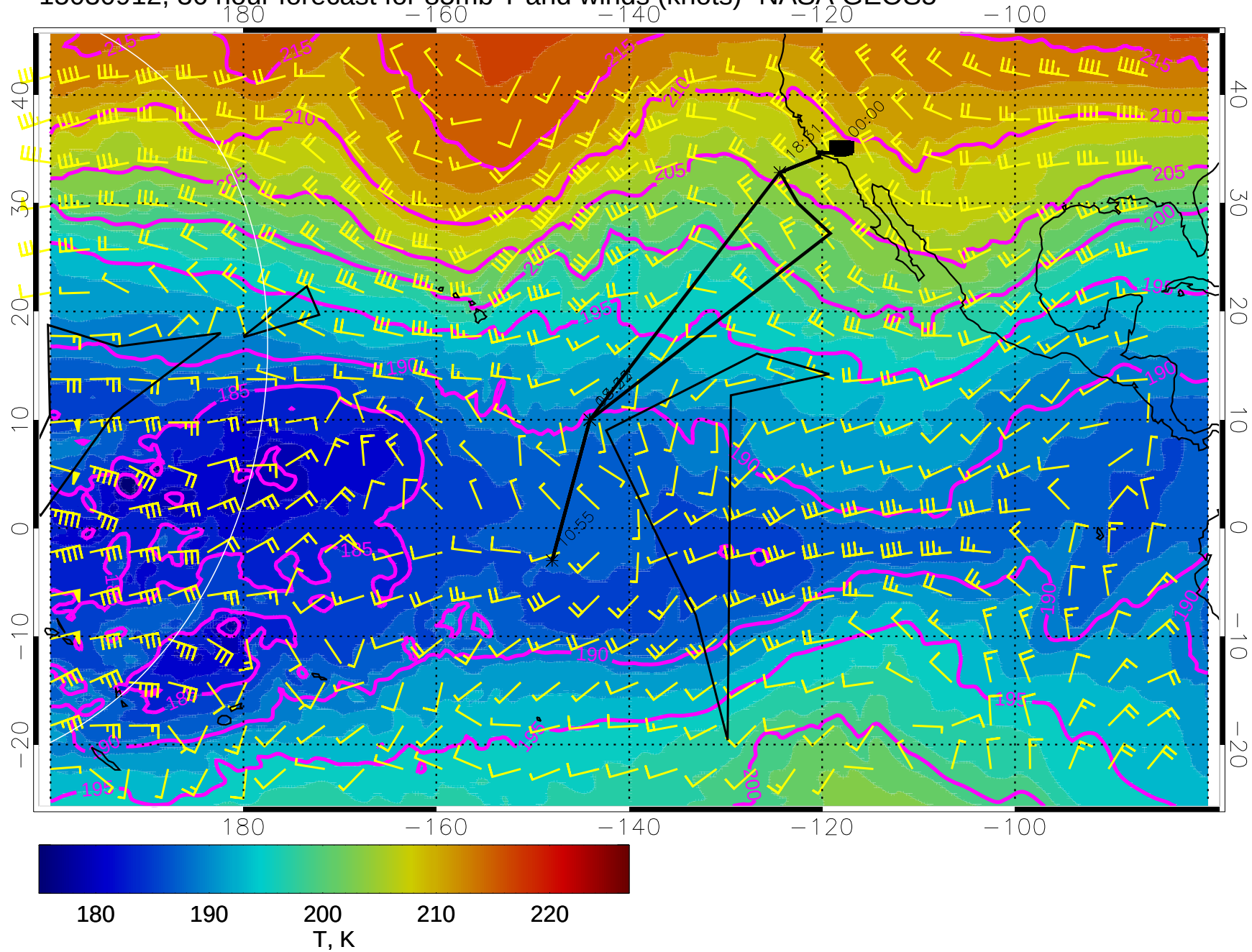
15030912, 36 hour forecast for 85mb T and winds (knots)- NASA GEOS5
