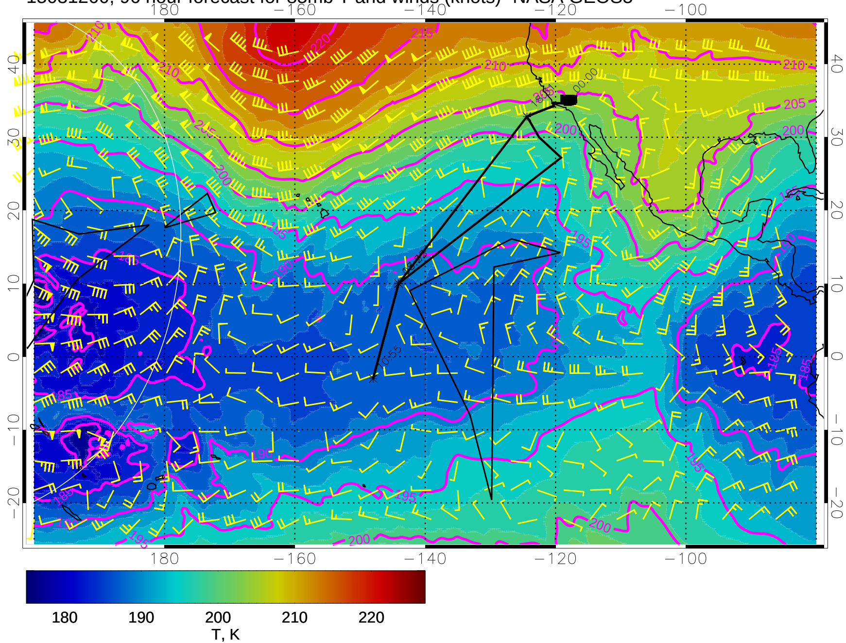
15031200, 96 hour forecast for 85mb T and winds (knots)- NASA GEOS5
