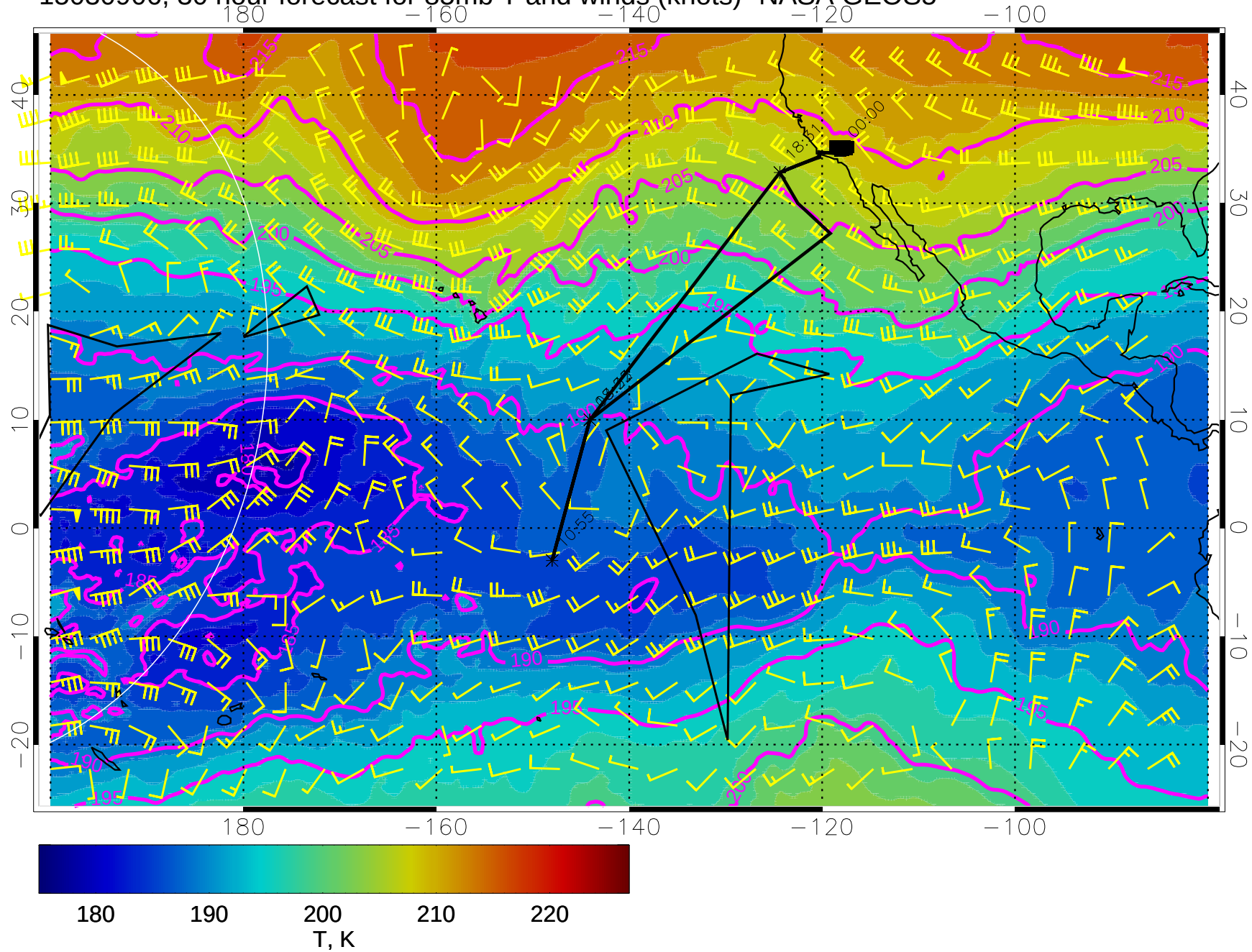
15030906, 30 hour forecast for 85mb T and winds (knots)- NASA GEOS5
