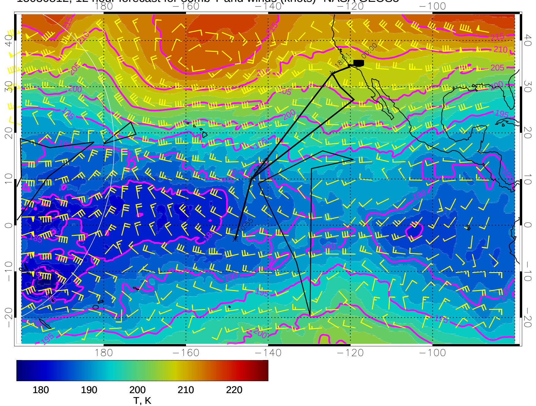
15030812, 12 hour forecast for 85mb T and winds (knots)- NASA GEOS5
