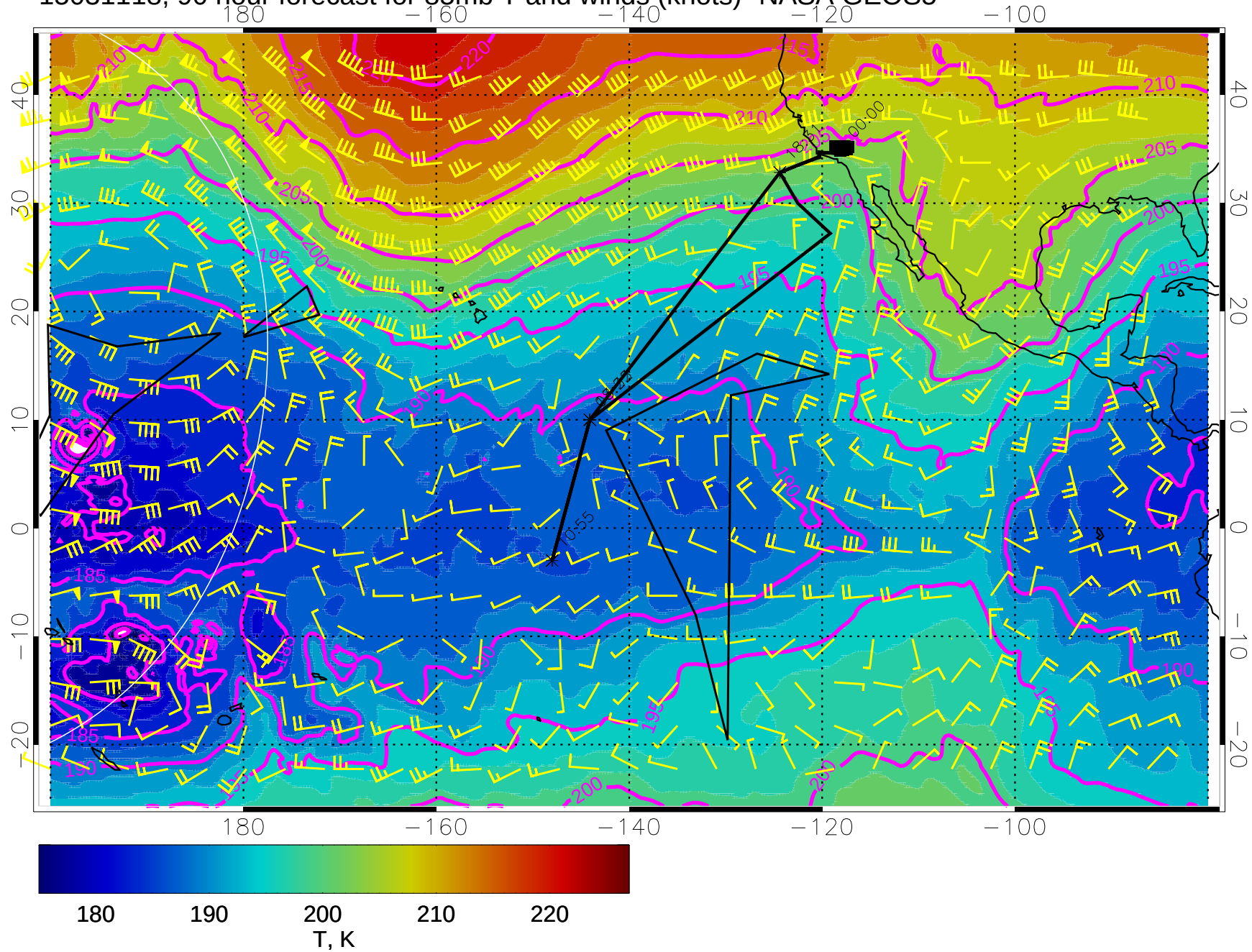
15031118, 90 hour forecast for 85mb T and winds (knots)- NASA GEOS5
