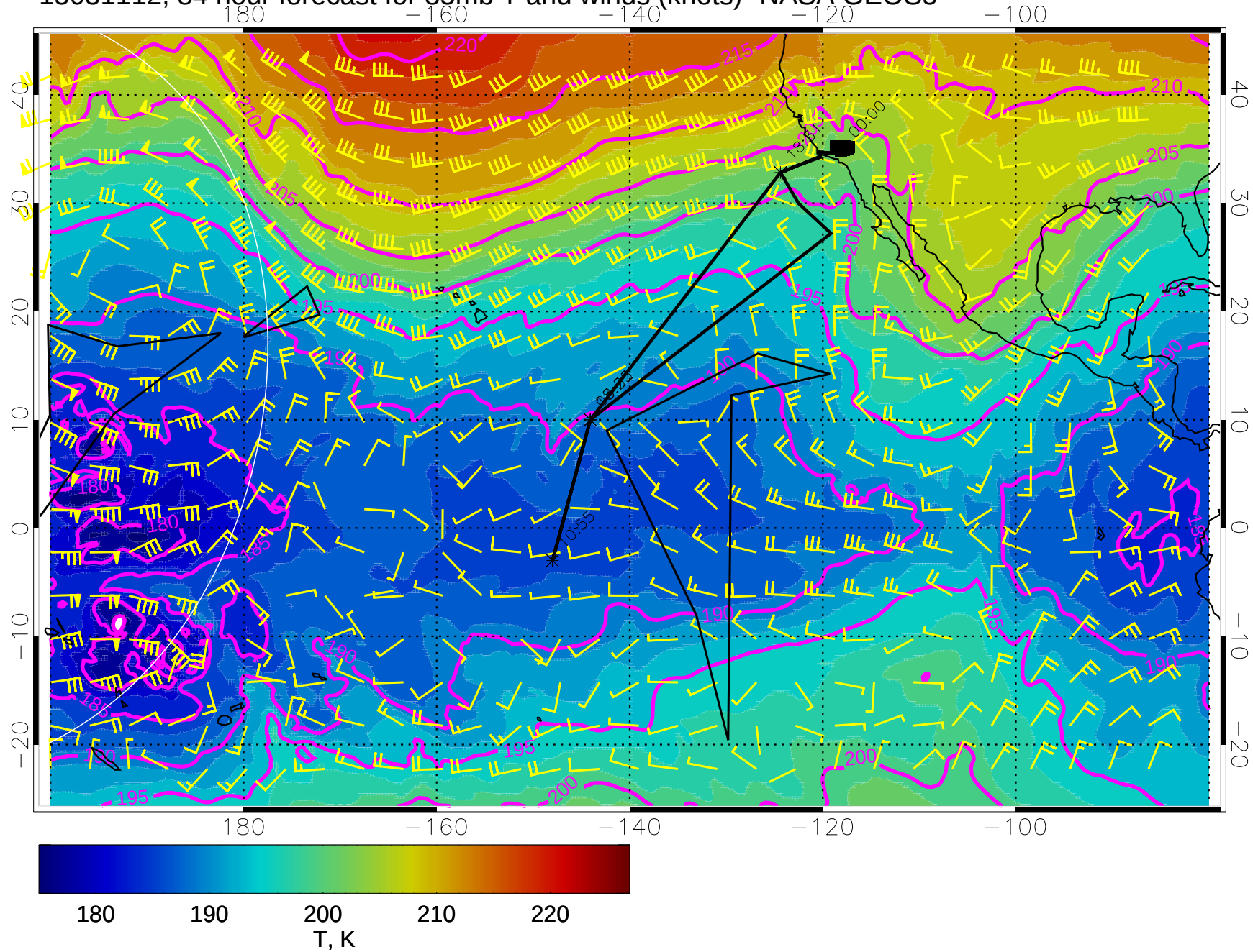
15031112, 84 hour forecast for 85mb T and winds (knots)- NASA GEOS5
