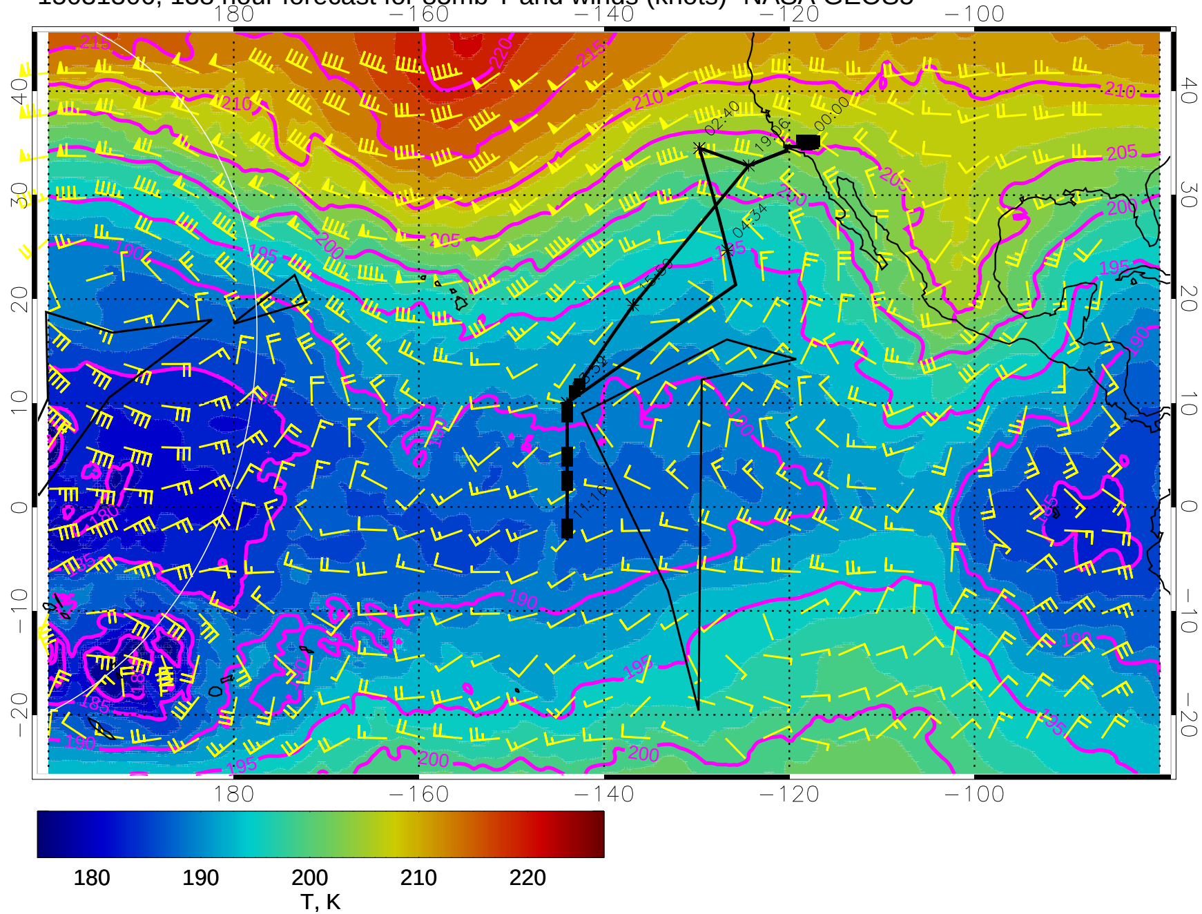
15031306, 138 hour forecast for 85mb T and winds (knots)- NASA GEOS5
