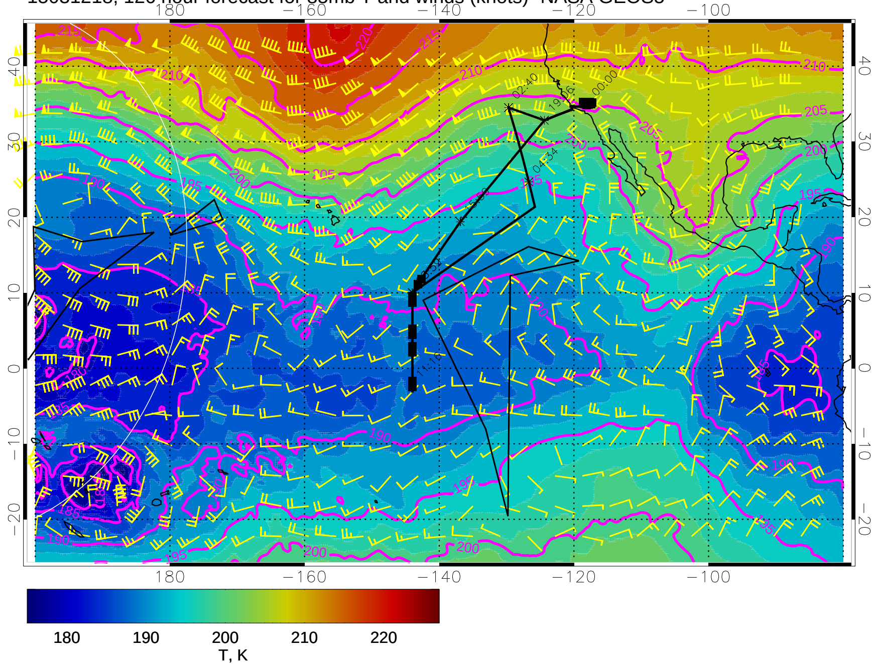
15031218, 126 hour forecast for 85mb T and winds (knots)- NASA GEOS5
