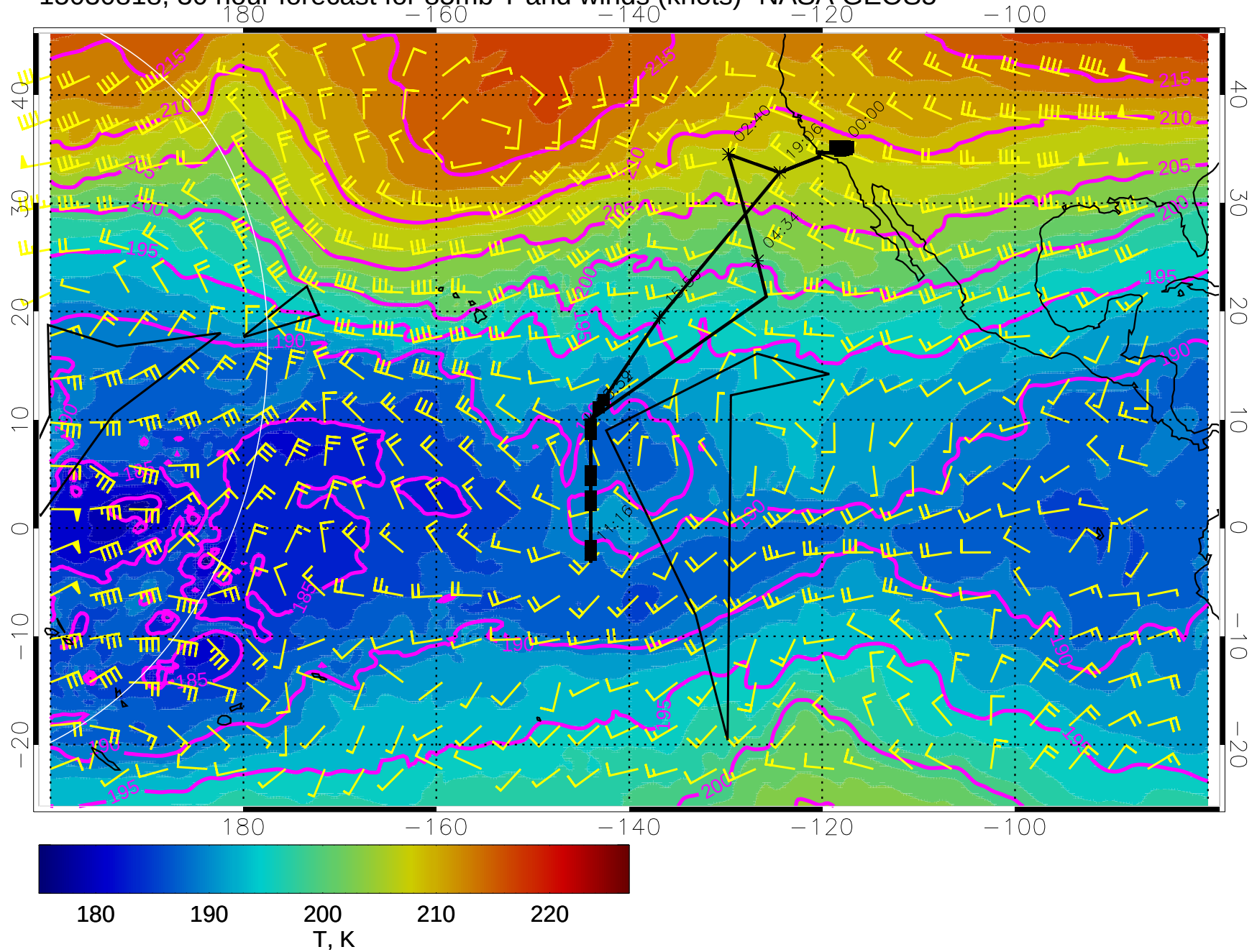
15030818, 30 hour forecast for 85mb T and winds (knots)- NASA GEOS5
