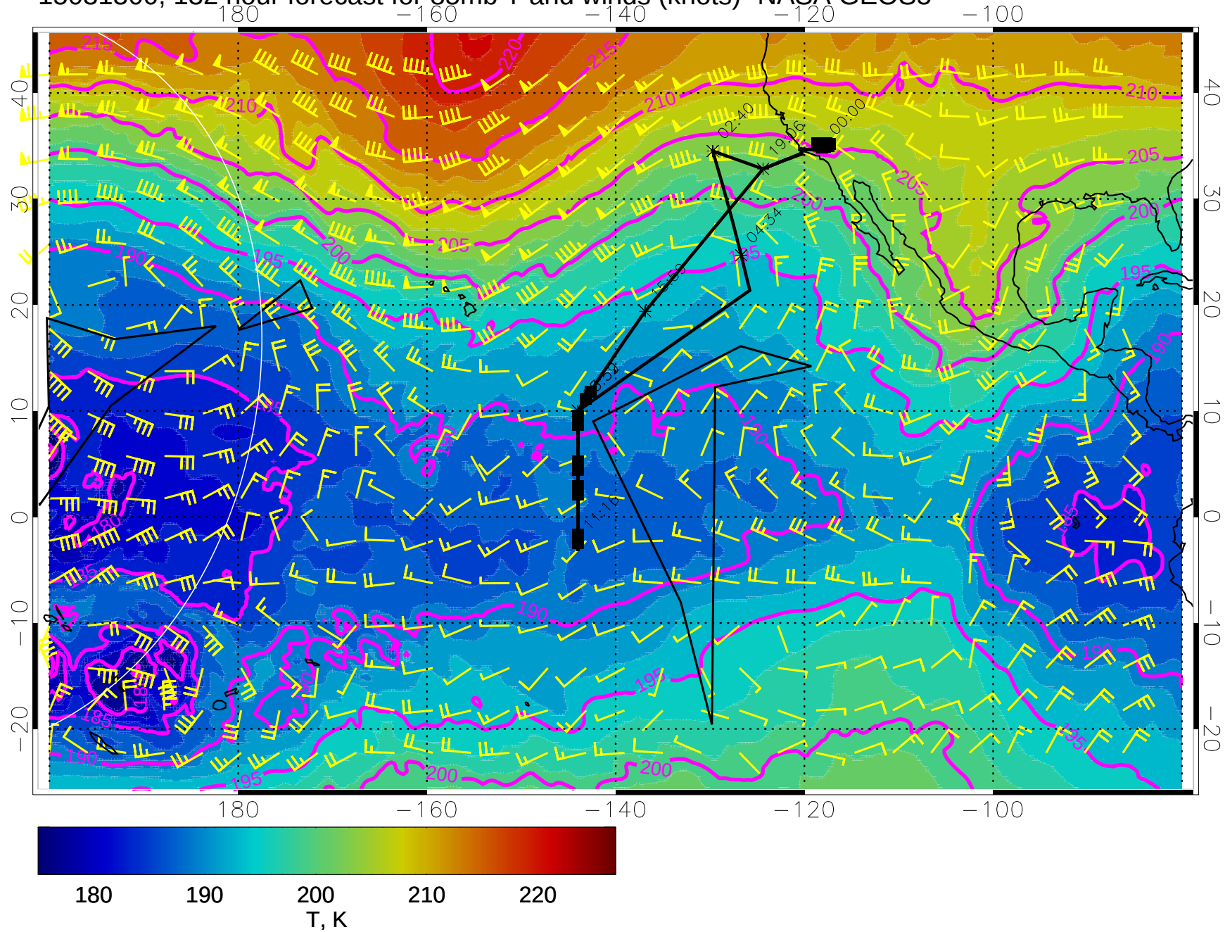
15031300, 132 hour forecast for 85mb T and winds (knots)- NASA GEOS5
