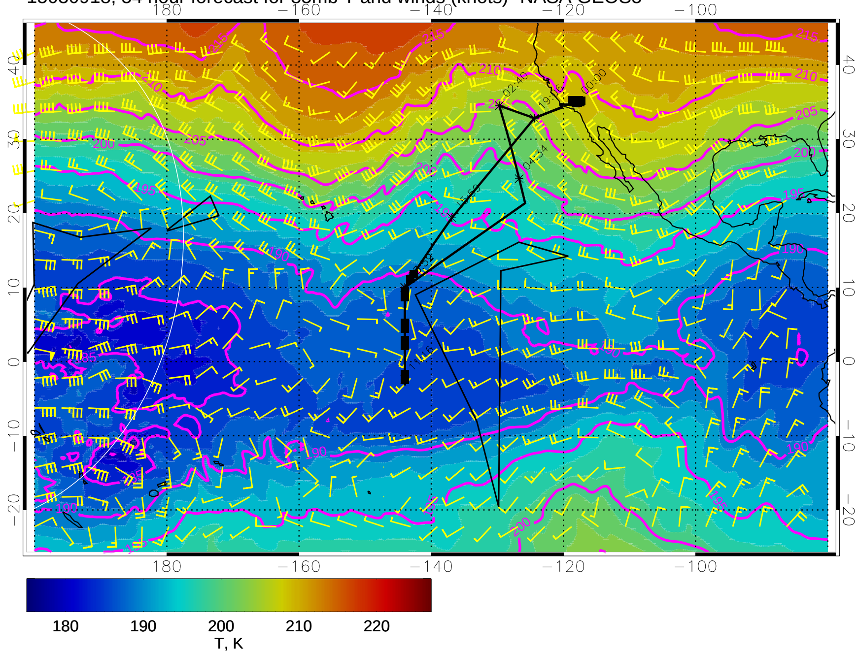
15030918, 54 hour forecast for 85mb T and winds (knots)- NASA GEOS5
