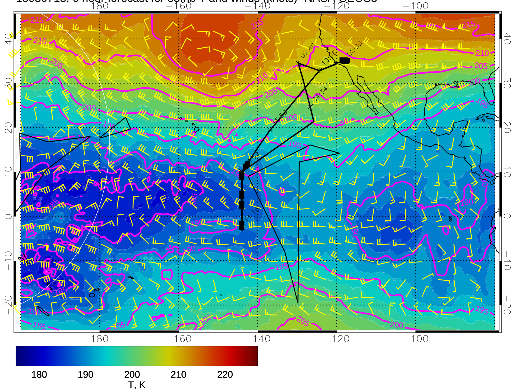
15030718, 6 hour forecast for 85mb T and winds (knots)- NASA GEOS5
