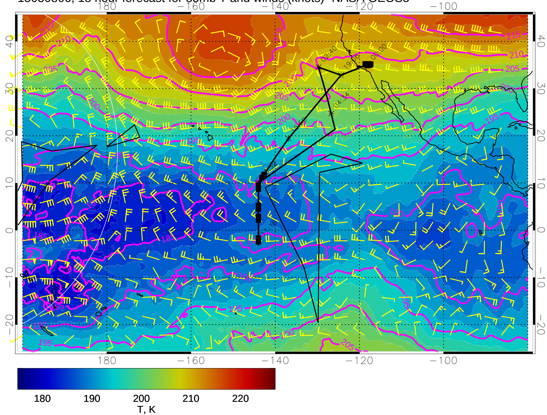
15030806, 18 hour forecast for 85mb T and winds (knots)- NASA GEOS5
