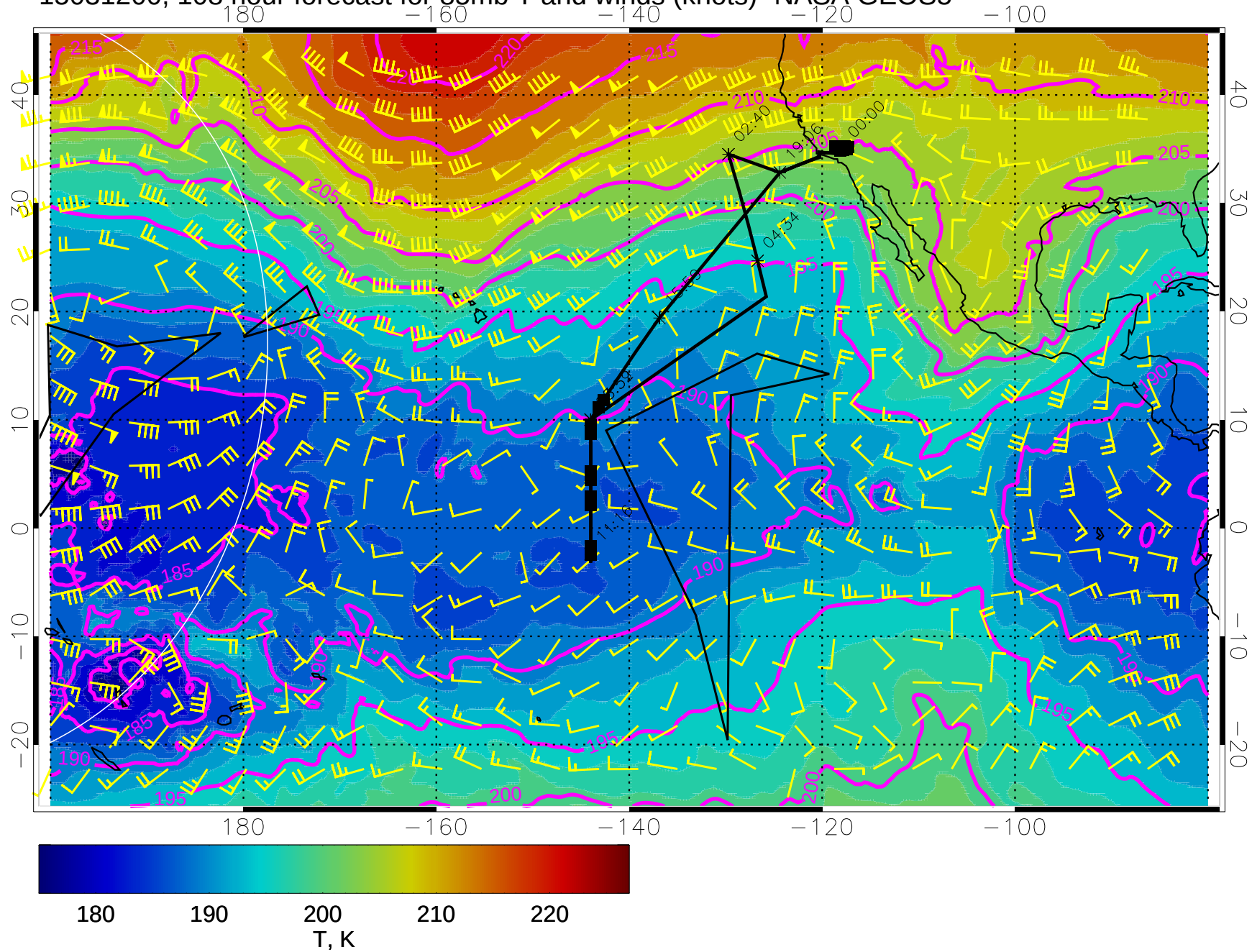
15031200, 108 hour forecast for 85mb T and winds (knots)- NASA GEOS5
