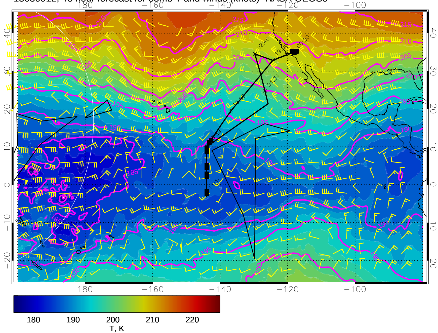
15030912, 48 hour forecast for 85mb T and winds (knots)- NASA GEOS5
