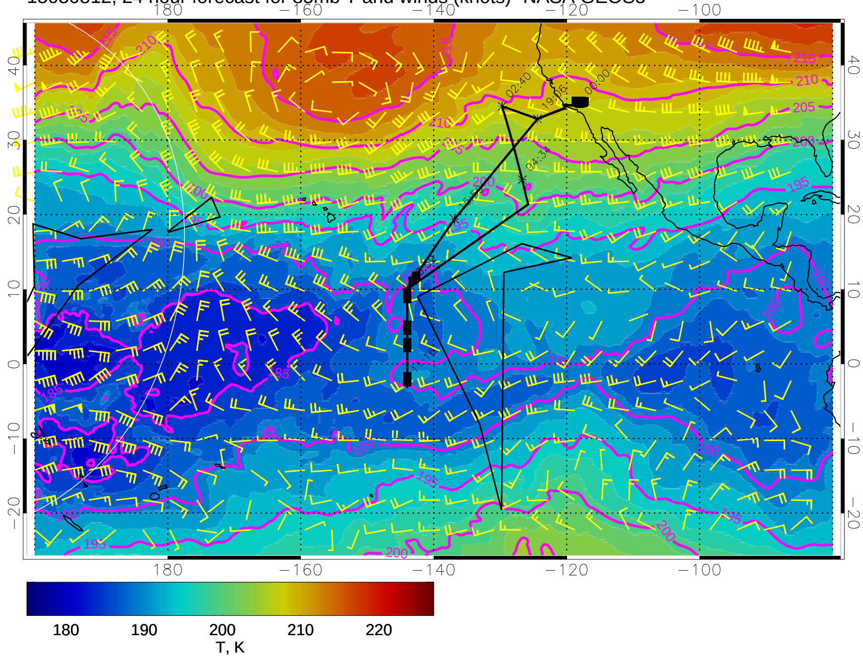
15030812, 24 hour forecast for 85mb T and winds (knots)- NASA GEOS5
