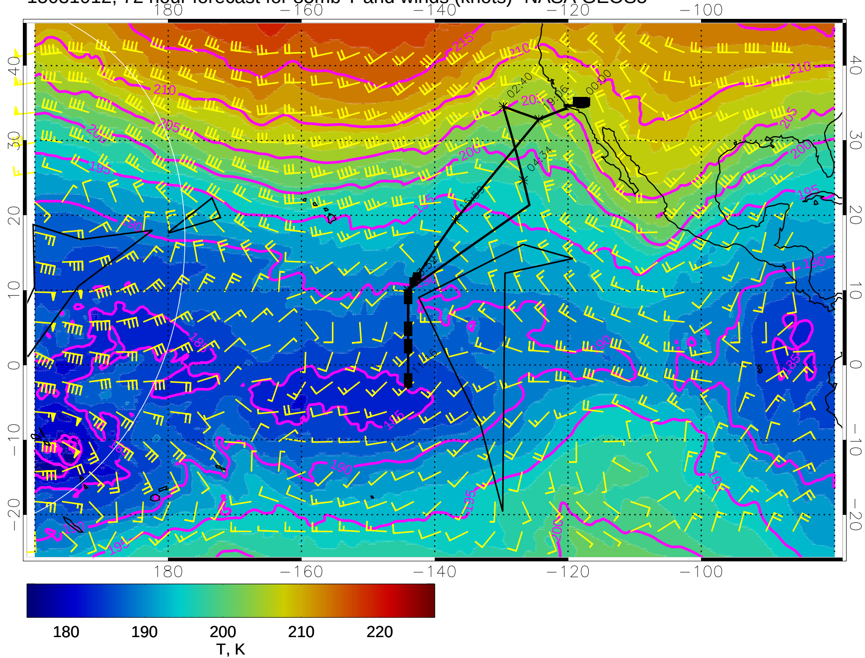
15031012, 72 hour forecast for 85mb T and winds (knots)- NASA GEOS5
