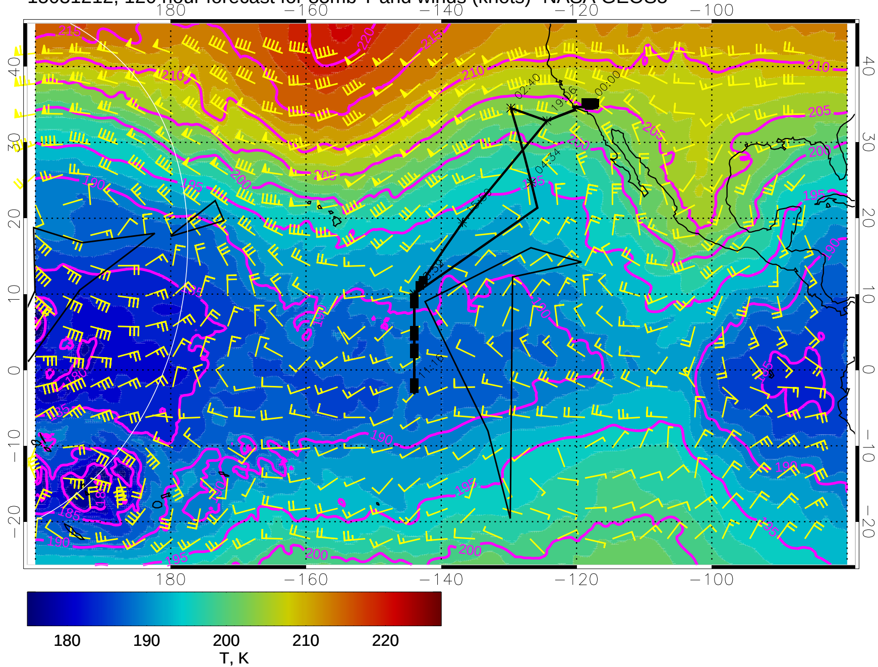
15031212, 120 hour forecast for 85mb T and winds (knots)- NASA GEOS5
