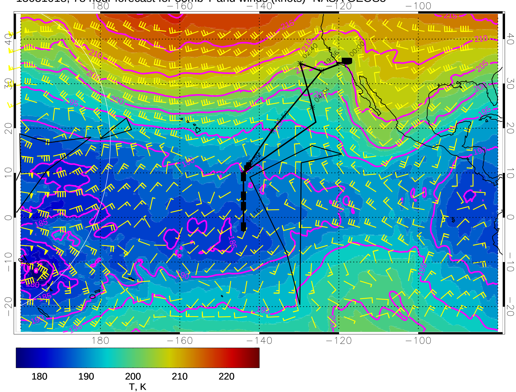
15031018, 78 hour forecast for 85mb T and winds (knots)- NASA GEOS5
