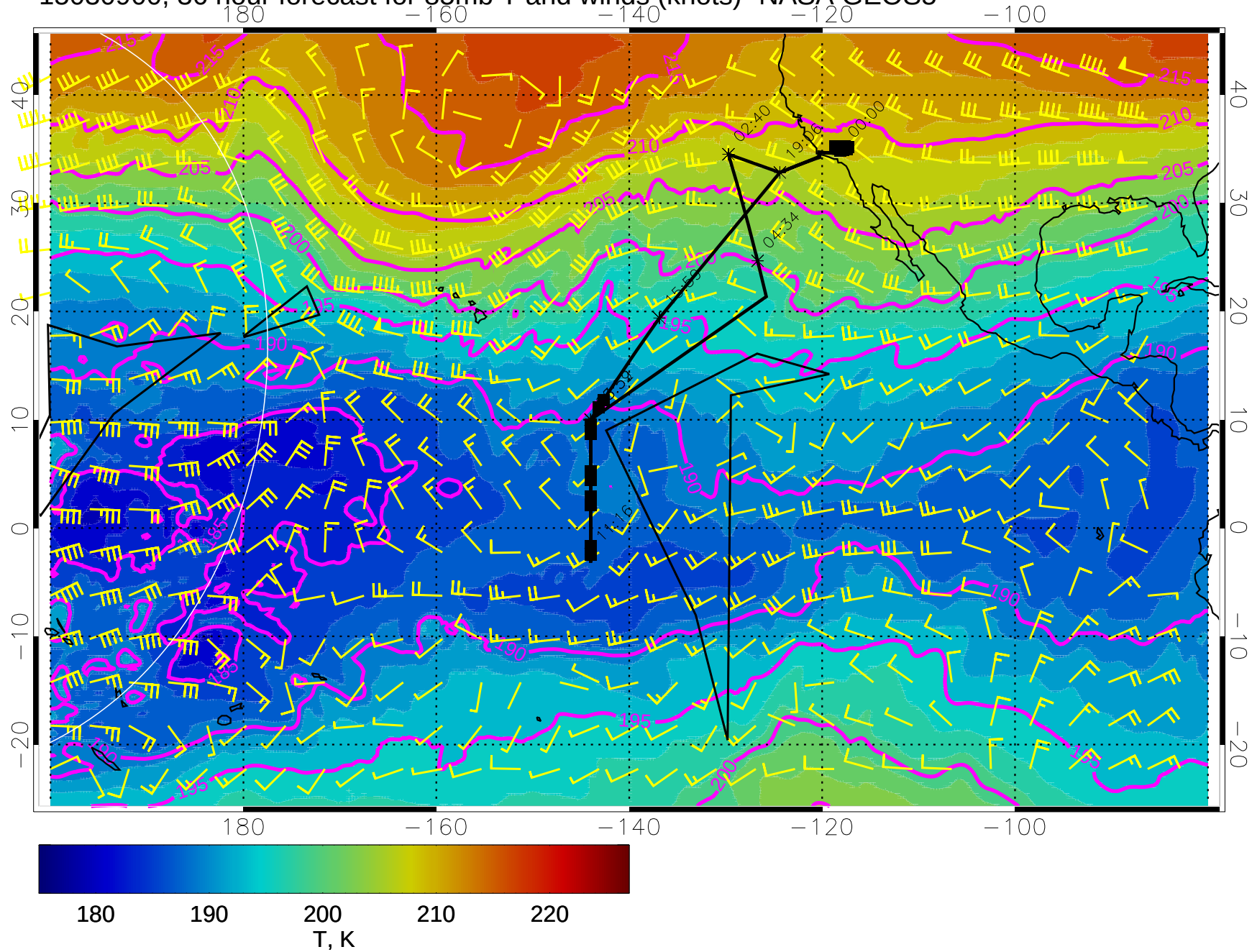
15030900, 36 hour forecast for 85mb T and winds (knots)- NASA GEOS5
