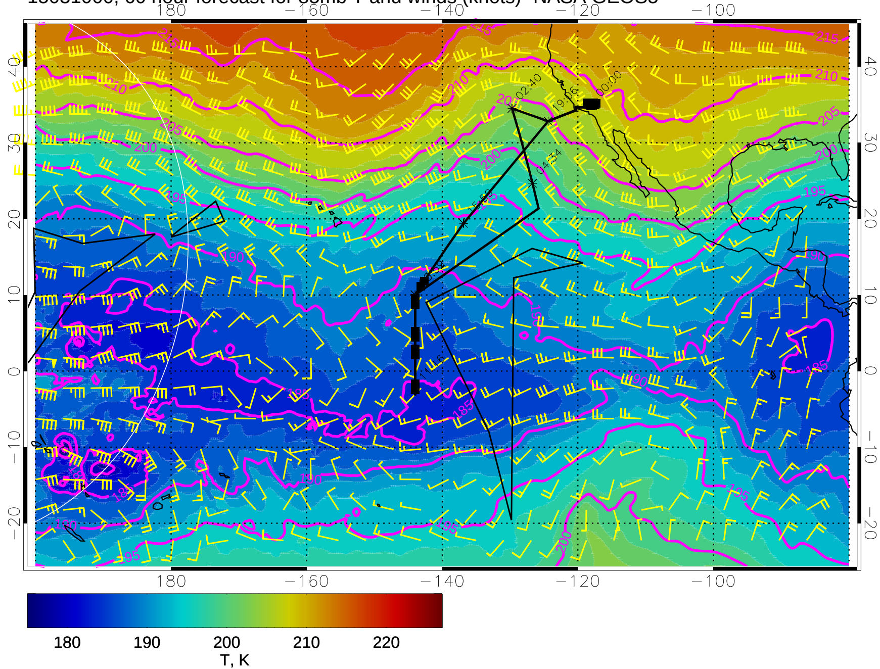
15031000, 60 hour forecast for 85mb T and winds (knots)- NASA GEOS5
