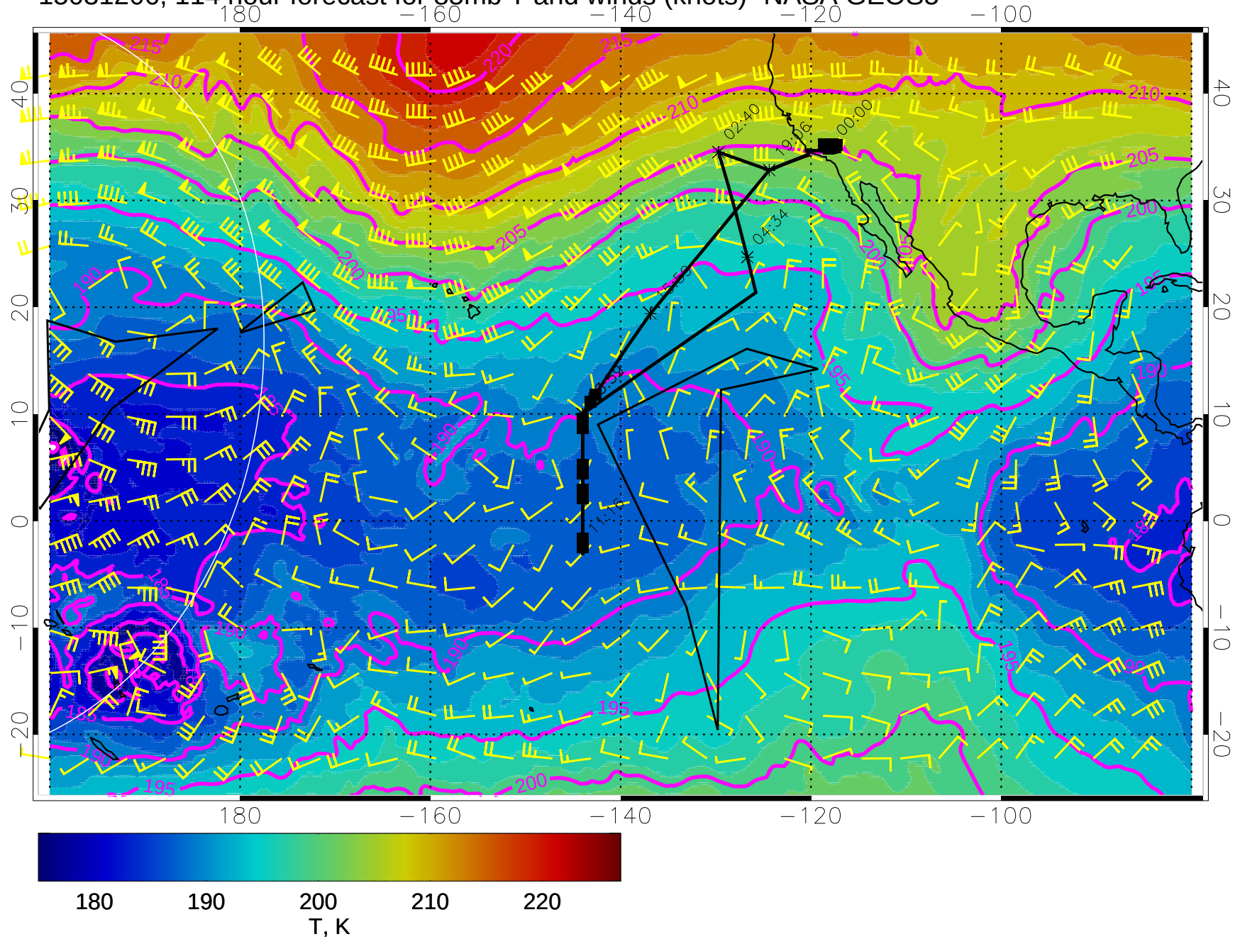
15031206, 114 hour forecast for 85mb T and winds (knots)- NASA GEOS5
