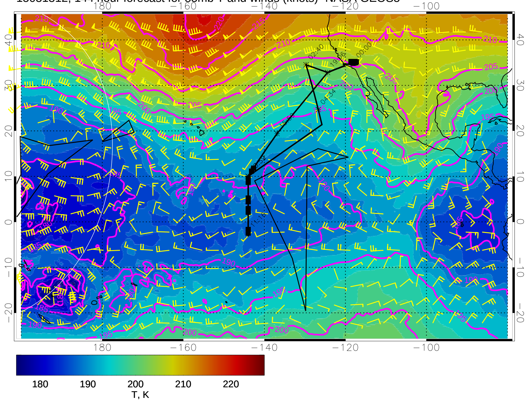
15031312, 144 hour forecast for 85mb T and winds (knots)- NASA GEOS5
