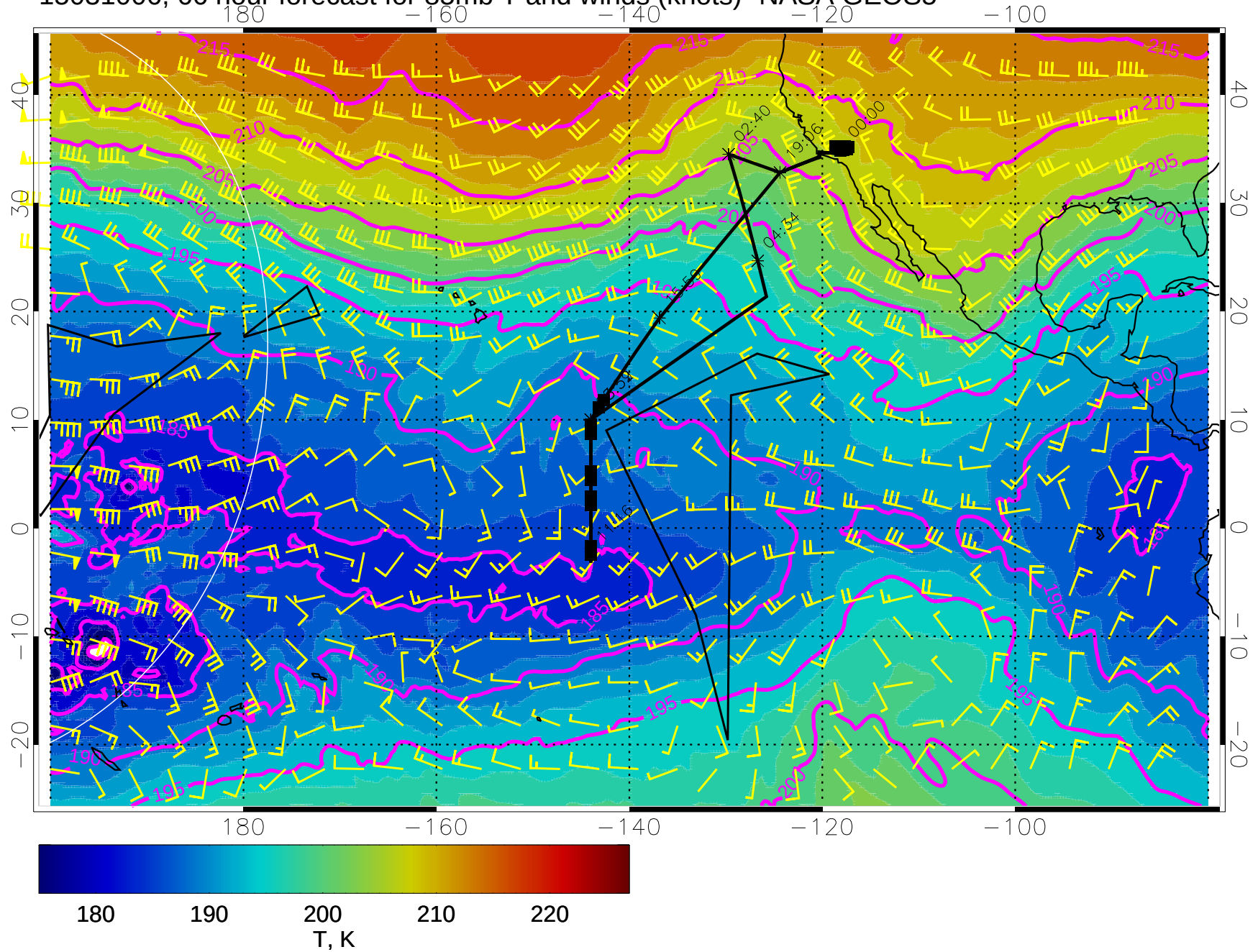
15031006, 66 hour forecast for 85mb T and winds (knots)- NASA GEOS5
