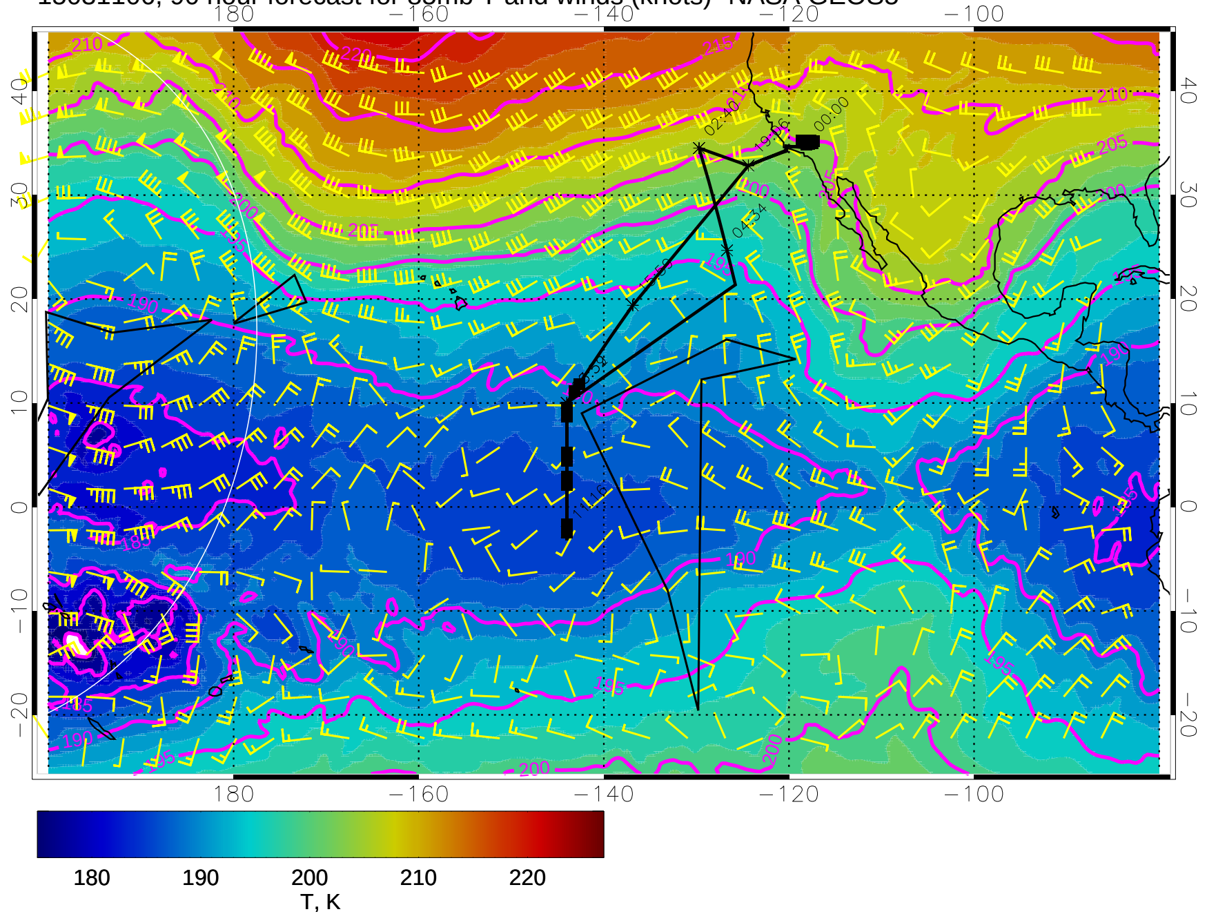
15031106, 90 hour forecast for 85mb T and winds (knots)- NASA GEOS5
