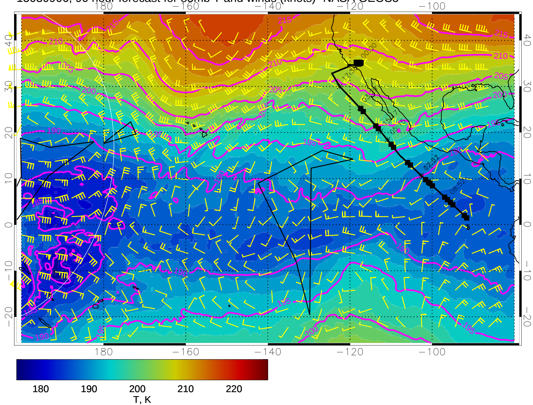
15030906, 90 hour forecast for 85mb T and winds (knots)- NASA GEOS5
