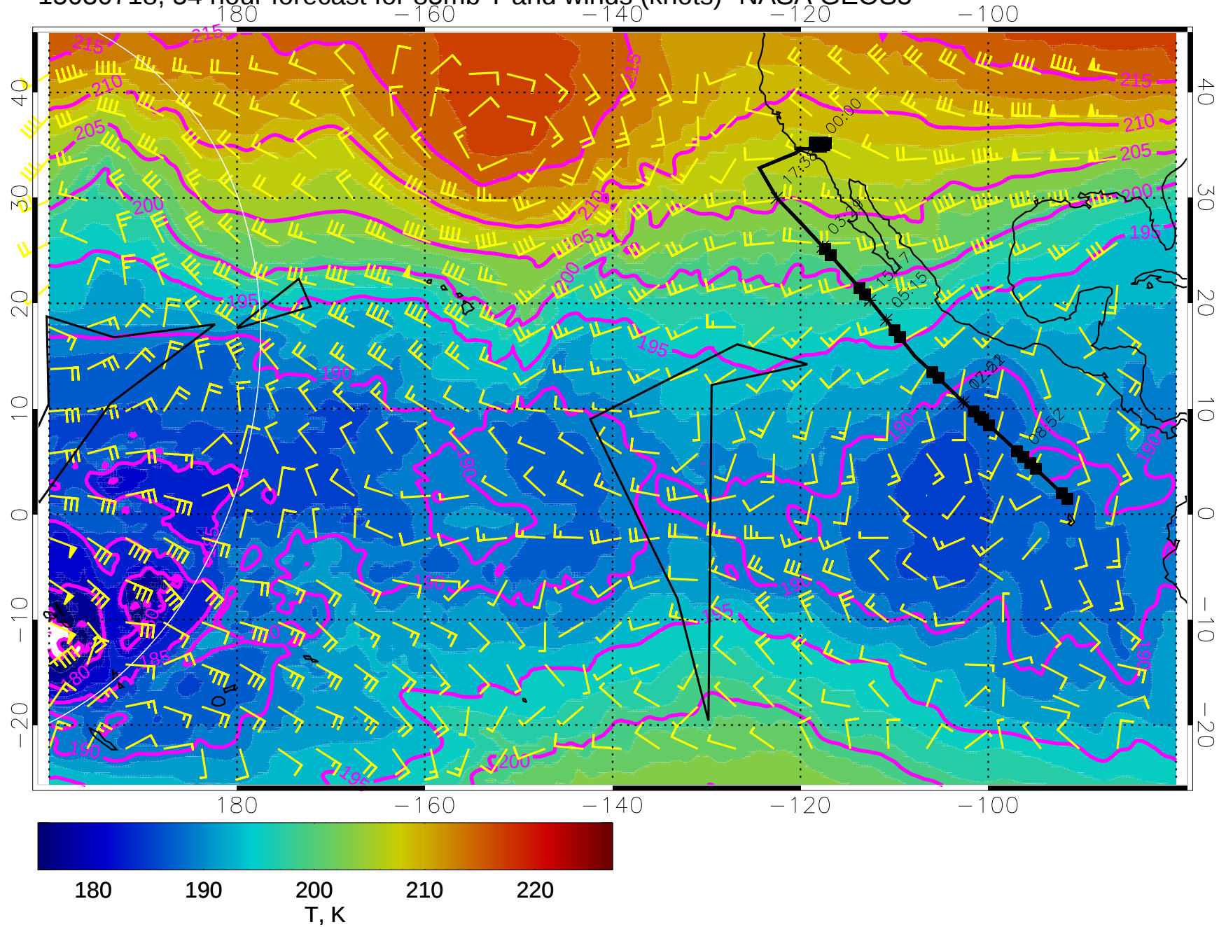
15030718, 54 hour forecast for 85mb T and winds (knots)- NASA GEOS5
