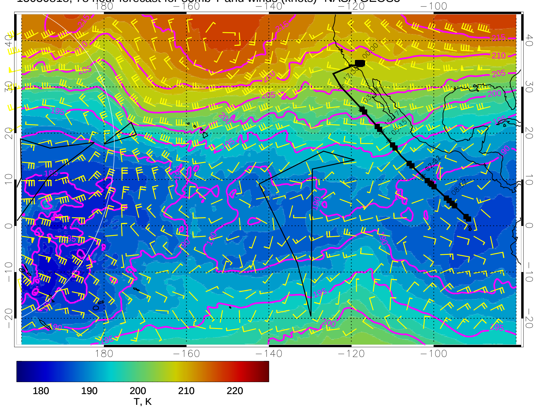
15030818, 78 hour forecast for 85mb T and winds (knots)- NASA GEOS5
