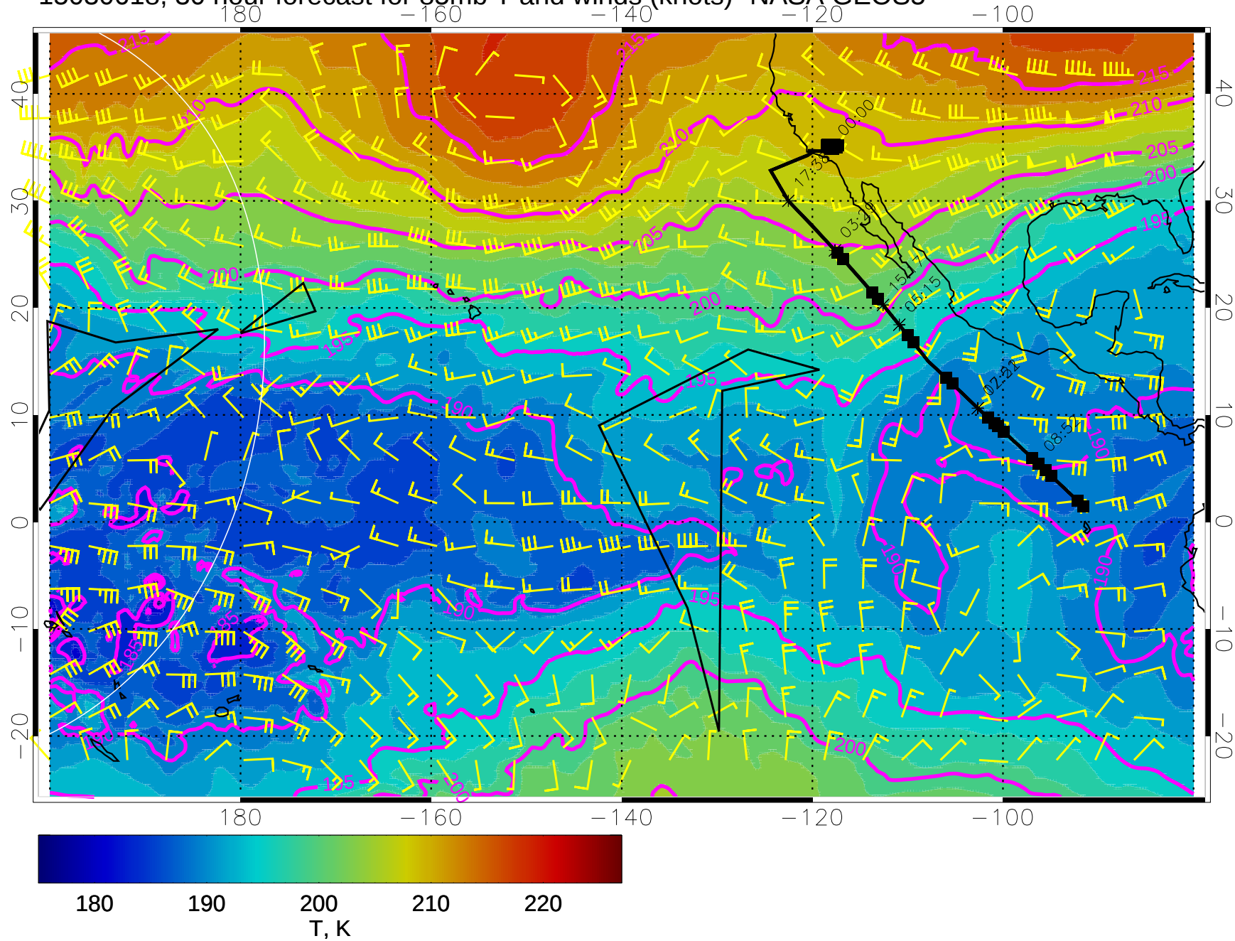
15030618, 30 hour forecast for 85mb T and winds (knots)- NASA GEOS5
