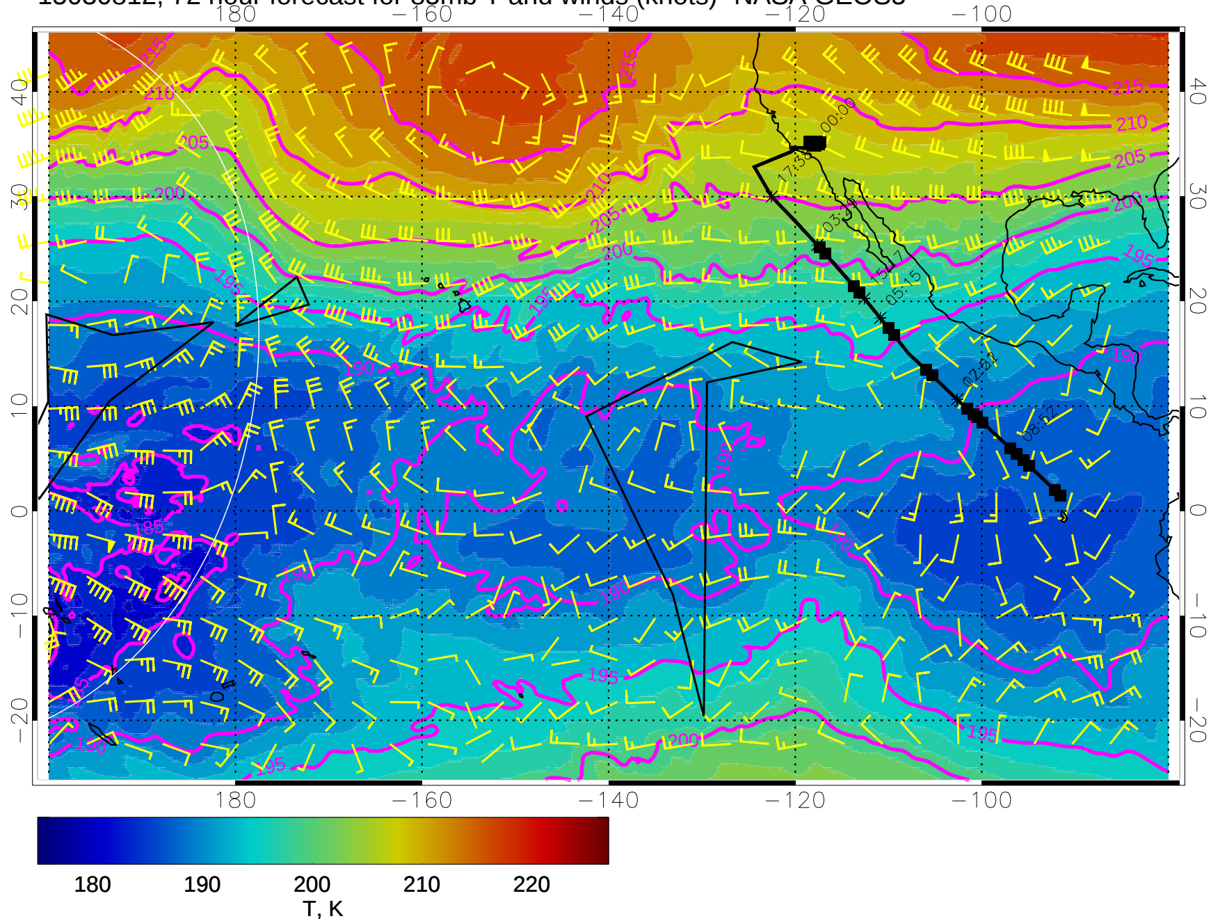
15030812, 72 hour forecast for 85mb T and winds (knots)- NASA GEOS5
