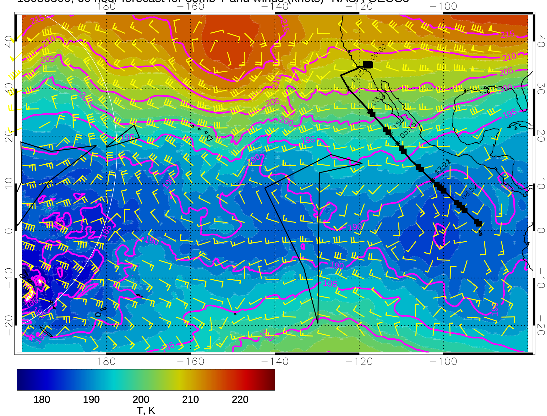
15030800, 60 hour forecast for 85mb T and winds (knots)- NASA GEOS5
