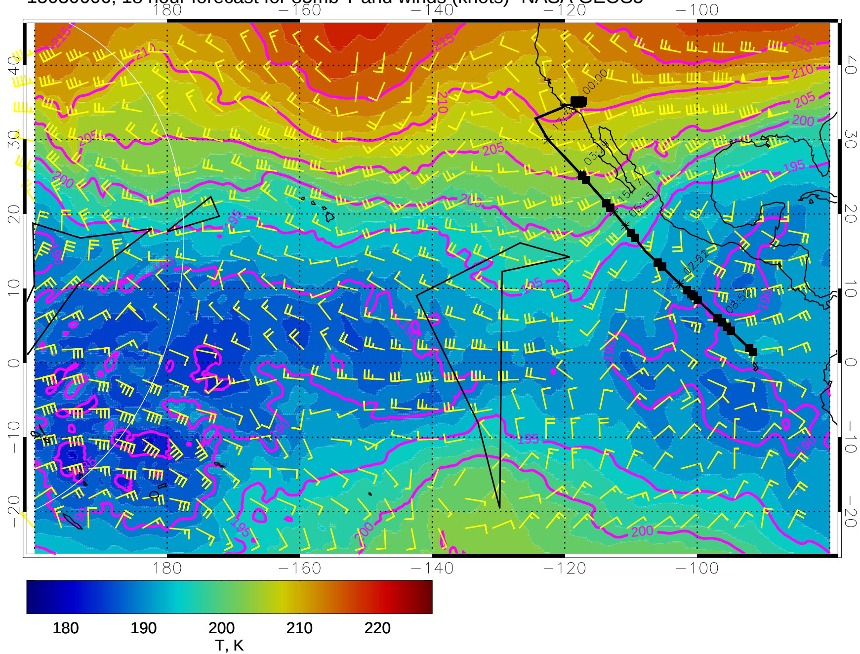
15030606, 18 hour forecast for 85mb T and winds (knots)- NASA GEOS5
