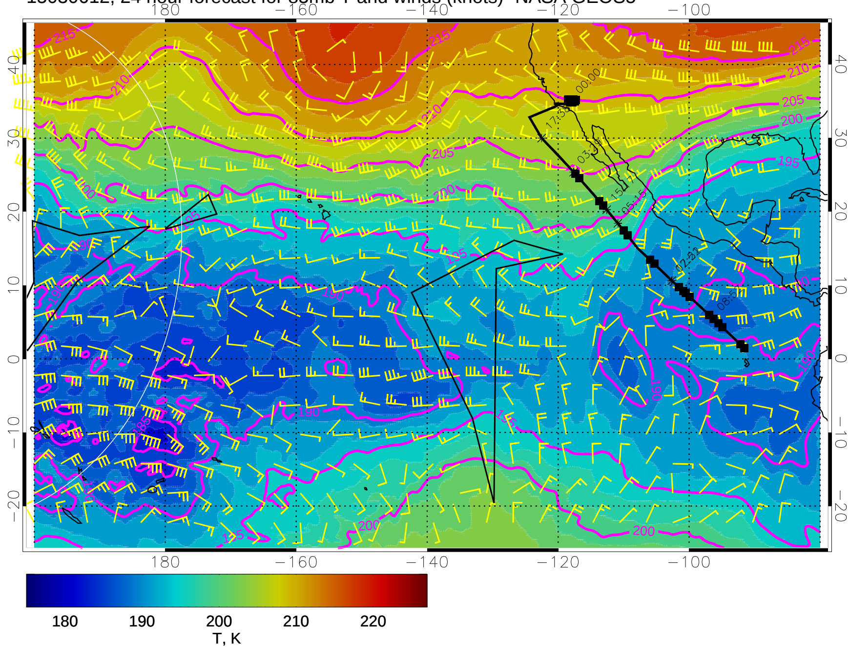
15030612, 24 hour forecast for 85mb T and winds (knots)- NASA GEOS5
