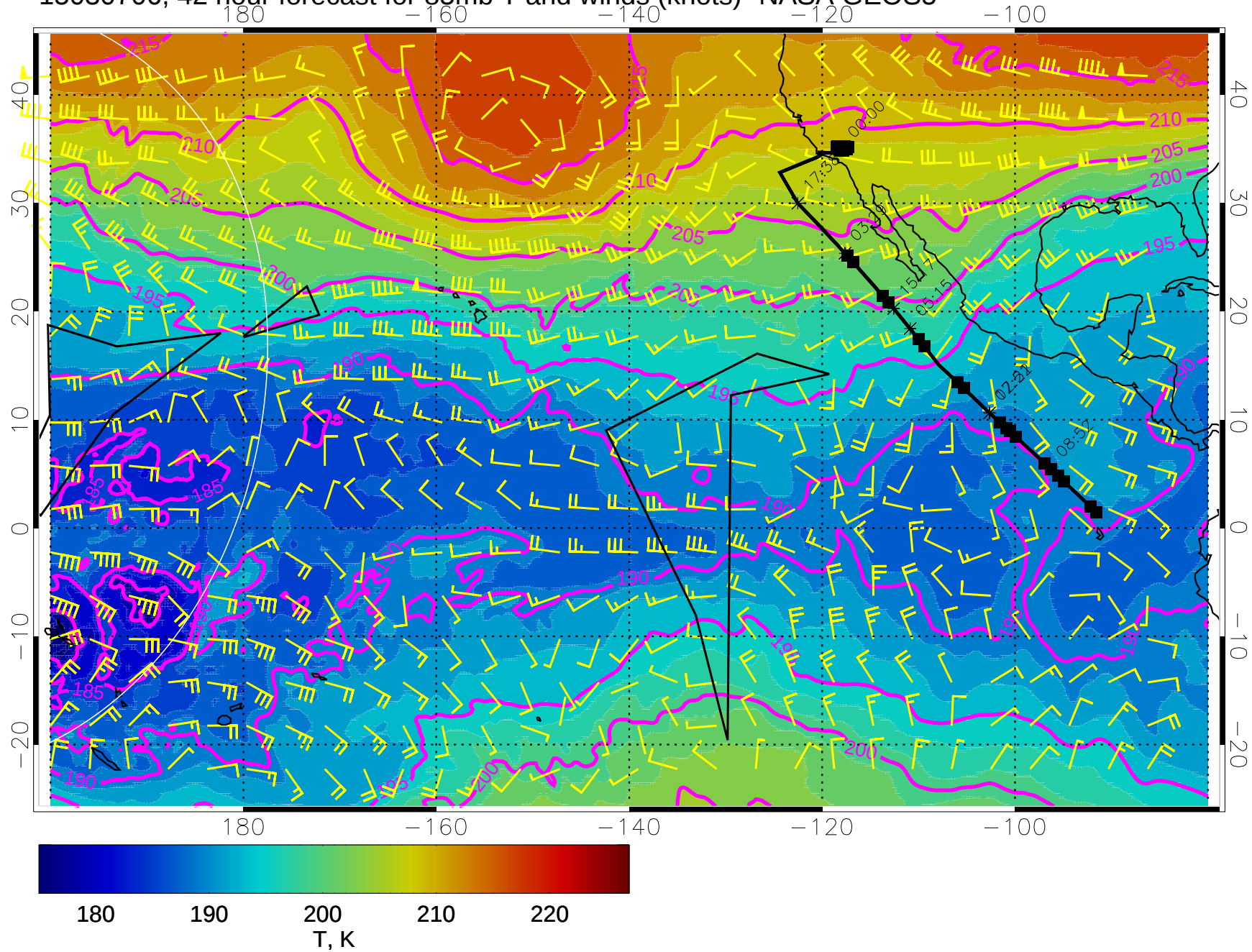
15030706, 42 hour forecast for 85mb T and winds (knots)- NASA GEOS5
