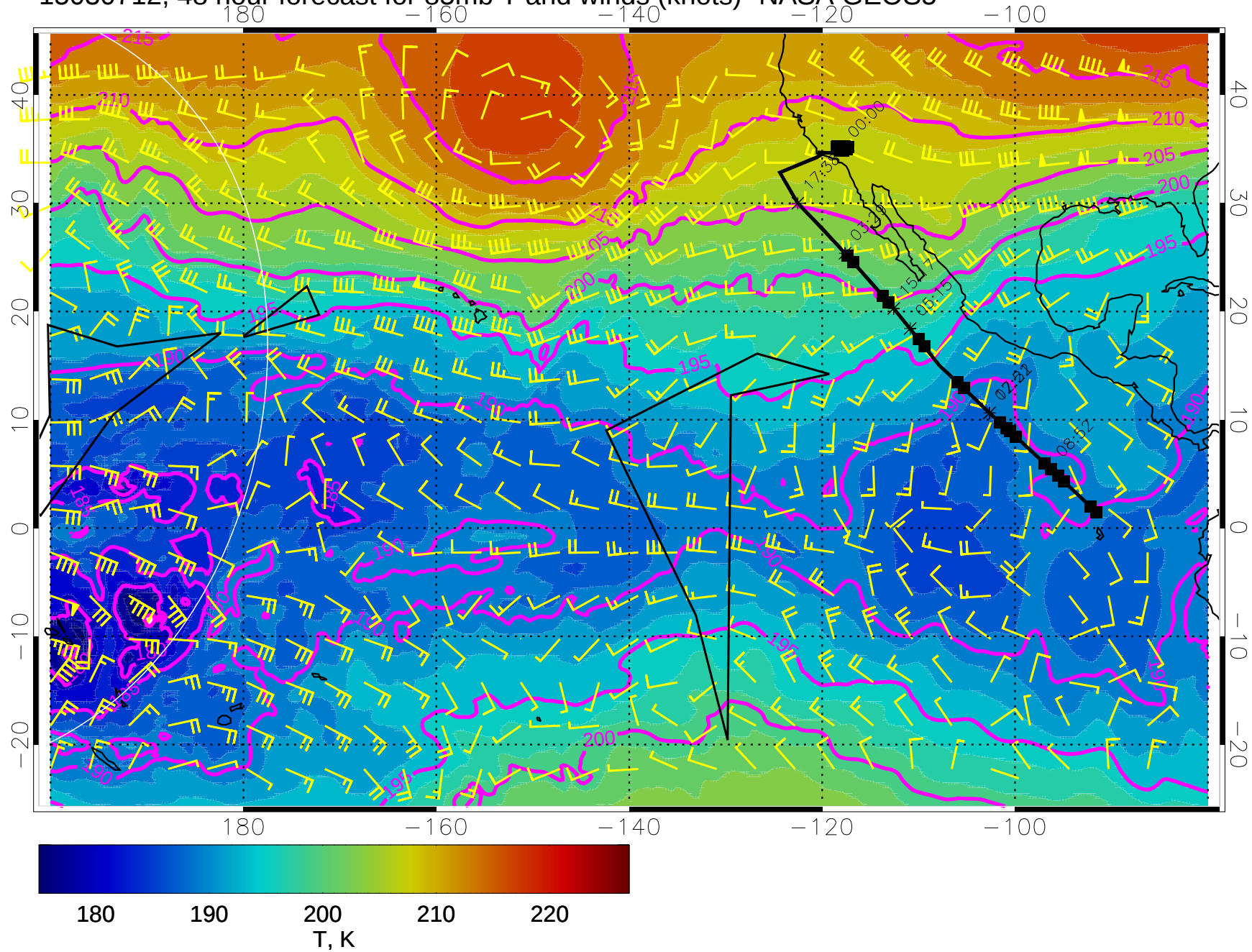
15030712, 48 hour forecast for 85mb T and winds (knots)- NASA GEOS5
