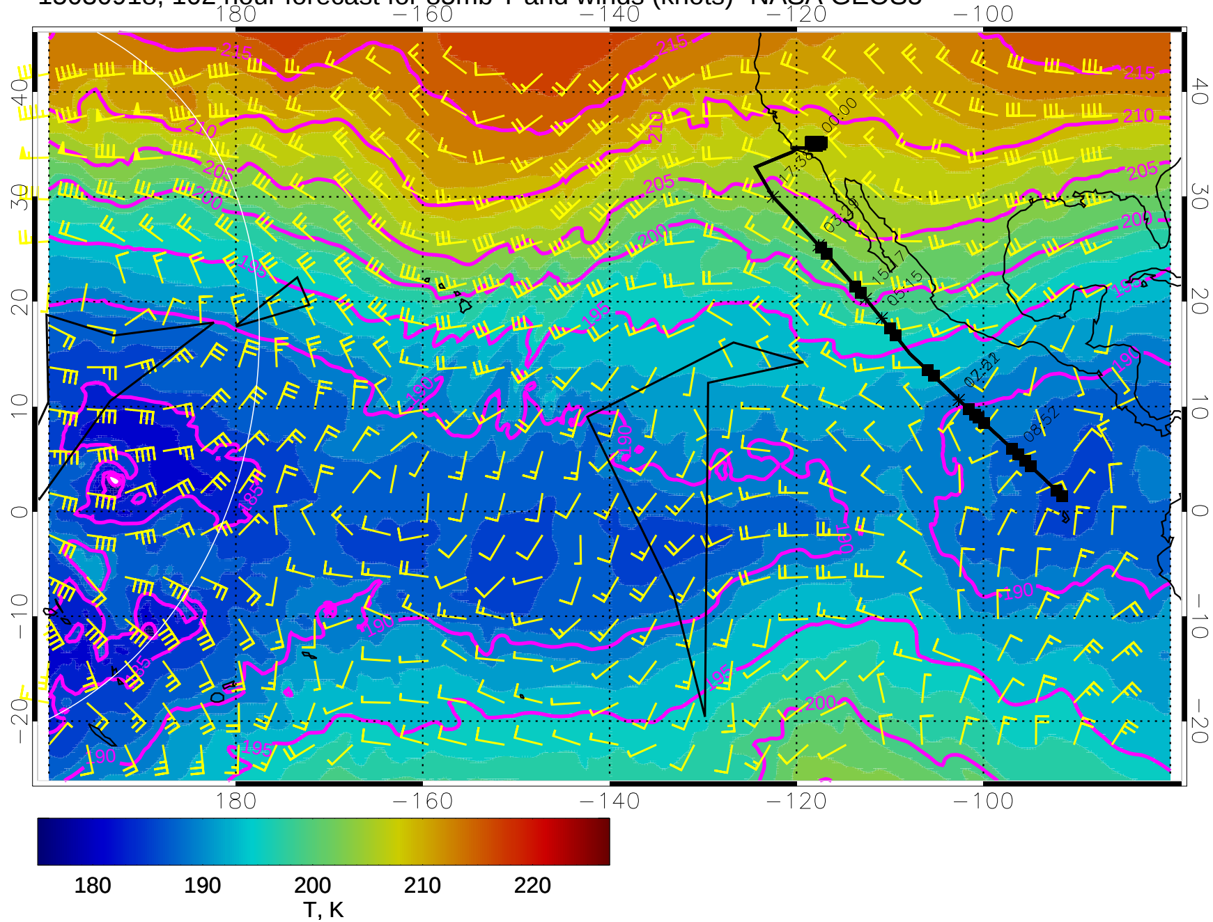
15030918, 102 hour forecast for 85mb T and winds (knots)- NASA GEOS5
