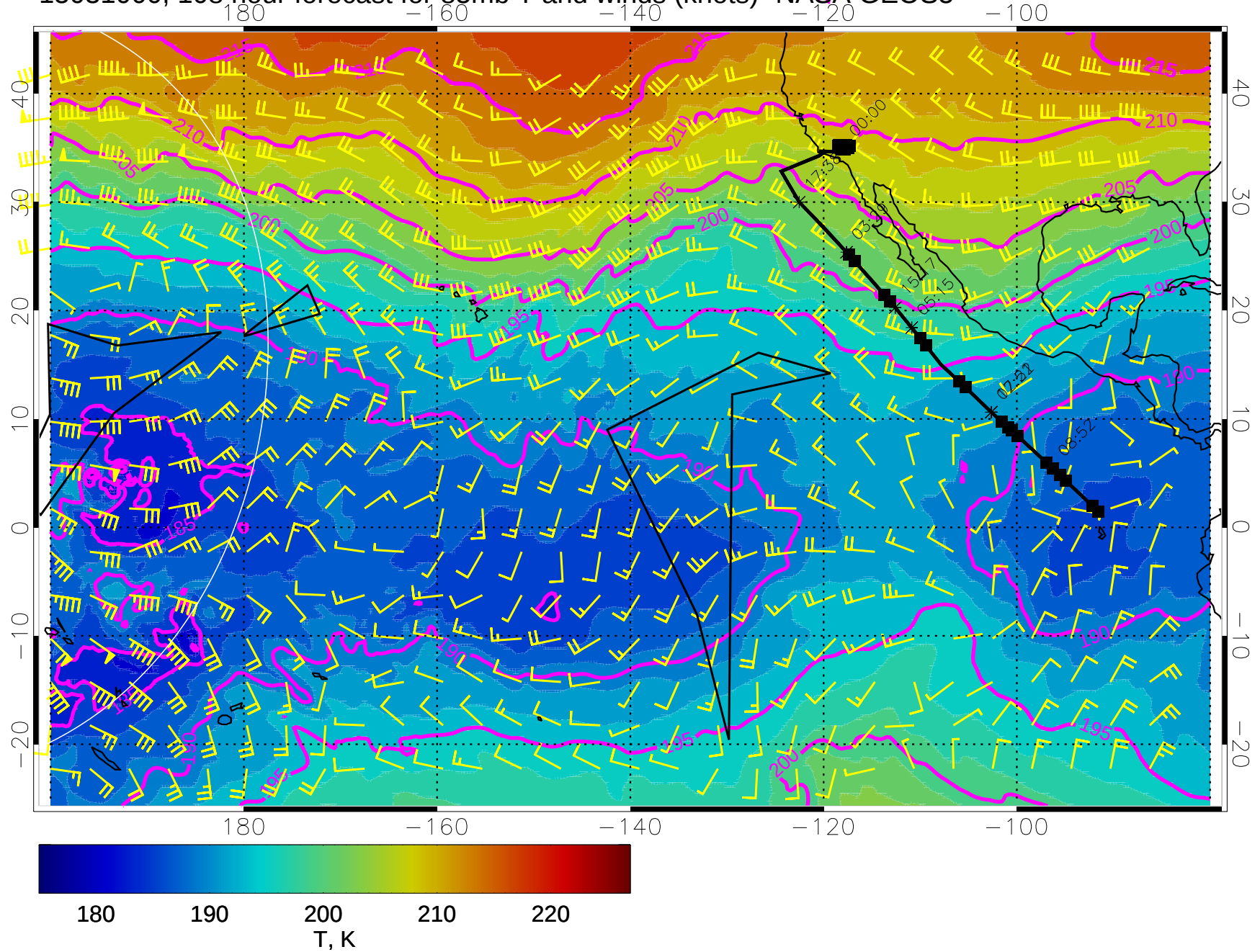
15031000, 108 hour forecast for 85mb T and winds (knots)- NASA GEOS5
