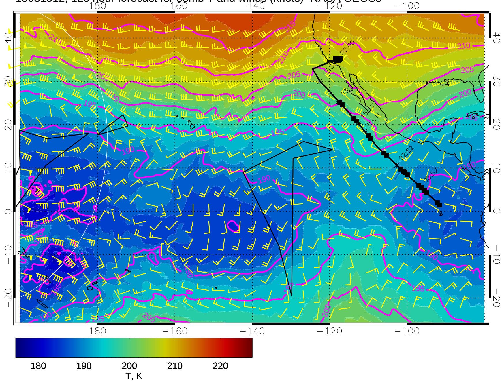
15031012, 120 hour forecast for 85mb T and winds (knots)- NASA GEOS5
