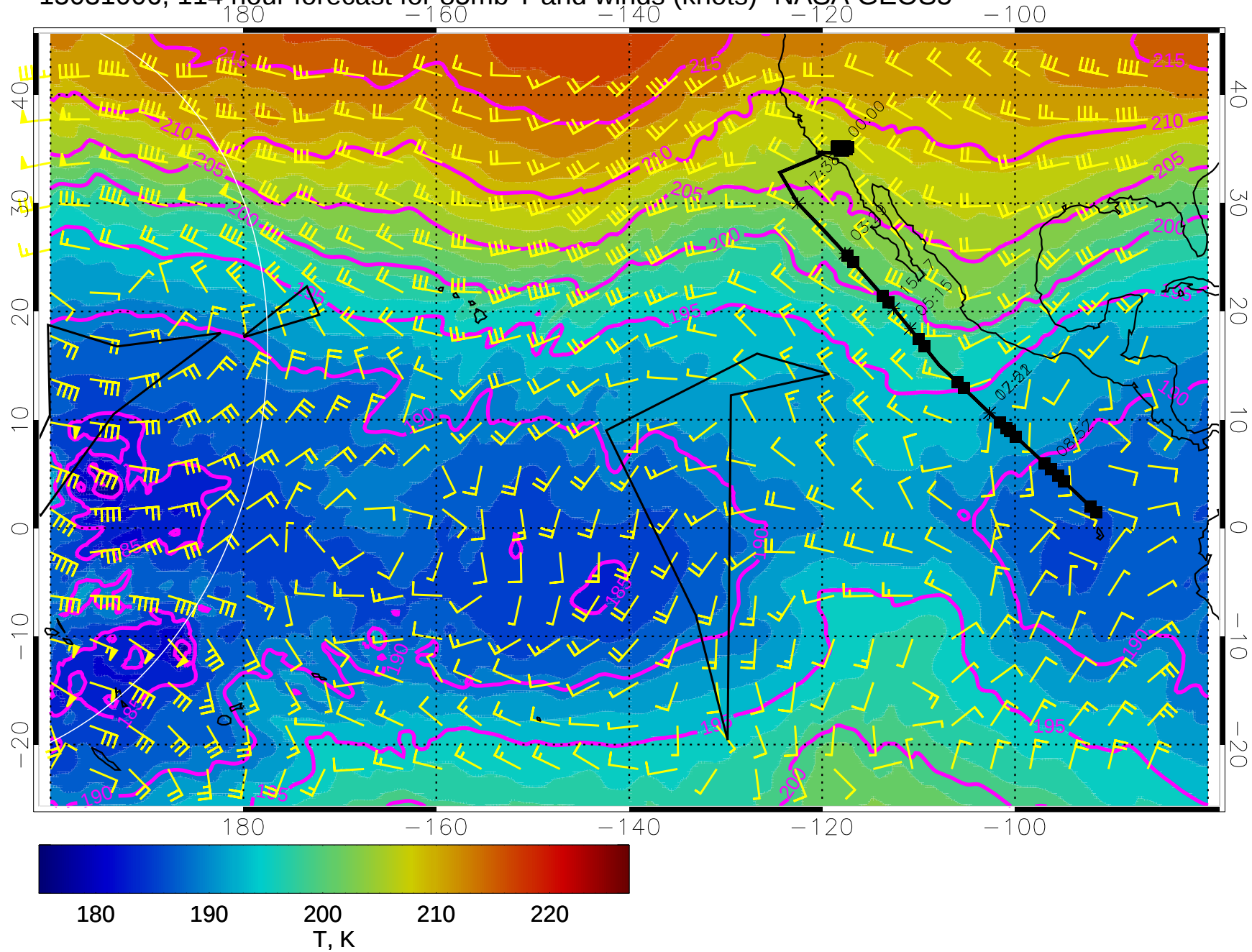
15031006, 114 hour forecast for 85mb T and winds (knots)- NASA GEOS5
