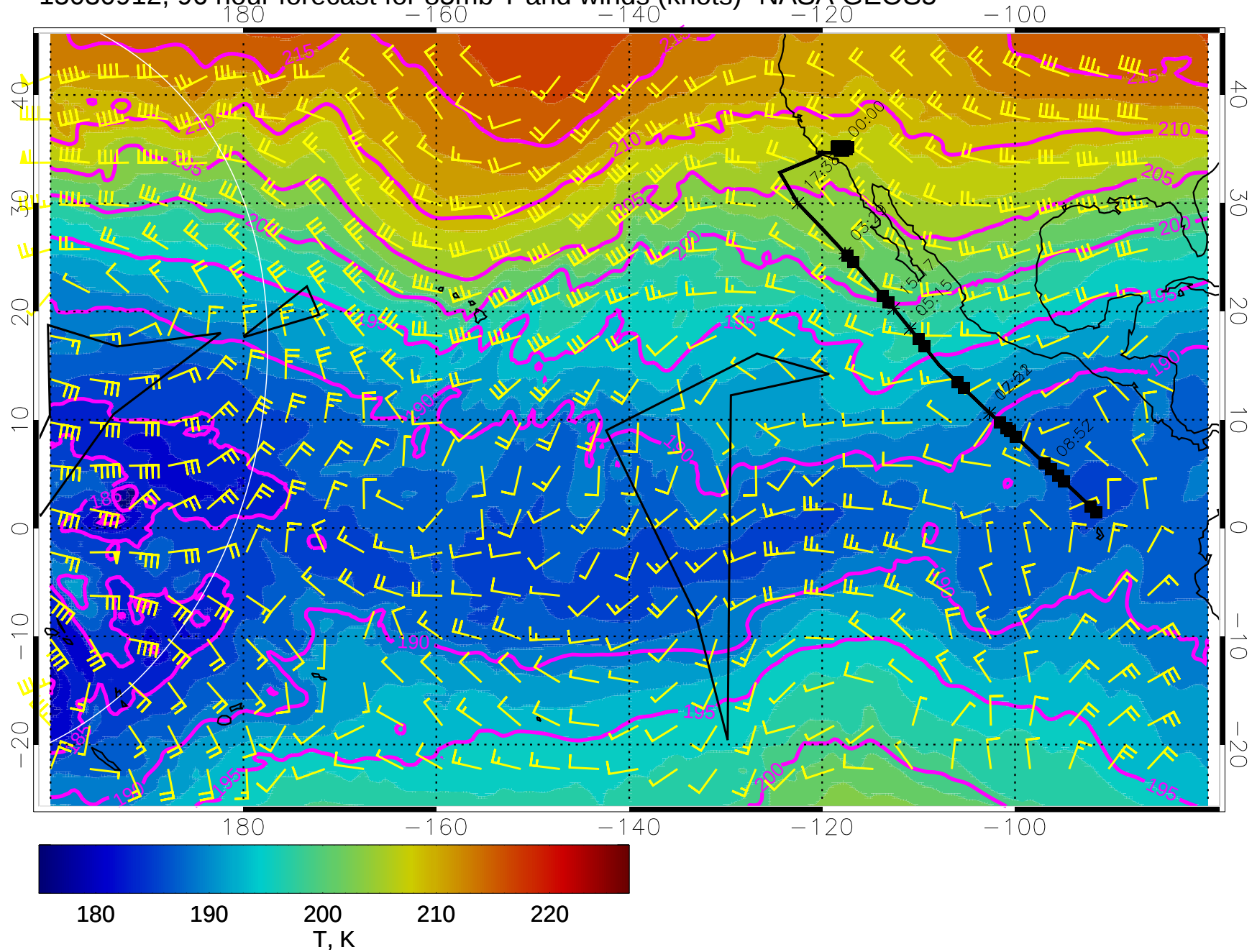
15030912, 96 hour forecast for 85mb T and winds (knots)- NASA GEOS5
