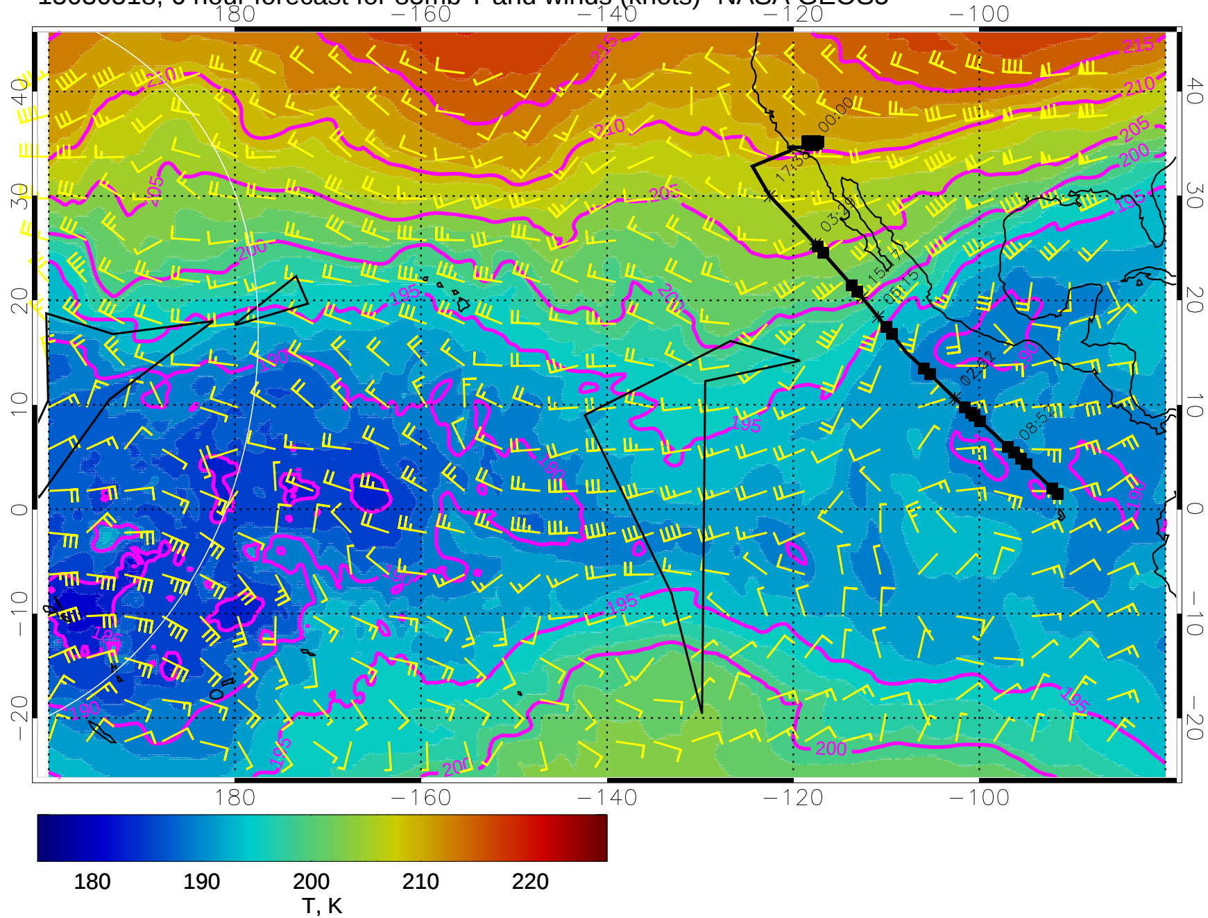
15030518, 6 hour forecast for 85mb T and winds (knots)- NASA GEOS5
