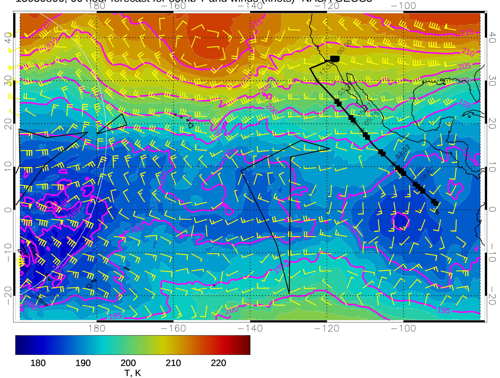
15030806, 66 hour forecast for 85mb T and winds (knots)- NASA GEOS5
