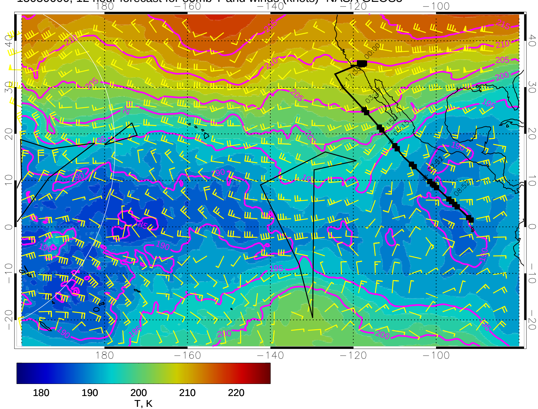
15030600, 12 hour forecast for 85mb T and winds (knots)- NASA GEOS5
