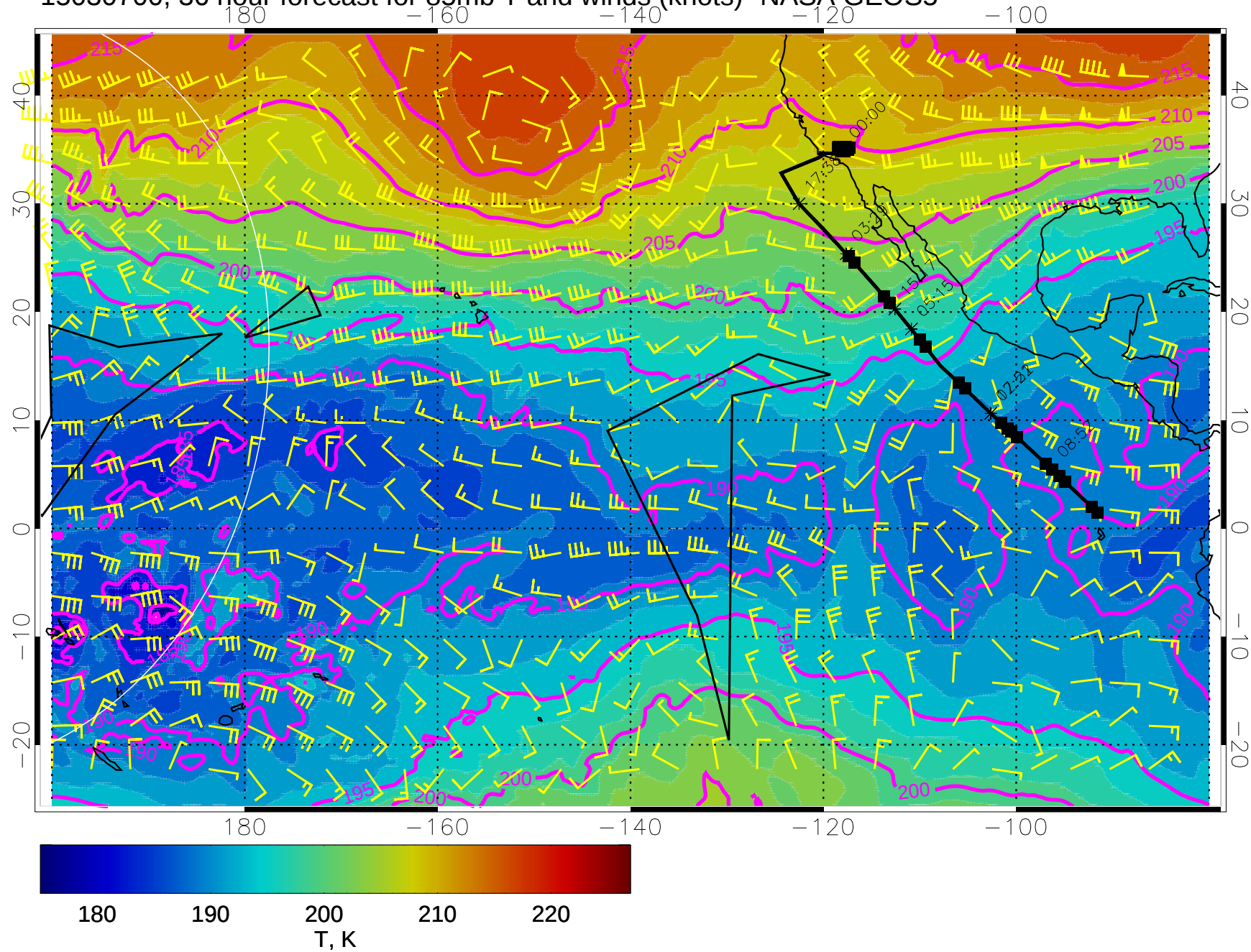
15030700, 36 hour forecast for 85mb T and winds (knots)- NASA GEOS5
