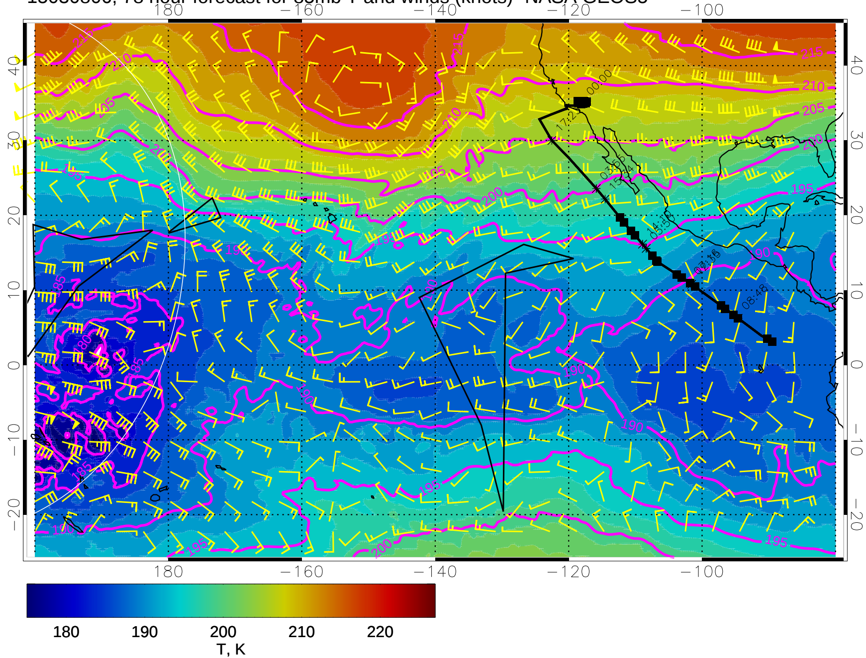
15030806, 78 hour forecast for 85mb T and winds (knots)- NASA GEOS5
