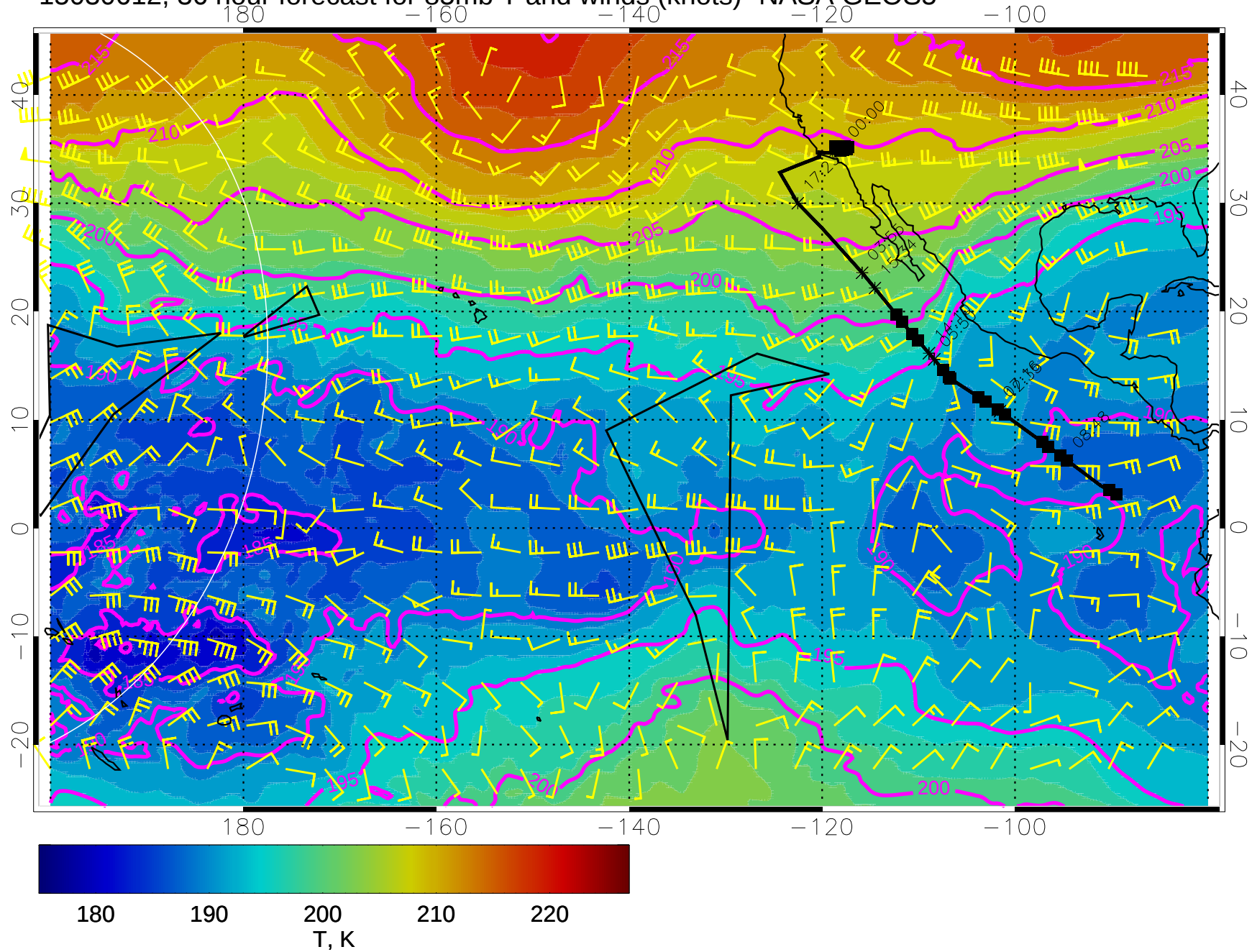
15030612, 36 hour forecast for 85mb T and winds (knots)- NASA GEOS5
