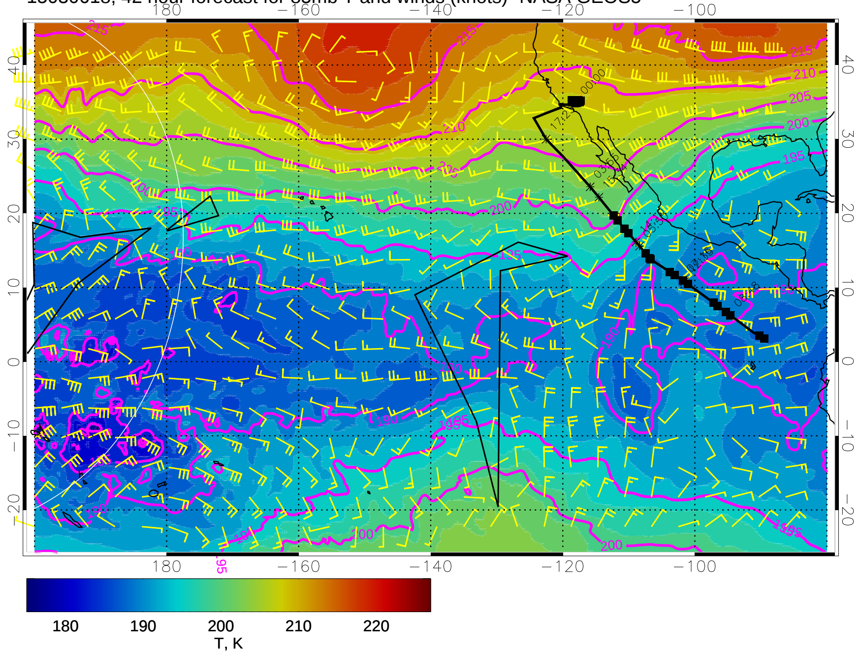
15030618, 42 hour forecast for 85mb T and winds (knots)- NASA GEOS5
