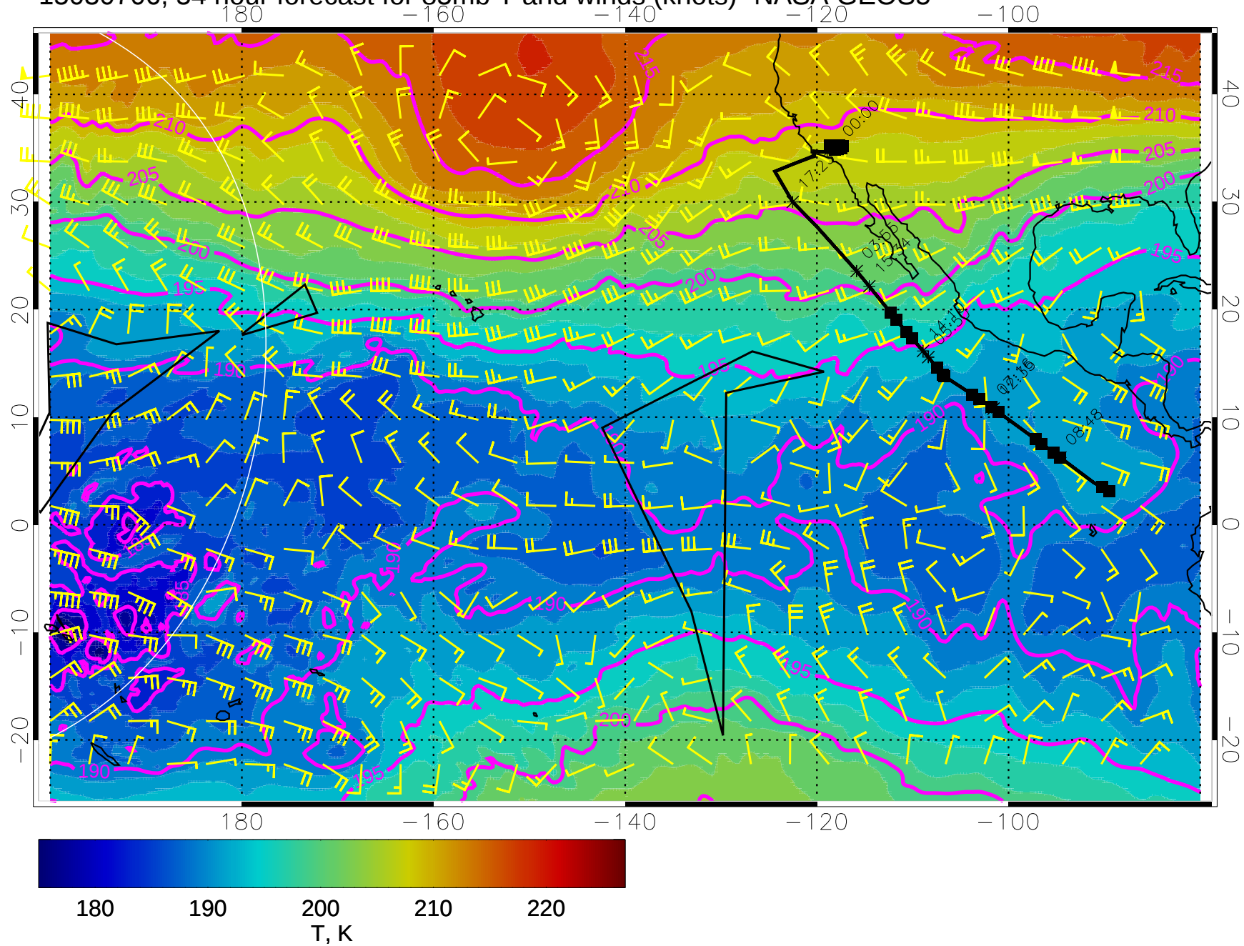
15030706, 54 hour forecast for 85mb T and winds (knots)- NASA GEOS5
