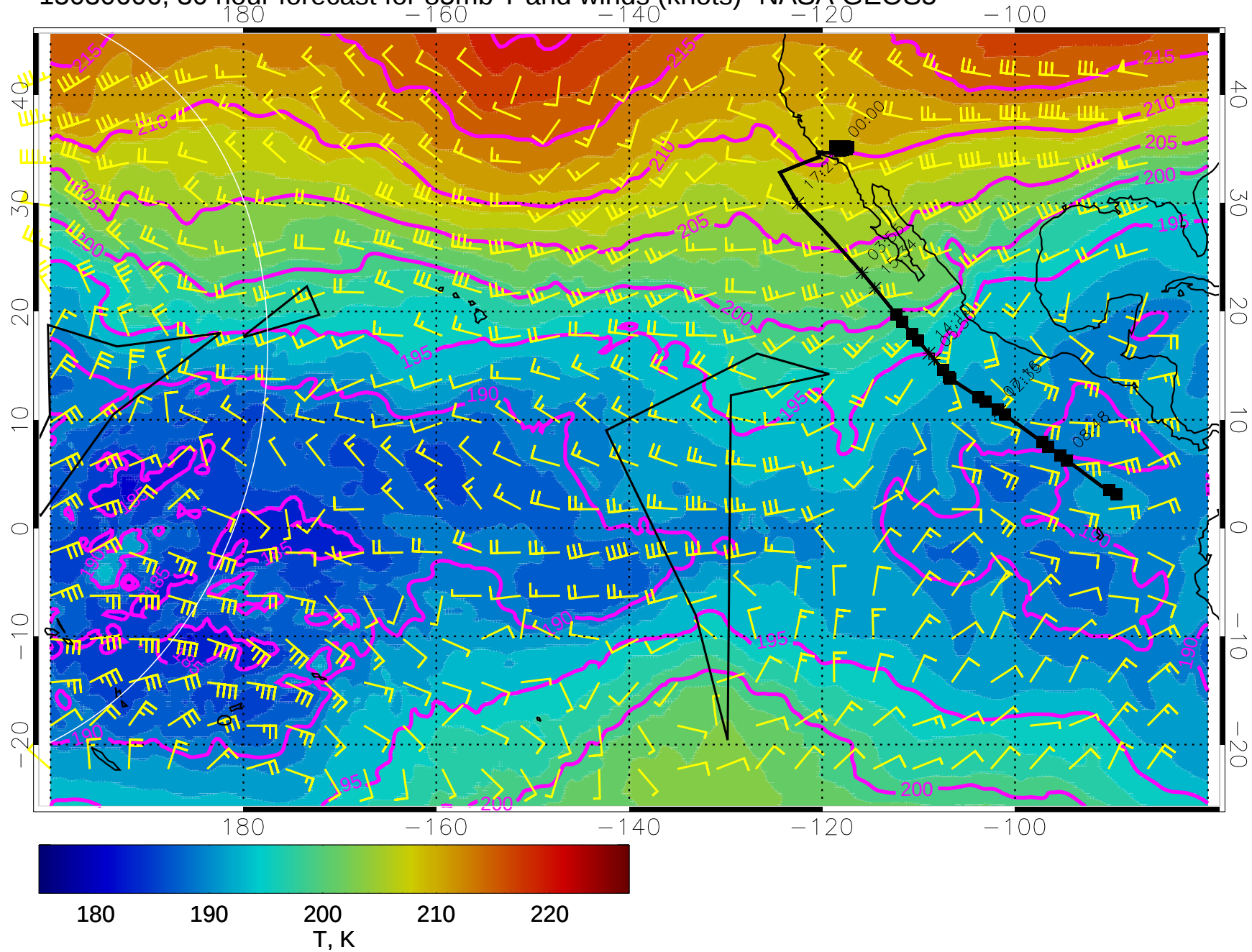
15030606, 30 hour forecast for 85mb T and winds (knots)- NASA GEOS5
