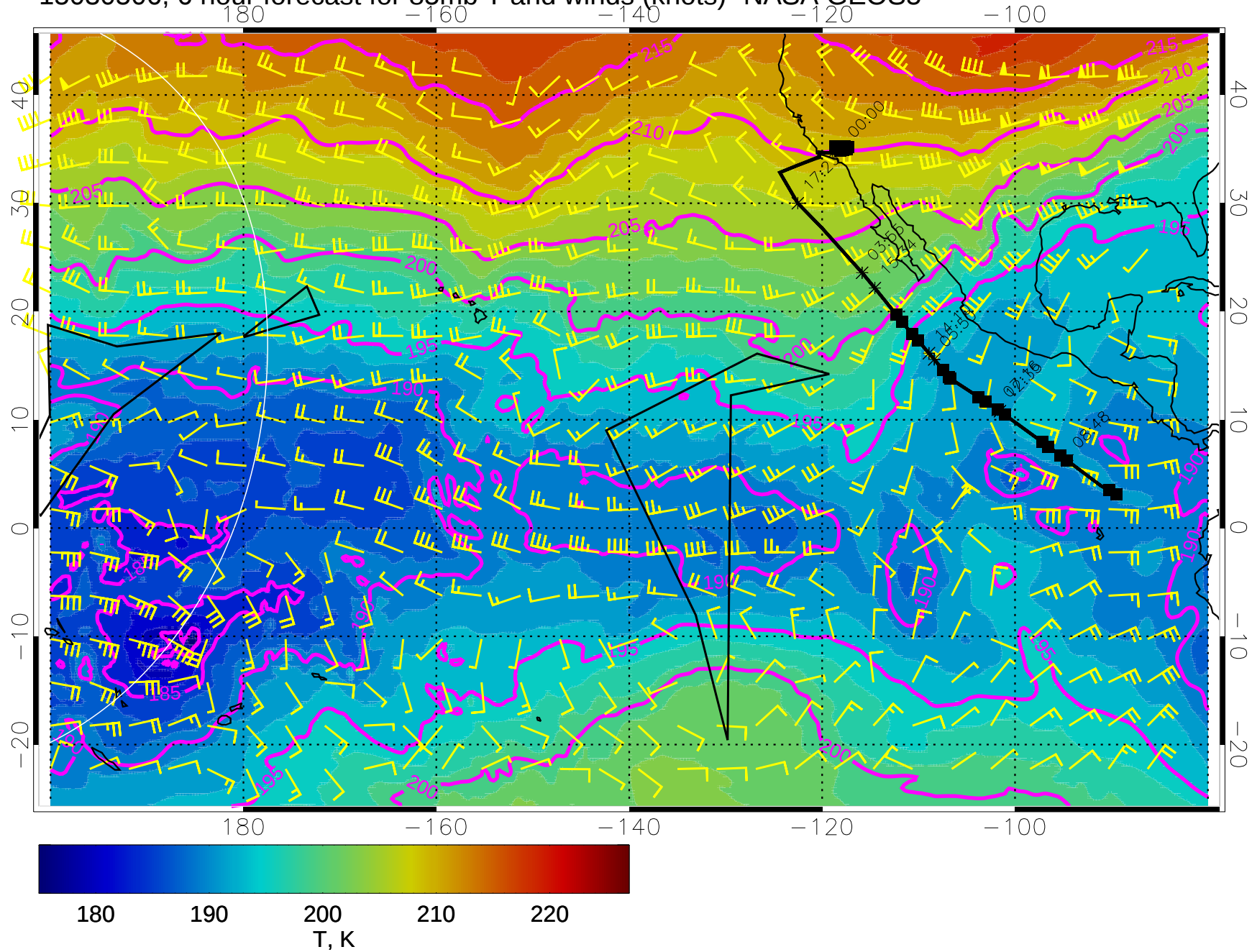
15030506, 6 hour forecast for 85mb T and winds (knots)- NASA GEOS5
