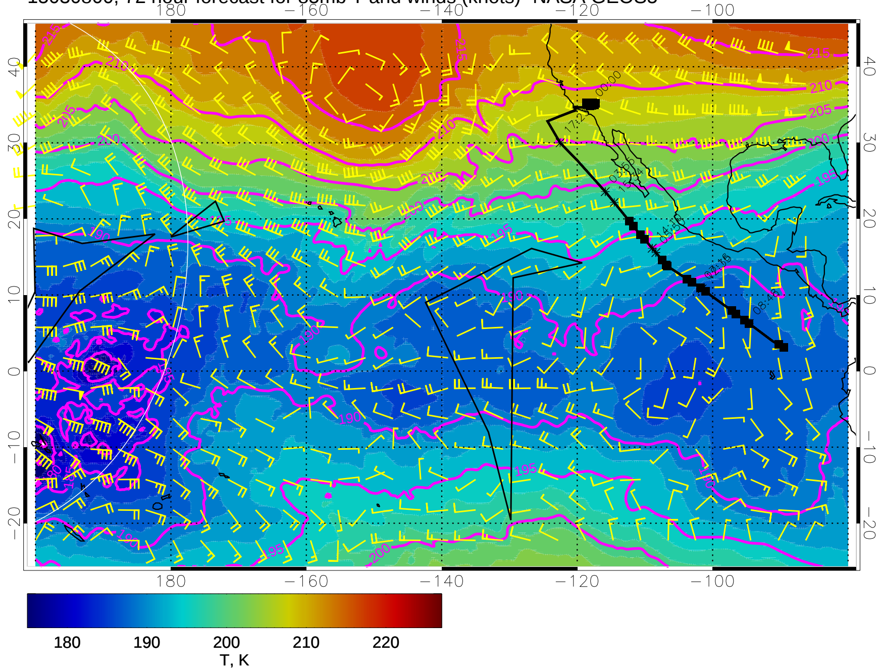
15030800, 72 hour forecast for 85mb T and winds (knots)- NASA GEOS5
