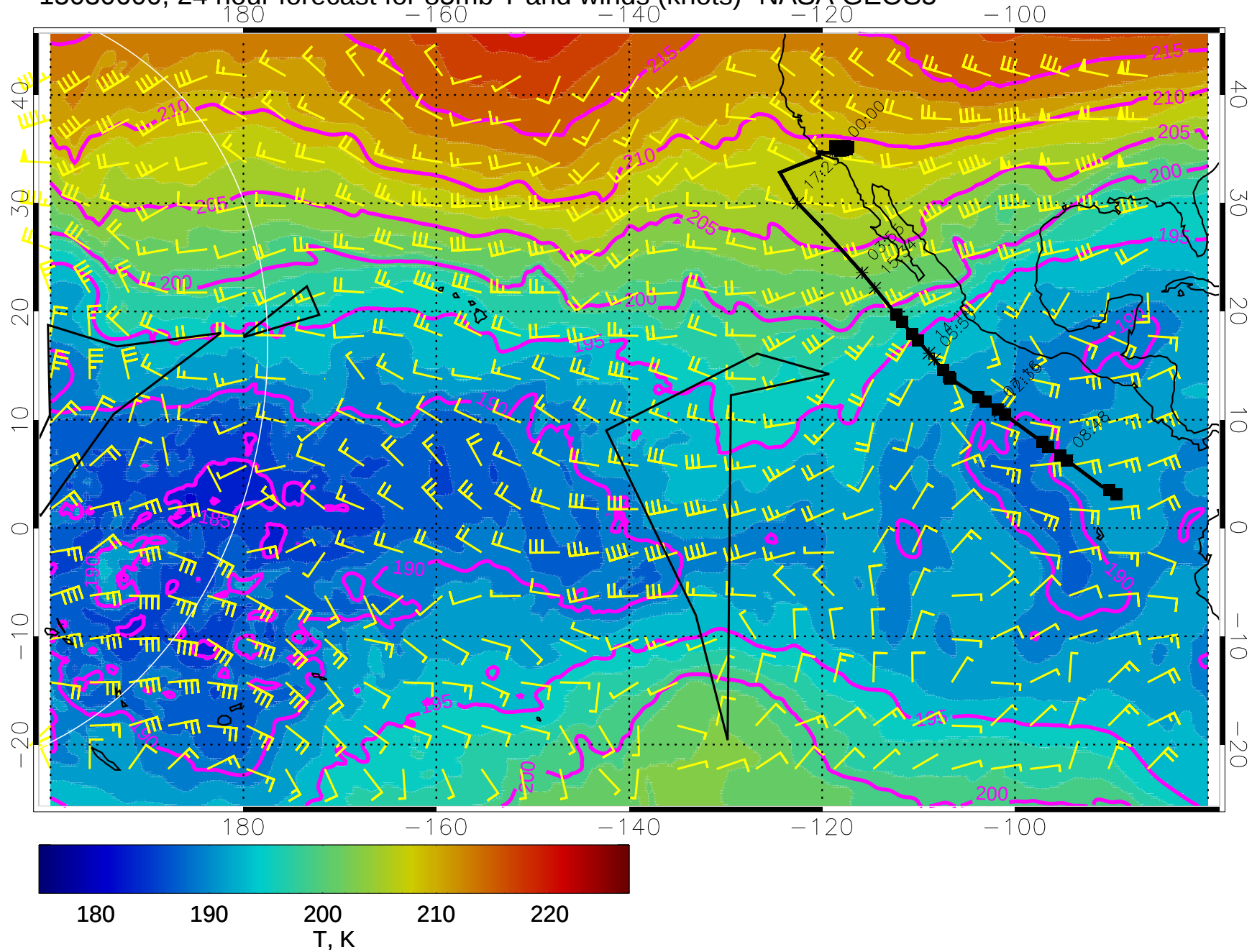
15030600, 24 hour forecast for 85mb T and winds (knots)- NASA GEOS5
