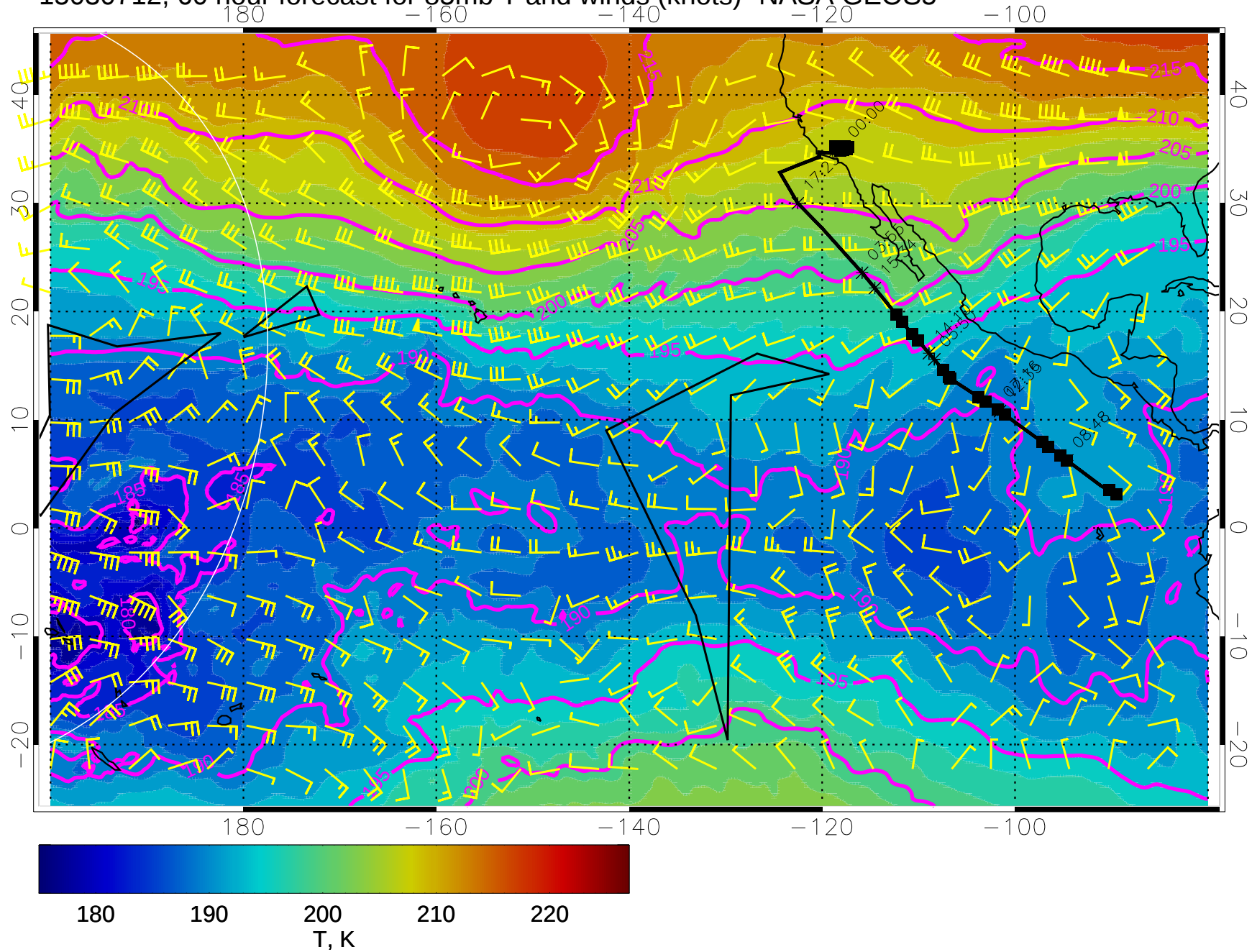
15030712, 60 hour forecast for 85mb T and winds (knots)- NASA GEOS5
