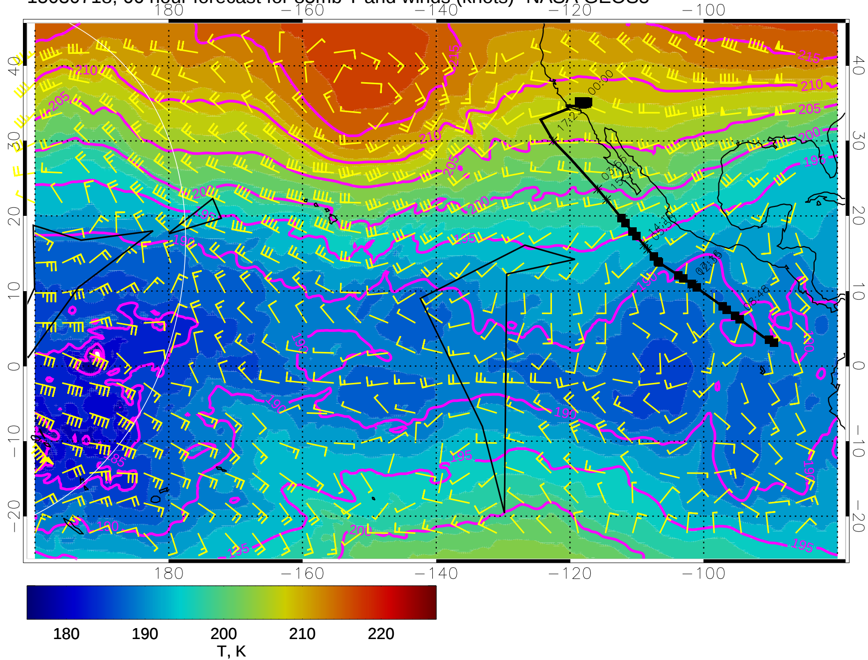
15030718, 66 hour forecast for 85mb T and winds (knots)- NASA GEOS5
