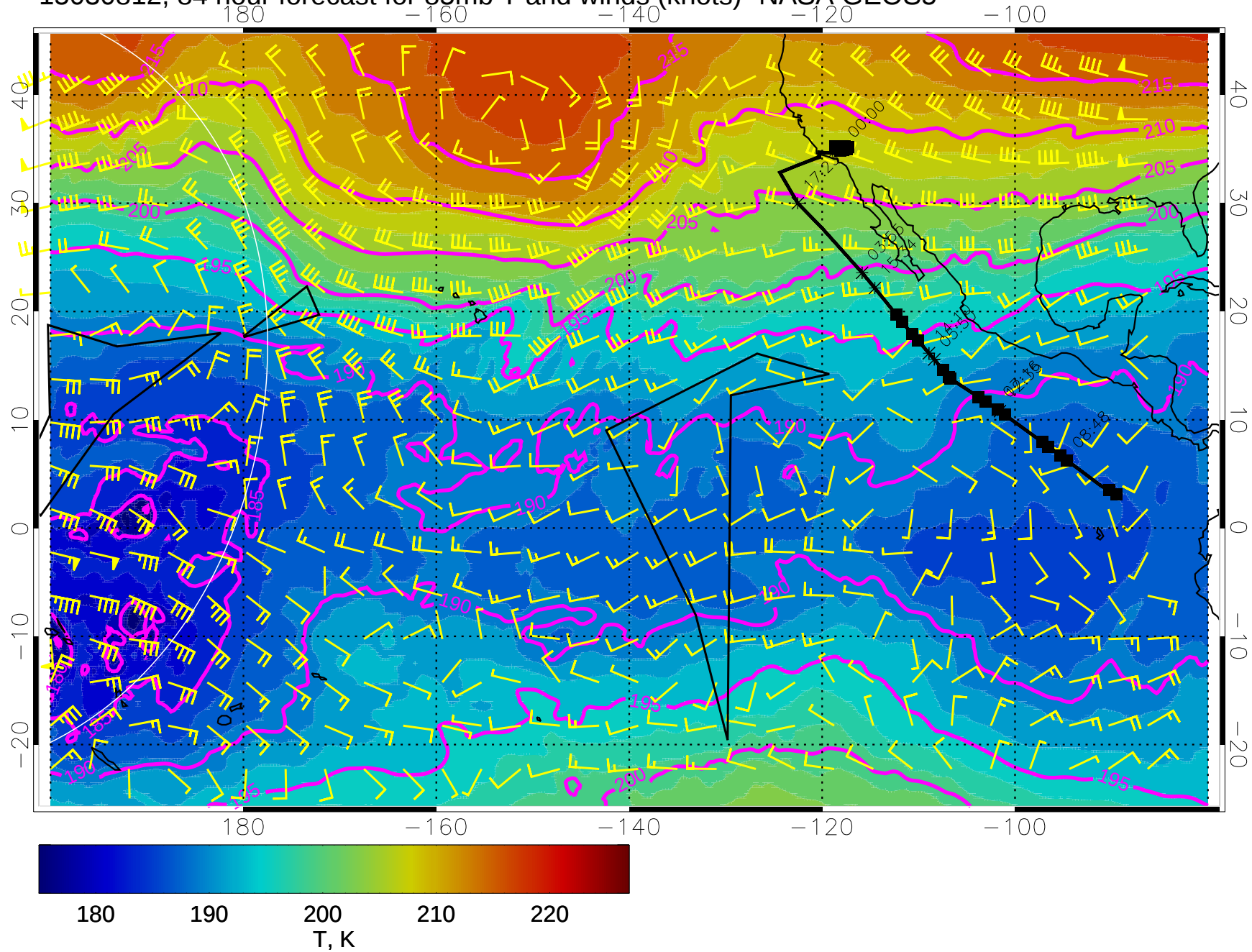
15030812, 84 hour forecast for 85mb T and winds (knots)- NASA GEOS5
