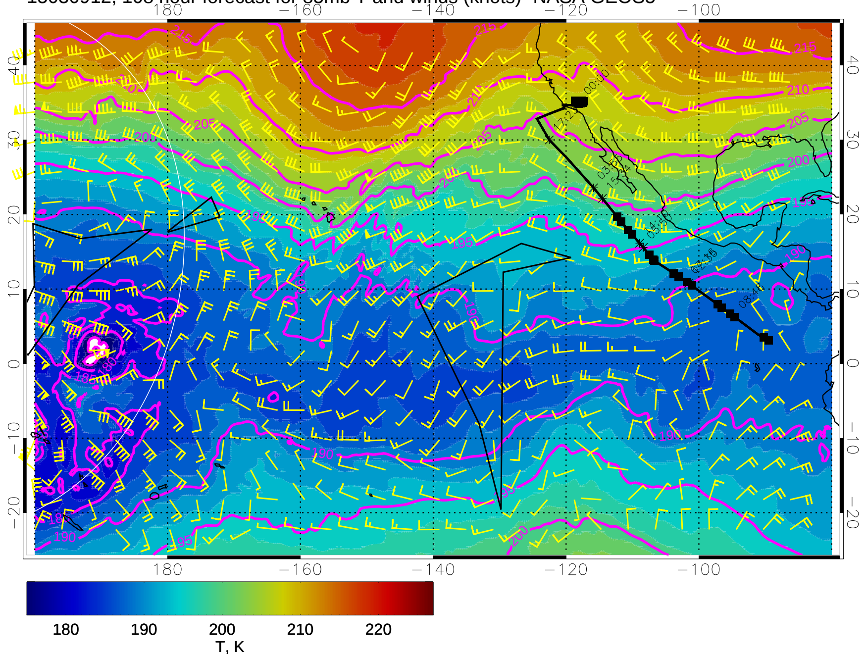
15030912, 108 hour forecast for 85mb T and winds (knots)- NASA GEOS5
