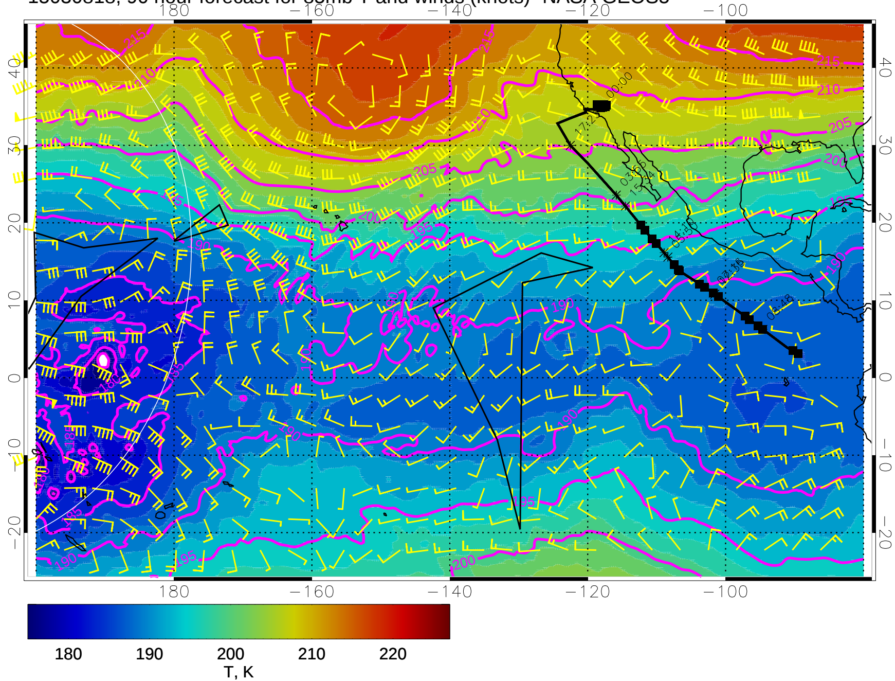
15030818, 90 hour forecast for 85mb T and winds (knots)- NASA GEOS5
