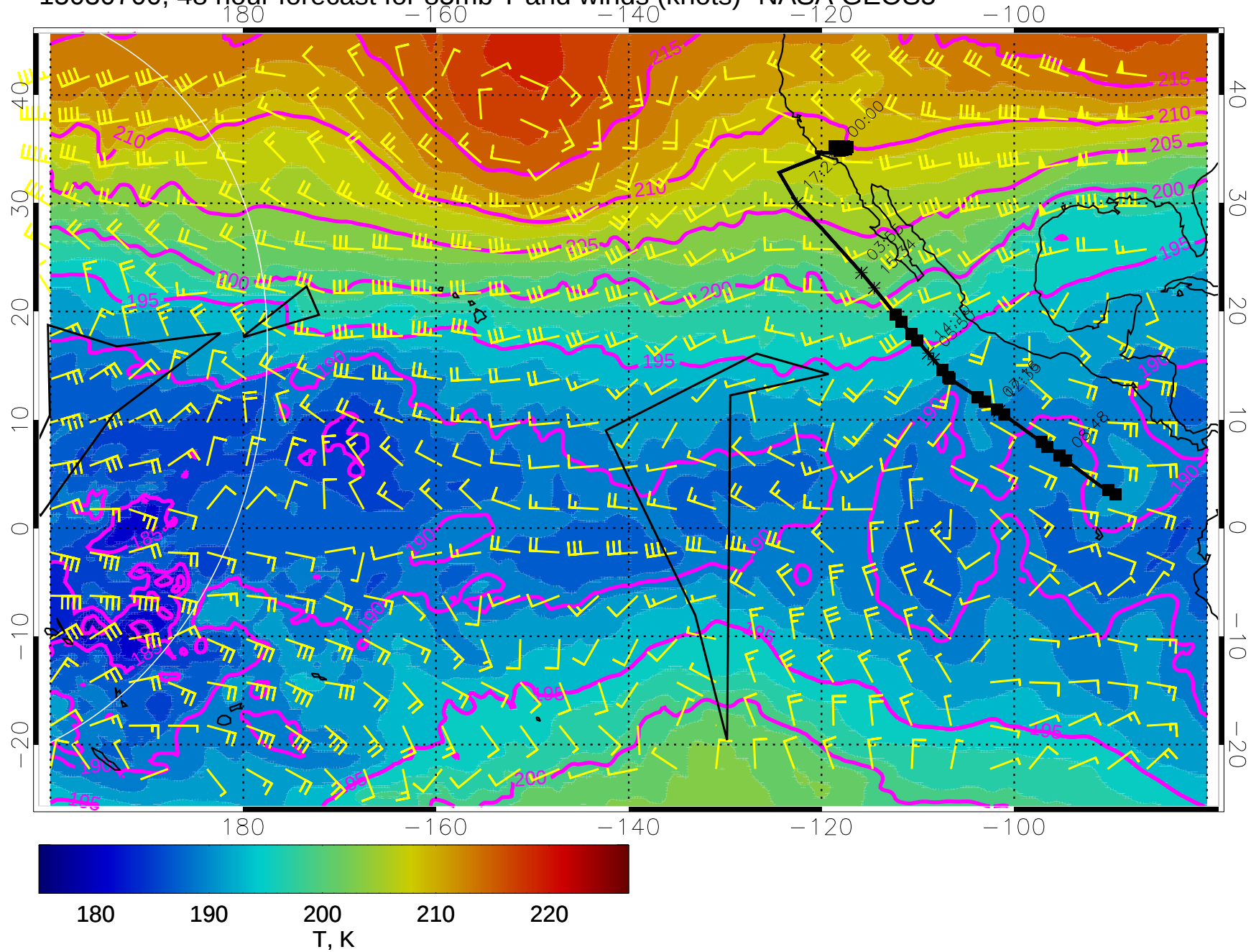
15030700, 48 hour forecast for 85mb T and winds (knots)- NASA GEOS5
