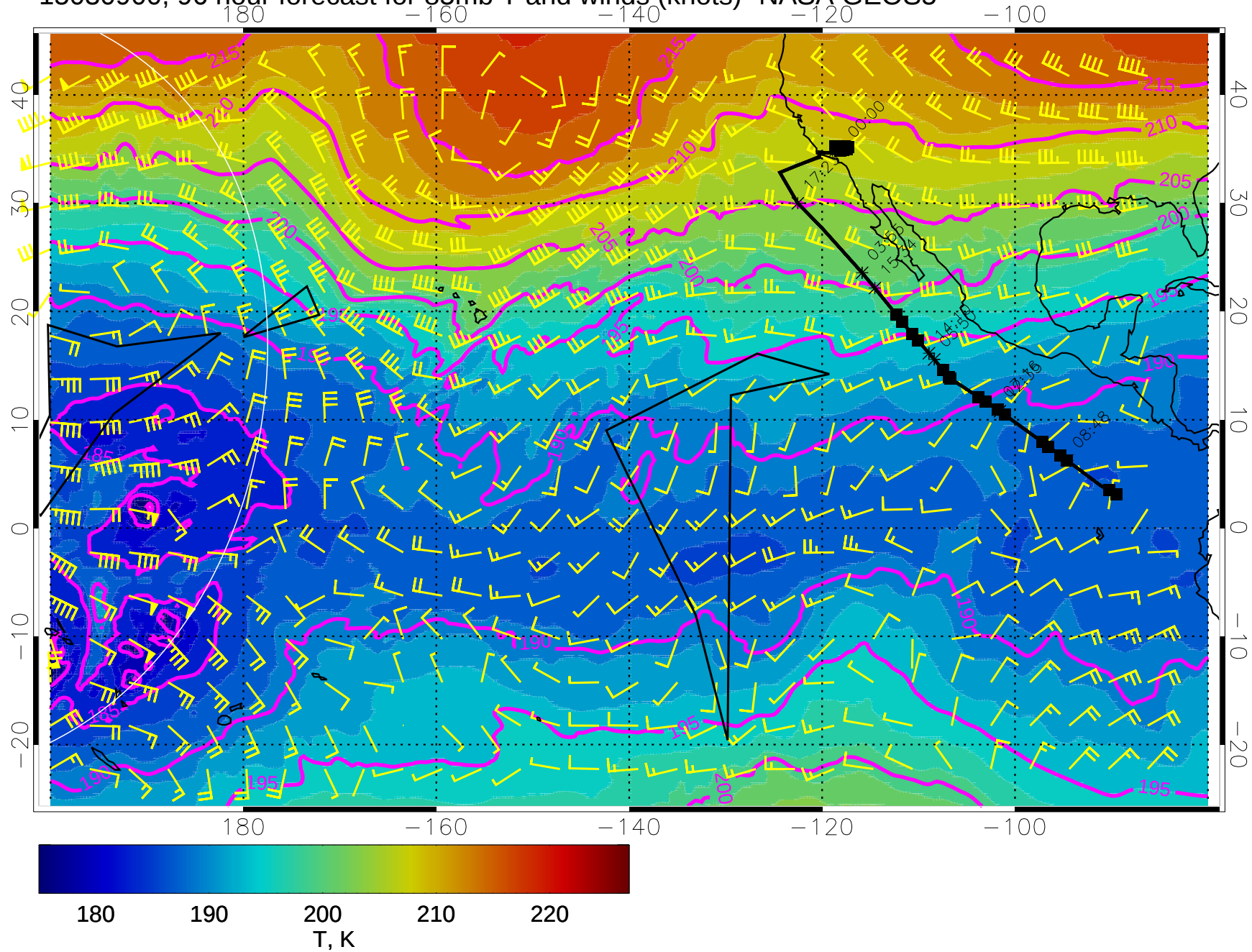
15030900, 96 hour forecast for 85mb T and winds (knots)- NASA GEOS5
