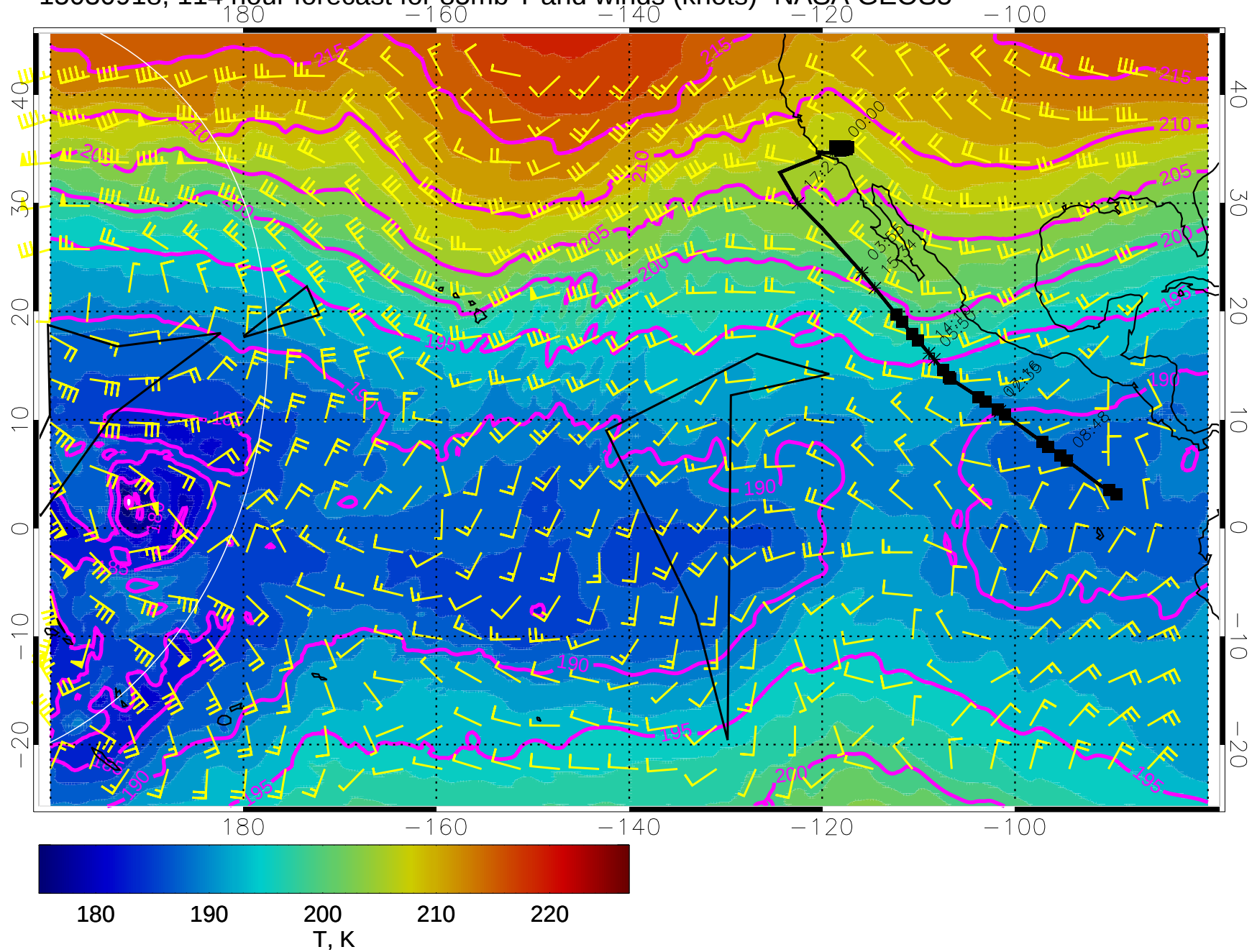
15030918, 114 hour forecast for 85mb T and winds (knots)- NASA GEOS5
