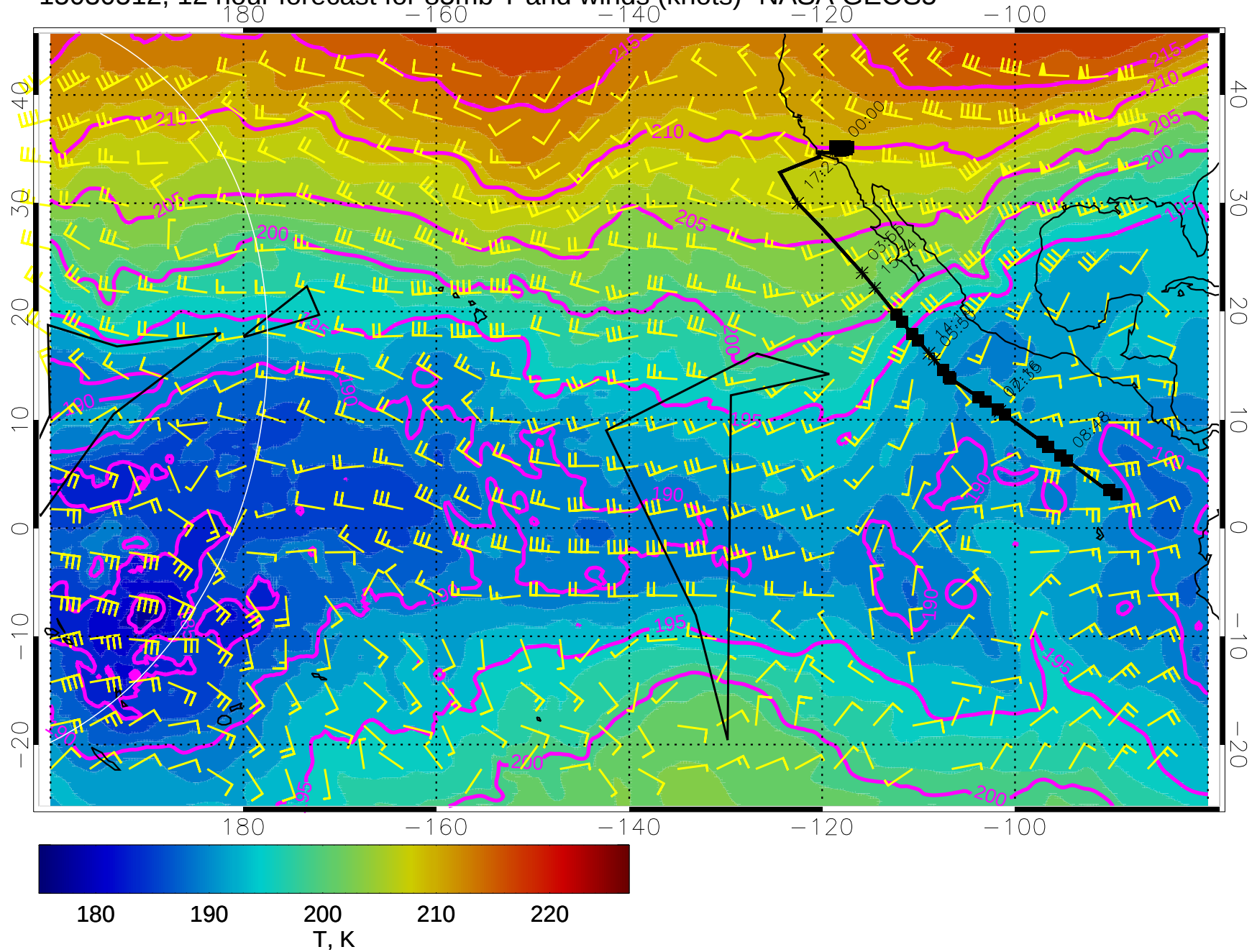
15030512, 12 hour forecast for 85mb T and winds (knots)- NASA GEOS5
