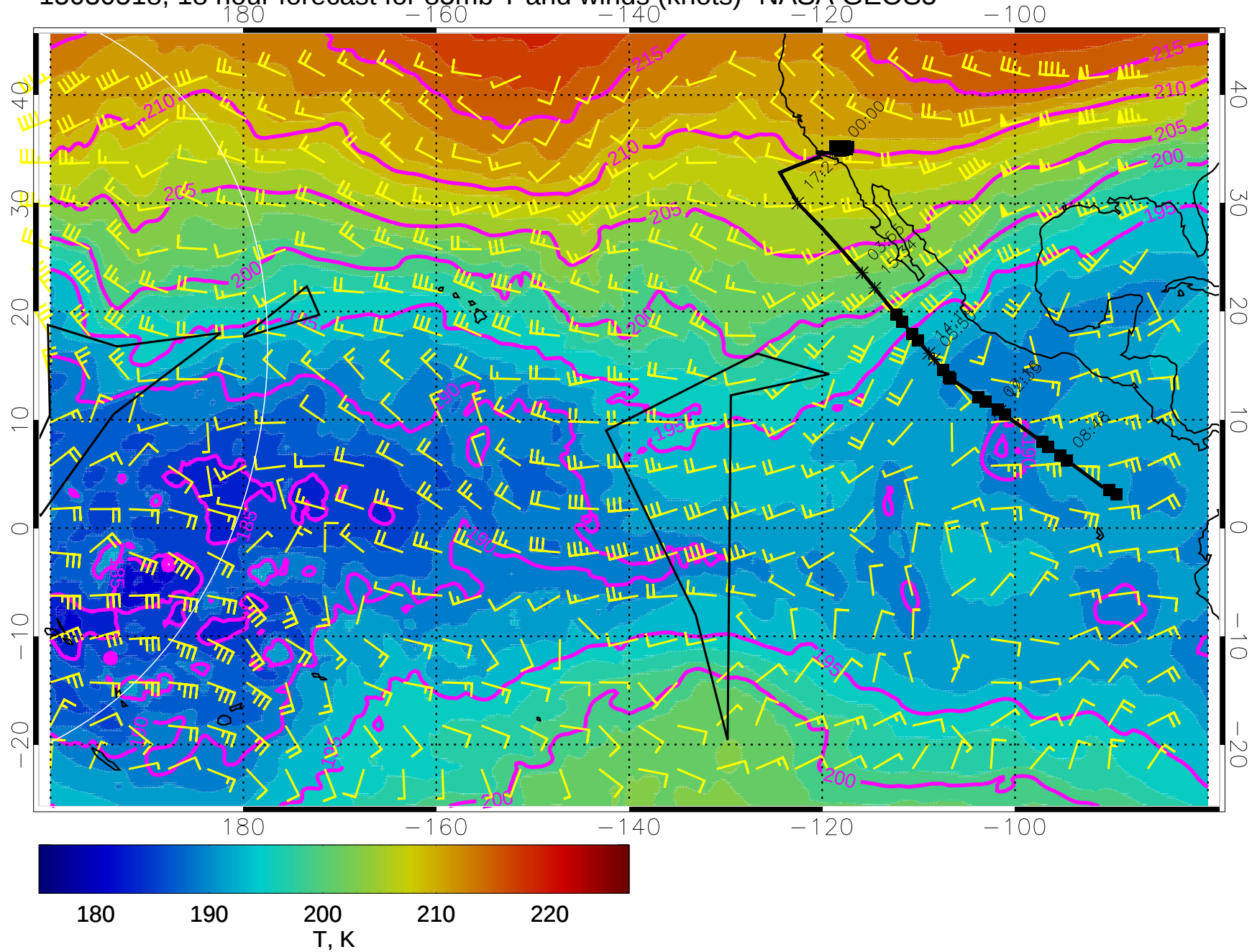
15030518, 18 hour forecast for 85mb T and winds (knots)- NASA GEOS5
