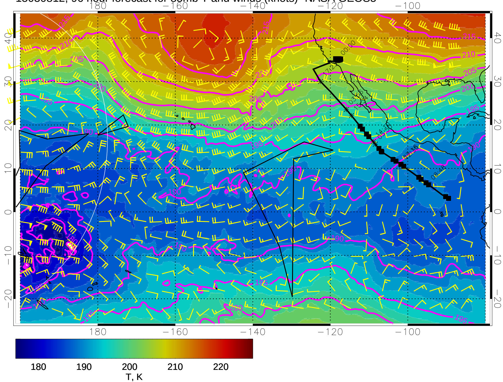
15030812, 96 hour forecast for 85mb T and winds (knots)- NASA GEOS5
