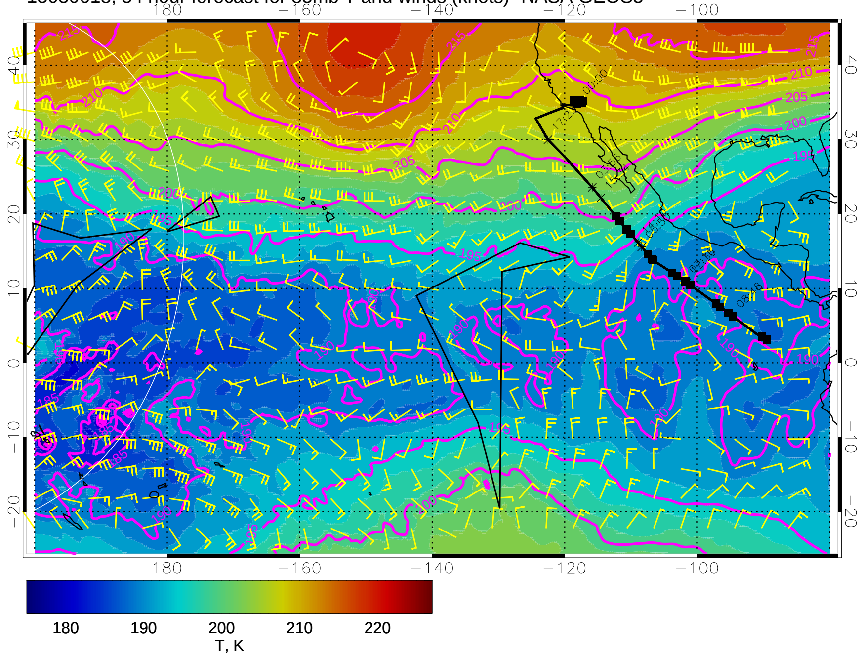
15030618, 54 hour forecast for 85mb T and winds (knots)- NASA GEOS5
