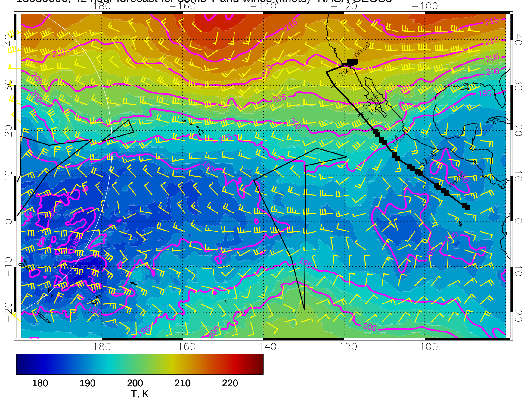
15030606, 42 hour forecast for 85mb T and winds (knots)- NASA GEOS5
