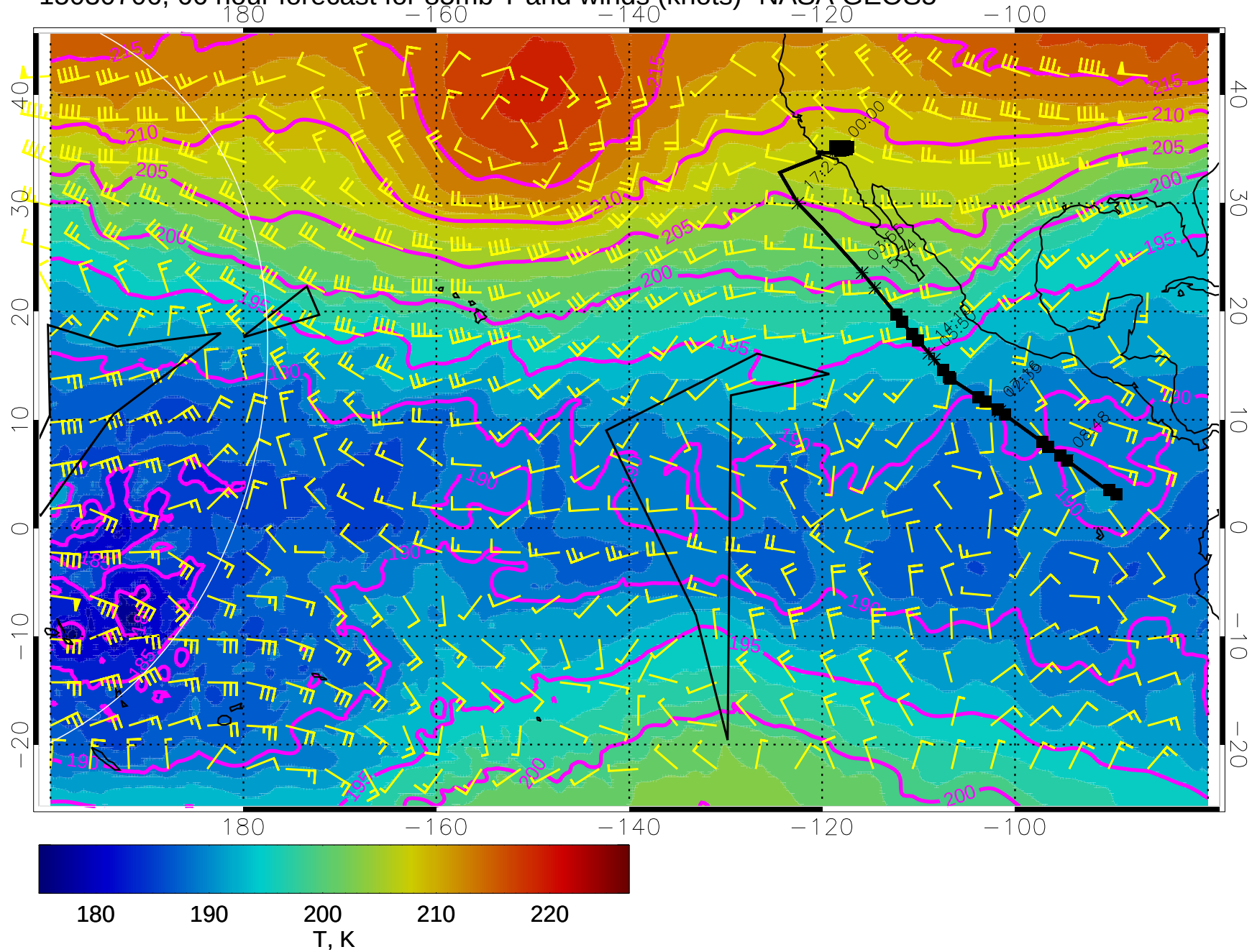
15030706, 66 hour forecast for 85mb T and winds (knots)- NASA GEOS5
