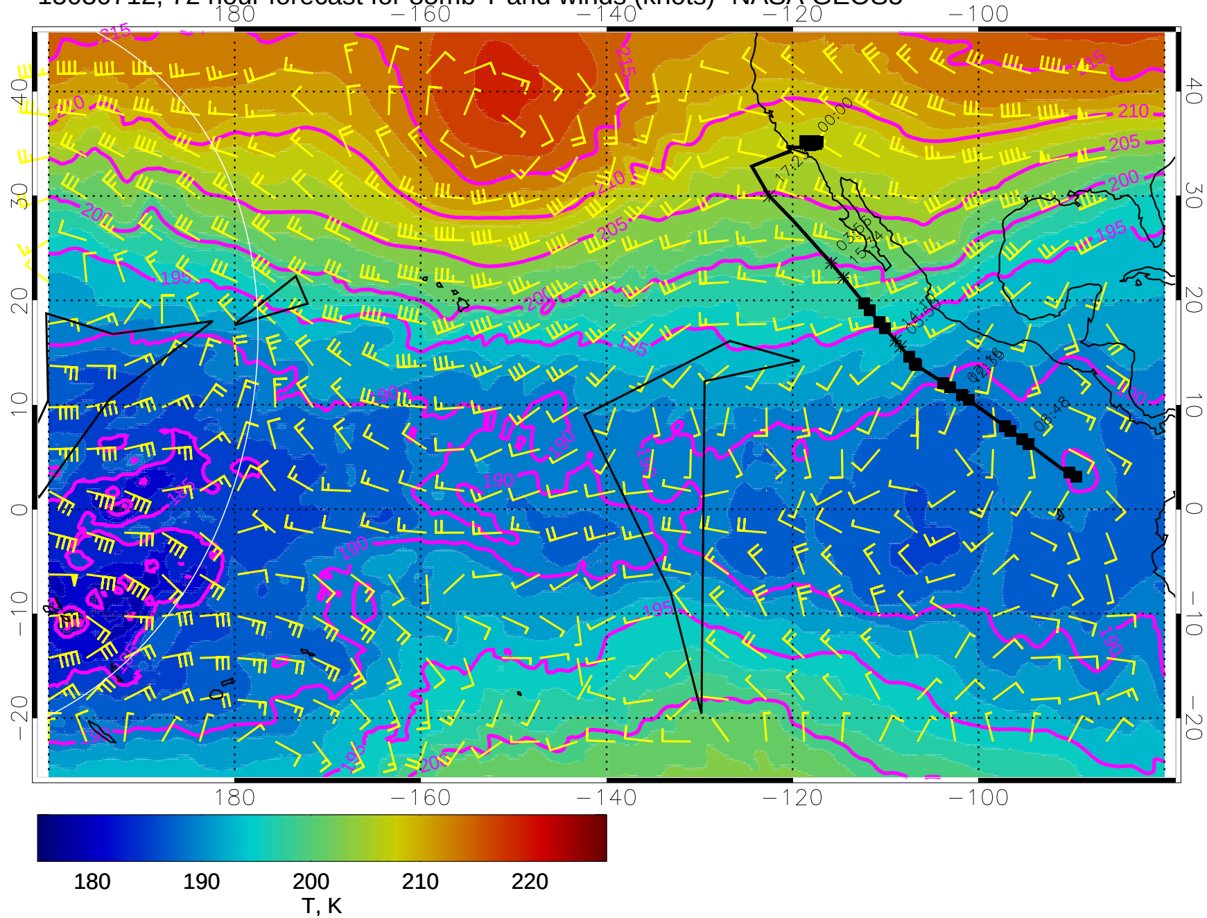
15030712, 72 hour forecast for 85mb T and winds (knots)- NASA GEOS5
