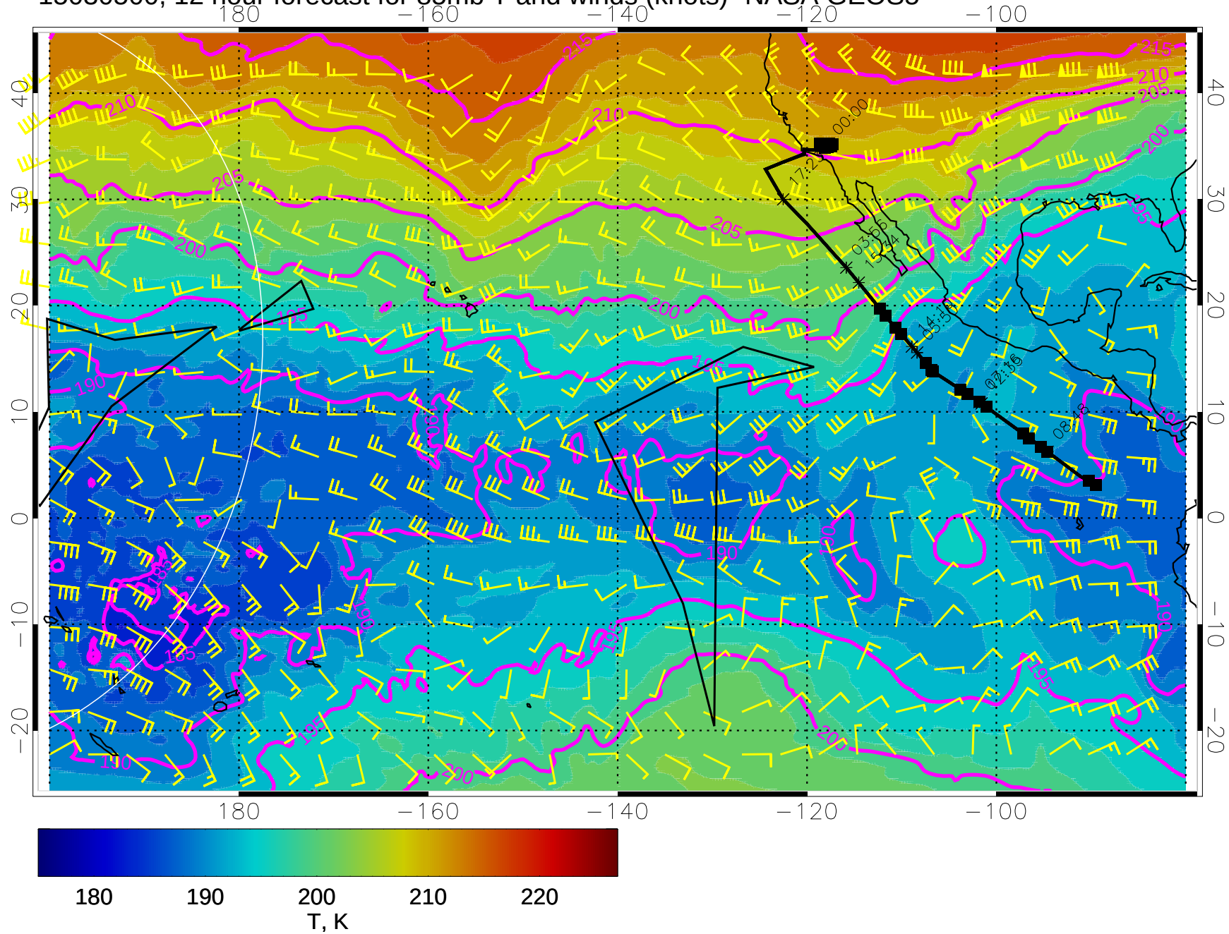
15030500, 12 hour forecast for 85mb T and winds (knots)- NASA GEOS5
