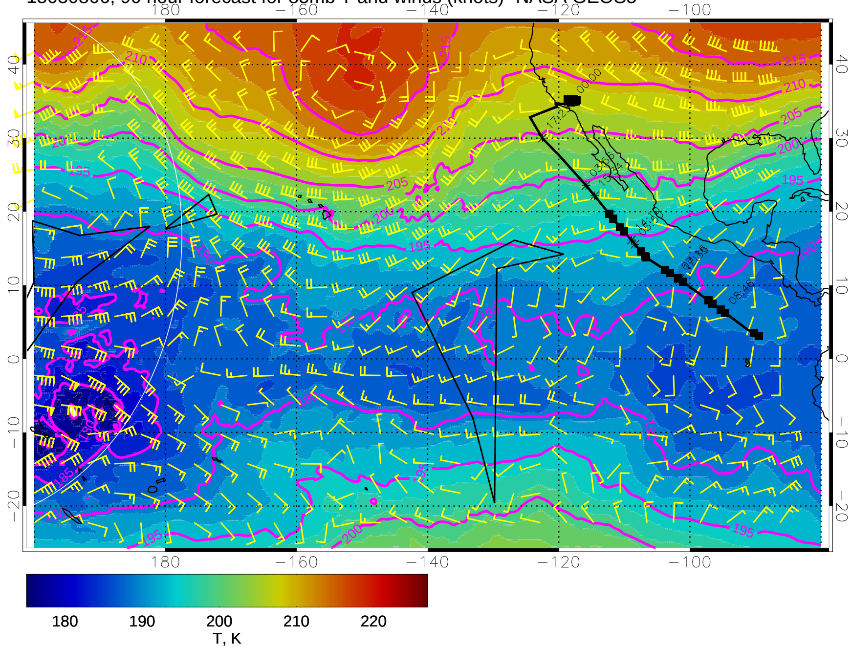
15030806, 90 hour forecast for 85mb T and winds (knots)- NASA GEOS5
