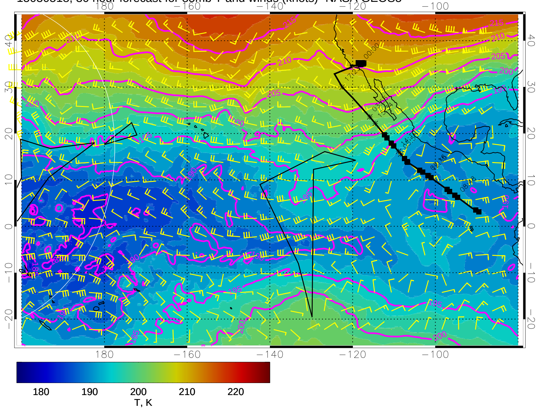
15030518, 30 hour forecast for 85mb T and winds (knots)- NASA GEOS5
