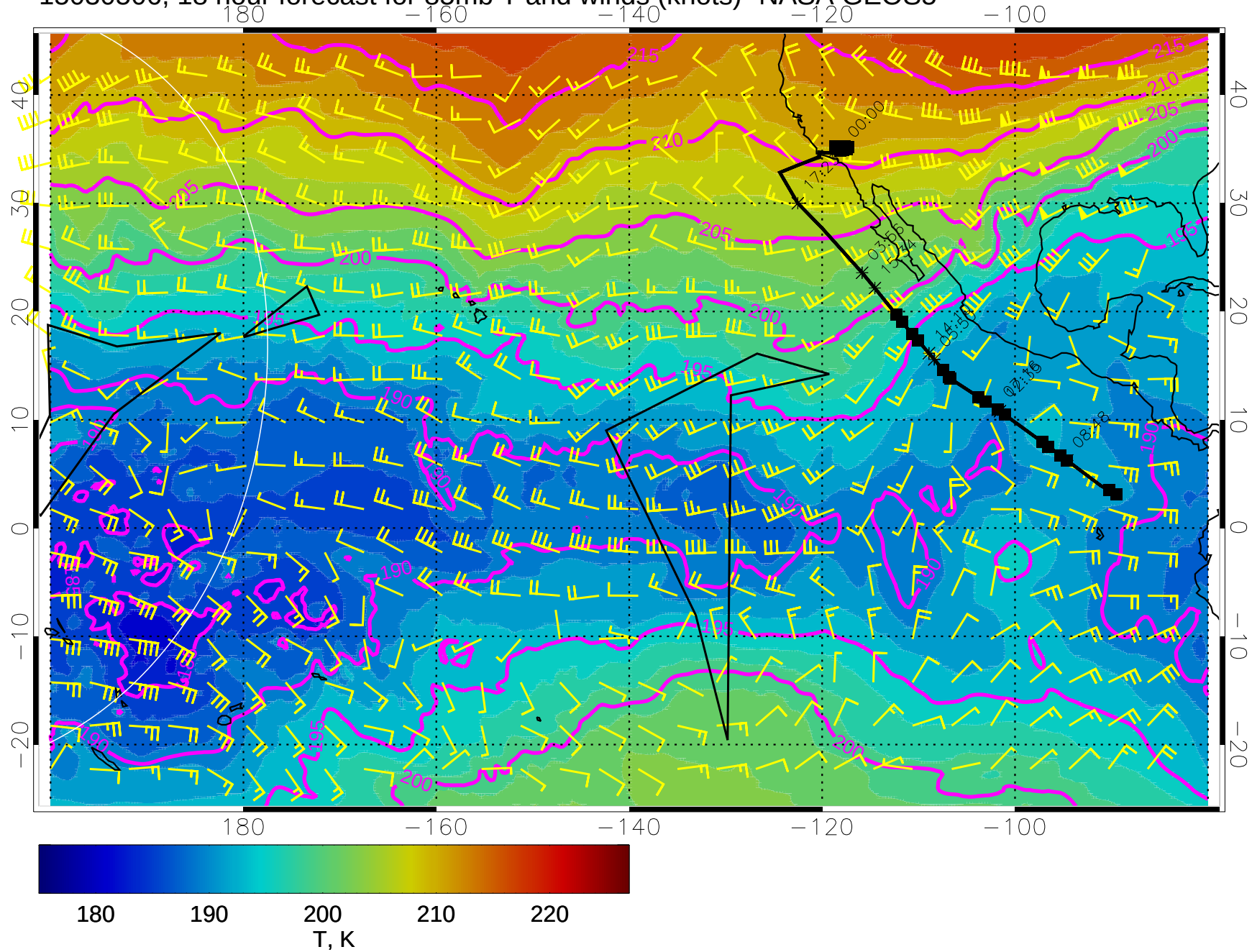
15030506, 18 hour forecast for 85mb T and winds (knots)- NASA GEOS5
