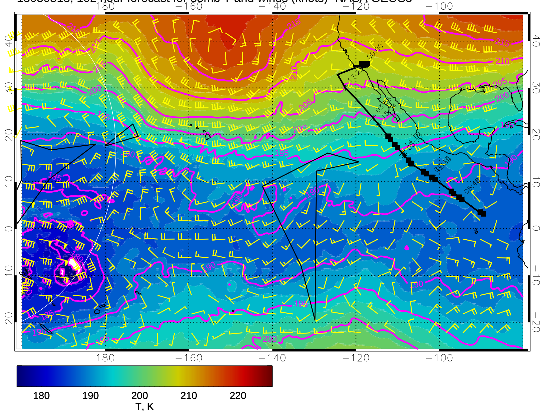
15030818, 102 hour forecast for 85mb T and winds (knots)- NASA GEOS5
