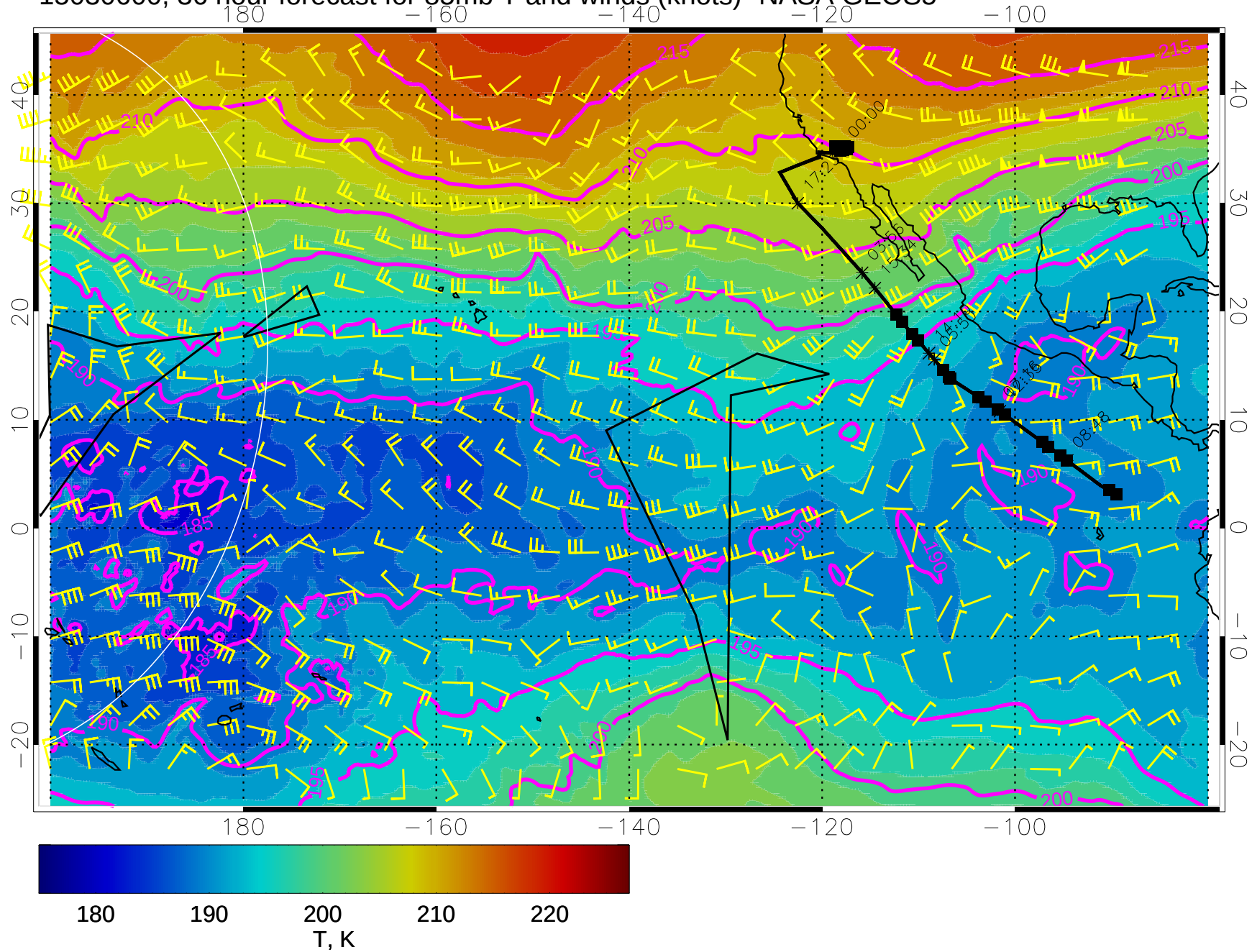
15030600, 36 hour forecast for 85mb T and winds (knots)- NASA GEOS5
