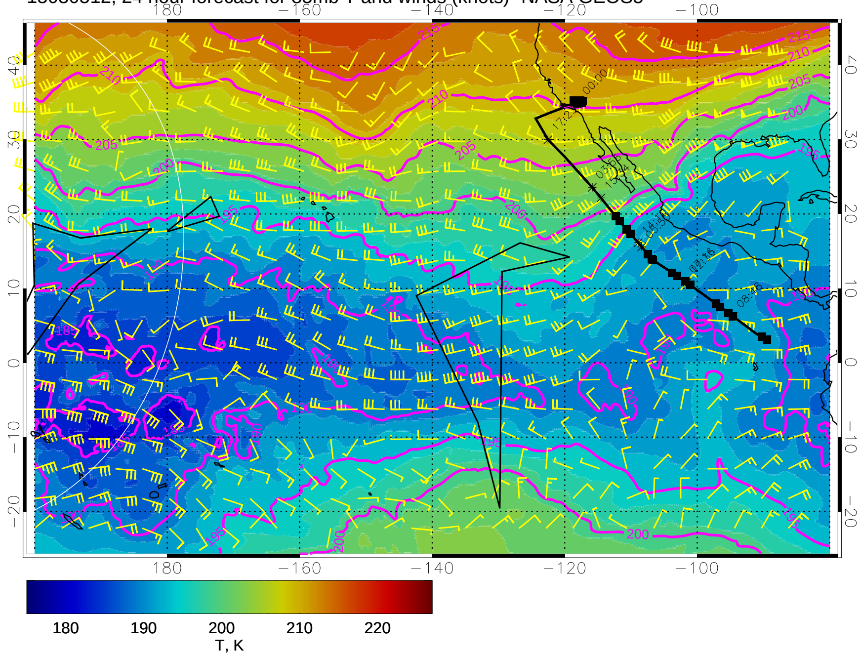
15030512, 24 hour forecast for 85mb T and winds (knots)- NASA GEOS5
