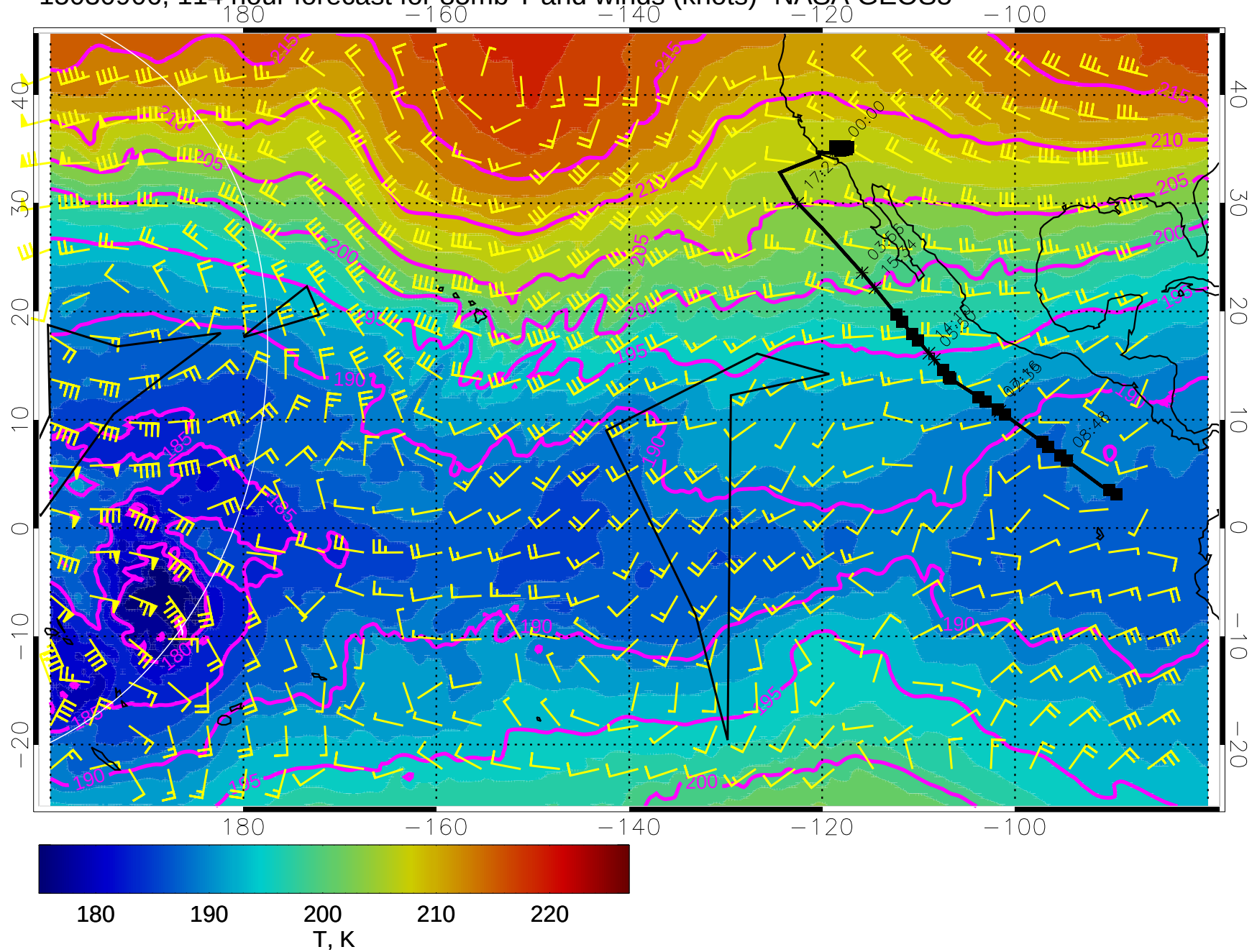
15030906, 114 hour forecast for 85mb T and winds (knots)- NASA GEOS5
