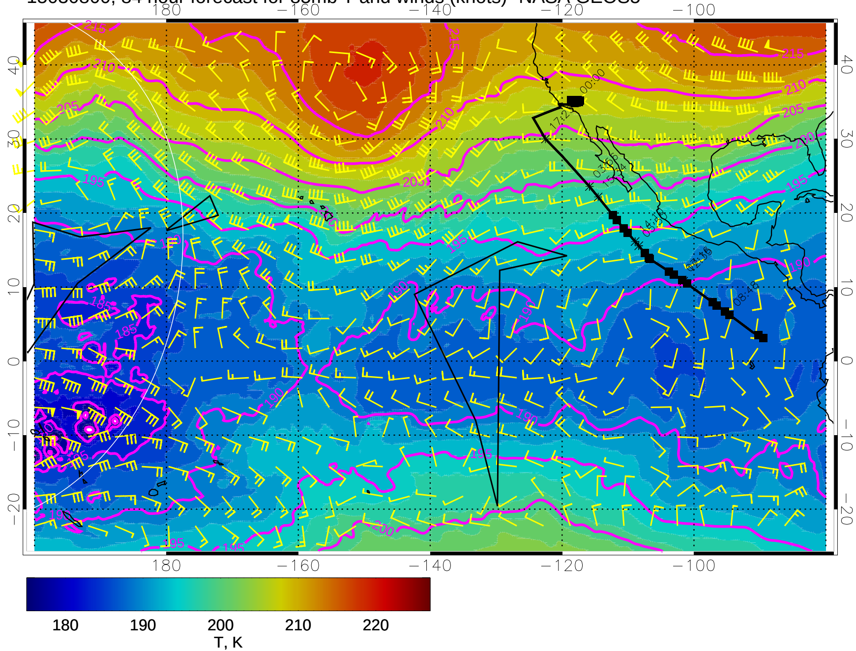
15030800, 84 hour forecast for 85mb T and winds (knots)- NASA GEOS5
