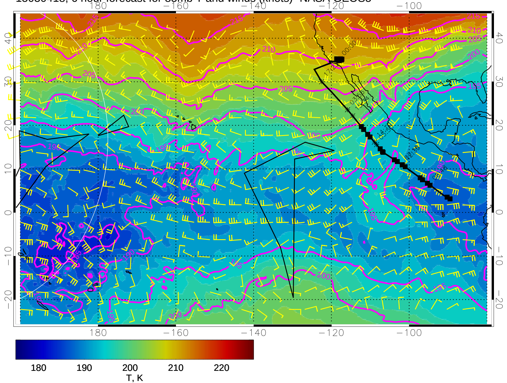
15030418, 6 hour forecast for 85mb T and winds (knots)- NASA GEOS5
