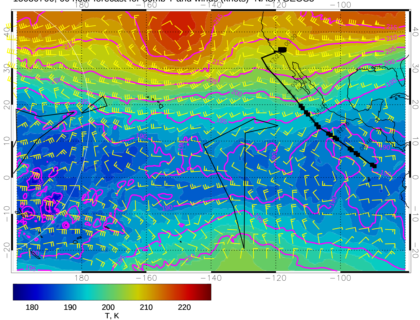
15030700, 60 hour forecast for 85mb T and winds (knots)- NASA GEOS5
