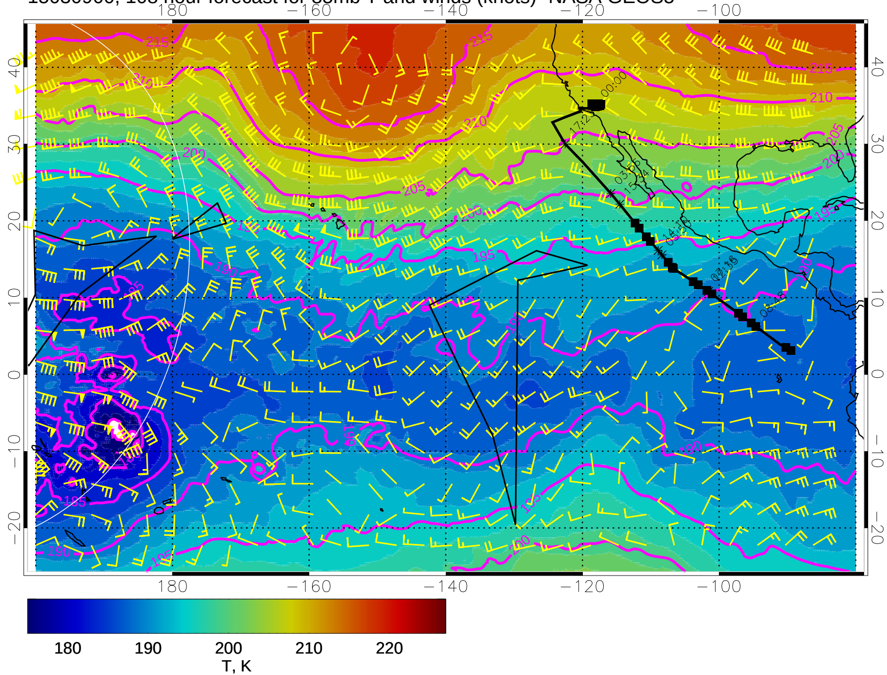
15030900, 108 hour forecast for 85mb T and winds (knots)- NASA GEOS5
