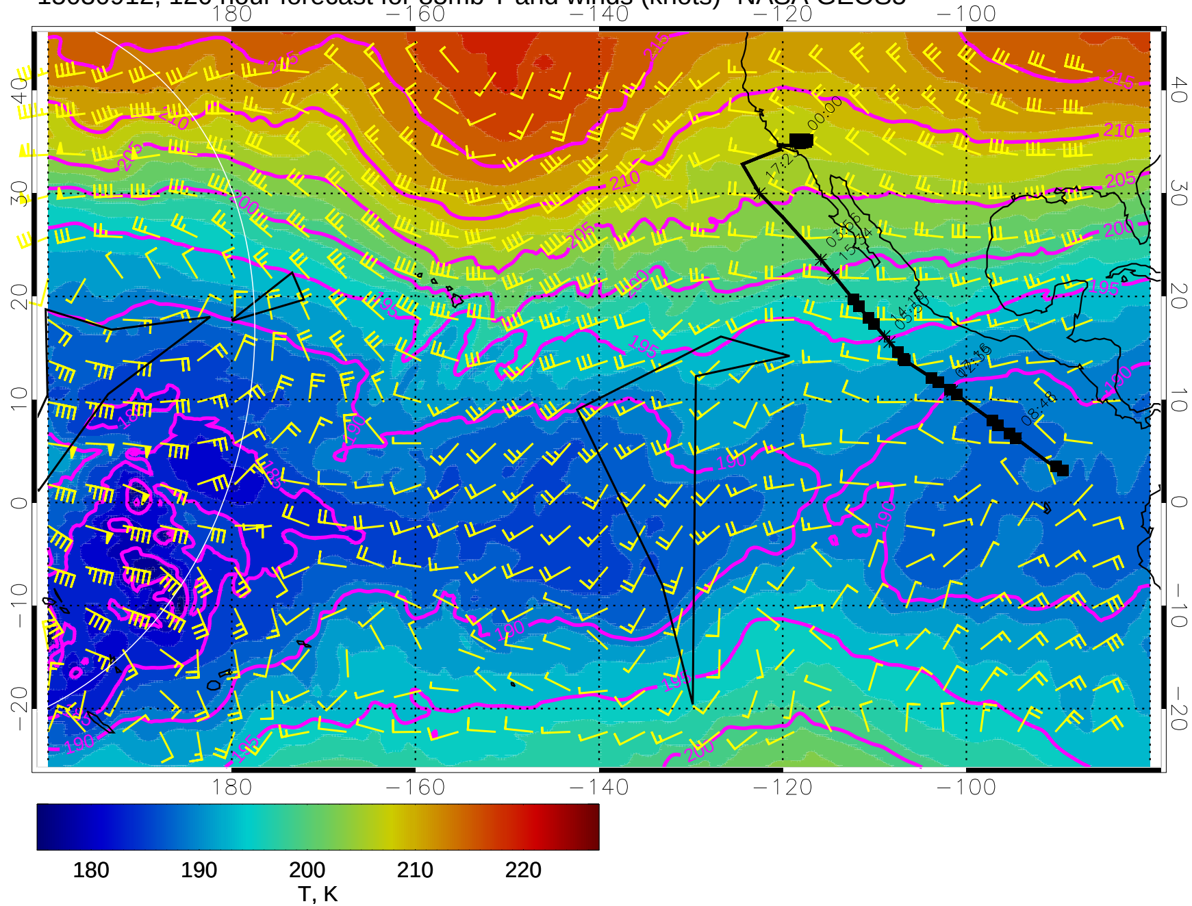
15030912, 120 hour forecast for 85mb T and winds (knots)- NASA GEOS5
