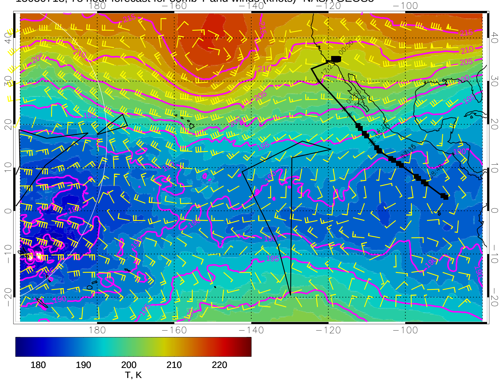
15030718, 78 hour forecast for 85mb T and winds (knots)- NASA GEOS5
