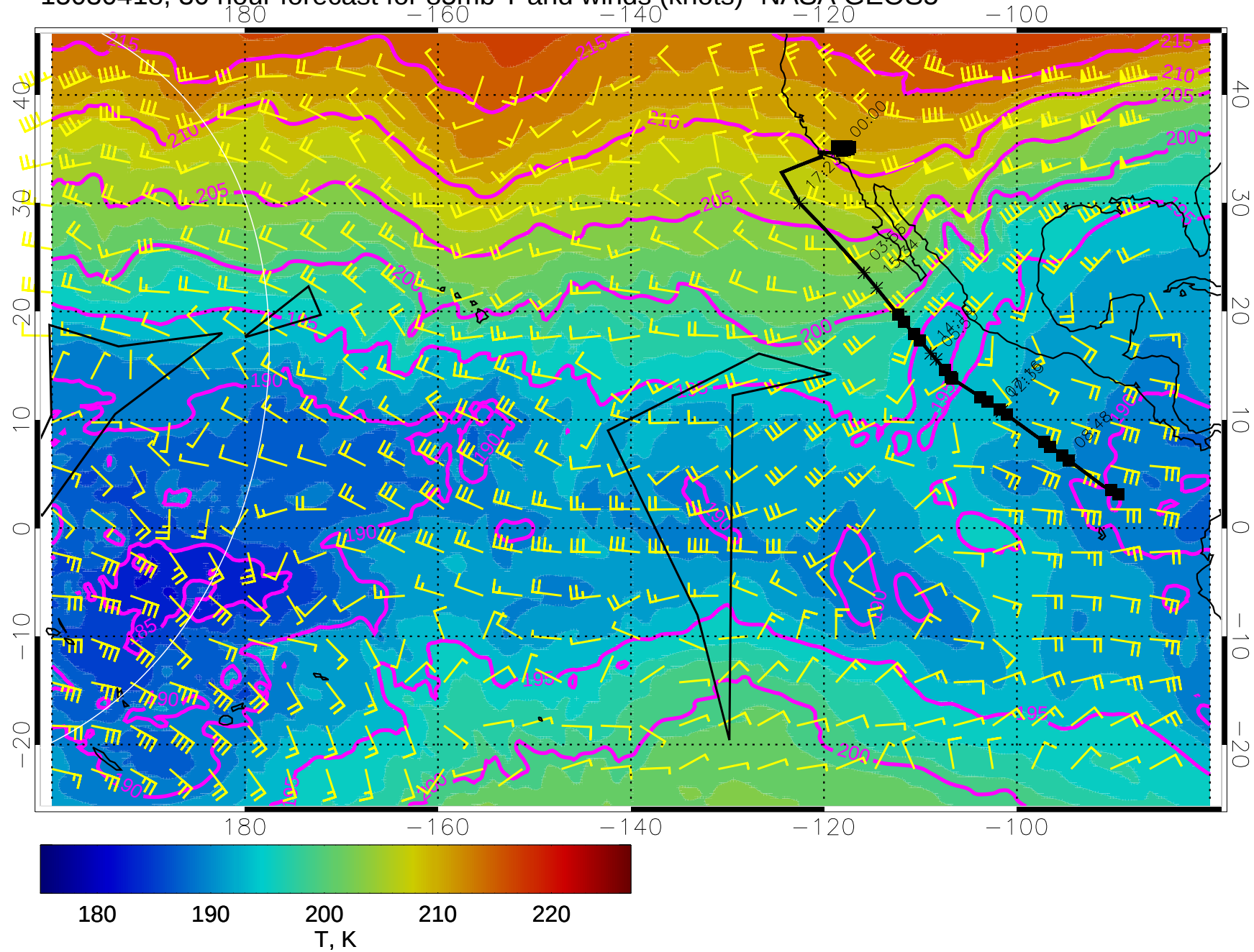
15030418, 30 hour forecast for 85mb T and winds (knots)- NASA GEOS5
