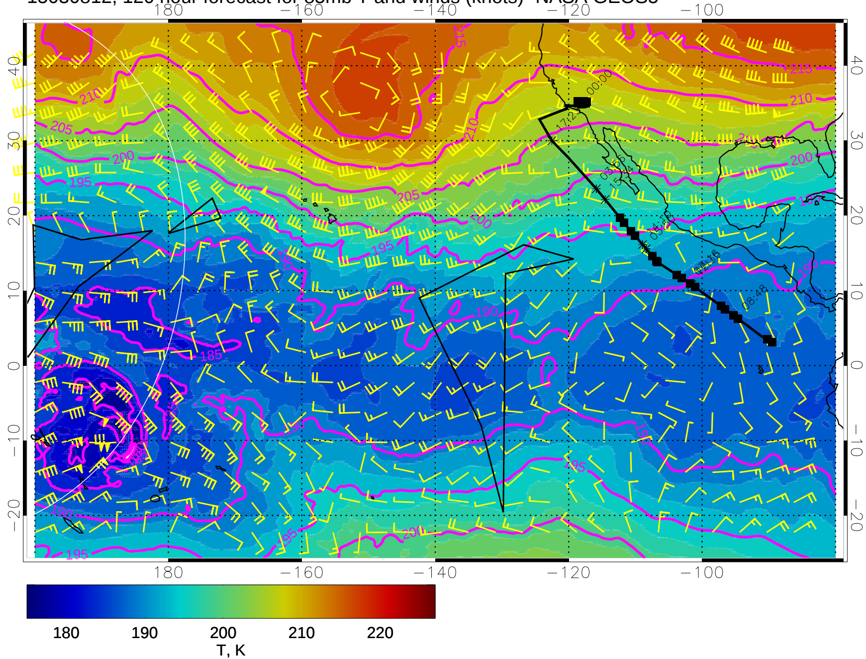
15030812, 120 hour forecast for 85mb T and winds (knots)- NASA GEOS5
