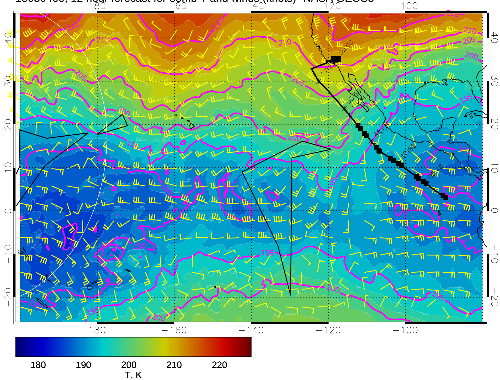
15030400, 12 hour forecast for 85mb T and winds (knots)- NASA GEOS5
