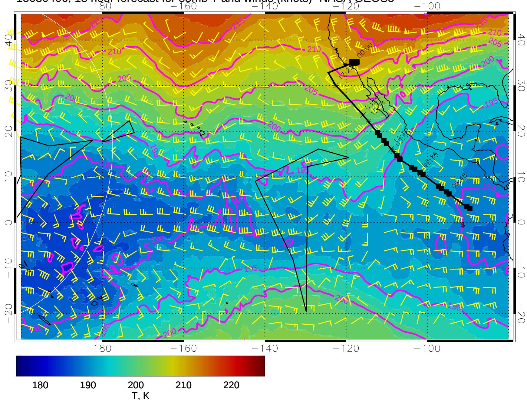
15030406, 18 hour forecast for 85mb T and winds (knots)- NASA GEOS5
