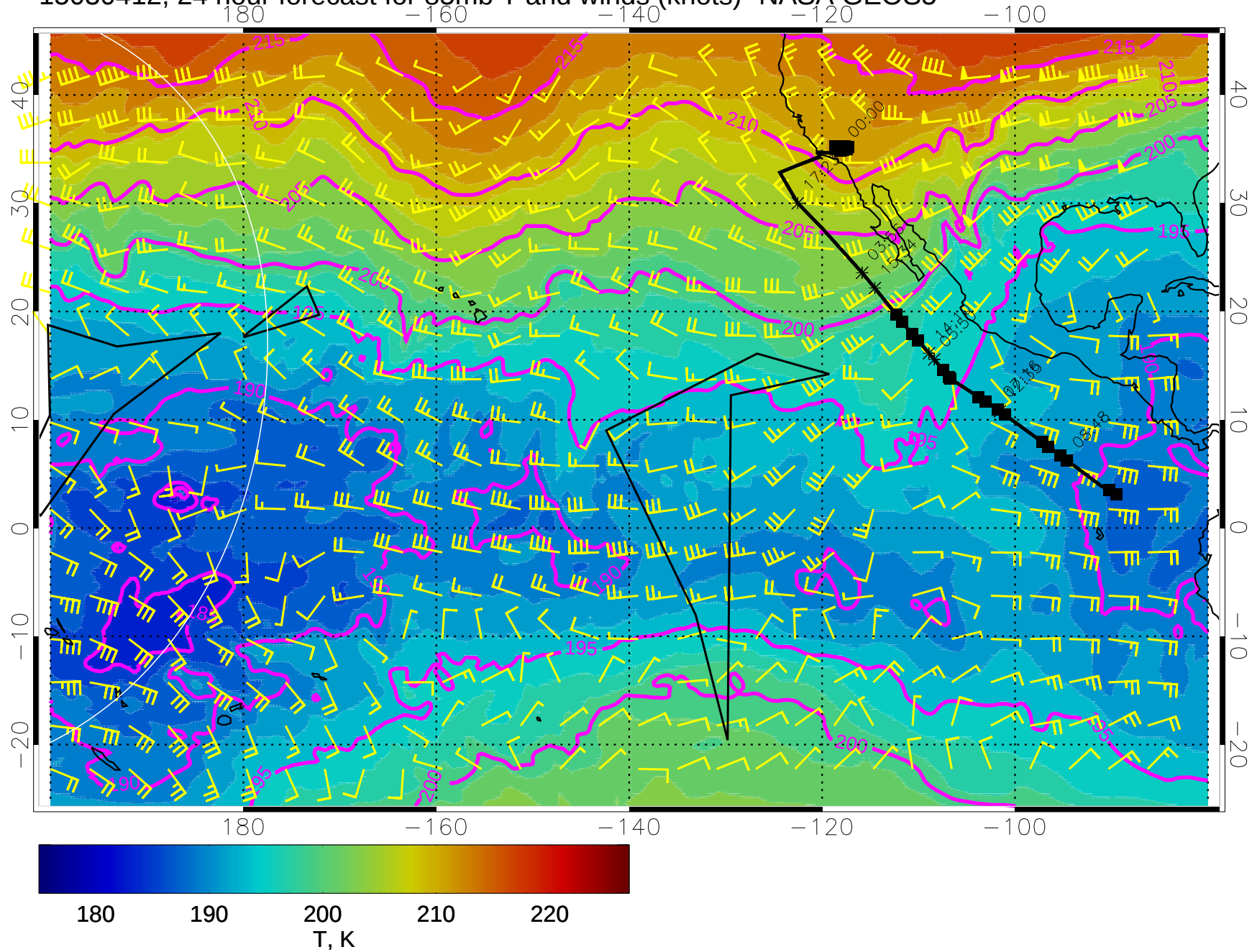
15030412, 24 hour forecast for 85mb T and winds (knots)- NASA GEOS5
