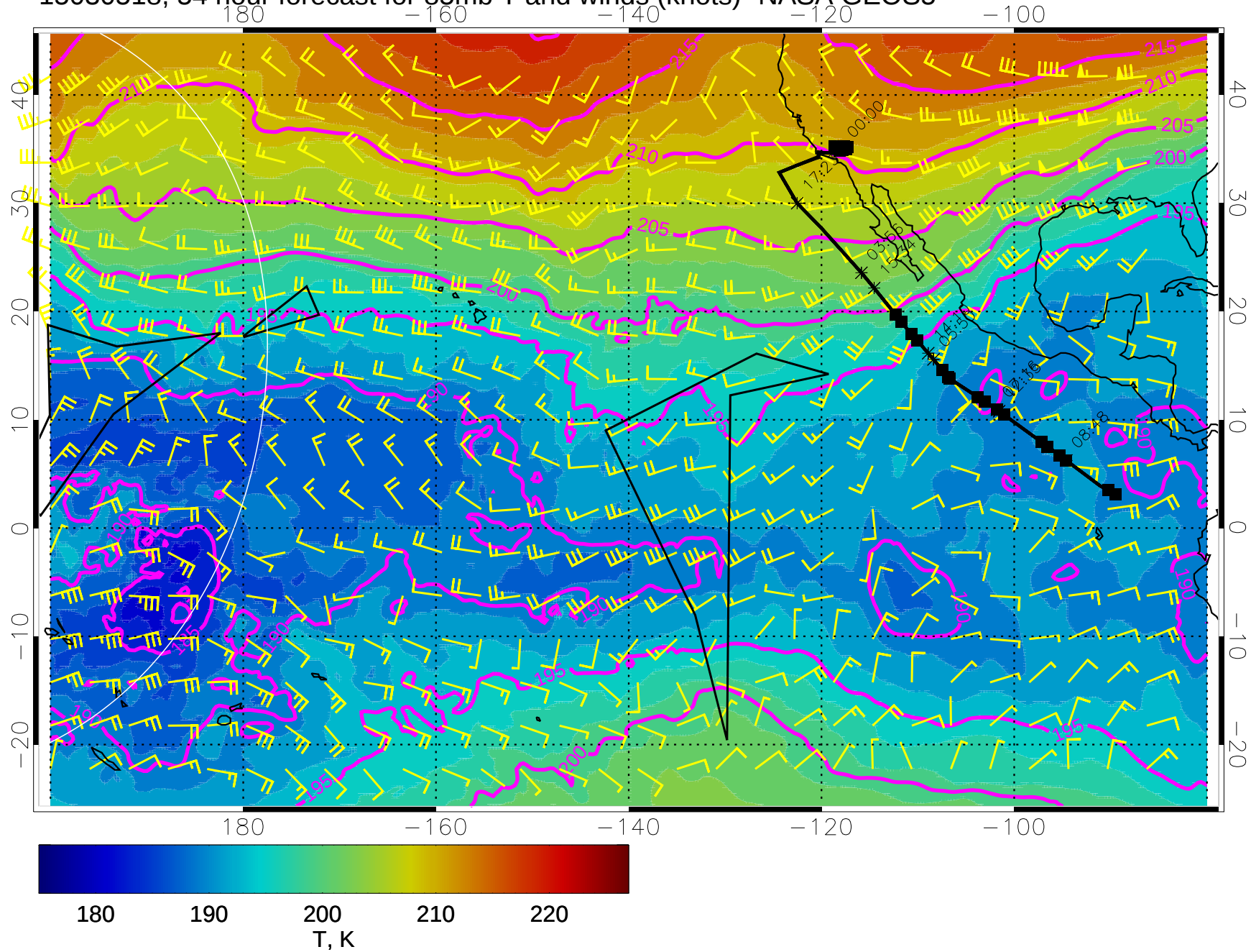
15030518, 54 hour forecast for 85mb T and winds (knots)- NASA GEOS5
