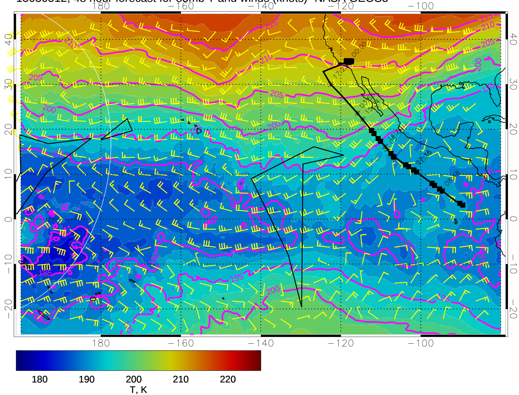
15030512, 48 hour forecast for 85mb T and winds (knots)- NASA GEOS5
