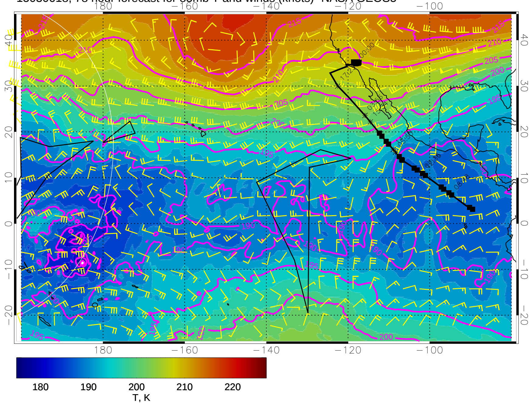
15030618, 78 hour forecast for 85mb T and winds (knots)- NASA GEOS5
