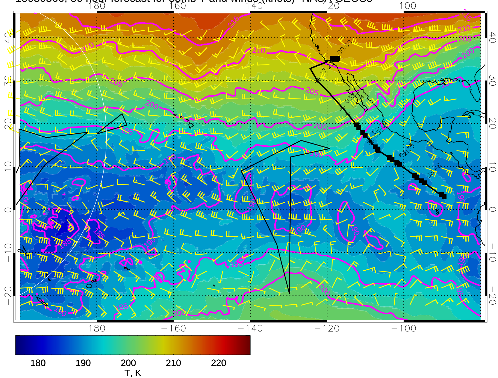
15030500, 36 hour forecast for 85mb T and winds (knots)- NASA GEOS5
