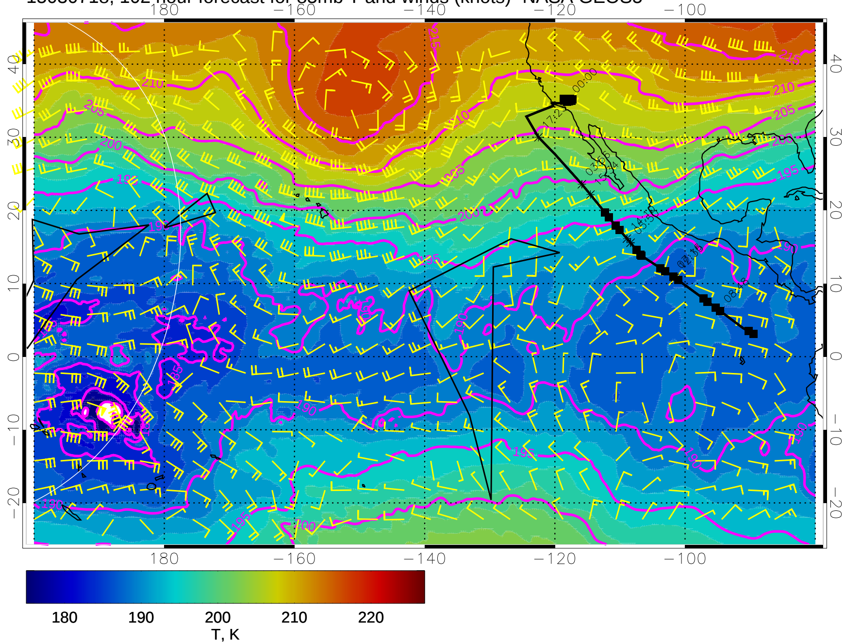
15030718, 102 hour forecast for 85mb T and winds (knots)- NASA GEOS5
