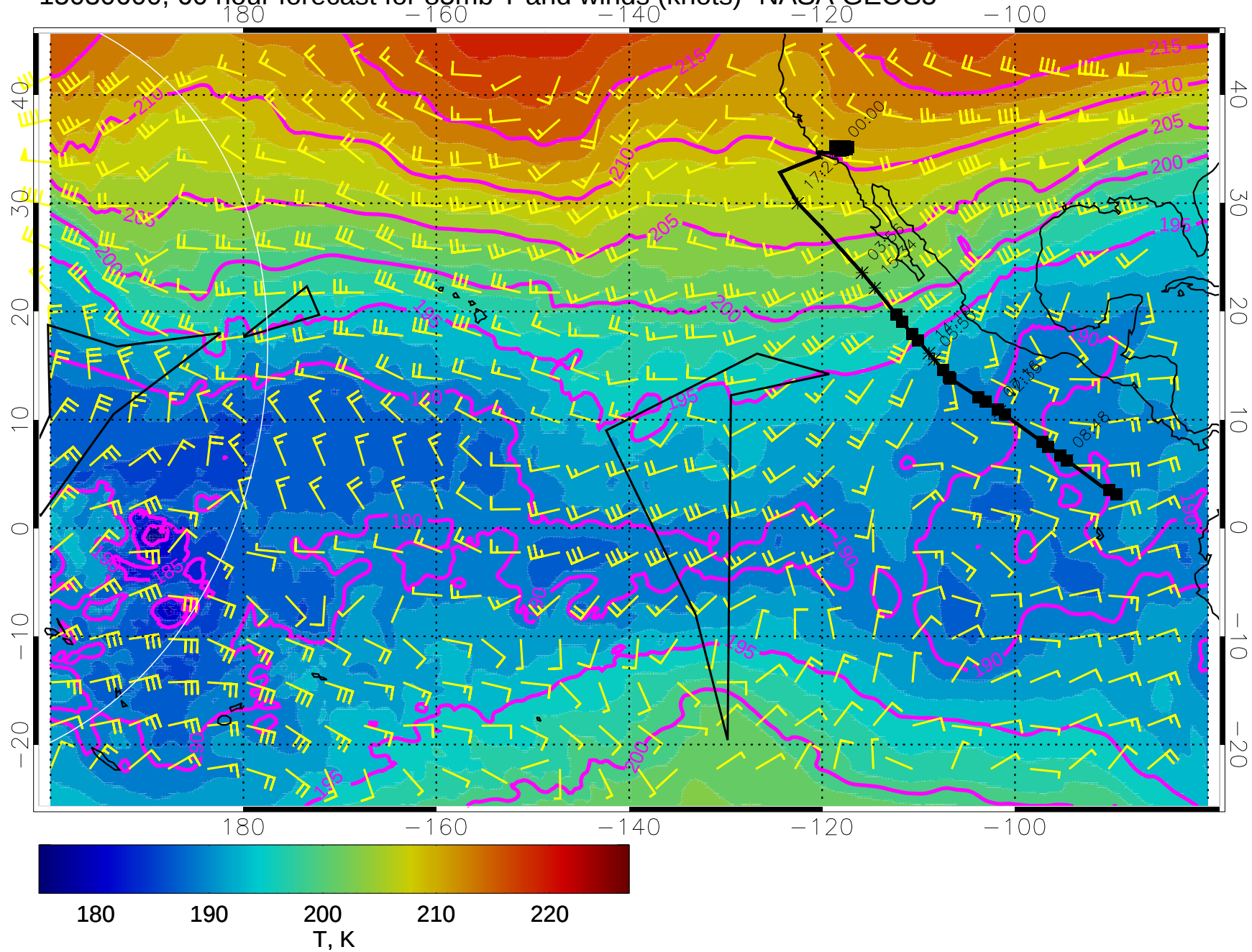
15030600, 60 hour forecast for 85mb T and winds (knots)- NASA GEOS5
