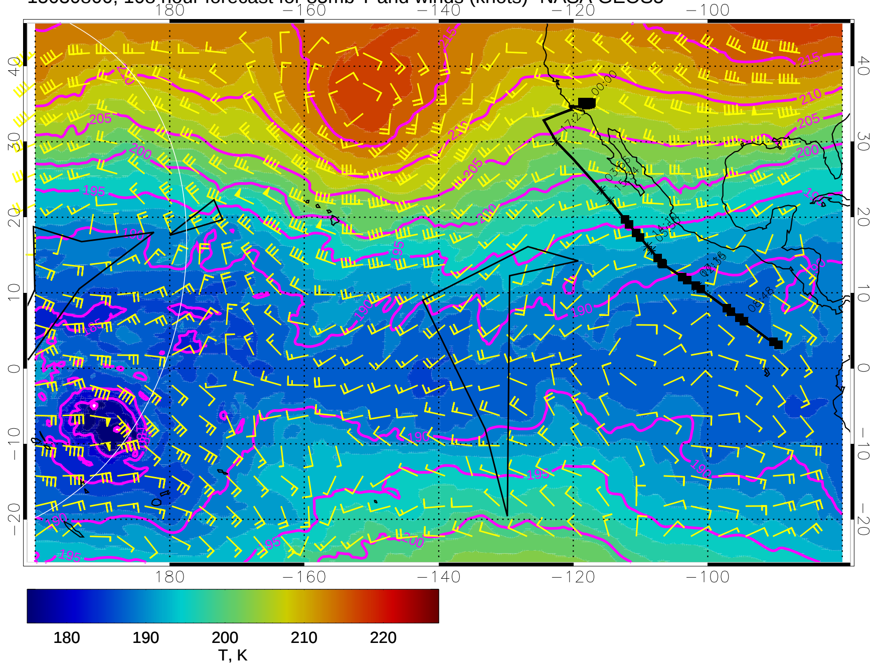
15030800, 108 hour forecast for 85mb T and winds (knots)- NASA GEOS5
