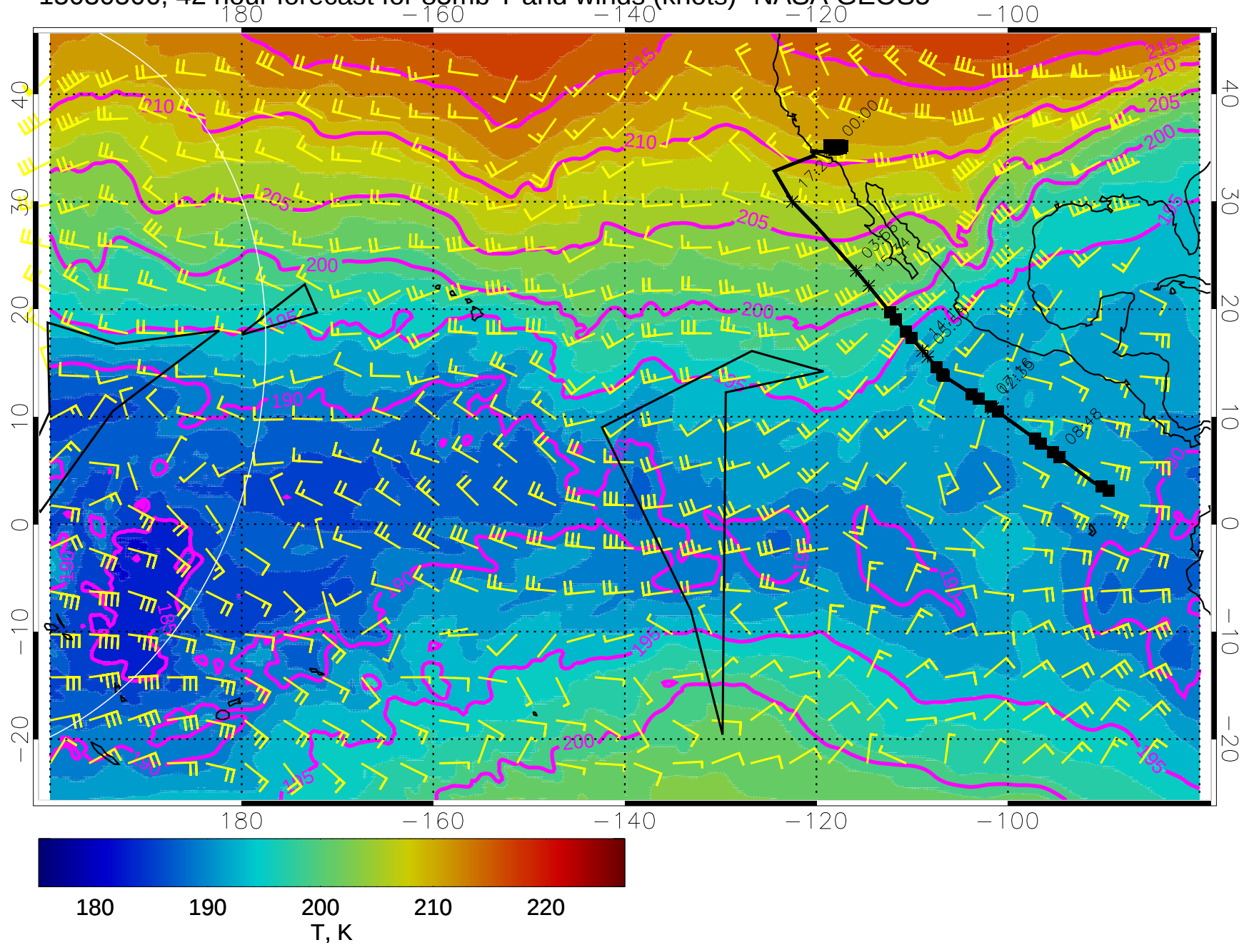
15030506, 42 hour forecast for 85mb T and winds (knots)- NASA GEOS5
