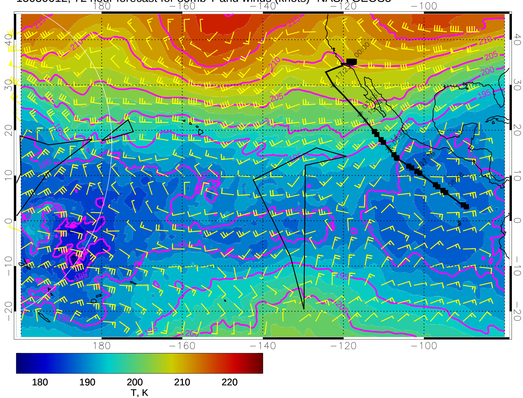
15030612, 72 hour forecast for 85mb T and winds (knots)- NASA GEOS5
