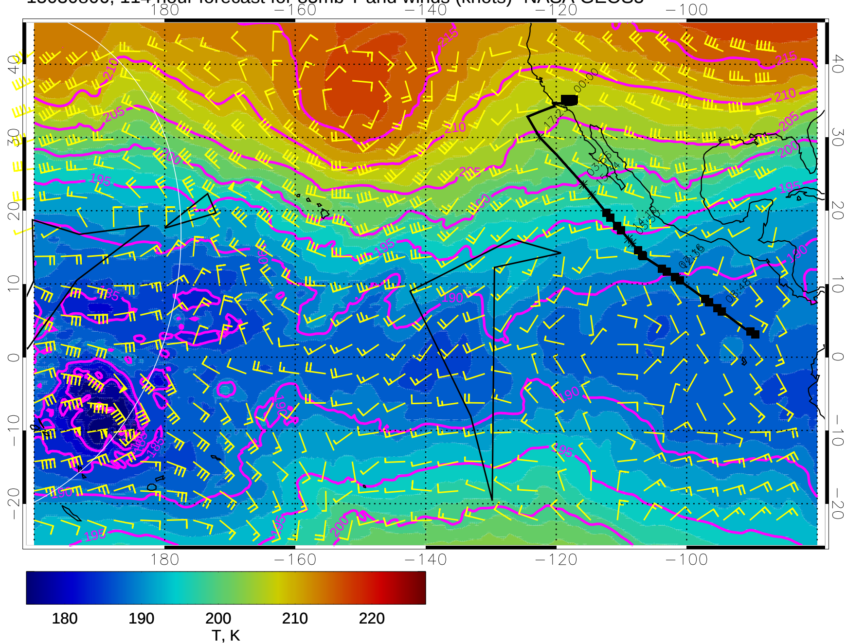
15030806, 114 hour forecast for 85mb T and winds (knots)- NASA GEOS5
