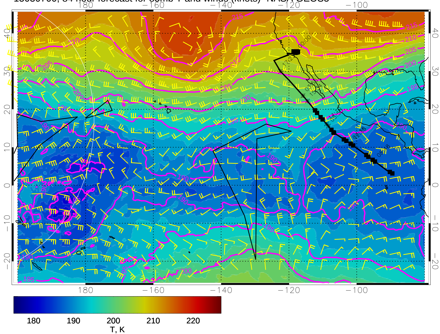
15030700, 84 hour forecast for 85mb T and winds (knots)- NASA GEOS5
