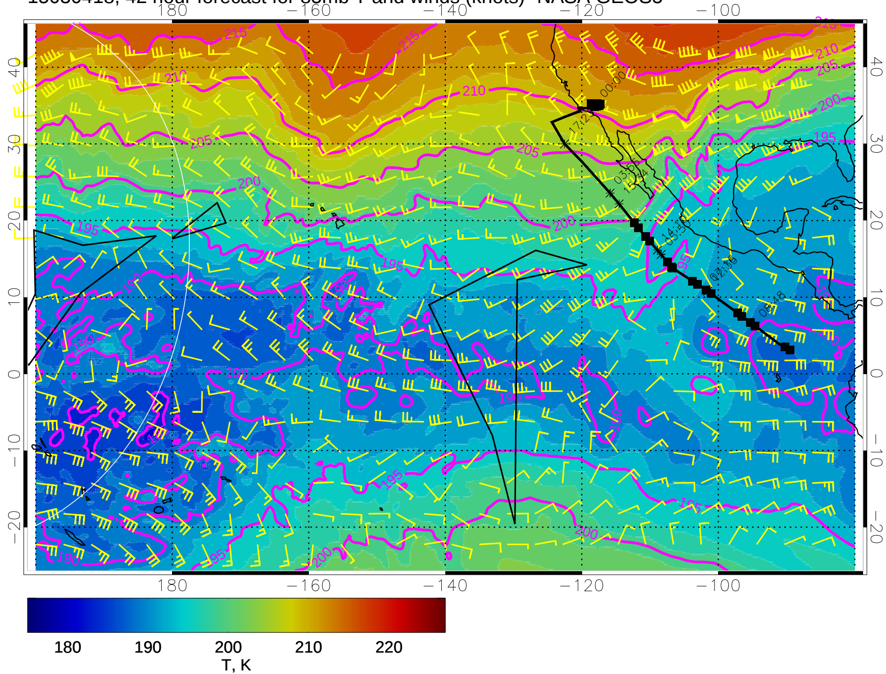
15030418, 42 hour forecast for 85mb T and winds (knots)- NASA GEOS5
