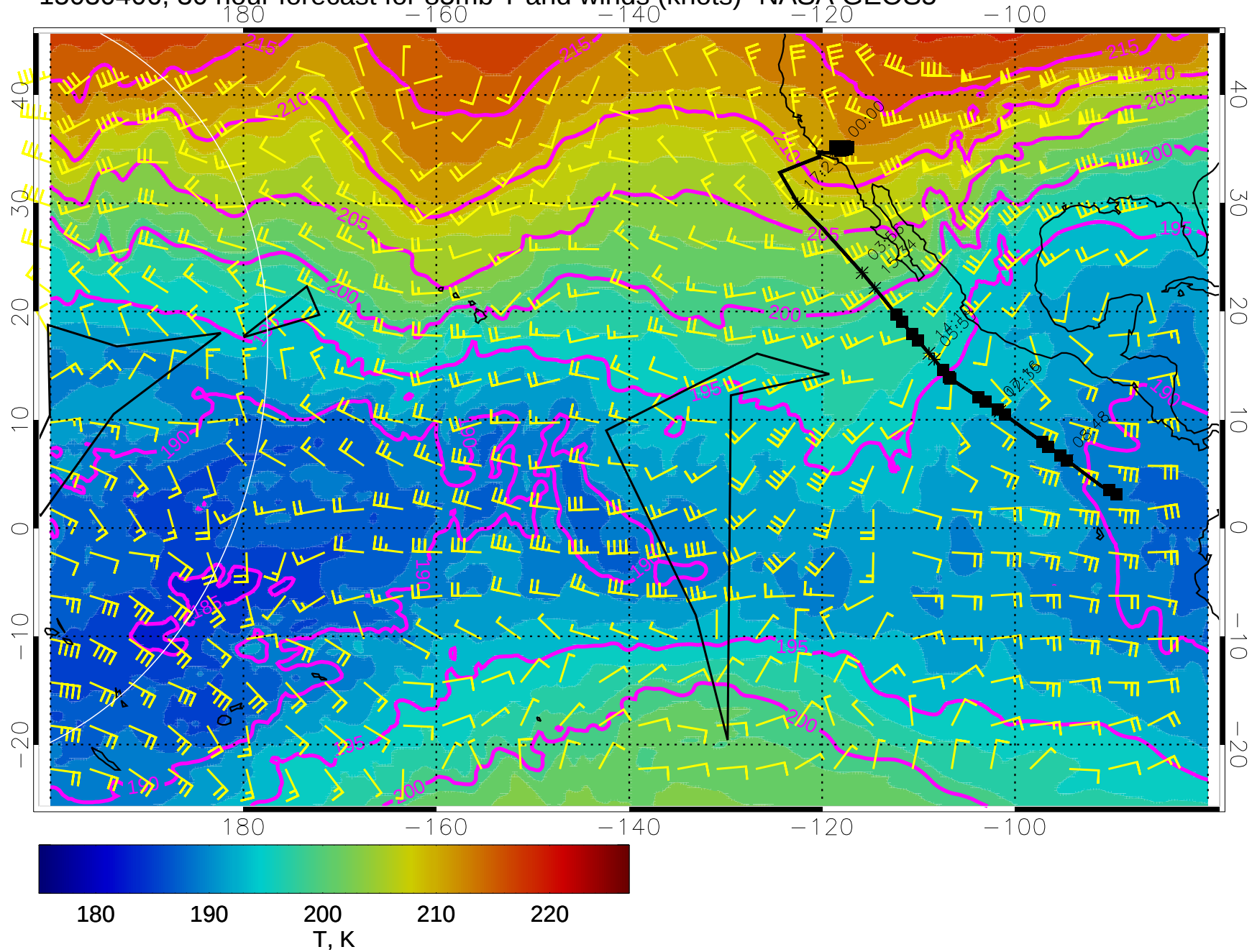
15030406, 30 hour forecast for 85mb T and winds (knots)- NASA GEOS5
