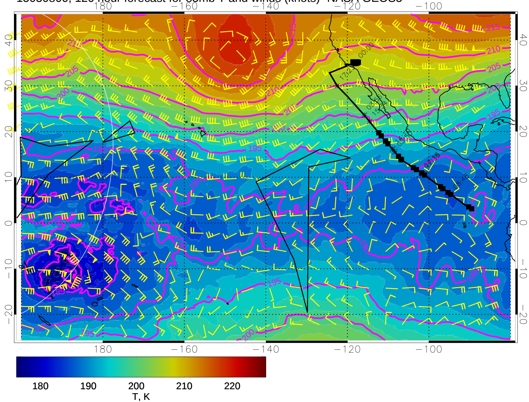
15030800, 120 hour forecast for 85mb T and winds (knots)- NASA GEOS5
