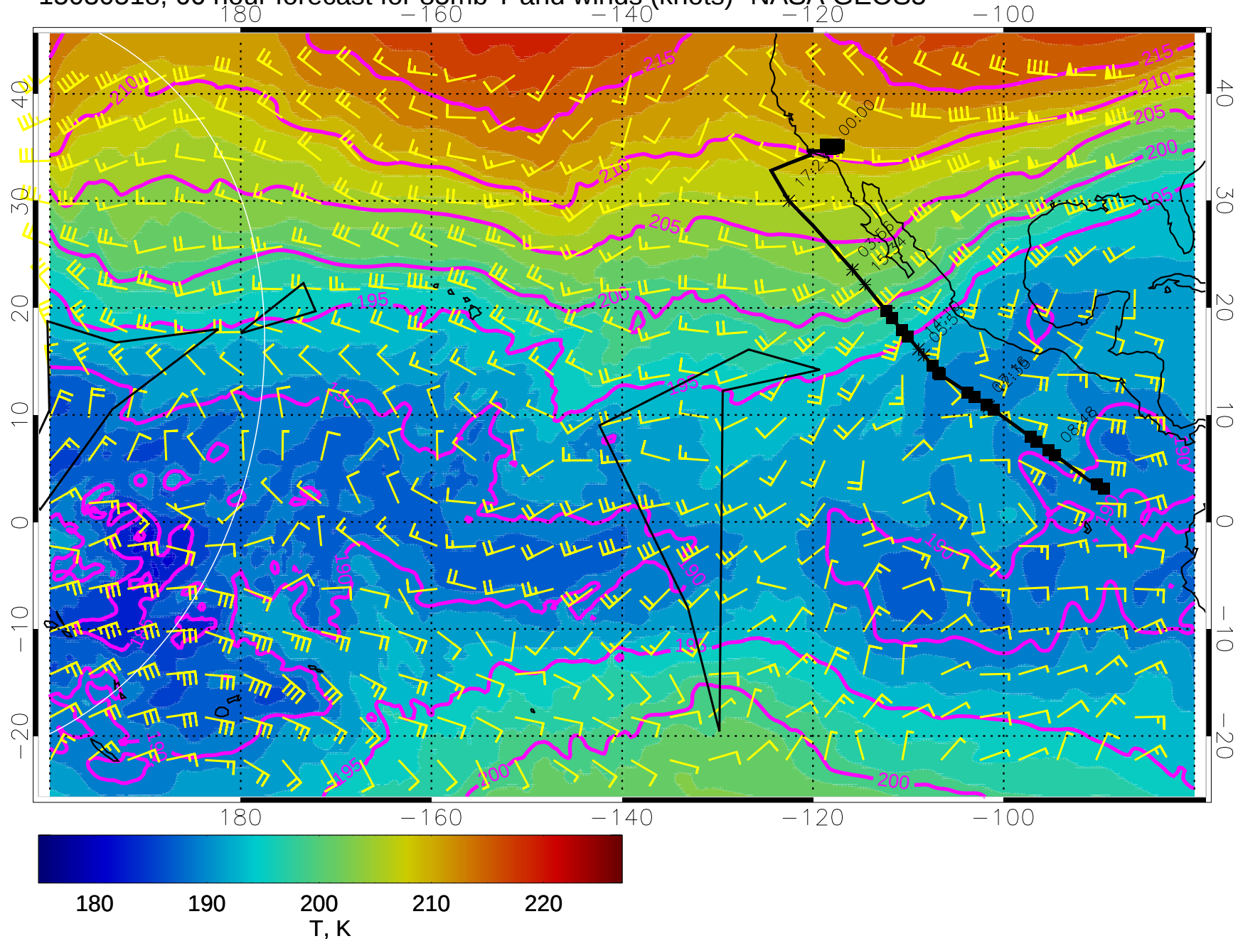
15030518, 66 hour forecast for 85mb T and winds (knots)- NASA GEOS5
