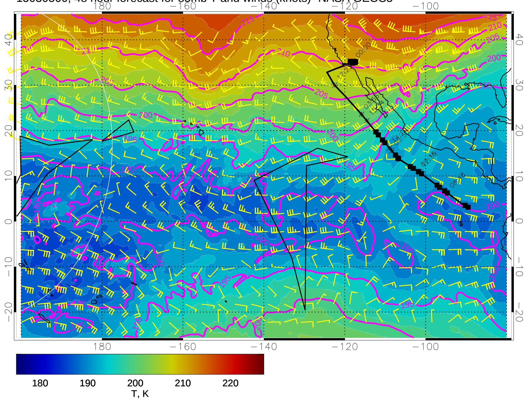
15030500, 48 hour forecast for 85mb T and winds (knots)- NASA GEOS5
