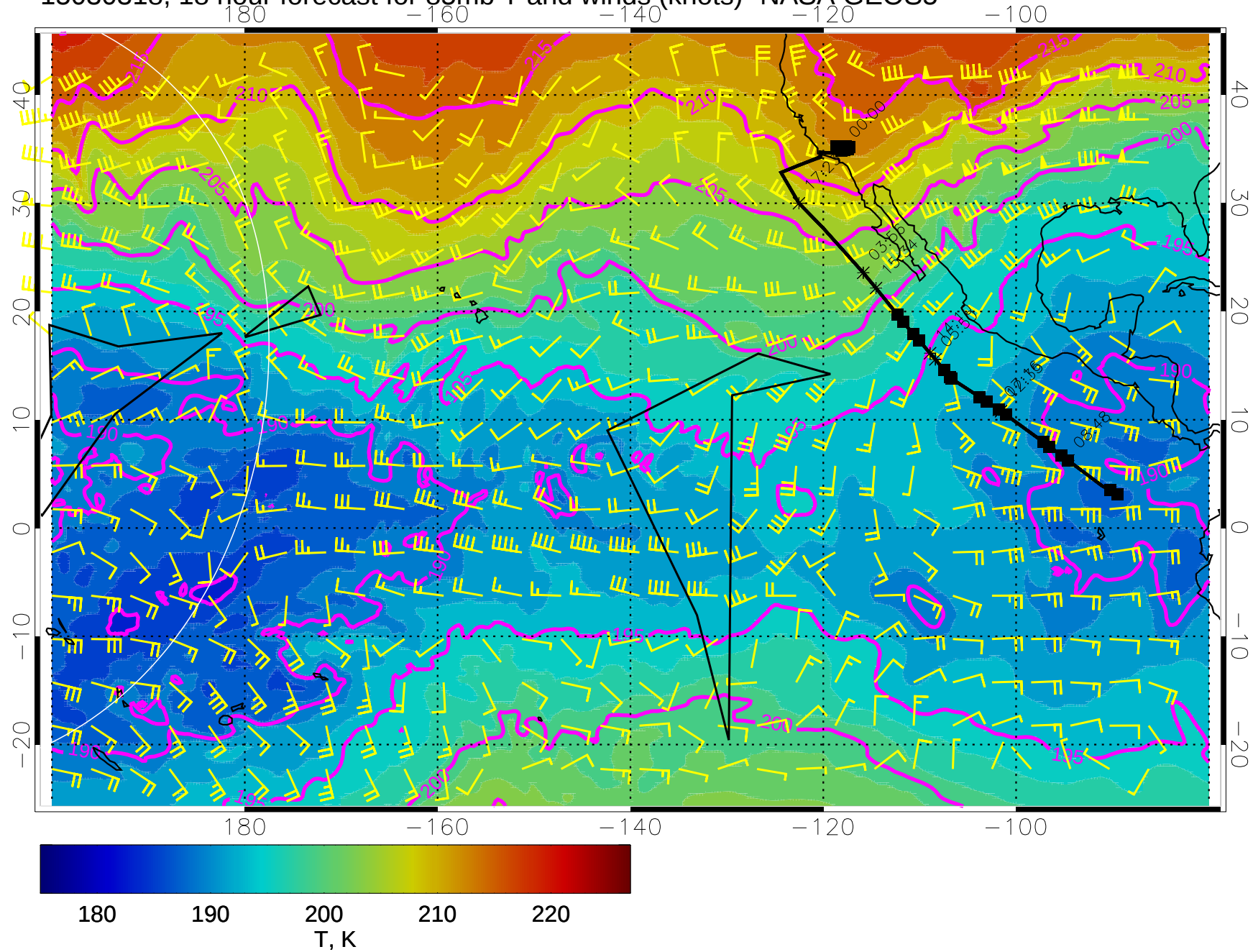
15030318, 18 hour forecast for 85mb T and winds (knots)- NASA GEOS5
