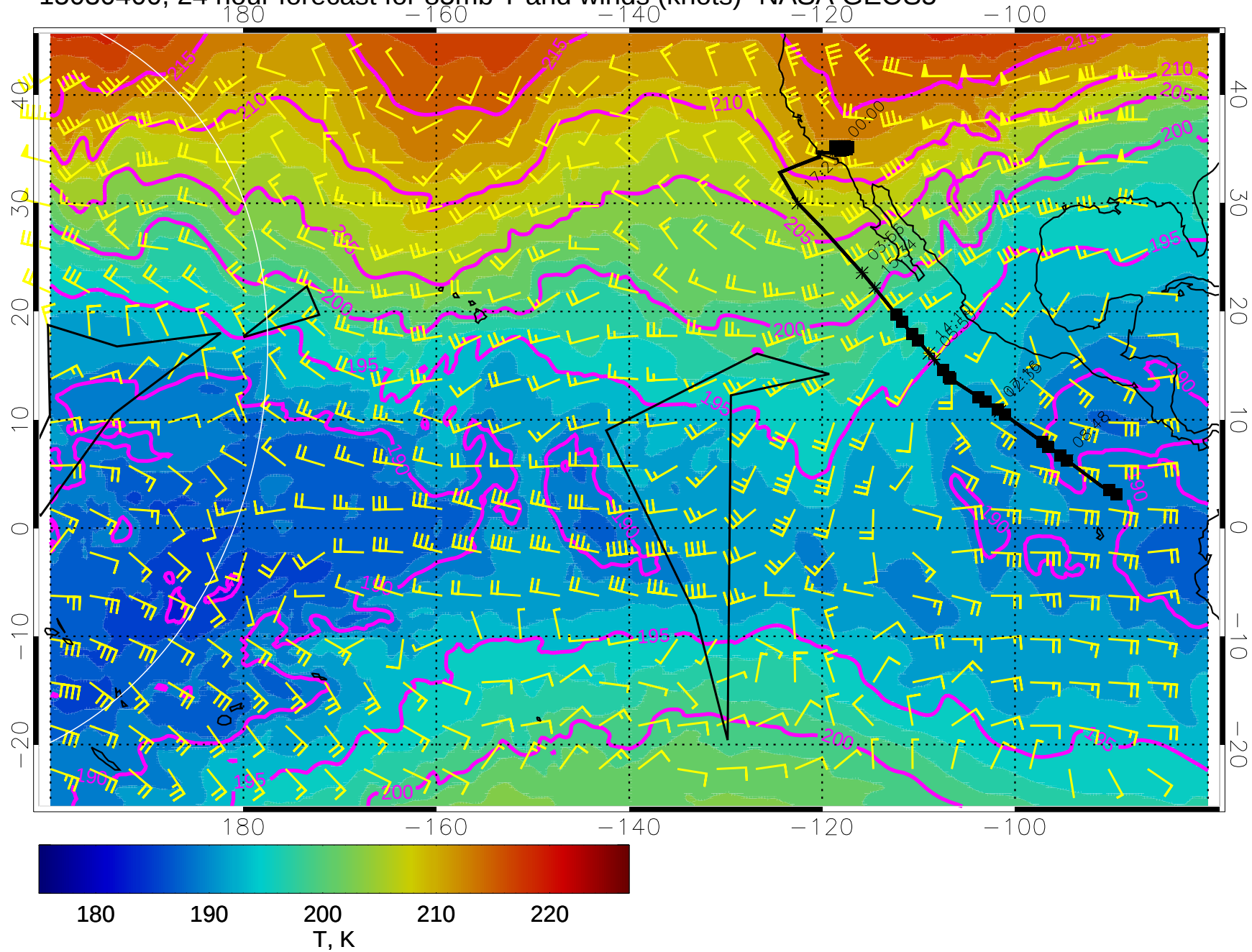
15030400, 24 hour forecast for 85mb T and winds (knots)- NASA GEOS5
