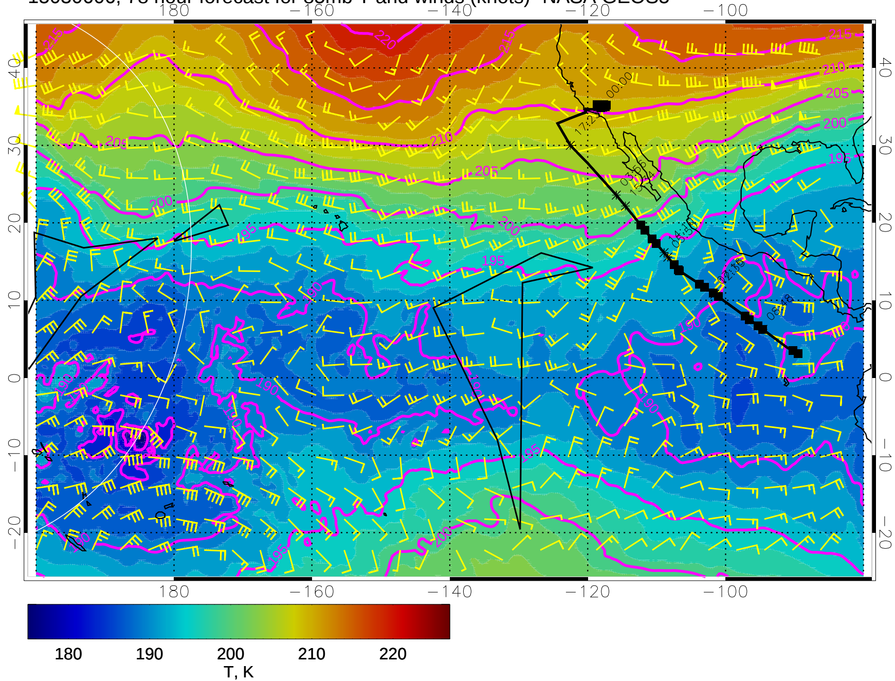
15030606, 78 hour forecast for 85mb T and winds (knots)- NASA GEOS5
