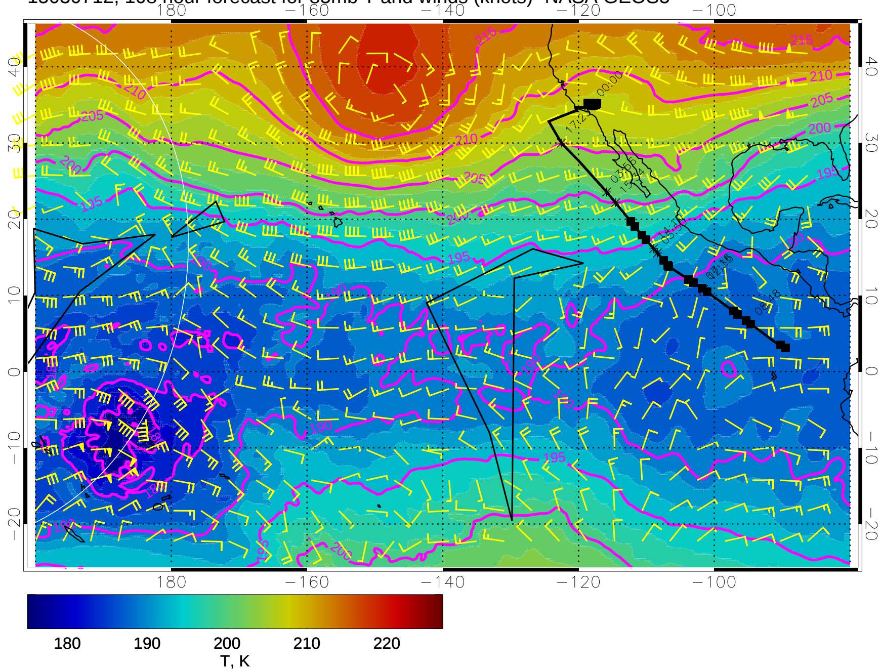
15030712, 108 hour forecast for 85mb T and winds (knots)- NASA GEOS5
