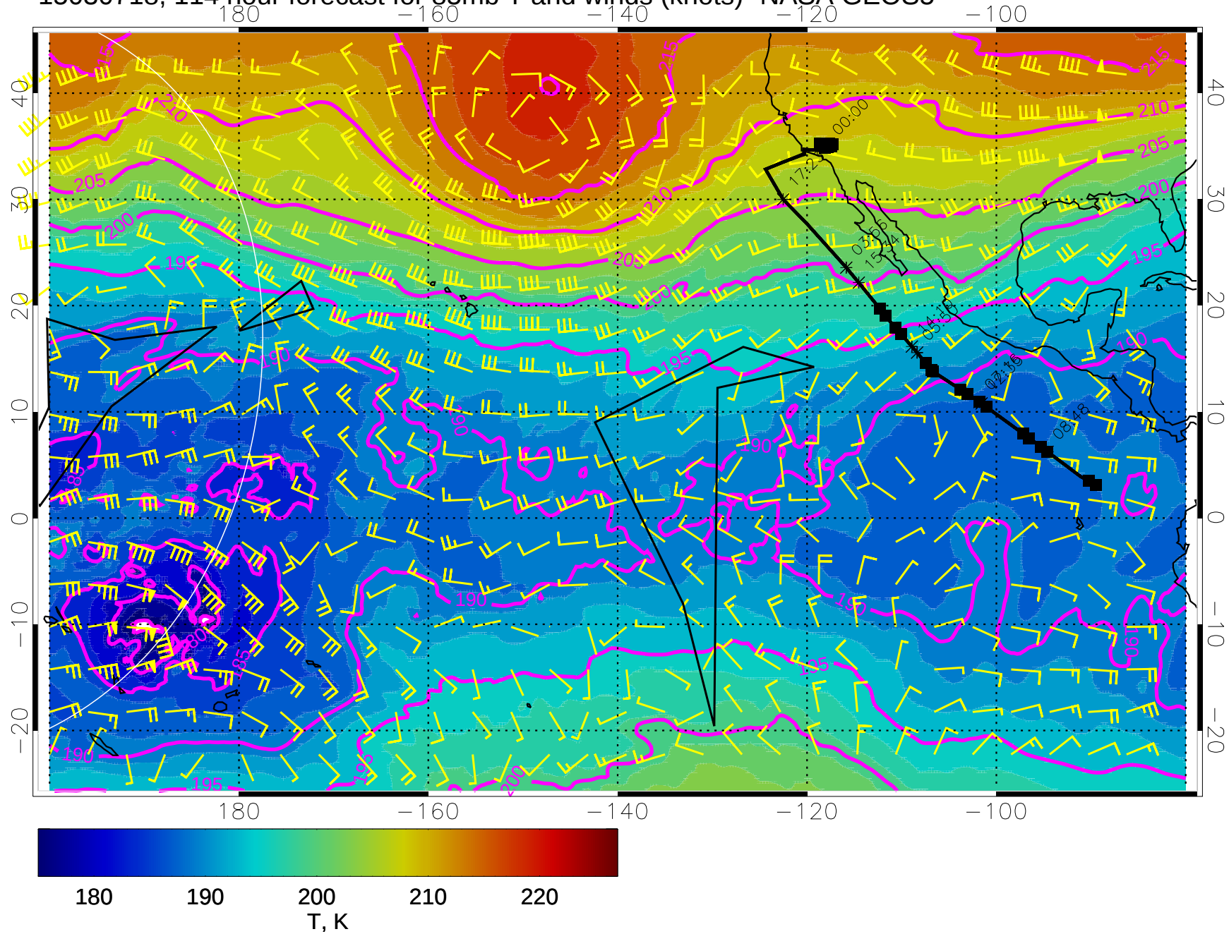
15030718, 114 hour forecast for 85mb T and winds (knots)- NASA GEOS5
