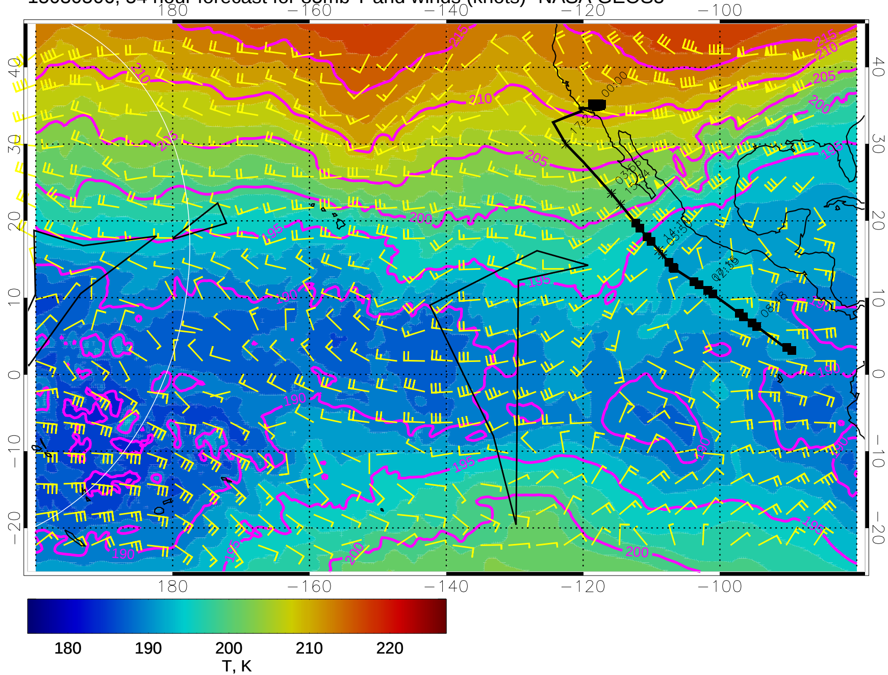
15030506, 54 hour forecast for 85mb T and winds (knots)- NASA GEOS5
