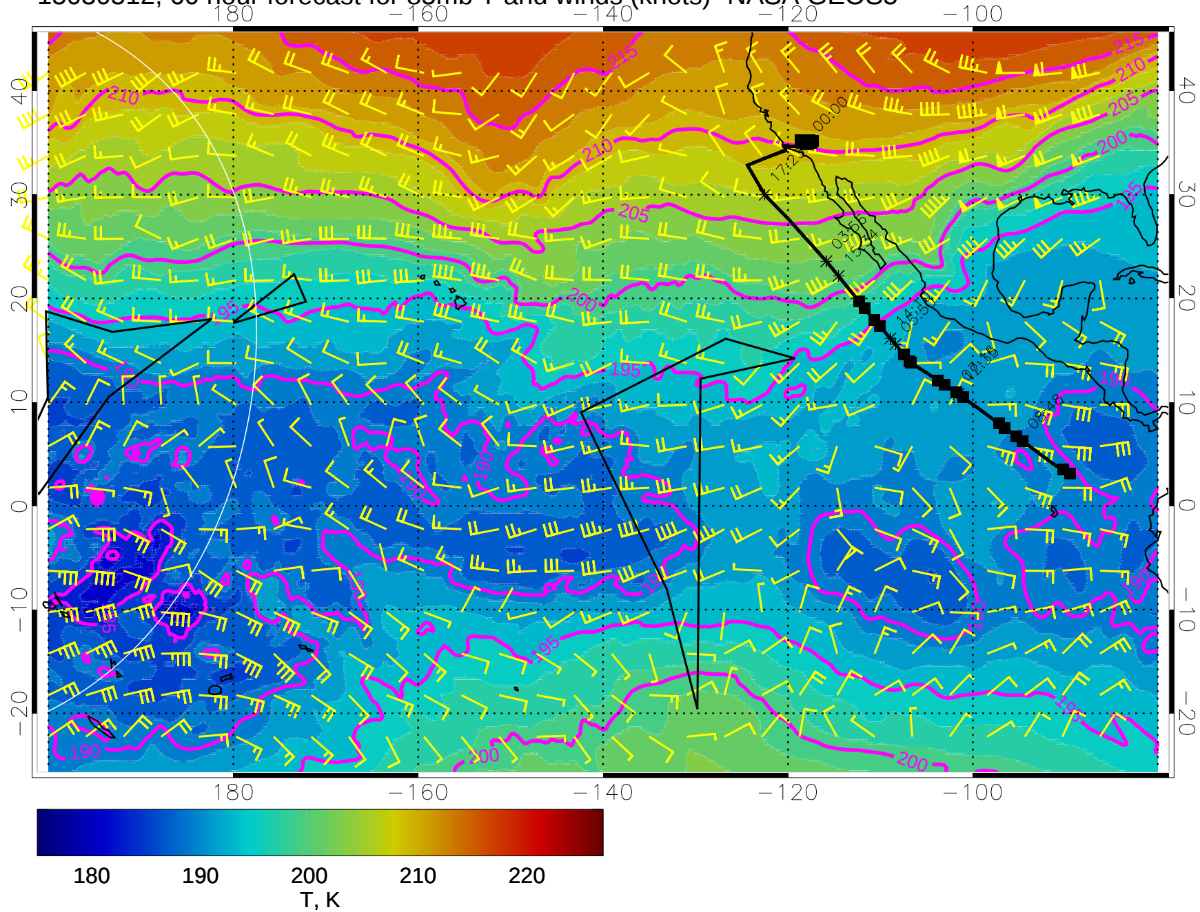
15030512, 60 hour forecast for 85mb T and winds (knots)- NASA GEOS5
