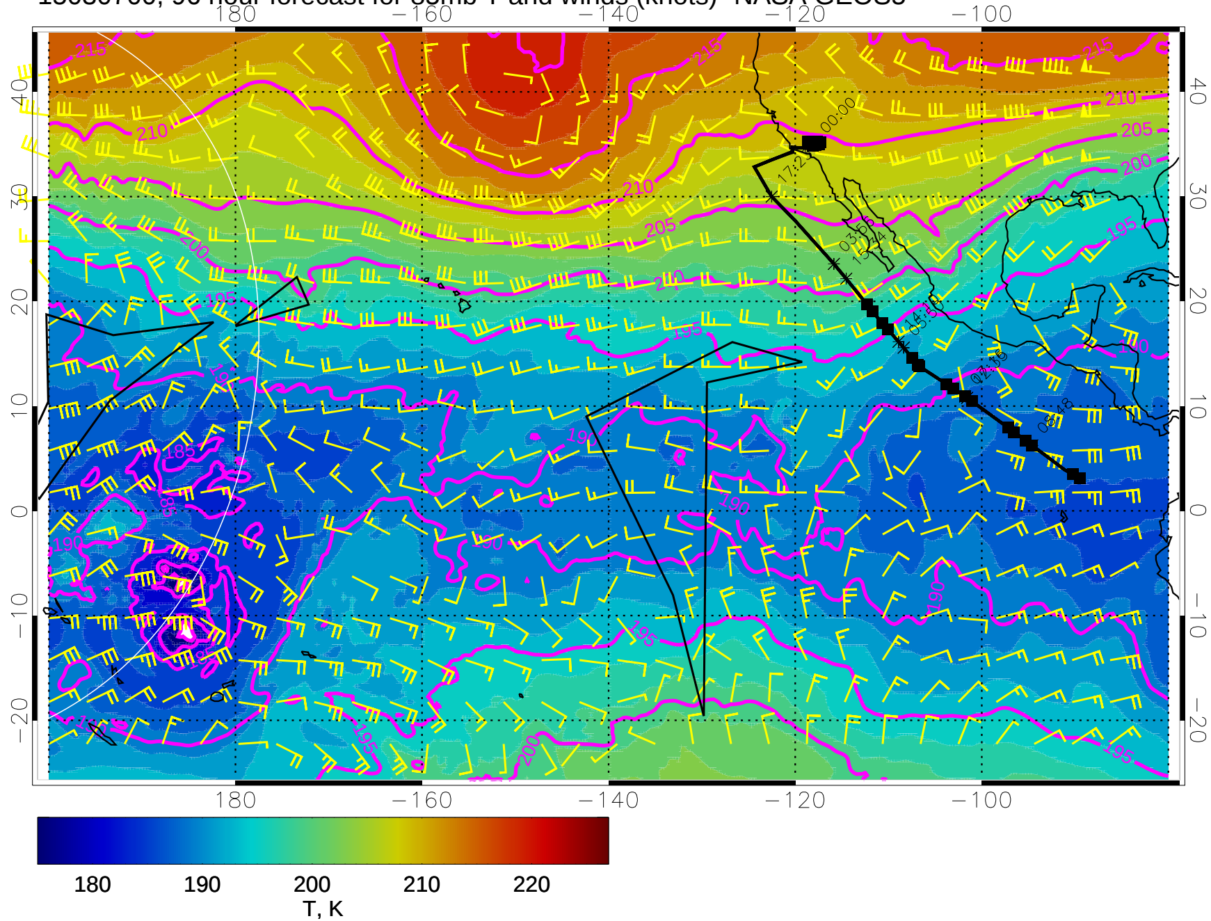
15030700, 96 hour forecast for 85mb T and winds (knots)- NASA GEOS5
