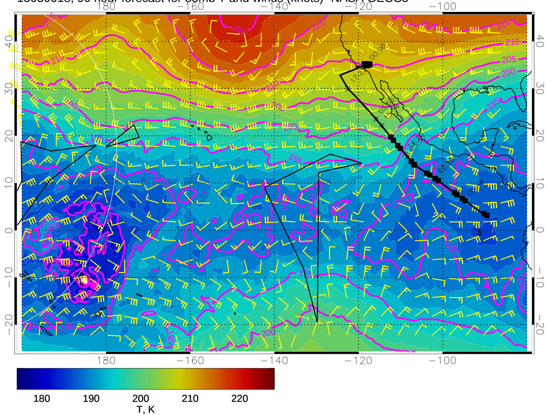
15030618, 90 hour forecast for 85mb T and winds (knots)- NASA GEOS5
