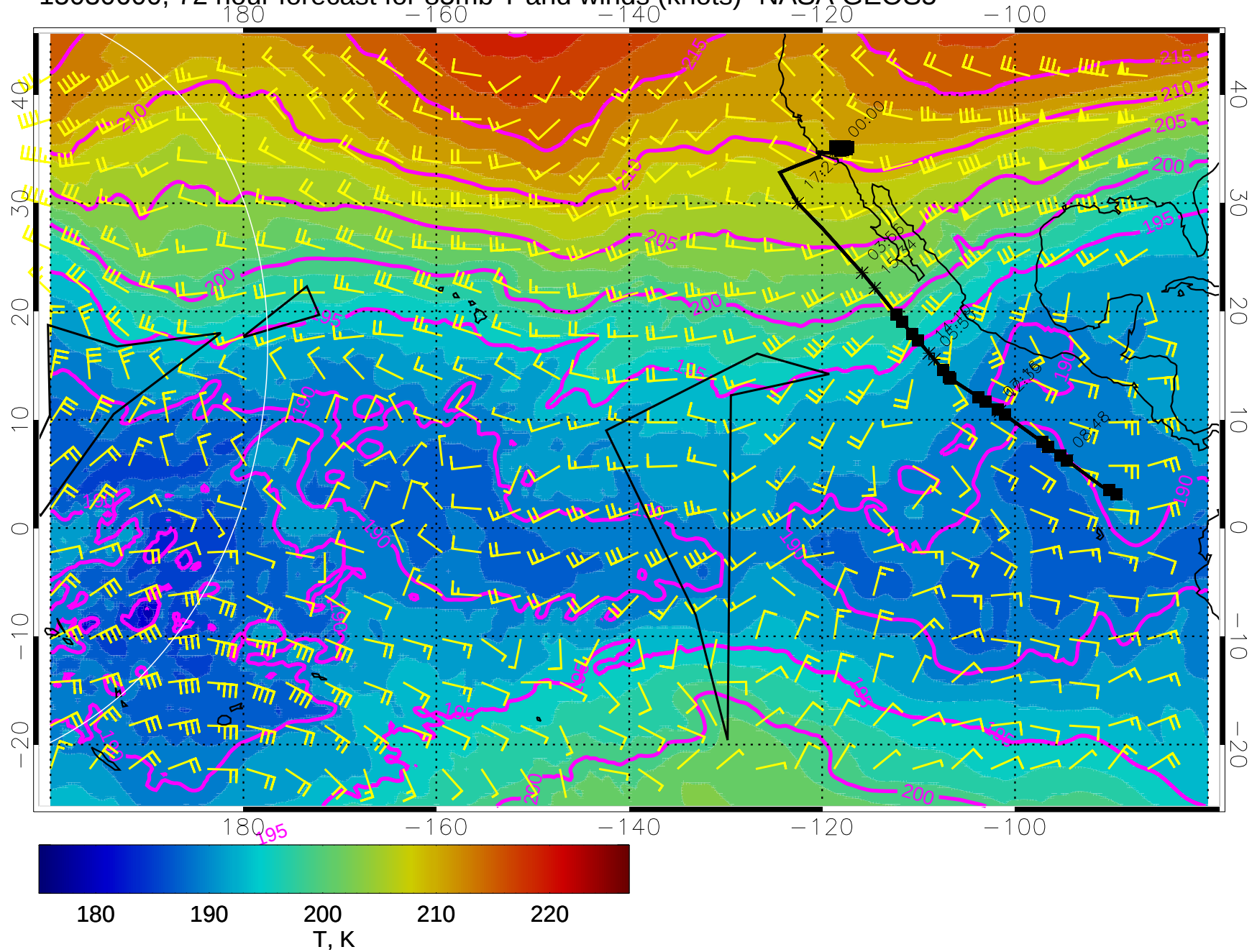
15030600, 72 hour forecast for 85mb T and winds (knots)- NASA GEOS5
