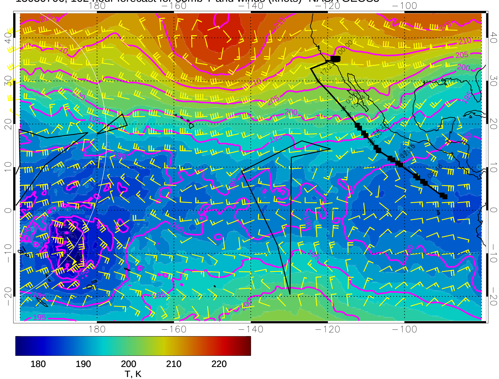
15030706, 102 hour forecast for 85mb T and winds (knots)- NASA GEOS5
