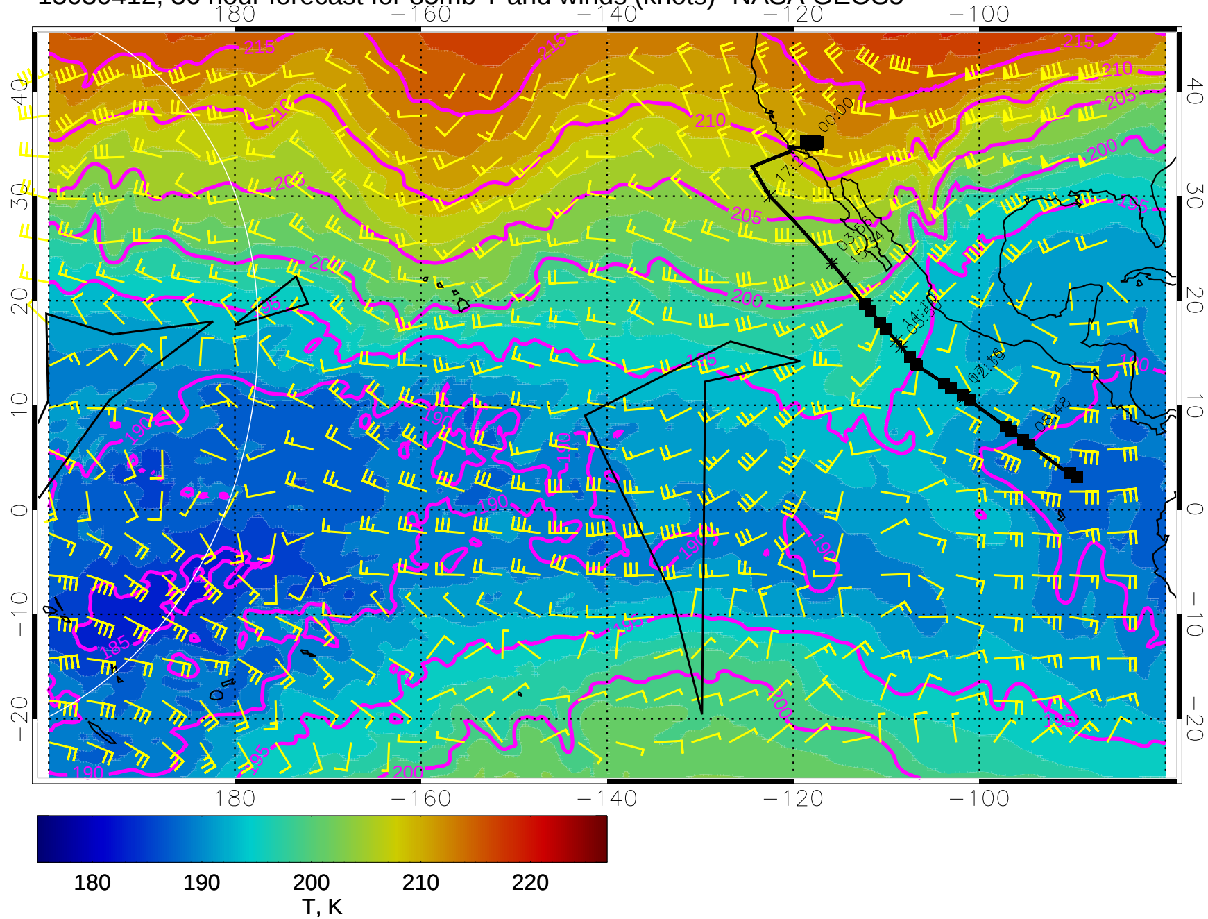
15030412, 36 hour forecast for 85mb T and winds (knots)- NASA GEOS5
