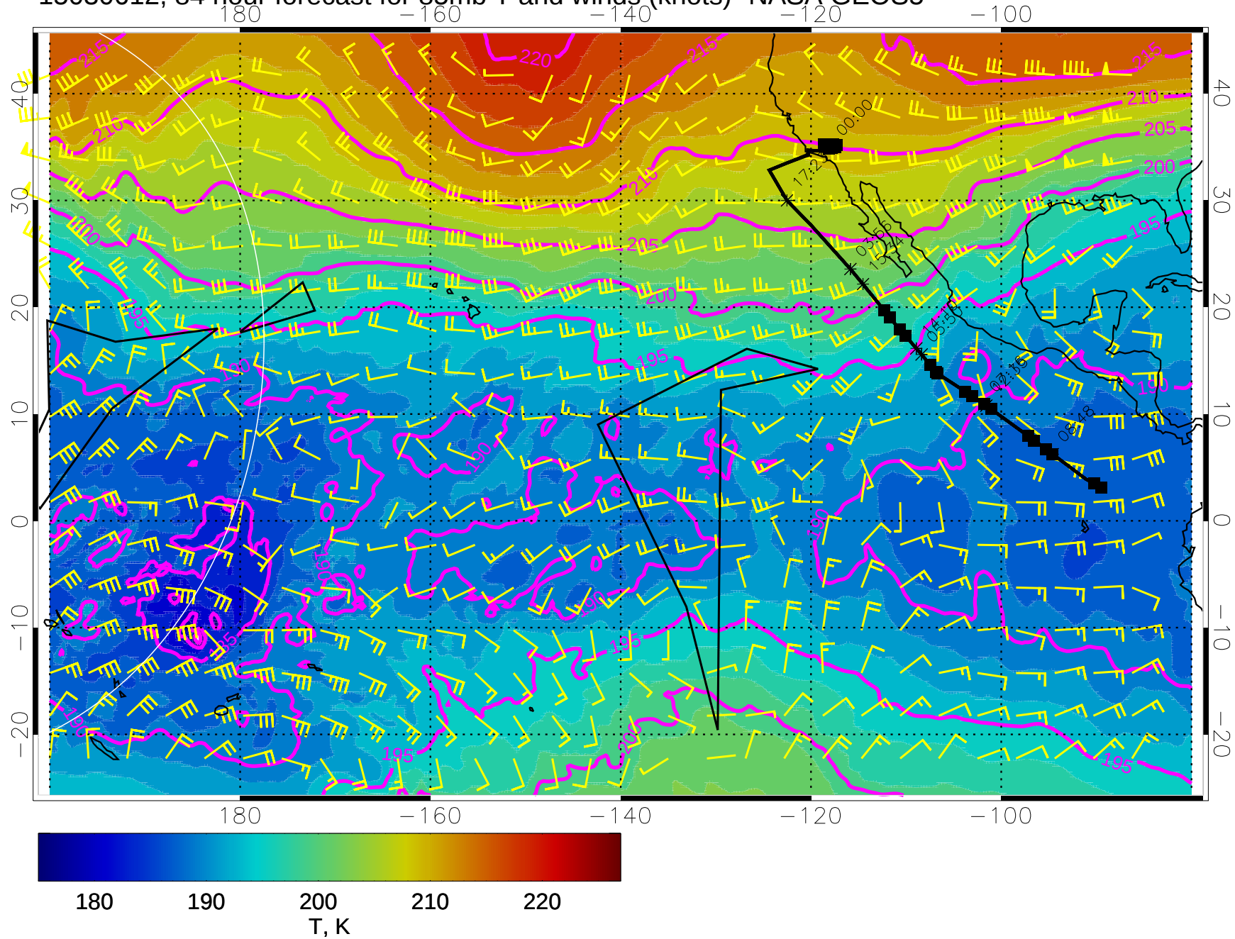
15030612, 84 hour forecast for 85mb T and winds (knots)- NASA GEOS5
