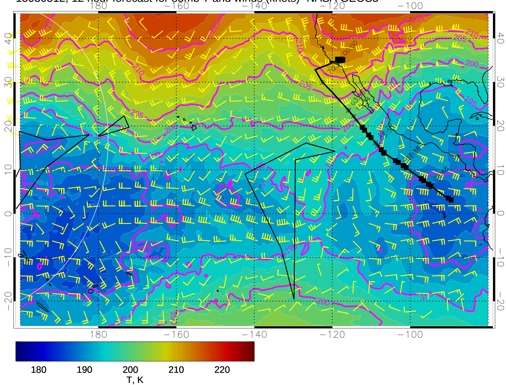
15030312, 12 hour forecast for 85mb T and winds (knots)- NASA GEOS5
