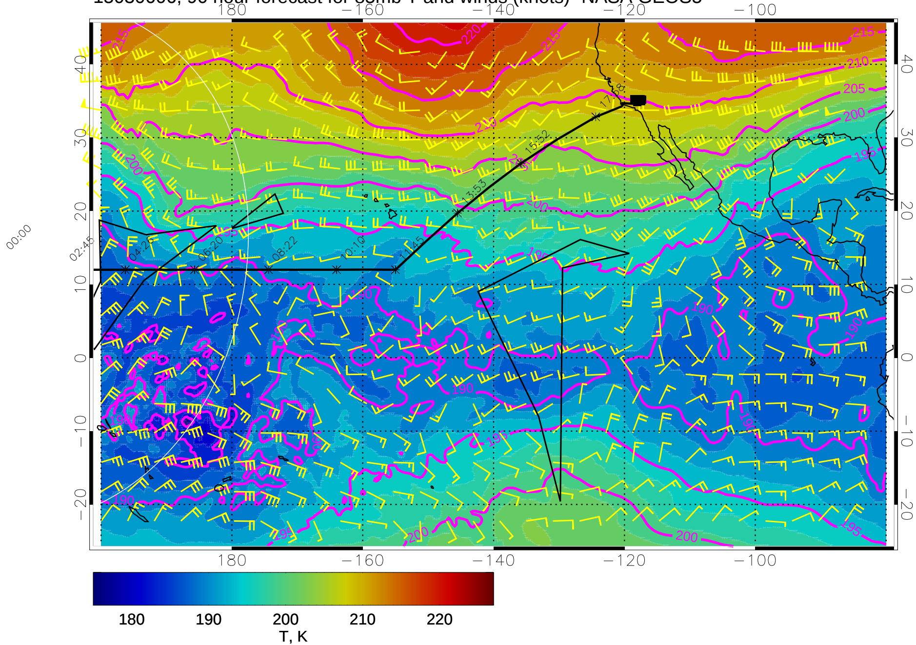
15030606, 90 hour forecast for 85mb T and winds (knots)- NASA GEOS5
