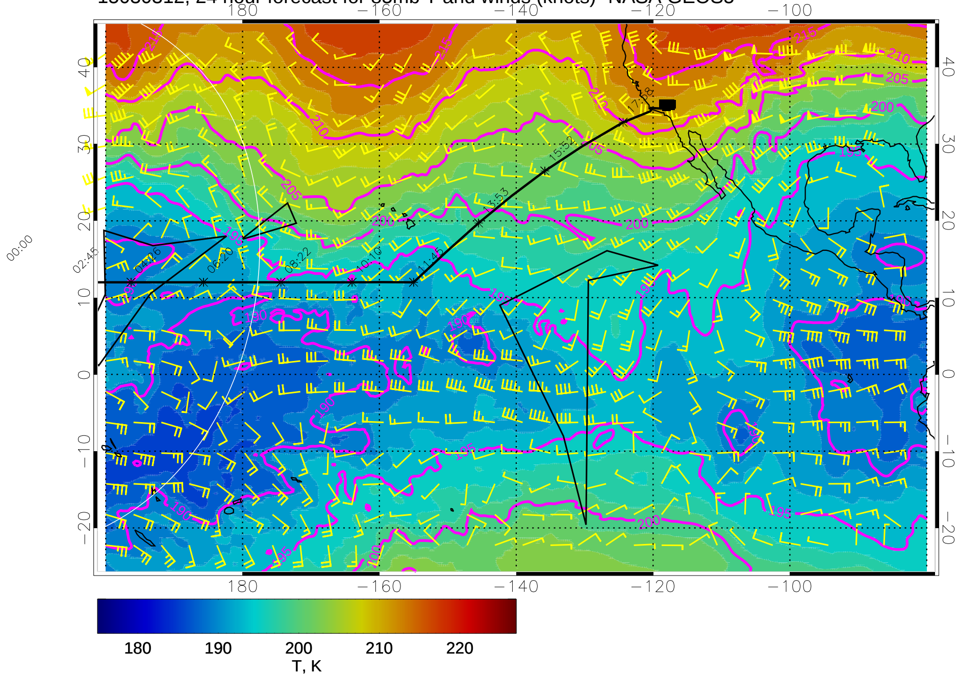
15030312, 24 hour forecast for 85mb T and winds (knots)- NASA GEOS5
