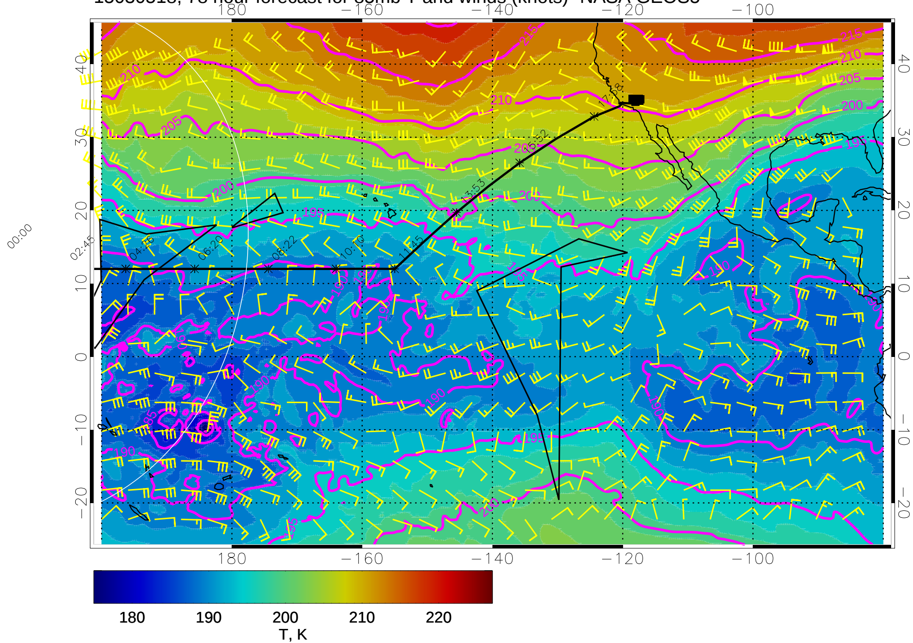
15030518, 78 hour forecast for 85mb T and winds (knots)- NASA GEOS5
