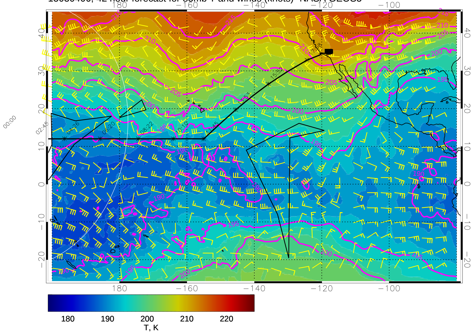
15030406, 42 hour forecast for 85mb T and winds (knots)- NASA GEOS5
