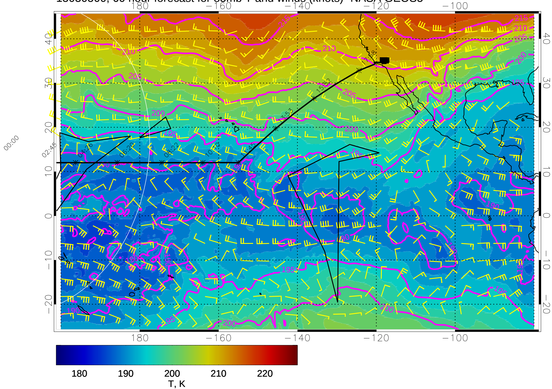
15030500, 60 hour forecast for 85mb T and winds (knots)- NASA GEOS5
