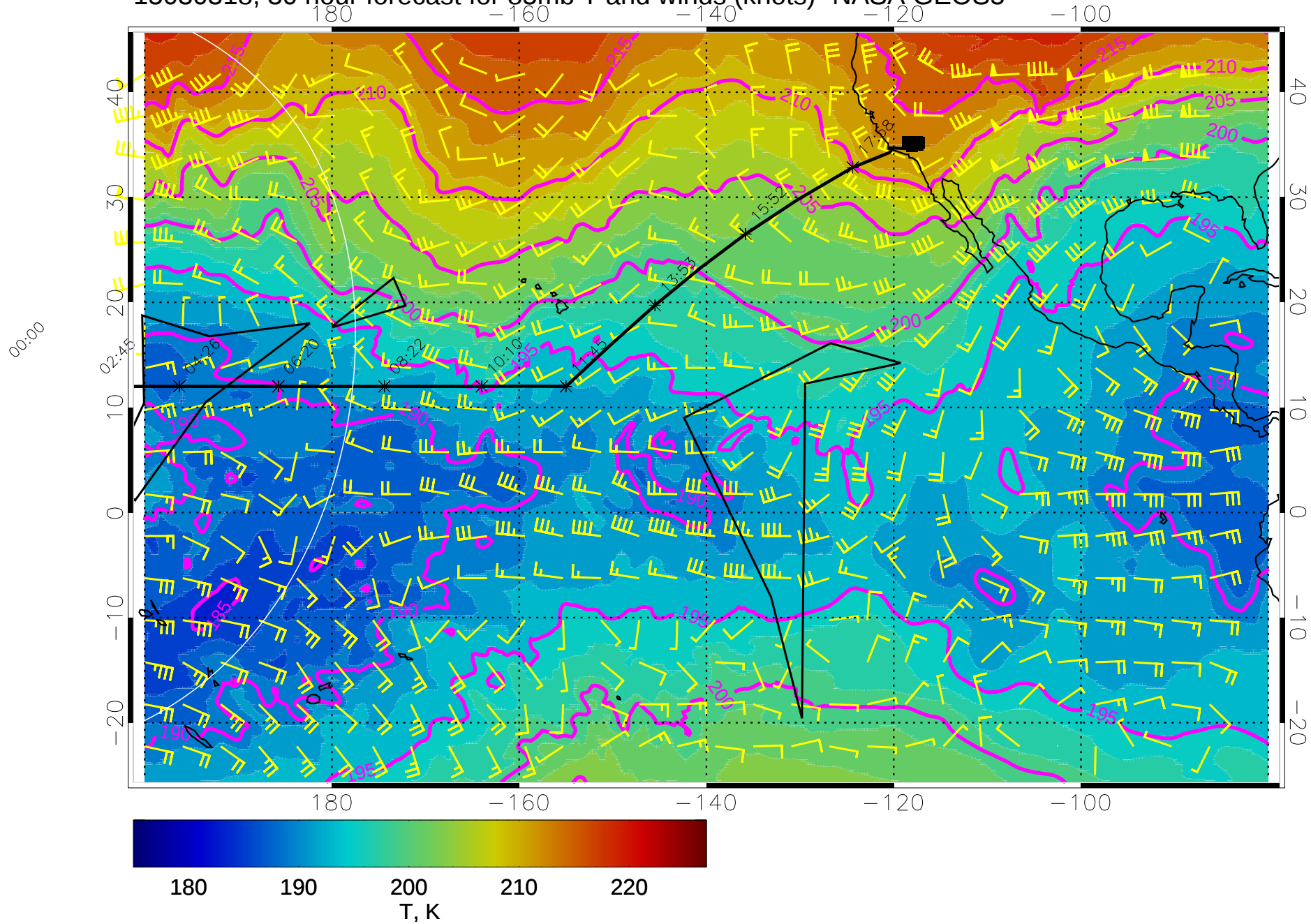
15030318, 30 hour forecast for 85mb T and winds (knots)- NASA GEOS5
