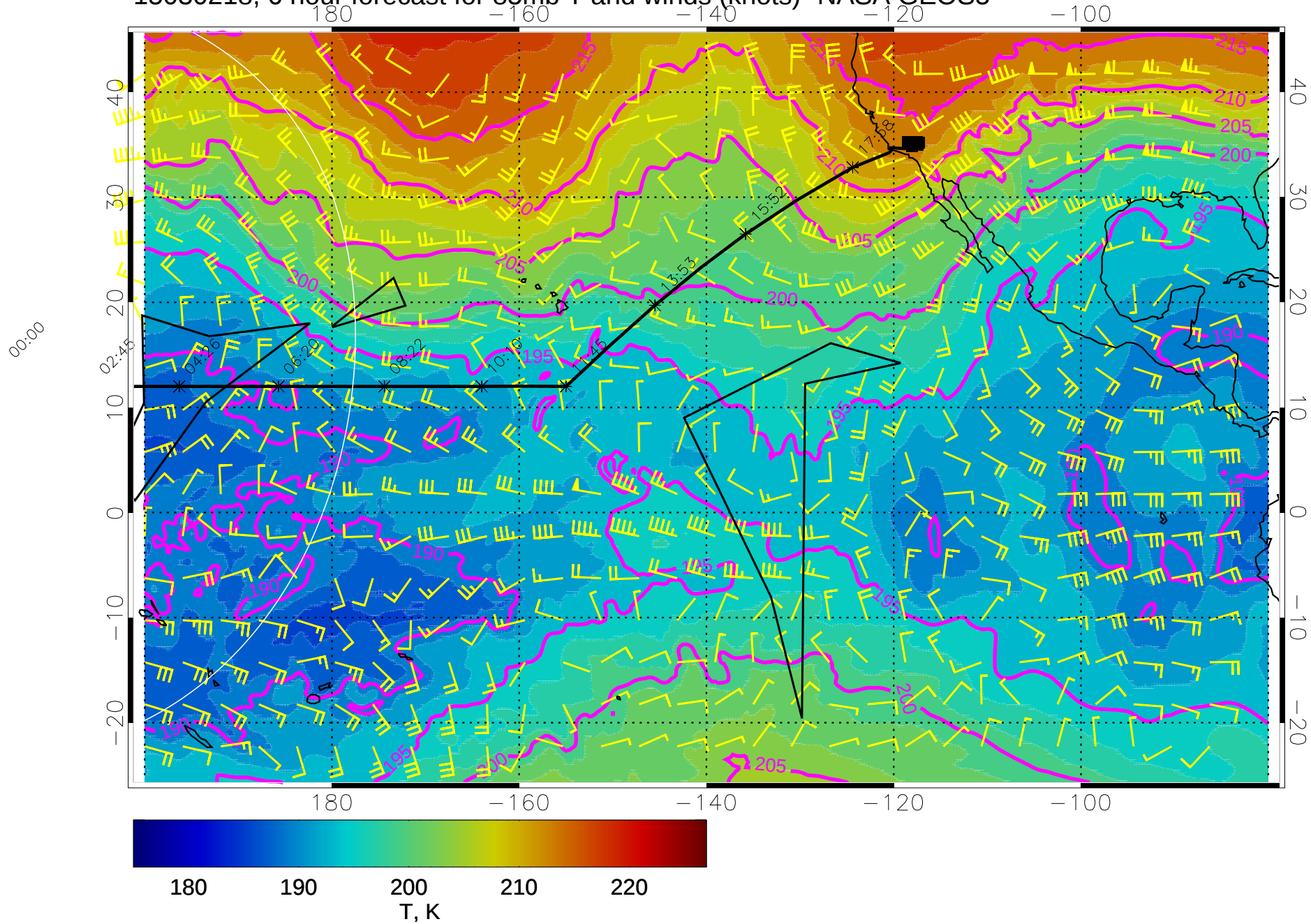
15030218, 6 hour forecast for 85mb T and winds (knots)- NASA GEOS5
