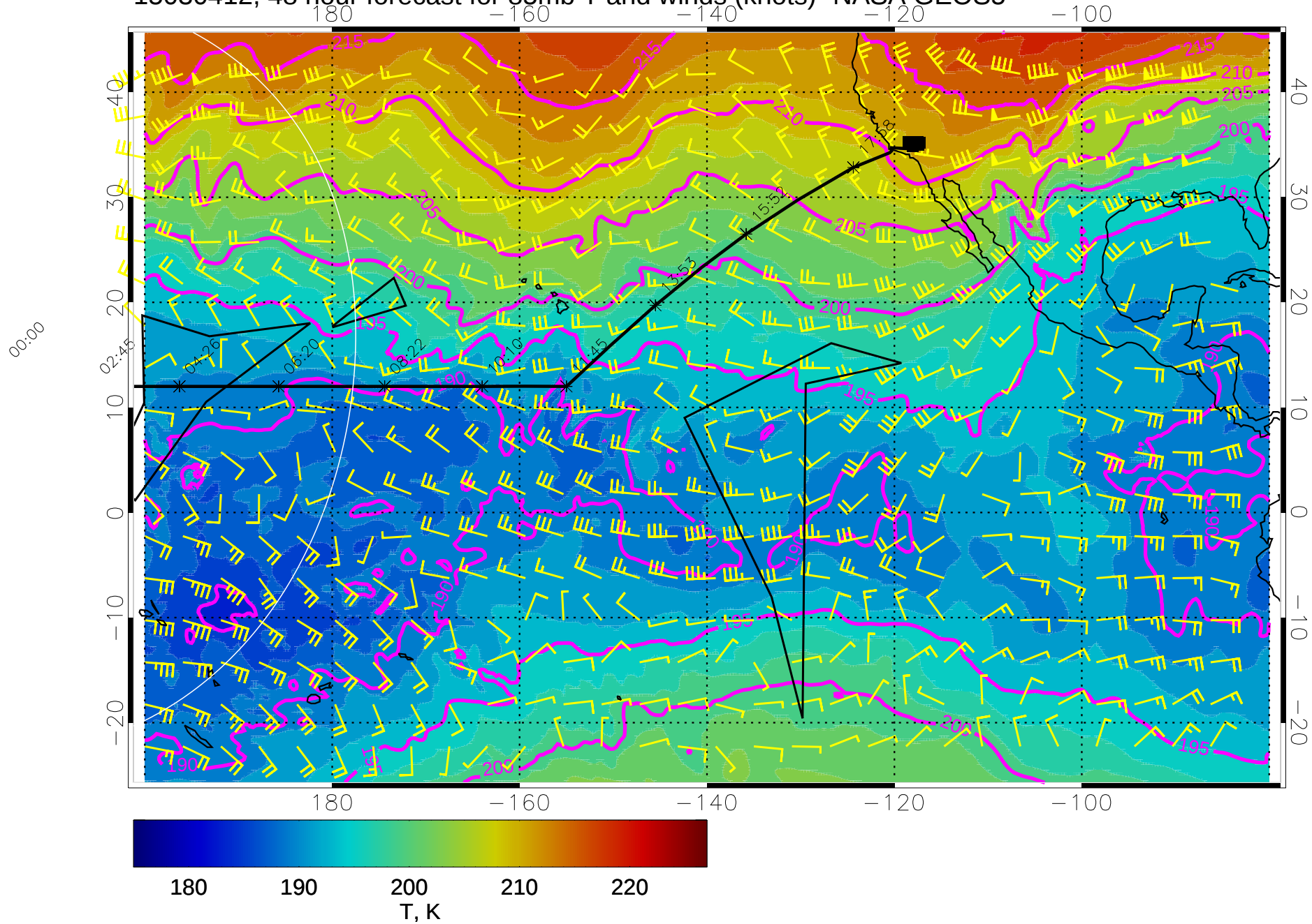
15030412, 48 hour forecast for 85mb T and winds (knots)- NASA GEOS5
