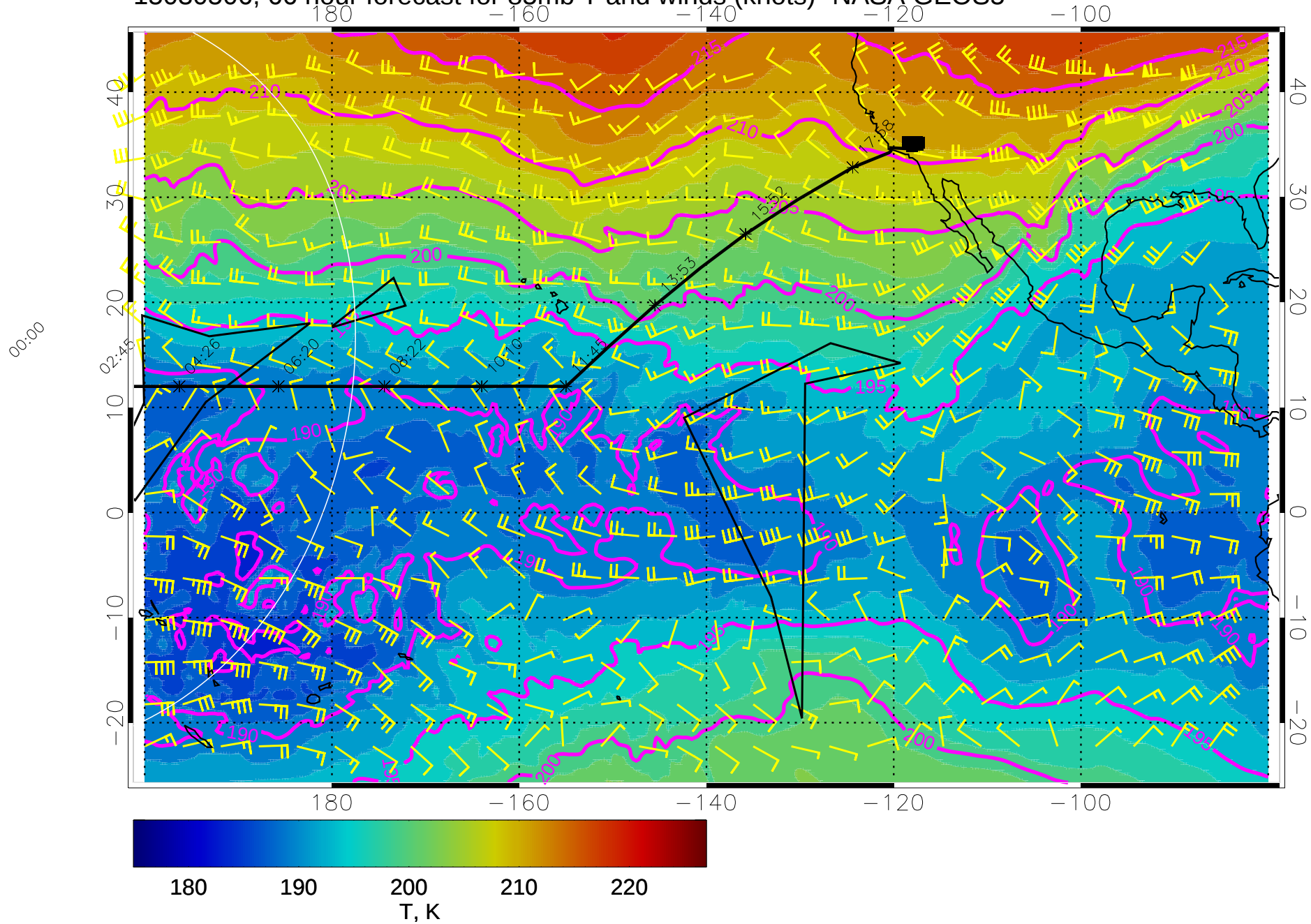
15030506, 66 hour forecast for 85mb T and winds (knots)- NASA GEOS5
