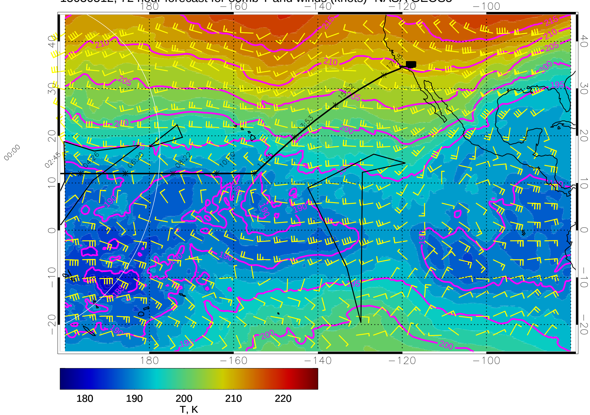
15030512, 72 hour forecast for 85mb T and winds (knots)- NASA GEOS5
