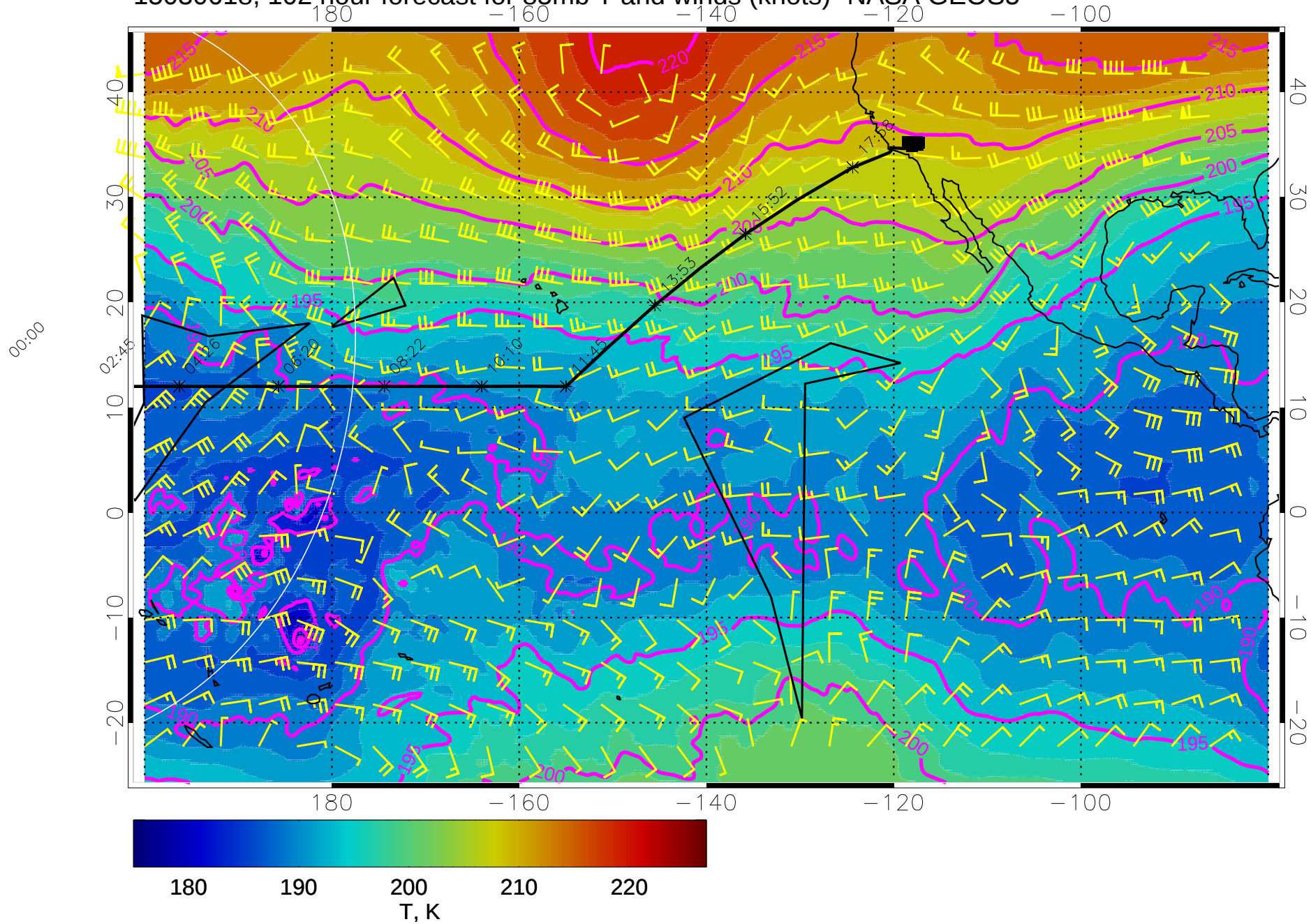
15030618, 102 hour forecast for 85mb T and winds (knots)- NASA GEOS5
