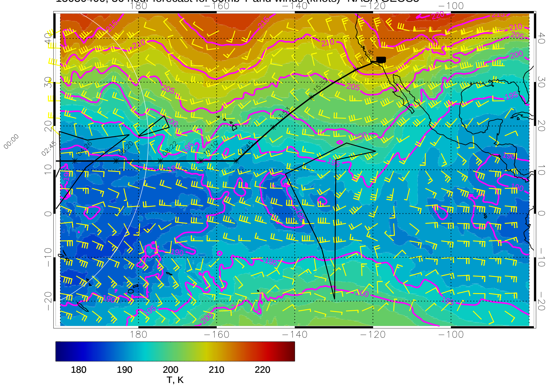
15030400, 36 hour forecast for 85mb T and winds (knots)- NASA GEOS5
