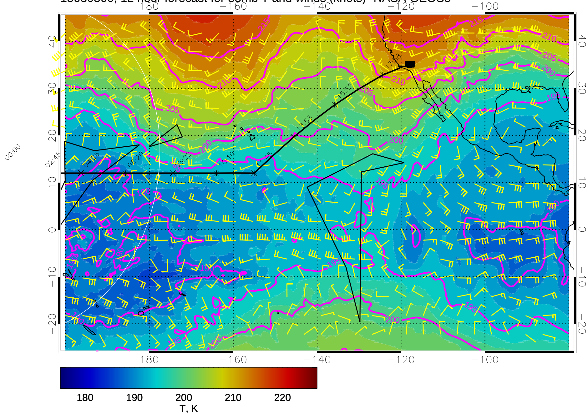
15030300, 12 hour forecast for 85mb T and winds (knots)- NASA GEOS5
