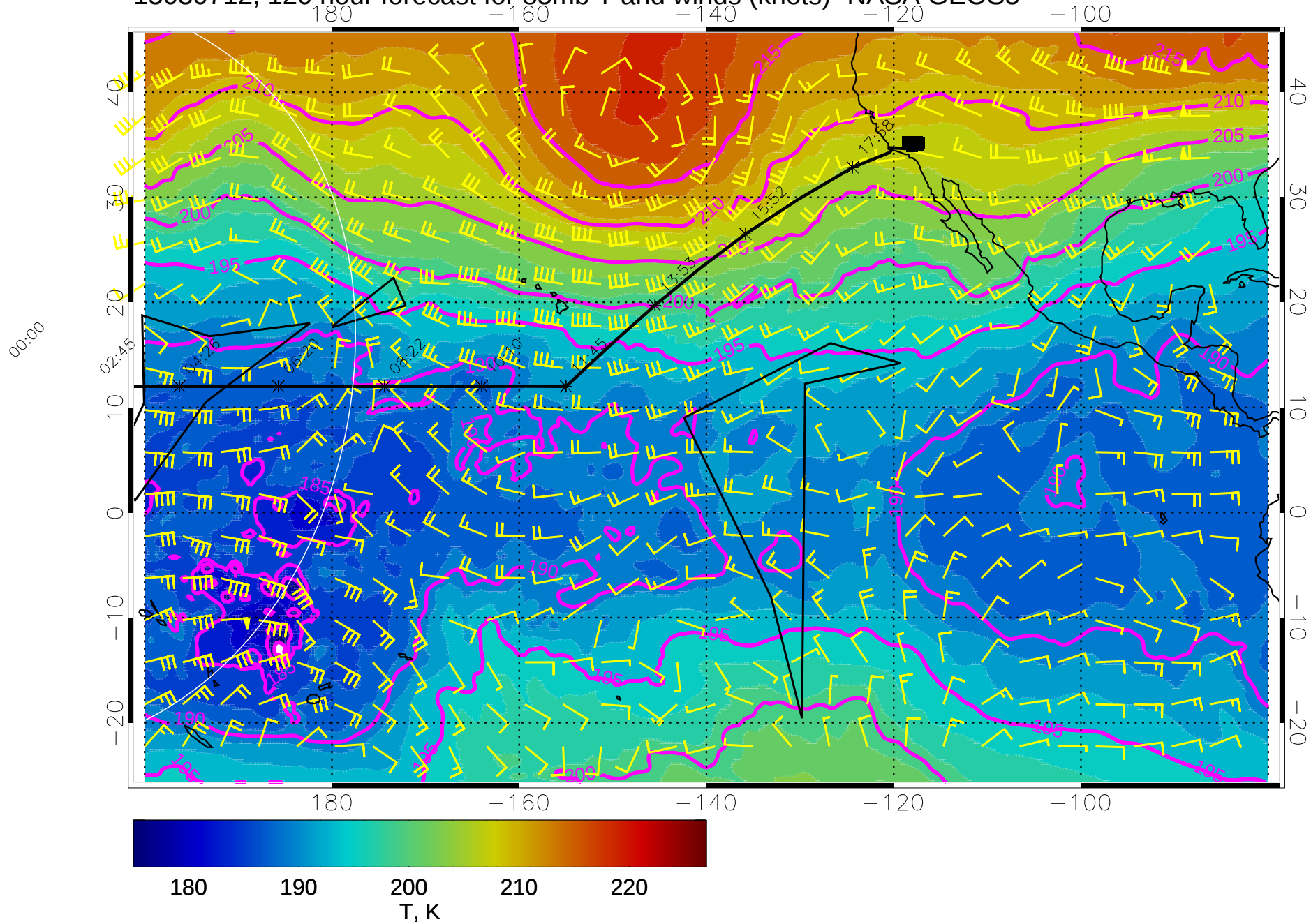
15030712, 120 hour forecast for 85mb T and winds (knots)- NASA GEOS5
