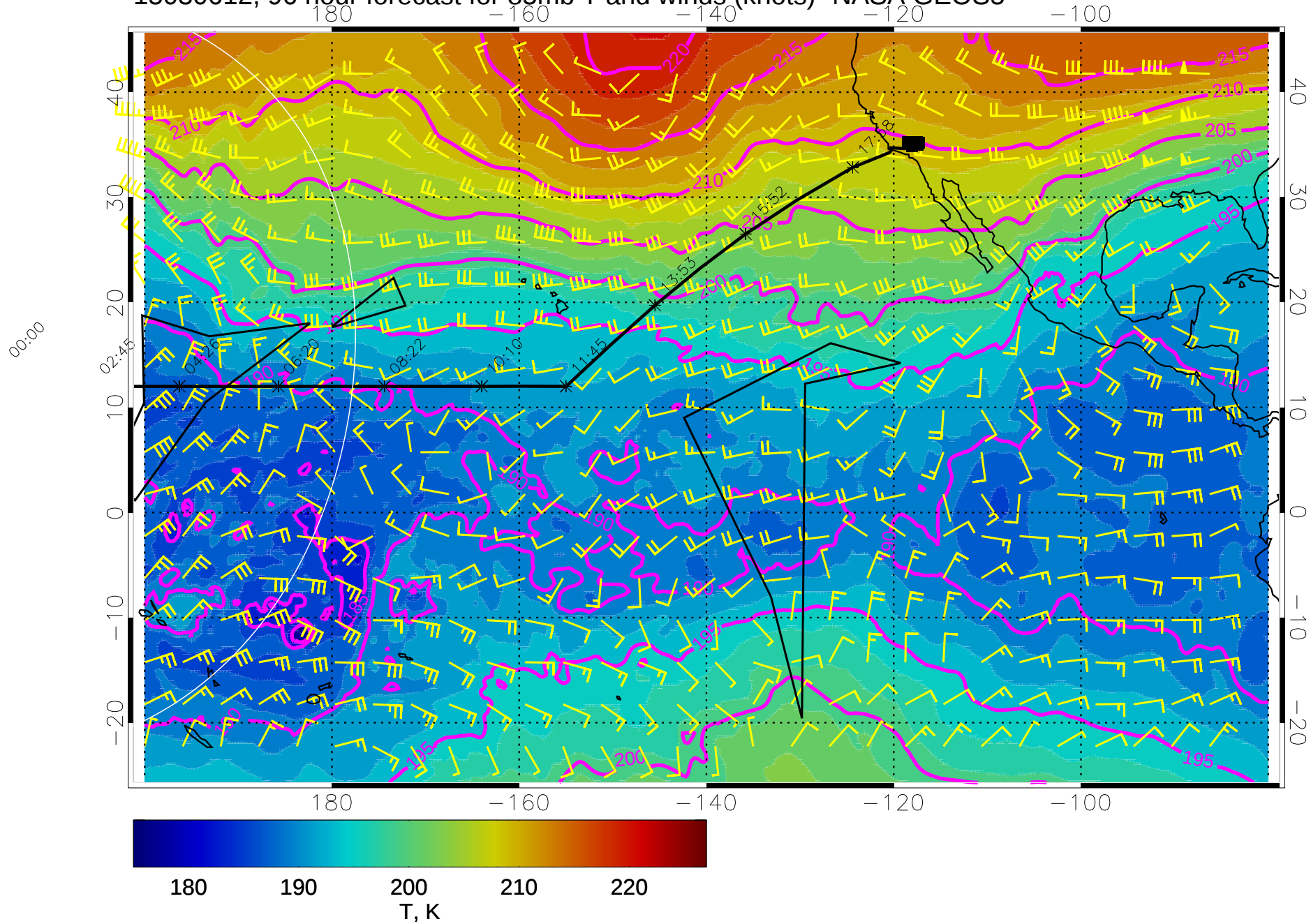
15030612, 96 hour forecast for 85mb T and winds (knots)- NASA GEOS5
