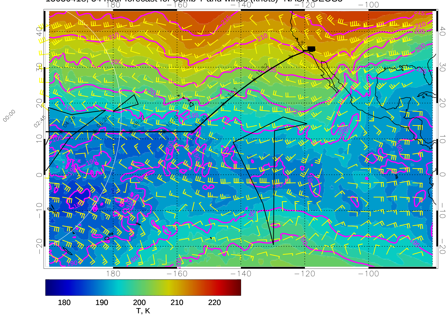
15030418, 54 hour forecast for 85mb T and winds (knots)- NASA GEOS5
