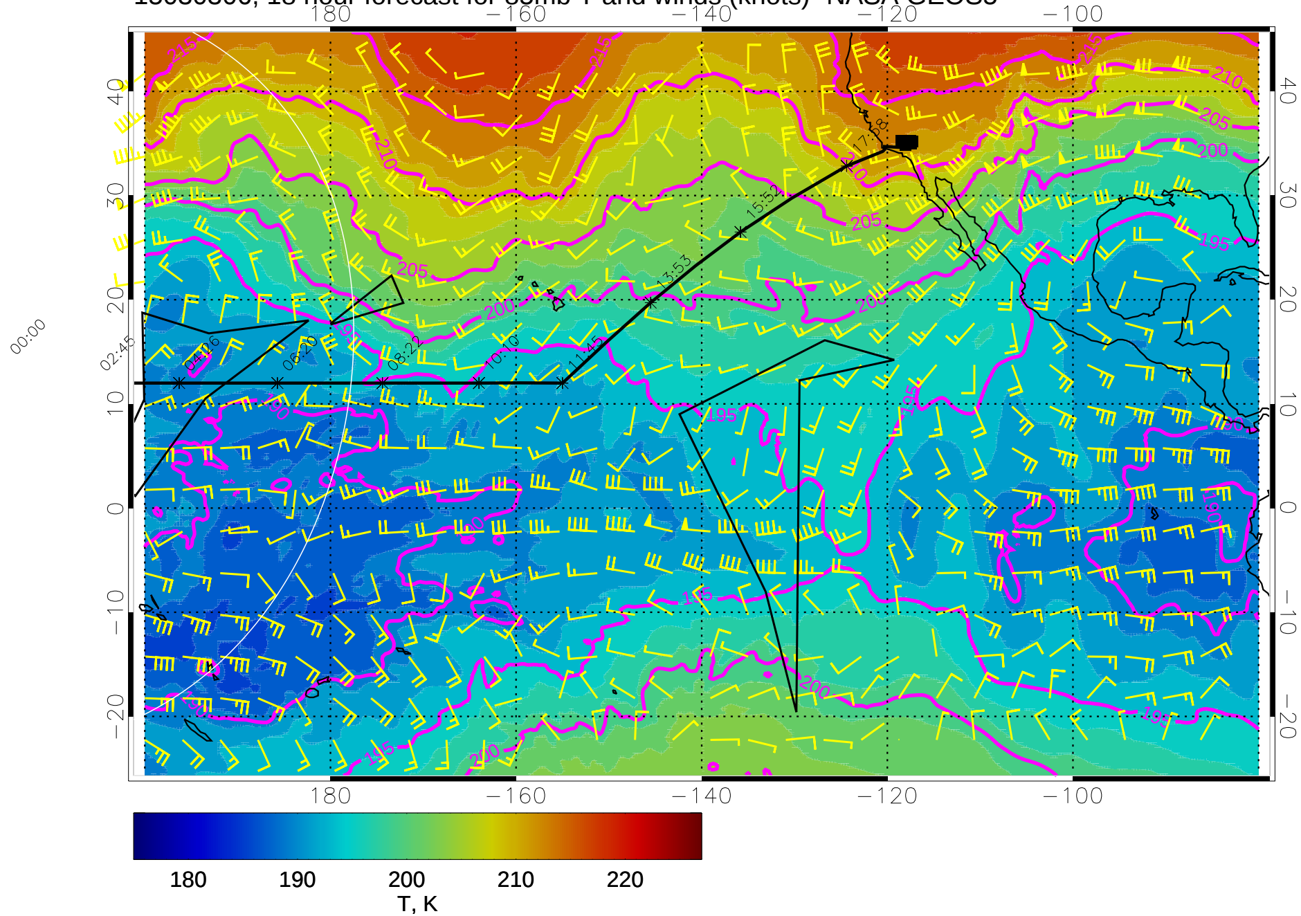
15030306, 18 hour forecast for 85mb T and winds (knots)- NASA GEOS5
