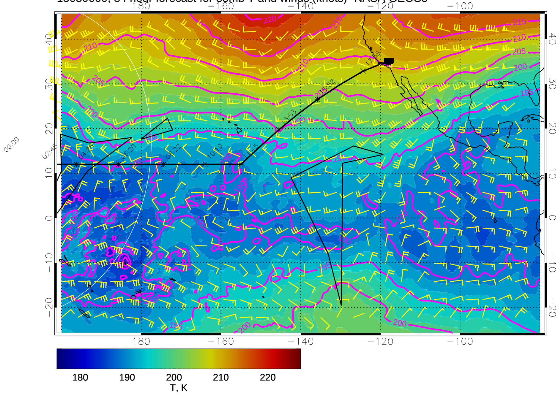
15030600, 84 hour forecast for 85mb T and winds (knots)- NASA GEOS5
