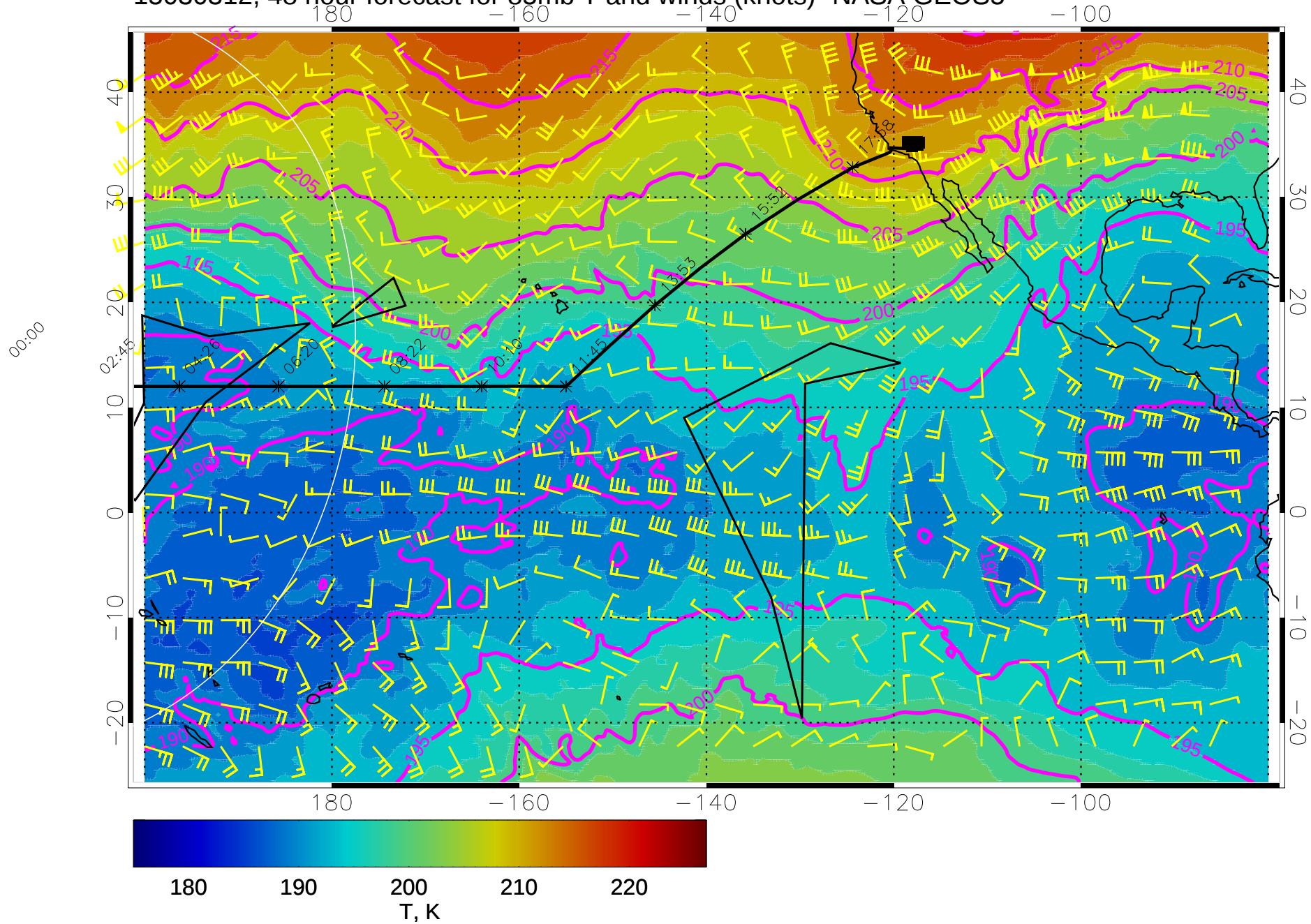
15030312, 48 hour forecast for 85mb T and winds (knots)- NASA GEOS5
