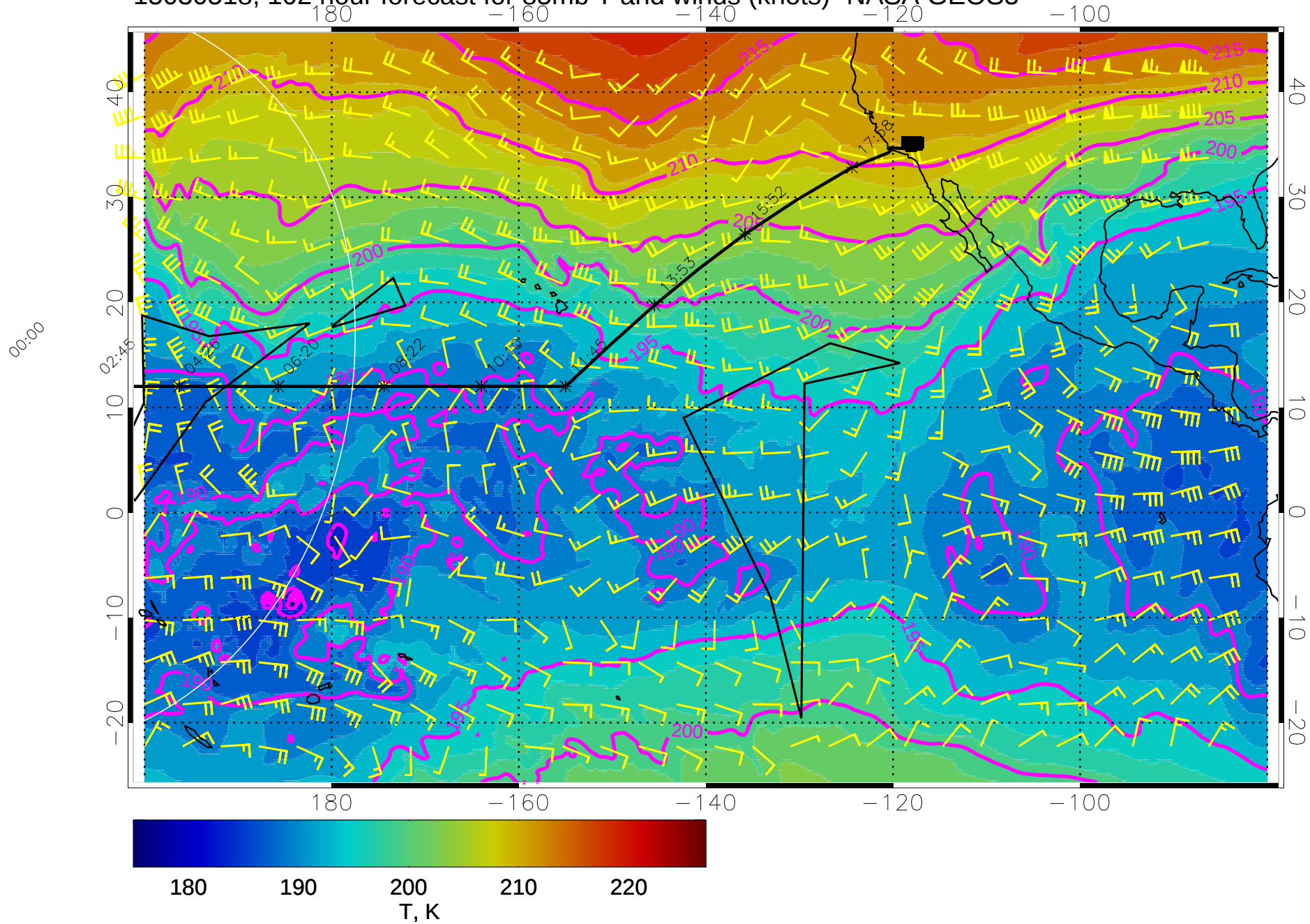
15030518, 102 hour forecast for 85mb T and winds (knots)- NASA GEOS5
