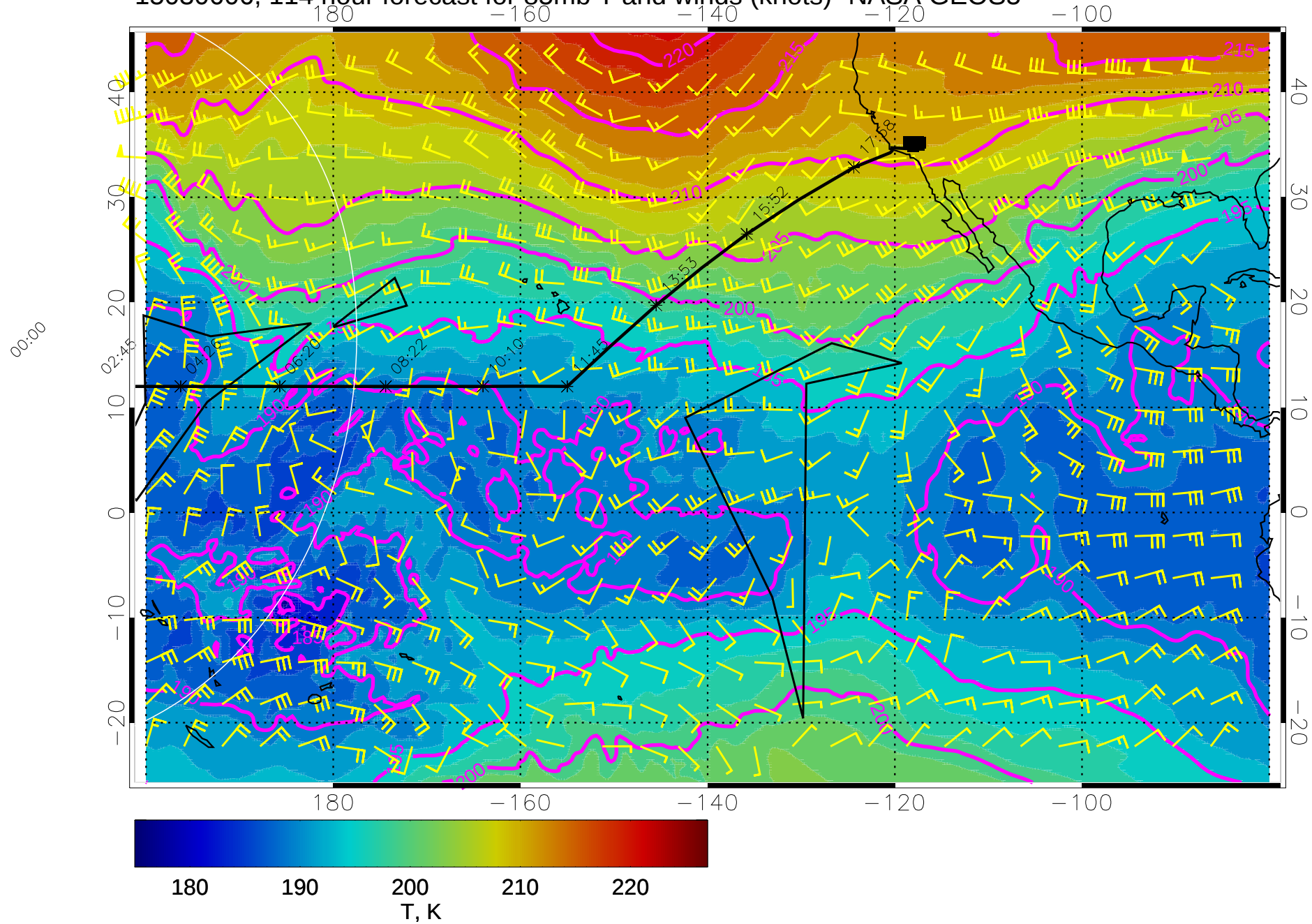
15030606, 114 hour forecast for 85mb T and winds (knots)- NASA GEOS5
