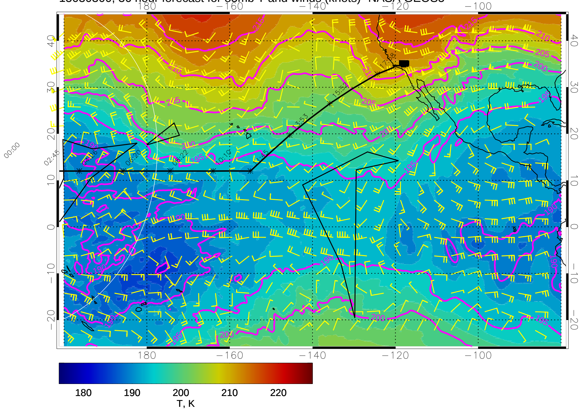
15030300, 36 hour forecast for 85mb T and winds (knots)- NASA GEOS5
