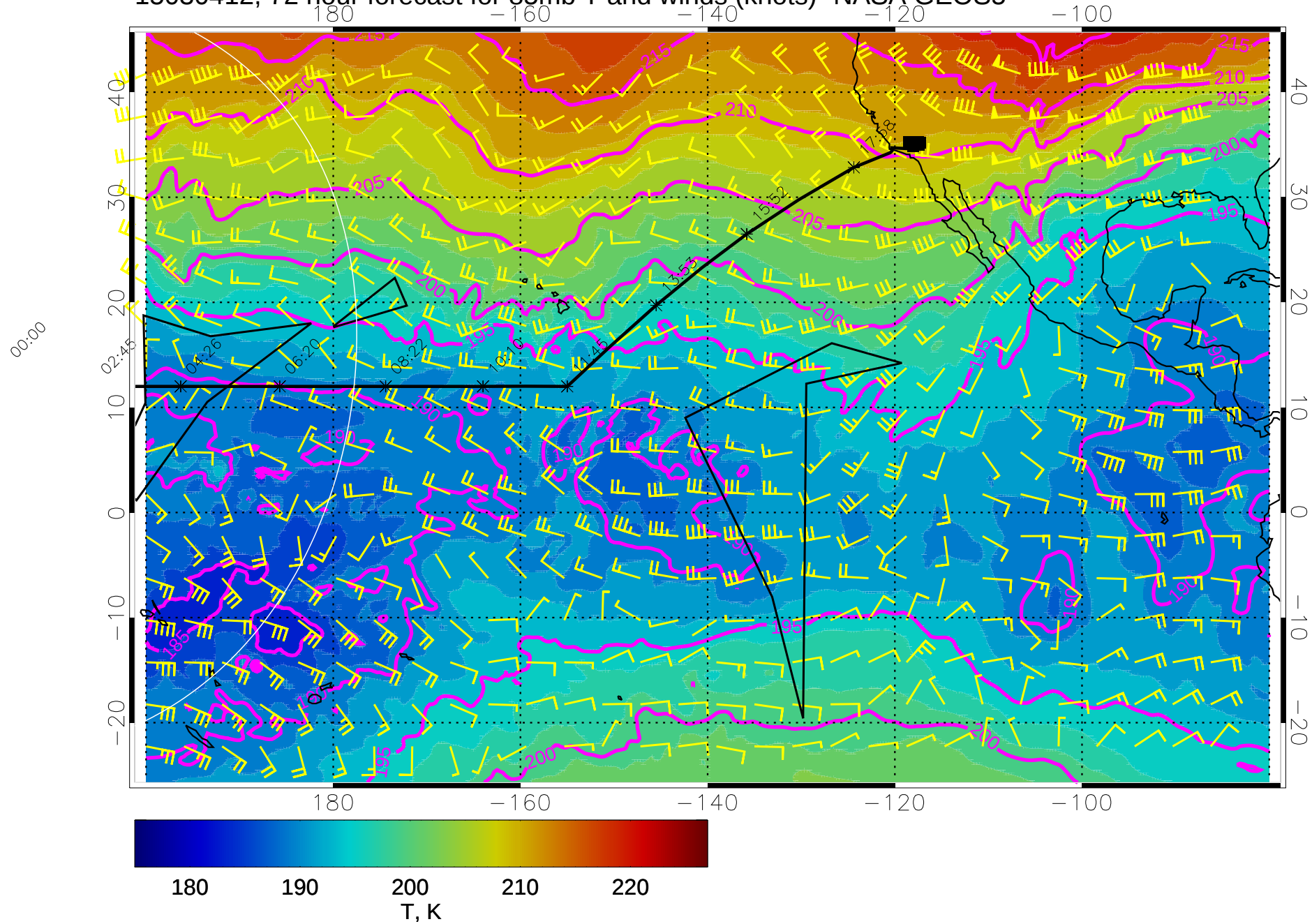
15030412, 72 hour forecast for 85mb T and winds (knots)- NASA GEOS5
