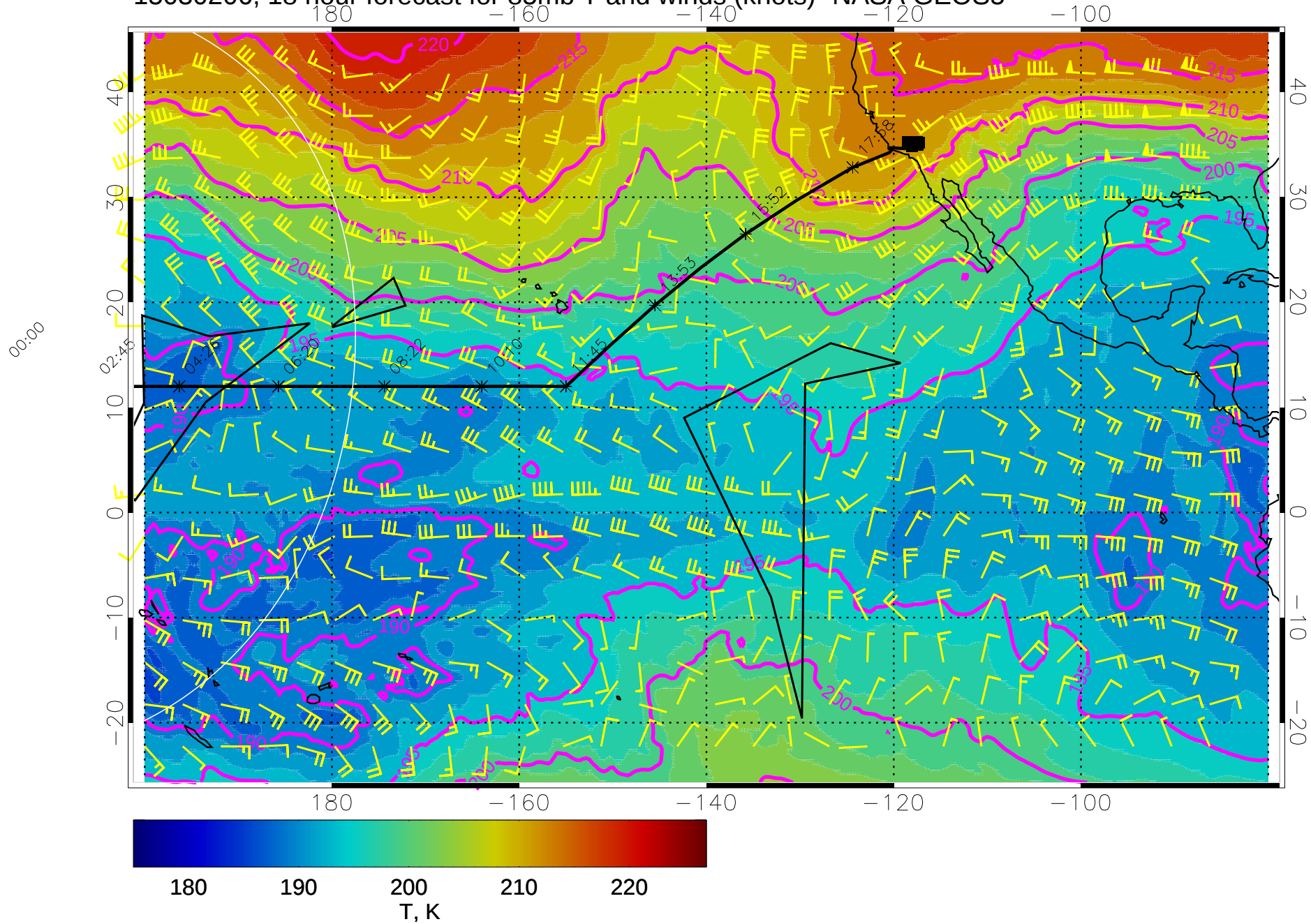
15030206, 18 hour forecast for 85mb T and winds (knots)- NASA GEOS5
