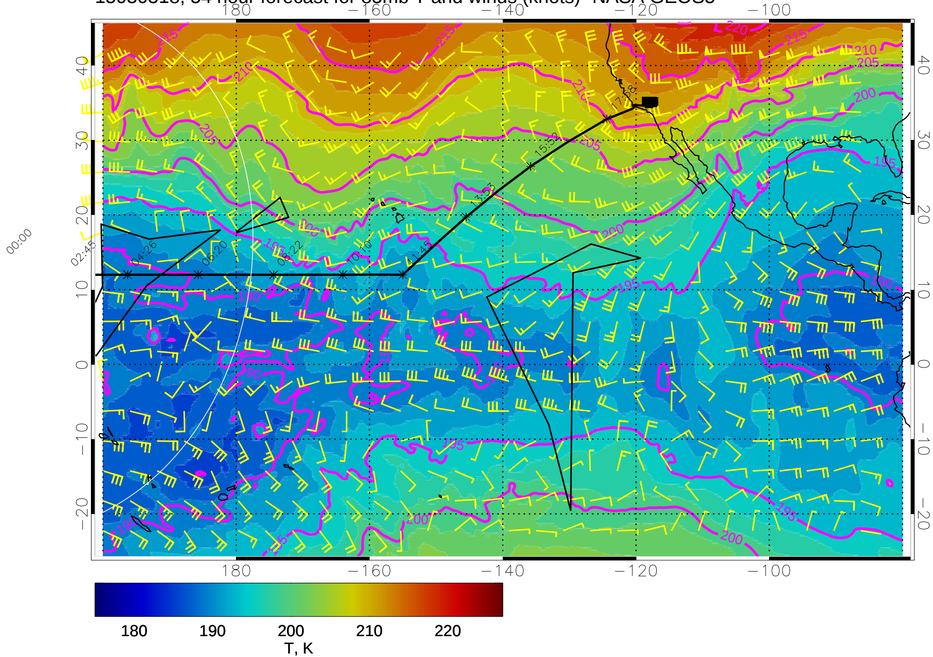
15030318, 54 hour forecast for 85mb T and winds (knots)- NASA GEOS5
