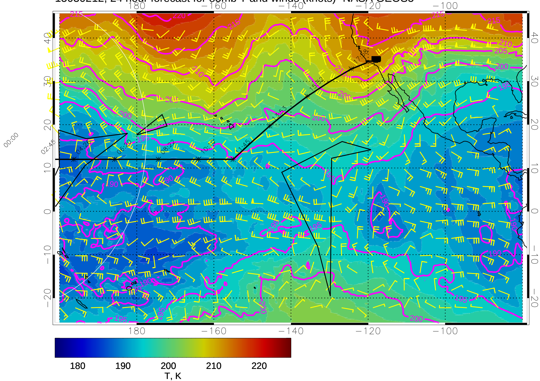
15030212, 24 hour forecast for 85mb T and winds (knots)- NASA GEOS5
