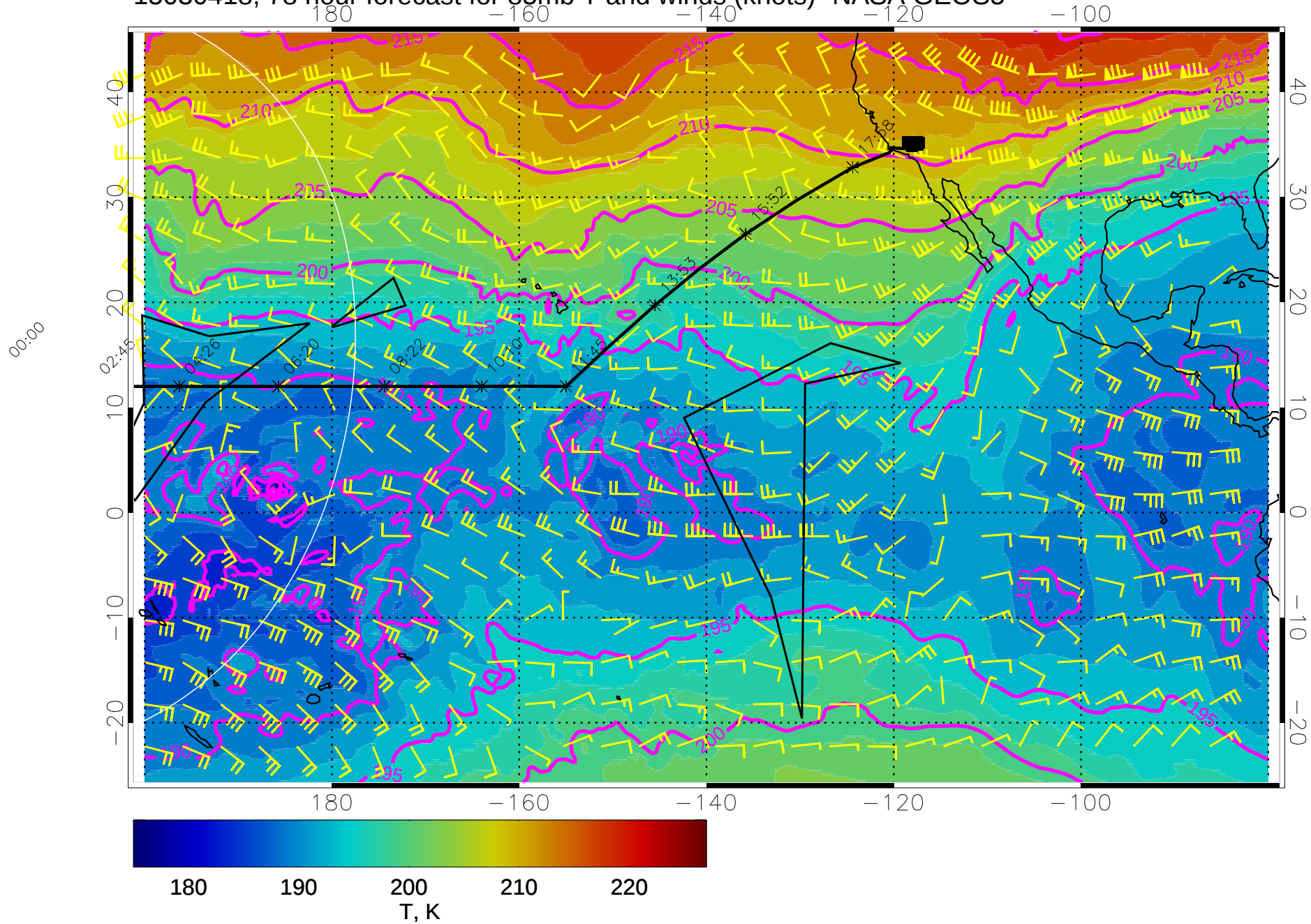
15030418, 78 hour forecast for 85mb T and winds (knots)- NASA GEOS5
