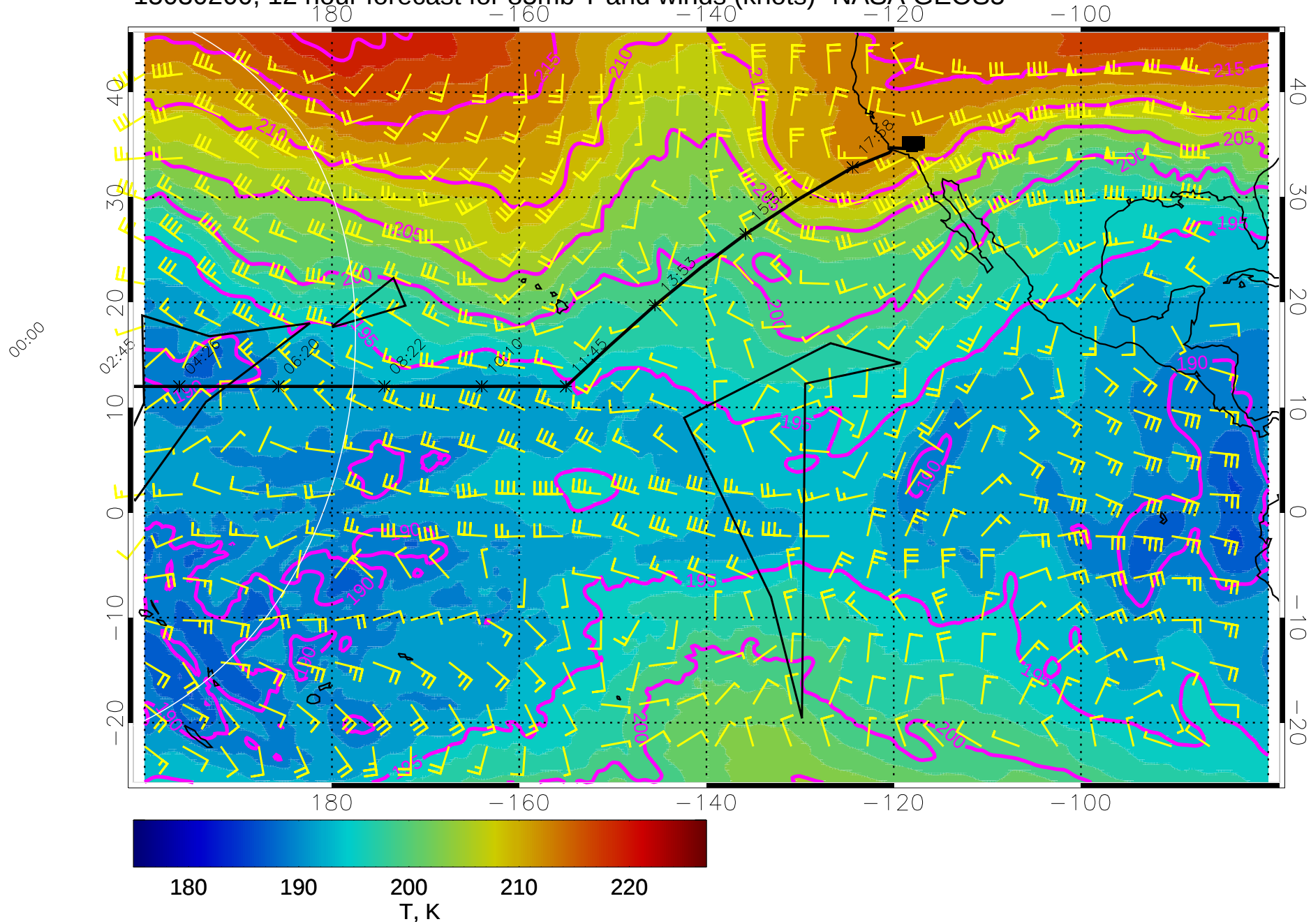
15030200, 12 hour forecast for 85mb T and winds (knots)- NASA GEOS5
