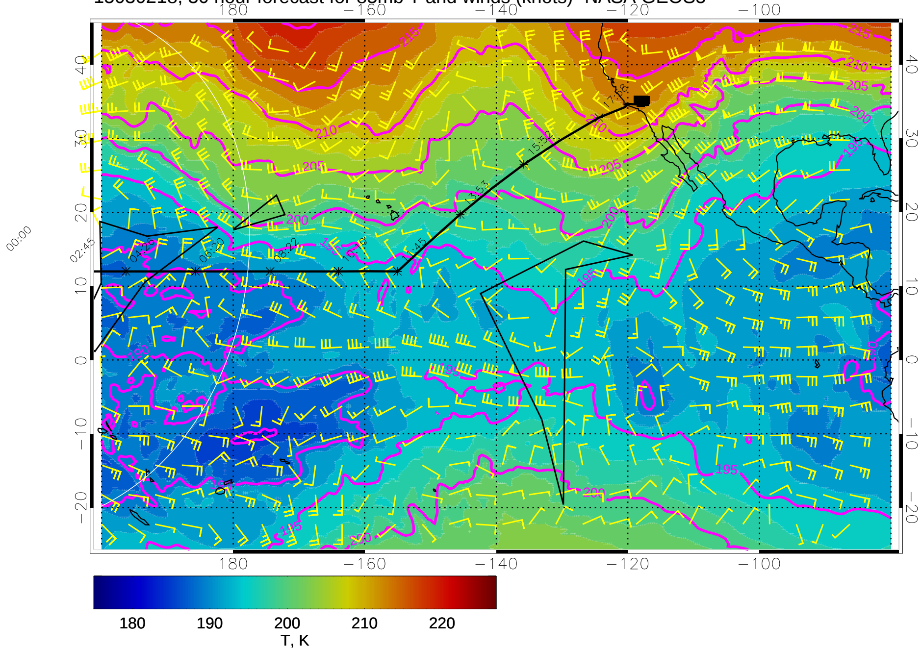
15030218, 30 hour forecast for 85mb T and winds (knots)- NASA GEOS5
