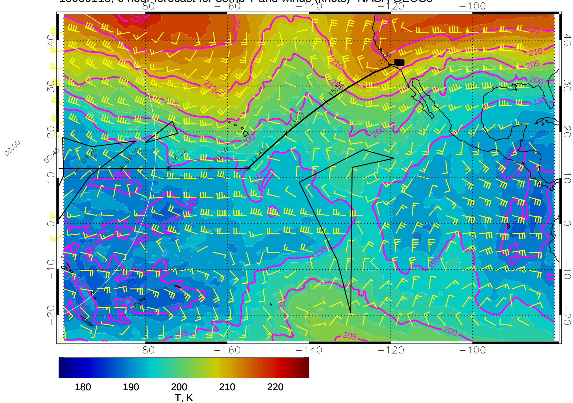
15030118, 6 hour forecast for 85mb T and winds (knots)- NASA GEOS5
