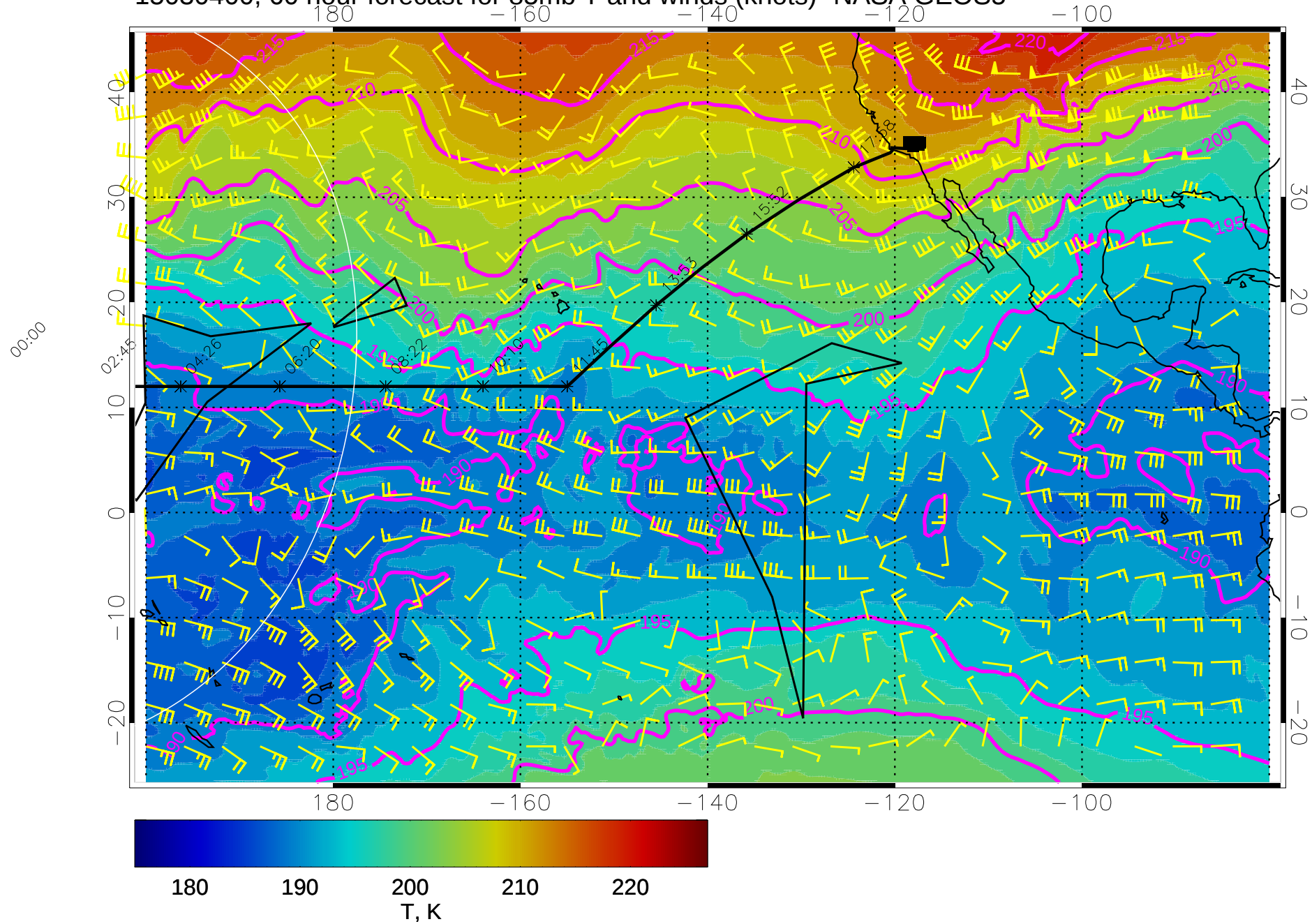
15030400, 60 hour forecast for 85mb T and winds (knots)- NASA GEOS5
