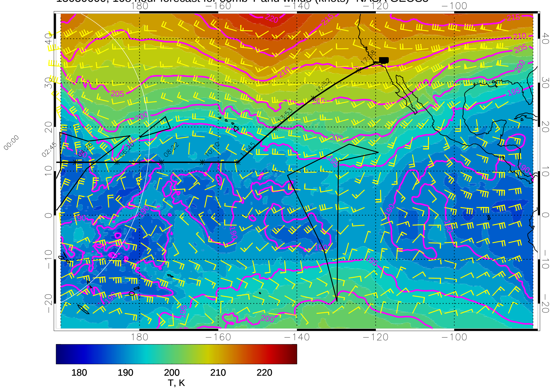
15030600, 108 hour forecast for 85mb T and winds (knots)- NASA GEOS5
