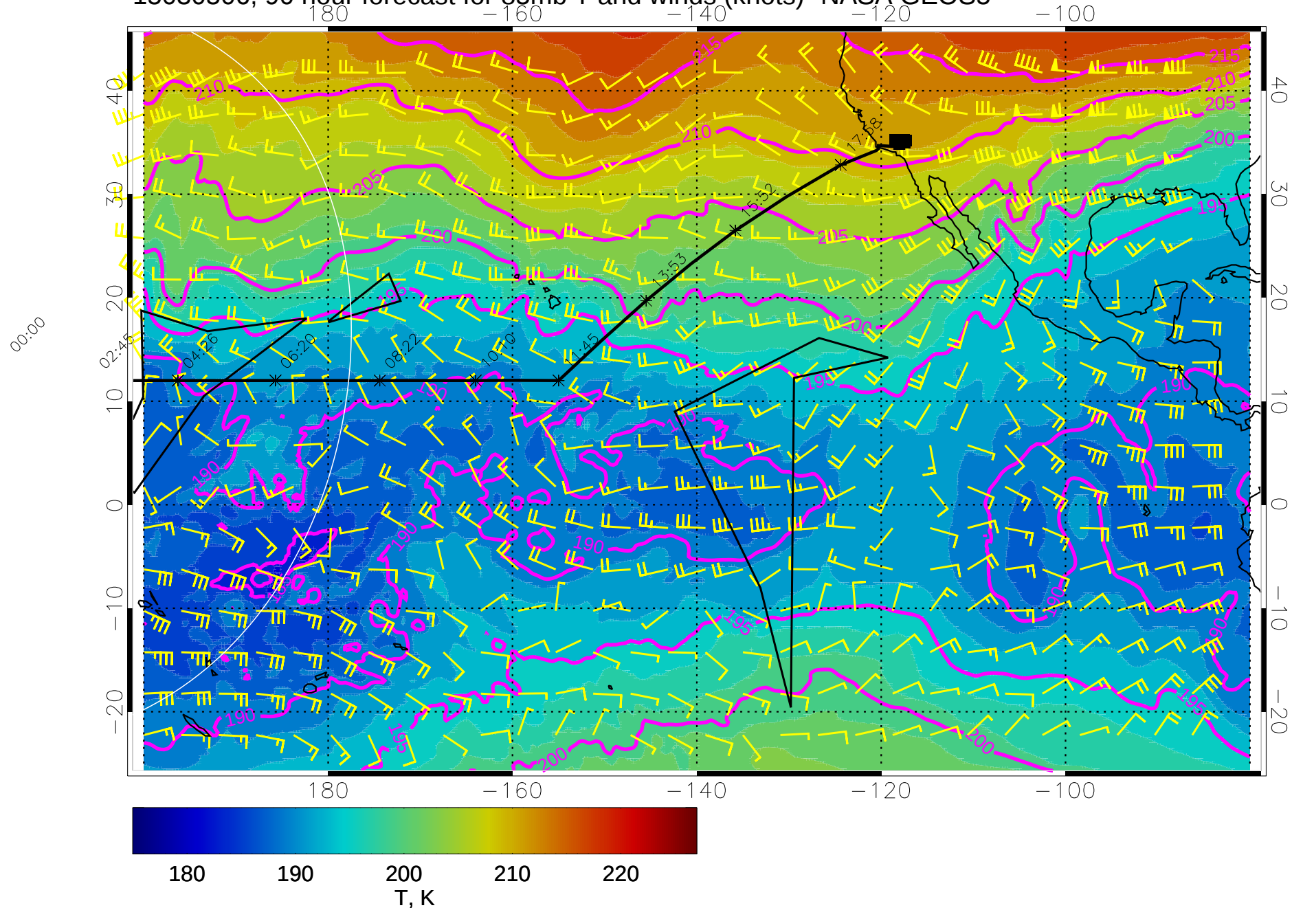
15030506, 90 hour forecast for 85mb T and winds (knots)- NASA GEOS5
