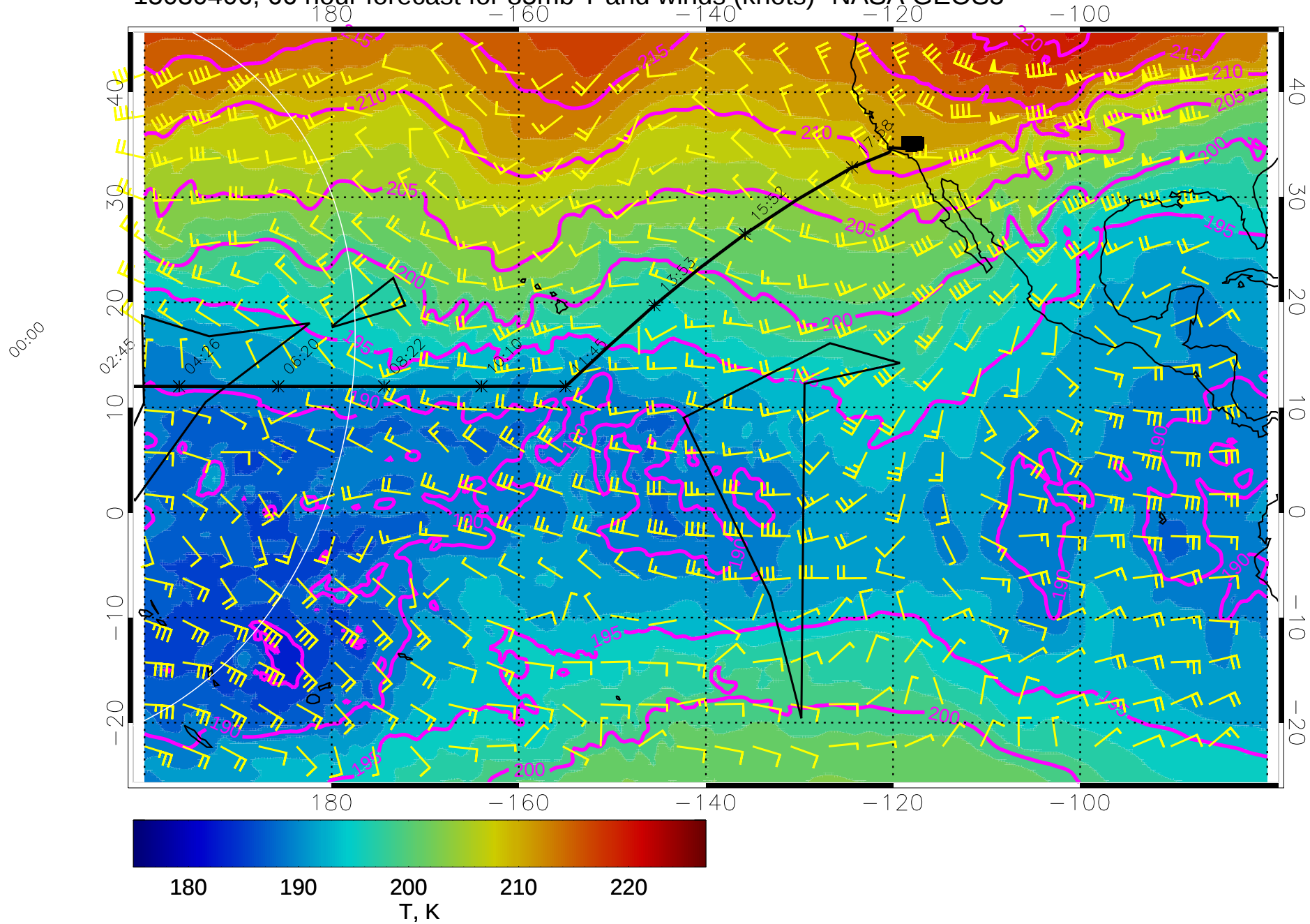
15030406, 66 hour forecast for 85mb T and winds (knots)- NASA GEOS5
