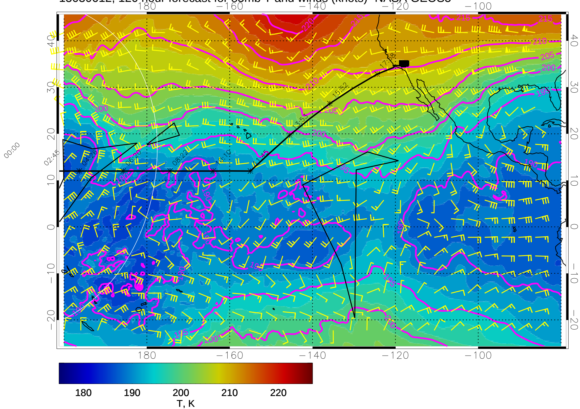
15030612, 120 hour forecast for 85mb T and winds (knots)- NASA GEOS5
