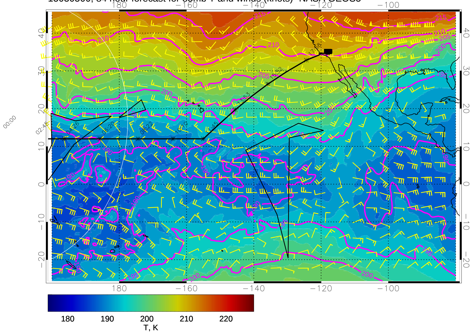
15030500, 84 hour forecast for 85mb T and winds (knots)- NASA GEOS5
