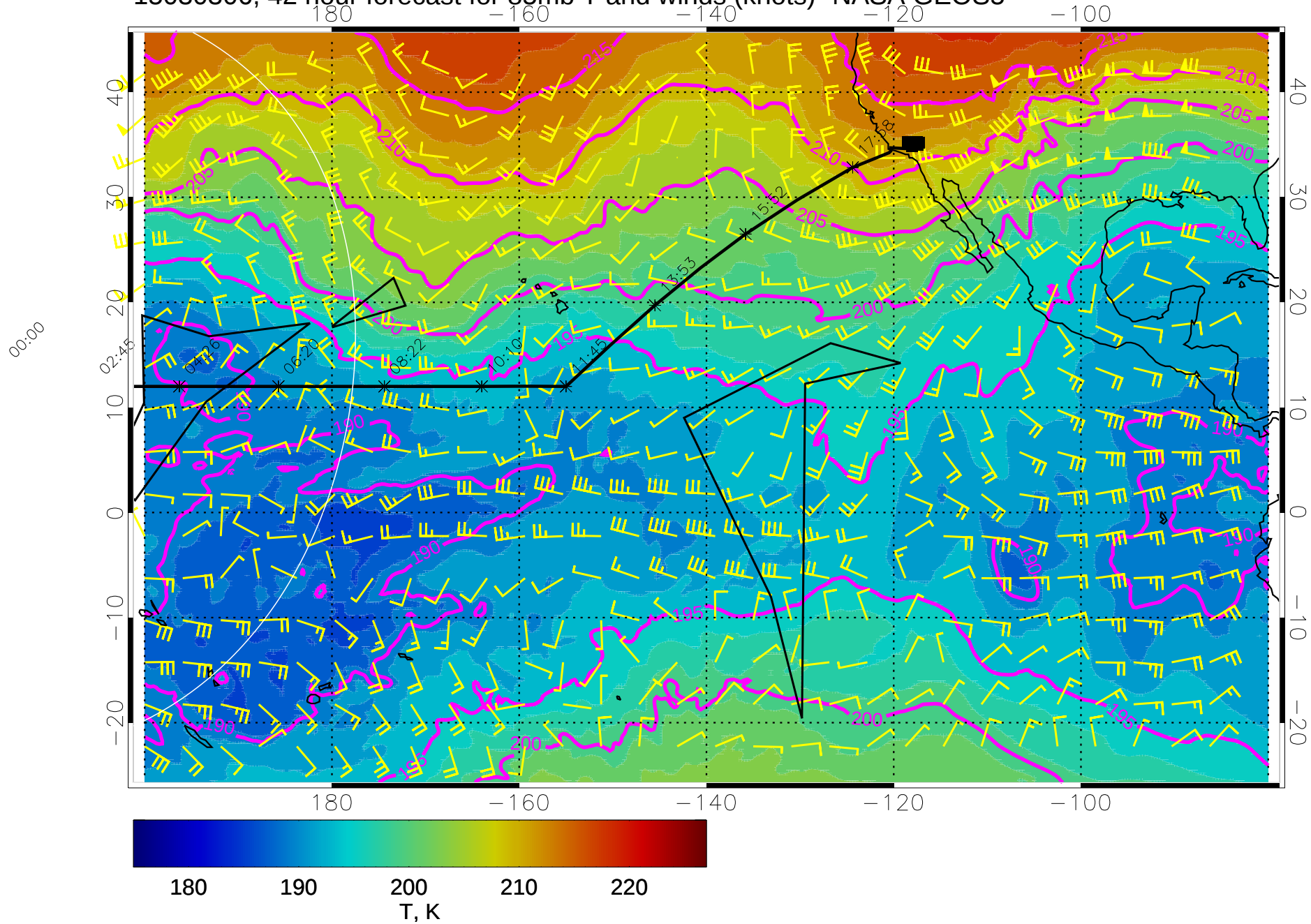
15030306, 42 hour forecast for 85mb T and winds (knots)- NASA GEOS5
