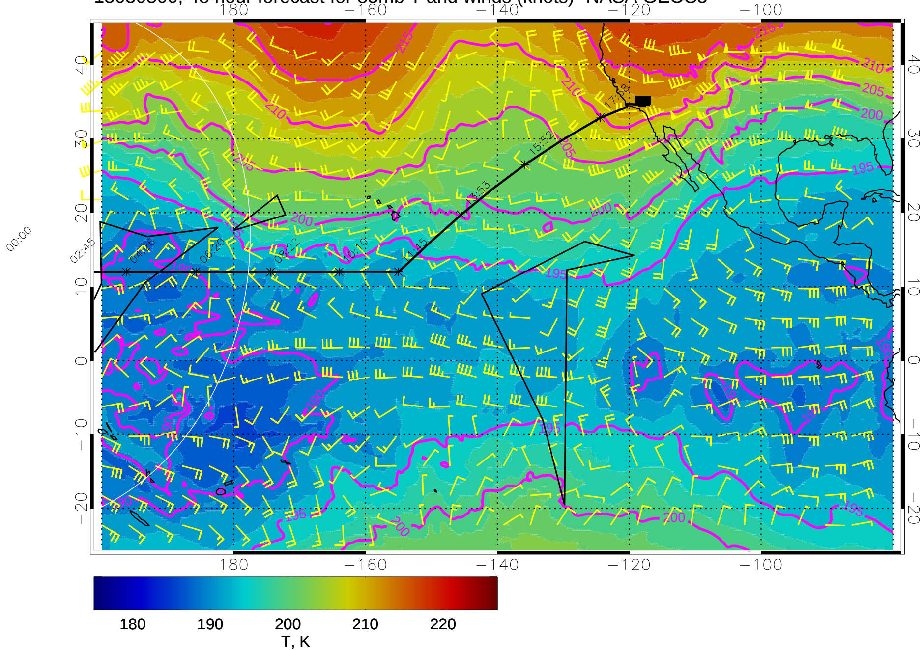
15030300, 48 hour forecast for 85mb T and winds (knots)- NASA GEOS5
