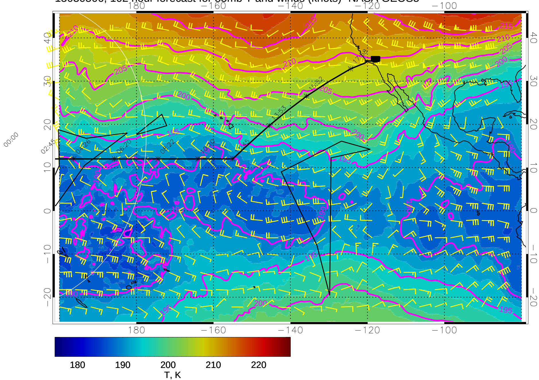
15030506, 102 hour forecast for 85mb T and winds (knots)- NASA GEOS5
