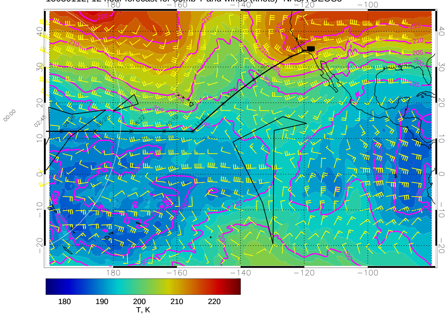
15030112, 12 hour forecast for 85mb T and winds (knots)- NASA GEOS5
