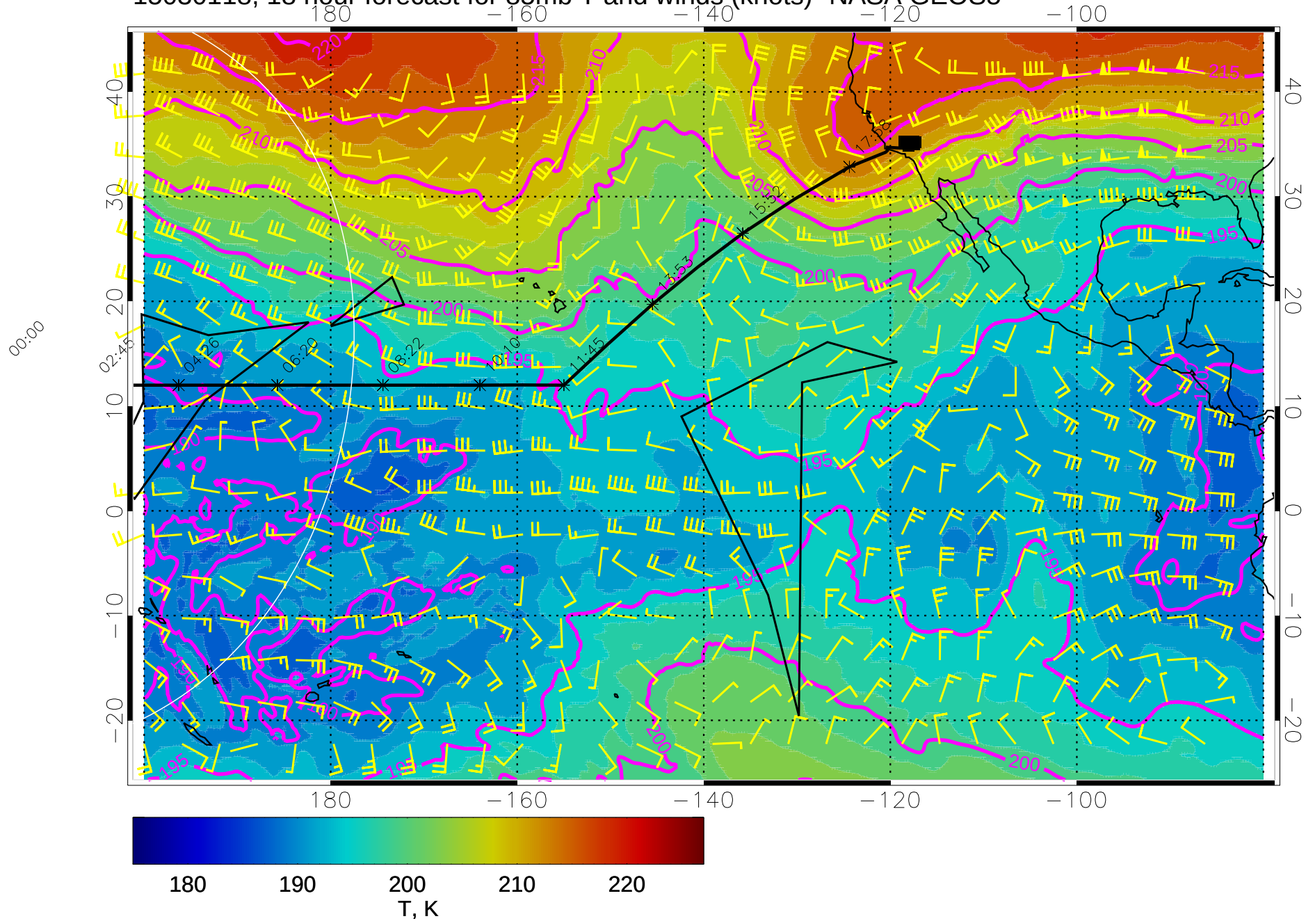
15030118, 18 hour forecast for 85mb T and winds (knots)- NASA GEOS5
