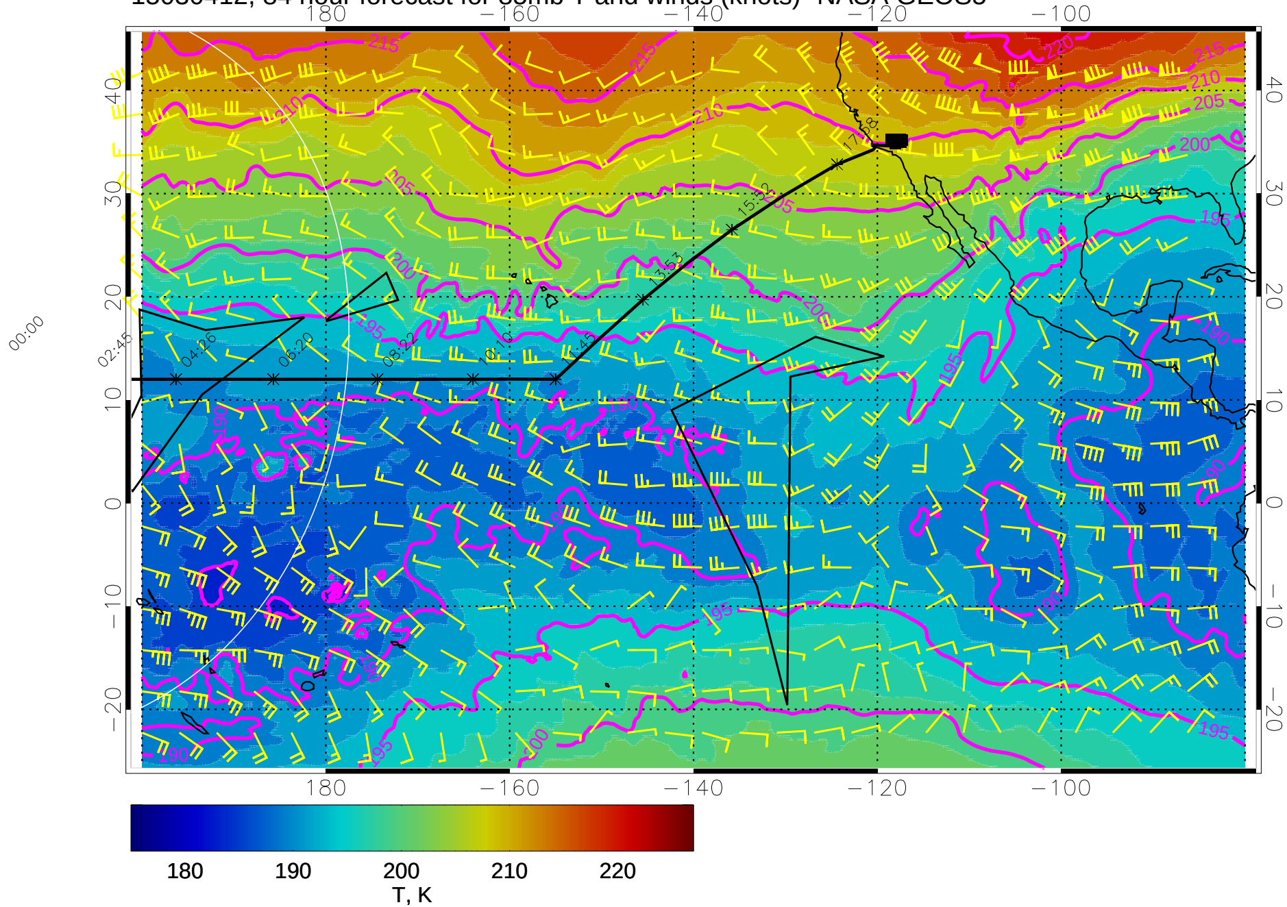
15030412, 84 hour forecast for 85mb T and winds (knots)- NASA GEOS5
