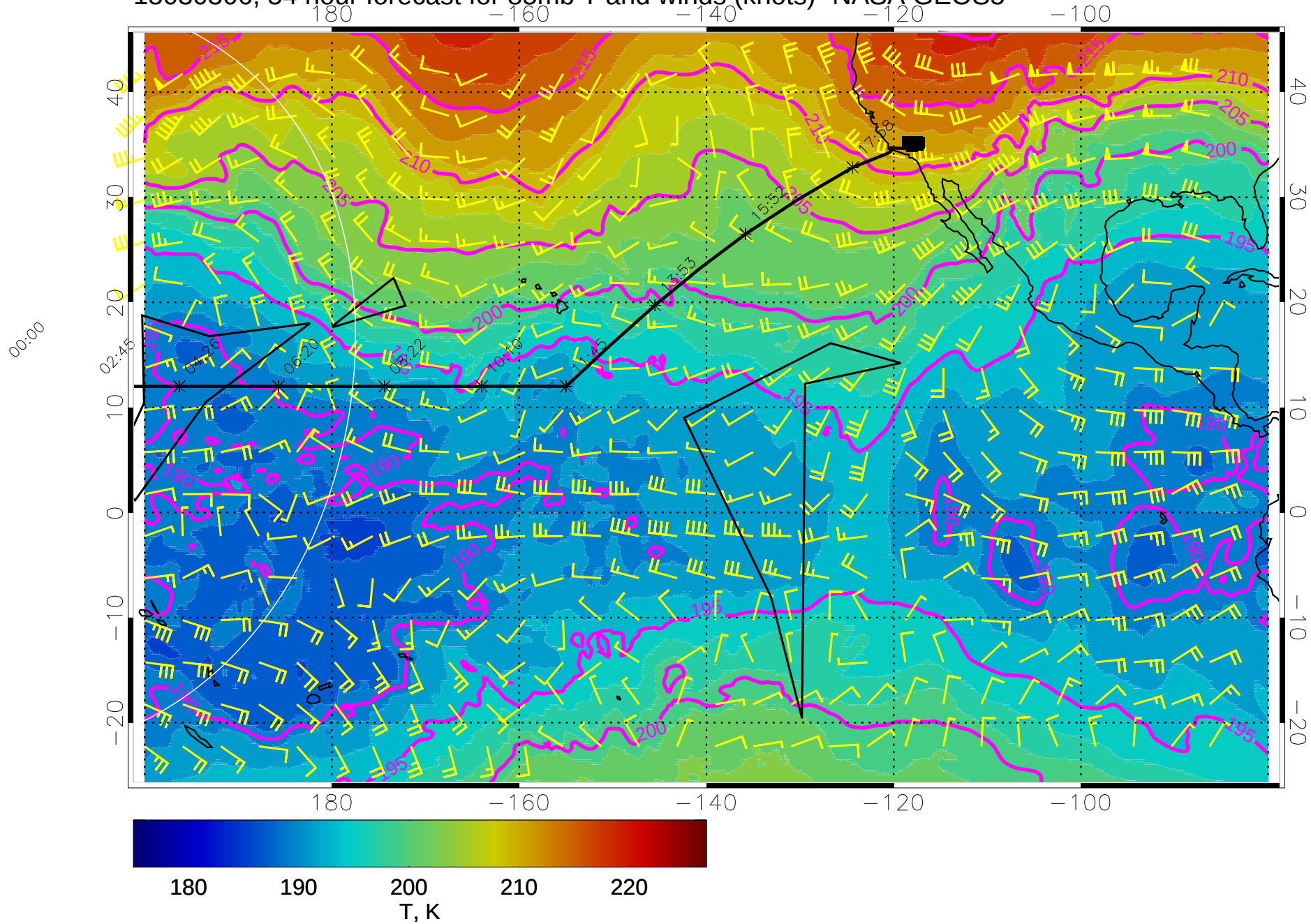
15030306, 54 hour forecast for 85mb T and winds (knots)- NASA GEOS5
