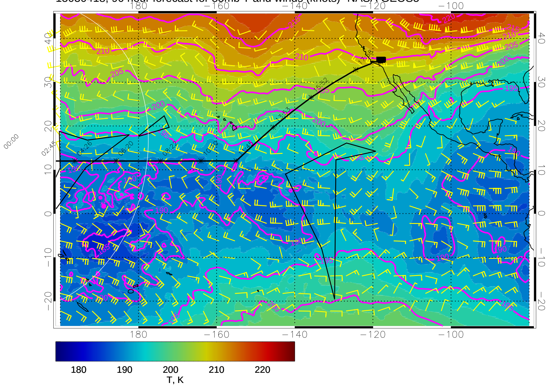
15030418, 90 hour forecast for 85mb T and winds (knots)- NASA GEOS5
