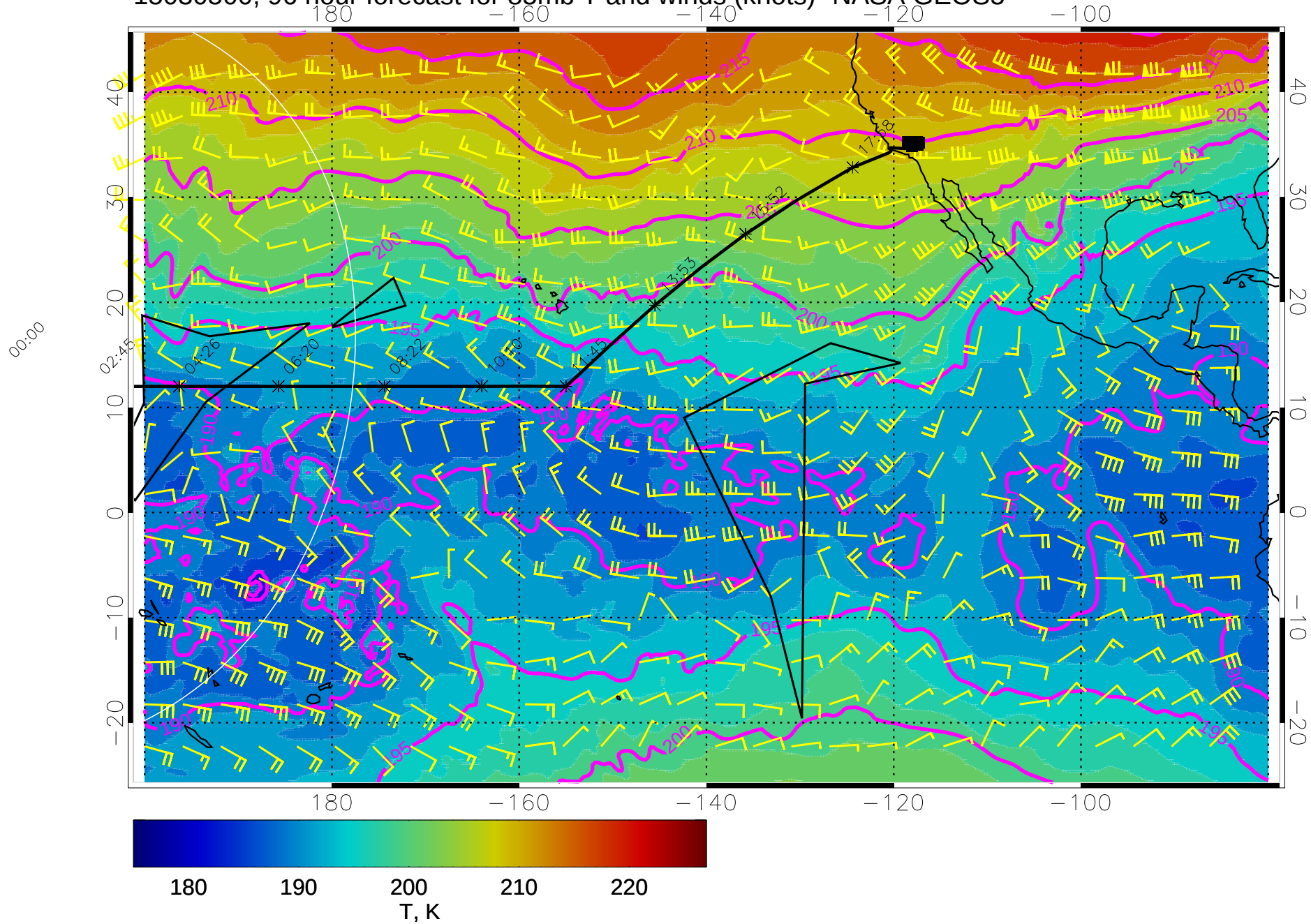
15030500, 96 hour forecast for 85mb T and winds (knots)- NASA GEOS5
