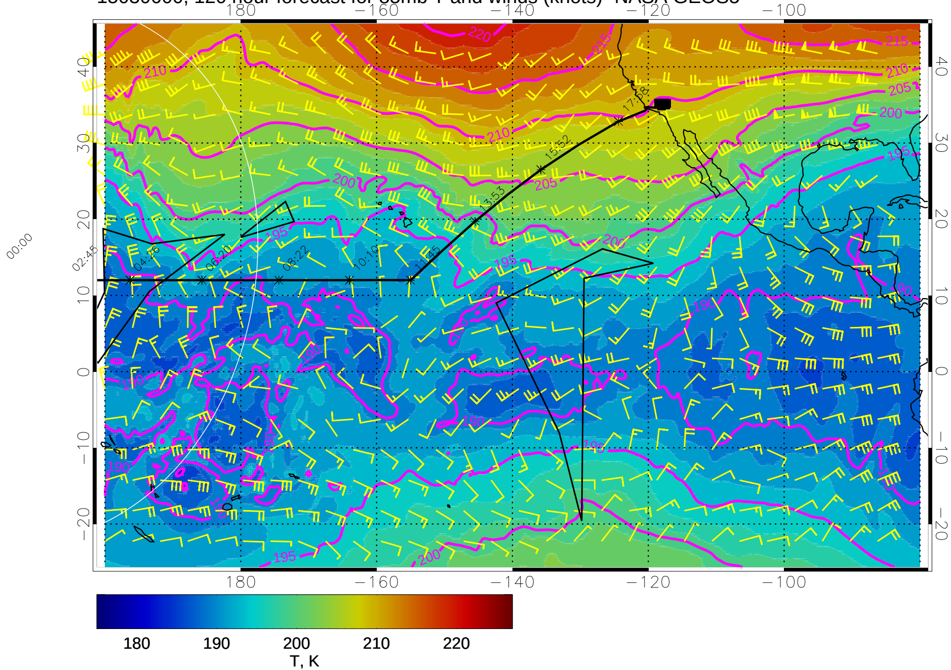
15030600, 120 hour forecast for 85mb T and winds (knots)- NASA GEOS5
