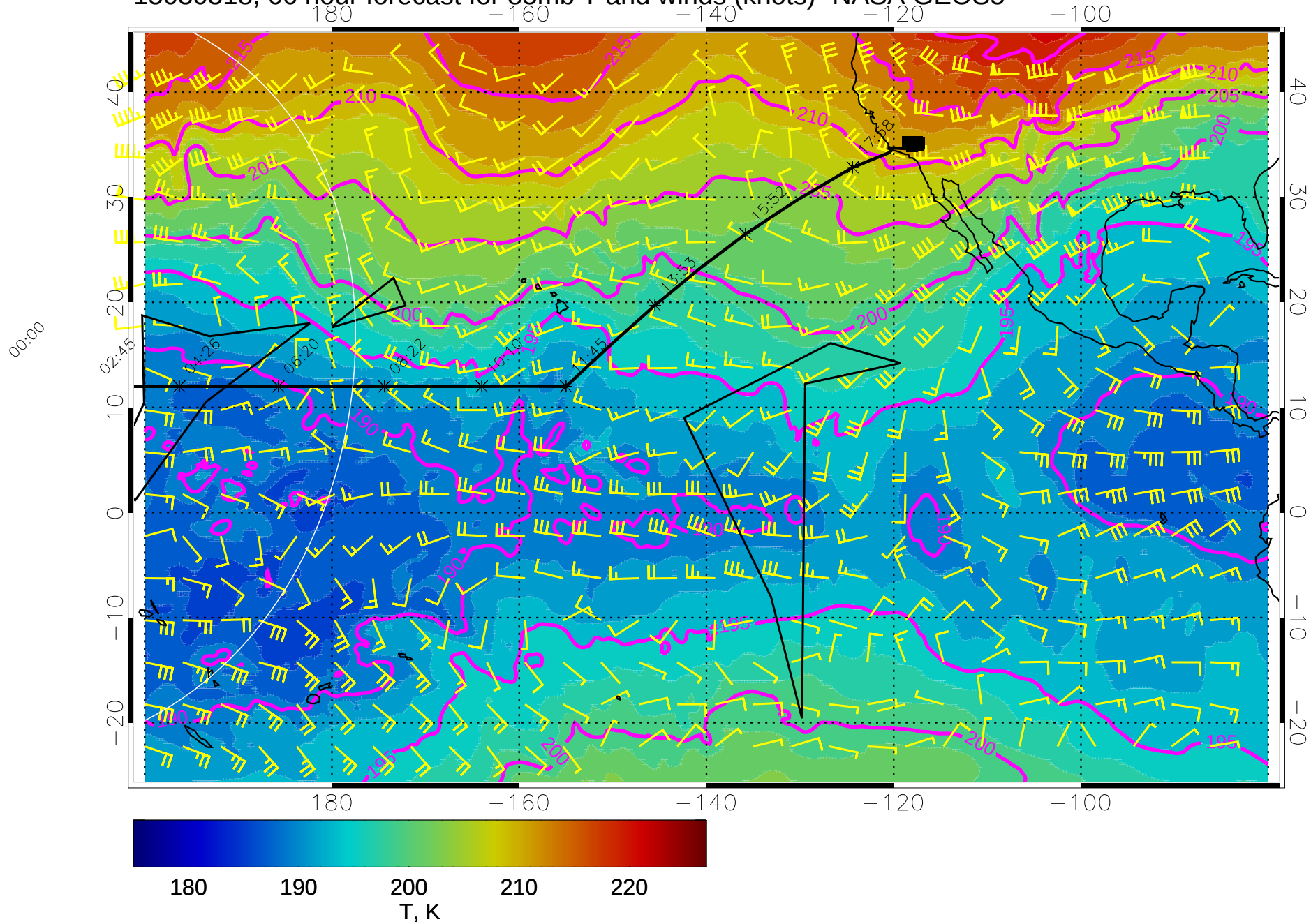
15030318, 66 hour forecast for 85mb T and winds (knots)- NASA GEOS5
