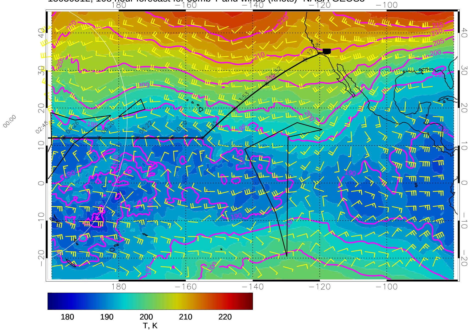
15030512, 108 hour forecast for 85mb T and winds (knots)- NASA GEOS5
