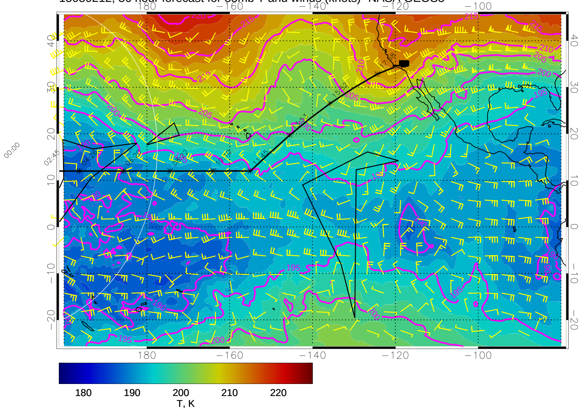
15030212, 36 hour forecast for 85mb T and winds (knots)- NASA GEOS5
