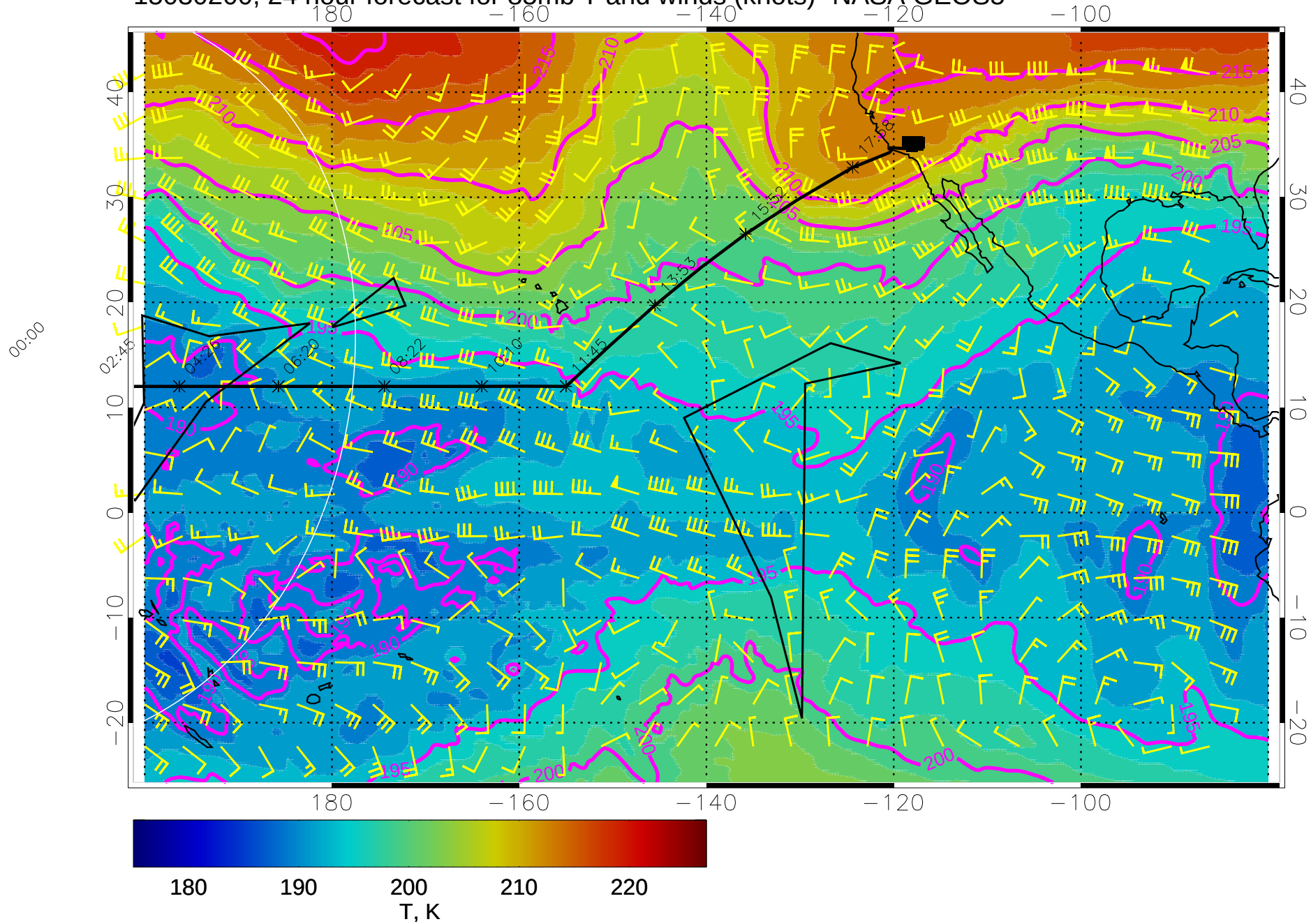
15030200, 24 hour forecast for 85mb T and winds (knots)- NASA GEOS5
