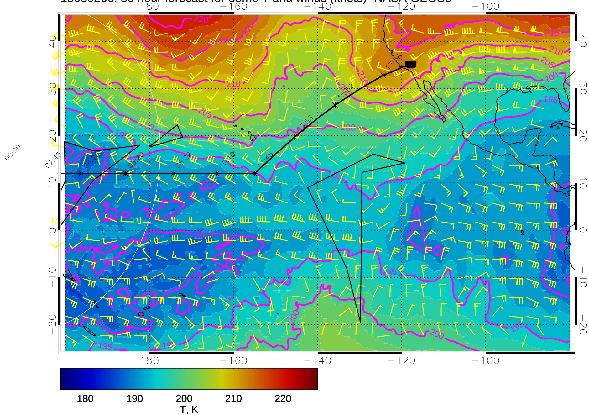
15030206, 30 hour forecast for 85mb T and winds (knots)- NASA GEOS5
