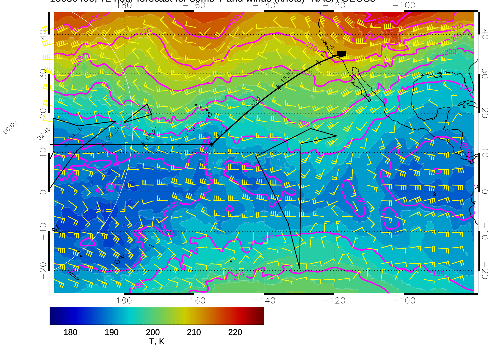
15030400, 72 hour forecast for 85mb T and winds (knots)- NASA GEOS5
