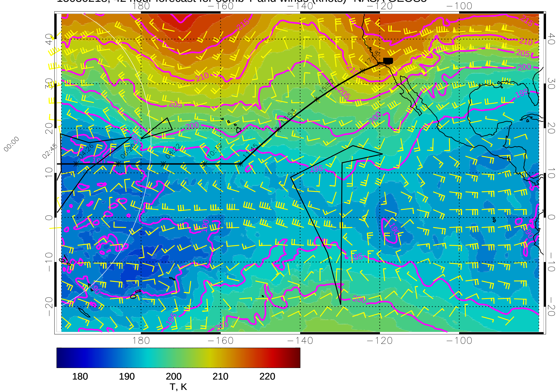
15030218, 42 hour forecast for 85mb T and winds (knots)- NASA GEOS5
