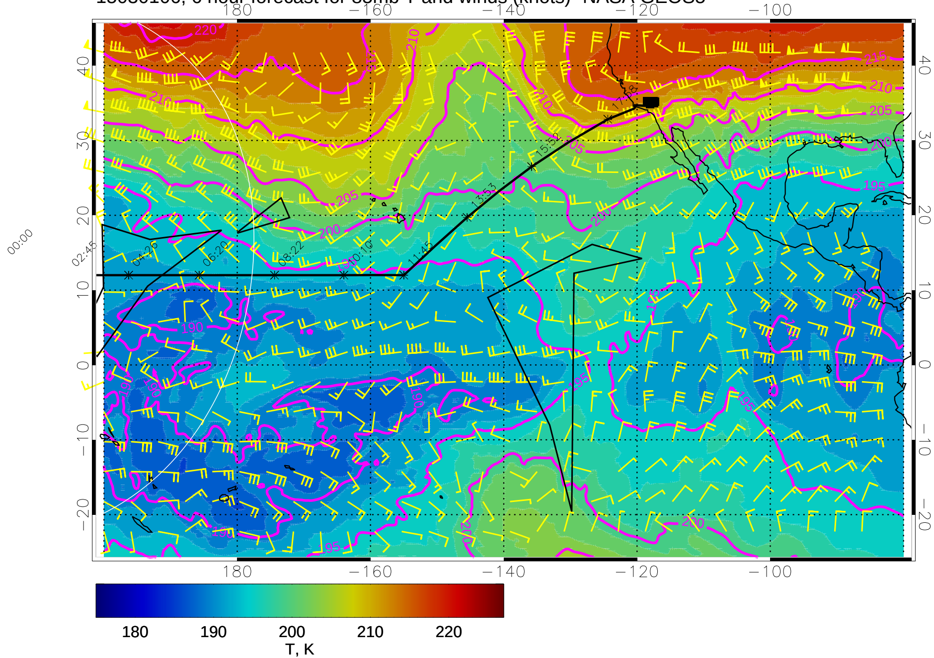
15030106, 6 hour forecast for 85mb T and winds (knots)- NASA GEOS5
