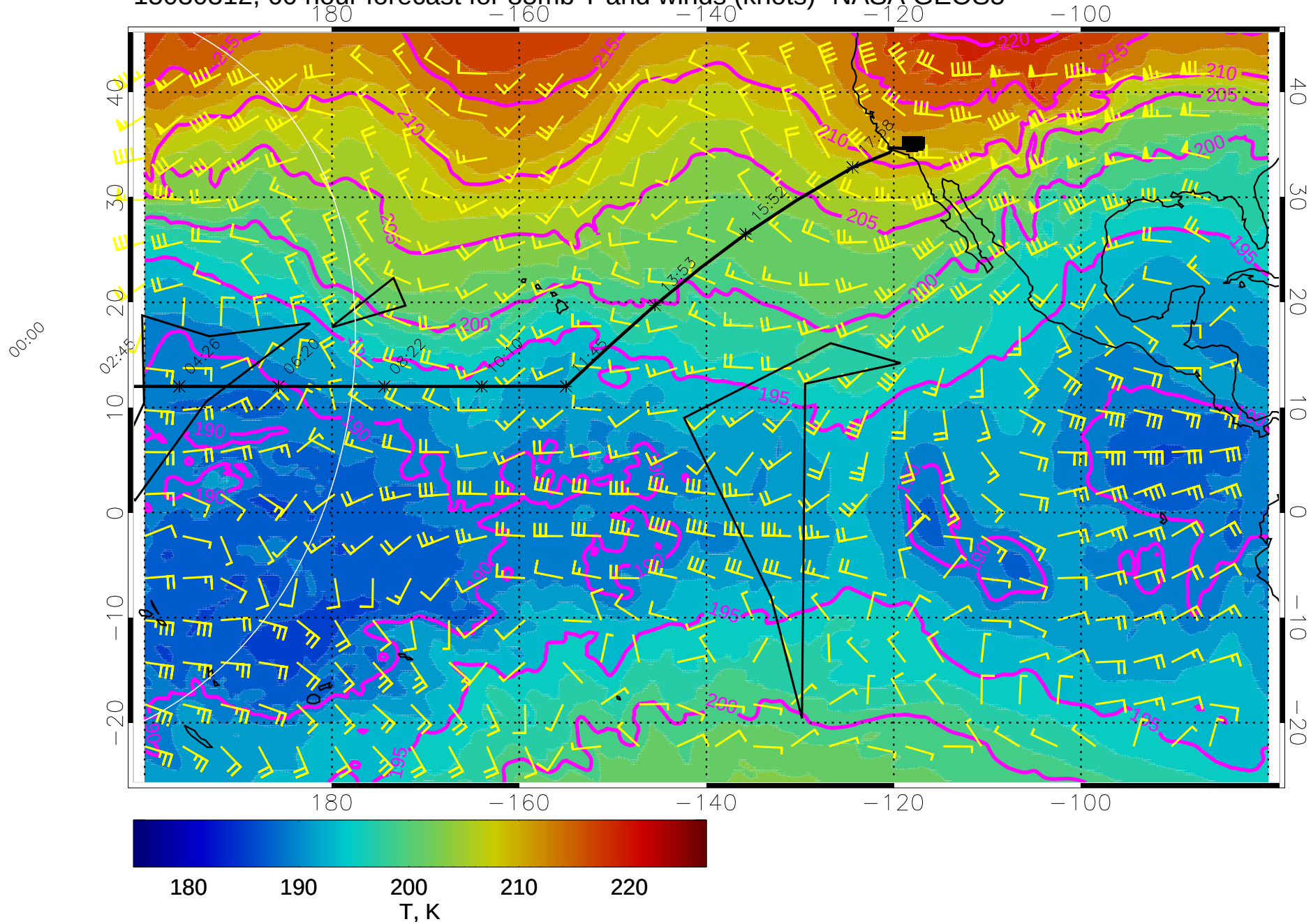
15030312, 60 hour forecast for 85mb T and winds (knots)- NASA GEOS5
