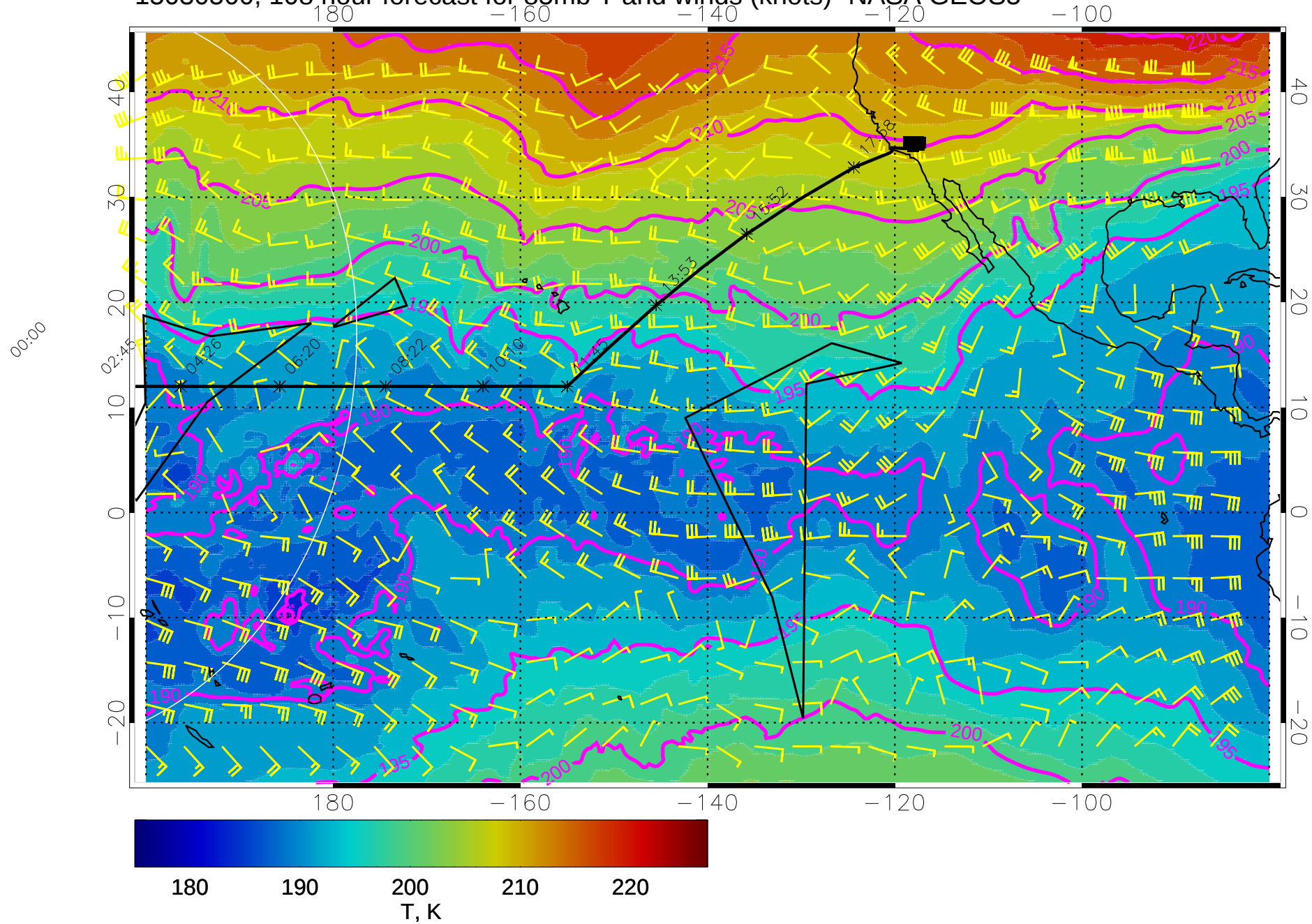
15030500, 108 hour forecast for 85mb T and winds (knots)- NASA GEOS5
