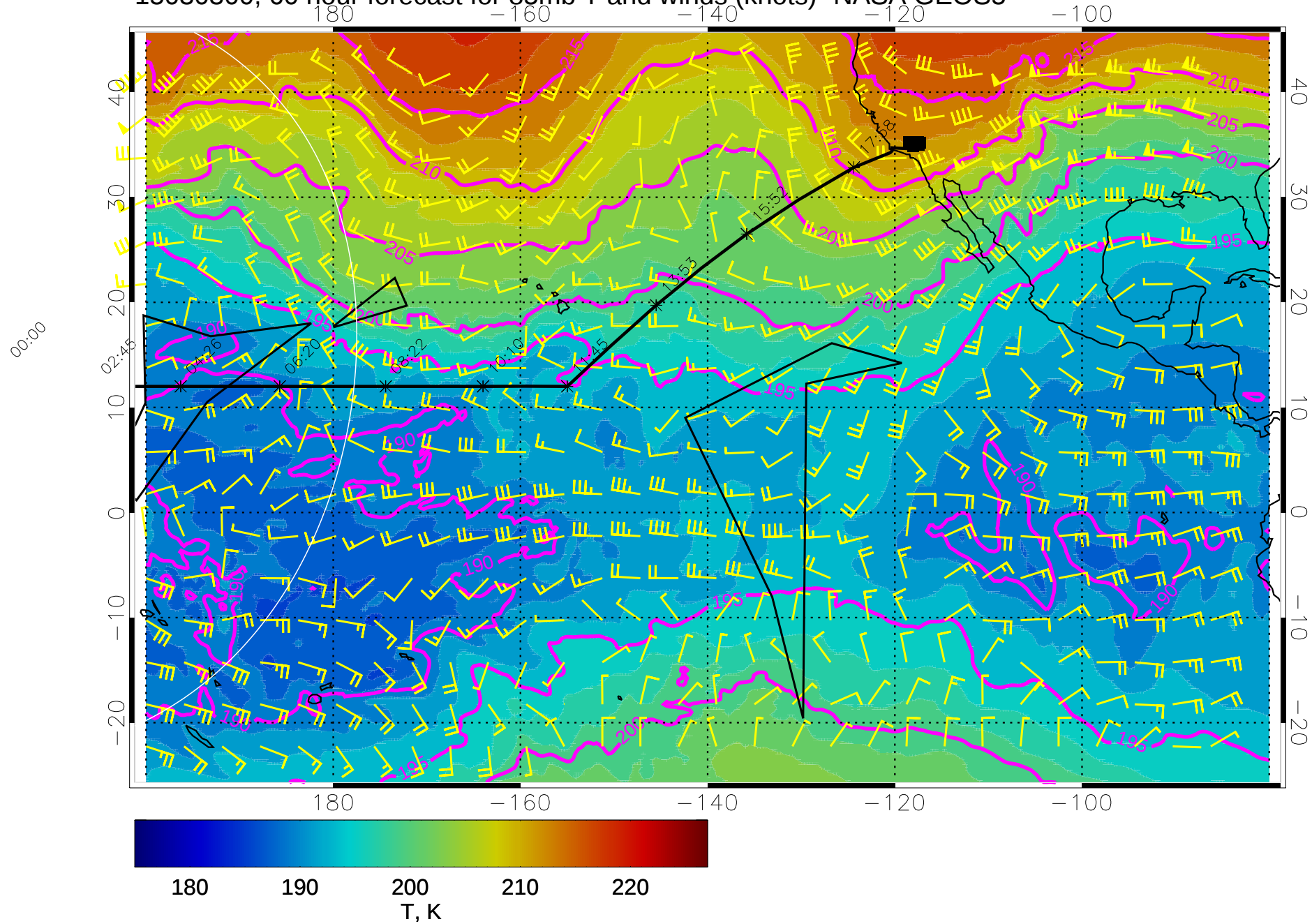
15030300, 60 hour forecast for 85mb T and winds (knots)- NASA GEOS5
