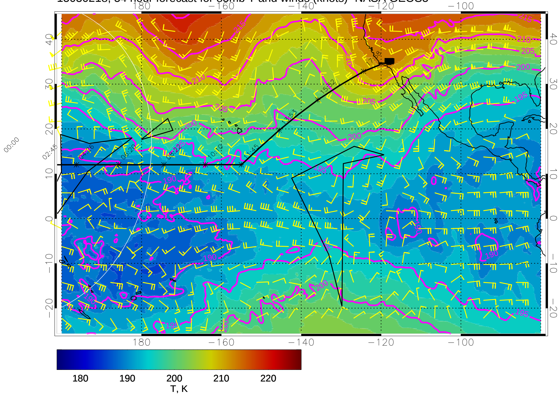
15030218, 54 hour forecast for 85mb T and winds (knots)- NASA GEOS5
