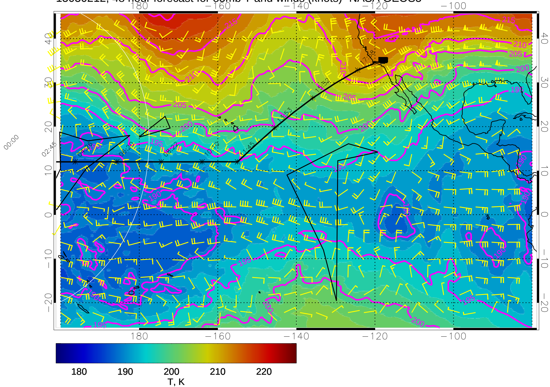
15030212, 48 hour forecast for 85mb T and winds (knots)- NASA GEOS5
