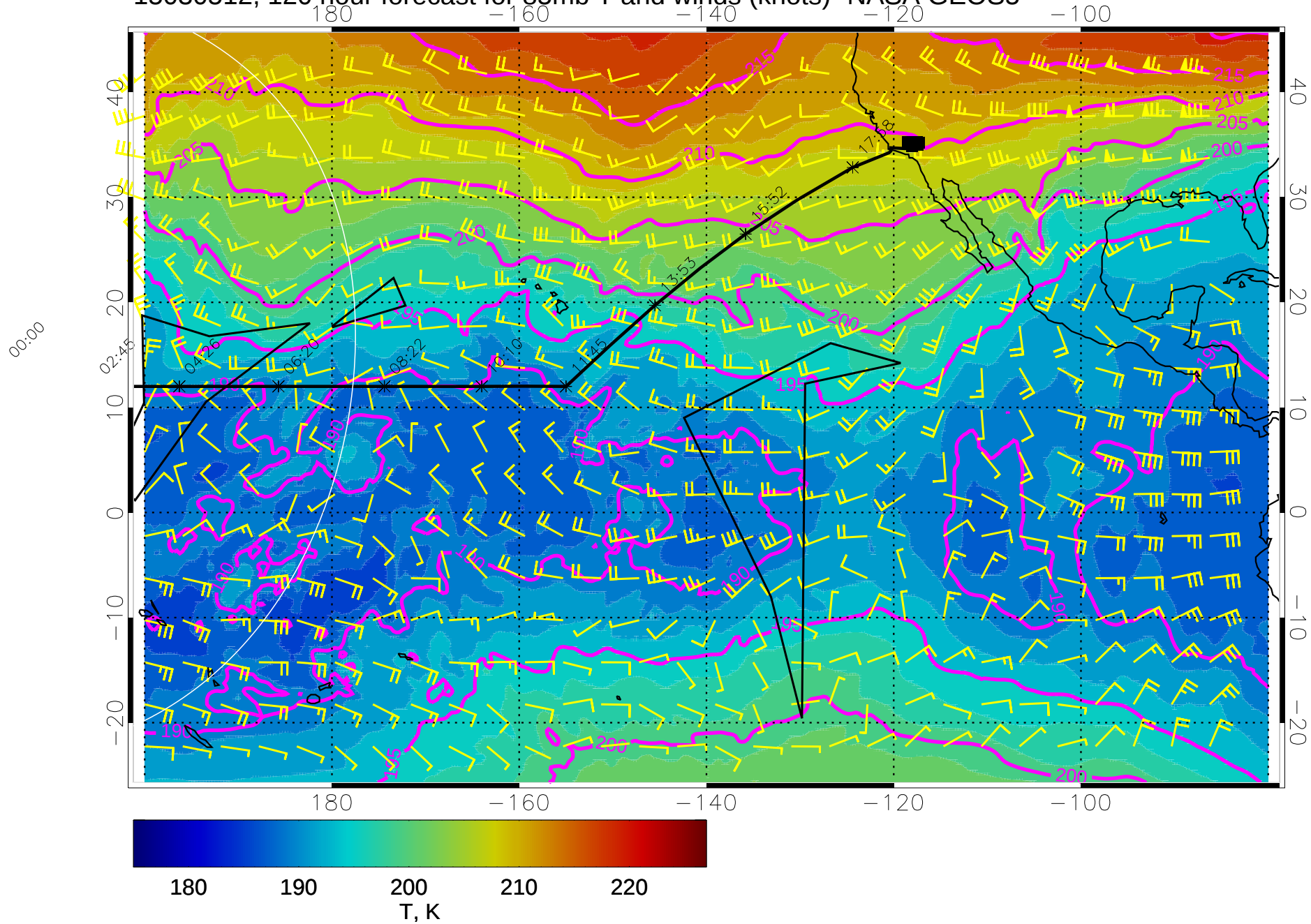
15030512, 120 hour forecast for 85mb T and winds (knots)- NASA GEOS5
