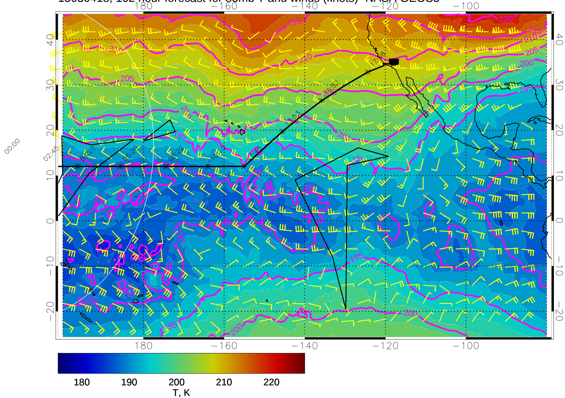
15030418, 102 hour forecast for 85mb T and winds (knots)- NASA GEOS5
