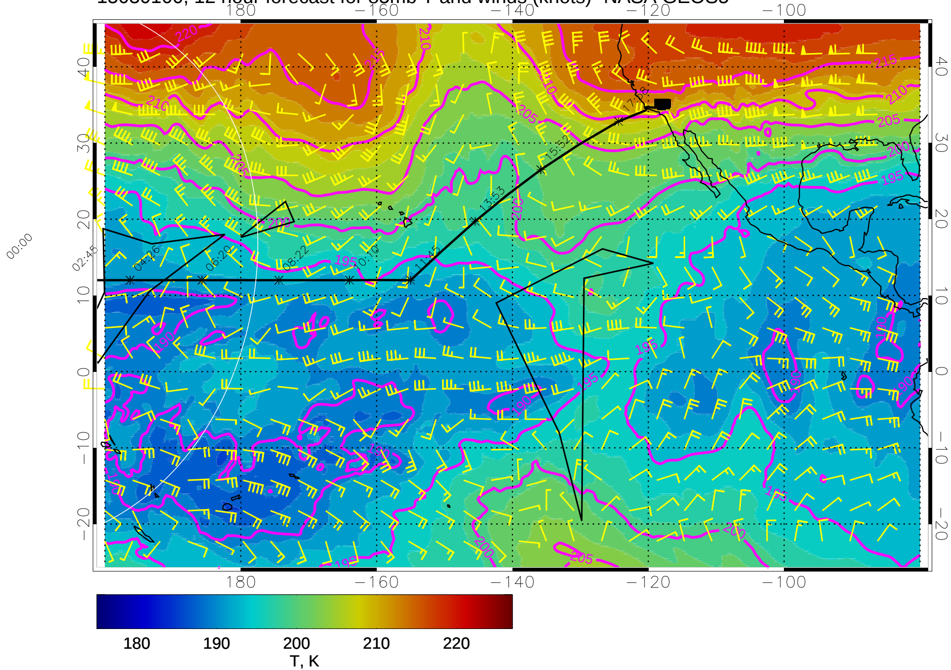
15030100, 12 hour forecast for 85mb T and winds (knots)- NASA GEOS5
