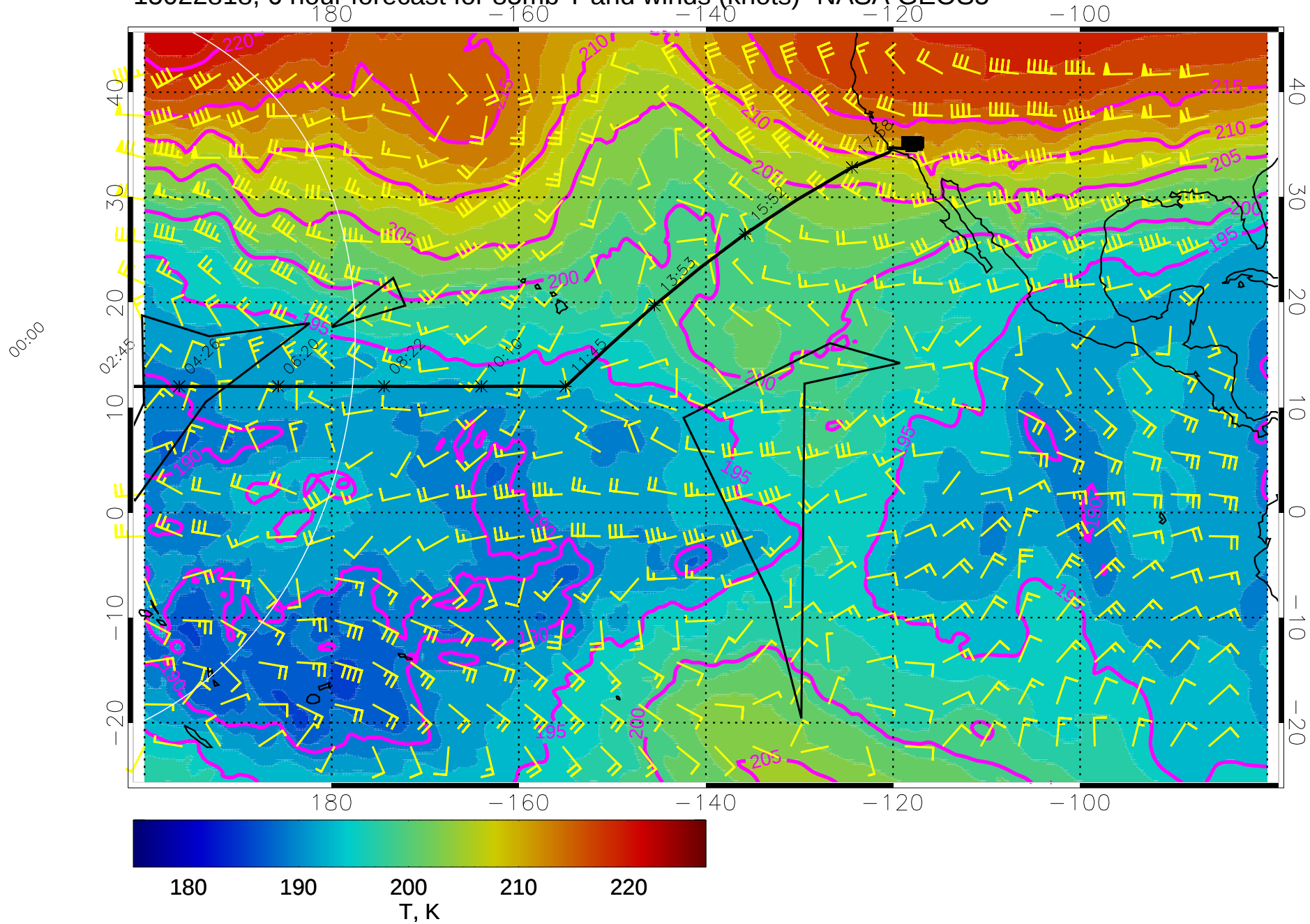
15022818, 6 hour forecast for 85mb T and winds (knots)- NASA GEOS5
