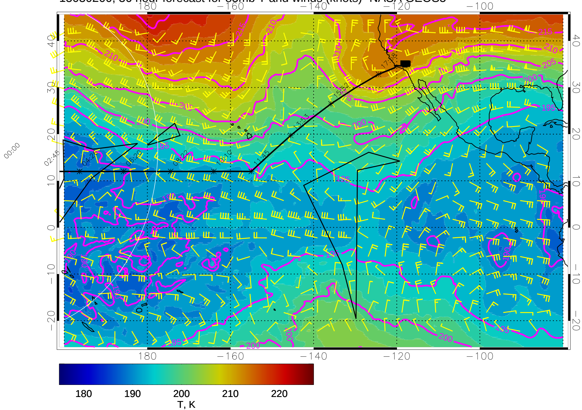
15030200, 36 hour forecast for 85mb T and winds (knots)- NASA GEOS5
