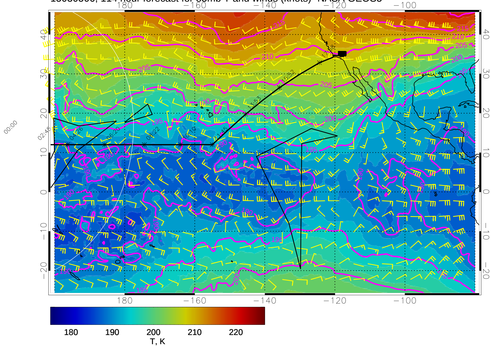
15030506, 114 hour forecast for 85mb T and winds (knots)- NASA GEOS5
