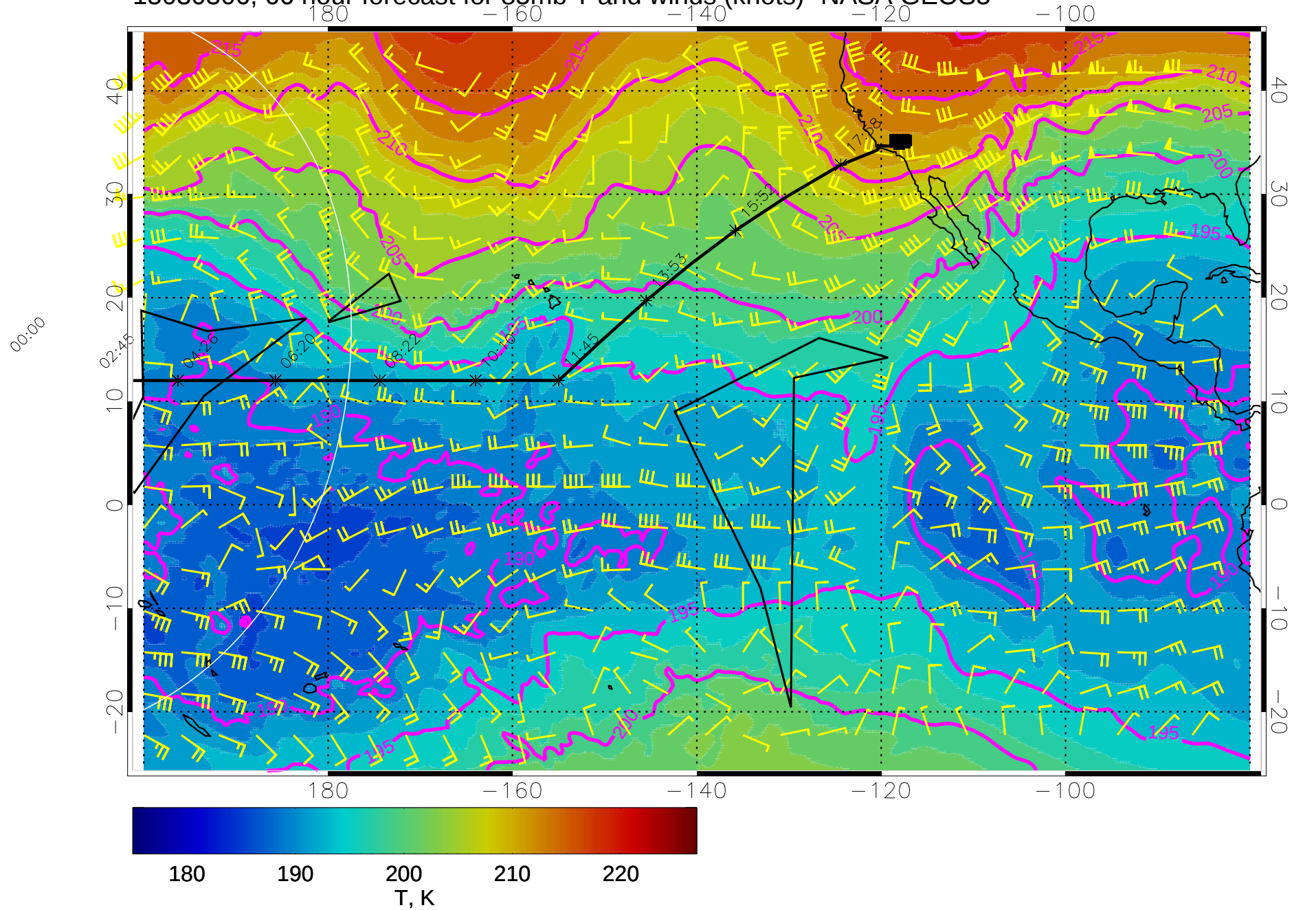
15030306, 66 hour forecast for 85mb T and winds (knots)- NASA GEOS5
