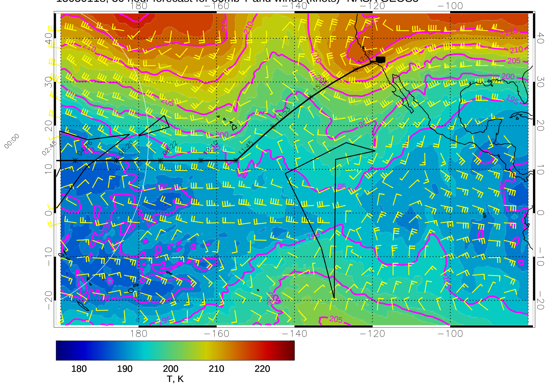
15030118, 30 hour forecast for 85mb T and winds (knots)- NASA GEOS5
