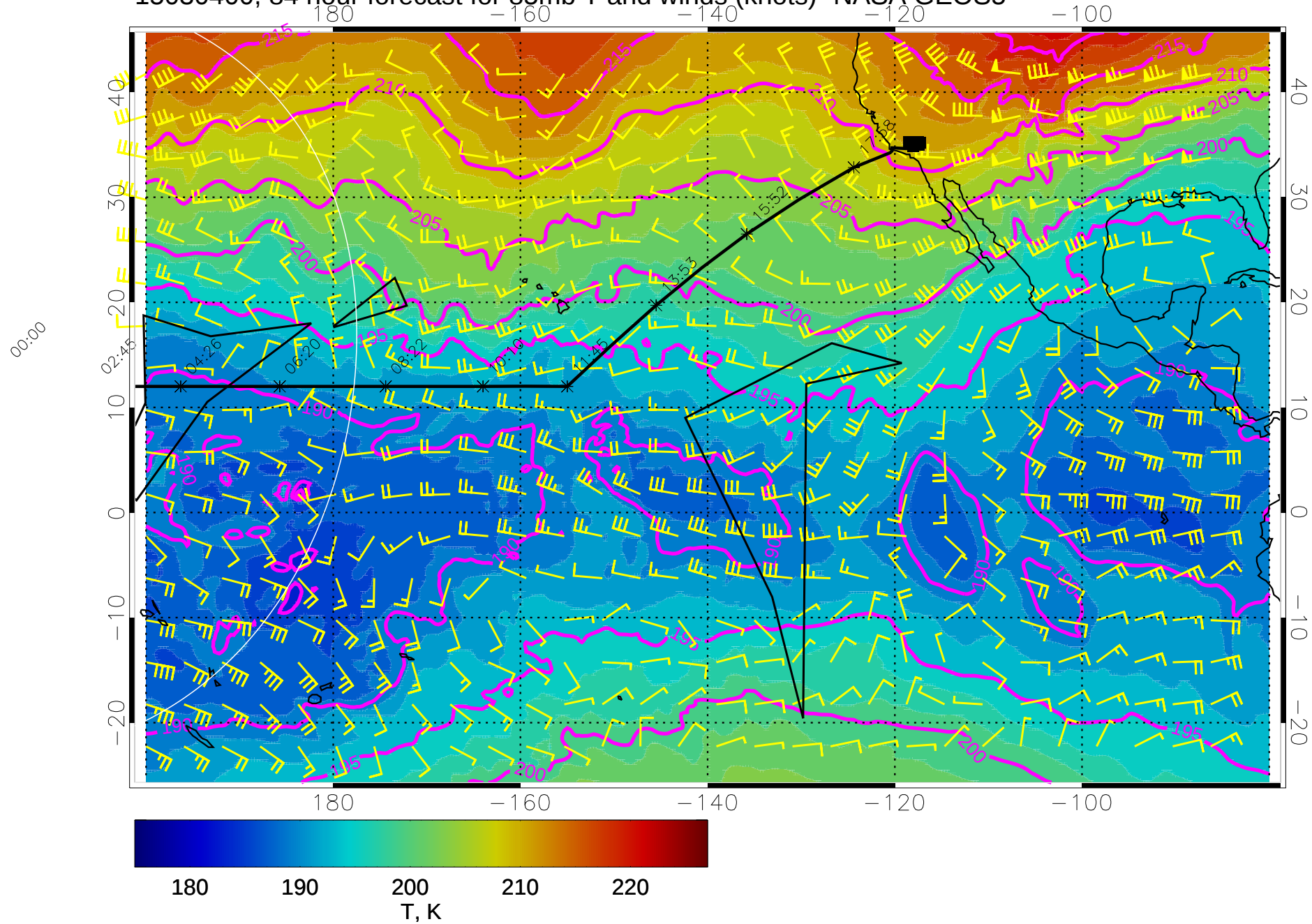
15030400, 84 hour forecast for 85mb T and winds (knots)- NASA GEOS5
