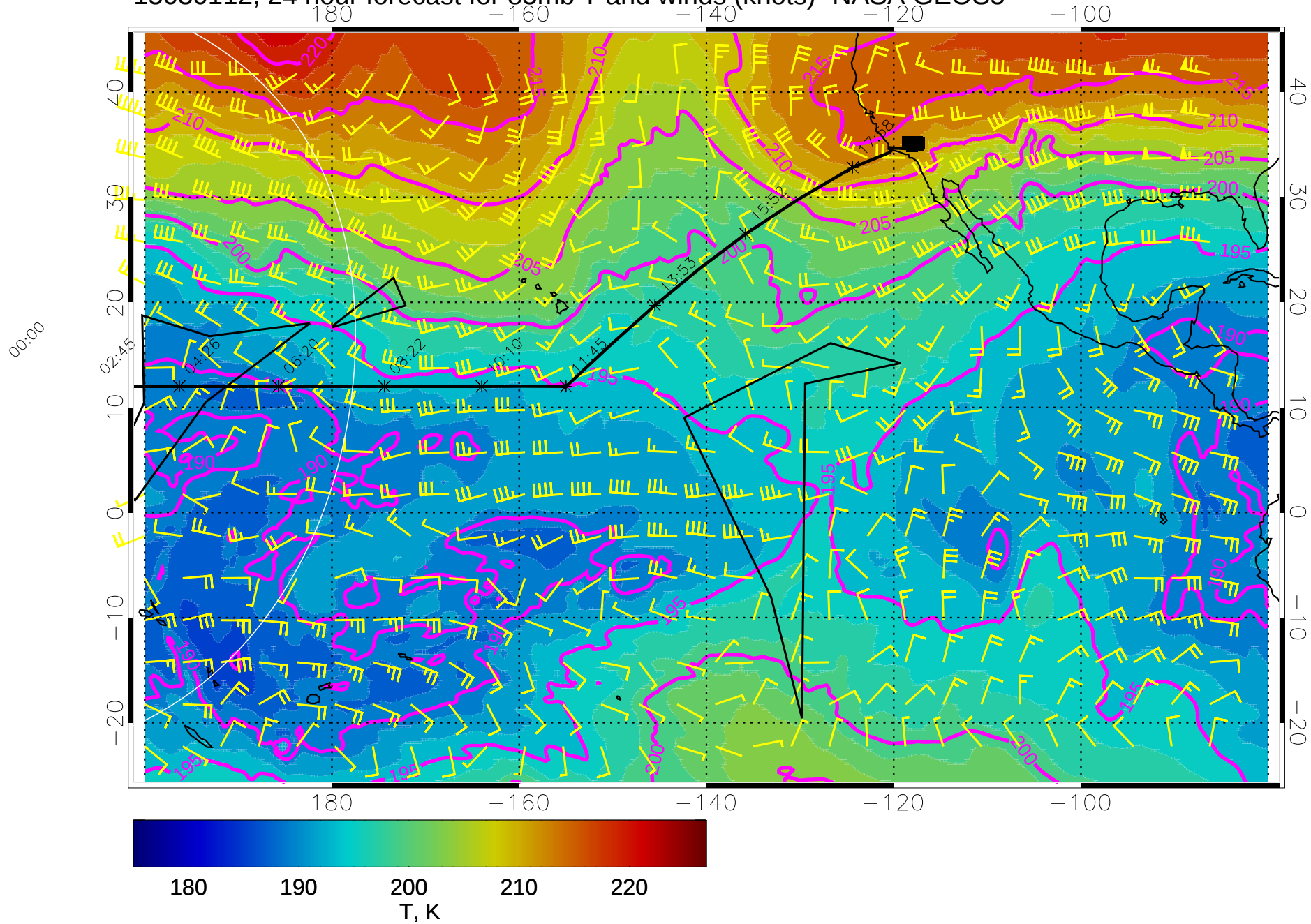
15030112, 24 hour forecast for 85mb T and winds (knots)- NASA GEOS5
