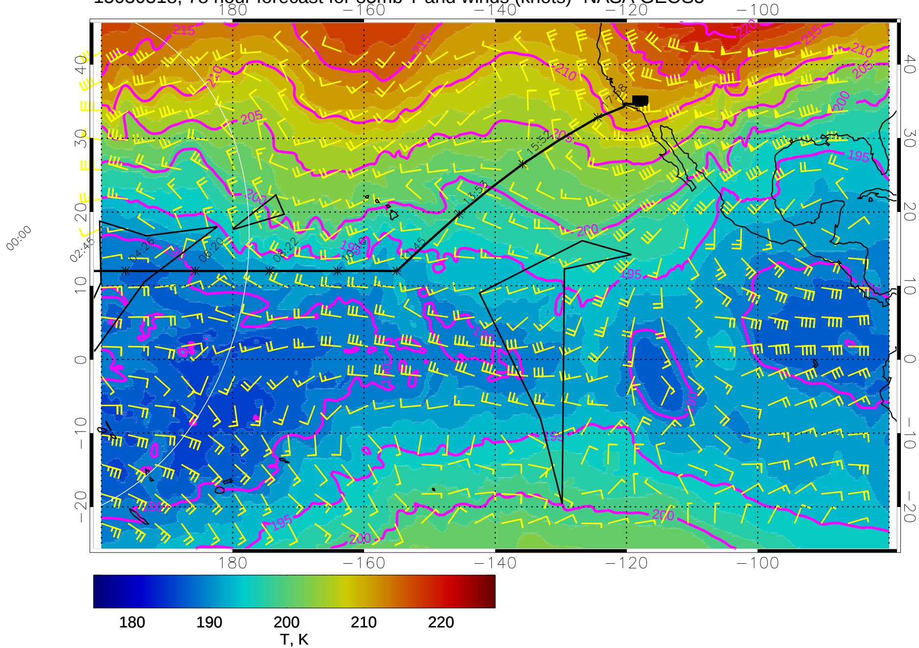
15030318, 78 hour forecast for 85mb T and winds (knots)- NASA GEOS5
