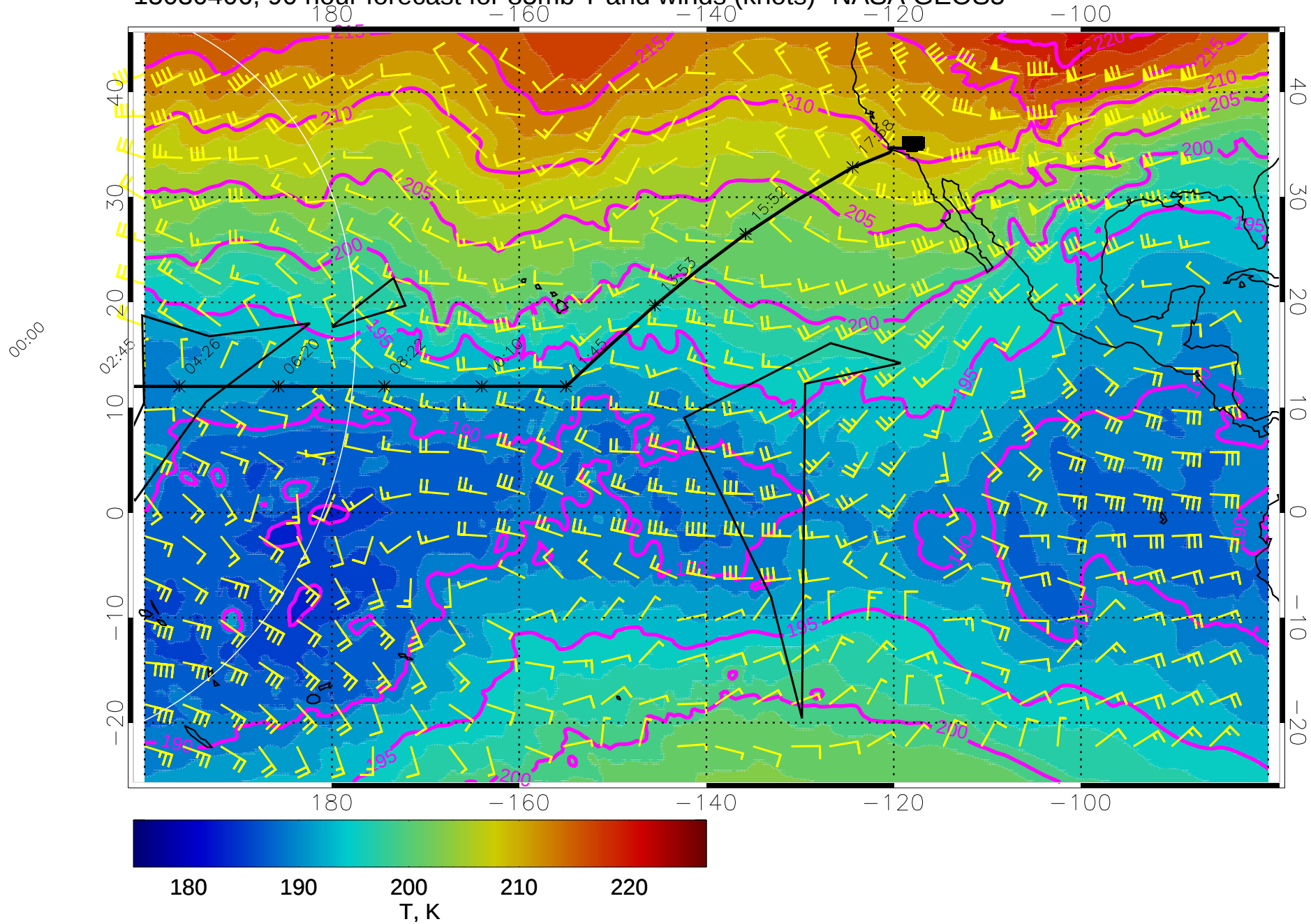
15030406, 90 hour forecast for 85mb T and winds (knots)- NASA GEOS5
