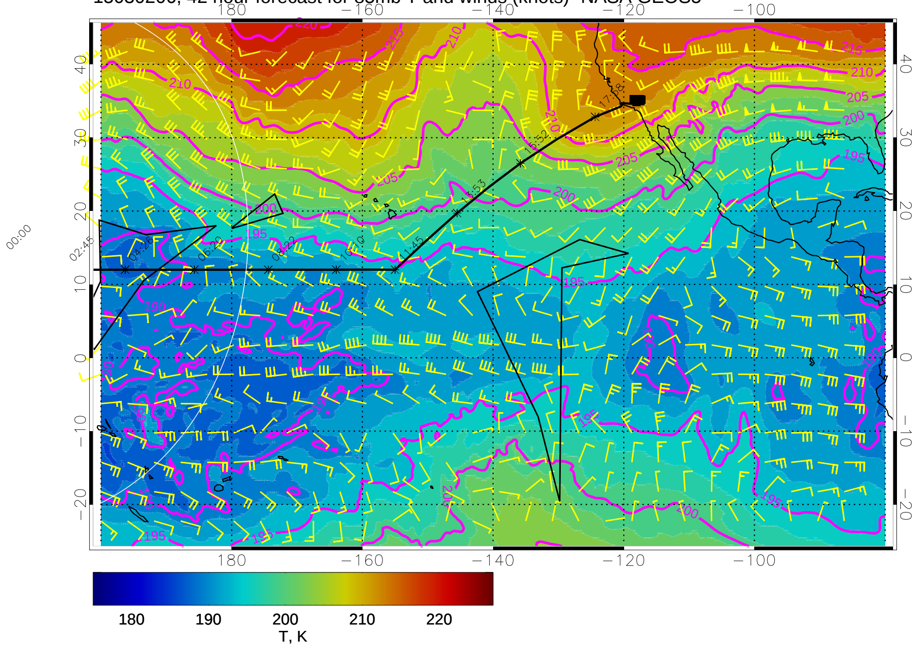
15030206, 42 hour forecast for 85mb T and winds (knots)- NASA GEOS5
