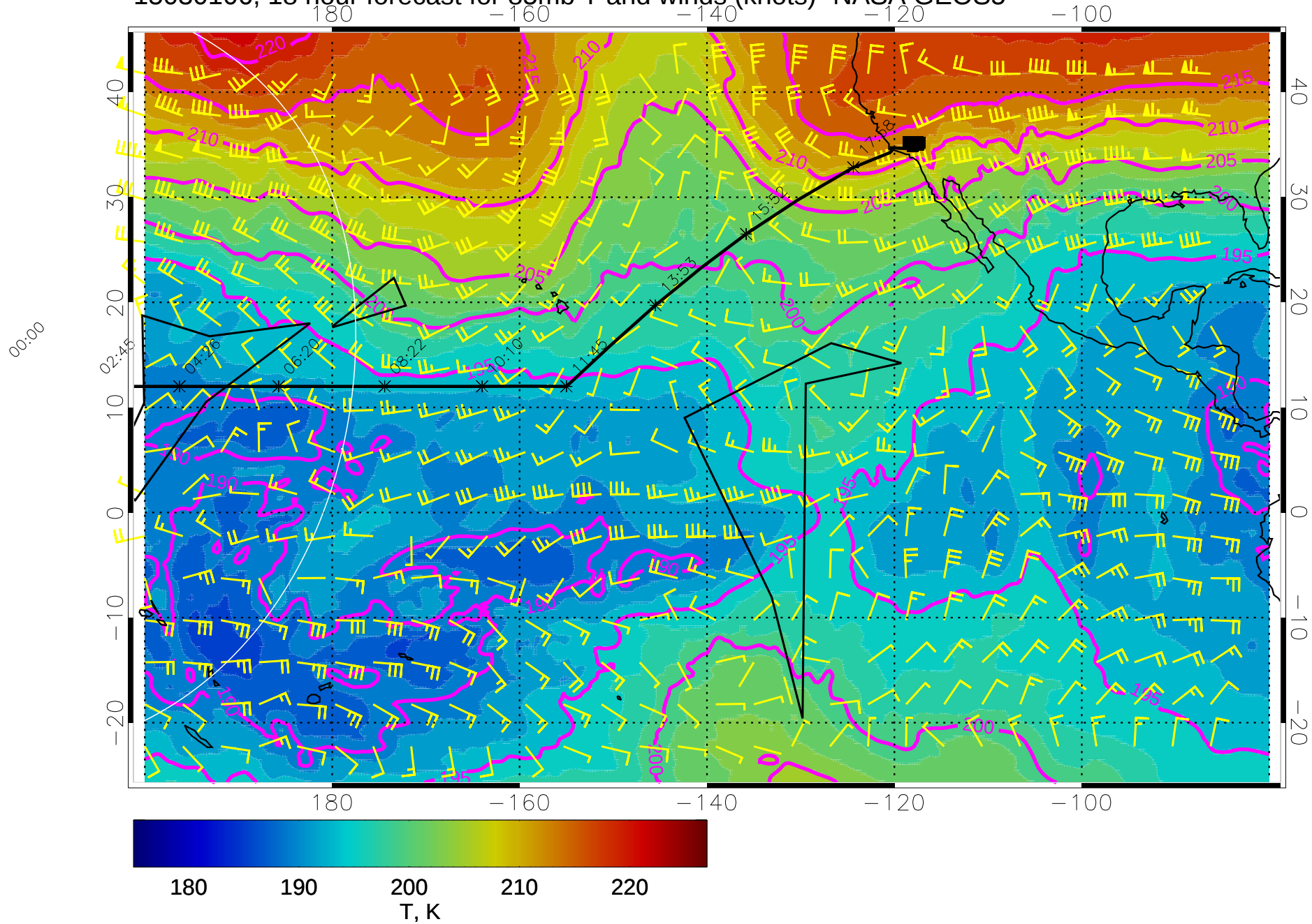
15030106, 18 hour forecast for 85mb T and winds (knots)- NASA GEOS5
