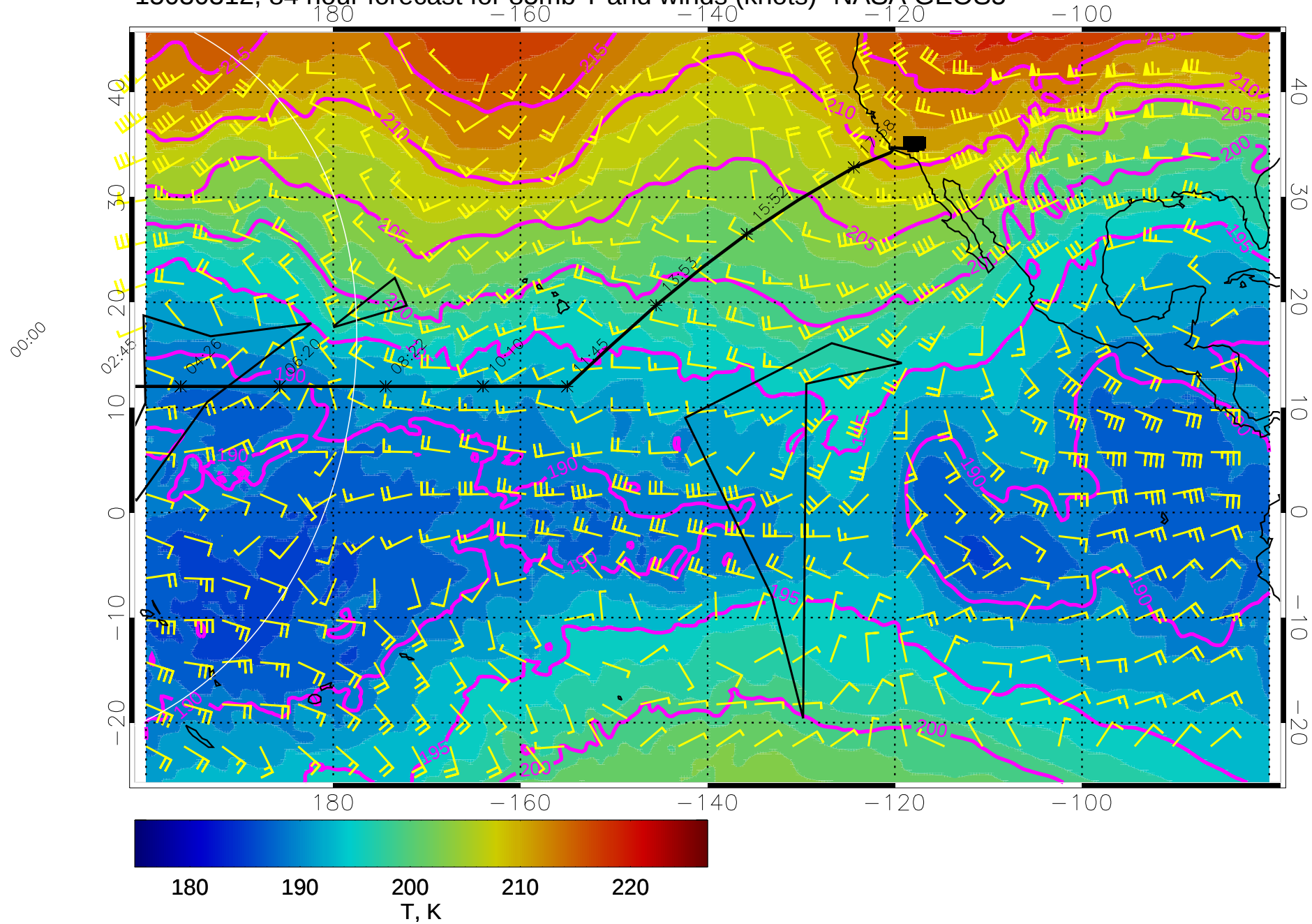
15030312, 84 hour forecast for 85mb T and winds (knots)- NASA GEOS5
