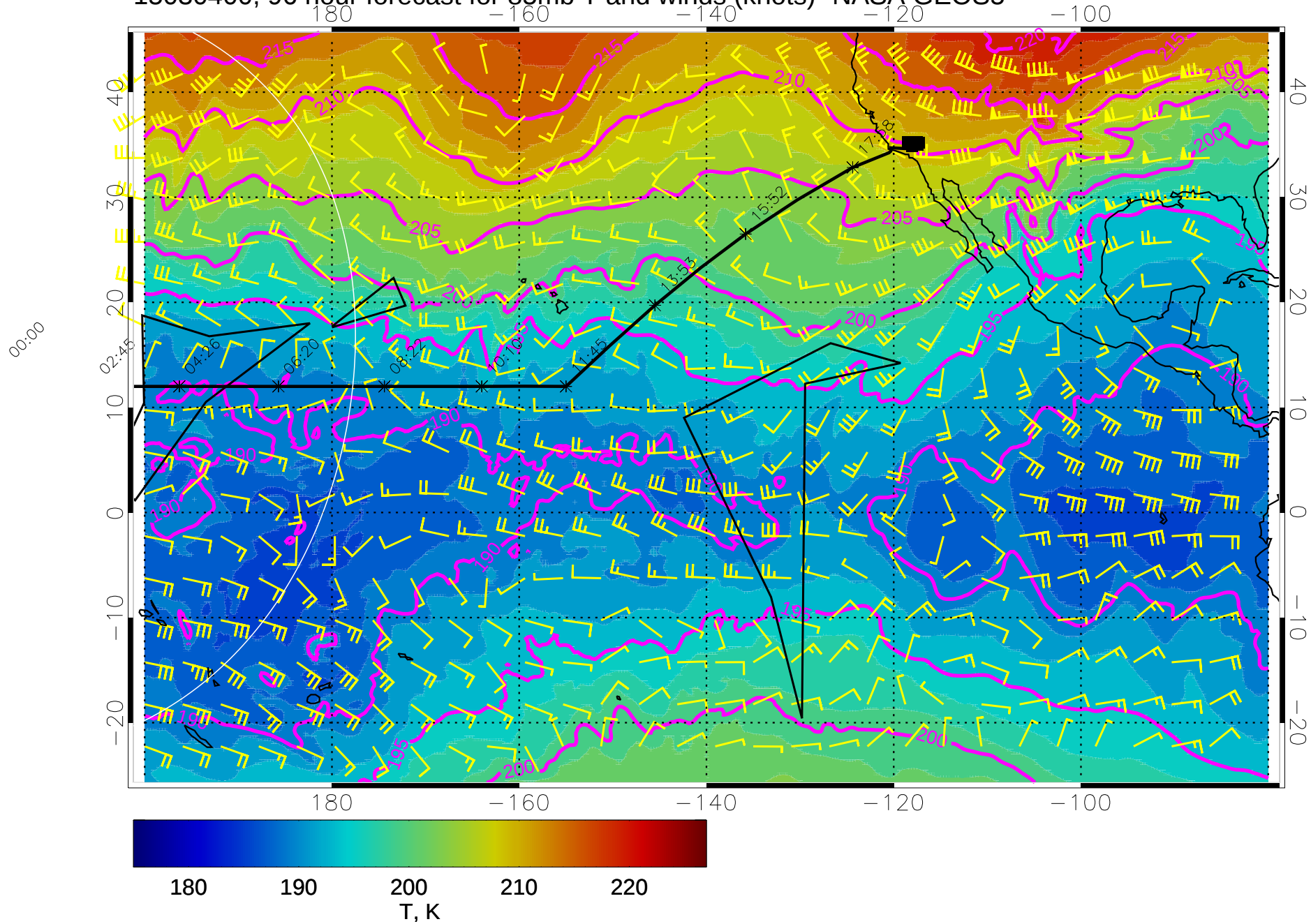
15030400, 96 hour forecast for 85mb T and winds (knots)- NASA GEOS5
