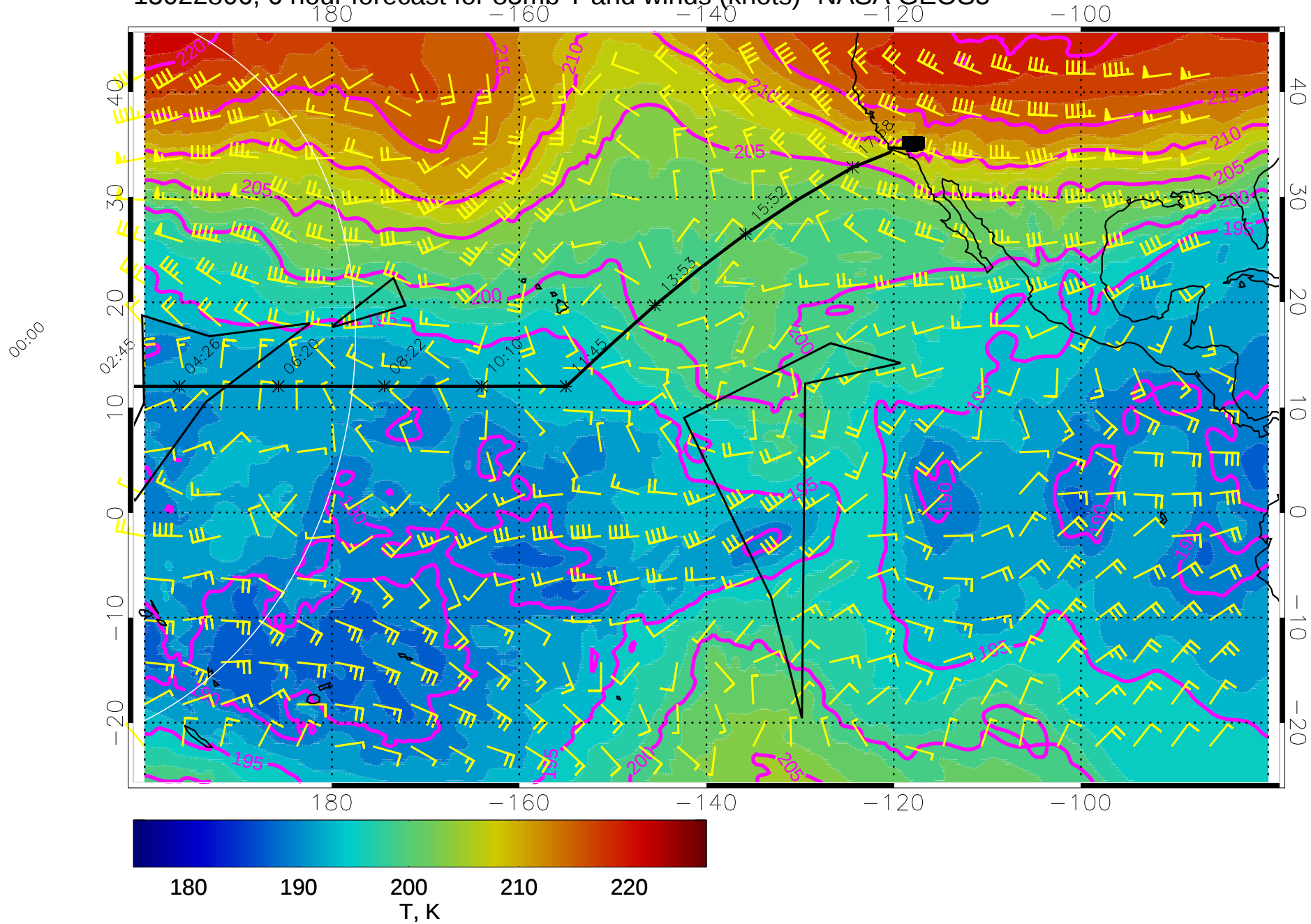
15022806, 6 hour forecast for 85mb T and winds (knots)- NASA GEOS5
