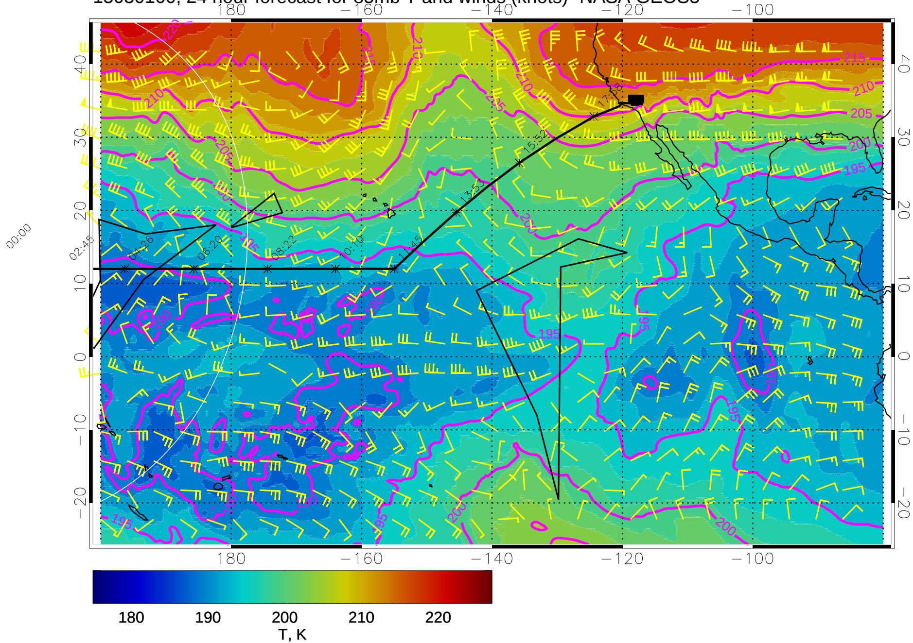
15030100, 24 hour forecast for 85mb T and winds (knots)- NASA GEOS5
