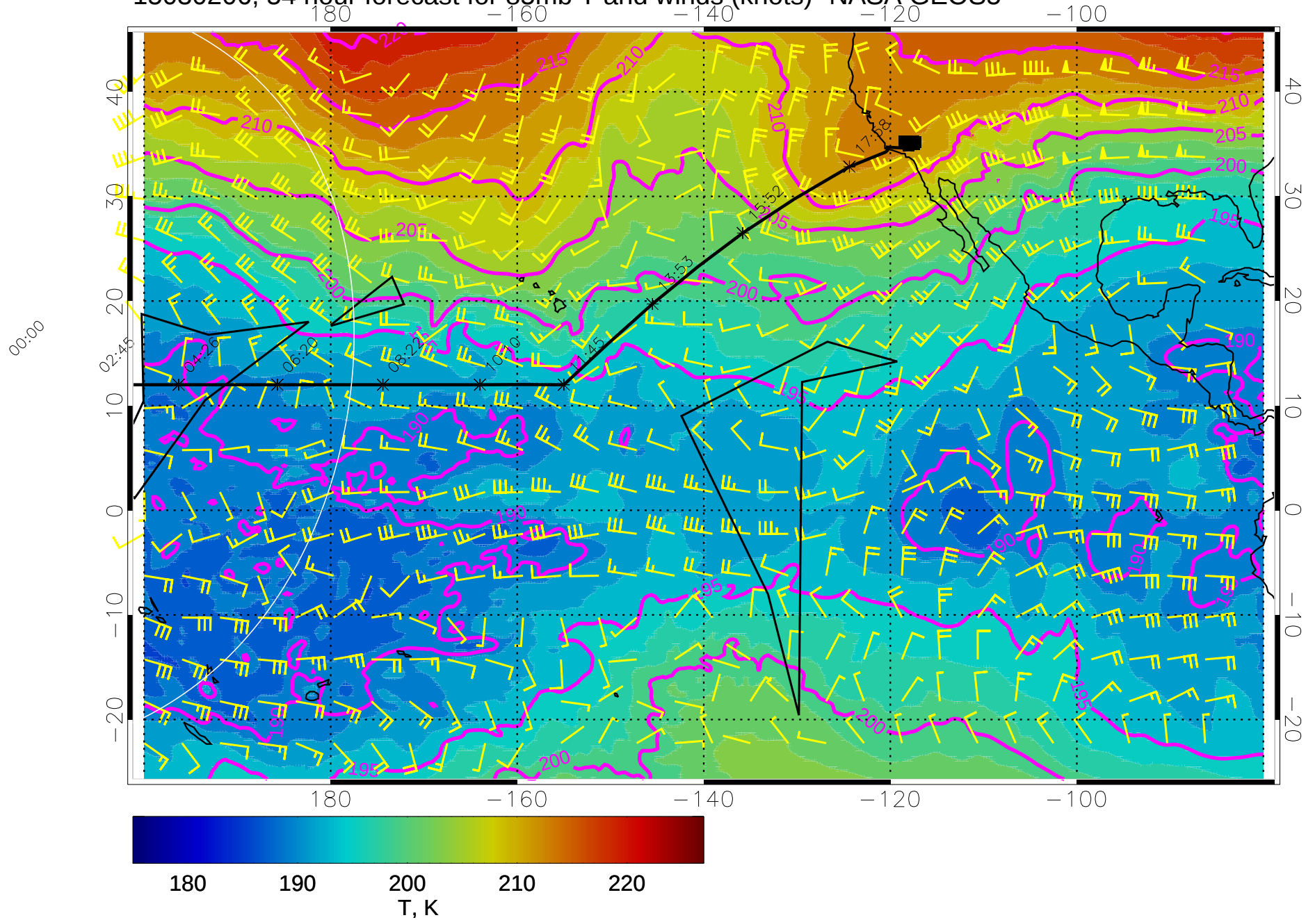
15030206, 54 hour forecast for 85mb T and winds (knots)- NASA GEOS5
