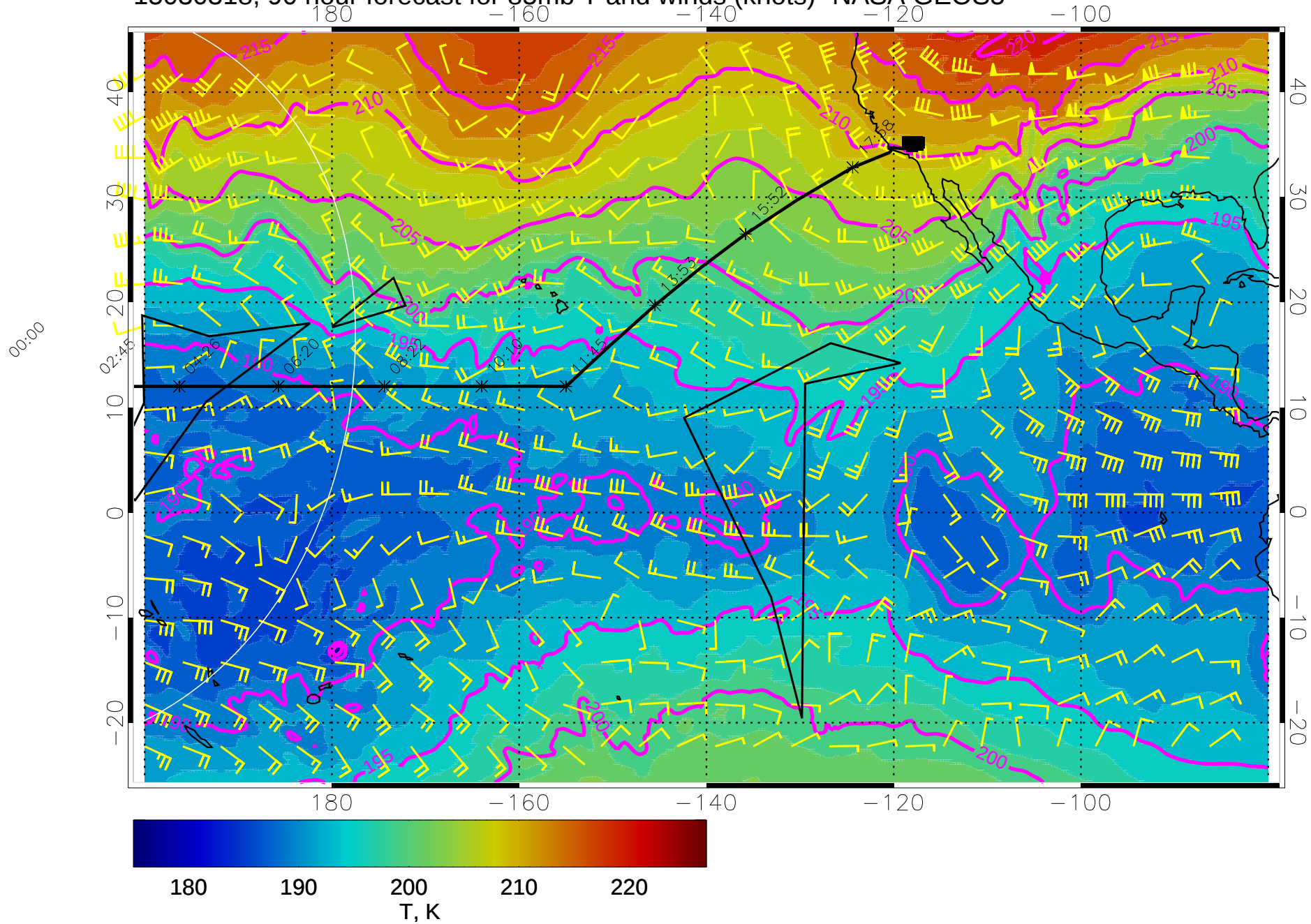
15030318, 90 hour forecast for 85mb T and winds (knots)- NASA GEOS5
