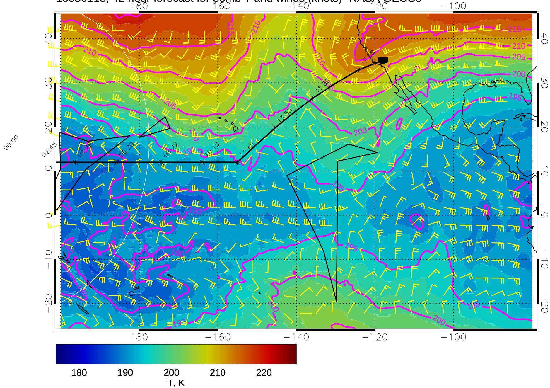
15030118, 42 hour forecast for 85mb T and winds (knots)- NASA GEOS5
