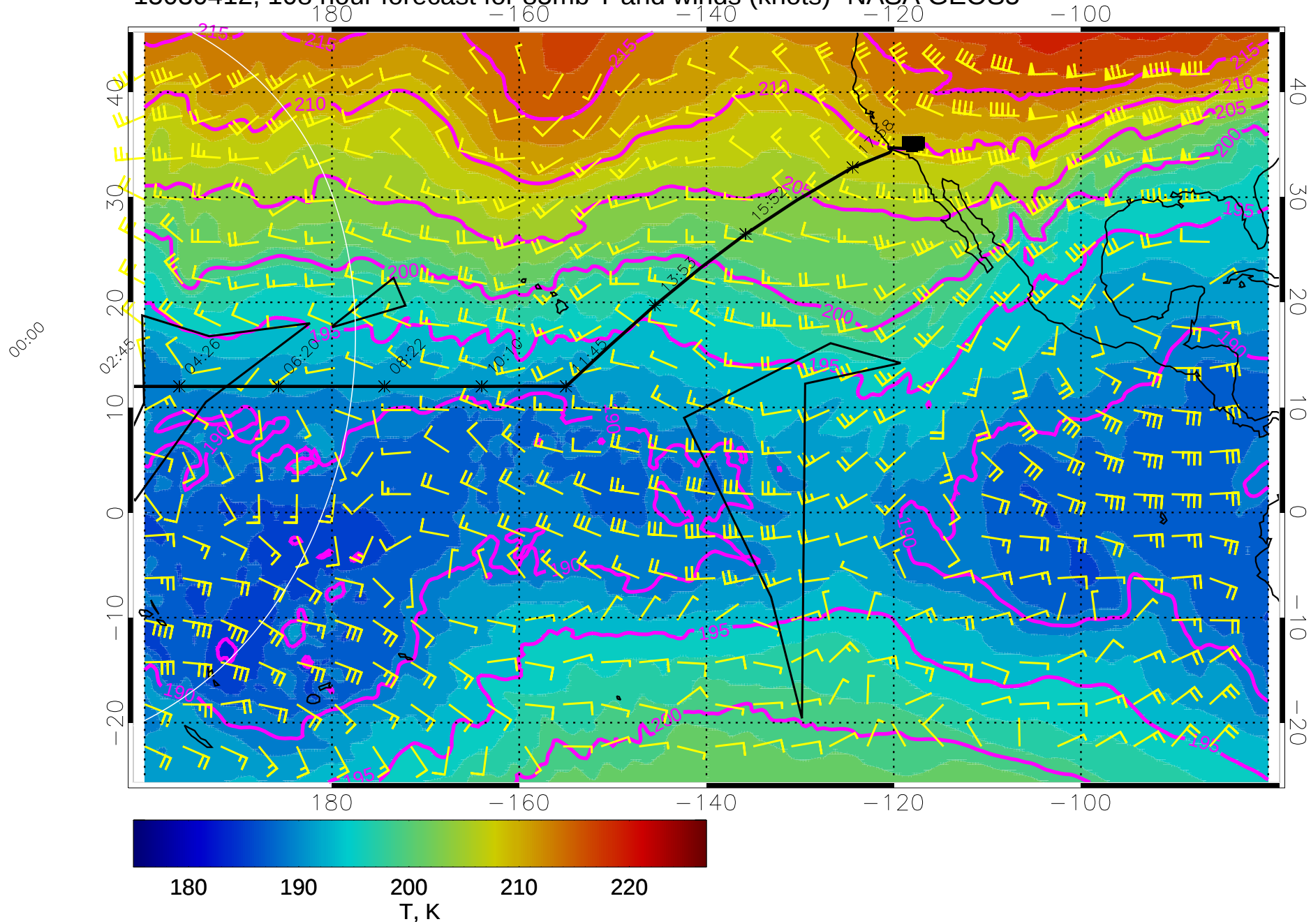
15030412, 108 hour forecast for 85mb T and winds (knots)- NASA GEOS5
