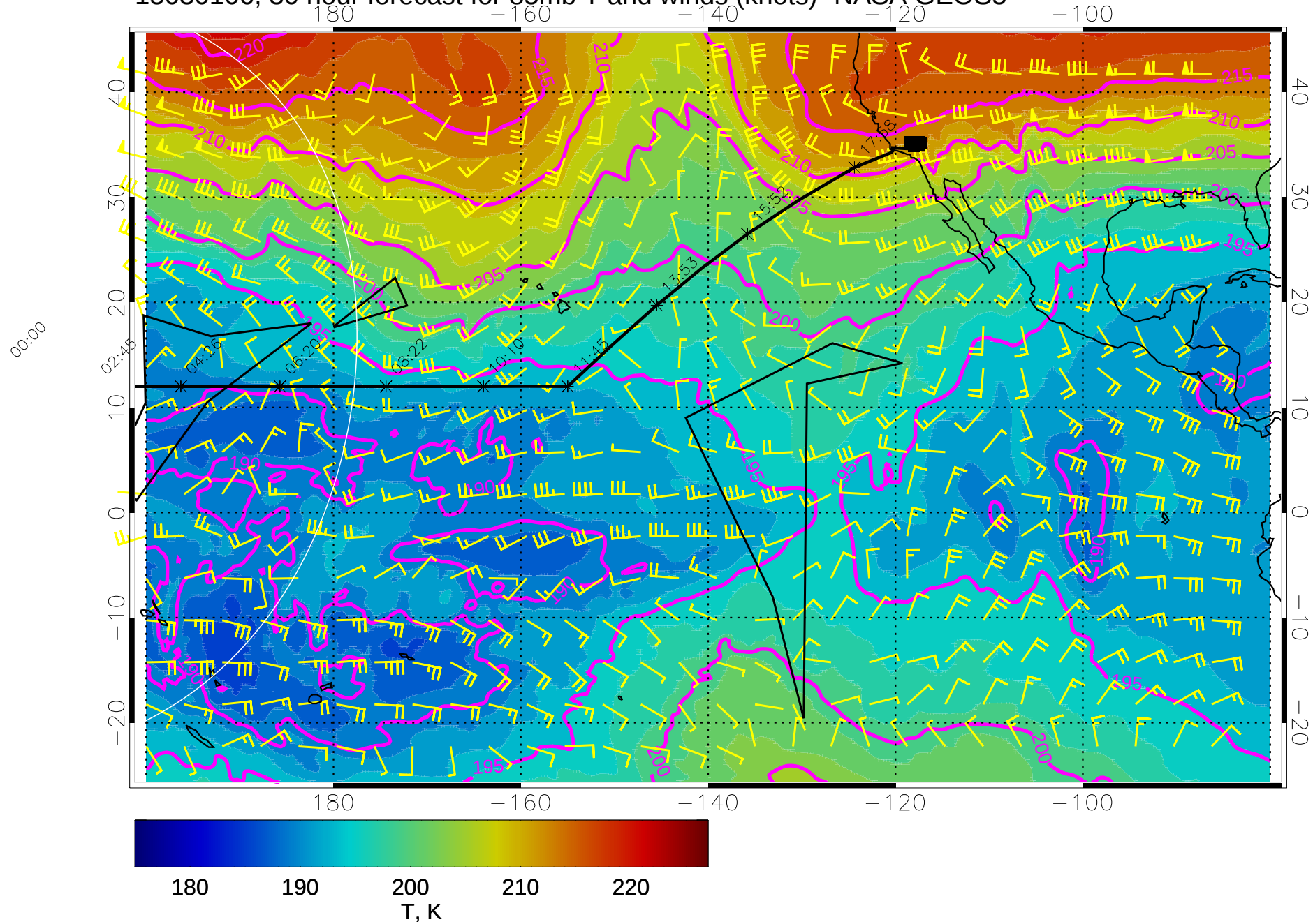
15030106, 30 hour forecast for 85mb T and winds (knots)- NASA GEOS5
