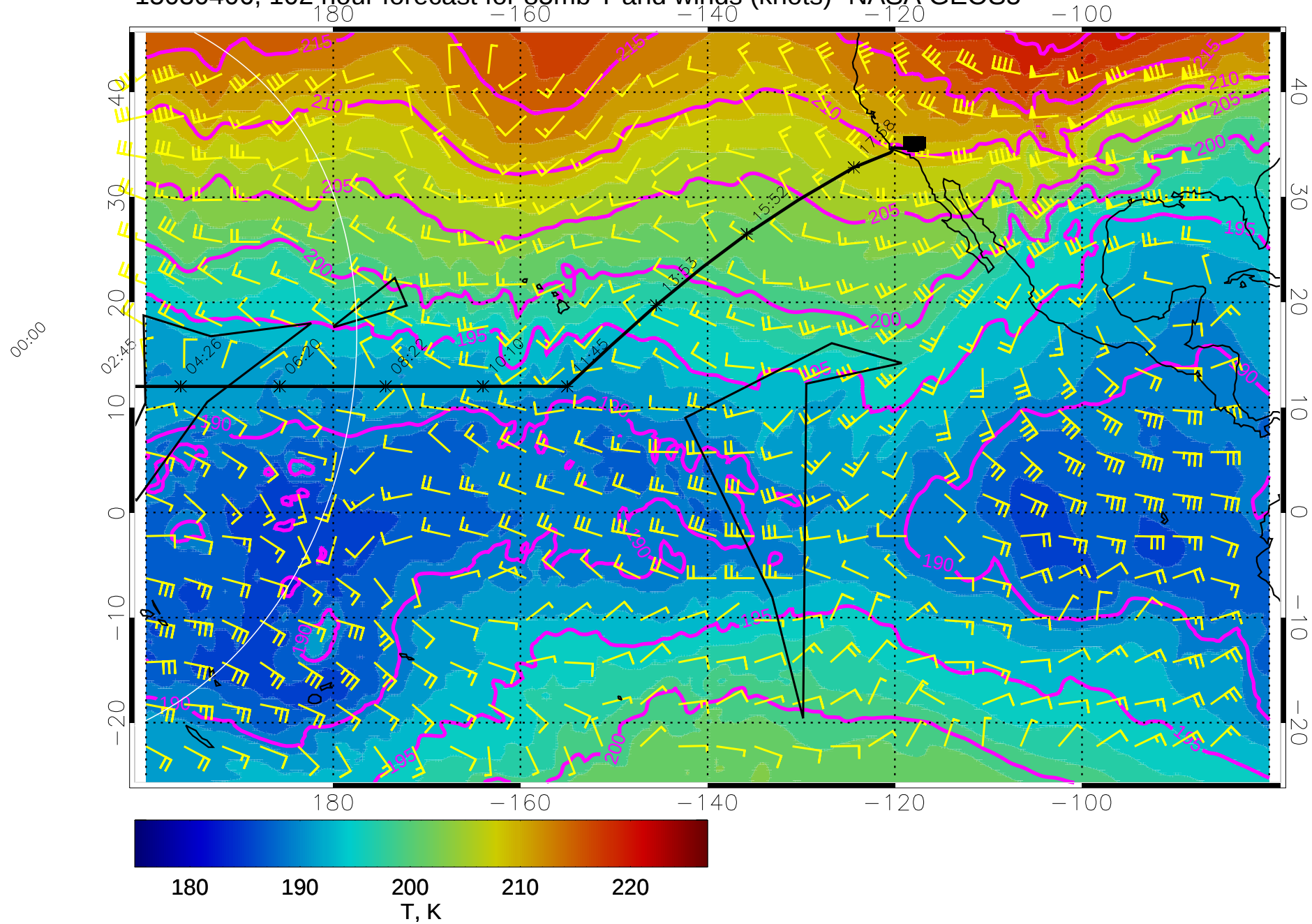
15030406, 102 hour forecast for 85mb T and winds (knots)- NASA GEOS5
