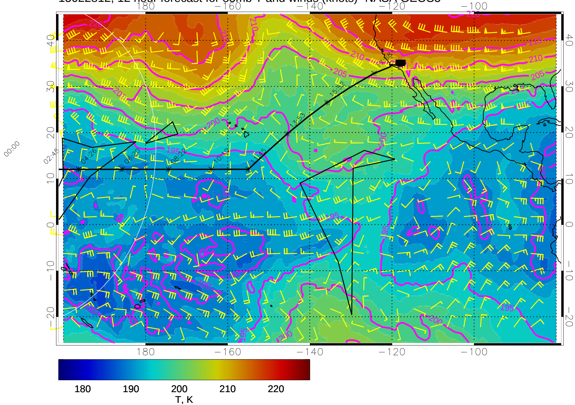
15022812, 12 hour forecast for 85mb T and winds (knots)- NASA GEOS5
