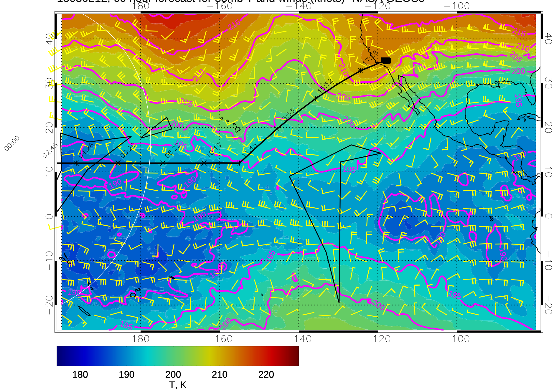
15030212, 60 hour forecast for 85mb T and winds (knots)- NASA GEOS5
