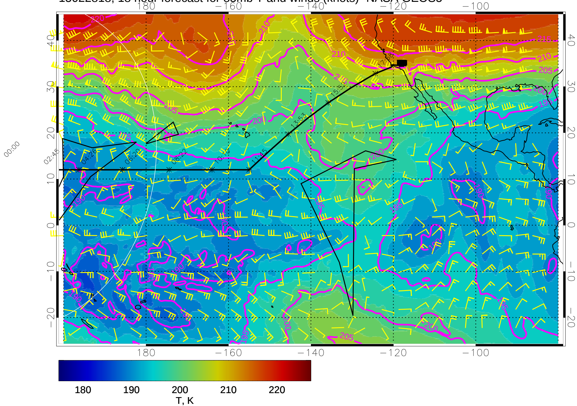
15022818, 18 hour forecast for 85mb T and winds (knots)- NASA GEOS5
