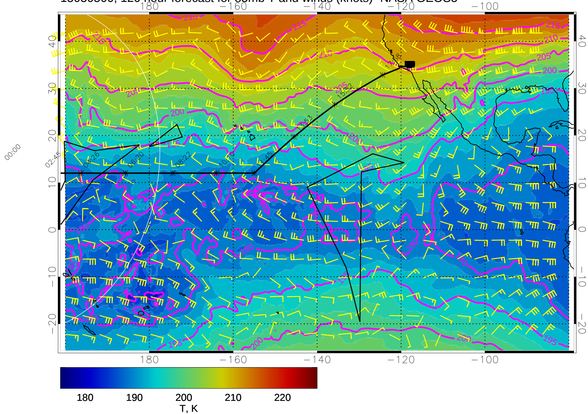
15030500, 120 hour forecast for 85mb T and winds (knots)- NASA GEOS5
