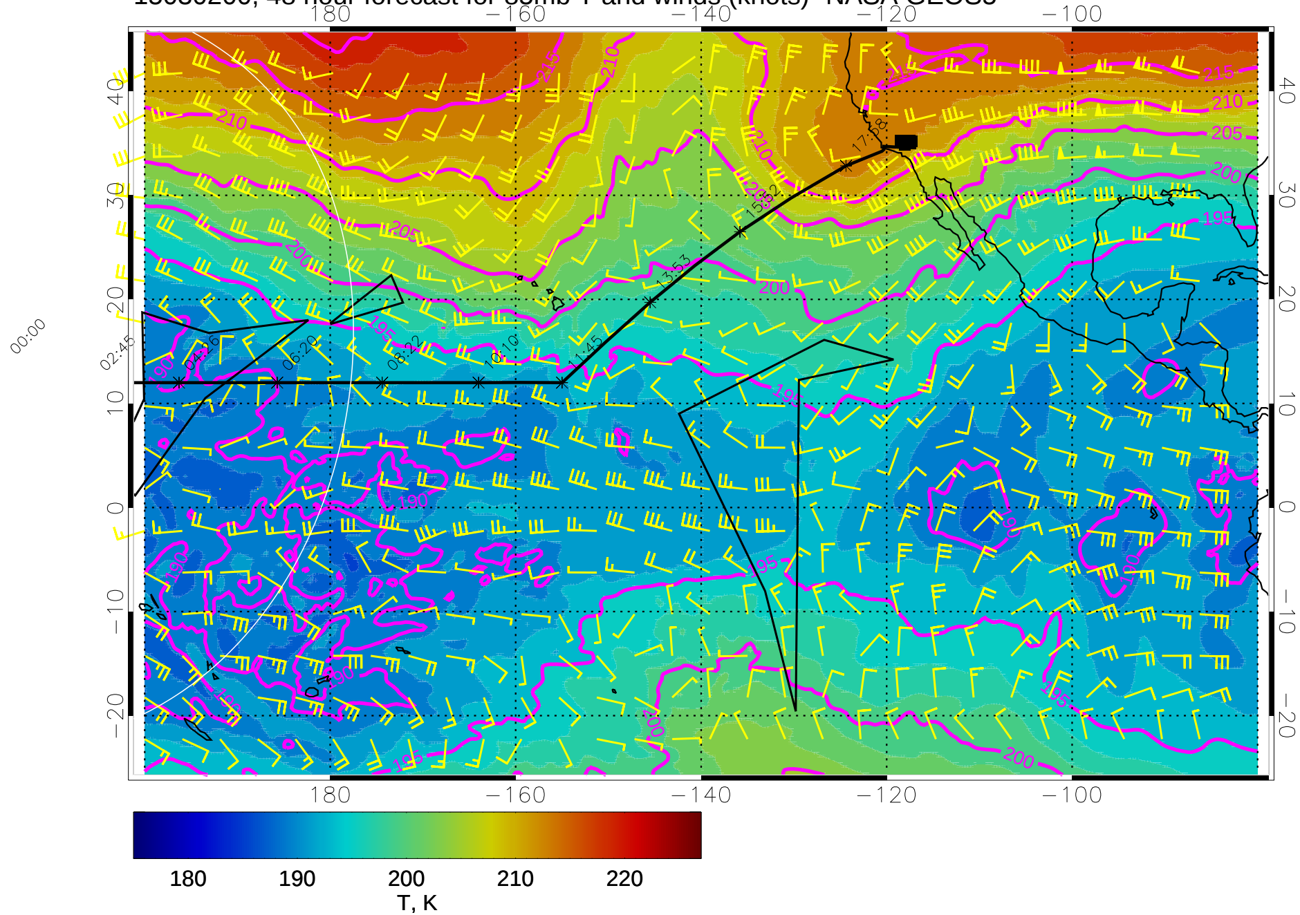
15030200, 48 hour forecast for 85mb T and winds (knots)- NASA GEOS5
