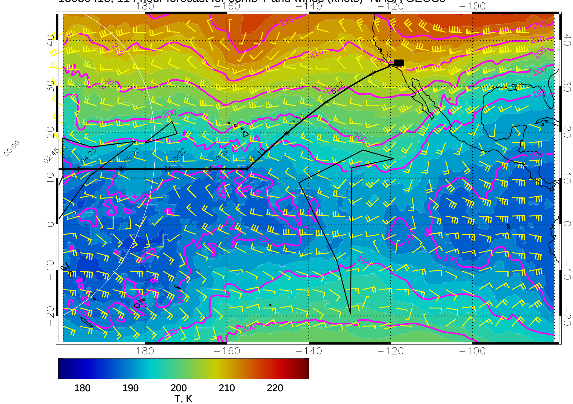
15030418, 114 hour forecast for 85mb T and winds (knots)- NASA GEOS5
