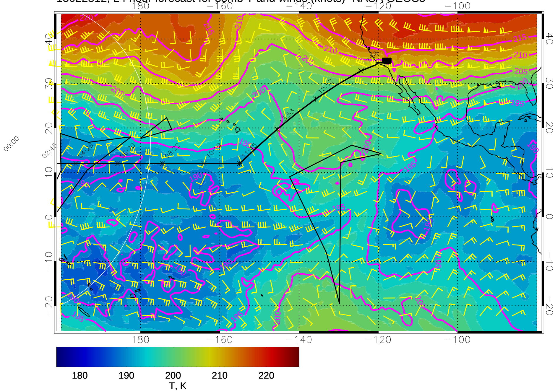
15022812, 24 hour forecast for 85mb T and winds (knots)- NASA GEOS5
