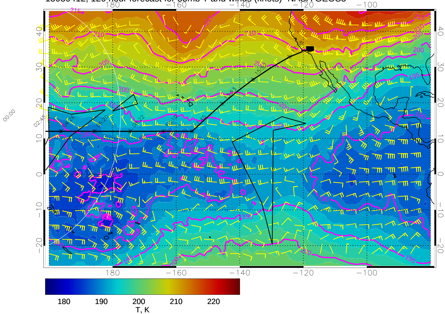
15030412, 120 hour forecast for 85mb T and winds (knots)- NASA GEOS5
