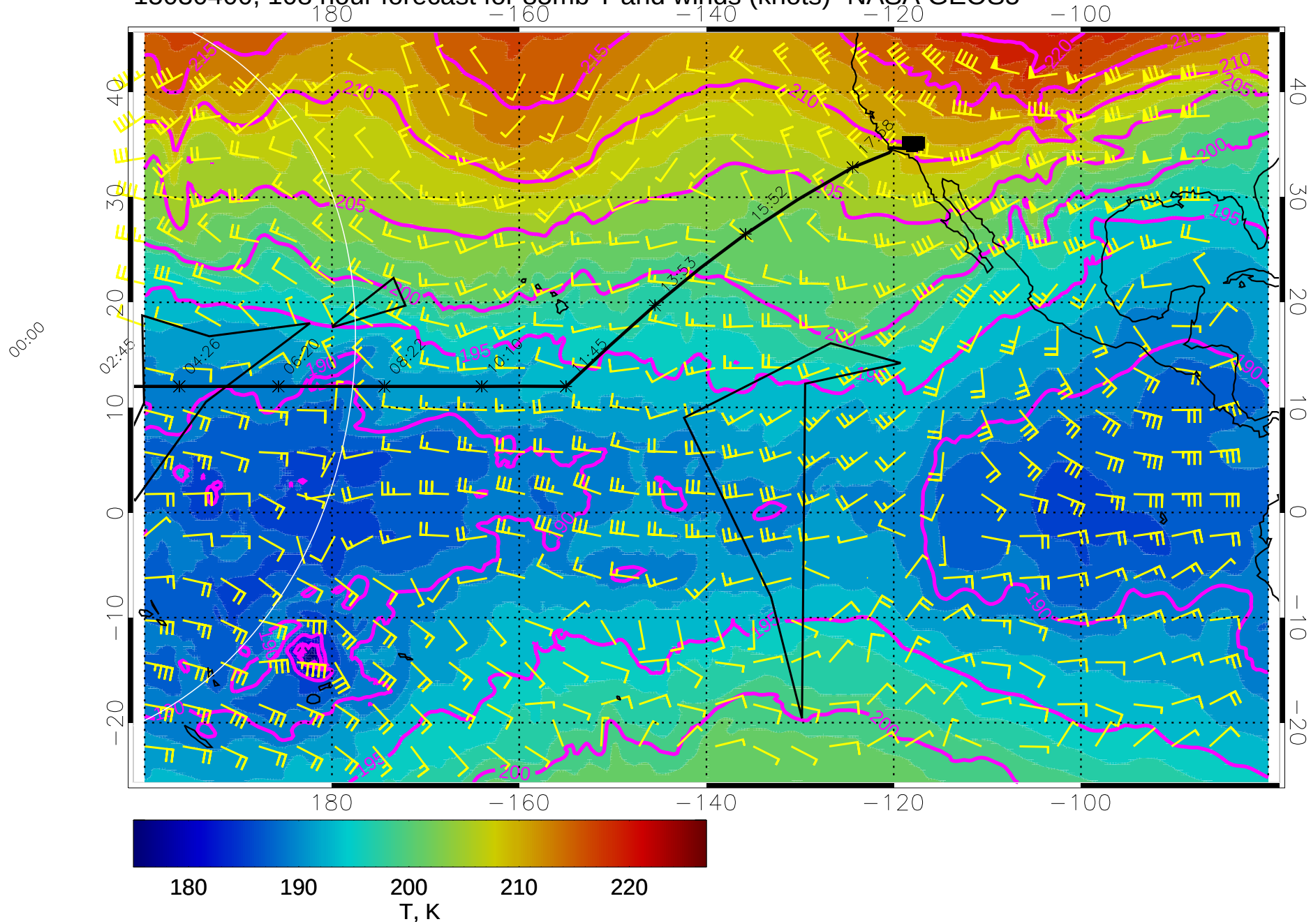
15030400, 108 hour forecast for 85mb T and winds (knots)- NASA GEOS5
