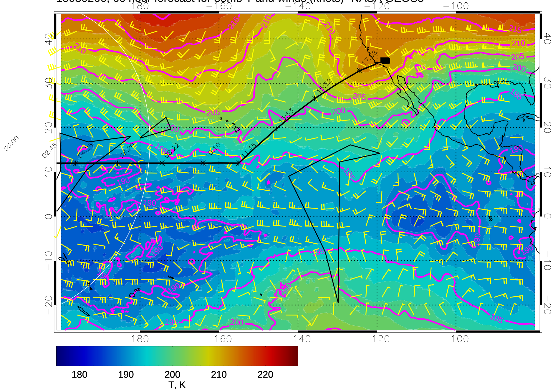
15030206, 66 hour forecast for 85mb T and winds (knots)- NASA GEOS5
