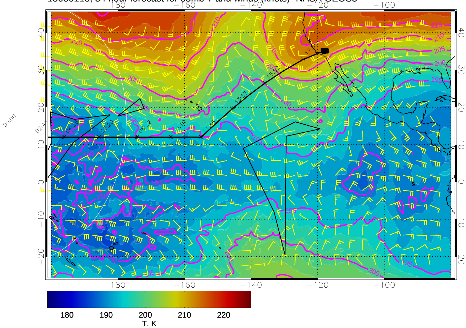
15030118, 54 hour forecast for 85mb T and winds (knots)- NASA GEOS5
