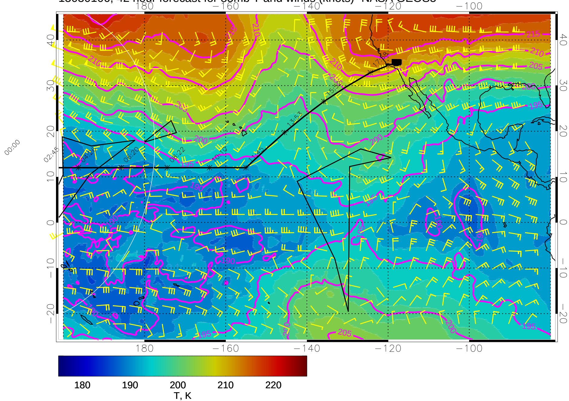
15030106, 42 hour forecast for 85mb T and winds (knots)- NASA GEOS5
