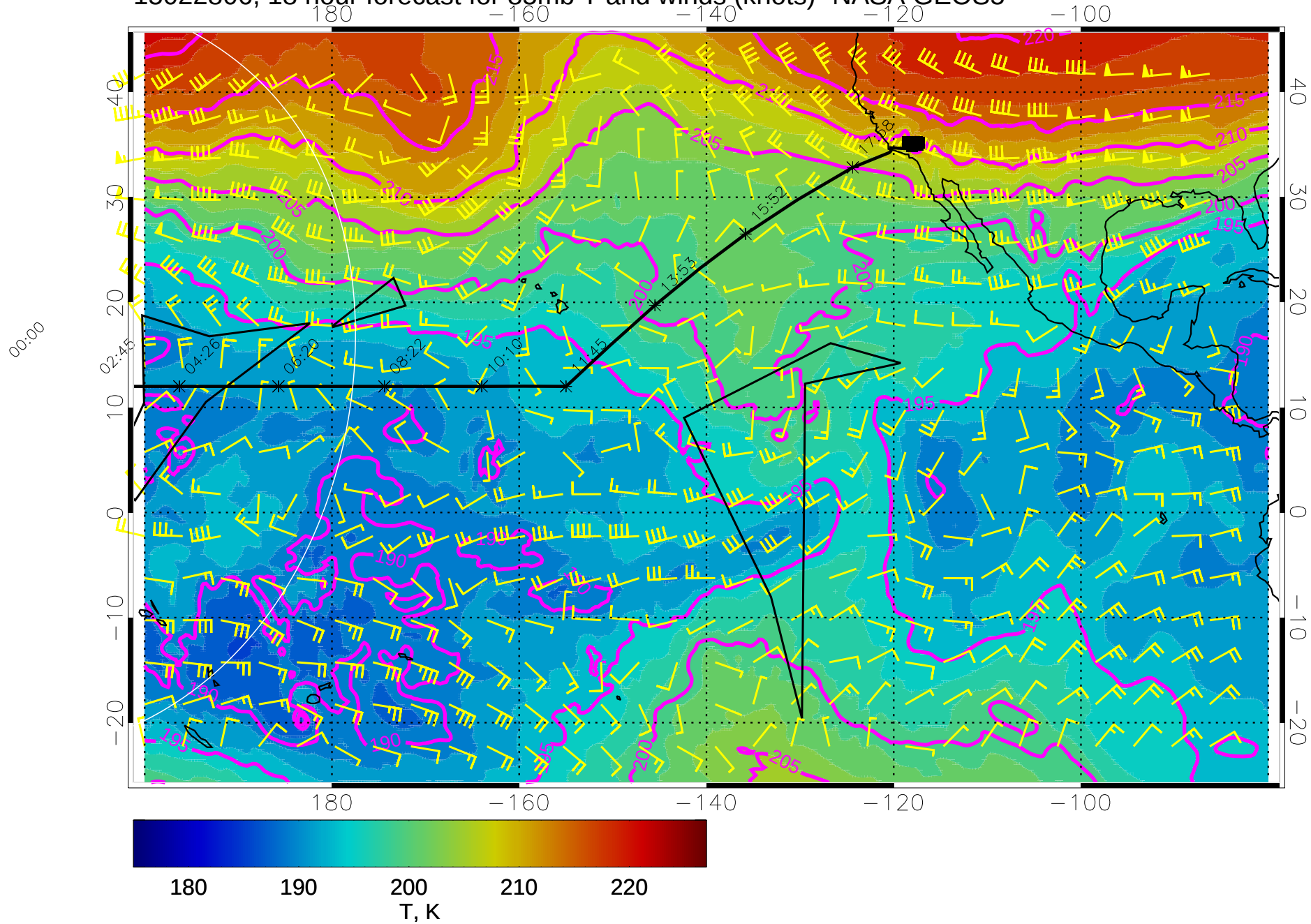
15022806, 18 hour forecast for 85mb T and winds (knots)- NASA GEOS5
