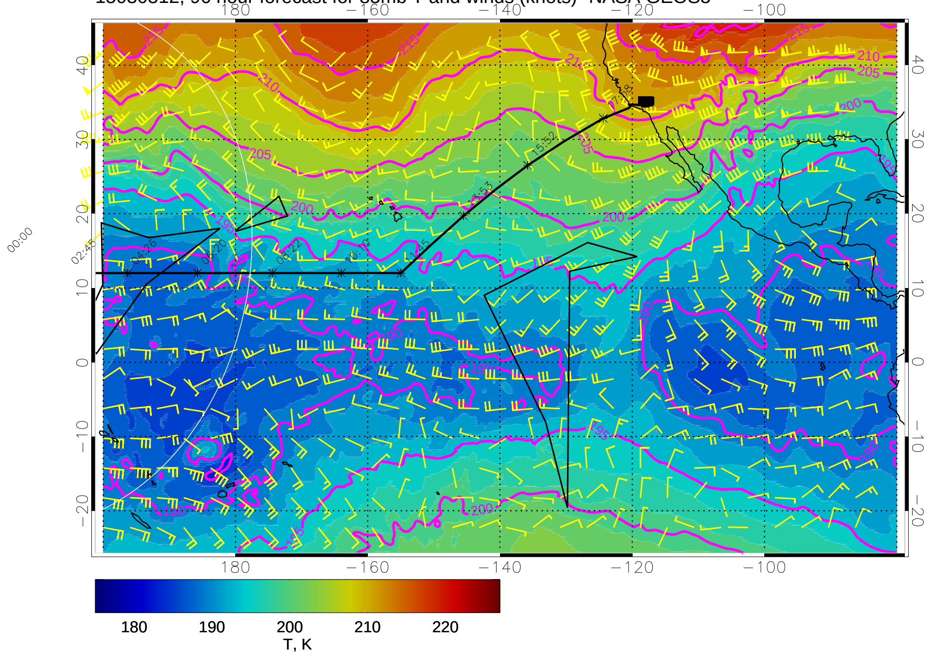
15030312, 96 hour forecast for 85mb T and winds (knots)- NASA GEOS5
