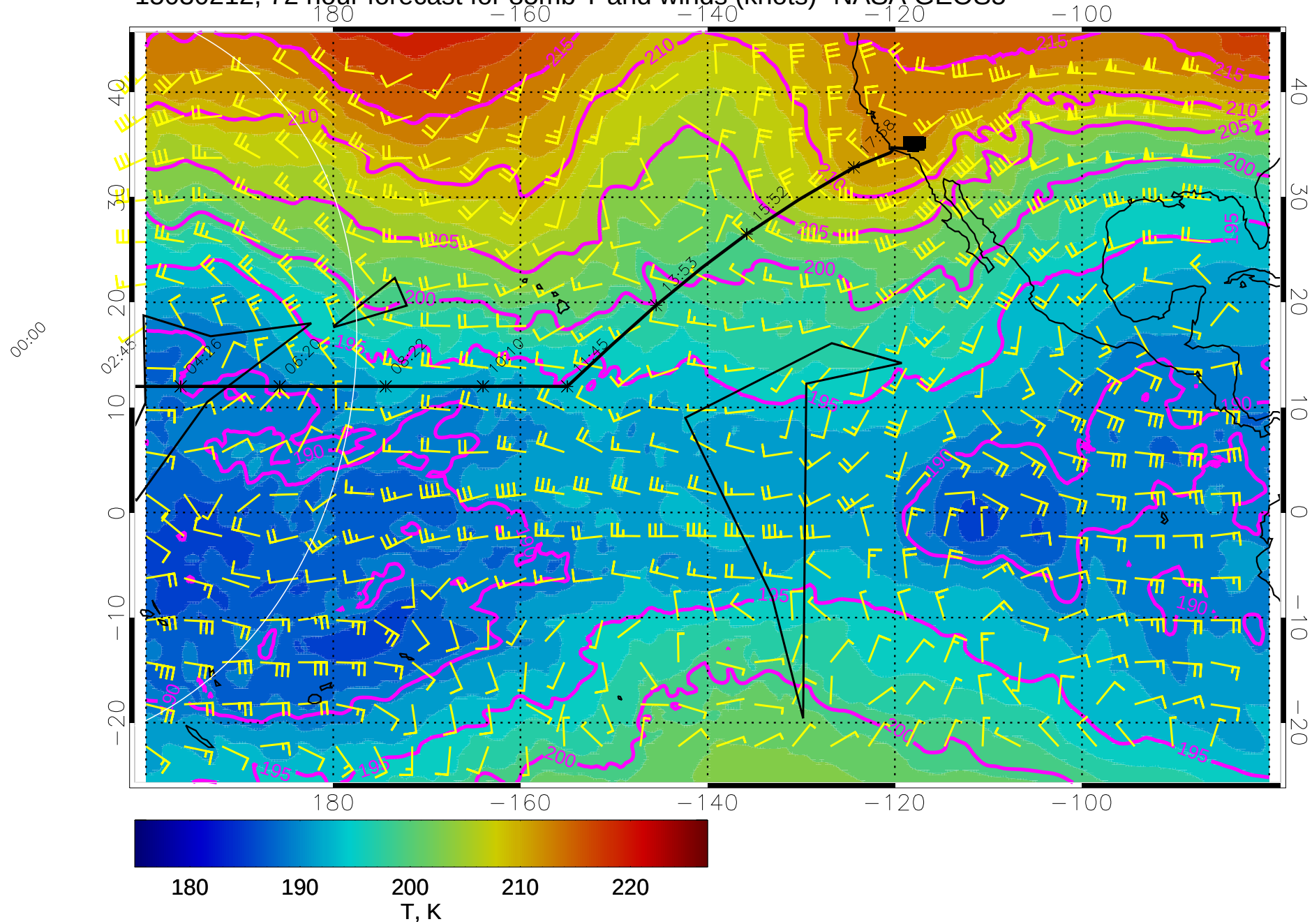
15030212, 72 hour forecast for 85mb T and winds (knots)- NASA GEOS5
