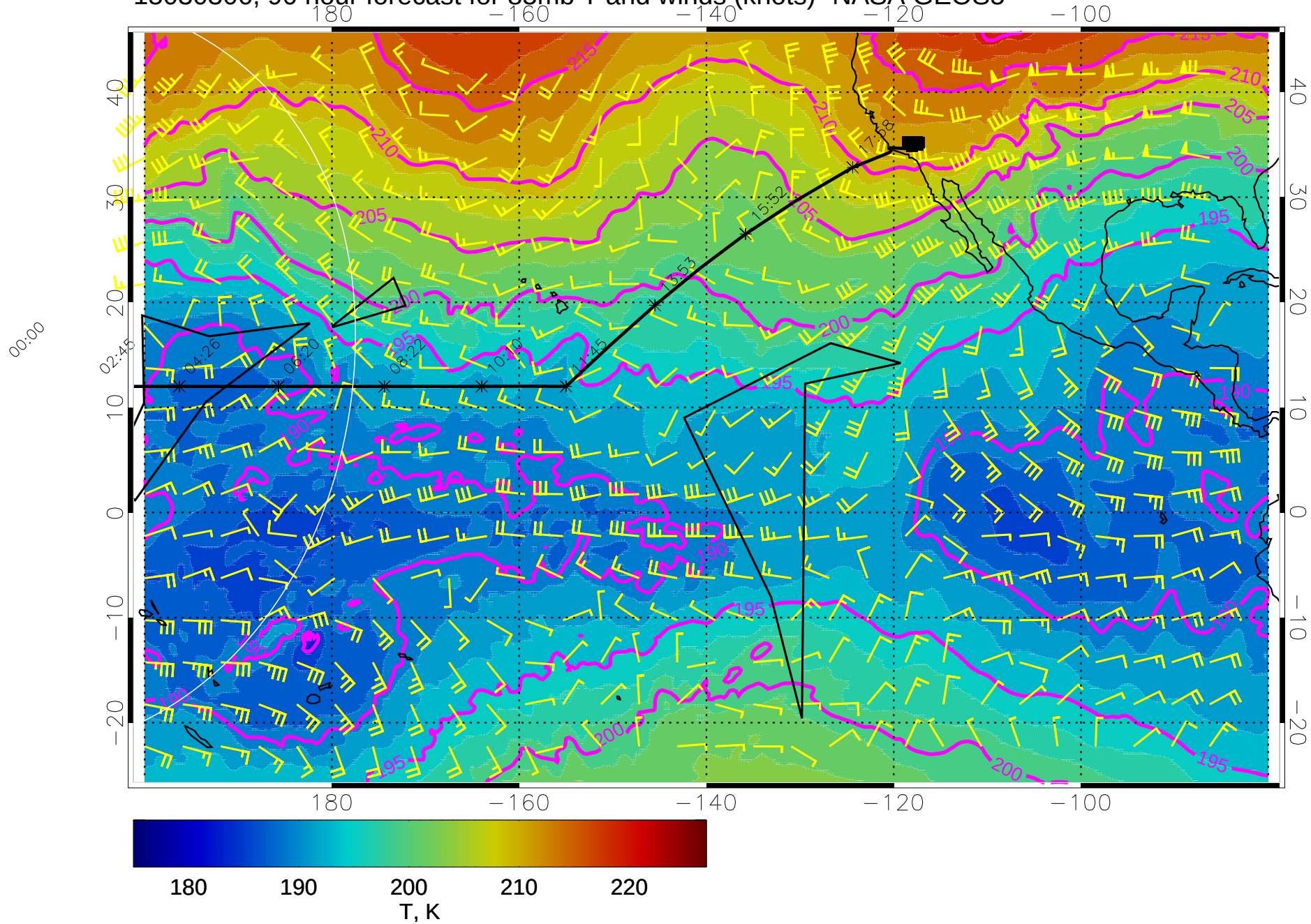
15030306, 90 hour forecast for 85mb T and winds (knots)- NASA GEOS5
