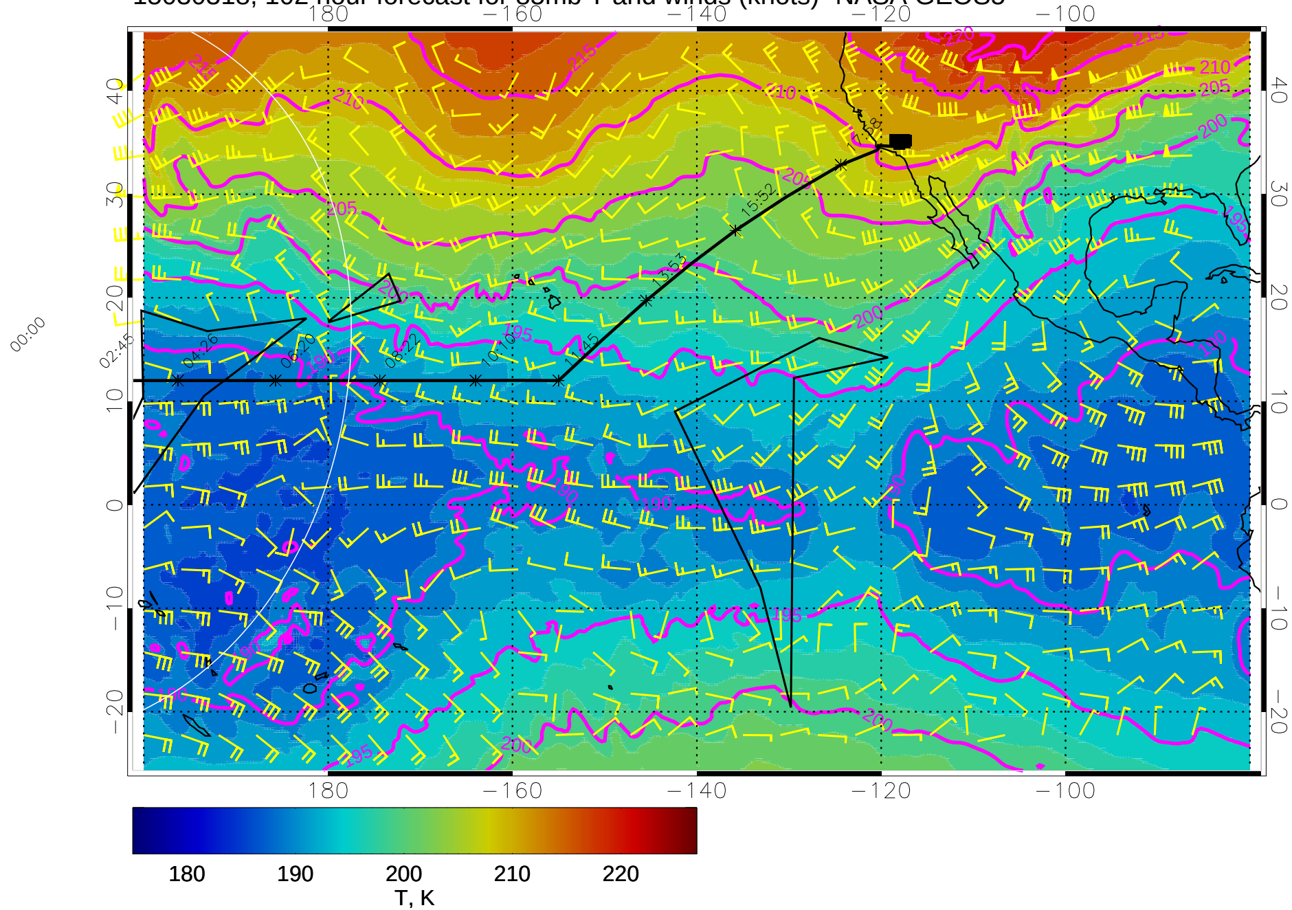
15030318, 102 hour forecast for 85mb T and winds (knots)- NASA GEOS5
