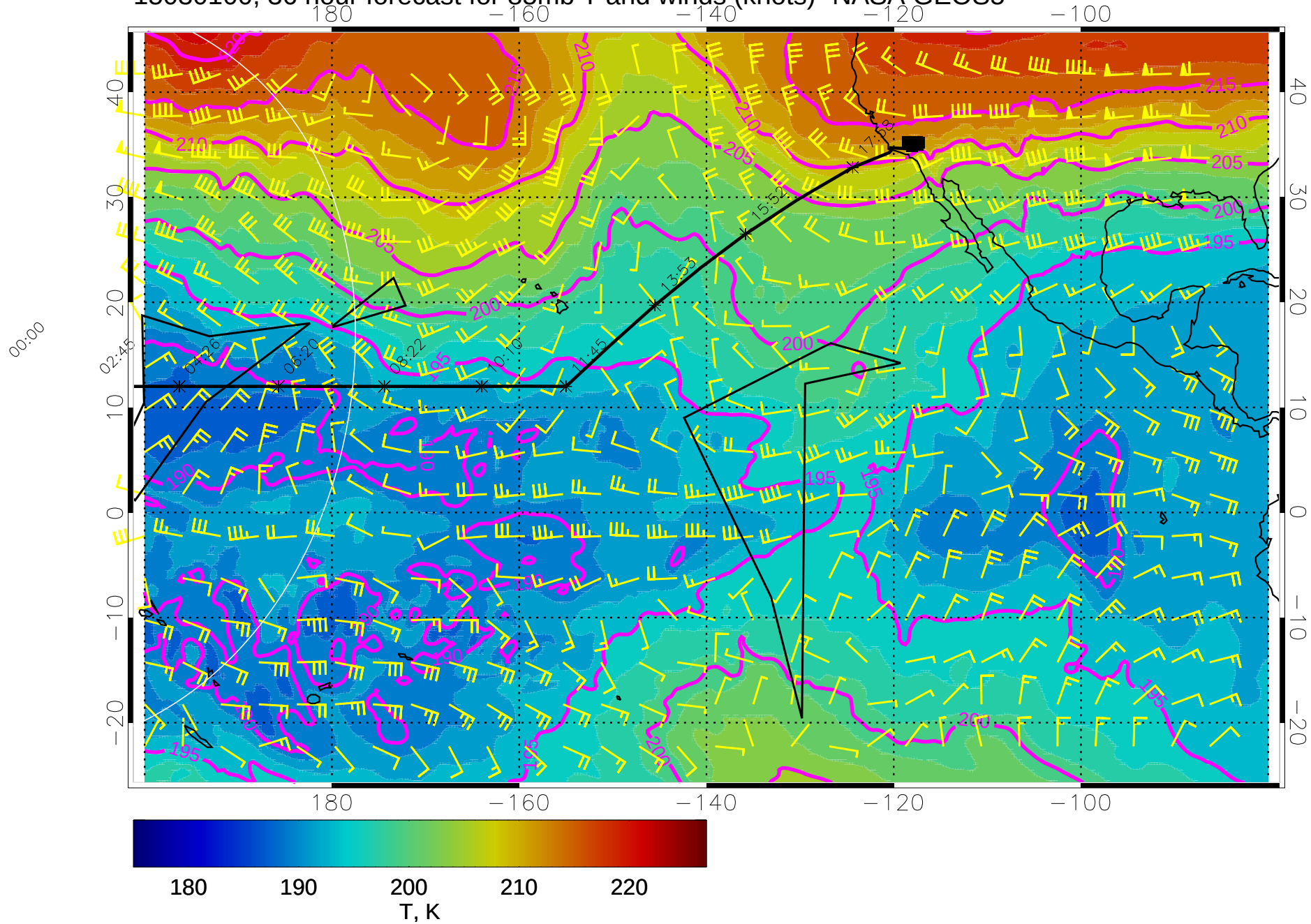
15030100, 36 hour forecast for 85mb T and winds (knots)- NASA GEOS5
