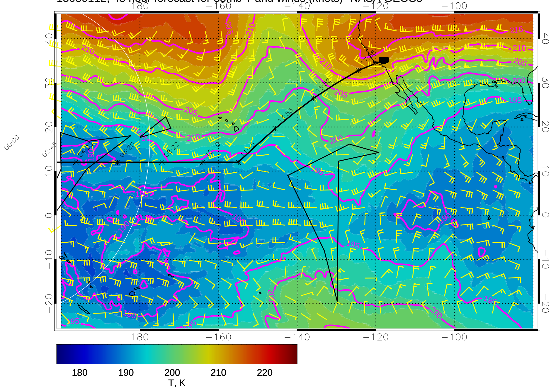
15030112, 48 hour forecast for 85mb T and winds (knots)- NASA GEOS5
