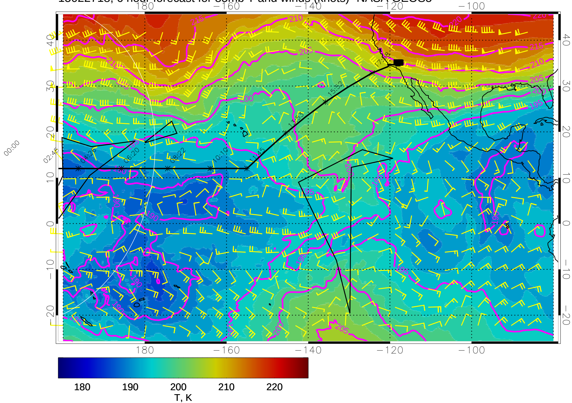
15022718, 6 hour forecast for 85mb T and winds (knots)- NASA GEOS5
