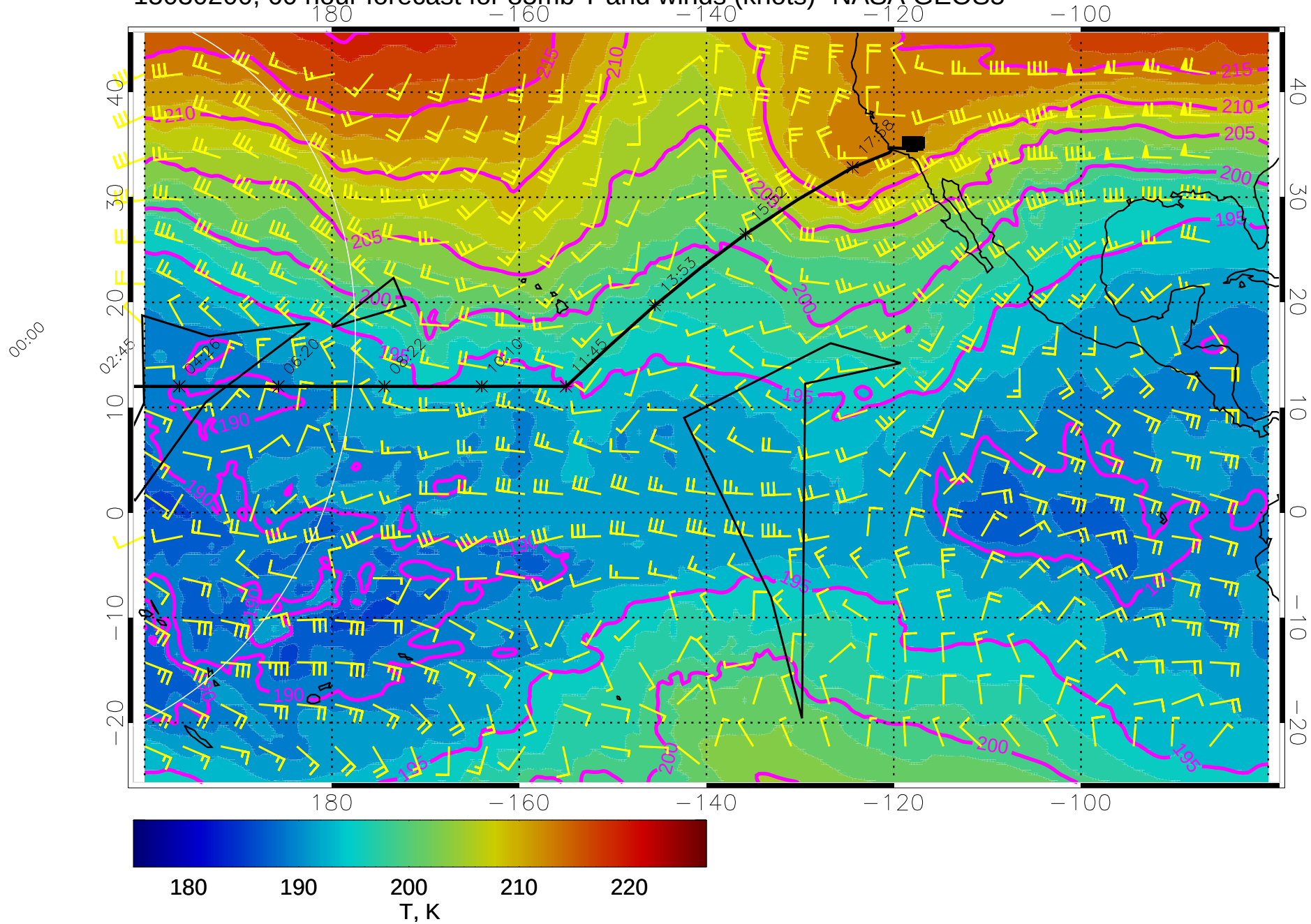
15030200, 60 hour forecast for 85mb T and winds (knots)- NASA GEOS5
