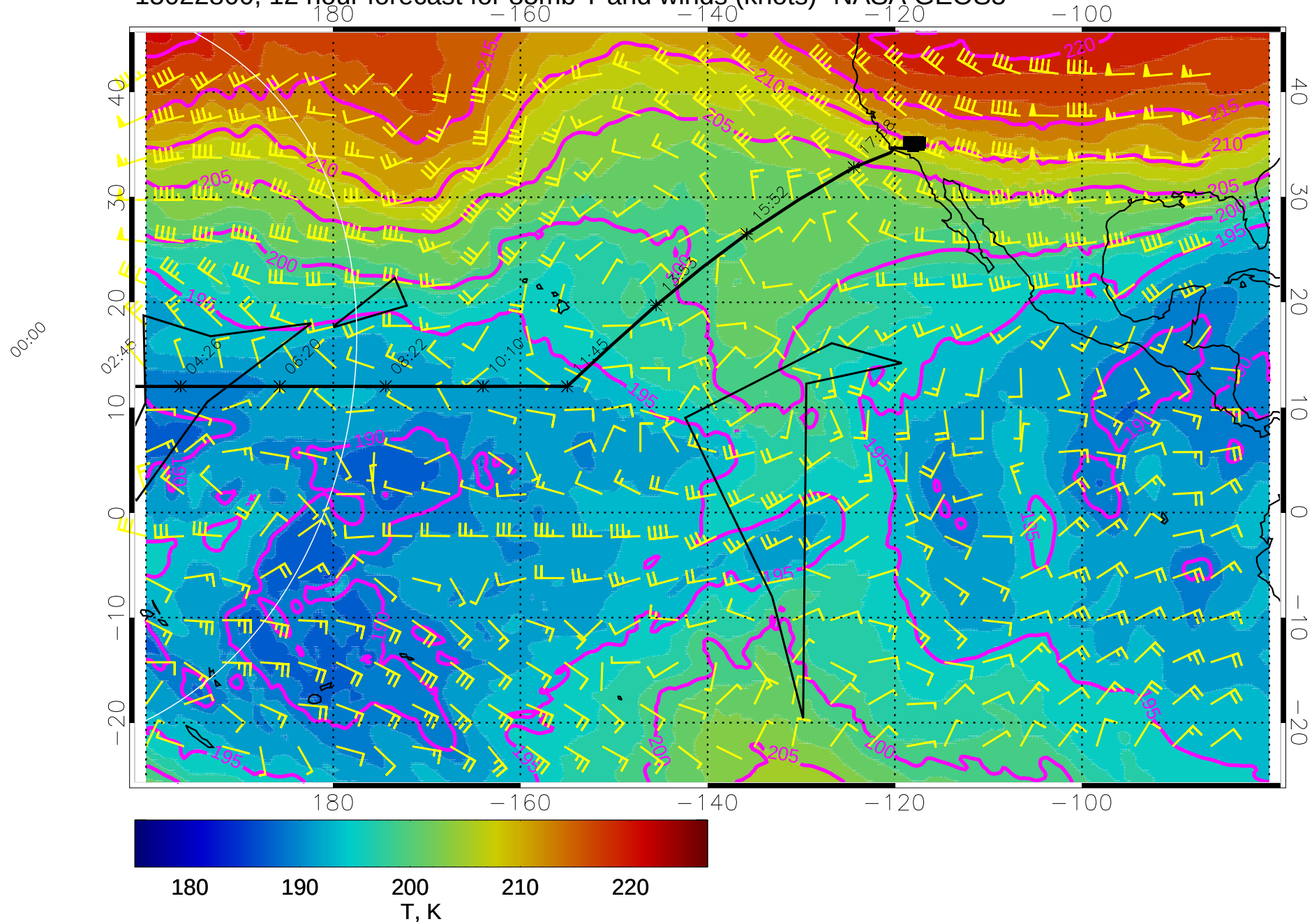
15022800, 12 hour forecast for 85mb T and winds (knots)- NASA GEOS5
