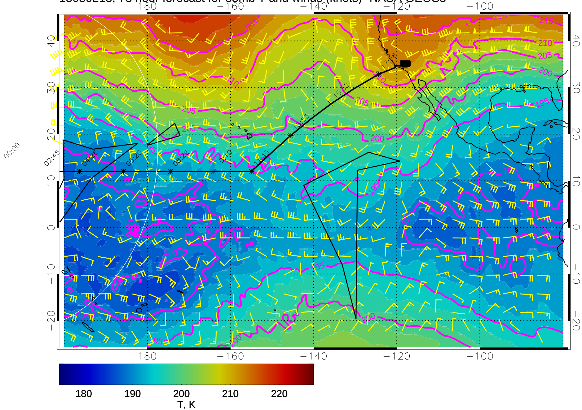
15030218, 78 hour forecast for 85mb T and winds (knots)- NASA GEOS5
