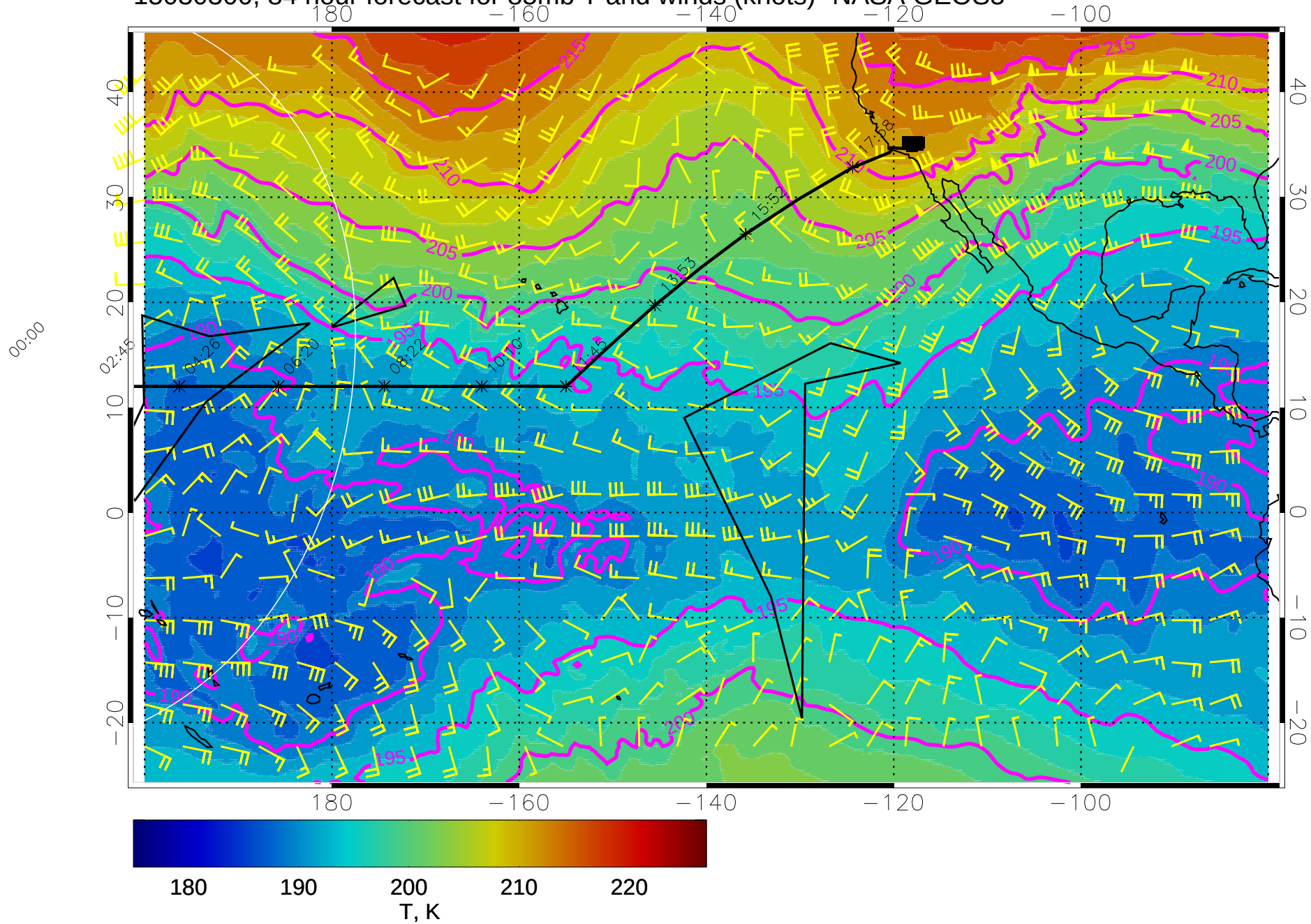
15030300, 84 hour forecast for 85mb T and winds (knots)- NASA GEOS5
