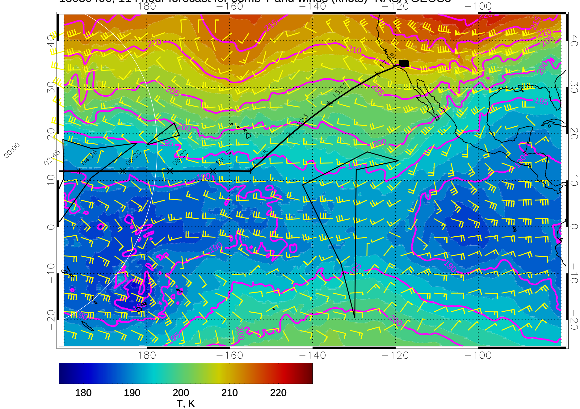
15030406, 114 hour forecast for 85mb T and winds (knots)- NASA GEOS5
