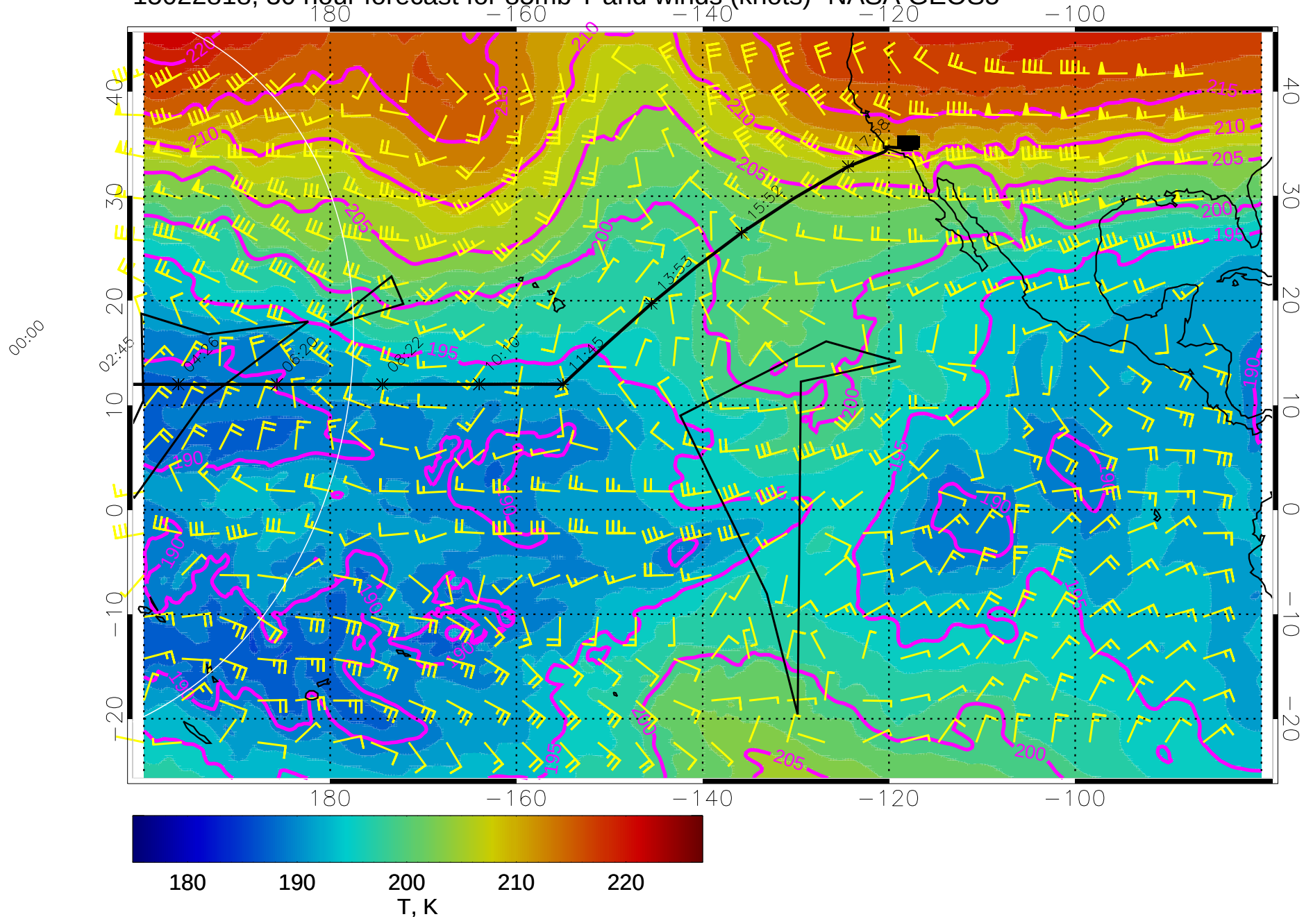
15022818, 30 hour forecast for 85mb T and winds (knots)- NASA GEOS5
