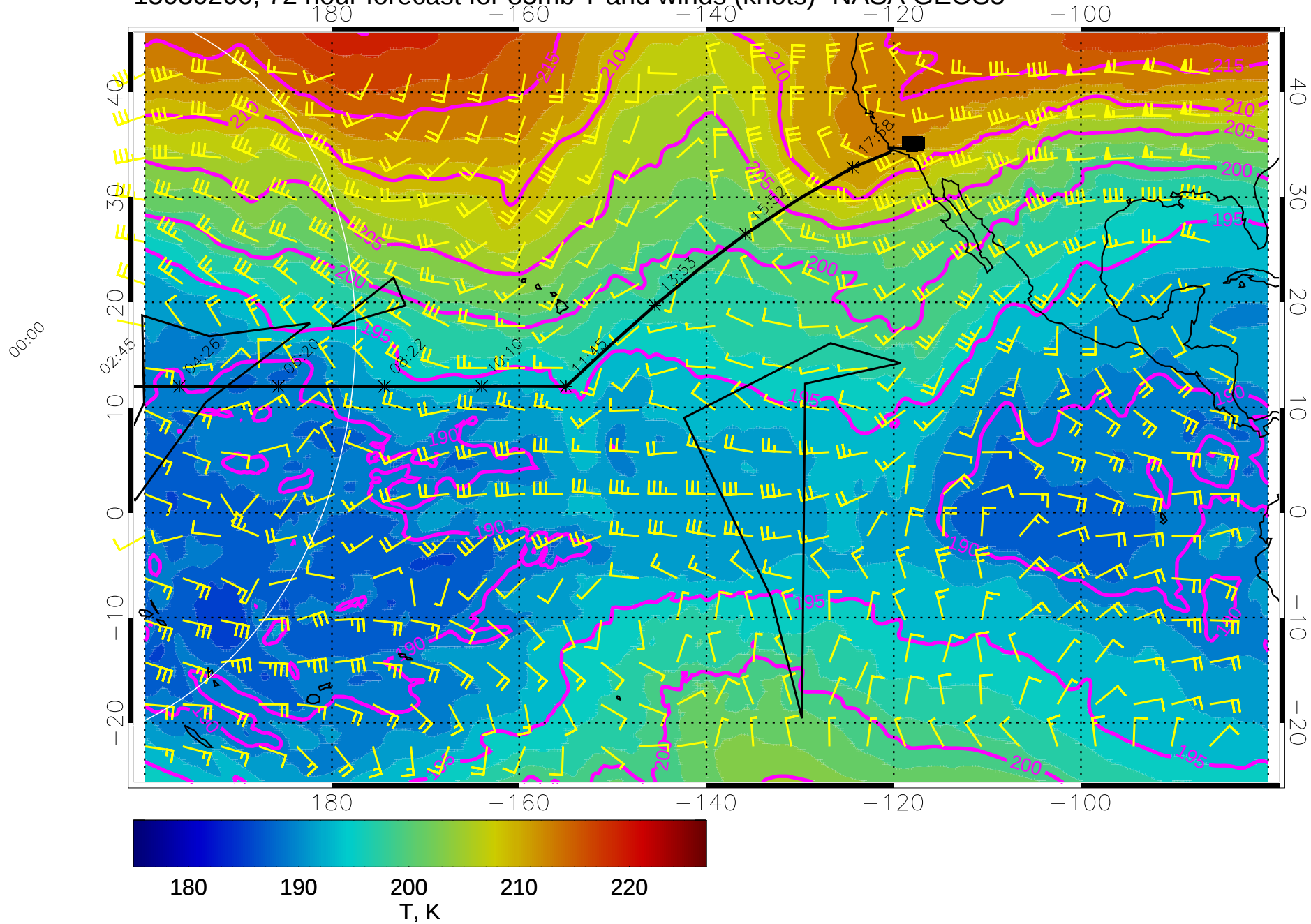
15030200, 72 hour forecast for 85mb T and winds (knots)- NASA GEOS5
