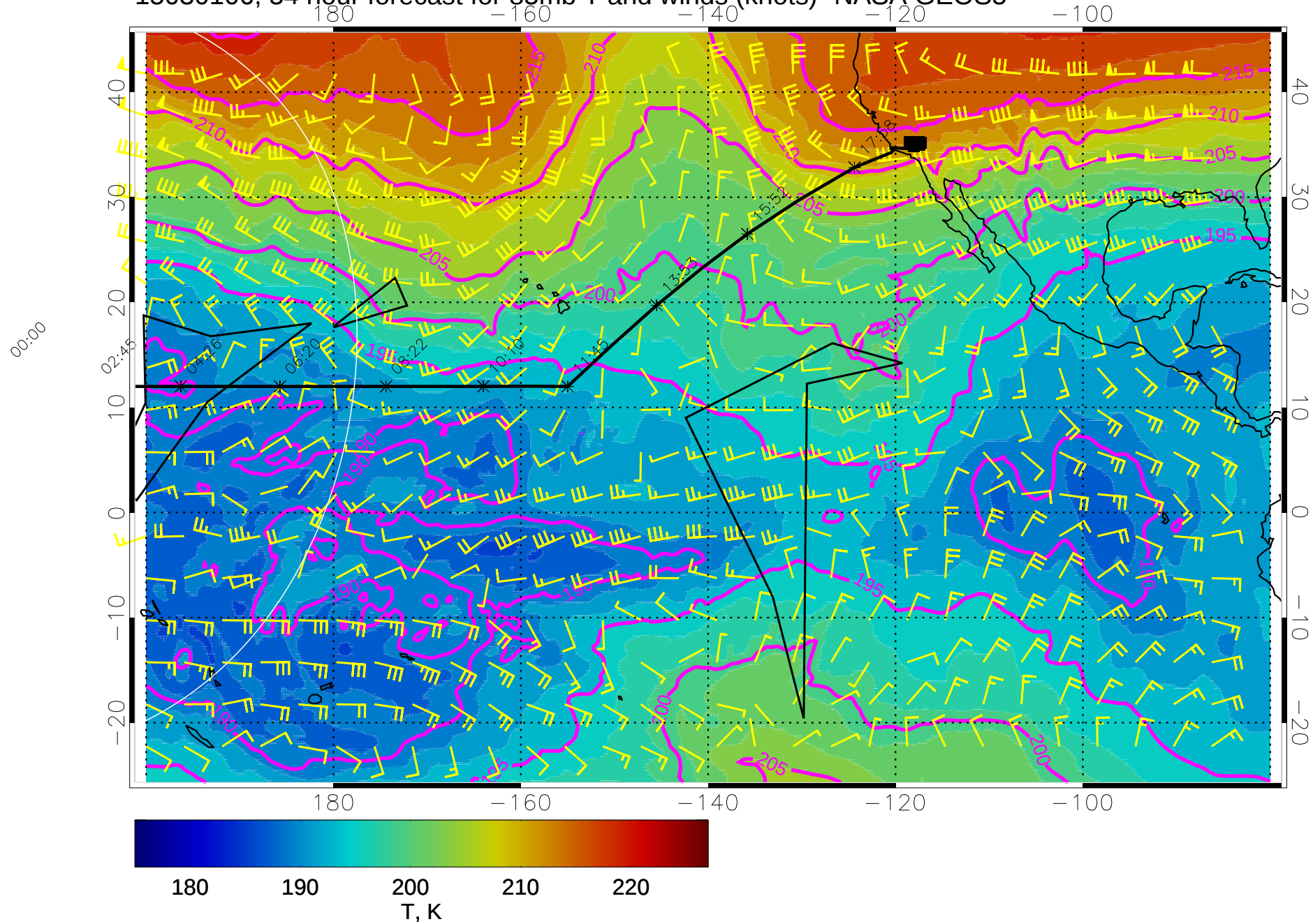
15030106, 54 hour forecast for 85mb T and winds (knots)- NASA GEOS5
