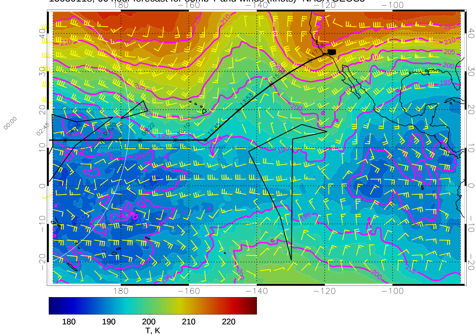
15030118, 66 hour forecast for 85mb T and winds (knots)- NASA GEOS5
