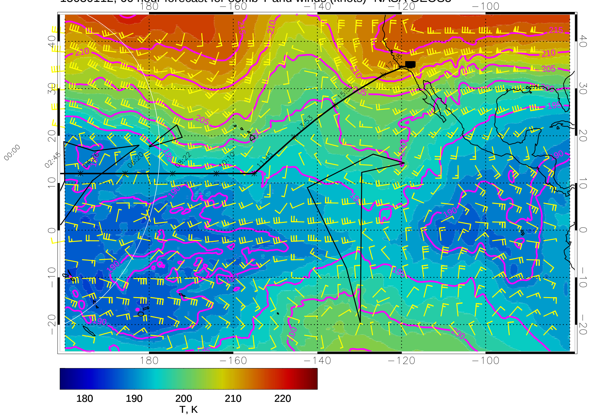
15030112, 60 hour forecast for 85mb T and winds (knots)- NASA GEOS5
