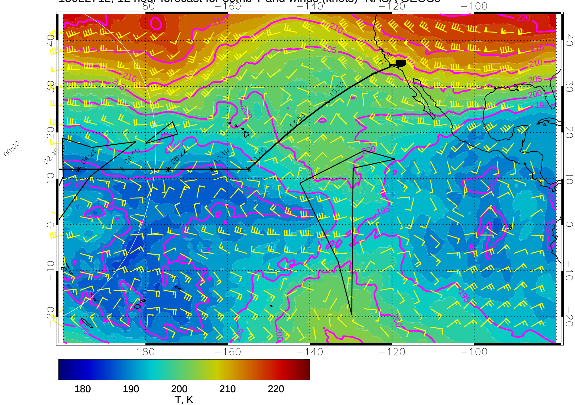
15022712, 12 hour forecast for 85mb T and winds (knots)- NASA GEOS5
