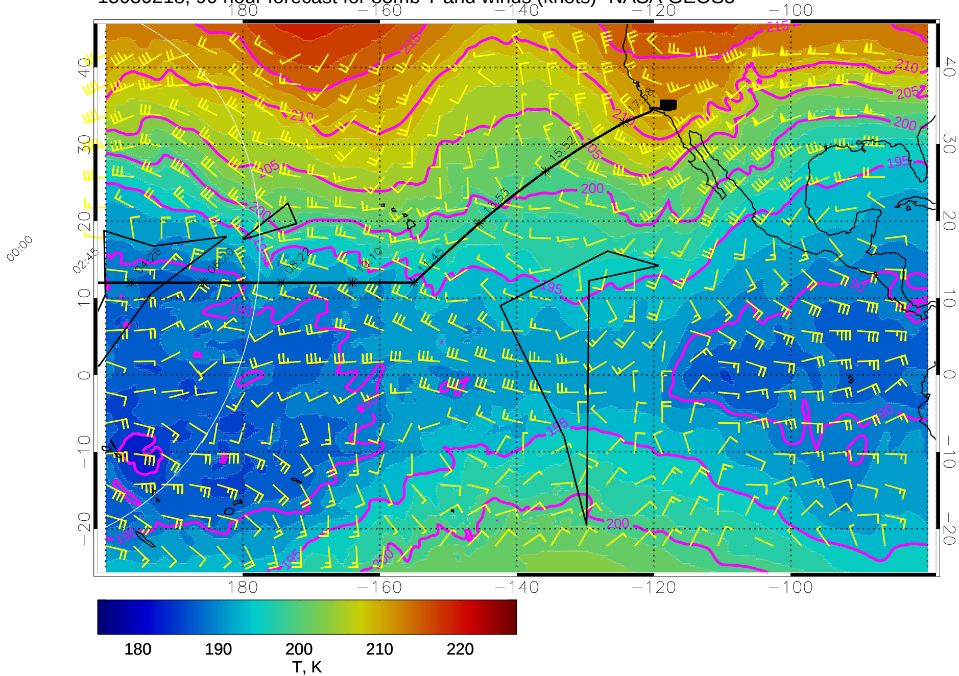
15030218, 90 hour forecast for 85mb T and winds (knots)- NASA GEOS5
