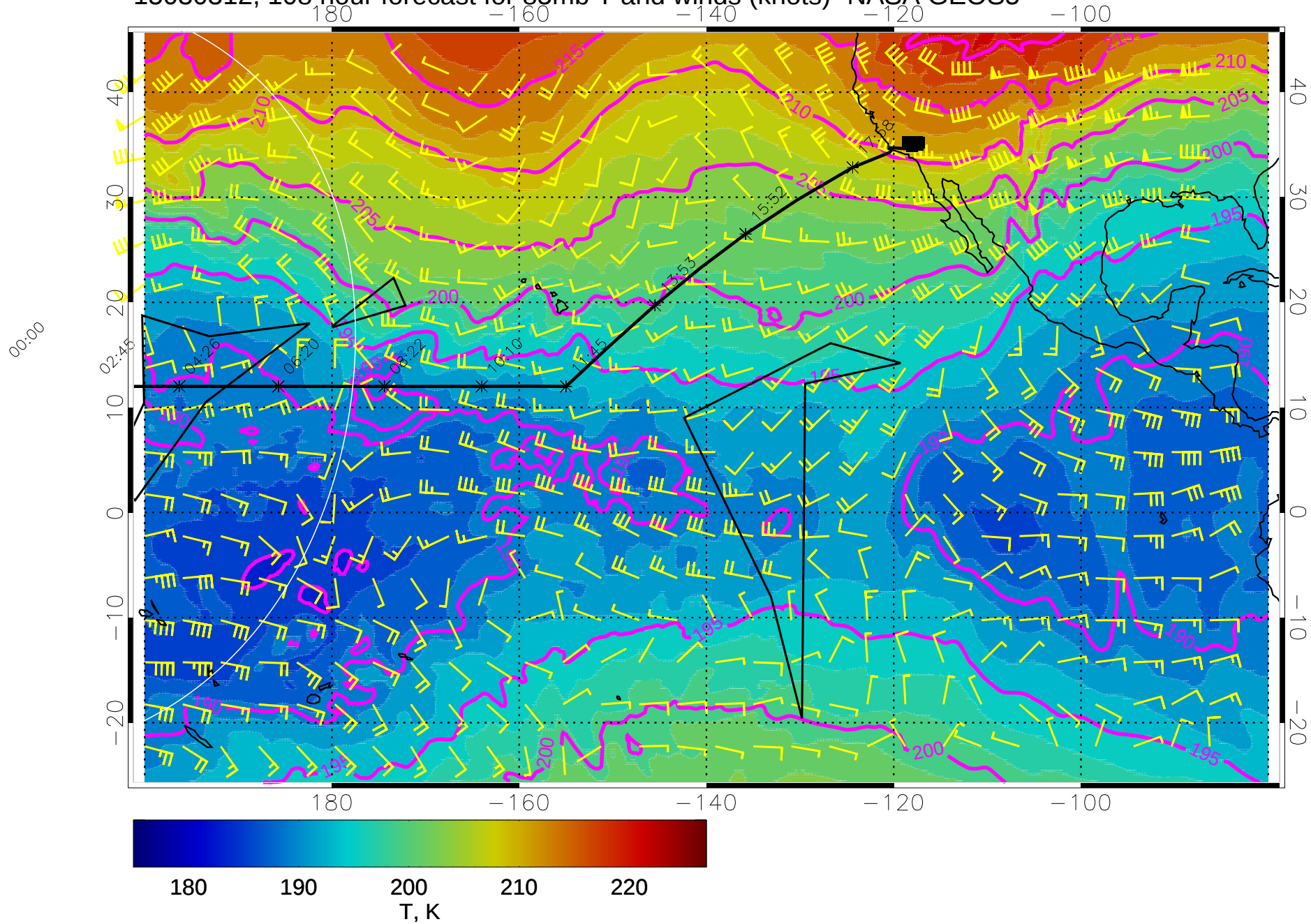
15030312, 108 hour forecast for 85mb T and winds (knots)- NASA GEOS5
