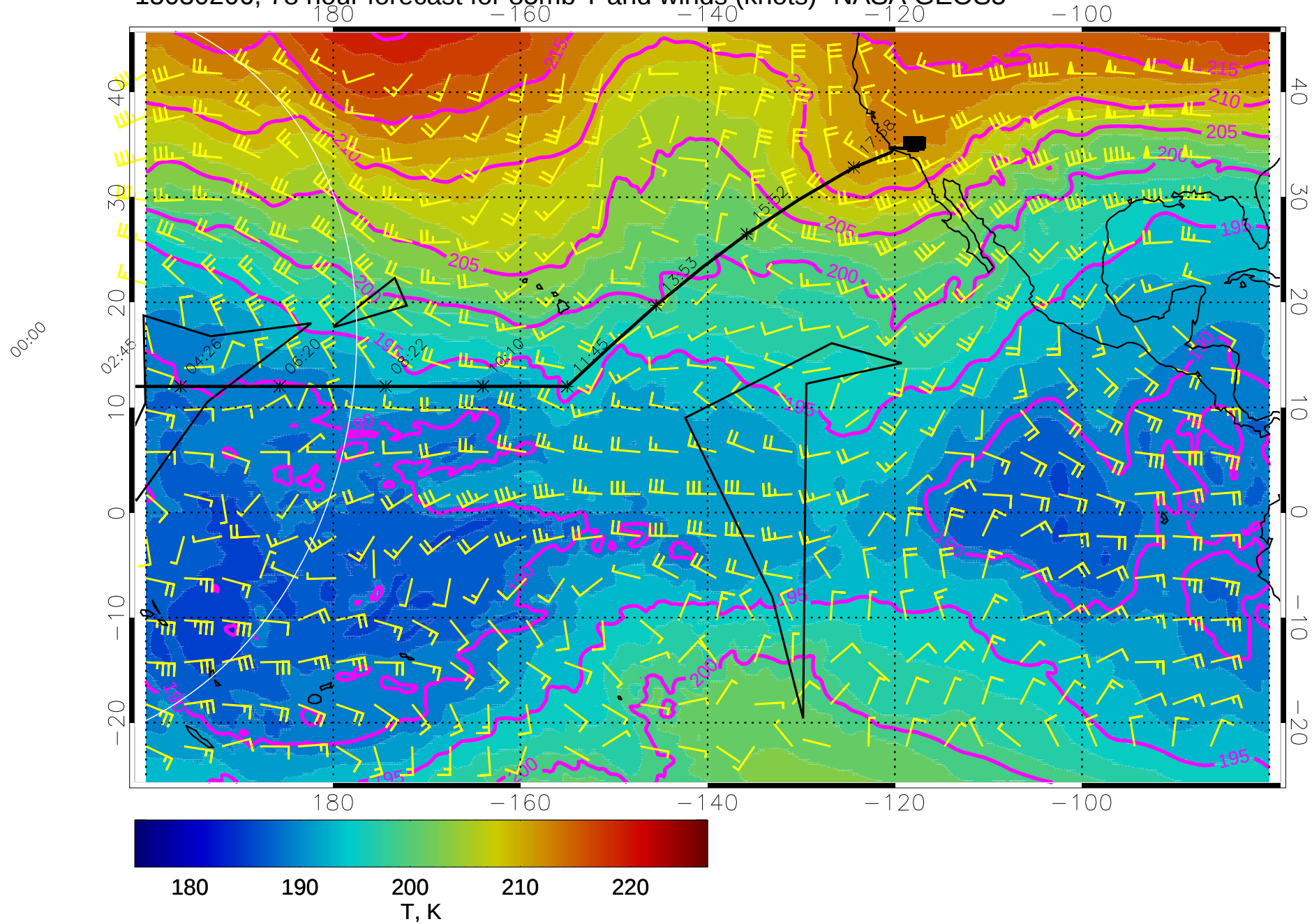
15030206, 78 hour forecast for 85mb T and winds (knots)- NASA GEOS5
