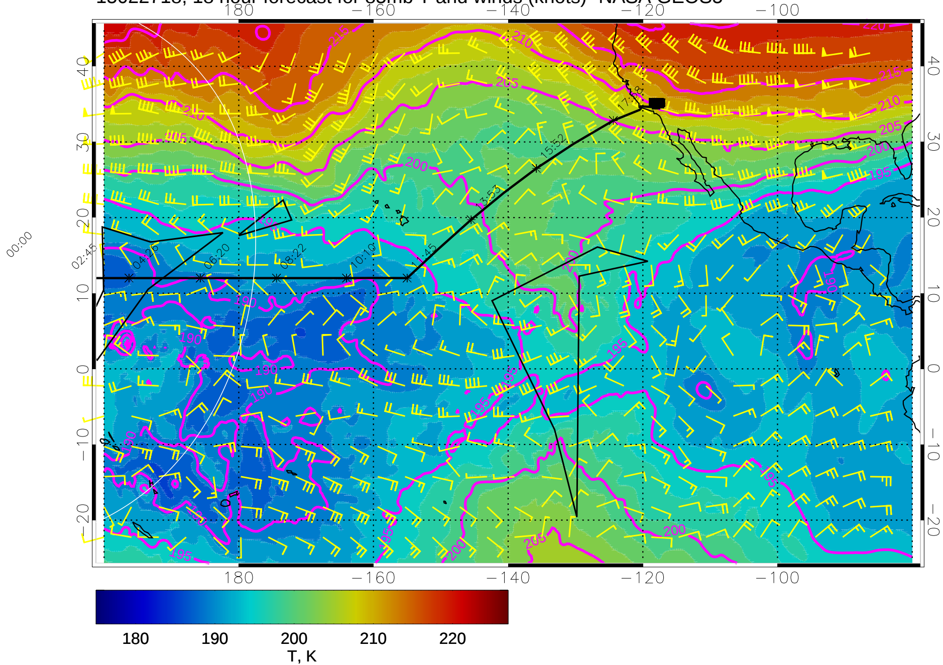
15022718, 18 hour forecast for 85mb T and winds (knots)- NASA GEOS5
