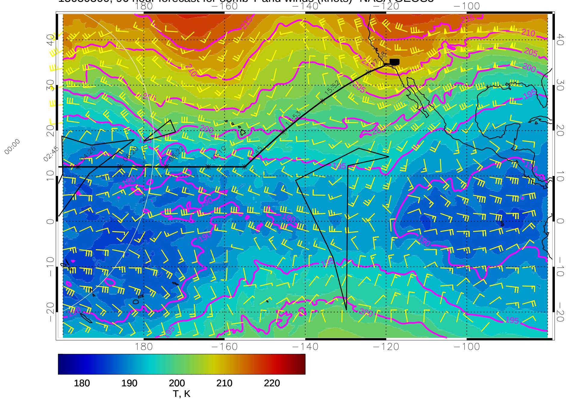
15030300, 96 hour forecast for 85mb T and winds (knots)- NASA GEOS5
