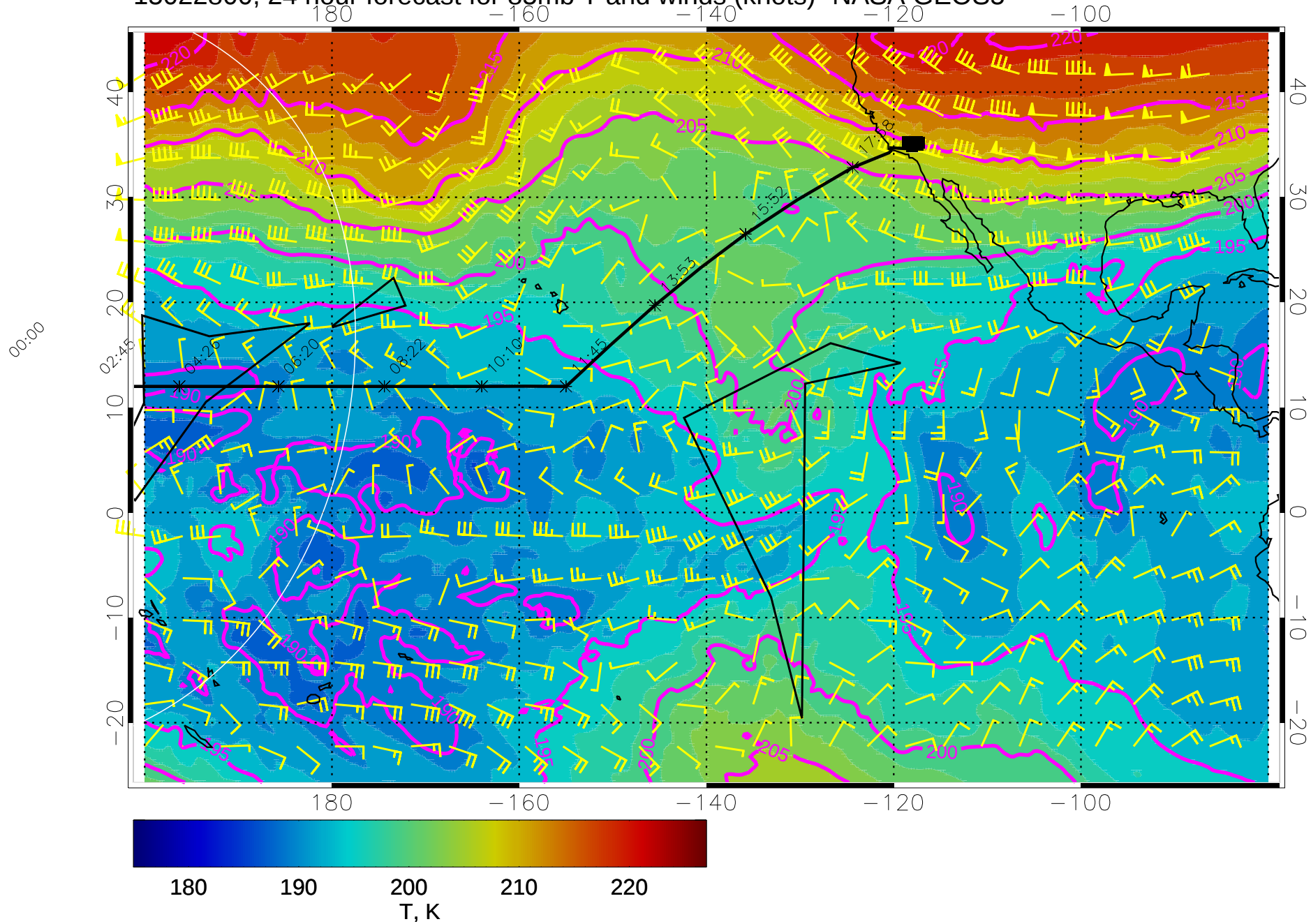
15022800, 24 hour forecast for 85mb T and winds (knots)- NASA GEOS5
