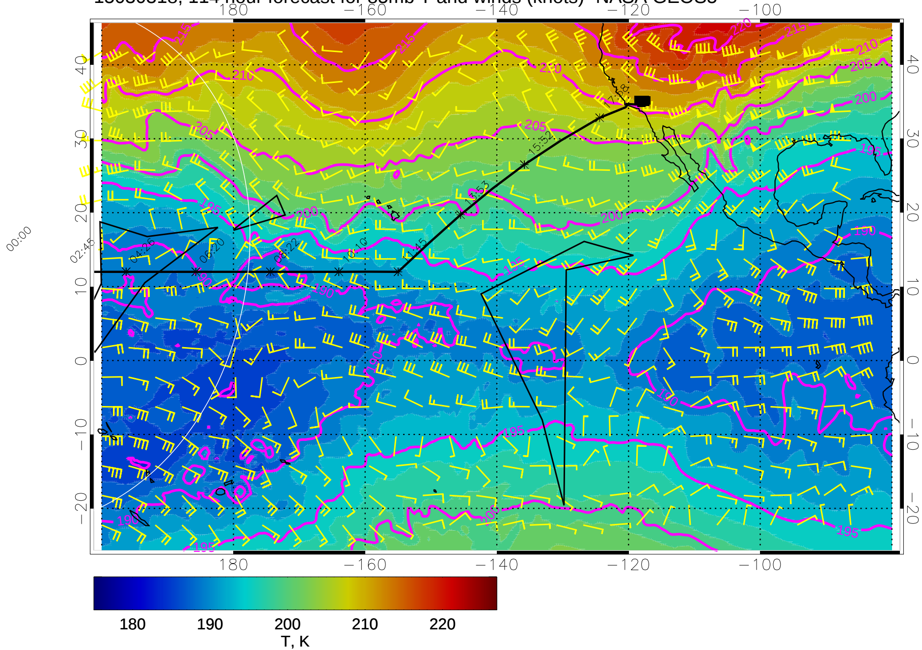
15030318, 114 hour forecast for 85mb T and winds (knots)- NASA GEOS5
