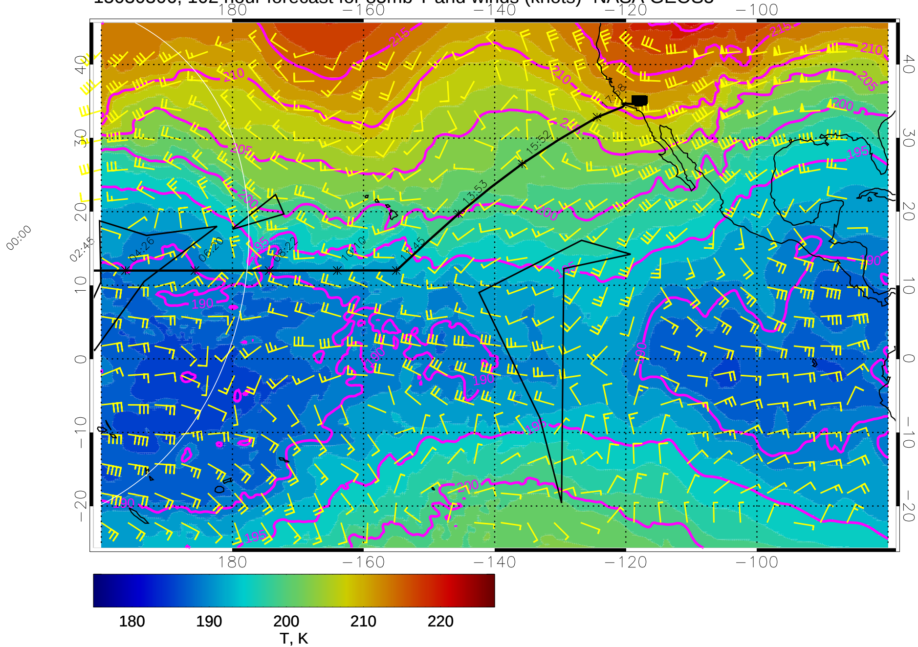
15030306, 102 hour forecast for 85mb T and winds (knots)- NASA GEOS5
