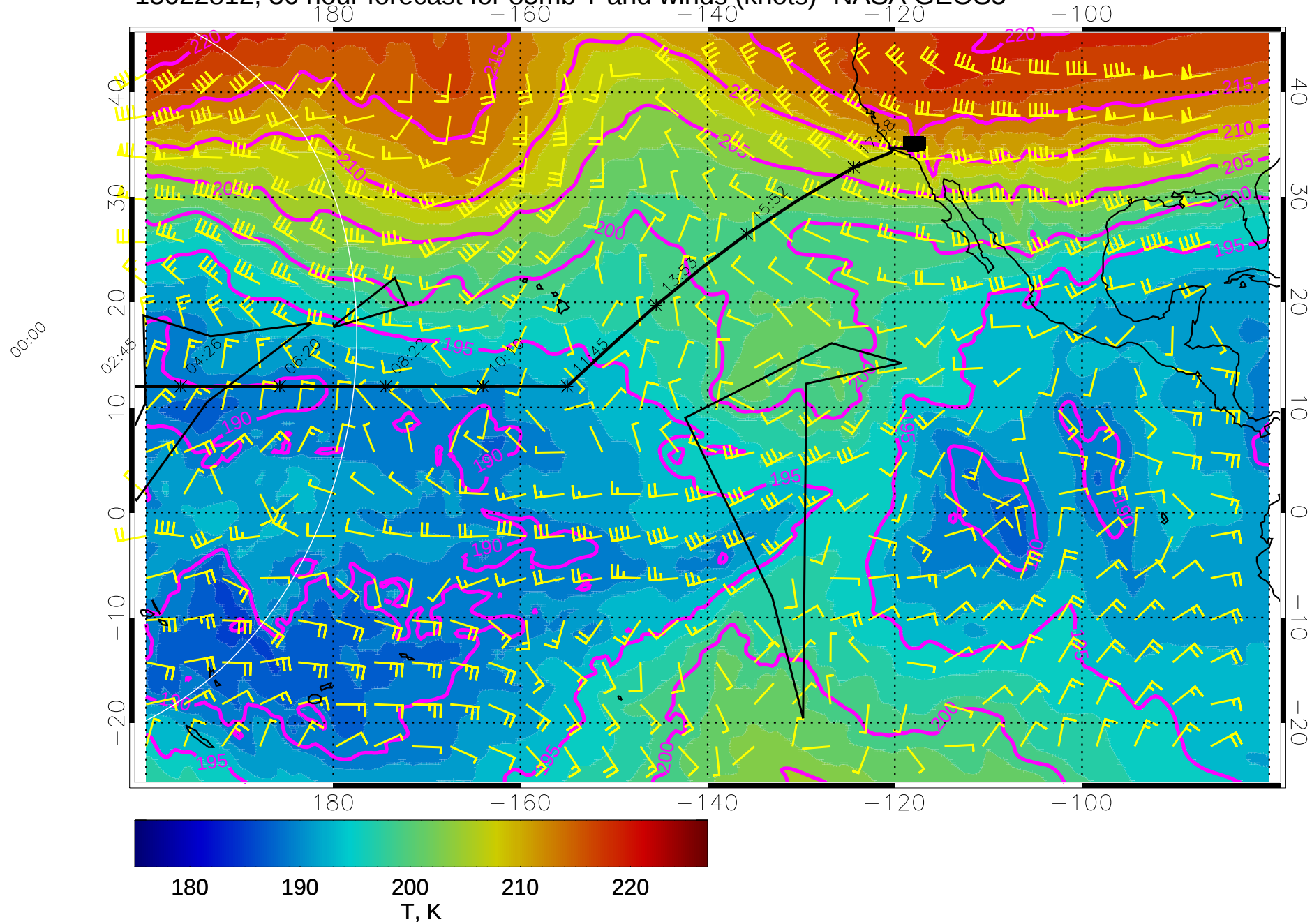
15022812, 36 hour forecast for 85mb T and winds (knots)- NASA GEOS5
