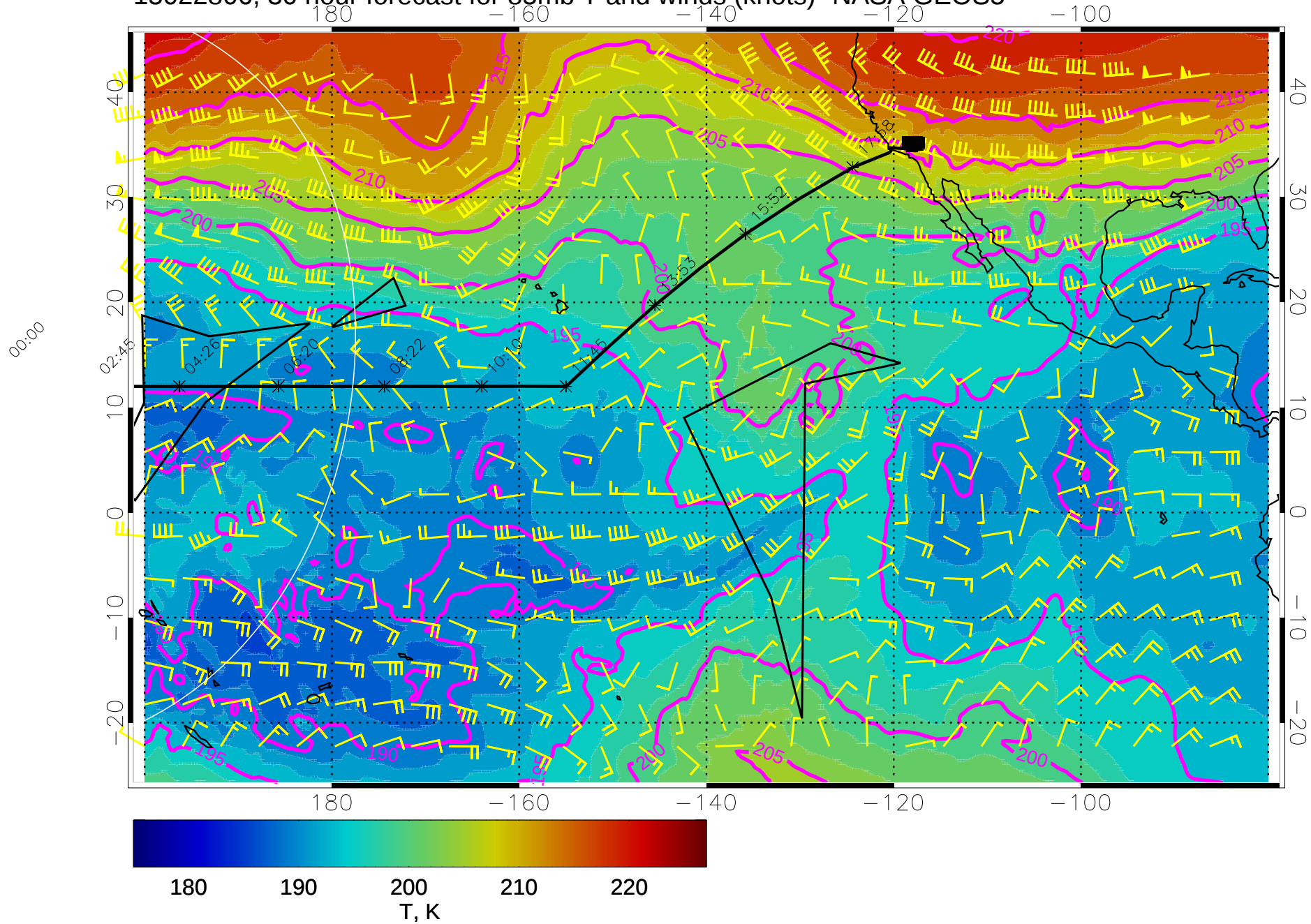
15022806, 30 hour forecast for 85mb T and winds (knots)- NASA GEOS5
