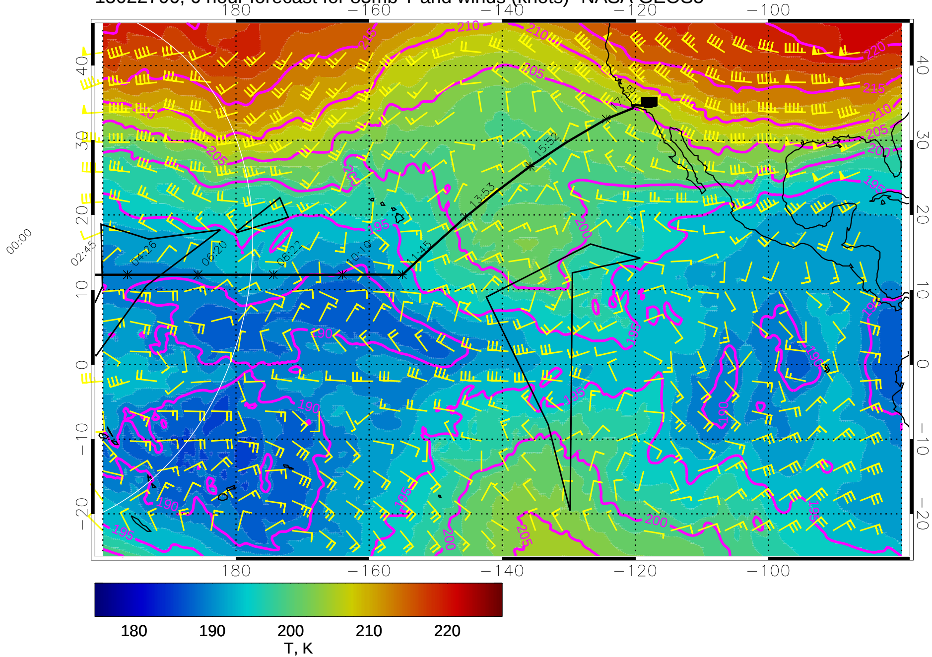
15022706, 6 hour forecast for 85mb T and winds (knots)- NASA GEOS5
