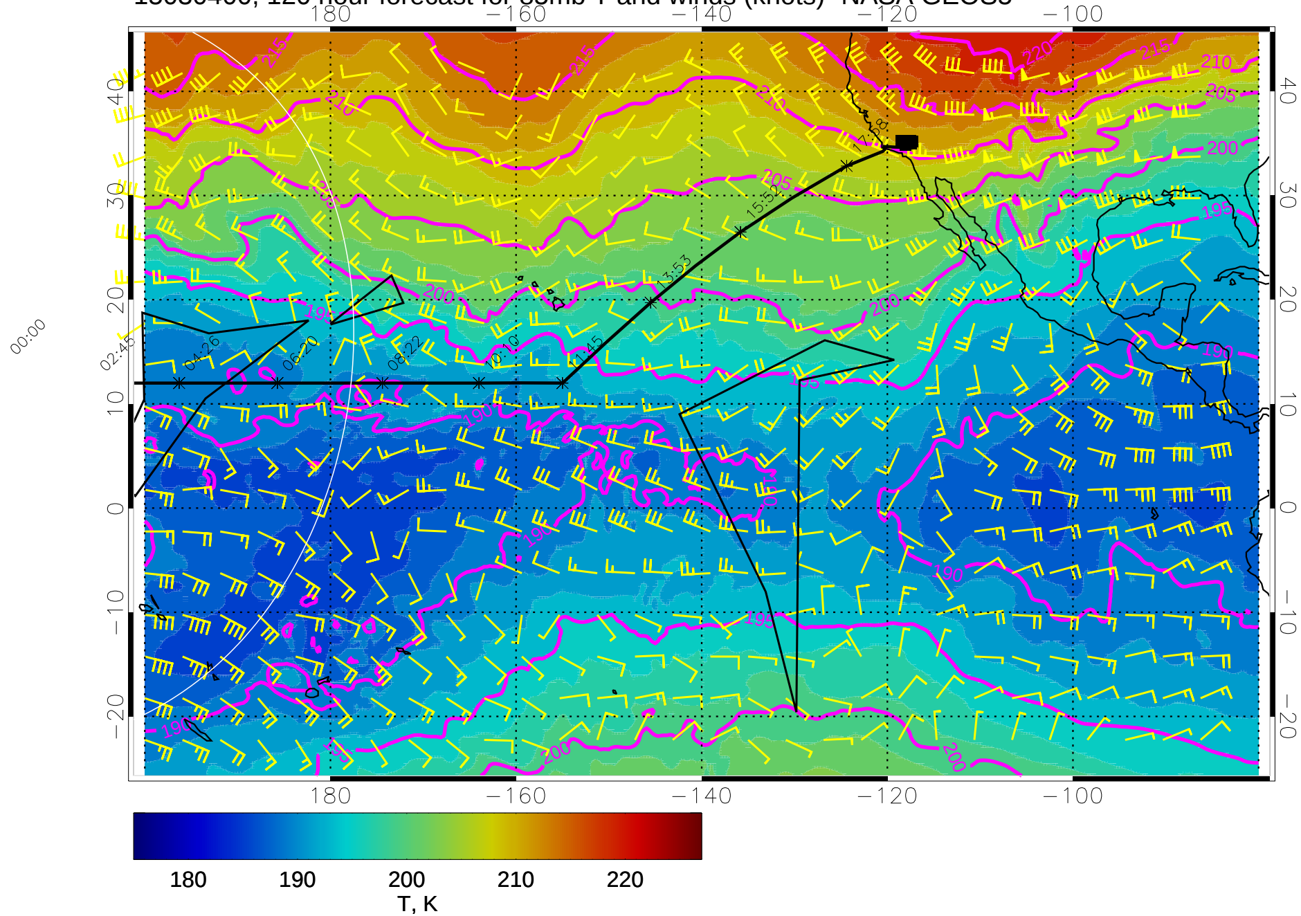
15030400, 120 hour forecast for 85mb T and winds (knots)- NASA GEOS5
