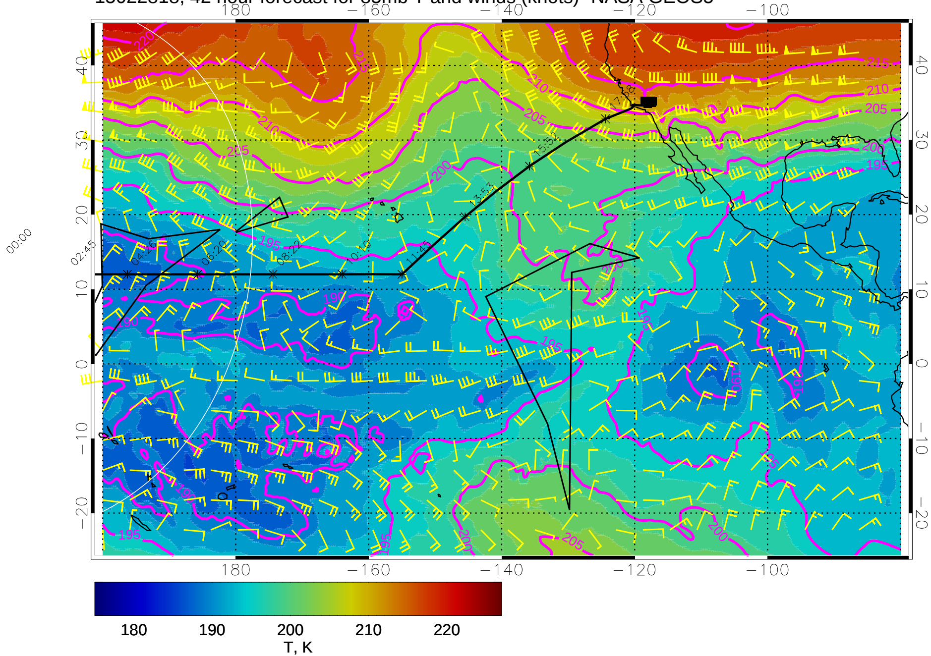
15022818, 42 hour forecast for 85mb T and winds (knots)- NASA GEOS5
