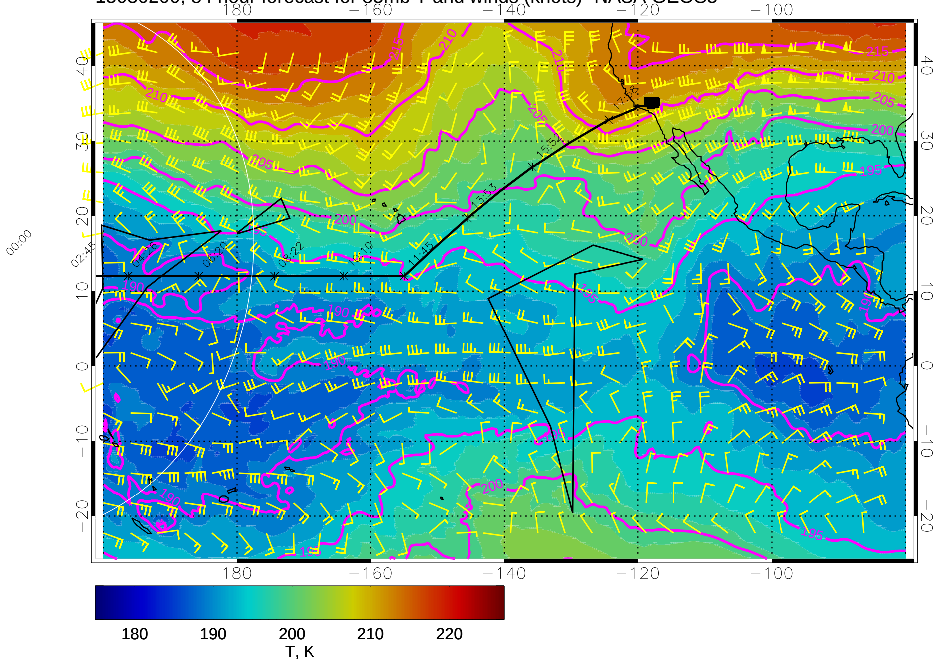
15030200, 84 hour forecast for 85mb T and winds (knots)- NASA GEOS5
