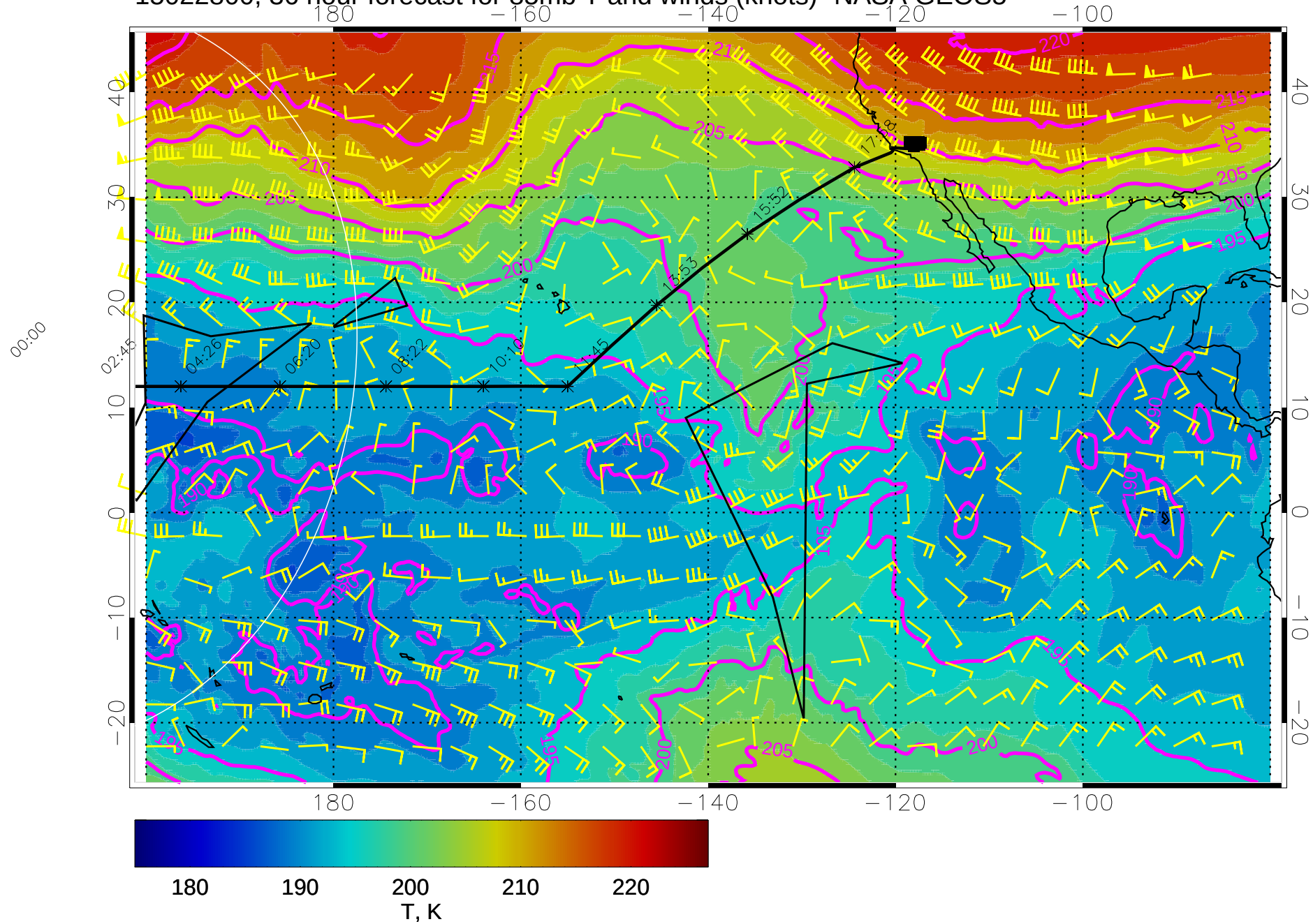
15022800, 36 hour forecast for 85mb T and winds (knots)- NASA GEOS5
