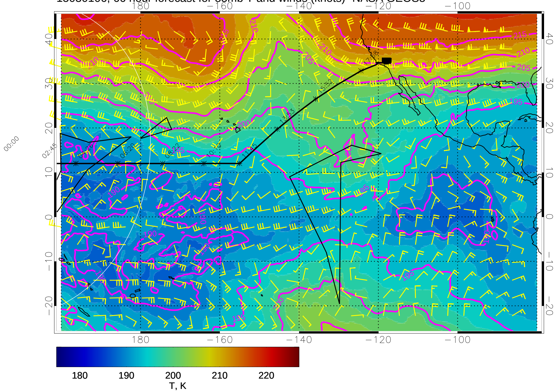
15030106, 66 hour forecast for 85mb T and winds (knots)- NASA GEOS5
