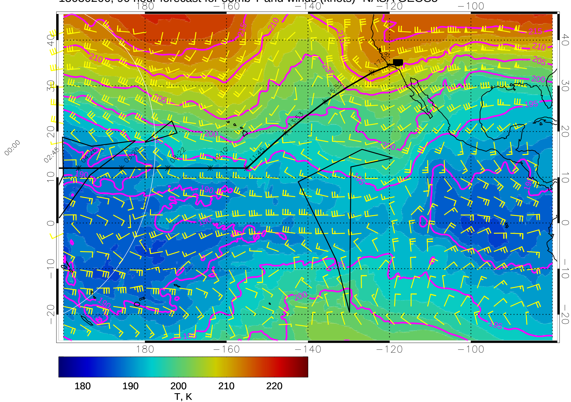
15030206, 90 hour forecast for 85mb T and winds (knots)- NASA GEOS5
