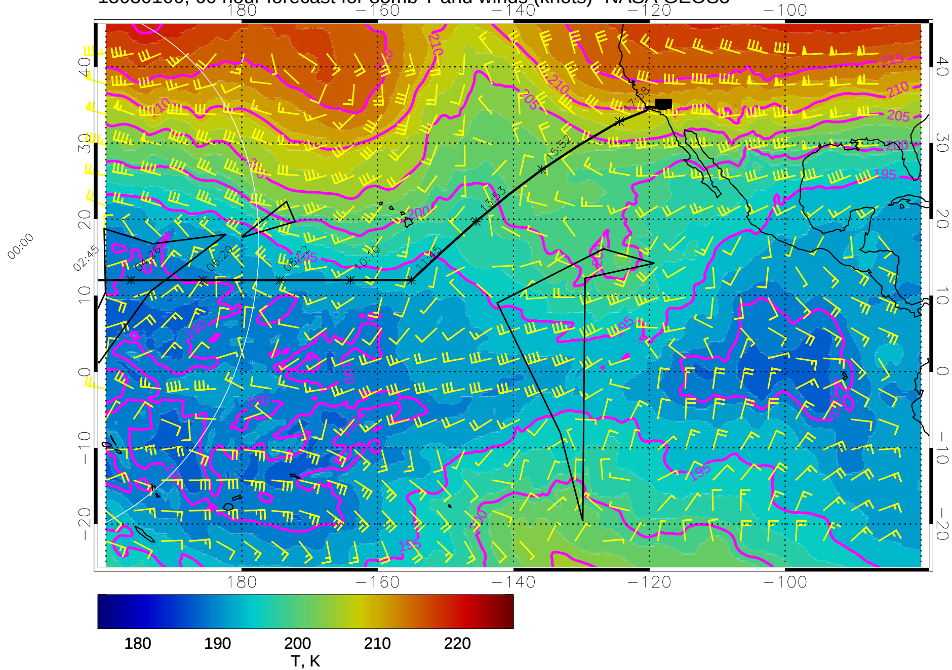
15030100, 60 hour forecast for 85mb T and winds (knots)- NASA GEOS5
