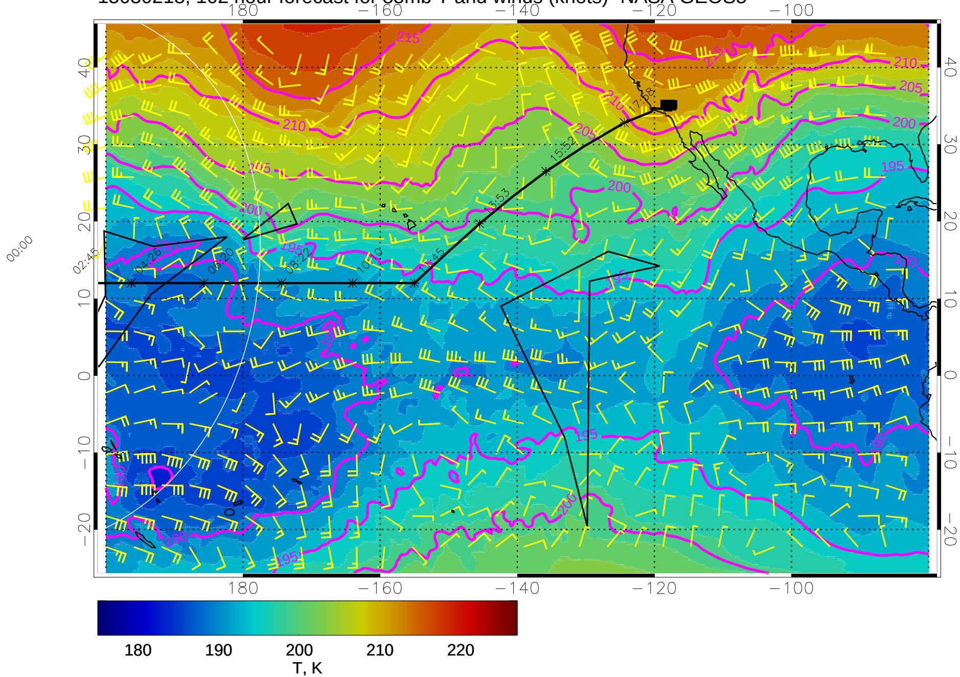
15030218, 102 hour forecast for 85mb T and winds (knots)- NASA GEOS5
