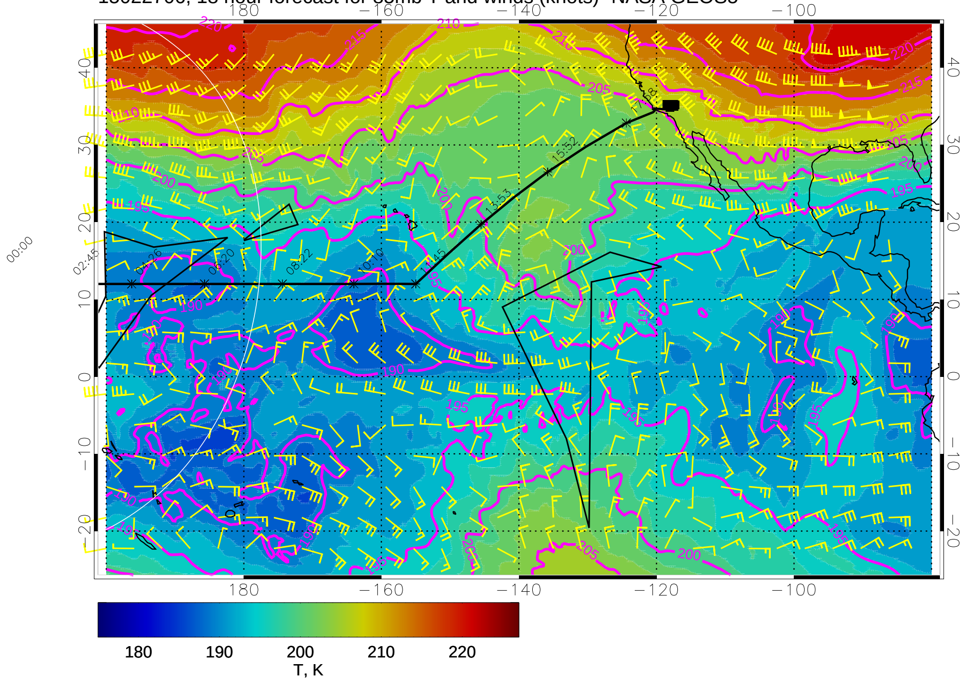
15022706, 18 hour forecast for 85mb T and winds (knots)- NASA GEOS5
