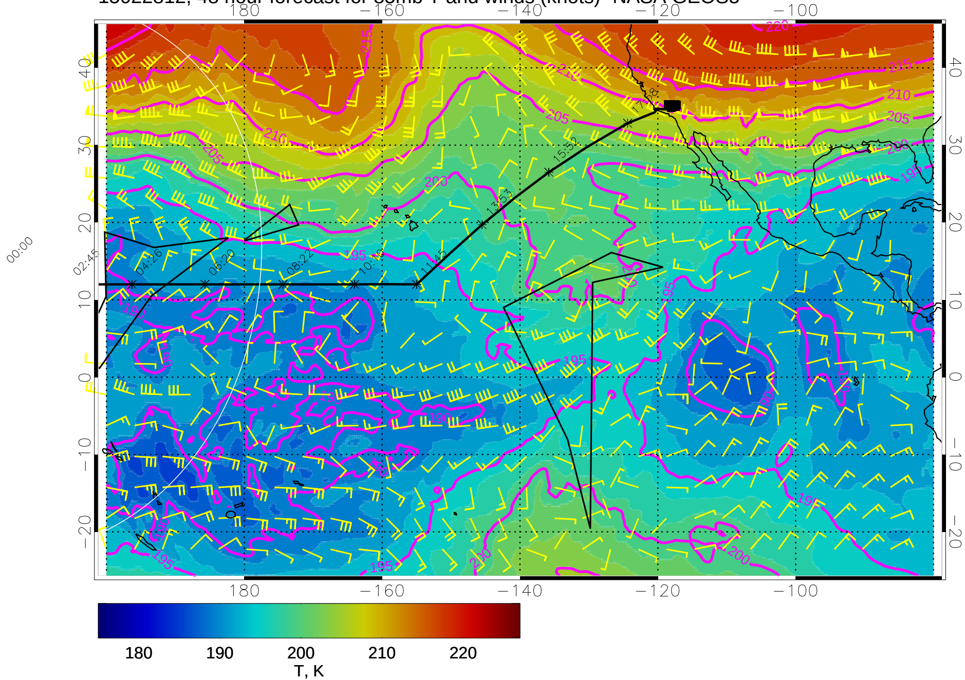
15022812, 48 hour forecast for 85mb T and winds (knots)- NASA GEOS5
