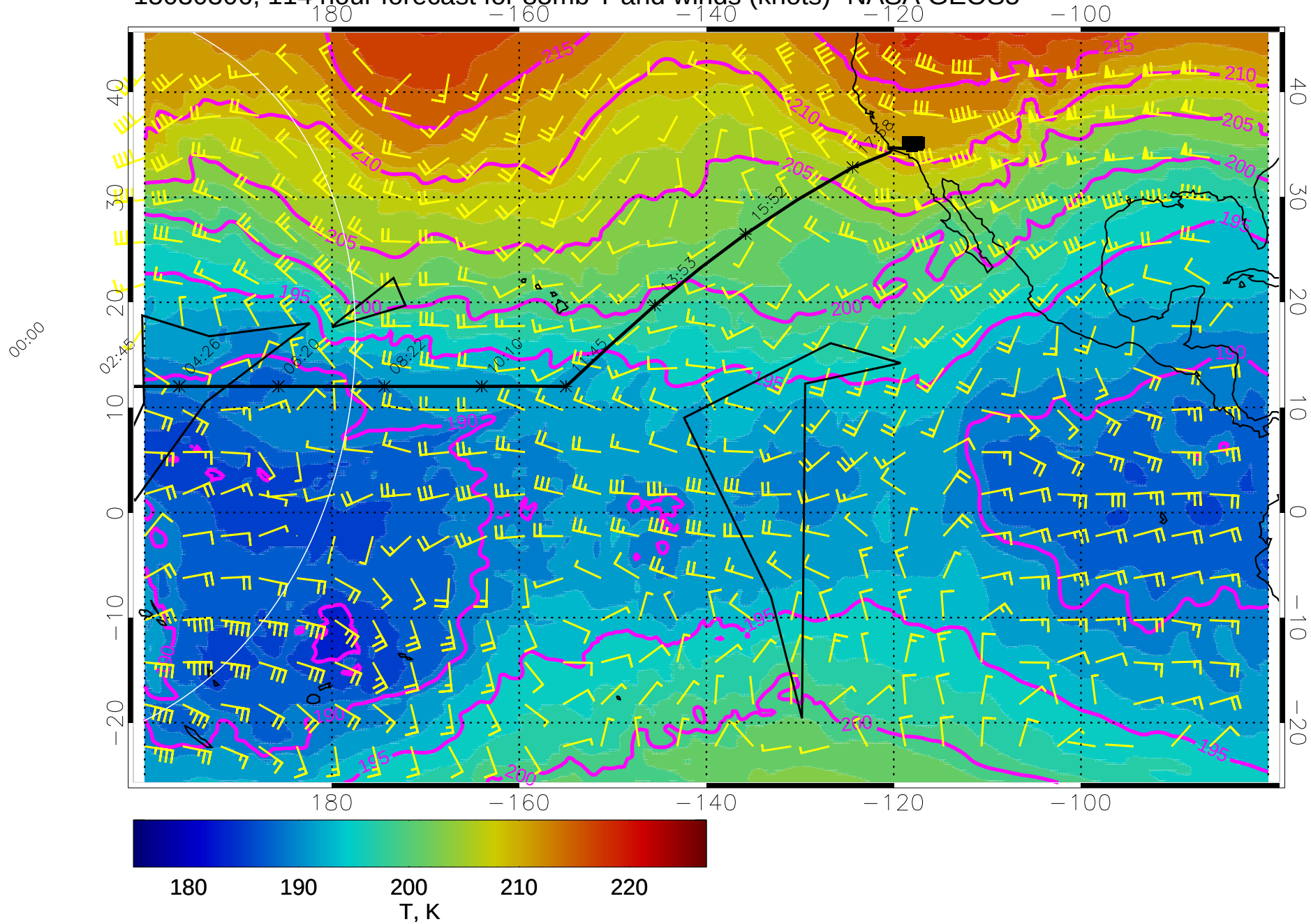
15030306, 114 hour forecast for 85mb T and winds (knots)- NASA GEOS5
