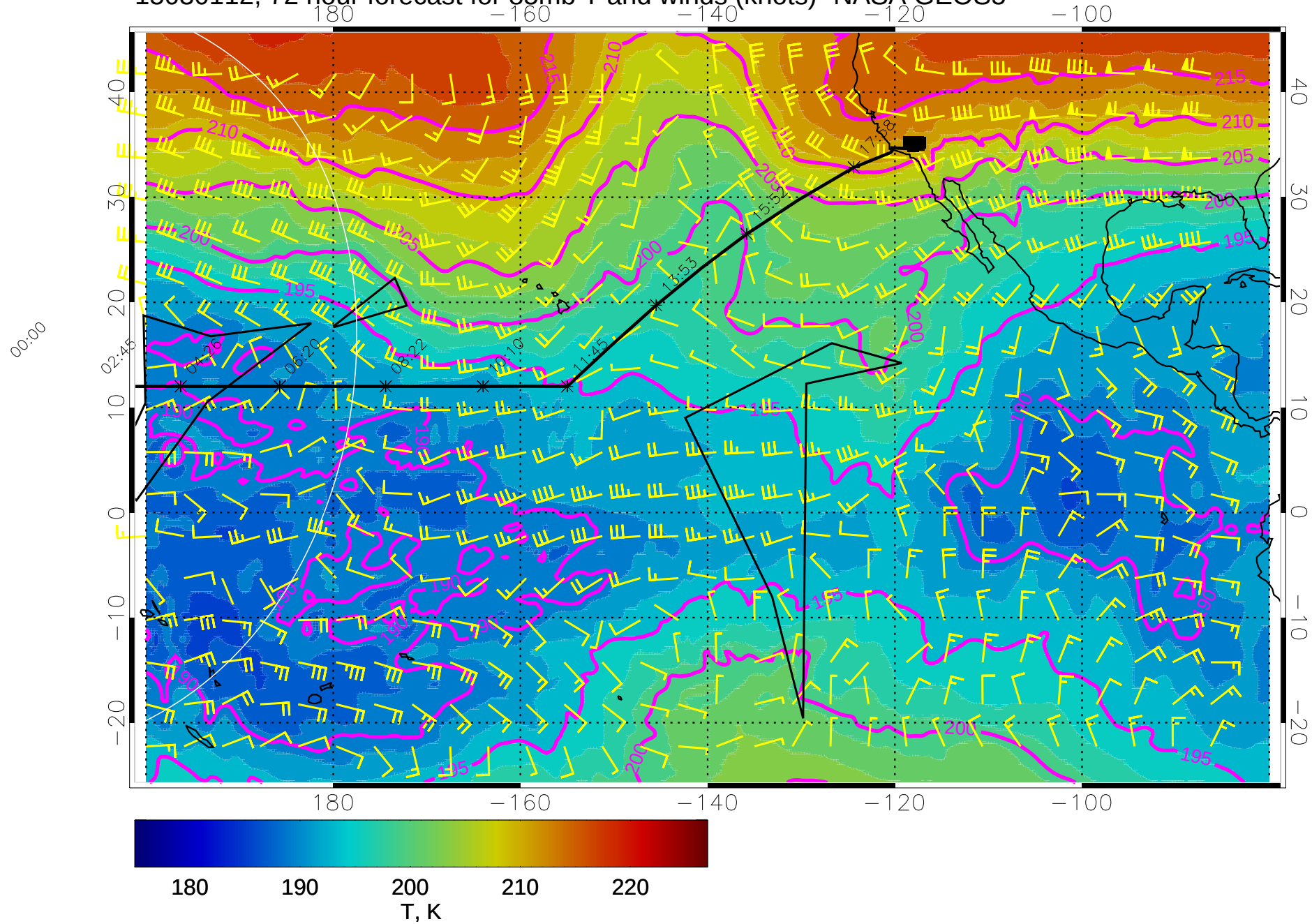
15030112, 72 hour forecast for 85mb T and winds (knots)- NASA GEOS5
