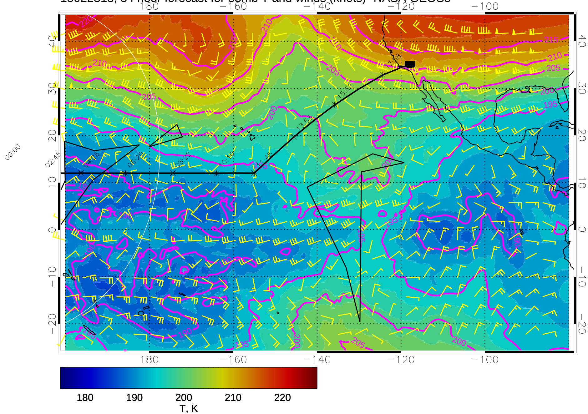
15022818, 54 hour forecast for 85mb T and winds (knots)- NASA GEOS5
