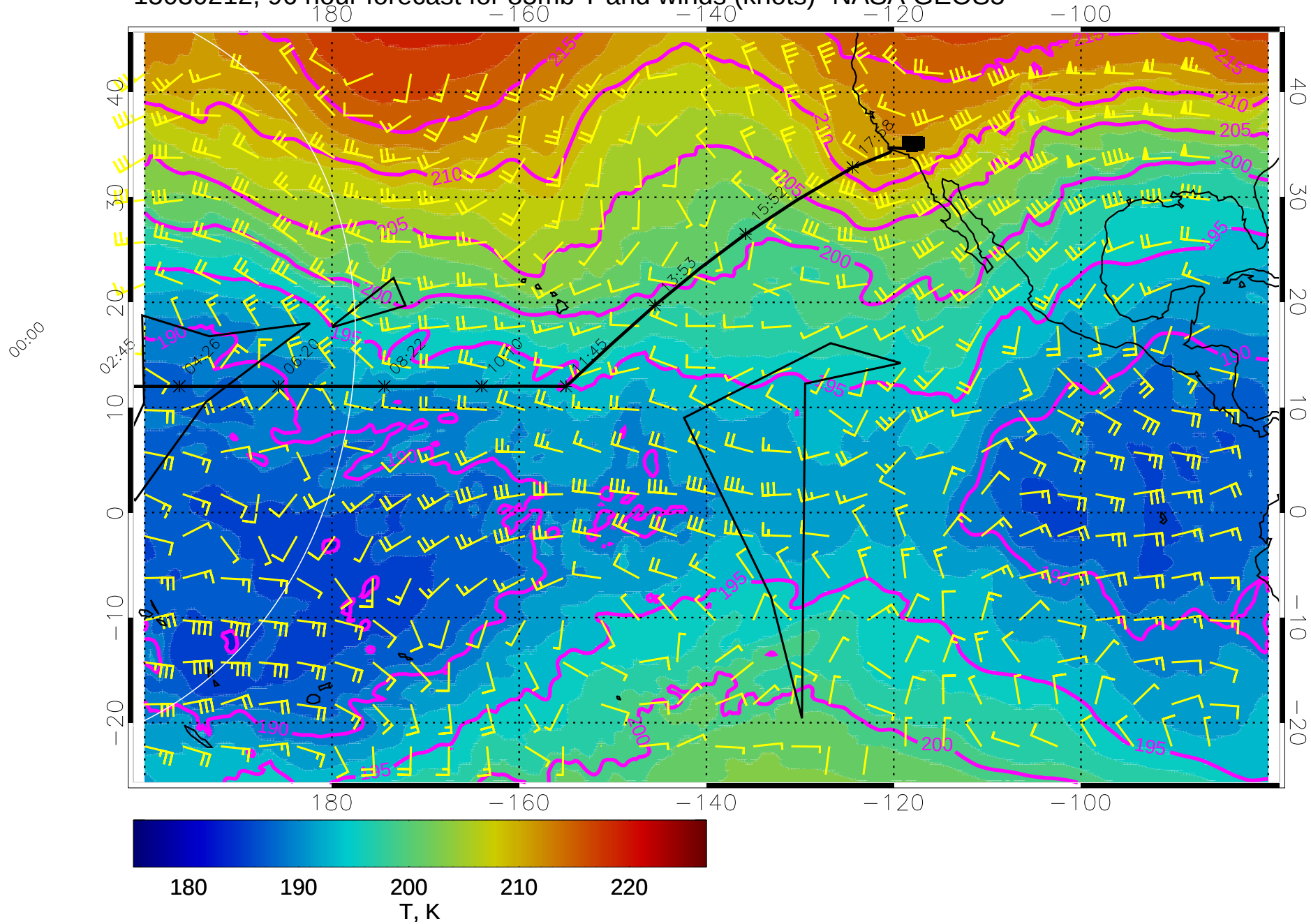
15030212, 96 hour forecast for 85mb T and winds (knots)- NASA GEOS5
