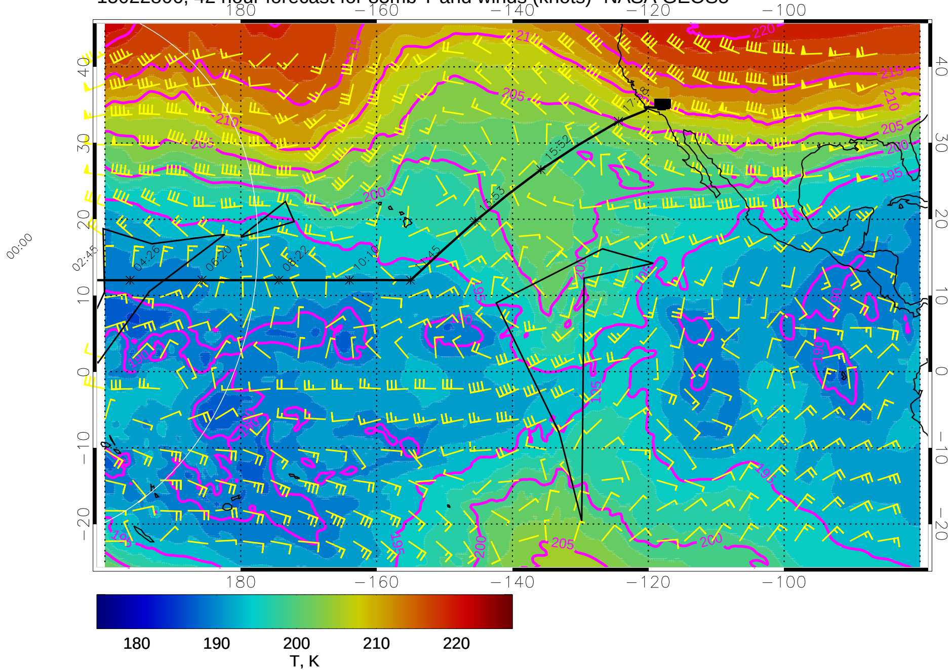
15022806, 42 hour forecast for 85mb T and winds (knots)- NASA GEOS5
