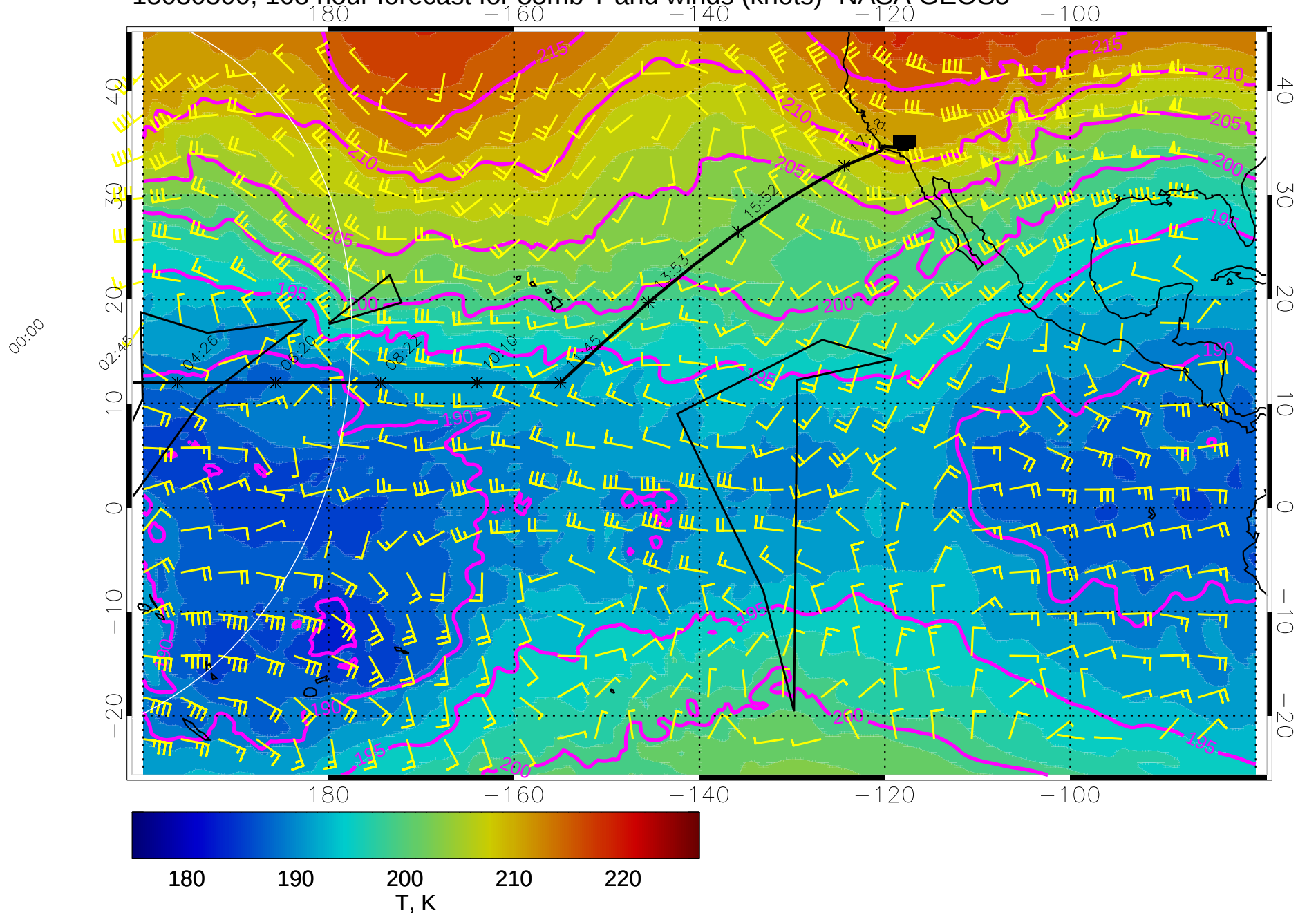
15030300, 108 hour forecast for 85mb T and winds (knots)- NASA GEOS5
