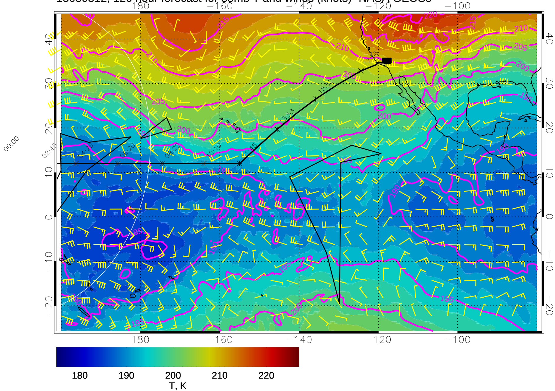
15030312, 120 hour forecast for 85mb T and winds (knots)- NASA GEOS5
