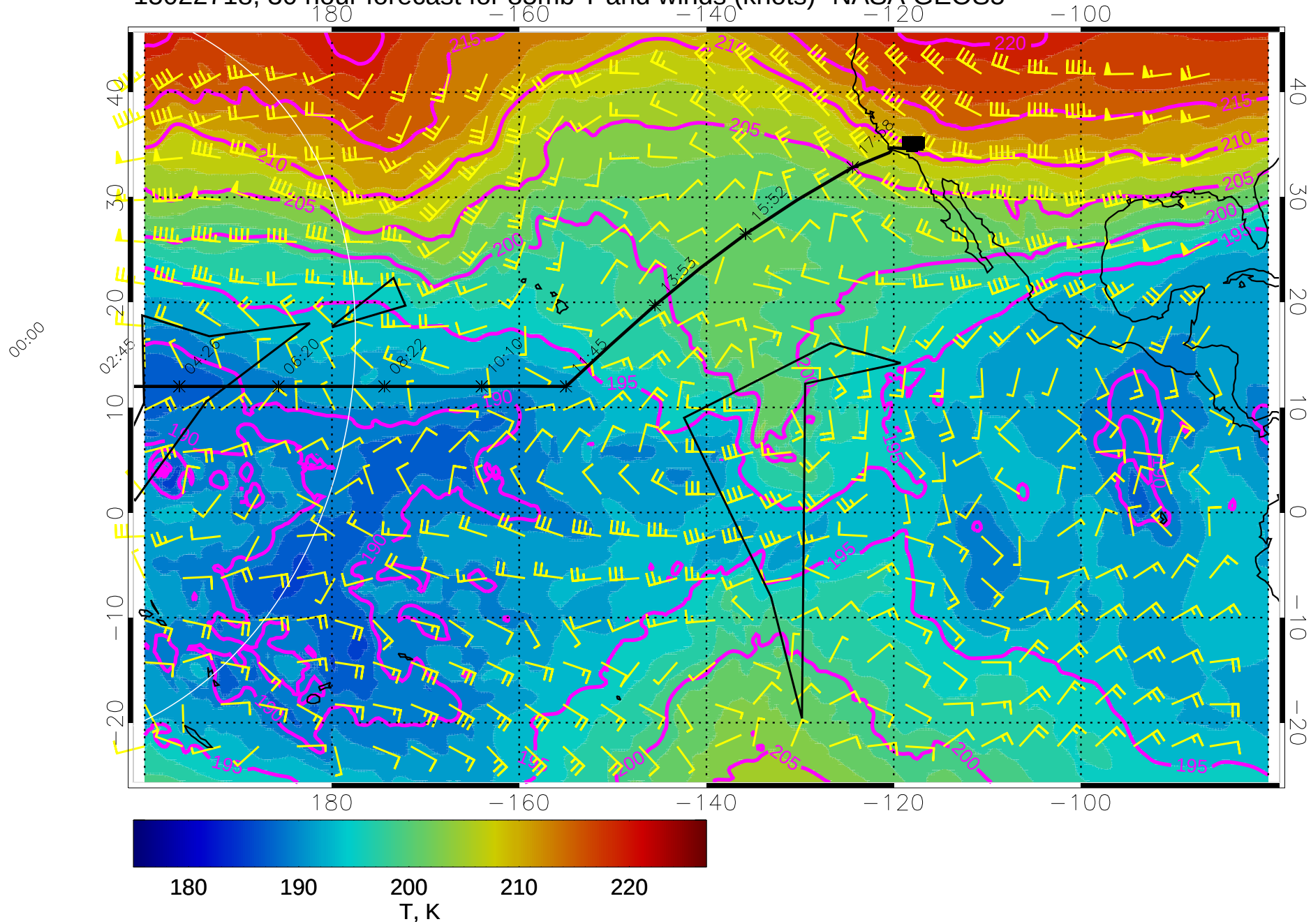
15022718, 30 hour forecast for 85mb T and winds (knots)- NASA GEOS5
