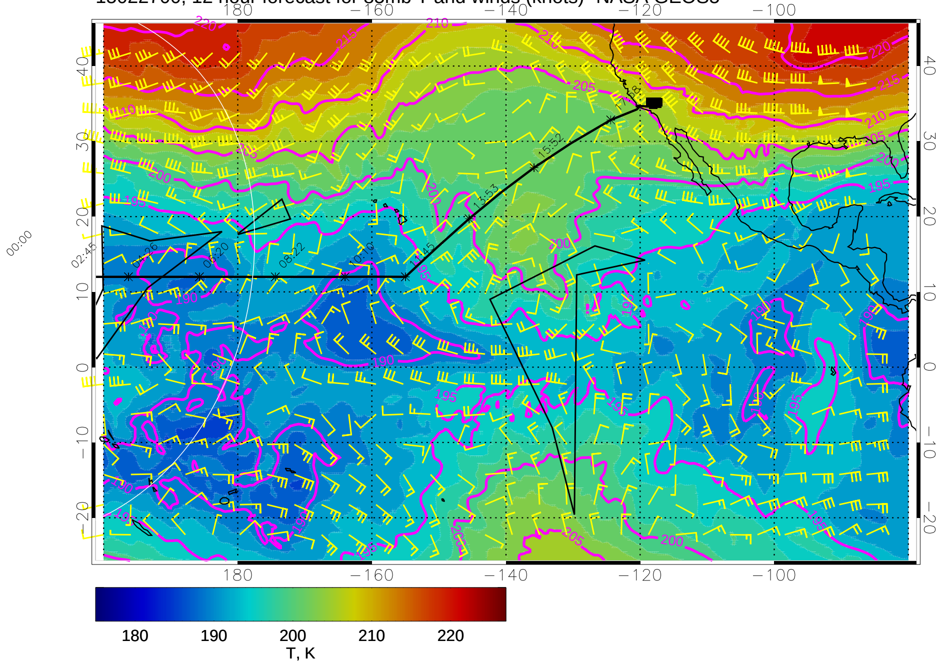
15022700, 12 hour forecast for 85mb T and winds (knots)- NASA GEOS5
