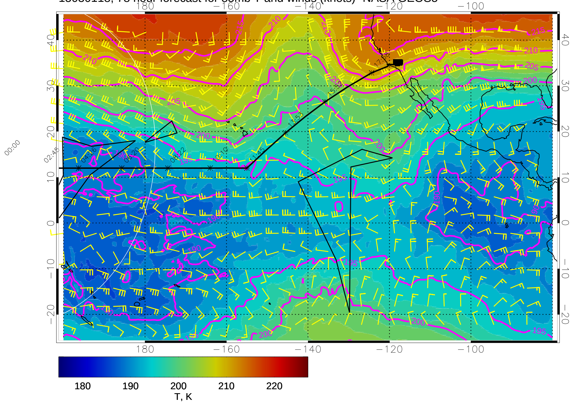
15030118, 78 hour forecast for 85mb T and winds (knots)- NASA GEOS5
