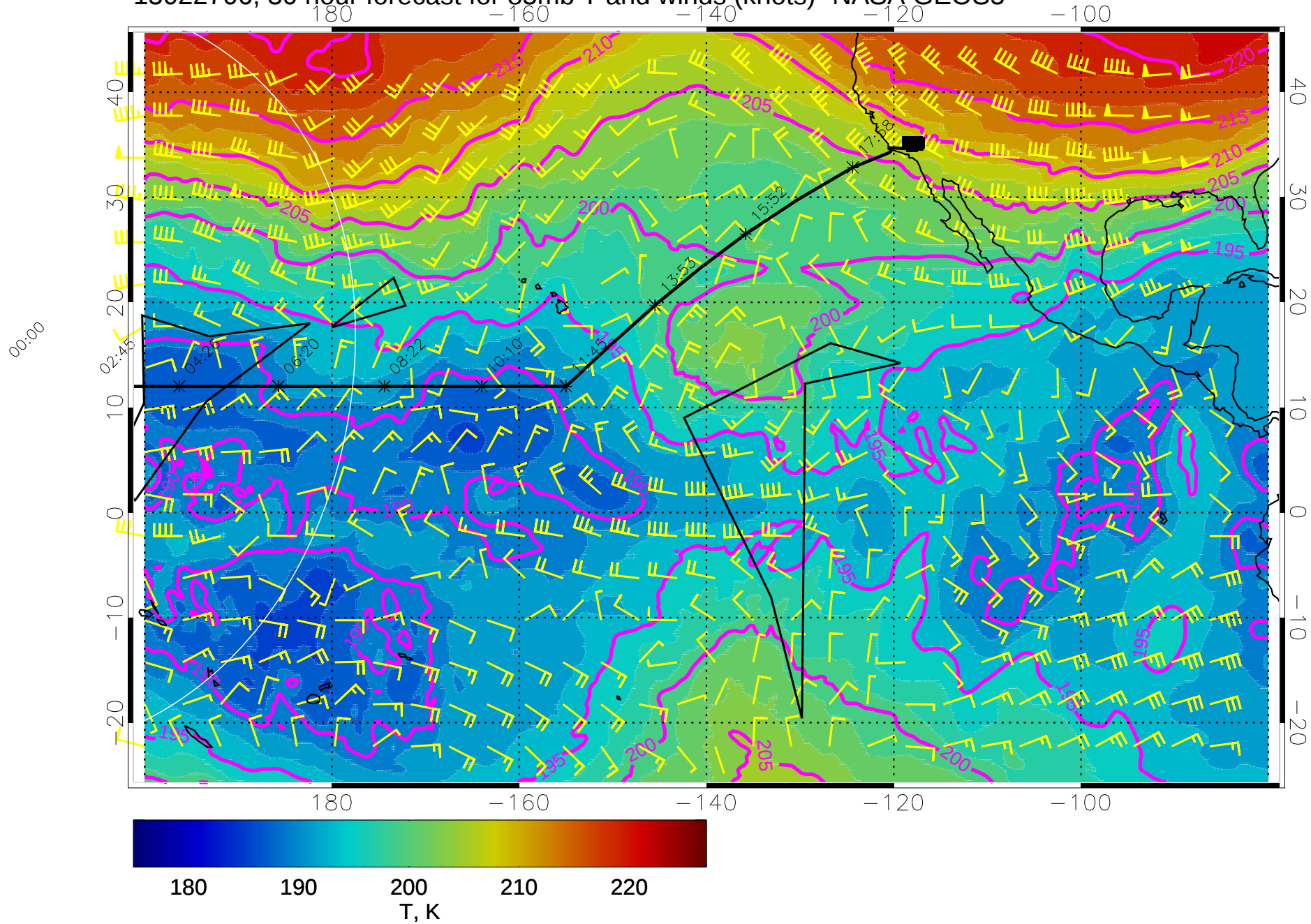
15022706, 30 hour forecast for 85mb T and winds (knots)- NASA GEOS5
