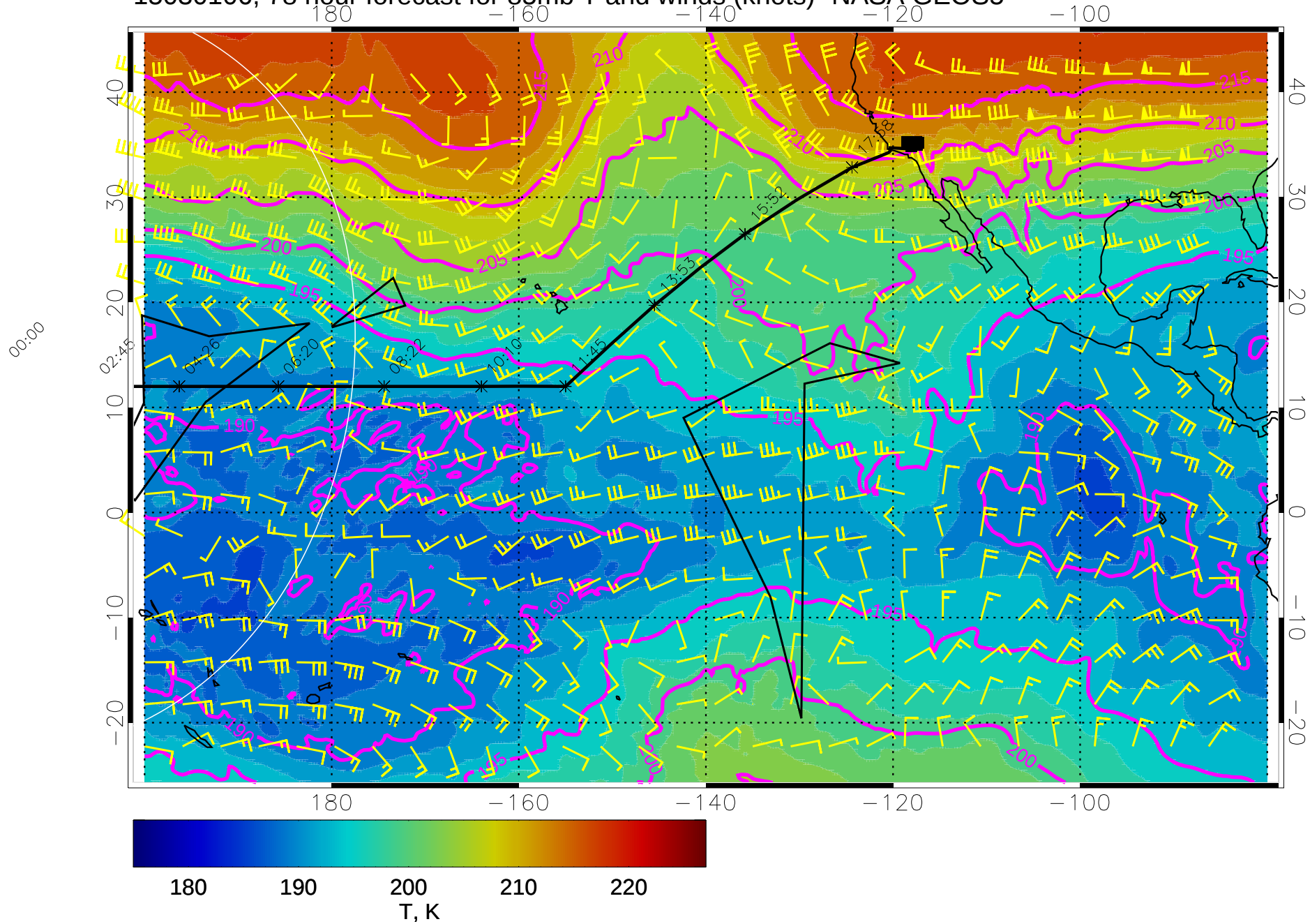
15030106, 78 hour forecast for 85mb T and winds (knots)- NASA GEOS5
