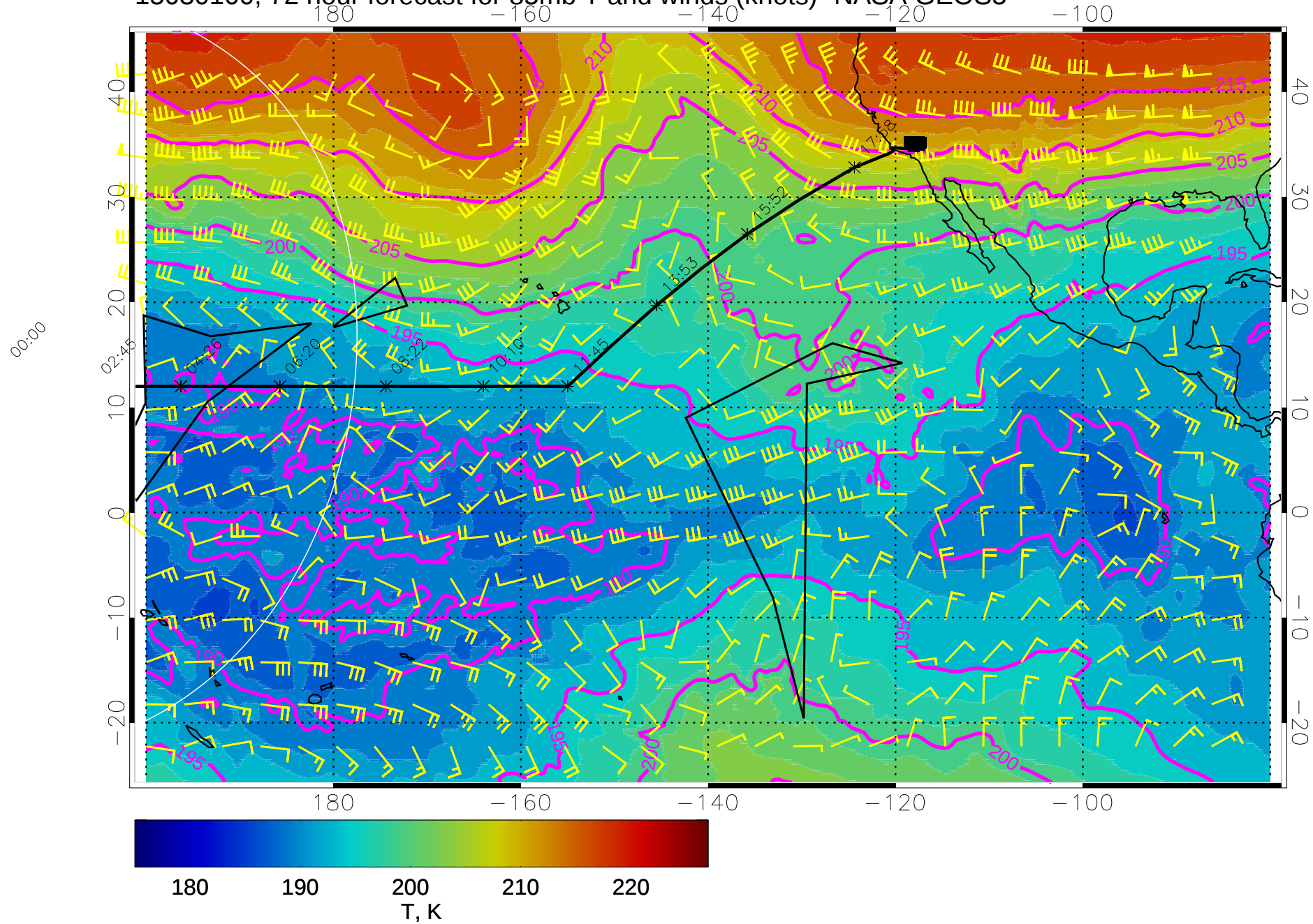
15030100, 72 hour forecast for 85mb T and winds (knots)- NASA GEOS5
