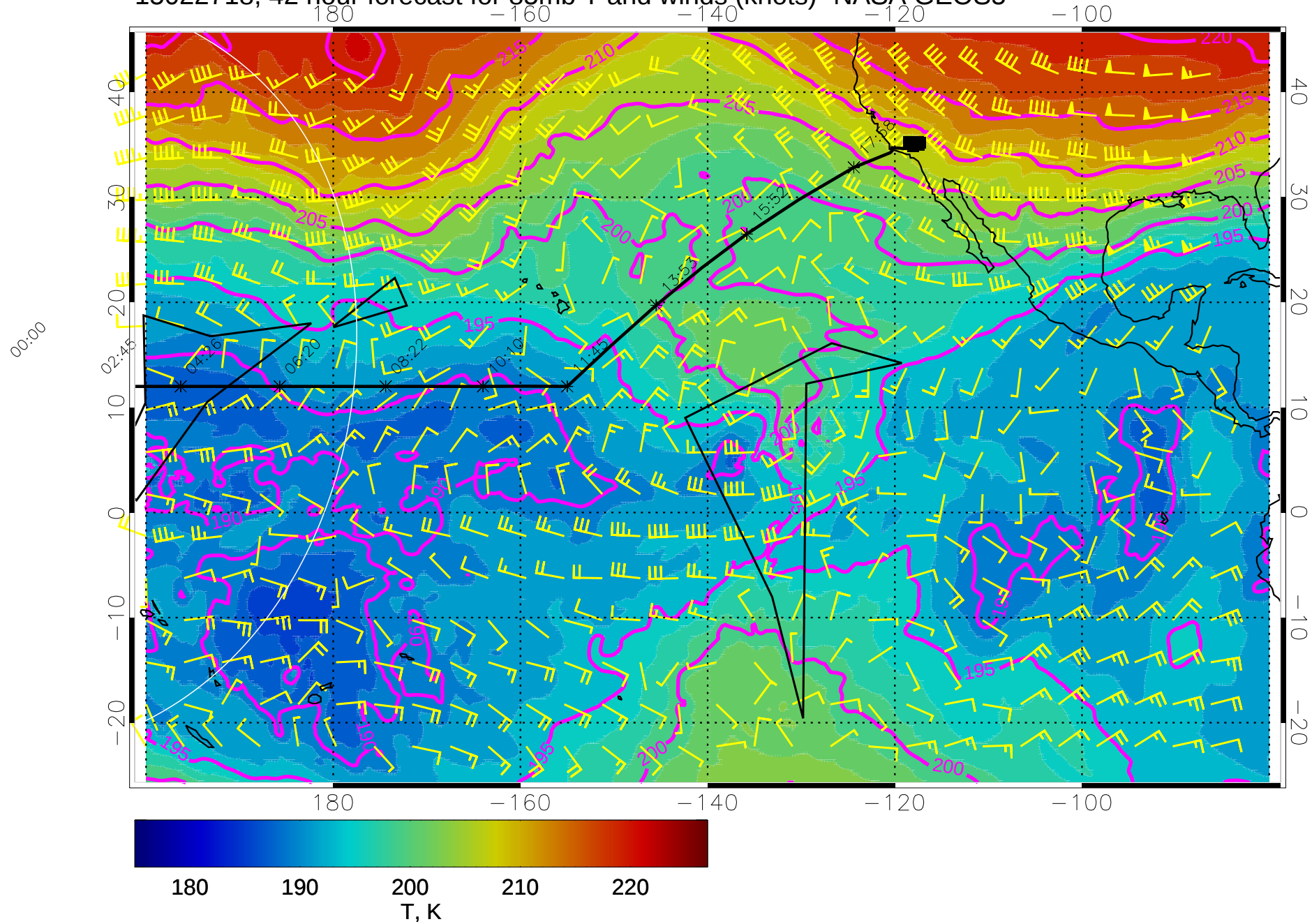
15022718, 42 hour forecast for 85mb T and winds (knots)- NASA GEOS5
