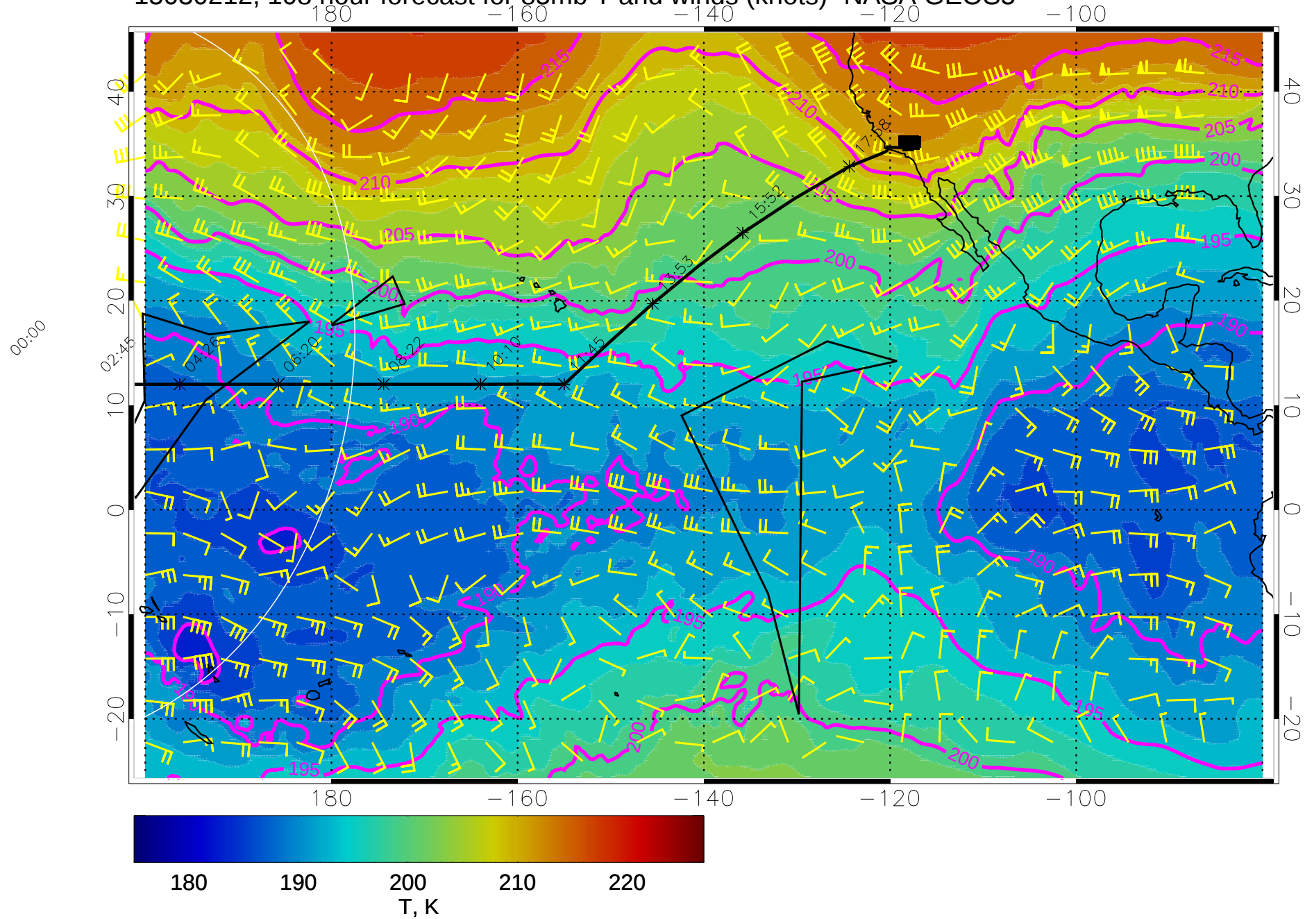
15030212, 108 hour forecast for 85mb T and winds (knots)- NASA GEOS5
