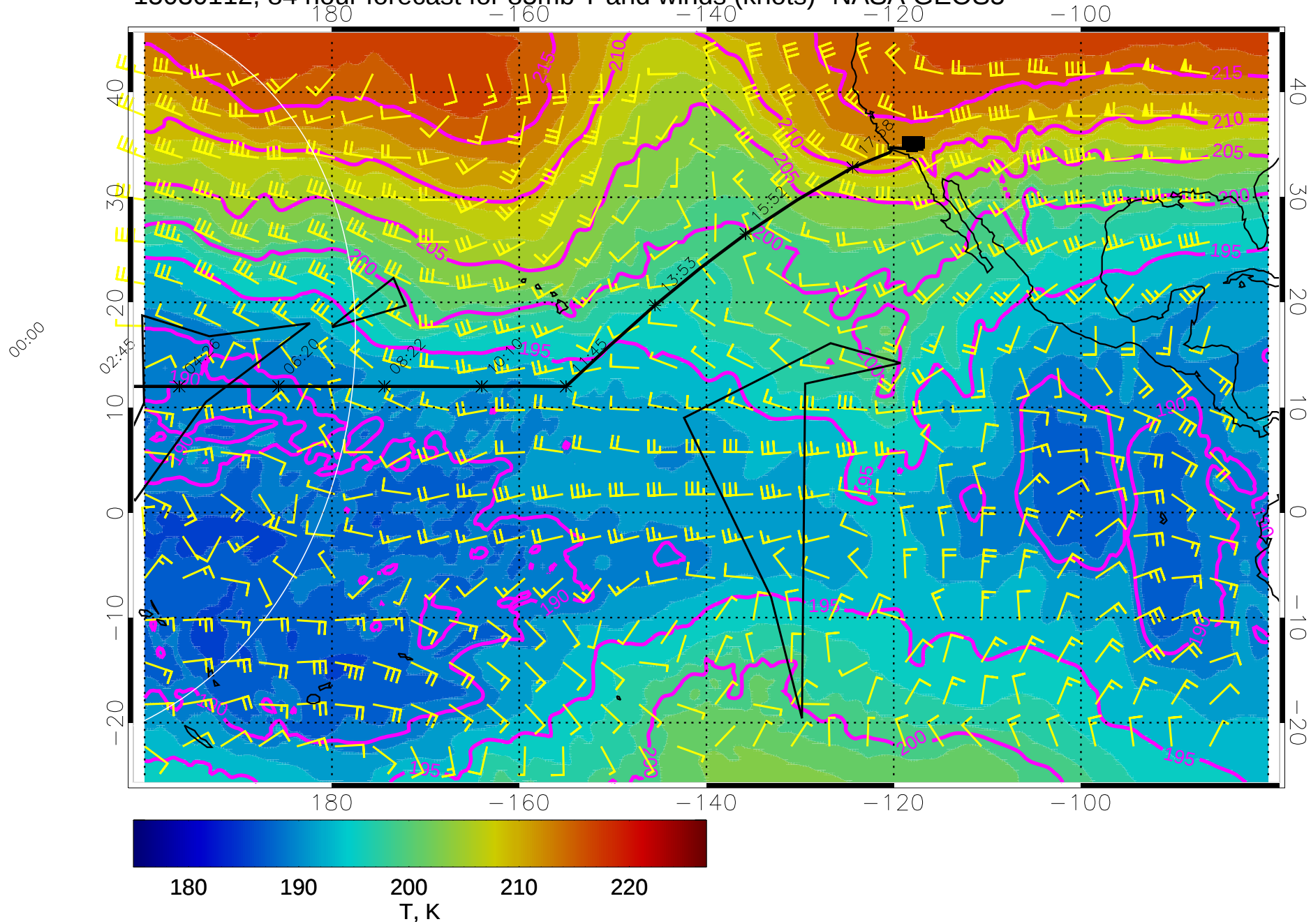
15030112, 84 hour forecast for 85mb T and winds (knots)- NASA GEOS5
