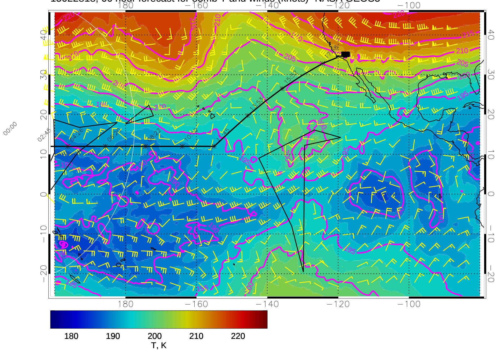
15022818, 66 hour forecast for 85mb T and winds (knots)- NASA GEOS5
