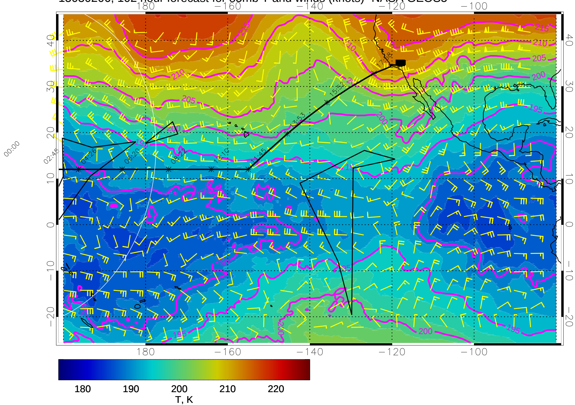
15030206, 102 hour forecast for 85mb T and winds (knots)- NASA GEOS5
