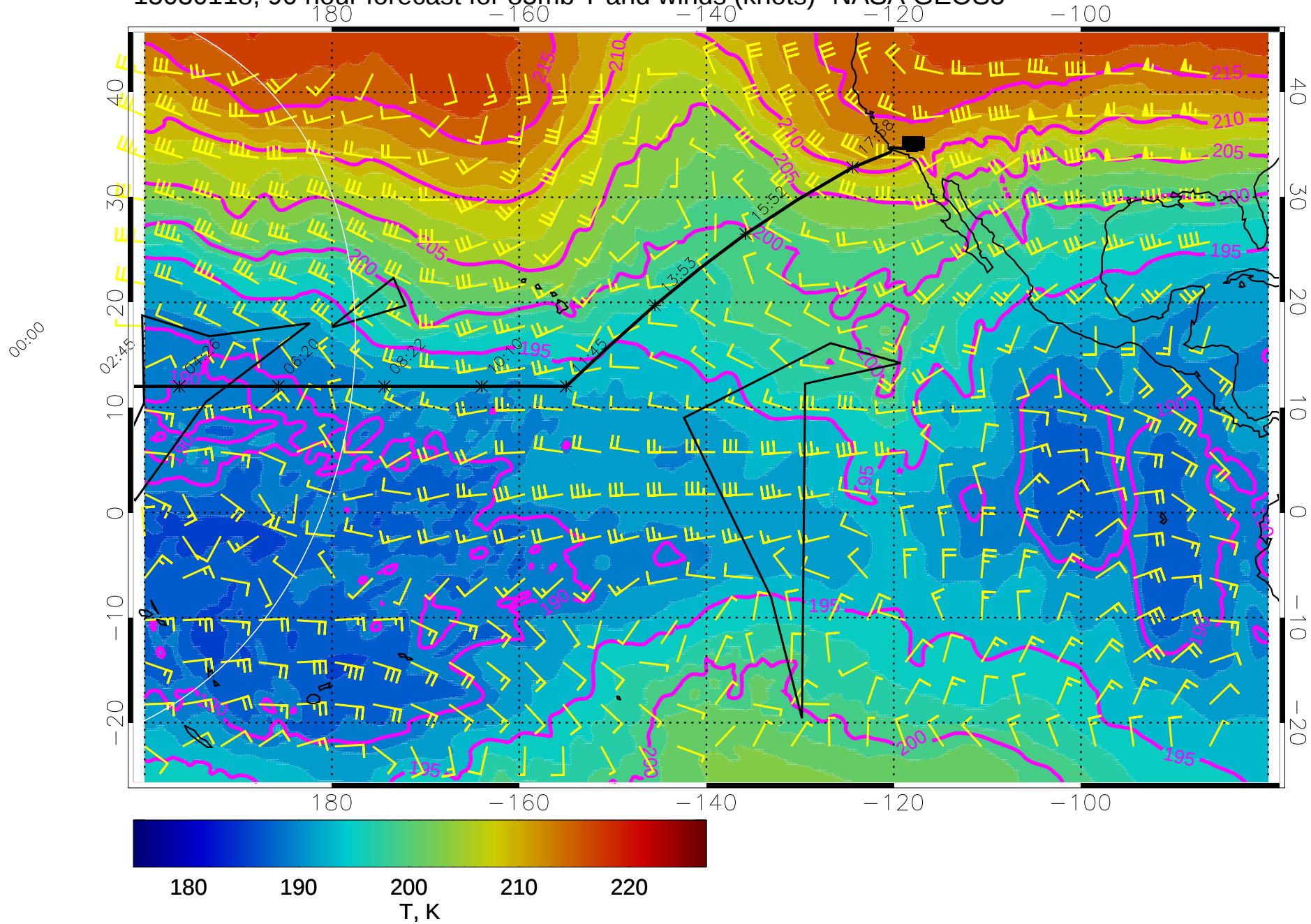
15030118, 90 hour forecast for 85mb T and winds (knots)- NASA GEOS5
