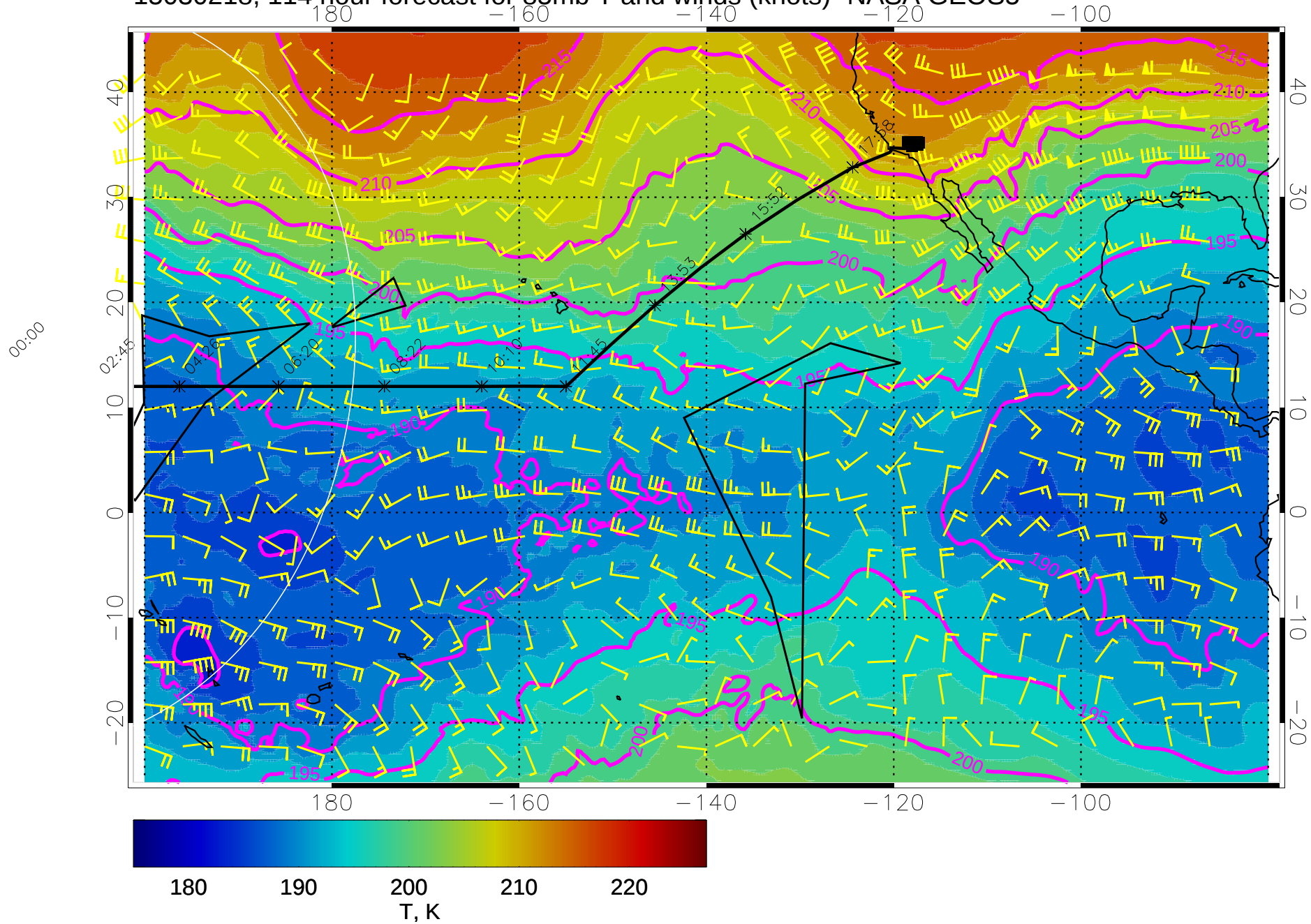
15030218, 114 hour forecast for 85mb T and winds (knots)- NASA GEOS5
