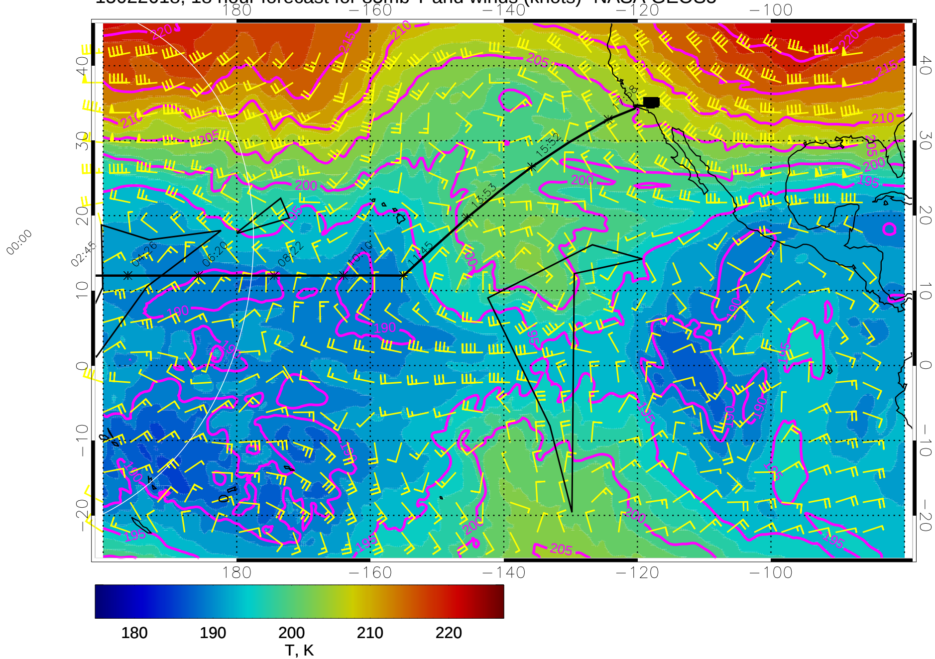
15022618, 18 hour forecast for 85mb T and winds (knots)- NASA GEOS5
