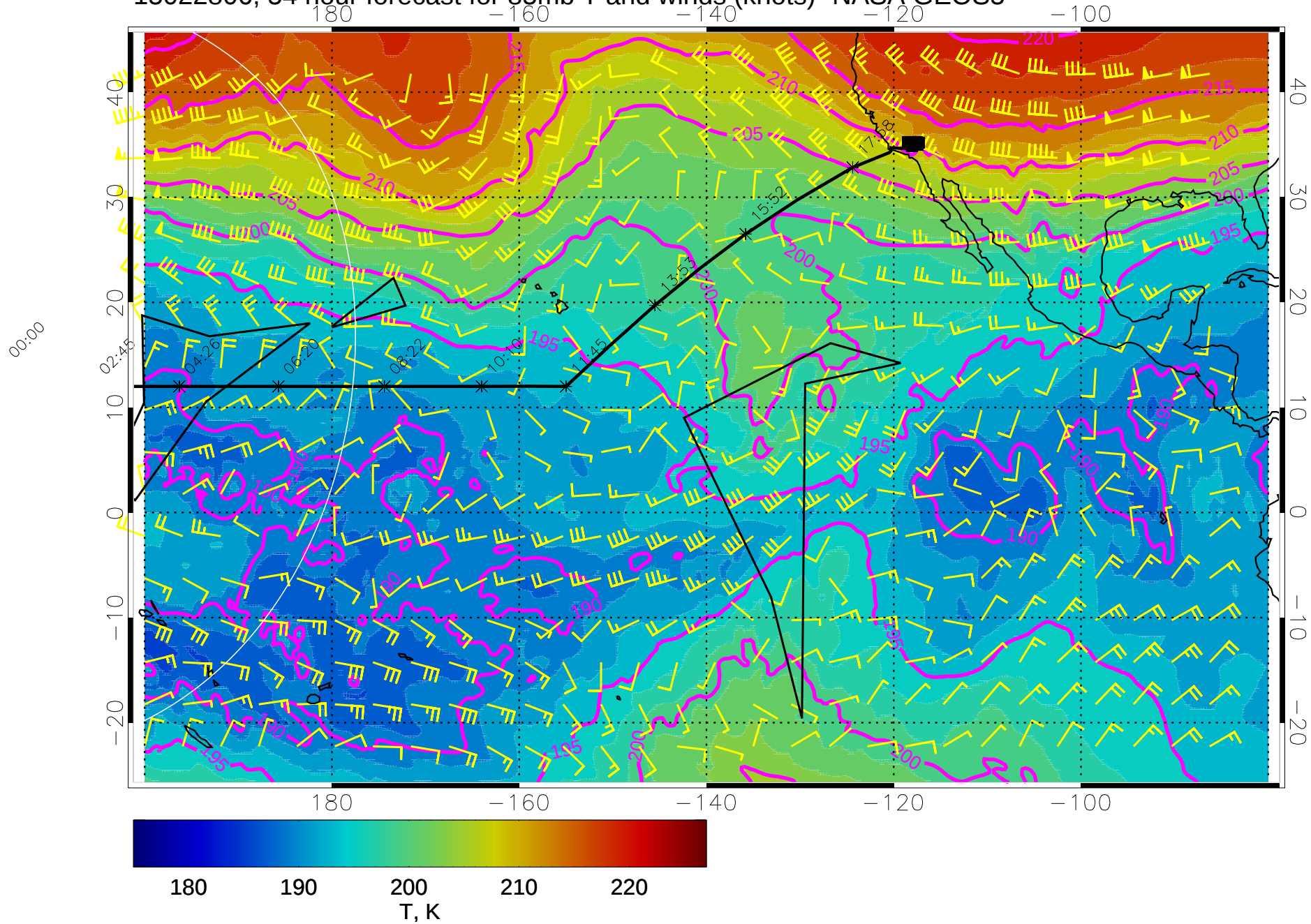
15022806, 54 hour forecast for 85mb T and winds (knots)- NASA GEOS5
