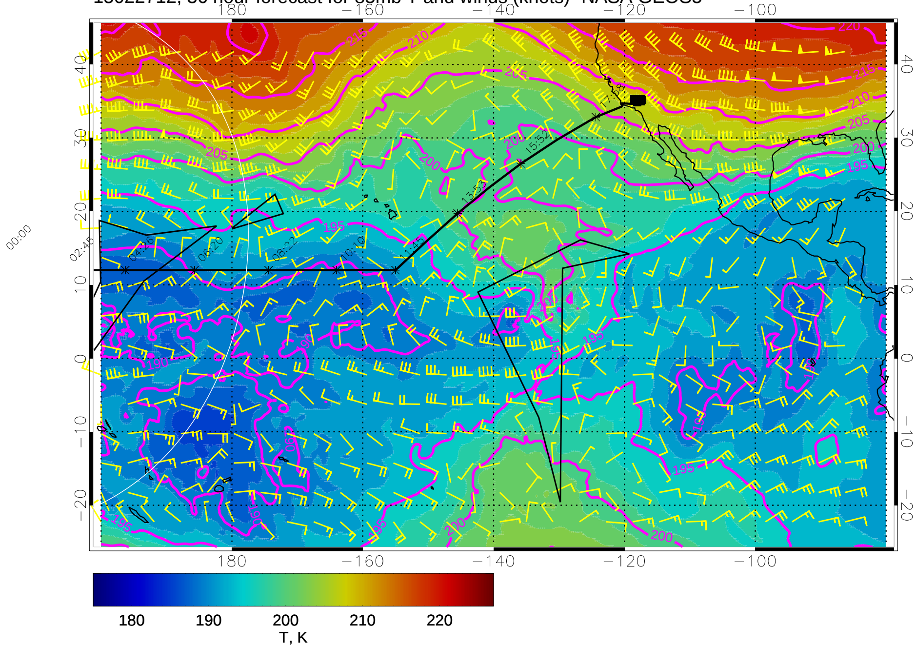
15022712, 36 hour forecast for 85mb T and winds (knots)- NASA GEOS5
