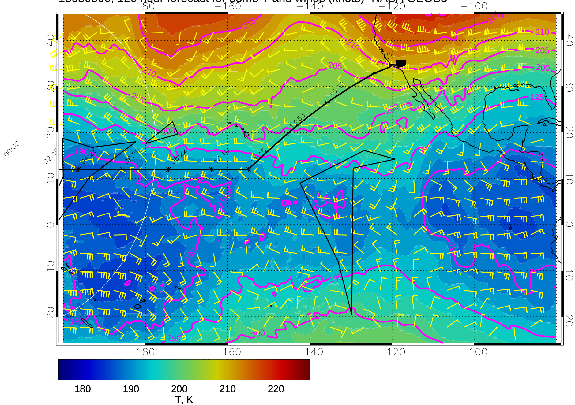
15030300, 120 hour forecast for 85mb T and winds (knots)- NASA GEOS5
