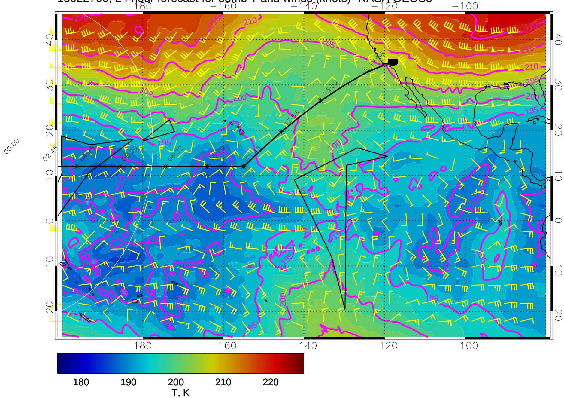
15022700, 24 hour forecast for 85mb T and winds (knots)- NASA GEOS5
