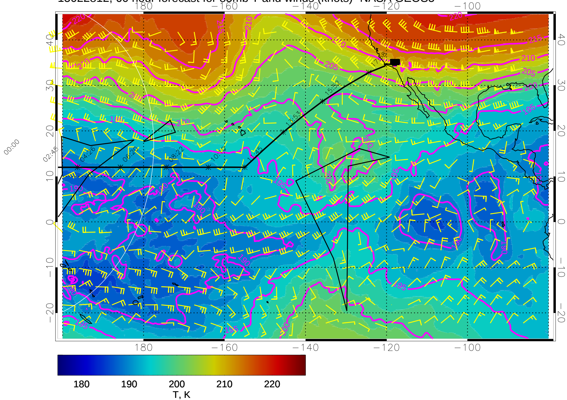
15022812, 60 hour forecast for 85mb T and winds (knots)- NASA GEOS5
