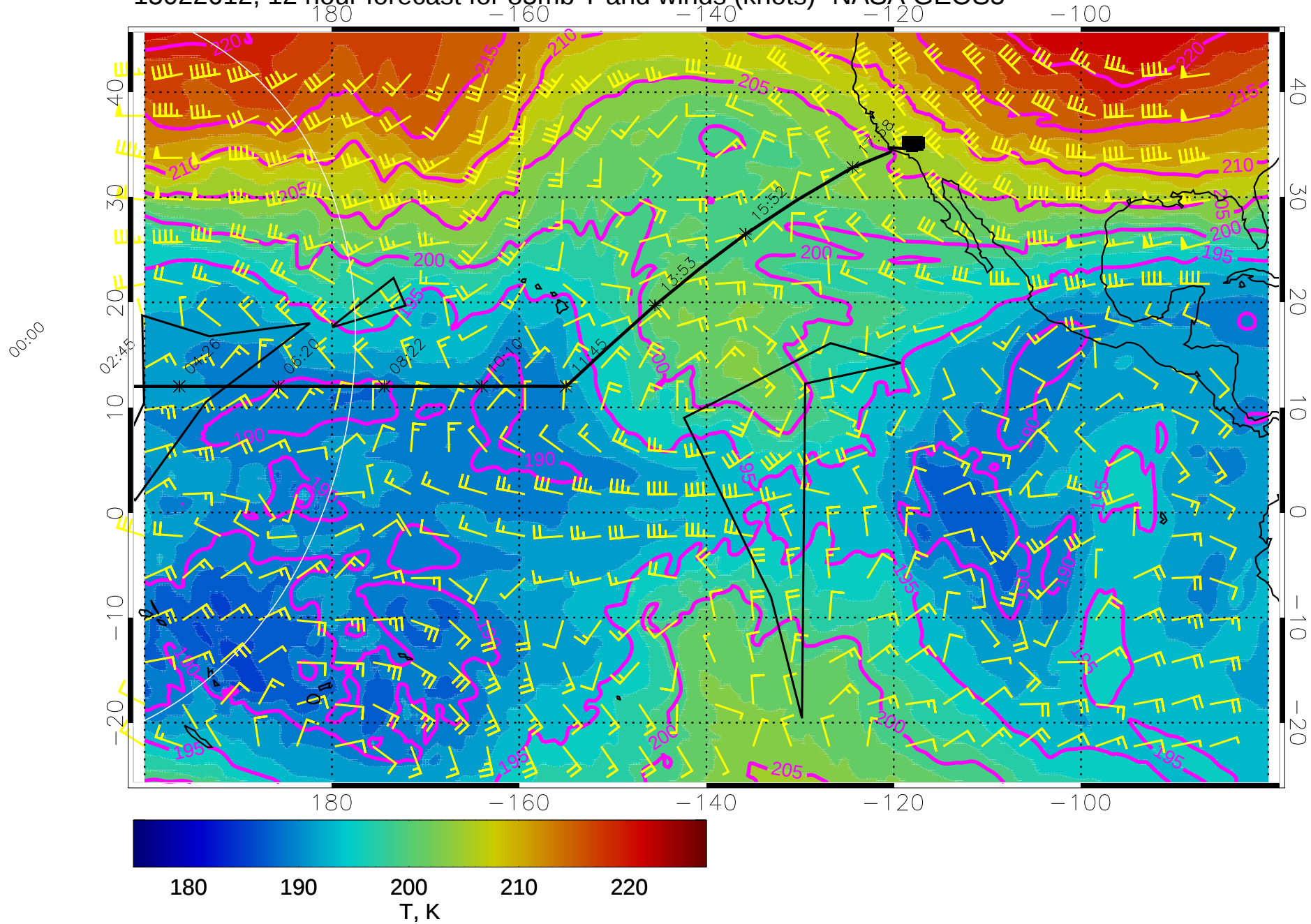
15022612, 12 hour forecast for 85mb T and winds (knots)- NASA GEOS5
