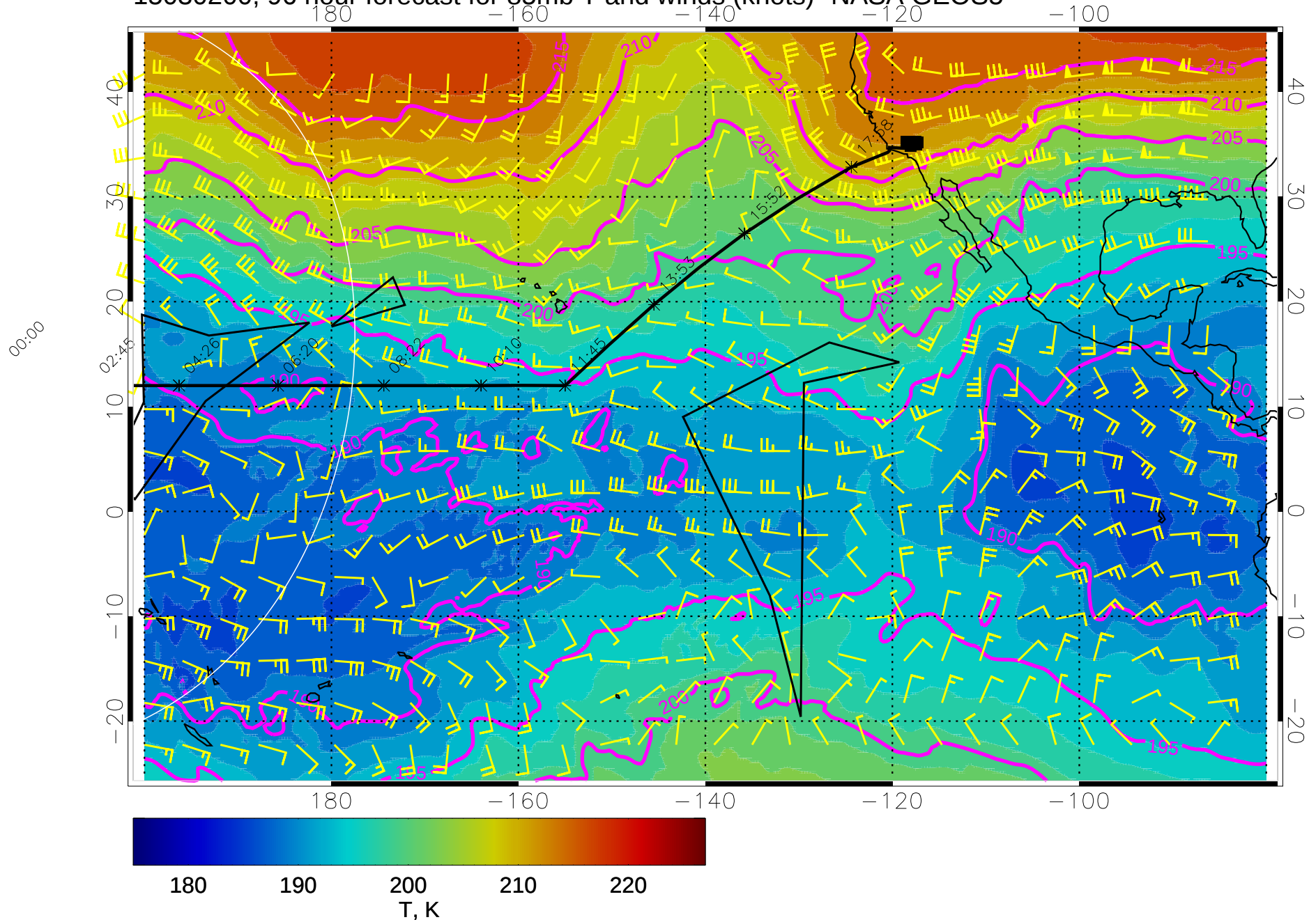
15030200, 96 hour forecast for 85mb T and winds (knots)- NASA GEOS5
