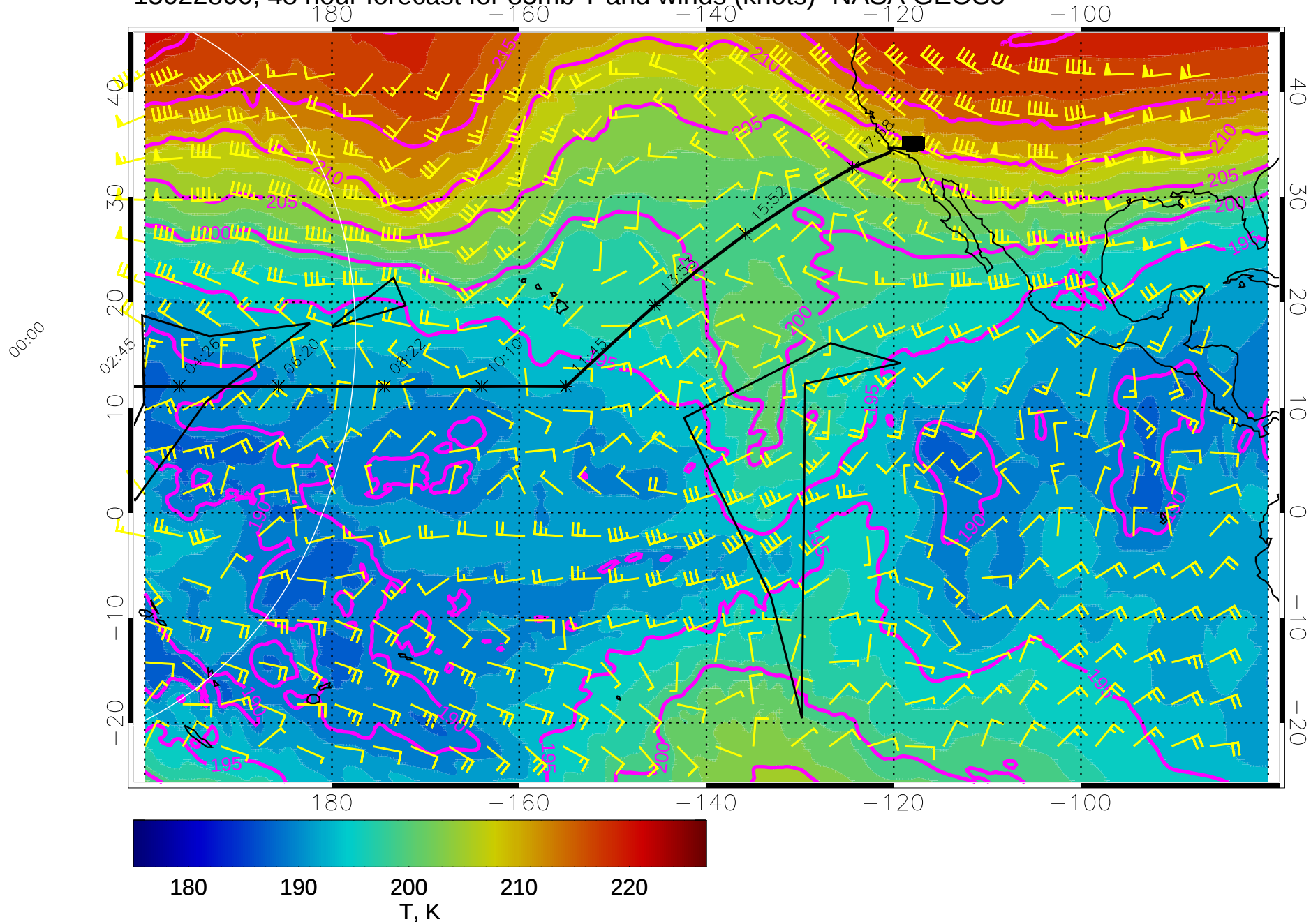
15022800, 48 hour forecast for 85mb T and winds (knots)- NASA GEOS5
