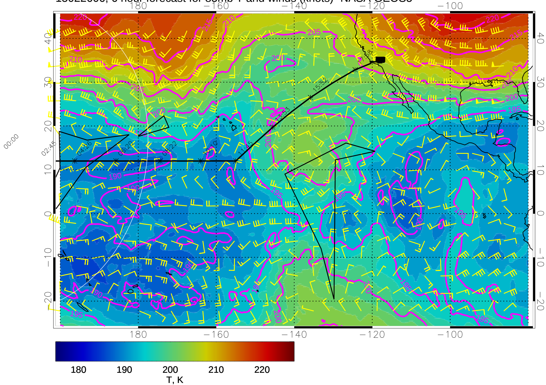
15022606, 6 hour forecast for 85mb T and winds (knots)- NASA GEOS5
