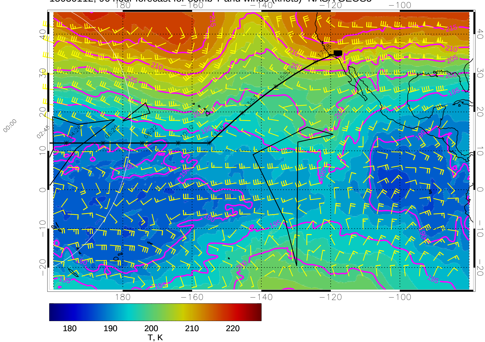
15030112, 96 hour forecast for 85mb T and winds (knots)- NASA GEOS5
