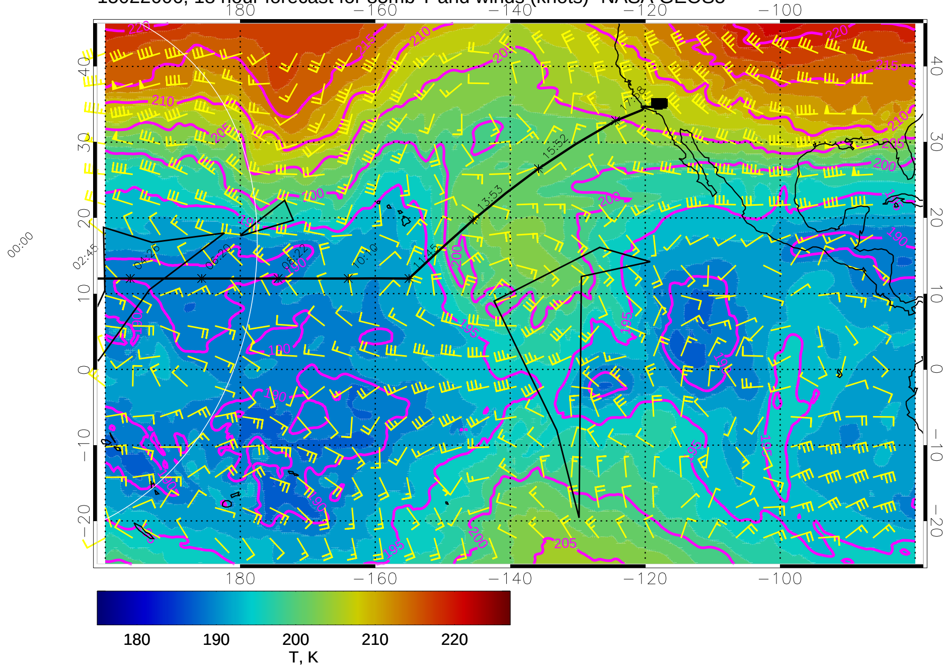
15022606, 18 hour forecast for 85mb T and winds (knots)- NASA GEOS5
