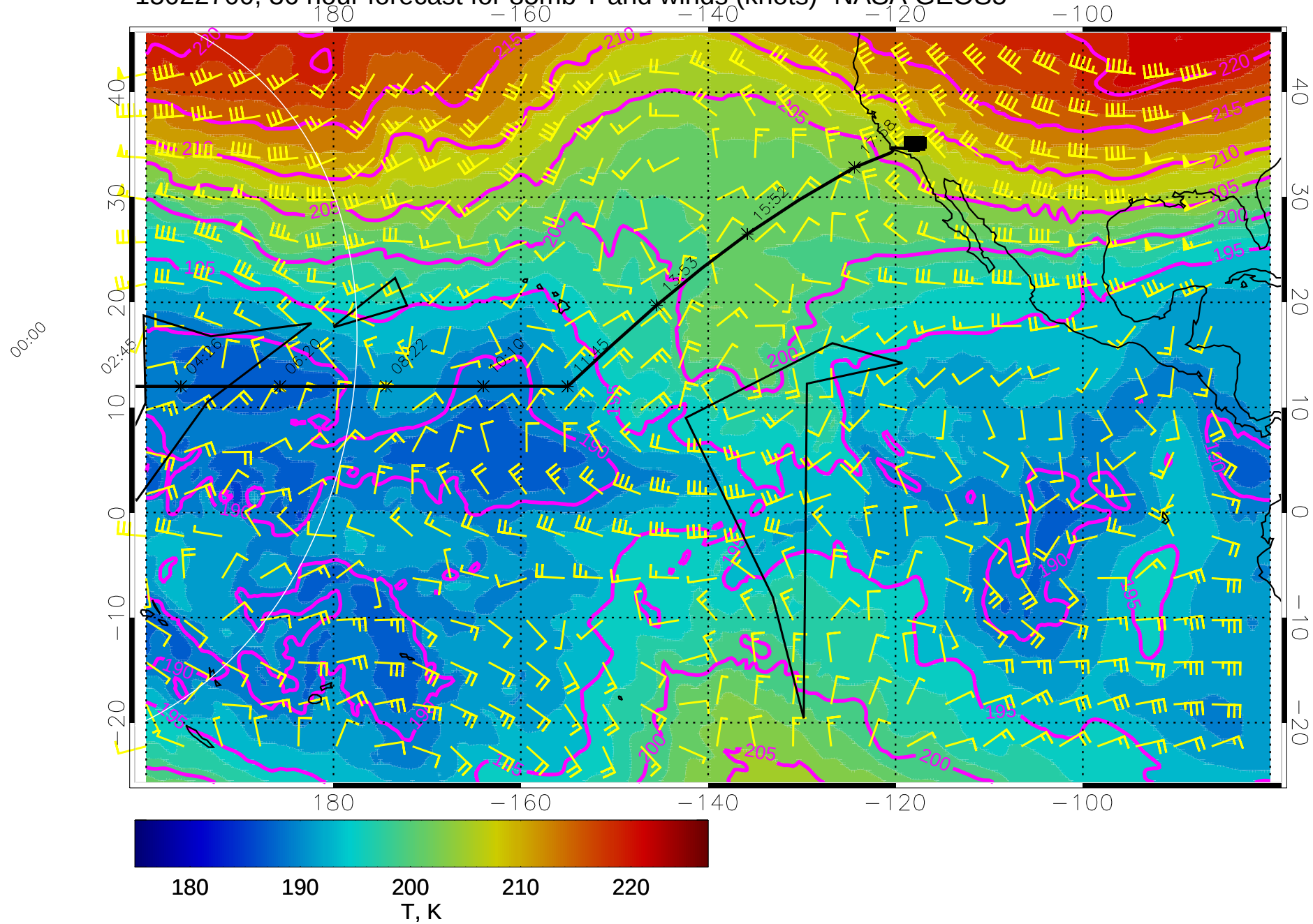
15022700, 36 hour forecast for 85mb T and winds (knots)- NASA GEOS5
