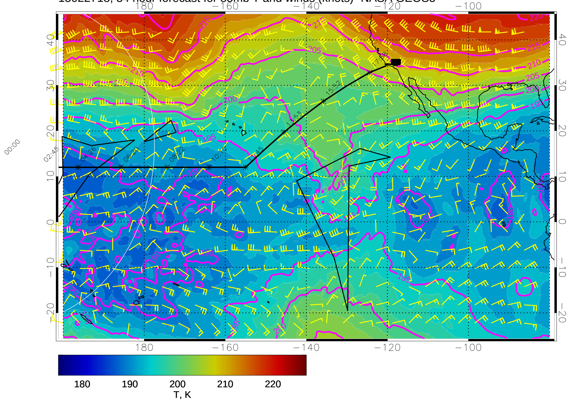
15022718, 54 hour forecast for 85mb T and winds (knots)- NASA GEOS5
