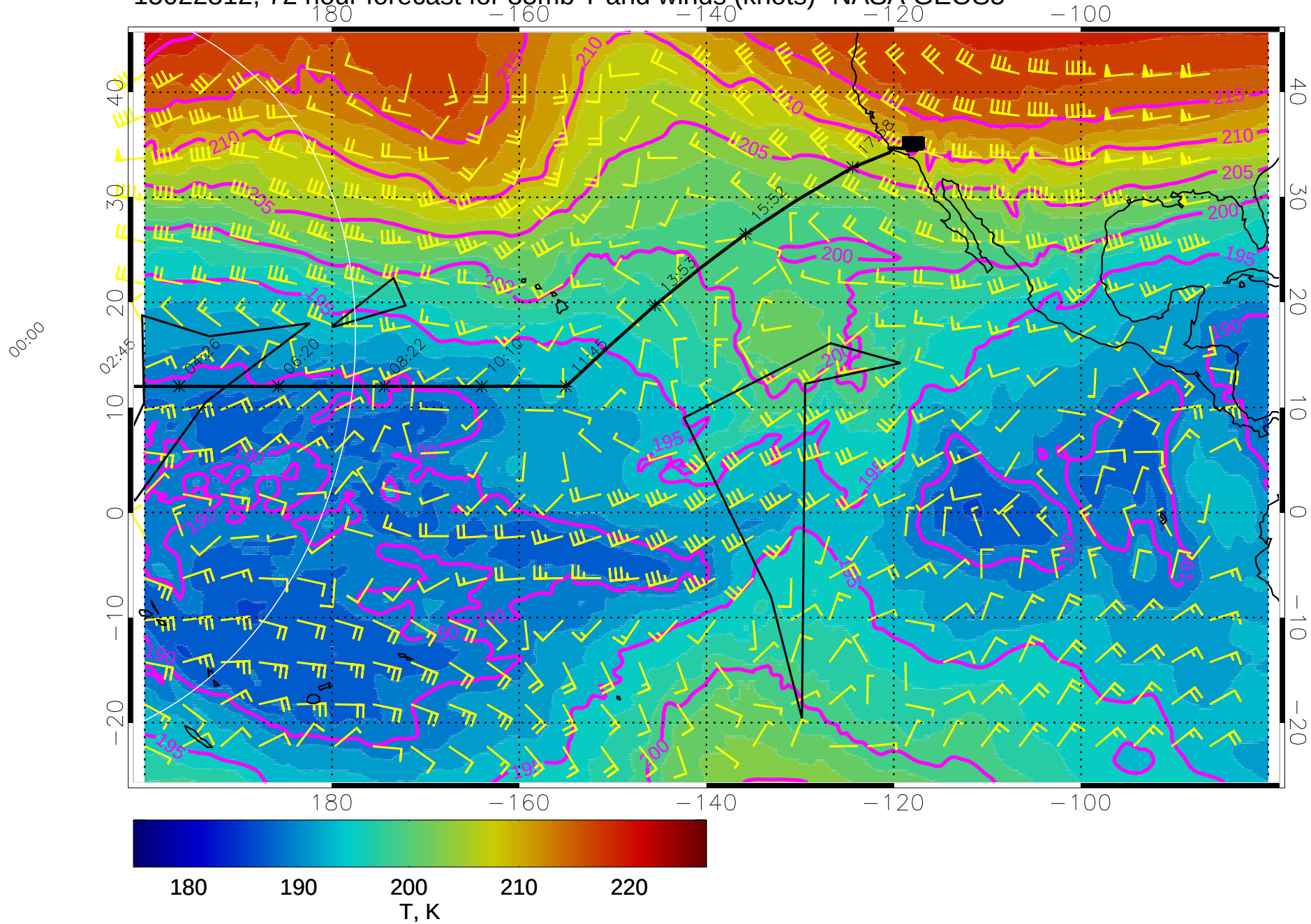
15022812, 72 hour forecast for 85mb T and winds (knots)- NASA GEOS5
