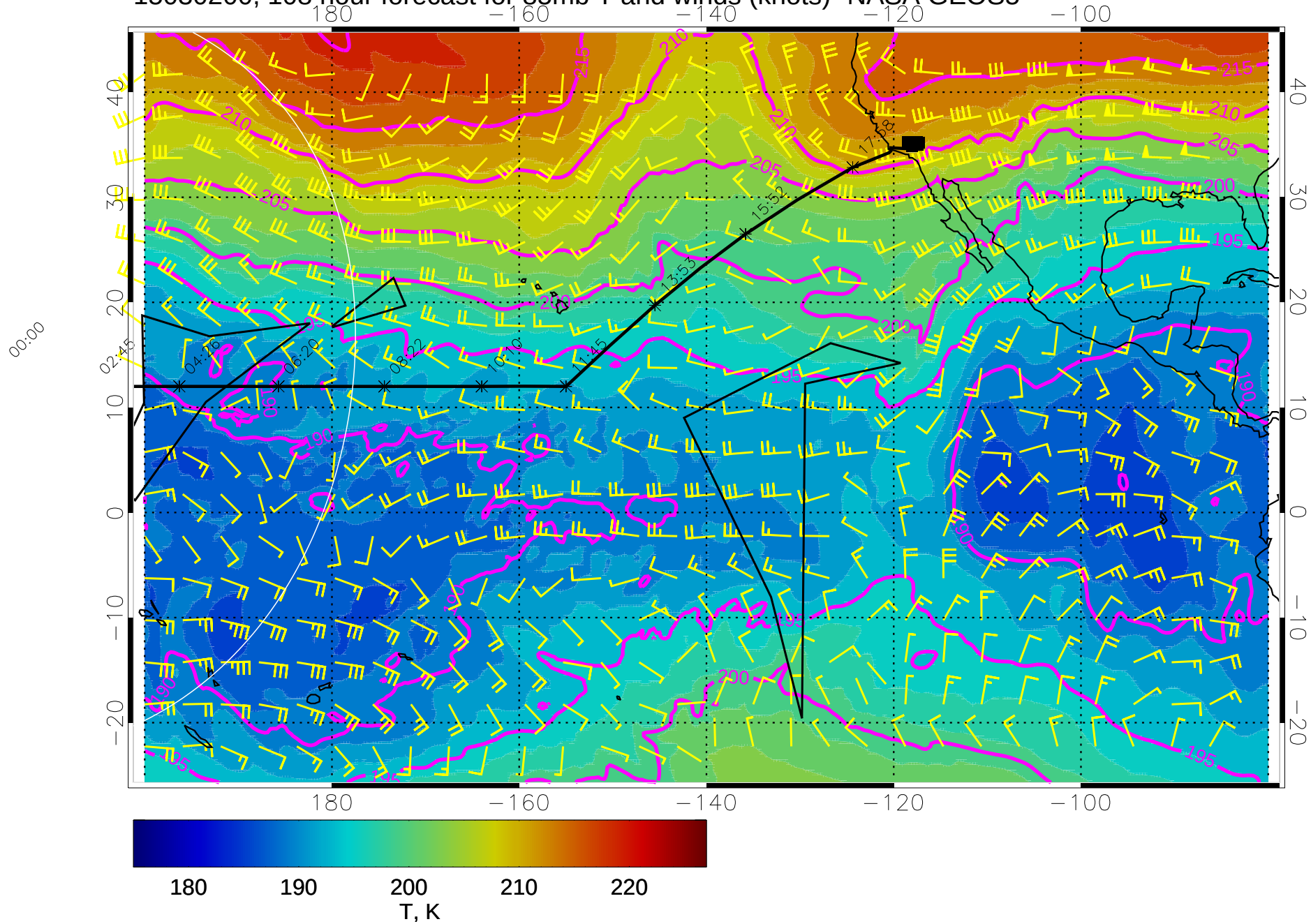
15030200, 108 hour forecast for 85mb T and winds (knots)- NASA GEOS5
