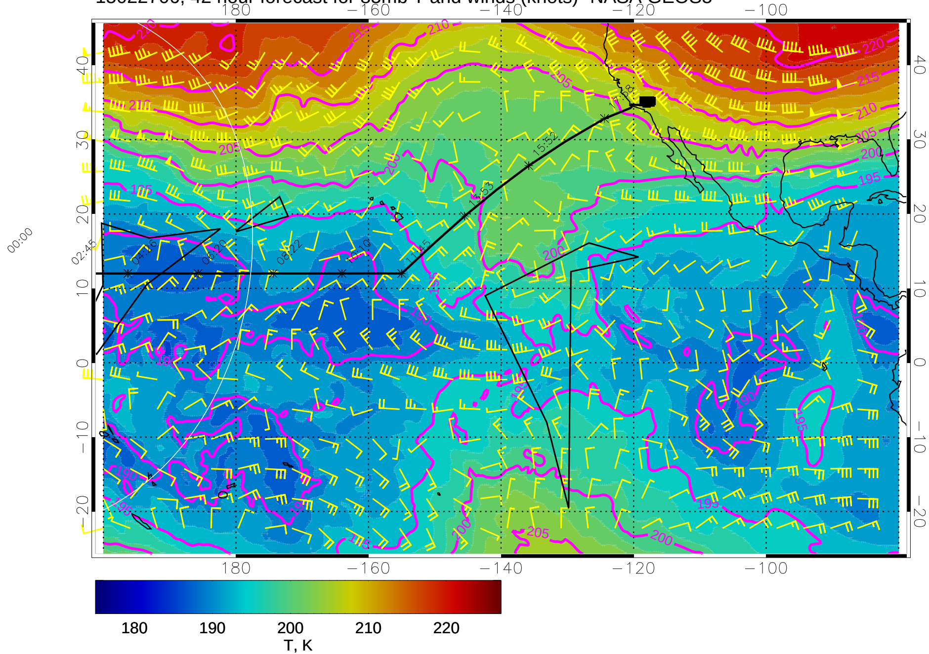
15022706, 42 hour forecast for 85mb T and winds (knots)- NASA GEOS5
