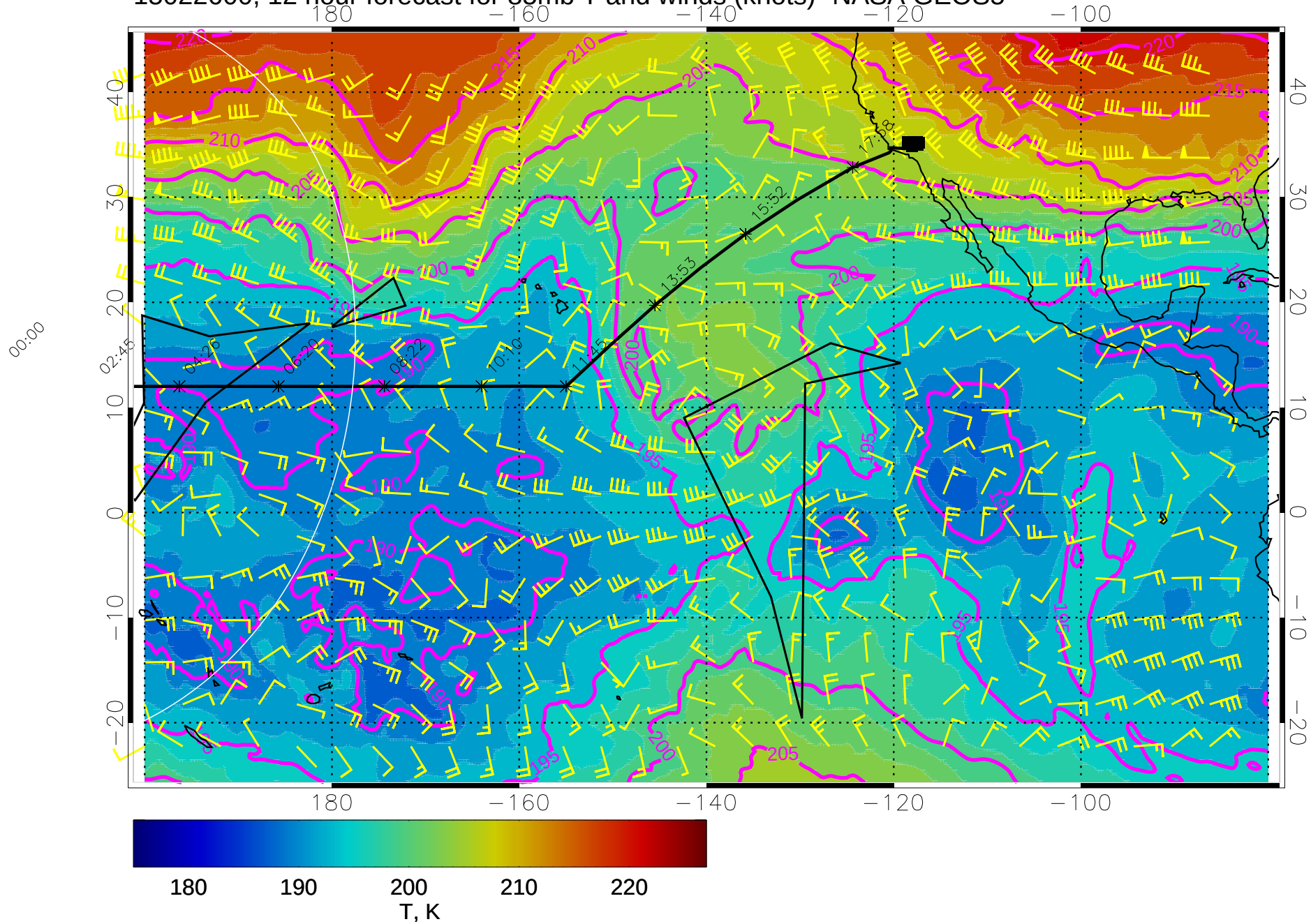
15022600, 12 hour forecast for 85mb T and winds (knots)- NASA GEOS5
