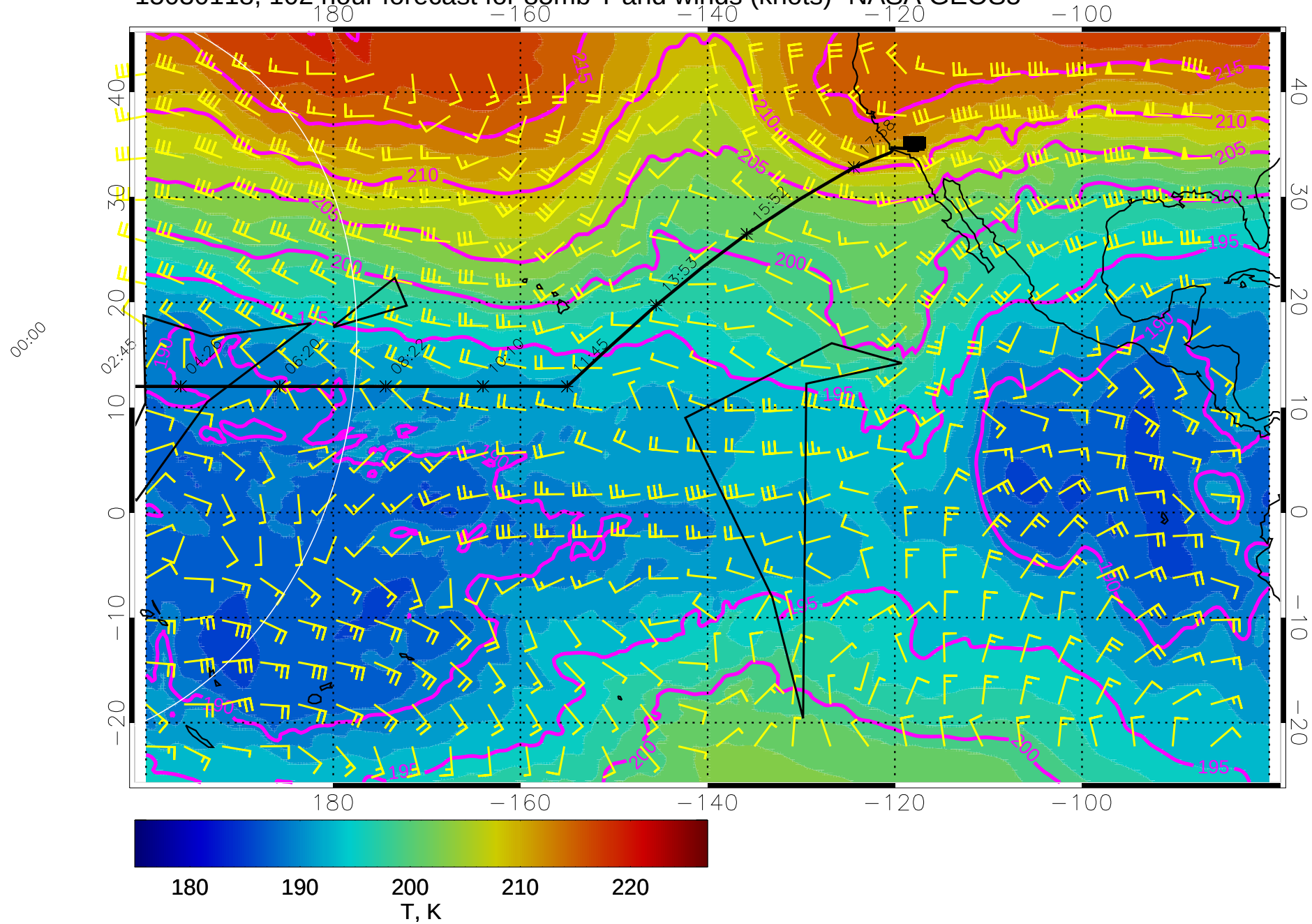
15030118, 102 hour forecast for 85mb T and winds (knots)- NASA GEOS5
