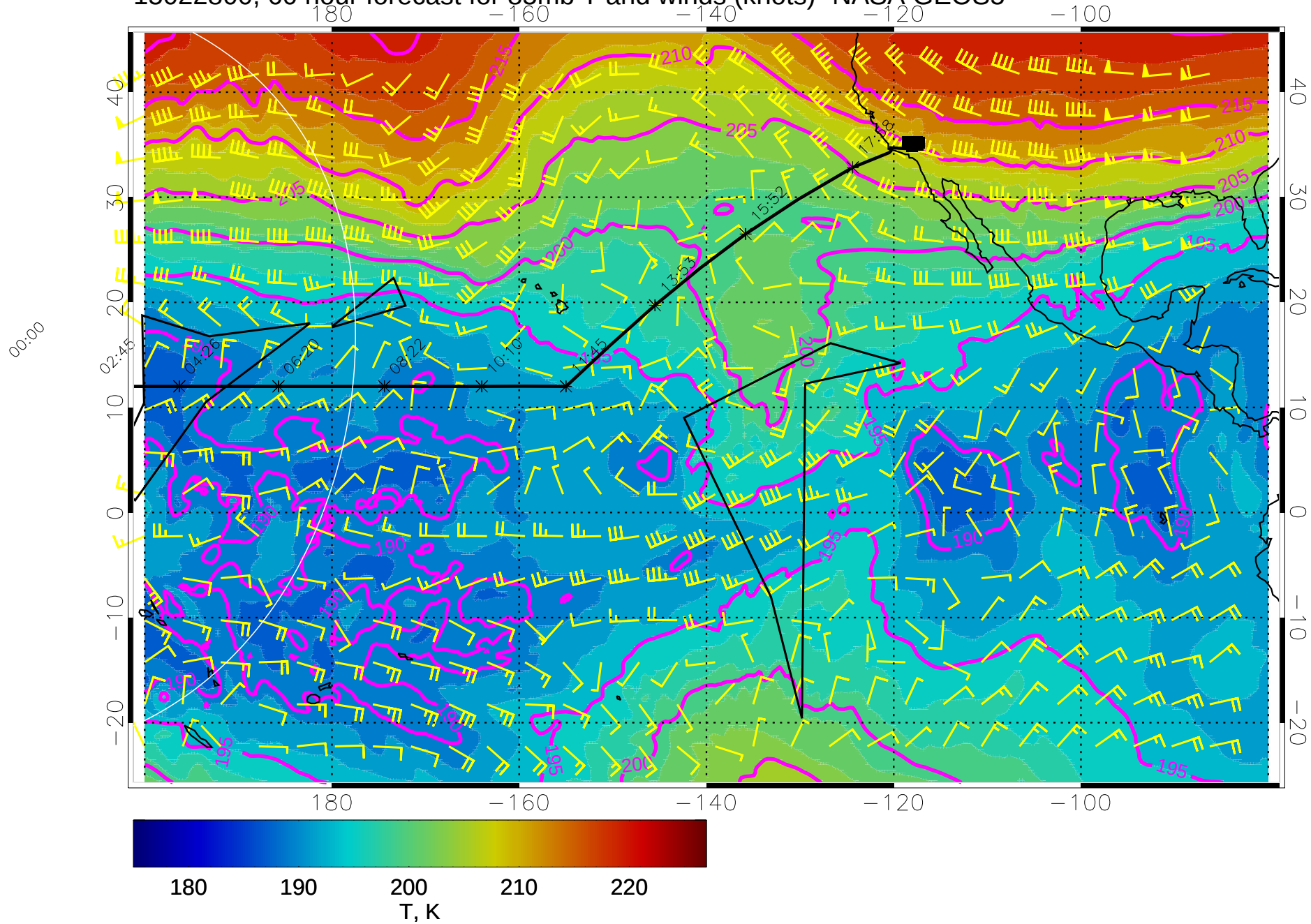
15022800, 60 hour forecast for 85mb T and winds (knots)- NASA GEOS5
