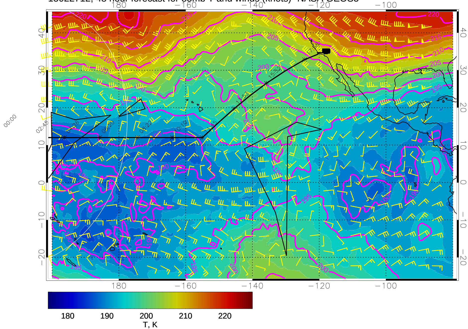
15022712, 48 hour forecast for 85mb T and winds (knots)- NASA GEOS5
