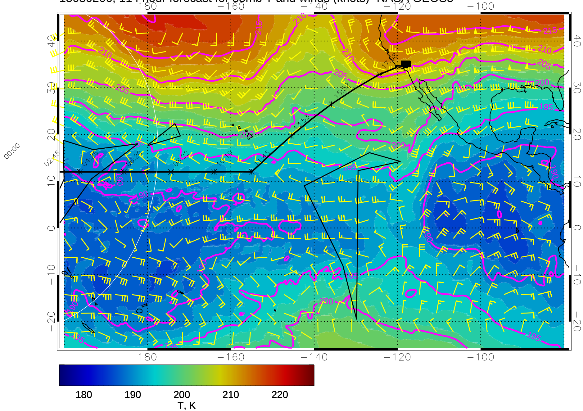
15030206, 114 hour forecast for 85mb T and winds (knots)- NASA GEOS5
