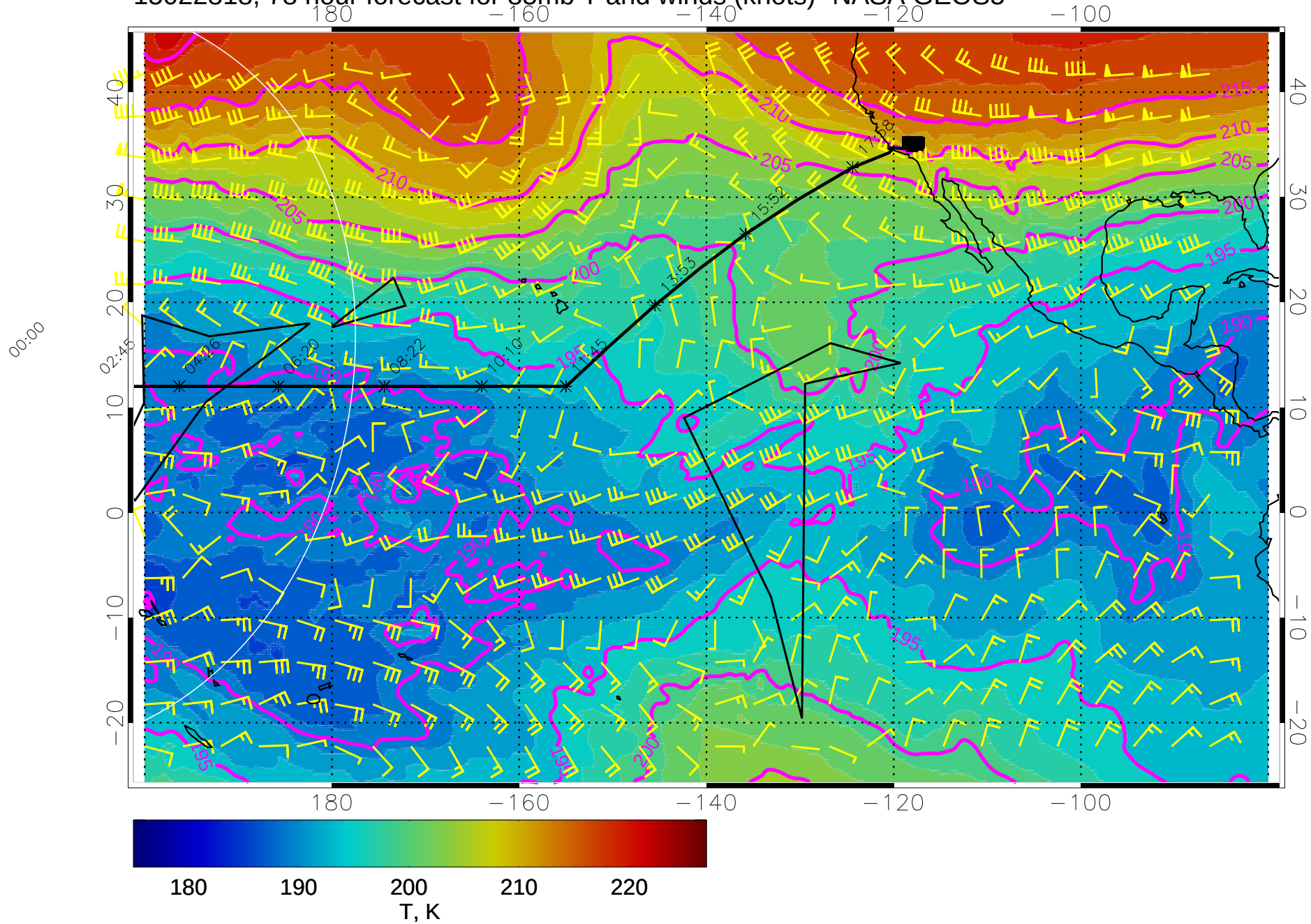
15022818, 78 hour forecast for 85mb T and winds (knots)- NASA GEOS5
