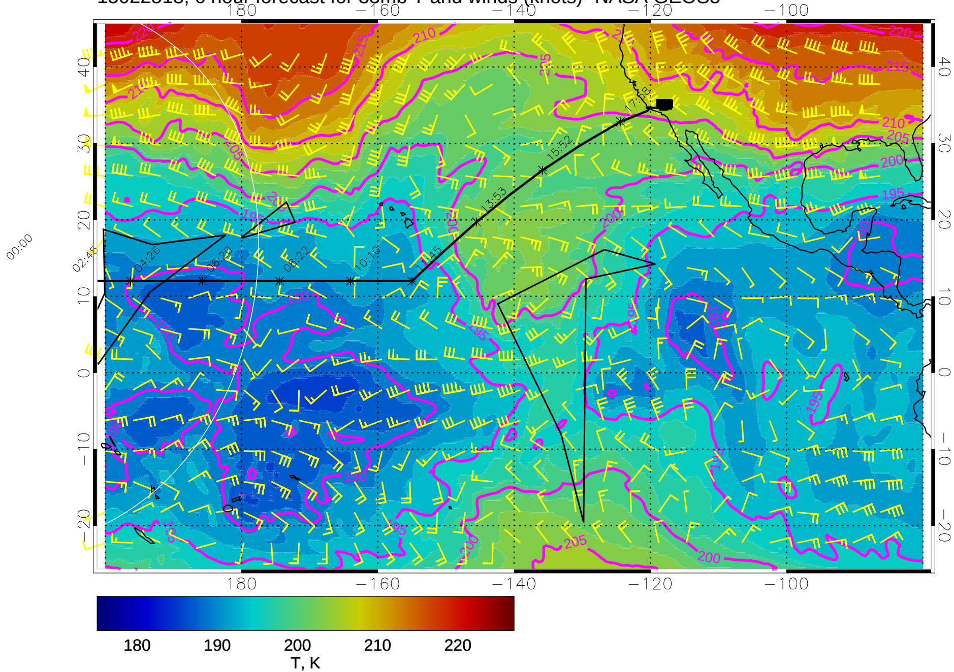
15022518, 6 hour forecast for 85mb T and winds (knots)- NASA GEOS5
