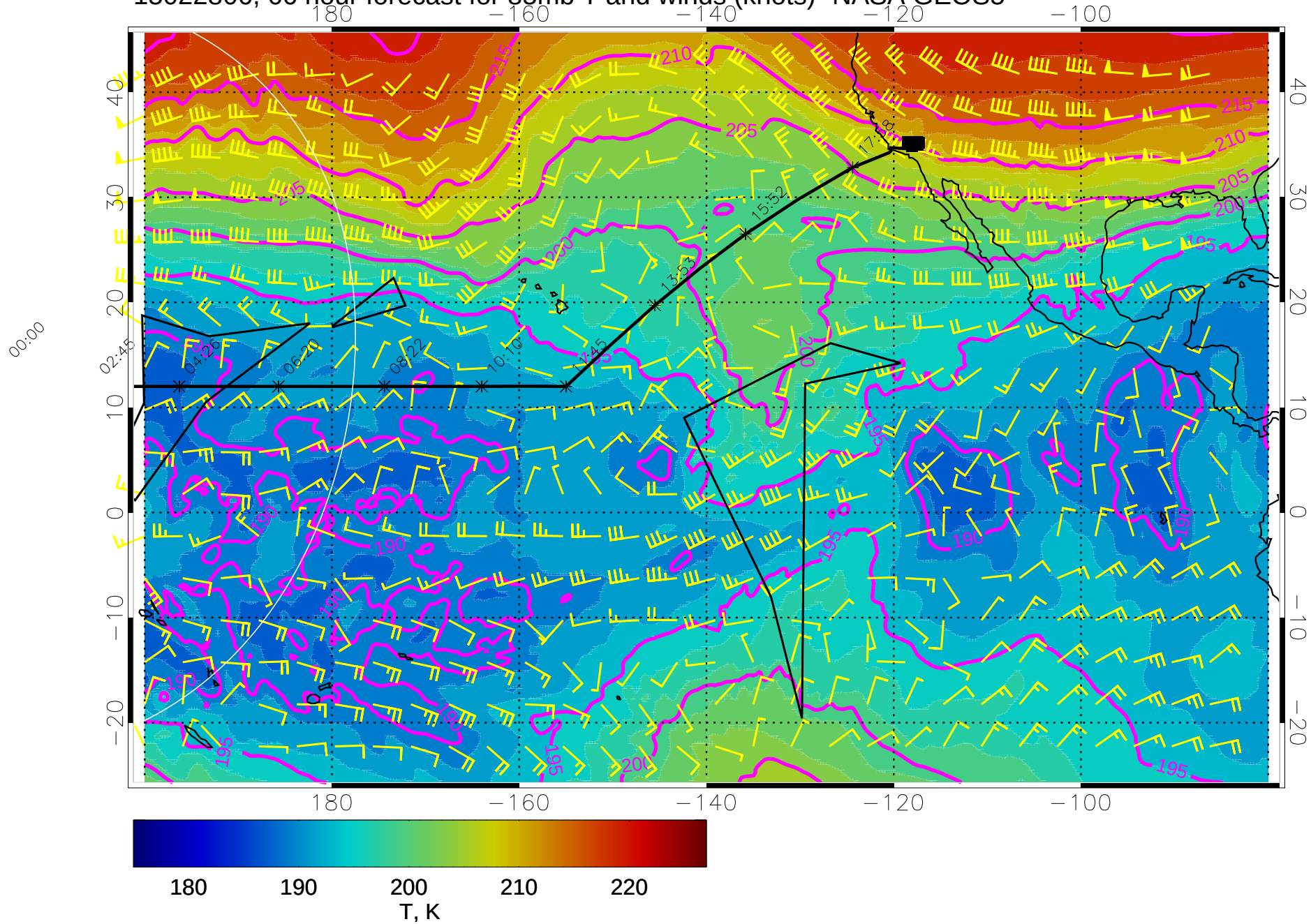
15022806, 66 hour forecast for 85mb T and winds (knots)- NASA GEOS5
