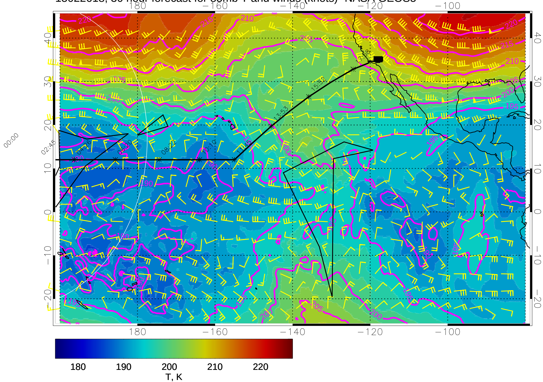
15022618, 30 hour forecast for 85mb T and winds (knots)- NASA GEOS5
