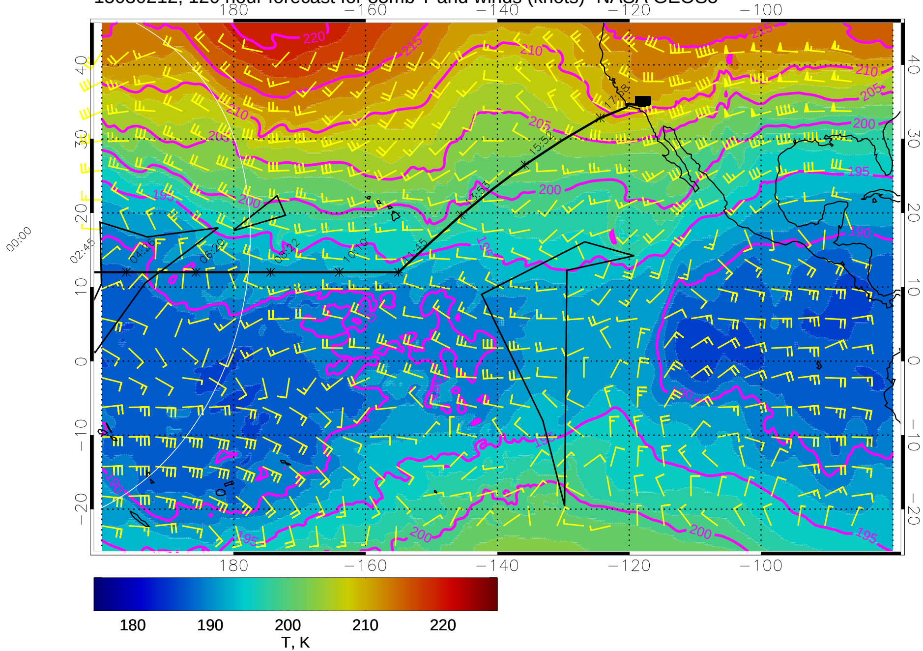
15030212, 120 hour forecast for 85mb T and winds (knots)- NASA GEOS5
