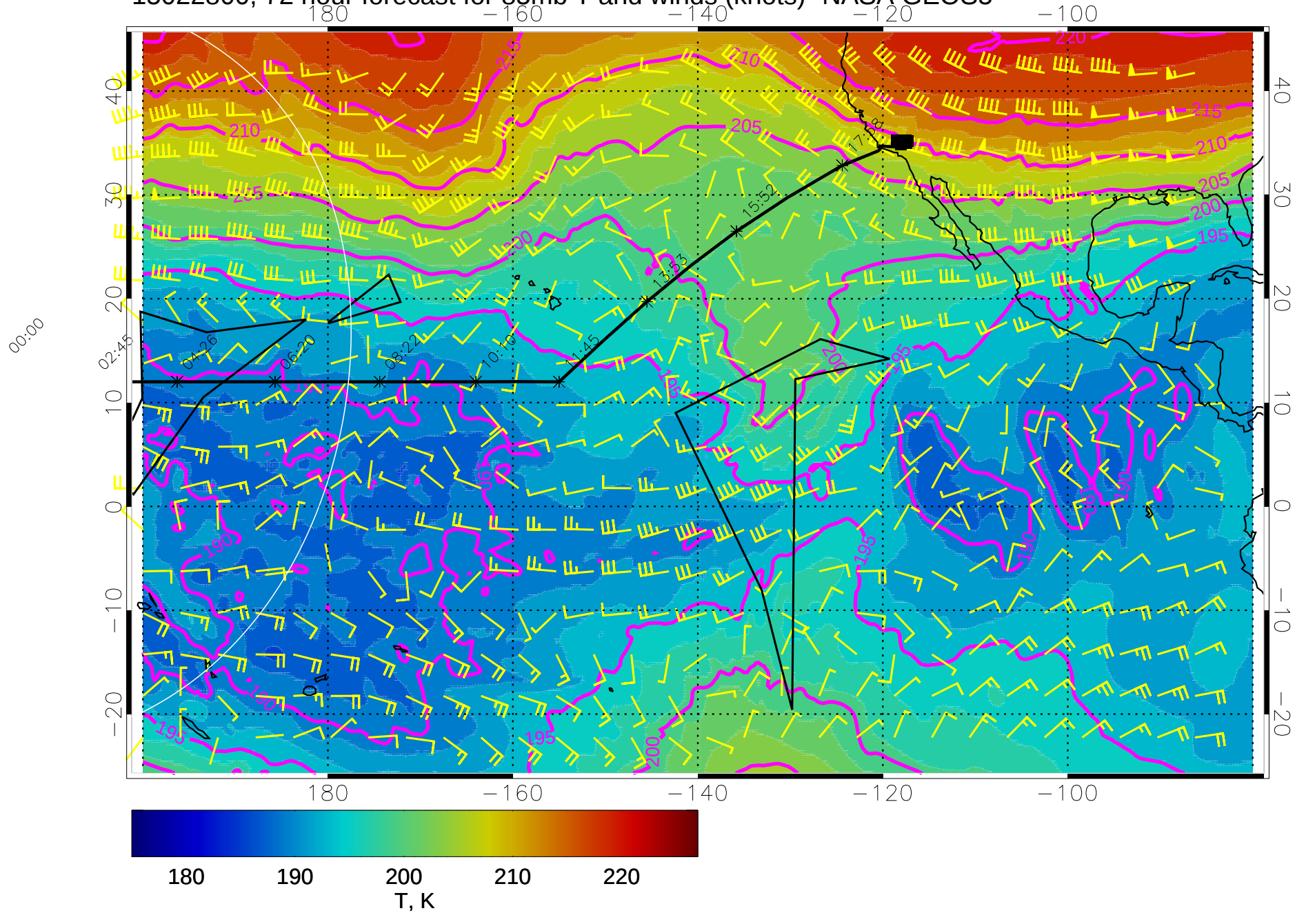
15022800, 72 hour forecast for 85mb T and winds (knots)- NASA GEOS5
