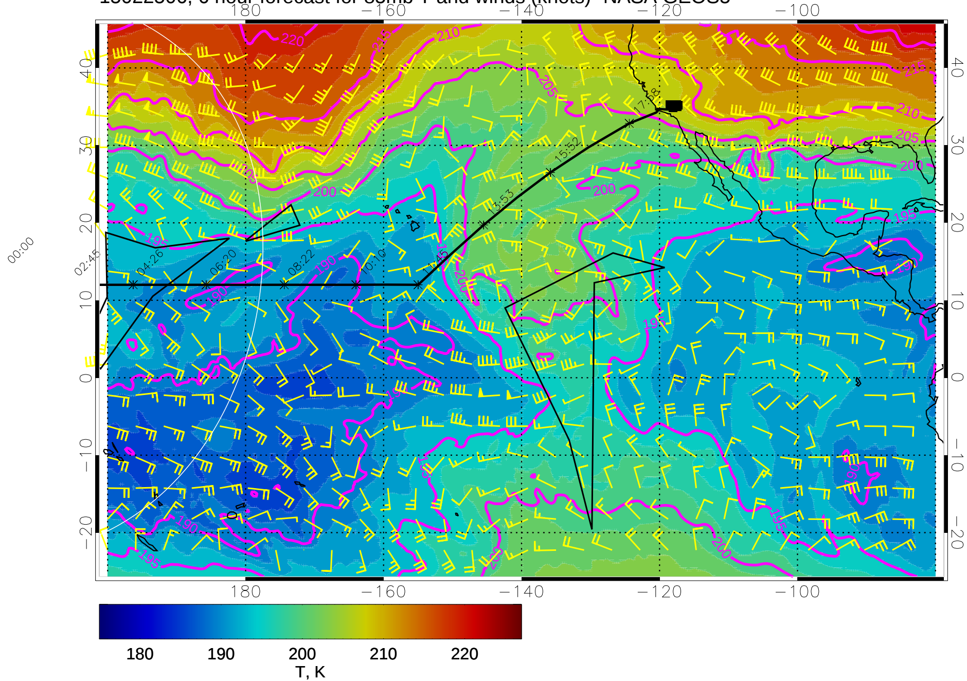
15022506, 6 hour forecast for 85mb T and winds (knots)- NASA GEOS5
