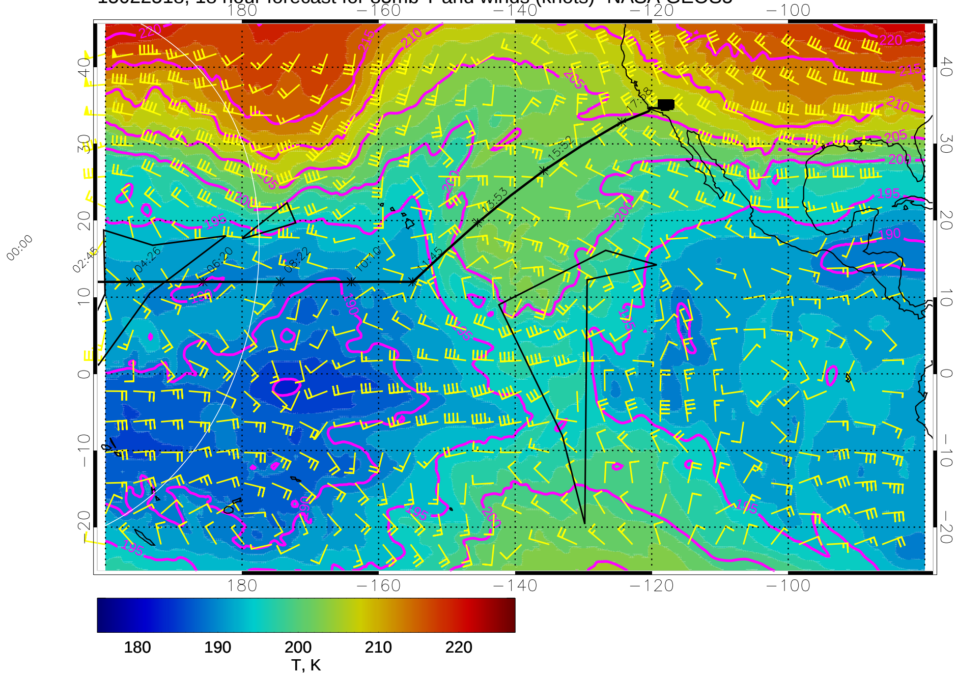
15022518, 18 hour forecast for 85mb T and winds (knots)- NASA GEOS5
