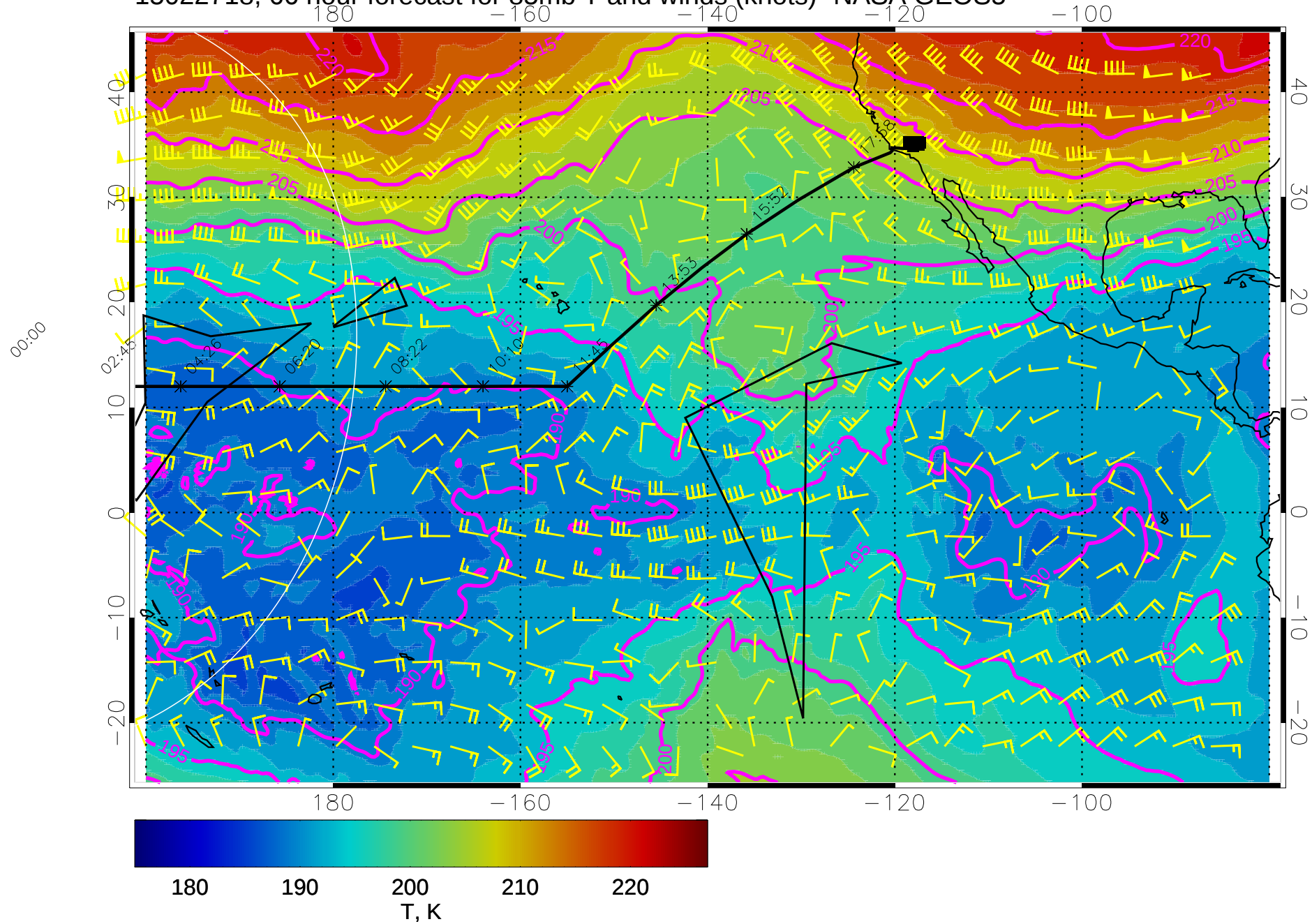
15022718, 66 hour forecast for 85mb T and winds (knots)- NASA GEOS5
