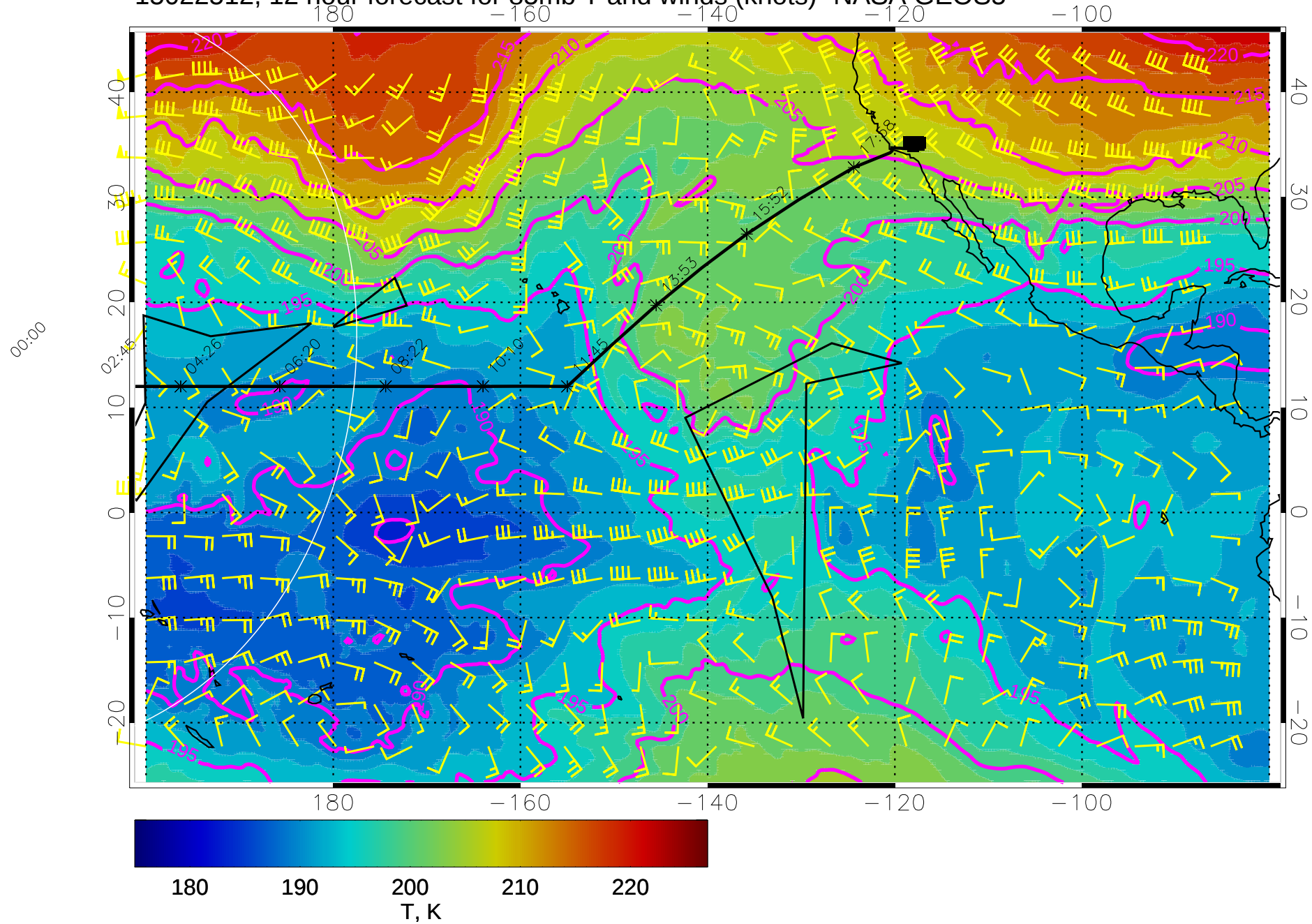
15022512, 12 hour forecast for 85mb T and winds (knots)- NASA GEOS5
