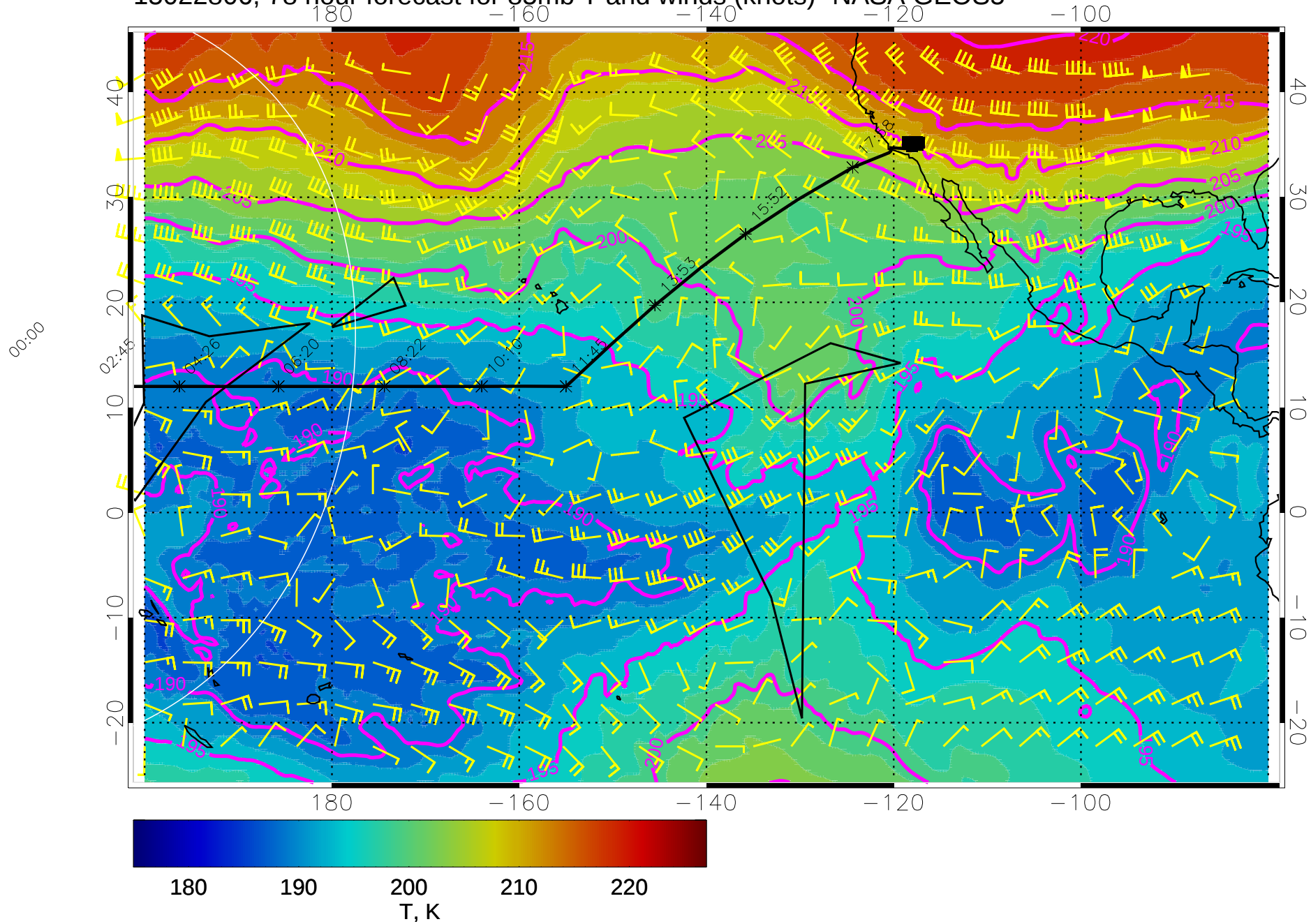
15022806, 78 hour forecast for 85mb T and winds (knots)- NASA GEOS5
