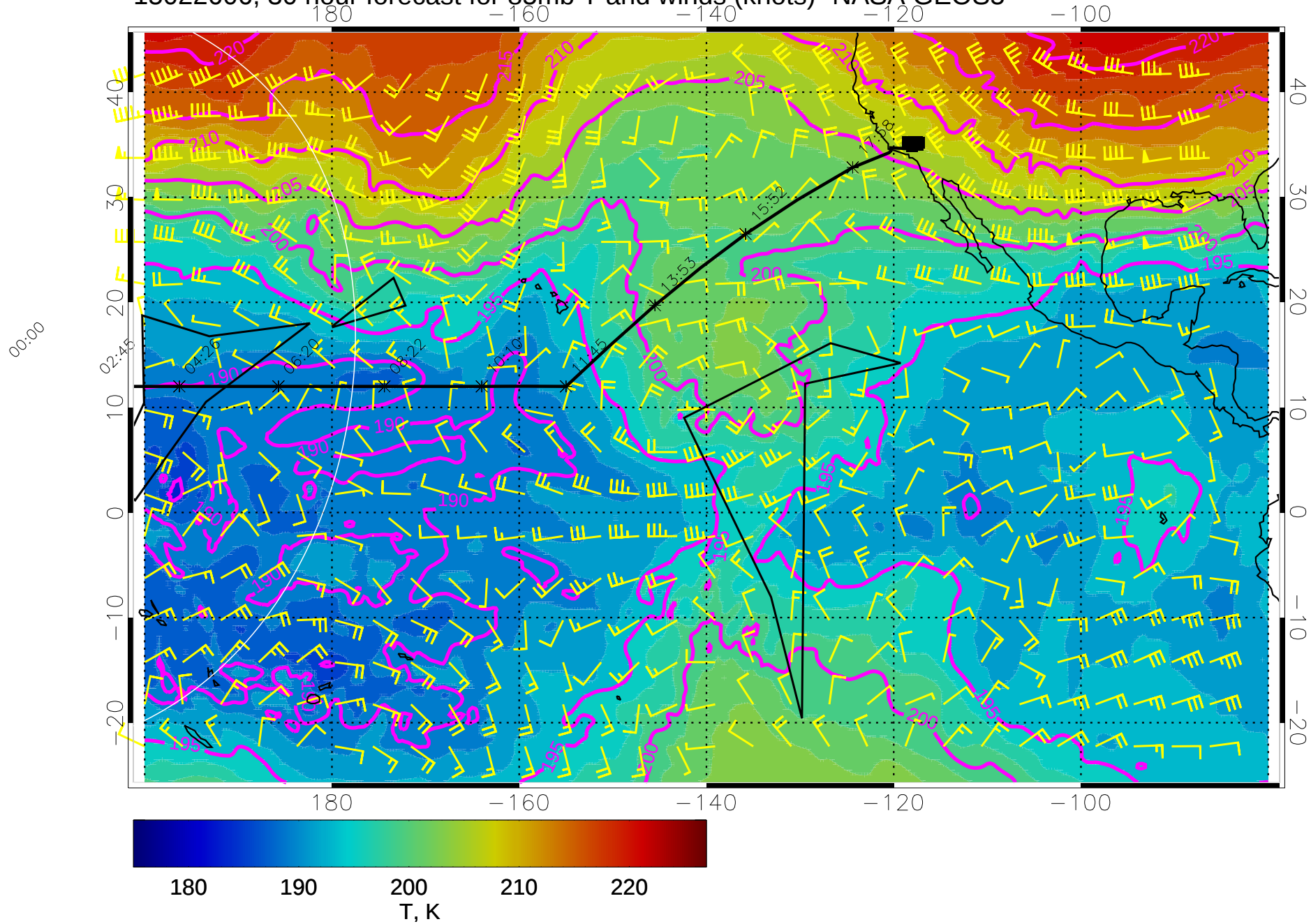
15022606, 30 hour forecast for 85mb T and winds (knots)- NASA GEOS5
