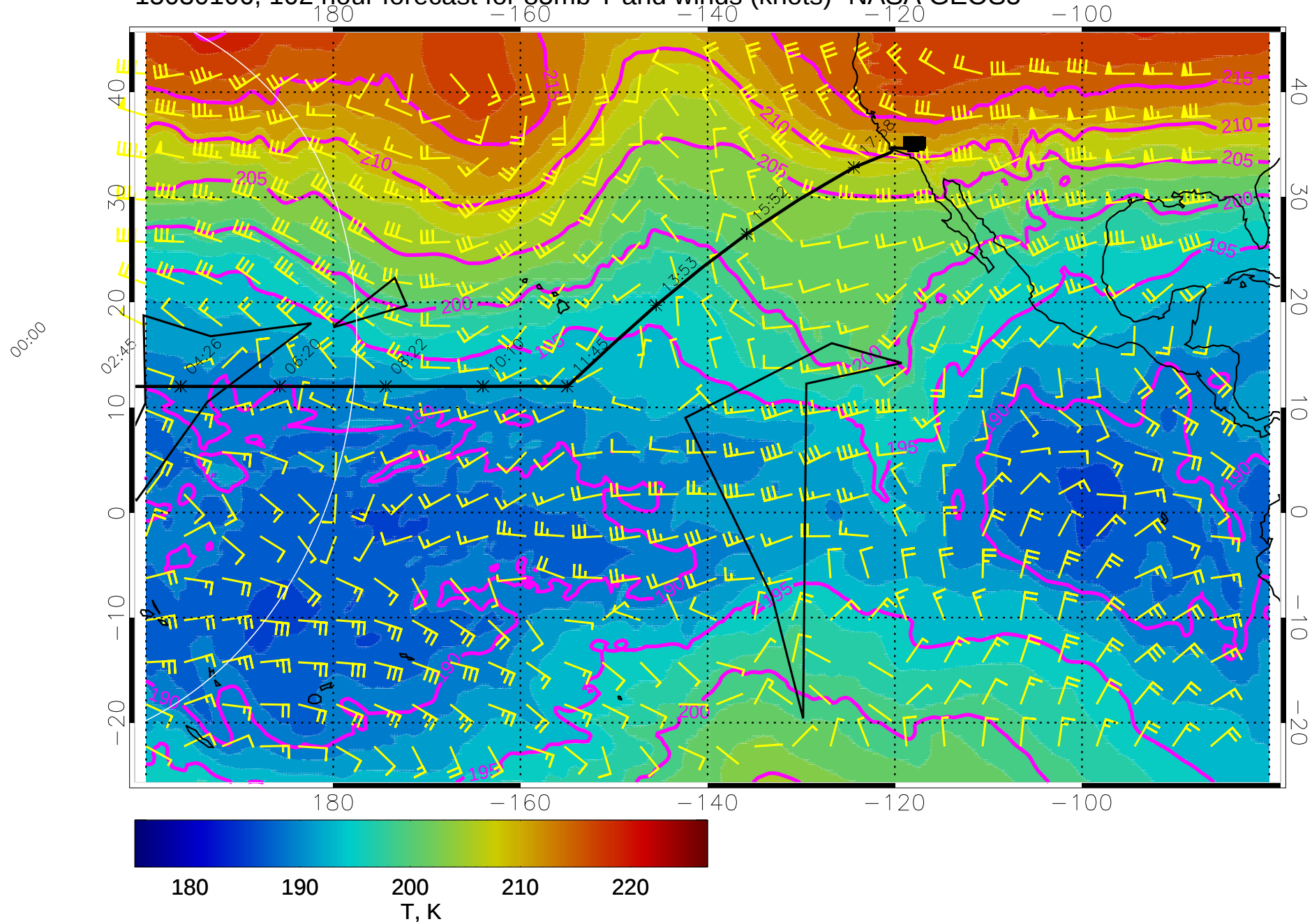
15030106, 102 hour forecast for 85mb T and winds (knots)- NASA GEOS5
