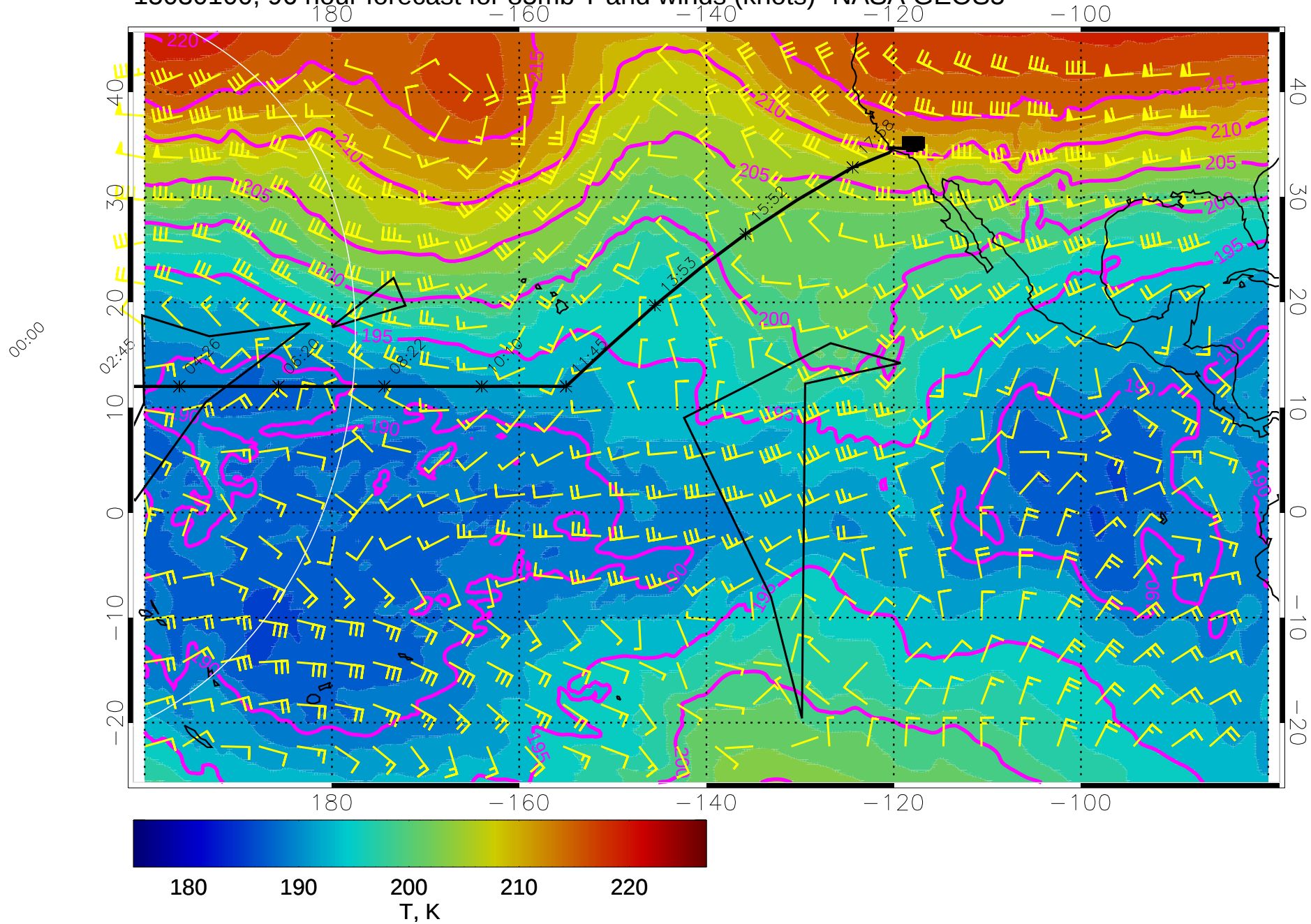
15030100, 96 hour forecast for 85mb T and winds (knots)- NASA GEOS5
