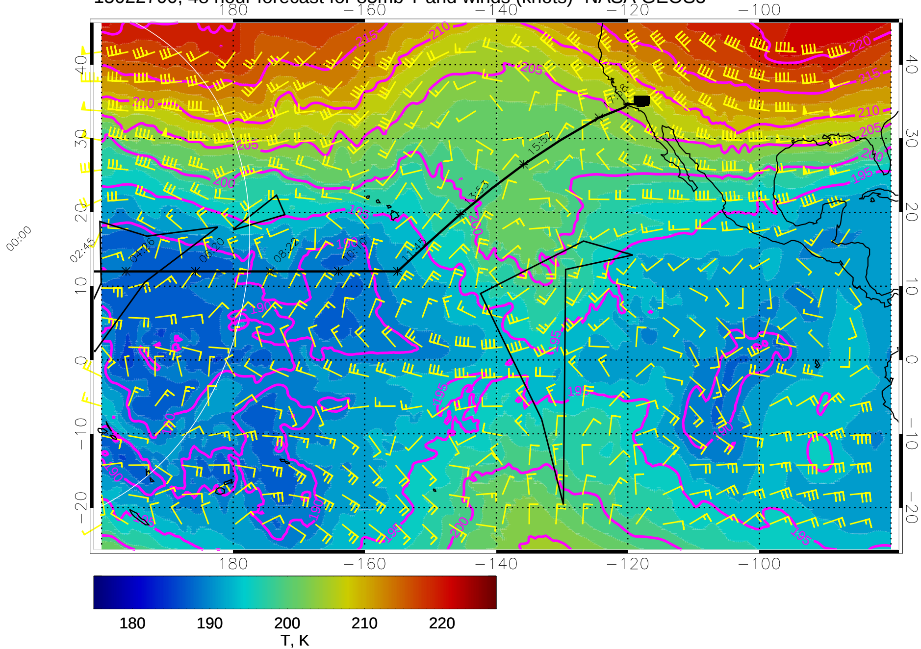
15022700, 48 hour forecast for 85mb T and winds (knots)- NASA GEOS5
