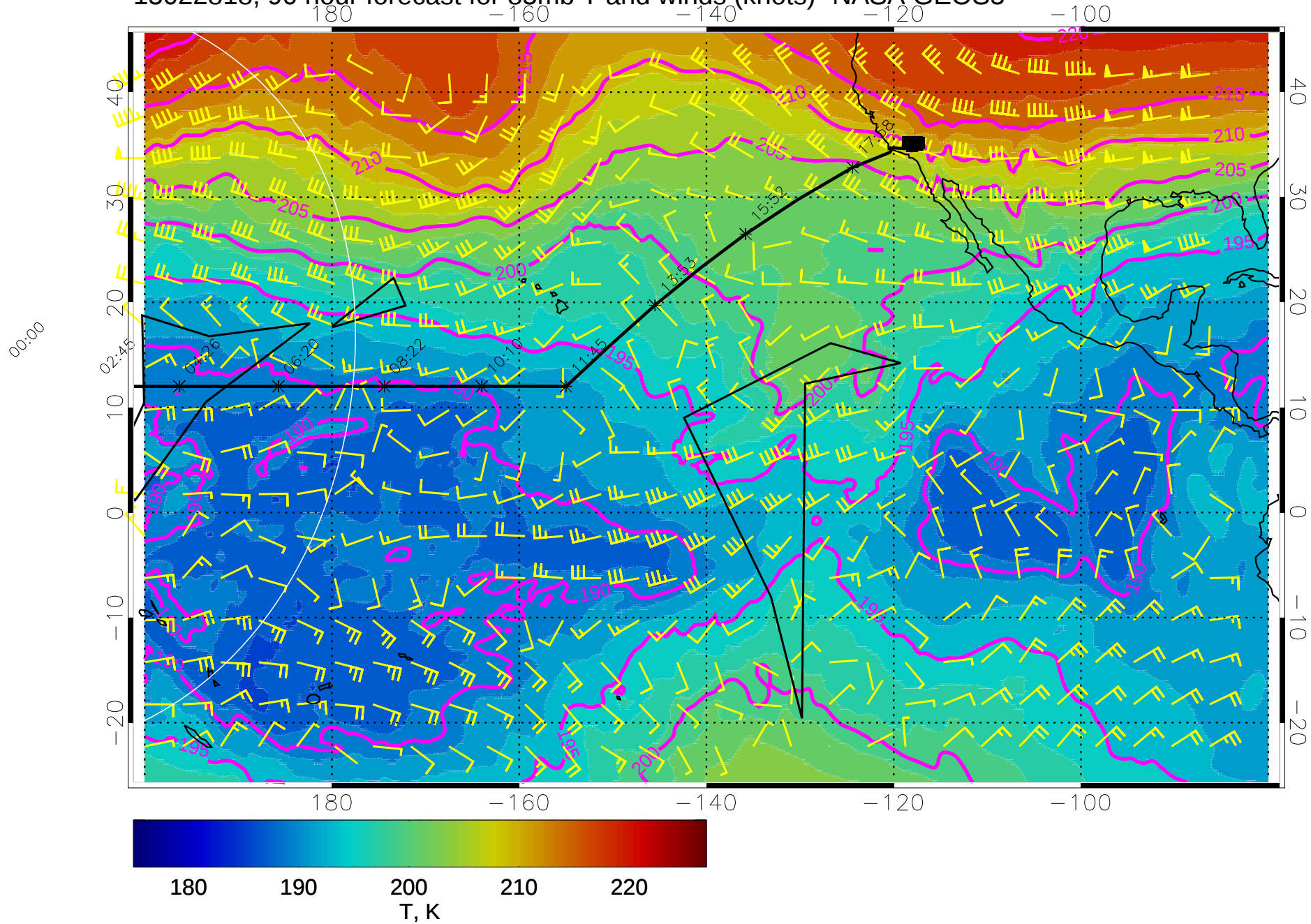
15022818, 90 hour forecast for 85mb T and winds (knots)- NASA GEOS5
