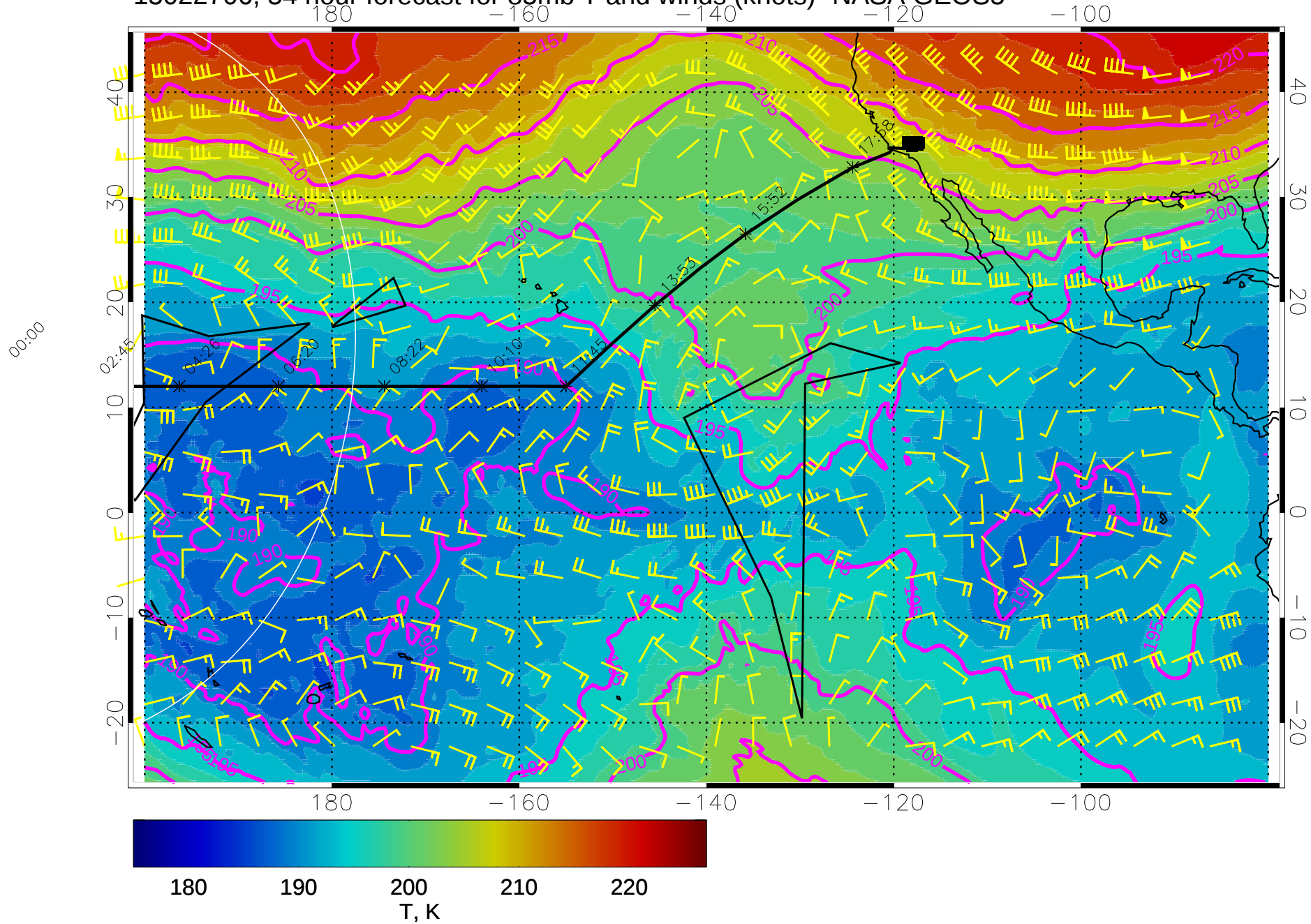
15022706, 54 hour forecast for 85mb T and winds (knots)- NASA GEOS5
