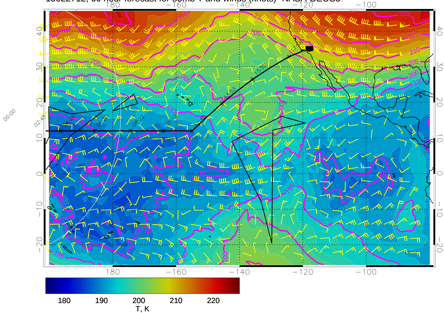
15022712, 60 hour forecast for 85mb T and winds (knots)- NASA GEOS5
