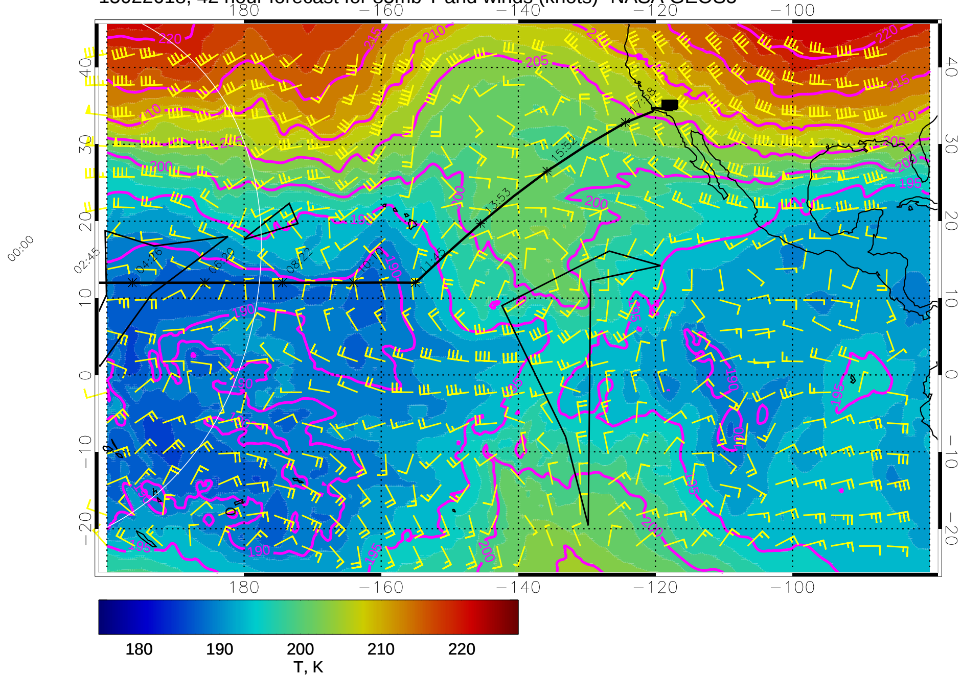
15022618, 42 hour forecast for 85mb T and winds (knots)- NASA GEOS5
