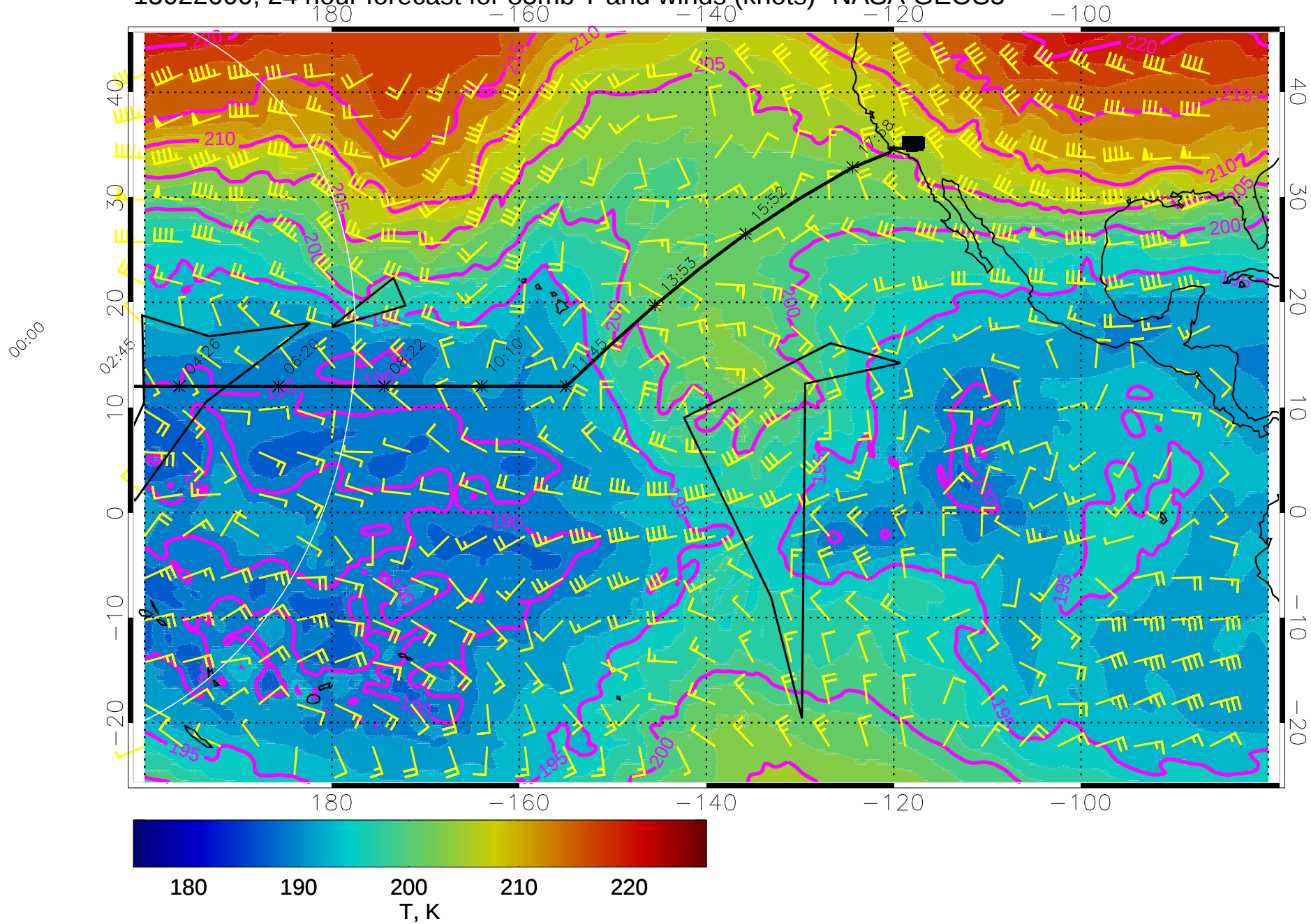
15022600, 24 hour forecast for 85mb T and winds (knots)- NASA GEOS5
