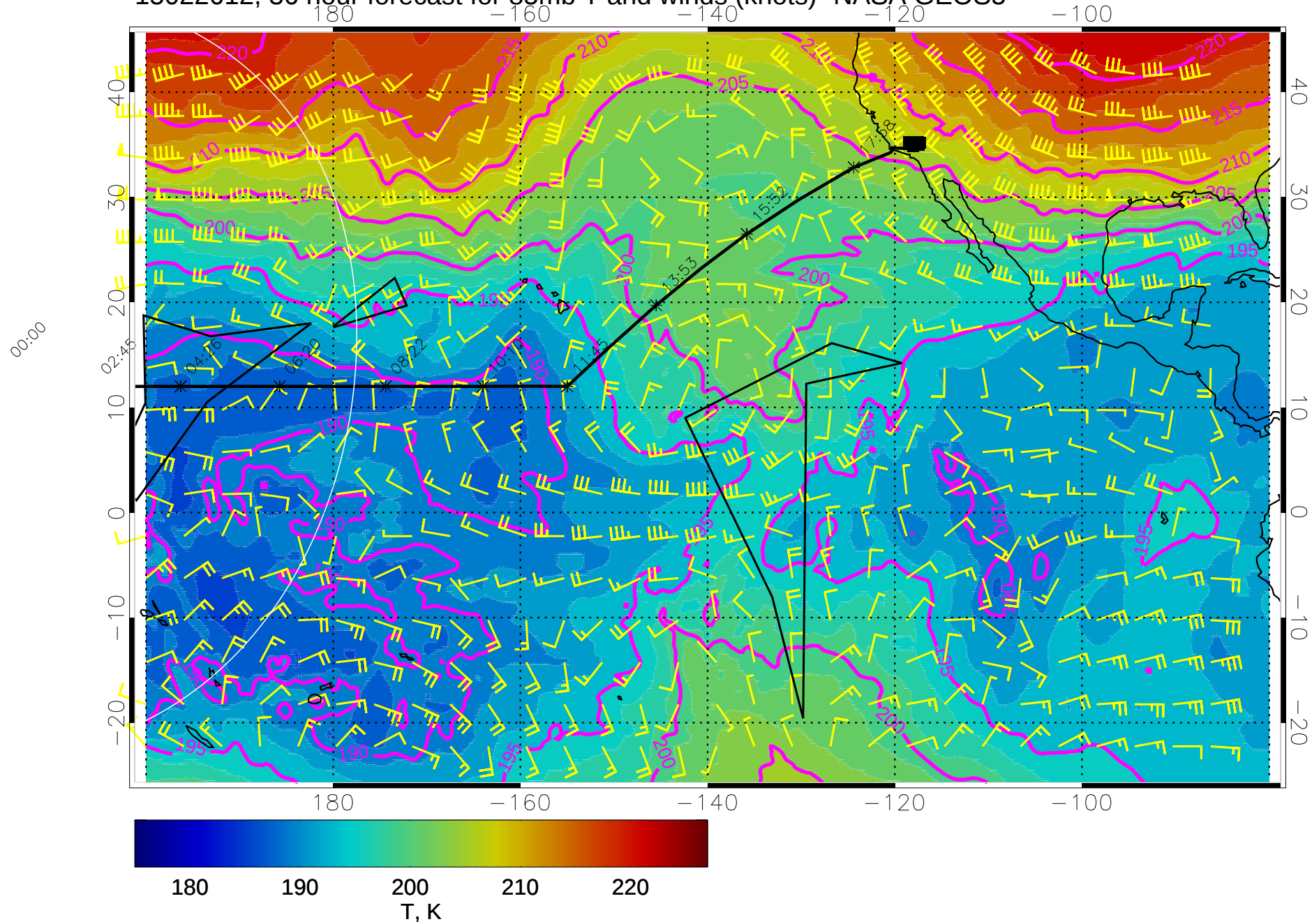
15022612, 36 hour forecast for 85mb T and winds (knots)- NASA GEOS5
