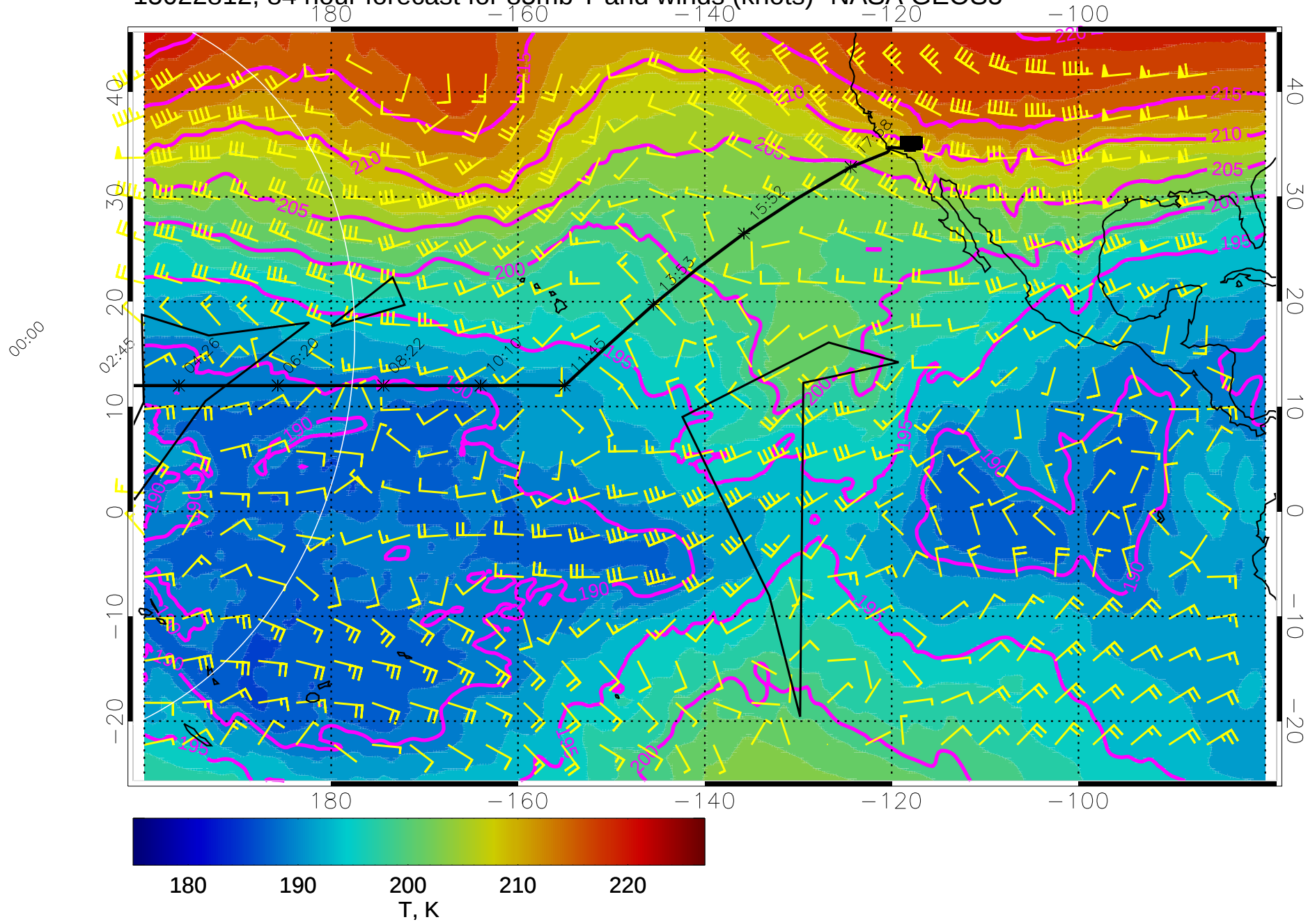
15022812, 84 hour forecast for 85mb T and winds (knots)- NASA GEOS5
