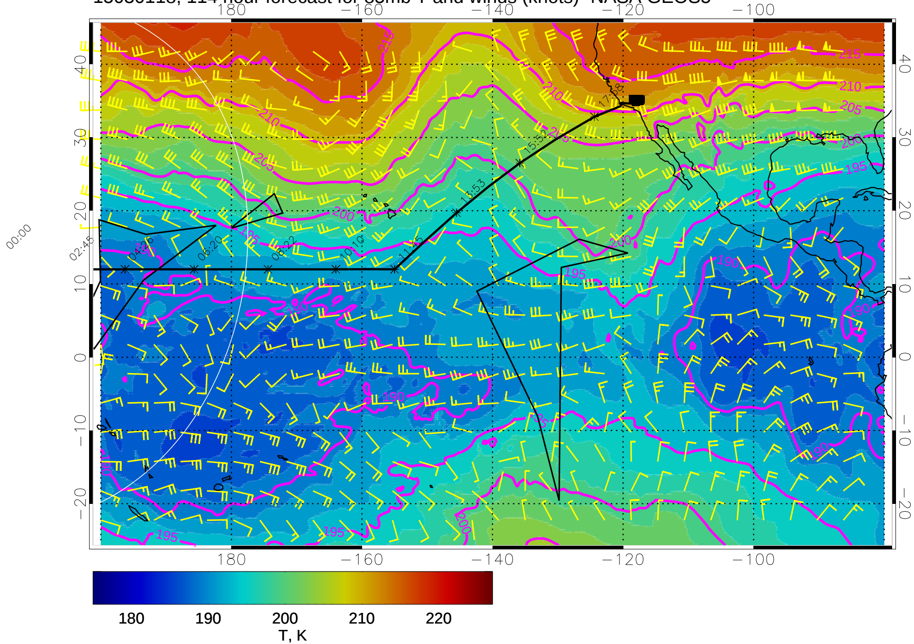
15030118, 114 hour forecast for 85mb T and winds (knots)- NASA GEOS5
