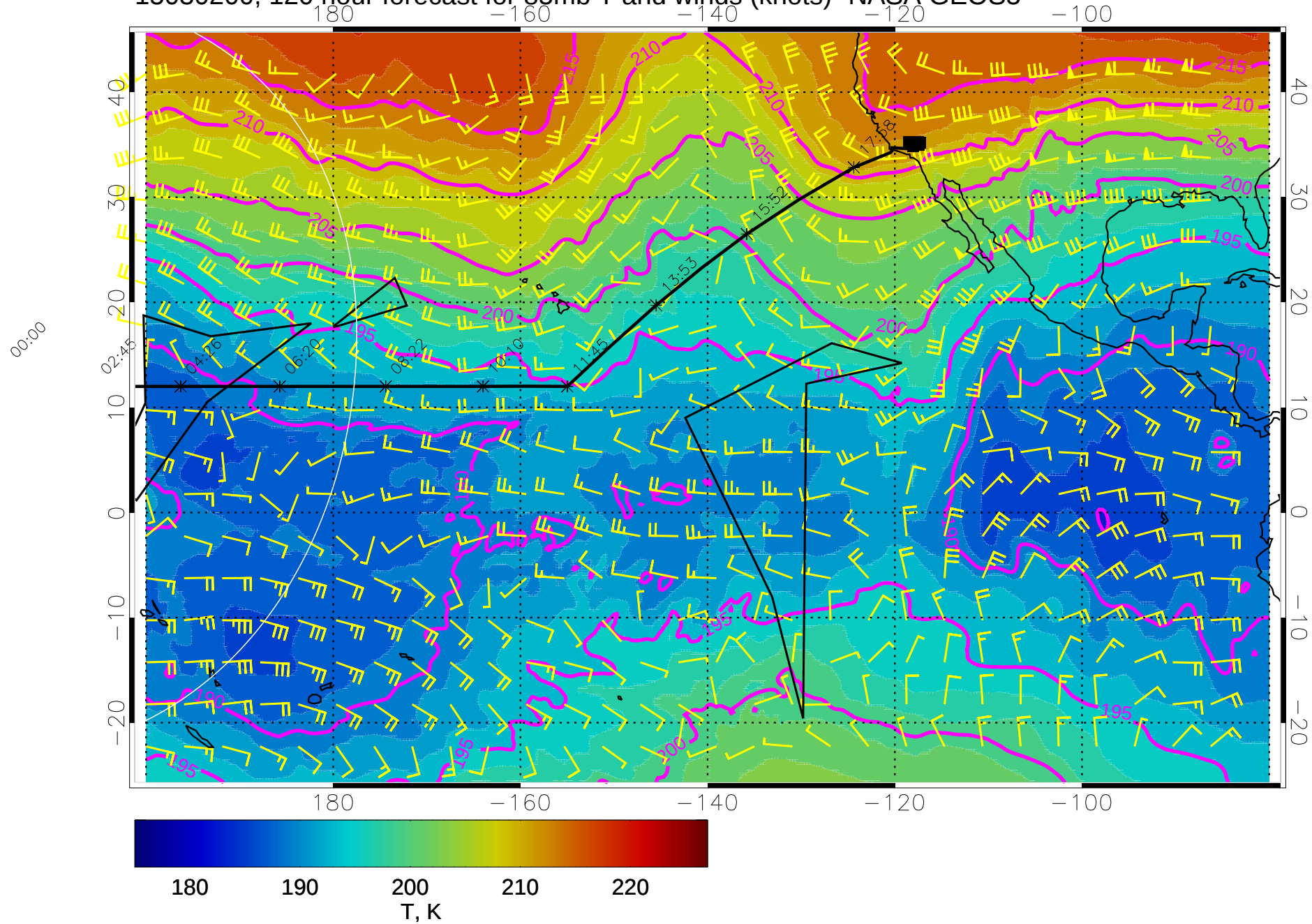
15030200, 120 hour forecast for 85mb T and winds (knots)- NASA GEOS5
