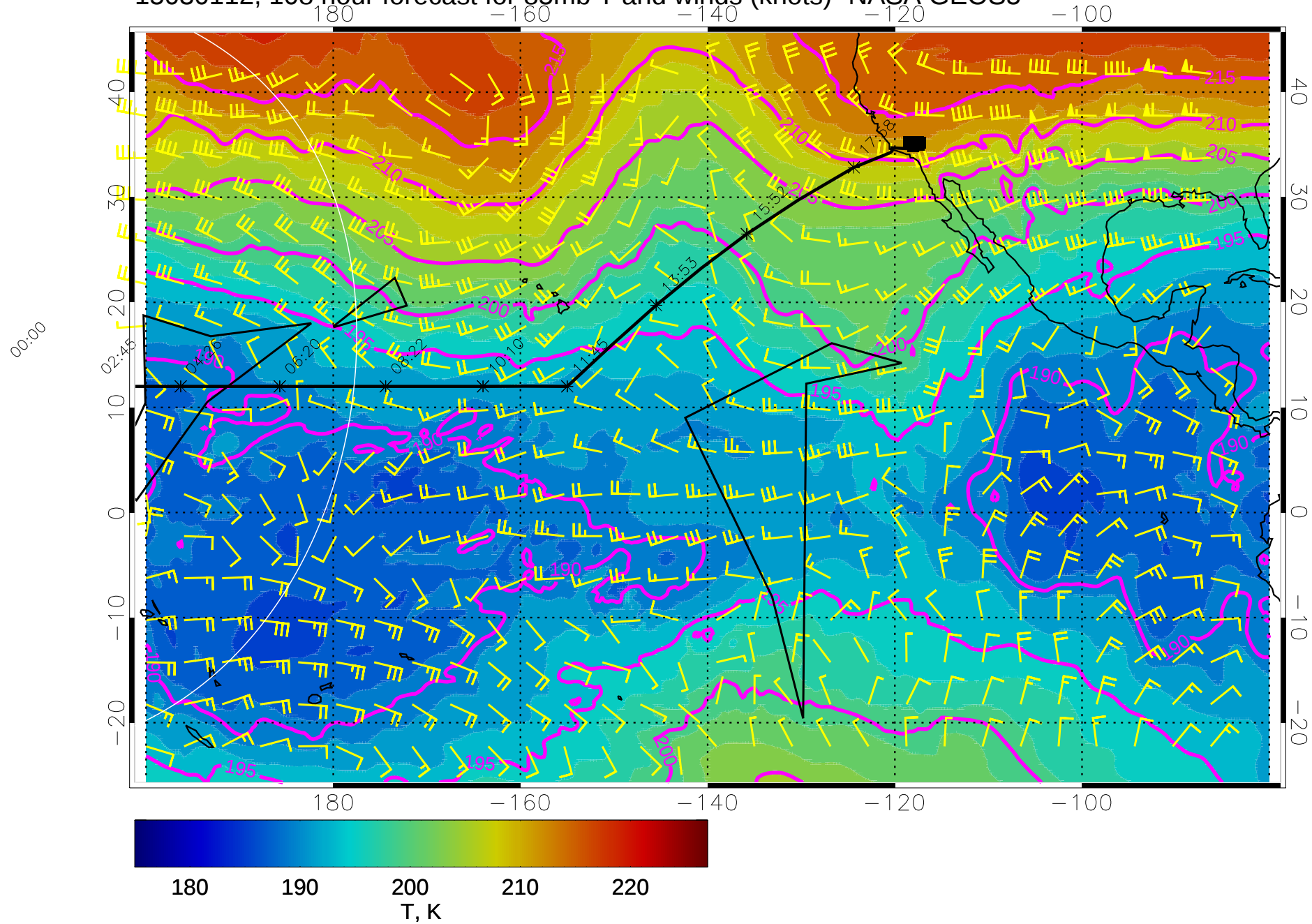
15030112, 108 hour forecast for 85mb T and winds (knots)- NASA GEOS5
