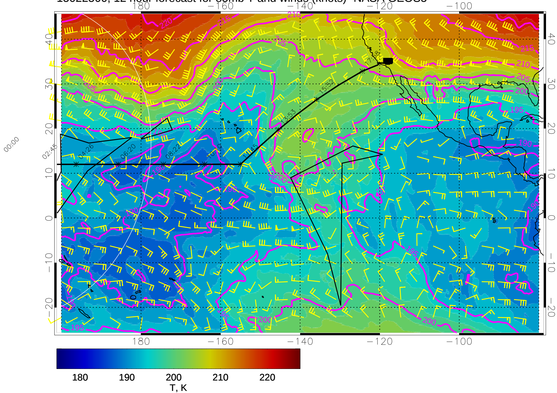
15022500, 12 hour forecast for 85mb T and winds (knots)- NASA GEOS5
