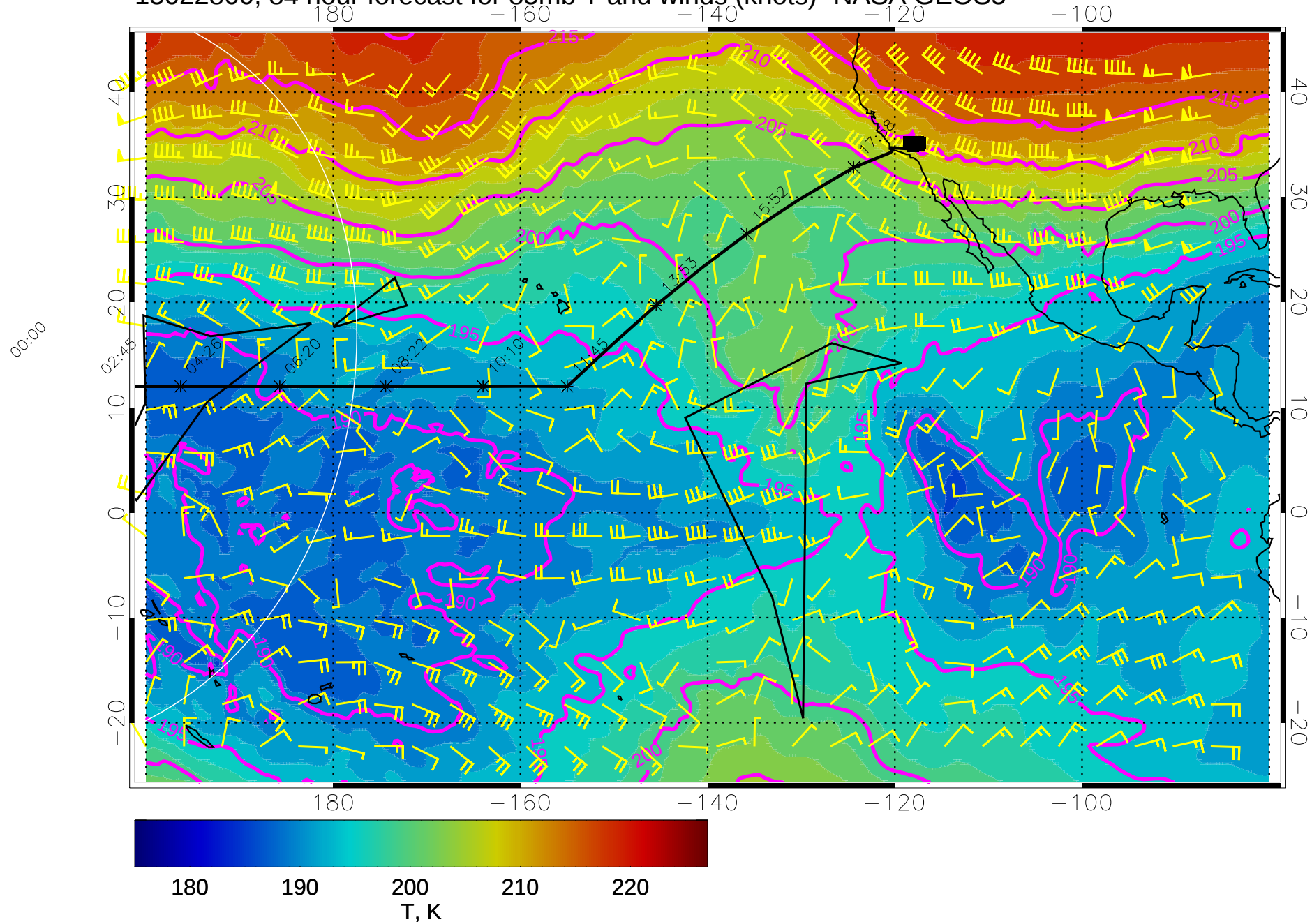
15022800, 84 hour forecast for 85mb T and winds (knots)- NASA GEOS5
