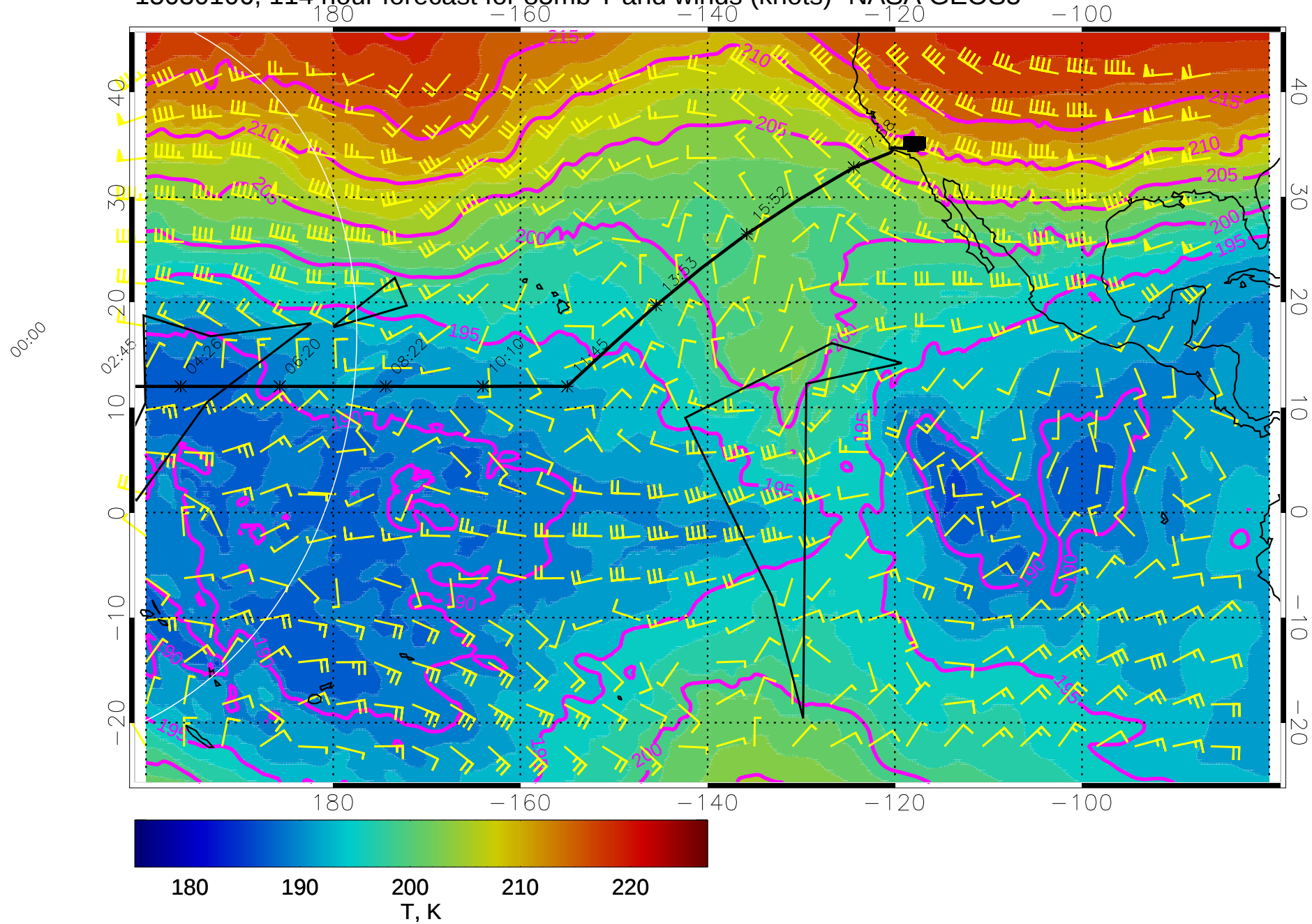
15030106, 114 hour forecast for 85mb T and winds (knots)- NASA GEOS5
