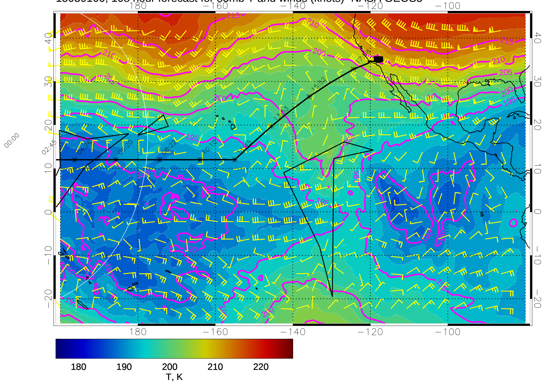
15030100, 108 hour forecast for 85mb T and winds (knots)- NASA GEOS5
