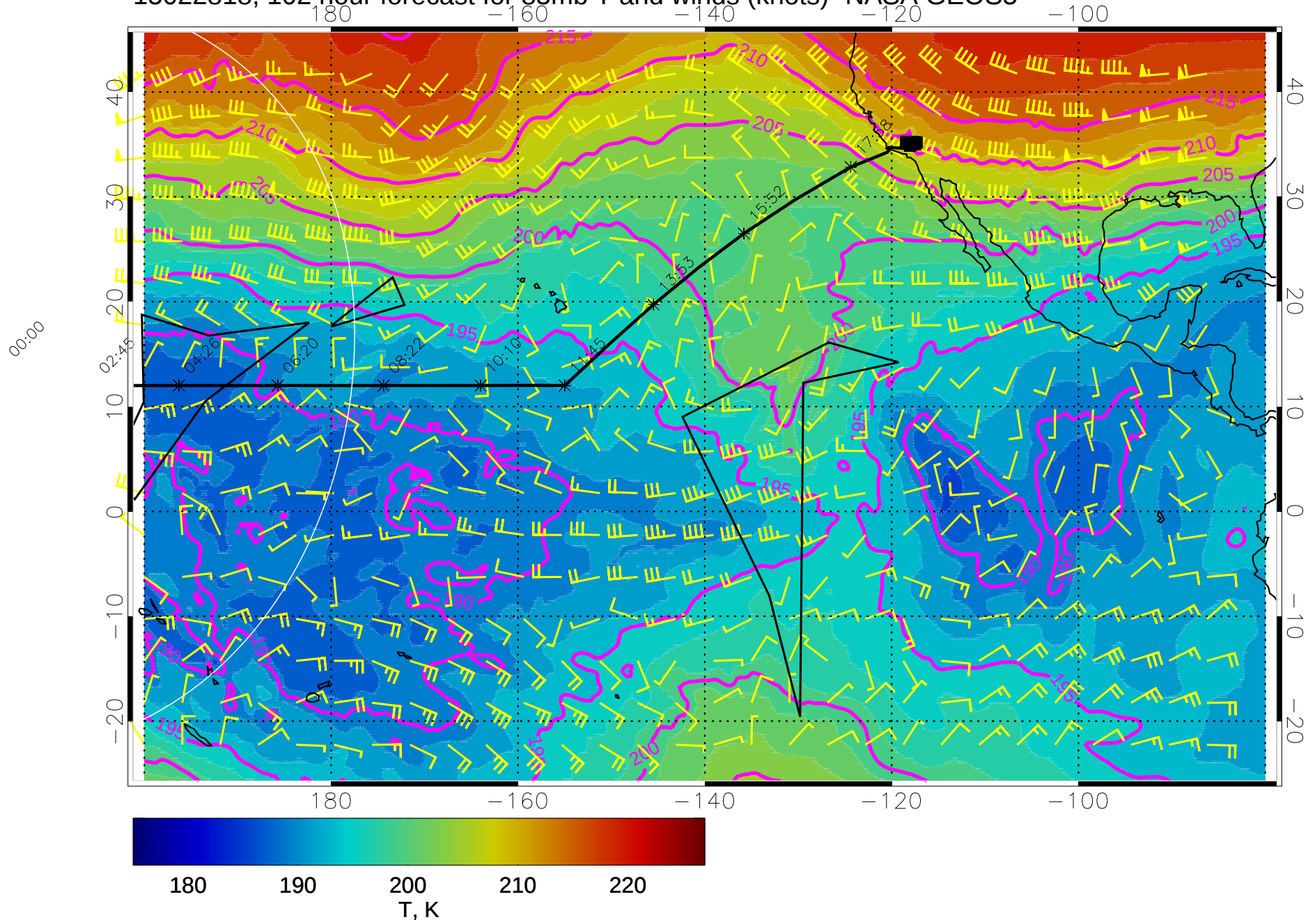
15022818, 102 hour forecast for 85mb T and winds (knots)- NASA GEOS5
