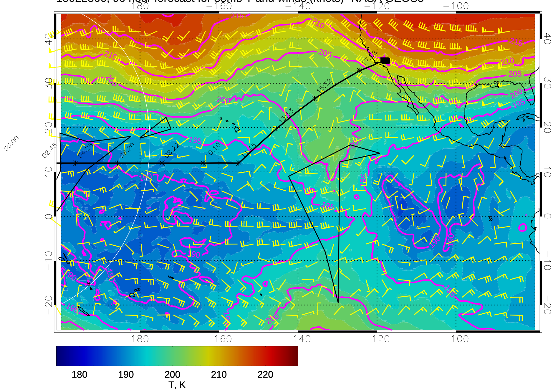
15022806, 90 hour forecast for 85mb T and winds (knots)- NASA GEOS5
