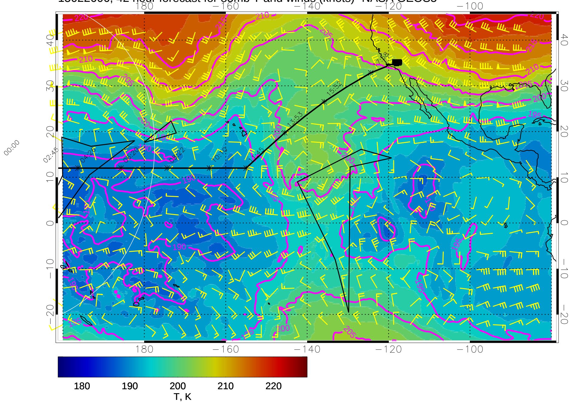
15022606, 42 hour forecast for 85mb T and winds (knots)- NASA GEOS5
