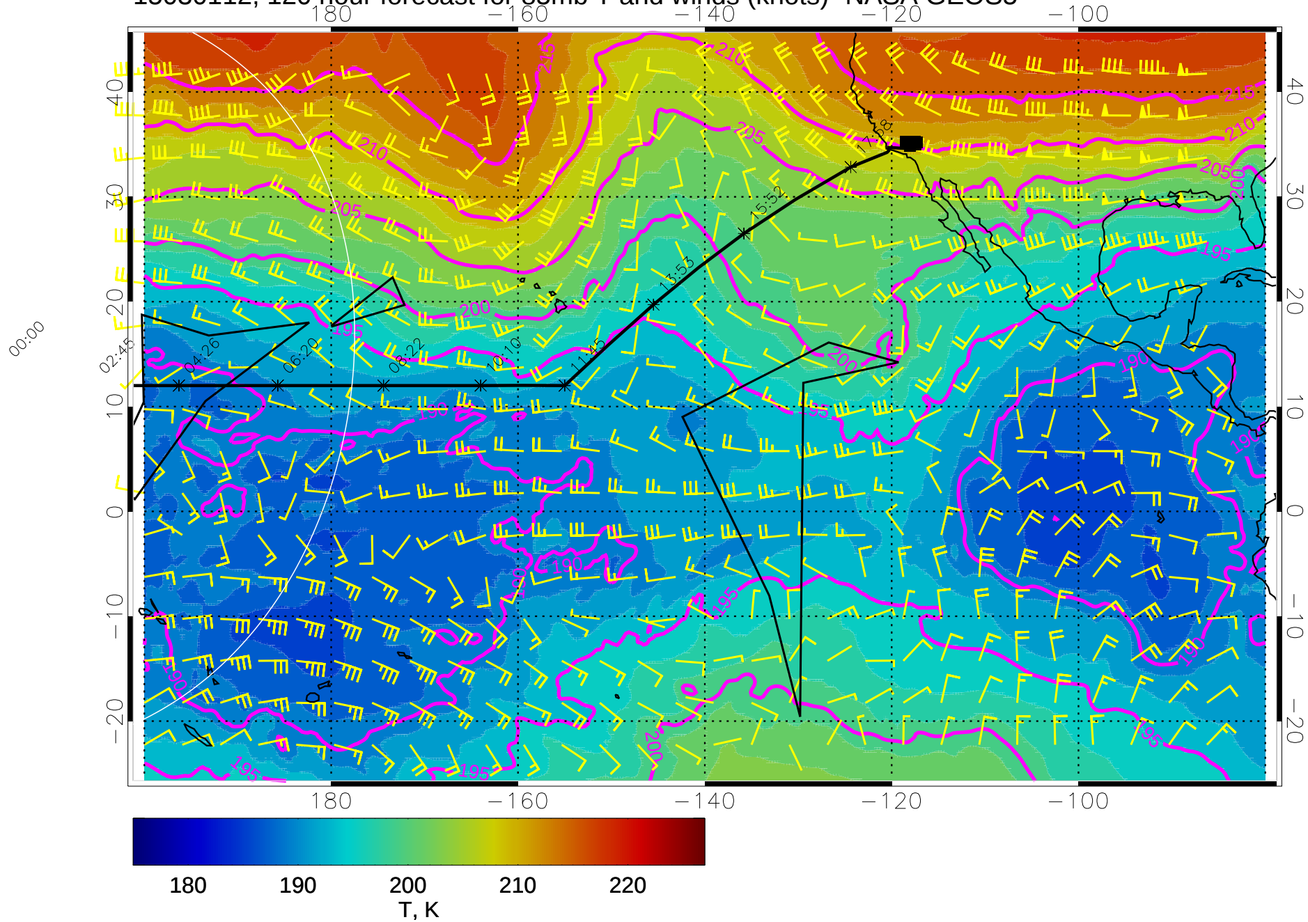
15030112, 120 hour forecast for 85mb T and winds (knots)- NASA GEOS5
