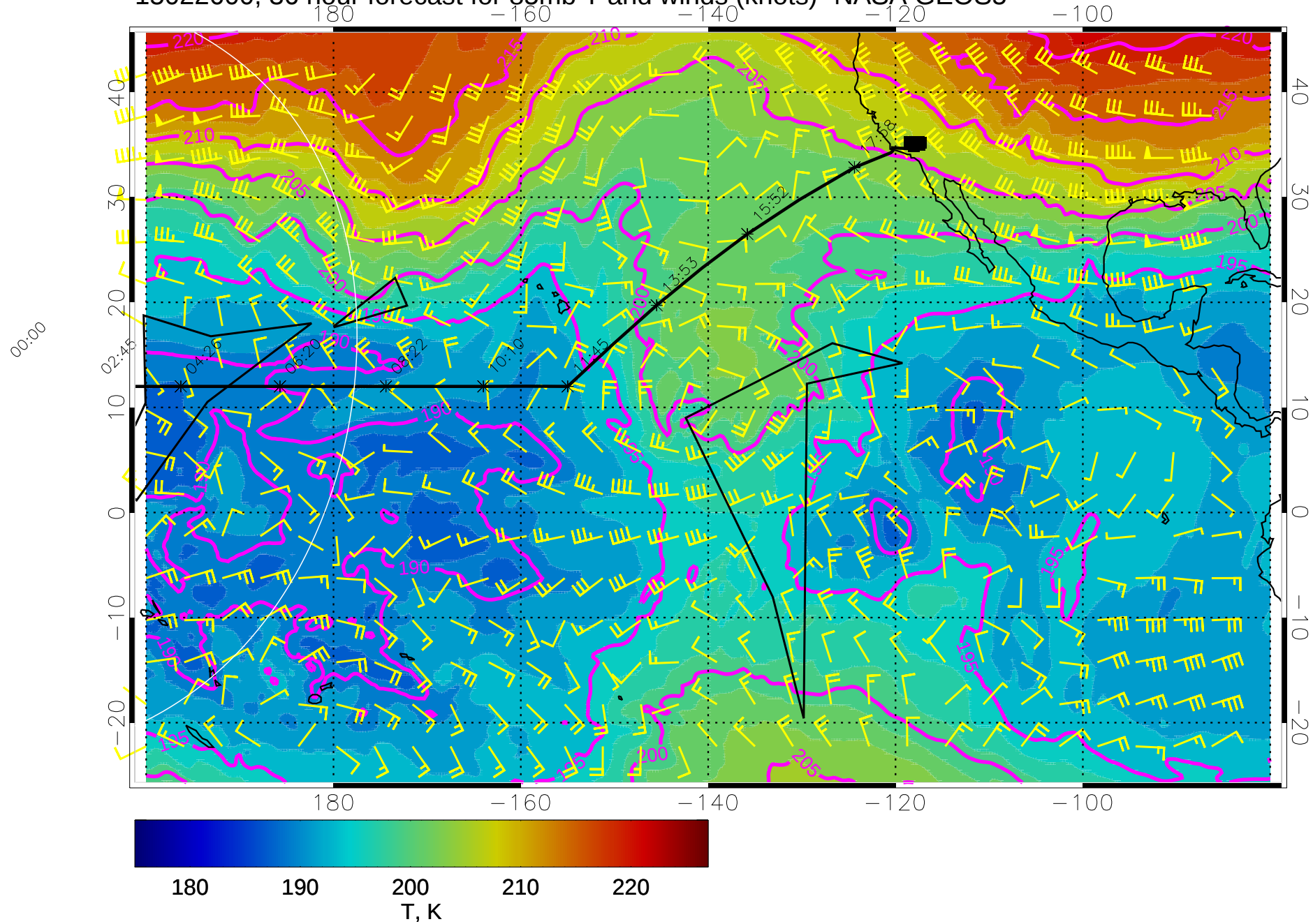
15022600, 36 hour forecast for 85mb T and winds (knots)- NASA GEOS5
