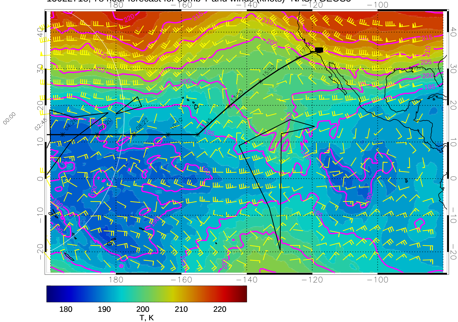
15022718, 78 hour forecast for 85mb T and winds (knots)- NASA GEOS5
