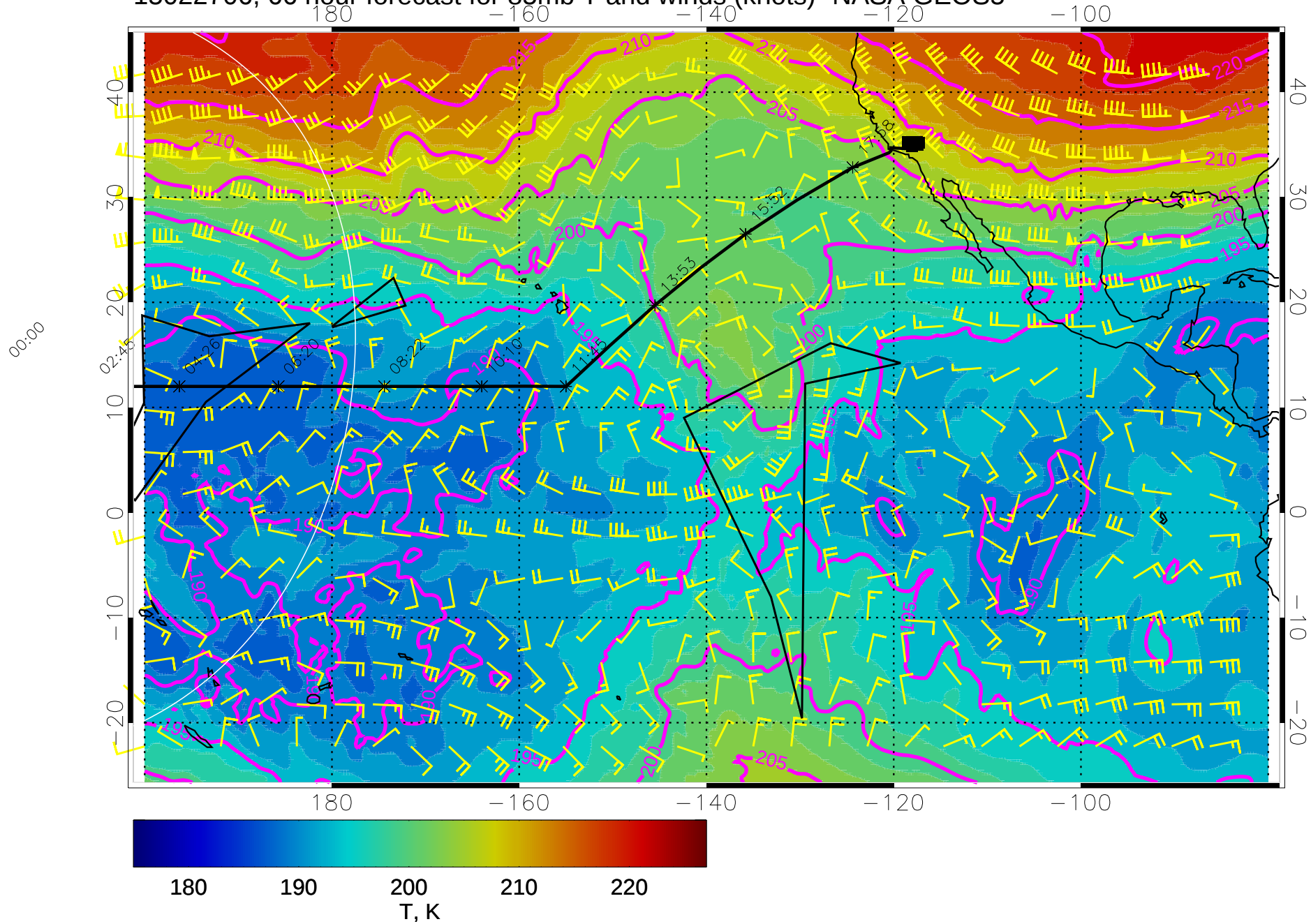
15022706, 66 hour forecast for 85mb T and winds (knots)- NASA GEOS5
