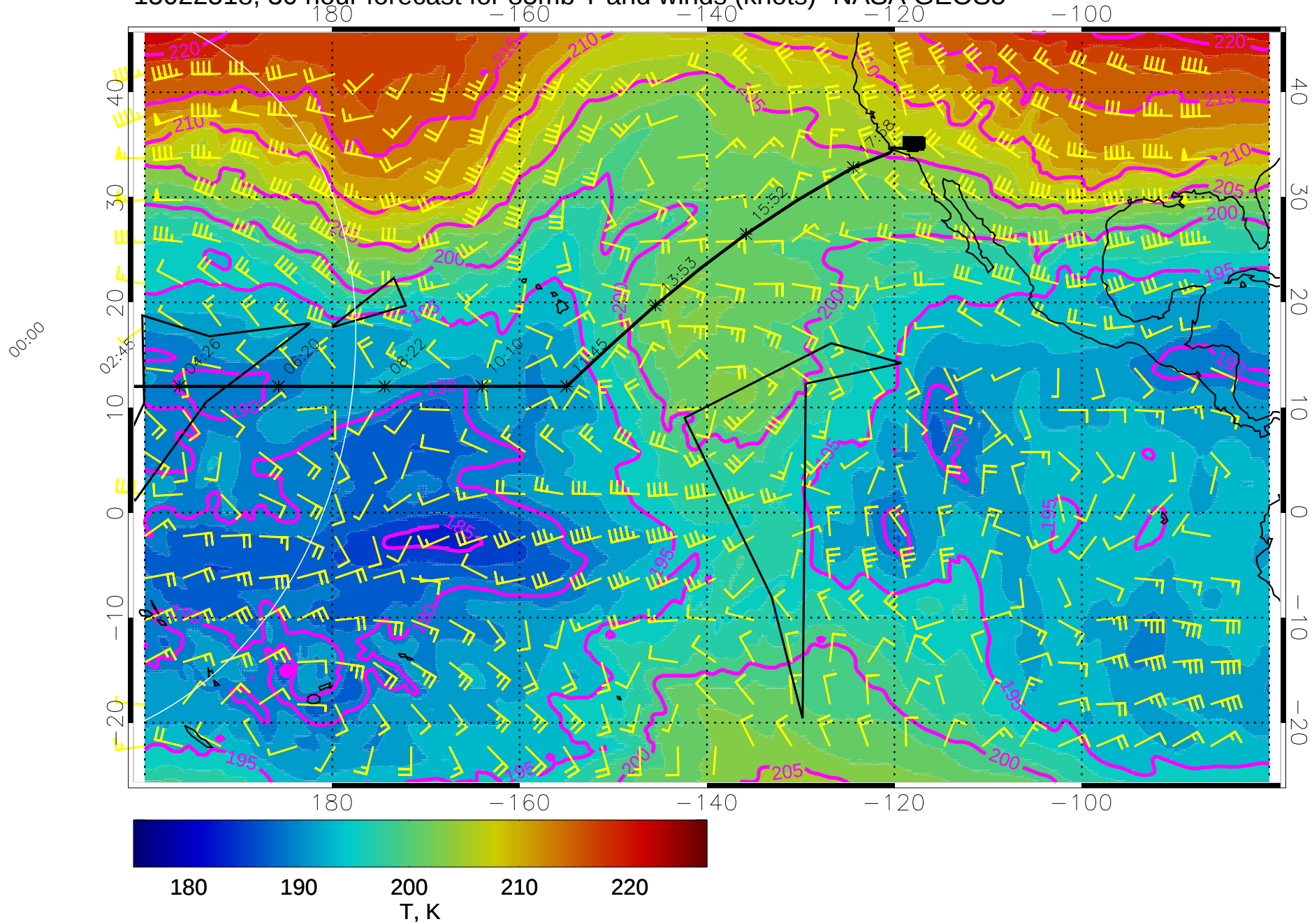
15022518, 30 hour forecast for 85mb T and winds (knots)- NASA GEOS5
