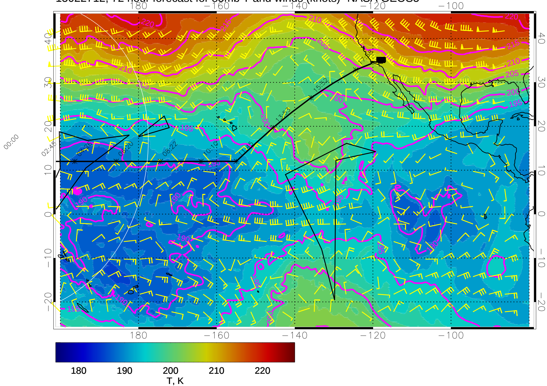
15022712, 72 hour forecast for 85mb T and winds (knots)- NASA GEOS5
