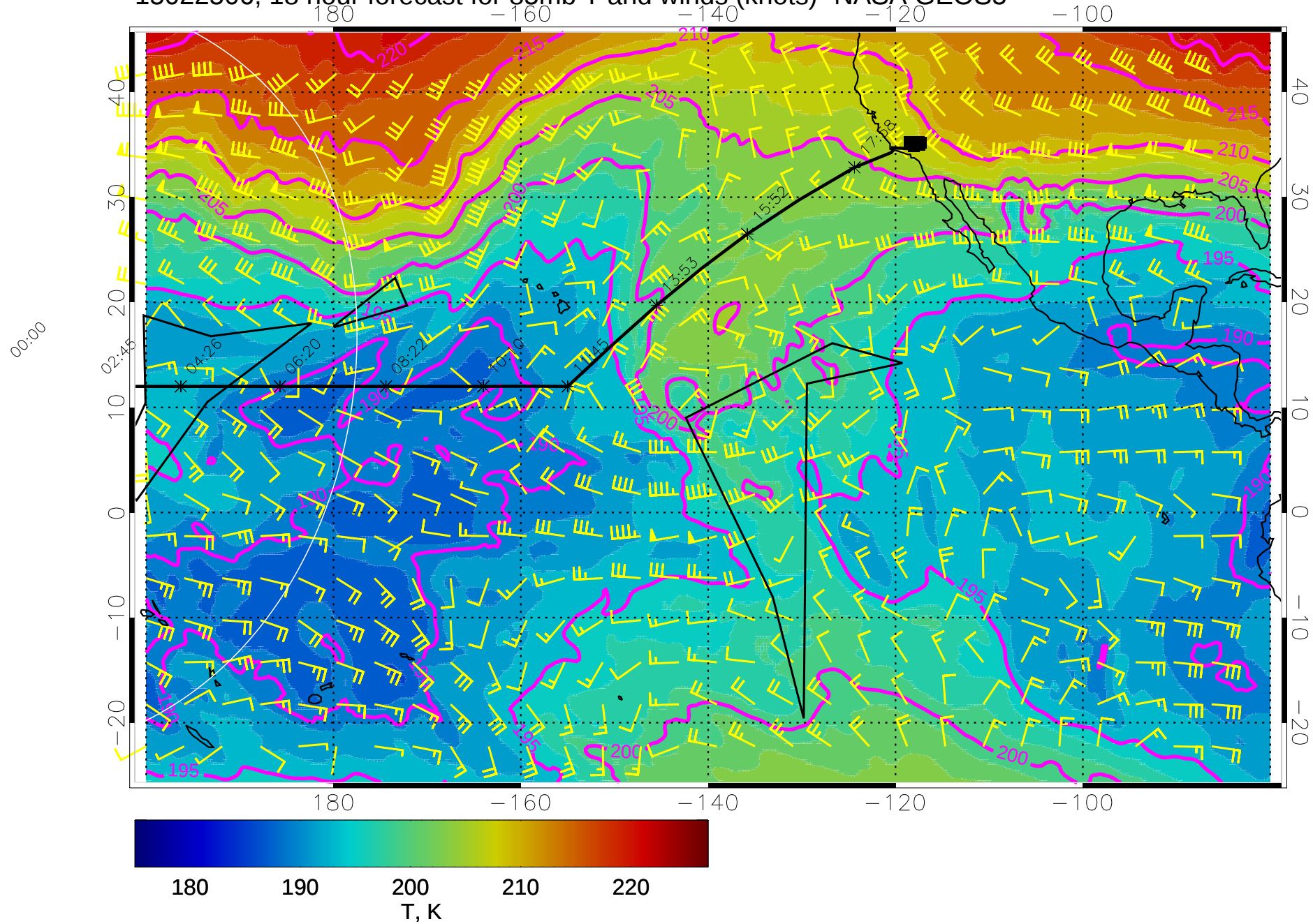
15022506, 18 hour forecast for 85mb T and winds (knots)- NASA GEOS5
