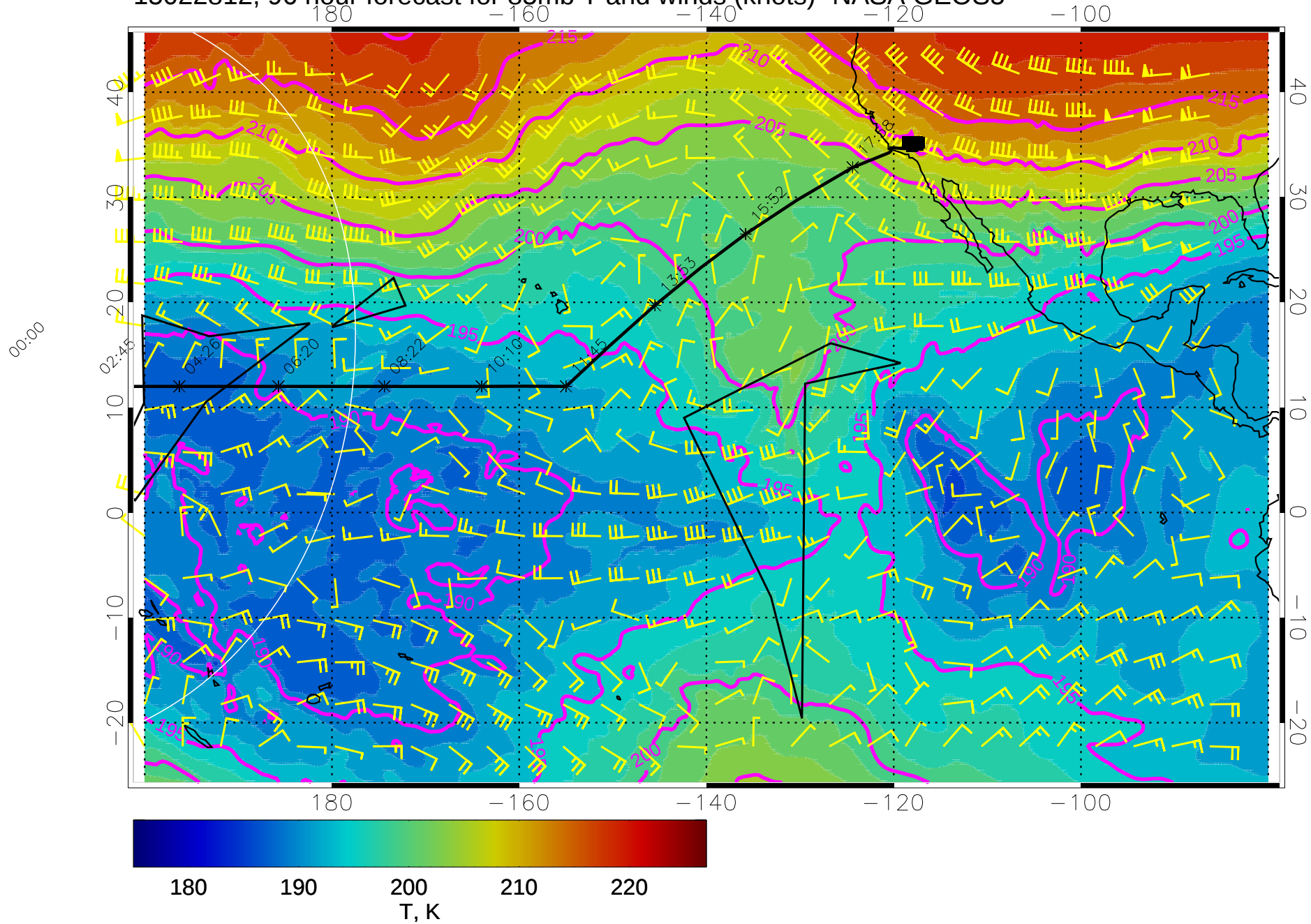
15022812, 96 hour forecast for 85mb T and winds (knots)- NASA GEOS5
