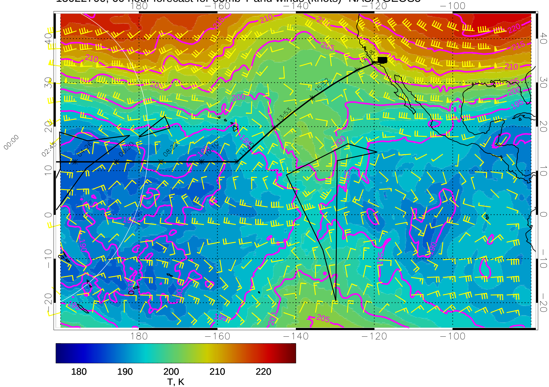
15022700, 60 hour forecast for 85mb T and winds (knots)- NASA GEOS5
