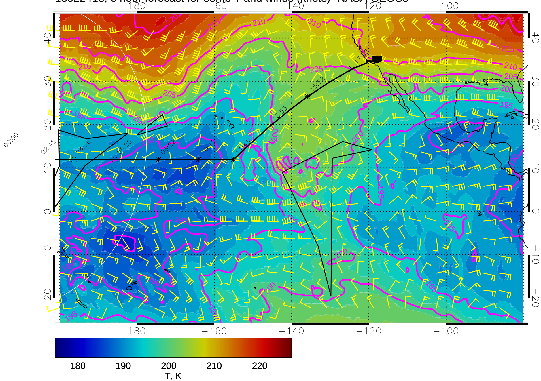
15022418, 6 hour forecast for 85mb T and winds (knots)- NASA GEOS5
