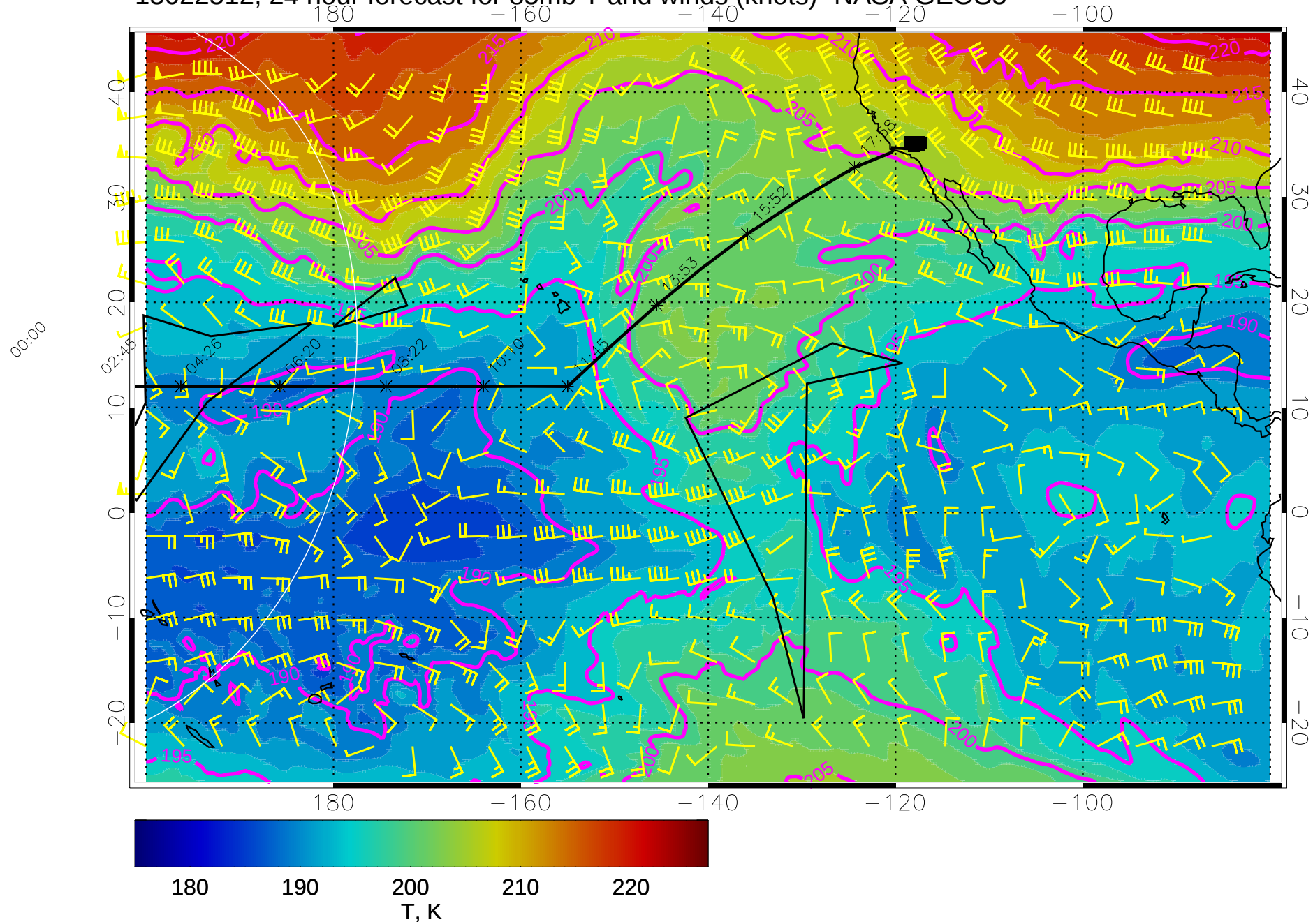
15022512, 24 hour forecast for 85mb T and winds (knots)- NASA GEOS5
