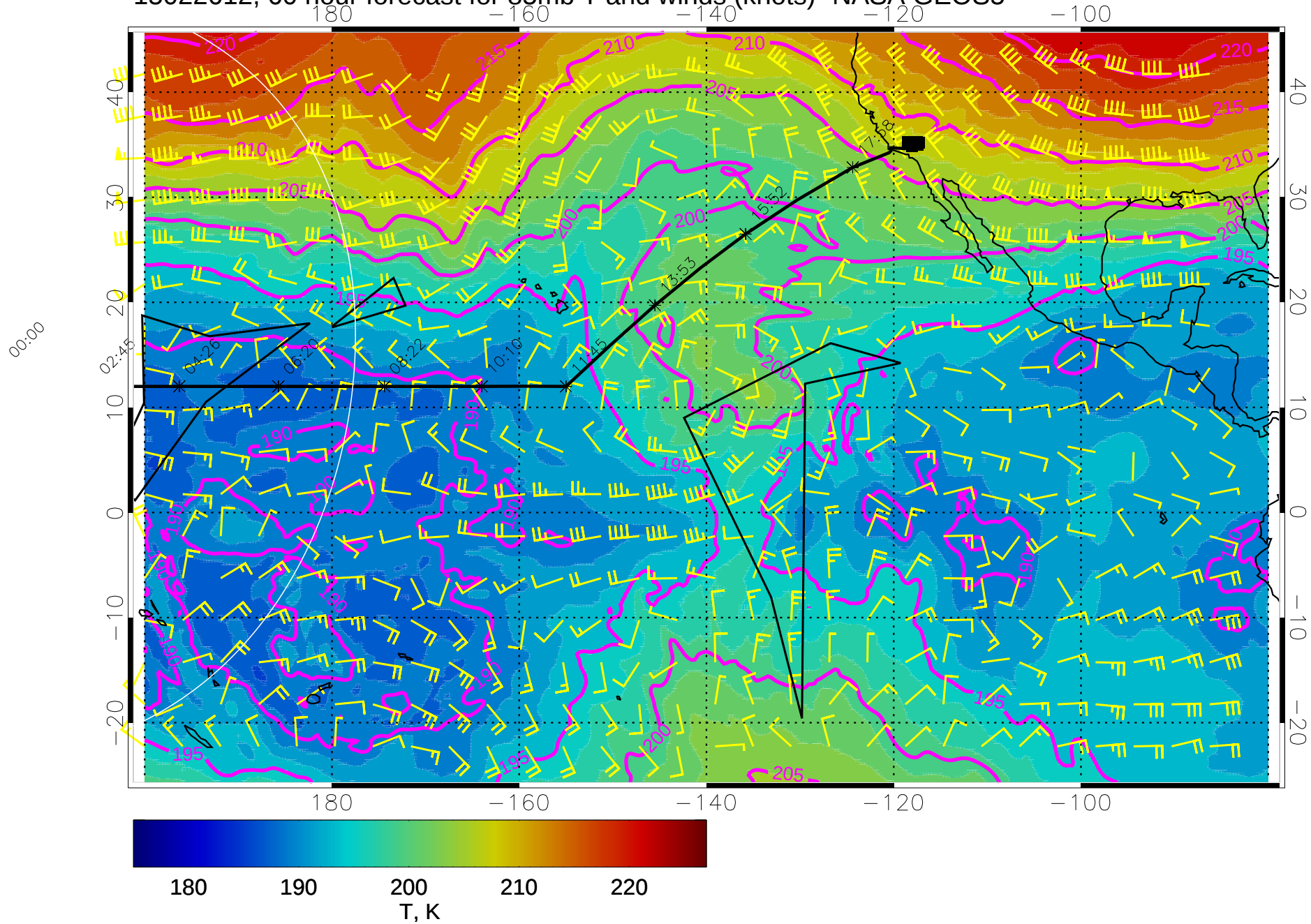
15022612, 60 hour forecast for 85mb T and winds (knots)- NASA GEOS5
