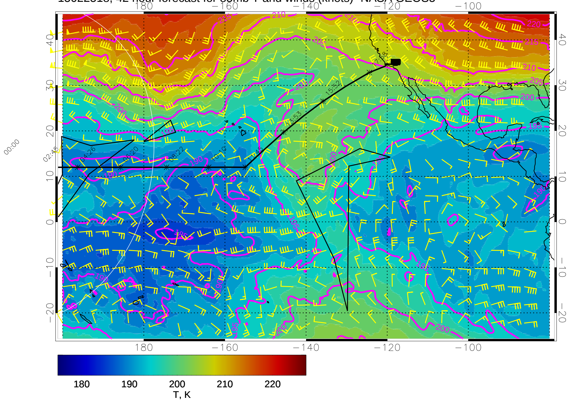
15022518, 42 hour forecast for 85mb T and winds (knots)- NASA GEOS5
