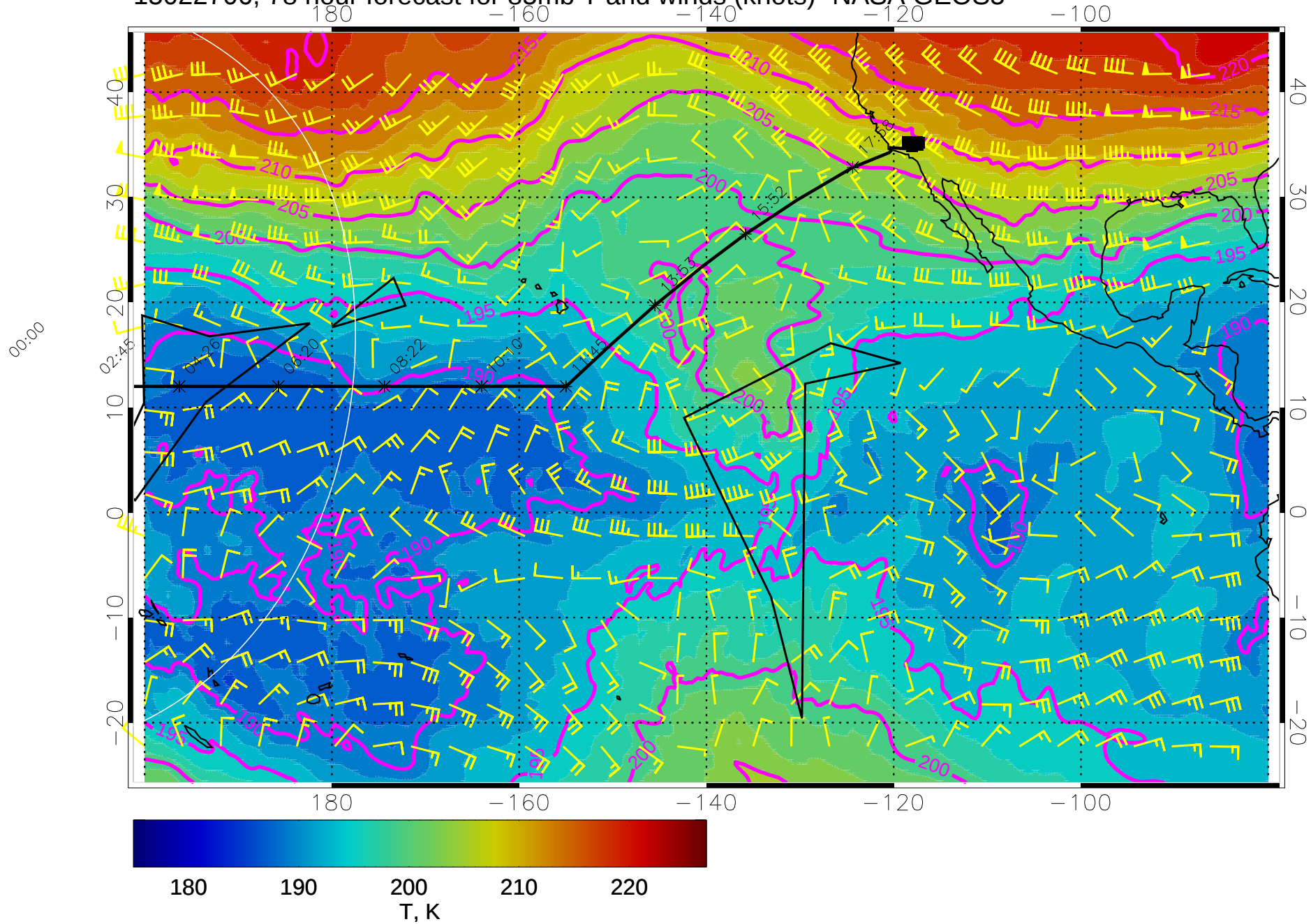
15022706, 78 hour forecast for 85mb T and winds (knots)- NASA GEOS5
