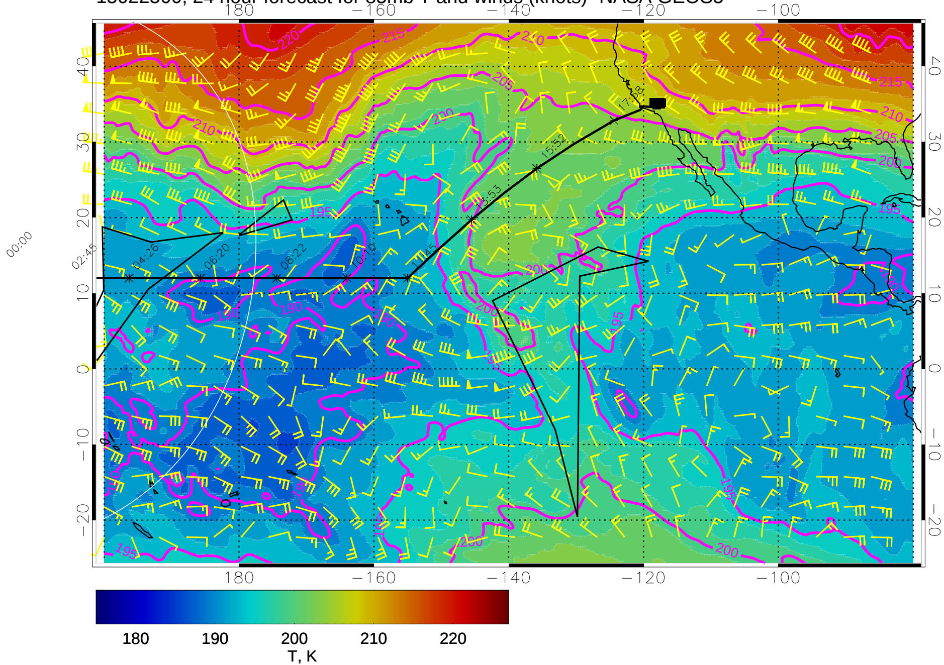
15022500, 24 hour forecast for 85mb T and winds (knots)- NASA GEOS5
