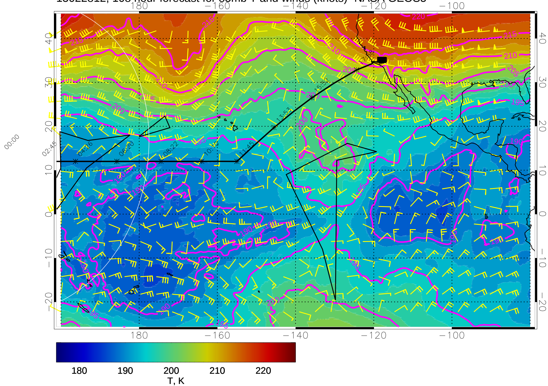
15022812, 108 hour forecast for 85mb T and winds (knots)- NASA GEOS5
