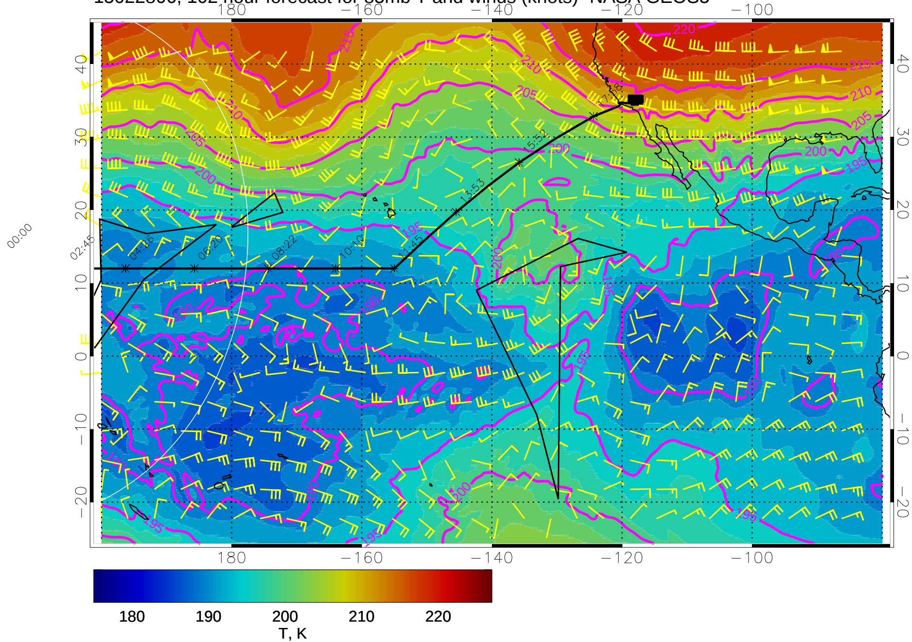
15022806, 102 hour forecast for 85mb T and winds (knots)- NASA GEOS5
