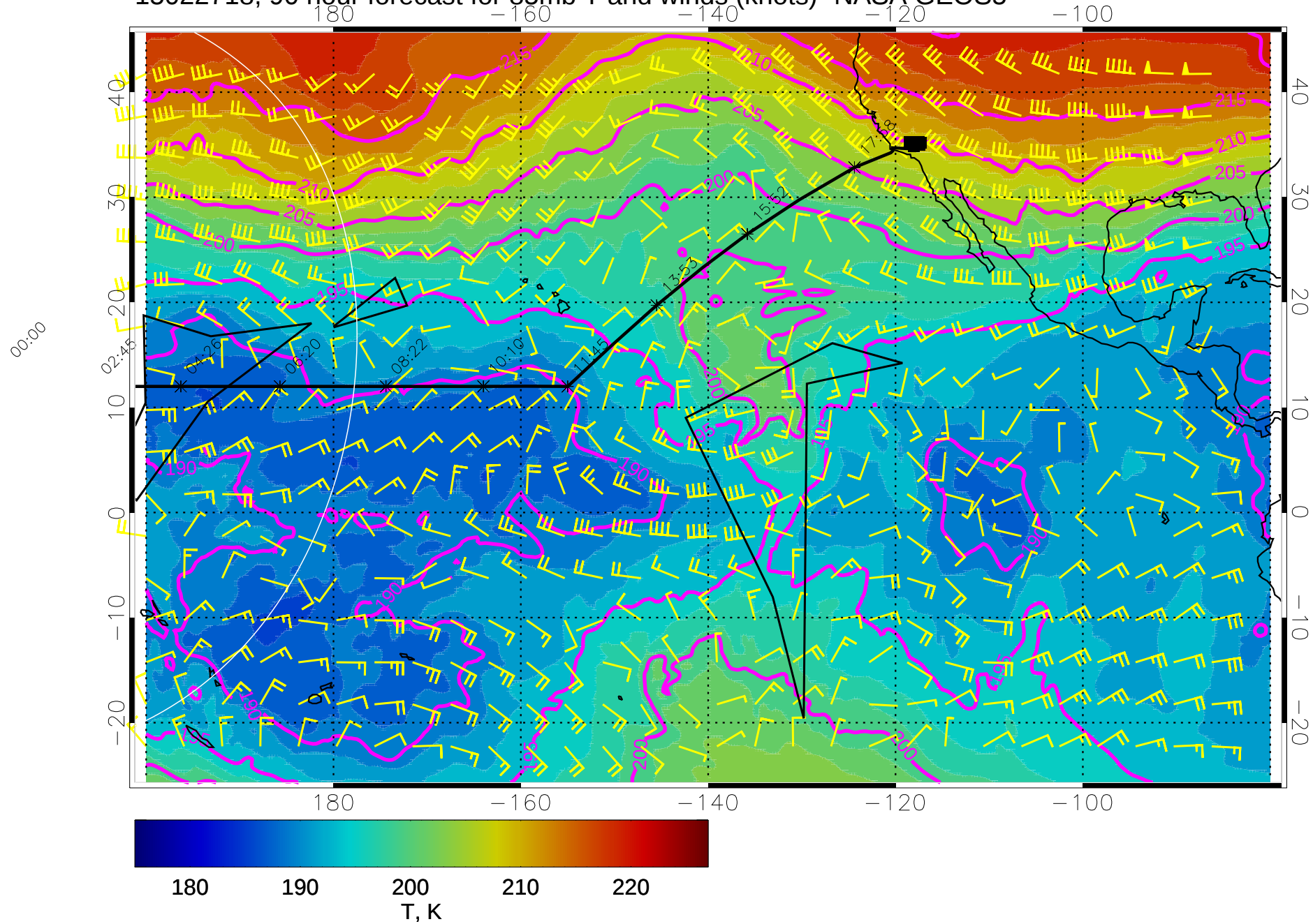
15022718, 90 hour forecast for 85mb T and winds (knots)- NASA GEOS5
