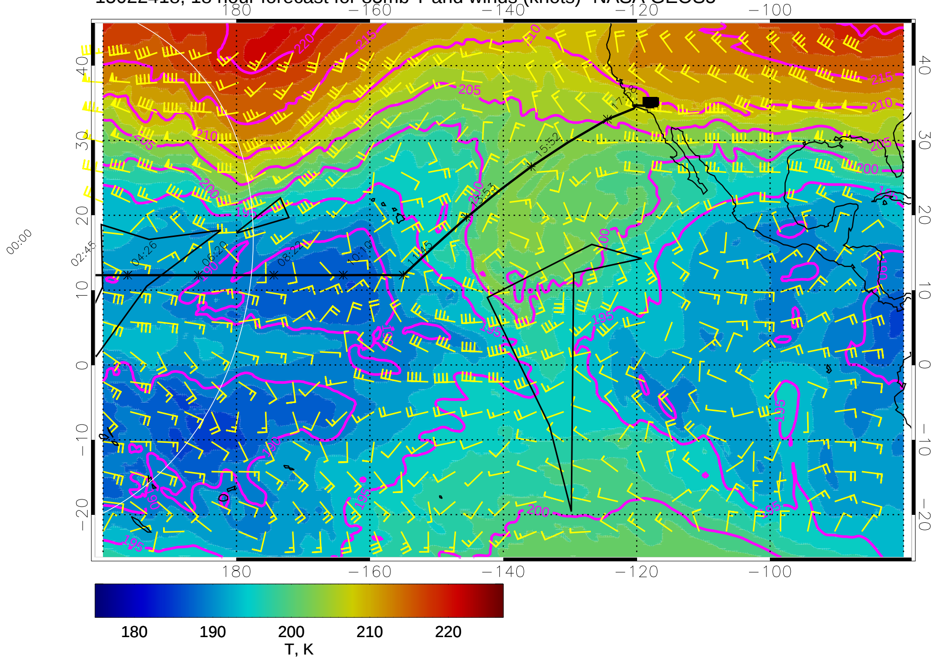
15022418, 18 hour forecast for 85mb T and winds (knots)- NASA GEOS5
