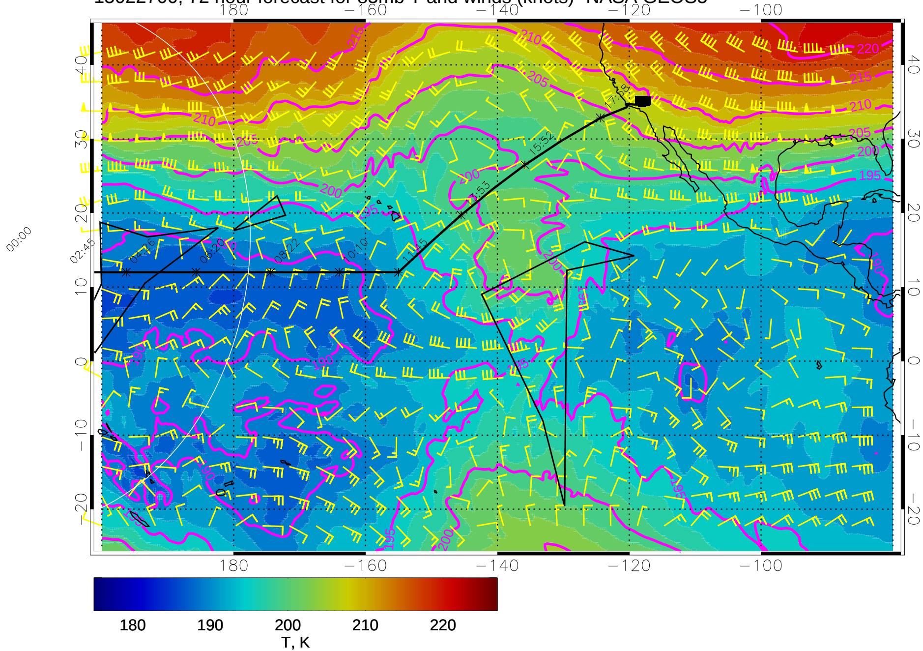
15022700, 72 hour forecast for 85mb T and winds (knots)- NASA GEOS5
