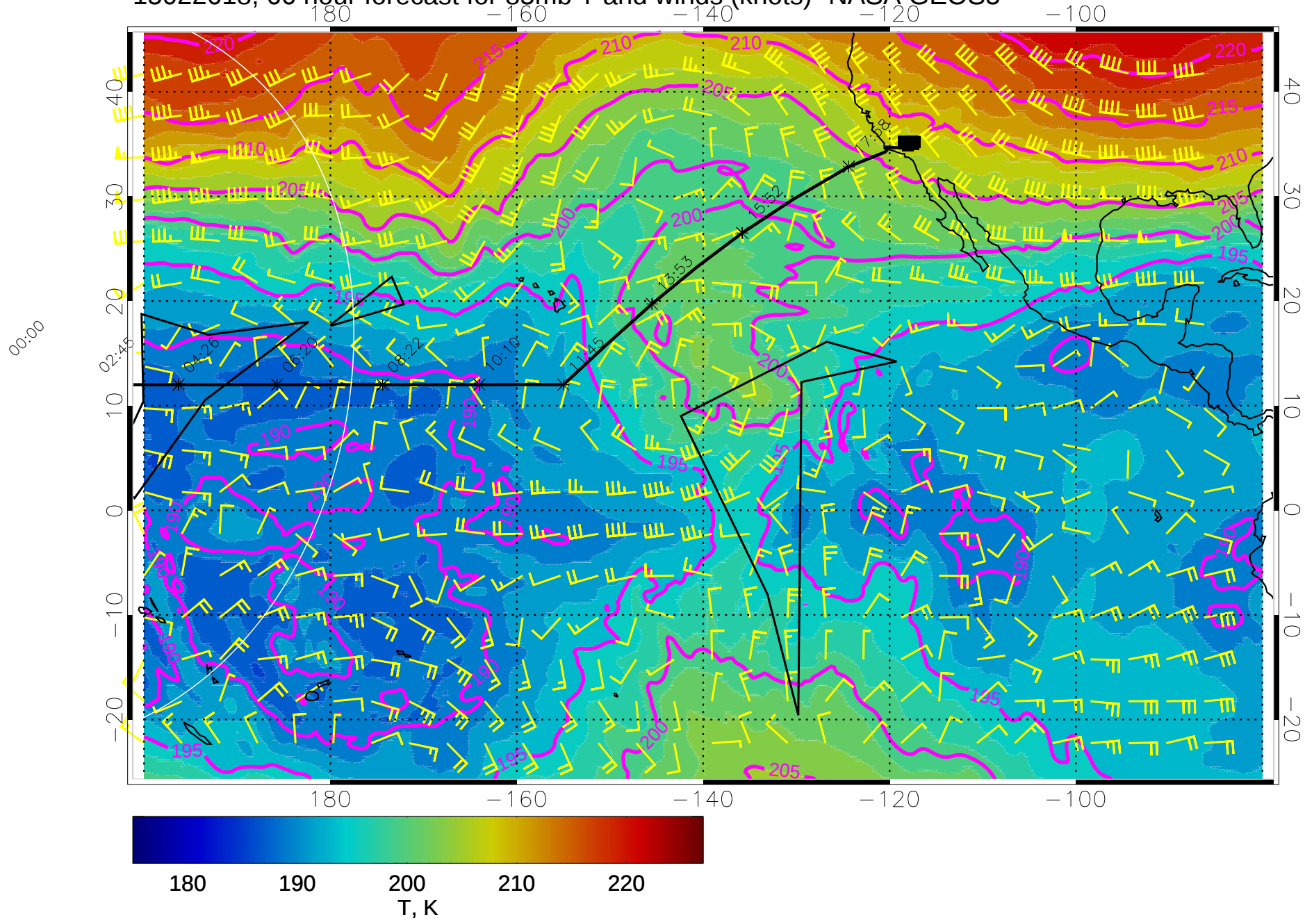
15022618, 66 hour forecast for 85mb T and winds (knots)- NASA GEOS5
