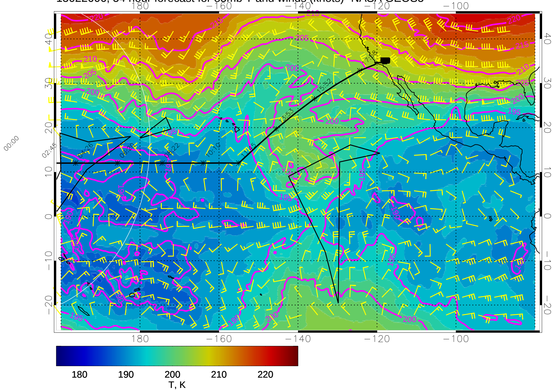
15022606, 54 hour forecast for 85mb T and winds (knots)- NASA GEOS5
