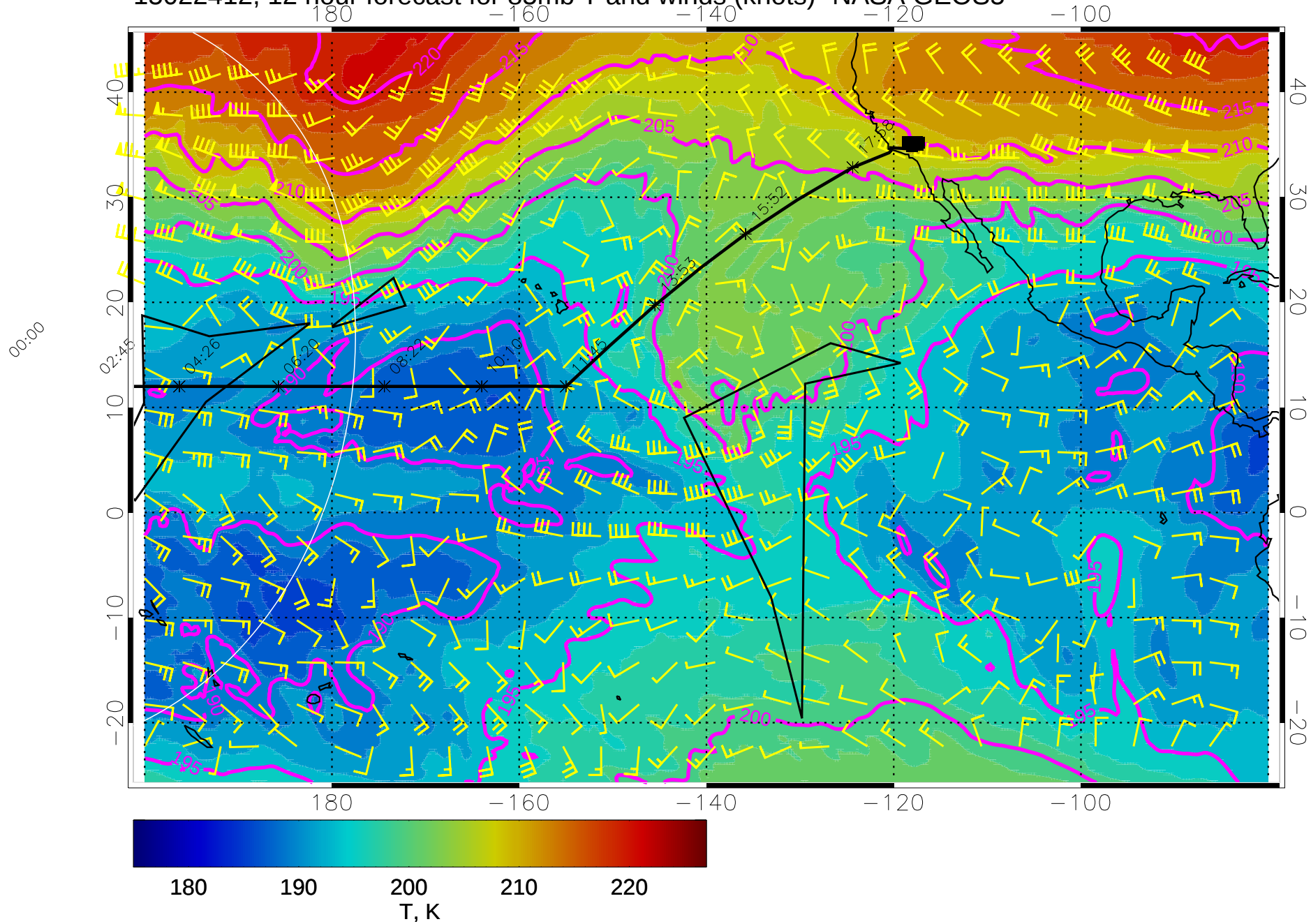
15022412, 12 hour forecast for 85mb T and winds (knots)- NASA GEOS5
