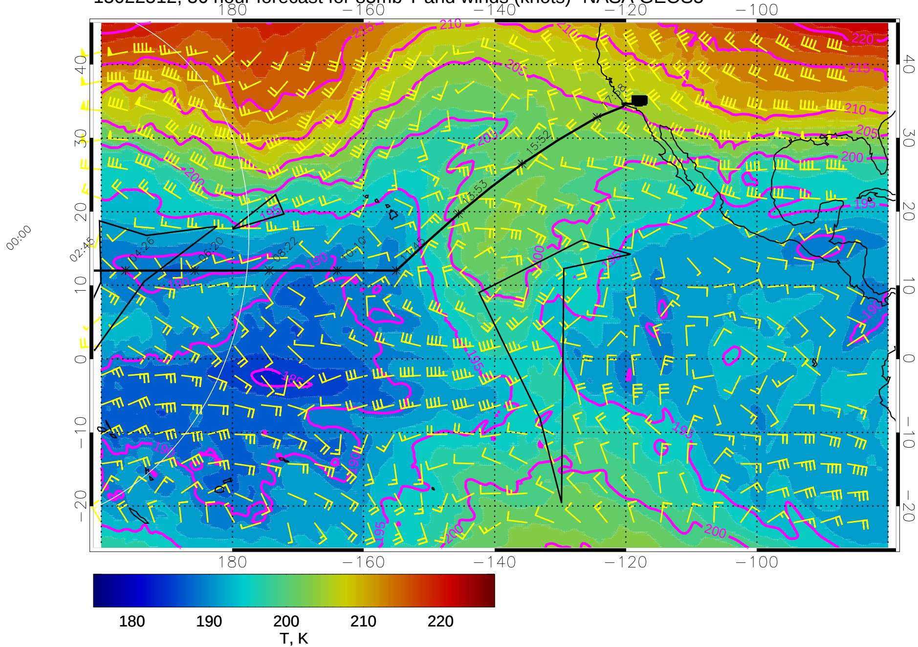
15022512, 36 hour forecast for 85mb T and winds (knots)- NASA GEOS5
