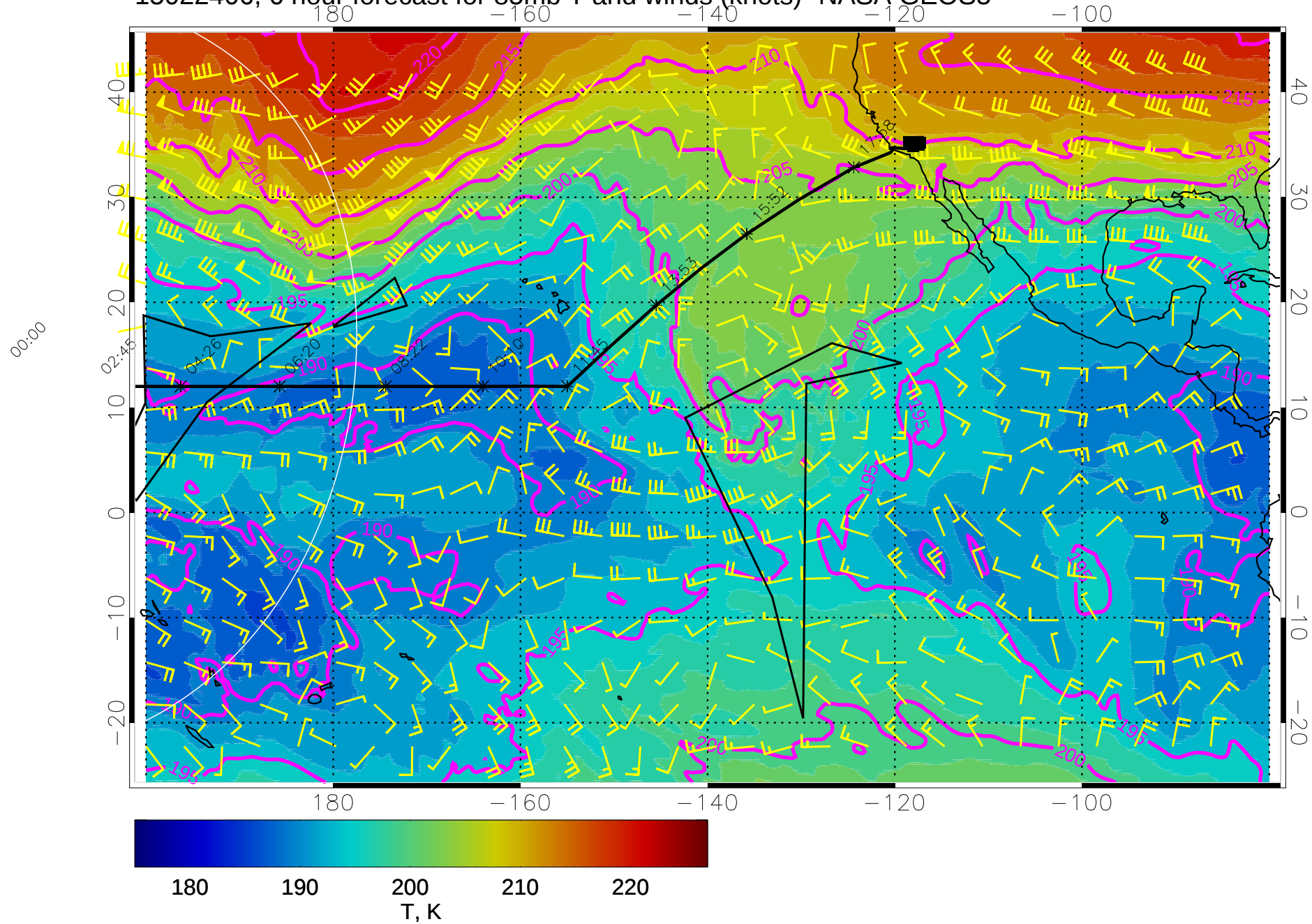
15022406, 6 hour forecast for 85mb T and winds (knots)- NASA GEOS5
