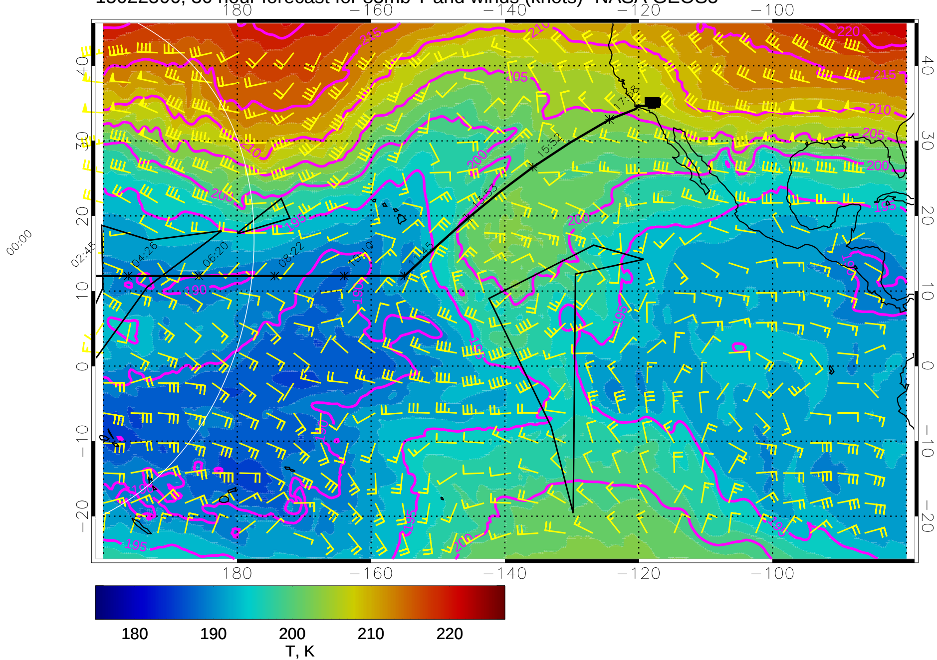
15022506, 30 hour forecast for 85mb T and winds (knots)- NASA GEOS5
