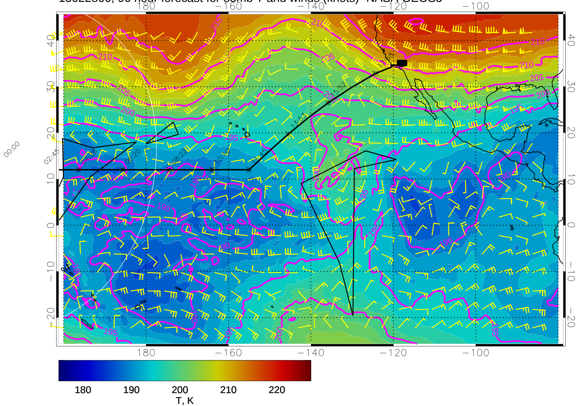
15022800, 96 hour forecast for 85mb T and winds (knots)- NASA GEOS5
