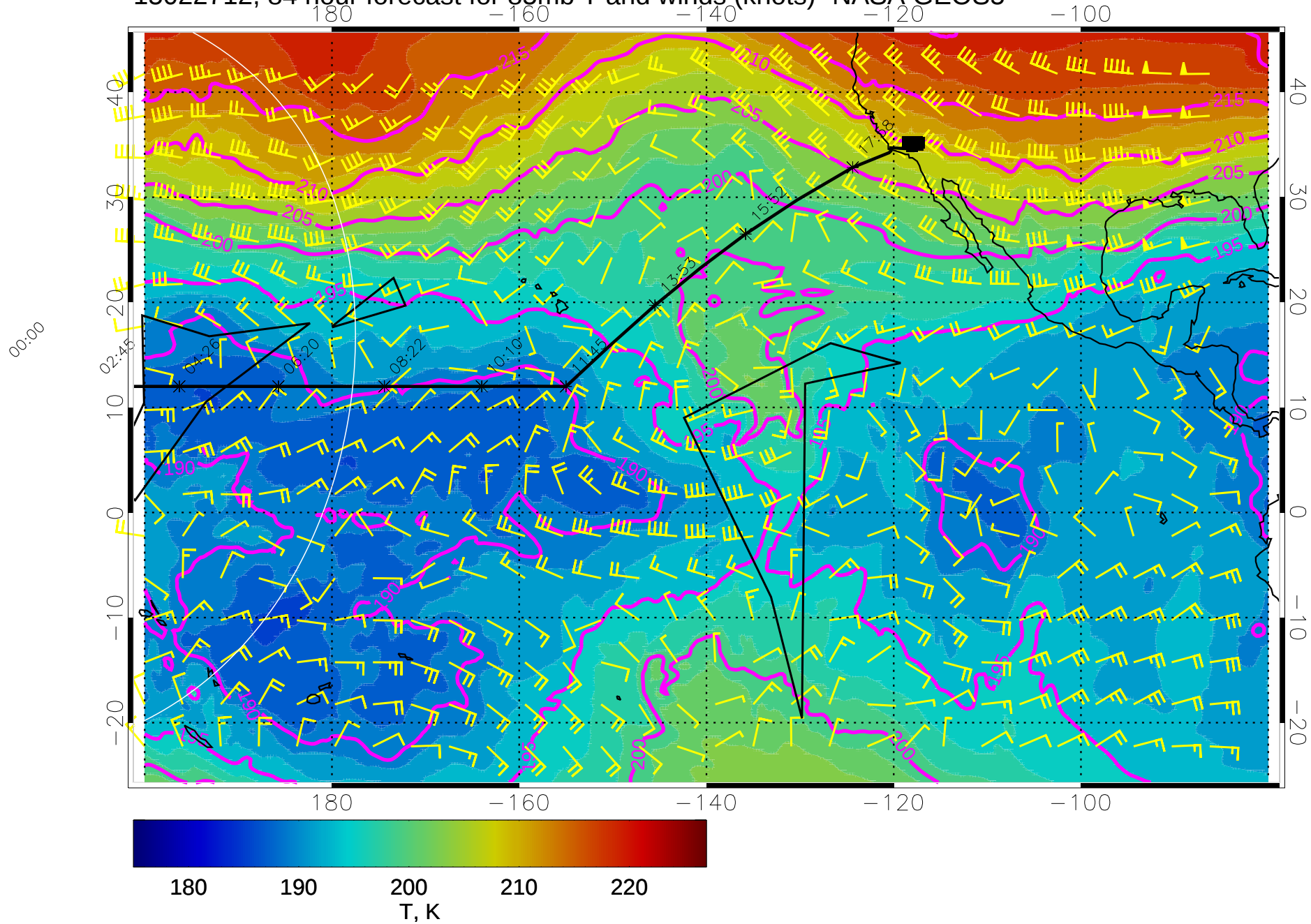
15022712, 84 hour forecast for 85mb T and winds (knots)- NASA GEOS5
