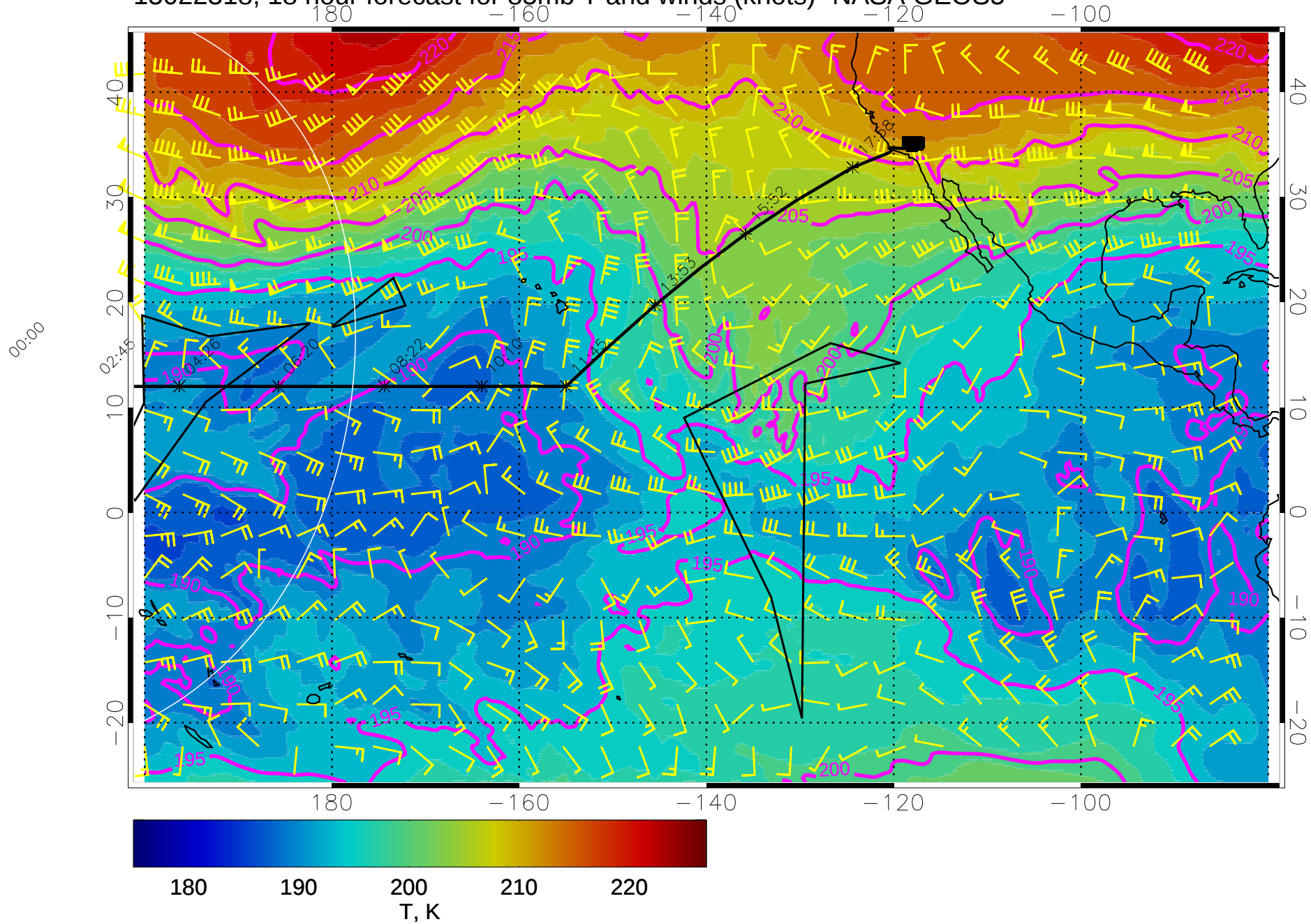
15022318, 18 hour forecast for 85mb T and winds (knots)- NASA GEOS5
