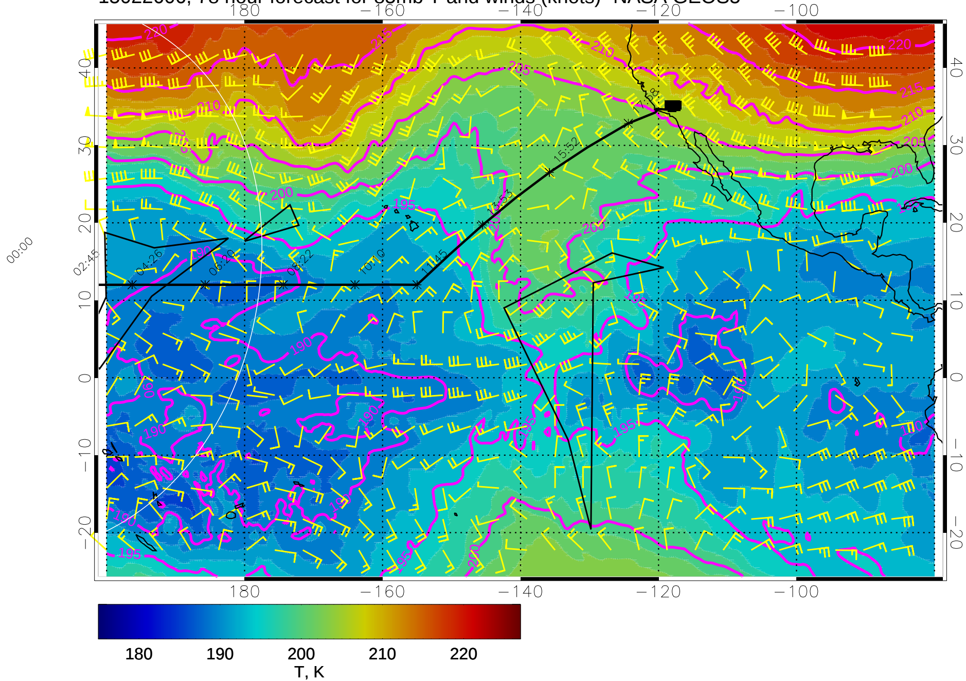
15022606, 78 hour forecast for 85mb T and winds (knots)- NASA GEOS5
