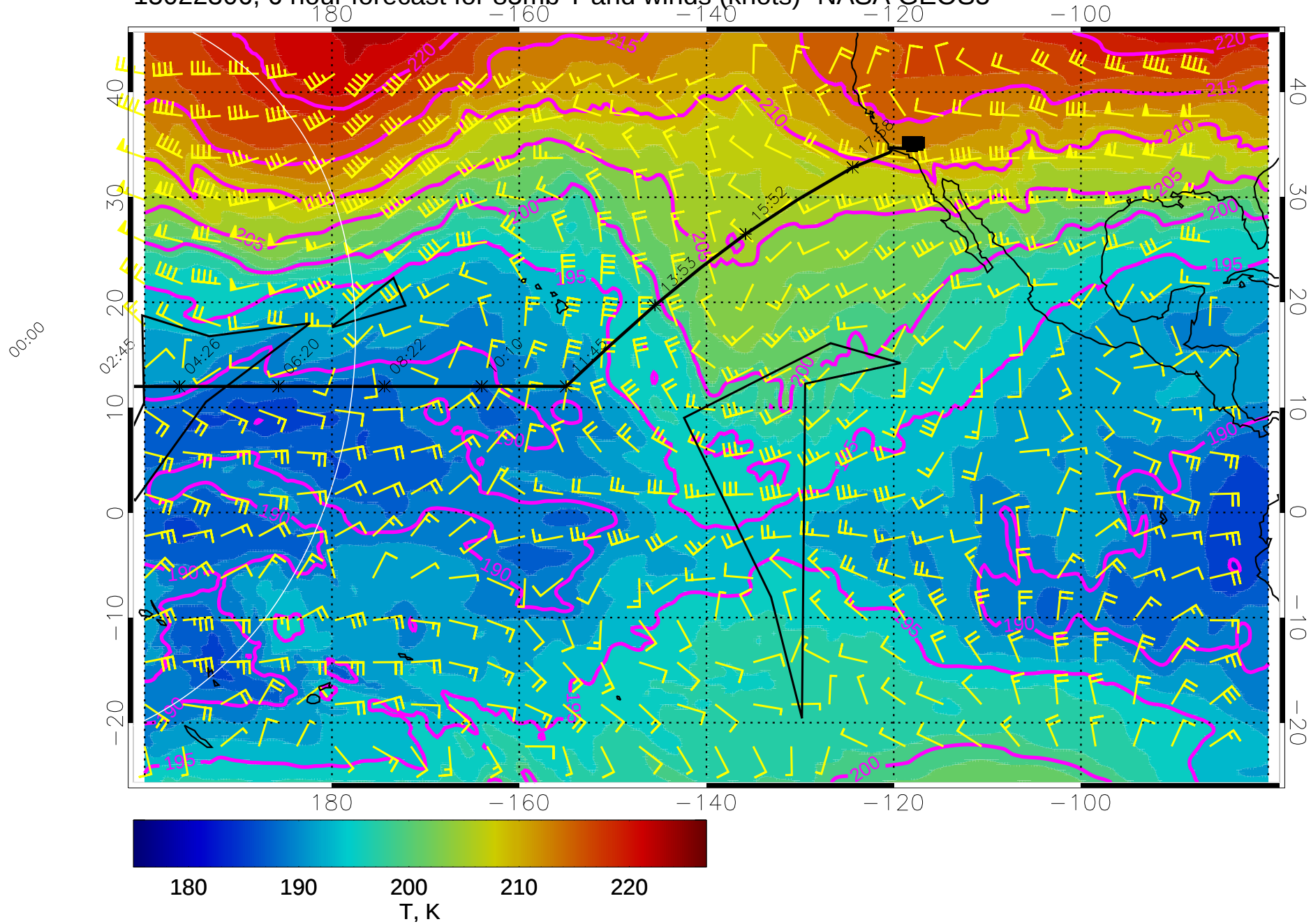
15022306, 6 hour forecast for 85mb T and winds (knots)- NASA GEOS5
