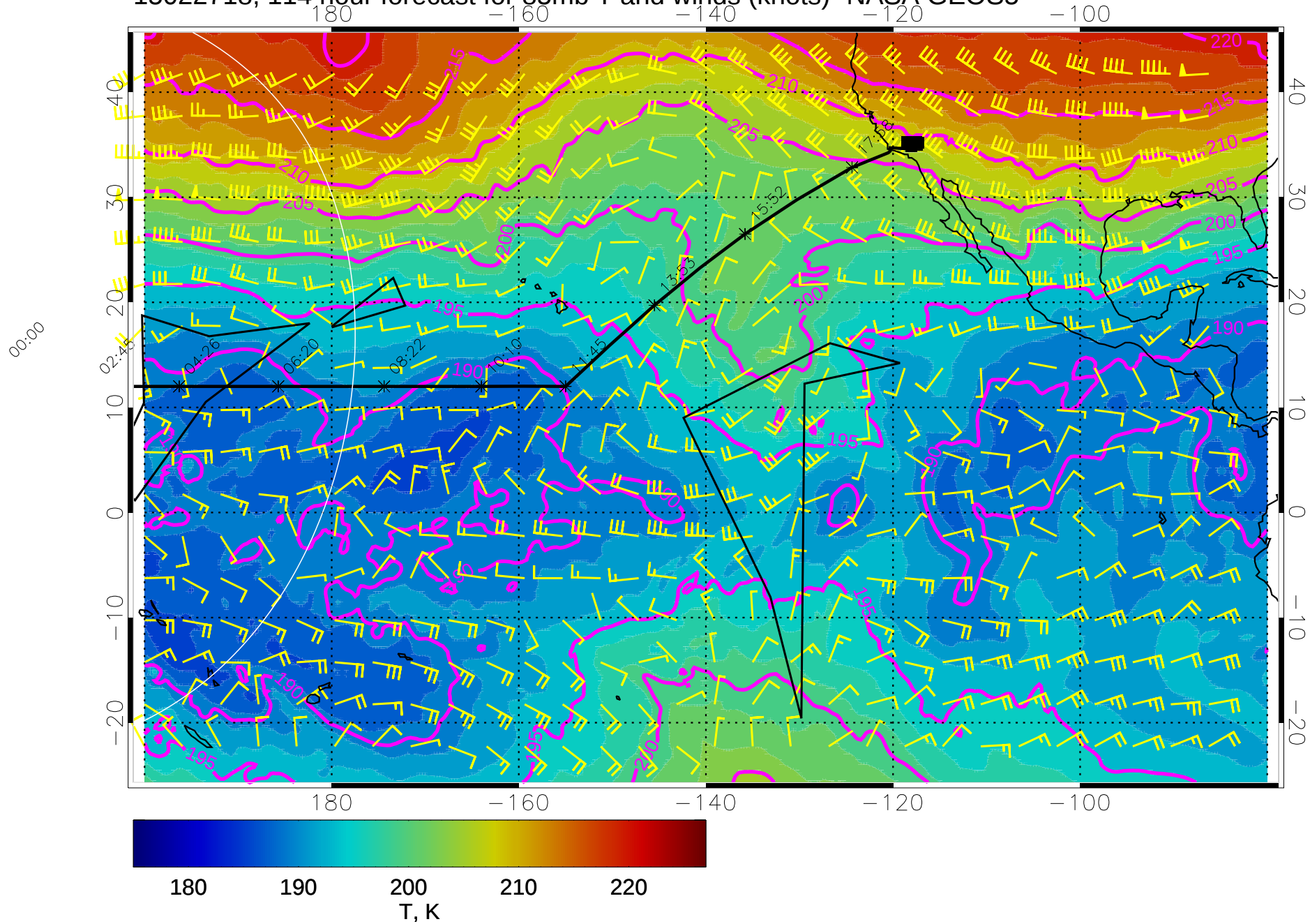
15022718, 114 hour forecast for 85mb T and winds (knots)- NASA GEOS5
