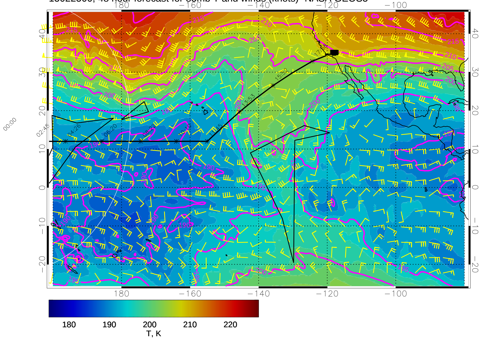
15022500, 48 hour forecast for 85mb T and winds (knots)- NASA GEOS5
