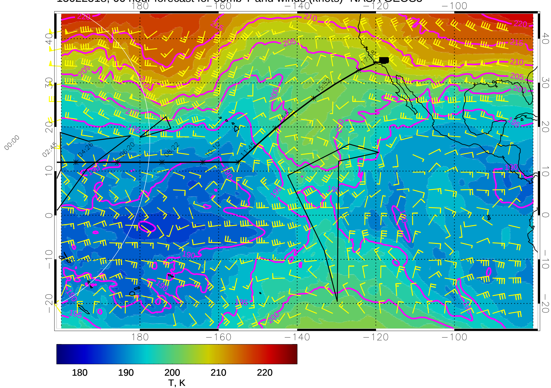
15022518, 66 hour forecast for 85mb T and winds (knots)- NASA GEOS5
