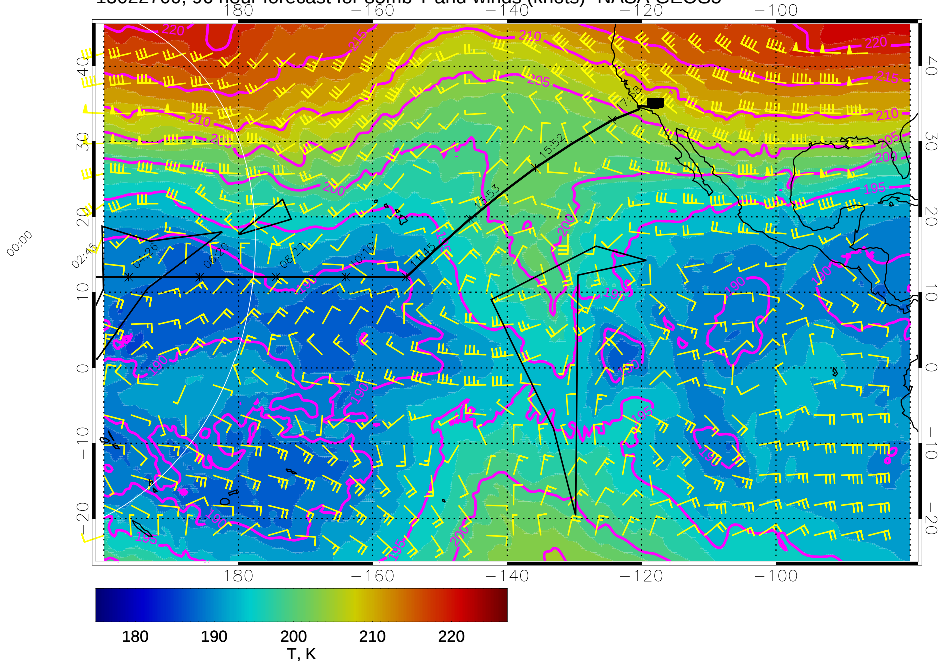
15022700, 96 hour forecast for 85mb T and winds (knots)- NASA GEOS5
