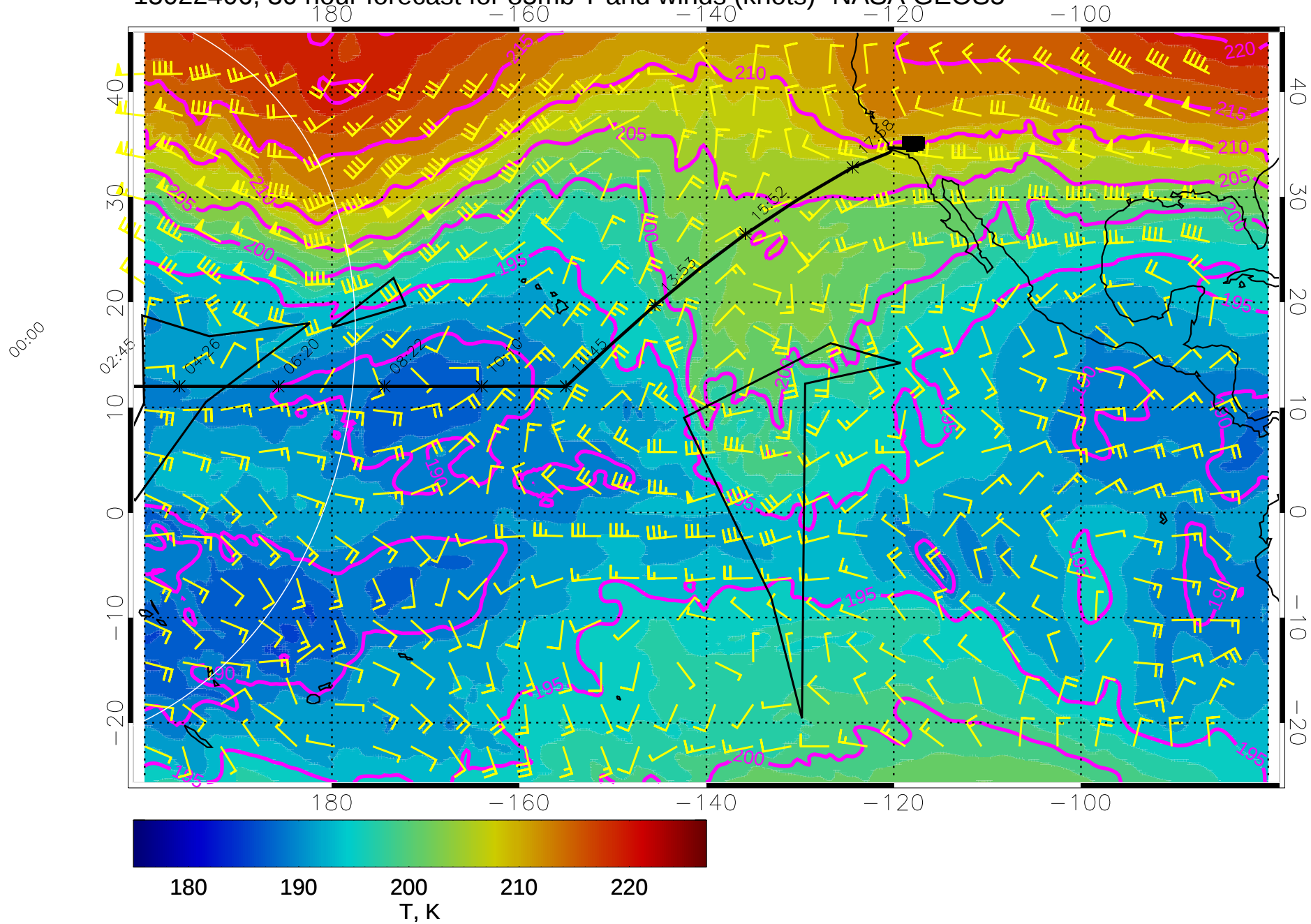
15022406, 30 hour forecast for 85mb T and winds (knots)- NASA GEOS5
