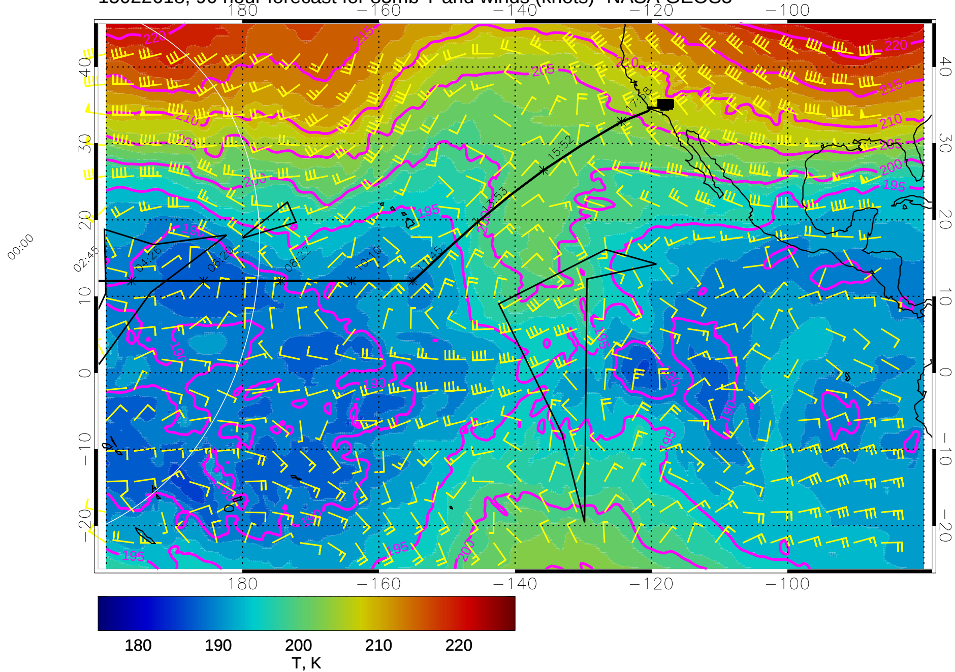
15022618, 90 hour forecast for 85mb T and winds (knots)- NASA GEOS5
