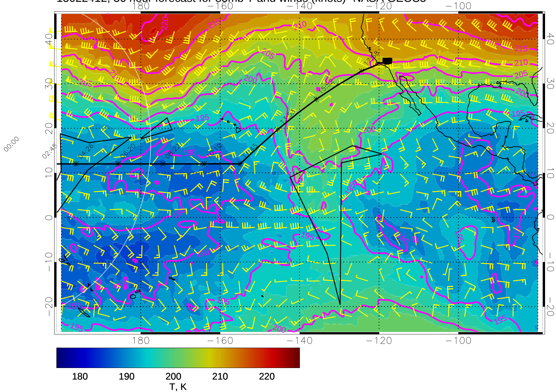
15022412, 36 hour forecast for 85mb T and winds (knots)- NASA GEOS5
