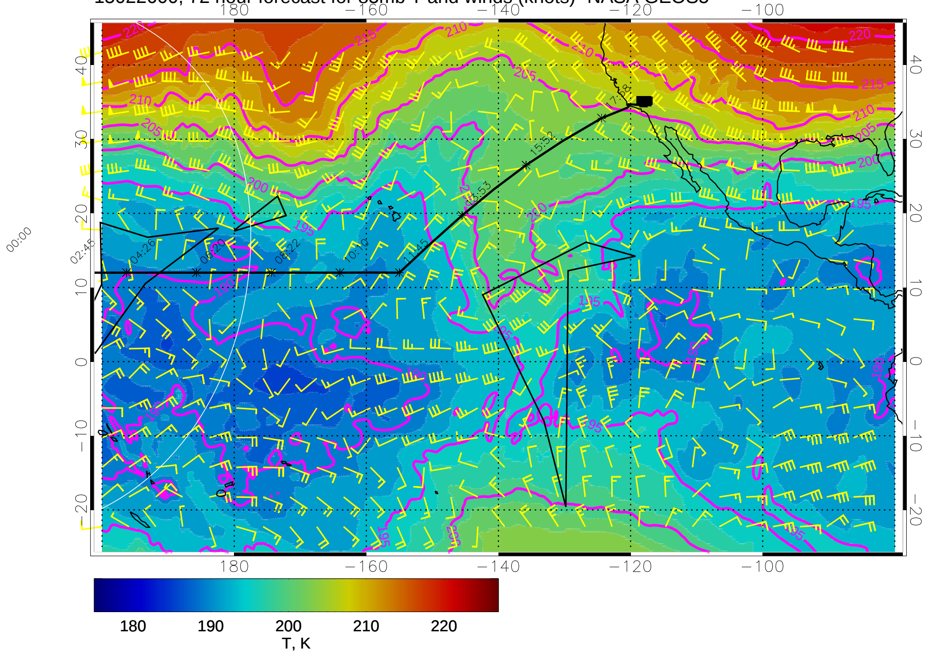
15022600, 72 hour forecast for 85mb T and winds (knots)- NASA GEOS5
