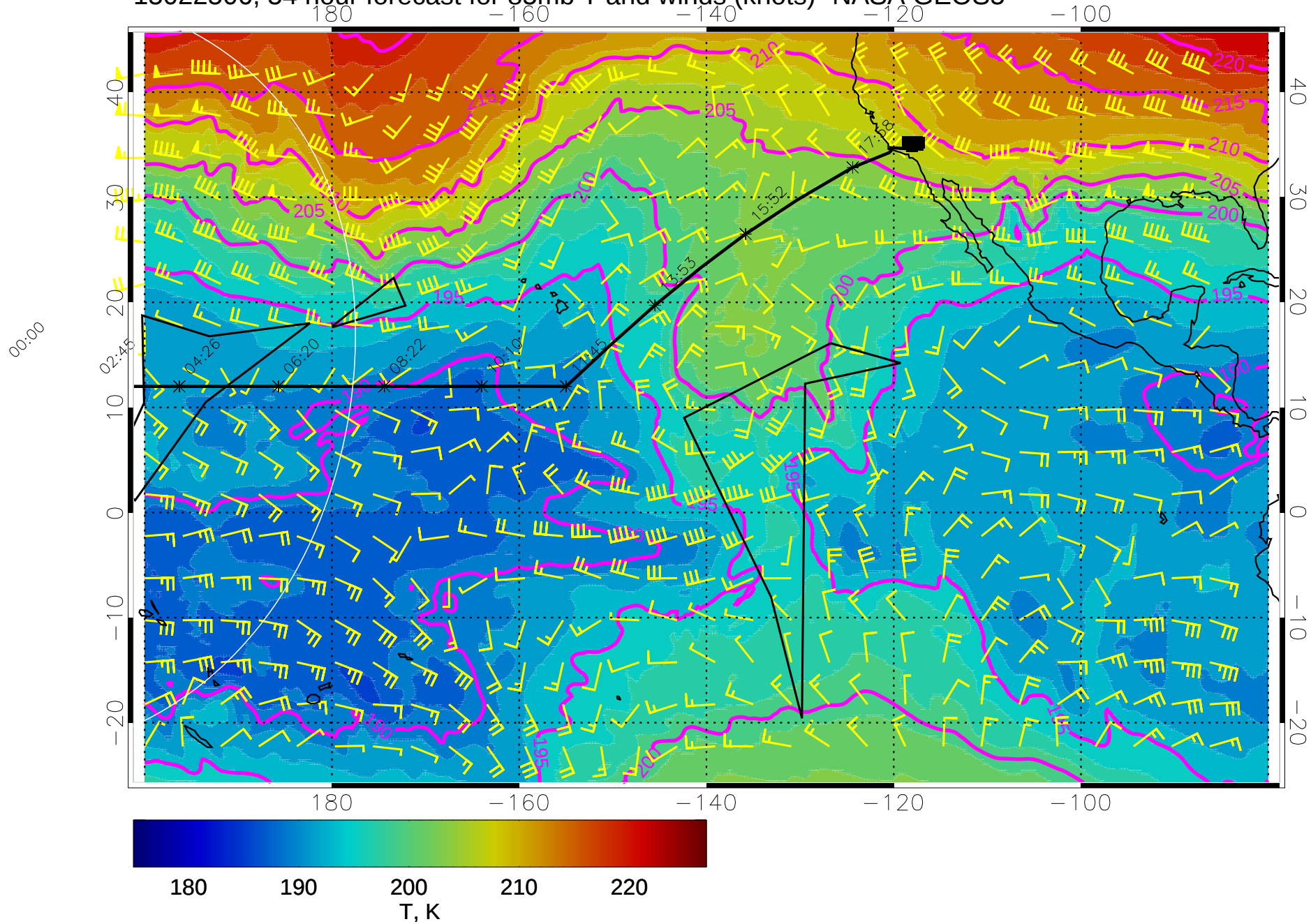
15022506, 54 hour forecast for 85mb T and winds (knots)- NASA GEOS5
