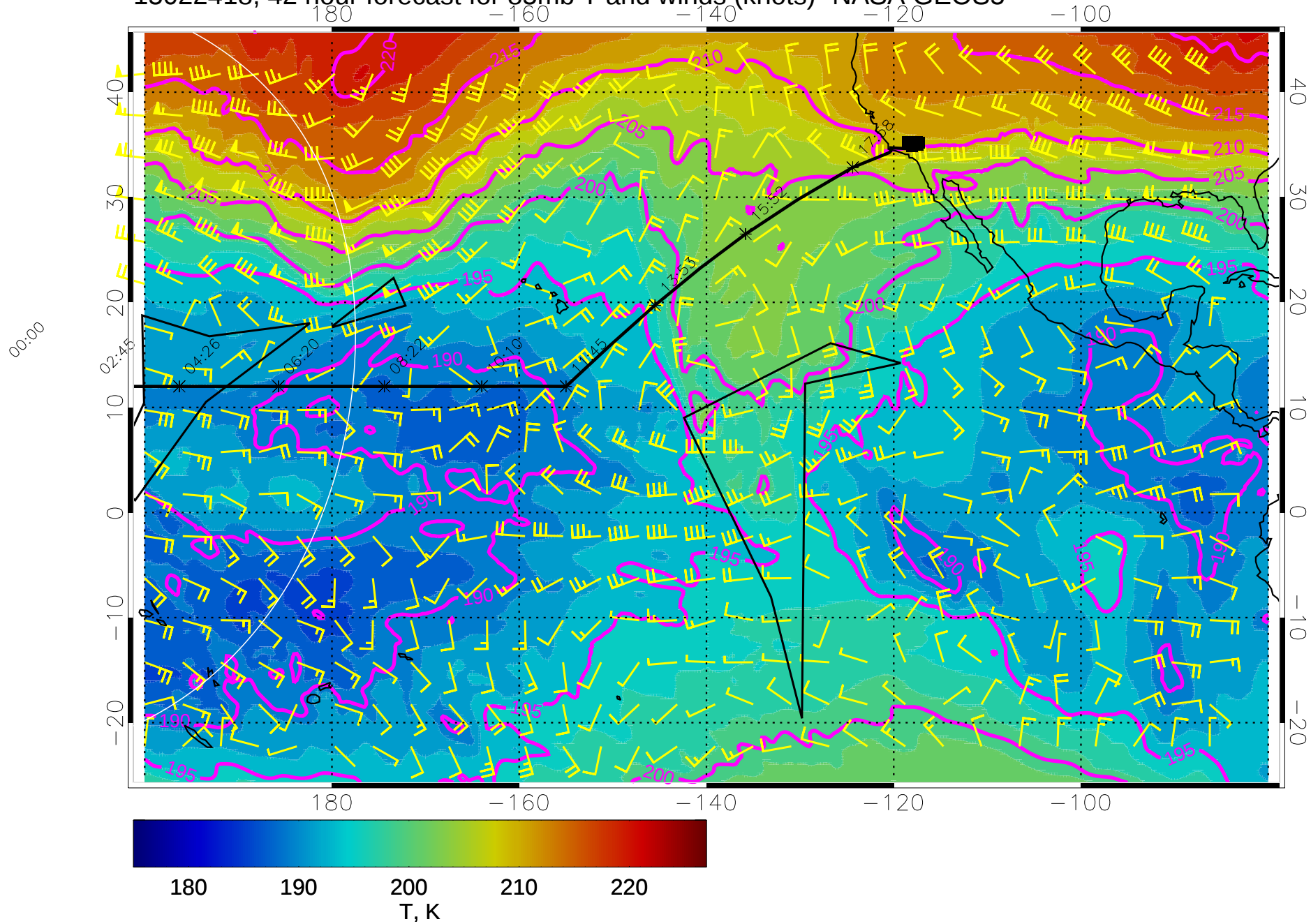
15022418, 42 hour forecast for 85mb T and winds (knots)- NASA GEOS5
