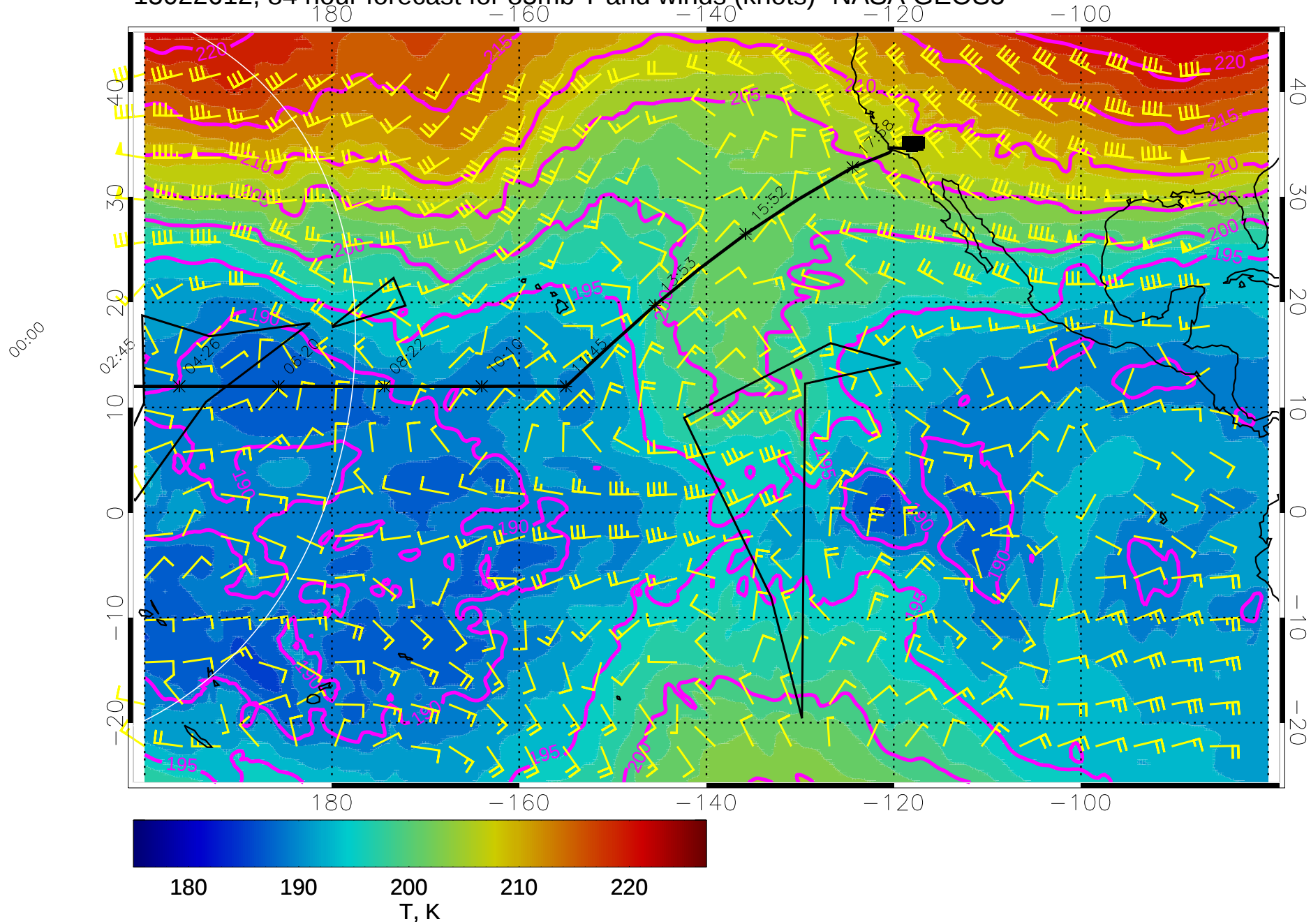
15022612, 84 hour forecast for 85mb T and winds (knots)- NASA GEOS5
