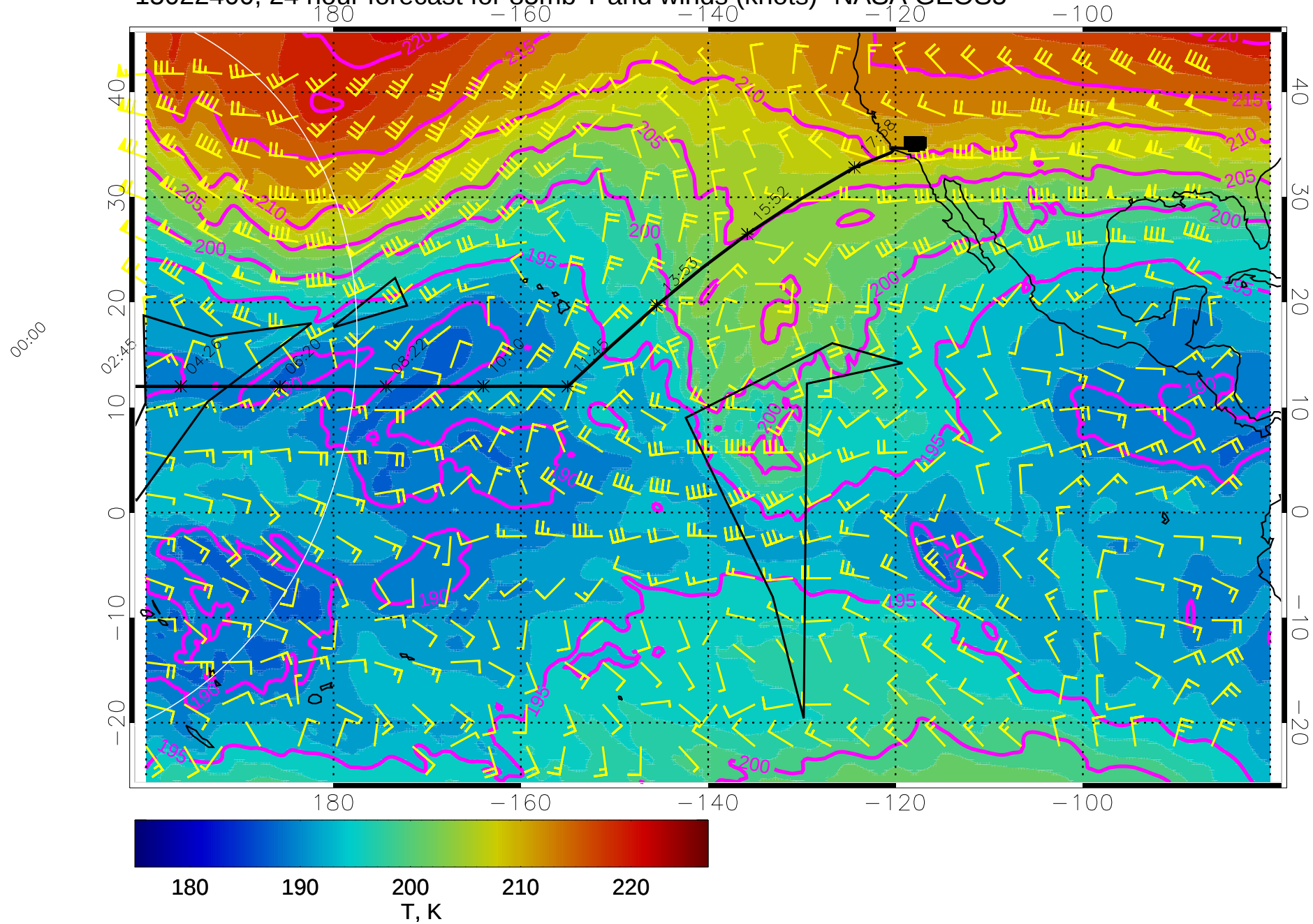
15022400, 24 hour forecast for 85mb T and winds (knots)- NASA GEOS5
