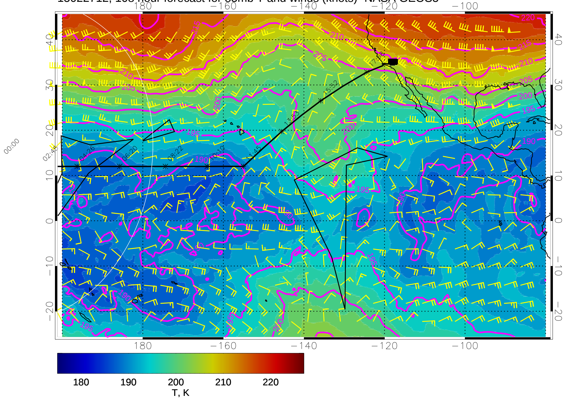
15022712, 108 hour forecast for 85mb T and winds (knots)- NASA GEOS5
