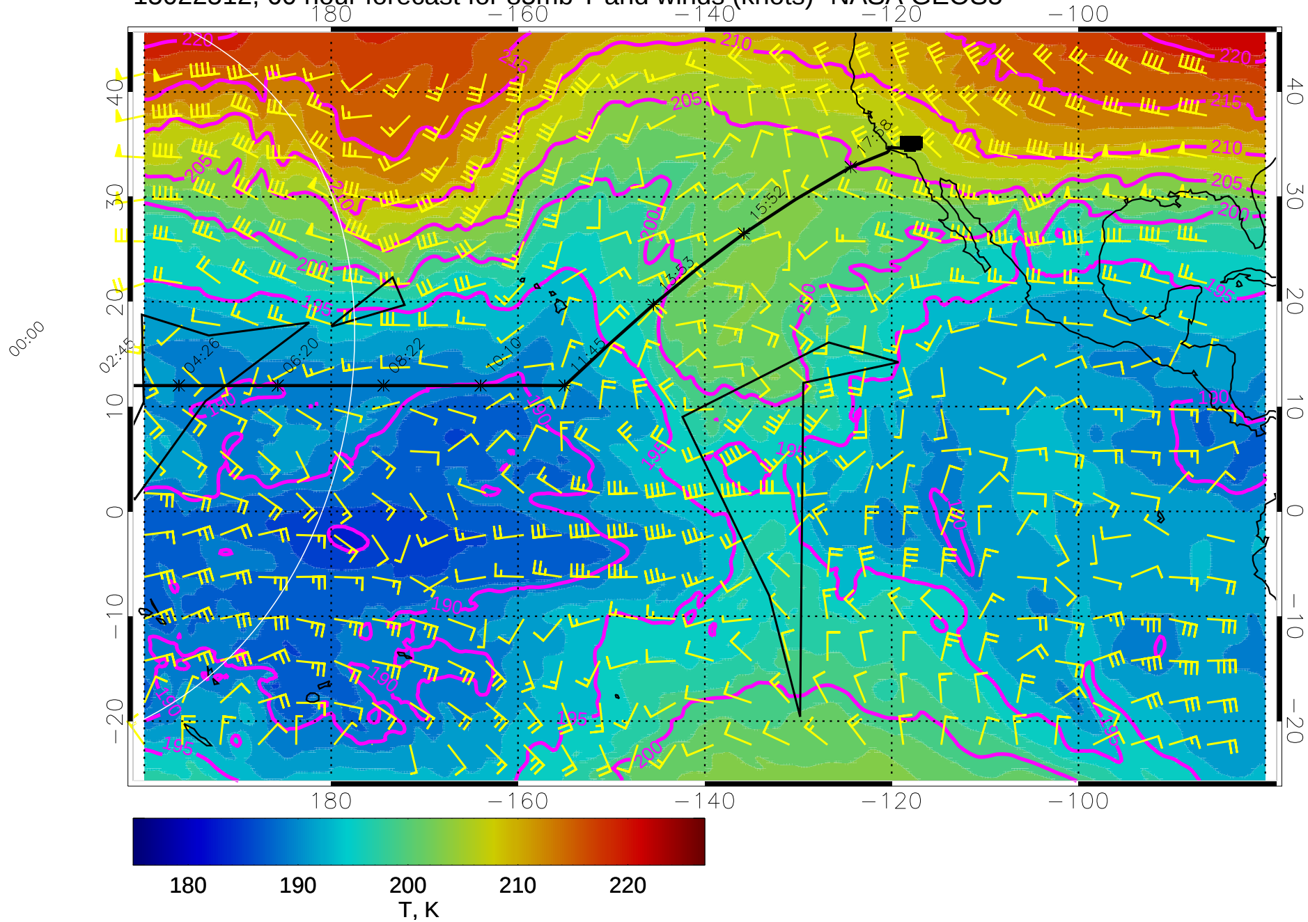
15022512, 60 hour forecast for 85mb T and winds (knots)- NASA GEOS5
