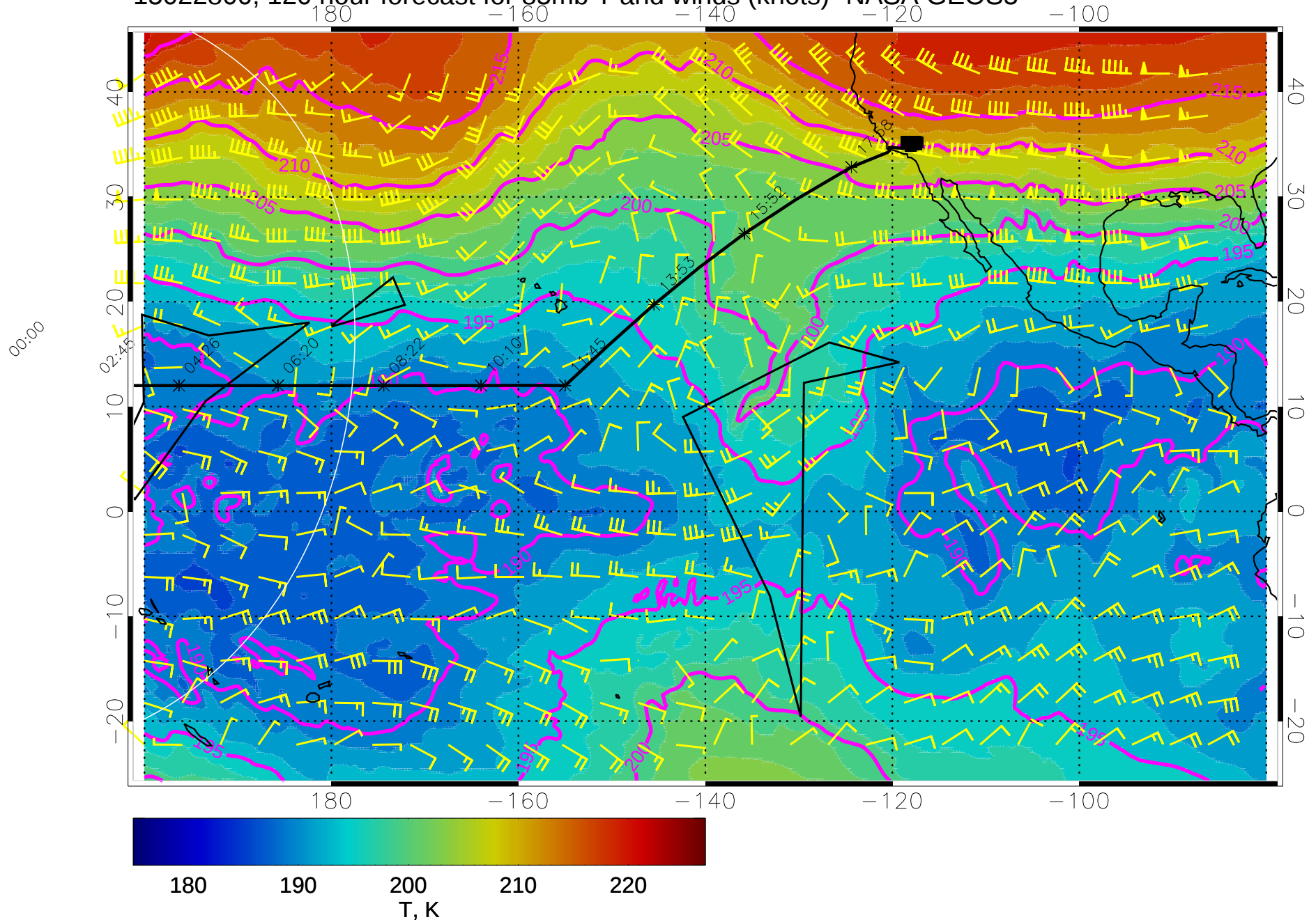
15022800, 120 hour forecast for 85mb T and winds (knots)- NASA GEOS5
