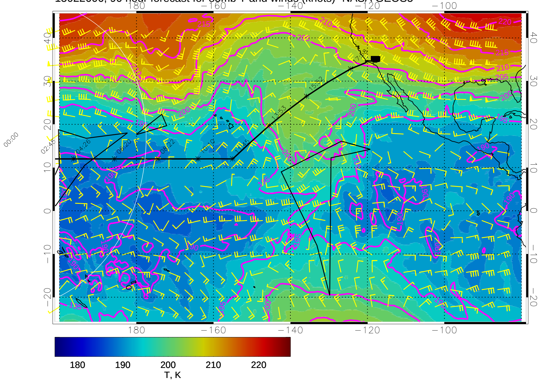
15022606, 90 hour forecast for 85mb T and winds (knots)- NASA GEOS5
