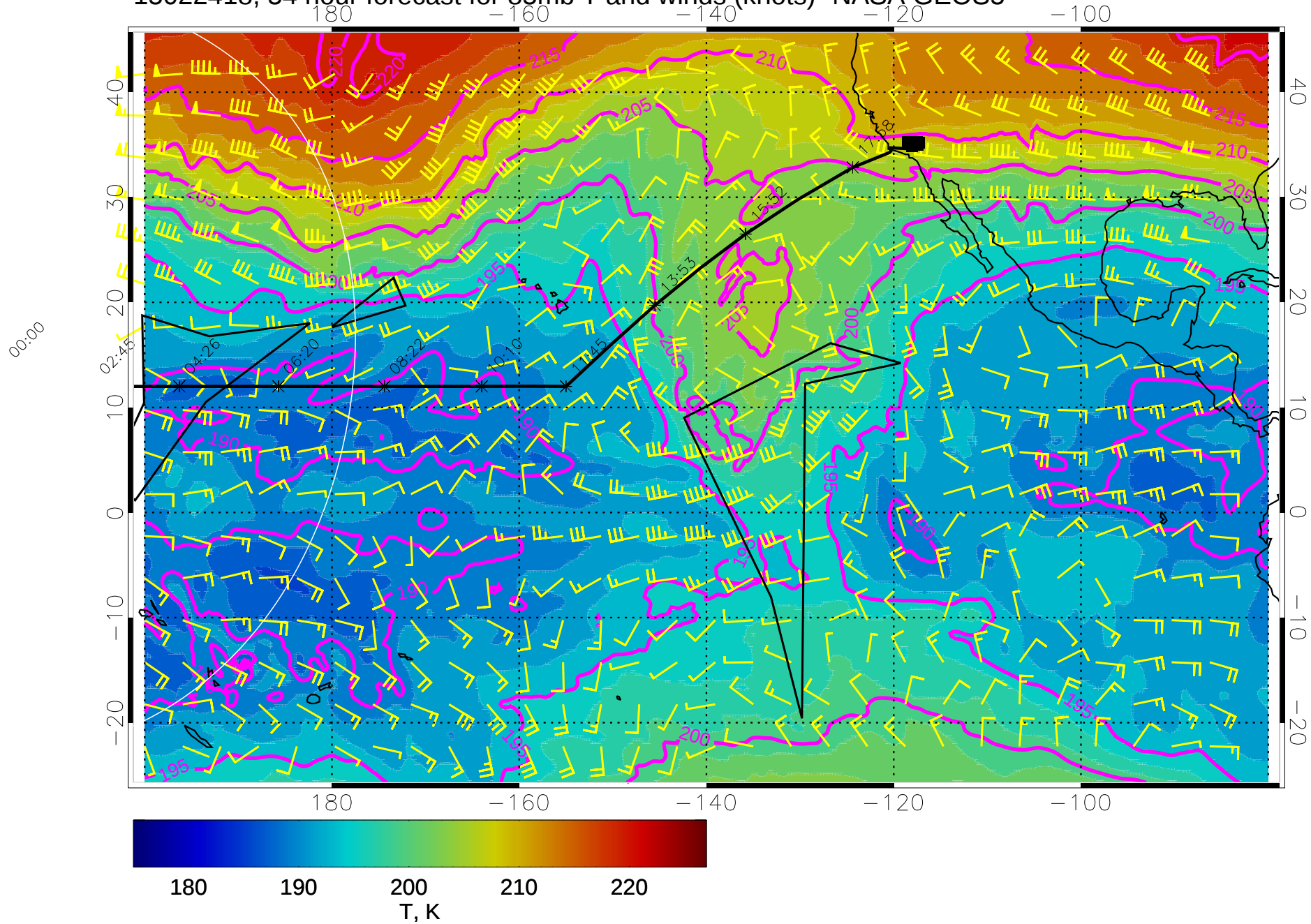
15022418, 54 hour forecast for 85mb T and winds (knots)- NASA GEOS5
