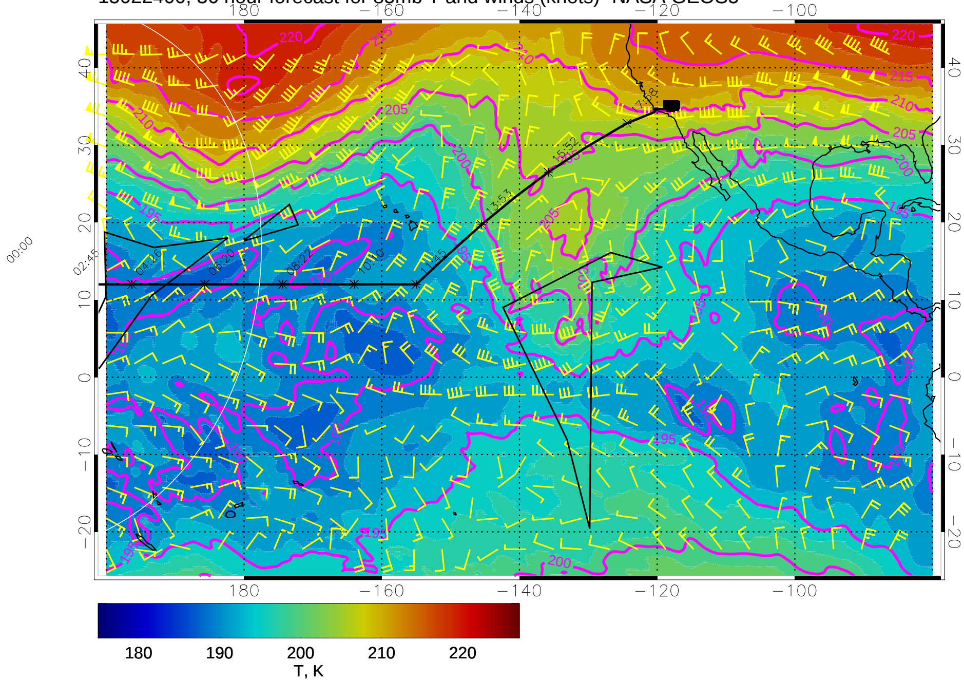
15022400, 36 hour forecast for 85mb T and winds (knots)- NASA GEOS5
