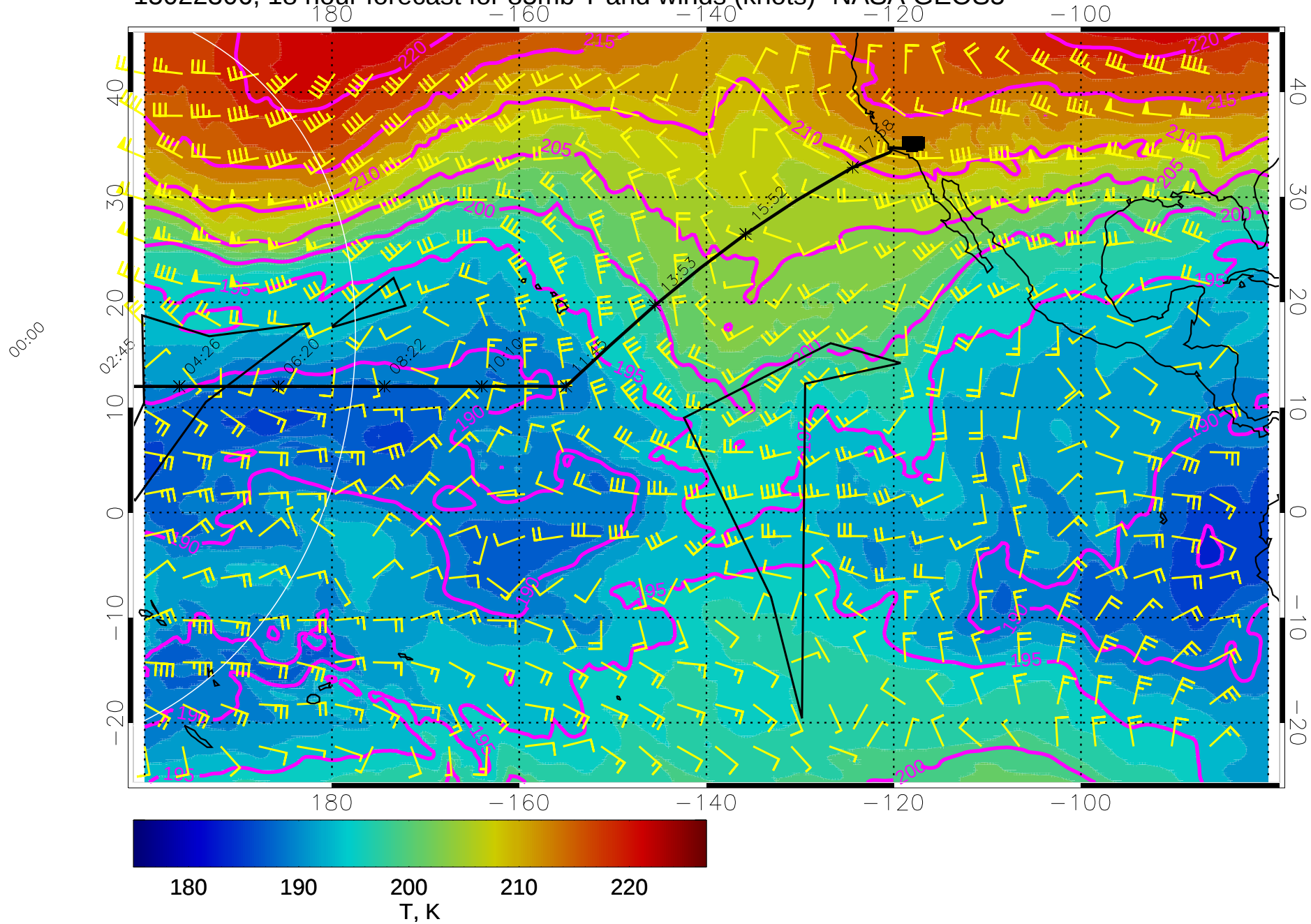
15022306, 18 hour forecast for 85mb T and winds (knots)- NASA GEOS5
