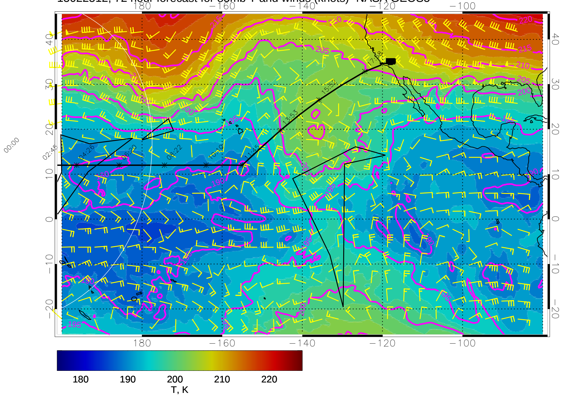
15022512, 72 hour forecast for 85mb T and winds (knots)- NASA GEOS5
