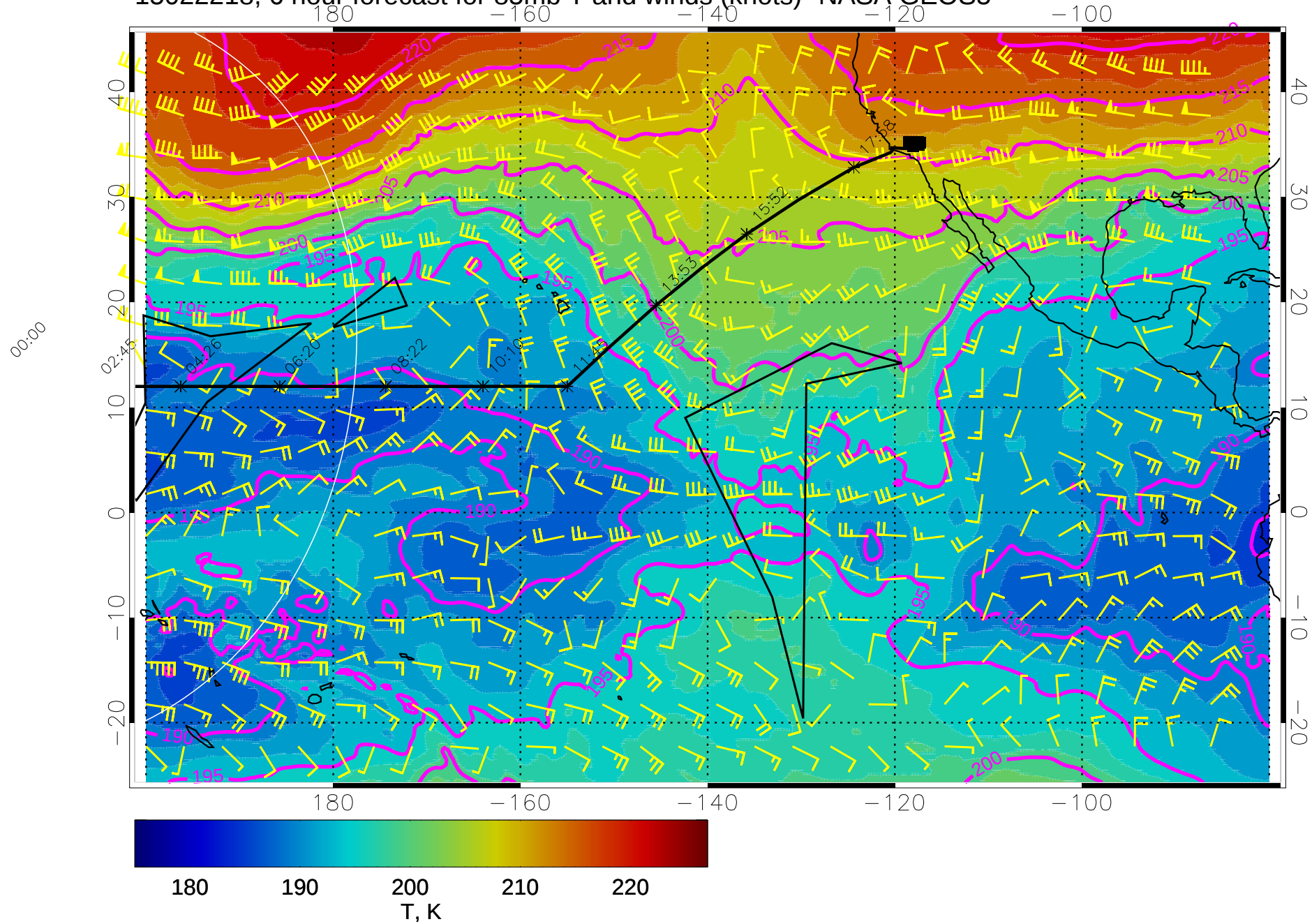
15022218, 6 hour forecast for 85mb T and winds (knots)- NASA GEOS5
