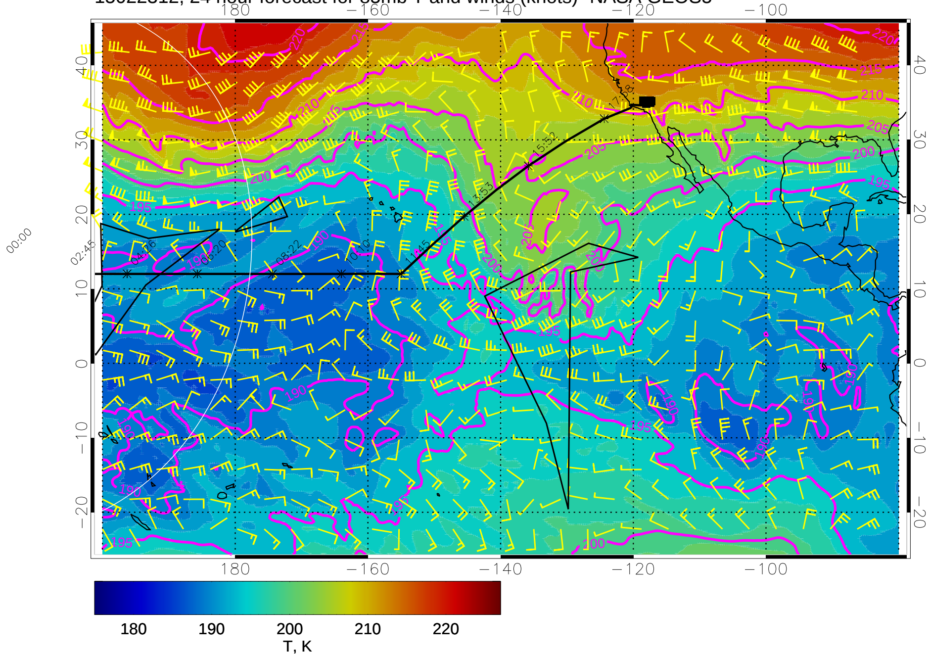
15022312, 24 hour forecast for 85mb T and winds (knots)- NASA GEOS5
