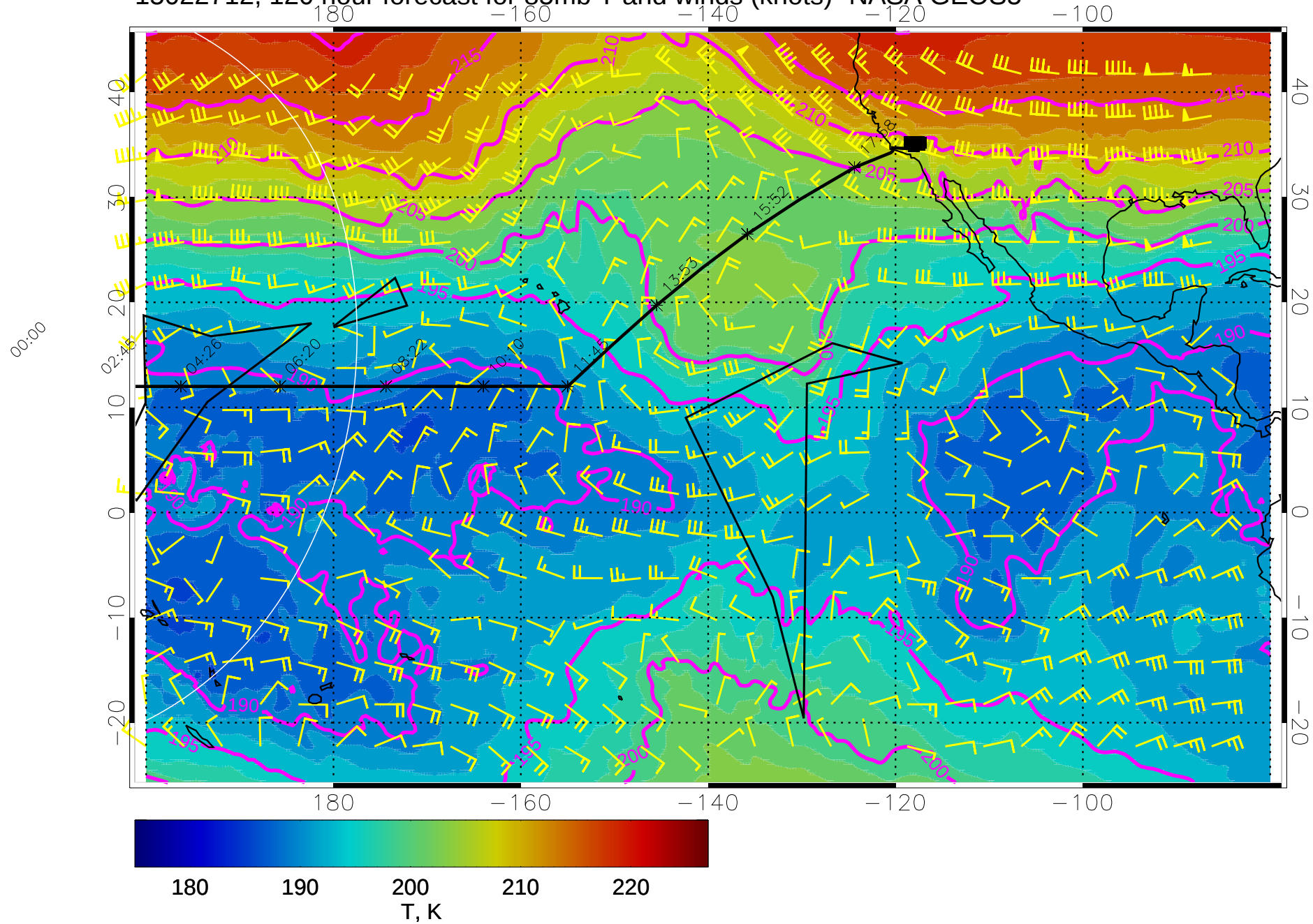
15022712, 120 hour forecast for 85mb T and winds (knots)- NASA GEOS5
