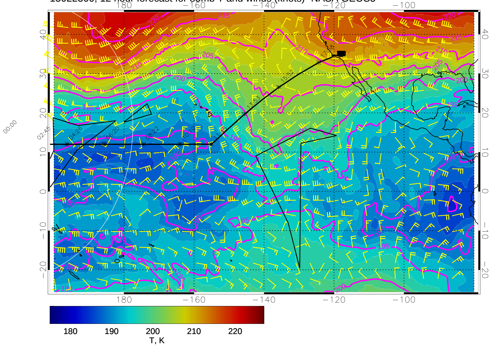
15022300, 12 hour forecast for 85mb T and winds (knots)- NASA GEOS5
