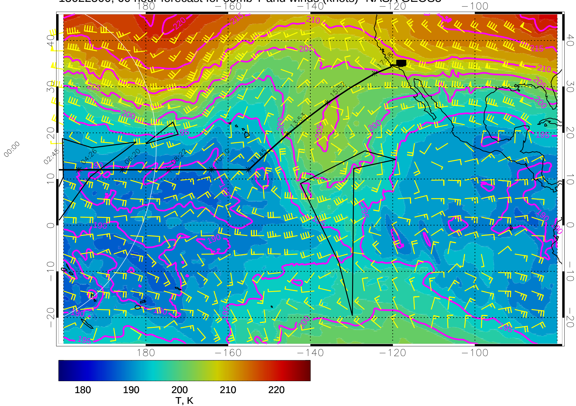
15022500, 60 hour forecast for 85mb T and winds (knots)- NASA GEOS5
