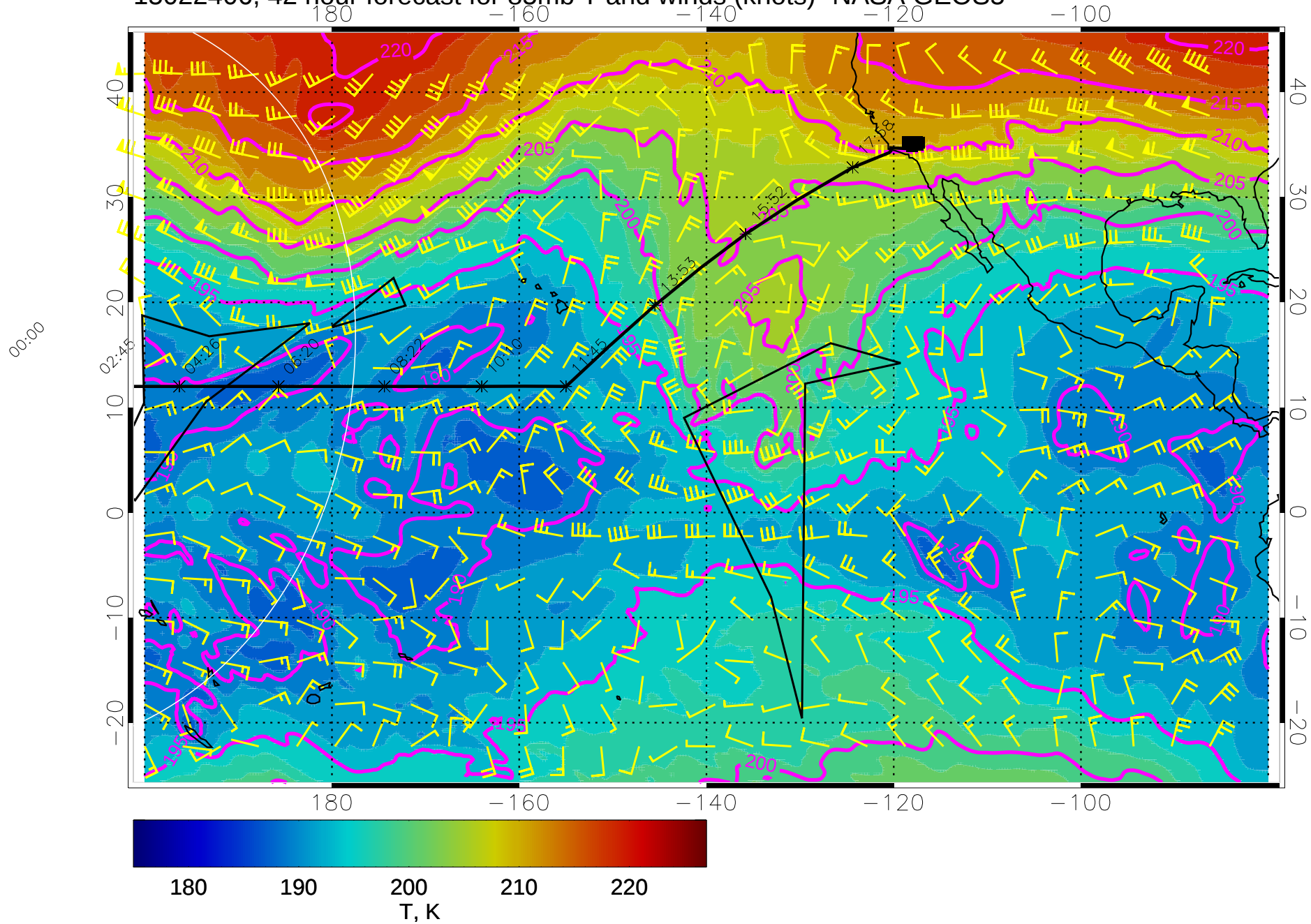
15022406, 42 hour forecast for 85mb T and winds (knots)- NASA GEOS5
