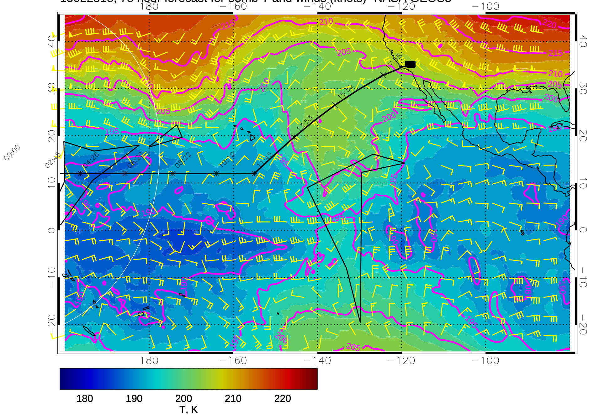
15022518, 78 hour forecast for 85mb T and winds (knots)- NASA GEOS5
