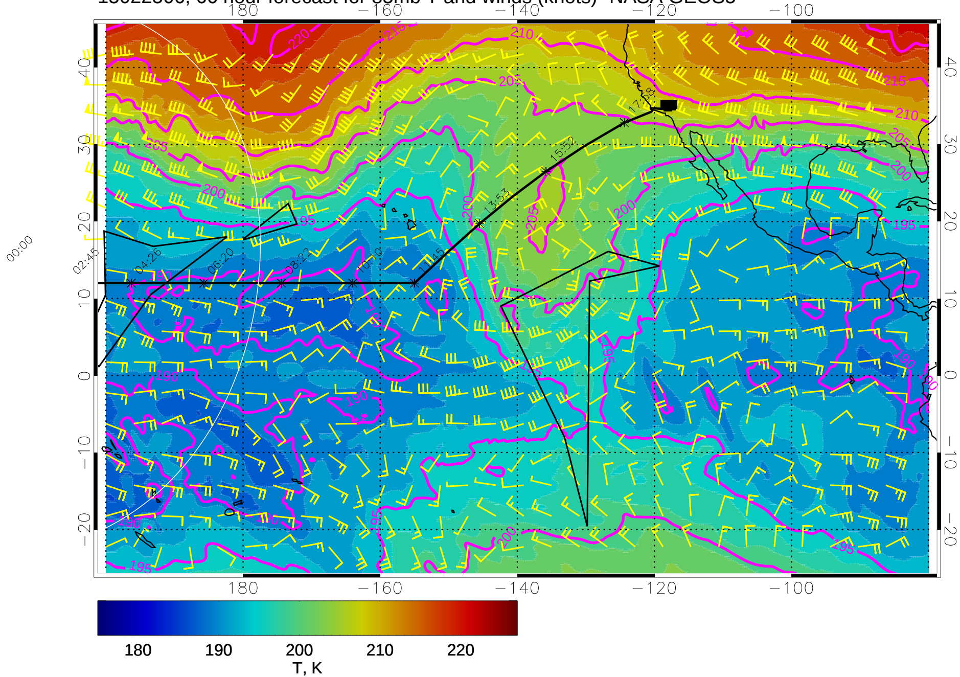
15022506, 66 hour forecast for 85mb T and winds (knots)- NASA GEOS5
