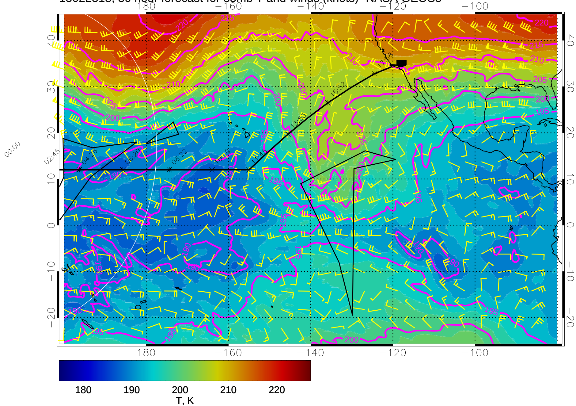
15022318, 30 hour forecast for 85mb T and winds (knots)- NASA GEOS5
