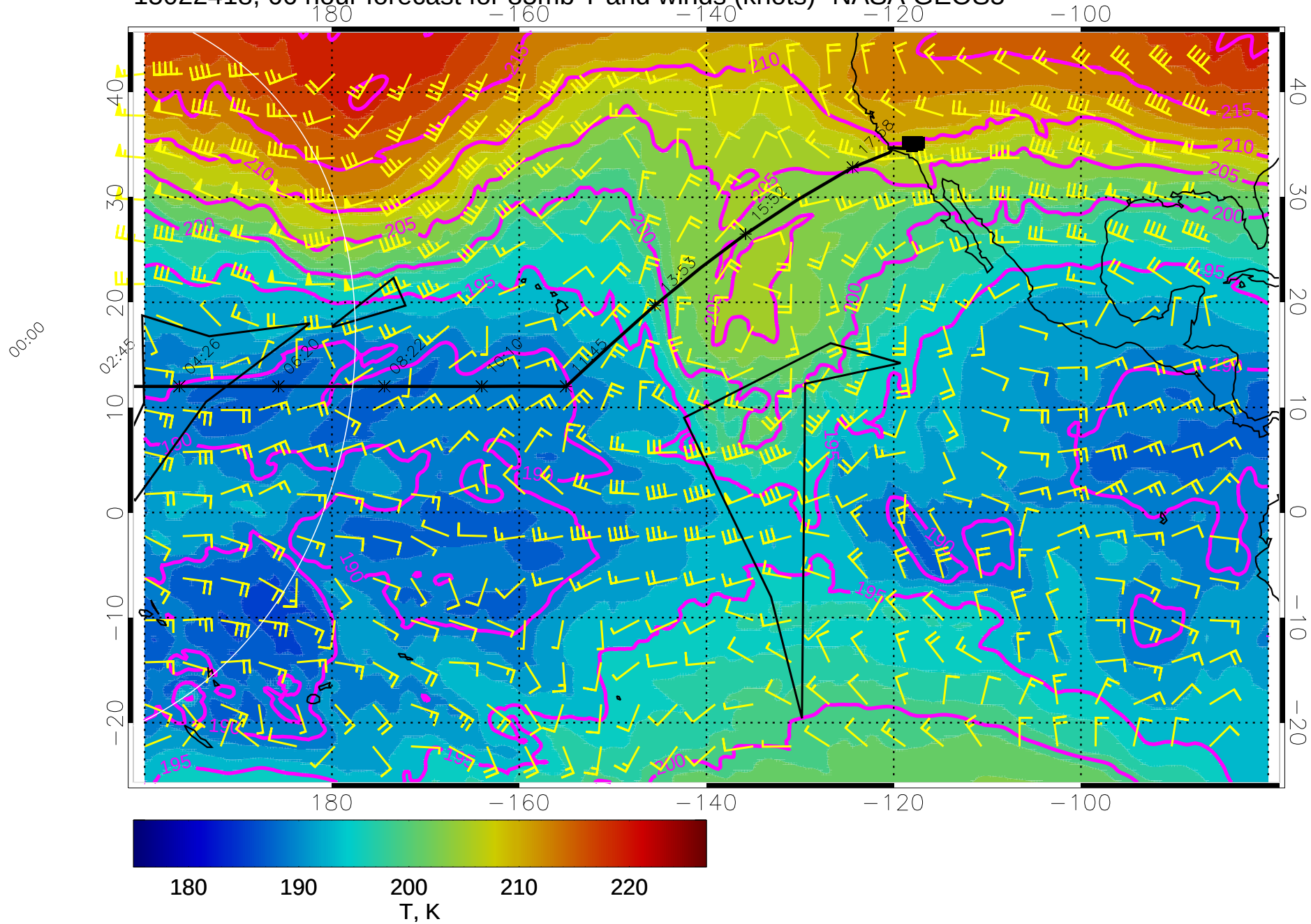
15022418, 66 hour forecast for 85mb T and winds (knots)- NASA GEOS5
