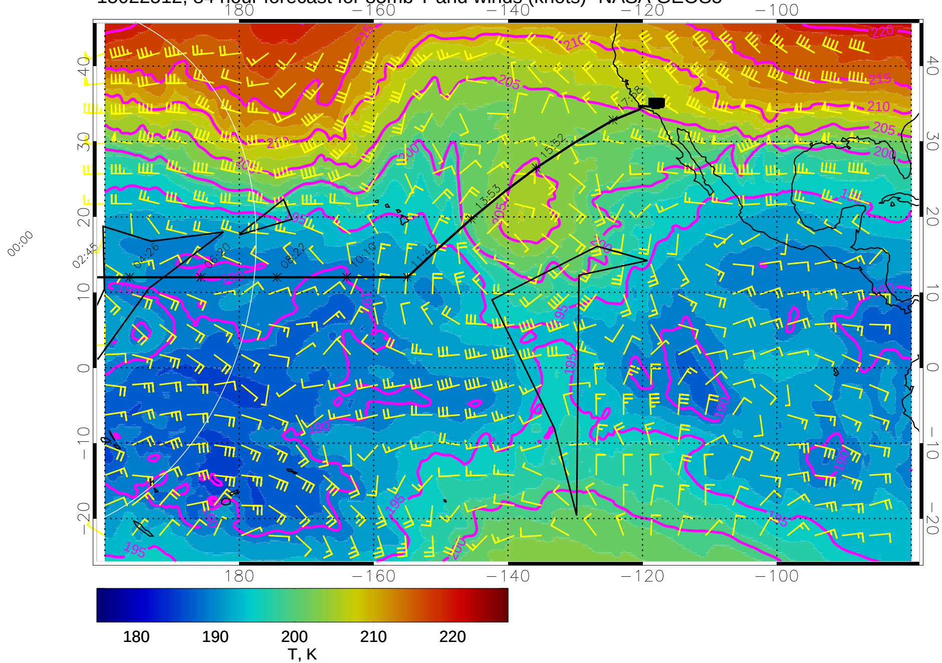
15022512, 84 hour forecast for 85mb T and winds (knots)- NASA GEOS5
