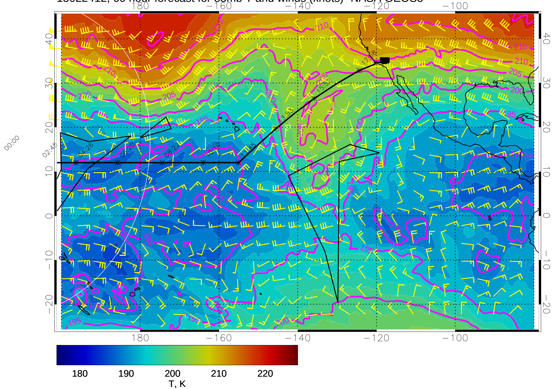
15022412, 60 hour forecast for 85mb T and winds (knots)- NASA GEOS5
