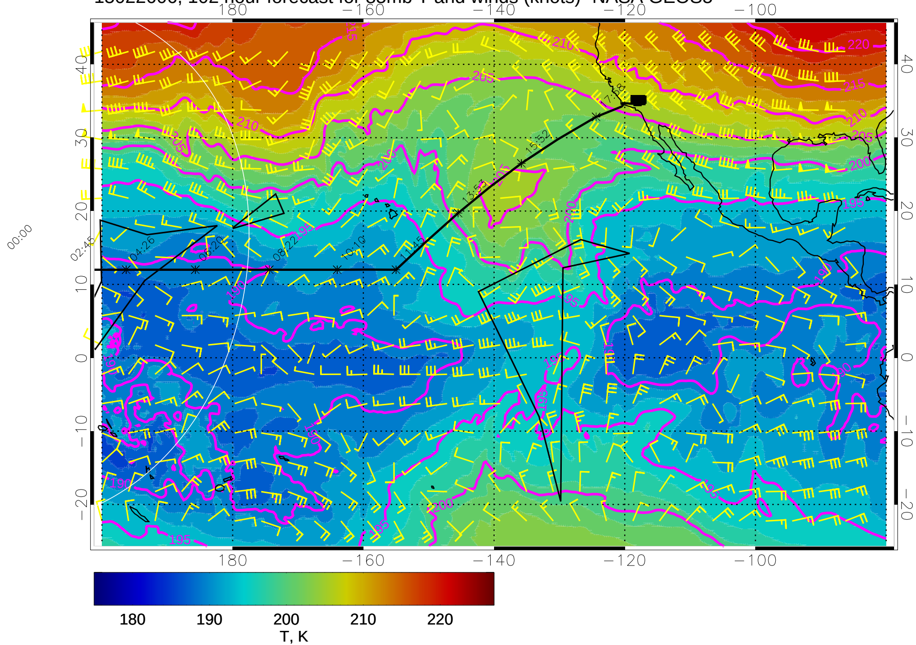
15022606, 102 hour forecast for 85mb T and winds (knots)- NASA GEOS5
