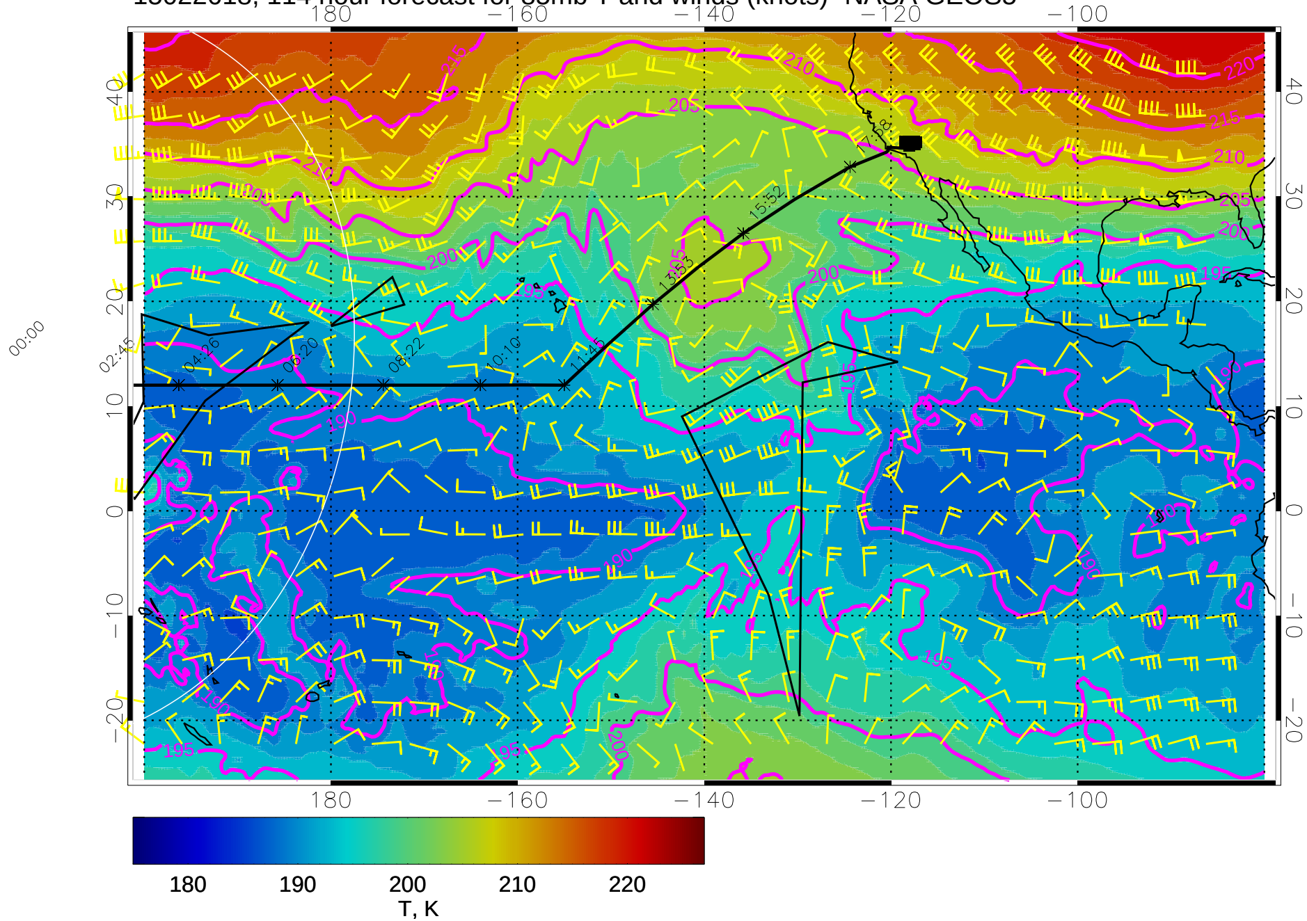
15022618, 114 hour forecast for 85mb T and winds (knots)- NASA GEOS5
