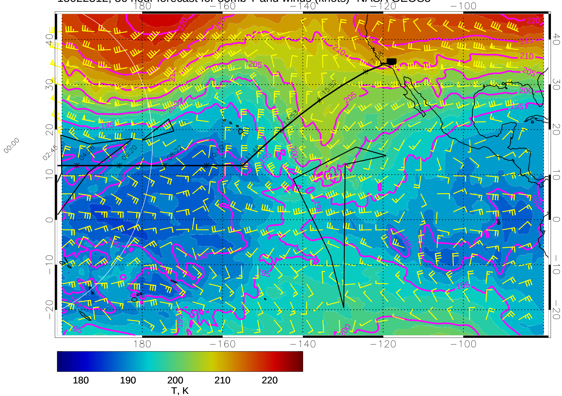
15022312, 36 hour forecast for 85mb T and winds (knots)- NASA GEOS5
