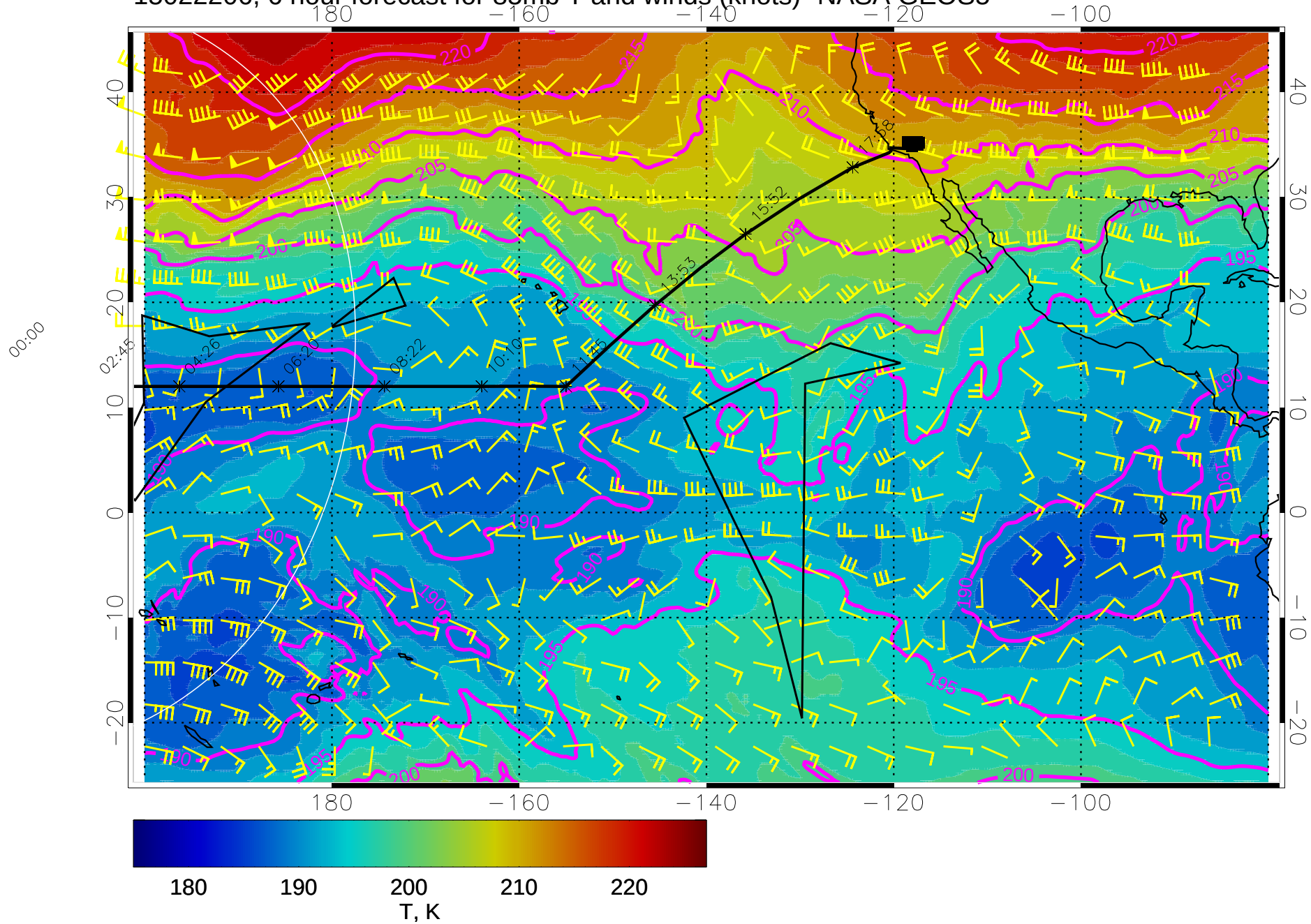
15022206, 6 hour forecast for 85mb T and winds (knots)- NASA GEOS5
