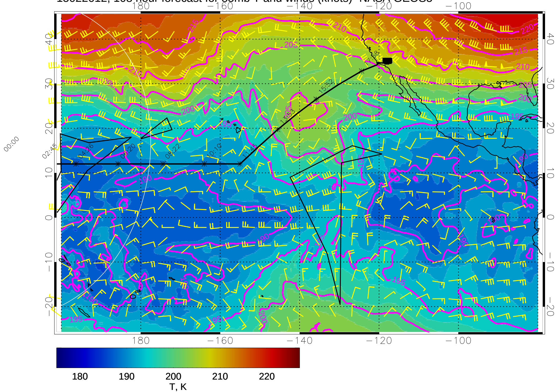
15022612, 108 hour forecast for 85mb T and winds (knots)- NASA GEOS5
