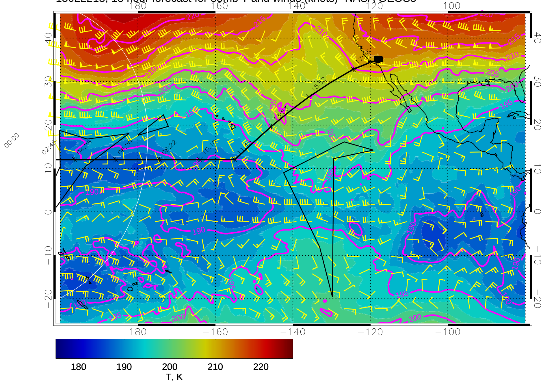
15022218, 18 hour forecast for 85mb T and winds (knots)- NASA GEOS5
