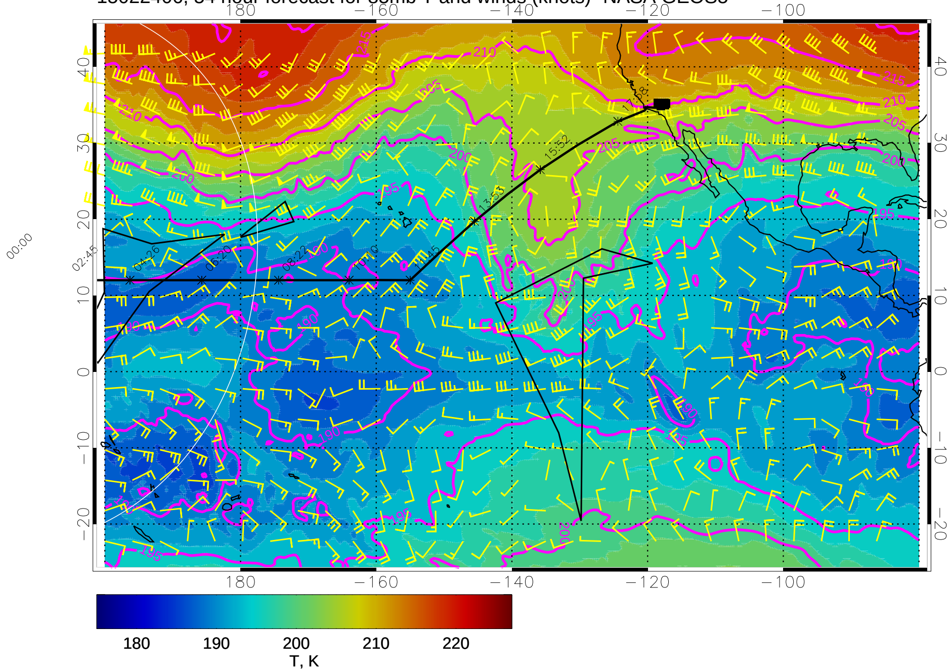
15022406, 54 hour forecast for 85mb T and winds (knots)- NASA GEOS5
