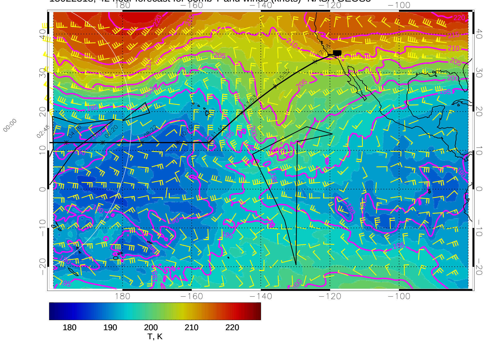
15022318, 42 hour forecast for 85mb T and winds (knots)- NASA GEOS5
