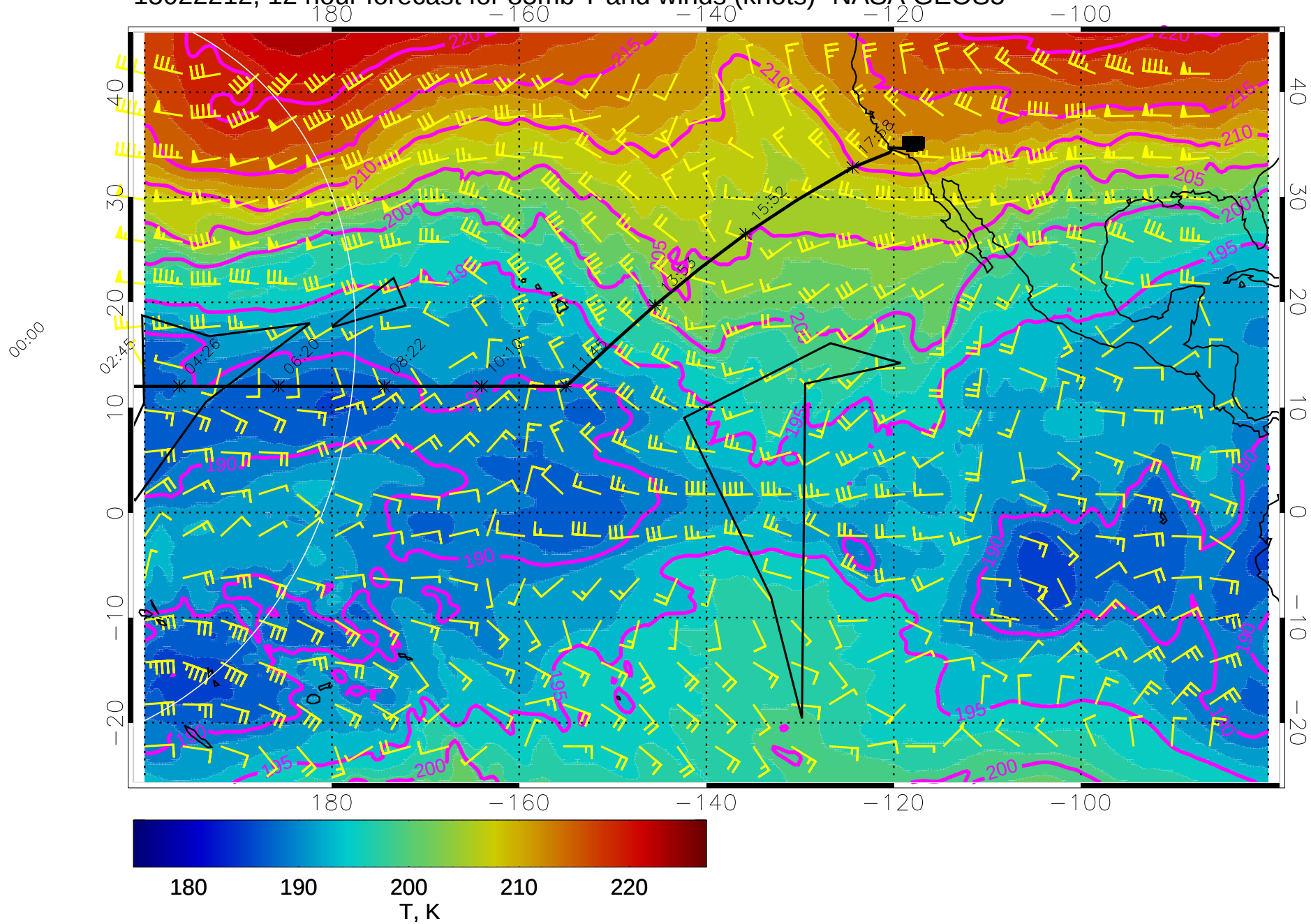
15022212, 12 hour forecast for 85mb T and winds (knots)- NASA GEOS5
