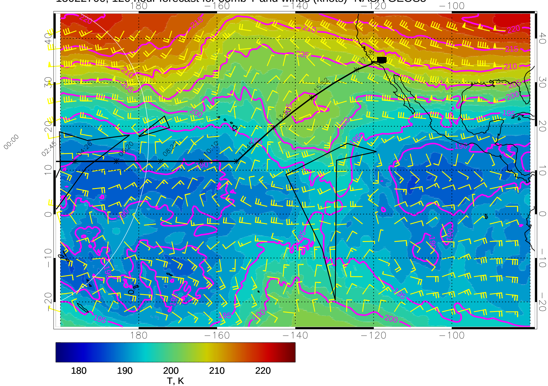
15022700, 120 hour forecast for 85mb T and winds (knots)- NASA GEOS5
