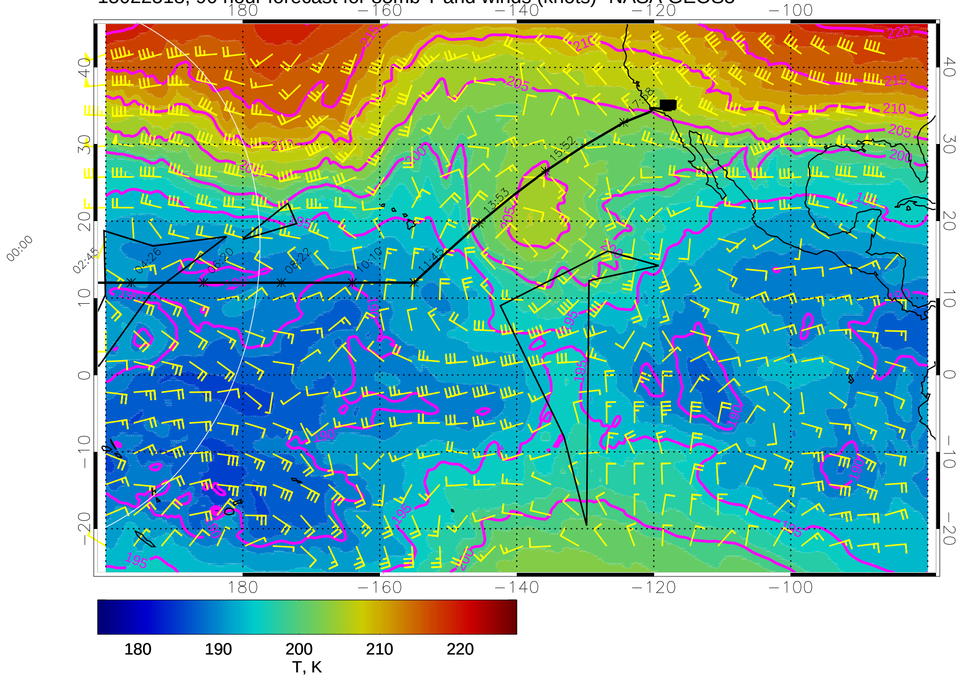
15022518, 90 hour forecast for 85mb T and winds (knots)- NASA GEOS5
