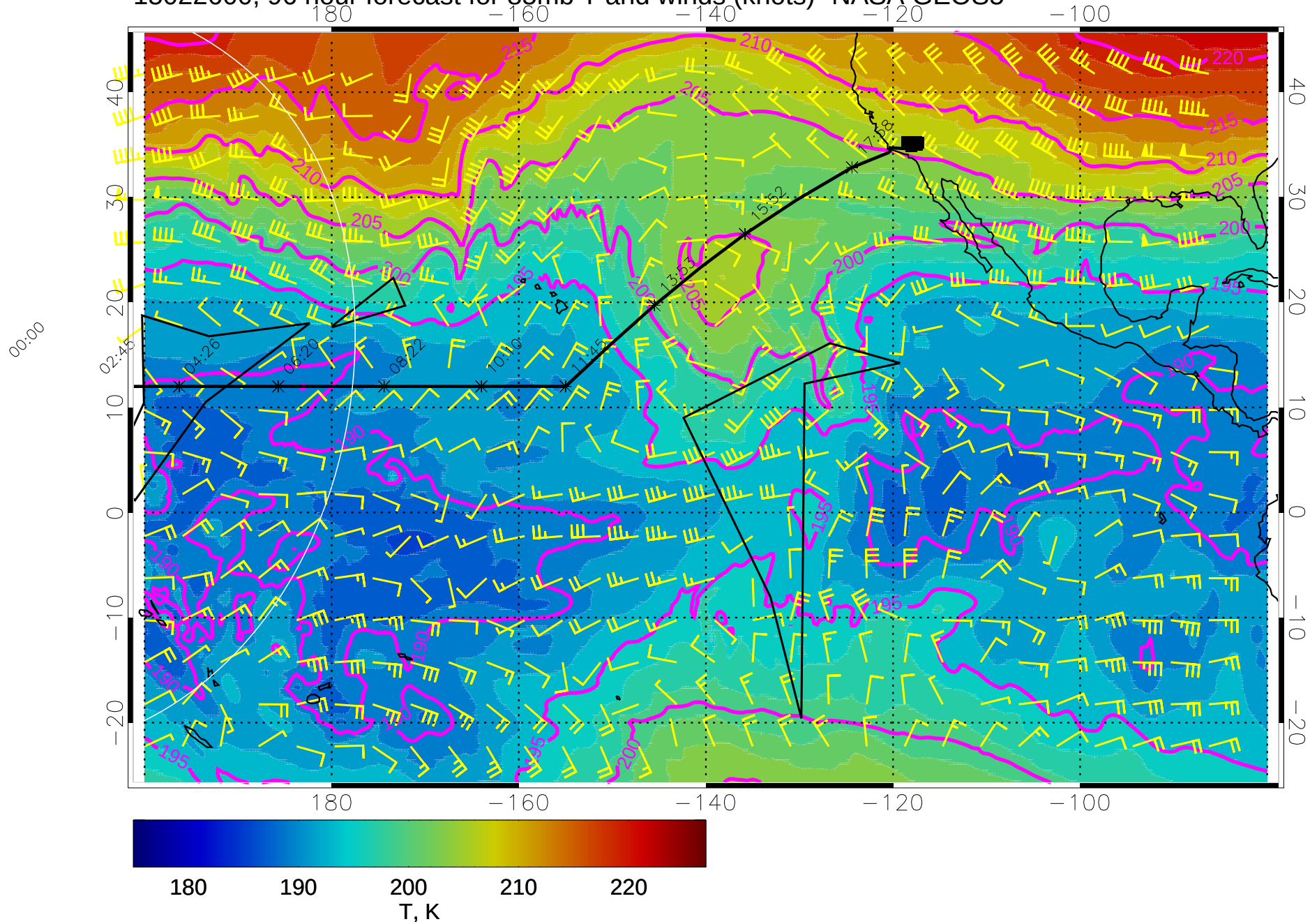
15022600, 96 hour forecast for 85mb T and winds (knots)- NASA GEOS5
