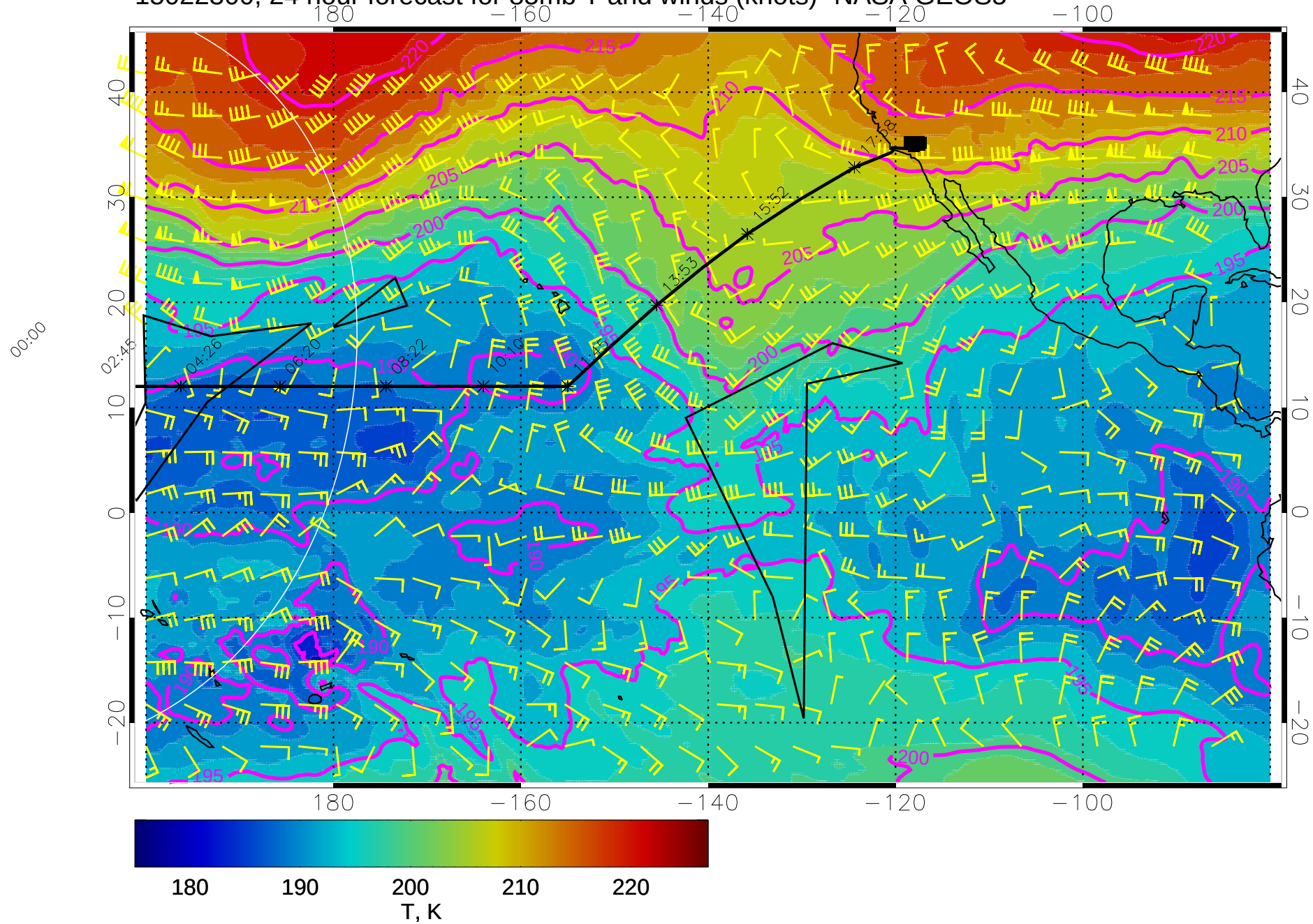
15022300, 24 hour forecast for 85mb T and winds (knots)- NASA GEOS5
