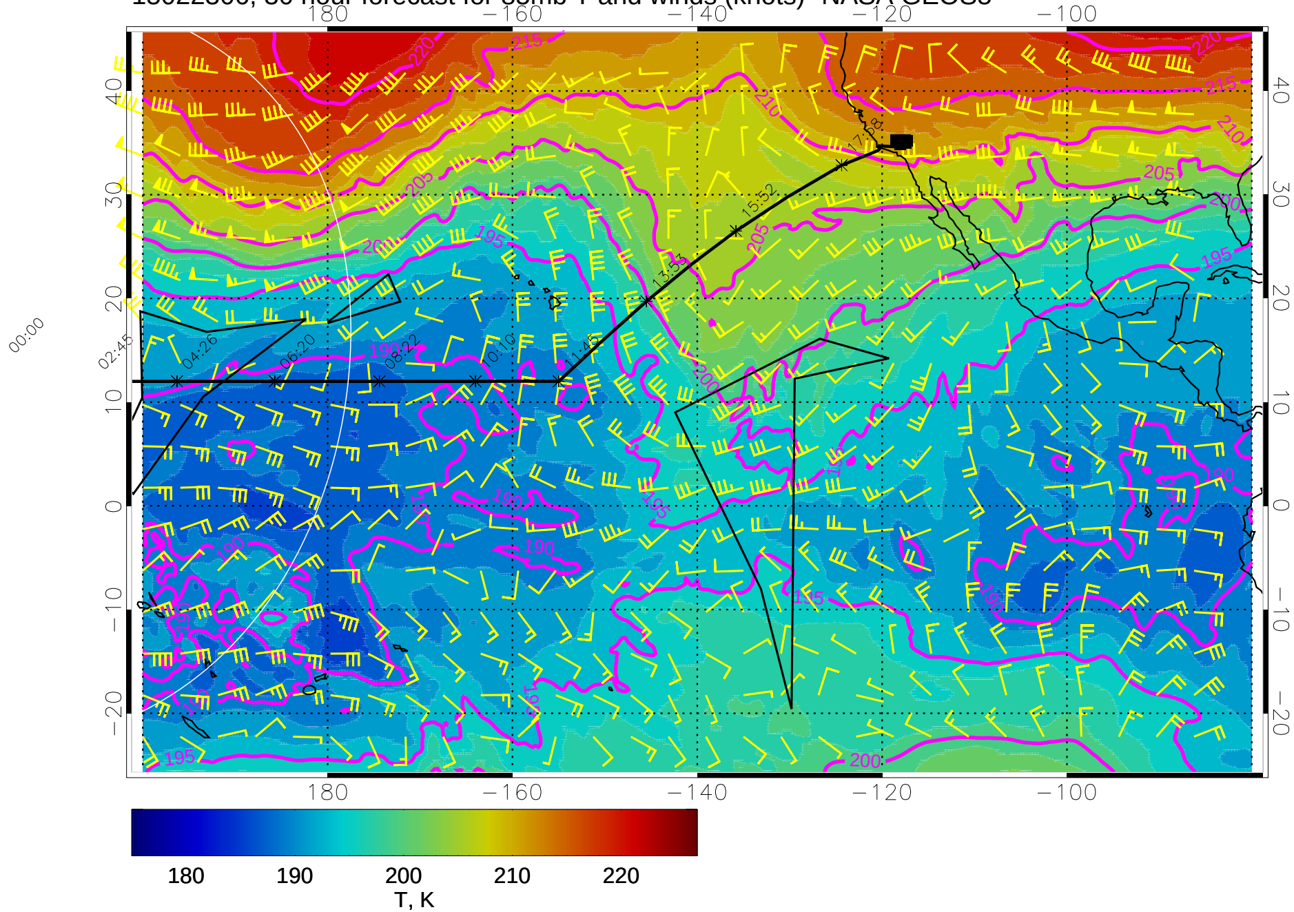
15022306, 30 hour forecast for 85mb T and winds (knots)- NASA GEOS5
