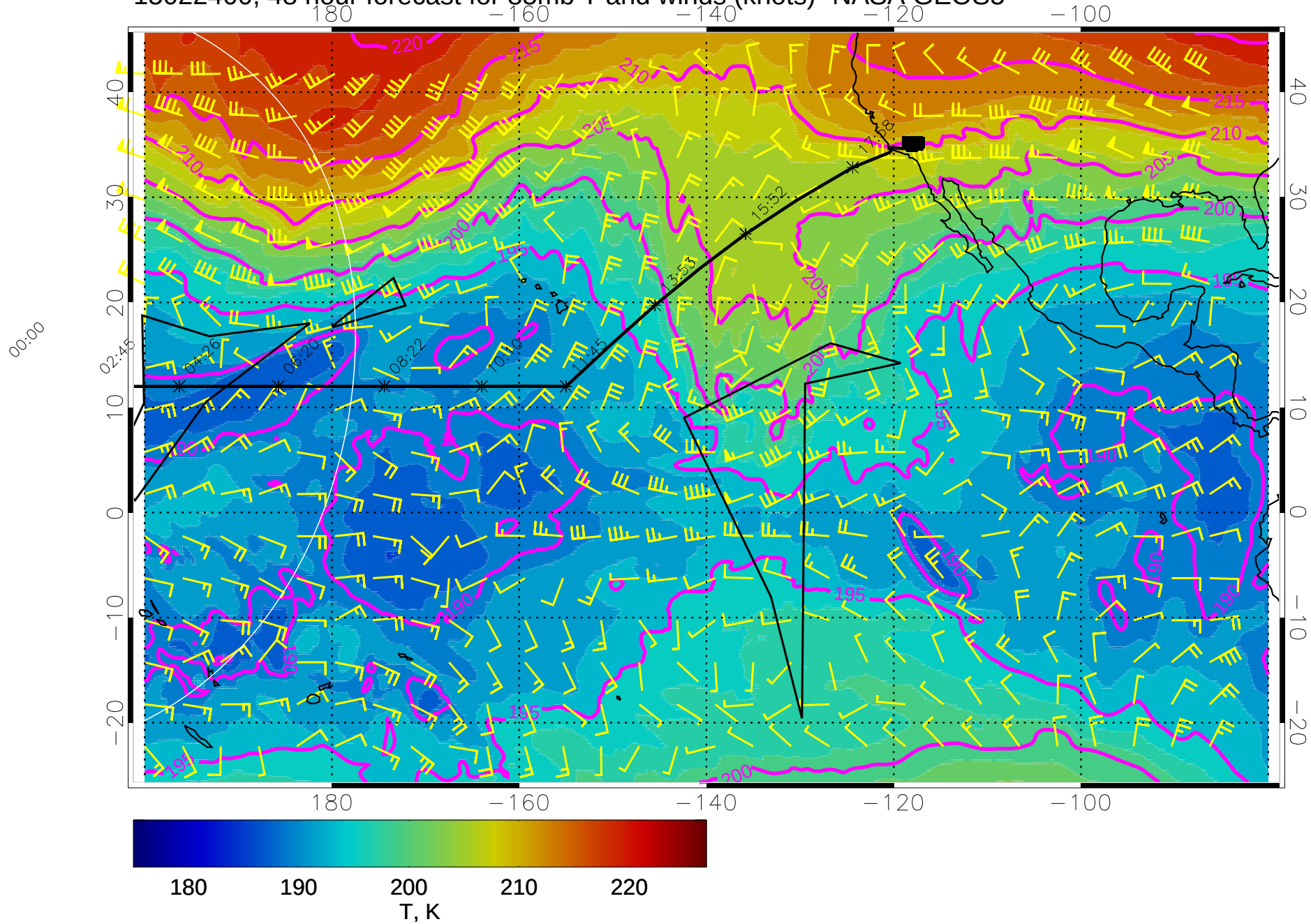
15022400, 48 hour forecast for 85mb T and winds (knots)- NASA GEOS5
