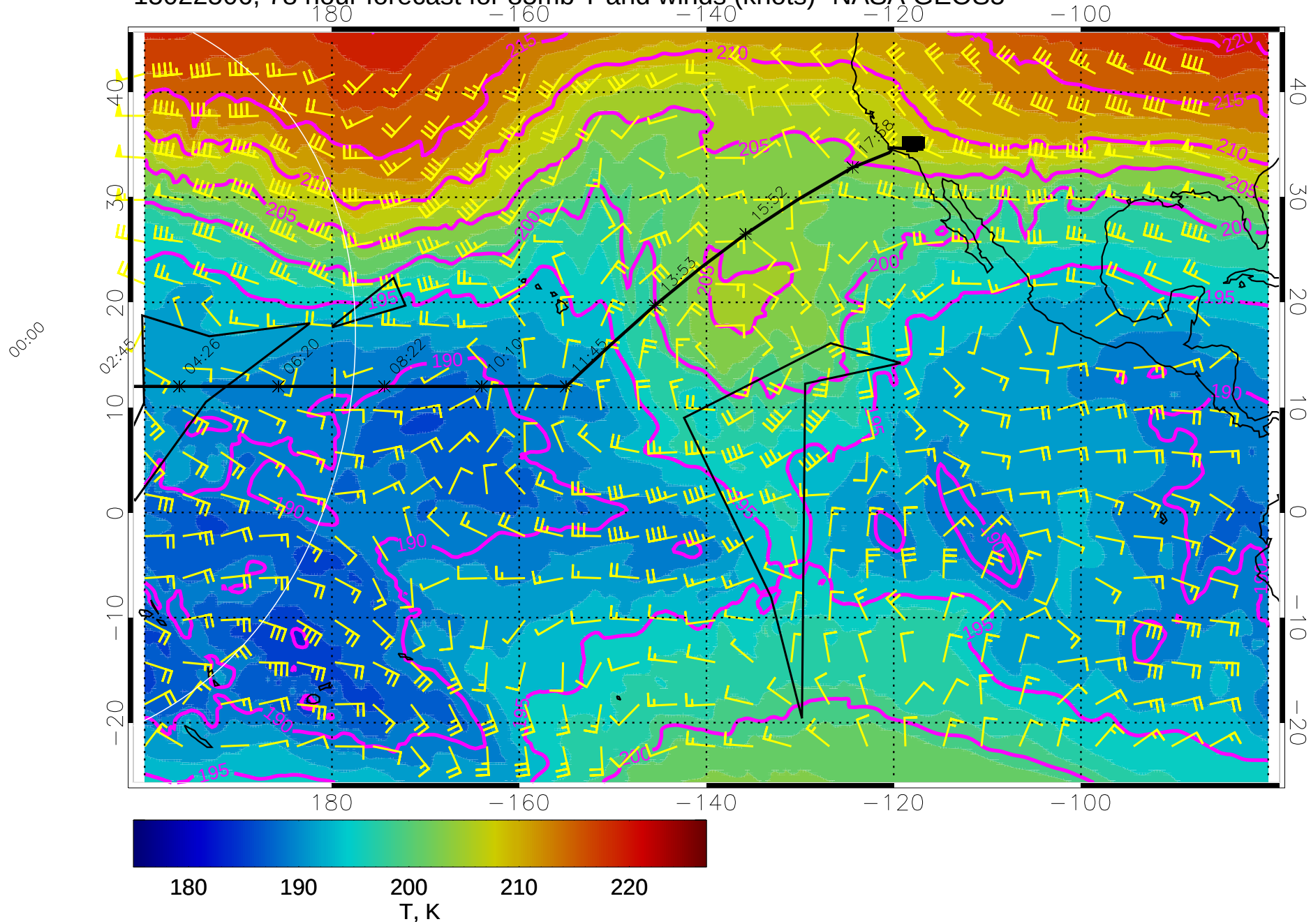
15022506, 78 hour forecast for 85mb T and winds (knots)- NASA GEOS5
