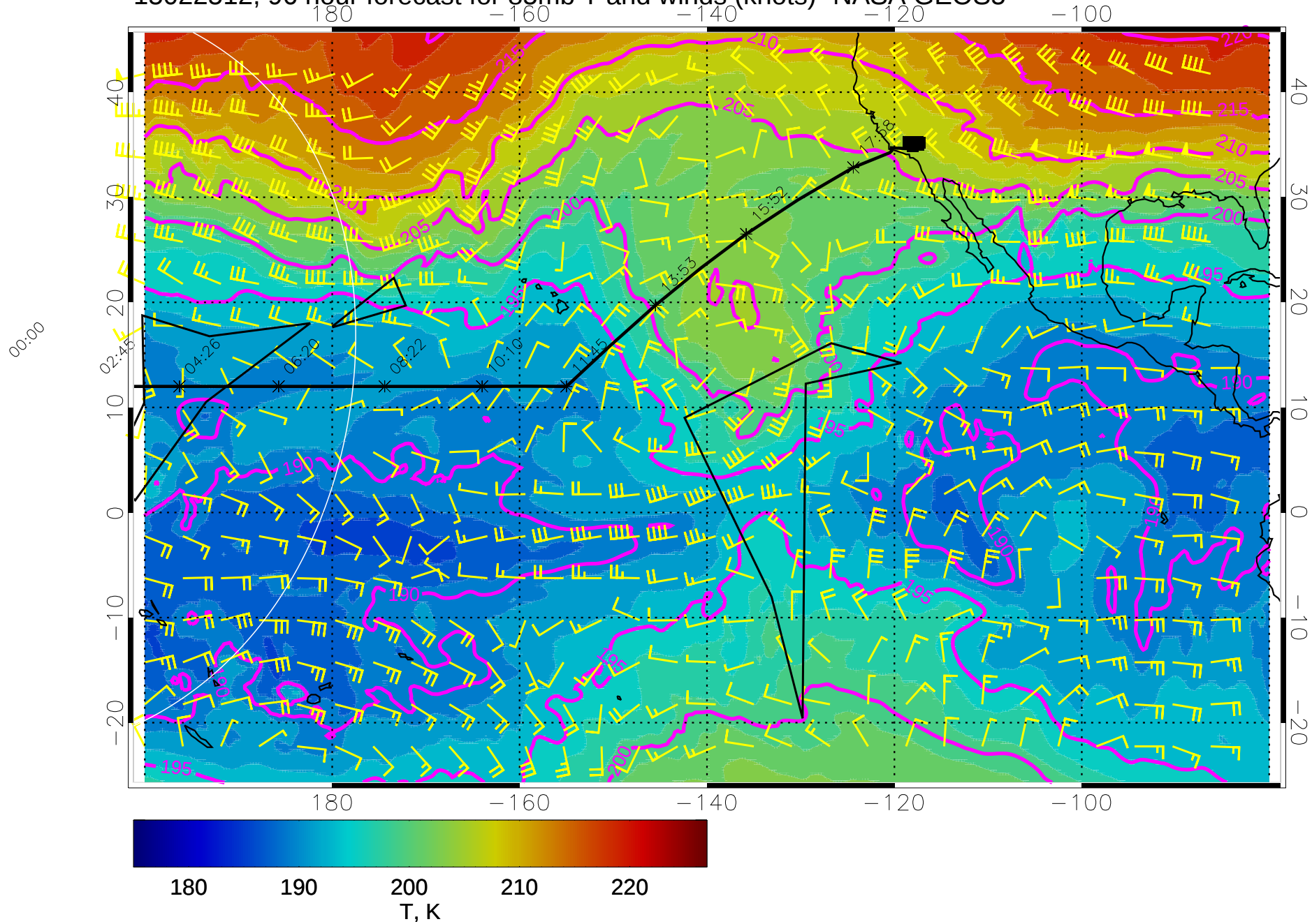
15022512, 96 hour forecast for 85mb T and winds (knots)- NASA GEOS5
