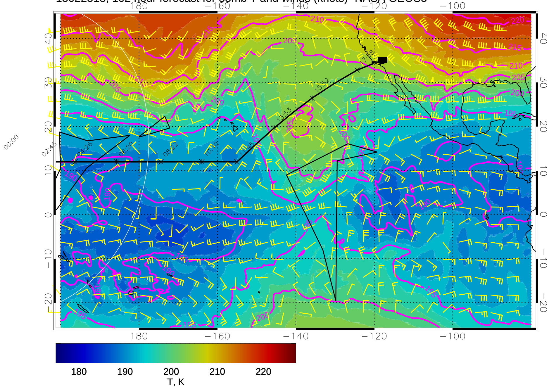
15022518, 102 hour forecast for 85mb T and winds (knots)- NASA GEOS5
