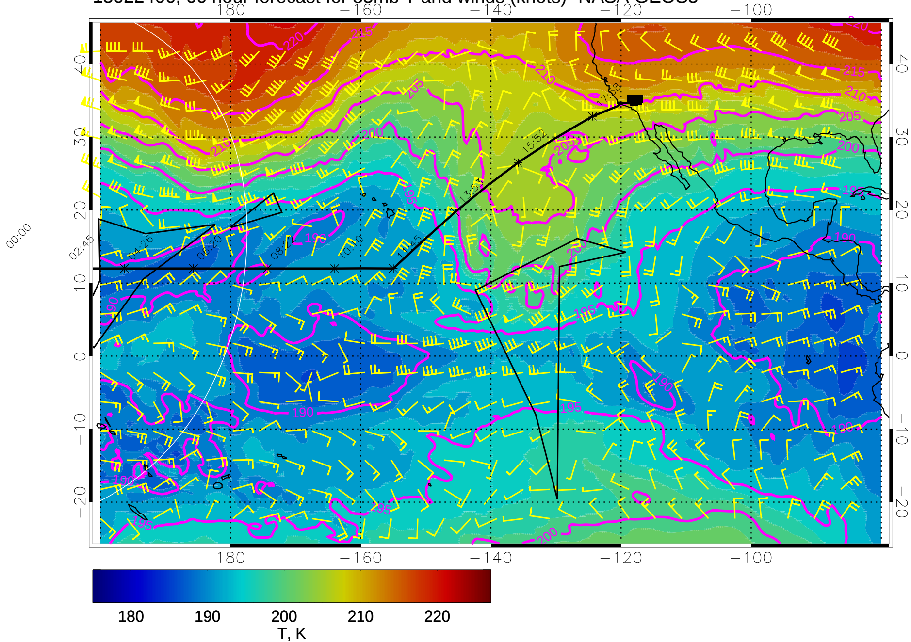
15022406, 66 hour forecast for 85mb T and winds (knots)- NASA GEOS5
