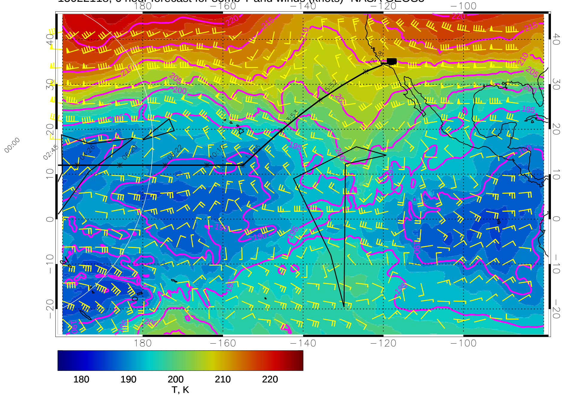
15022118, 6 hour forecast for 85mb T and winds (knots)- NASA GEOS5
