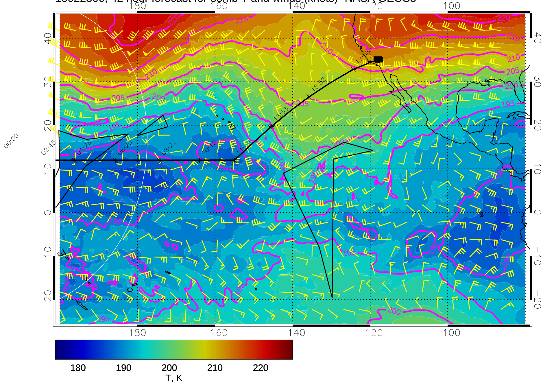
15022306, 42 hour forecast for 85mb T and winds (knots)- NASA GEOS5
