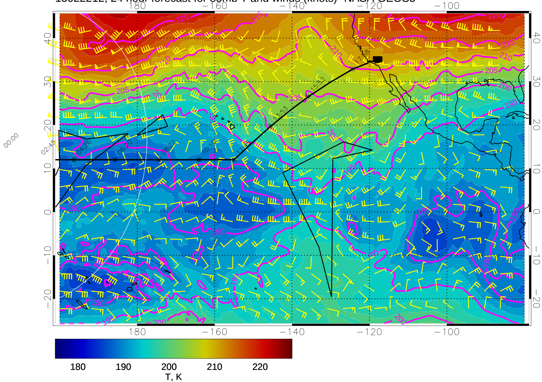
15022212, 24 hour forecast for 85mb T and winds (knots)- NASA GEOS5
