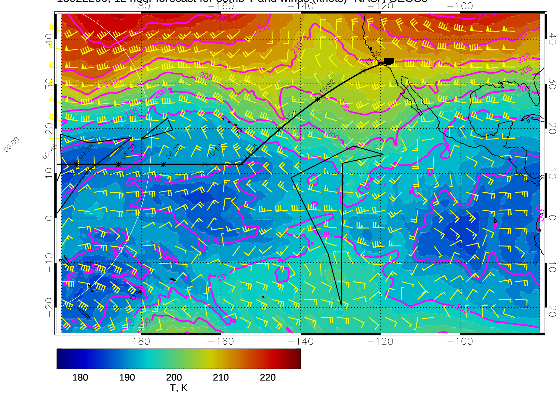
15022200, 12 hour forecast for 85mb T and winds (knots)- NASA GEOS5
