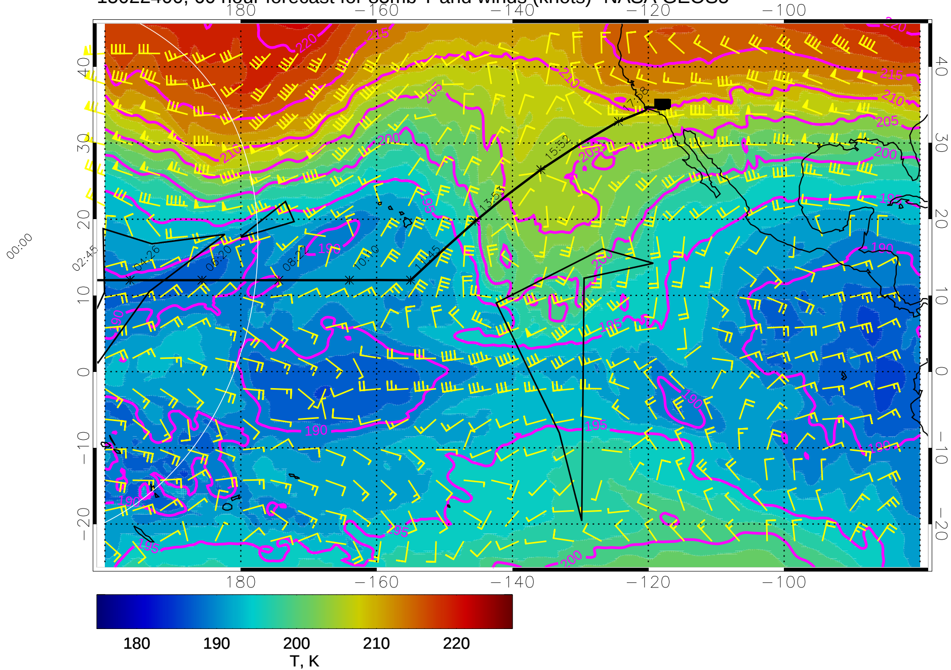
15022400, 60 hour forecast for 85mb T and winds (knots)- NASA GEOS5
