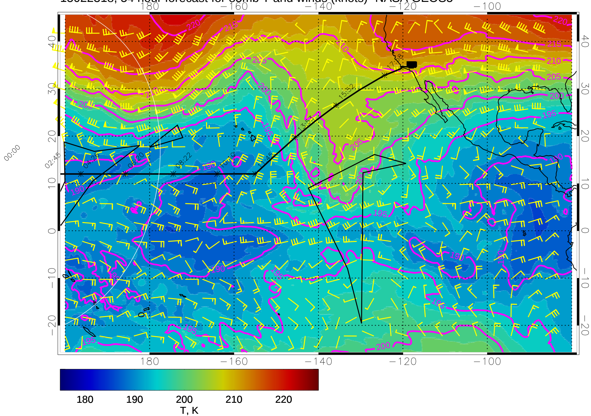
15022318, 54 hour forecast for 85mb T and winds (knots)- NASA GEOS5
