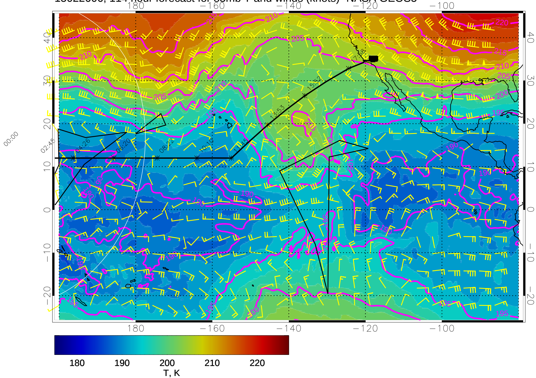
15022606, 114 hour forecast for 85mb T and winds (knots)- NASA GEOS5
