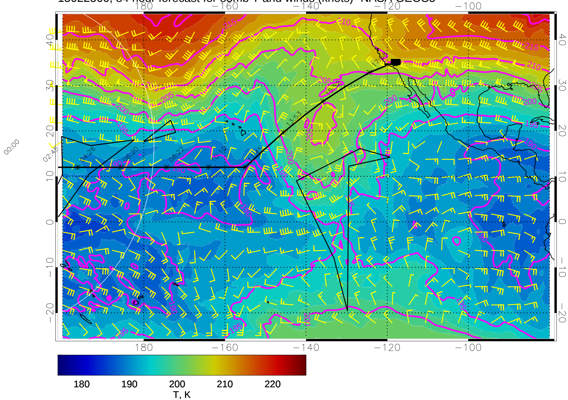
15022500, 84 hour forecast for 85mb T and winds (knots)- NASA GEOS5
