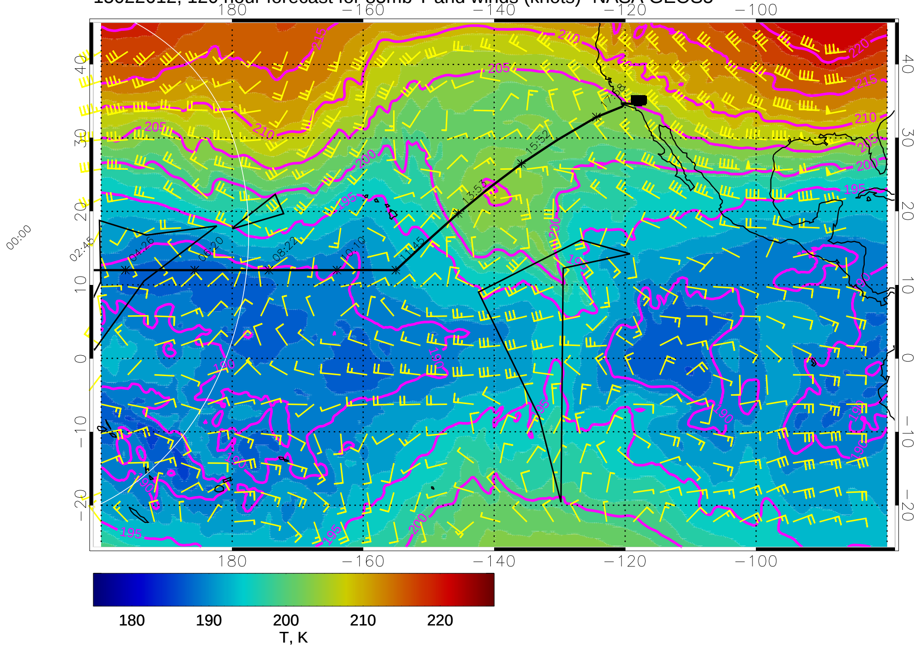
15022612, 120 hour forecast for 85mb T and winds (knots)- NASA GEOS5
