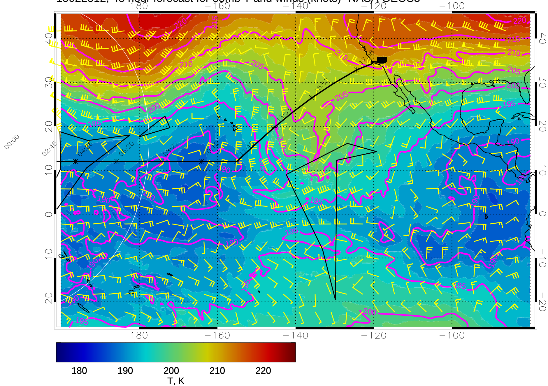
15022312, 48 hour forecast for 85mb T and winds (knots)- NASA GEOS5
