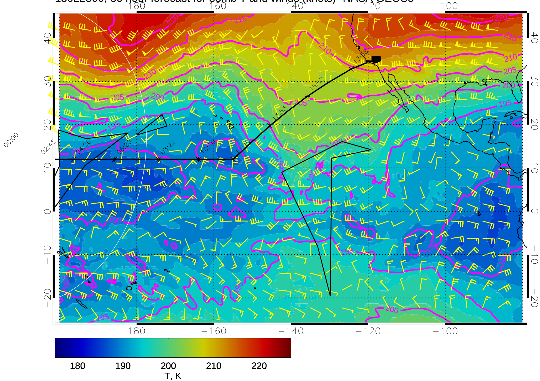
15022300, 36 hour forecast for 85mb T and winds (knots)- NASA GEOS5
