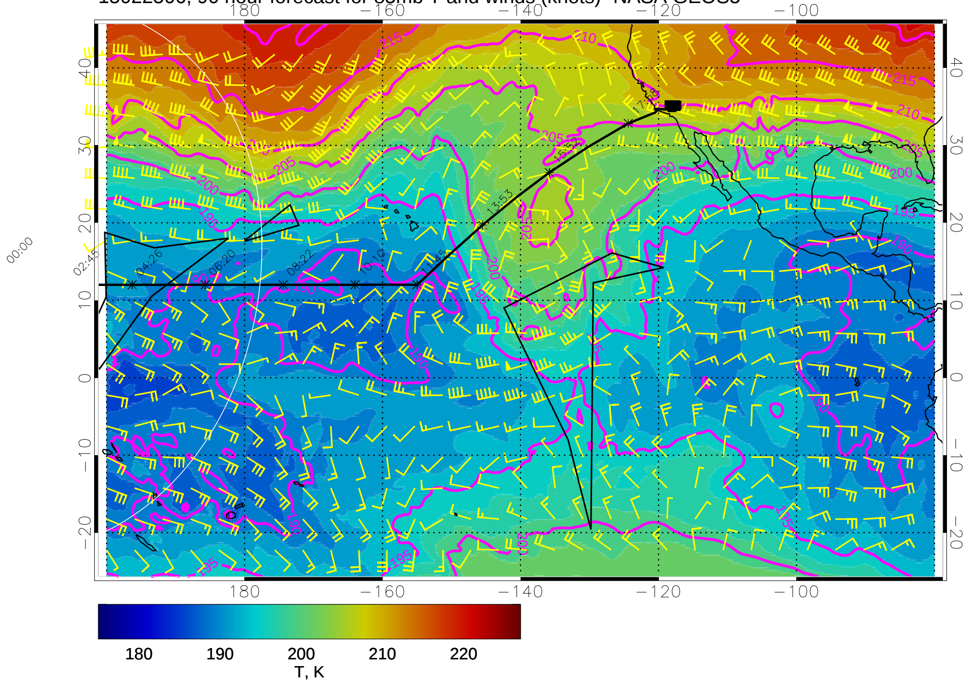
15022506, 90 hour forecast for 85mb T and winds (knots)- NASA GEOS5
