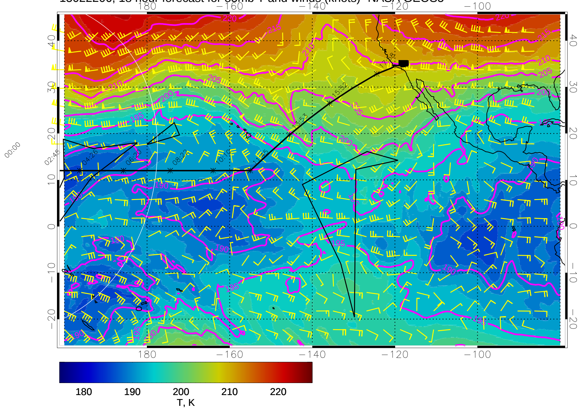
15022206, 18 hour forecast for 85mb T and winds (knots)- NASA GEOS5
