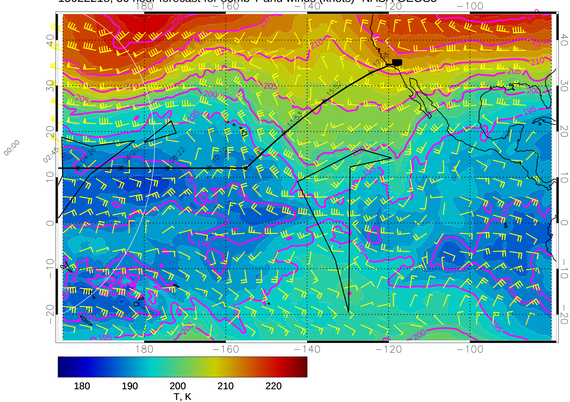
15022218, 30 hour forecast for 85mb T and winds (knots)- NASA GEOS5
