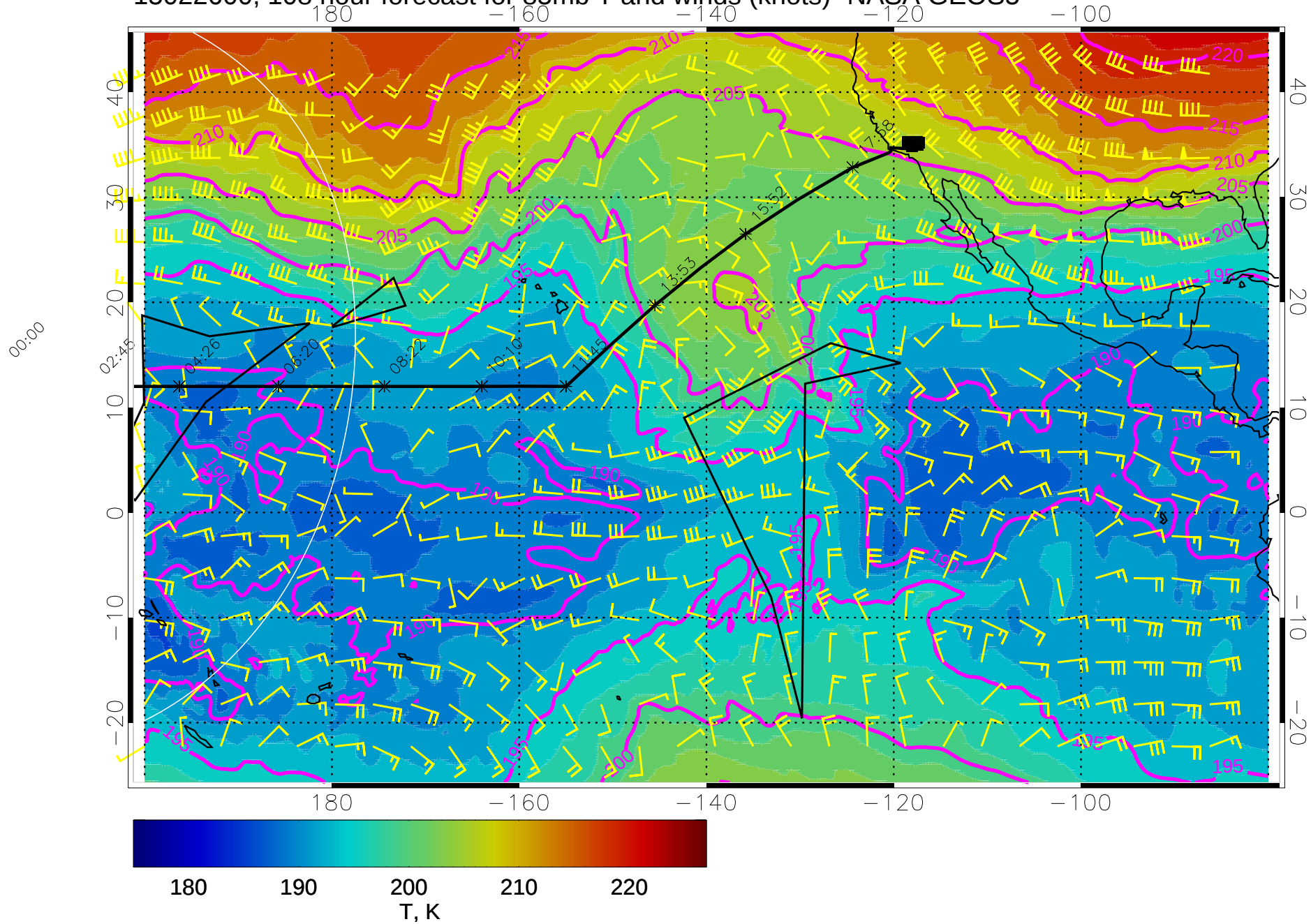
15022600, 108 hour forecast for 85mb T and winds (knots)- NASA GEOS5
