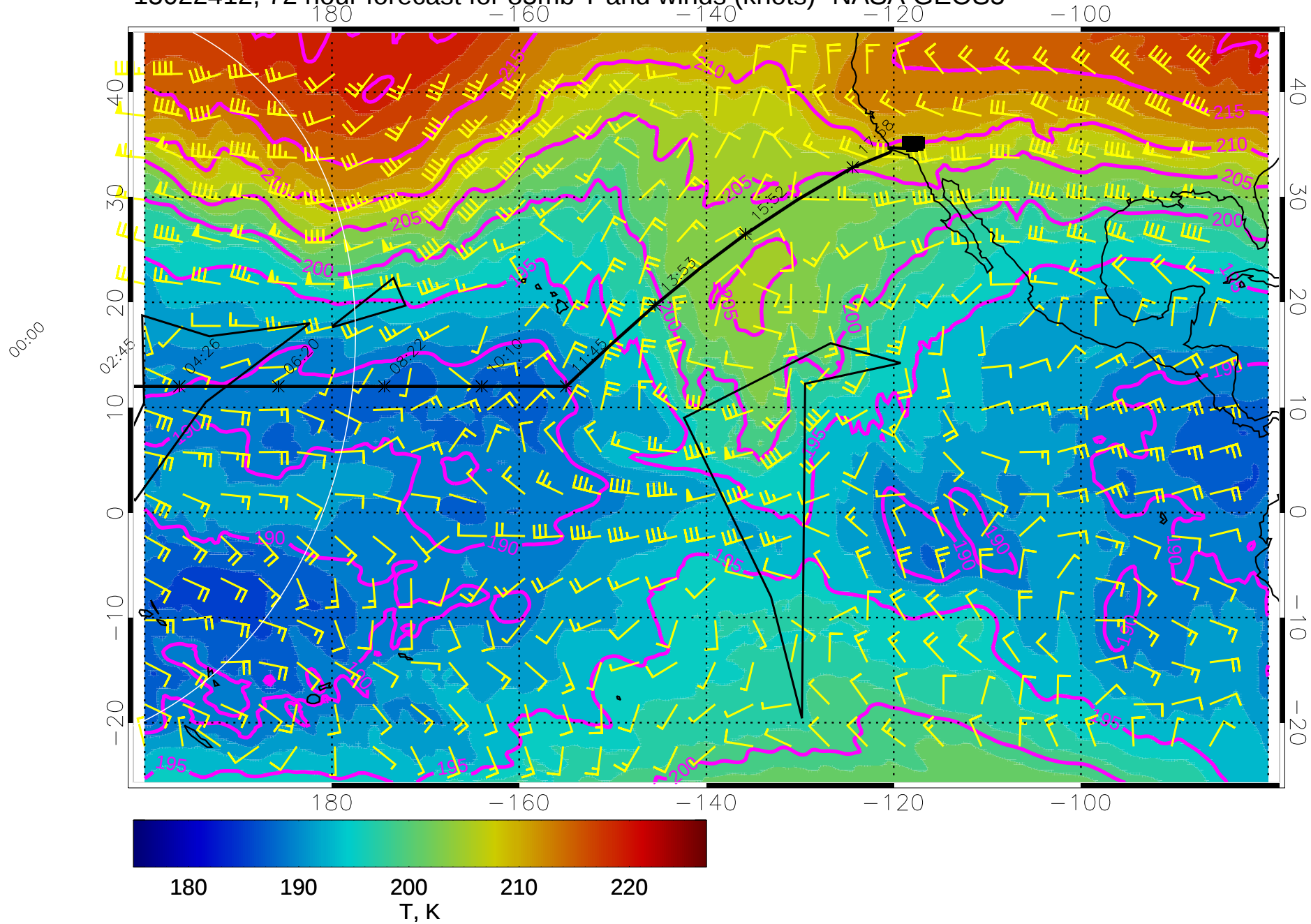
15022412, 72 hour forecast for 85mb T and winds (knots)- NASA GEOS5
