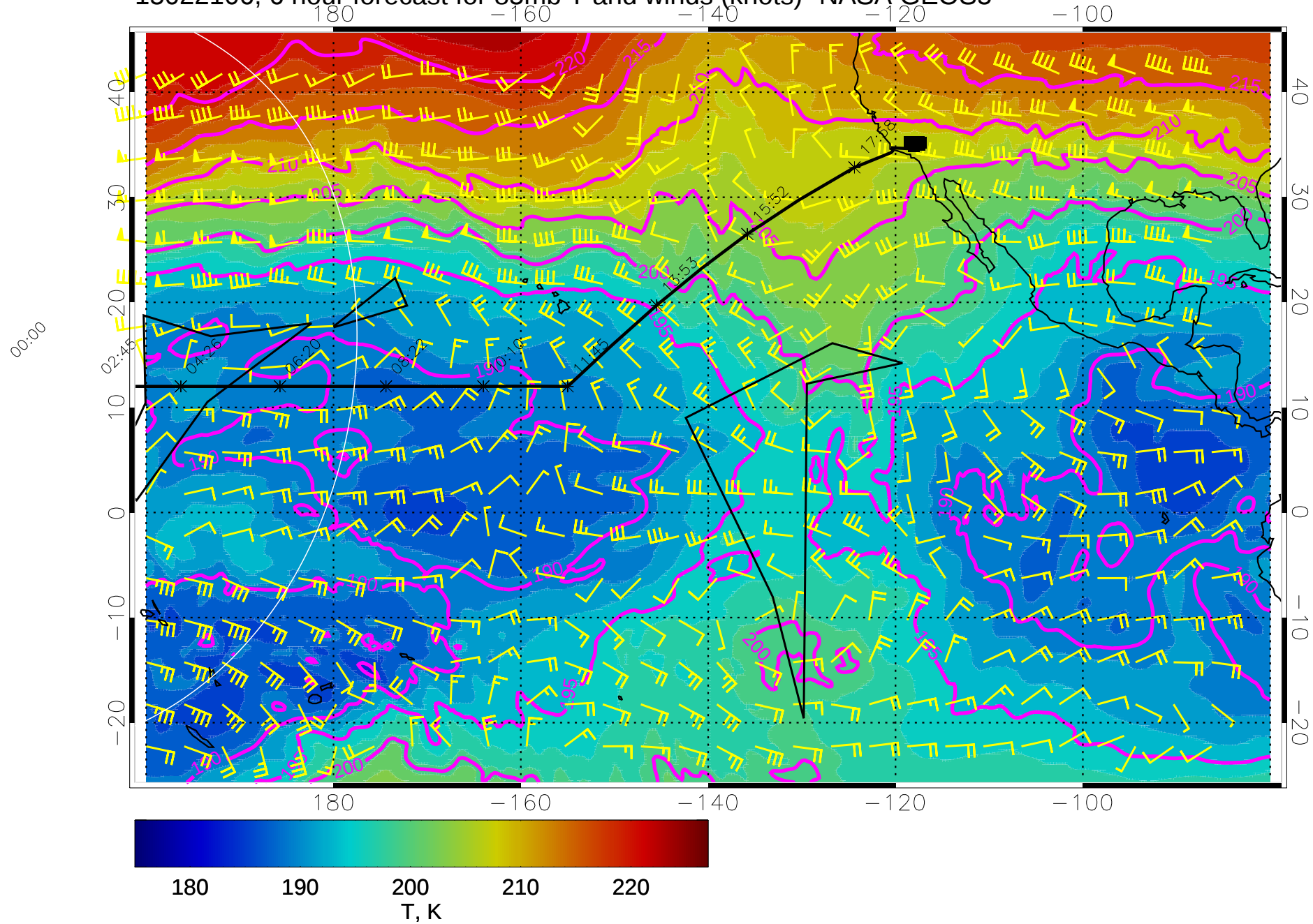
15022106, 6 hour forecast for 85mb T and winds (knots)- NASA GEOS5
