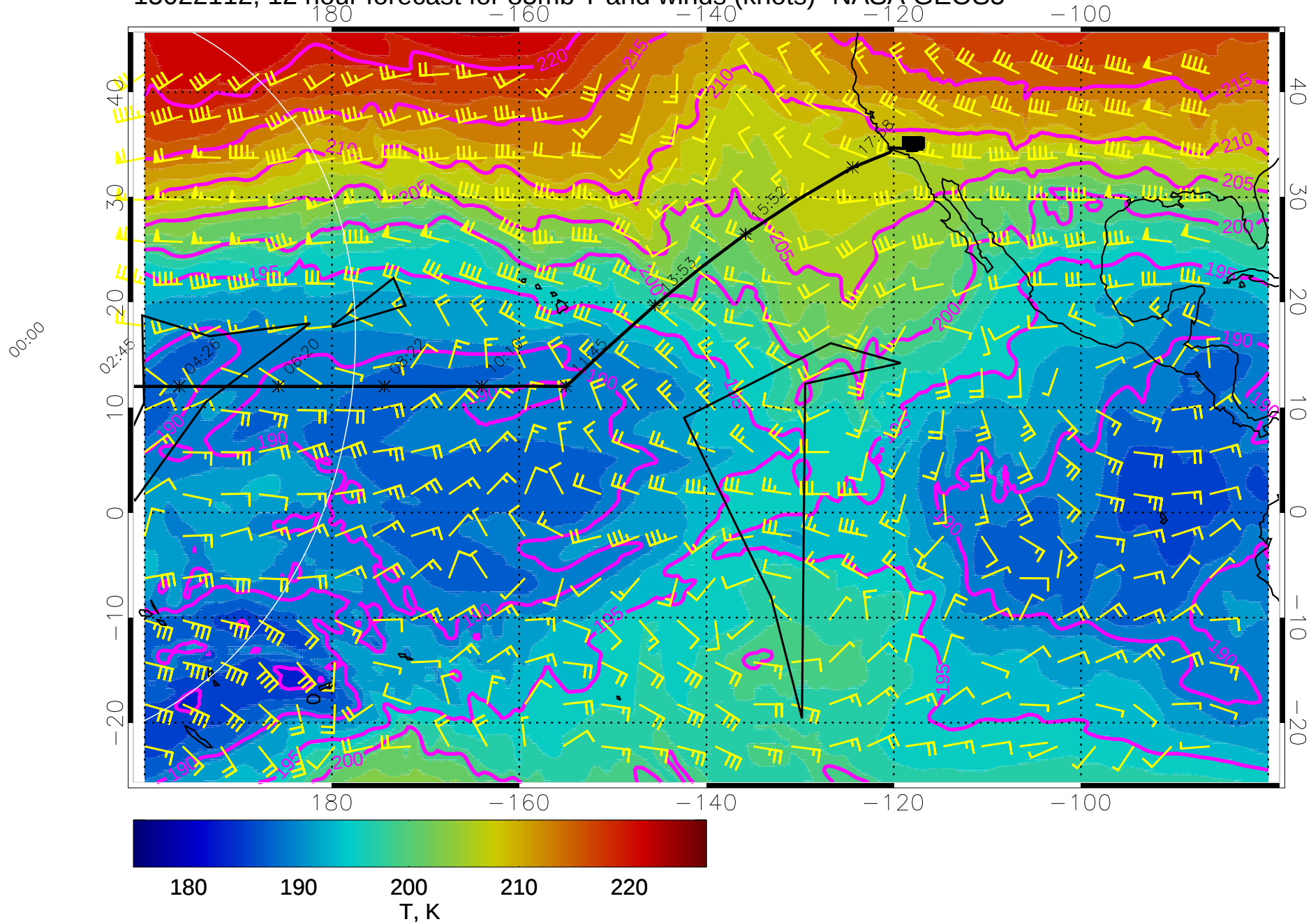
15022112, 12 hour forecast for 85mb T and winds (knots)- NASA GEOS5
