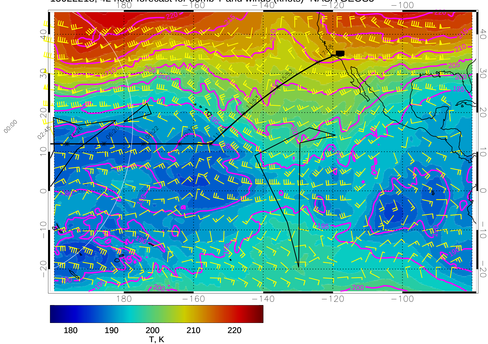
15022218, 42 hour forecast for 85mb T and winds (knots)- NASA GEOS5
