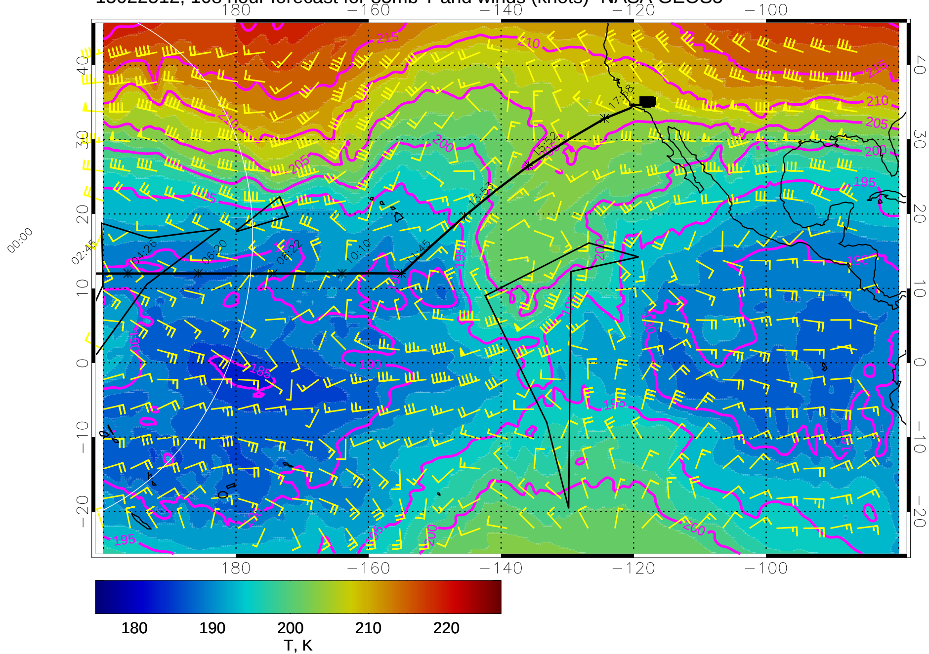
15022512, 108 hour forecast for 85mb T and winds (knots)- NASA GEOS5
