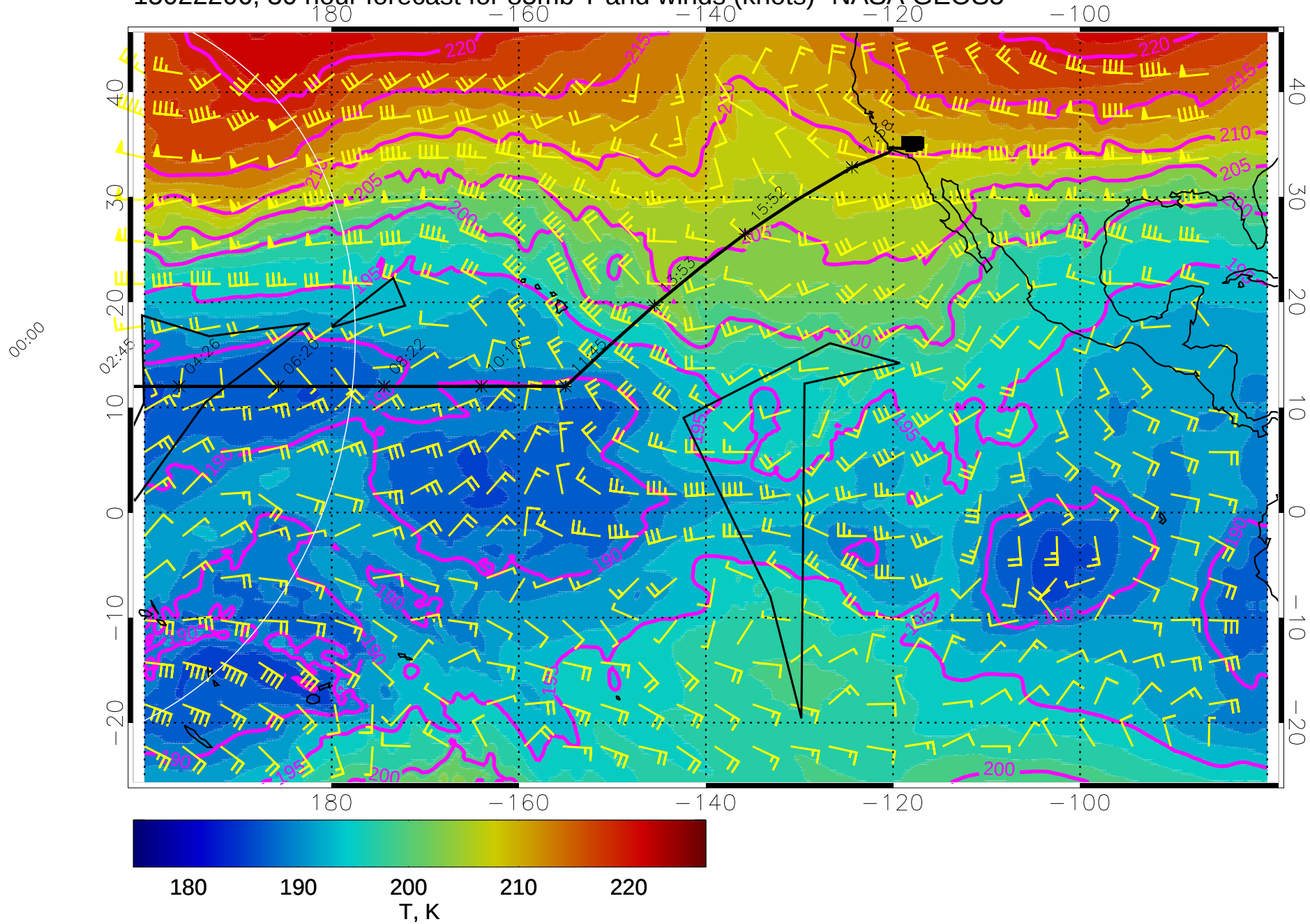
15022206, 30 hour forecast for 85mb T and winds (knots)- NASA GEOS5
