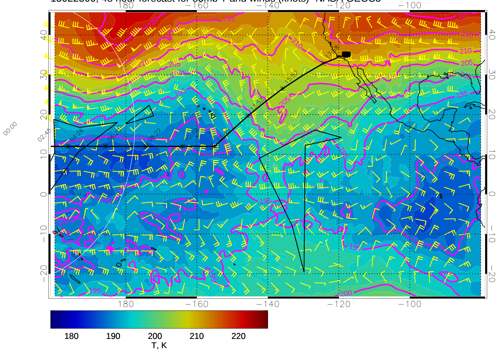
15022300, 48 hour forecast for 85mb T and winds (knots)- NASA GEOS5
