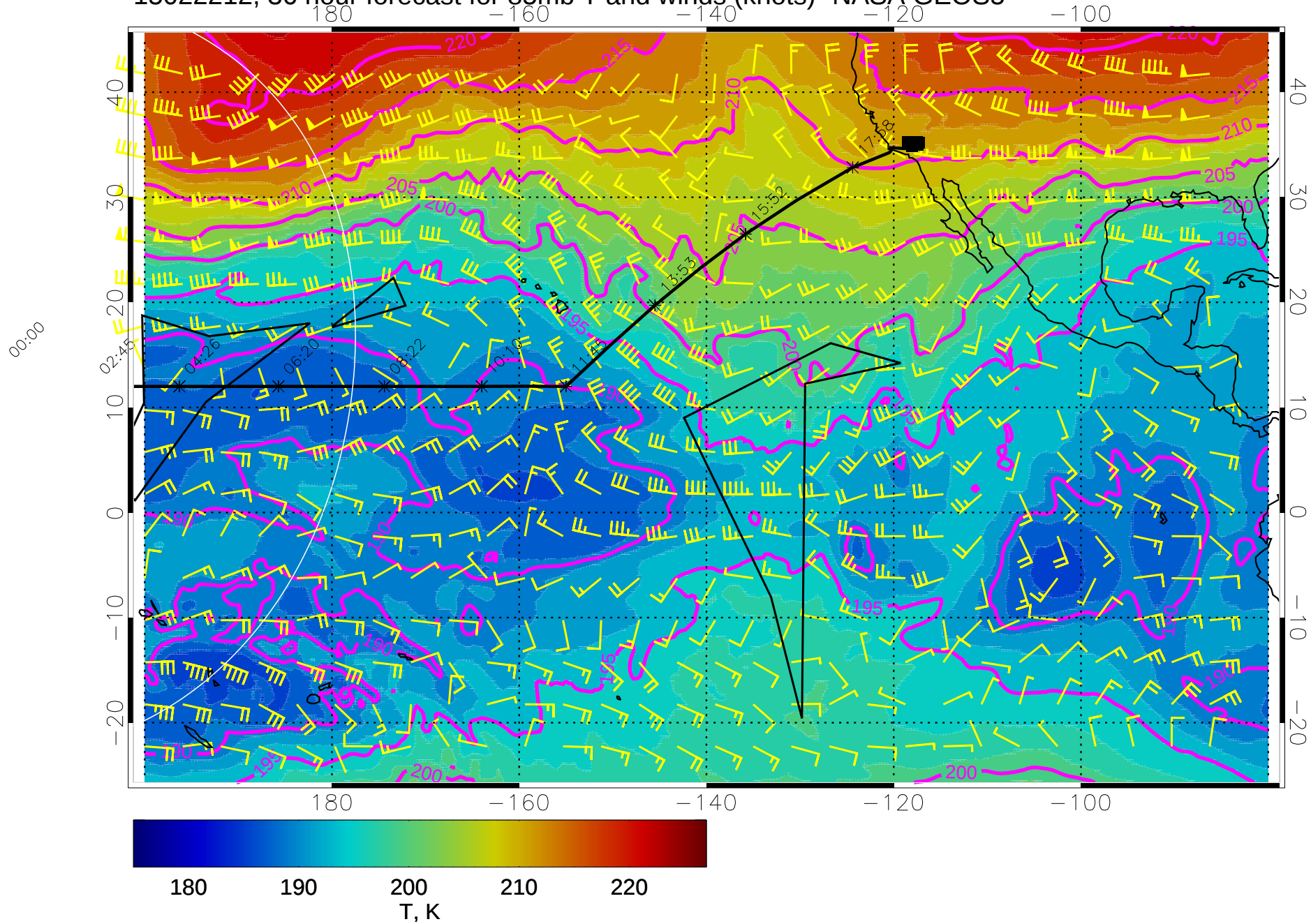
15022212, 36 hour forecast for 85mb T and winds (knots)- NASA GEOS5
