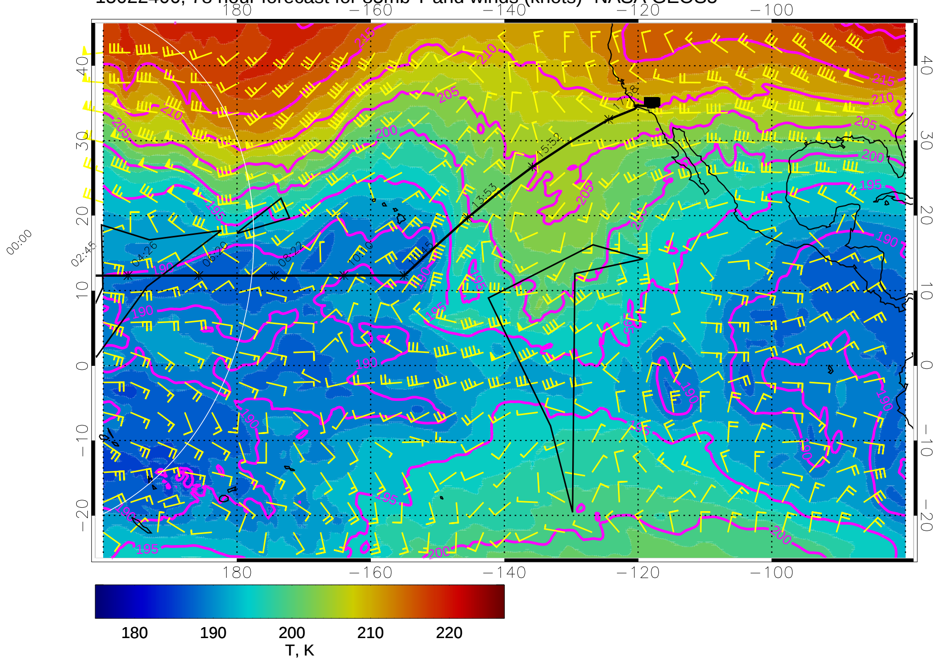
15022406, 78 hour forecast for 85mb T and winds (knots)- NASA GEOS5
