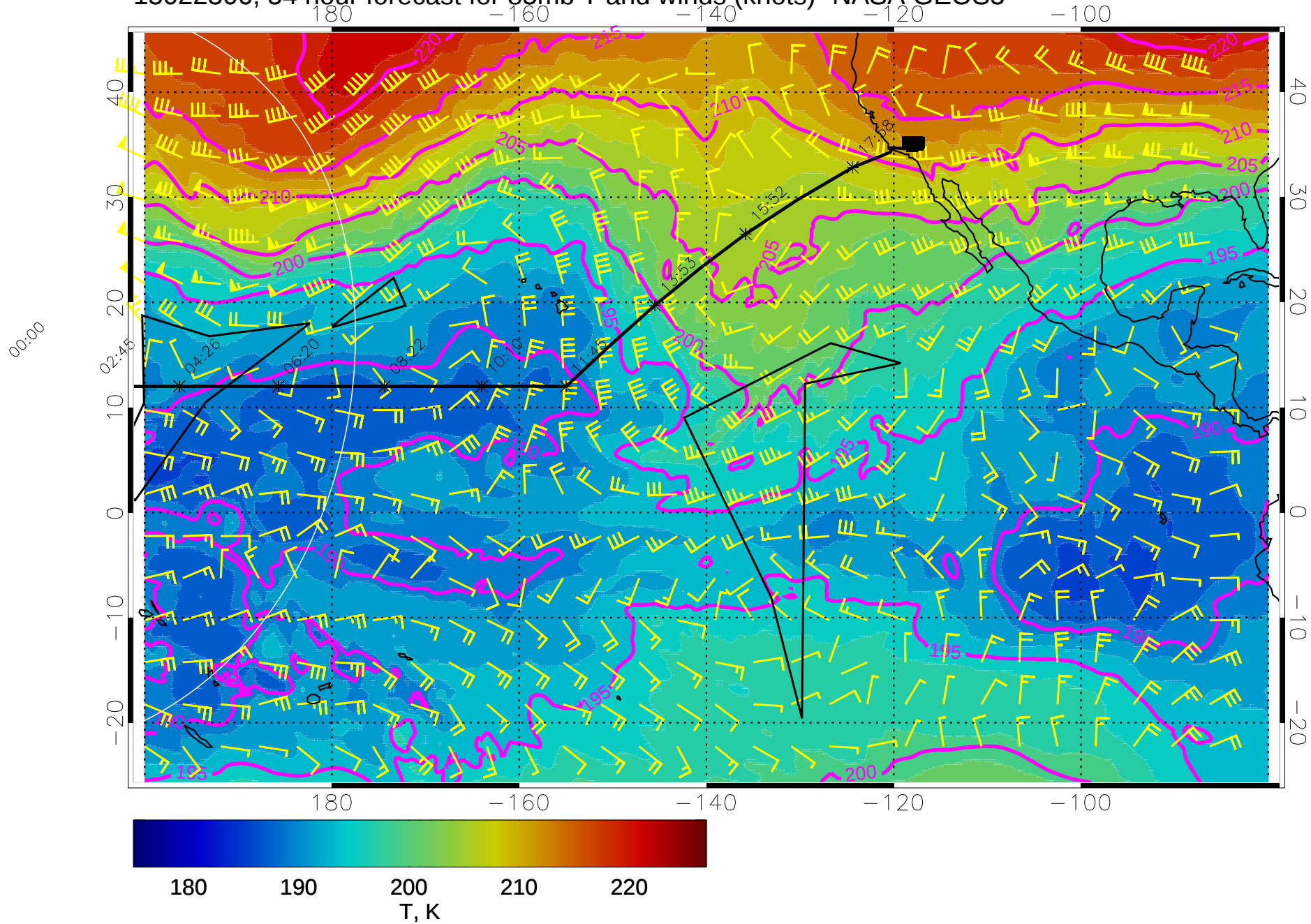
15022306, 54 hour forecast for 85mb T and winds (knots)- NASA GEOS5
