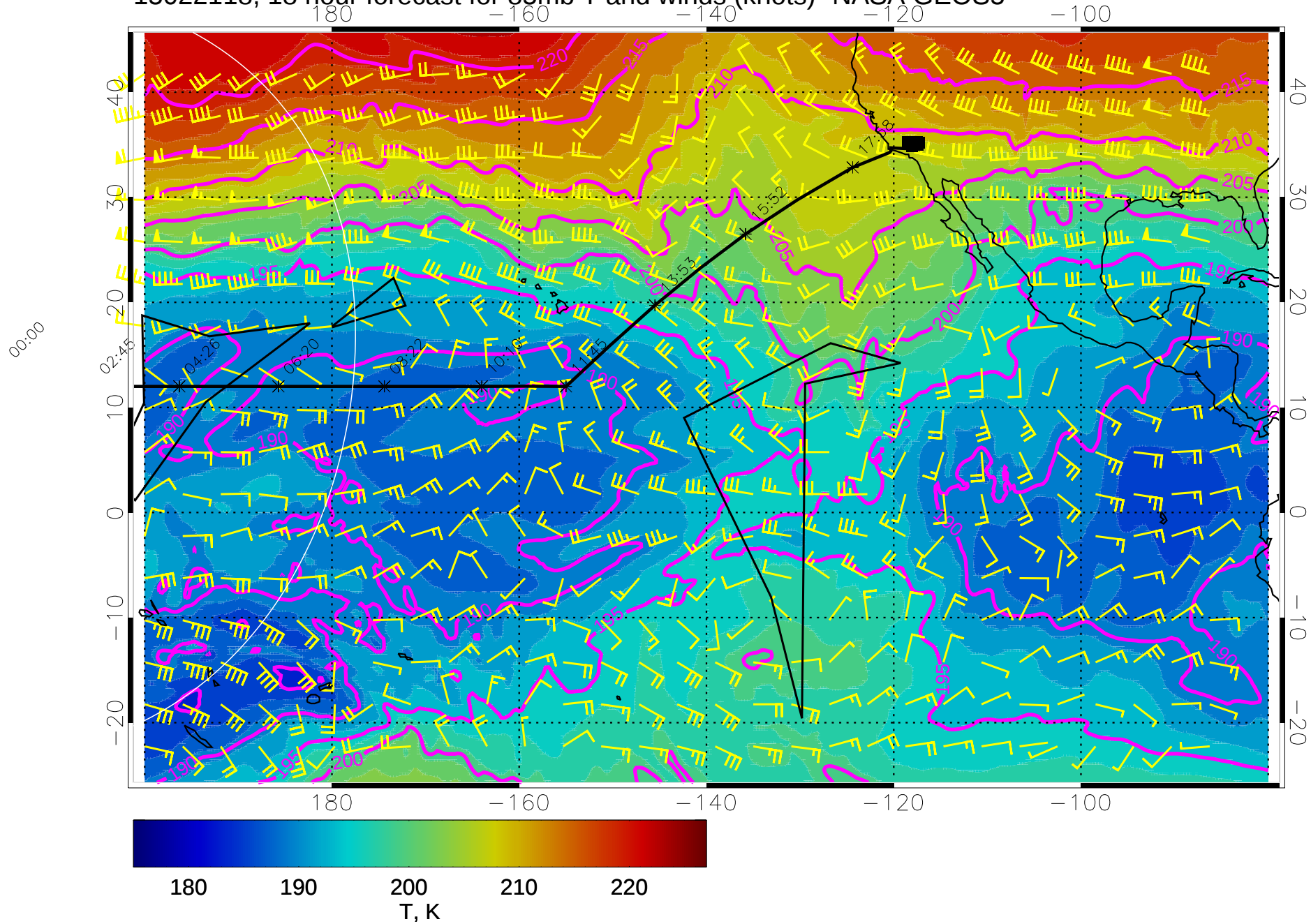
15022118, 18 hour forecast for 85mb T and winds (knots)- NASA GEOS5
