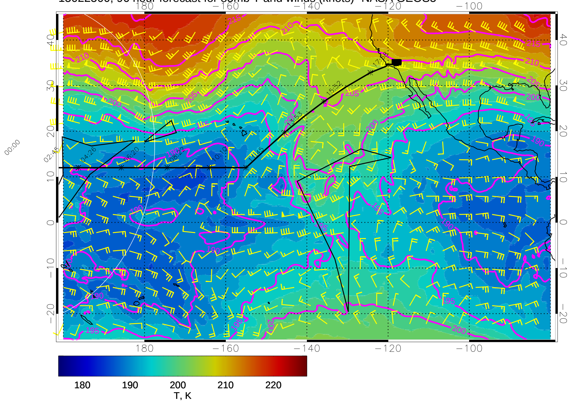
15022500, 96 hour forecast for 85mb T and winds (knots)- NASA GEOS5
