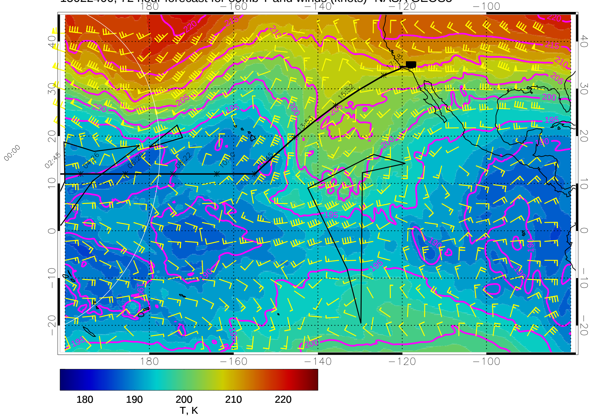
15022400, 72 hour forecast for 85mb T and winds (knots)- NASA GEOS5
