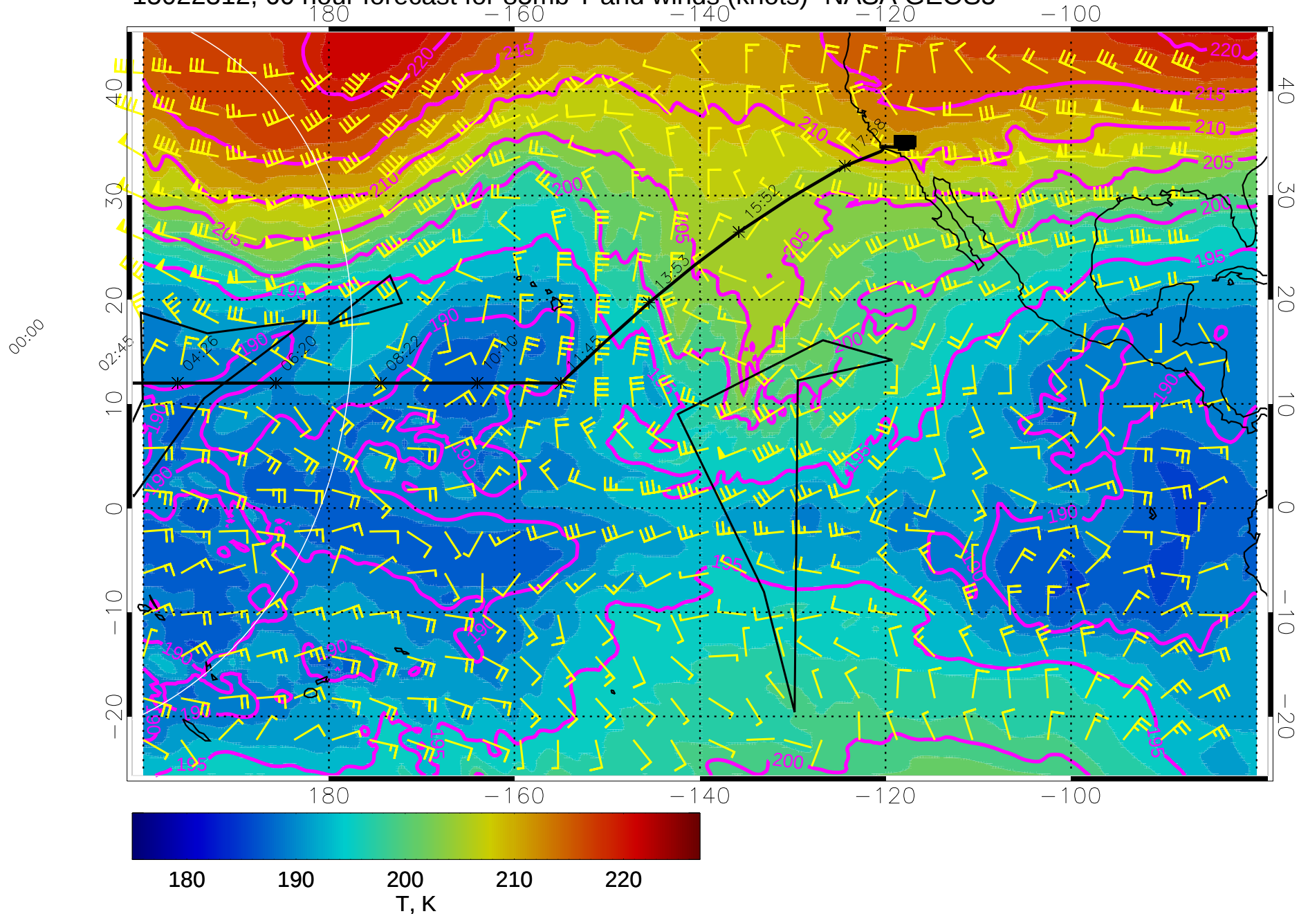
15022312, 60 hour forecast for 85mb T and winds (knots)- NASA GEOS5
