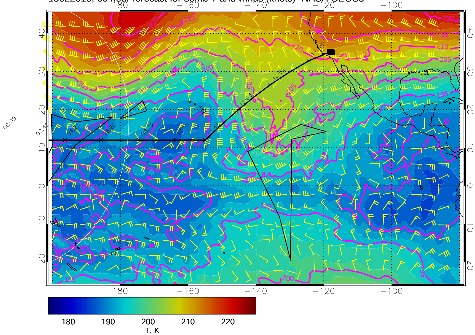
15022318, 66 hour forecast for 85mb T and winds (knots)- NASA GEOS5
