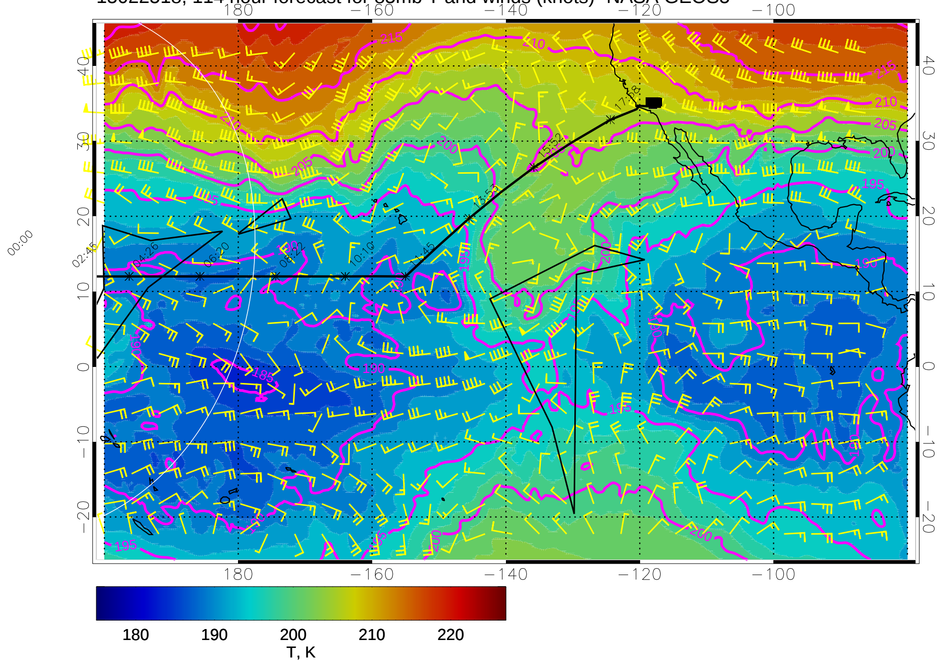
15022518, 114 hour forecast for 85mb T and winds (knots)- NASA GEOS5
