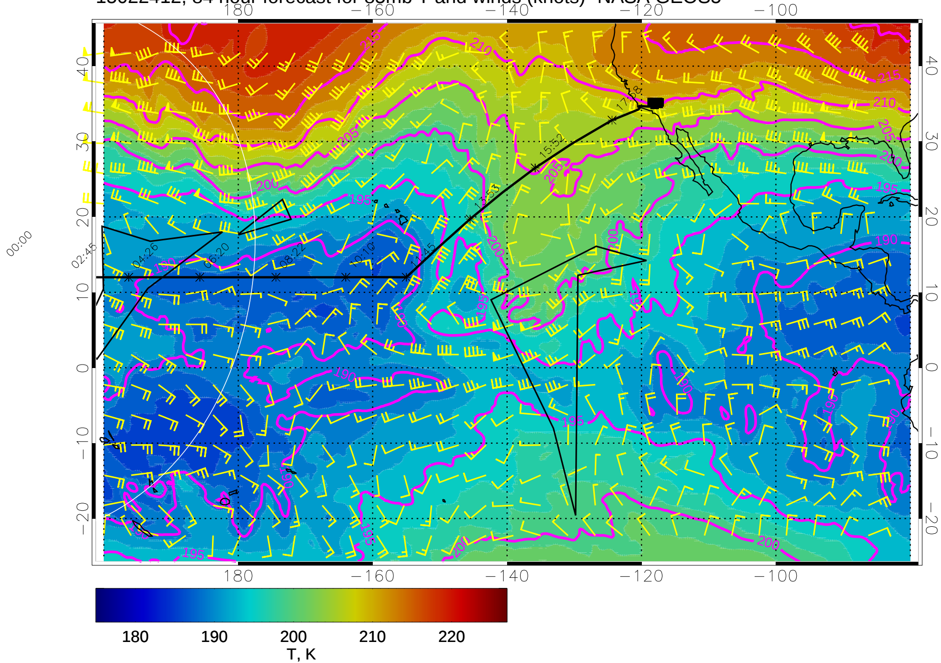
15022412, 84 hour forecast for 85mb T and winds (knots)- NASA GEOS5
