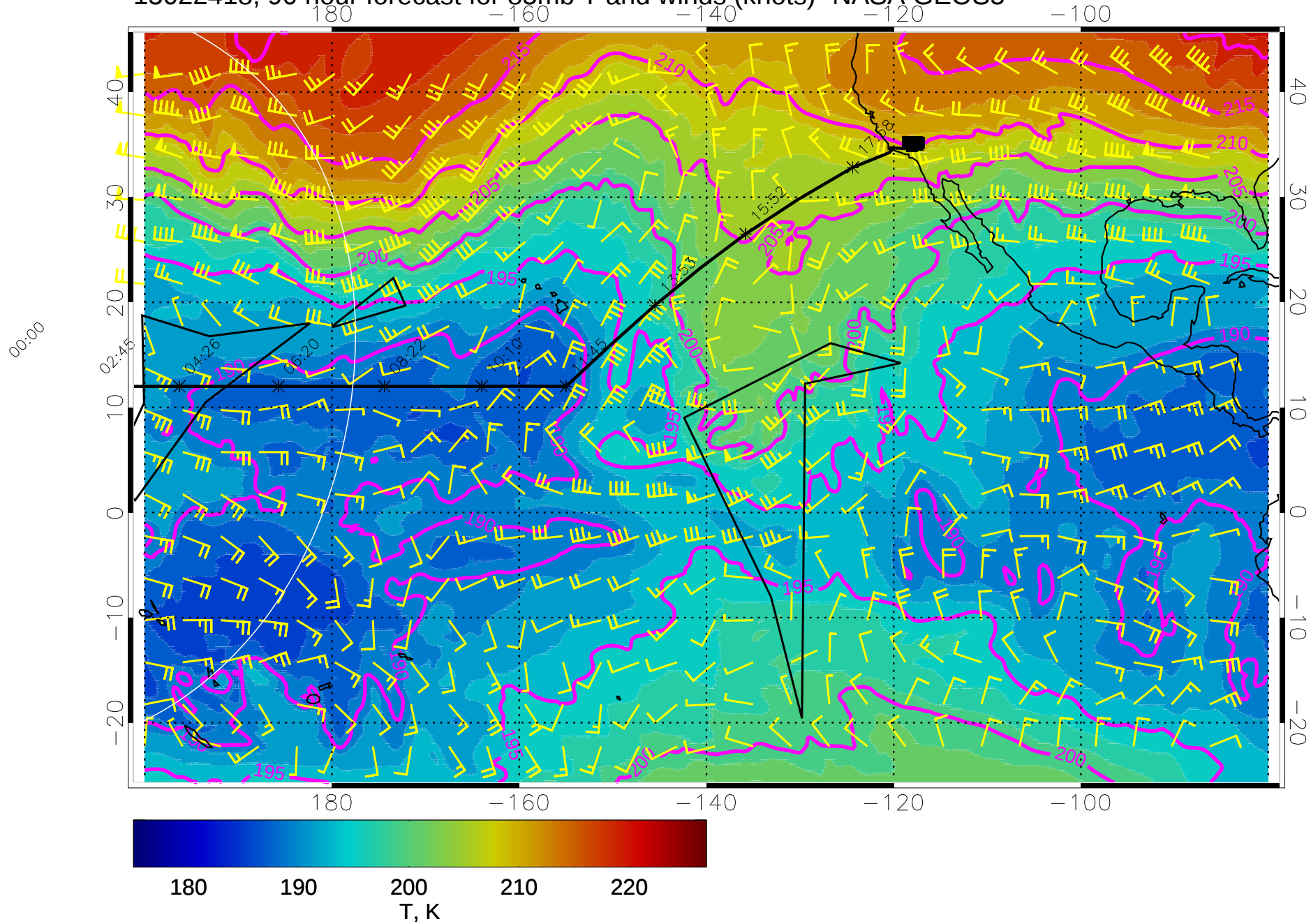
15022418, 90 hour forecast for 85mb T and winds (knots)- NASA GEOS5
