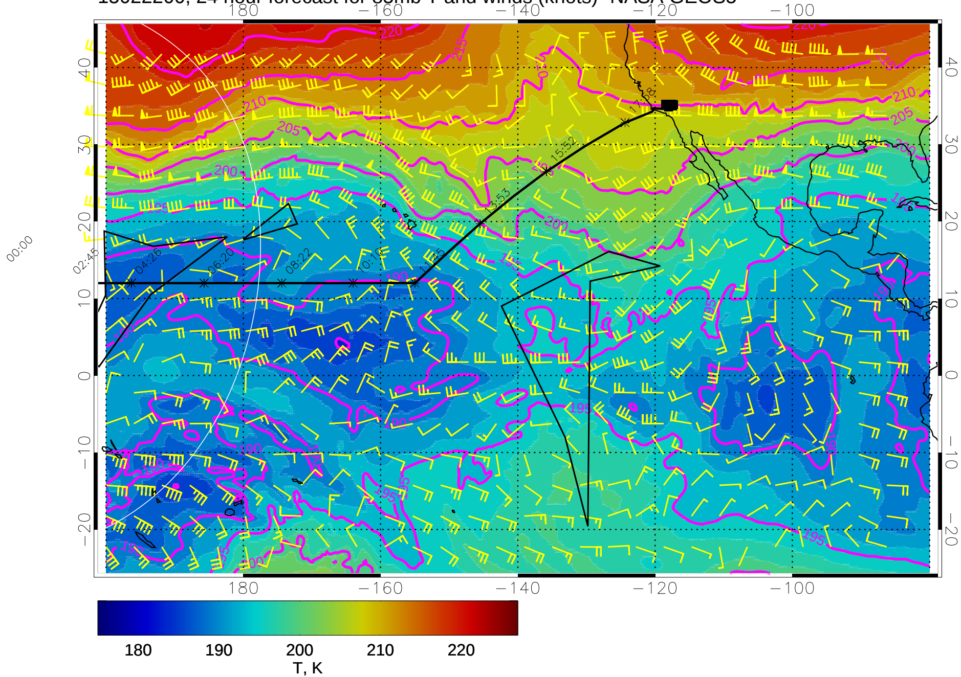
15022200, 24 hour forecast for 85mb T and winds (knots)- NASA GEOS5
