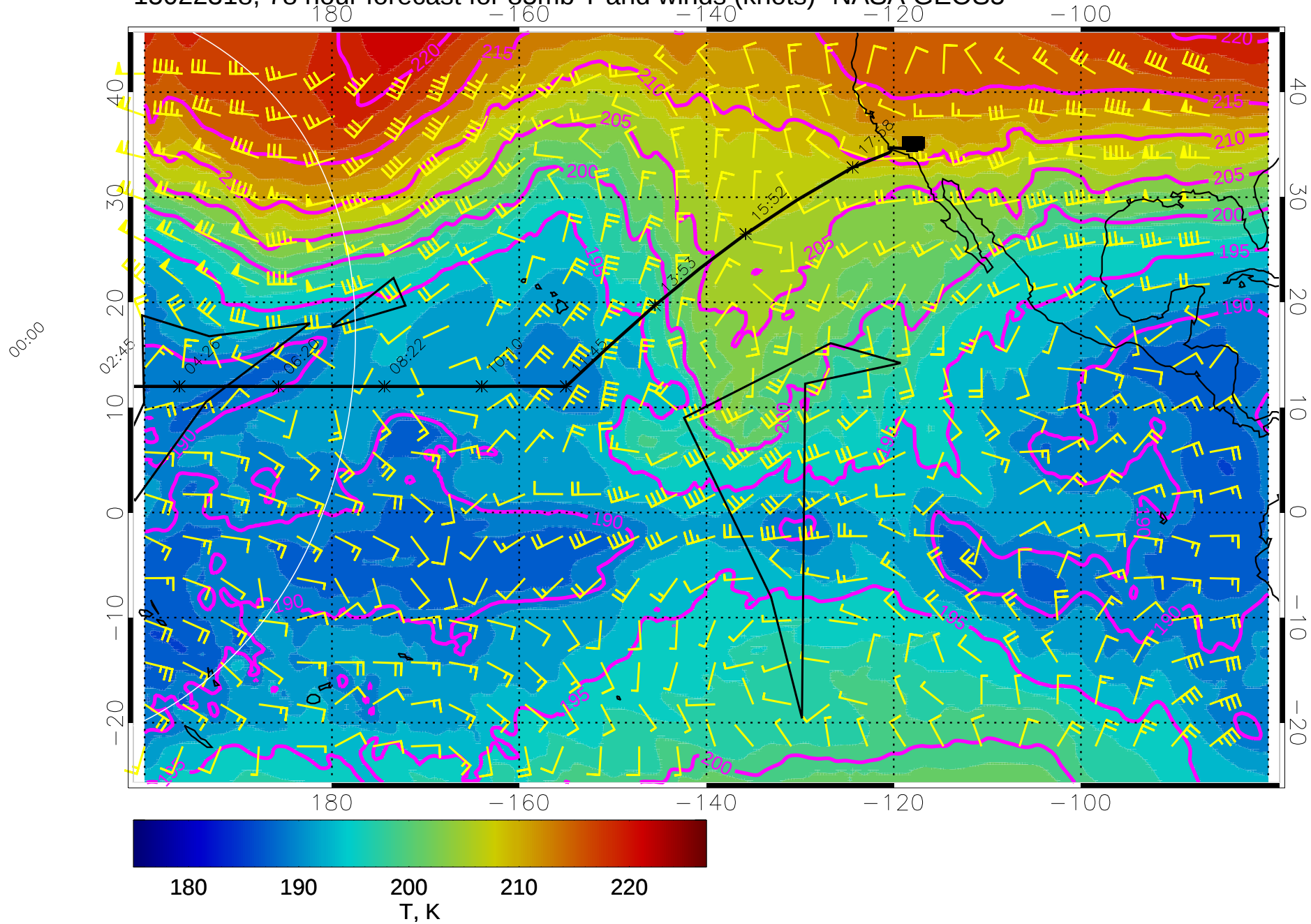
15022318, 78 hour forecast for 85mb T and winds (knots)- NASA GEOS5
