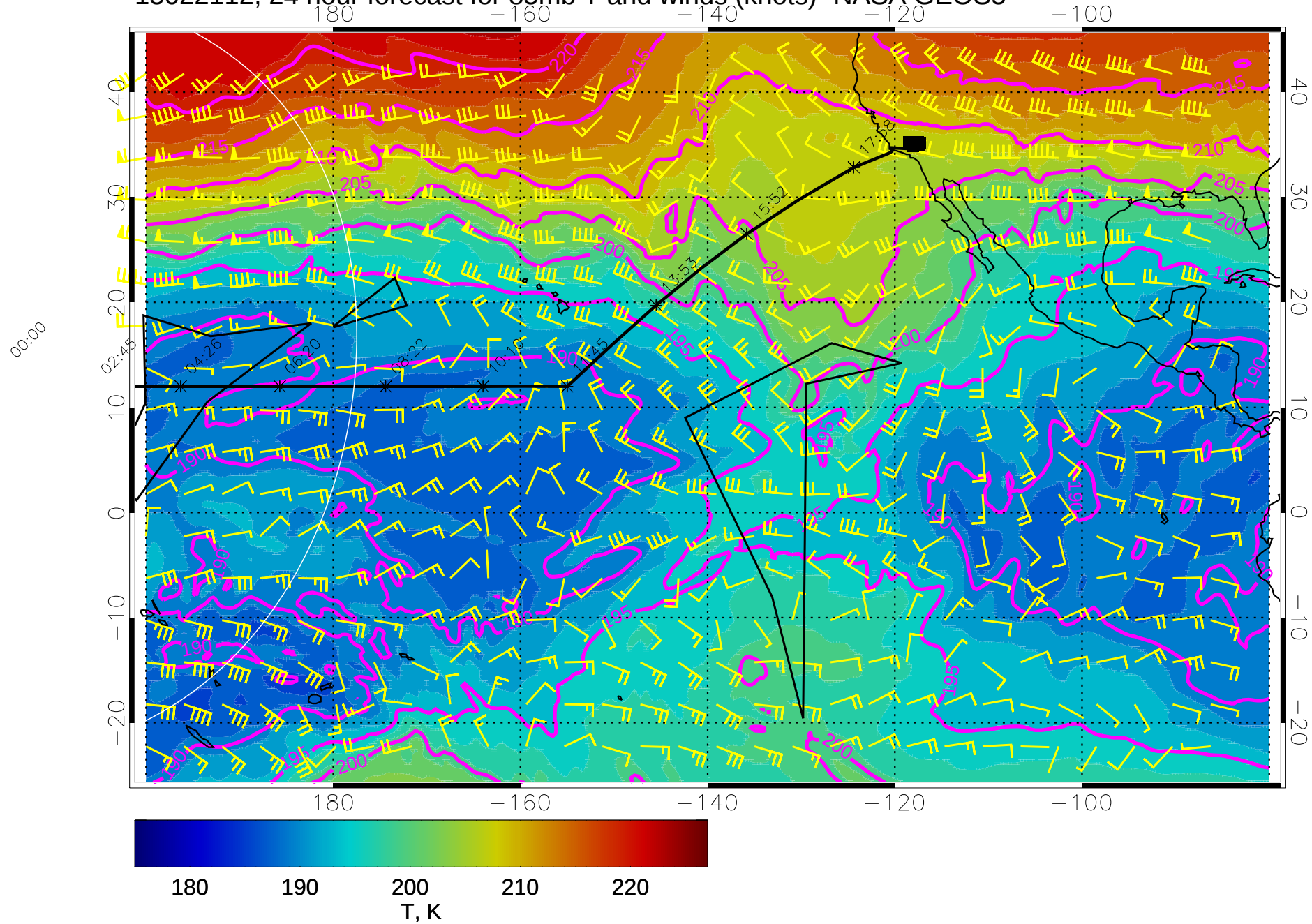
15022112, 24 hour forecast for 85mb T and winds (knots)- NASA GEOS5
