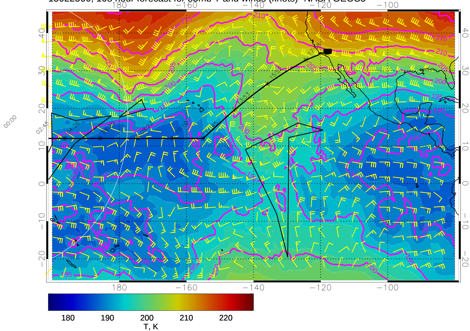
15022500, 108 hour forecast for 85mb T and winds (knots)- NASA GEOS5
