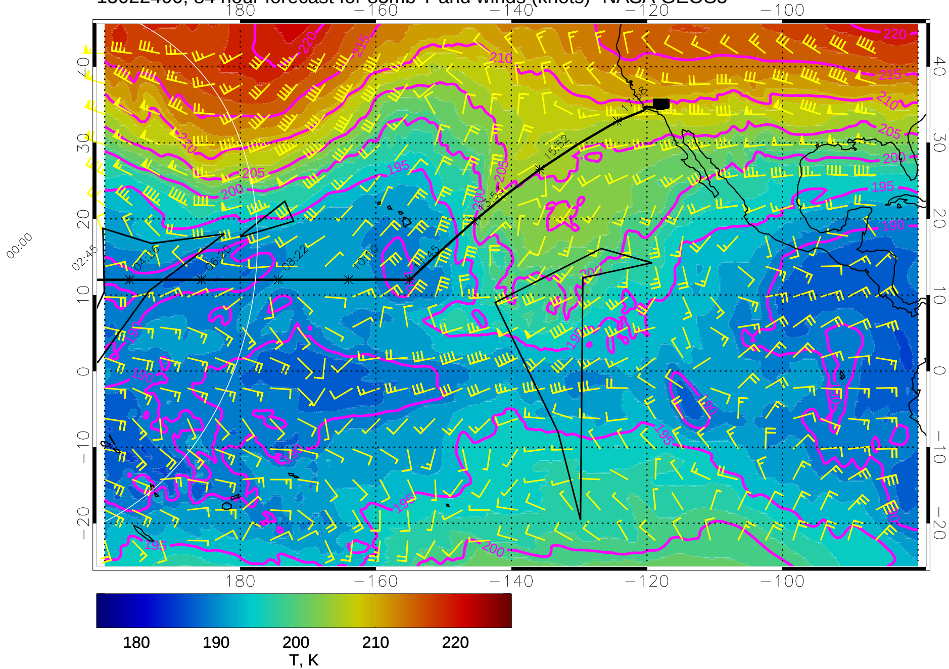
15022400, 84 hour forecast for 85mb T and winds (knots)- NASA GEOS5
