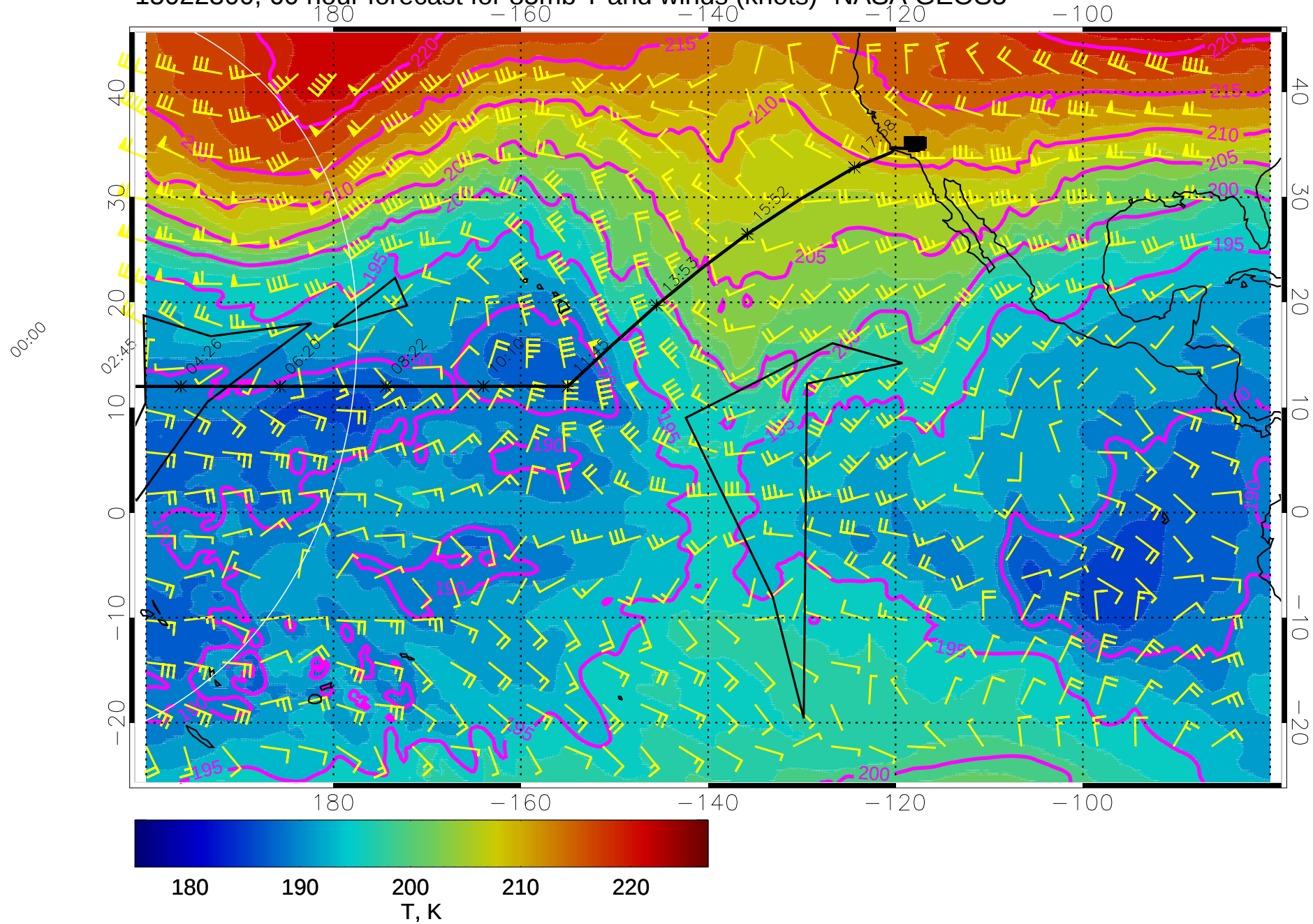
15022300, 60 hour forecast for 85mb T and winds (knots)- NASA GEOS5
