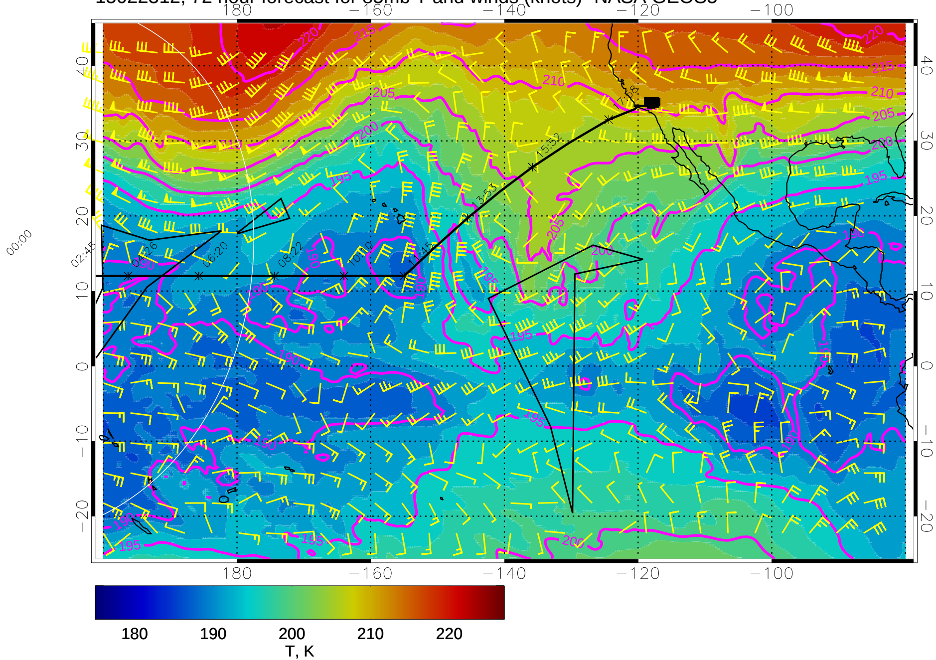
15022312, 72 hour forecast for 85mb T and winds (knots)- NASA GEOS5
