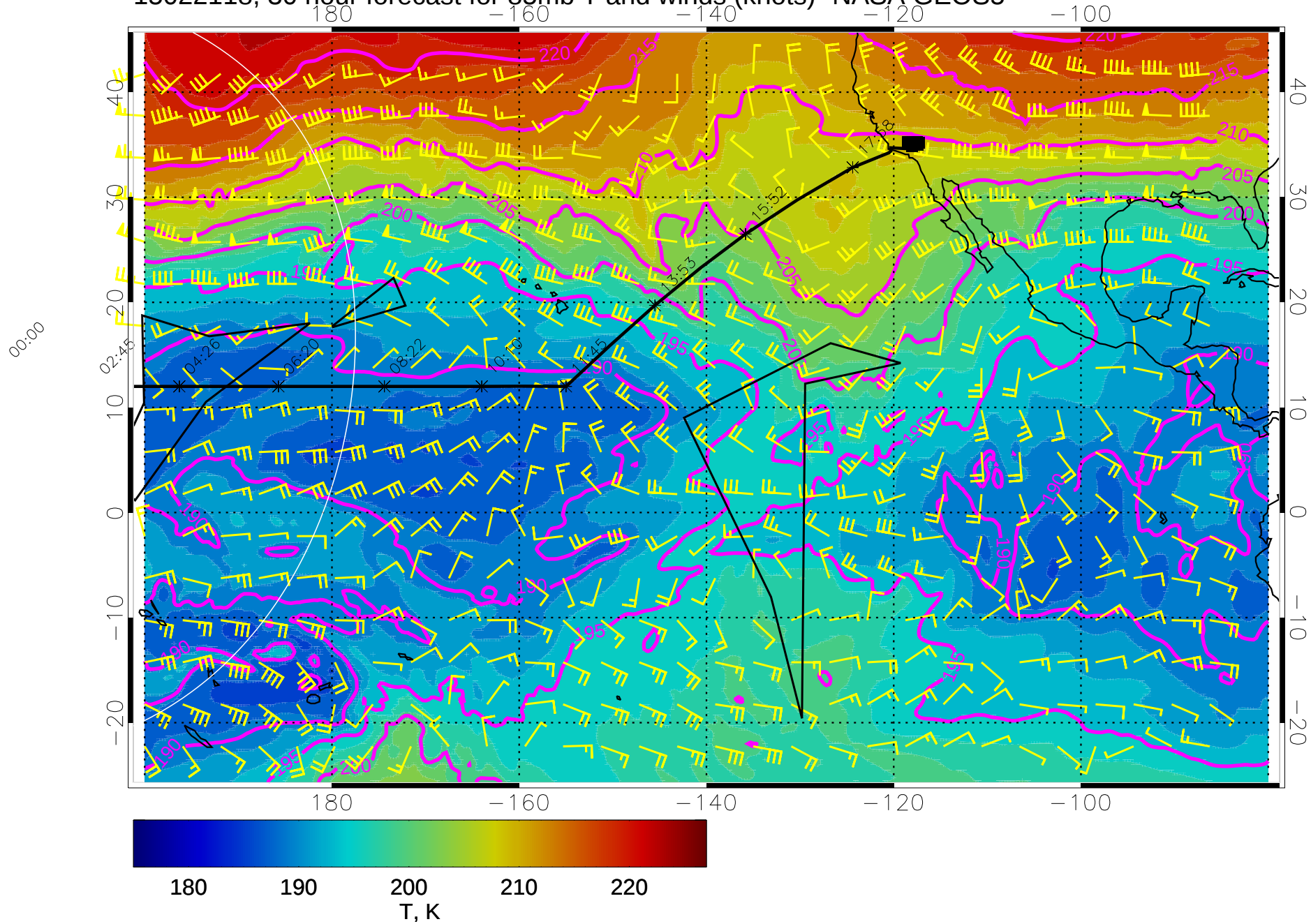
15022118, 30 hour forecast for 85mb T and winds (knots)- NASA GEOS5
