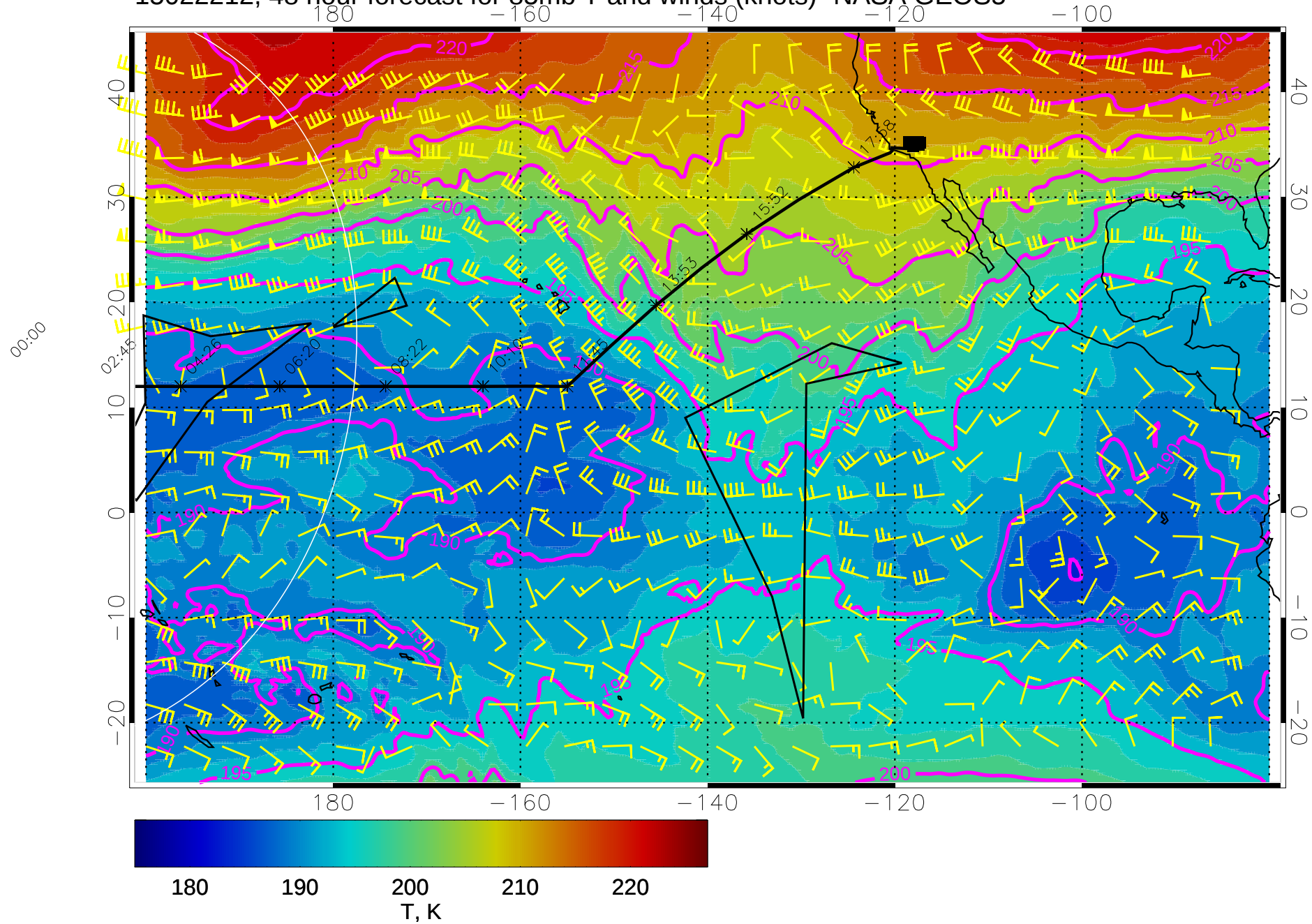
15022212, 48 hour forecast for 85mb T and winds (knots)- NASA GEOS5
