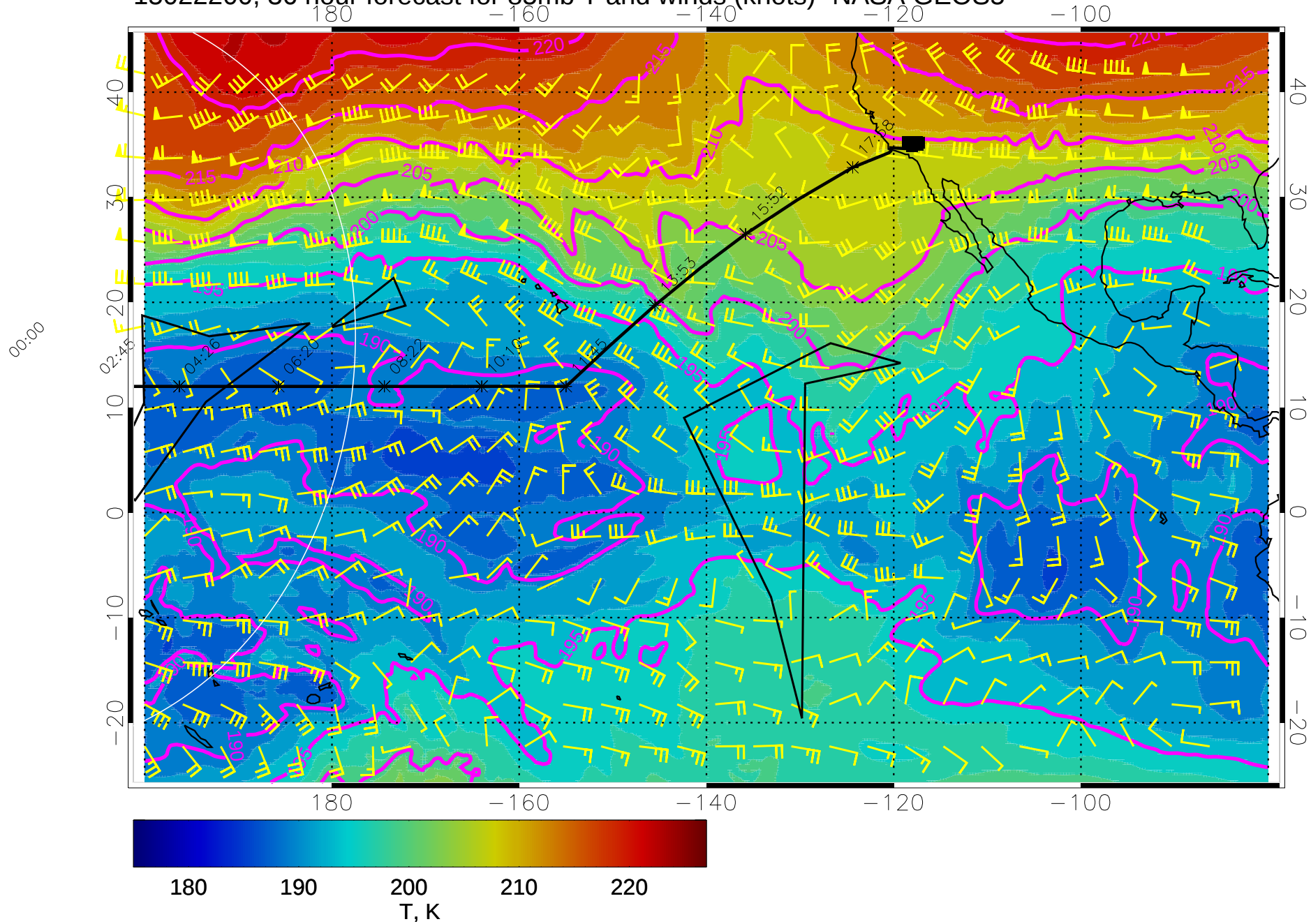
15022200, 36 hour forecast for 85mb T and winds (knots)- NASA GEOS5
