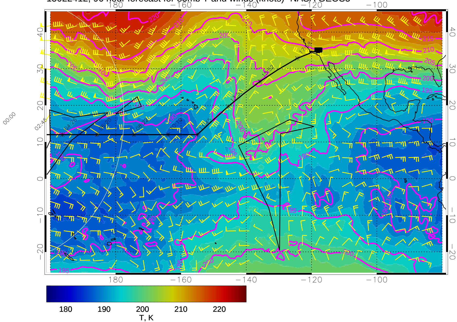
15022412, 96 hour forecast for 85mb T and winds (knots)- NASA GEOS5
