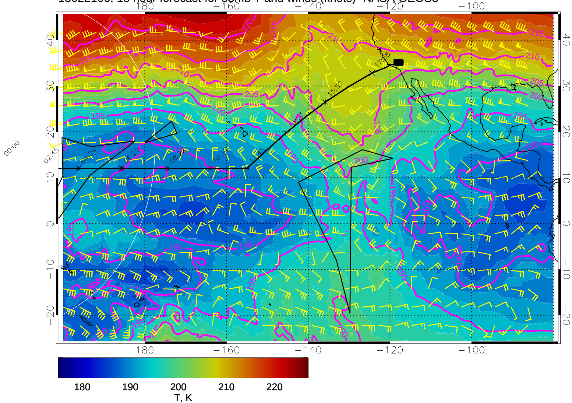
15022106, 18 hour forecast for 85mb T and winds (knots)- NASA GEOS5
