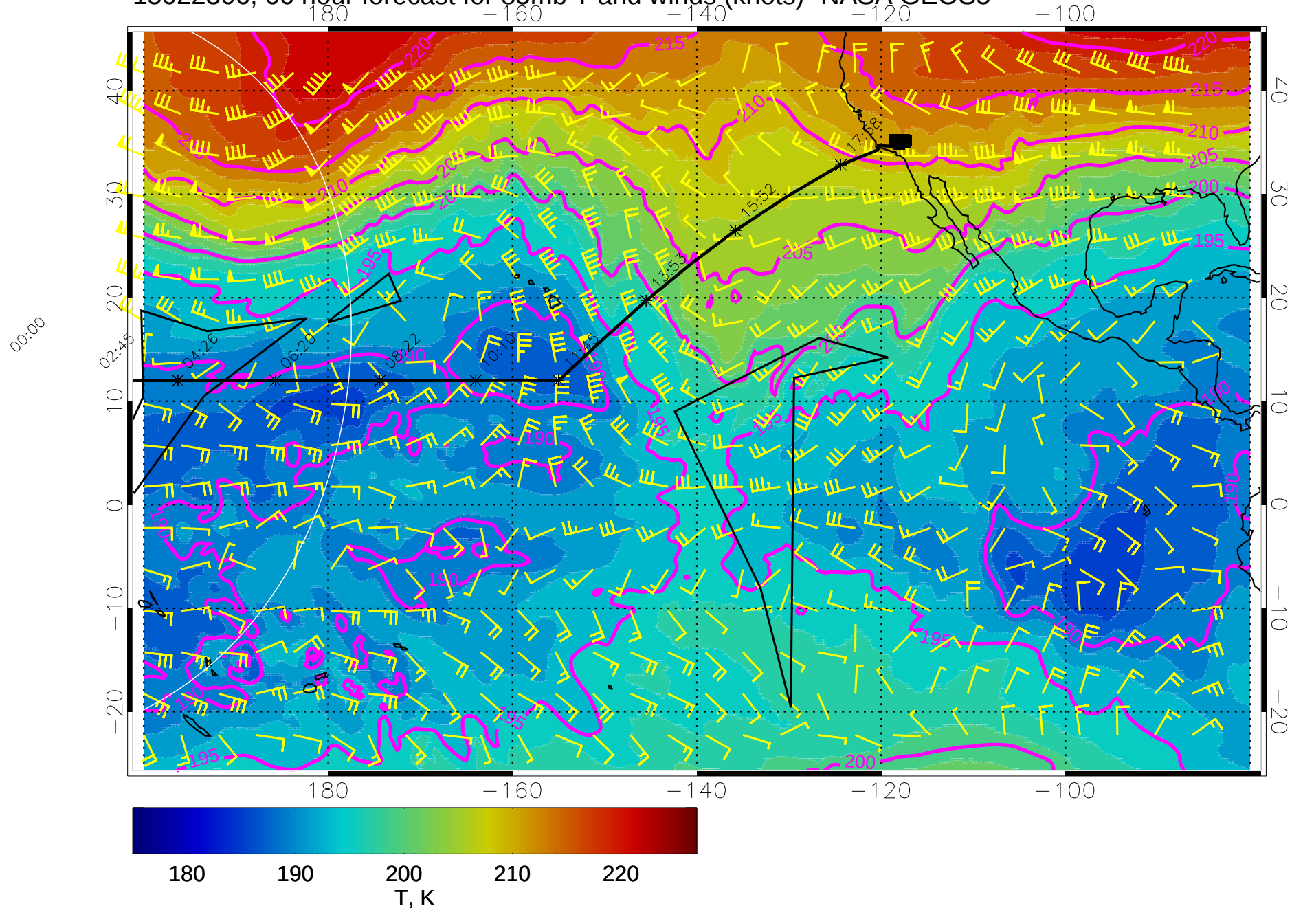
15022306, 66 hour forecast for 85mb T and winds (knots)- NASA GEOS5
