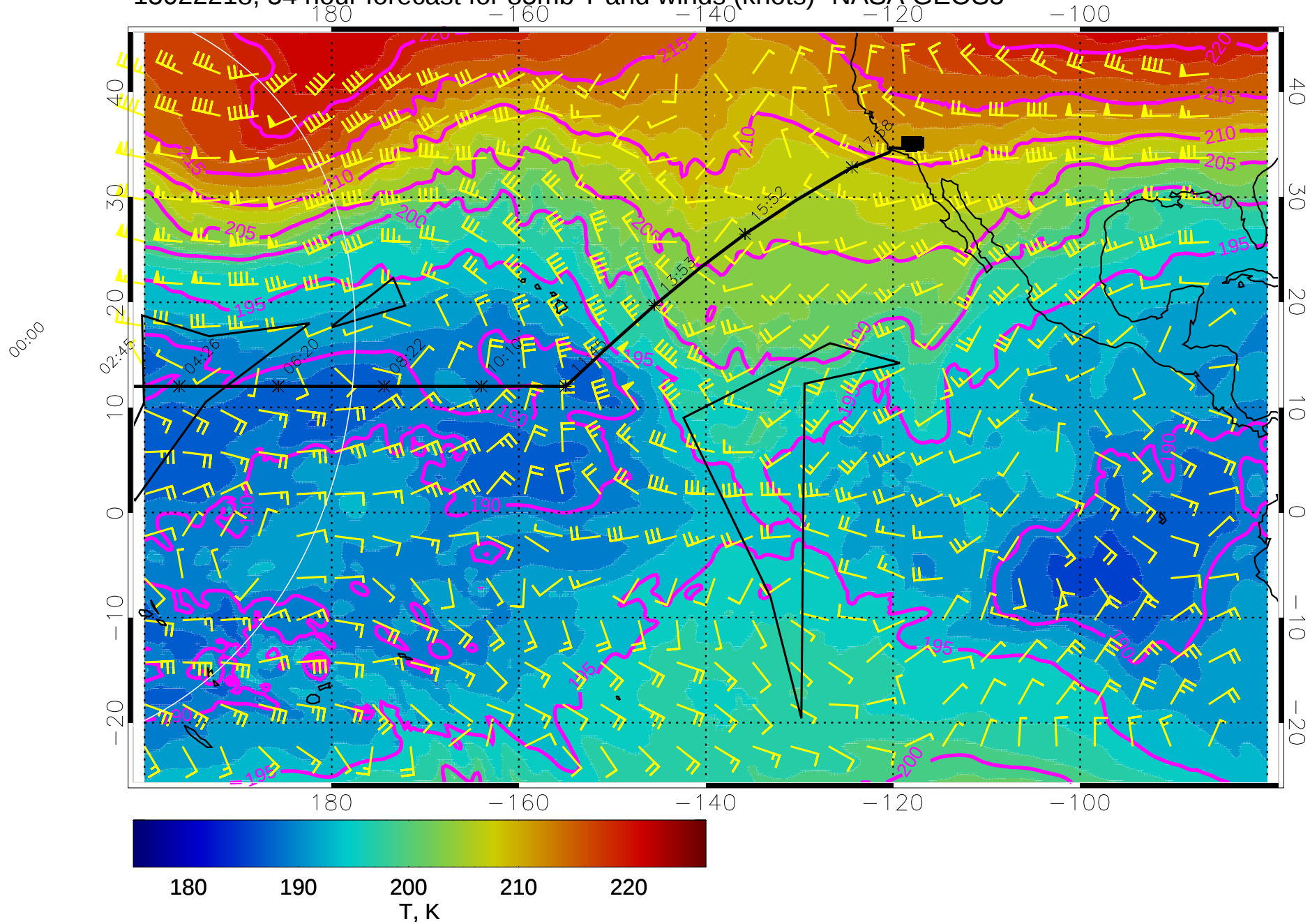
15022218, 54 hour forecast for 85mb T and winds (knots)- NASA GEOS5
