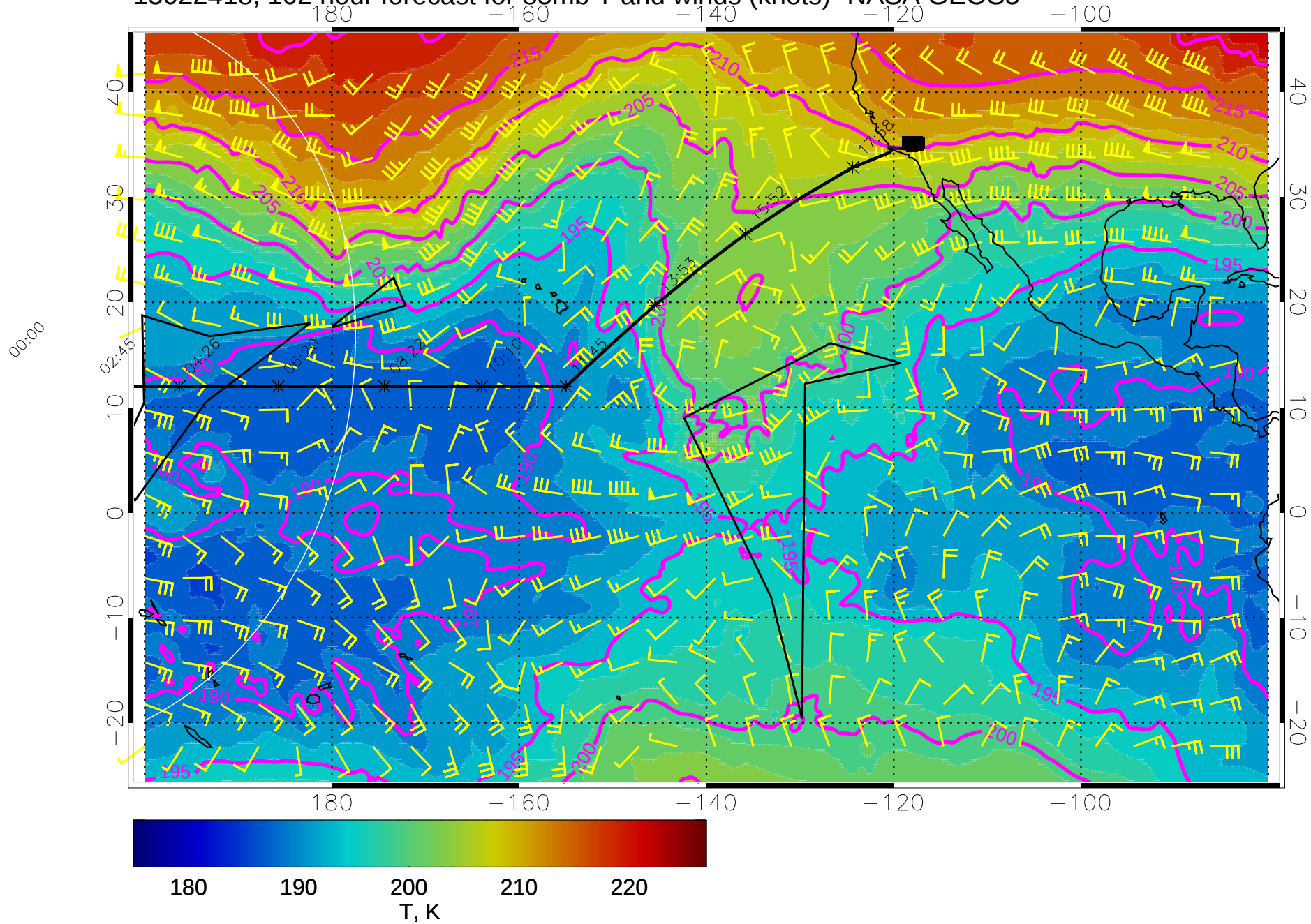
15022418, 102 hour forecast for 85mb T and winds (knots)- NASA GEOS5
