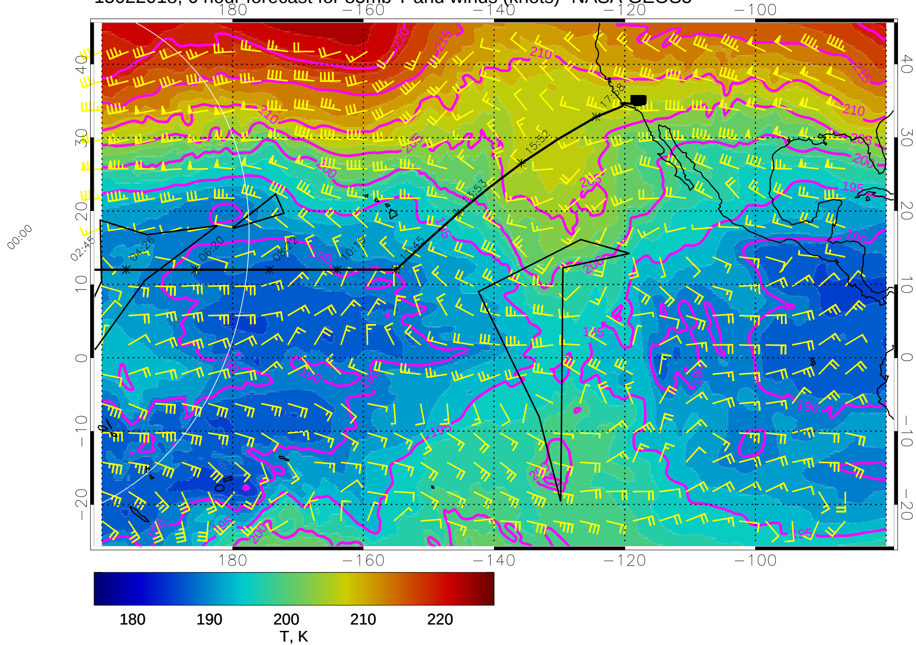
15022018, 6 hour forecast for 85mb T and winds (knots)- NASA GEOS5
