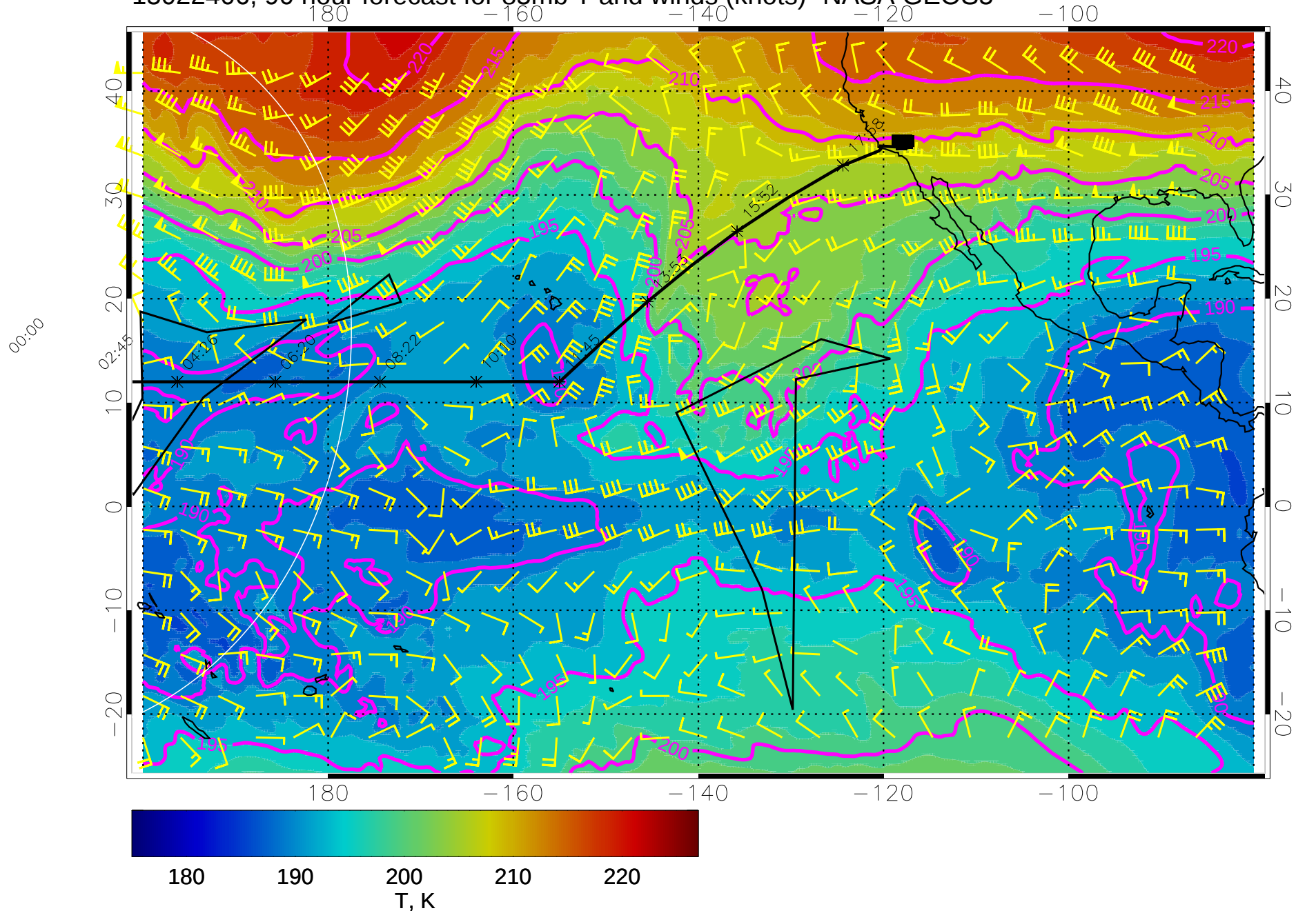
15022406, 90 hour forecast for 85mb T and winds (knots)- NASA GEOS5
