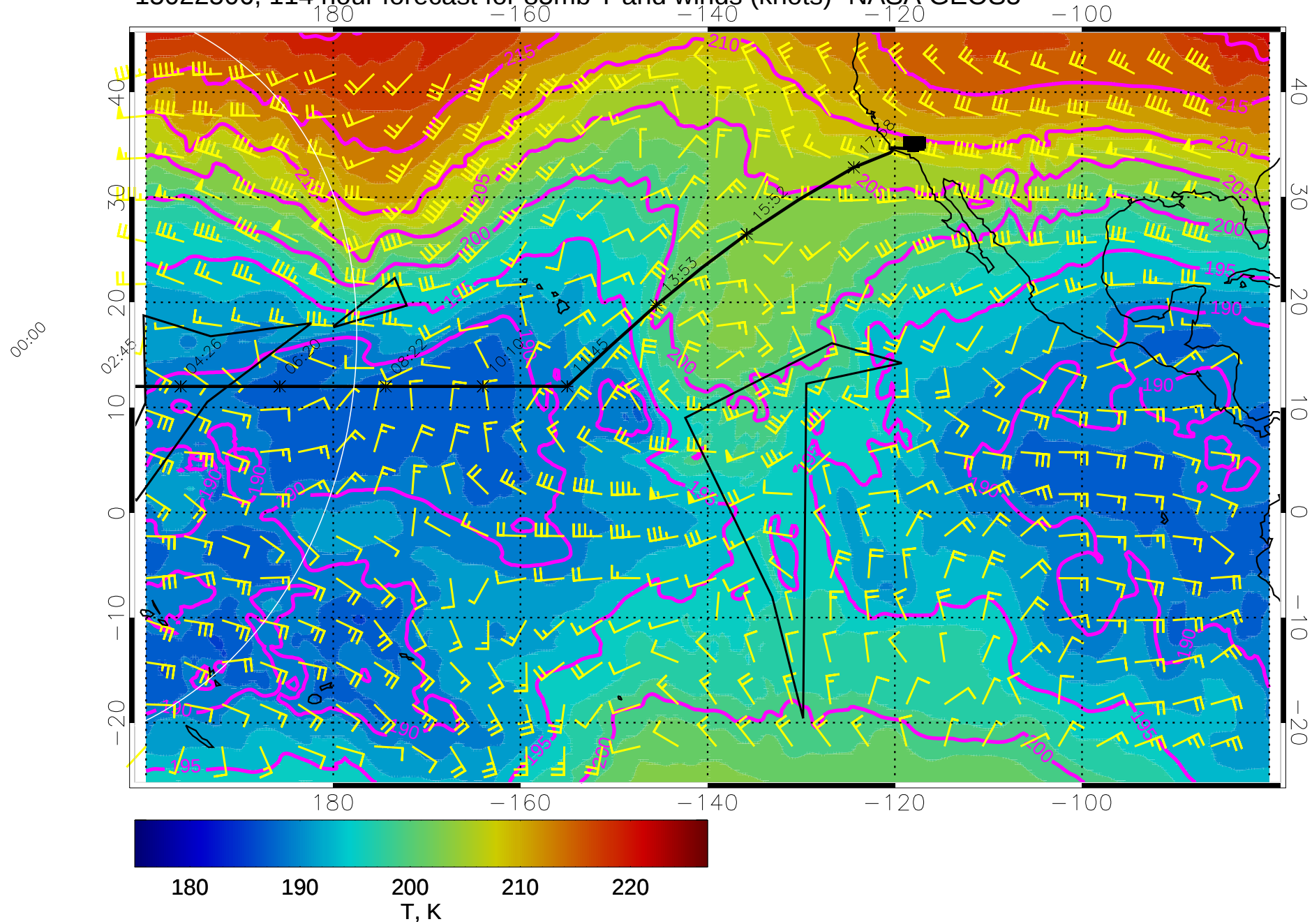
15022506, 114 hour forecast for 85mb T and winds (knots)- NASA GEOS5
