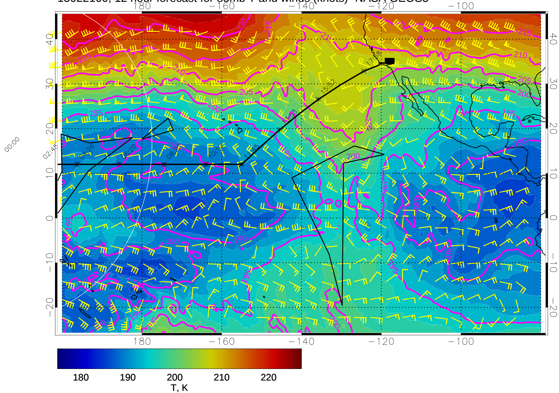
15022100, 12 hour forecast for 85mb T and winds (knots)- NASA GEOS5
