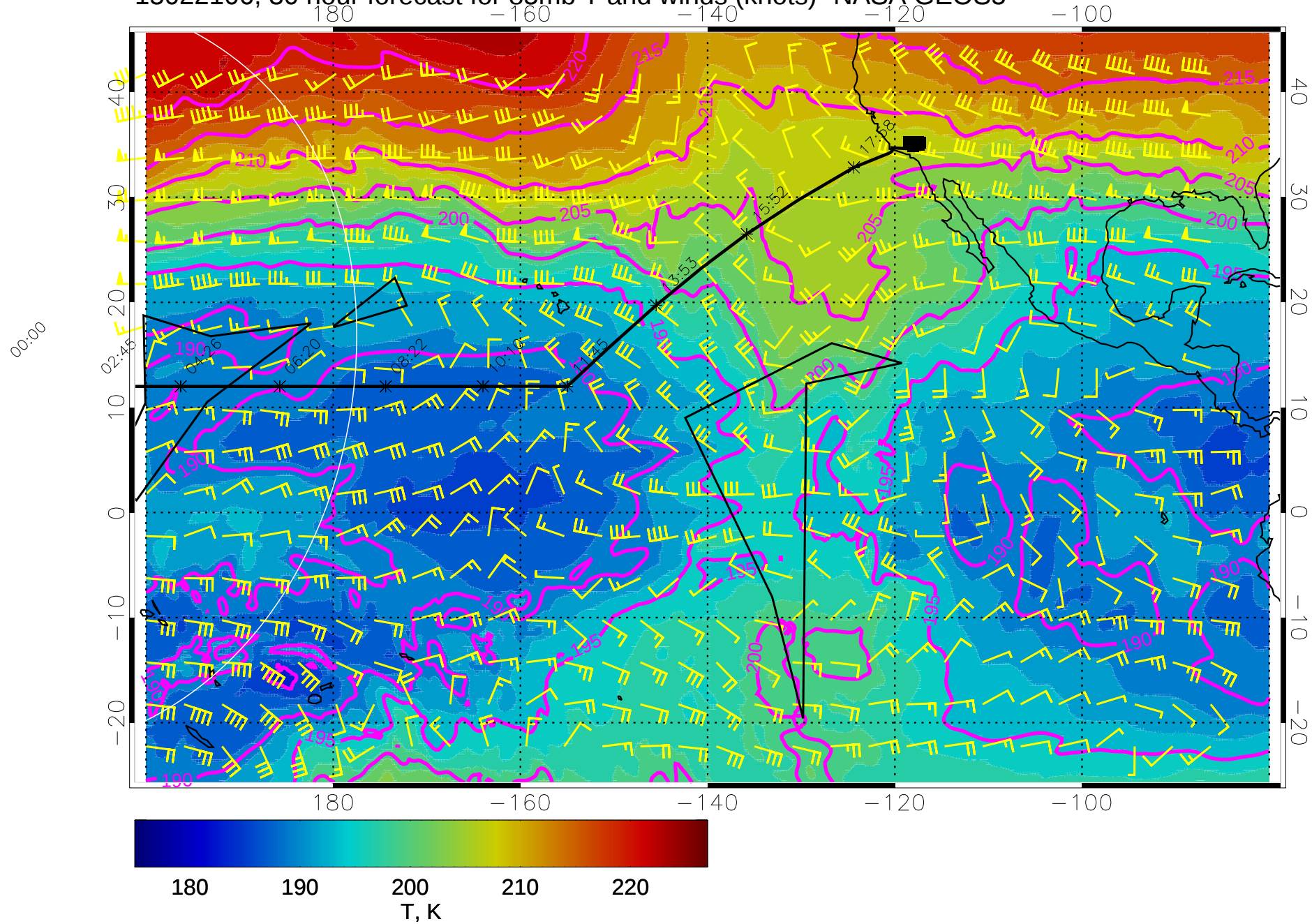
15022106, 30 hour forecast for 85mb T and winds (knots)- NASA GEOS5
