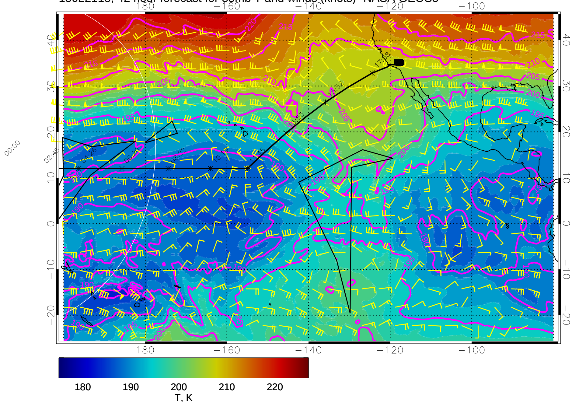
15022118, 42 hour forecast for 85mb T and winds (knots)- NASA GEOS5
