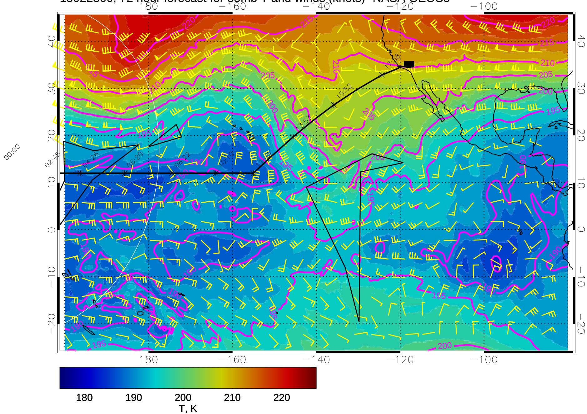
15022300, 72 hour forecast for 85mb T and winds (knots)- NASA GEOS5
