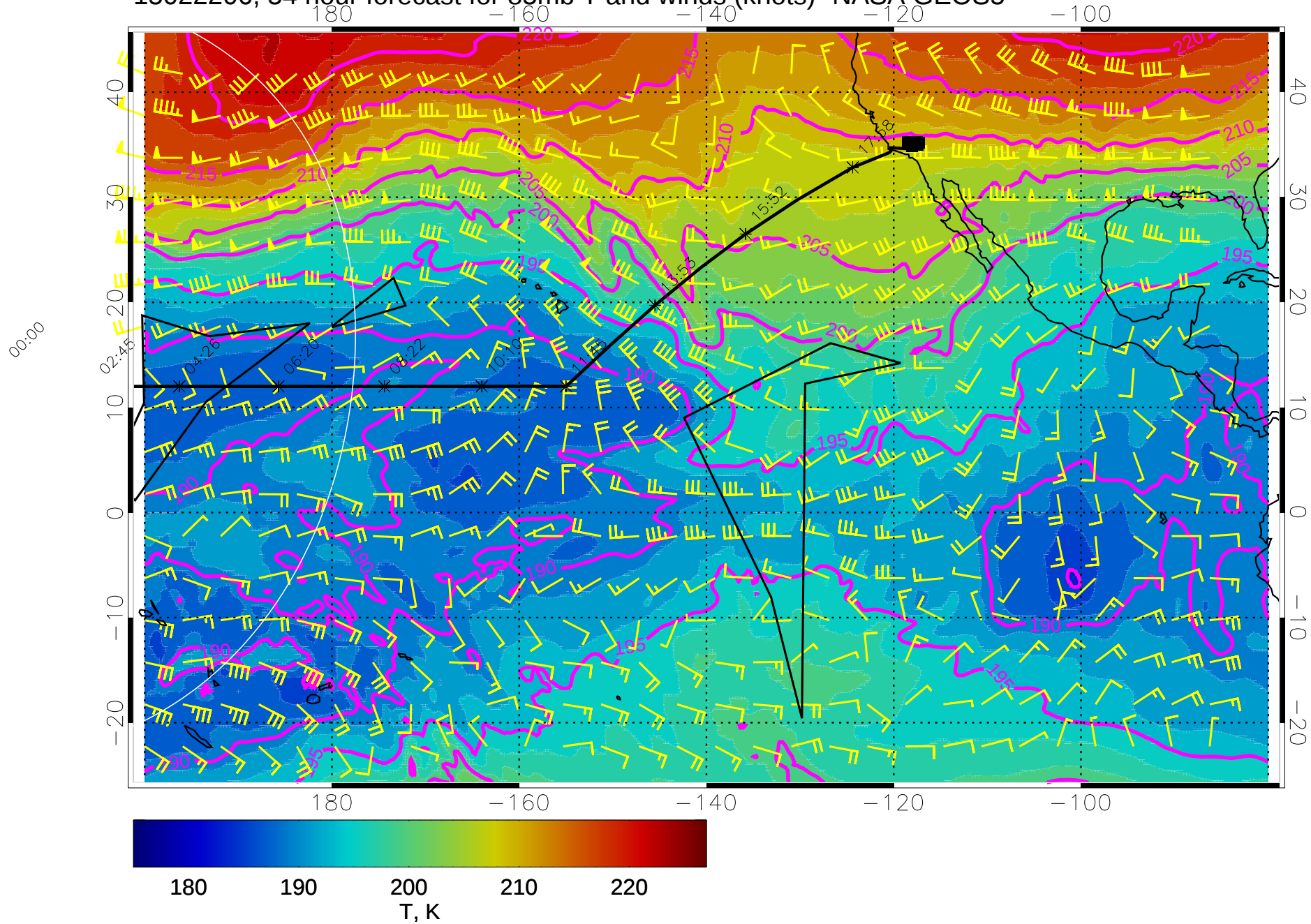
15022206, 54 hour forecast for 85mb T and winds (knots)- NASA GEOS5
