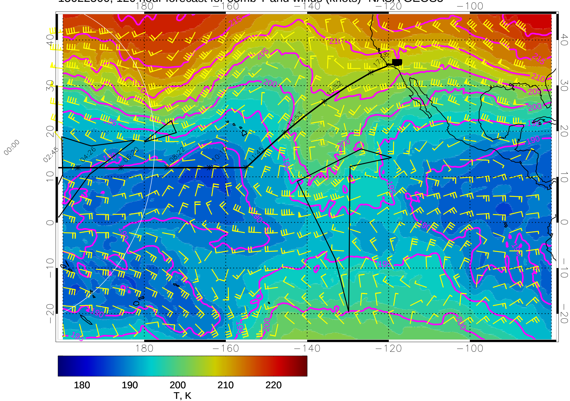
15022500, 120 hour forecast for 85mb T and winds (knots)- NASA GEOS5
