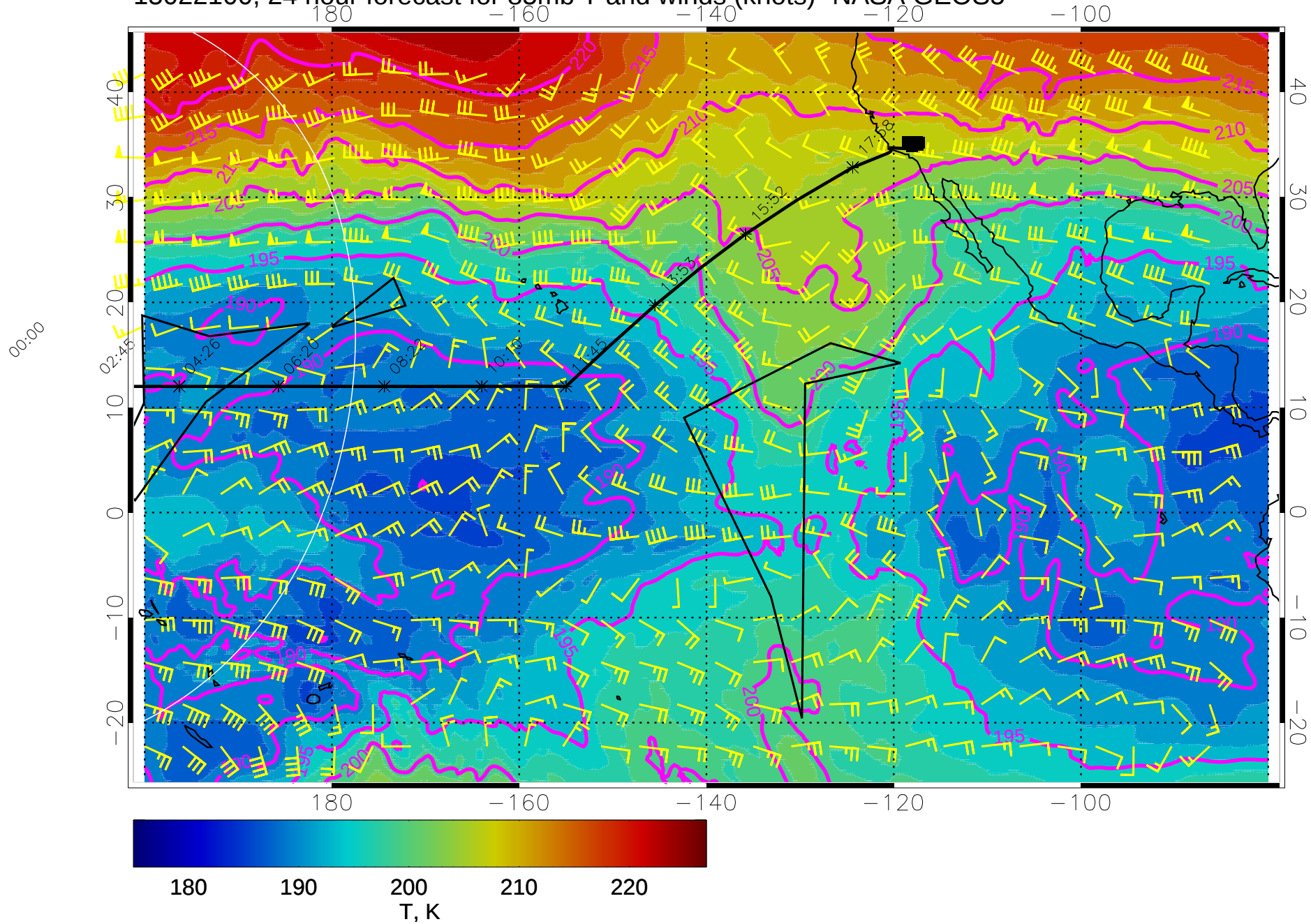
15022100, 24 hour forecast for 85mb T and winds (knots)- NASA GEOS5
