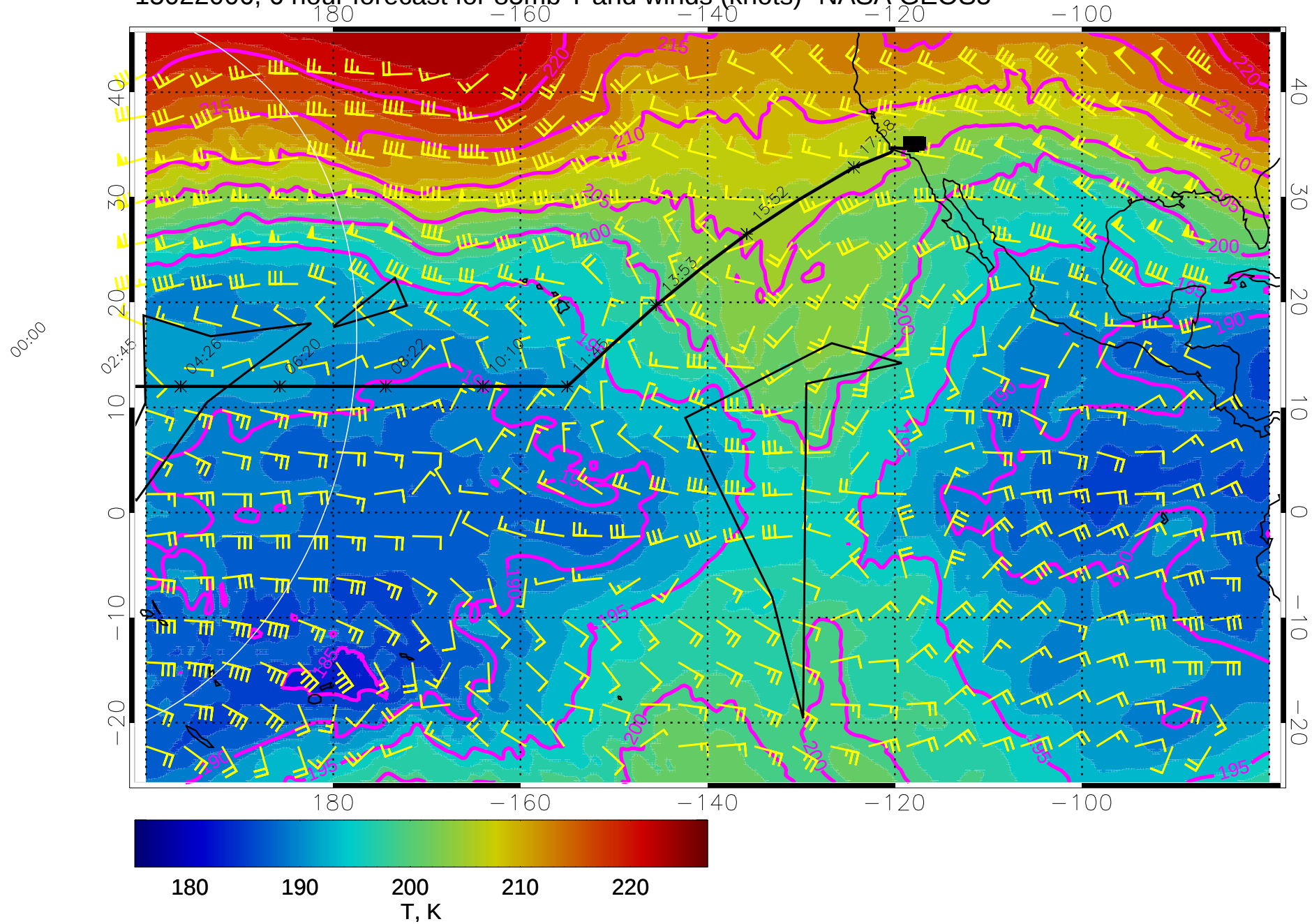
15022006, 6 hour forecast for 85mb T and winds (knots)- NASA GEOS5
