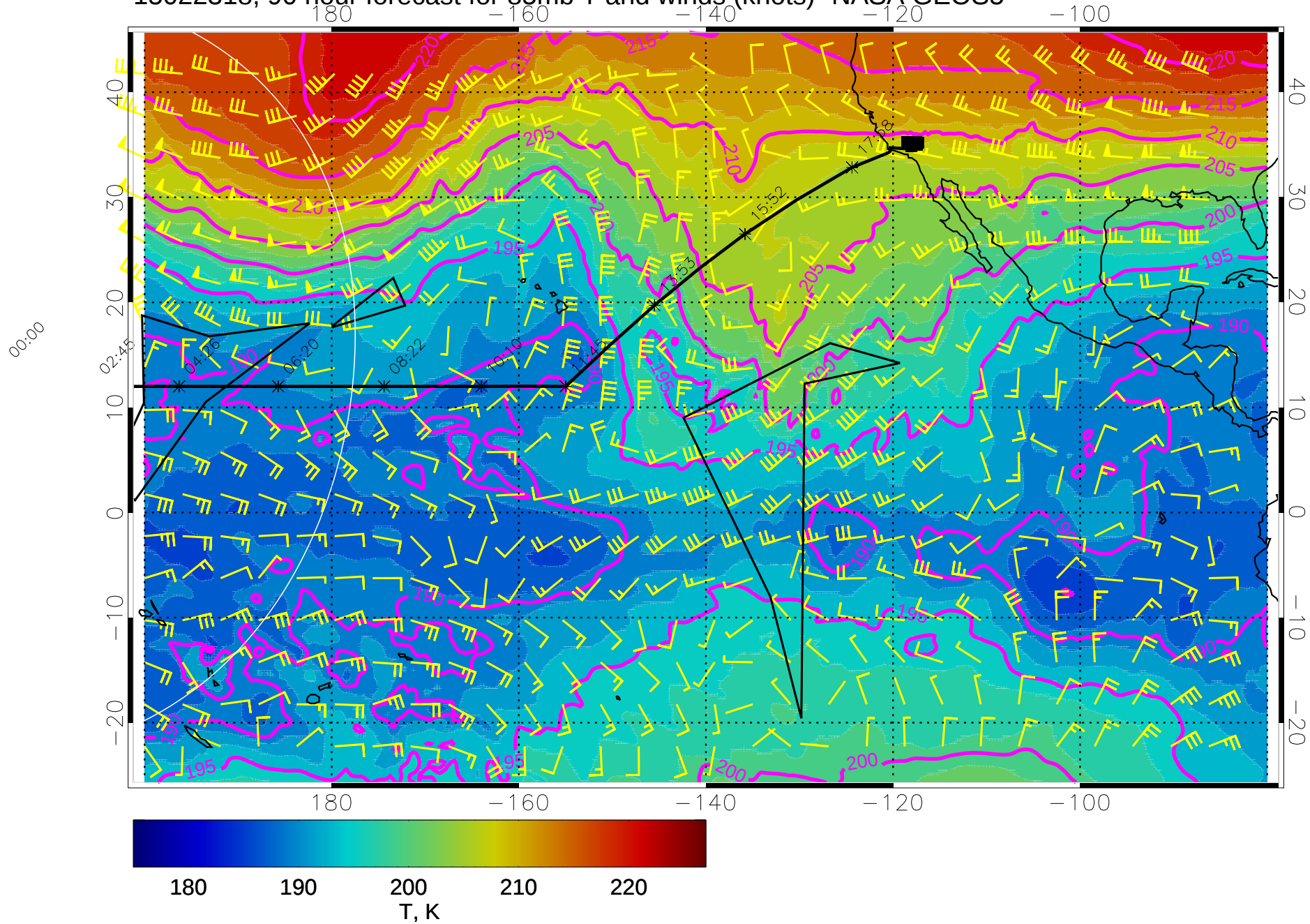
15022318, 90 hour forecast for 85mb T and winds (knots)- NASA GEOS5
