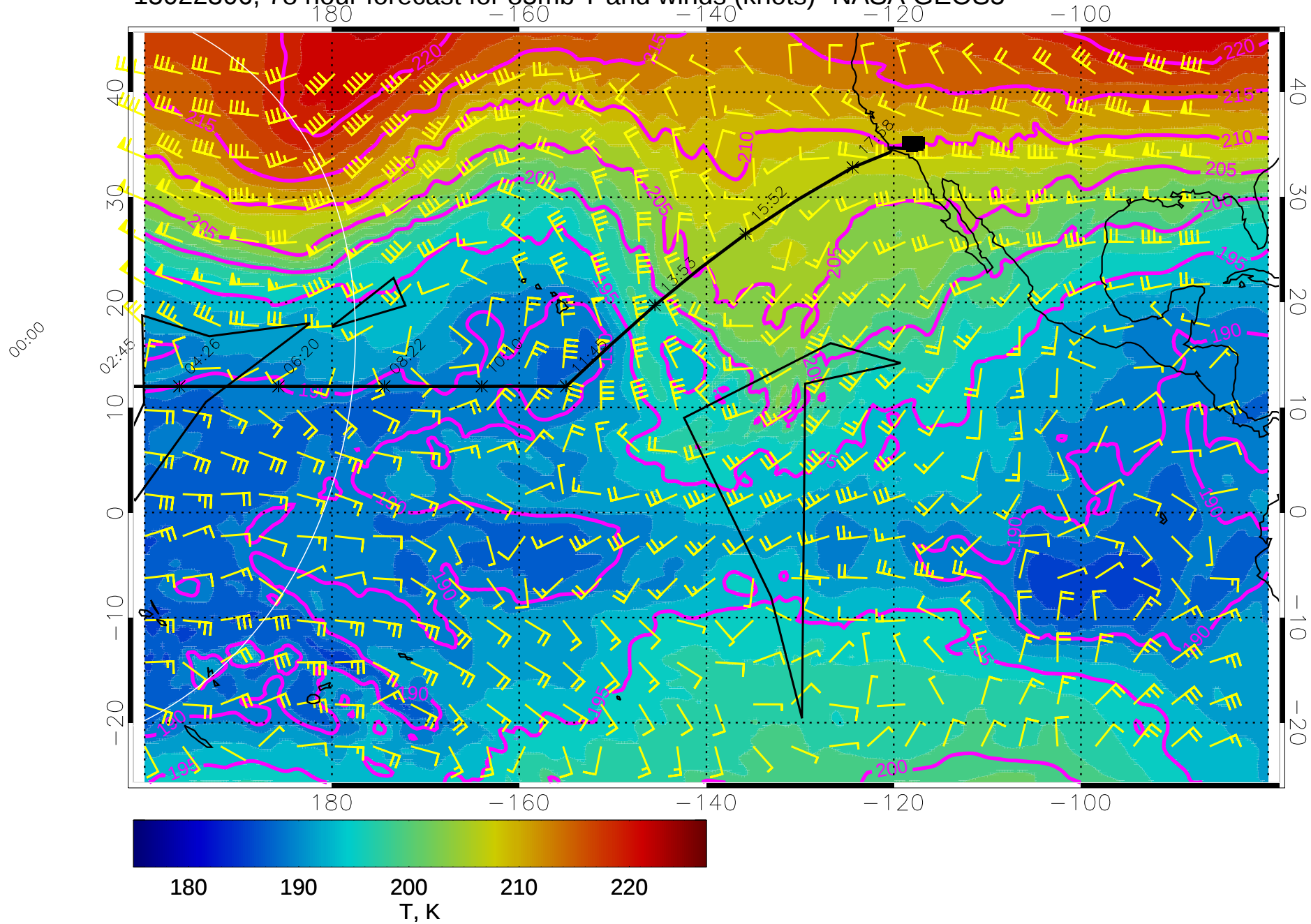
15022306, 78 hour forecast for 85mb T and winds (knots)- NASA GEOS5
