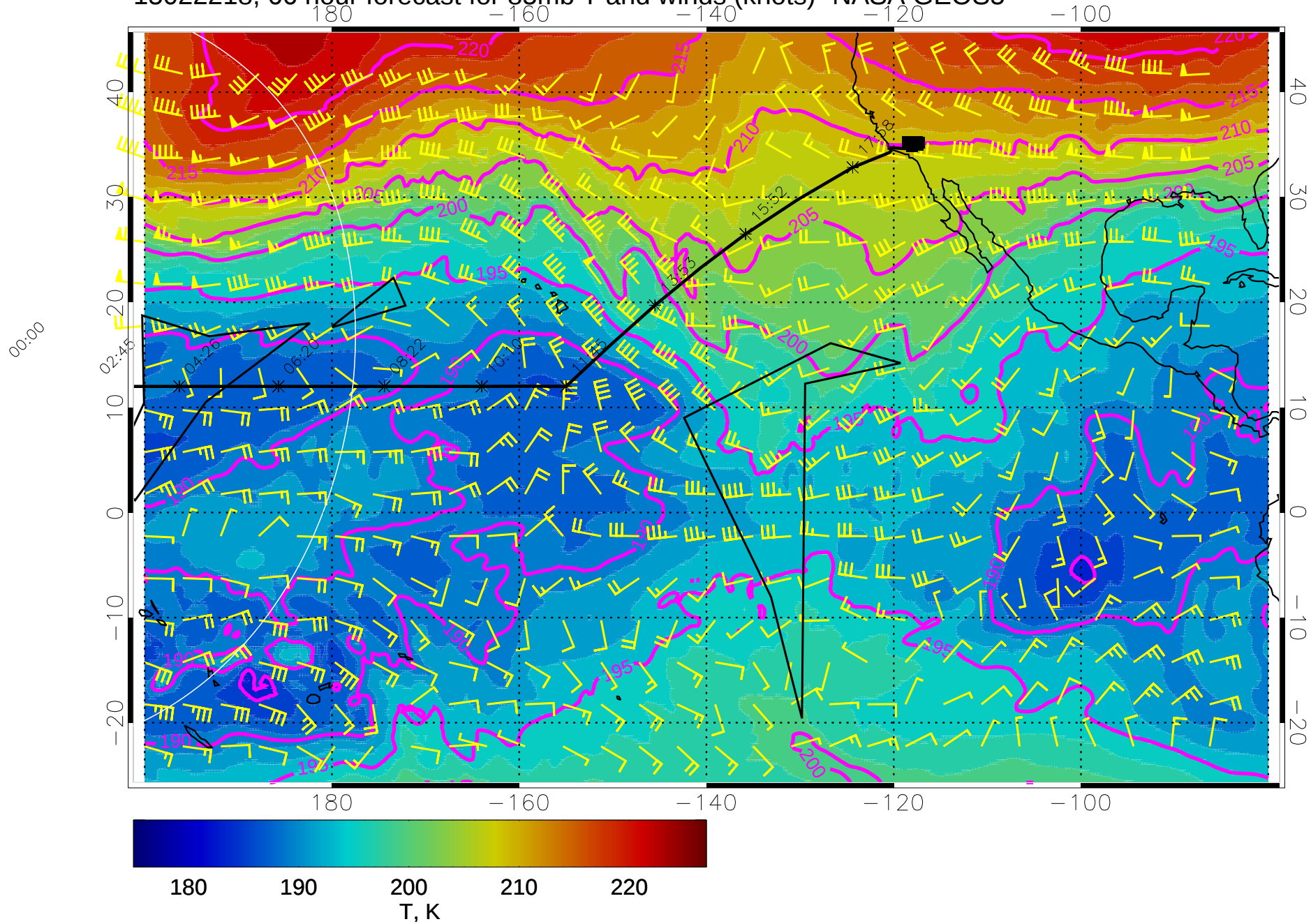
15022218, 66 hour forecast for 85mb T and winds (knots)- NASA GEOS5
