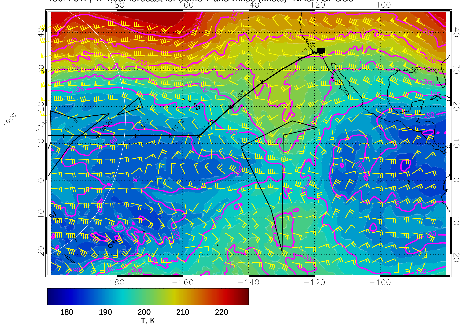
15022012, 12 hour forecast for 85mb T and winds (knots)- NASA GEOS5
