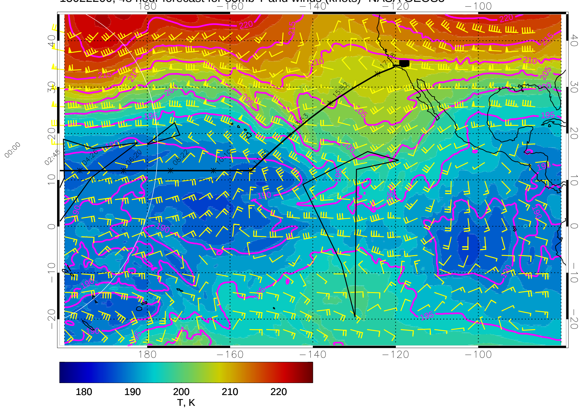
15022200, 48 hour forecast for 85mb T and winds (knots)- NASA GEOS5
