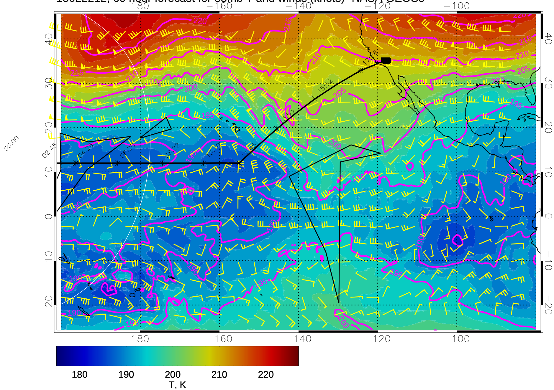
15022212, 60 hour forecast for 85mb T and winds (knots)- NASA GEOS5
