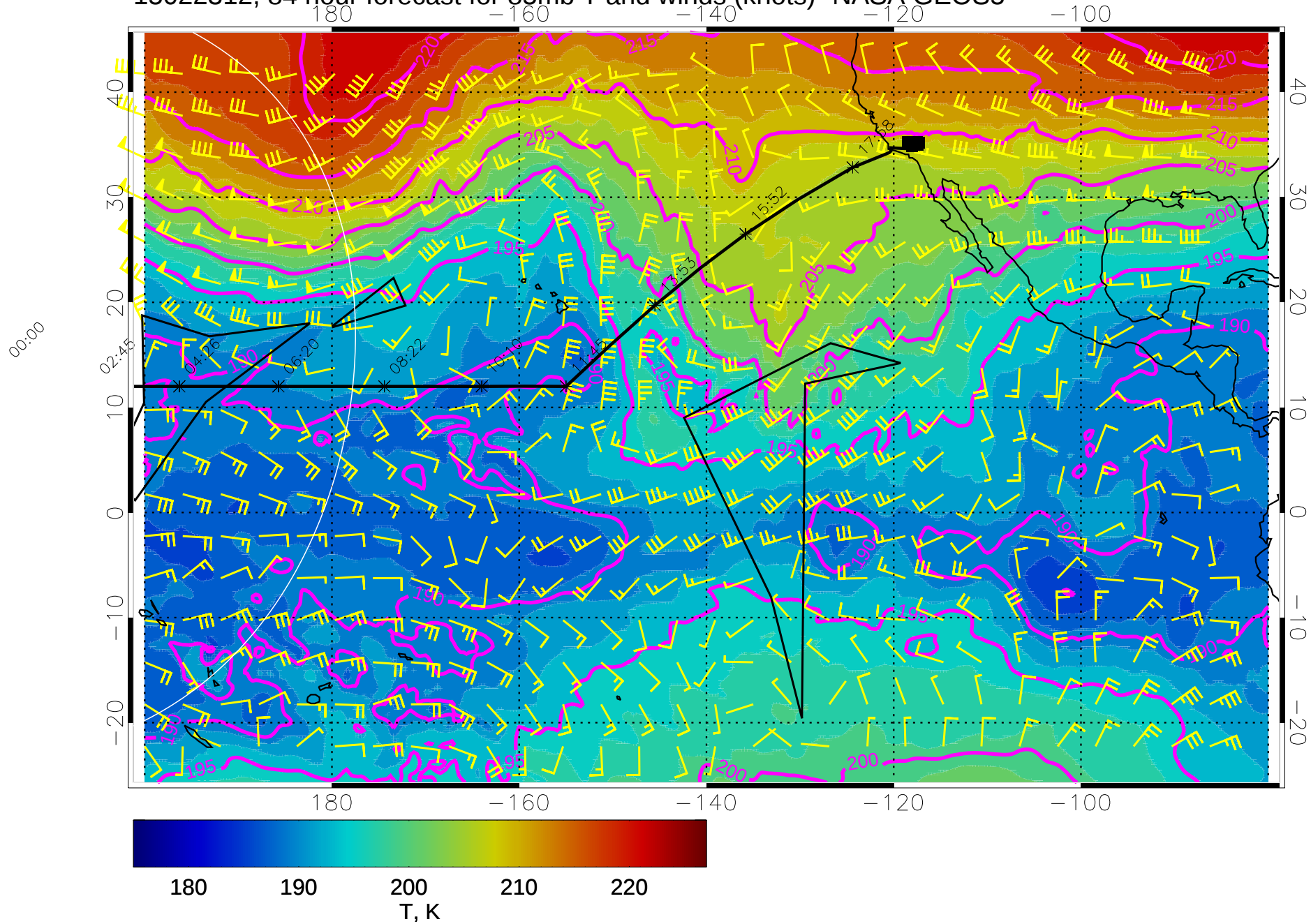
15022312, 84 hour forecast for 85mb T and winds (knots)- NASA GEOS5
