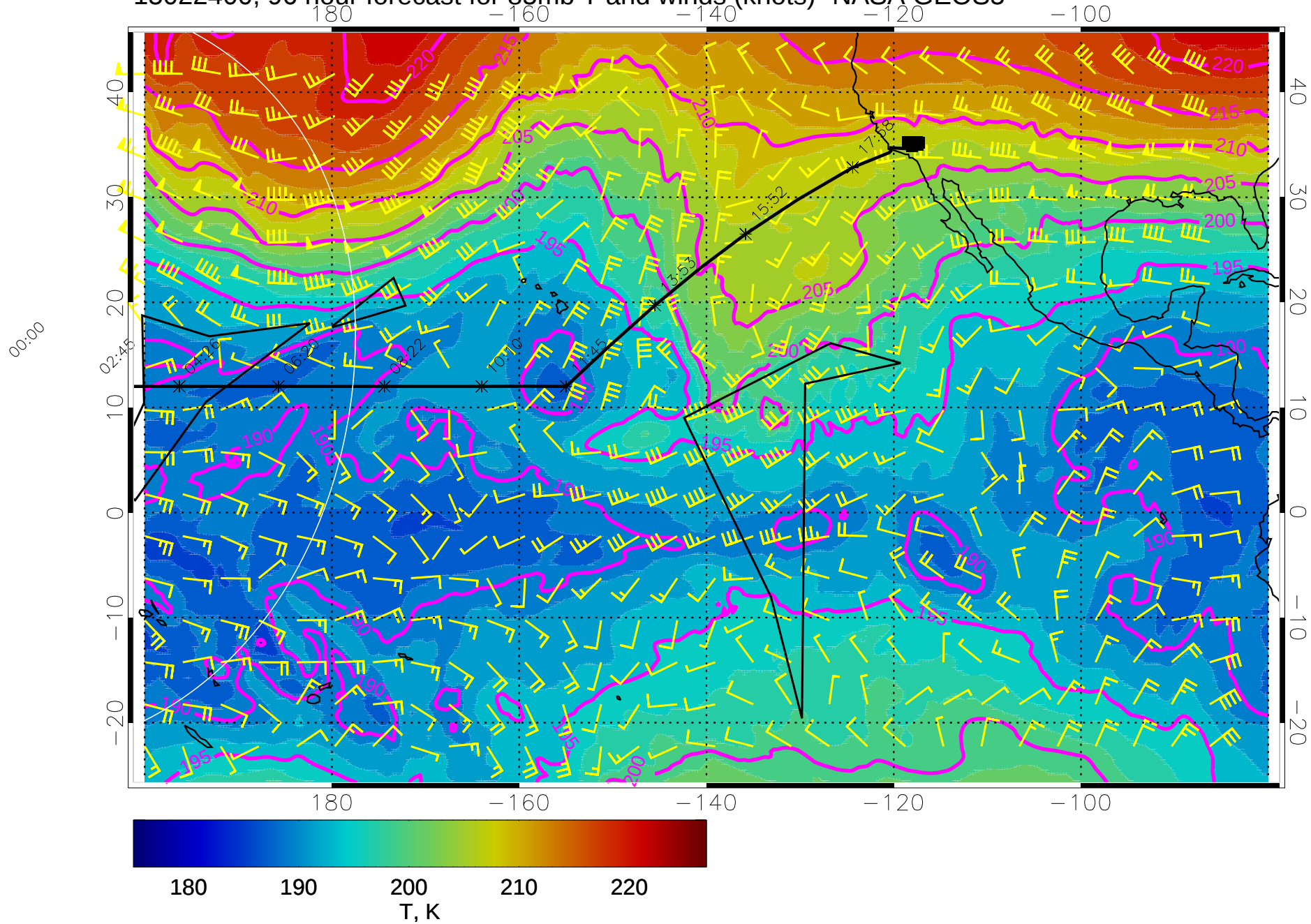
15022400, 96 hour forecast for 85mb T and winds (knots)- NASA GEOS5
