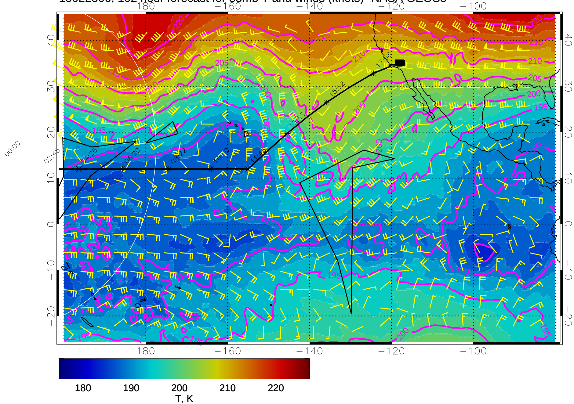
15022306, 102 hour forecast for 85mb T and winds (knots)- NASA GEOS5
