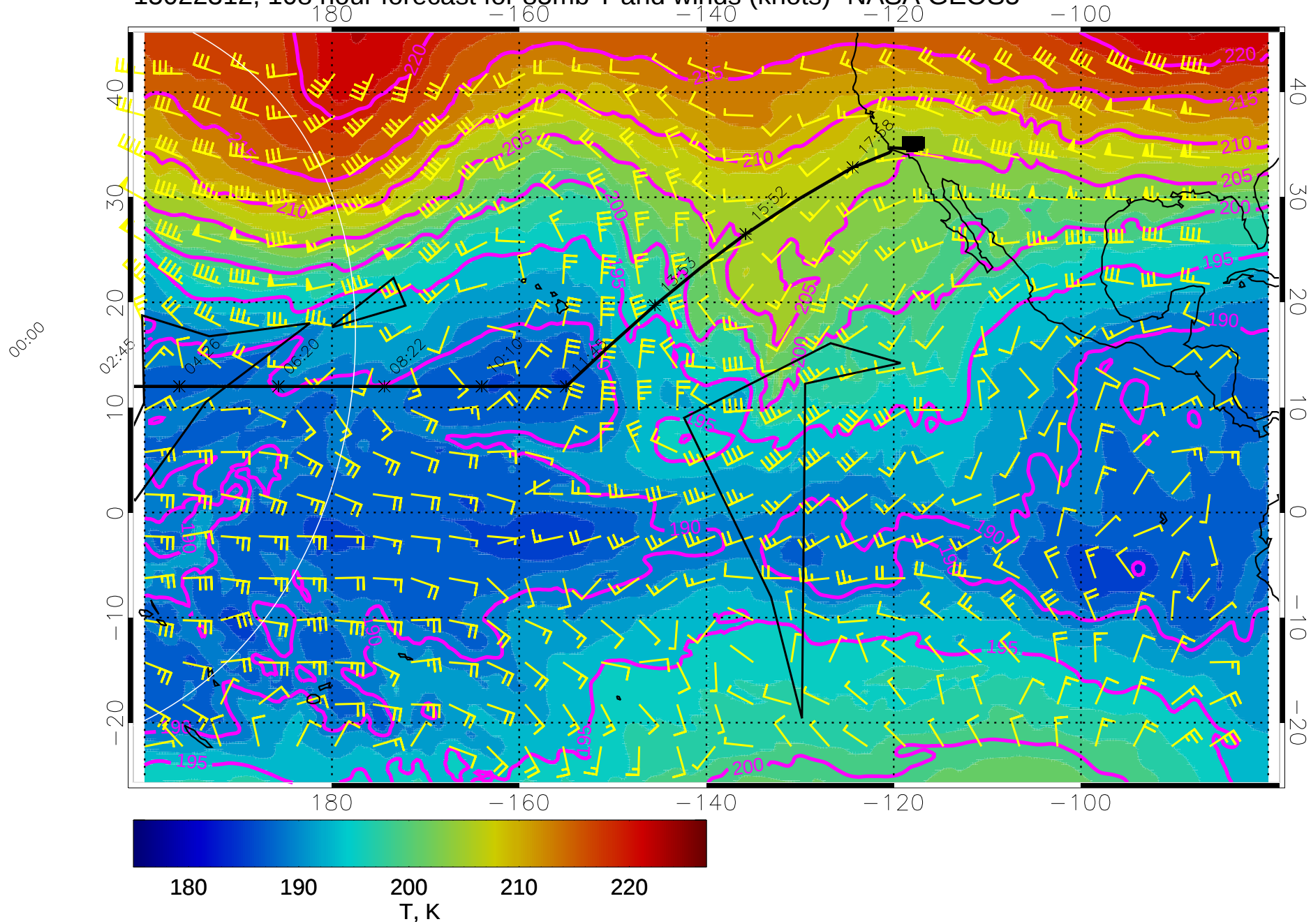
15022312, 108 hour forecast for 85mb T and winds (knots)- NASA GEOS5
