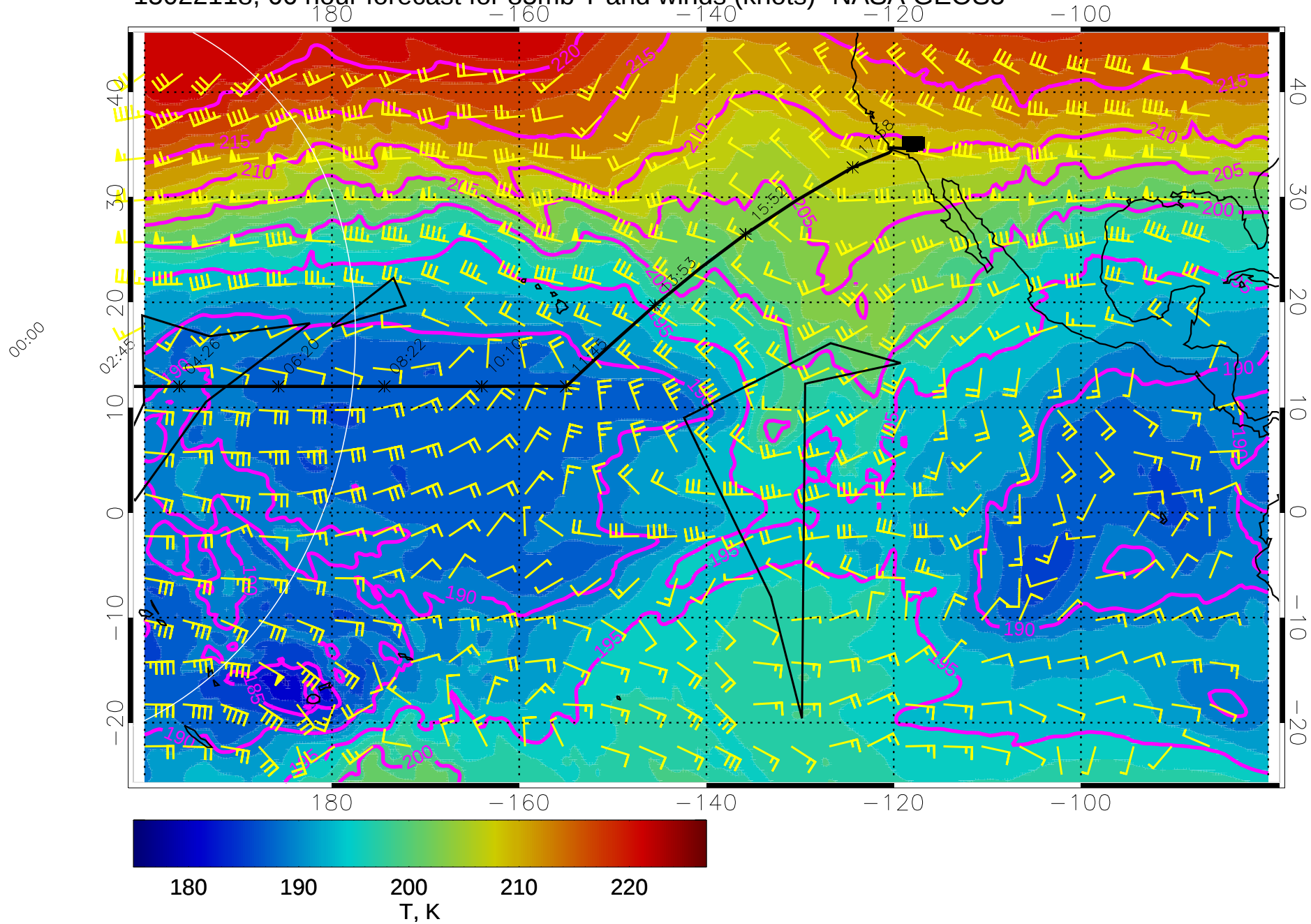
15022118, 66 hour forecast for 85mb T and winds (knots)- NASA GEOS5
