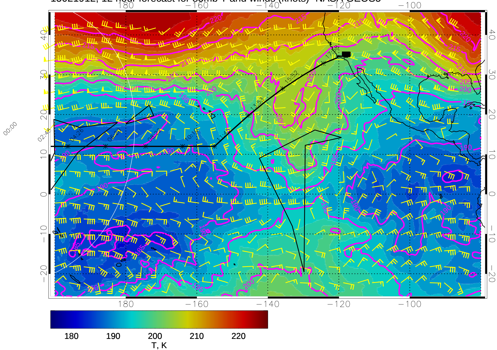
15021912, 12 hour forecast for 85mb T and winds (knots)- NASA GEOS5
