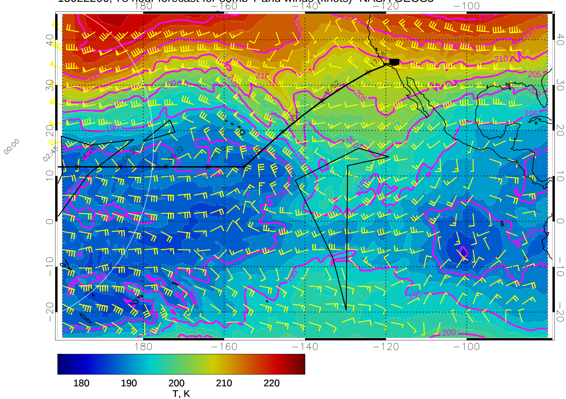
15022206, 78 hour forecast for 85mb T and winds (knots)- NASA GEOS5
