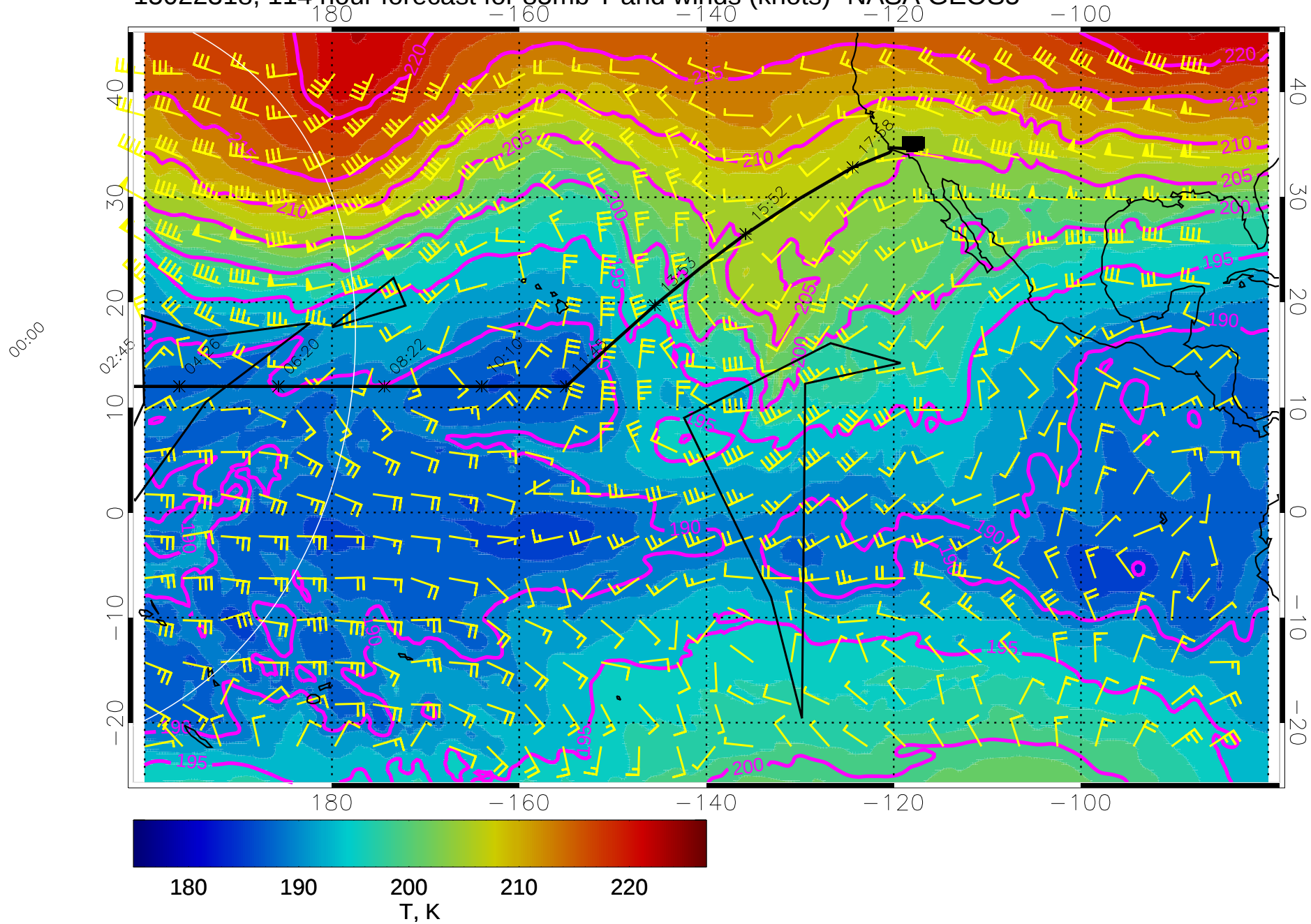
15022318, 114 hour forecast for 85mb T and winds (knots)- NASA GEOS5
