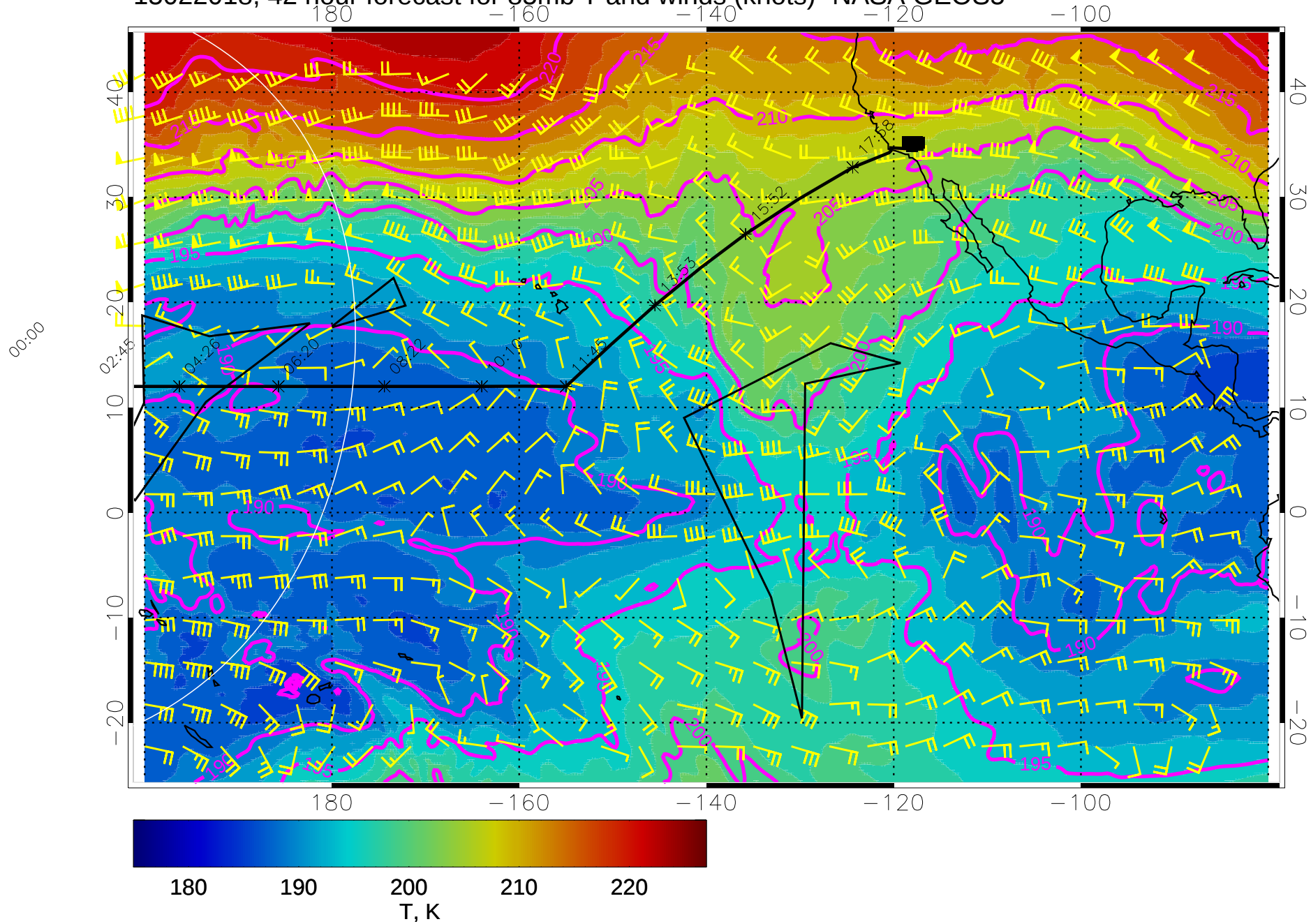
15022018, 42 hour forecast for 85mb T and winds (knots)- NASA GEOS5
