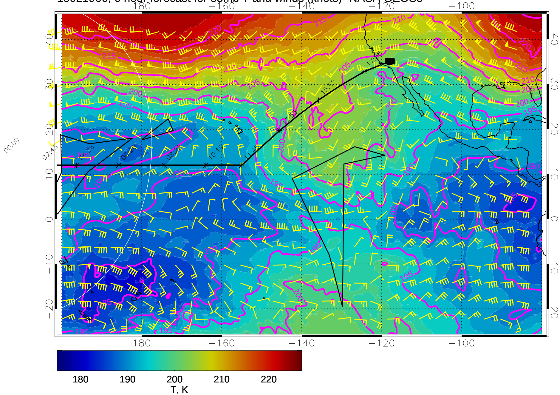
15021906, 6 hour forecast for 85mb T and winds (knots)- NASA GEOS5
