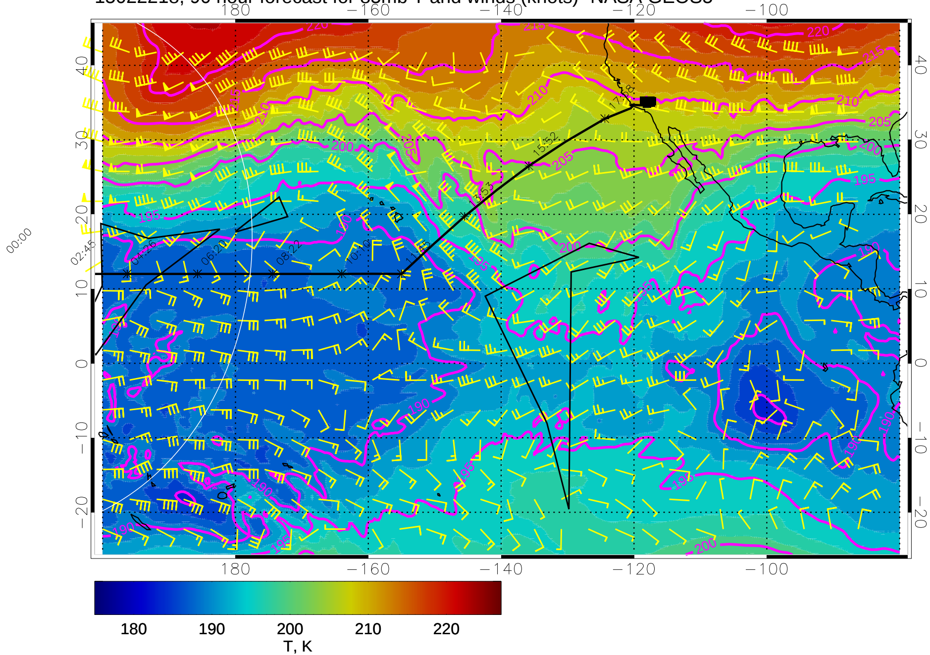
15022218, 90 hour forecast for 85mb T and winds (knots)- NASA GEOS5
