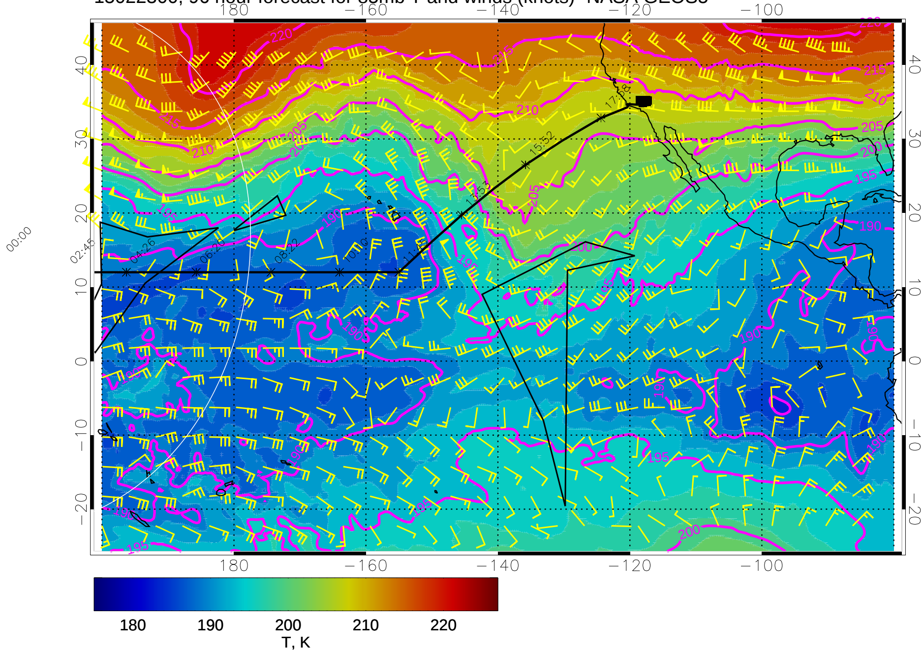
15022300, 96 hour forecast for 85mb T and winds (knots)- NASA GEOS5
