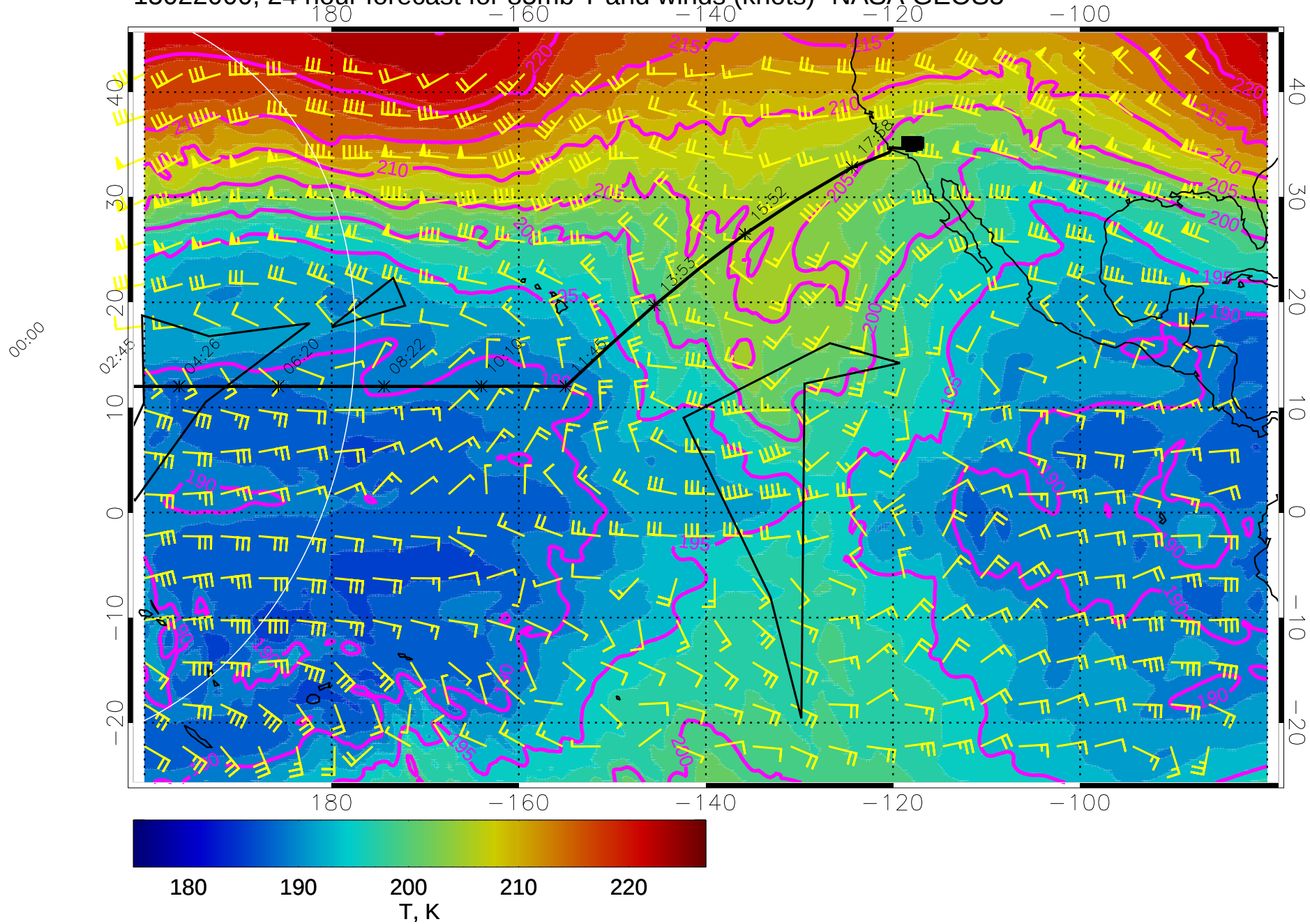
15022000, 24 hour forecast for 85mb T and winds (knots)- NASA GEOS5
