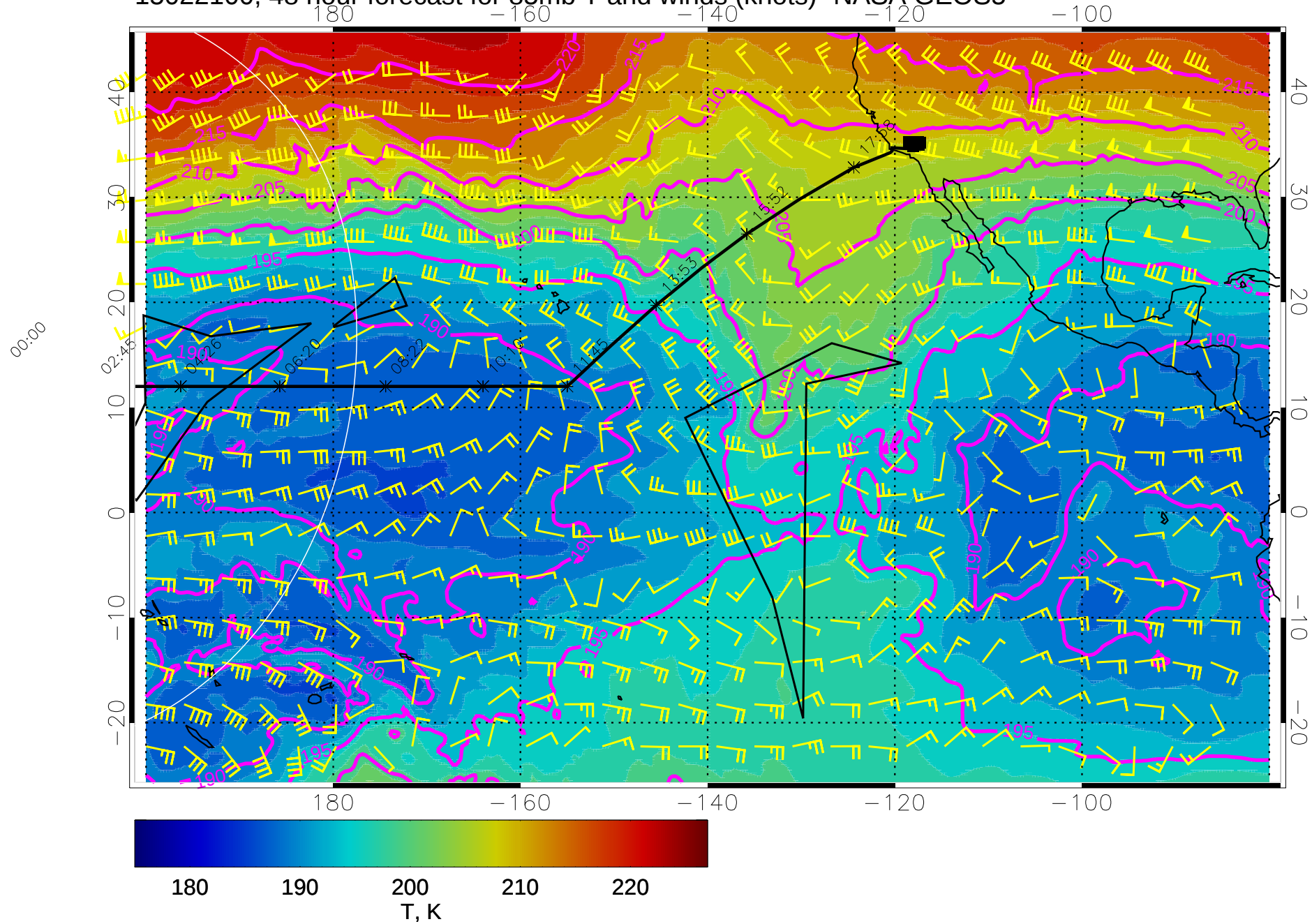
15022100, 48 hour forecast for 85mb T and winds (knots)- NASA GEOS5
