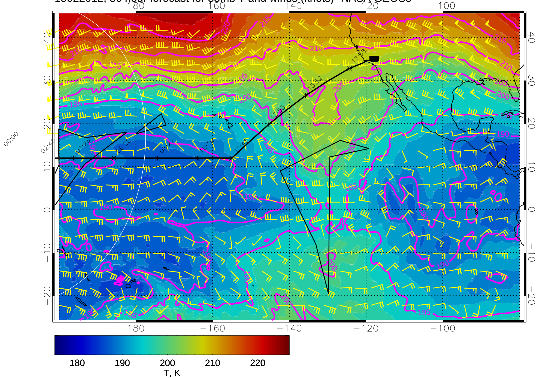
15022012, 36 hour forecast for 85mb T and winds (knots)- NASA GEOS5
