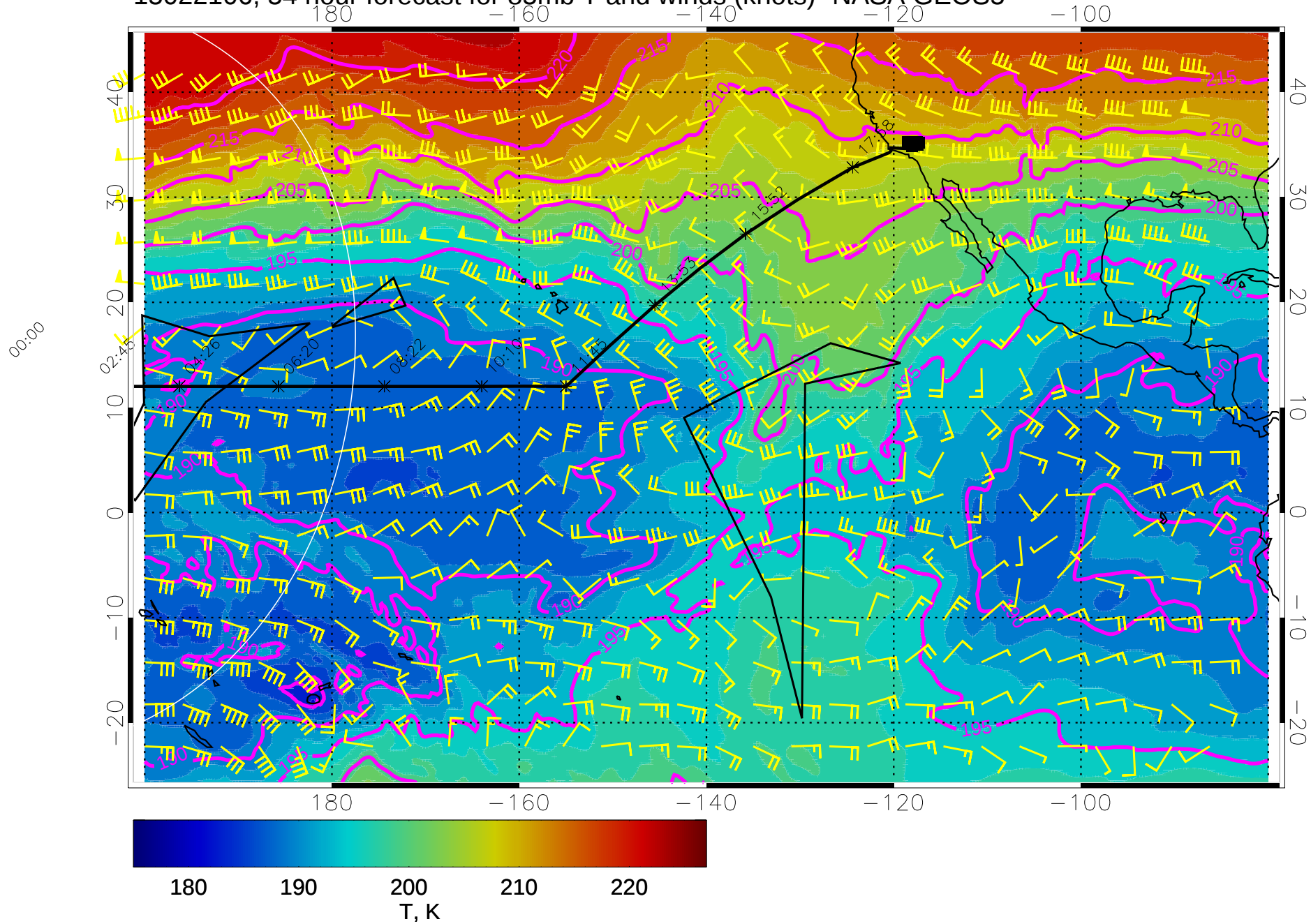
15022106, 54 hour forecast for 85mb T and winds (knots)- NASA GEOS5
