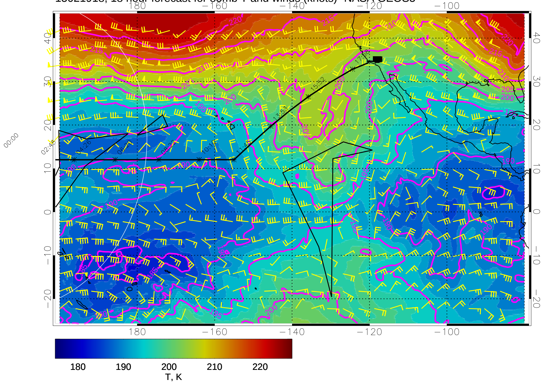
15021918, 18 hour forecast for 85mb T and winds (knots)- NASA GEOS5
