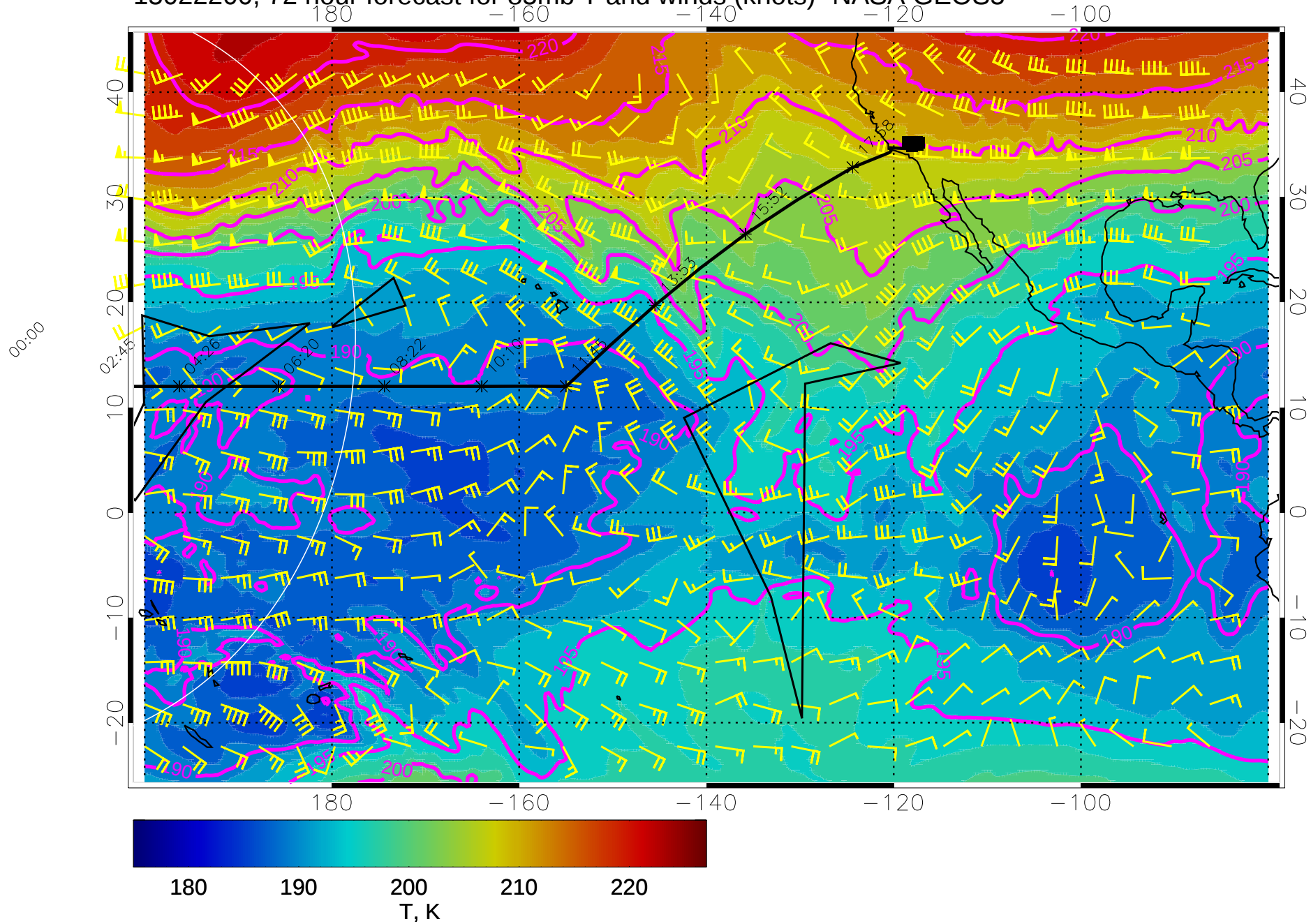
15022200, 72 hour forecast for 85mb T and winds (knots)- NASA GEOS5
