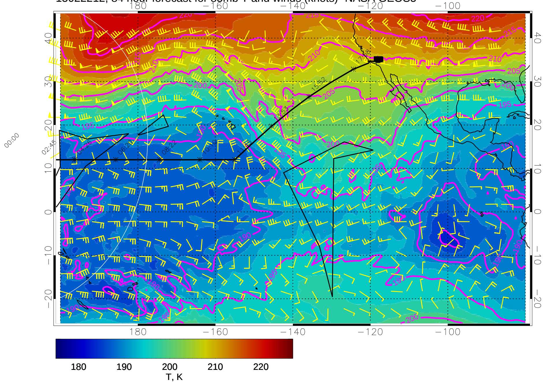
15022212, 84 hour forecast for 85mb T and winds (knots)- NASA GEOS5
