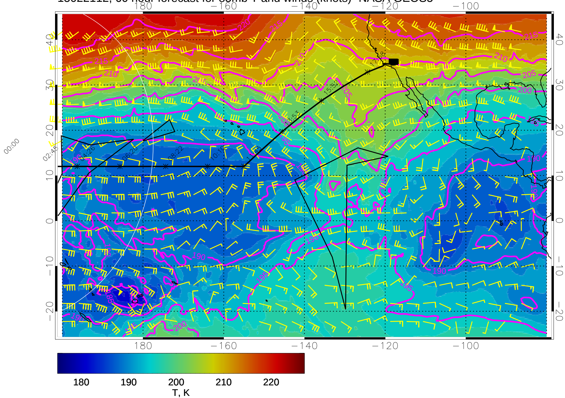
15022112, 60 hour forecast for 85mb T and winds (knots)- NASA GEOS5
