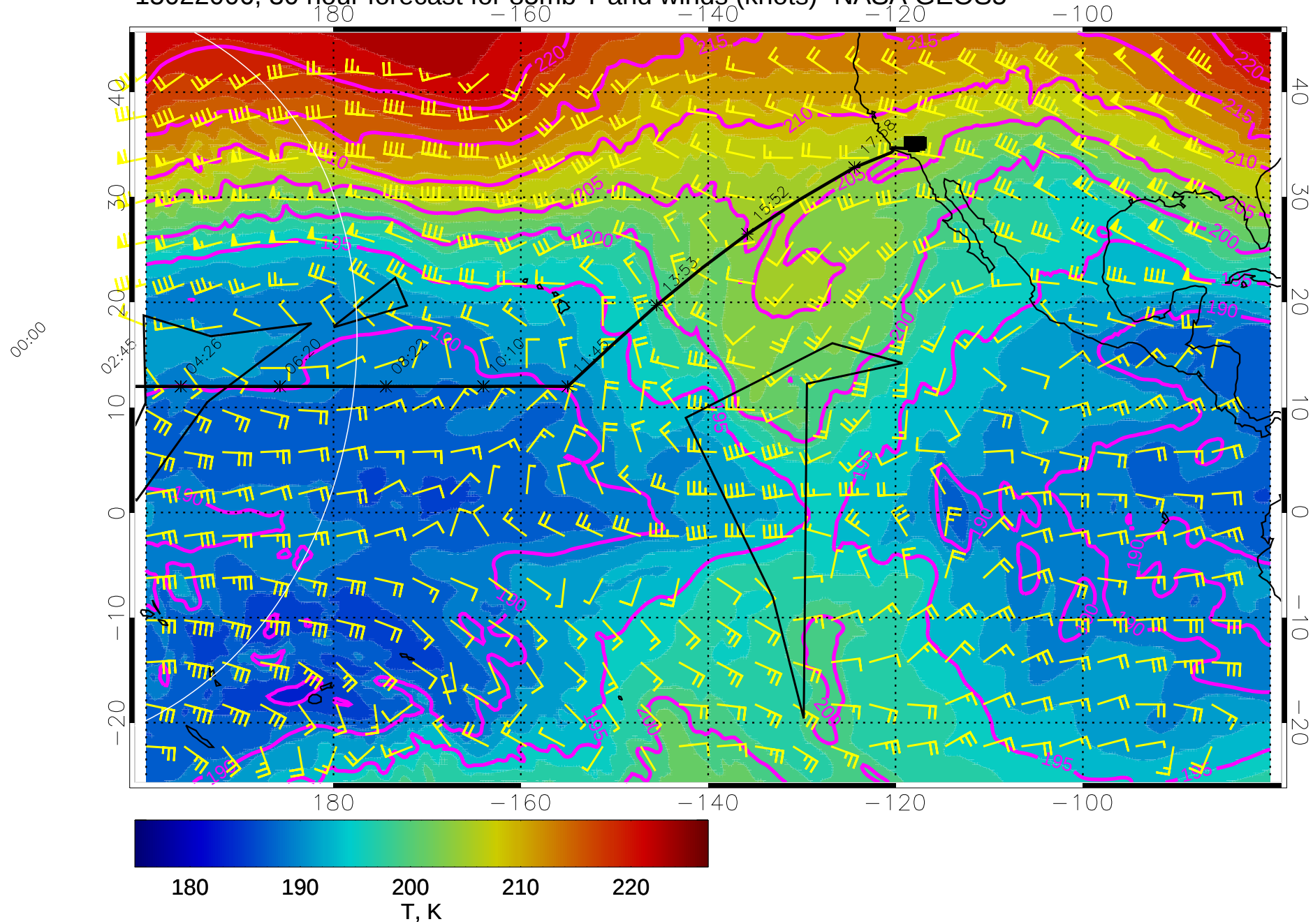
15022006, 30 hour forecast for 85mb T and winds (knots)- NASA GEOS5
