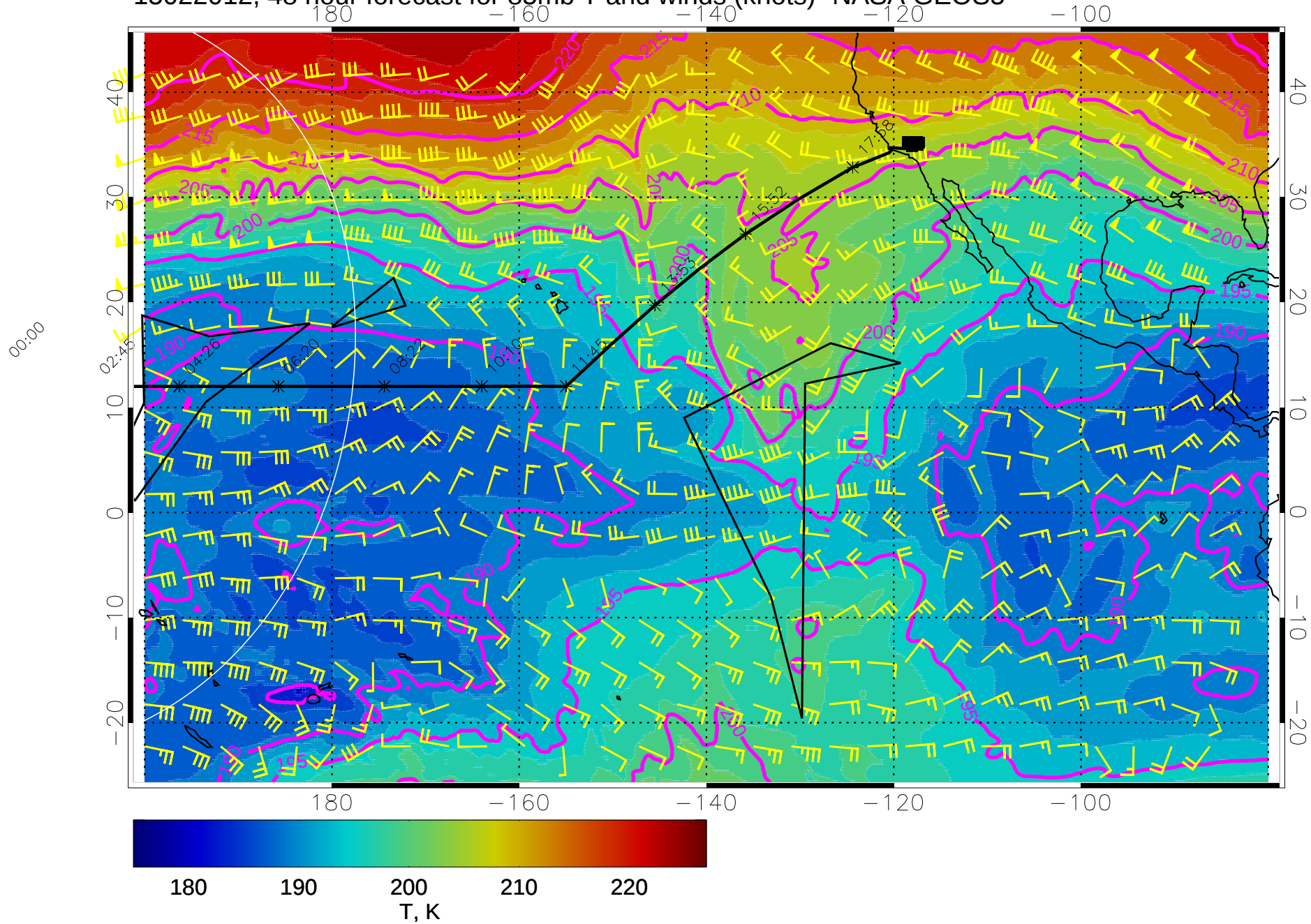
15022012, 48 hour forecast for 85mb T and winds (knots)- NASA GEOS5
