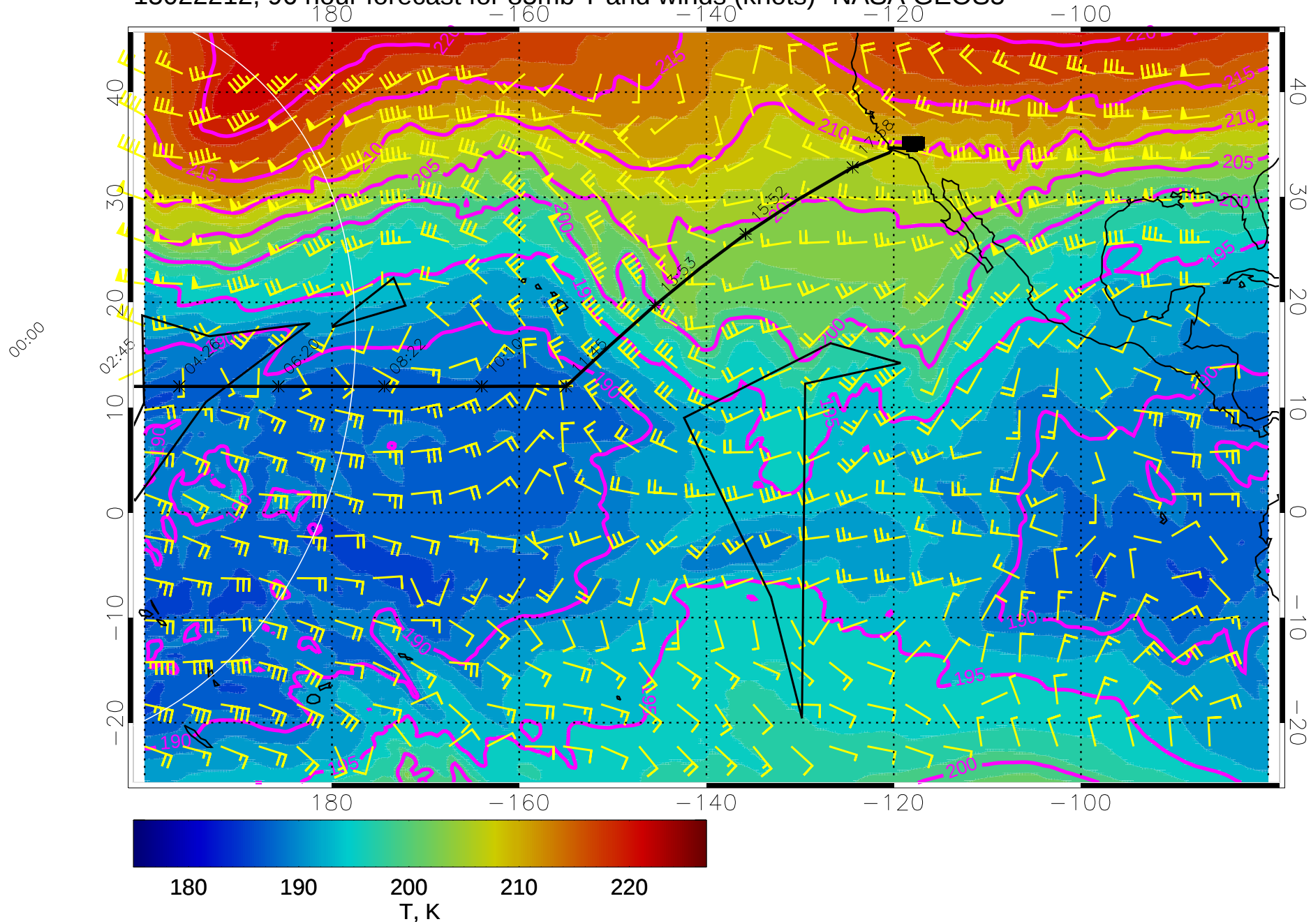
15022212, 96 hour forecast for 85mb T and winds (knots)- NASA GEOS5
