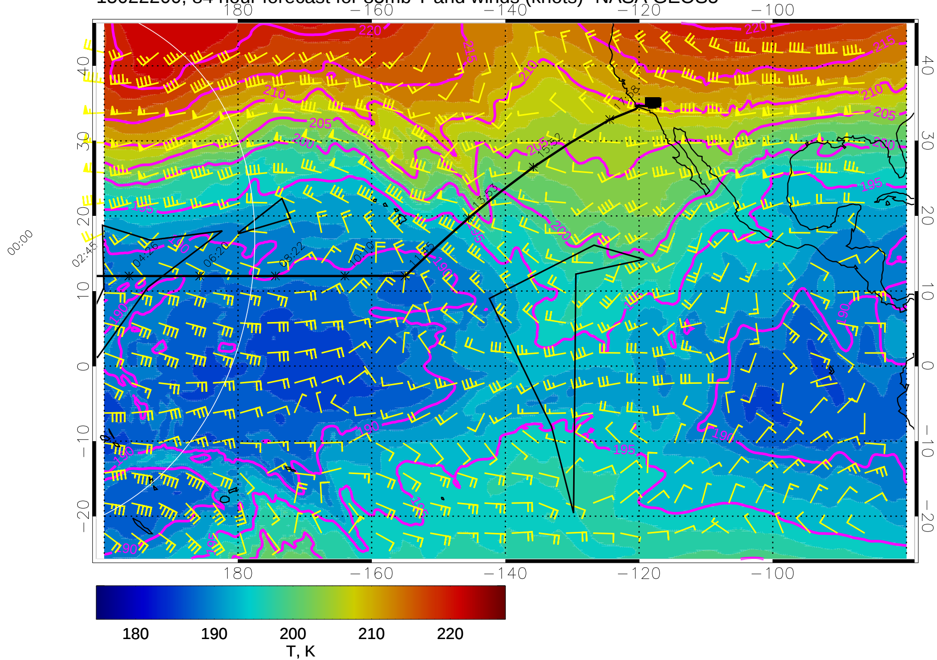
15022200, 84 hour forecast for 85mb T and winds (knots)- NASA GEOS5
