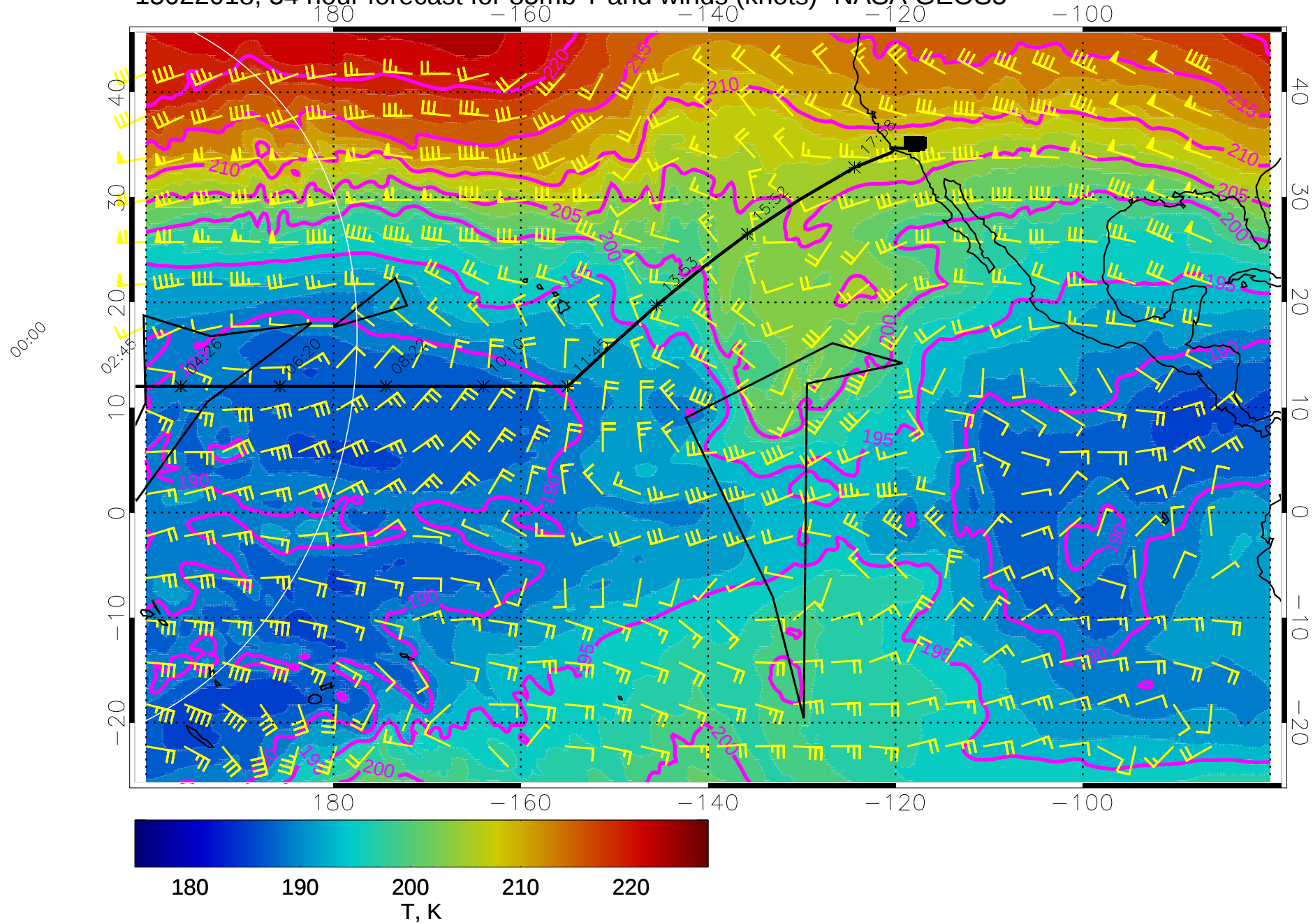
15022018, 54 hour forecast for 85mb T and winds (knots)- NASA GEOS5
