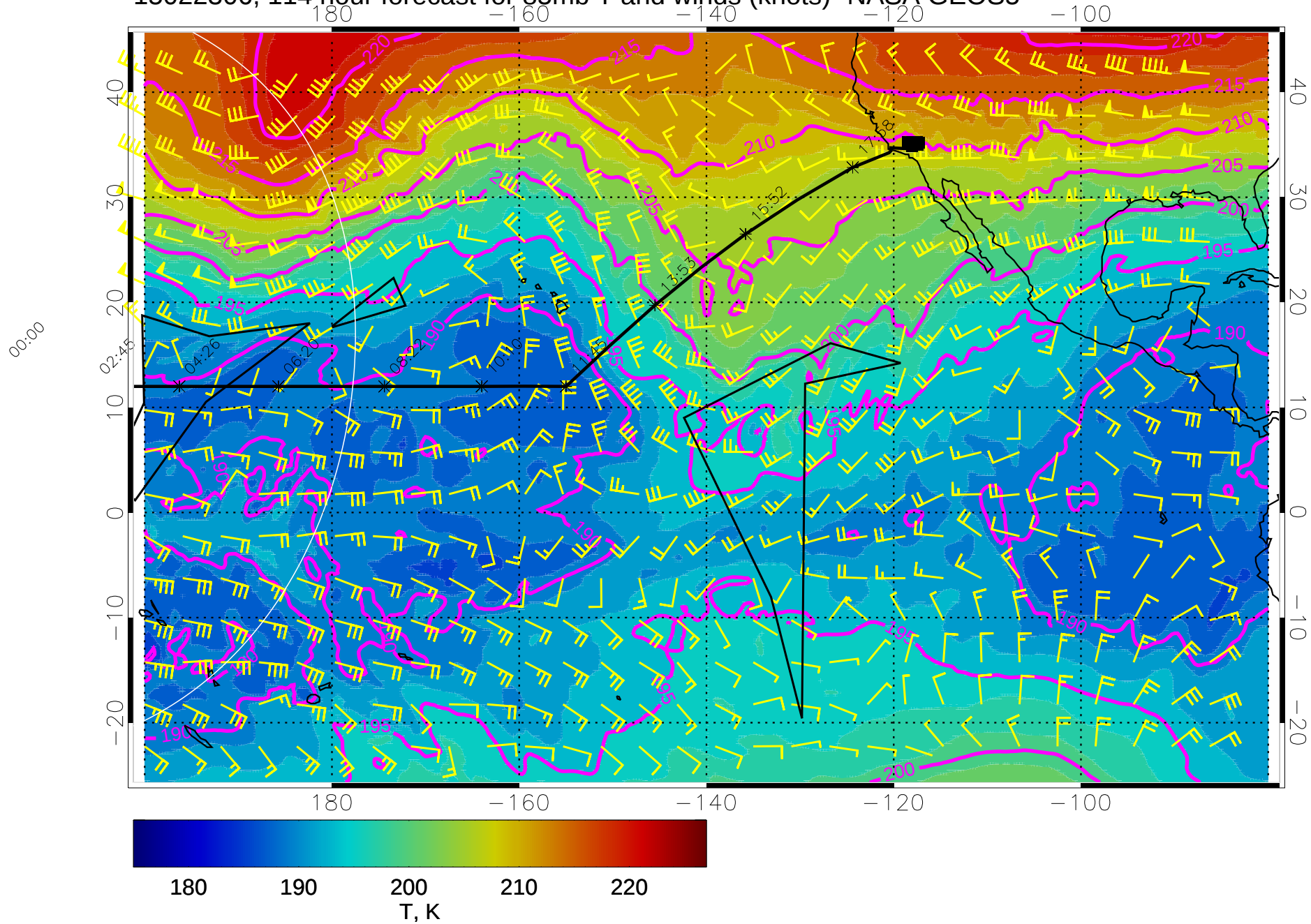
15022306, 114 hour forecast for 85mb T and winds (knots)- NASA GEOS5
