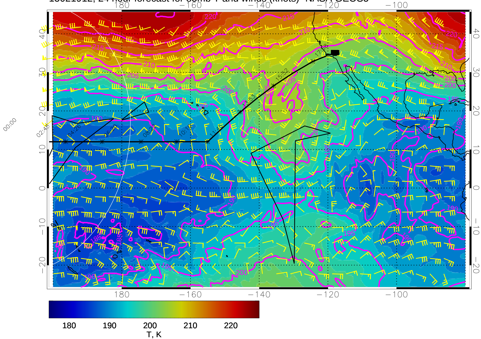
15021912, 24 hour forecast for 85mb T and winds (knots)- NASA GEOS5
