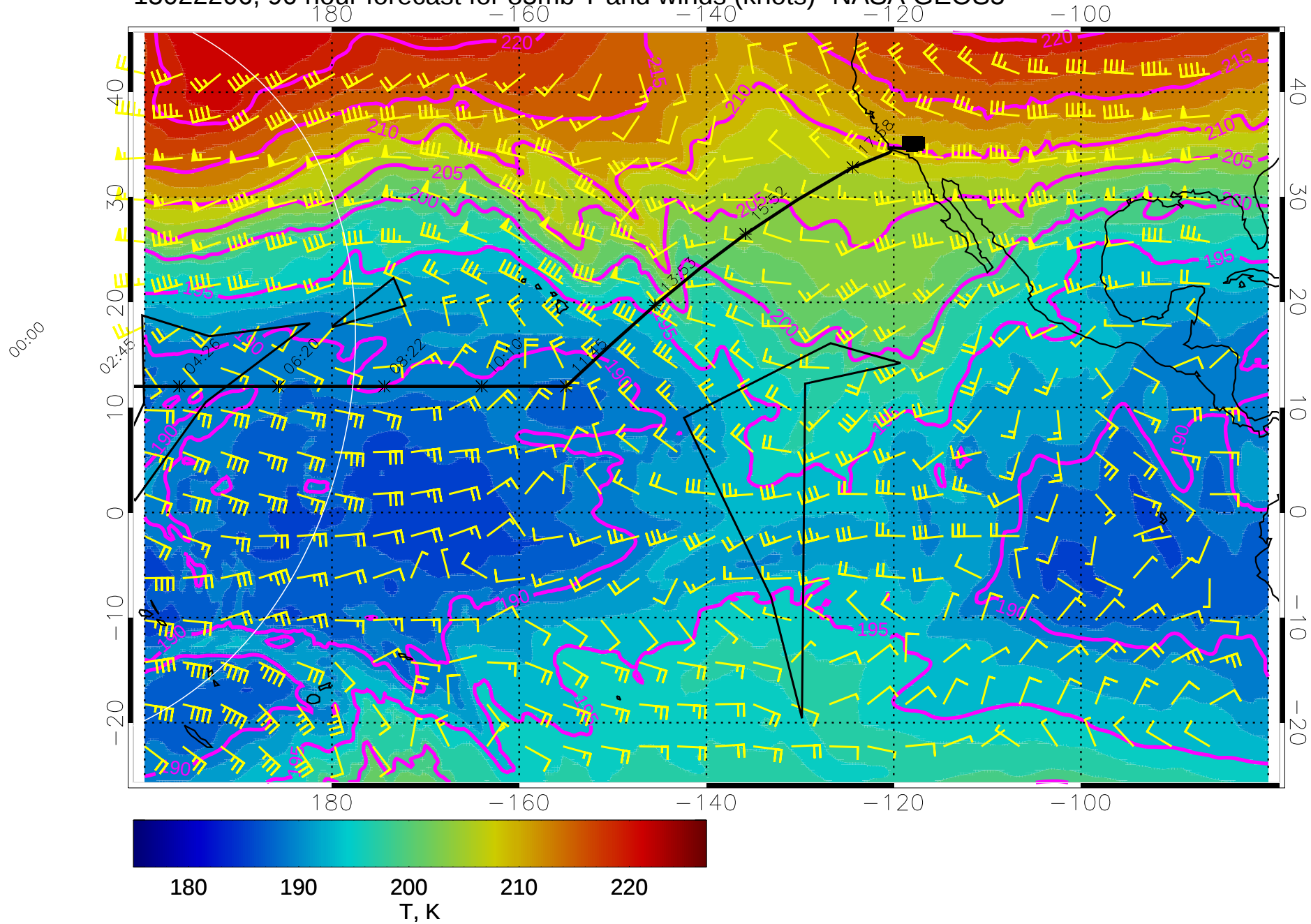
15022206, 90 hour forecast for 85mb T and winds (knots)- NASA GEOS5
