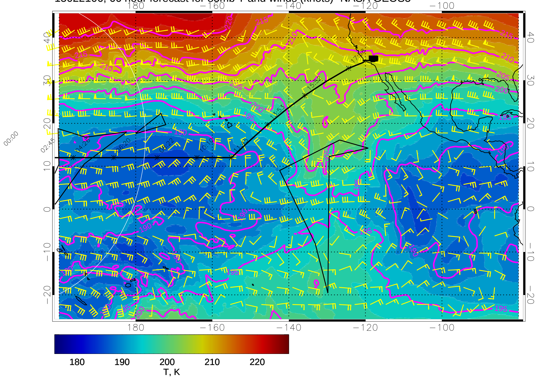
15022106, 66 hour forecast for 85mb T and winds (knots)- NASA GEOS5
