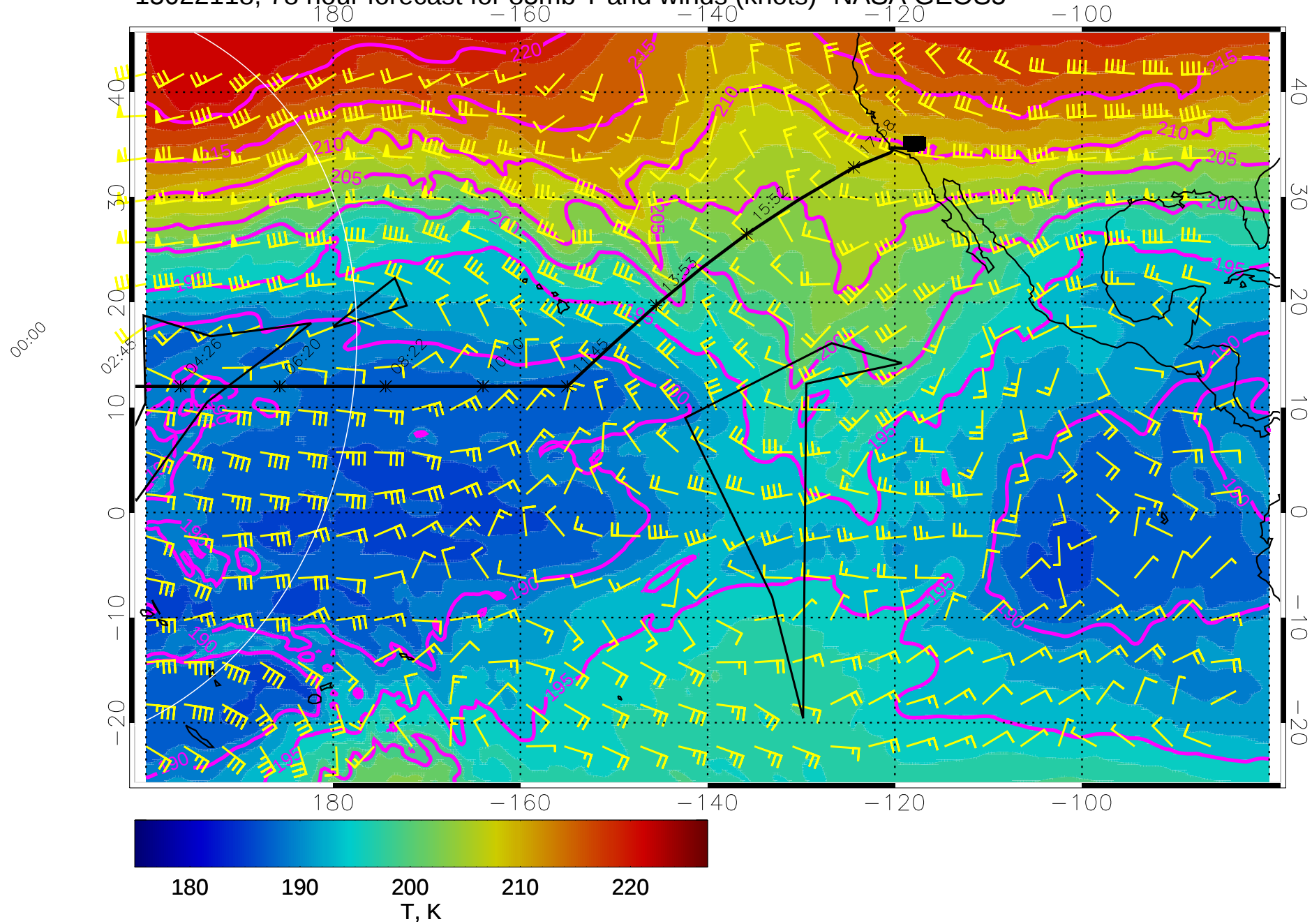
15022118, 78 hour forecast for 85mb T and winds (knots)- NASA GEOS5
