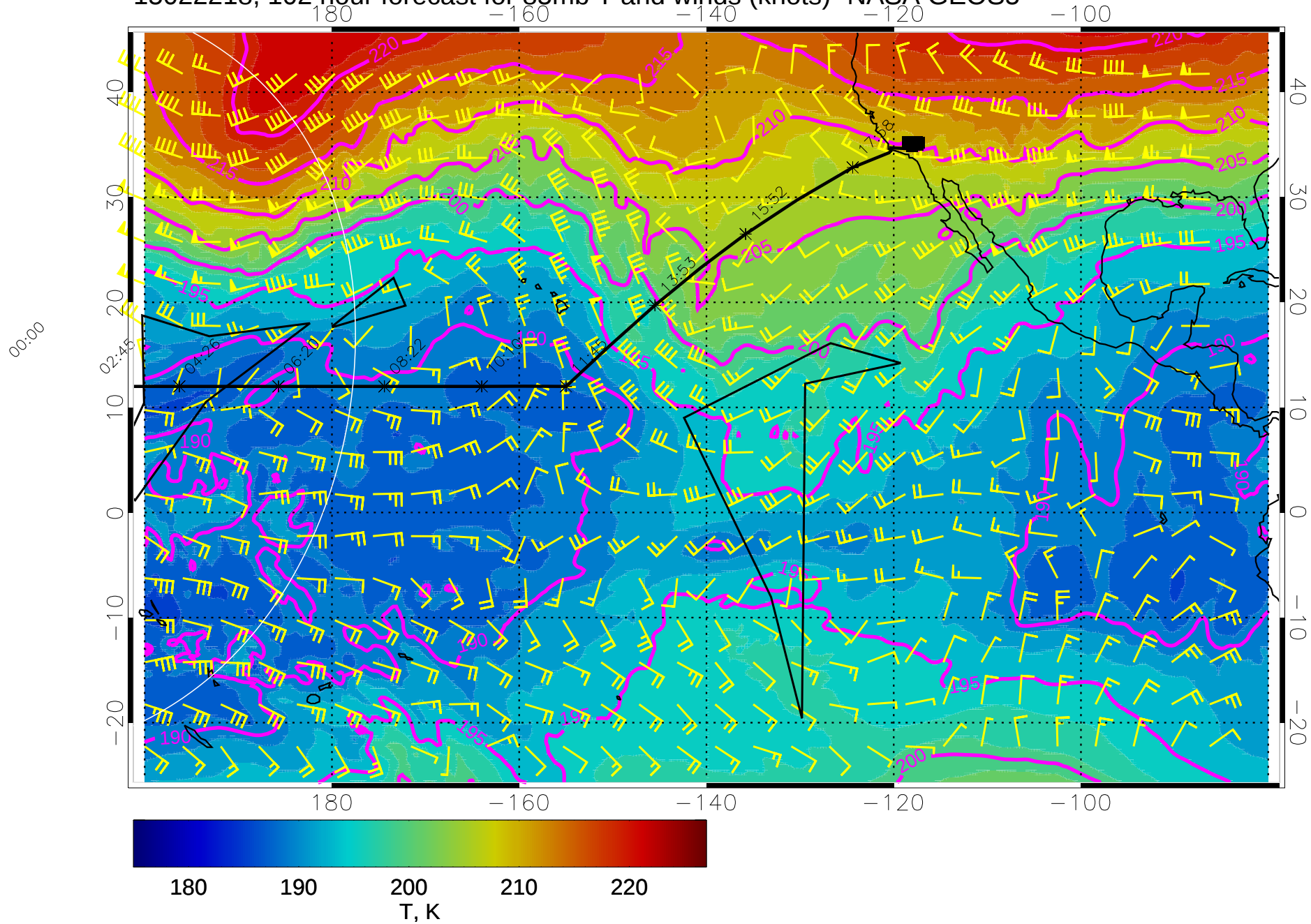
15022218, 102 hour forecast for 85mb T and winds (knots)- NASA GEOS5
