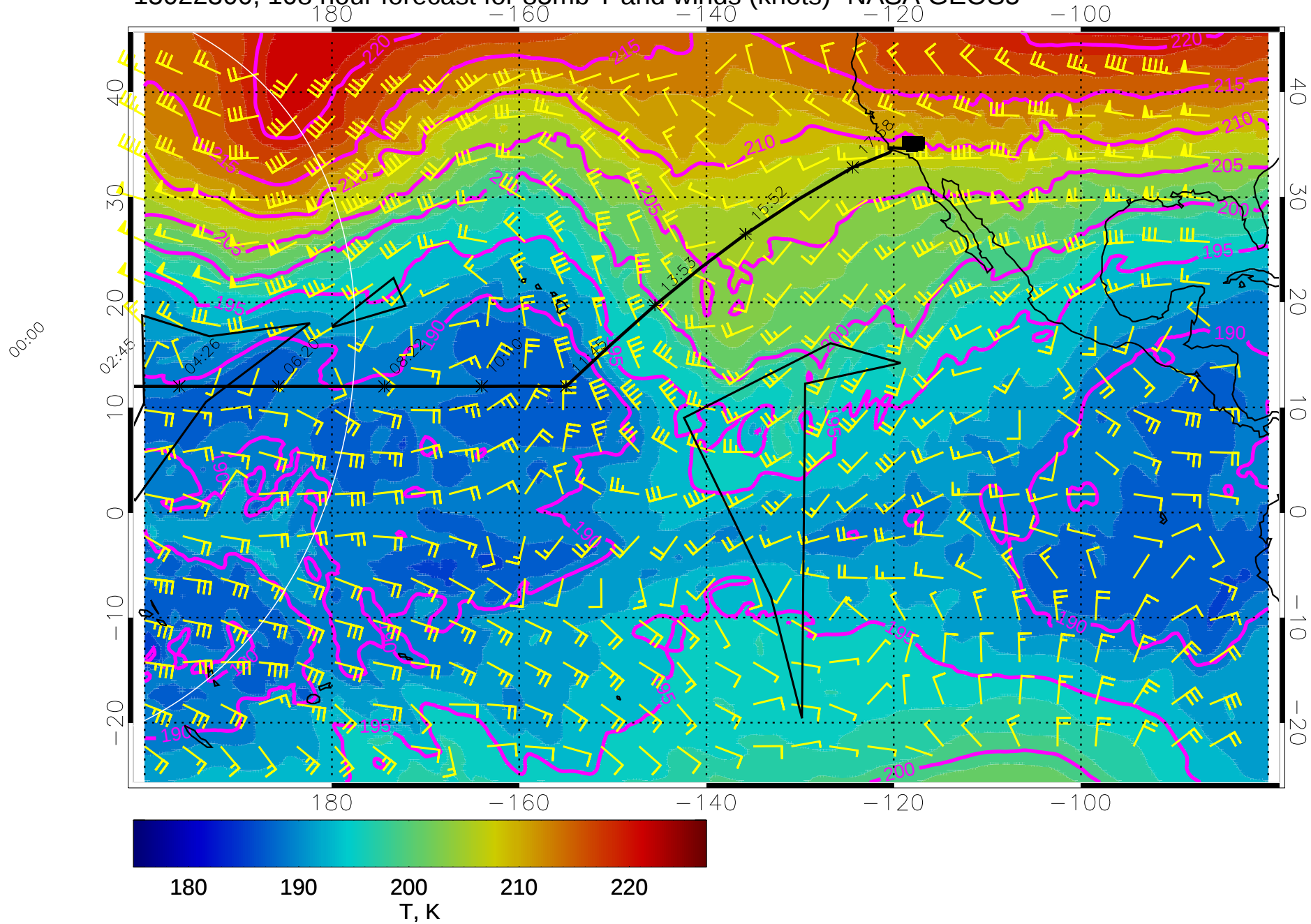
15022300, 108 hour forecast for 85mb T and winds (knots)- NASA GEOS5
