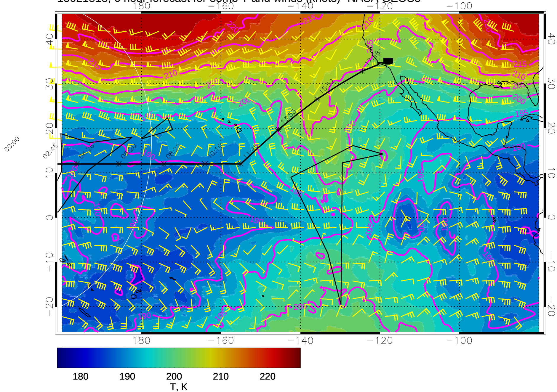
15021818, 6 hour forecast for 85mb T and winds (knots)- NASA GEOS5
