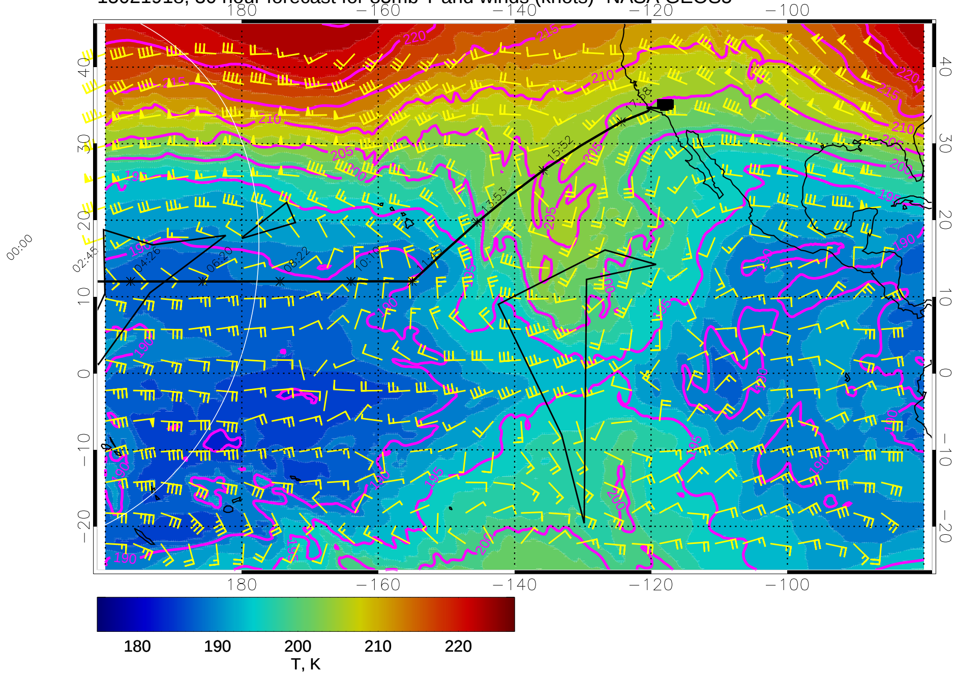
15021918, 30 hour forecast for 85mb T and winds (knots)- NASA GEOS5
