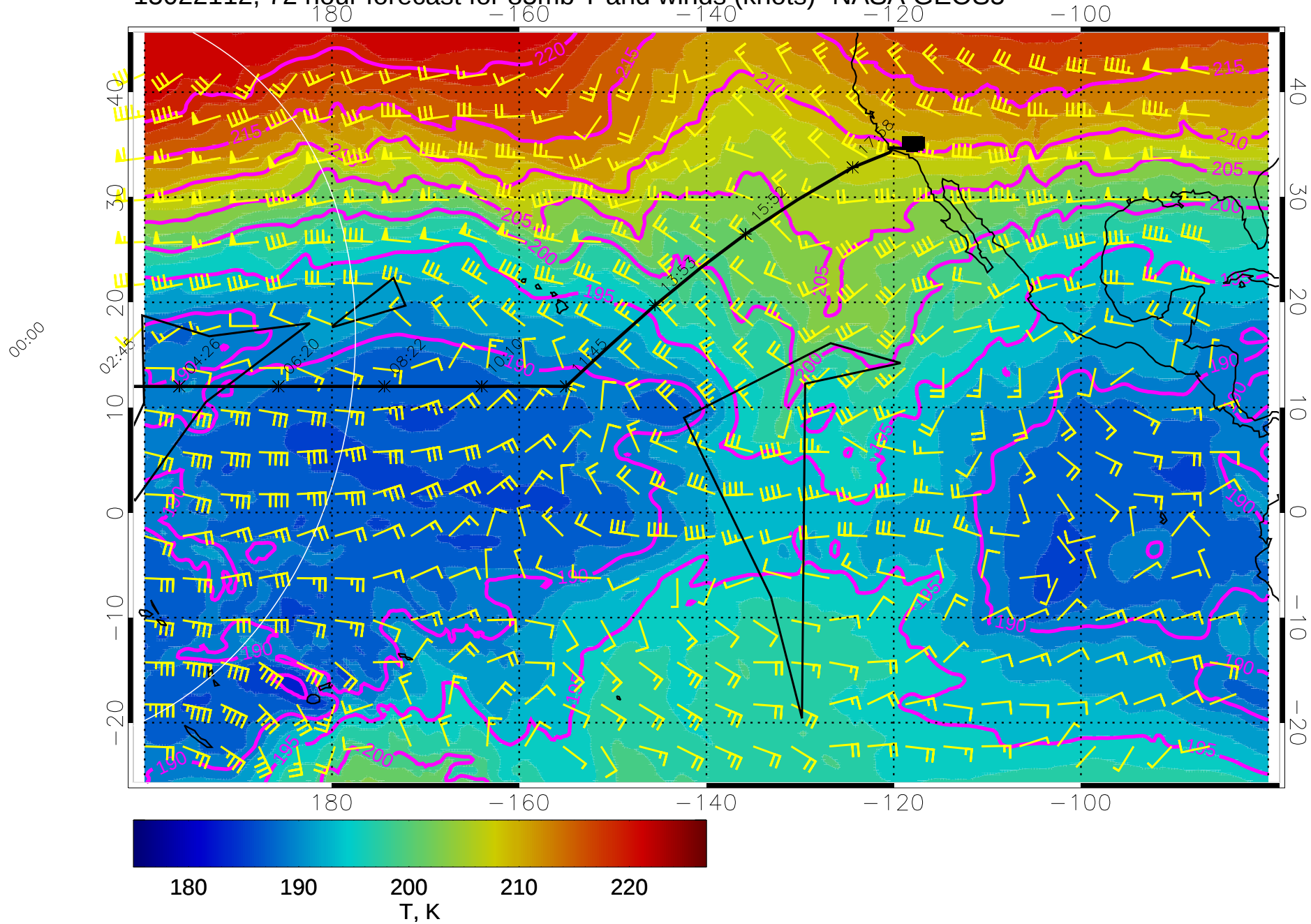
15022112, 72 hour forecast for 85mb T and winds (knots)- NASA GEOS5
