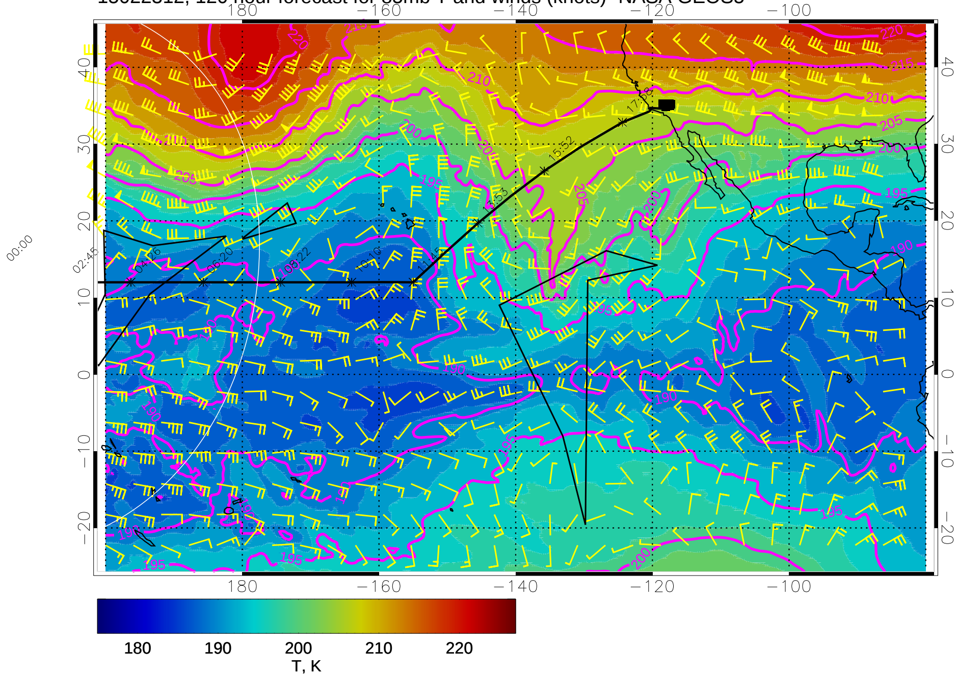
15022312, 120 hour forecast for 85mb T and winds (knots)- NASA GEOS5
