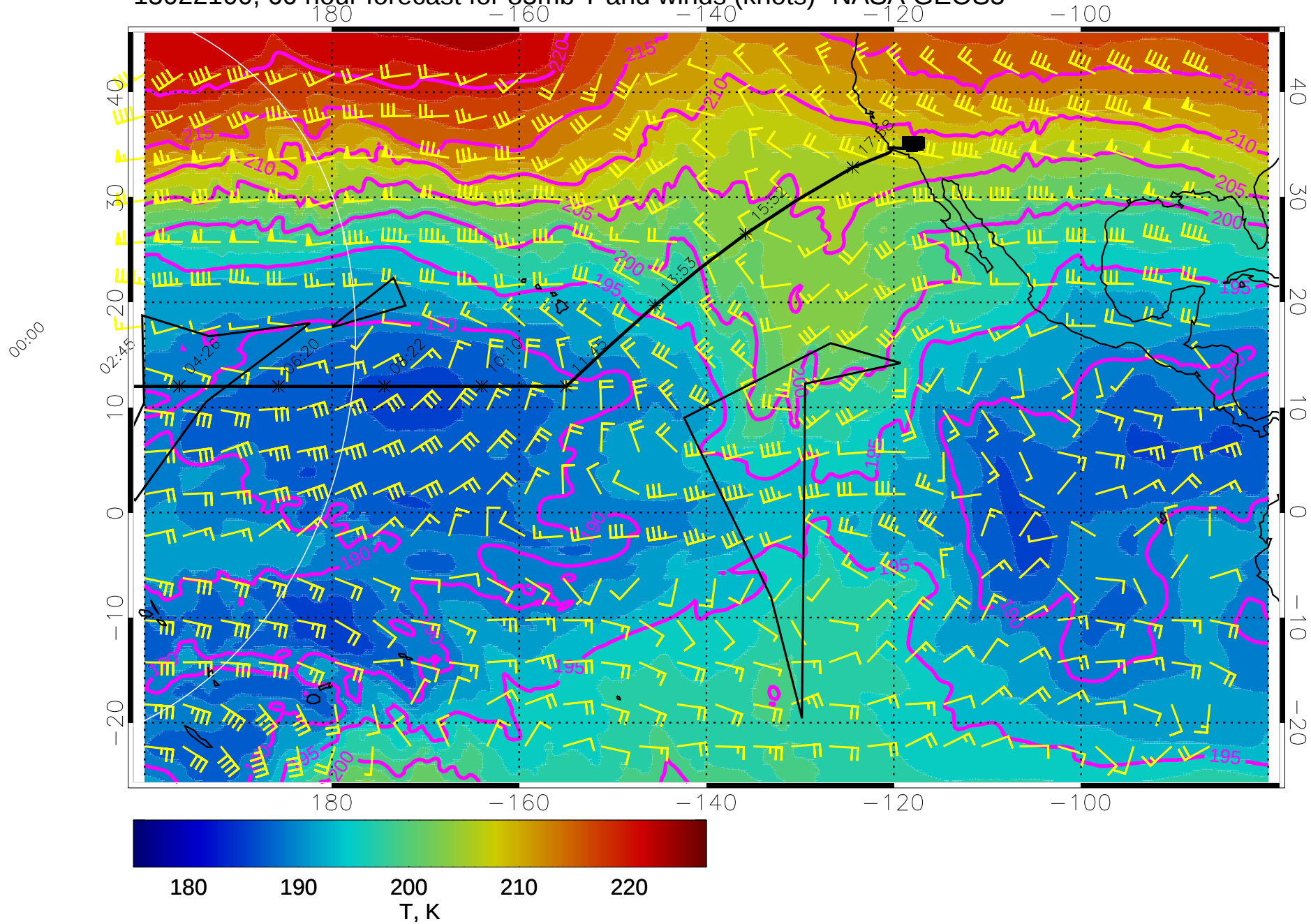
15022100, 60 hour forecast for 85mb T and winds (knots)- NASA GEOS5
