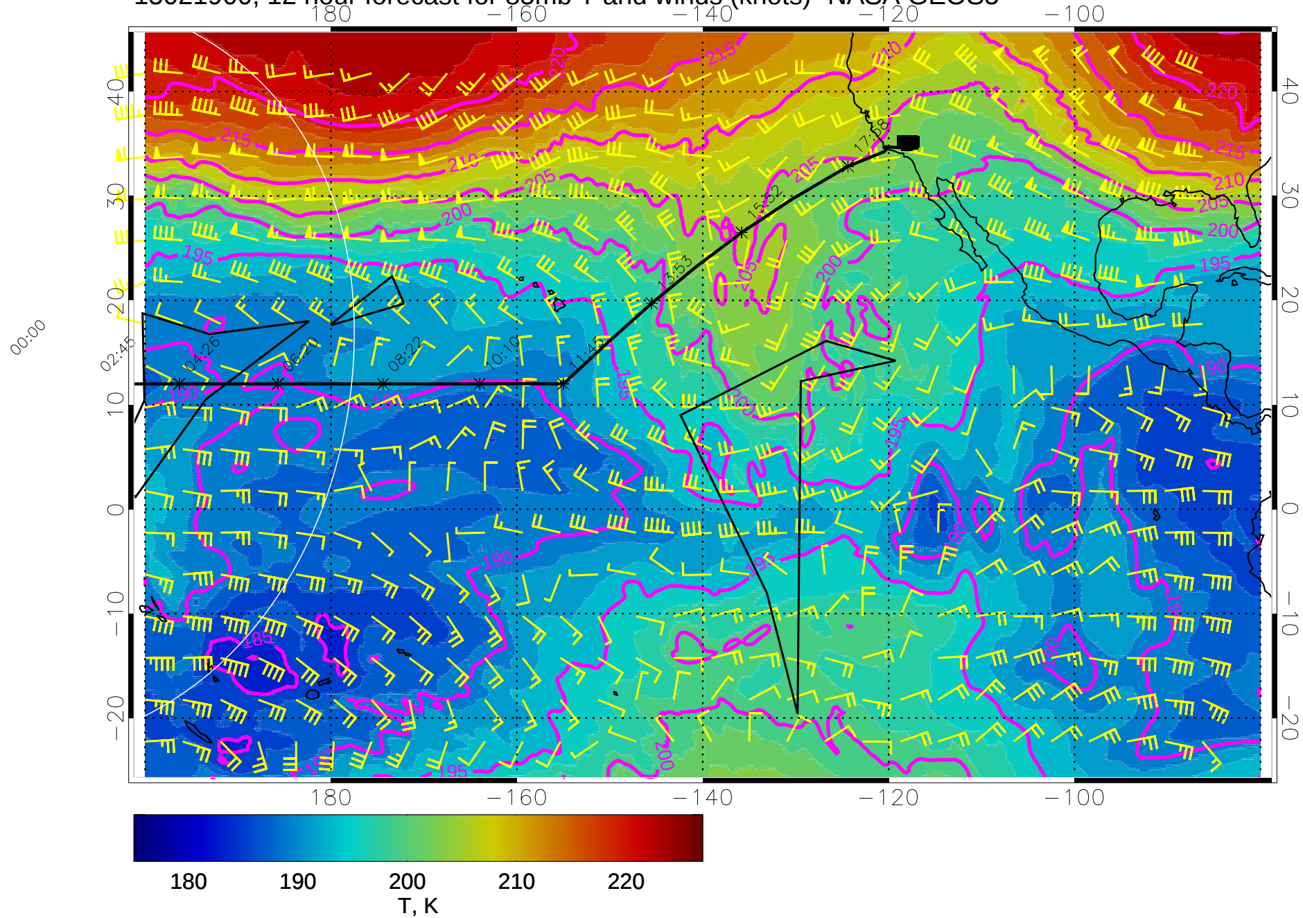
15021900, 12 hour forecast for 85mb T and winds (knots)- NASA GEOS5
