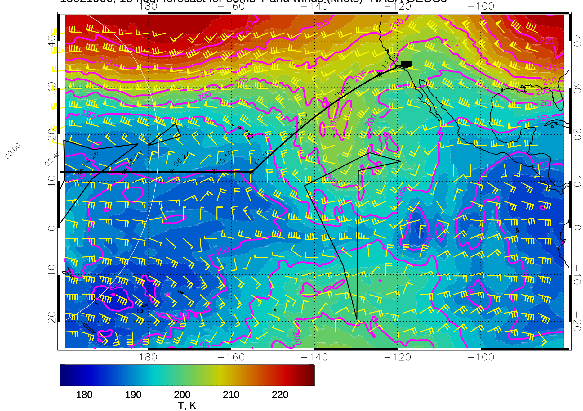
15021906, 18 hour forecast for 85mb T and winds (knots)- NASA GEOS5
