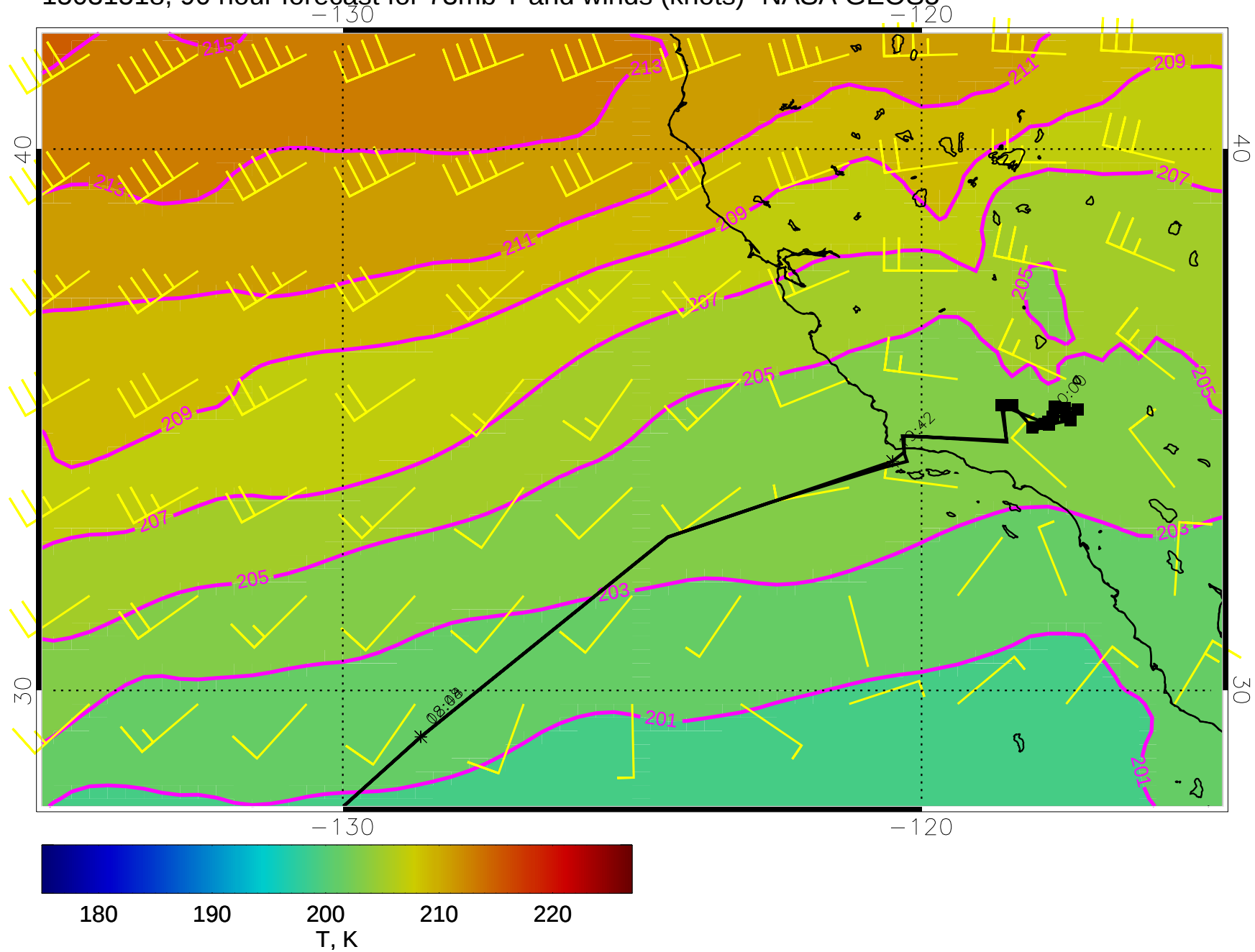
15031518, 90 hour forecast for 73mb T and winds (knots)- NASA GEOS5
