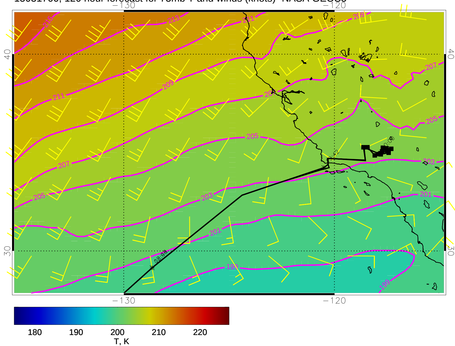
15031700, 120 hour forecast for 73mb T and winds (knots)- NASA GEOS5
