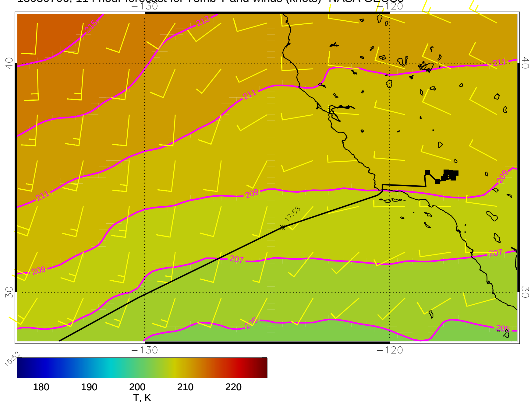
15030706, 114 hour forecast for 73mb T and winds (knots)- NASA GEOS5
