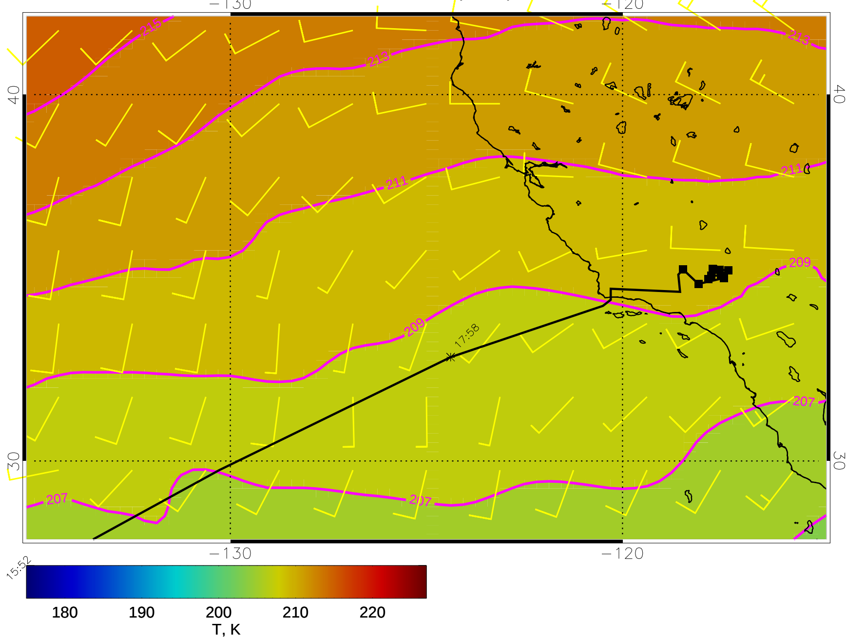
15030518, 114 hour forecast for 73mb T and winds (knots)- NASA GEOS5
