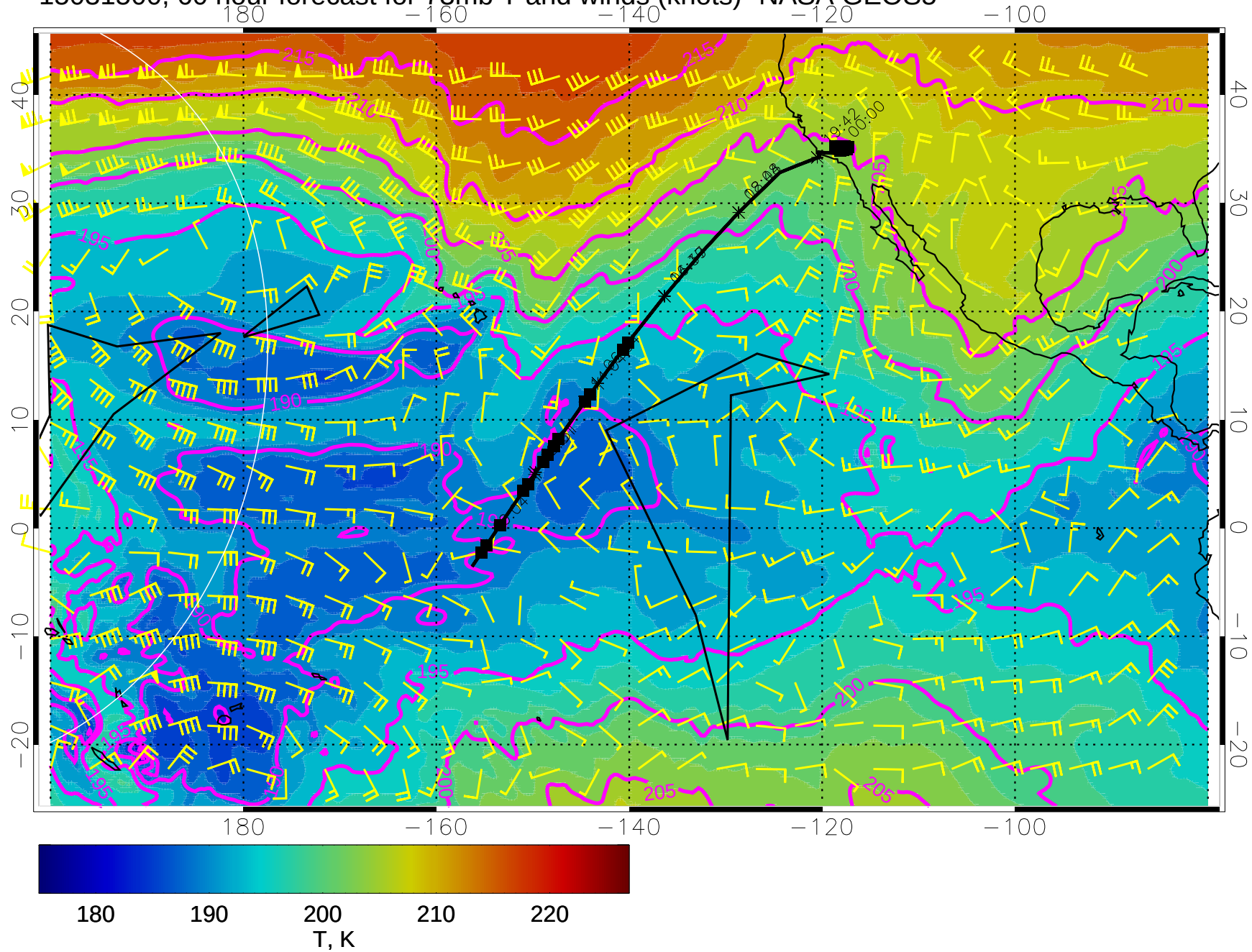
15031500, 60 hour forecast for 73mb T and winds (knots)- NASA GEOS5
