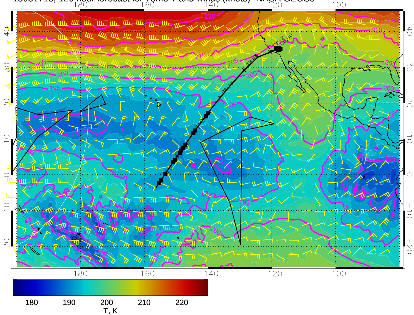
15031718, 126 hour forecast for 73mb T and winds (knots)- NASA GEOS5
