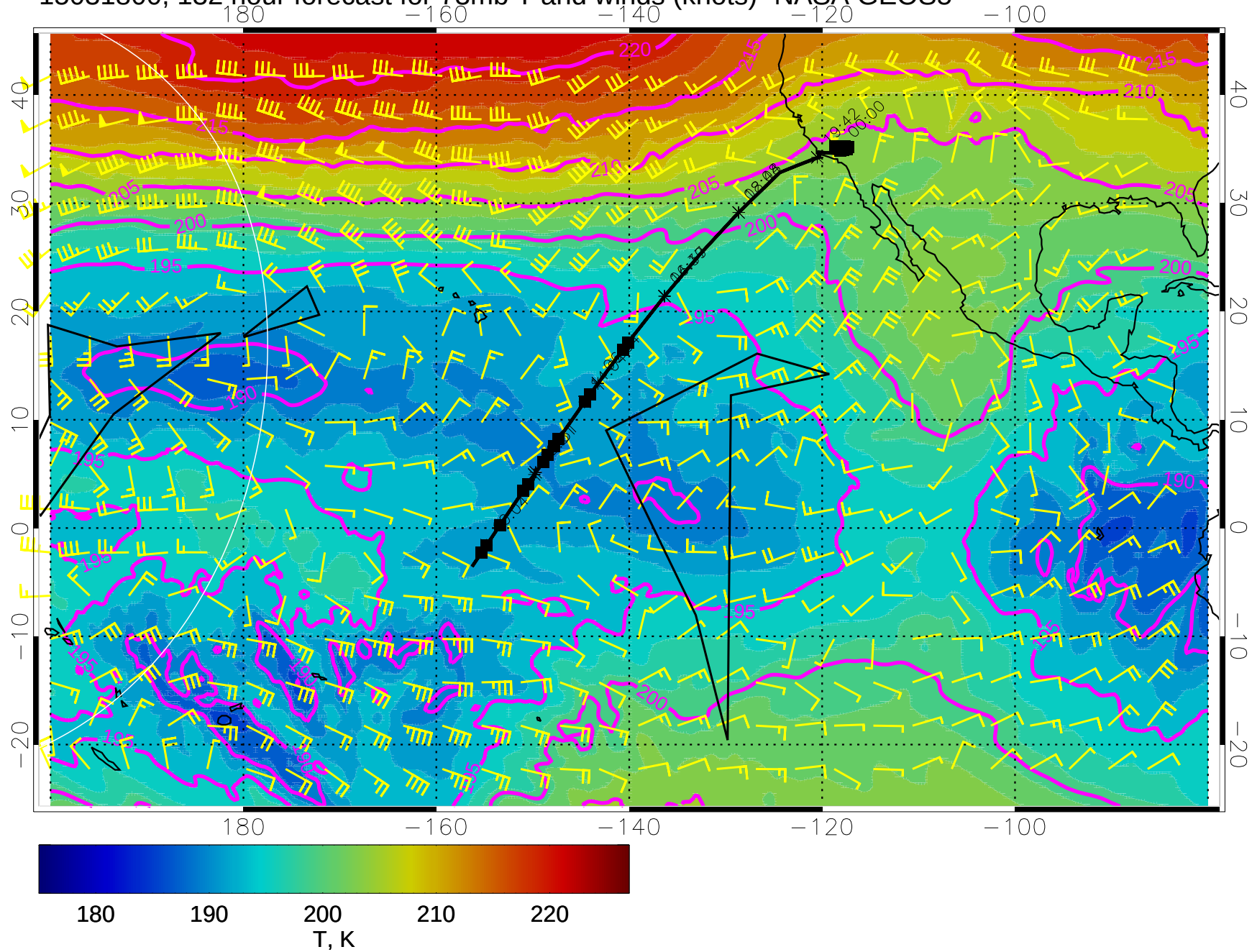
15031800, 132 hour forecast for 73mb T and winds (knots)- NASA GEOS5
