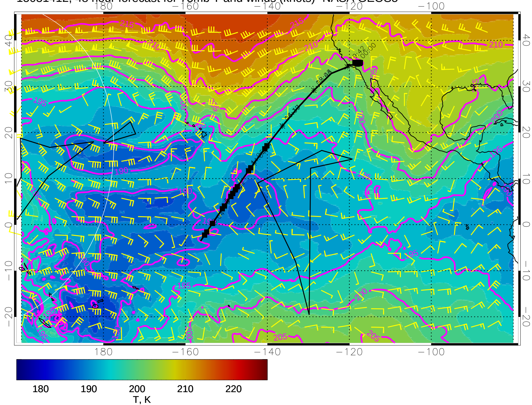
15031412, 48 hour forecast for 73mb T and winds (knots)- NASA GEOS5
