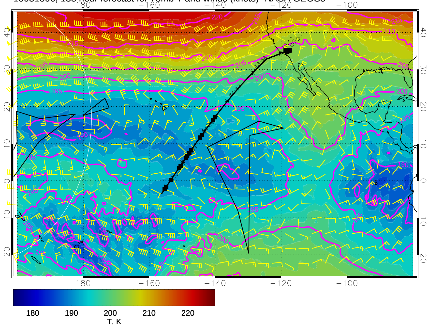
15031806, 138 hour forecast for 73mb T and winds (knots)- NASA GEOS5
