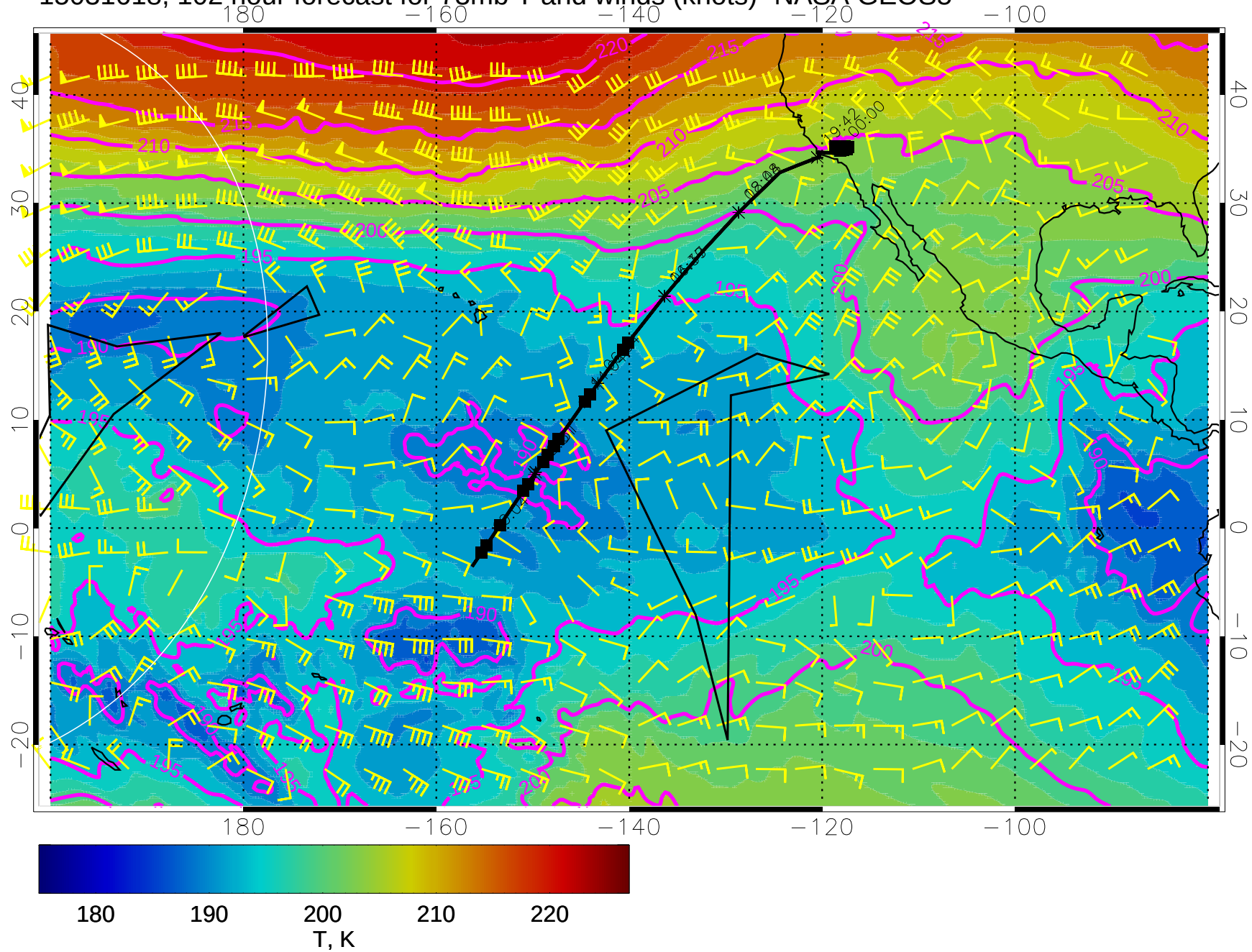
15031618, 102 hour forecast for 73mb T and winds (knots)- NASA GEOS5
