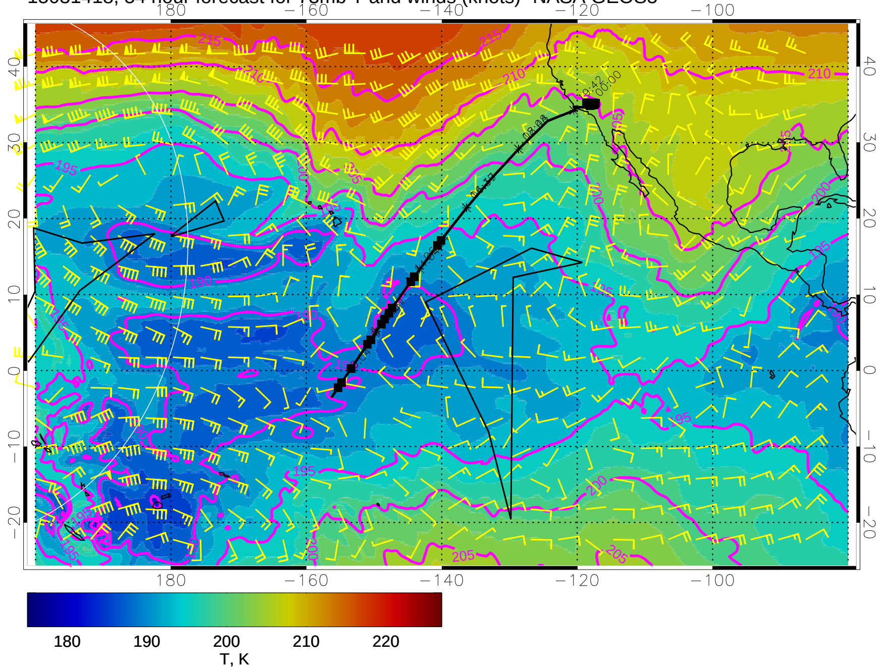
15031418, 54 hour forecast for 73mb T and winds (knots)- NASA GEOS5
