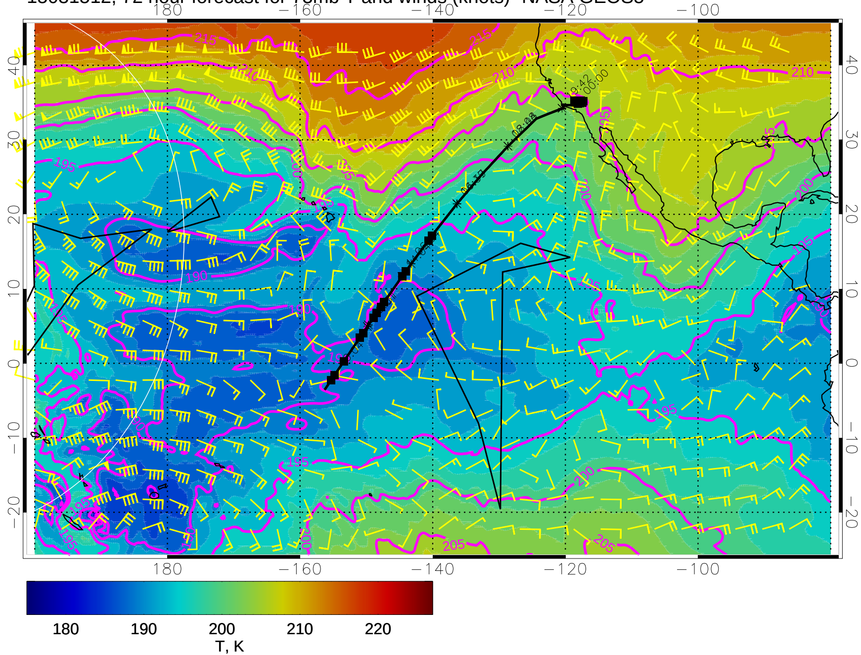
15031512, 72 hour forecast for 73mb T and winds (knots)- NASA GEOS5
