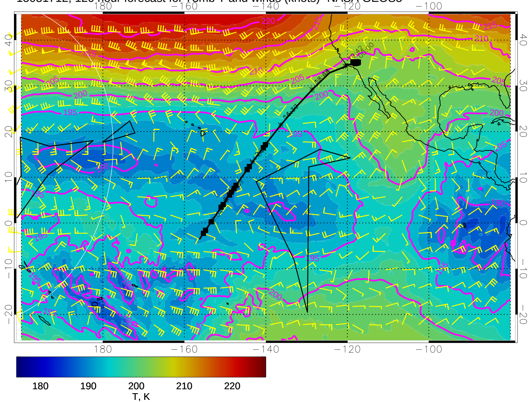
15031712, 120 hour forecast for 73mb T and winds (knots)- NASA GEOS5
