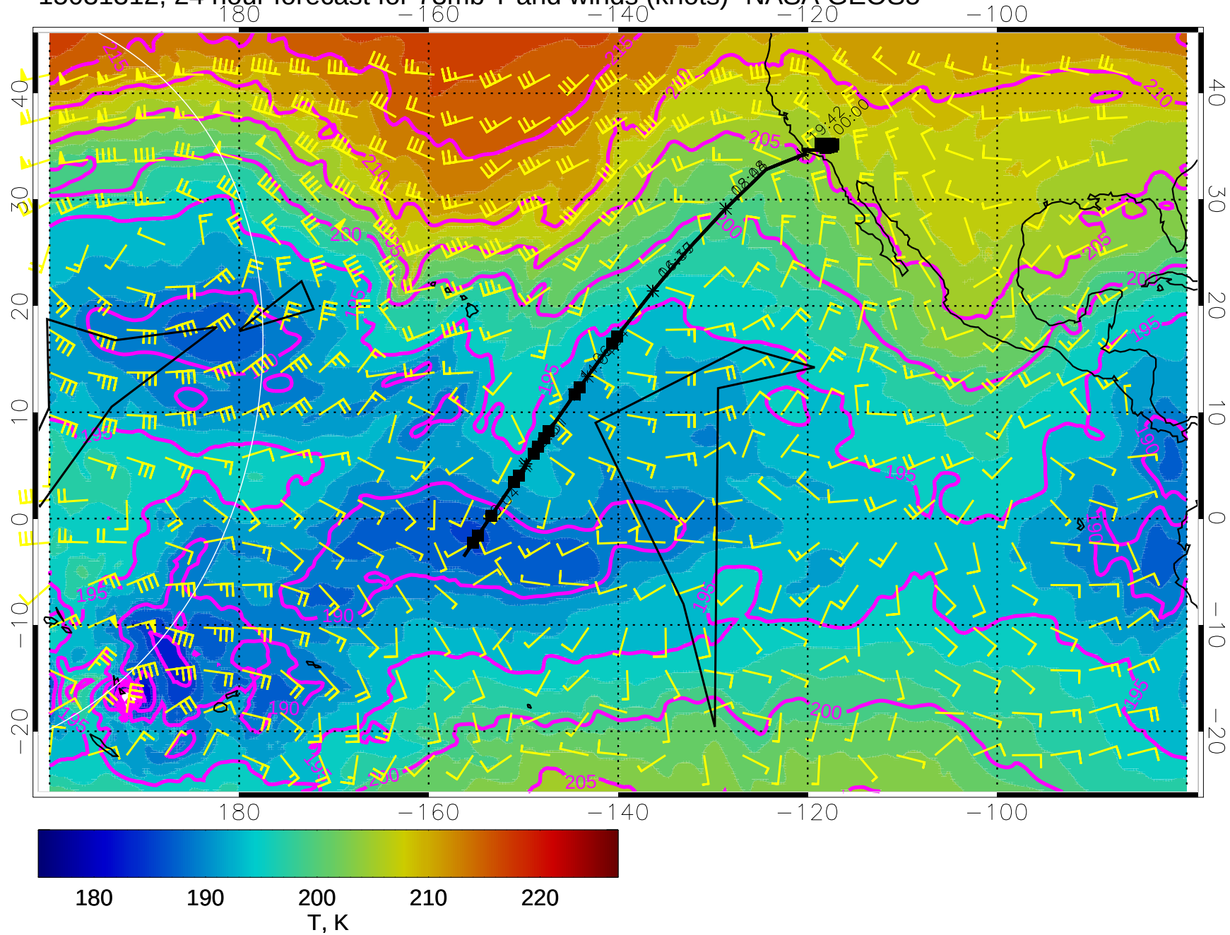
15031312, 24 hour forecast for 73mb T and winds (knots)- NASA GEOS5
