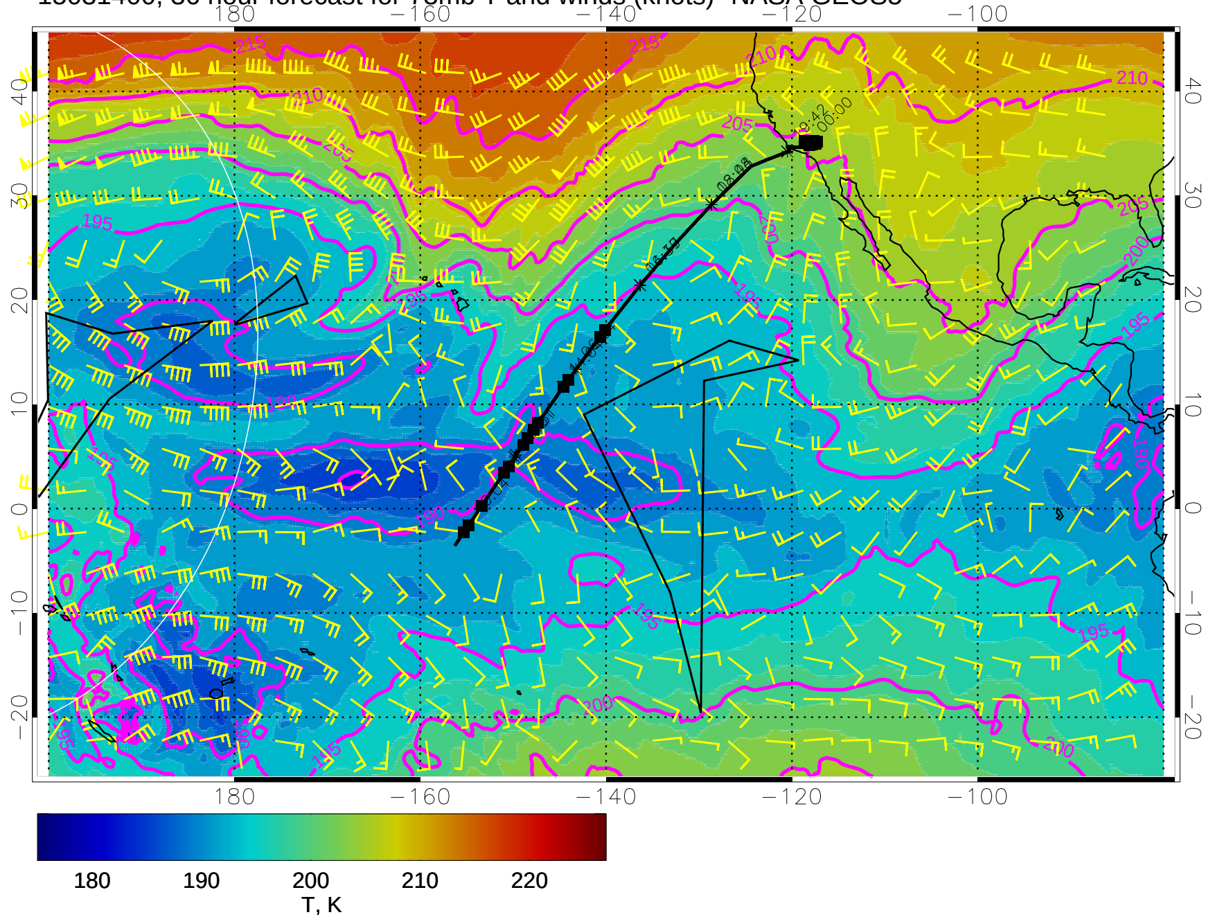
15031400, 36 hour forecast for 73mb T and winds (knots)- NASA GEOS5
