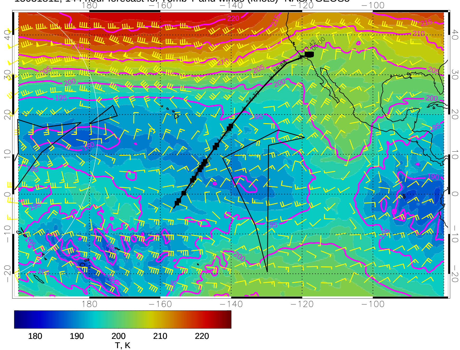
15031812, 144 hour forecast for 73mb T and winds (knots)- NASA GEOS5
