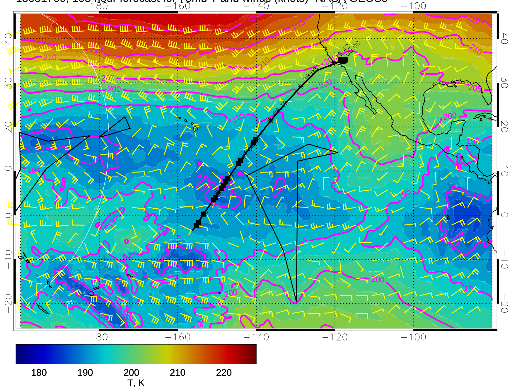
15031700, 108 hour forecast for 73mb T and winds (knots)- NASA GEOS5
