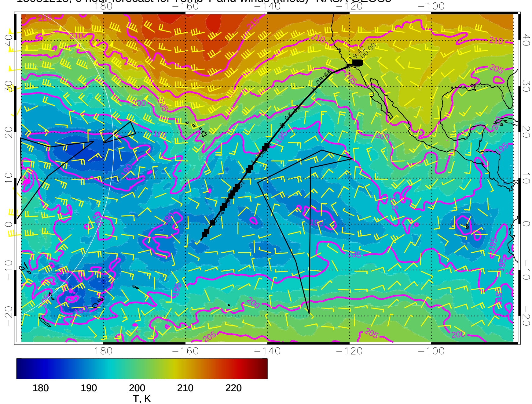
15031218, 6 hour forecast for 73mb T and winds (knots)- NASA GEOS5
