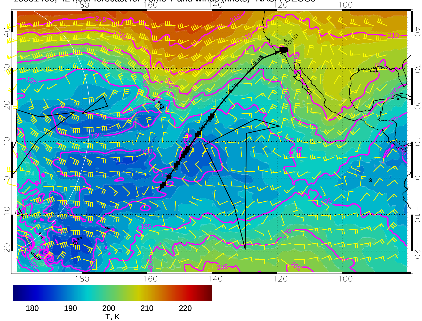
15031406, 42 hour forecast for 73mb T and winds (knots)- NASA GEOS5
