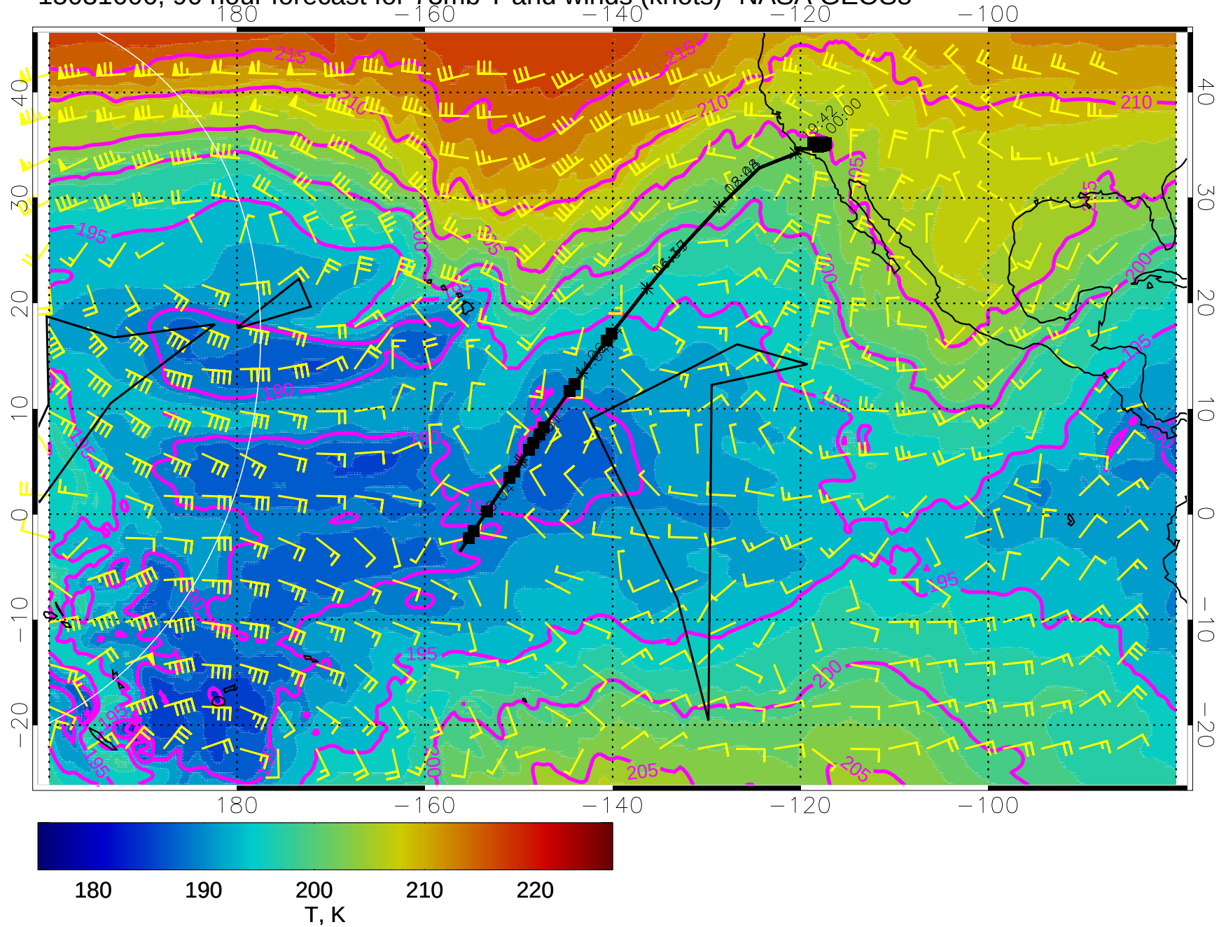
15031606, 90 hour forecast for 73mb T and winds (knots)- NASA GEOS5
