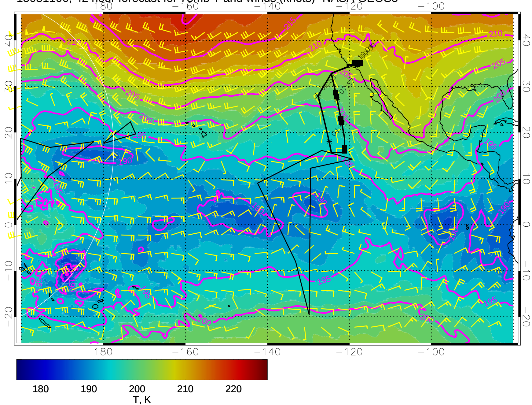
15031106, 42 hour forecast for 73mb T and winds (knots)- NASA GEOS5
