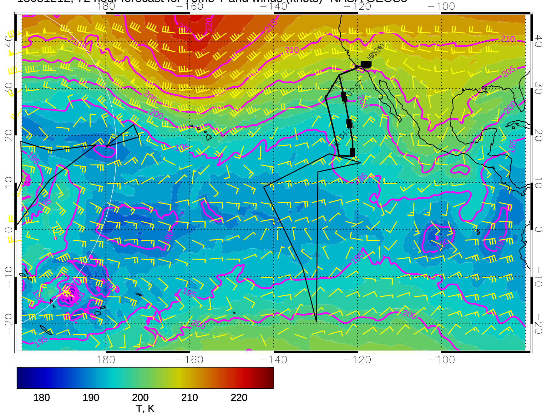
15031212, 72 hour forecast for 73mb T and winds (knots)- NASA GEOS5
