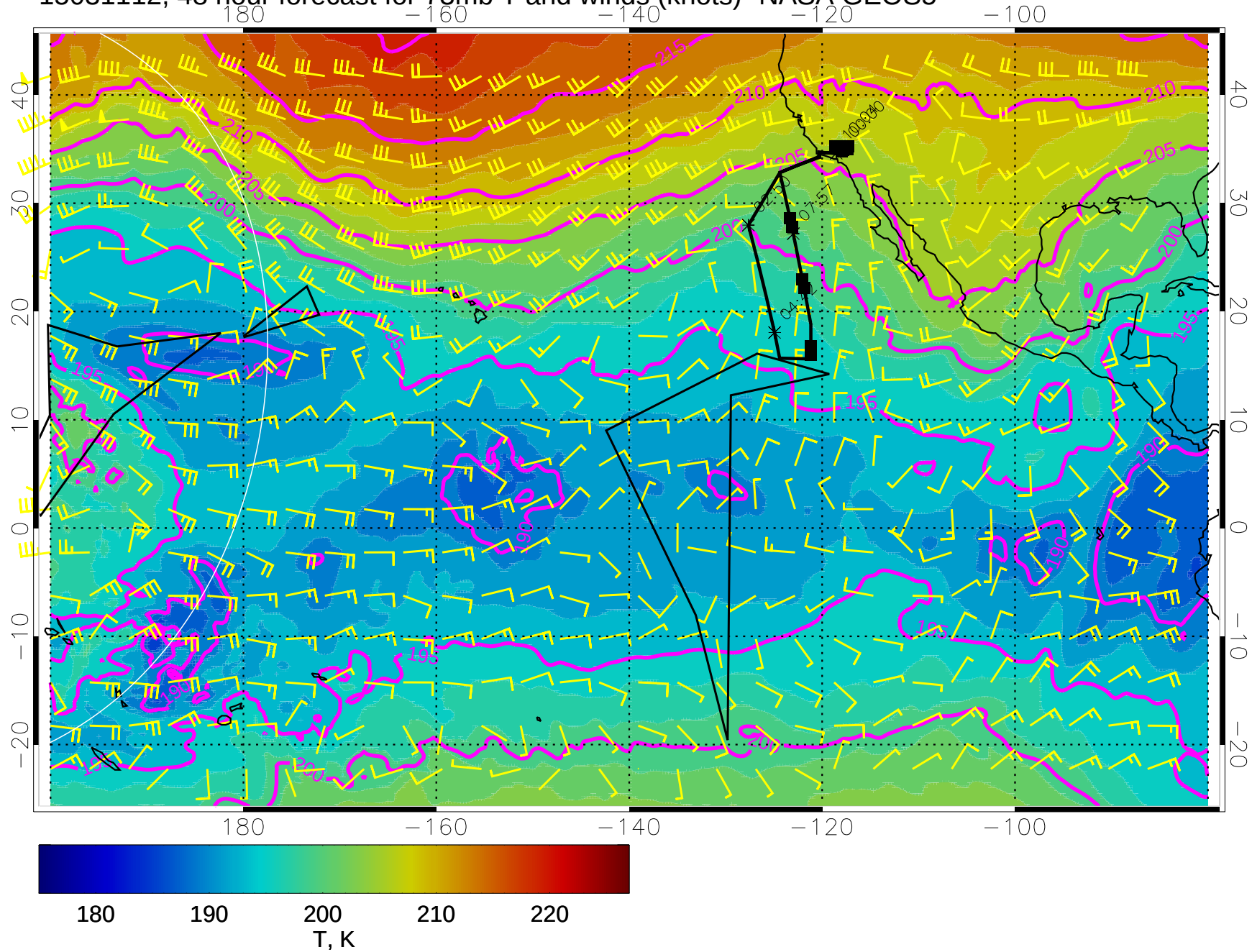
15031112, 48 hour forecast for 73mb T and winds (knots)- NASA GEOS5
