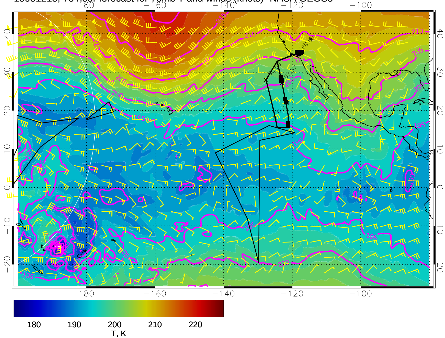
15031218, 78 hour forecast for 73mb T and winds (knots)- NASA GEOS5
