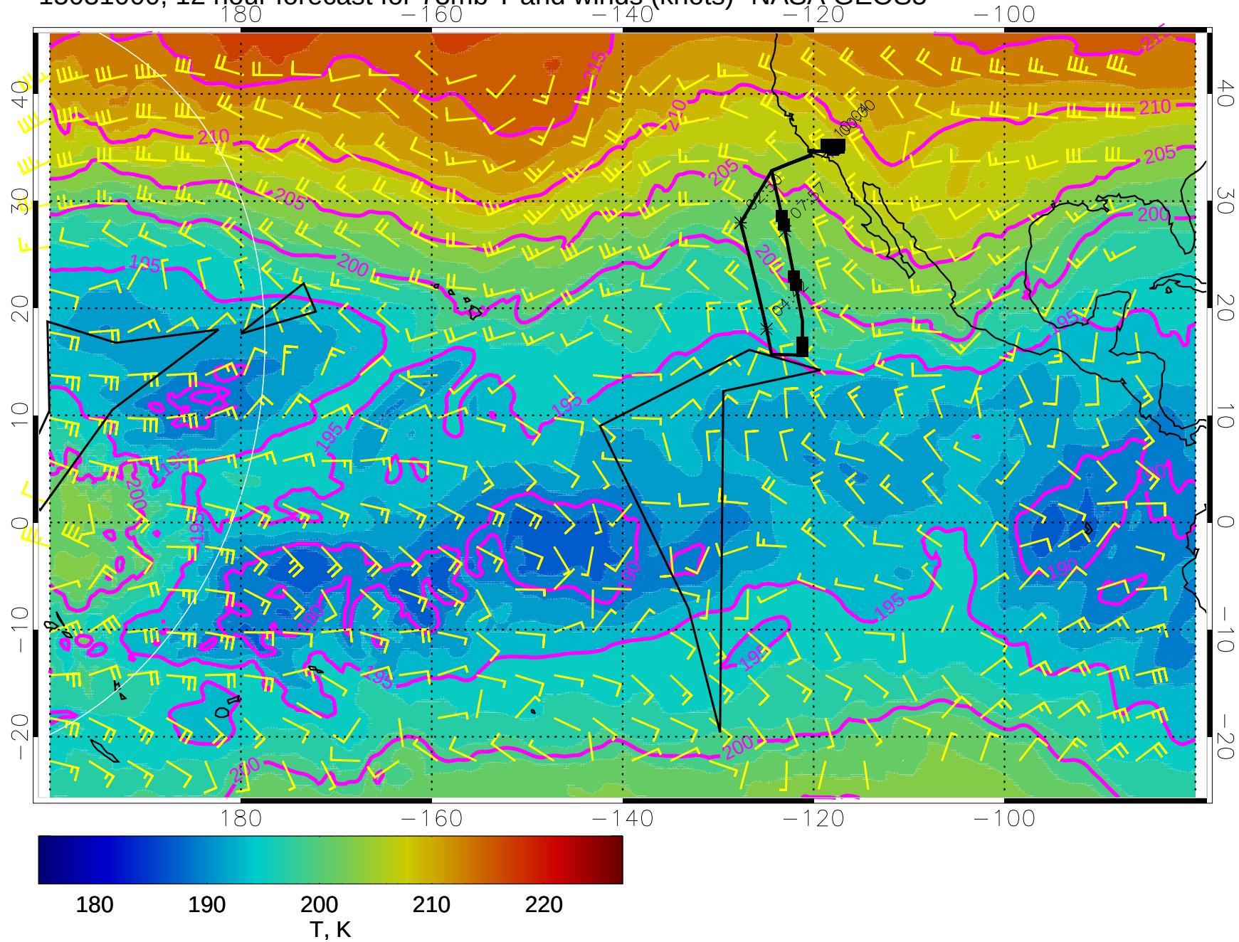
15031000, 12 hour forecast for 73mb T and winds (knots)- NASA GEOS5
