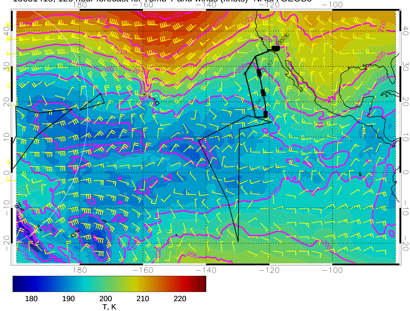
15031418, 126 hour forecast for 73mb T and winds (knots)- NASA GEOS5
