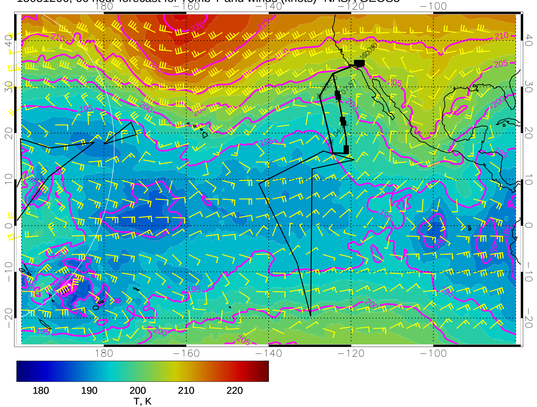
15031206, 66 hour forecast for 73mb T and winds (knots)- NASA GEOS5
