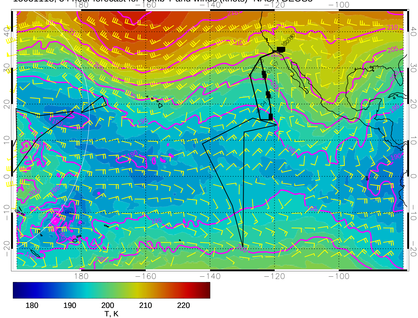
15031118, 54 hour forecast for 73mb T and winds (knots)- NASA GEOS5
