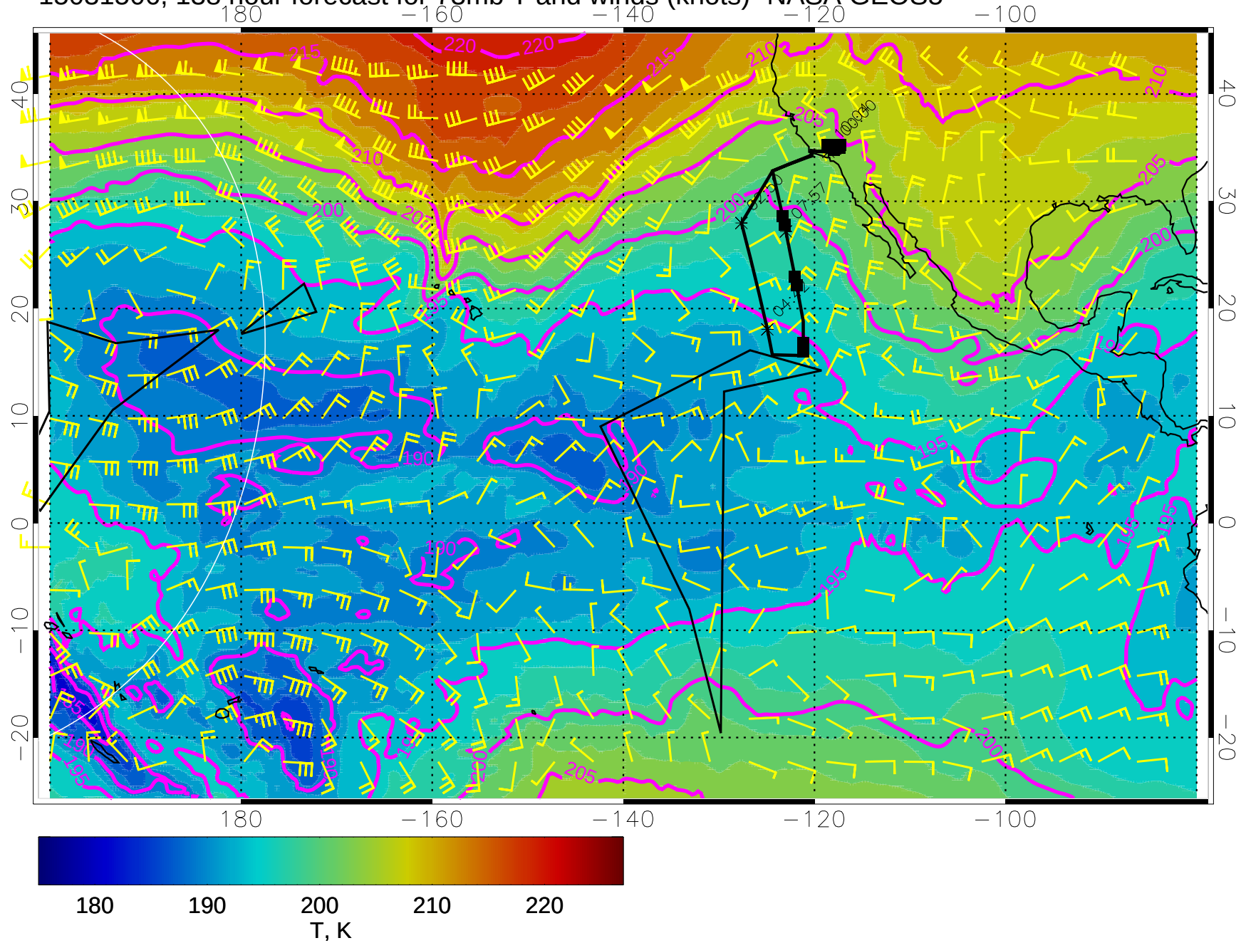
15031506, 138 hour forecast for 73mb T and winds (knots)- NASA GEOS5
