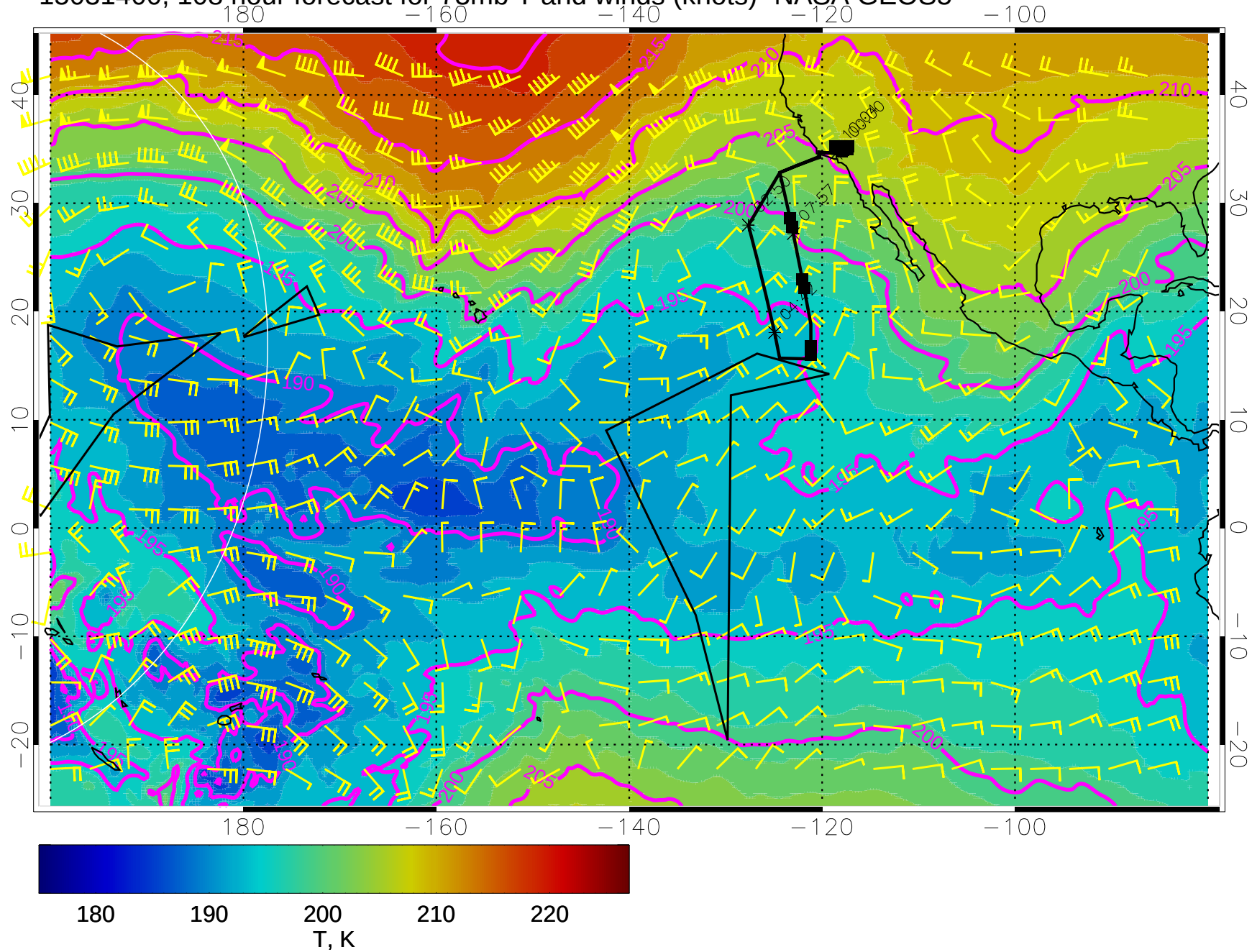
15031400, 108 hour forecast for 73mb T and winds (knots)- NASA GEOS5
