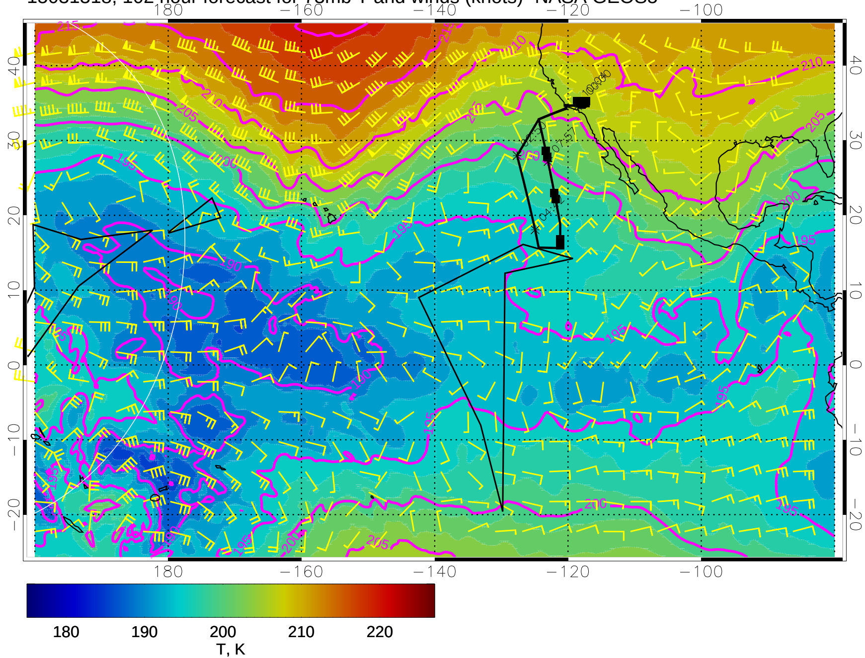
15031318, 102 hour forecast for 73mb T and winds (knots)- NASA GEOS5
