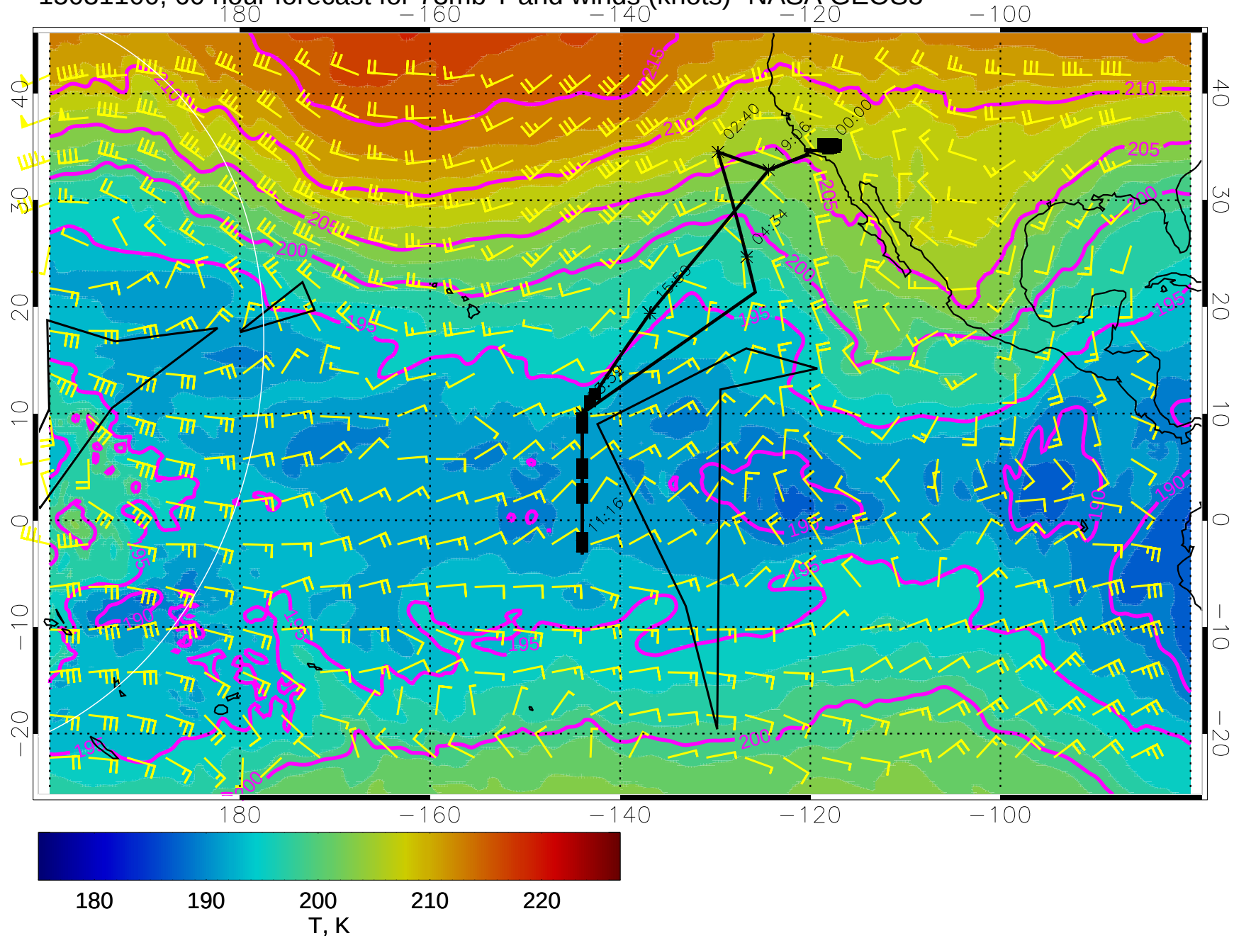
15031100, 60 hour forecast for 73mb T and winds (knots)- NASA GEOS5
