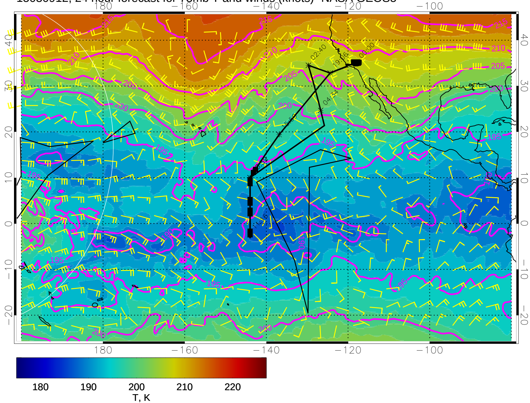
15030912, 24 hour forecast for 73mb T and winds (knots)- NASA GEOS5
