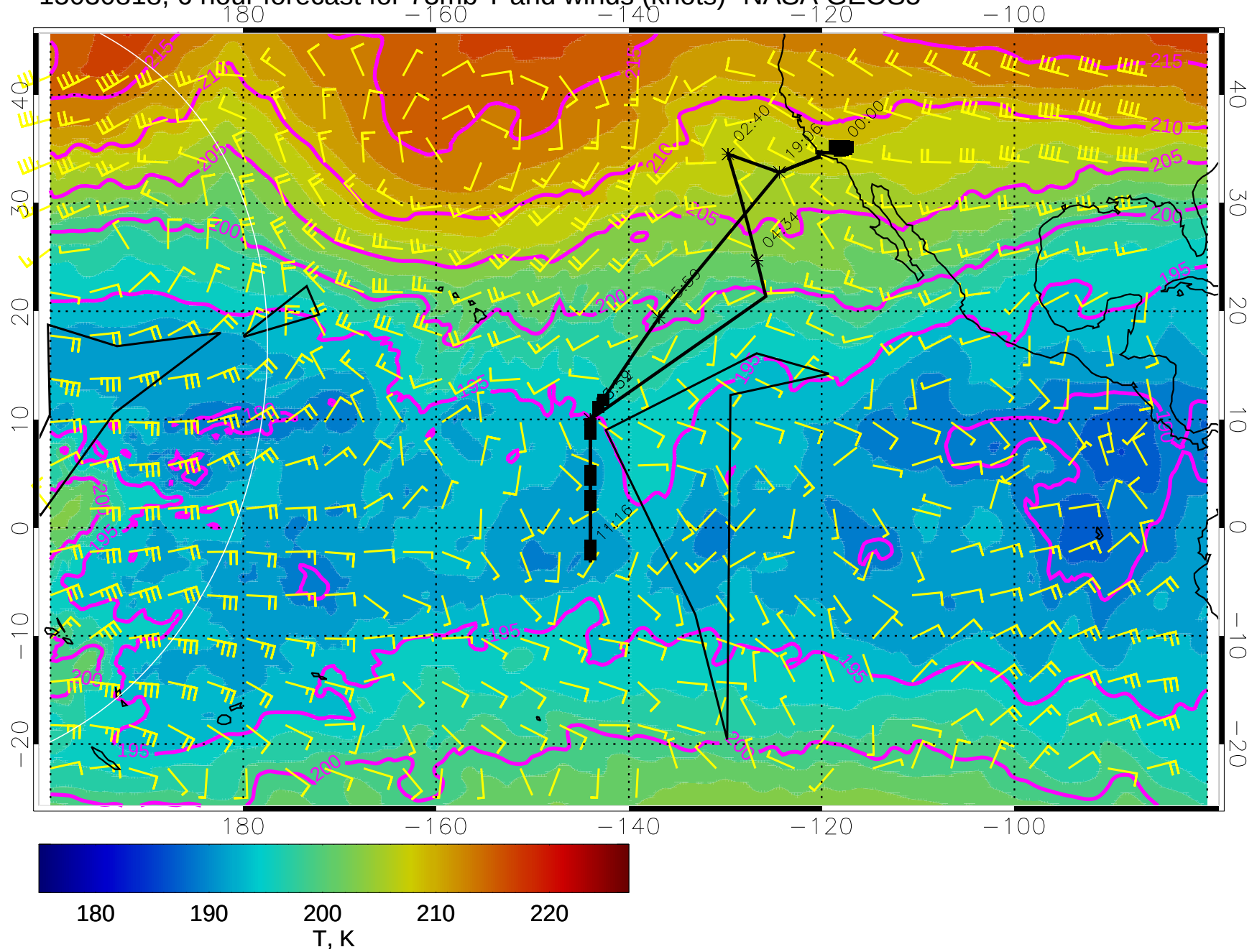
15030818, 6 hour forecast for 73mb T and winds (knots)- NASA GEOS5
