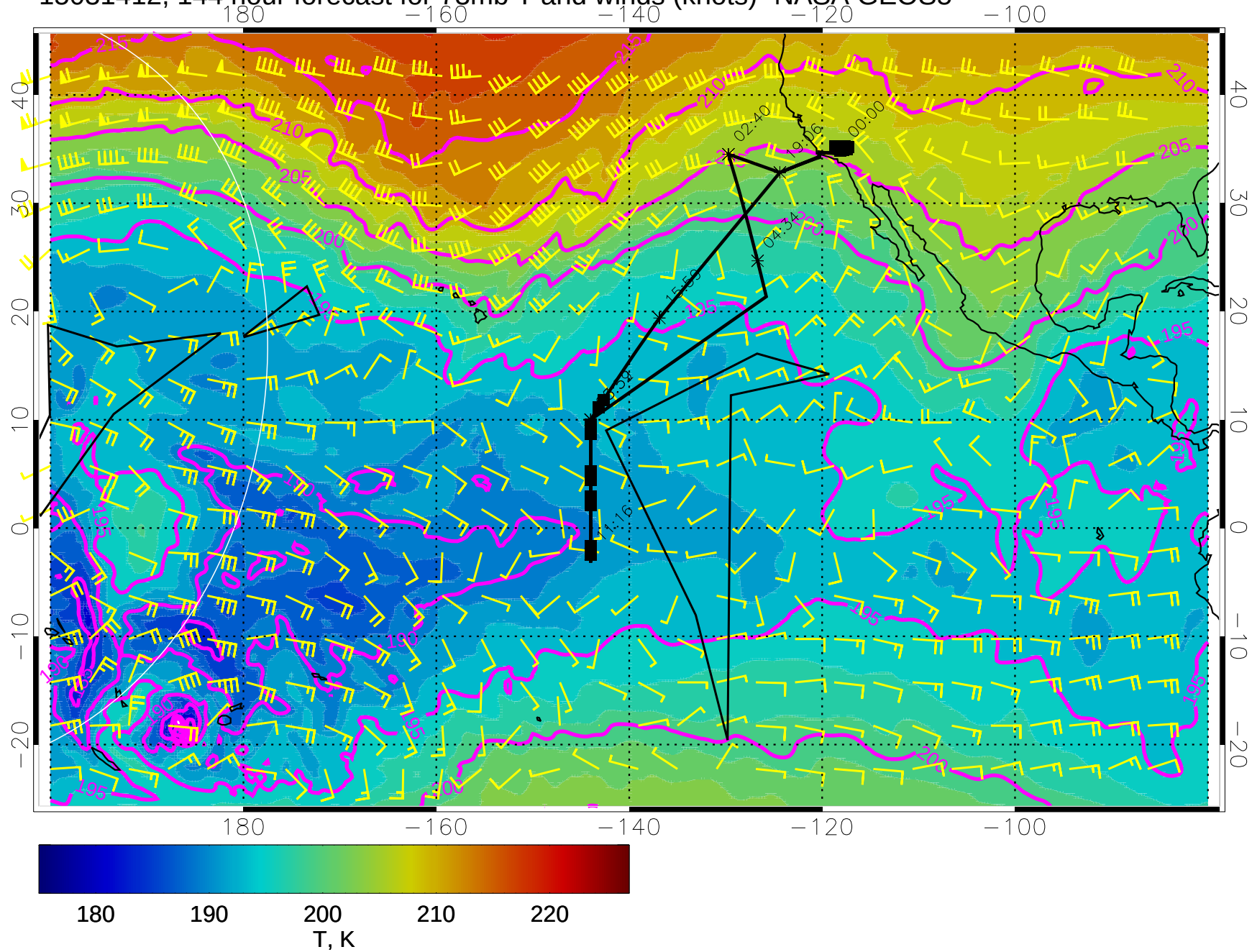
15031412, 144 hour forecast for 73mb T and winds (knots)- NASA GEOS5
