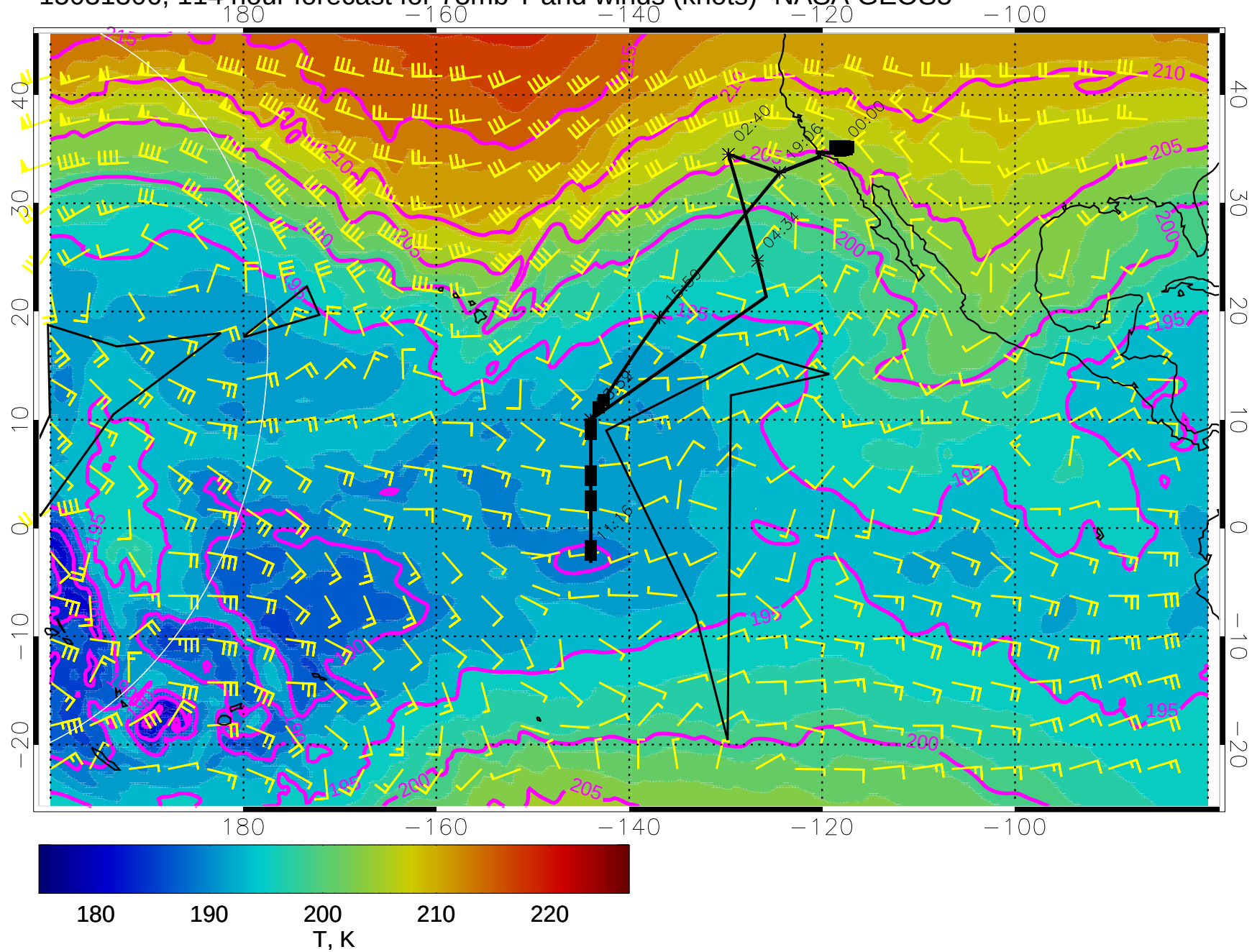
15031306, 114 hour forecast for 73mb T and winds (knots)- NASA GEOS5
