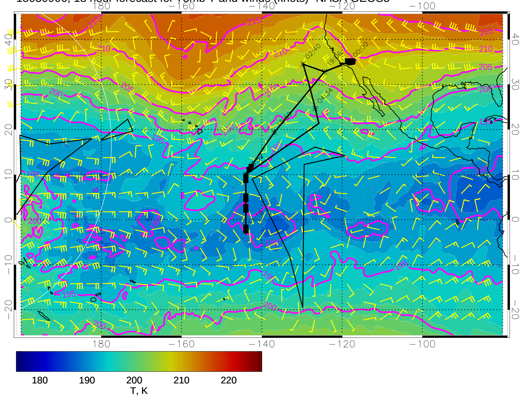
15030906, 18 hour forecast for 73mb T and winds (knots)- NASA GEOS5
