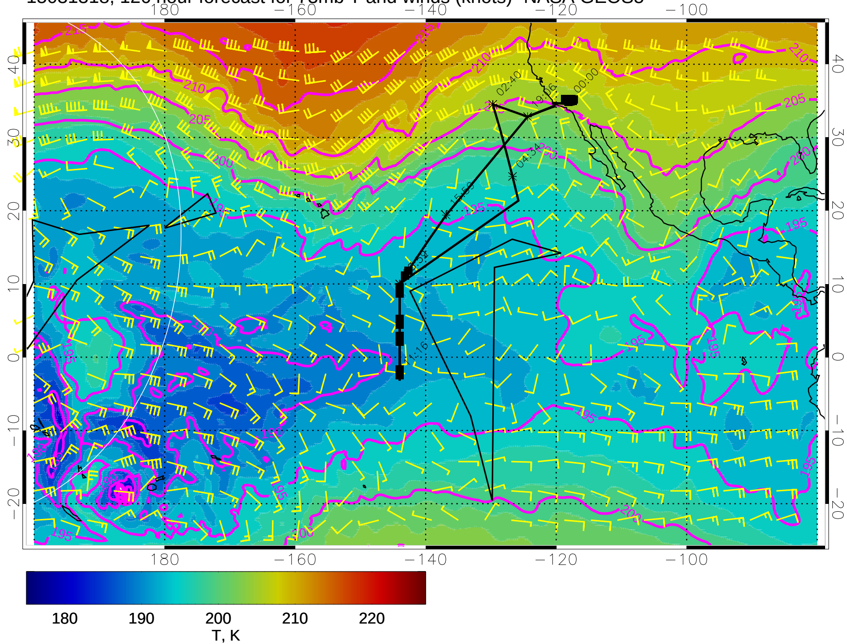
15031318, 126 hour forecast for 73mb T and winds (knots)- NASA GEOS5
