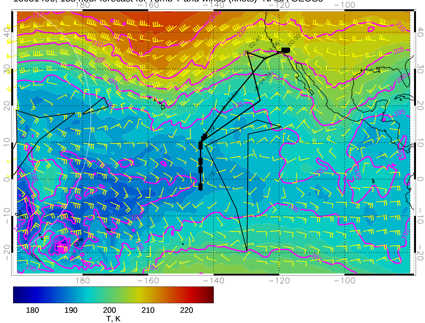
15031406, 138 hour forecast for 73mb T and winds (knots)- NASA GEOS5
