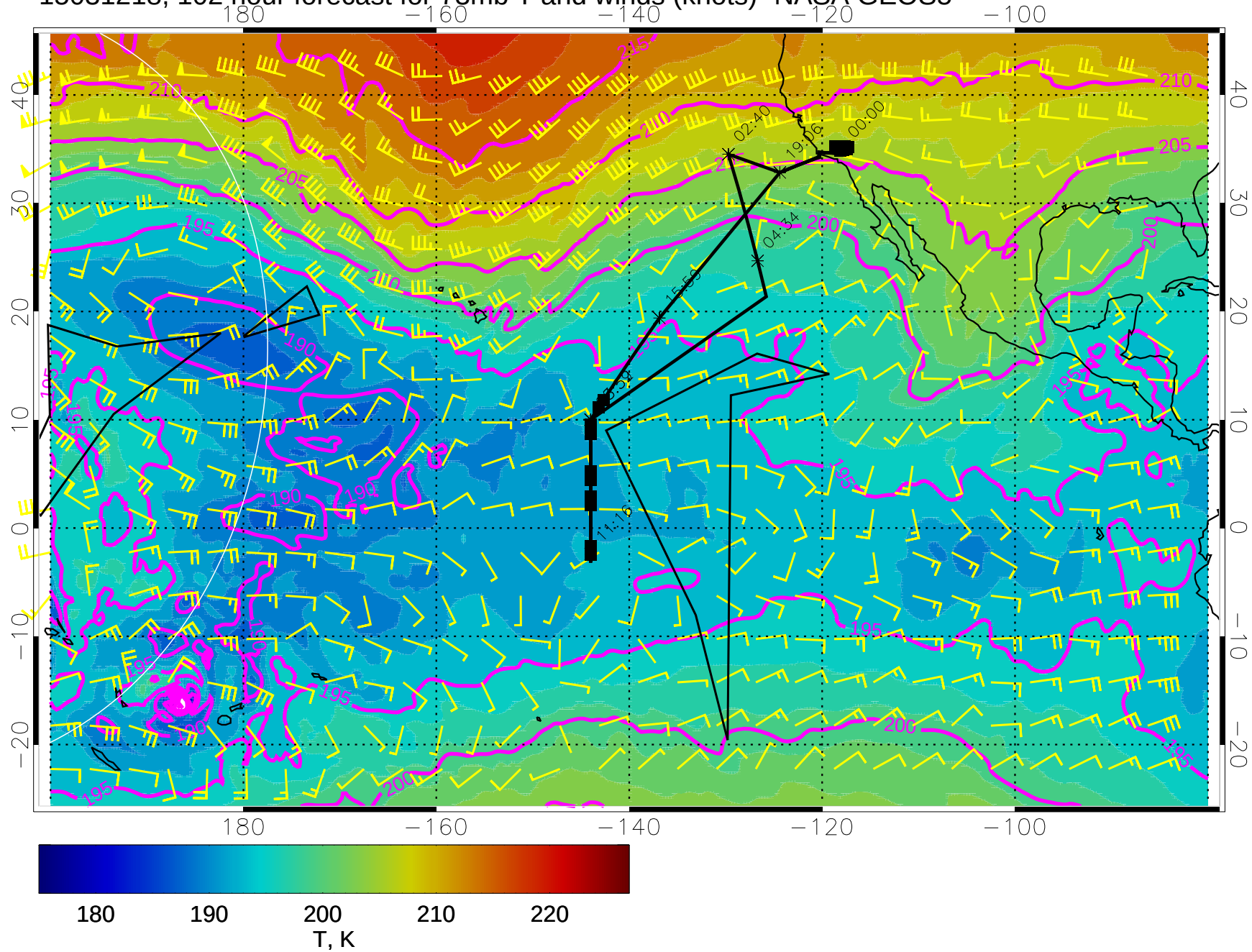
15031218, 102 hour forecast for 73mb T and winds (knots)- NASA GEOS5
