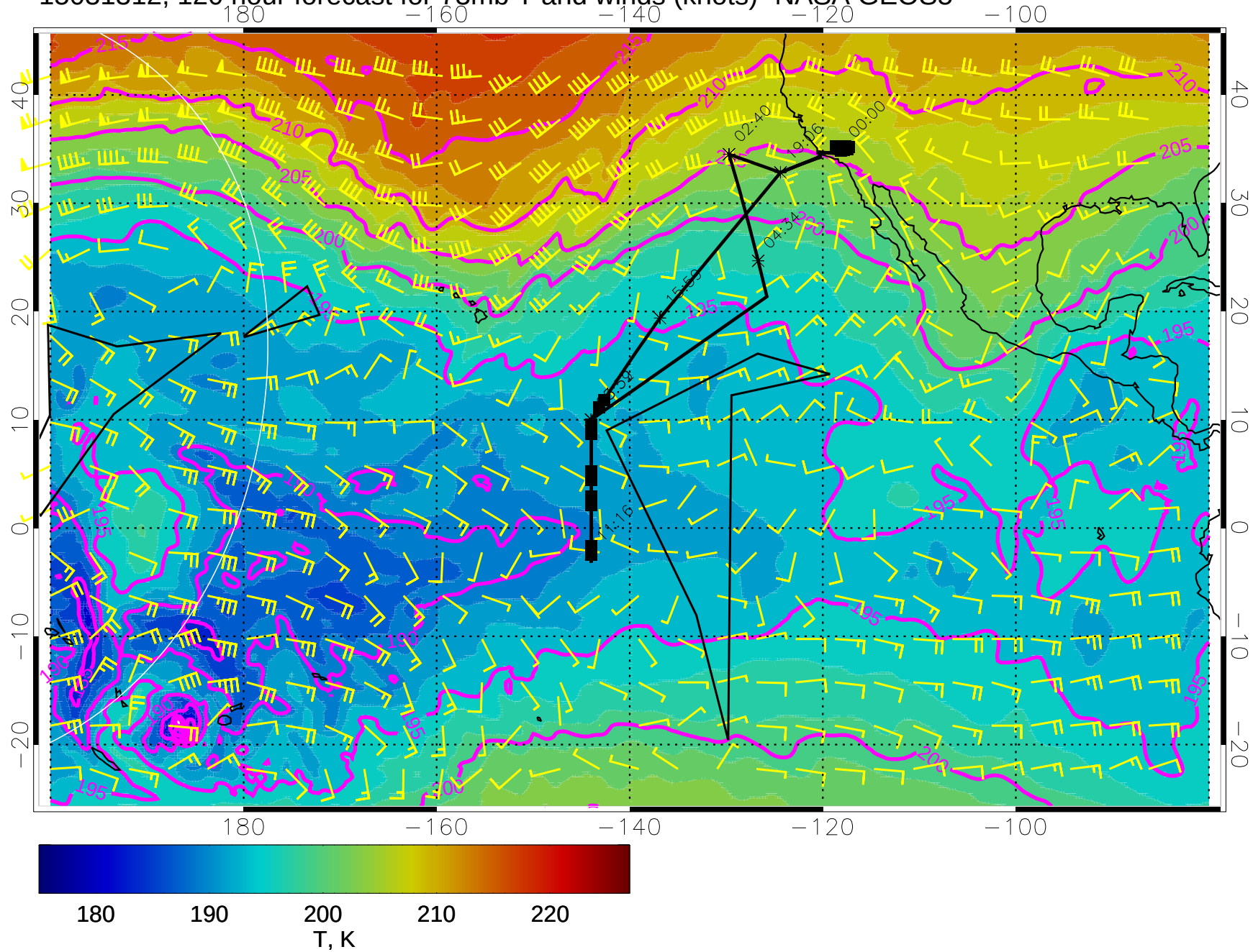
15031312, 120 hour forecast for 73mb T and winds (knots)- NASA GEOS5
