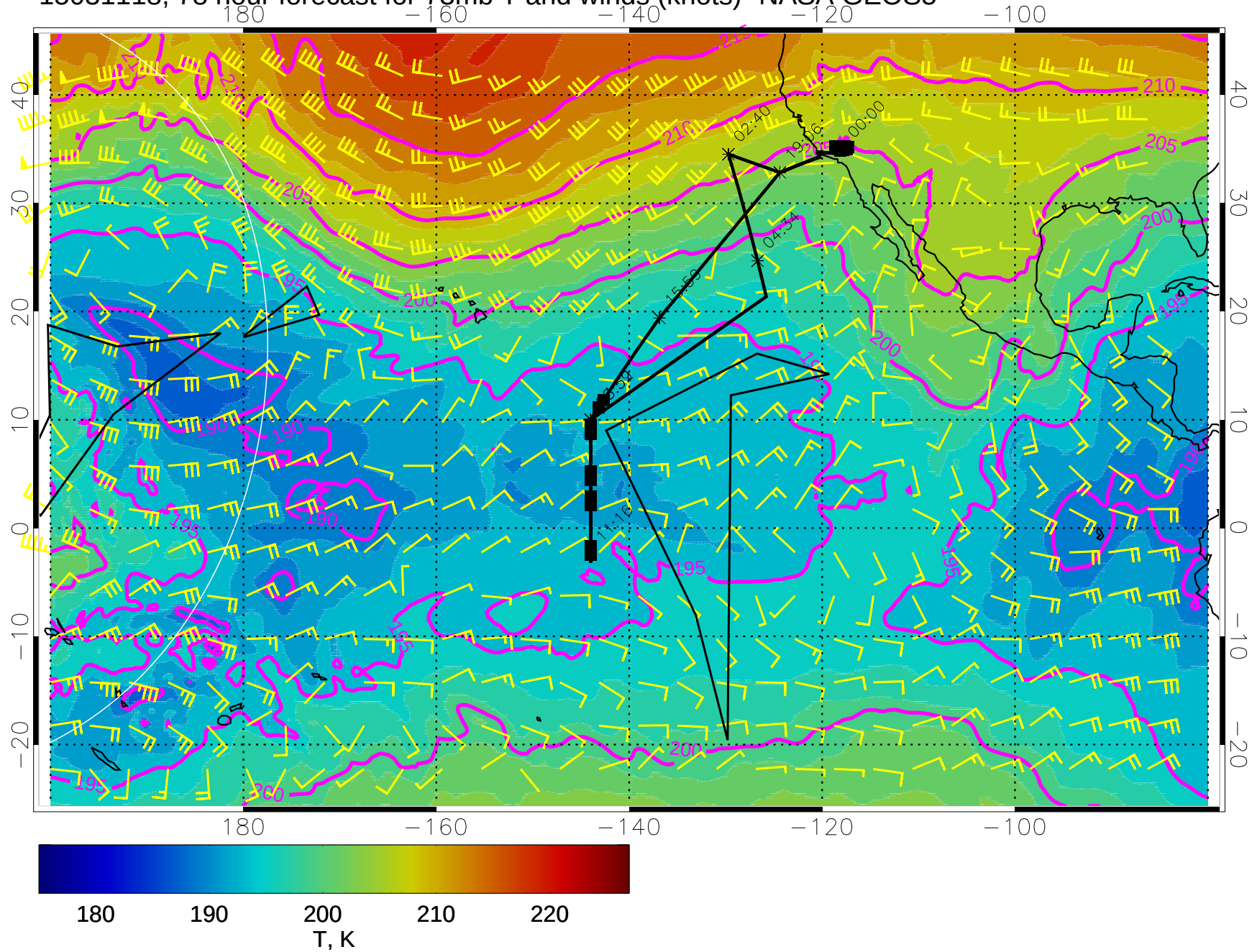
15031118, 78 hour forecast for 73mb T and winds (knots)- NASA GEOS5
