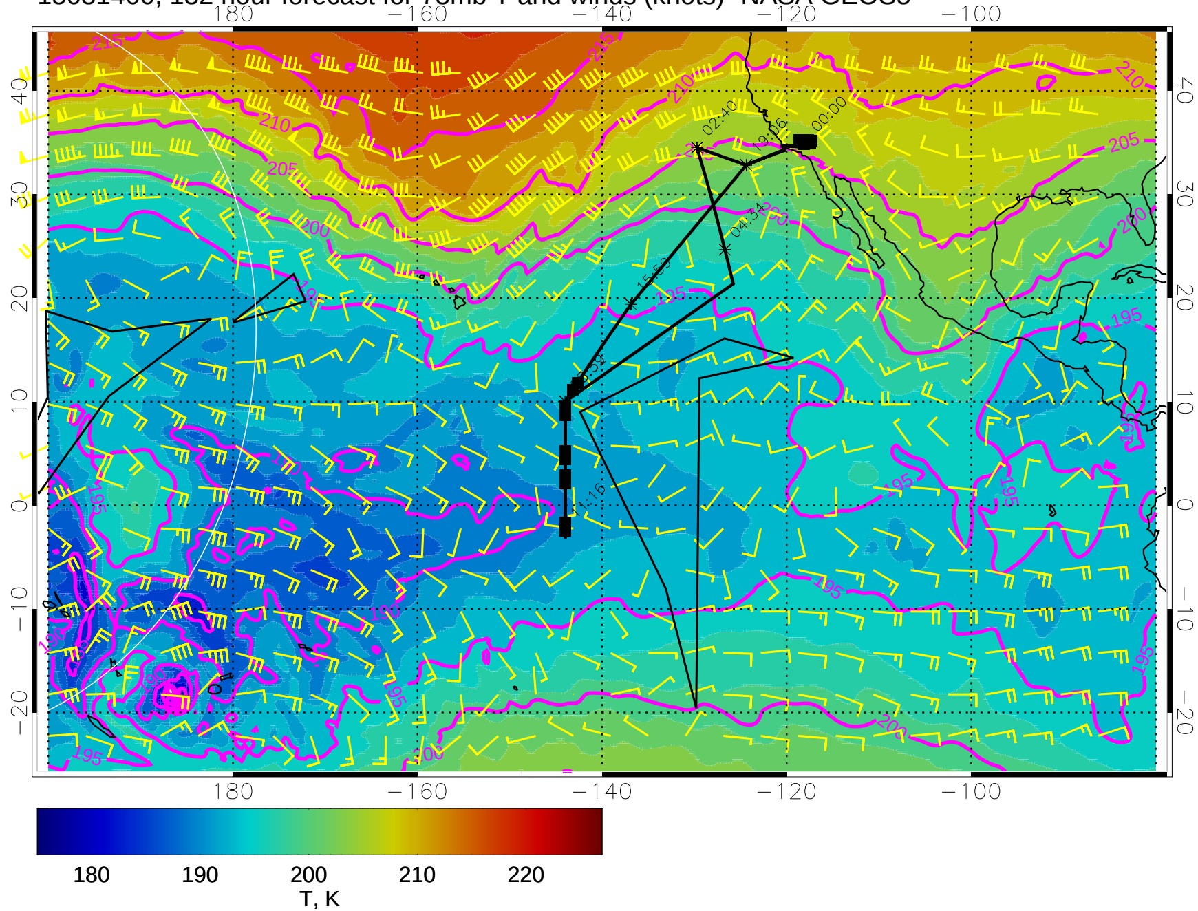
15031400, 132 hour forecast for 73mb T and winds (knots)- NASA GEOS5
