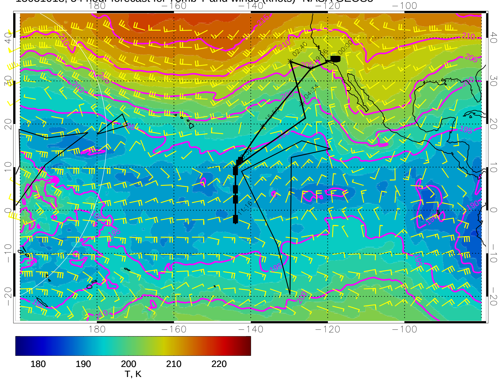
15031018, 54 hour forecast for 73mb T and winds (knots)- NASA GEOS5
