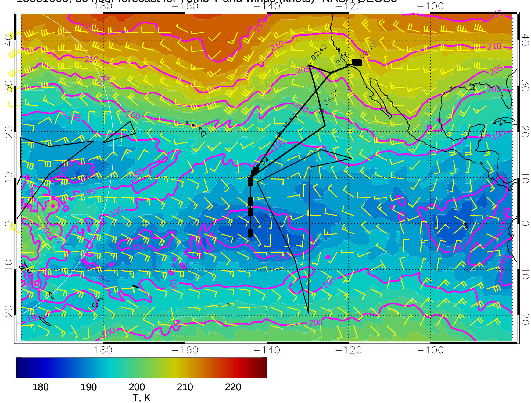
15031000, 36 hour forecast for 73mb T and winds (knots)- NASA GEOS5
