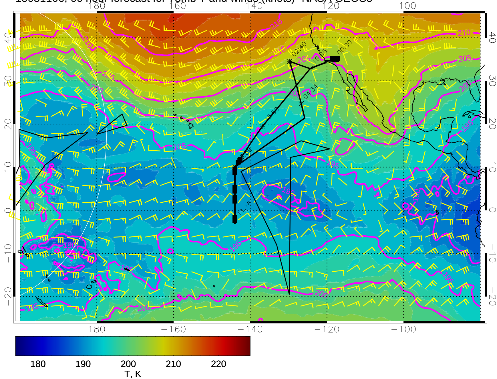
15031106, 66 hour forecast for 73mb T and winds (knots)- NASA GEOS5
