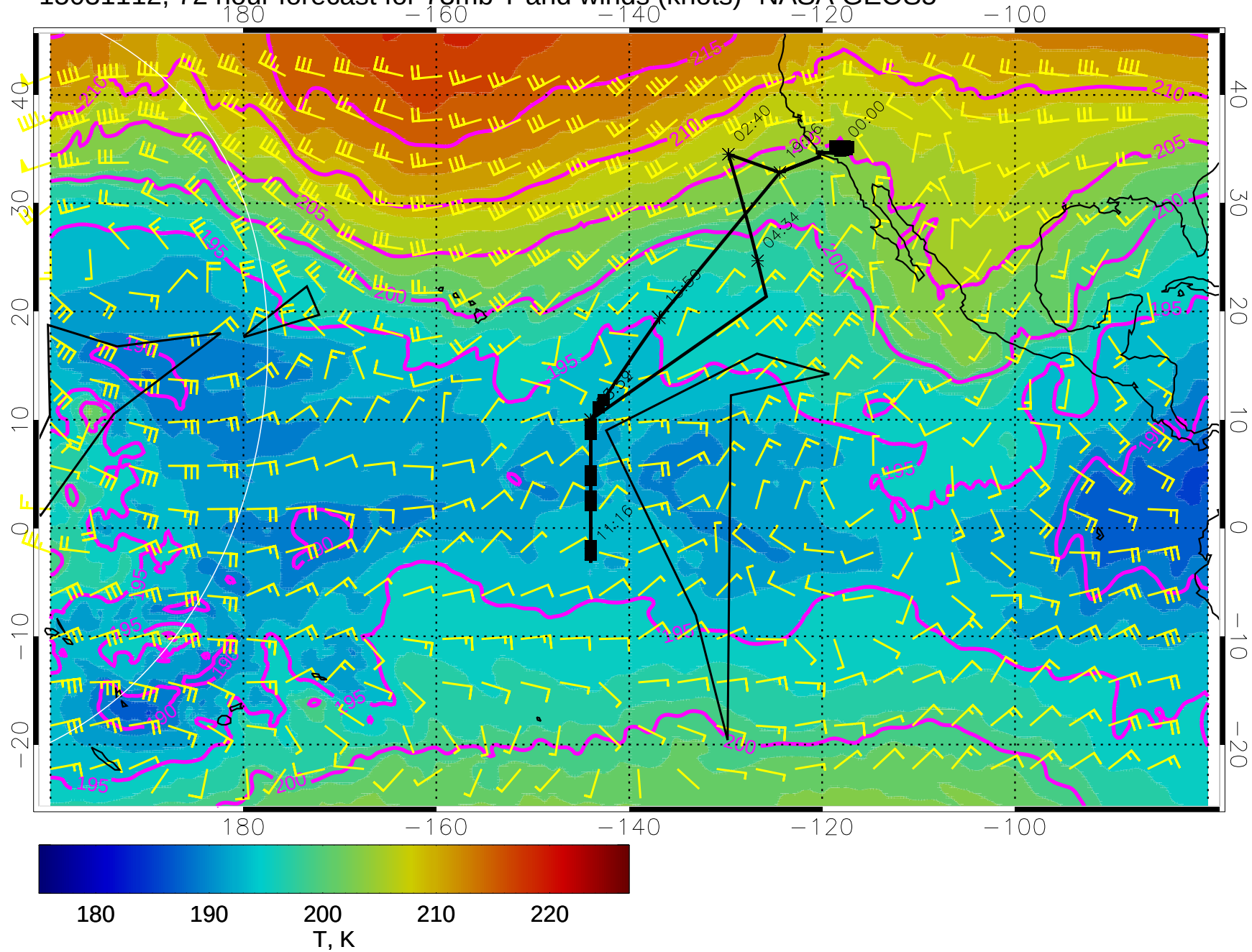
15031112, 72 hour forecast for 73mb T and winds (knots)- NASA GEOS5
