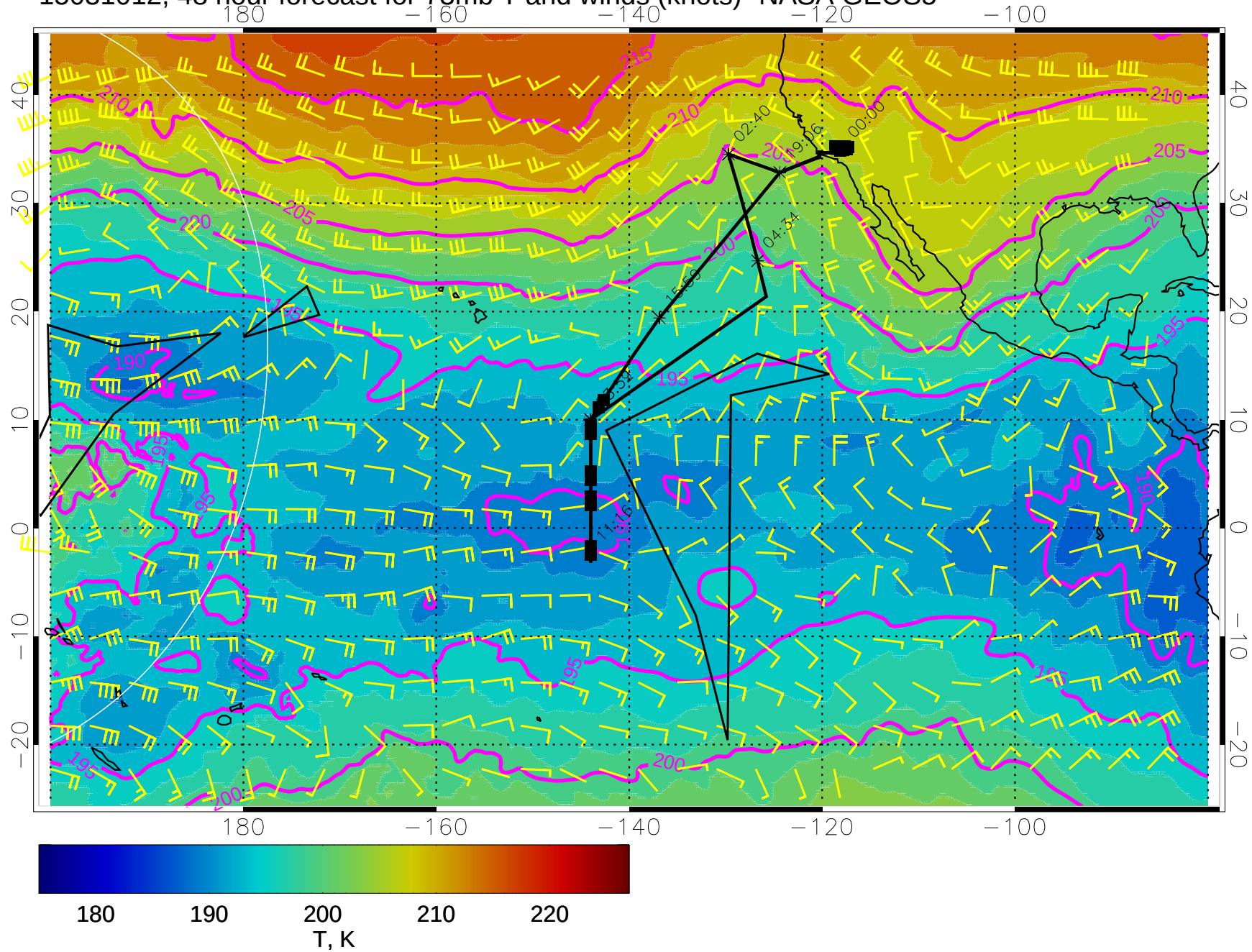
15031012, 48 hour forecast for 73mb T and winds (knots)- NASA GEOS5
