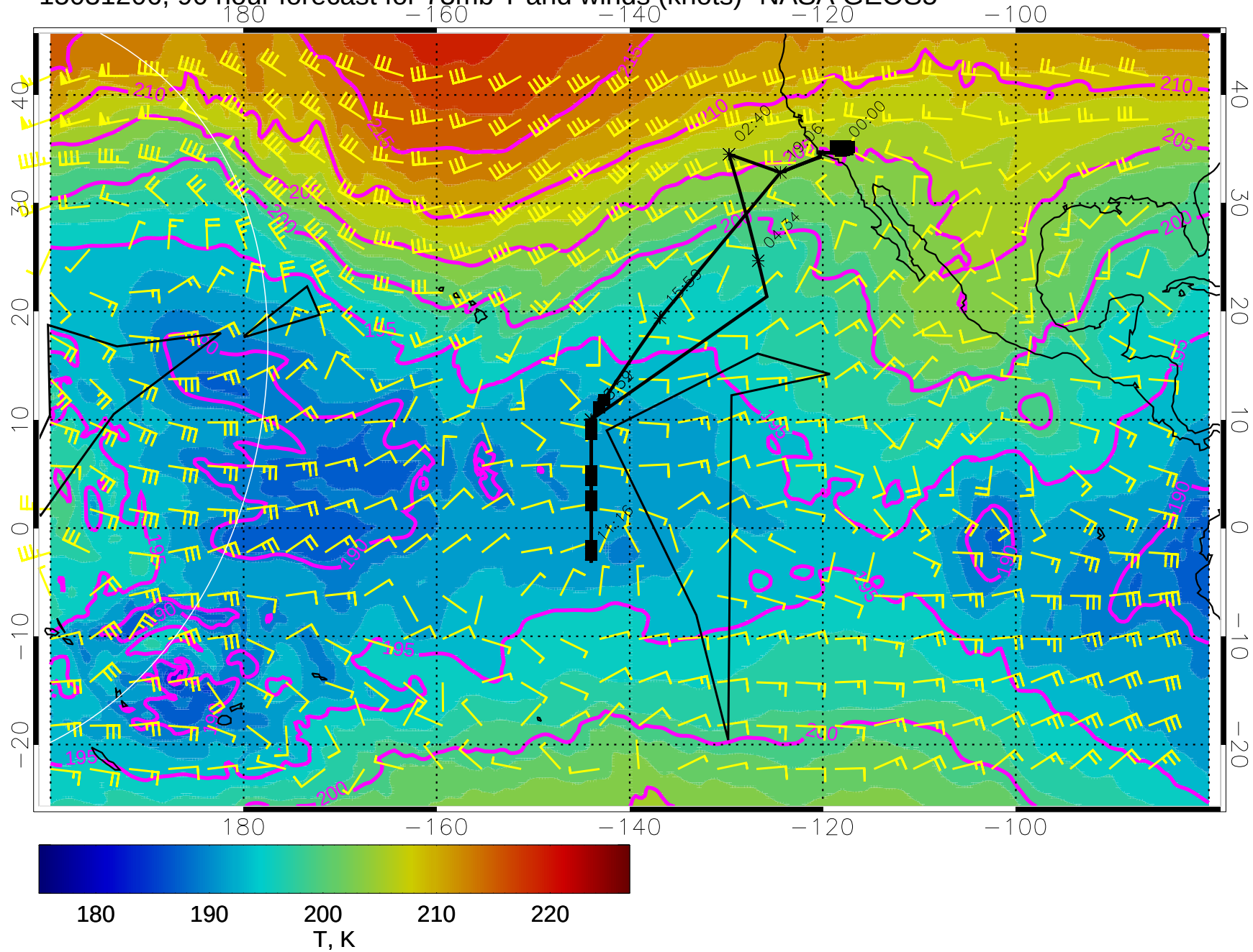
15031206, 90 hour forecast for 73mb T and winds (knots)- NASA GEOS5
