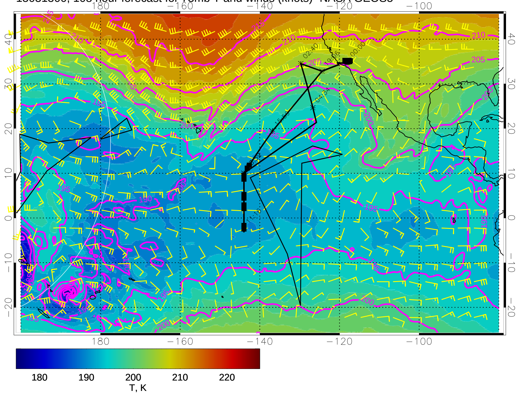
15031300, 108 hour forecast for 73mb T and winds (knots)- NASA GEOS5
