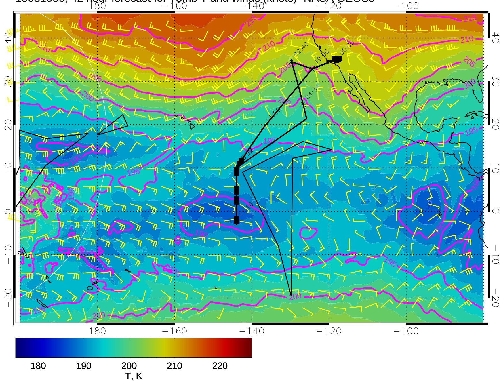
15031006, 42 hour forecast for 73mb T and winds (knots)- NASA GEOS5
