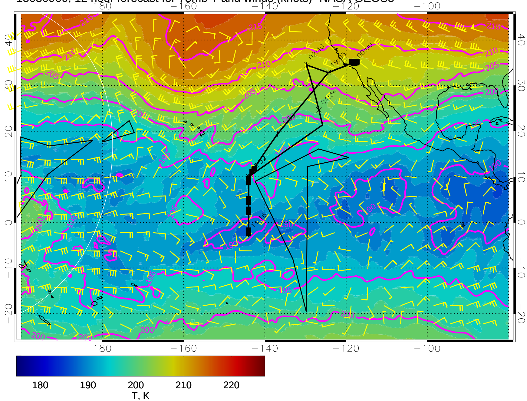
15030900, 12 hour forecast for 73mb T and winds (knots)- NASA GEOS5
