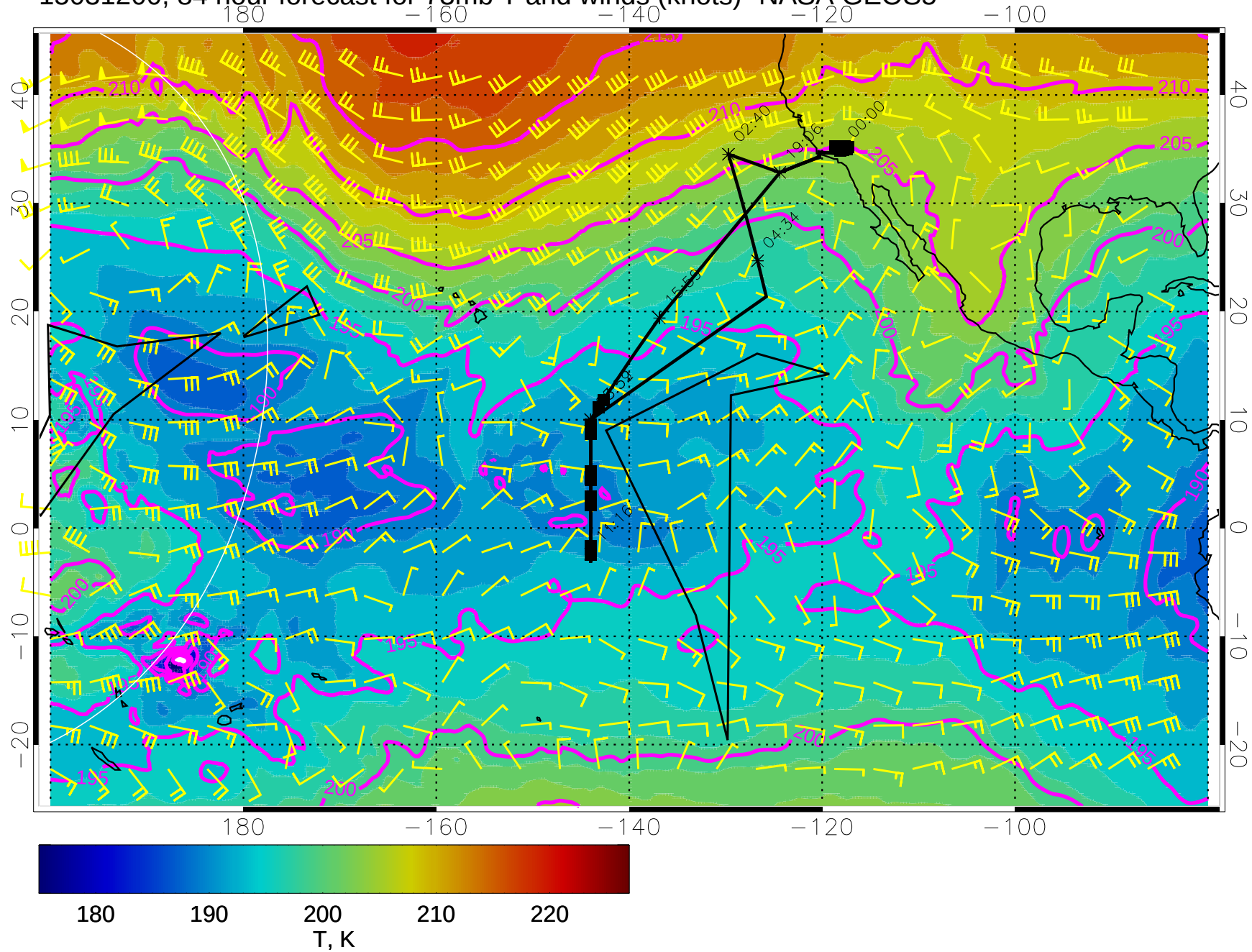
15031200, 84 hour forecast for 73mb T and winds (knots)- NASA GEOS5
