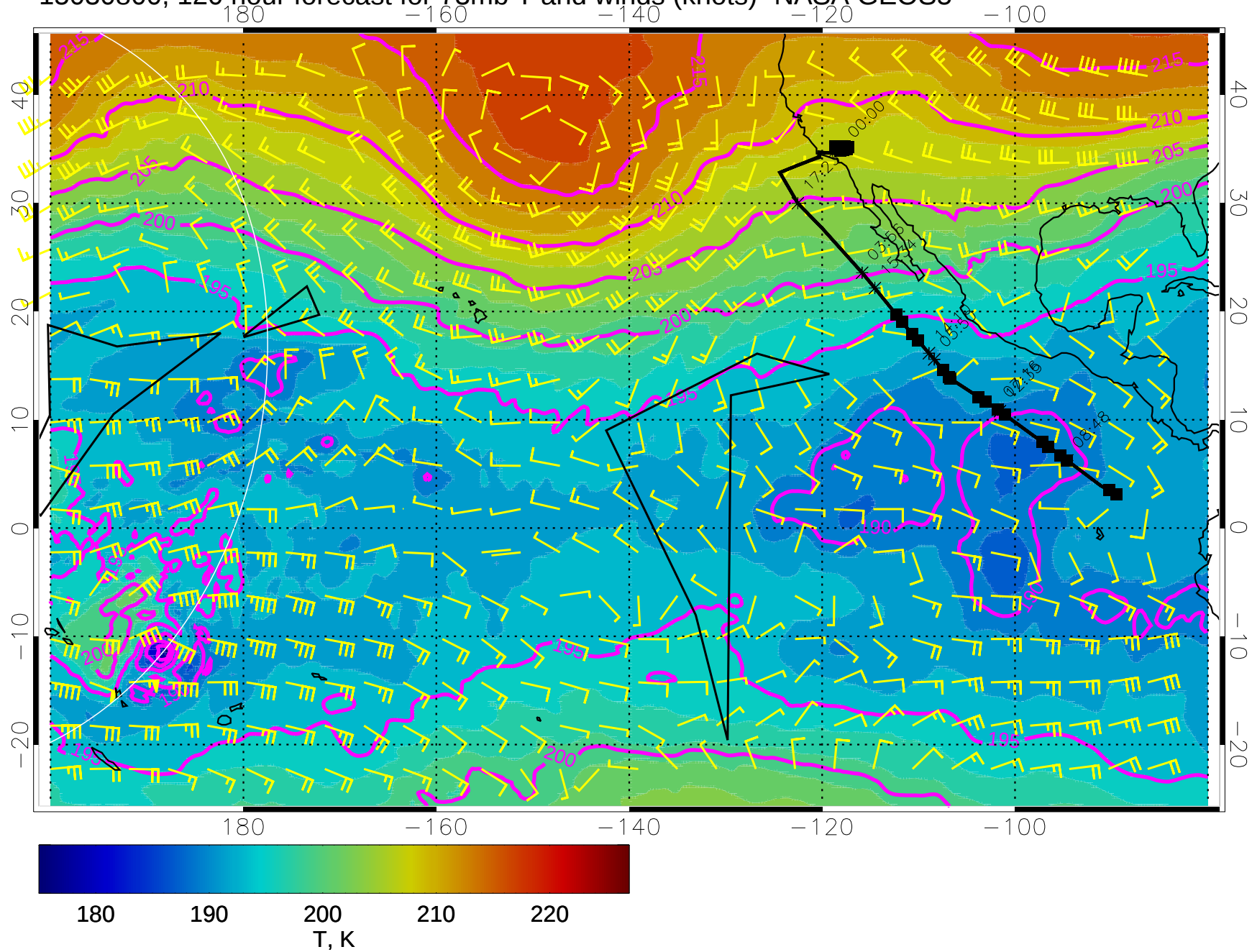
15030800, 120 hour forecast for 73mb T and winds (knots)- NASA GEOS5
