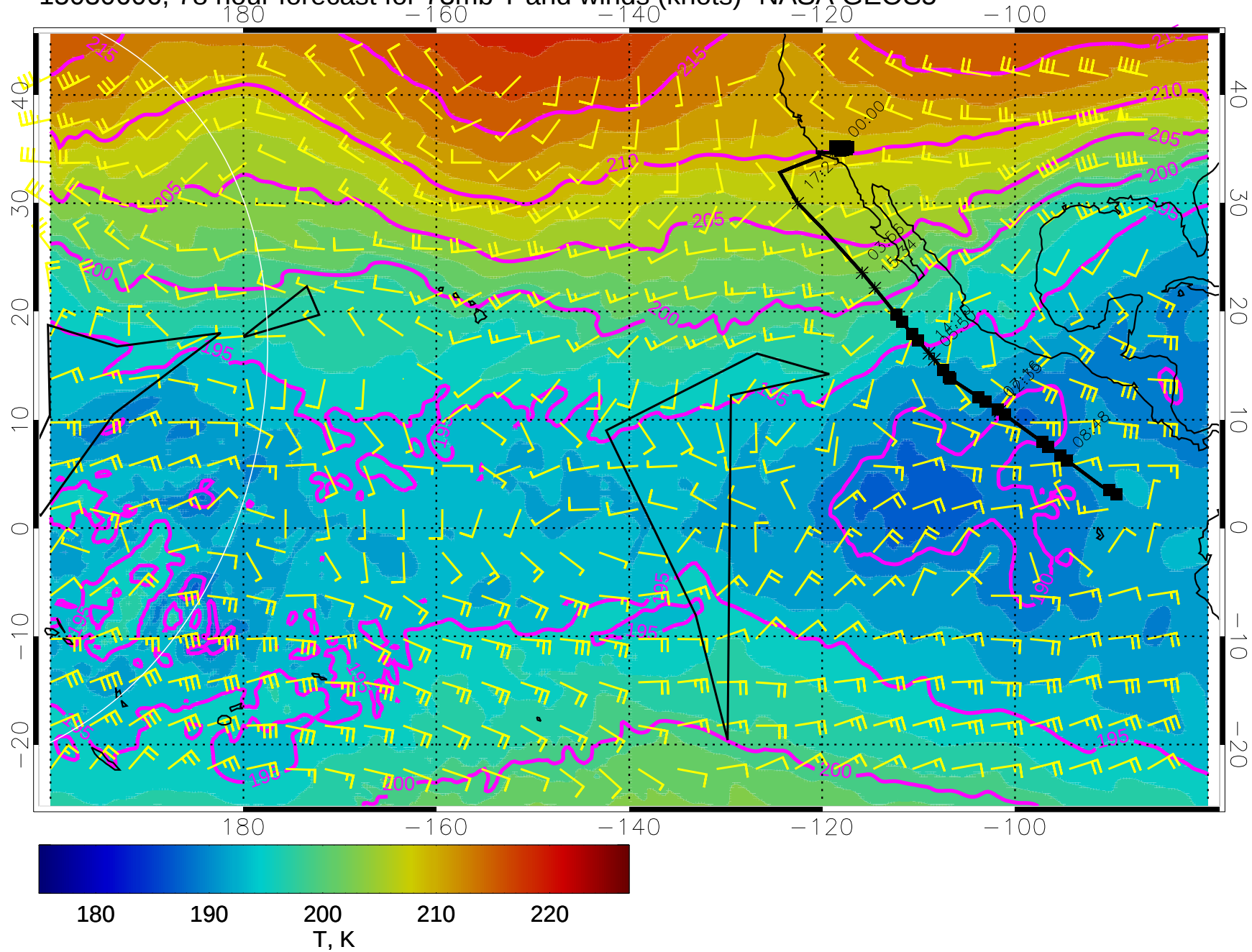
15030606, 78 hour forecast for 73mb T and winds (knots)- NASA GEOS5
