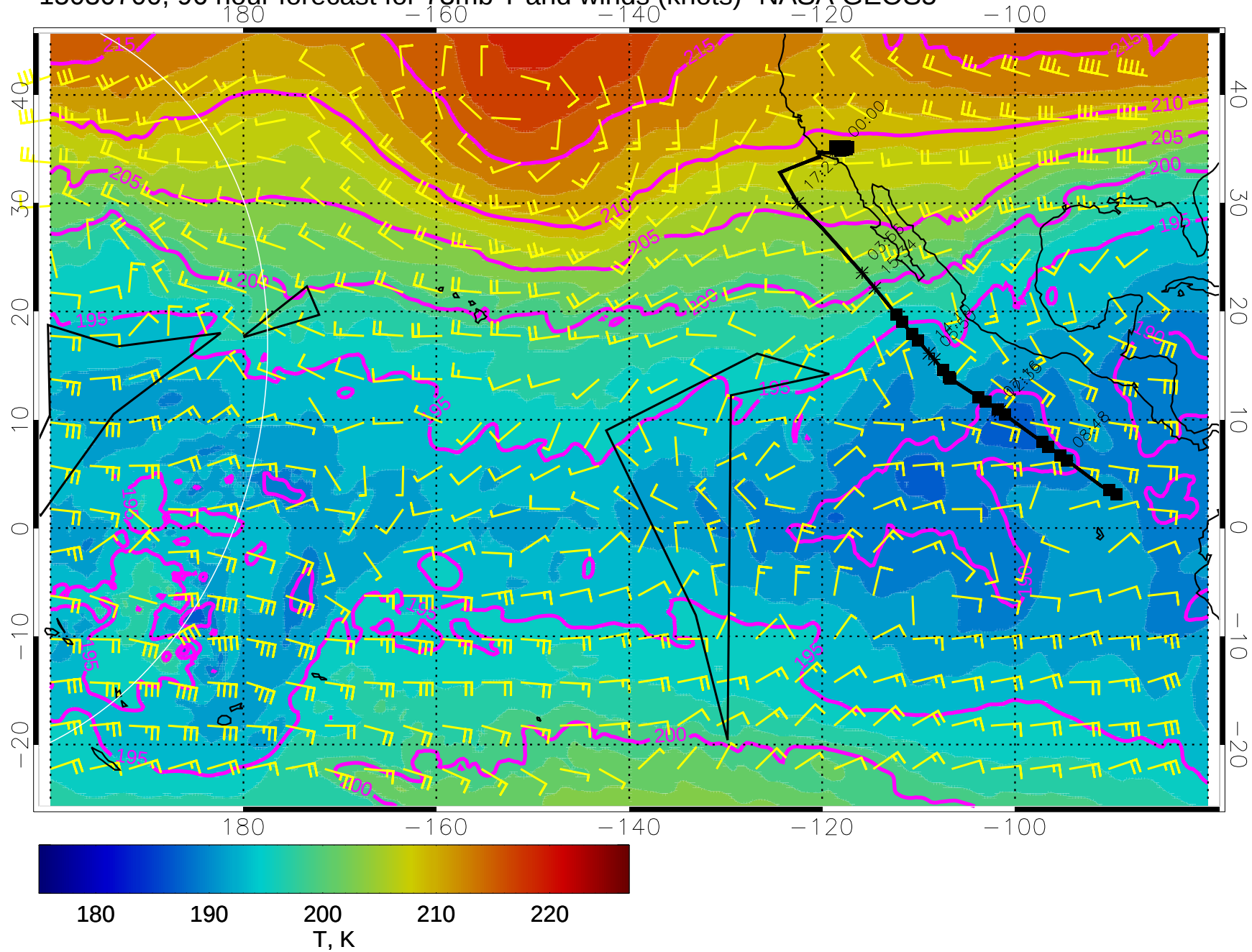
15030700, 96 hour forecast for 73mb T and winds (knots)- NASA GEOS5
