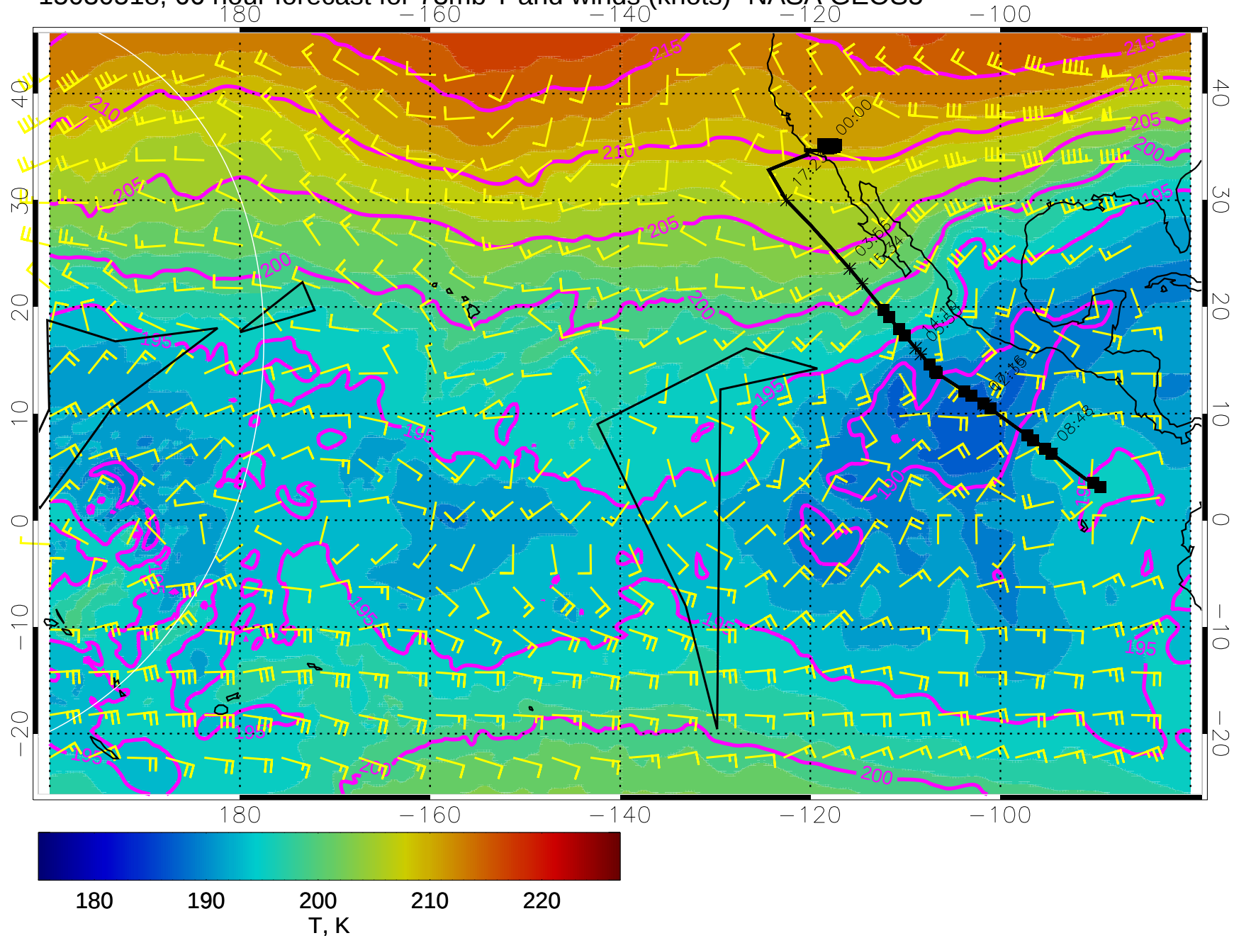
15030518, 66 hour forecast for 73mb T and winds (knots)- NASA GEOS5
