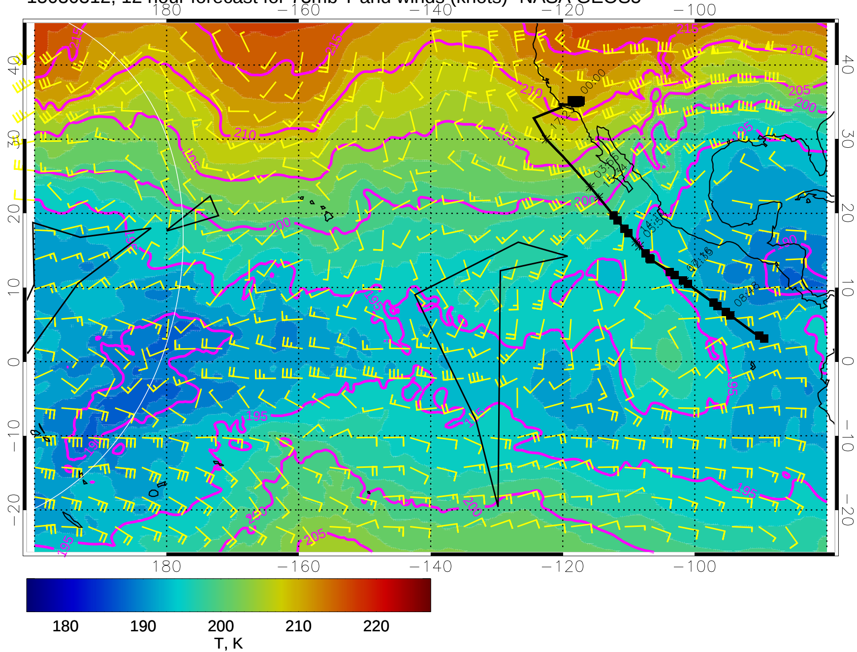
15030312, 12 hour forecast for 73mb T and winds (knots)- NASA GEOS5
