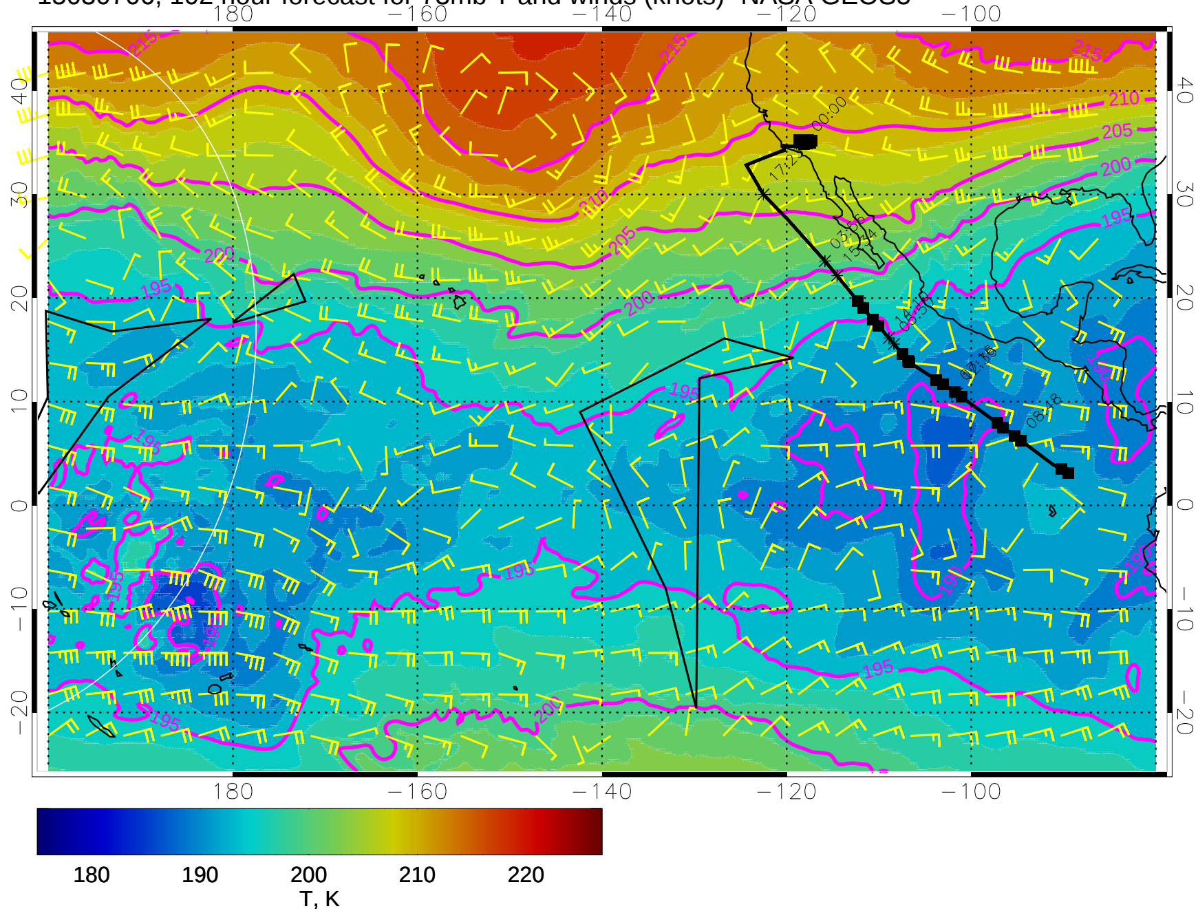
15030706, 102 hour forecast for 73mb T and winds (knots)- NASA GEOS5
