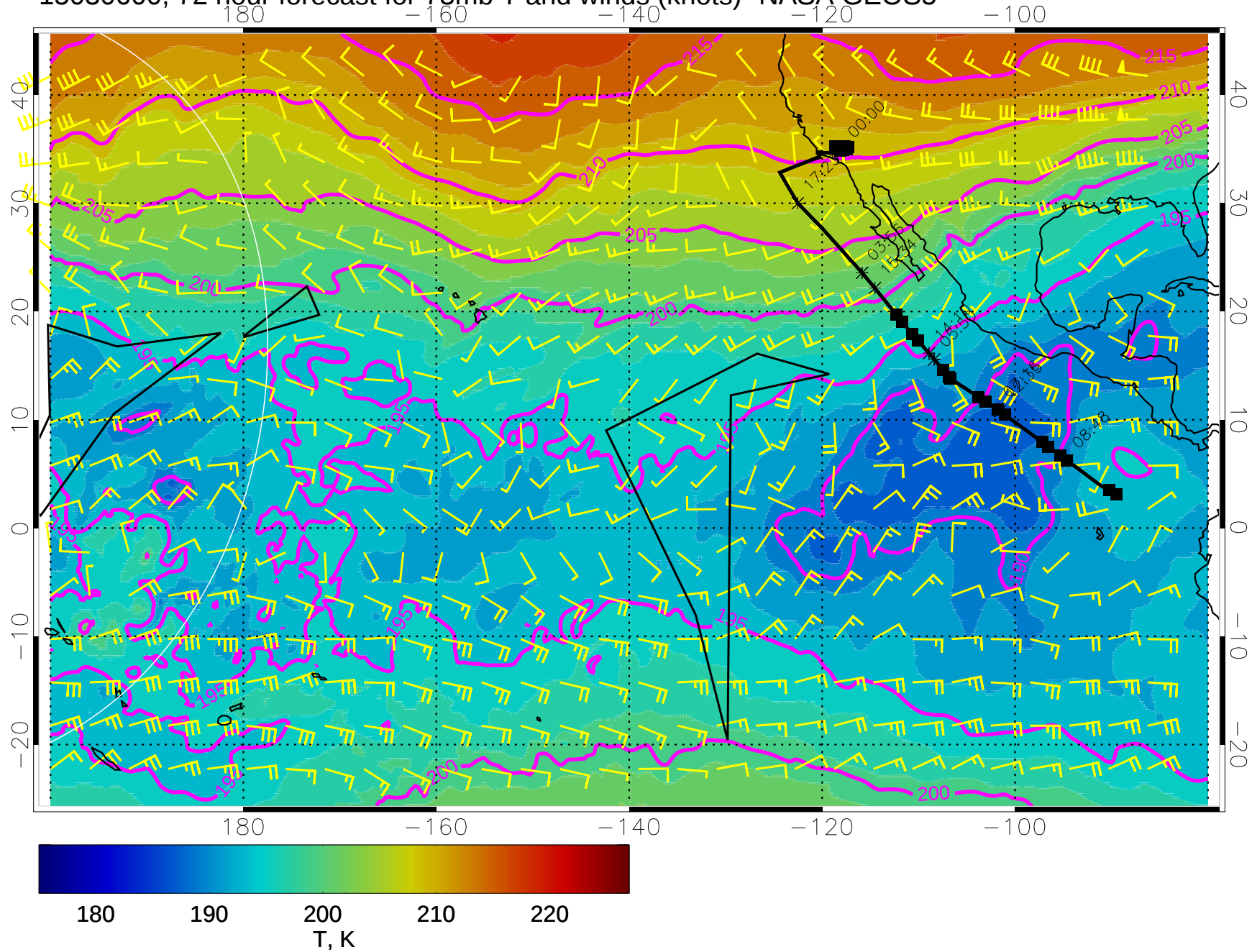
15030600, 72 hour forecast for 73mb T and winds (knots)- NASA GEOS5
