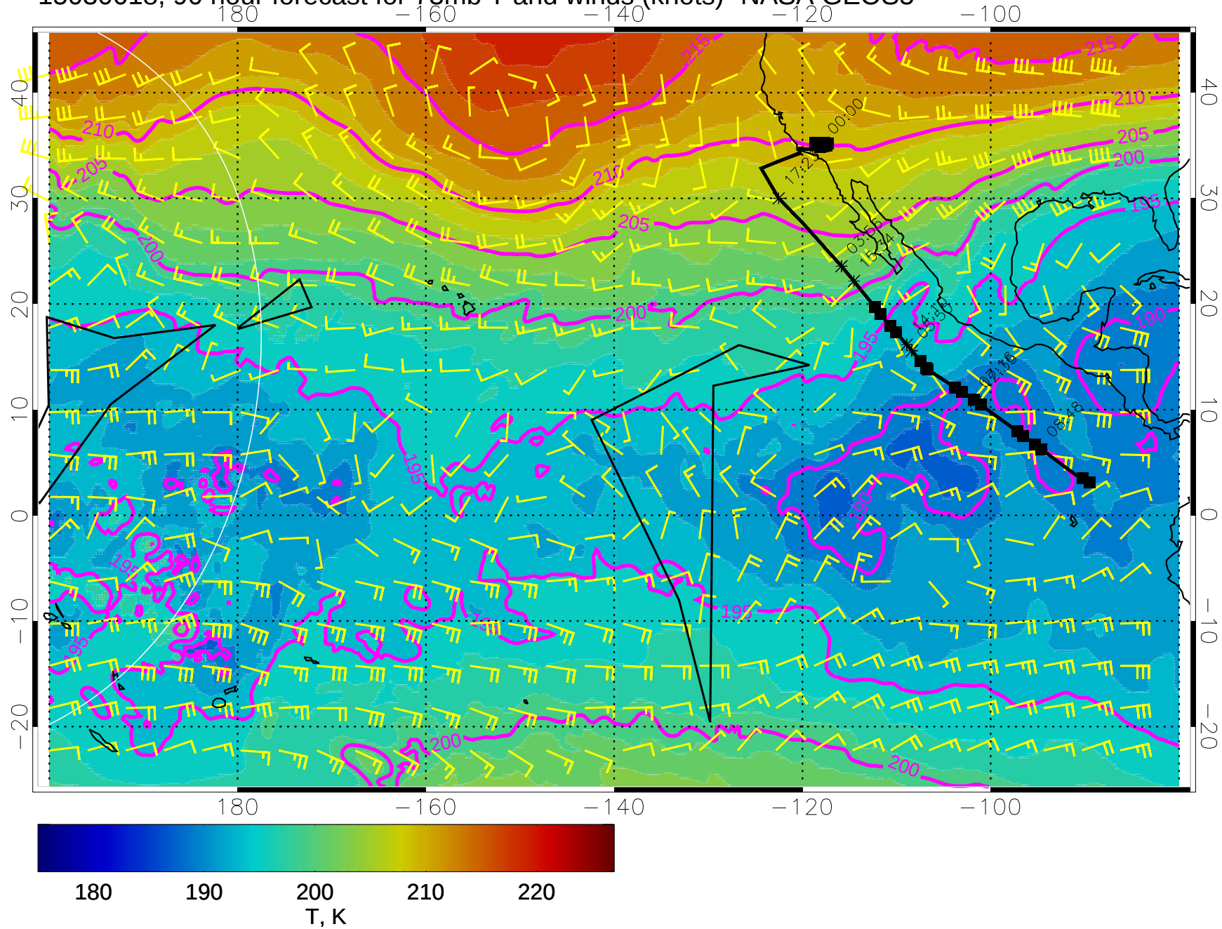
15030618, 90 hour forecast for 73mb T and winds (knots)- NASA GEOS5
