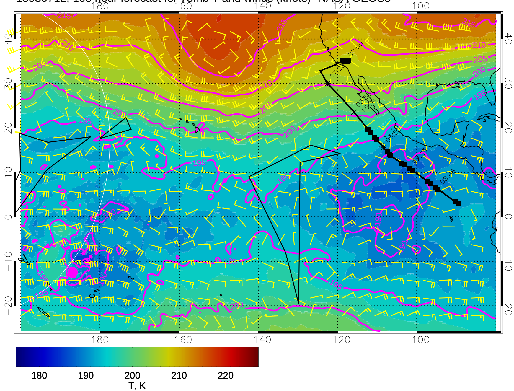
15030712, 108 hour forecast for 73mb T and winds (knots)- NASA GEOS5
