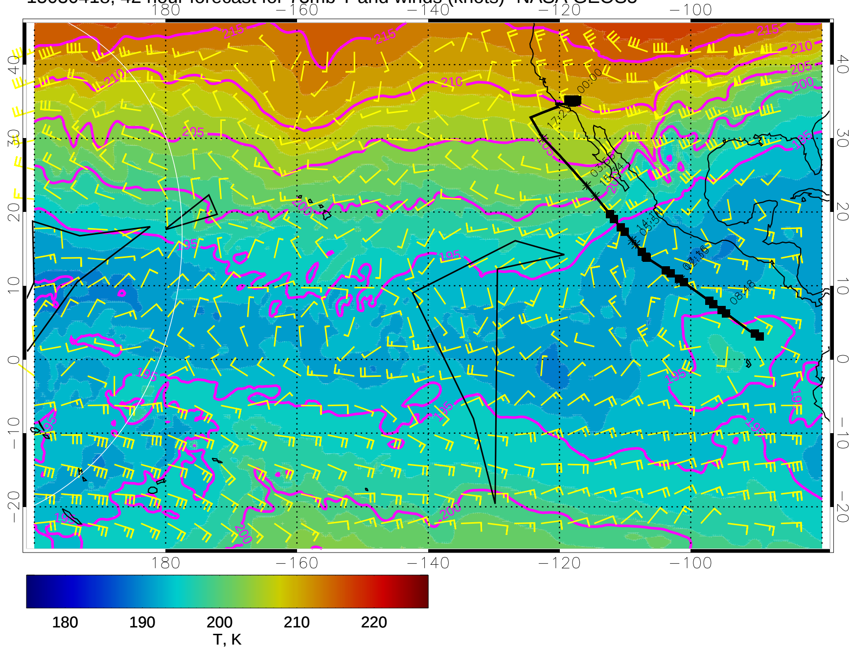
15030418, 42 hour forecast for 73mb T and winds (knots)- NASA GEOS5
