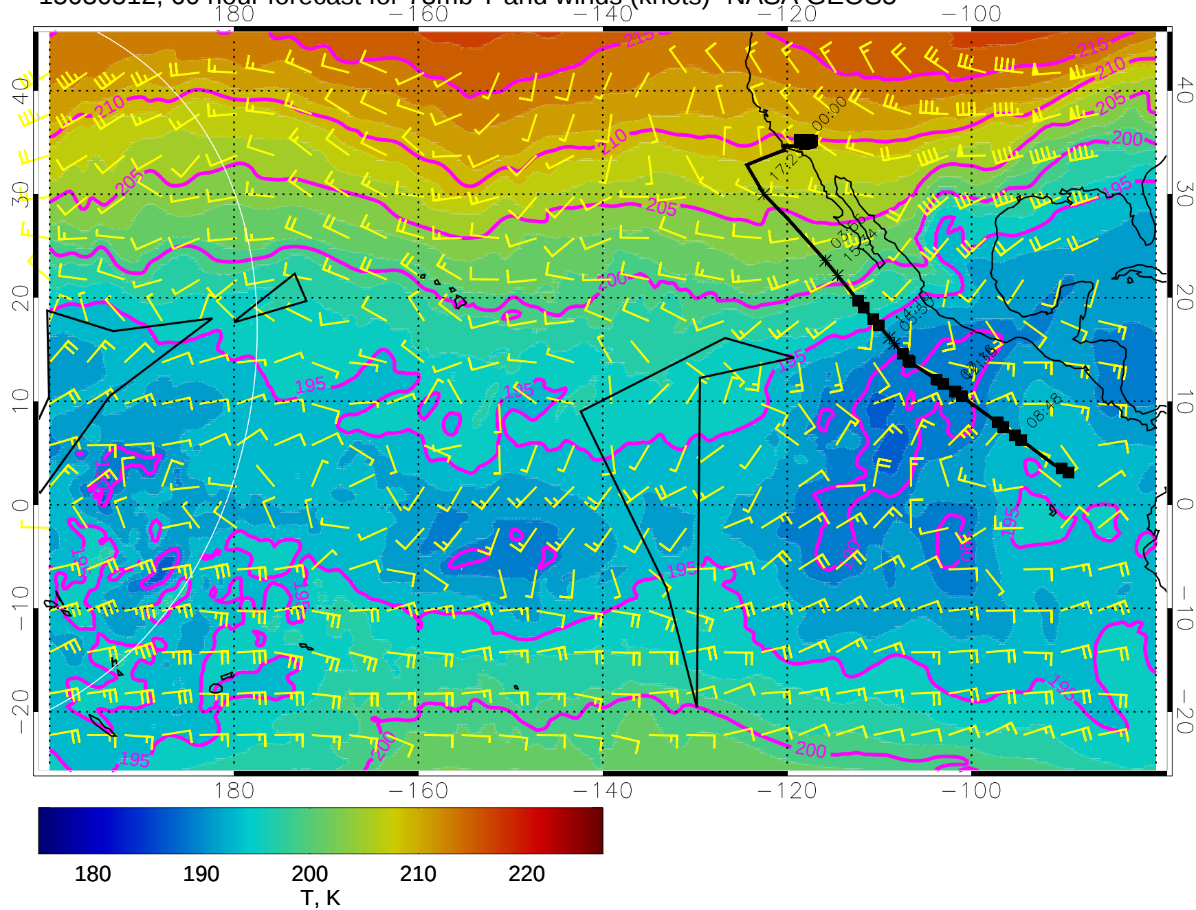
15030512, 60 hour forecast for 73mb T and winds (knots)- NASA GEOS5
