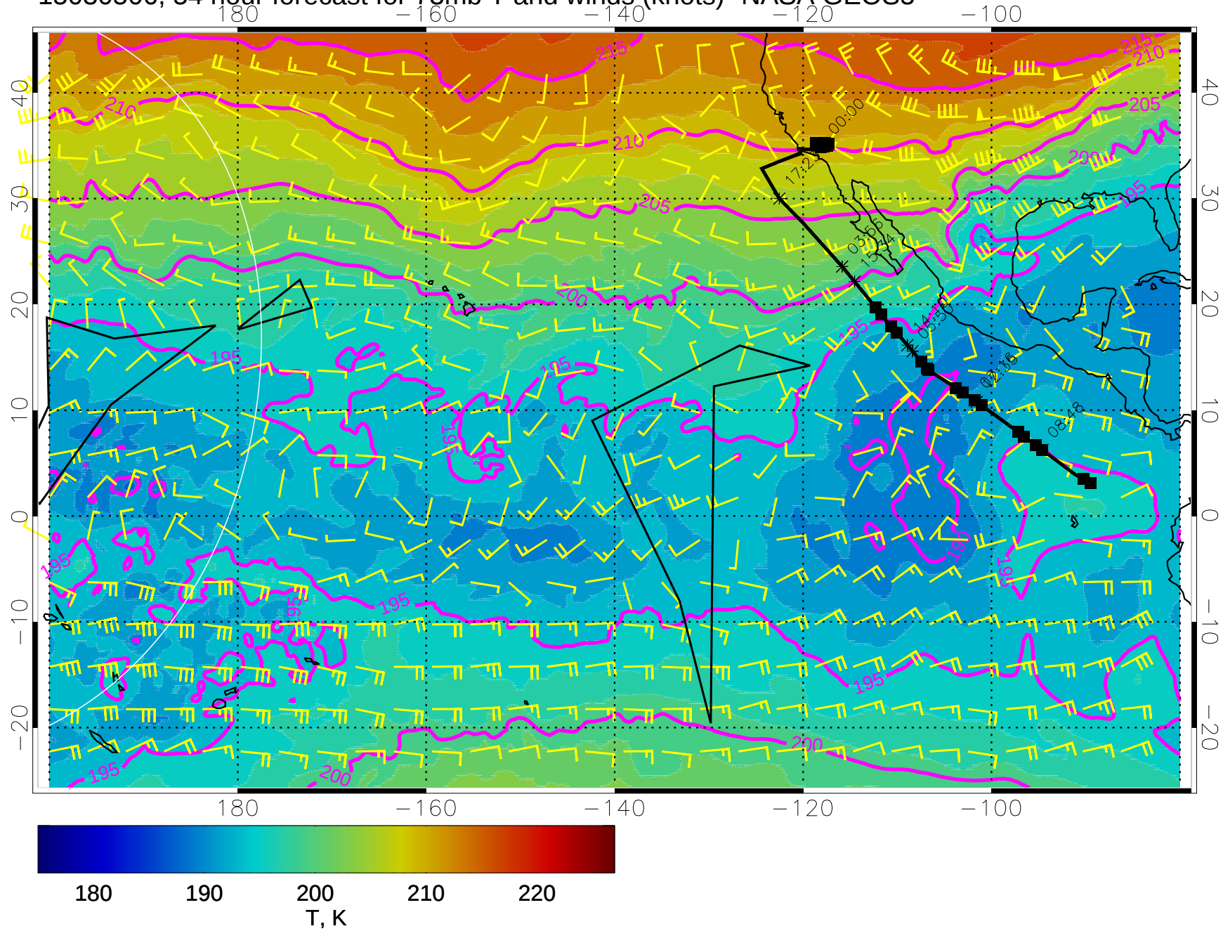
15030506, 54 hour forecast for 73mb T and winds (knots)- NASA GEOS5
