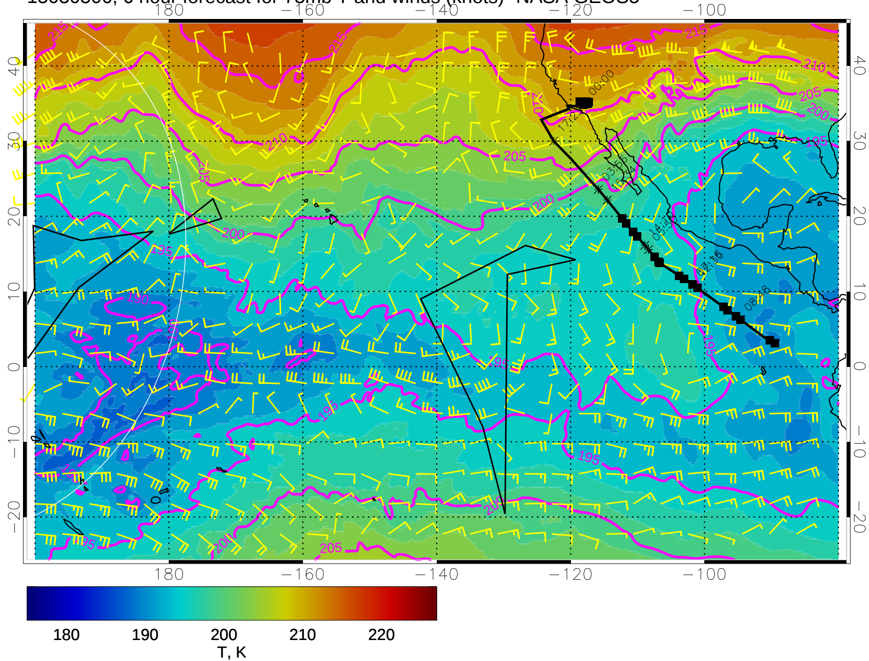
15030306, 6 hour forecast for 73mb T and winds (knots)- NASA GEOS5
