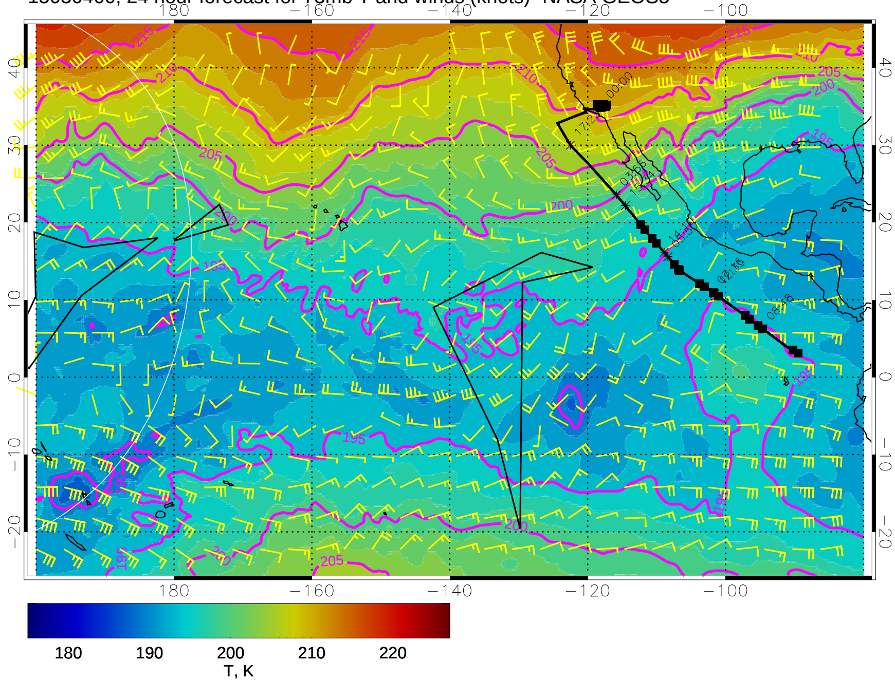
15030400, 24 hour forecast for 73mb T and winds (knots)- NASA GEOS5
