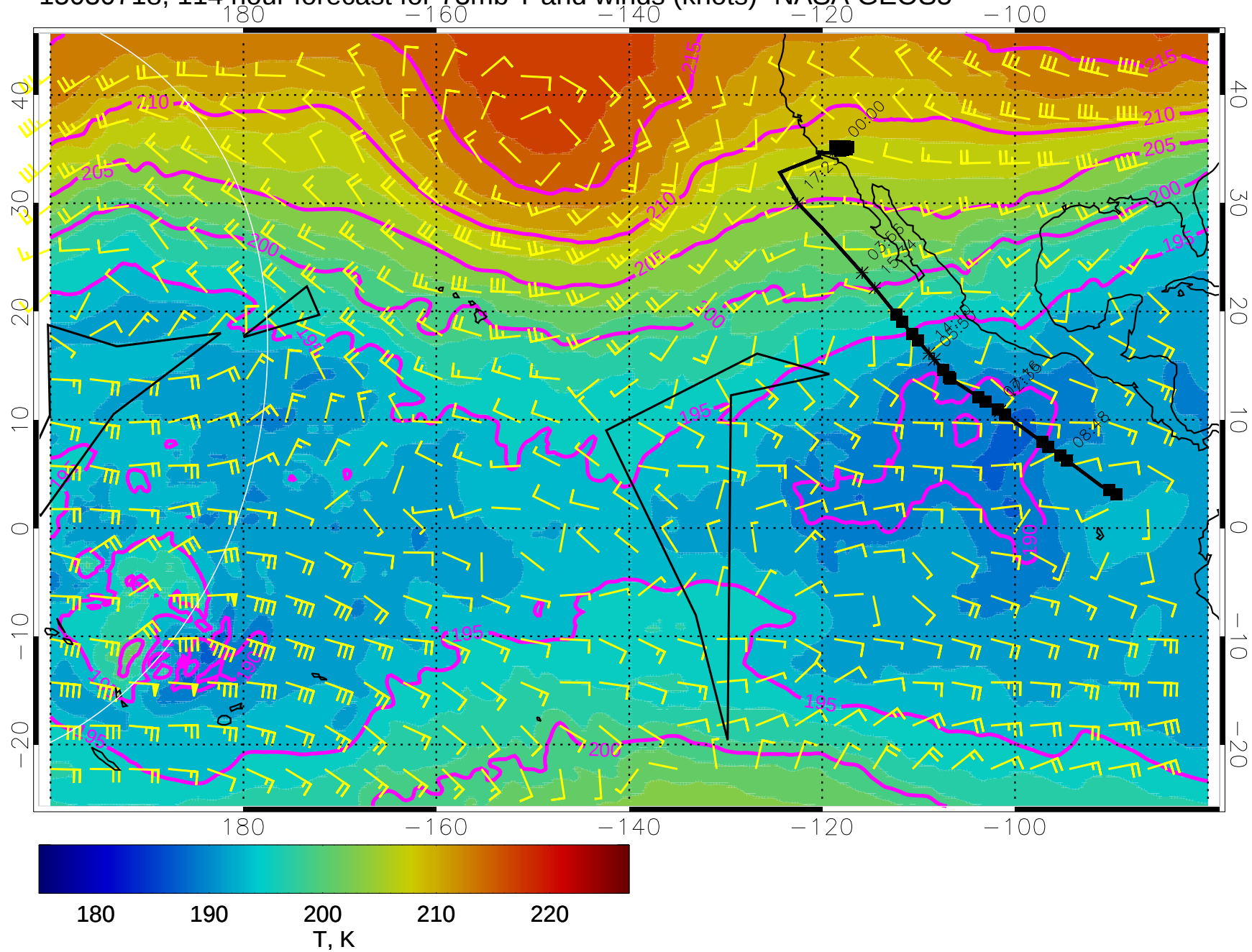
15030718, 114 hour forecast for 73mb T and winds (knots)- NASA GEOS5
