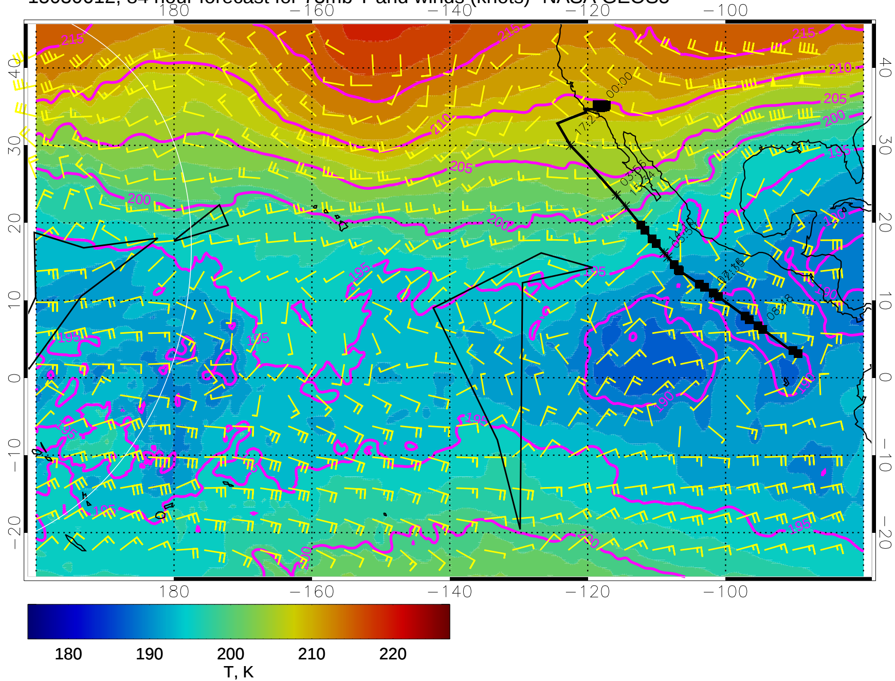
15030612, 84 hour forecast for 73mb T and winds (knots)- NASA GEOS5
