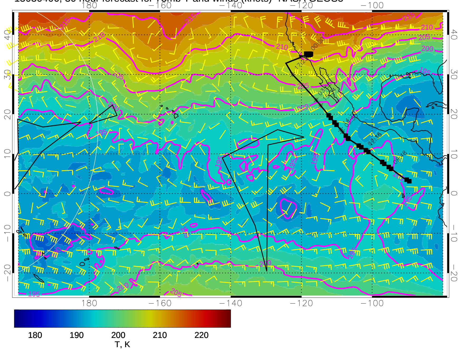
15030406, 30 hour forecast for 73mb T and winds (knots)- NASA GEOS5
