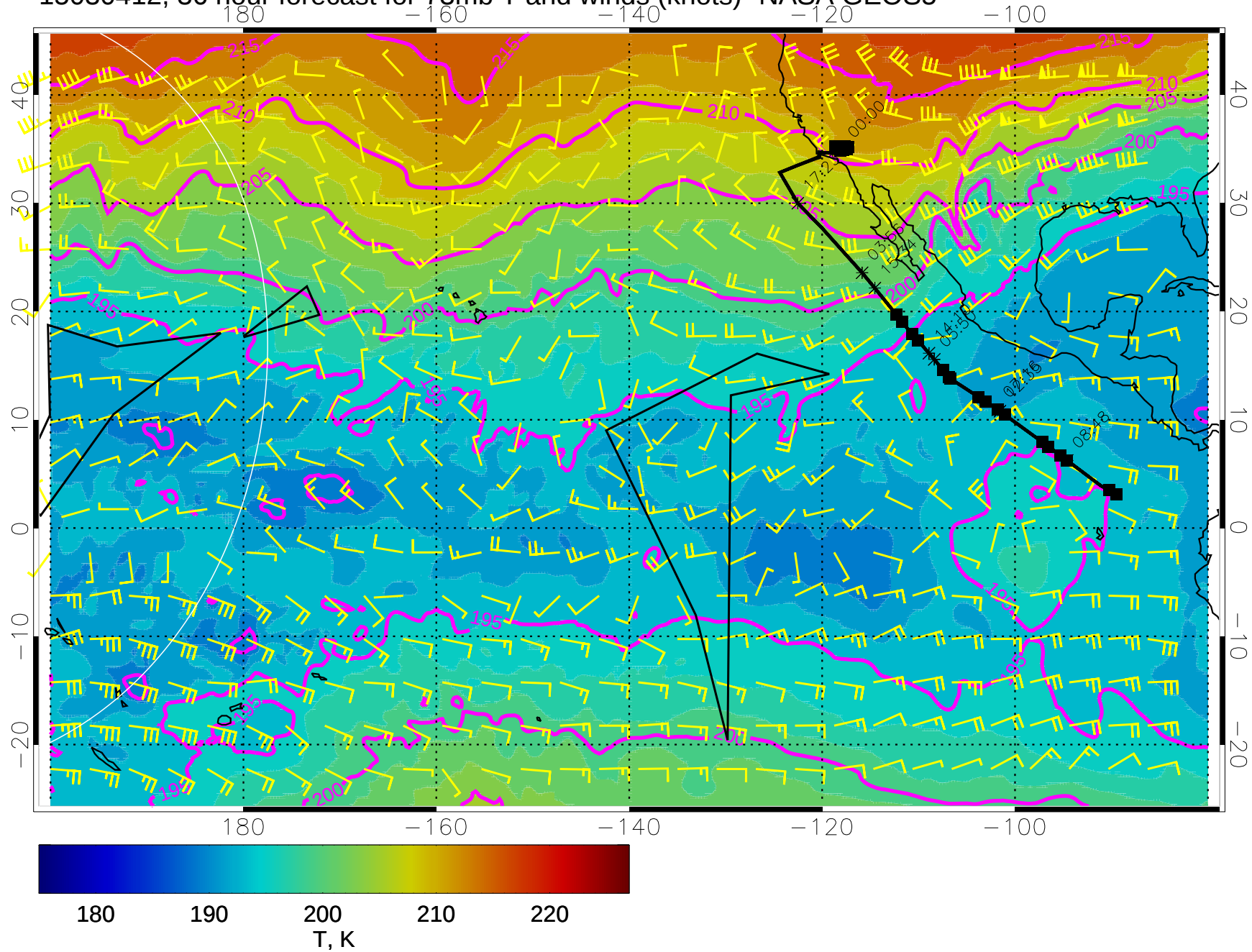
15030412, 36 hour forecast for 73mb T and winds (knots)- NASA GEOS5
