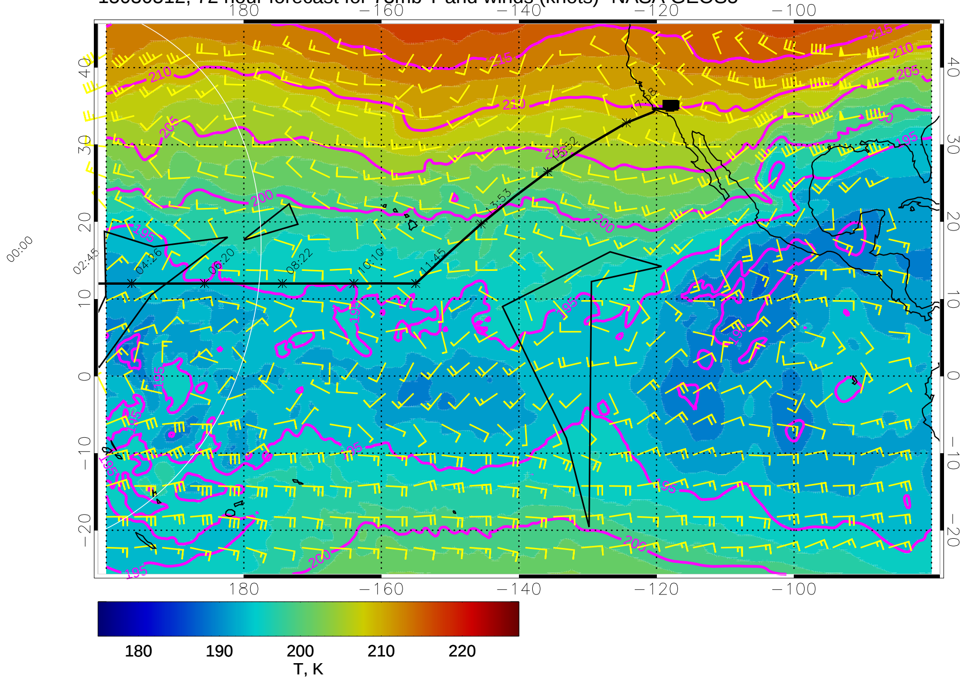
15030512, 72 hour forecast for 73mb T and winds (knots)- NASA GEOS5
