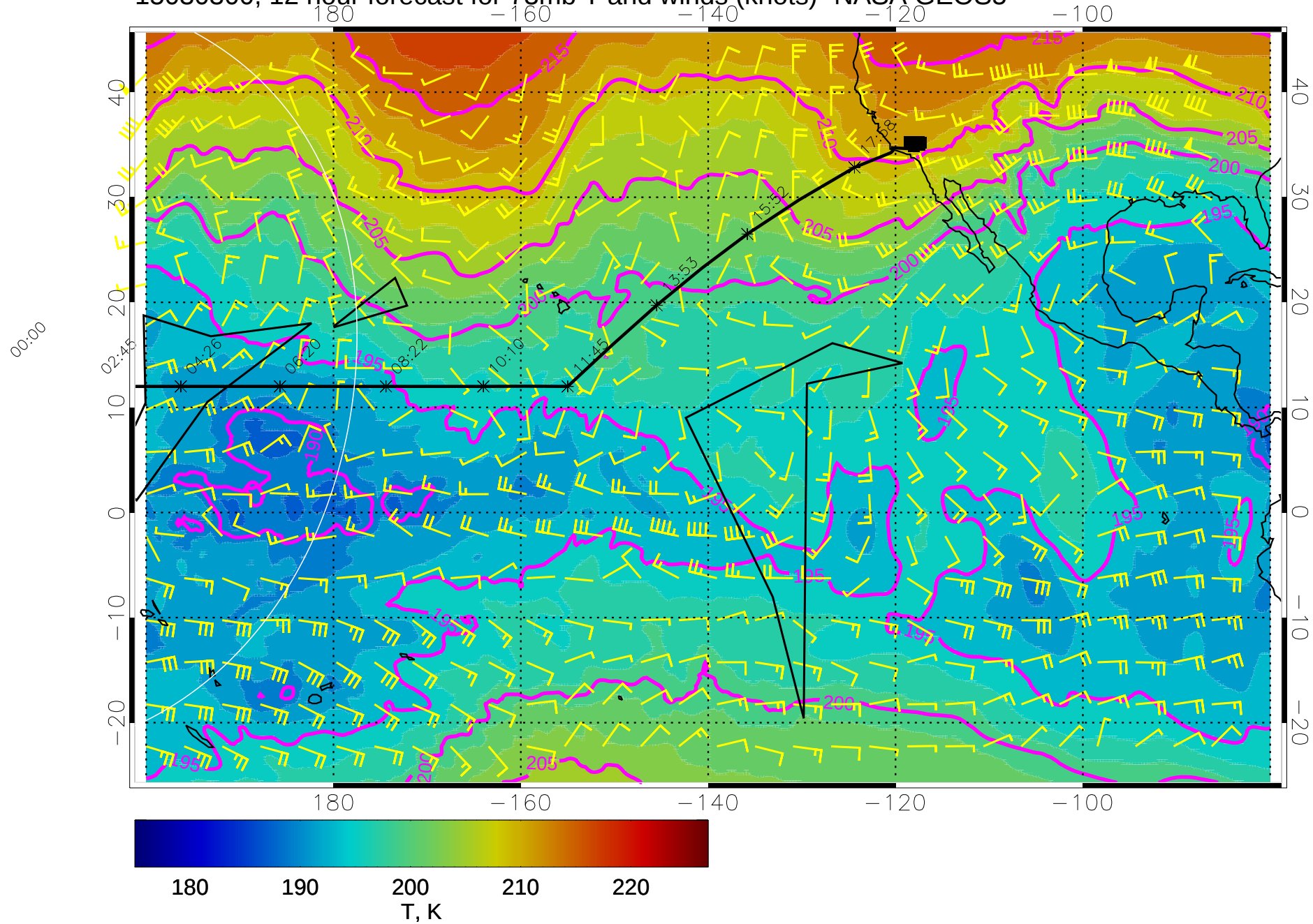
15030300, 12 hour forecast for 73mb T and winds (knots)- NASA GEOS5
