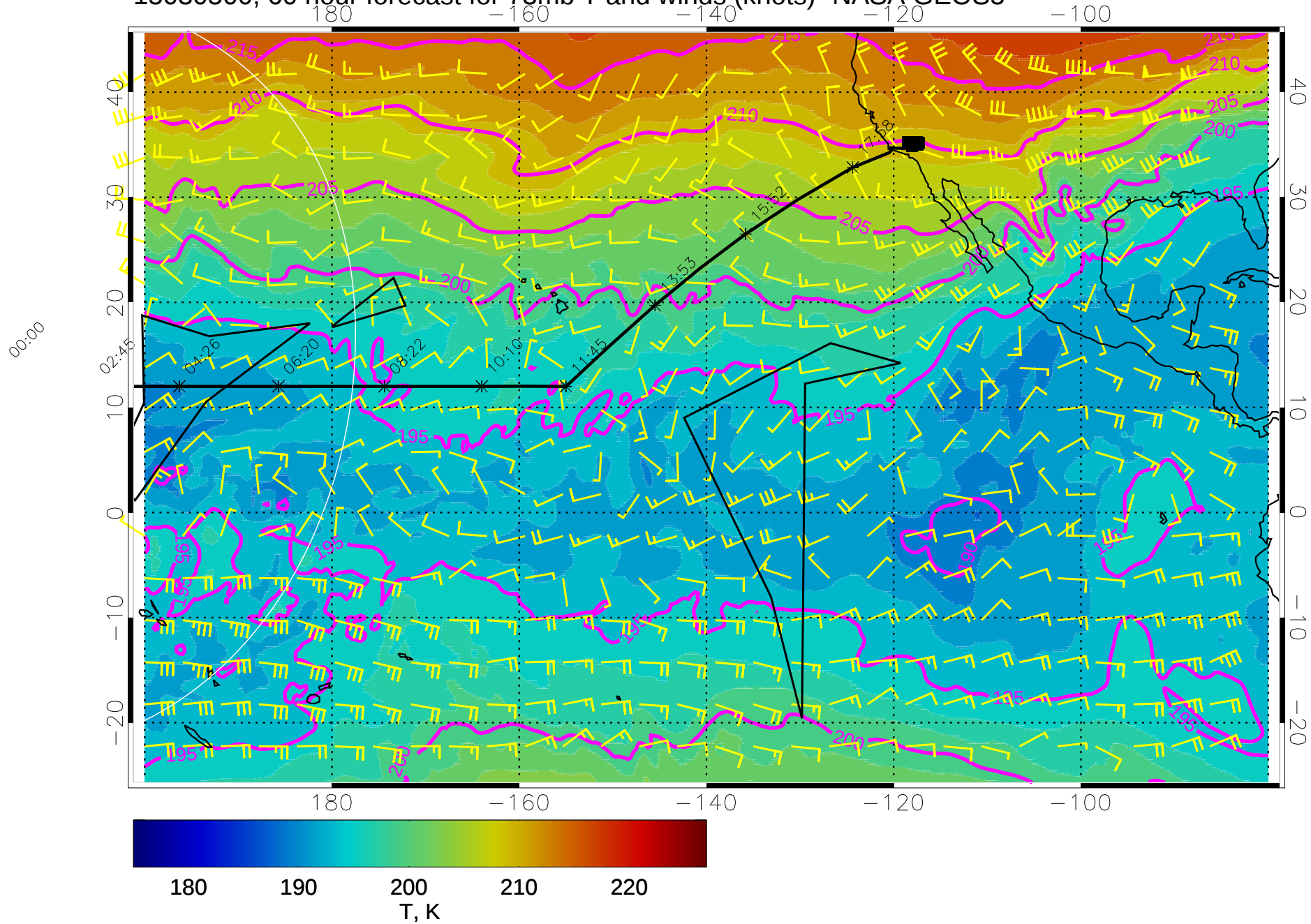
15030500, 60 hour forecast for 73mb T and winds (knots)- NASA GEOS5
