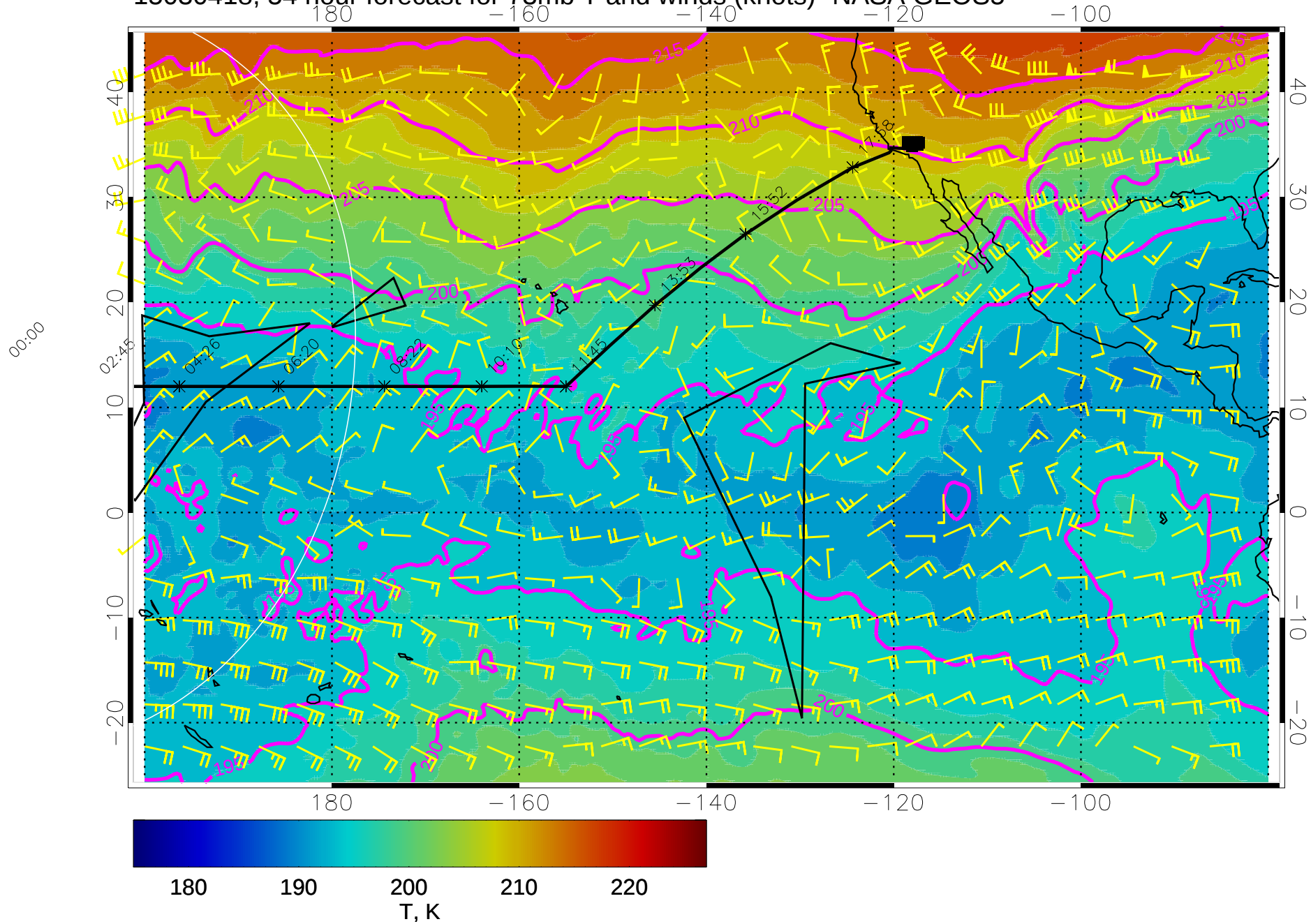
15030418, 54 hour forecast for 73mb T and winds (knots)- NASA GEOS5
