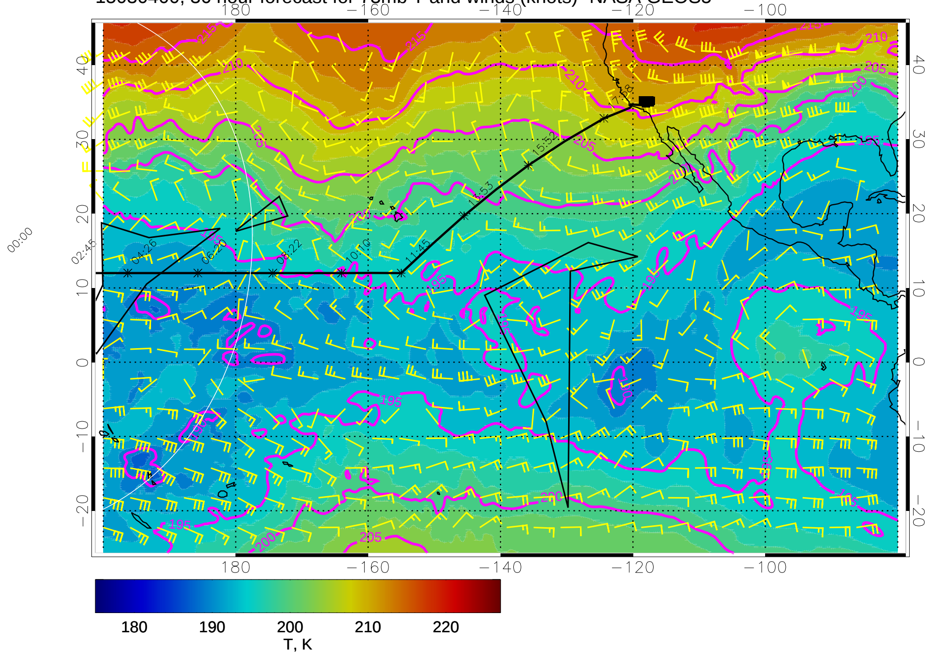
15030400, 36 hour forecast for 73mb T and winds (knots)- NASA GEOS5
