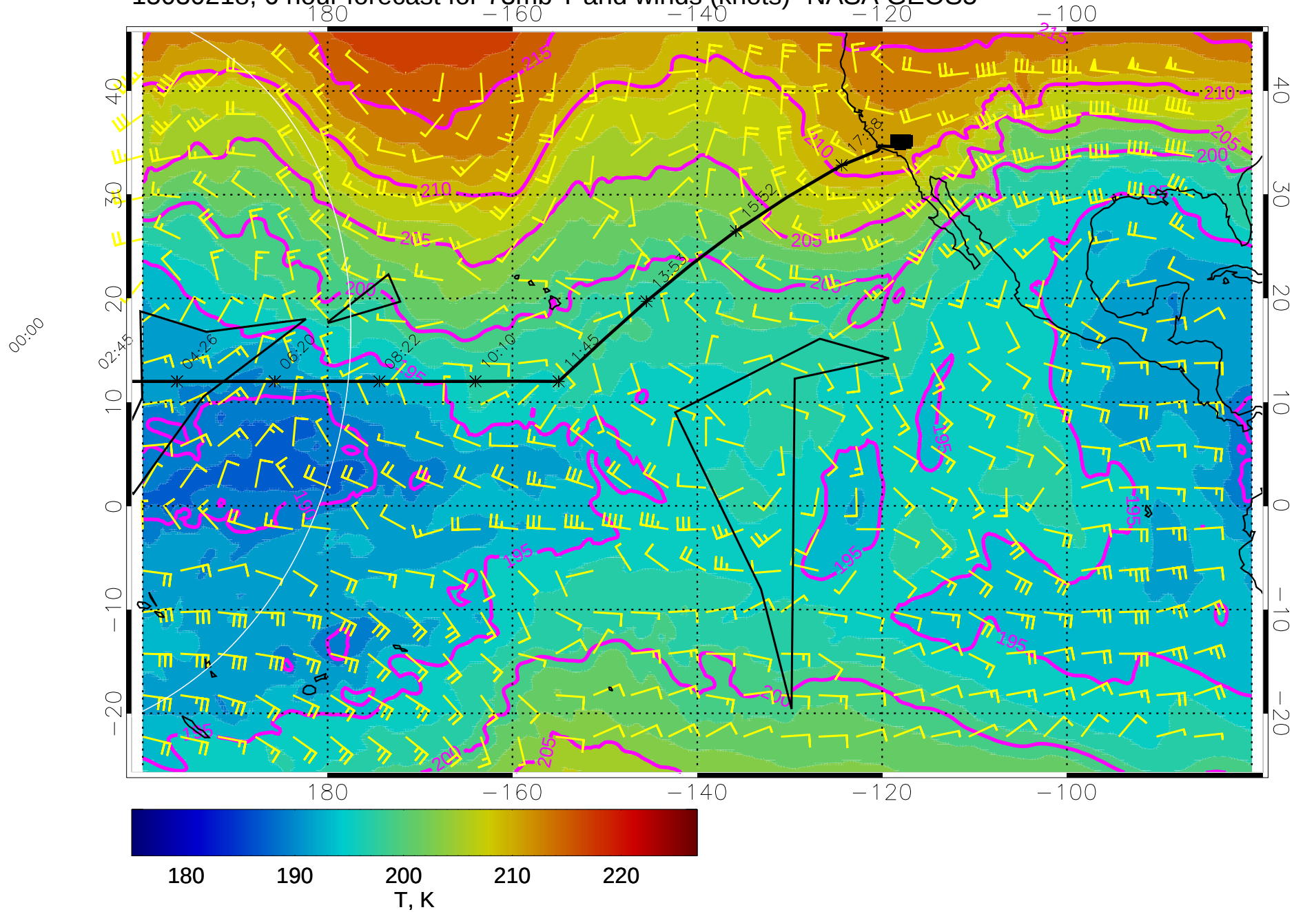
15030218, 6 hour forecast for 73mb T and winds (knots)- NASA GEOS5
