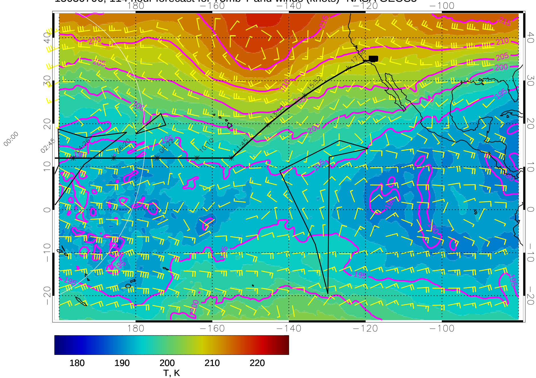
15030706, 114 hour forecast for 73mb T and winds (knots)- NASA GEOS5
