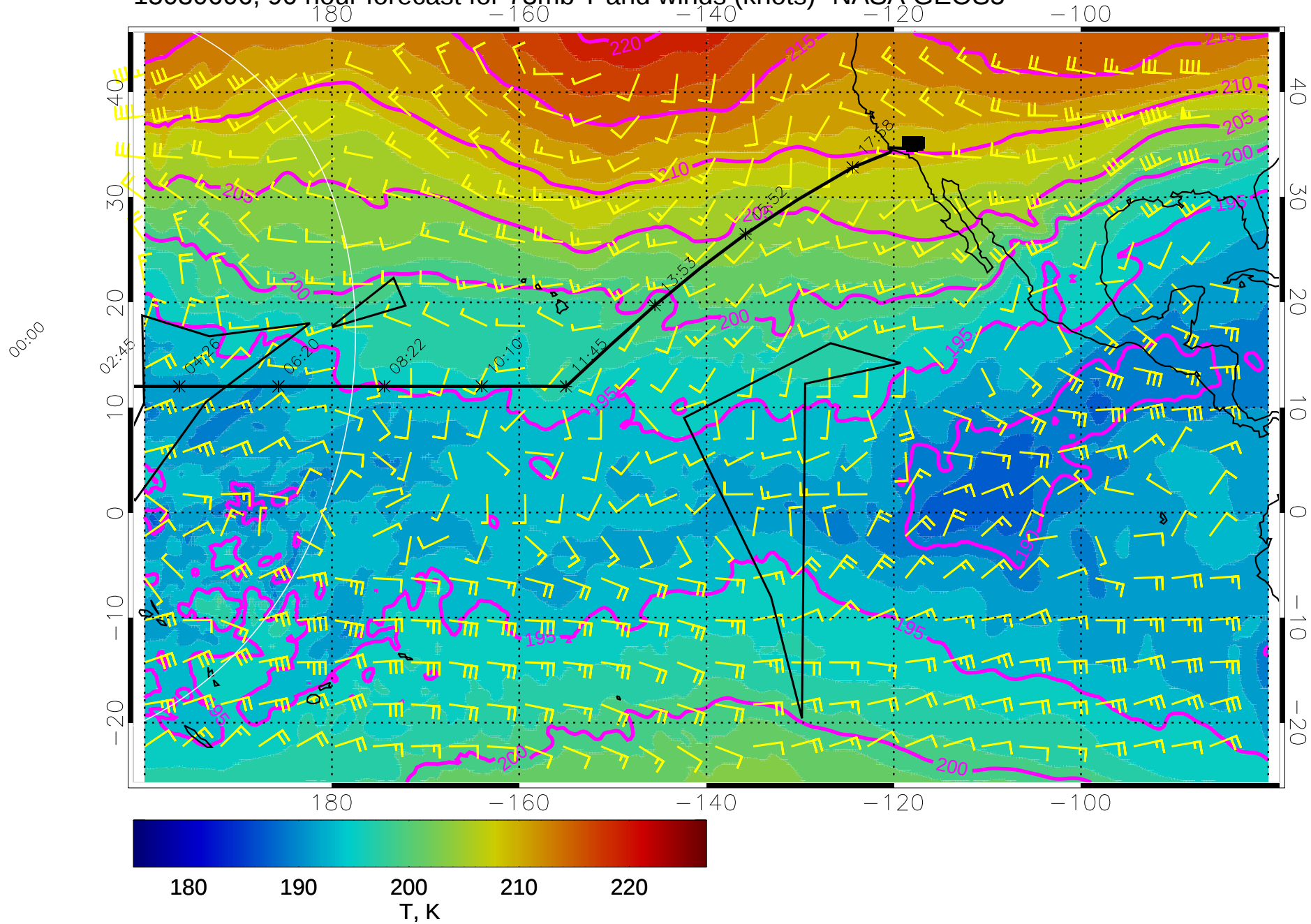
15030606, 90 hour forecast for 73mb T and winds (knots)- NASA GEOS5
