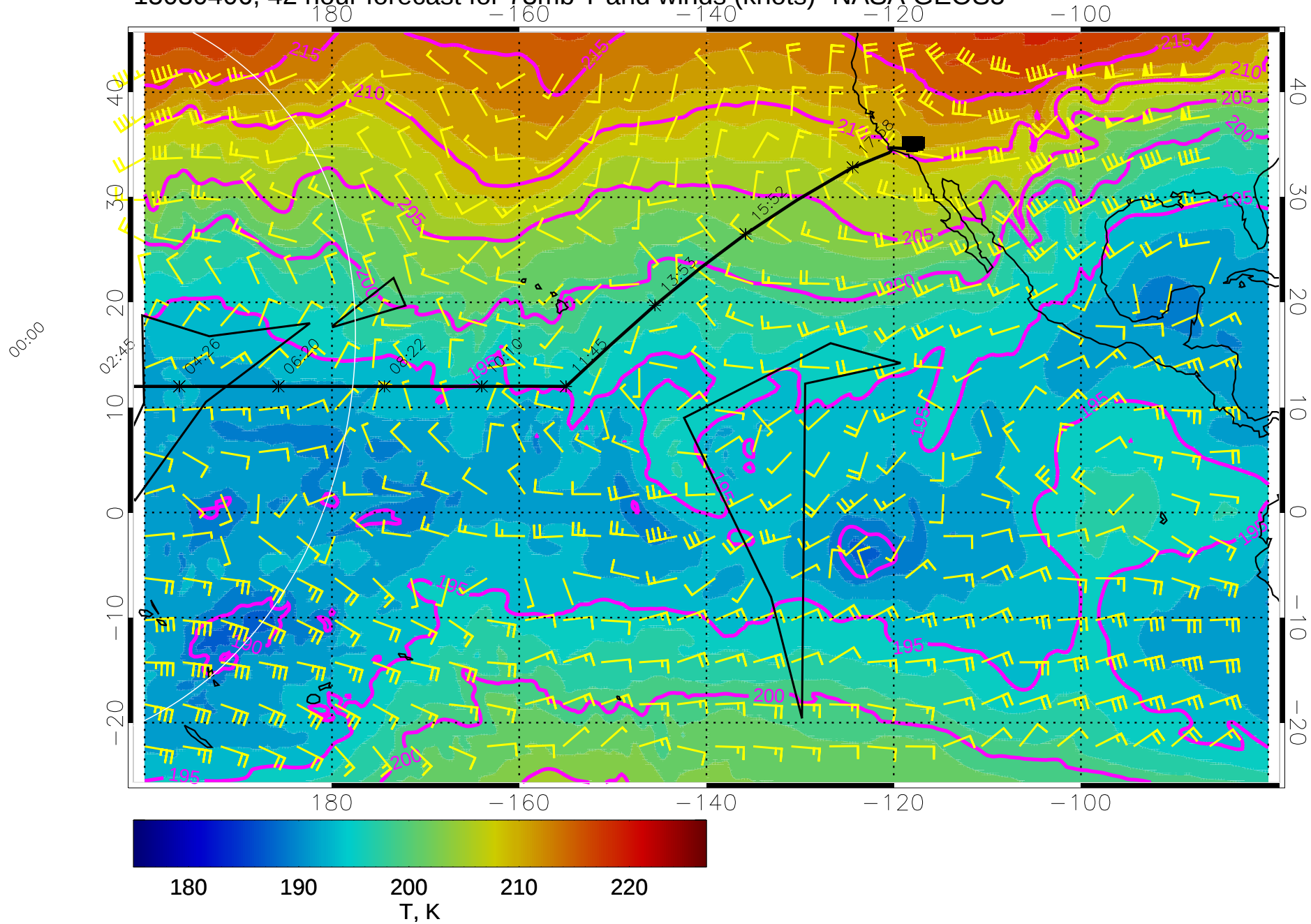
15030406, 42 hour forecast for 73mb T and winds (knots)- NASA GEOS5
