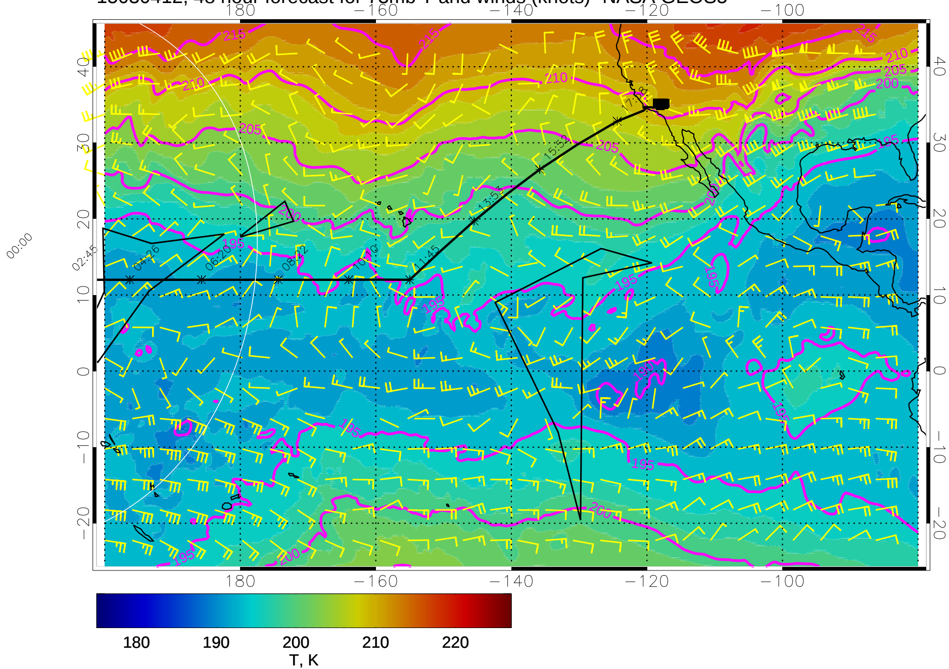
15030412, 48 hour forecast for 73mb T and winds (knots)- NASA GEOS5
