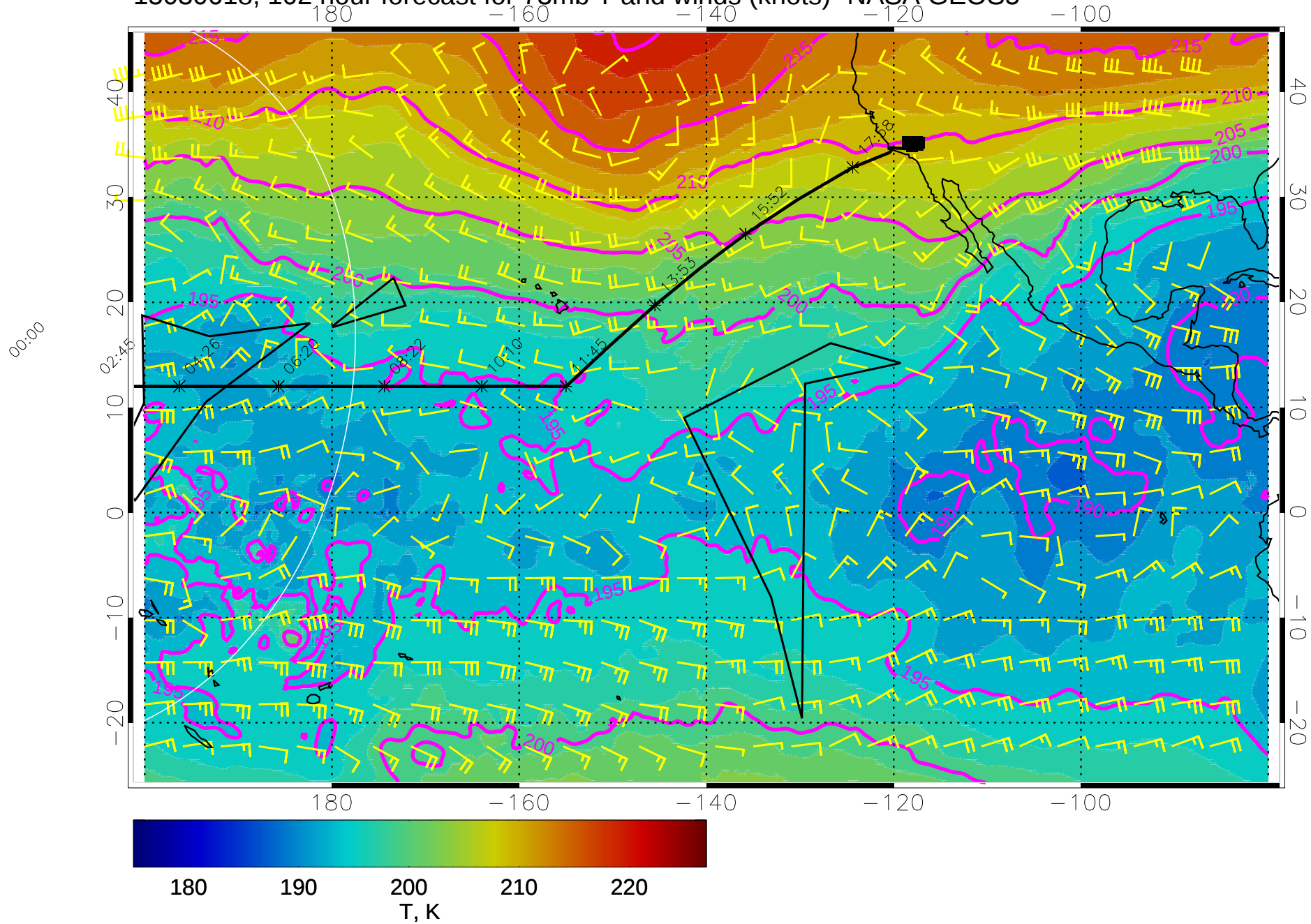
15030618, 102 hour forecast for 73mb T and winds (knots)- NASA GEOS5
