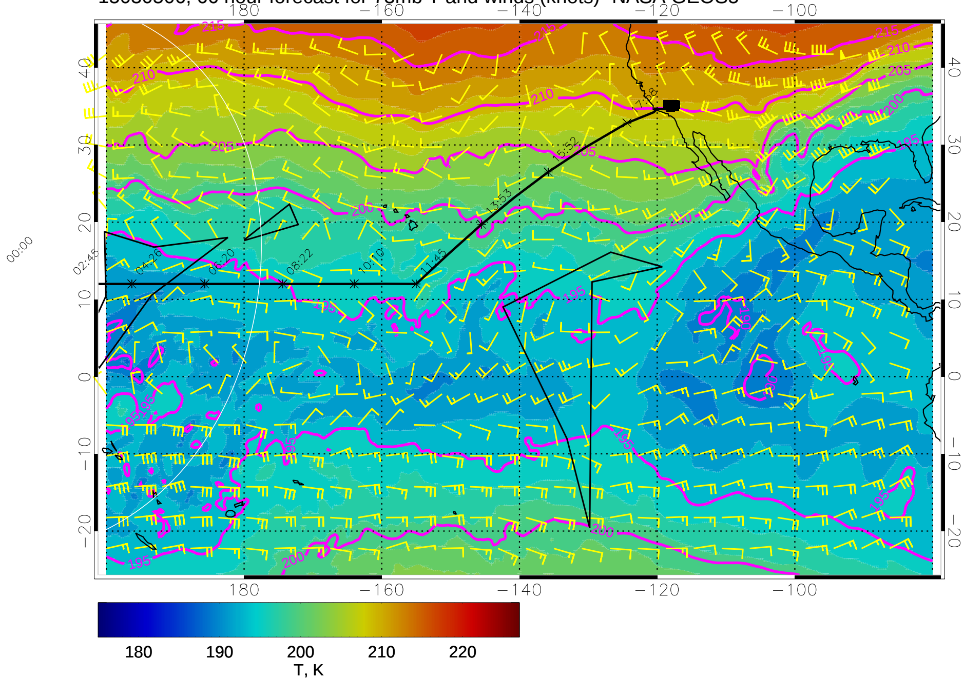
15030506, 66 hour forecast for 73mb T and winds (knots)- NASA GEOS5
