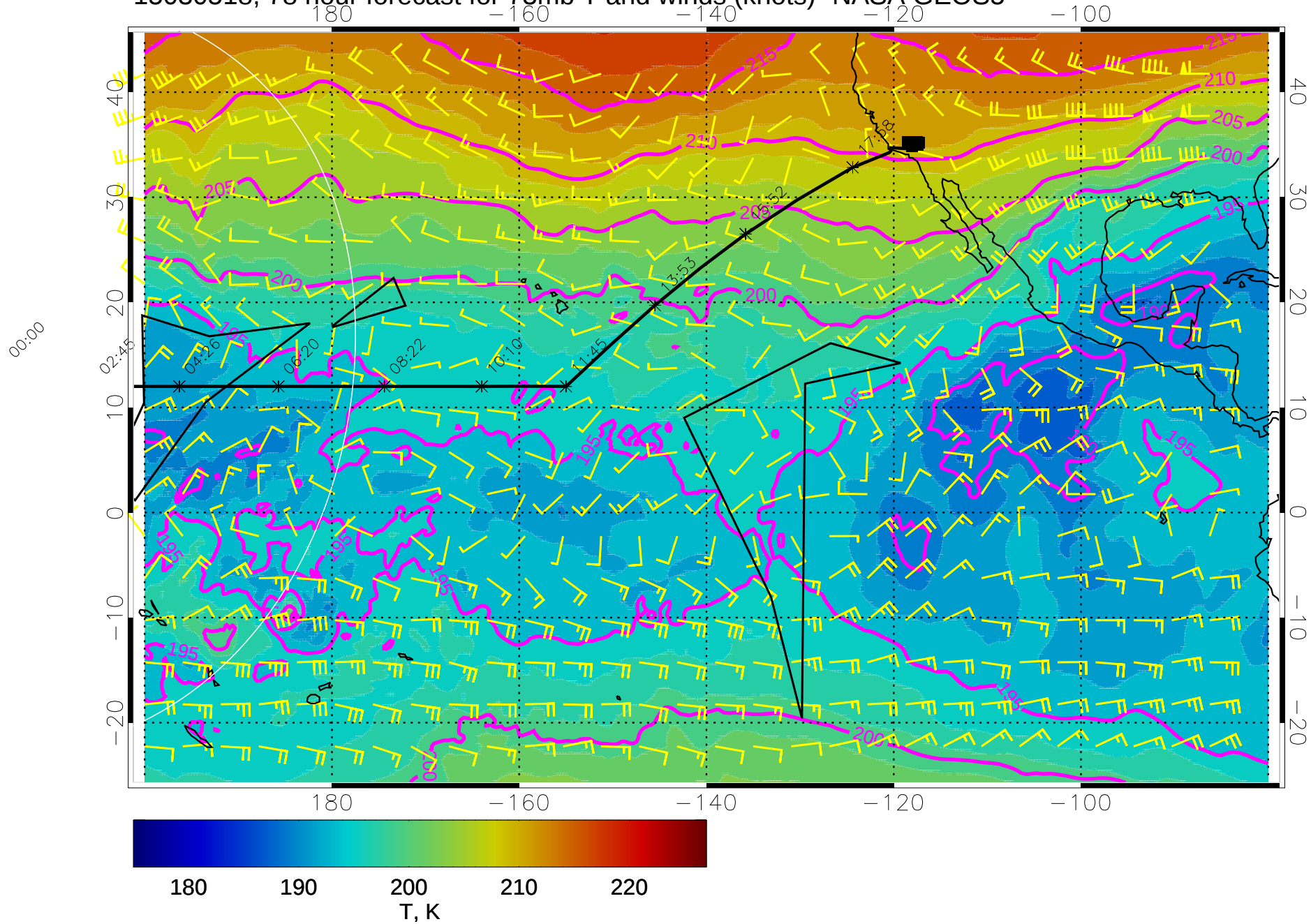
15030518, 78 hour forecast for 73mb T and winds (knots)- NASA GEOS5
