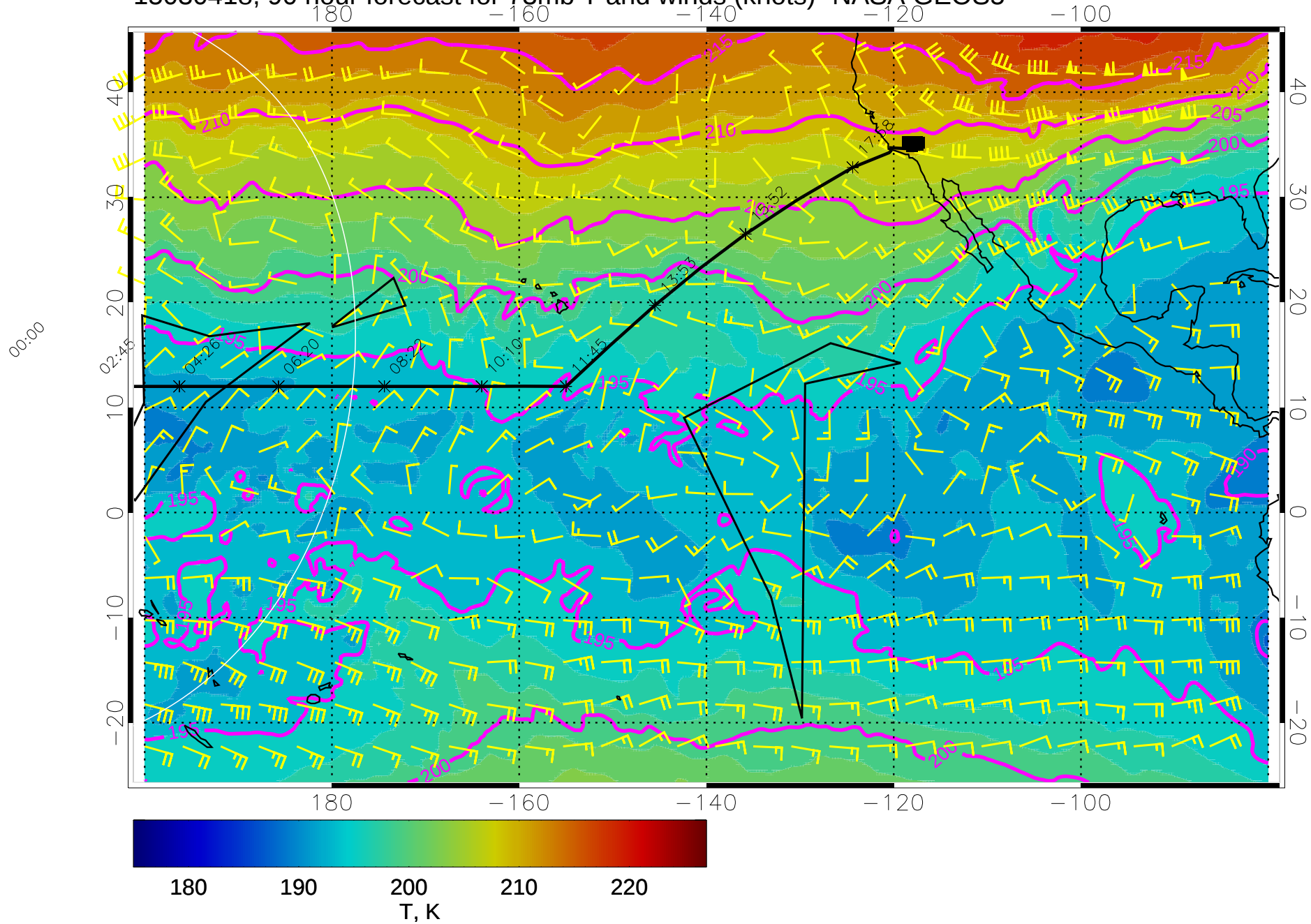
15030418, 90 hour forecast for 73mb T and winds (knots)- NASA GEOS5
