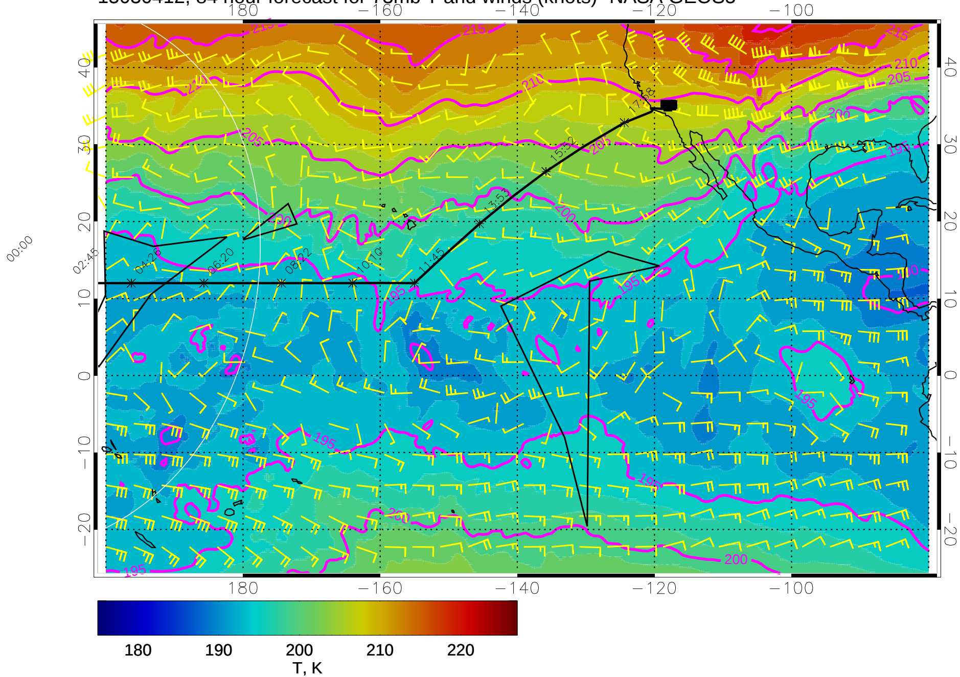
15030412, 84 hour forecast for 73mb T and winds (knots)- NASA GEOS5
