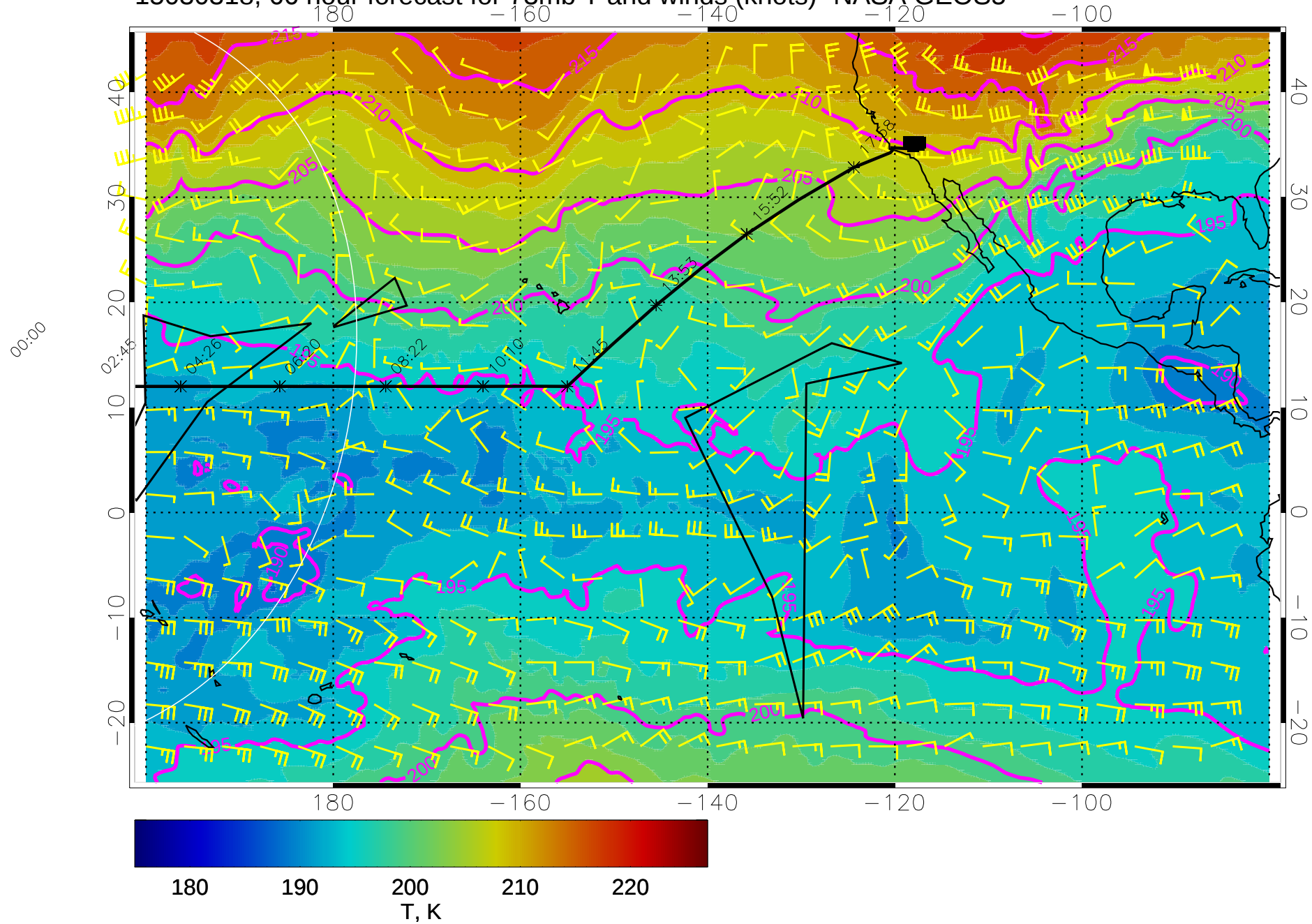
15030318, 66 hour forecast for 73mb T and winds (knots)- NASA GEOS5
