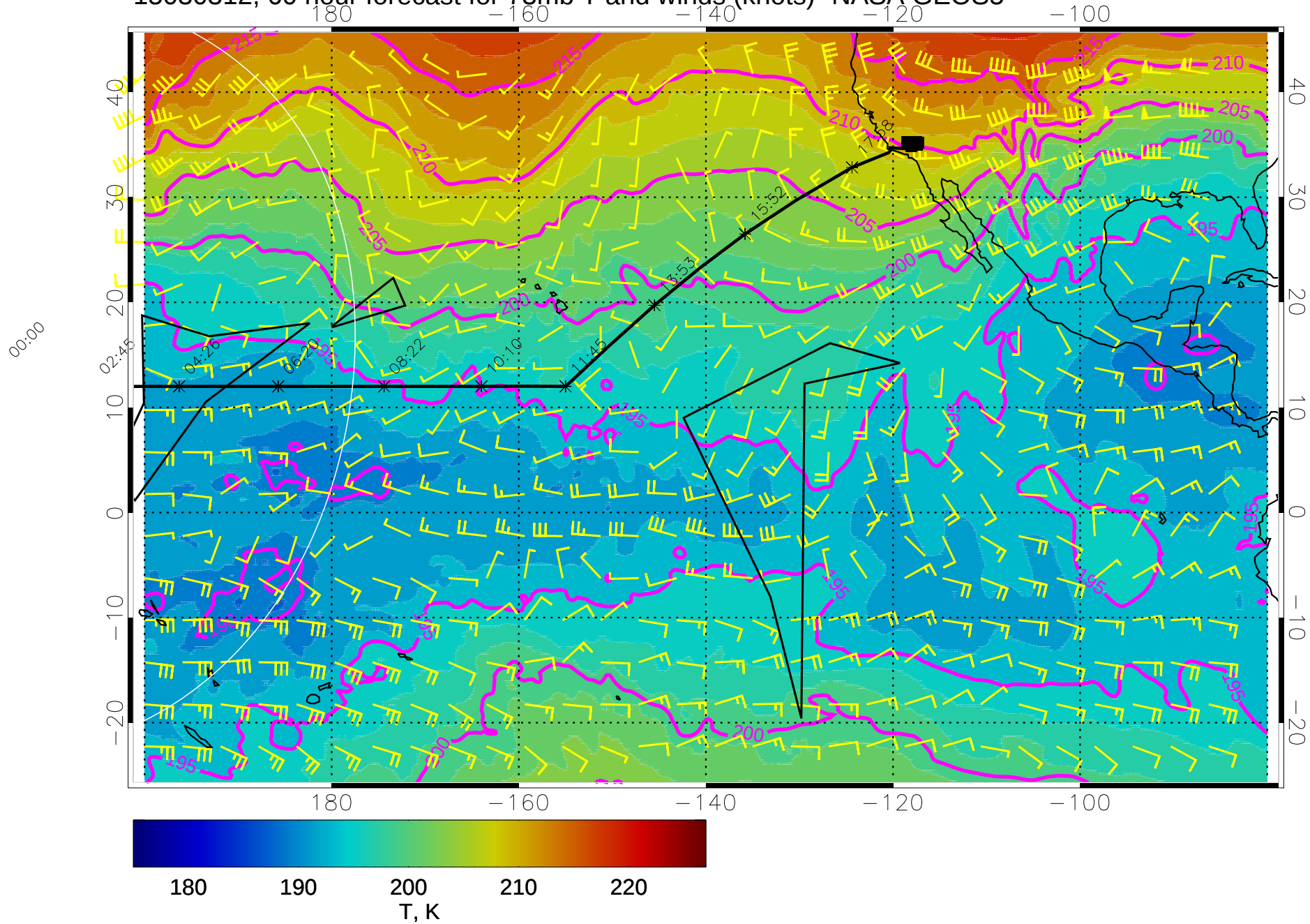
15030312, 60 hour forecast for 73mb T and winds (knots)- NASA GEOS5
