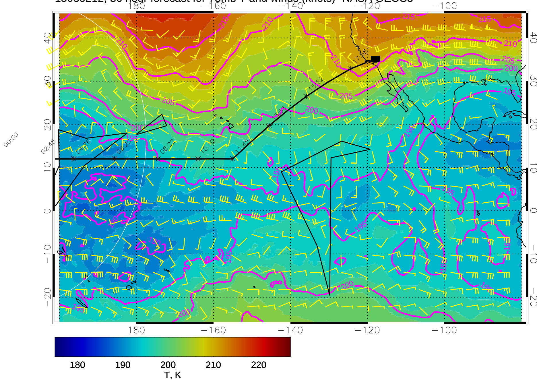
15030212, 36 hour forecast for 73mb T and winds (knots)- NASA GEOS5
