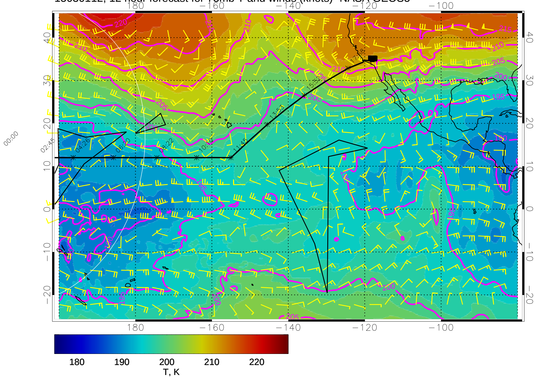
15030112, 12 hour forecast for 73mb T and winds (knots)- NASA GEOS5
