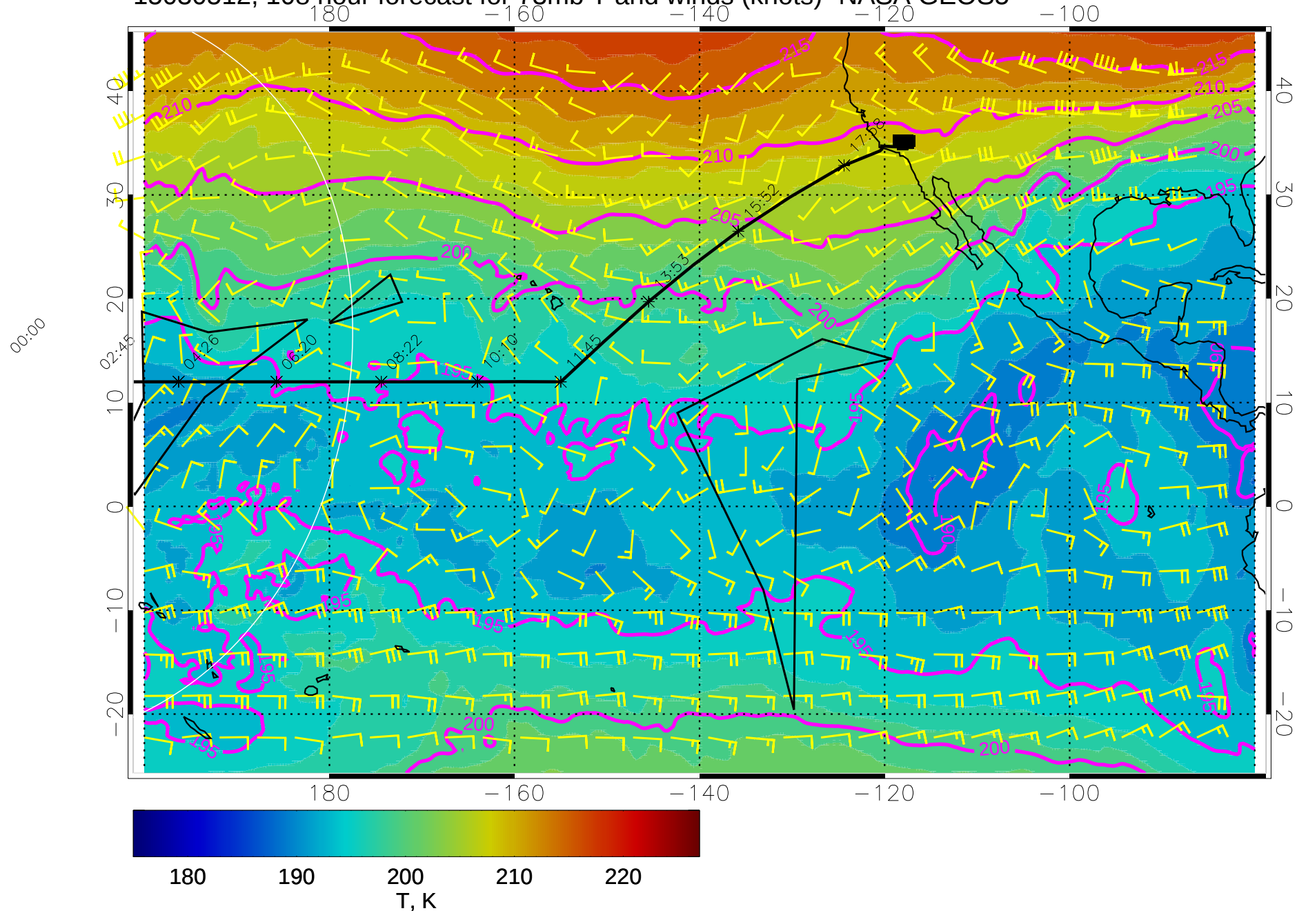
15030512, 108 hour forecast for 73mb T and winds (knots)- NASA GEOS5
