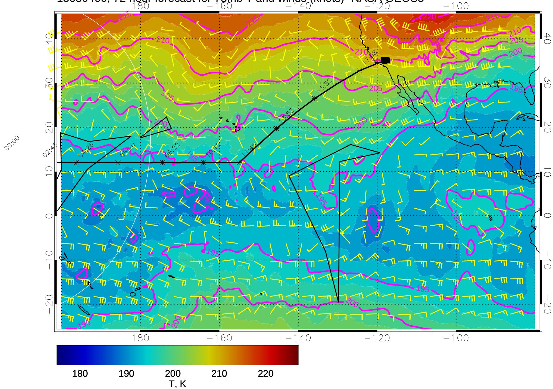
15030400, 72 hour forecast for 73mb T and winds (knots)- NASA GEOS5
