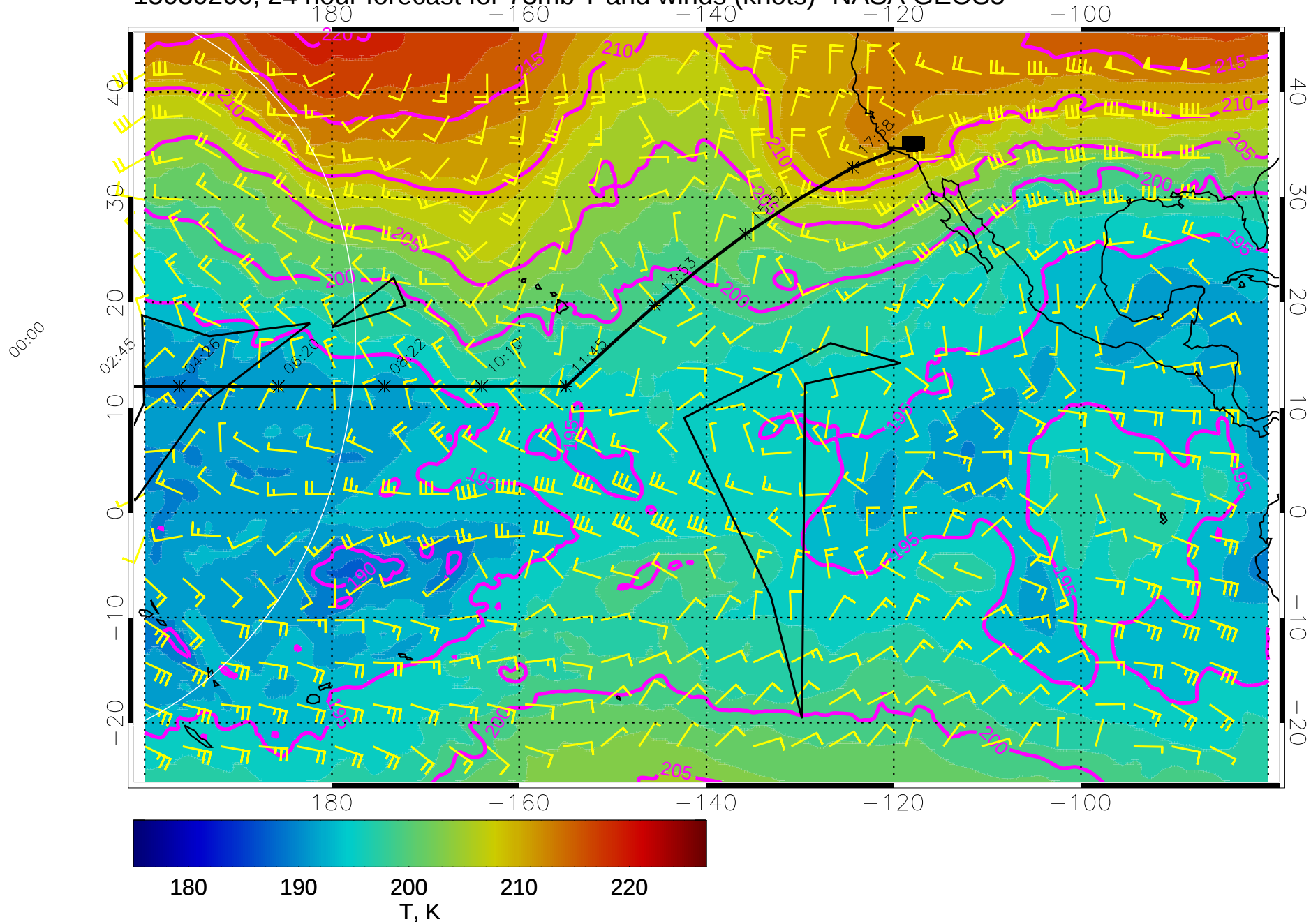
15030200, 24 hour forecast for 73mb T and winds (knots)- NASA GEOS5
