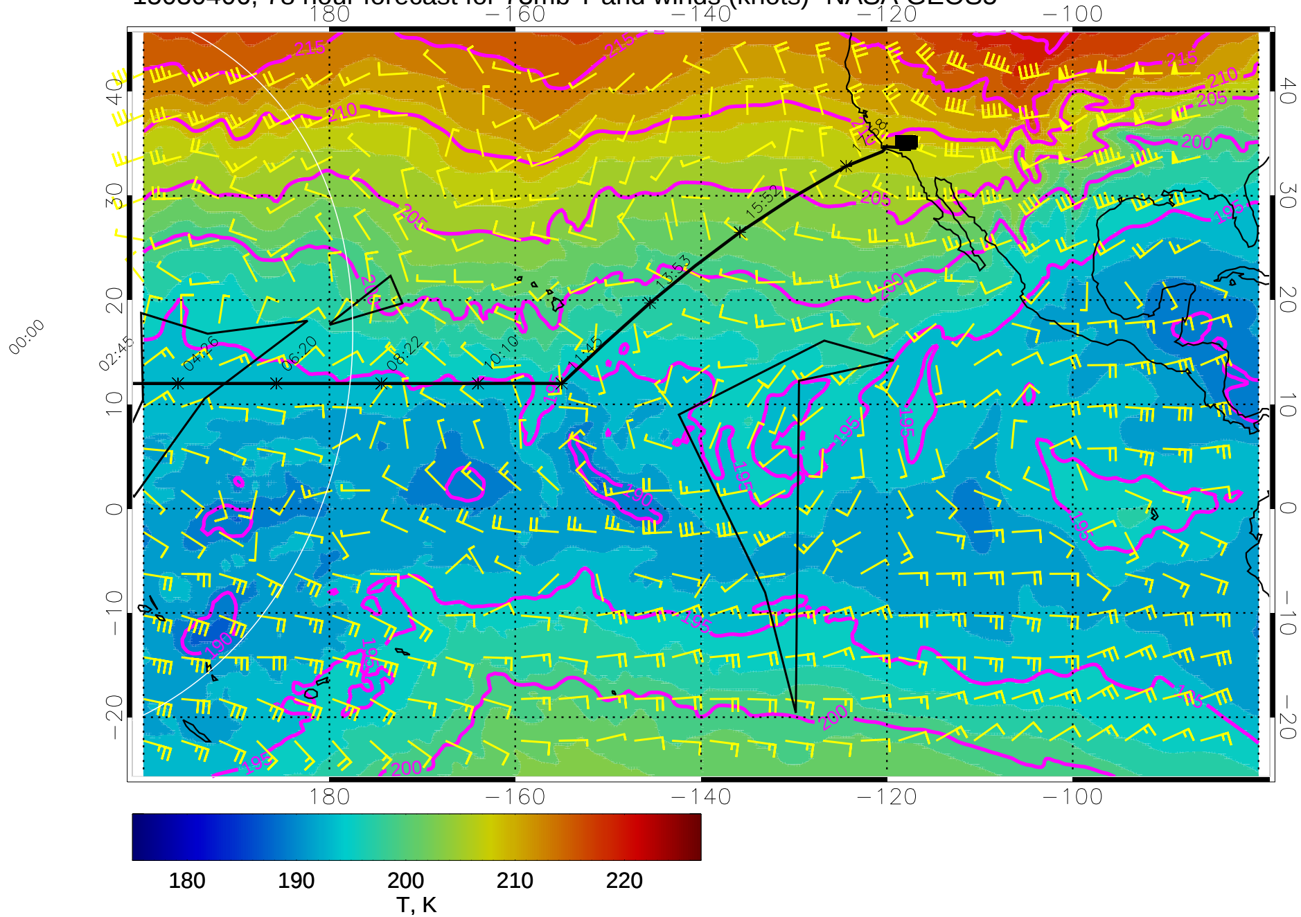
15030406, 78 hour forecast for 73mb T and winds (knots)- NASA GEOS5
