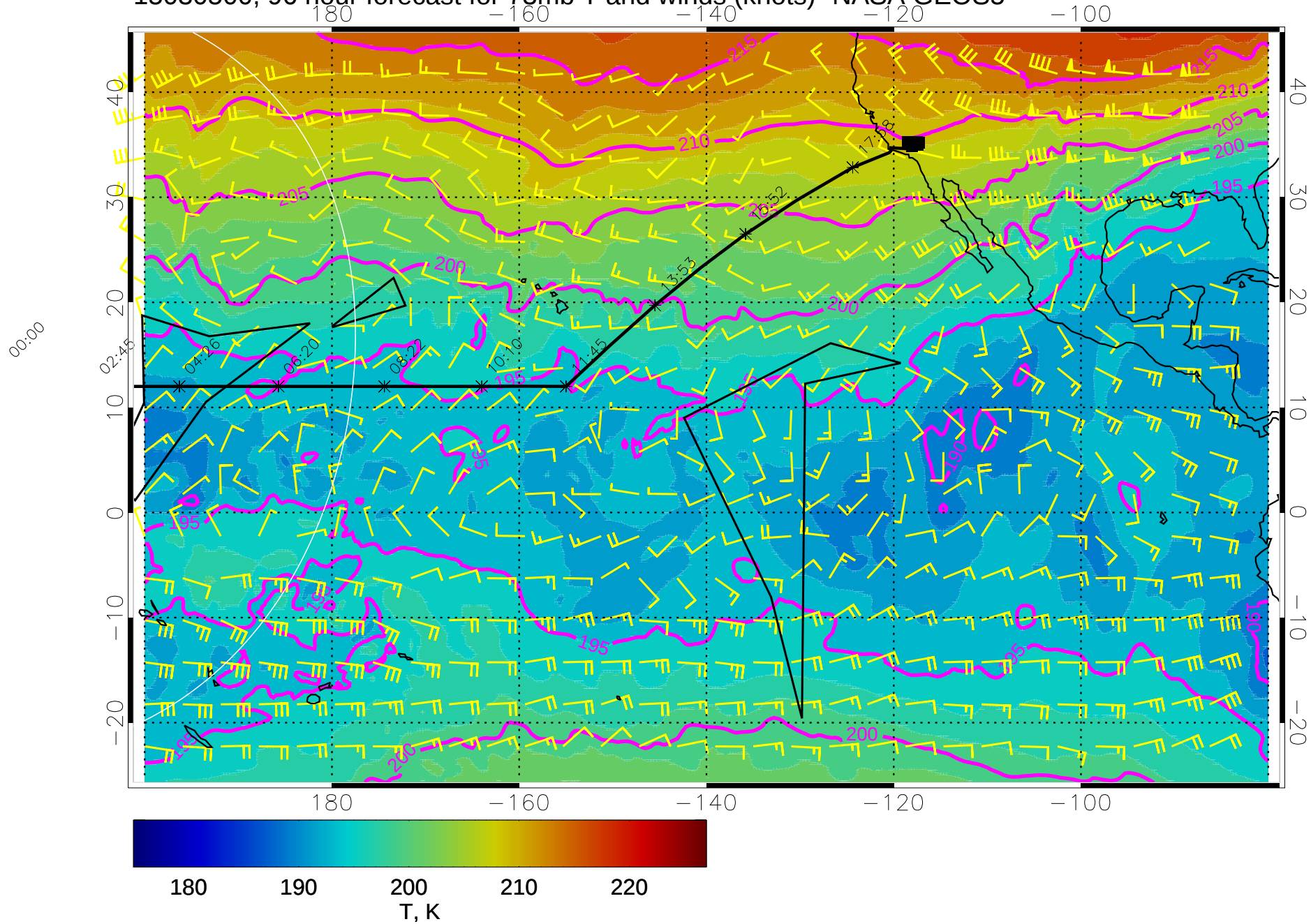
15030500, 96 hour forecast for 73mb T and winds (knots)- NASA GEOS5
