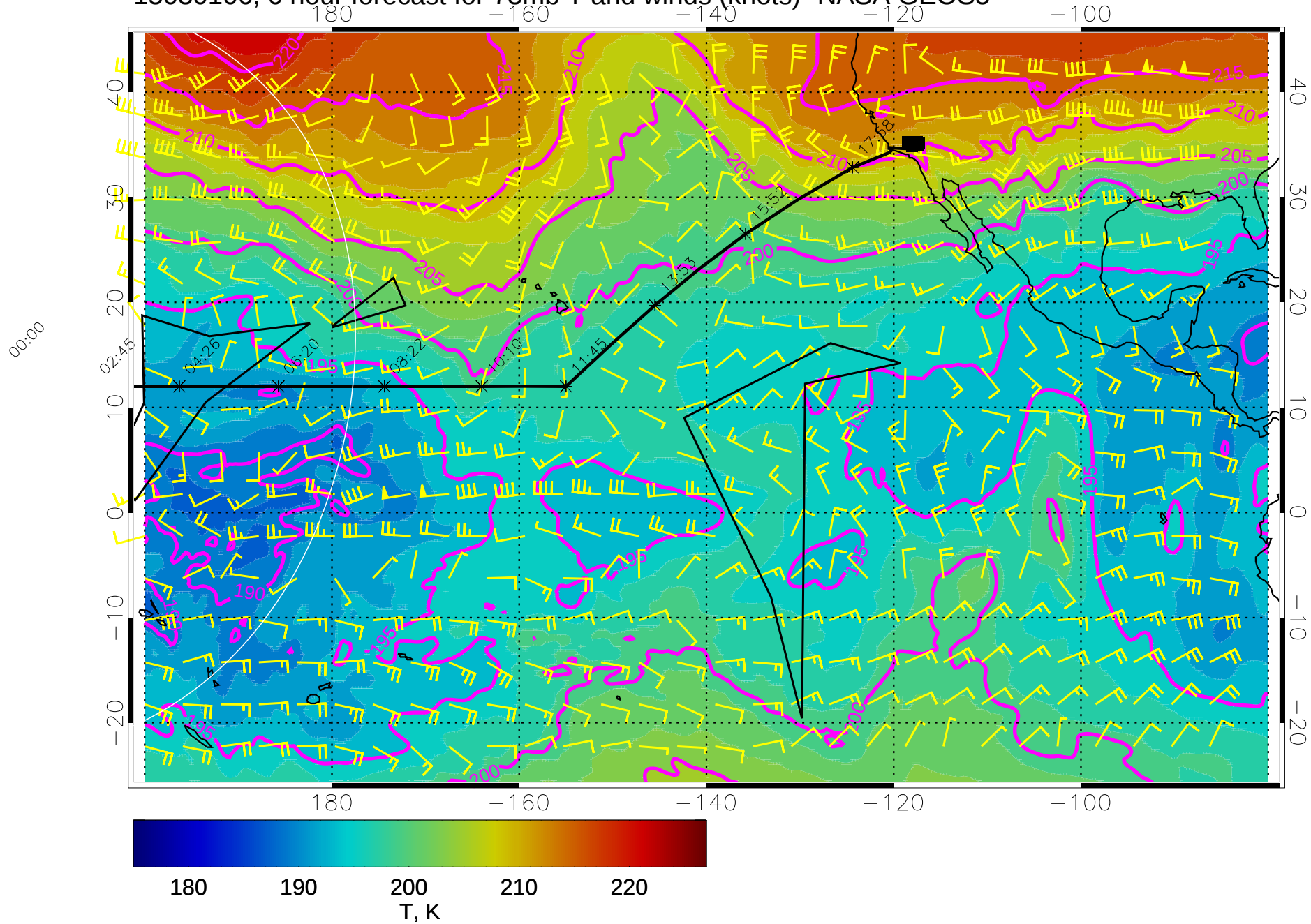
15030106, 6 hour forecast for 73mb T and winds (knots)- NASA GEOS5
