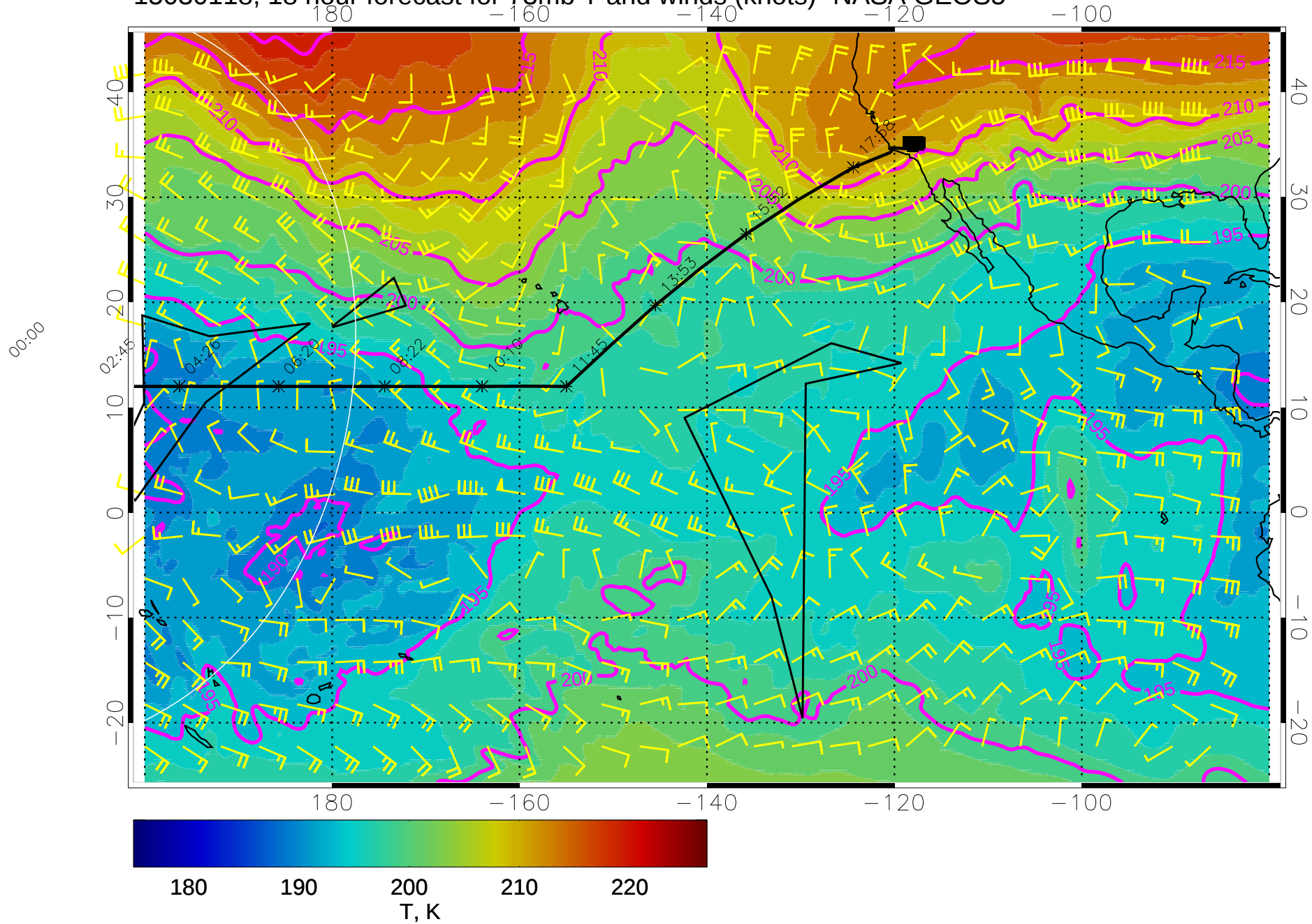
15030118, 18 hour forecast for 73mb T and winds (knots)- NASA GEOS5
