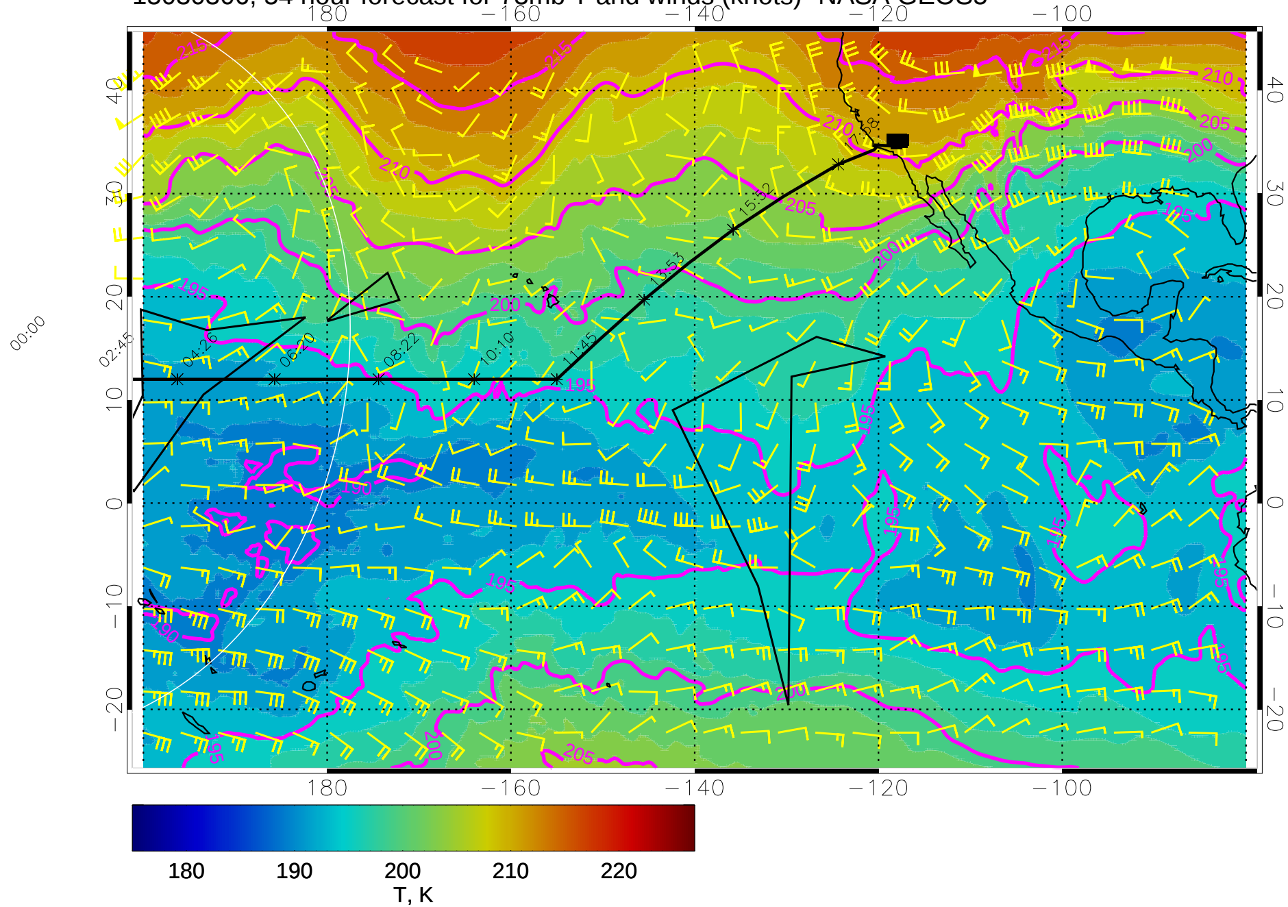
15030306, 54 hour forecast for 73mb T and winds (knots)- NASA GEOS5
