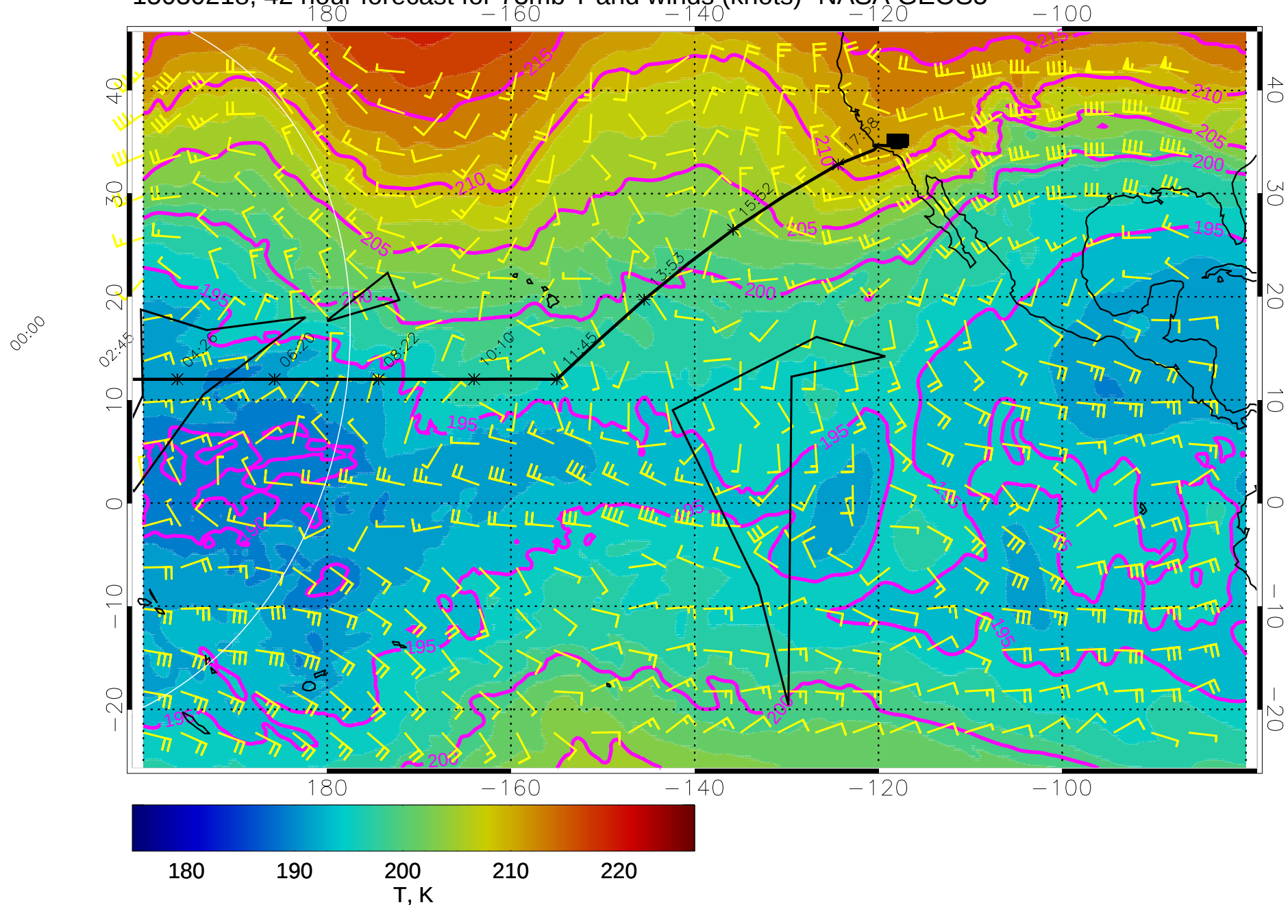
15030218, 42 hour forecast for 73mb T and winds (knots)- NASA GEOS5
