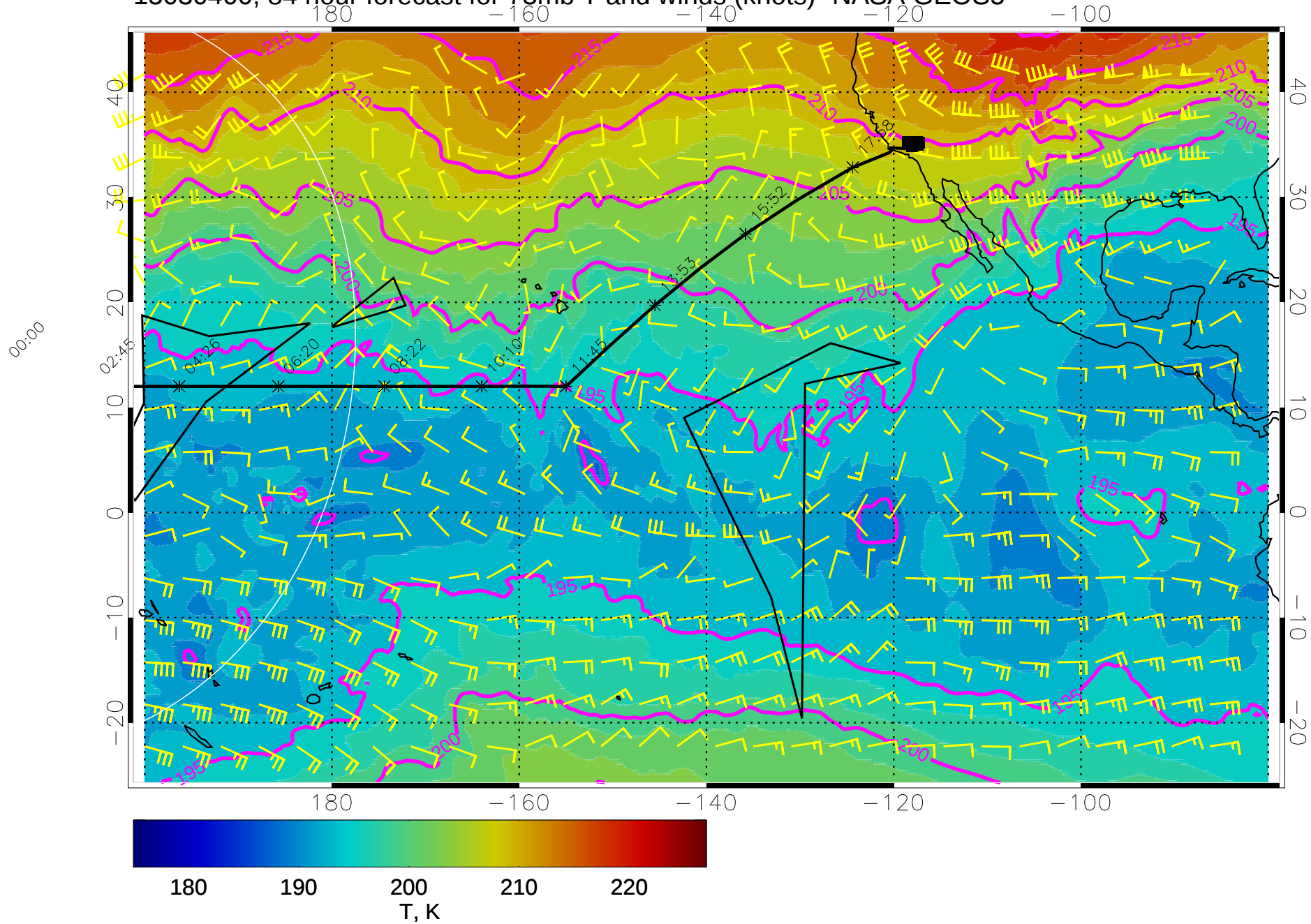
15030400, 84 hour forecast for 73mb T and winds (knots)- NASA GEOS5
