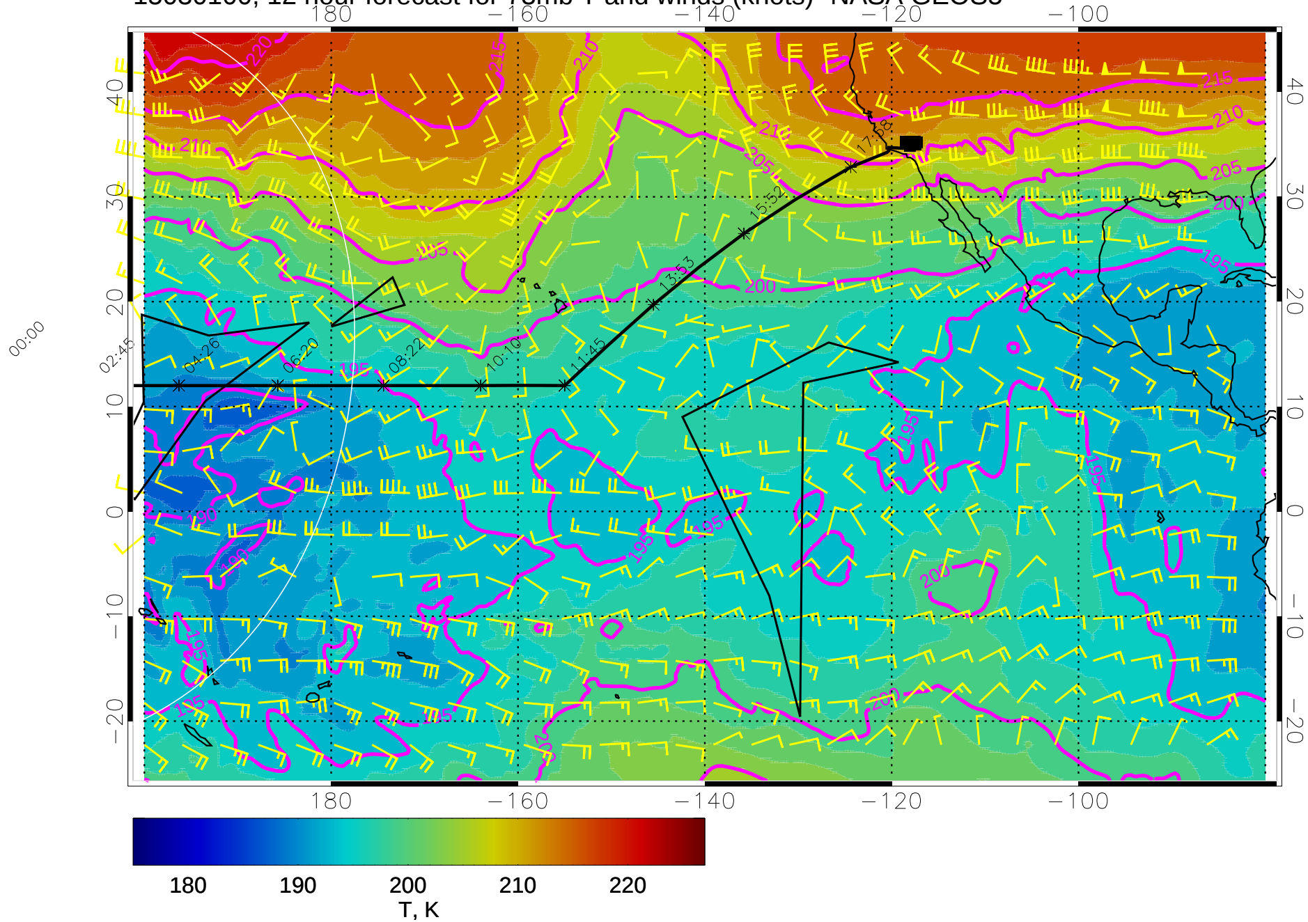
15030100, 12 hour forecast for 73mb T and winds (knots)- NASA GEOS5
