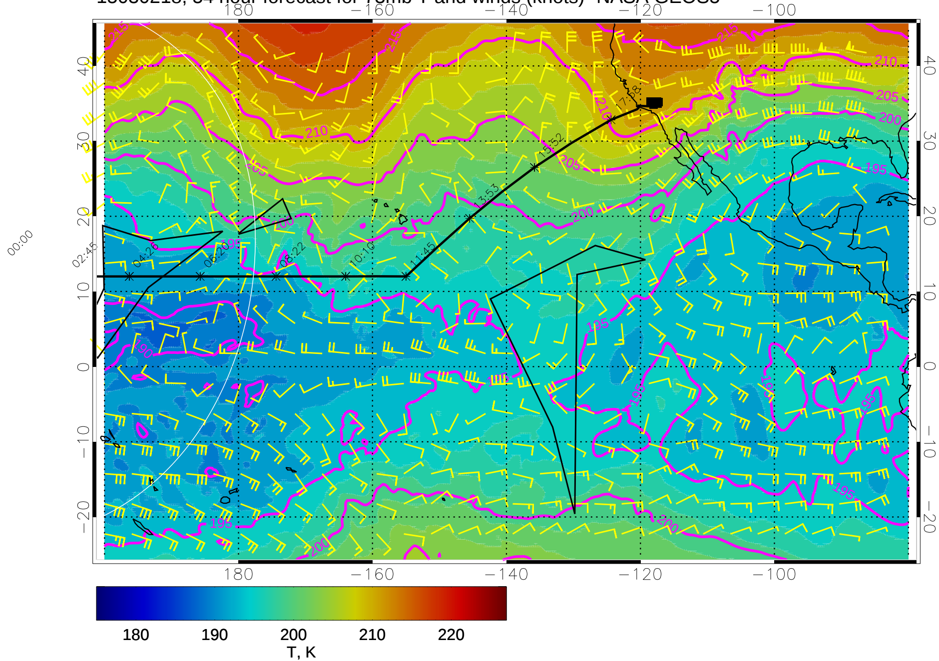
15030218, 54 hour forecast for 73mb T and winds (knots)- NASA GEOS5
