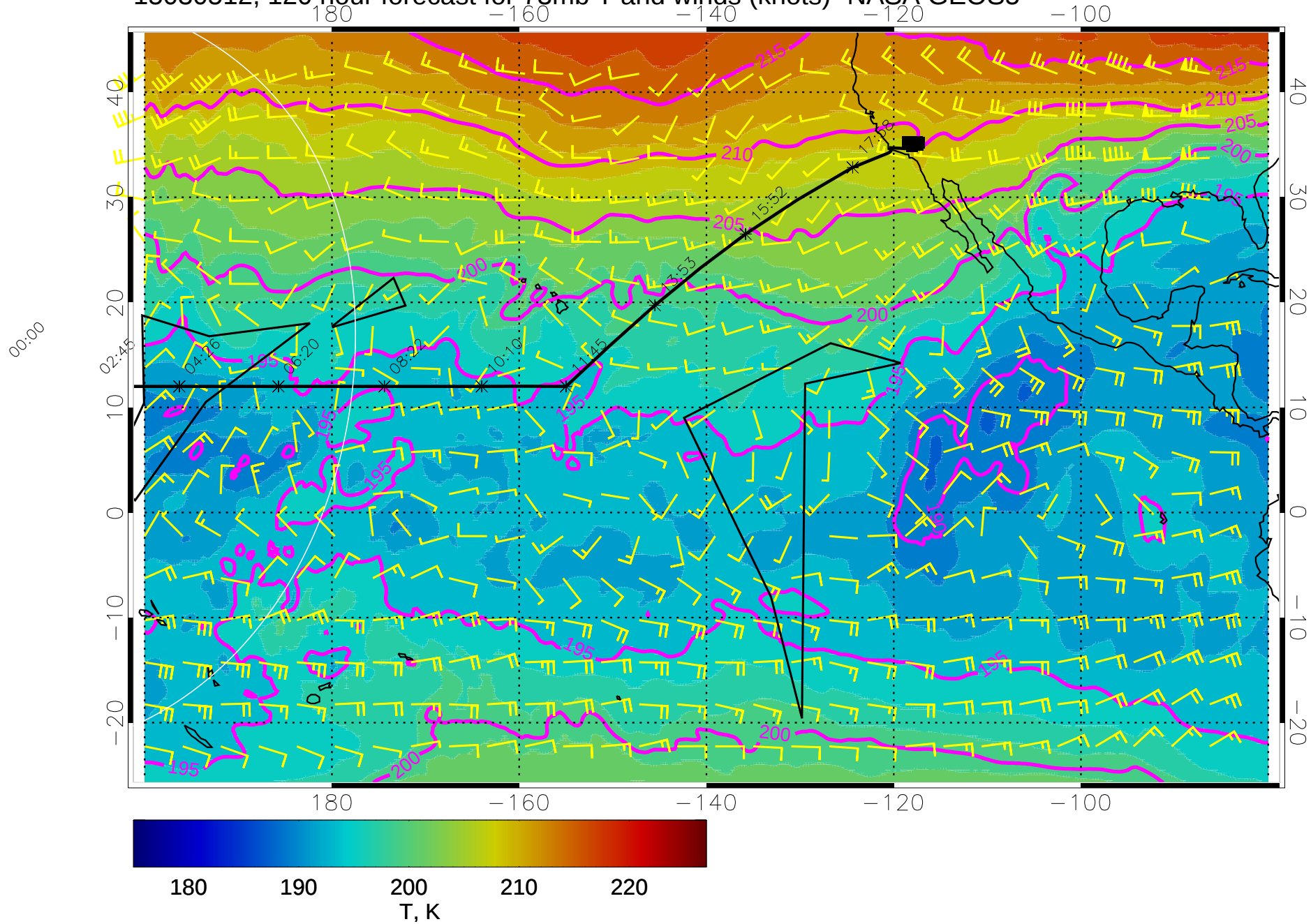
15030512, 120 hour forecast for 73mb T and winds (knots)- NASA GEOS5
