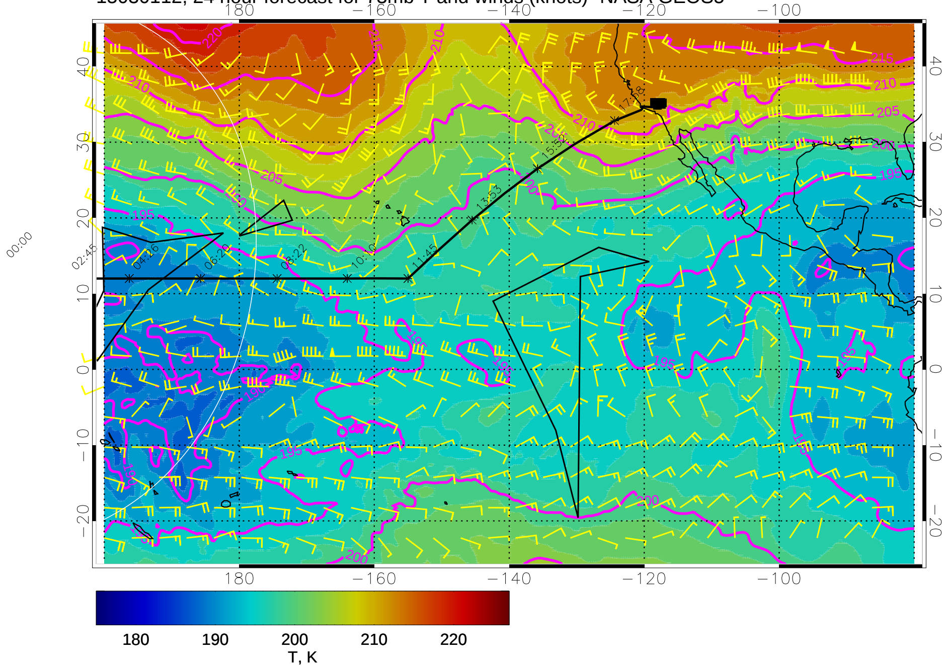
15030112, 24 hour forecast for 73mb T and winds (knots)- NASA GEOS5
