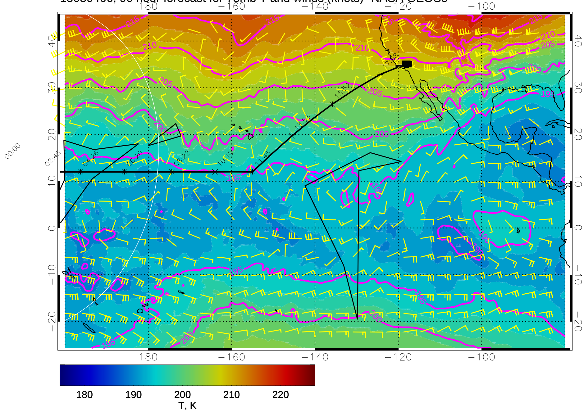
15030406, 90 hour forecast for 73mb T and winds (knots)- NASA GEOS5
