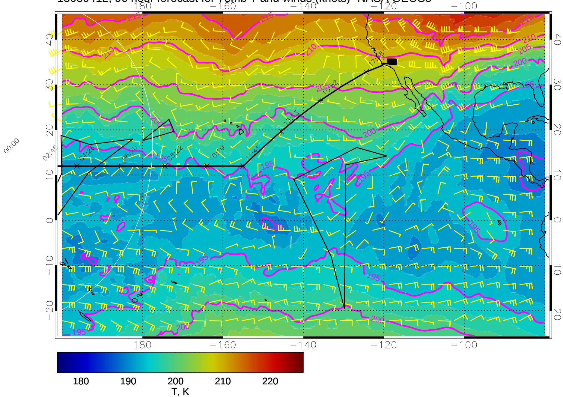
15030412, 96 hour forecast for 73mb T and winds (knots)- NASA GEOS5
