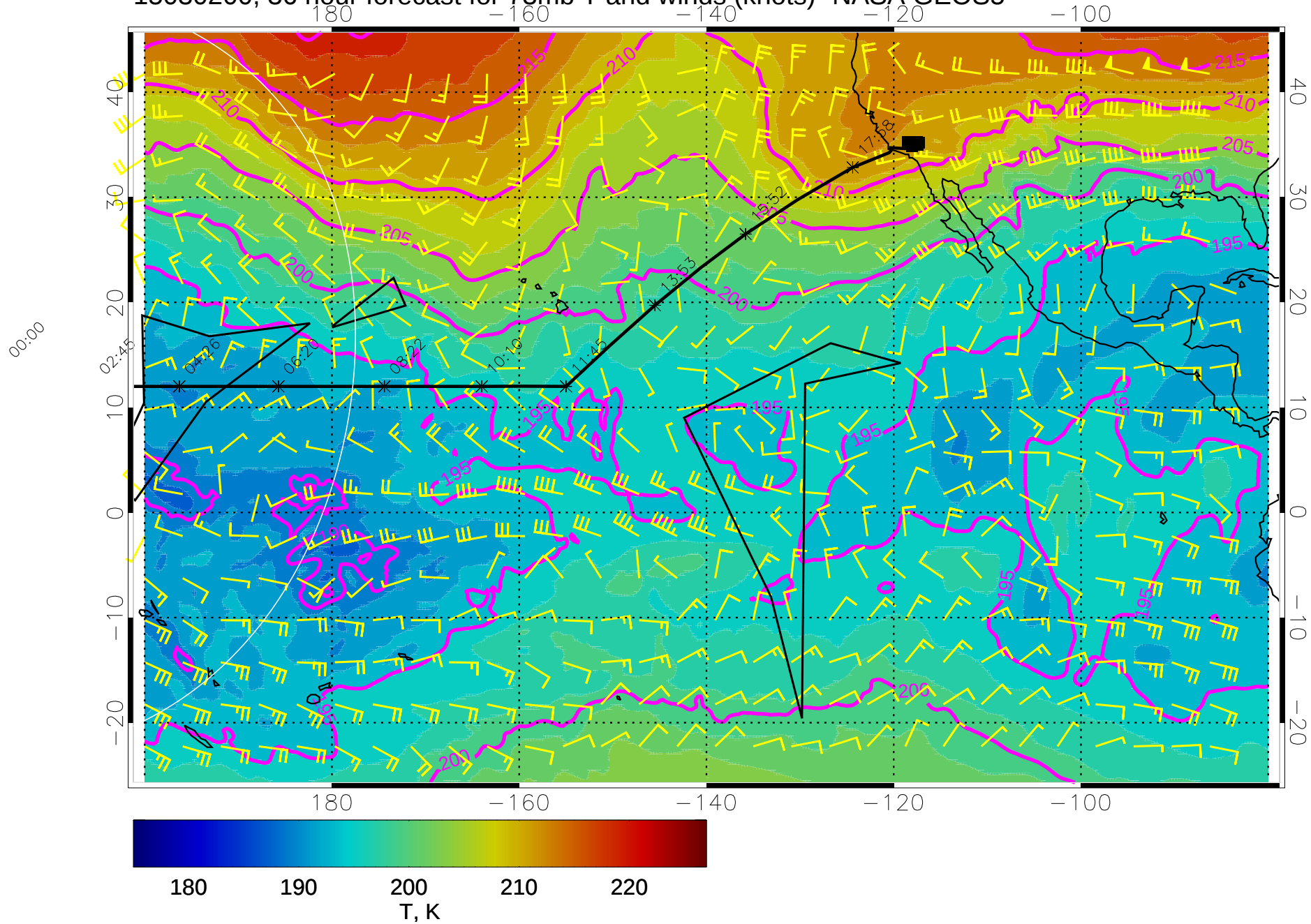
15030200, 36 hour forecast for 73mb T and winds (knots)- NASA GEOS5
