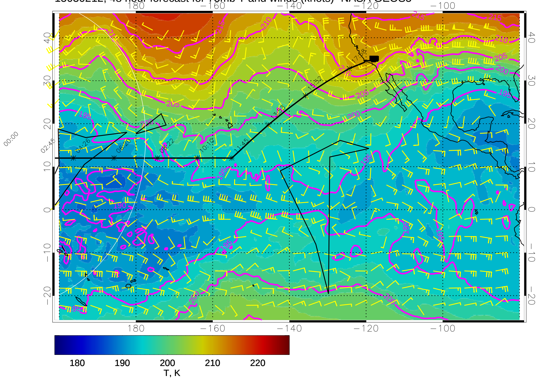
15030212, 48 hour forecast for 73mb T and winds (knots)- NASA GEOS5
