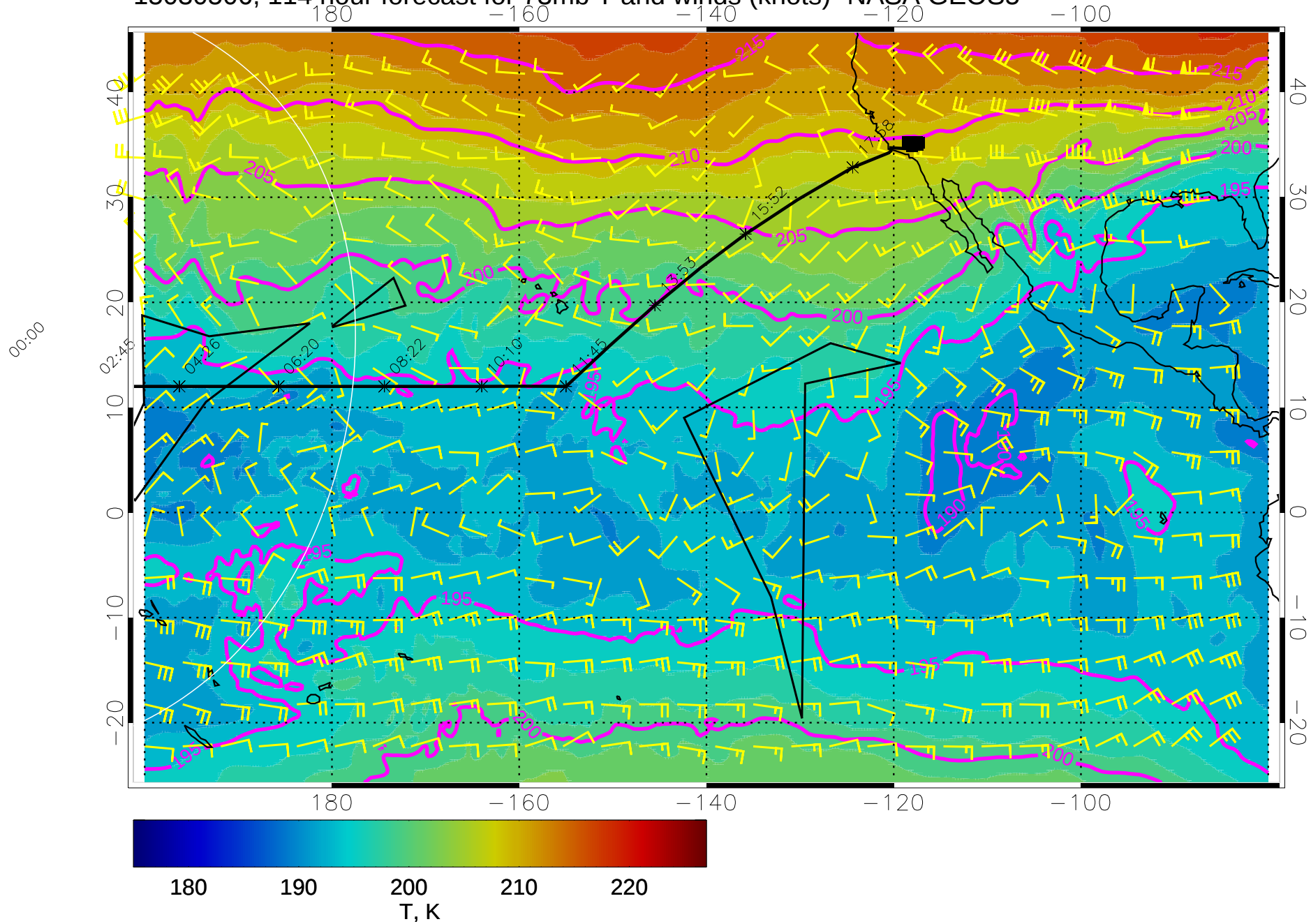
15030506, 114 hour forecast for 73mb T and winds (knots)- NASA GEOS5
