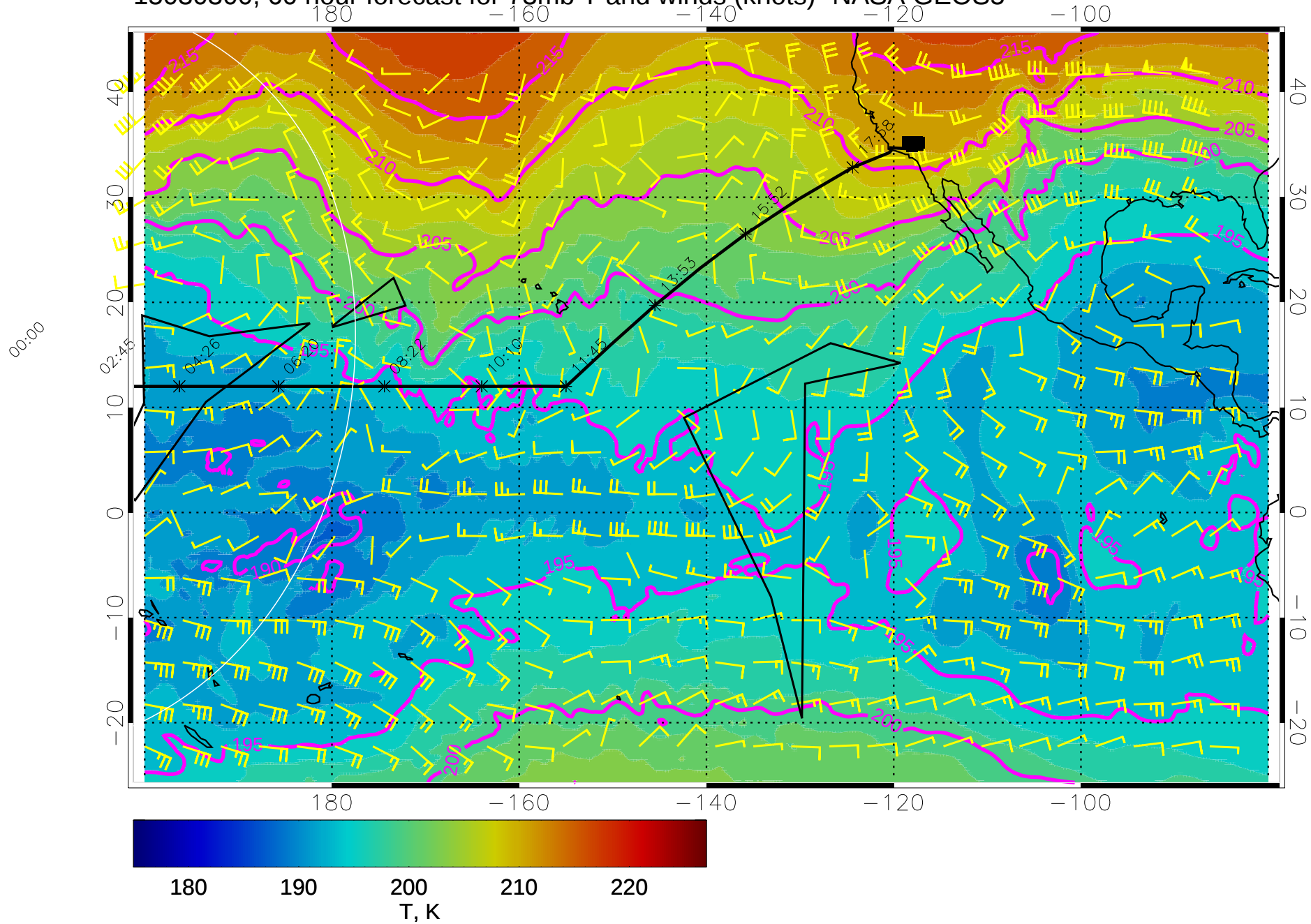
15030300, 60 hour forecast for 73mb T and winds (knots)- NASA GEOS5
