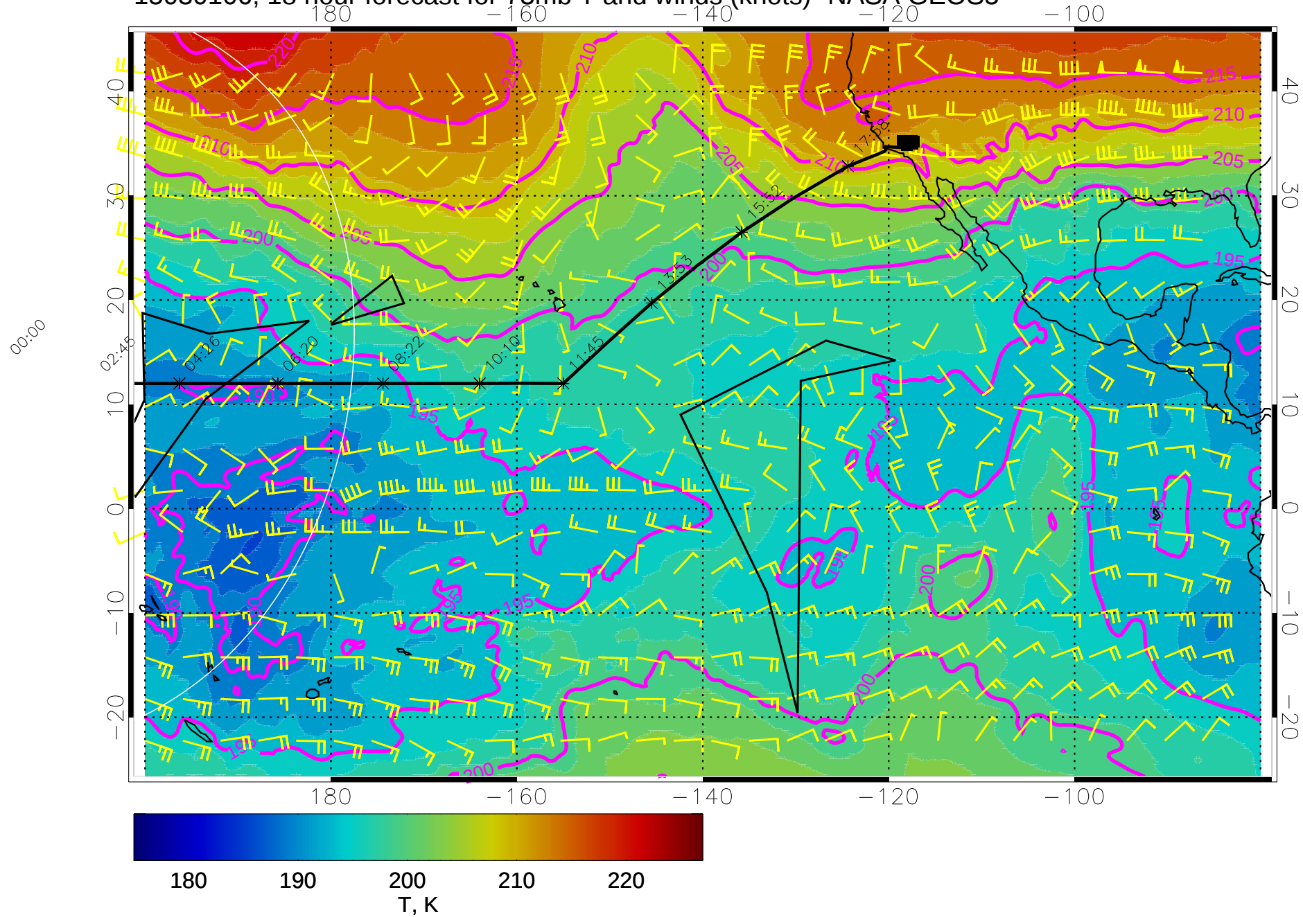
15030106, 18 hour forecast for 73mb T and winds (knots)- NASA GEOS5
