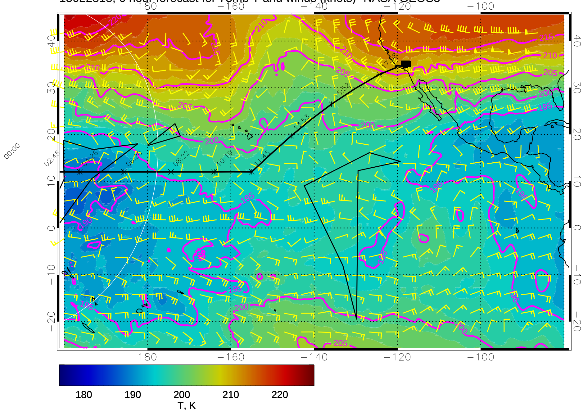
15022818, 6 hour forecast for 73mb T and winds (knots)- NASA GEOS5
