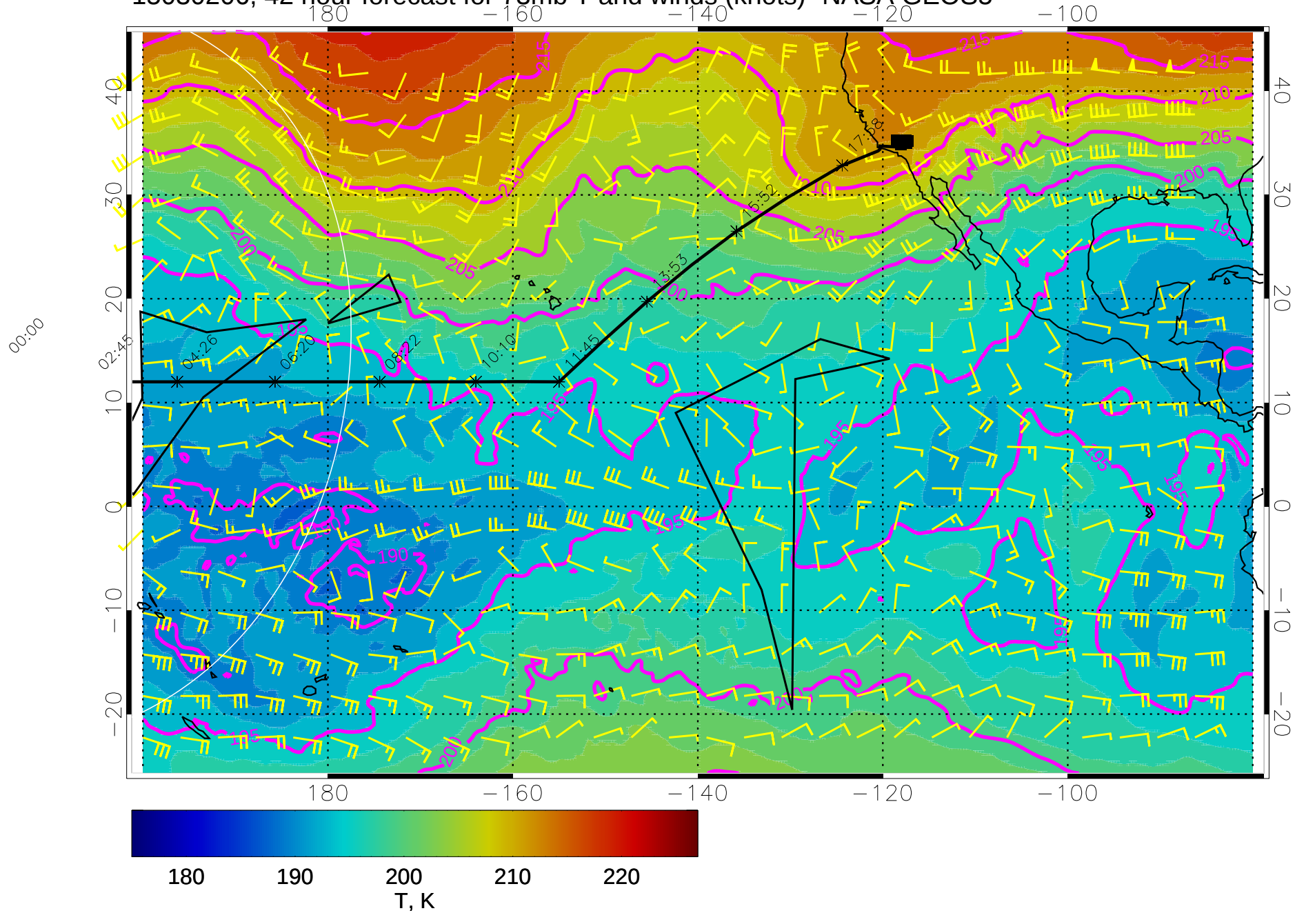
15030206, 42 hour forecast for 73mb T and winds (knots)- NASA GEOS5
