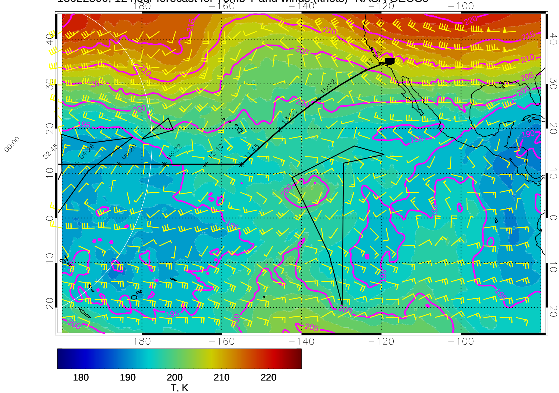
15022800, 12 hour forecast for 73mb T and winds (knots)- NASA GEOS5
