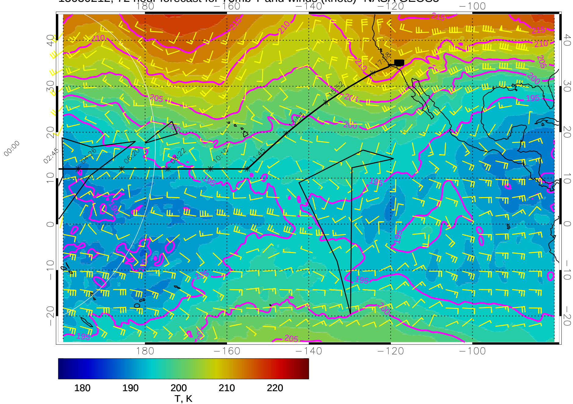
15030212, 72 hour forecast for 73mb T and winds (knots)- NASA GEOS5
