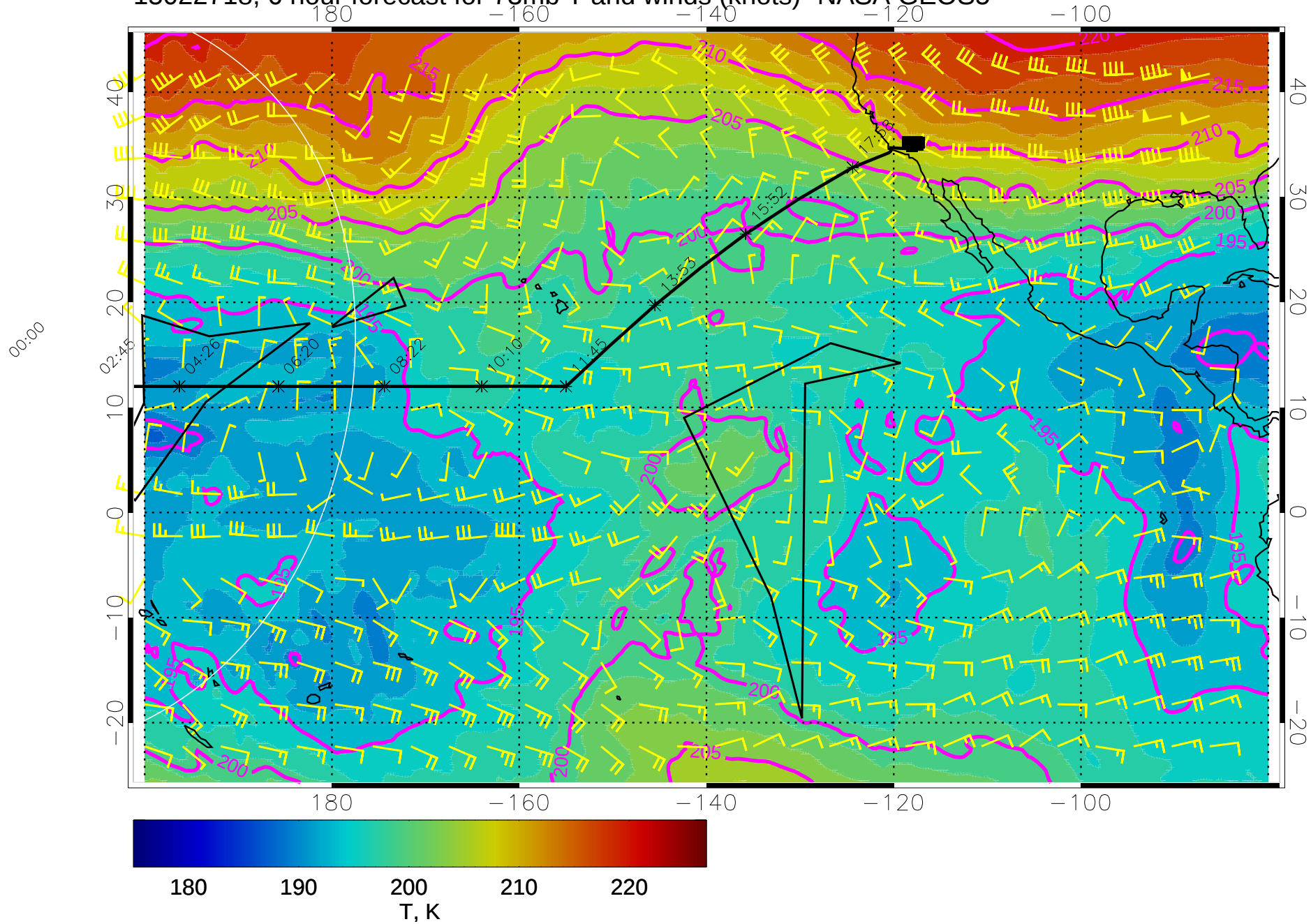
15022718, 6 hour forecast for 73mb T and winds (knots)- NASA GEOS5
