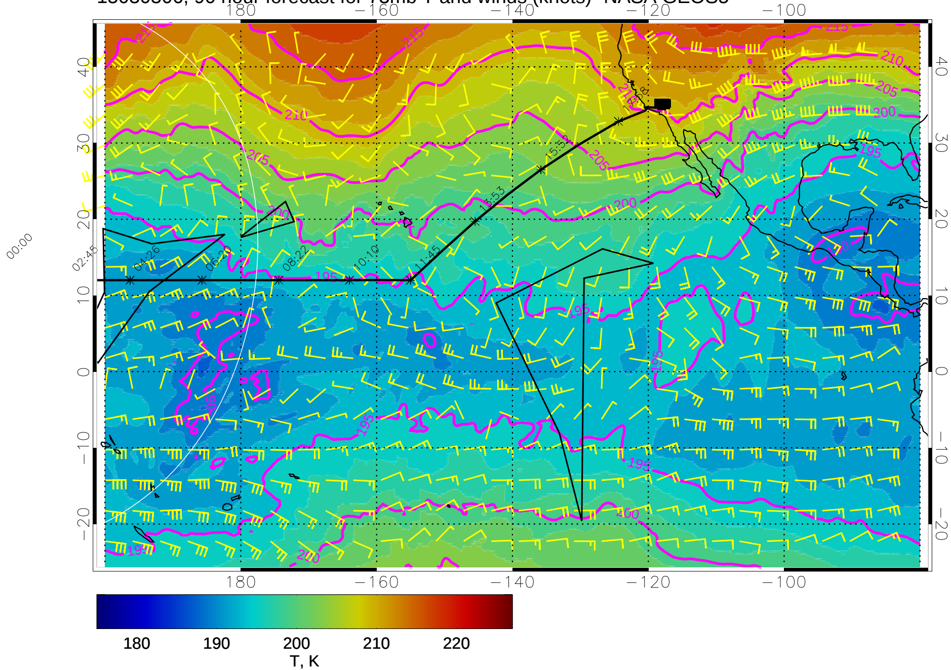
15030306, 90 hour forecast for 73mb T and winds (knots)- NASA GEOS5
