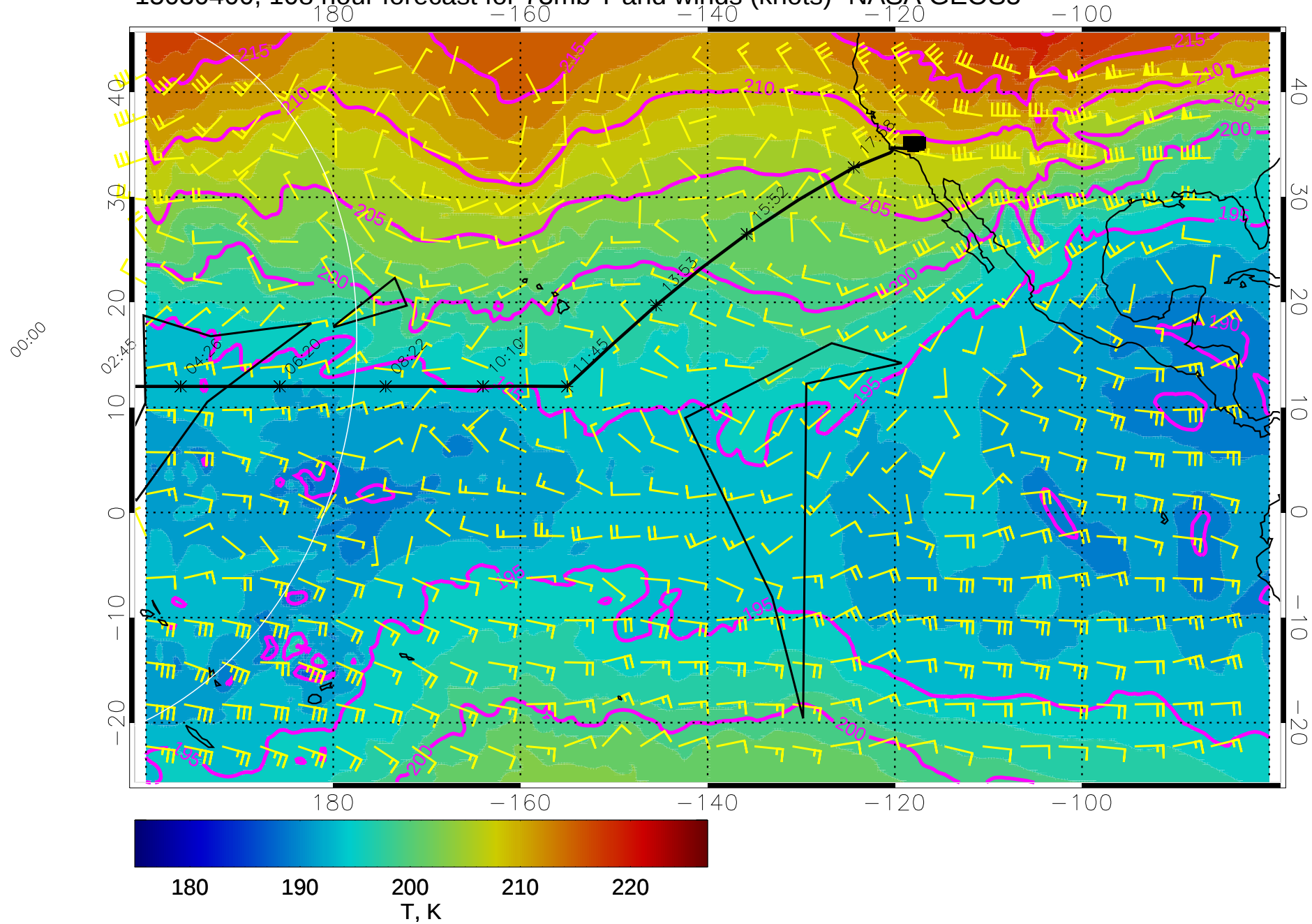
15030400, 108 hour forecast for 73mb T and winds (knots)- NASA GEOS5
