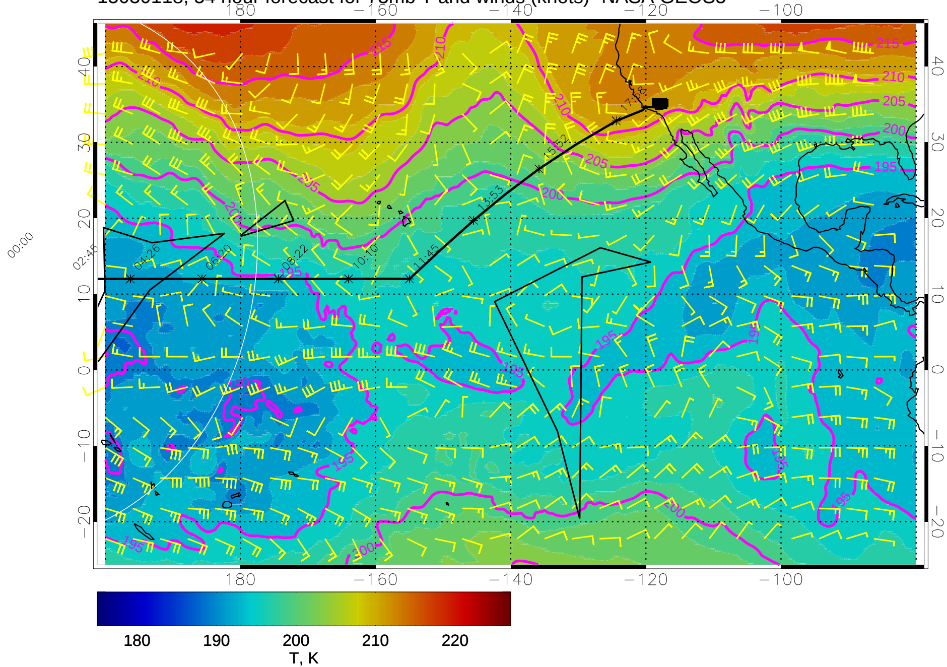
15030118, 54 hour forecast for 73mb T and winds (knots)- NASA GEOS5
