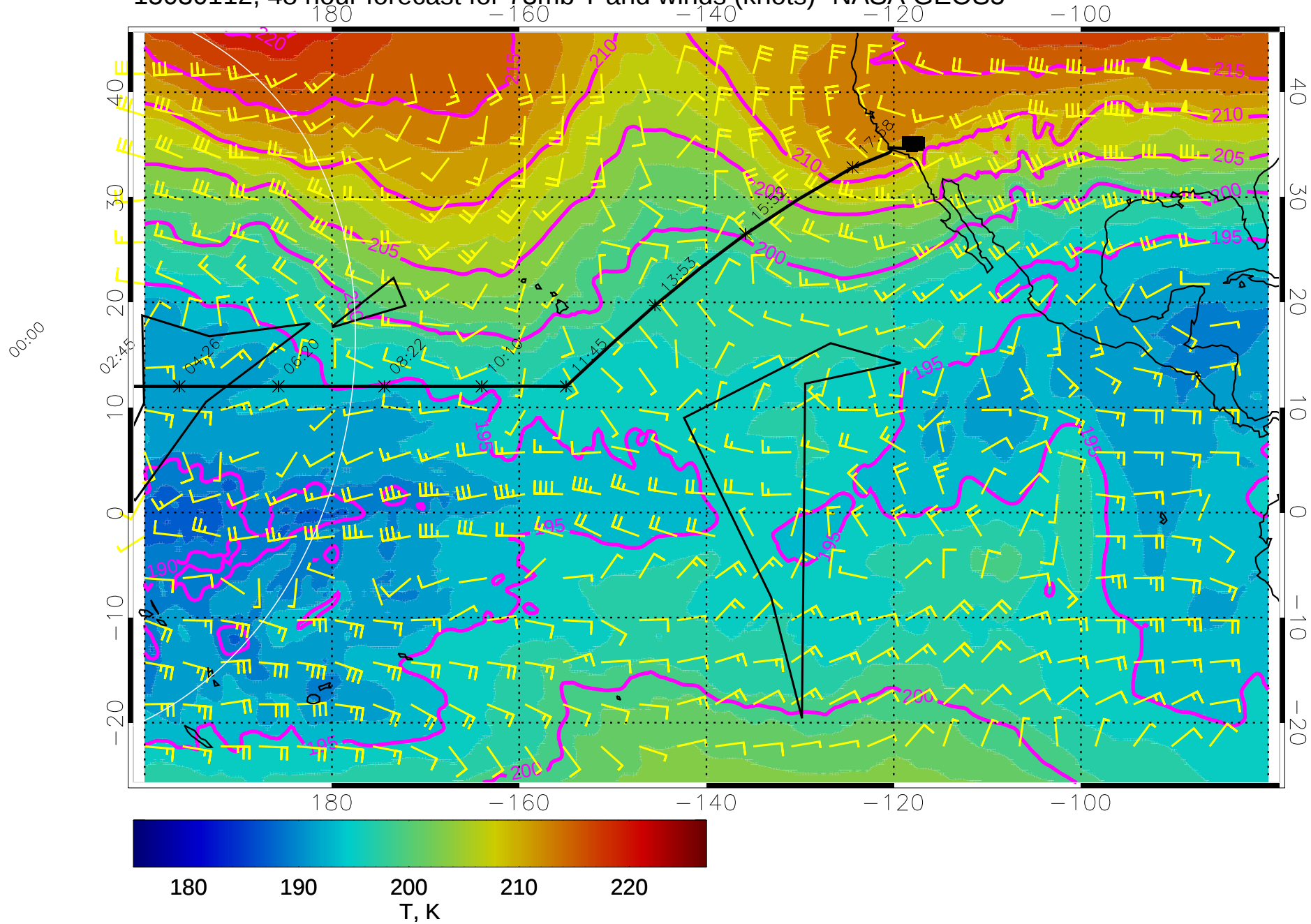
15030112, 48 hour forecast for 73mb T and winds (knots)- NASA GEOS5
