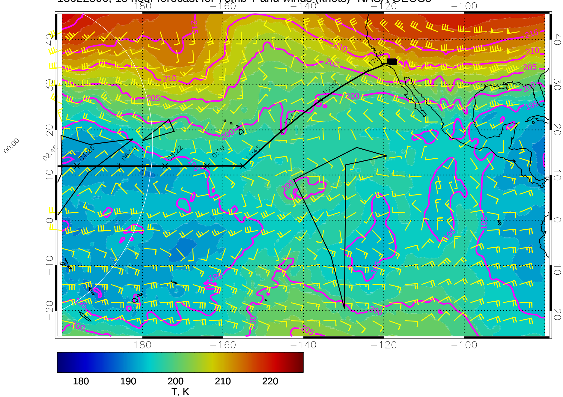
15022806, 18 hour forecast for 73mb T and winds (knots)- NASA GEOS5
