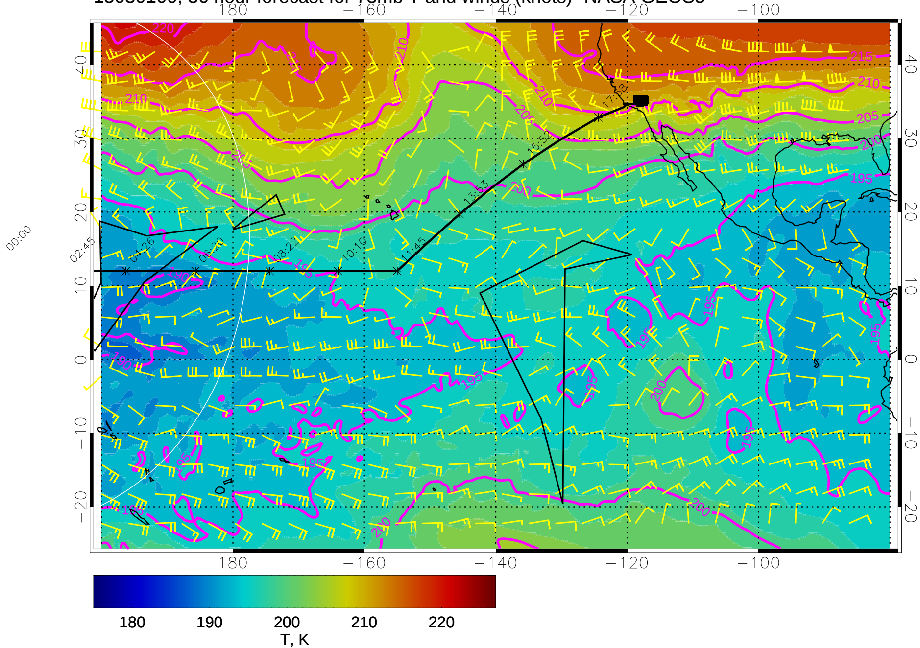
15030100, 36 hour forecast for 73mb T and winds (knots)- NASA GEOS5
