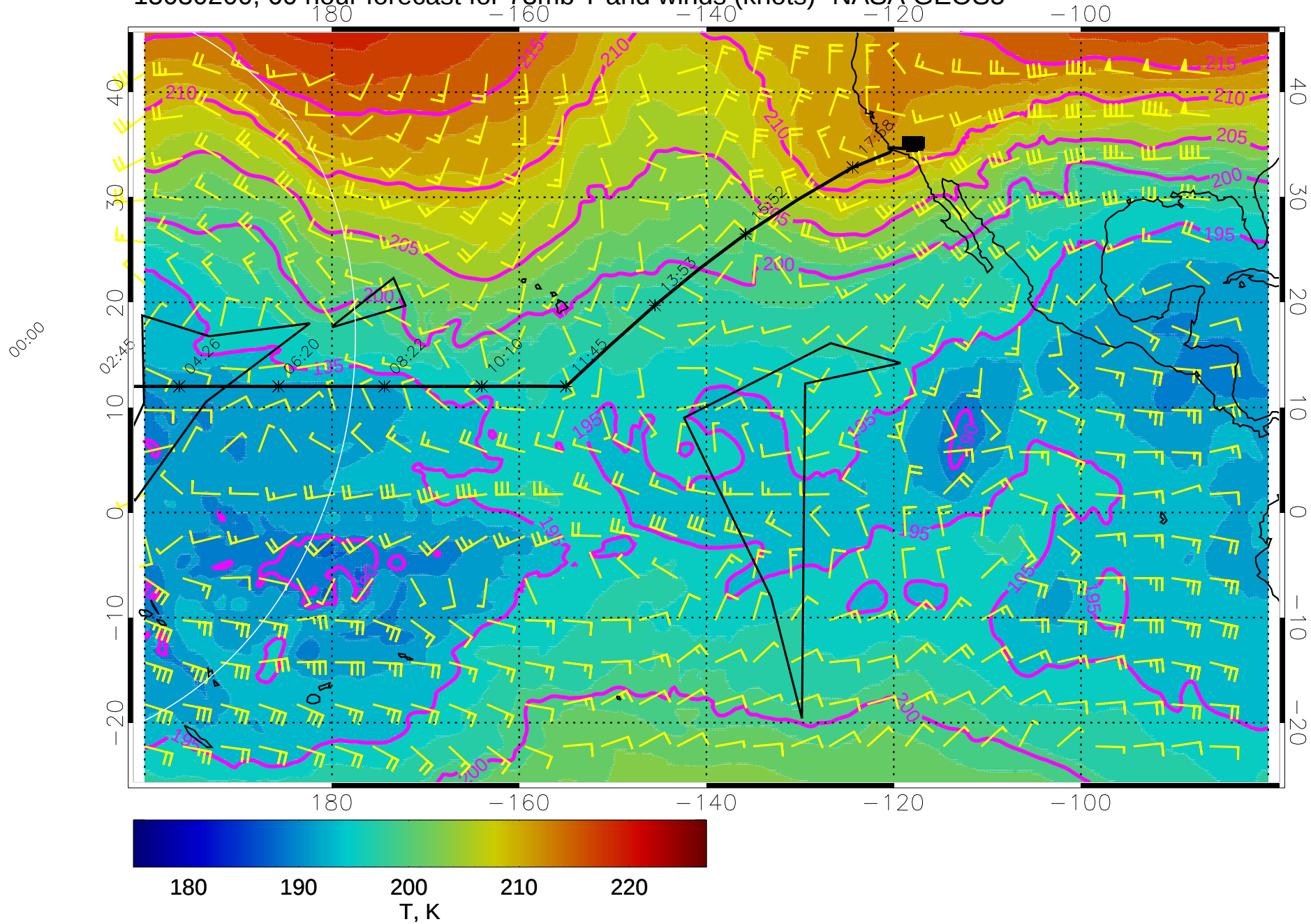
15030200, 60 hour forecast for 73mb T and winds (knots)- NASA GEOS5
