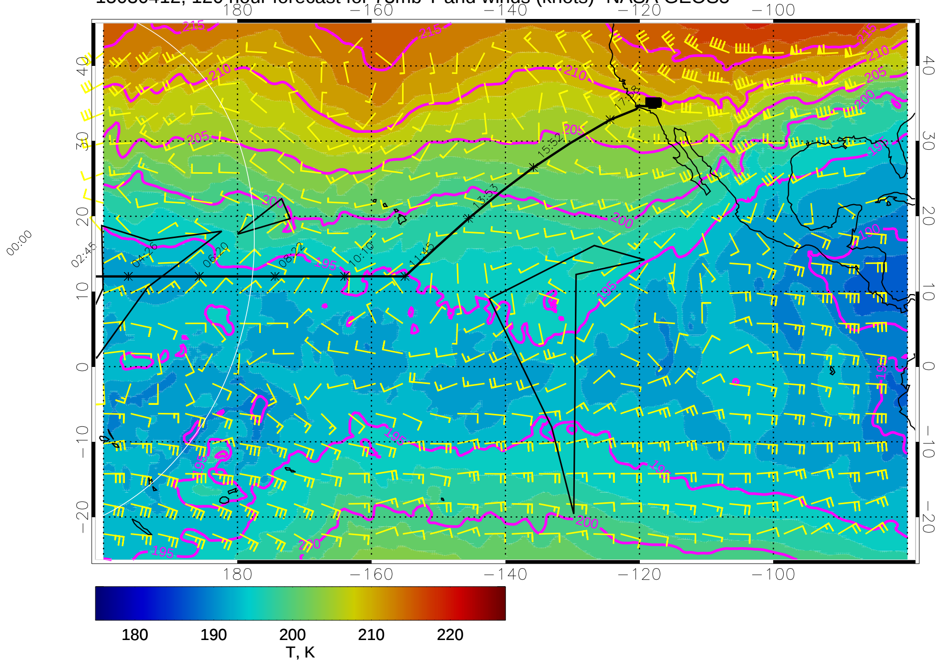
15030412, 120 hour forecast for 73mb T and winds (knots)- NASA GEOS5
