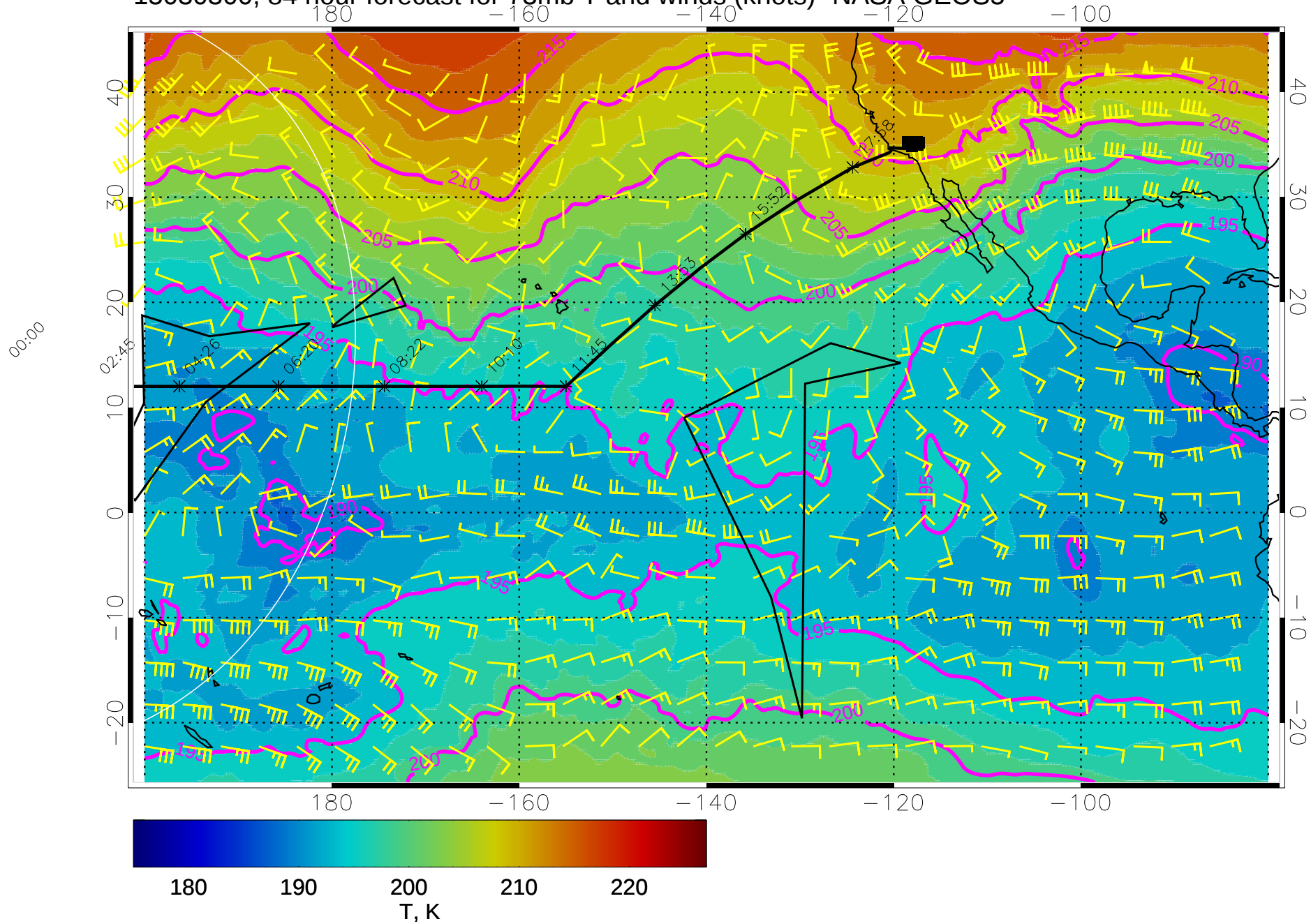
15030300, 84 hour forecast for 73mb T and winds (knots)- NASA GEOS5
