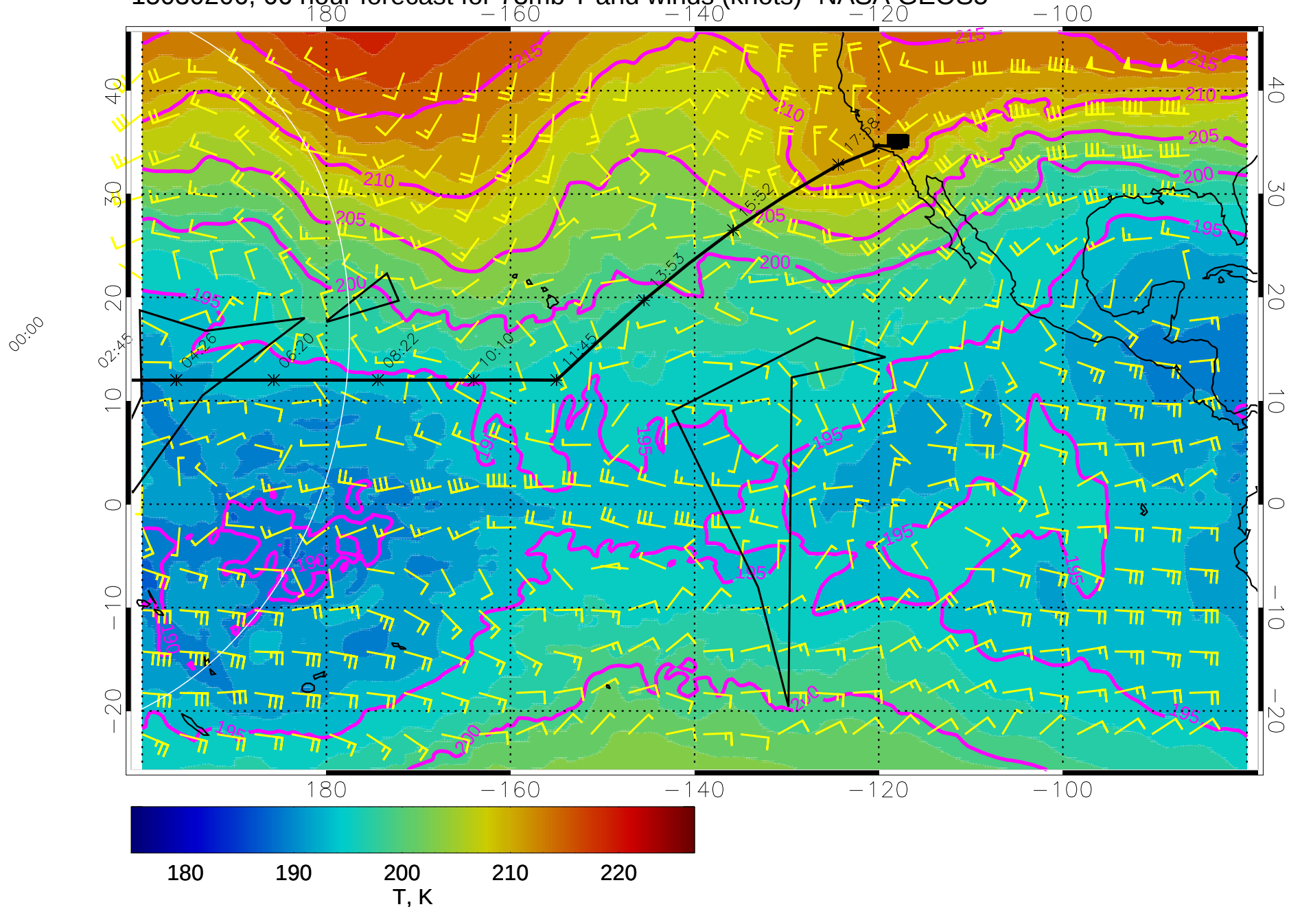
15030206, 66 hour forecast for 73mb T and winds (knots)- NASA GEOS5
