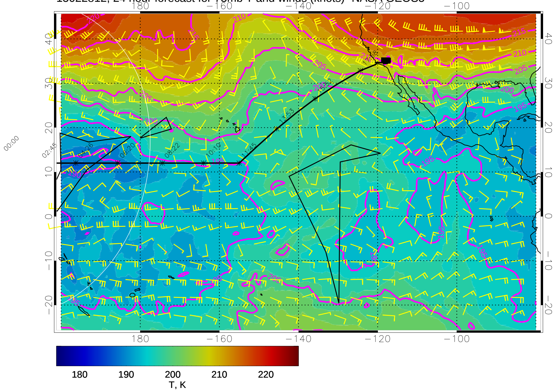
15022812, 24 hour forecast for 73mb T and winds (knots)- NASA GEOS5
