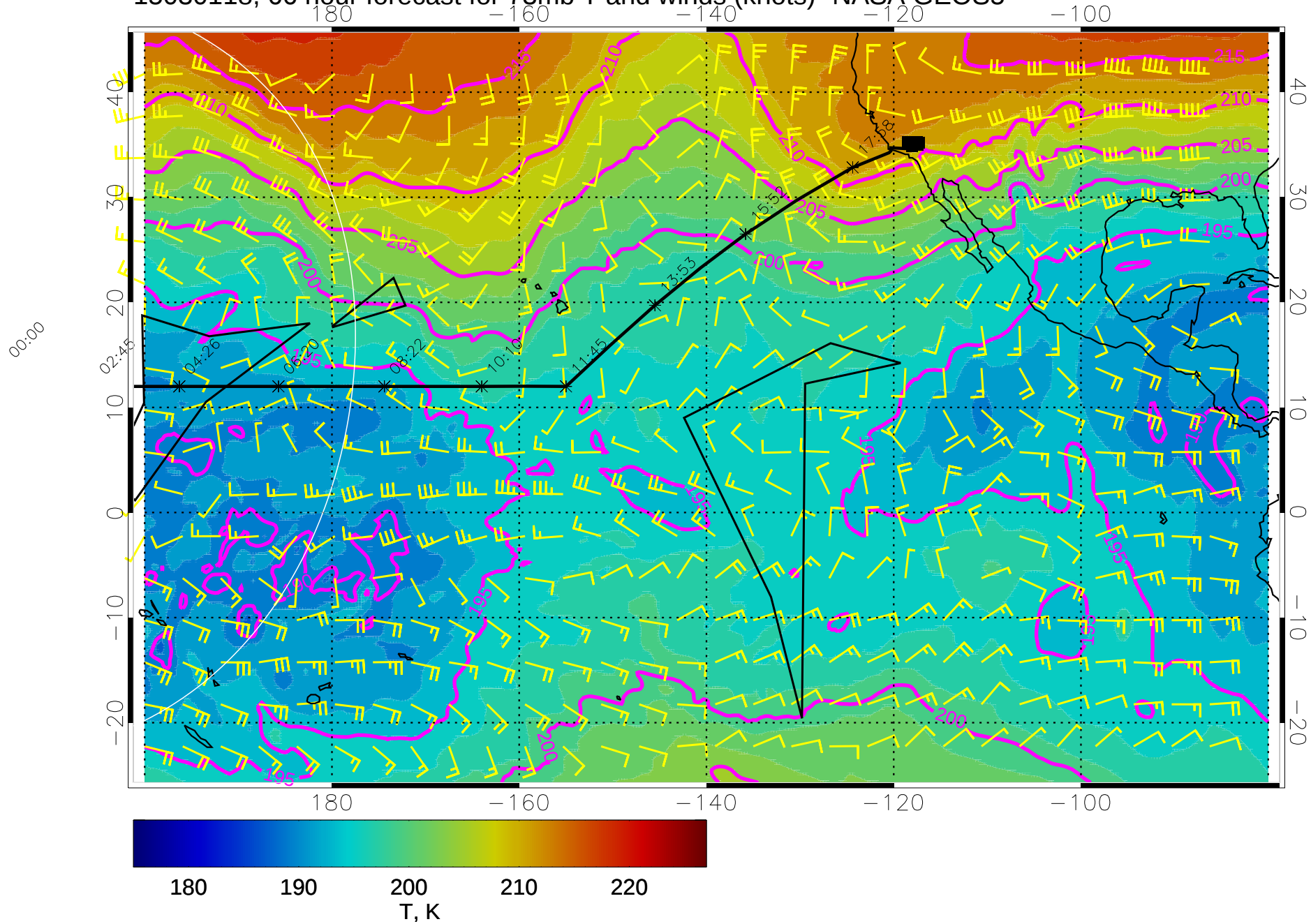
15030118, 66 hour forecast for 73mb T and winds (knots)- NASA GEOS5
