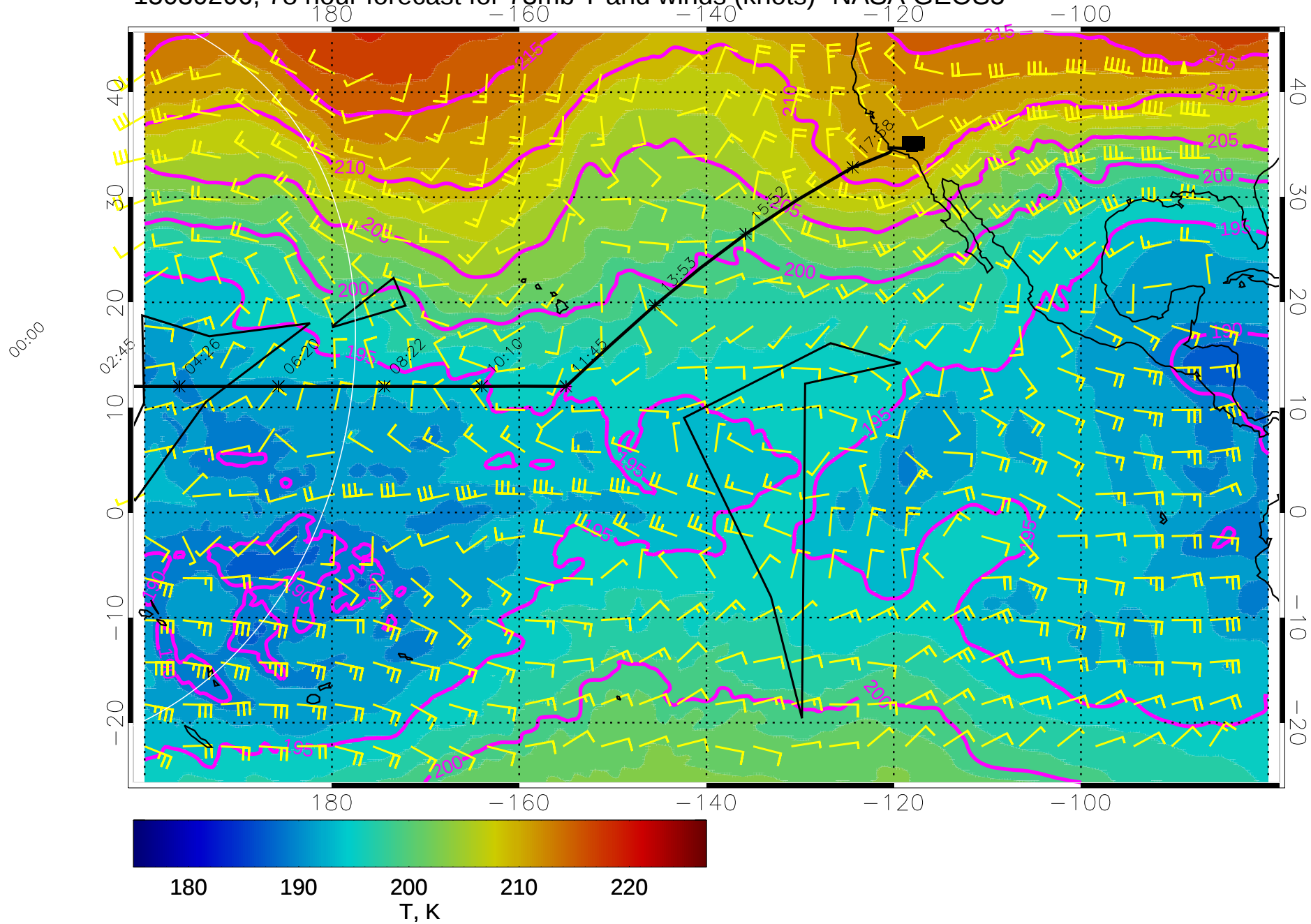
15030206, 78 hour forecast for 73mb T and winds (knots)- NASA GEOS5
