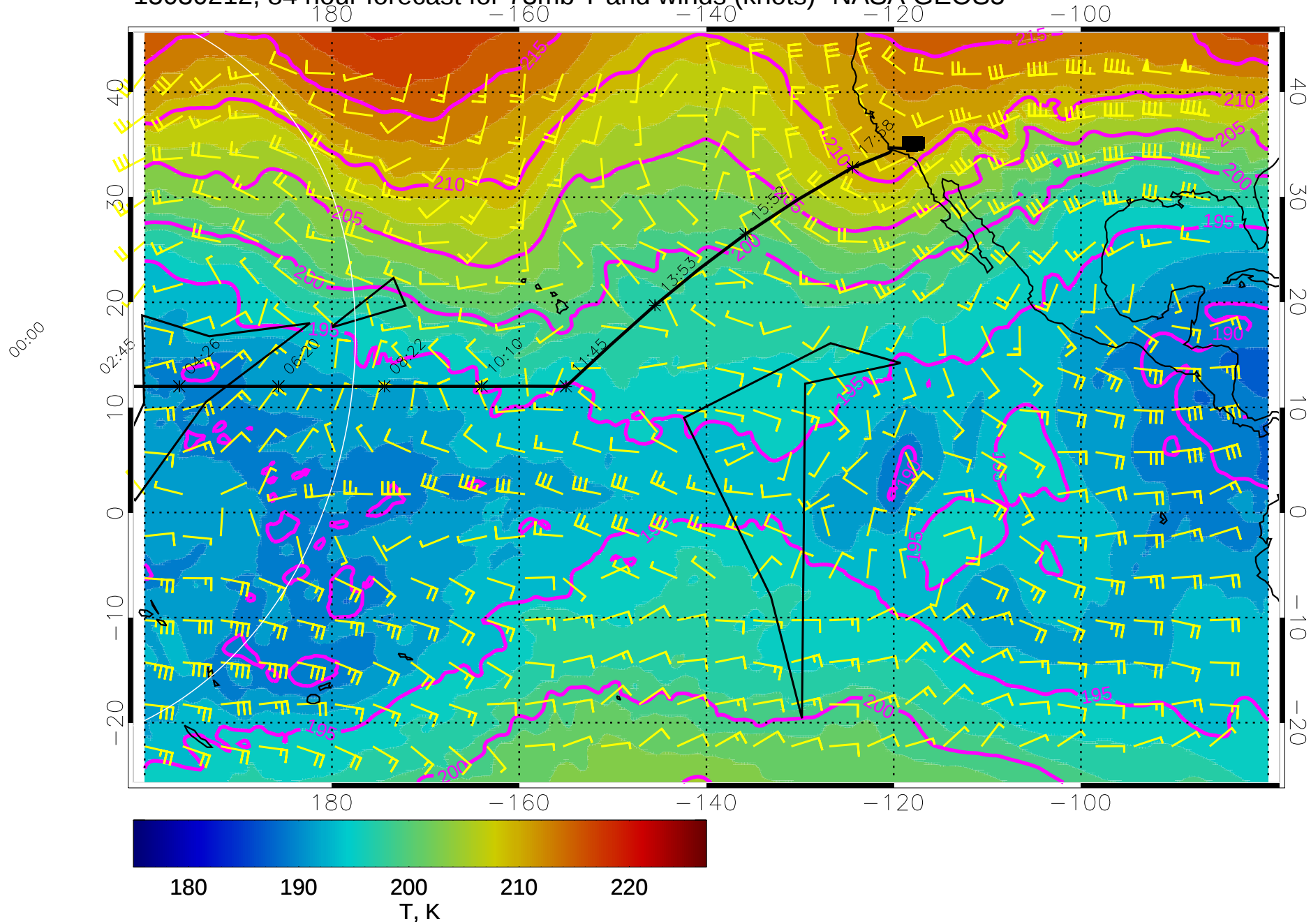
15030212, 84 hour forecast for 73mb T and winds (knots)- NASA GEOS5
