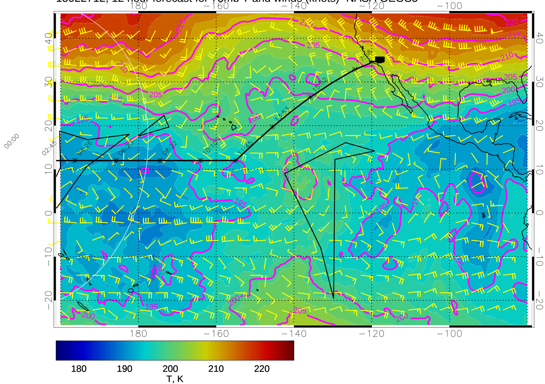
15022712, 12 hour forecast for 73mb T and winds (knots)- NASA GEOS5
