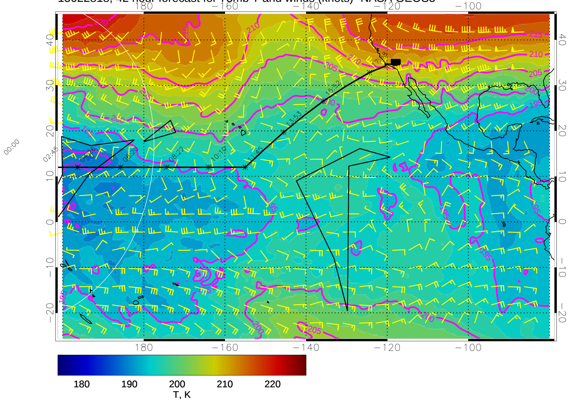
15022818, 42 hour forecast for 73mb T and winds (knots)- NASA GEOS5
