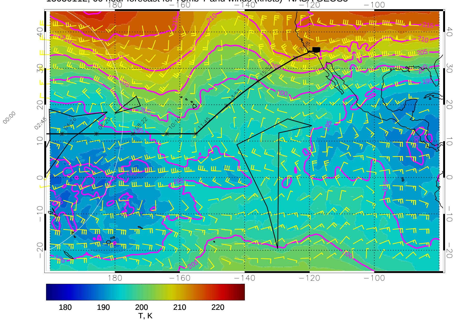
15030112, 60 hour forecast for 73mb T and winds (knots)- NASA GEOS5
