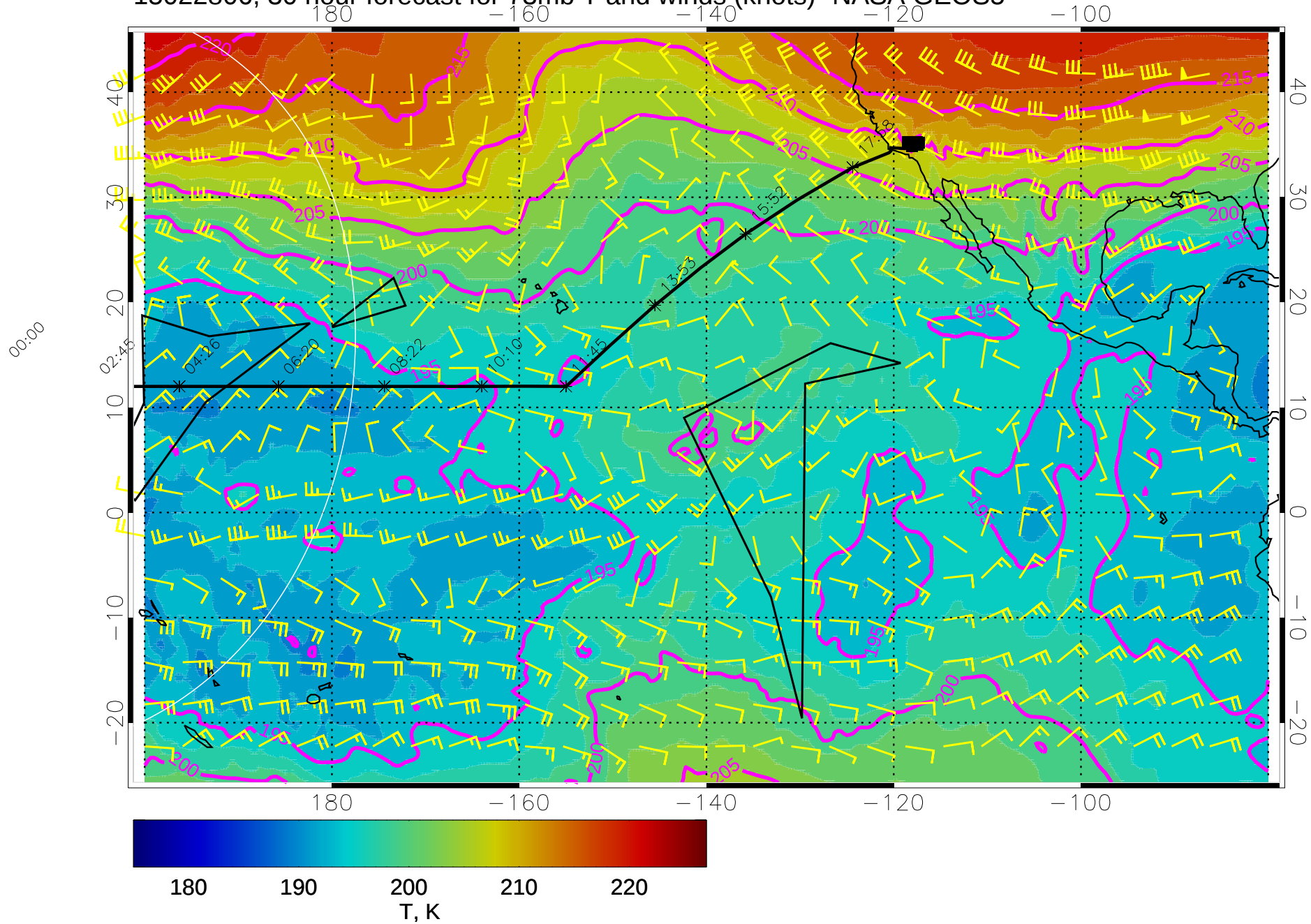
15022806, 30 hour forecast for 73mb T and winds (knots)- NASA GEOS5
