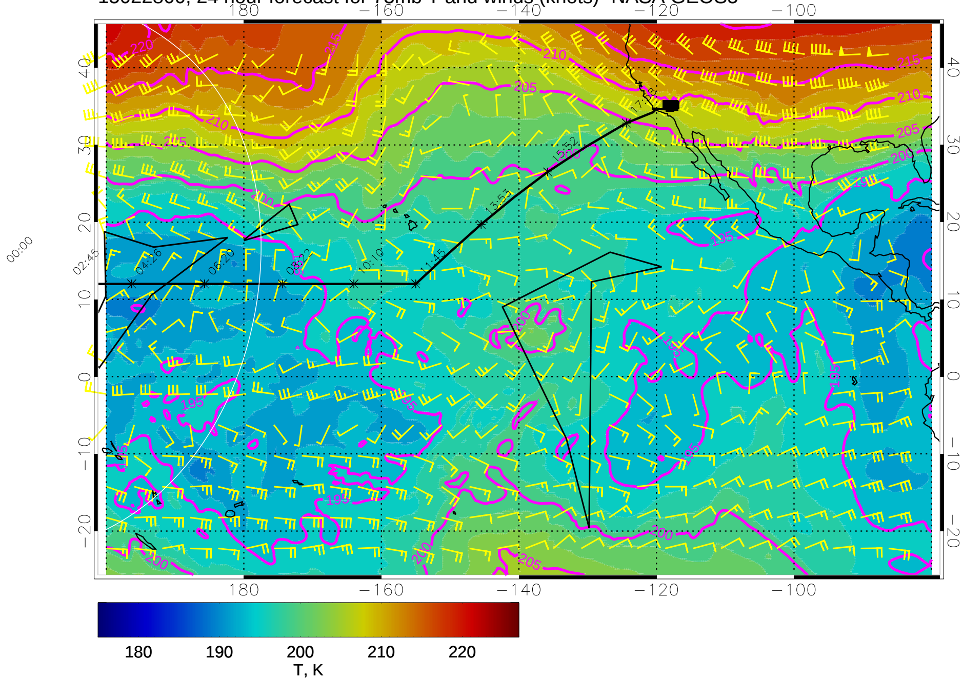
15022800, 24 hour forecast for 73mb T and winds (knots)- NASA GEOS5
