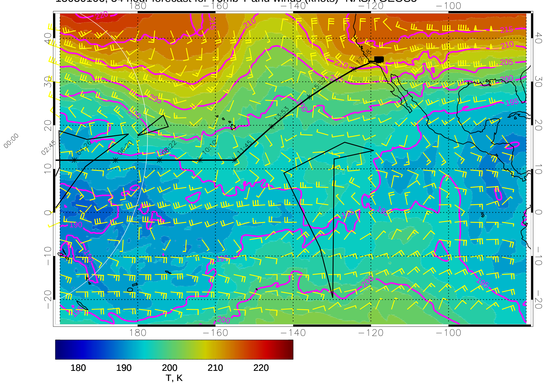
15030106, 54 hour forecast for 73mb T and winds (knots)- NASA GEOS5
