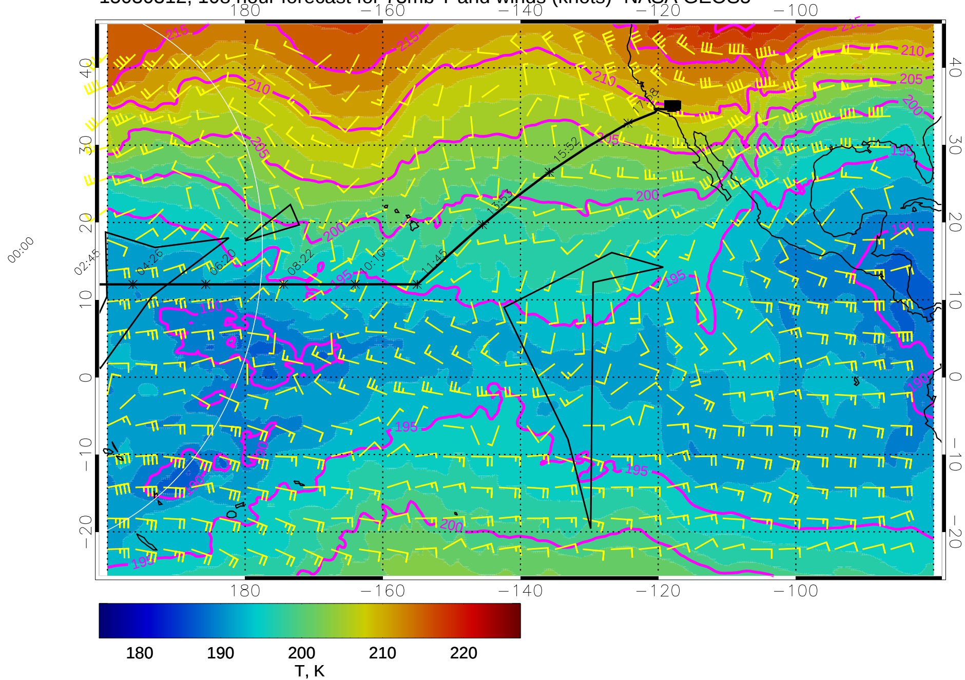
15030312, 108 hour forecast for 73mb T and winds (knots)- NASA GEOS5
