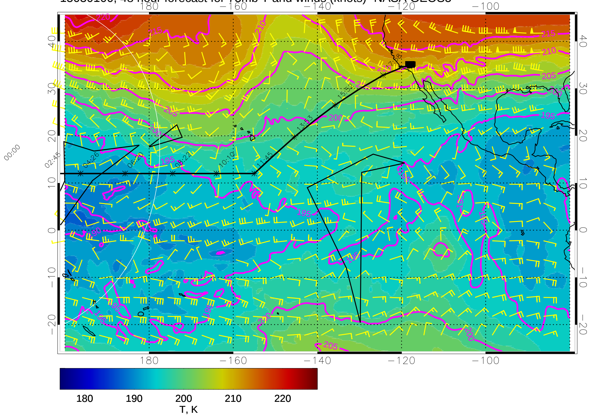
15030100, 48 hour forecast for 73mb T and winds (knots)- NASA GEOS5
