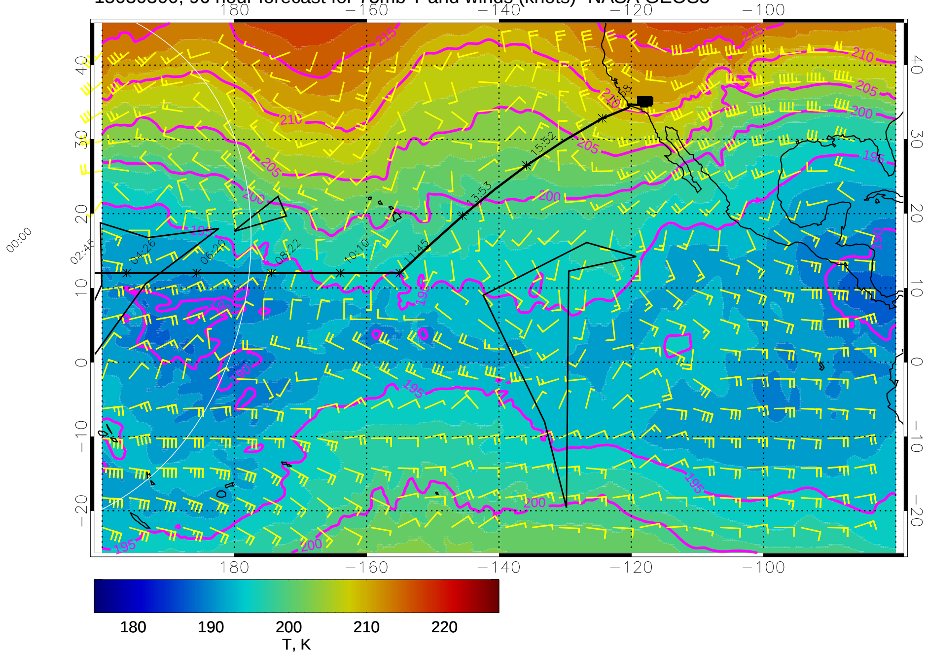
15030300, 96 hour forecast for 73mb T and winds (knots)- NASA GEOS5
