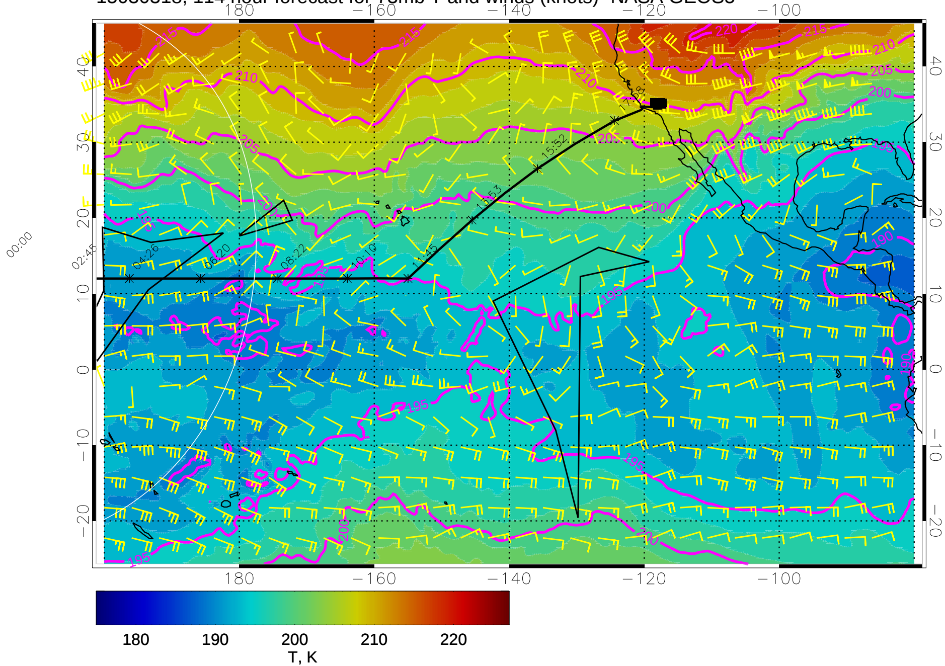
15030318, 114 hour forecast for 73mb T and winds (knots)- NASA GEOS5
