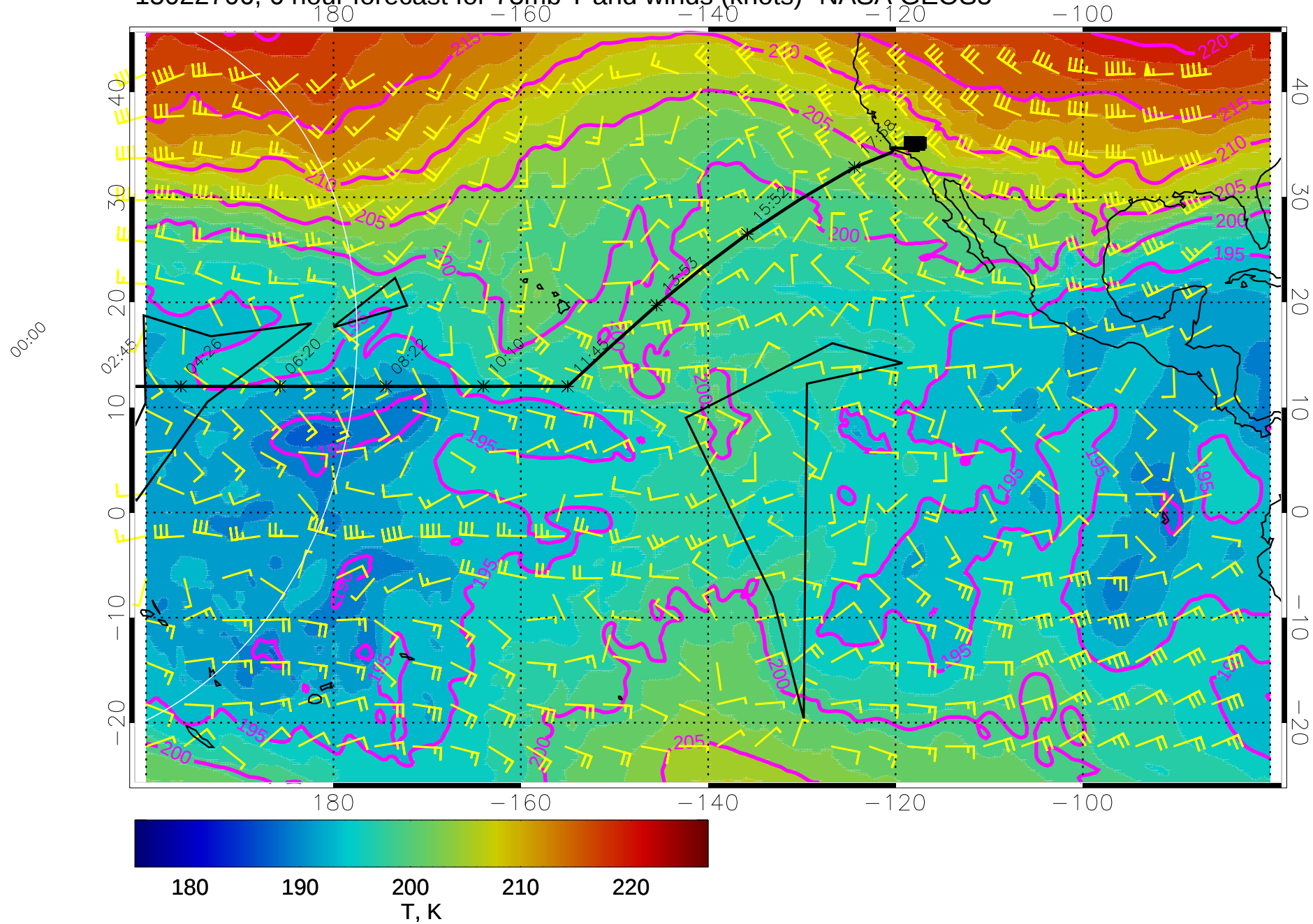
15022706, 6 hour forecast for 73mb T and winds (knots)- NASA GEOS5
