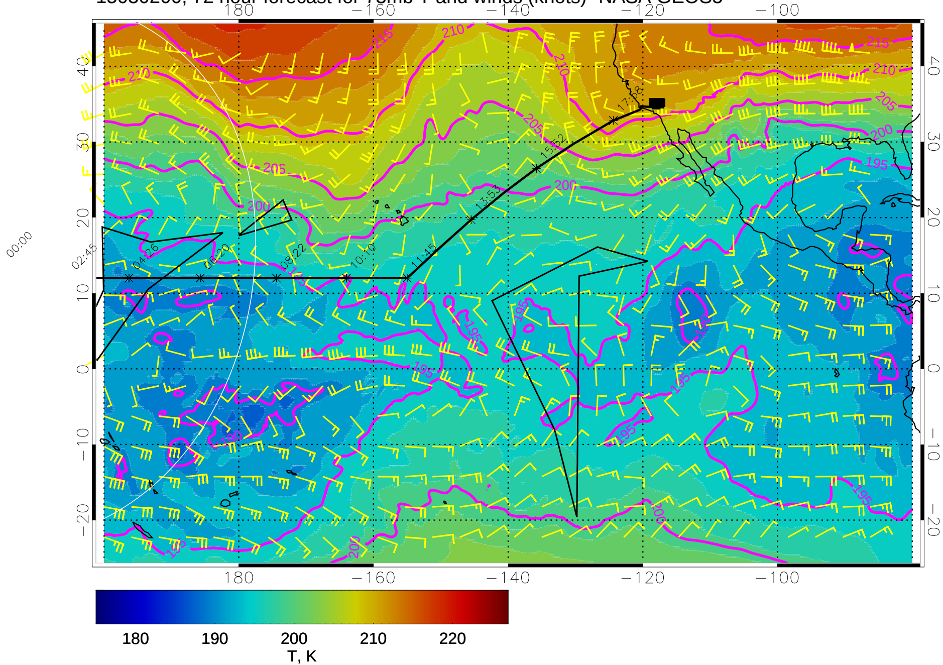
15030200, 72 hour forecast for 73mb T and winds (knots)- NASA GEOS5
