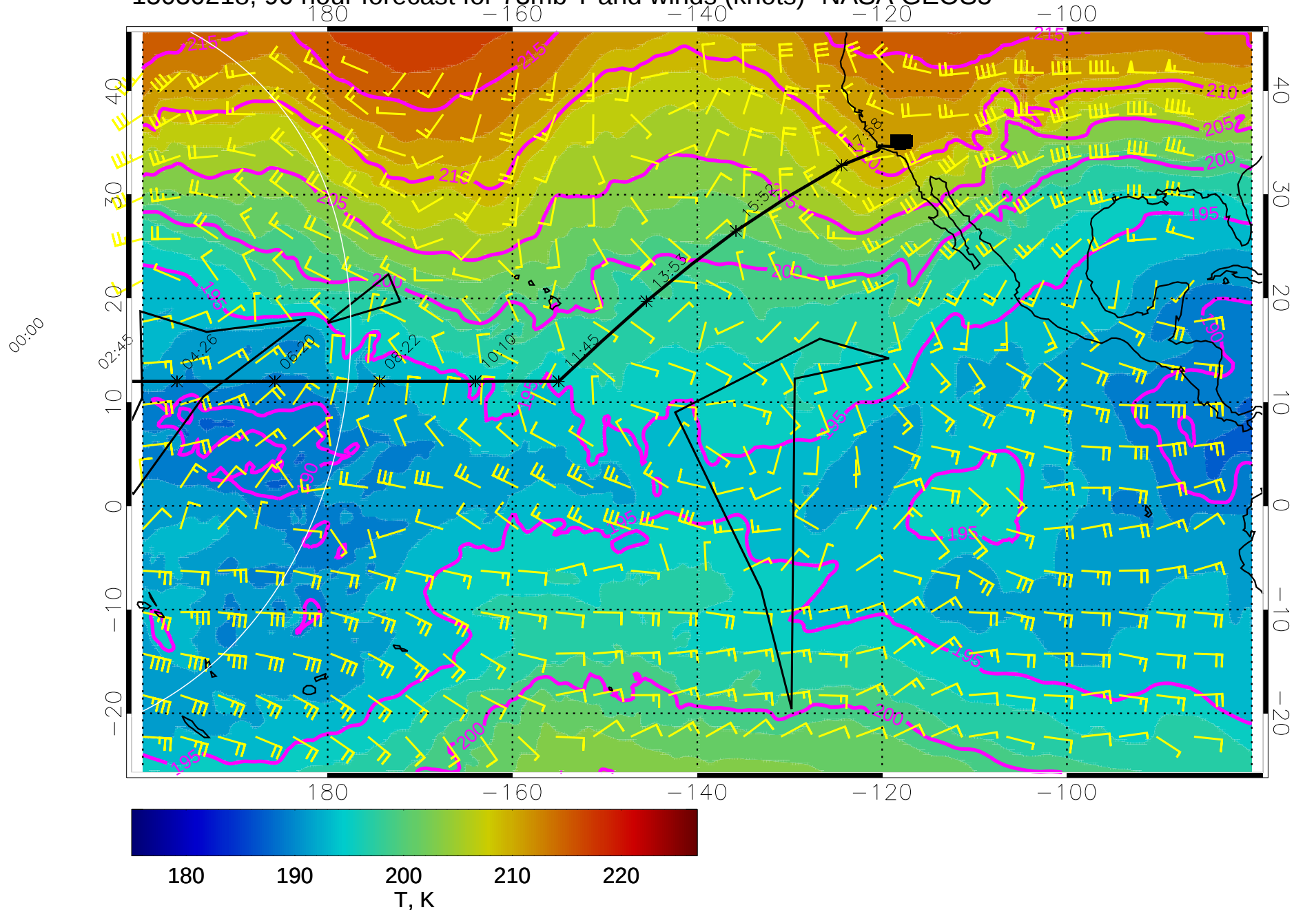
15030218, 90 hour forecast for 73mb T and winds (knots)- NASA GEOS5
