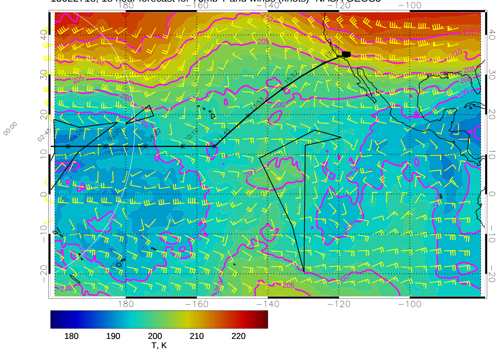
15022718, 18 hour forecast for 73mb T and winds (knots)- NASA GEOS5
