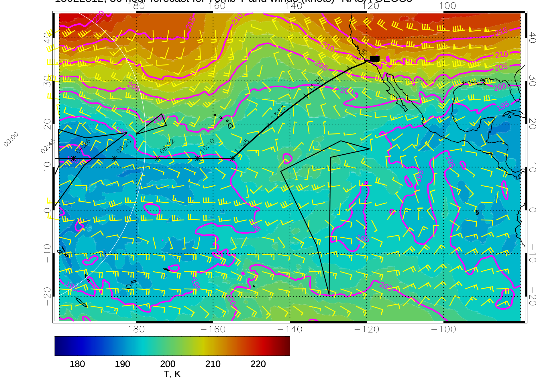
15022812, 36 hour forecast for 73mb T and winds (knots)- NASA GEOS5
