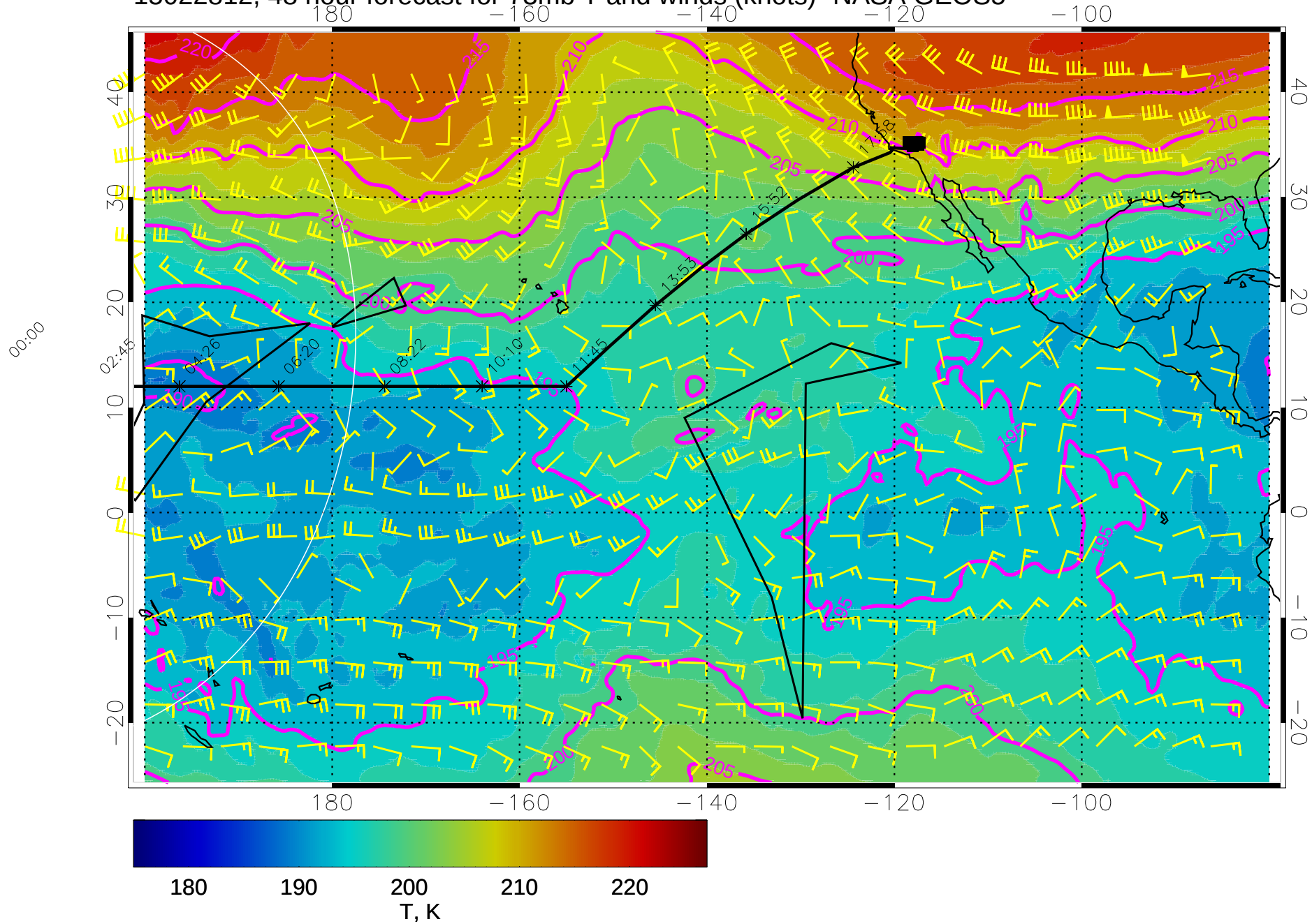
15022812, 48 hour forecast for 73mb T and winds (knots)- NASA GEOS5
