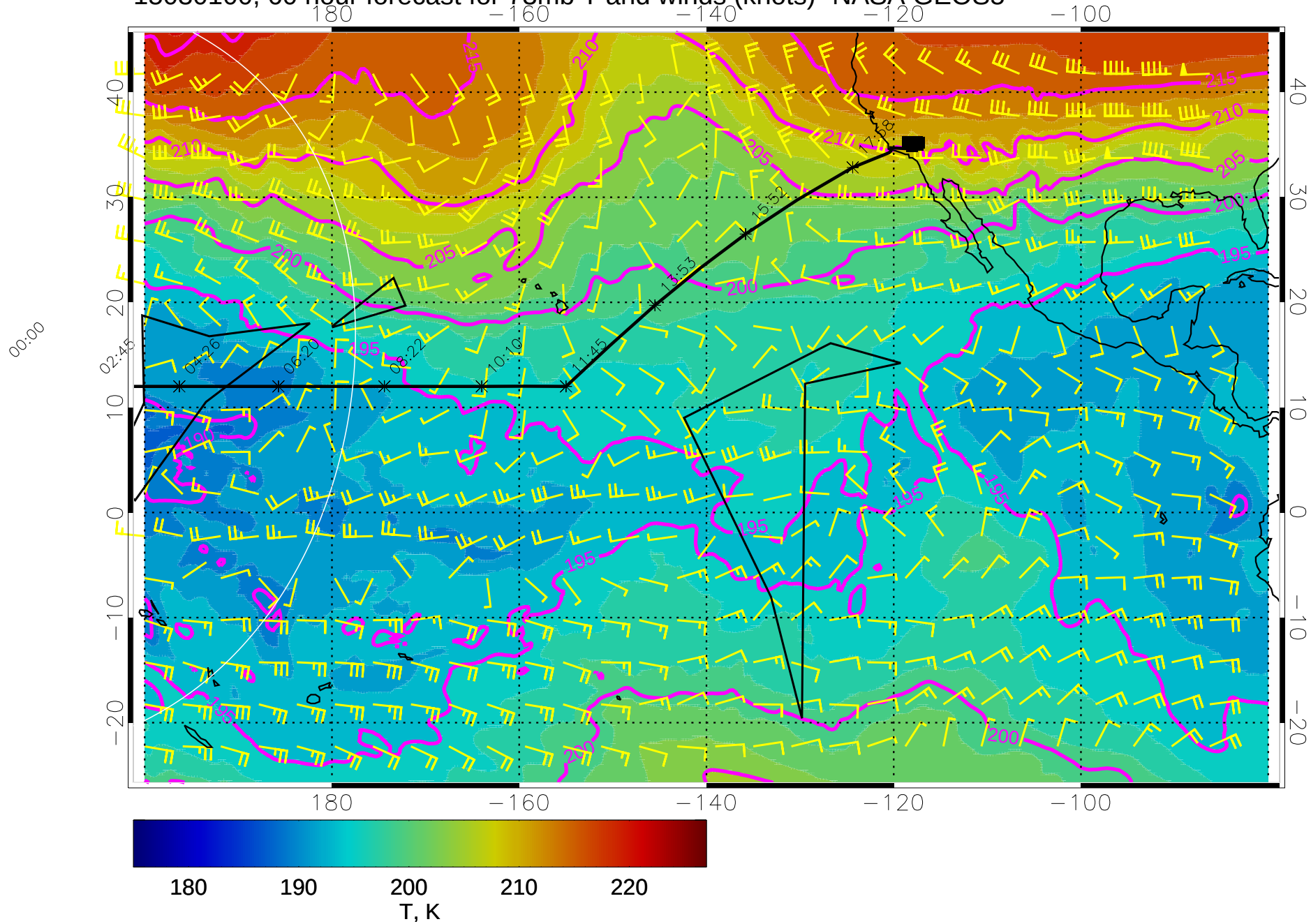
15030100, 60 hour forecast for 73mb T and winds (knots)- NASA GEOS5
