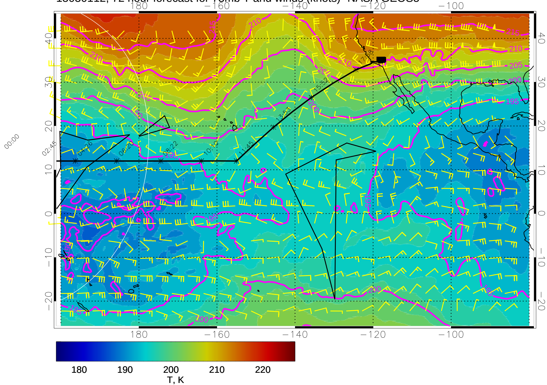
15030112, 72 hour forecast for 73mb T and winds (knots)- NASA GEOS5
