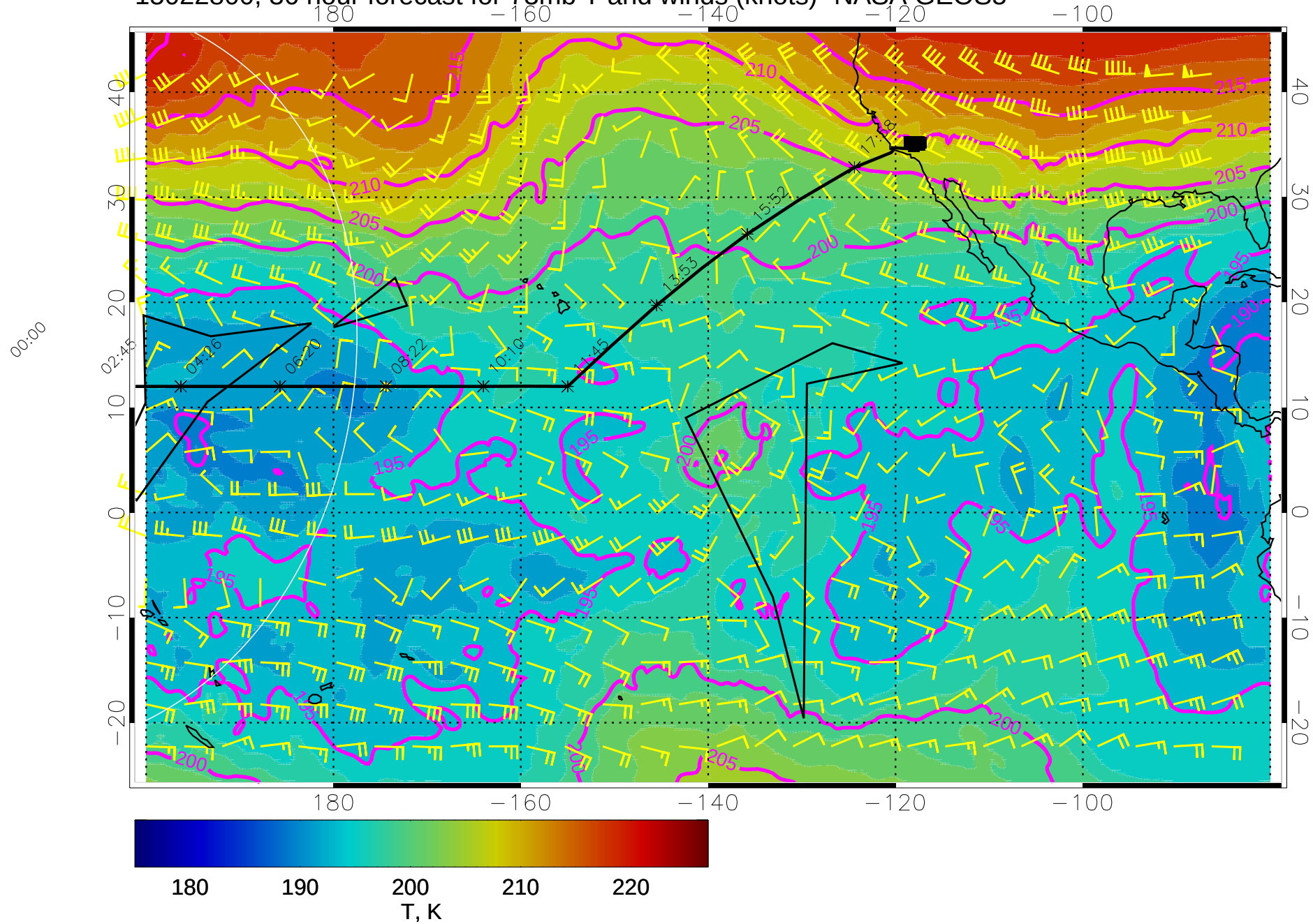
15022800, 36 hour forecast for 73mb T and winds (knots)- NASA GEOS5
