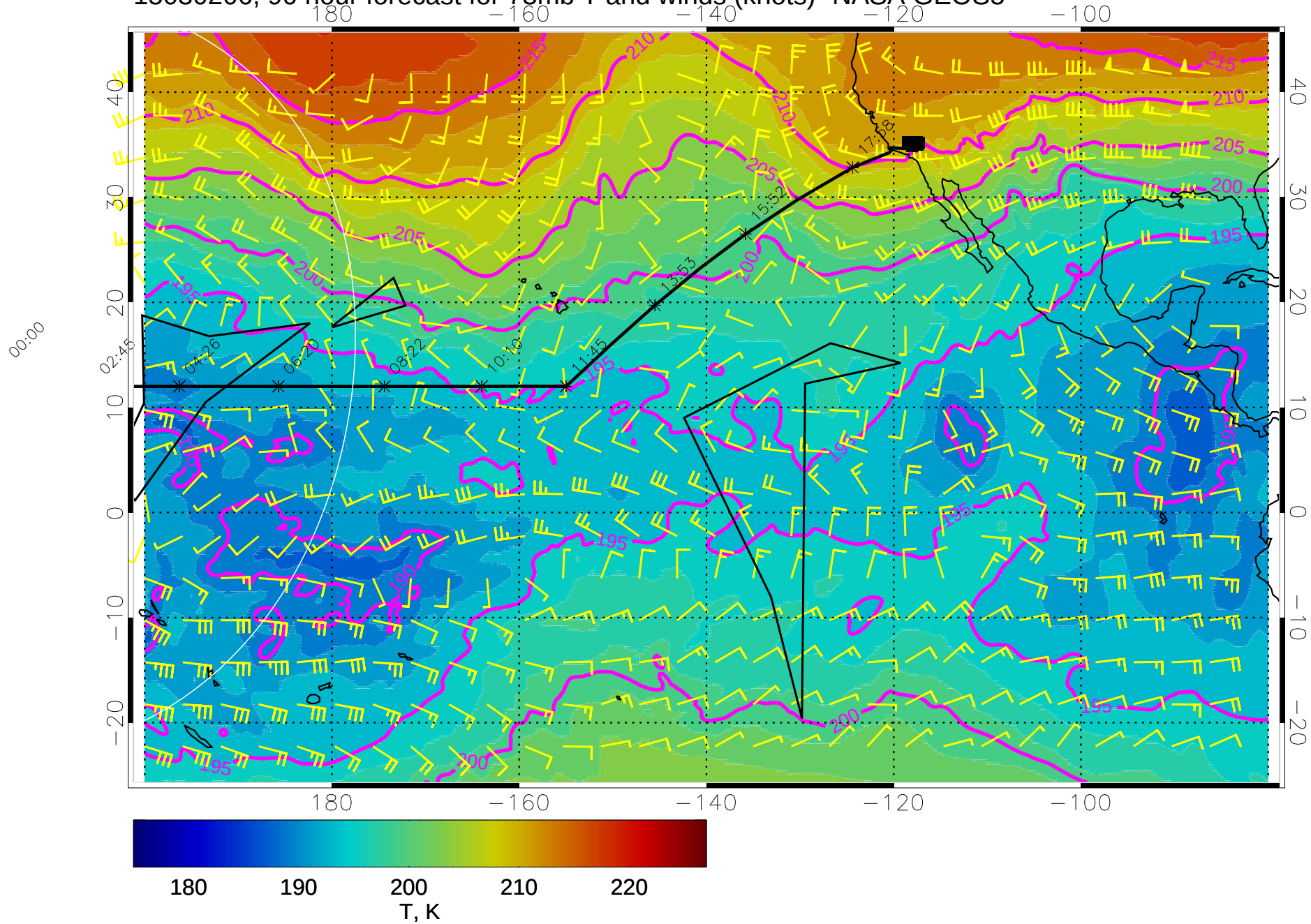
15030206, 90 hour forecast for 73mb T and winds (knots)- NASA GEOS5
