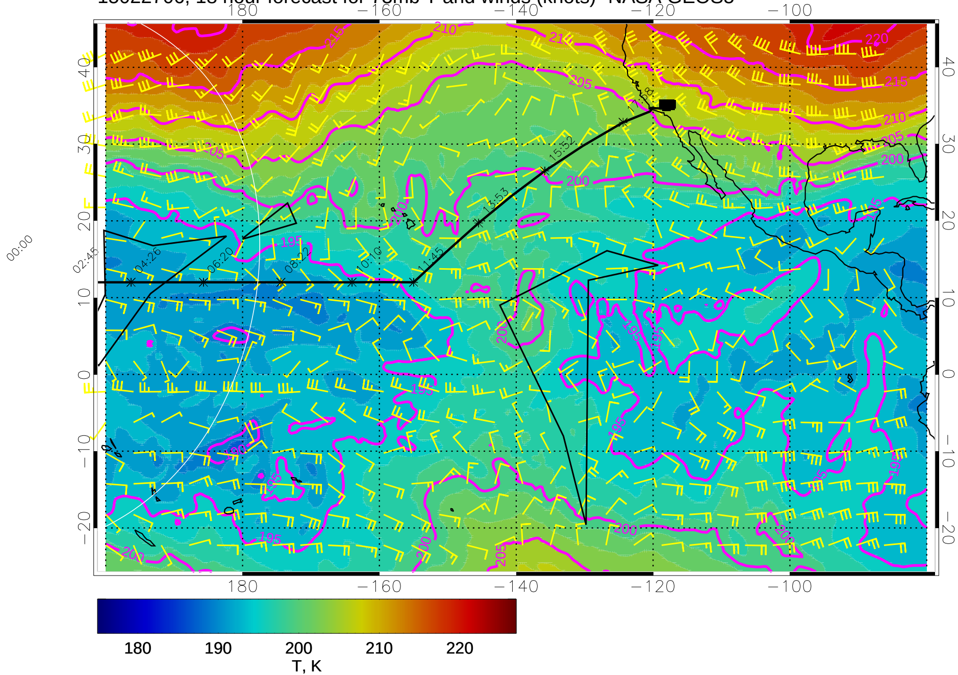
15022706, 18 hour forecast for 73mb T and winds (knots)- NASA GEOS5
