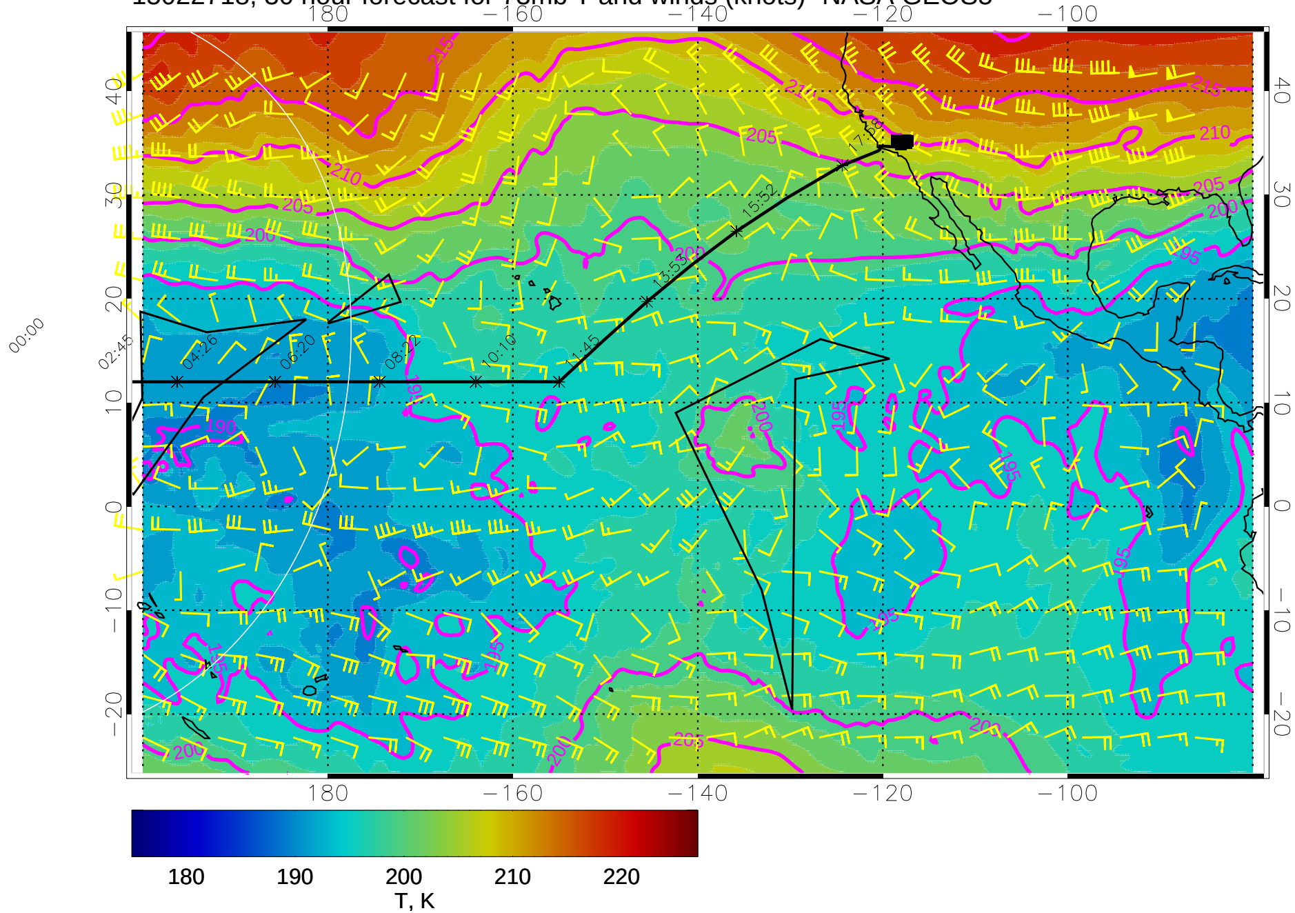
15022718, 30 hour forecast for 73mb T and winds (knots)- NASA GEOS5
