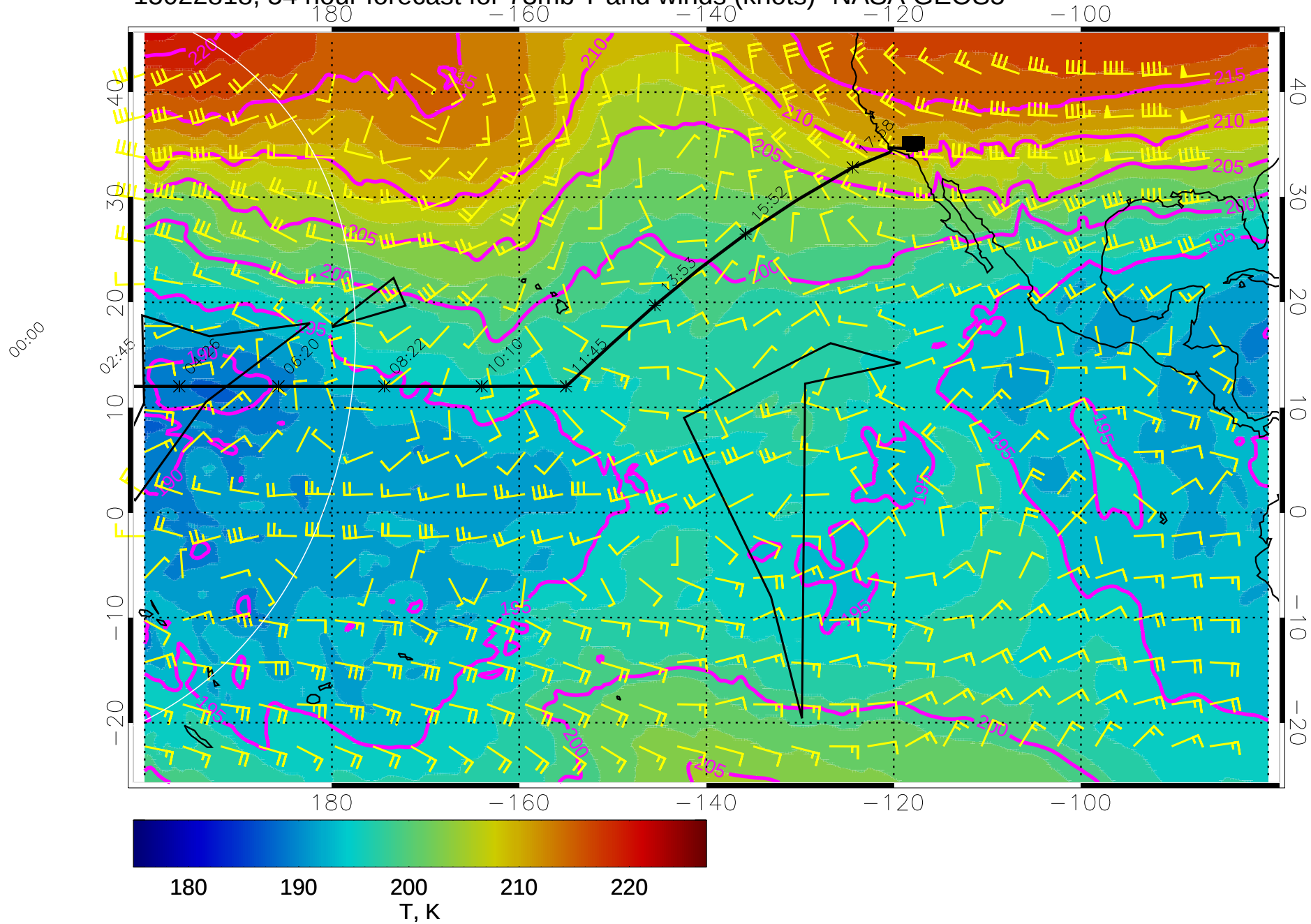
15022818, 54 hour forecast for 73mb T and winds (knots)- NASA GEOS5
