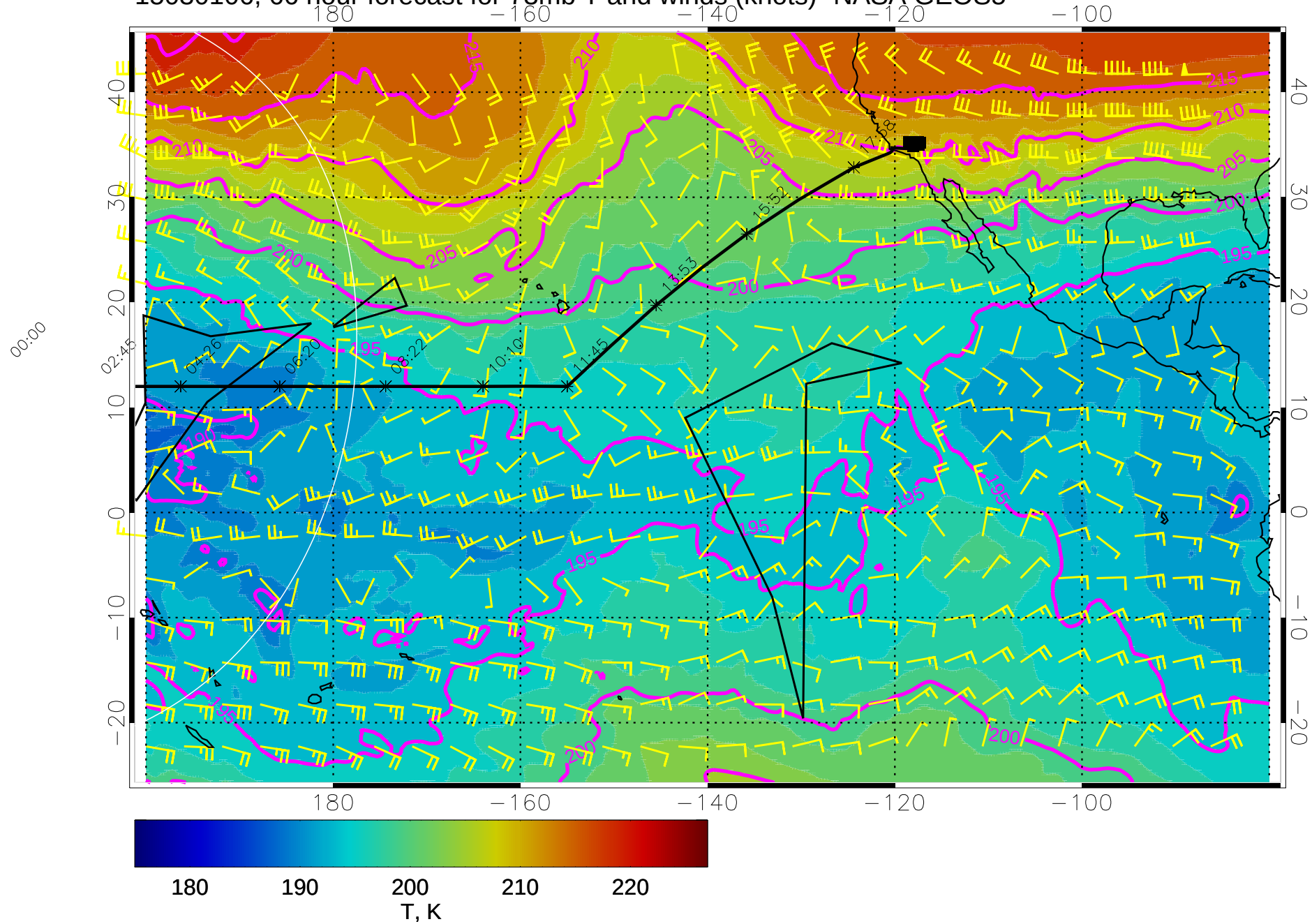
15030106, 66 hour forecast for 73mb T and winds (knots)- NASA GEOS5
