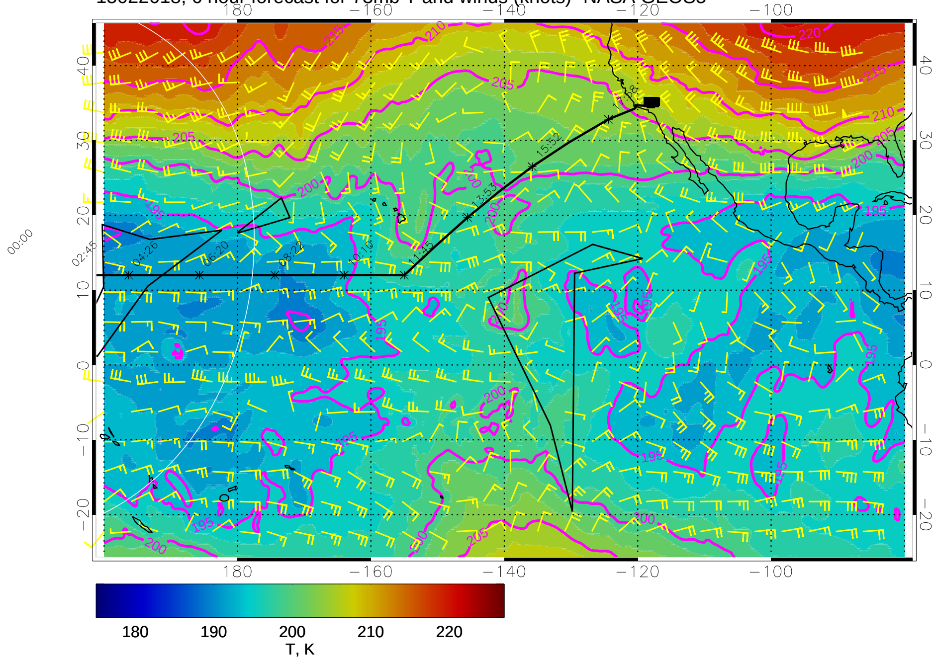
15022618, 6 hour forecast for 73mb T and winds (knots)- NASA GEOS5
