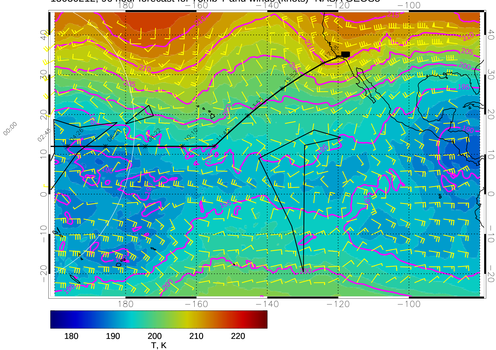
15030212, 96 hour forecast for 73mb T and winds (knots)- NASA GEOS5
