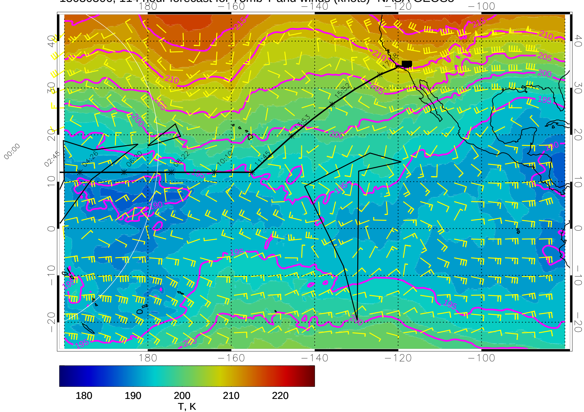
15030306, 114 hour forecast for 73mb T and winds (knots)- NASA GEOS5
