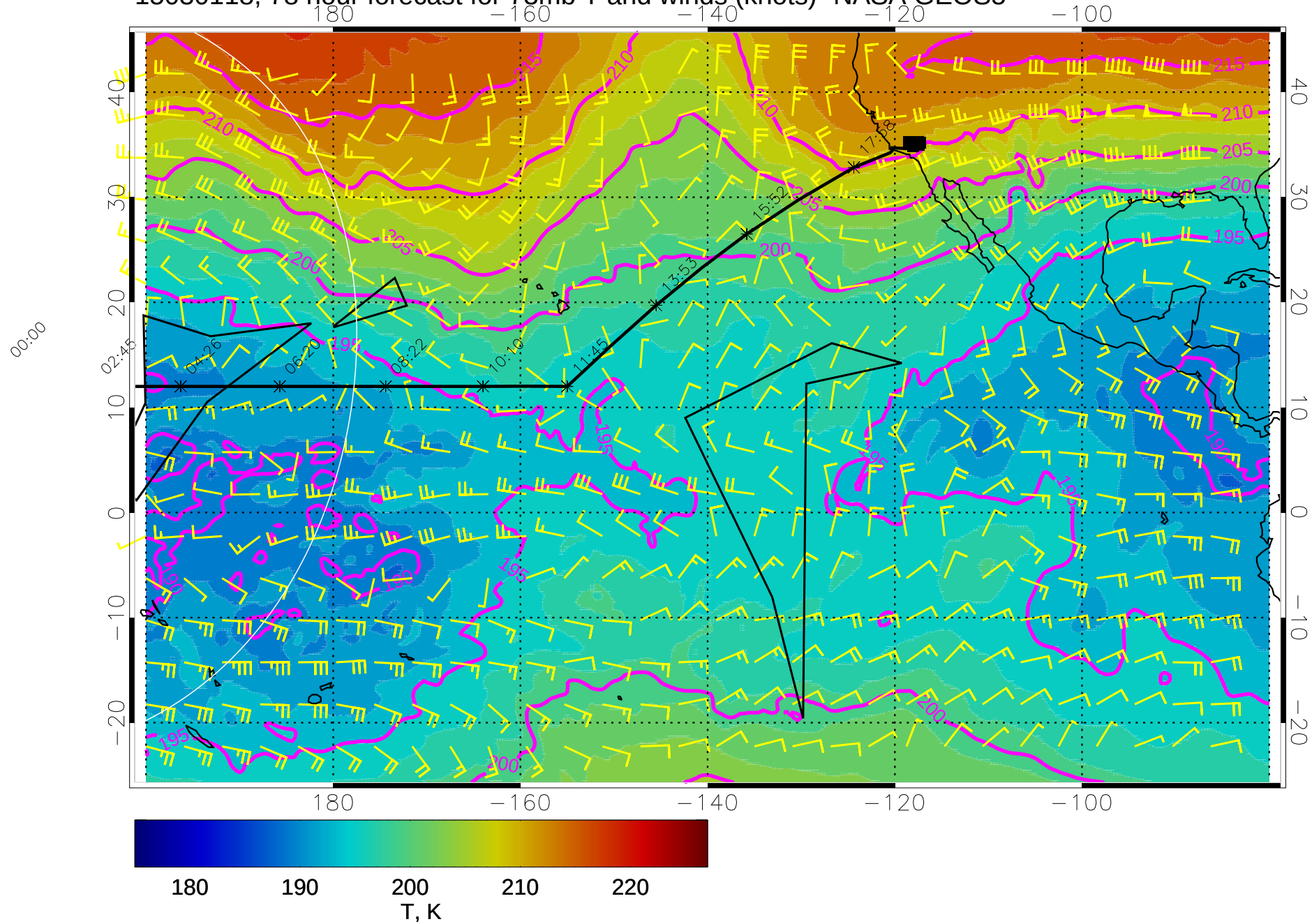
15030118, 78 hour forecast for 73mb T and winds (knots)- NASA GEOS5
