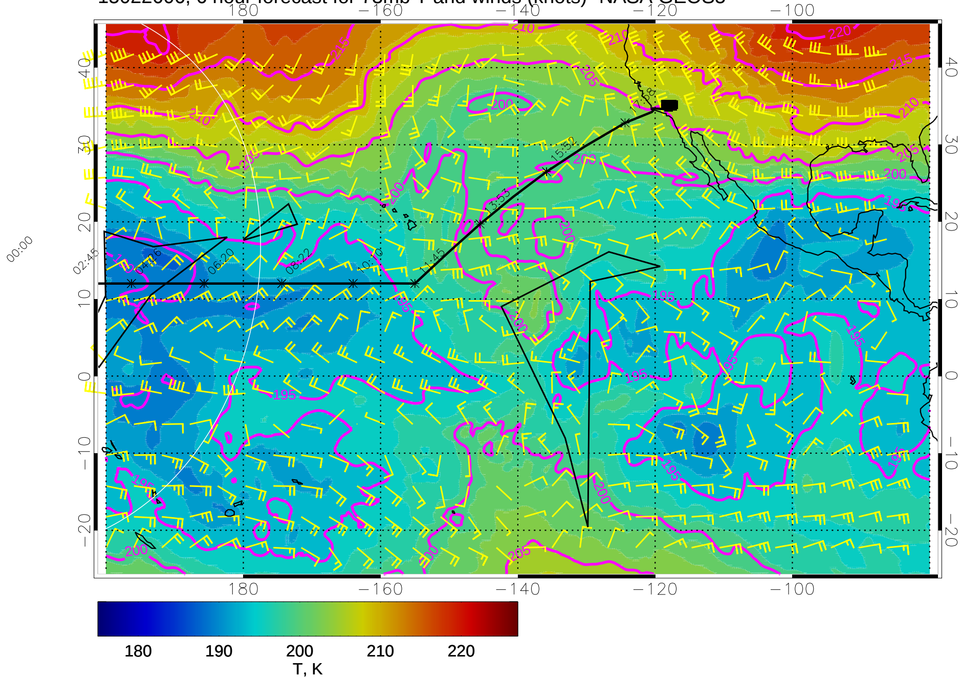
15022606, 6 hour forecast for 73mb T and winds (knots)- NASA GEOS5
