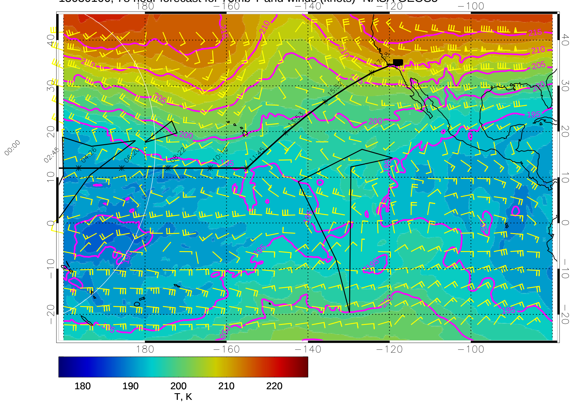
15030106, 78 hour forecast for 73mb T and winds (knots)- NASA GEOS5
