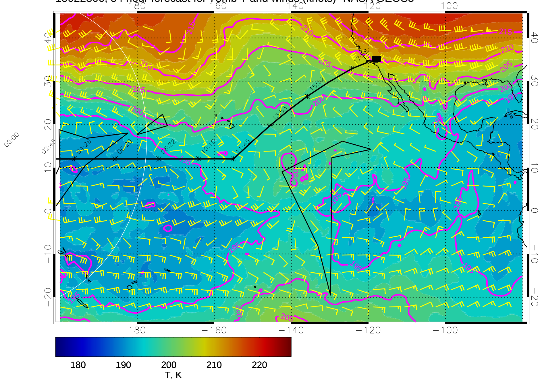
15022806, 54 hour forecast for 73mb T and winds (knots)- NASA GEOS5
