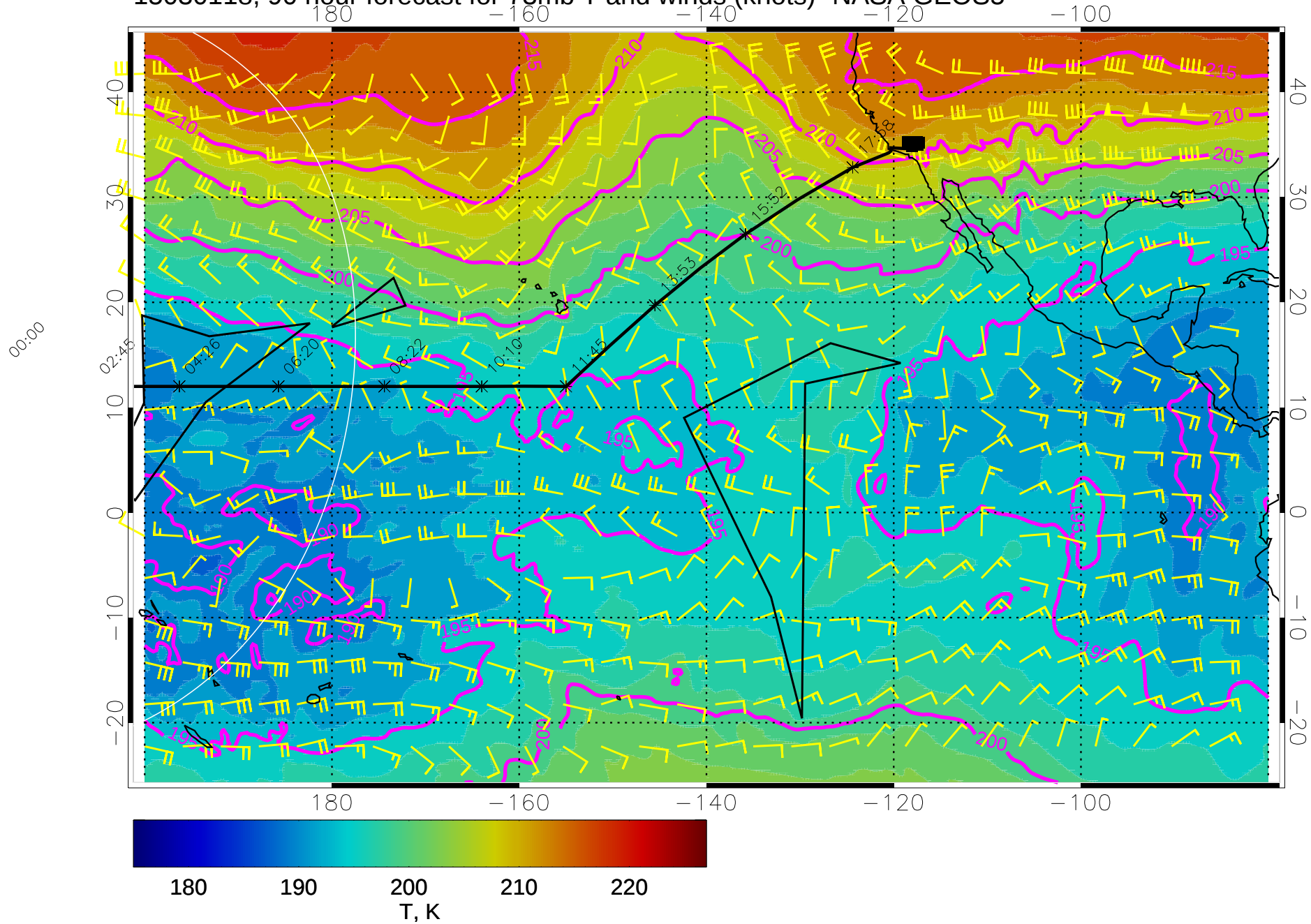
15030118, 90 hour forecast for 73mb T and winds (knots)- NASA GEOS5
