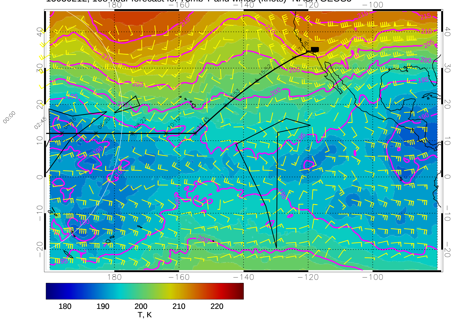
15030212, 108 hour forecast for 73mb T and winds (knots)- NASA GEOS5
