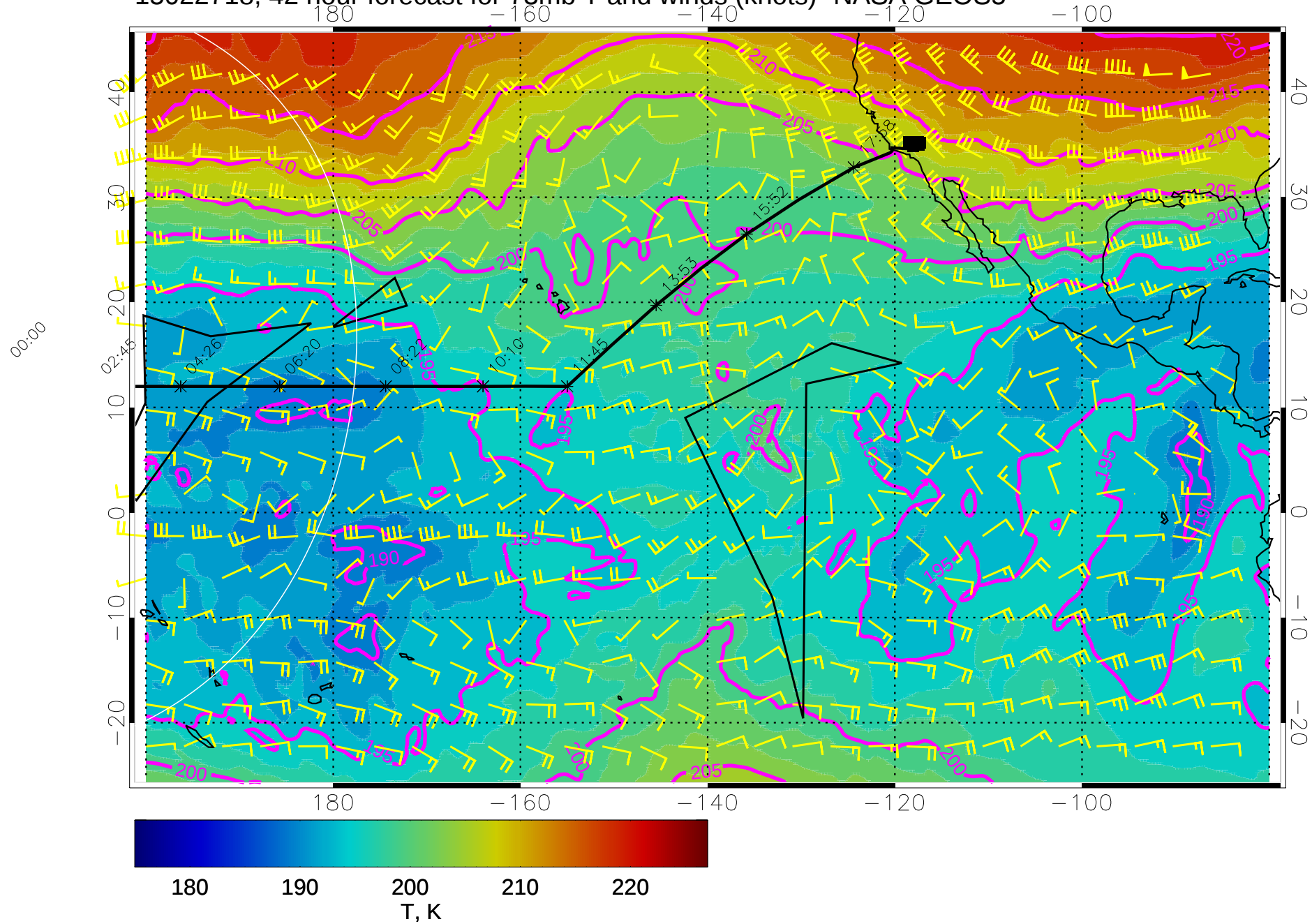
15022718, 42 hour forecast for 73mb T and winds (knots)- NASA GEOS5
