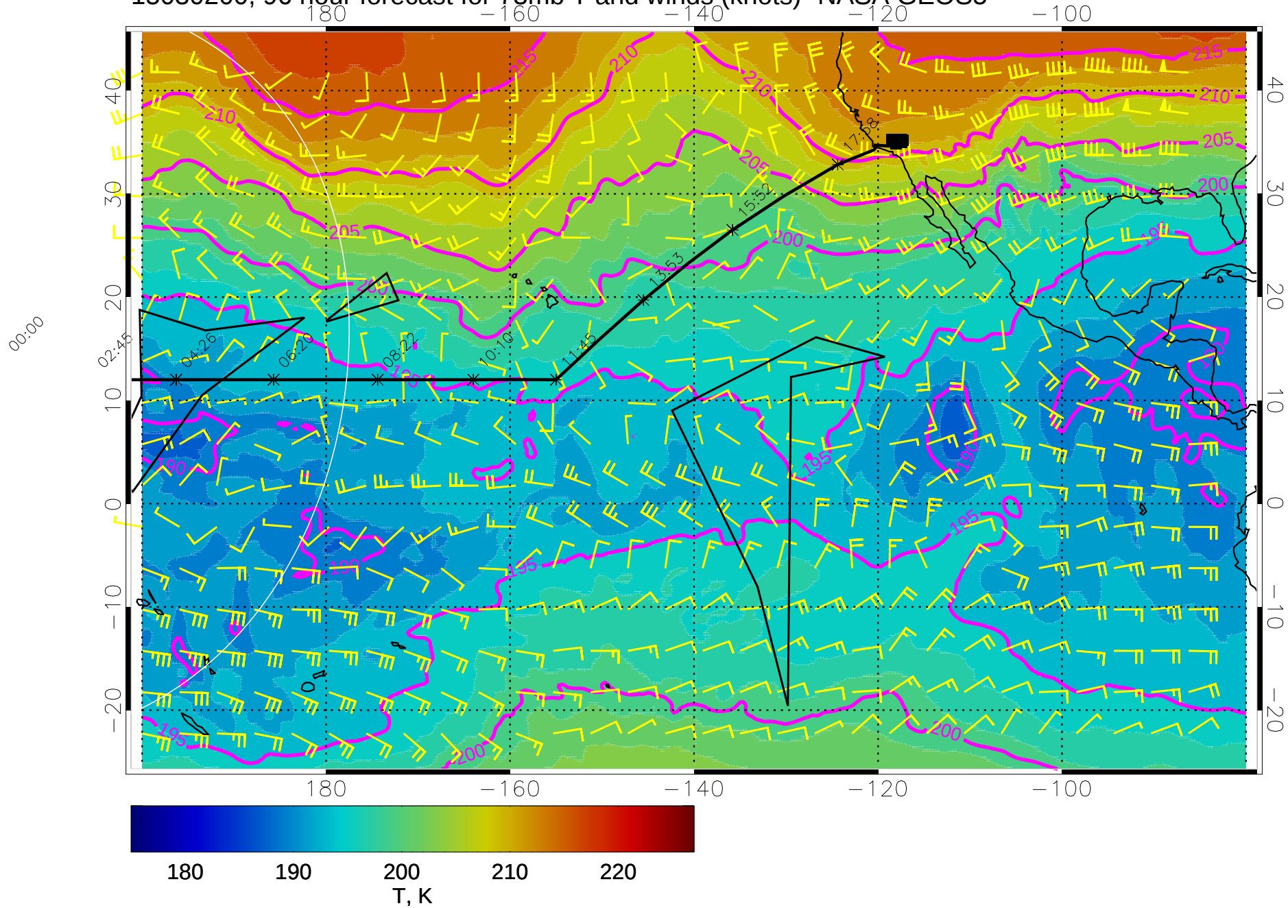
15030200, 96 hour forecast for 73mb T and winds (knots)- NASA GEOS5
