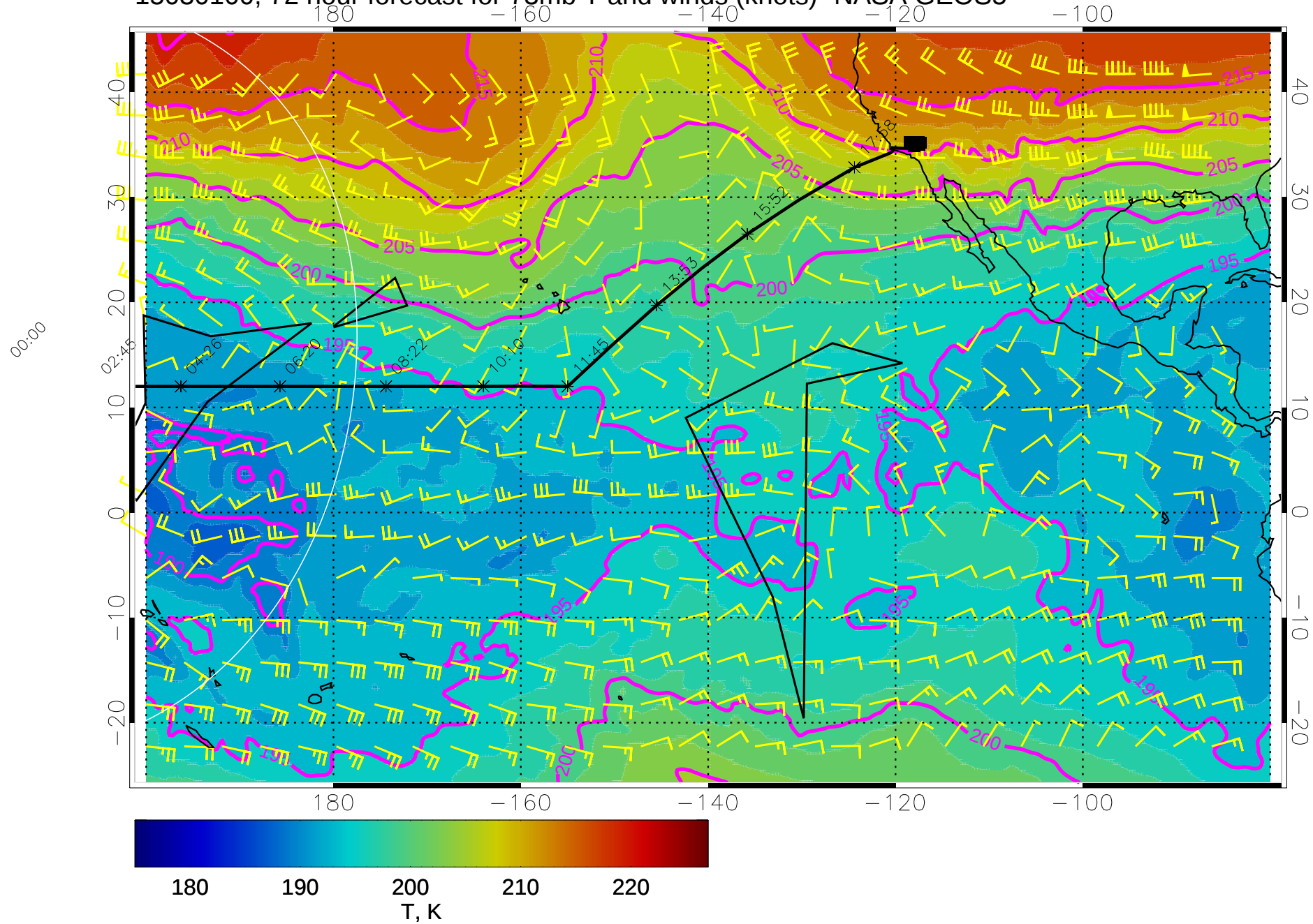
15030100, 72 hour forecast for 73mb T and winds (knots)- NASA GEOS5
