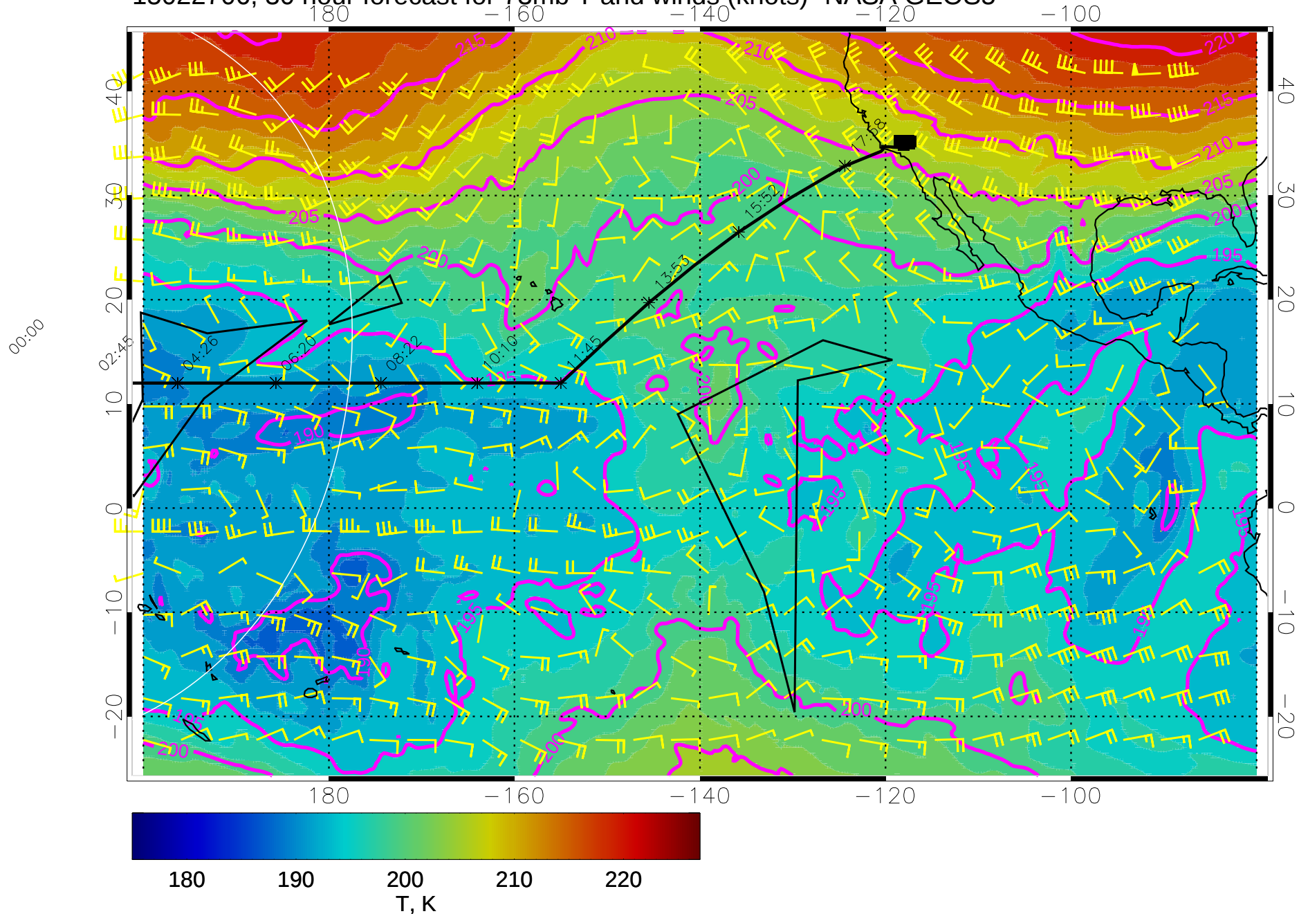
15022706, 30 hour forecast for 73mb T and winds (knots)- NASA GEOS5
