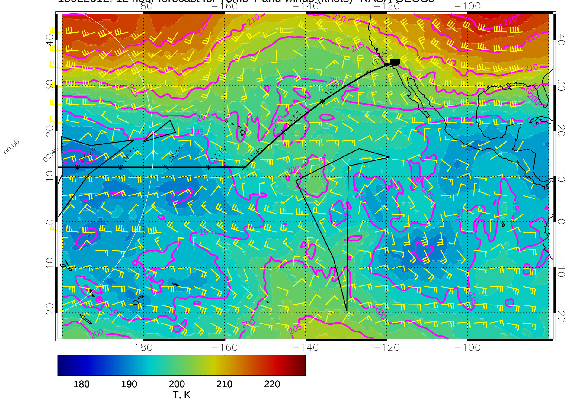
15022612, 12 hour forecast for 73mb T and winds (knots)- NASA GEOS5
