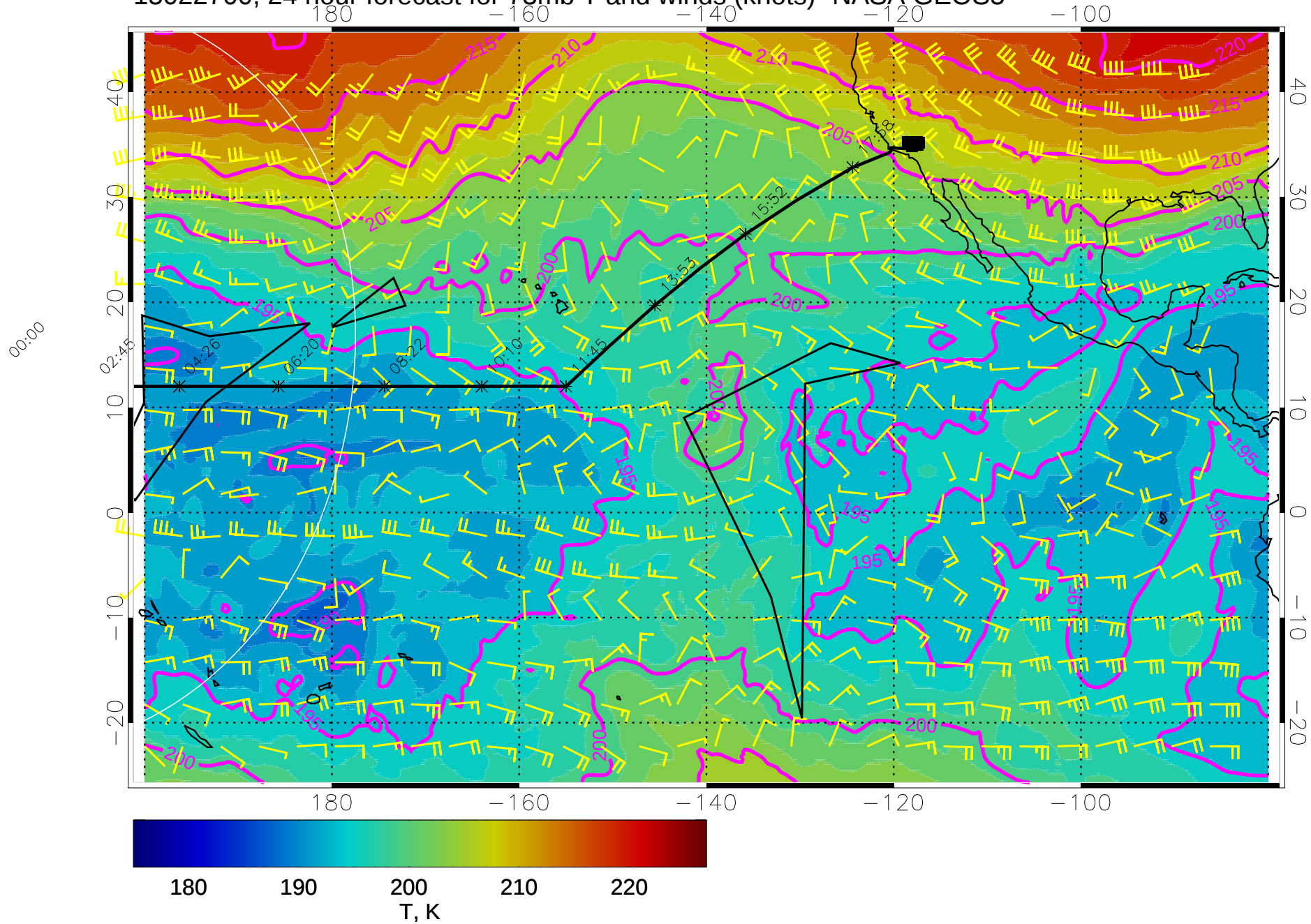
15022700, 24 hour forecast for 73mb T and winds (knots)- NASA GEOS5
