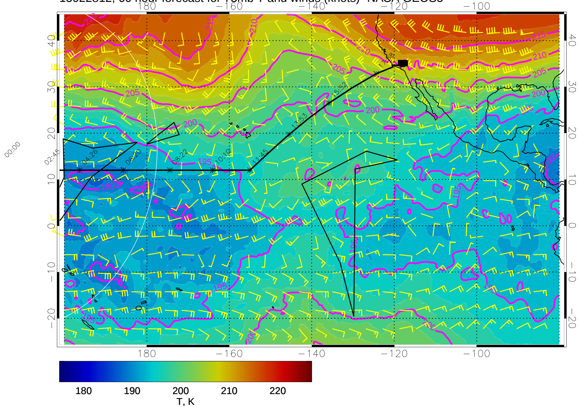
15022812, 60 hour forecast for 73mb T and winds (knots)- NASA GEOS5
