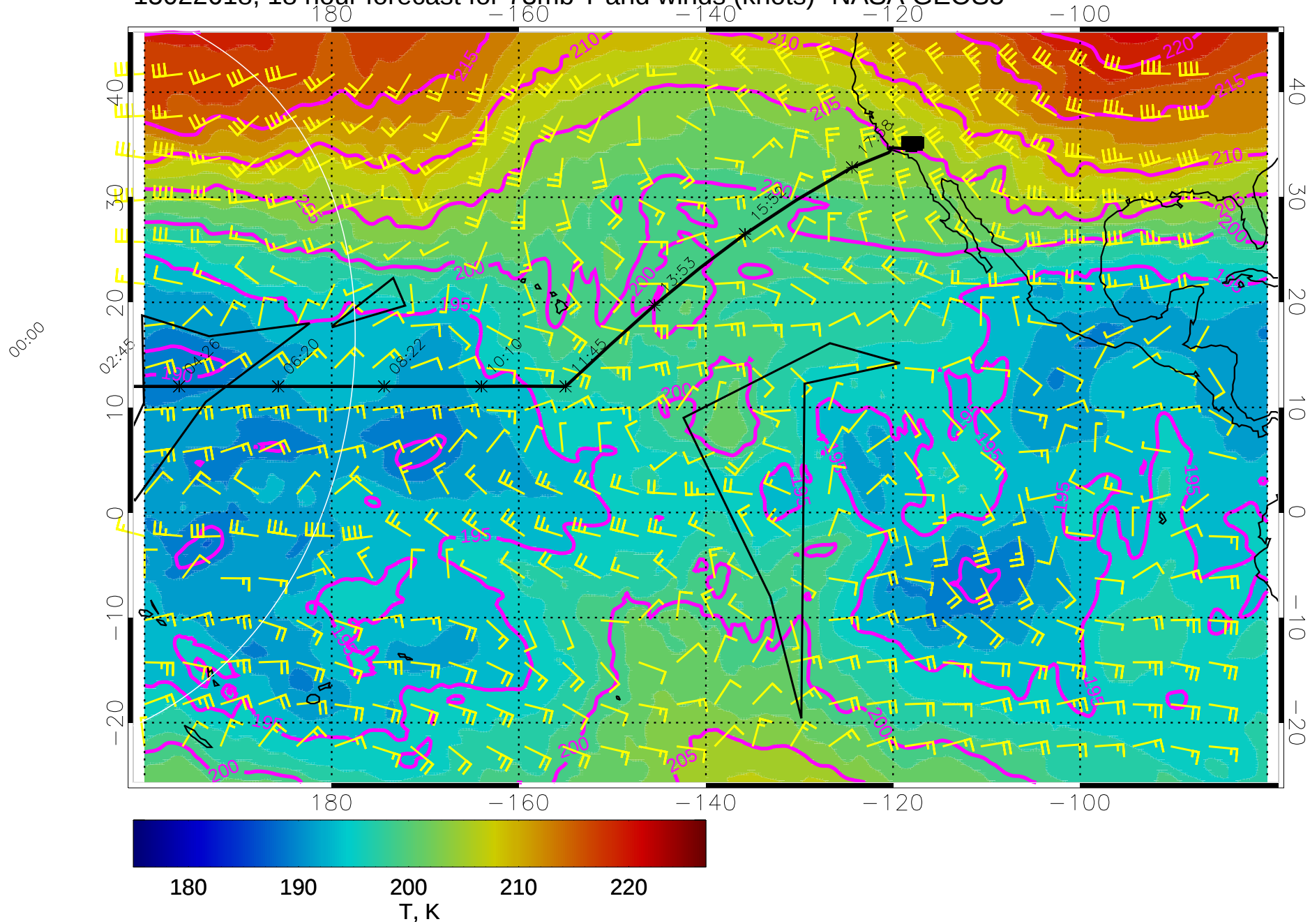
15022618, 18 hour forecast for 73mb T and winds (knots)- NASA GEOS5
