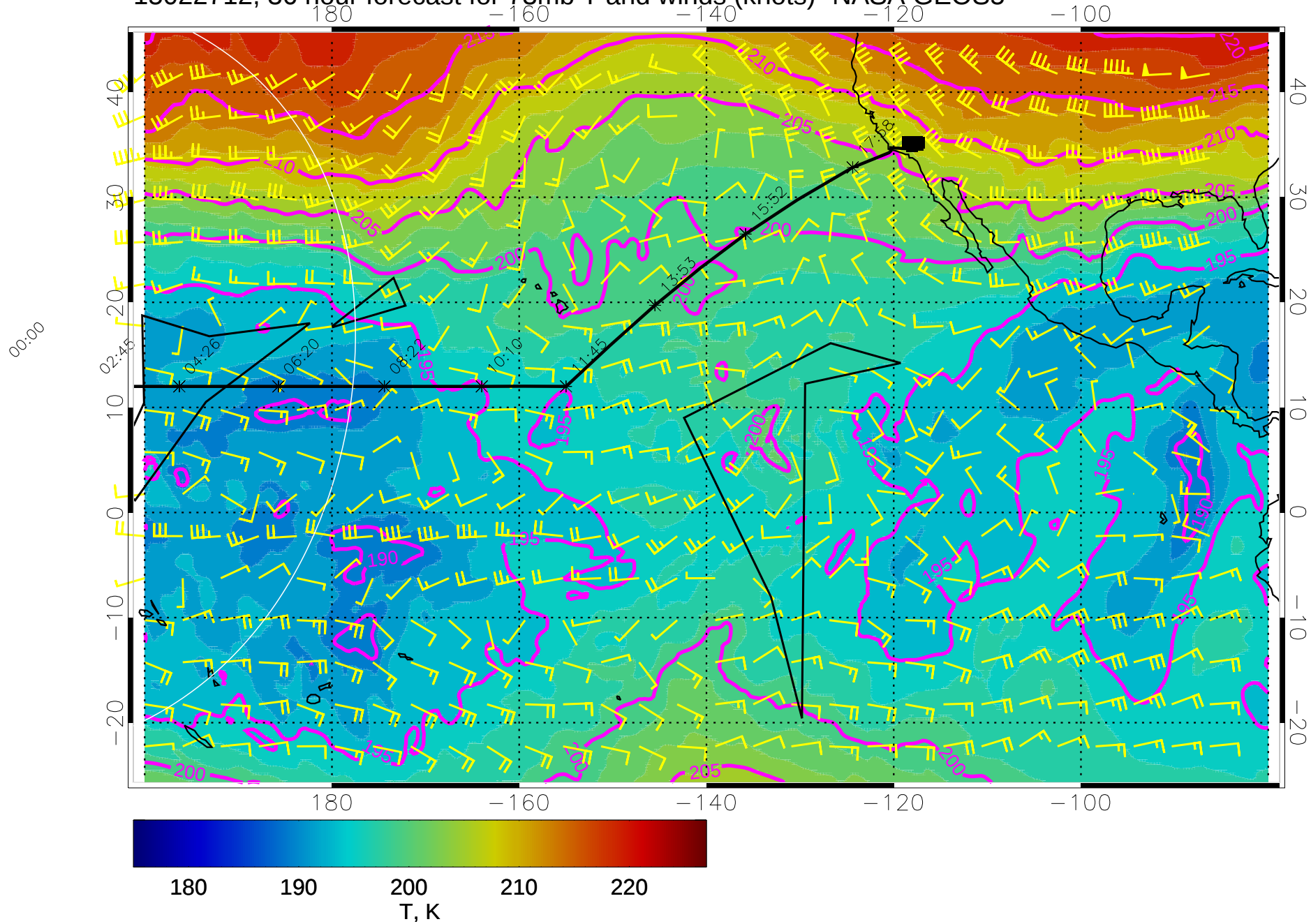
15022712, 36 hour forecast for 73mb T and winds (knots)- NASA GEOS5
