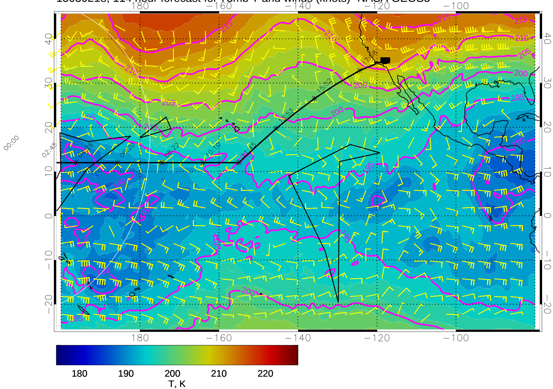
15030218, 114 hour forecast for 73mb T and winds (knots)- NASA GEOS5
