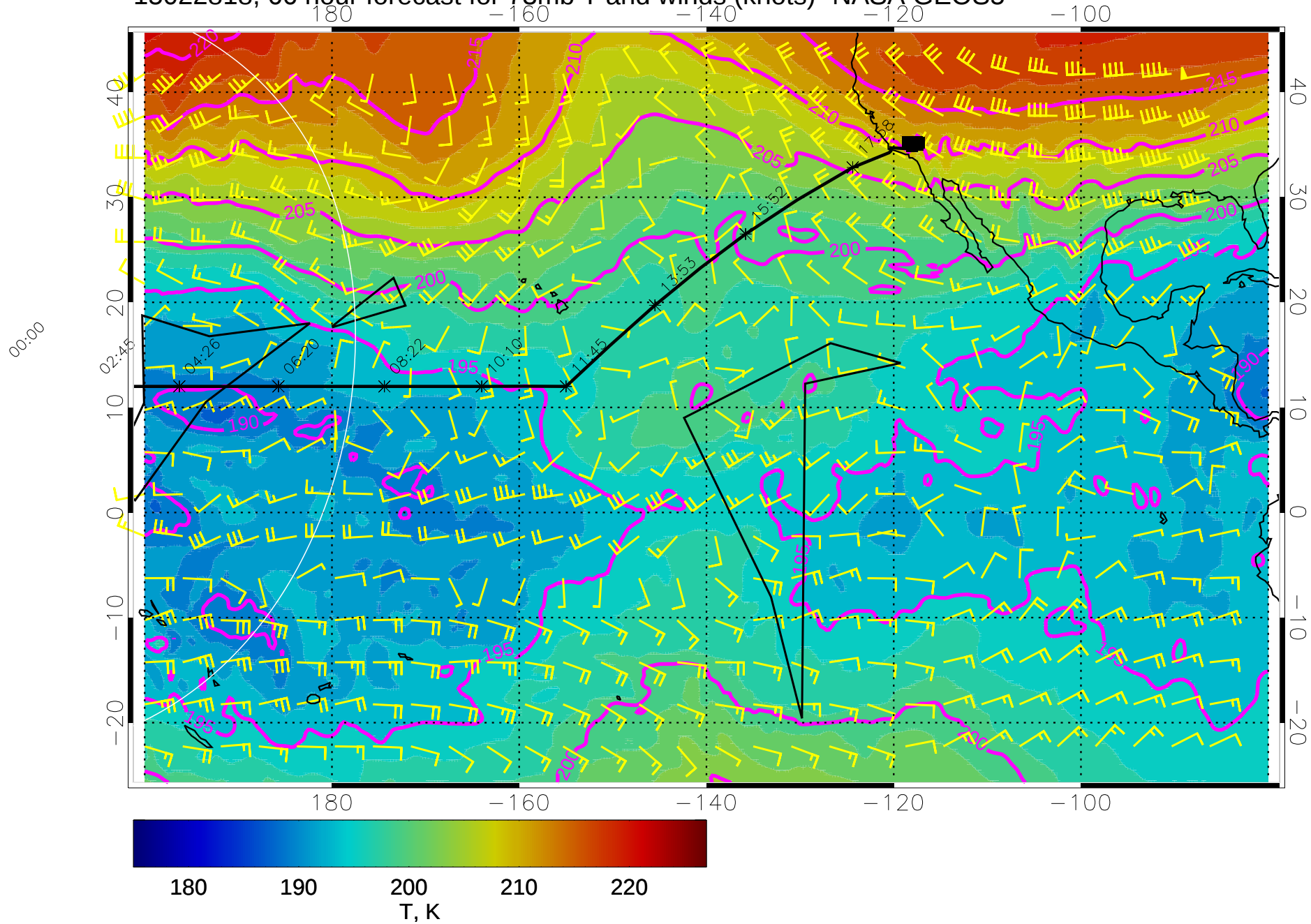
15022818, 66 hour forecast for 73mb T and winds (knots)- NASA GEOS5
