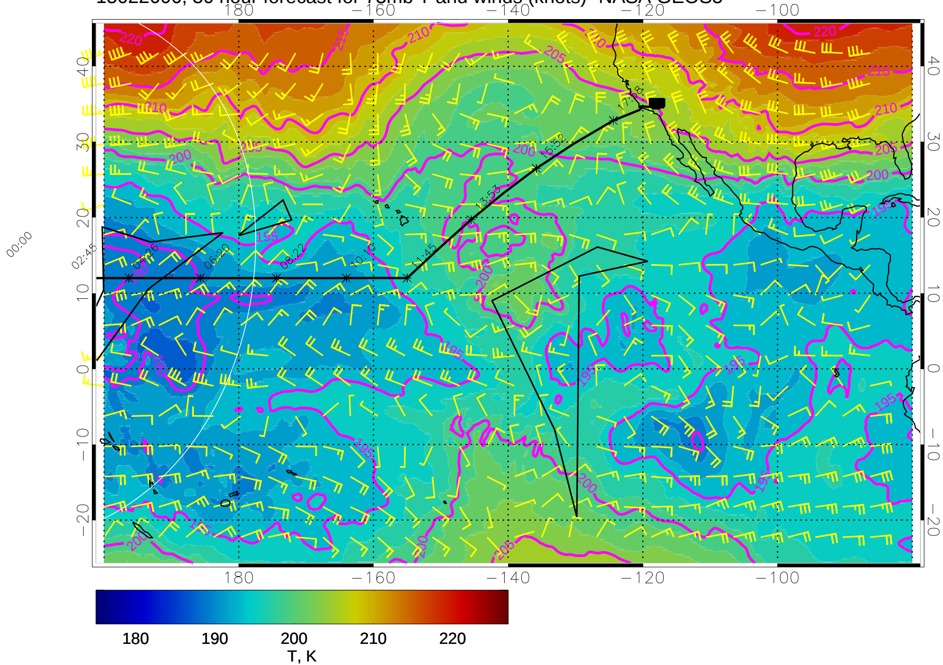
15022606, 30 hour forecast for 73mb T and winds (knots)- NASA GEOS5
