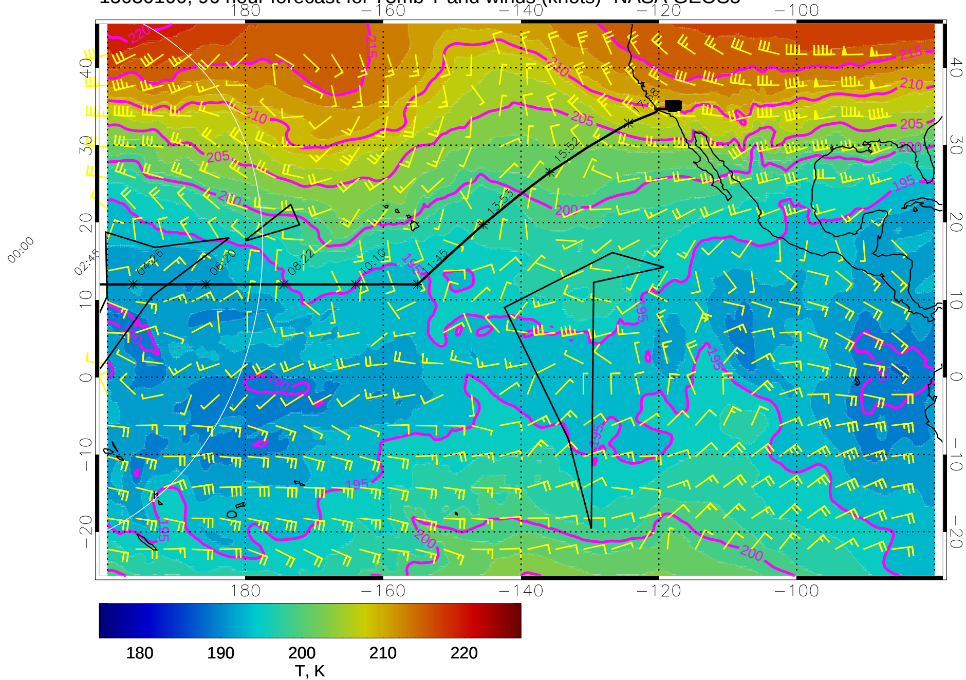
15030100, 96 hour forecast for 73mb T and winds (knots)- NASA GEOS5
