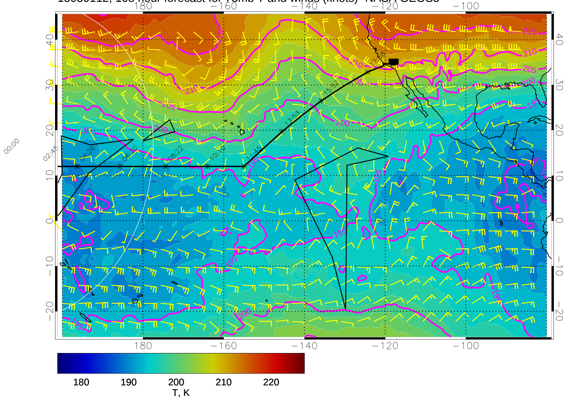
15030112, 108 hour forecast for 73mb T and winds (knots)- NASA GEOS5
