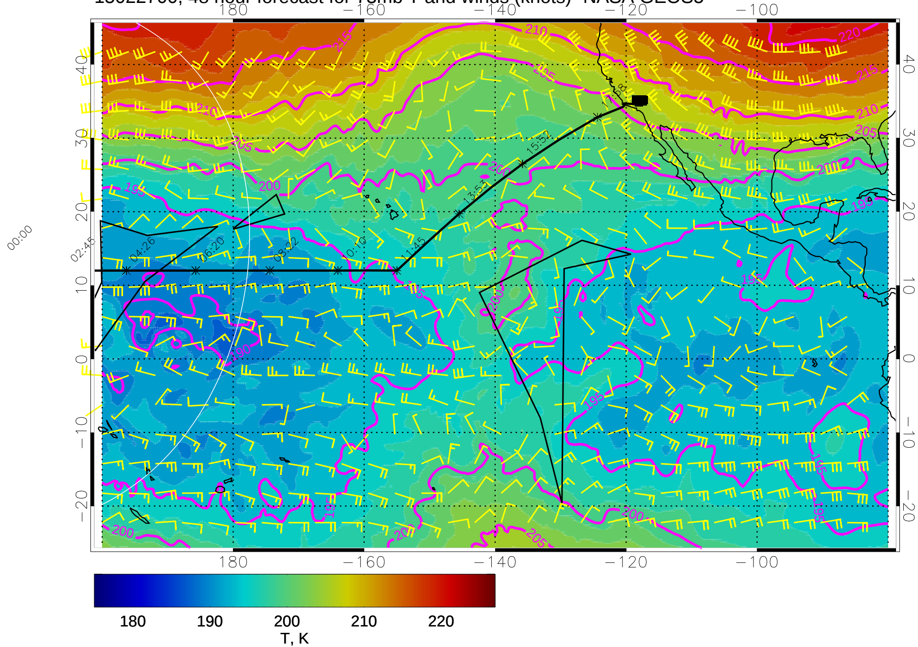
15022700, 48 hour forecast for 73mb T and winds (knots)- NASA GEOS5
