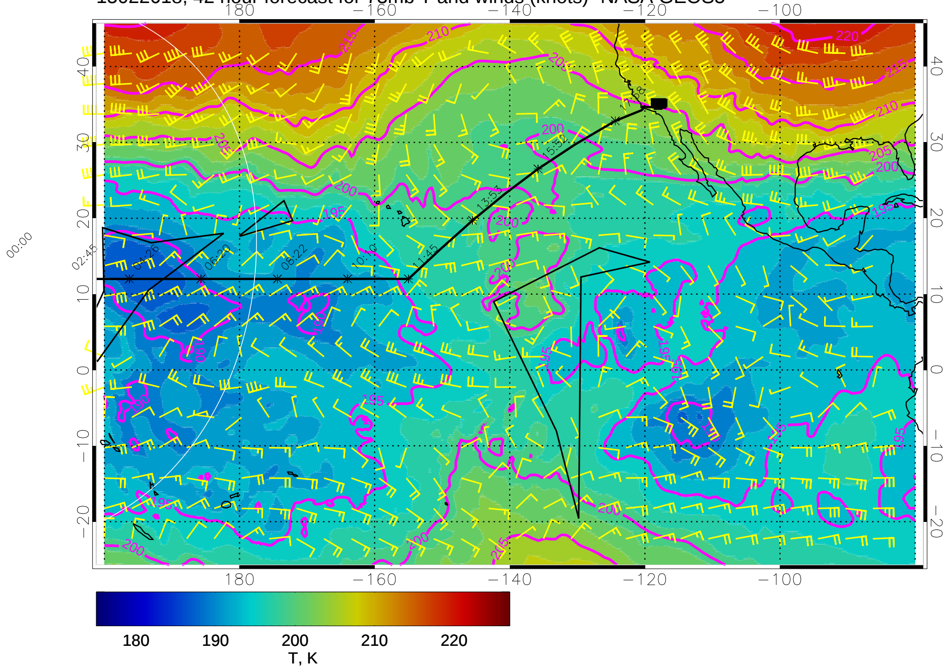
15022618, 42 hour forecast for 73mb T and winds (knots)- NASA GEOS5
