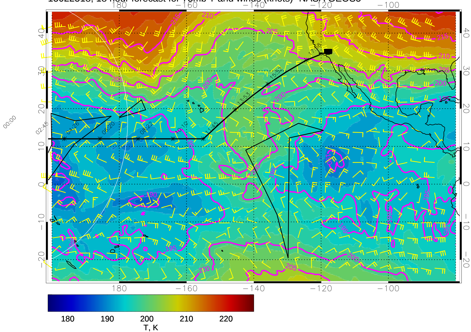
15022518, 18 hour forecast for 73mb T and winds (knots)- NASA GEOS5
