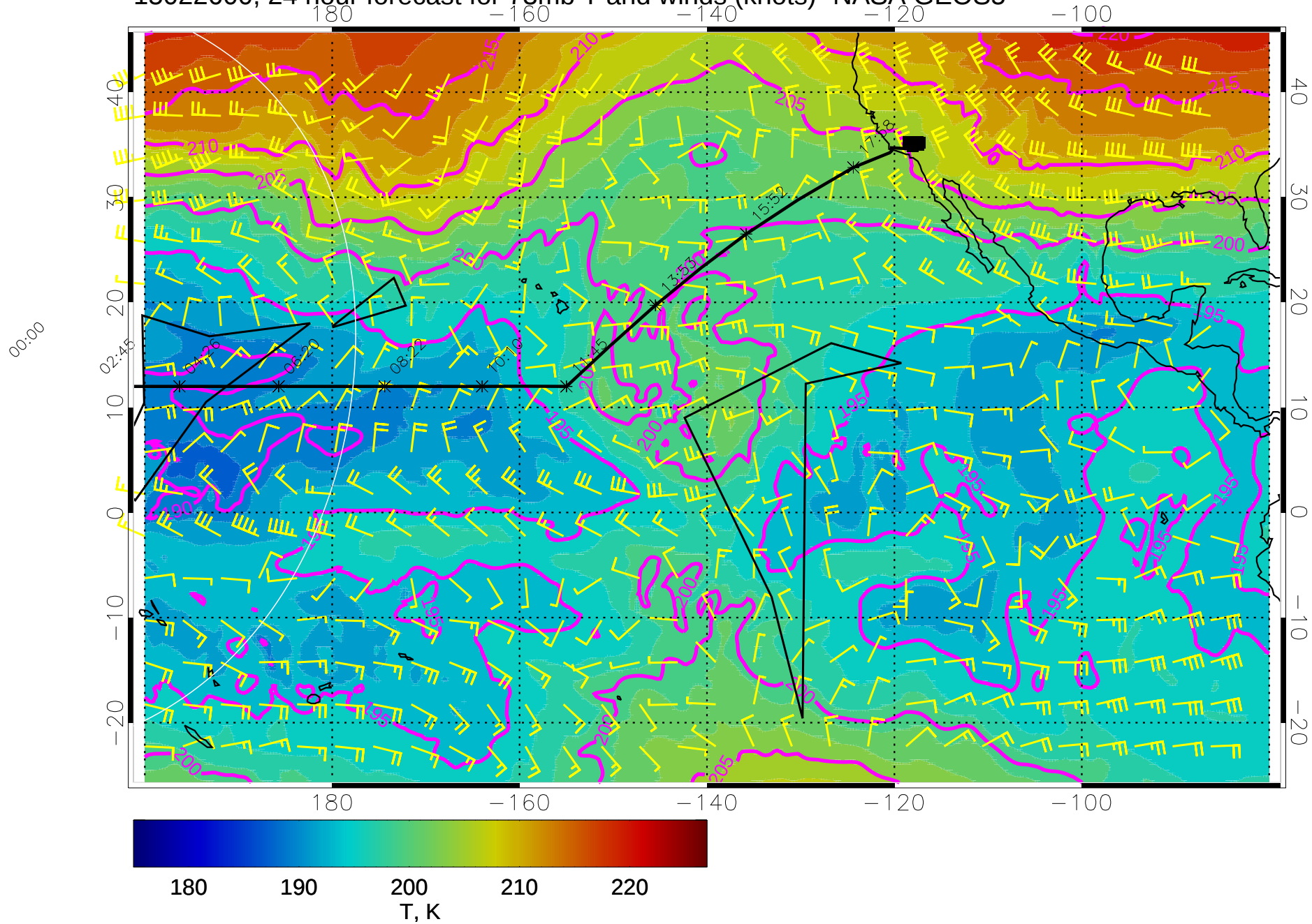
15022600, 24 hour forecast for 73mb T and winds (knots)- NASA GEOS5
