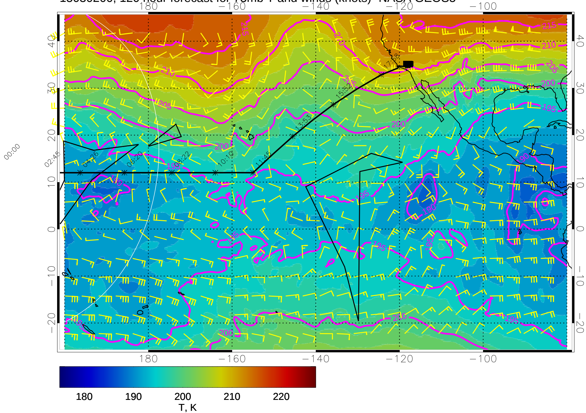
15030200, 120 hour forecast for 73mb T and winds (knots)- NASA GEOS5
