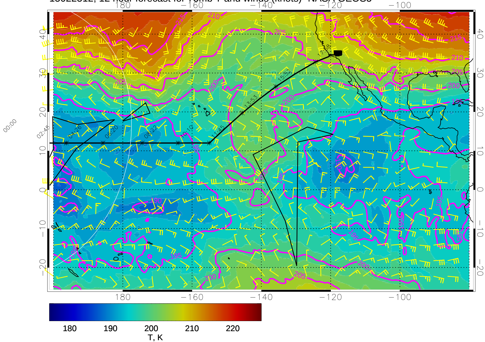
15022512, 12 hour forecast for 73mb T and winds (knots)- NASA GEOS5
