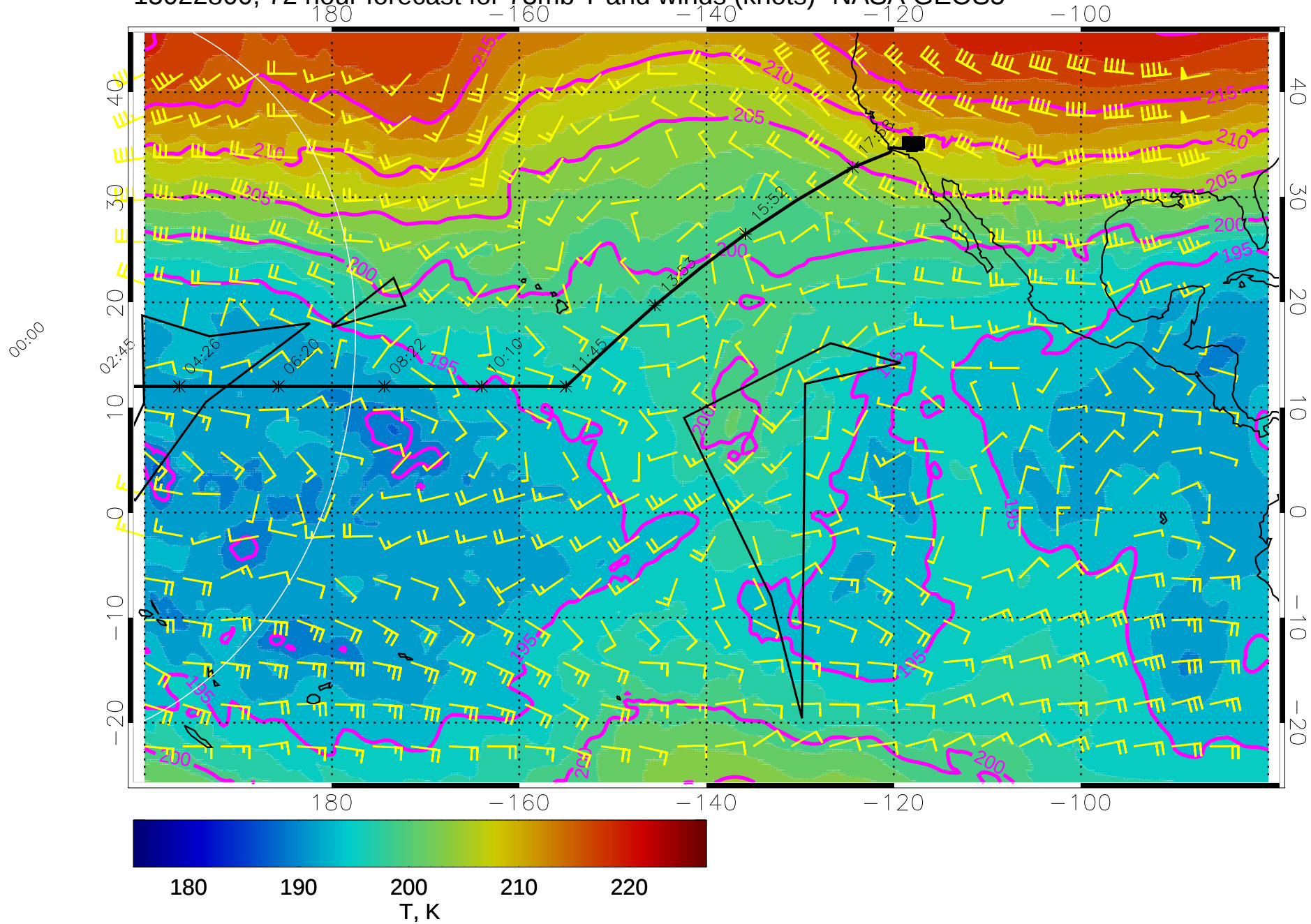
15022800, 72 hour forecast for 73mb T and winds (knots)- NASA GEOS5
