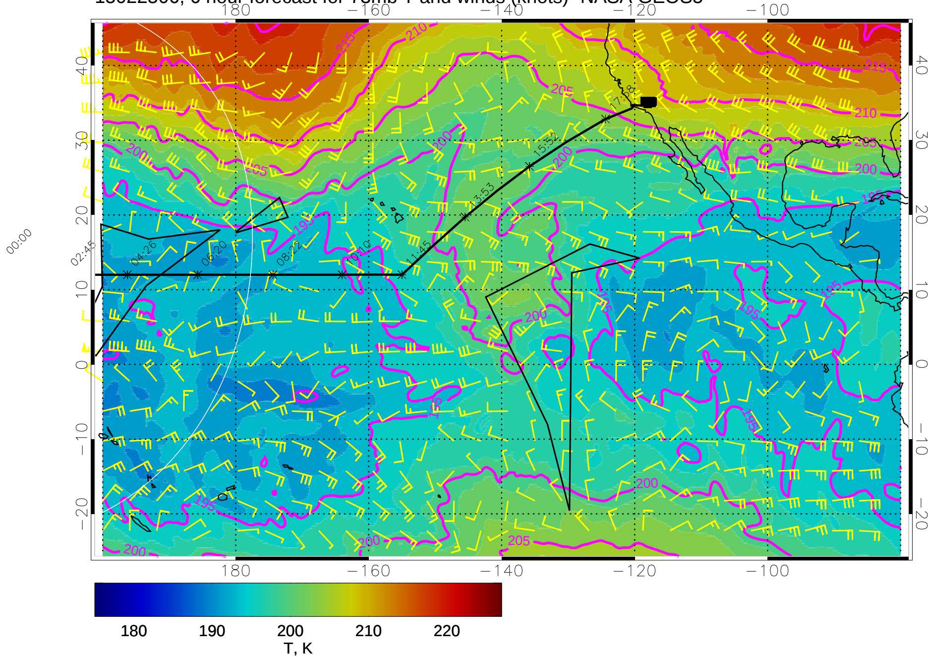
15022506, 6 hour forecast for 73mb T and winds (knots)- NASA GEOS5
