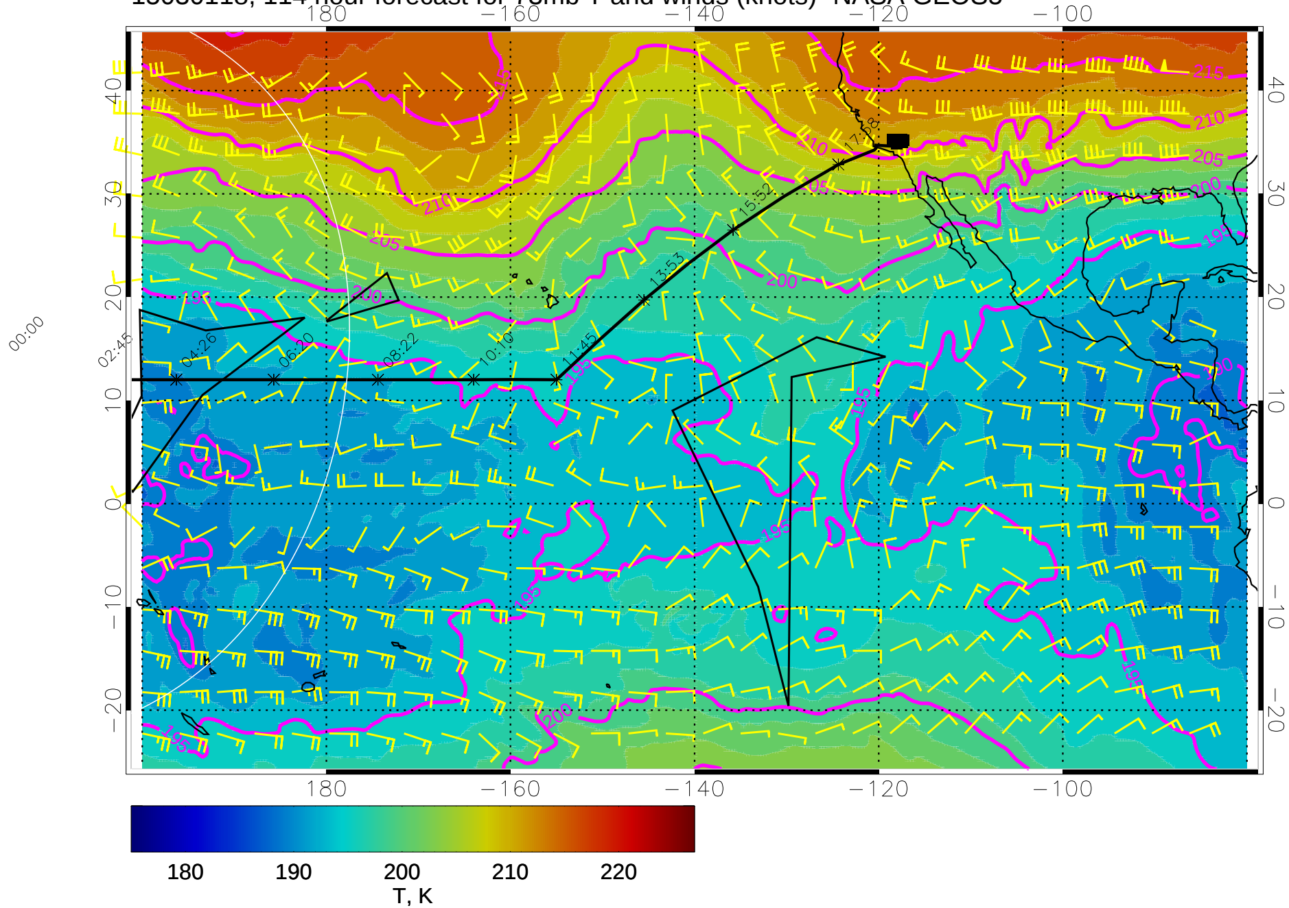
15030118, 114 hour forecast for 73mb T and winds (knots)- NASA GEOS5
