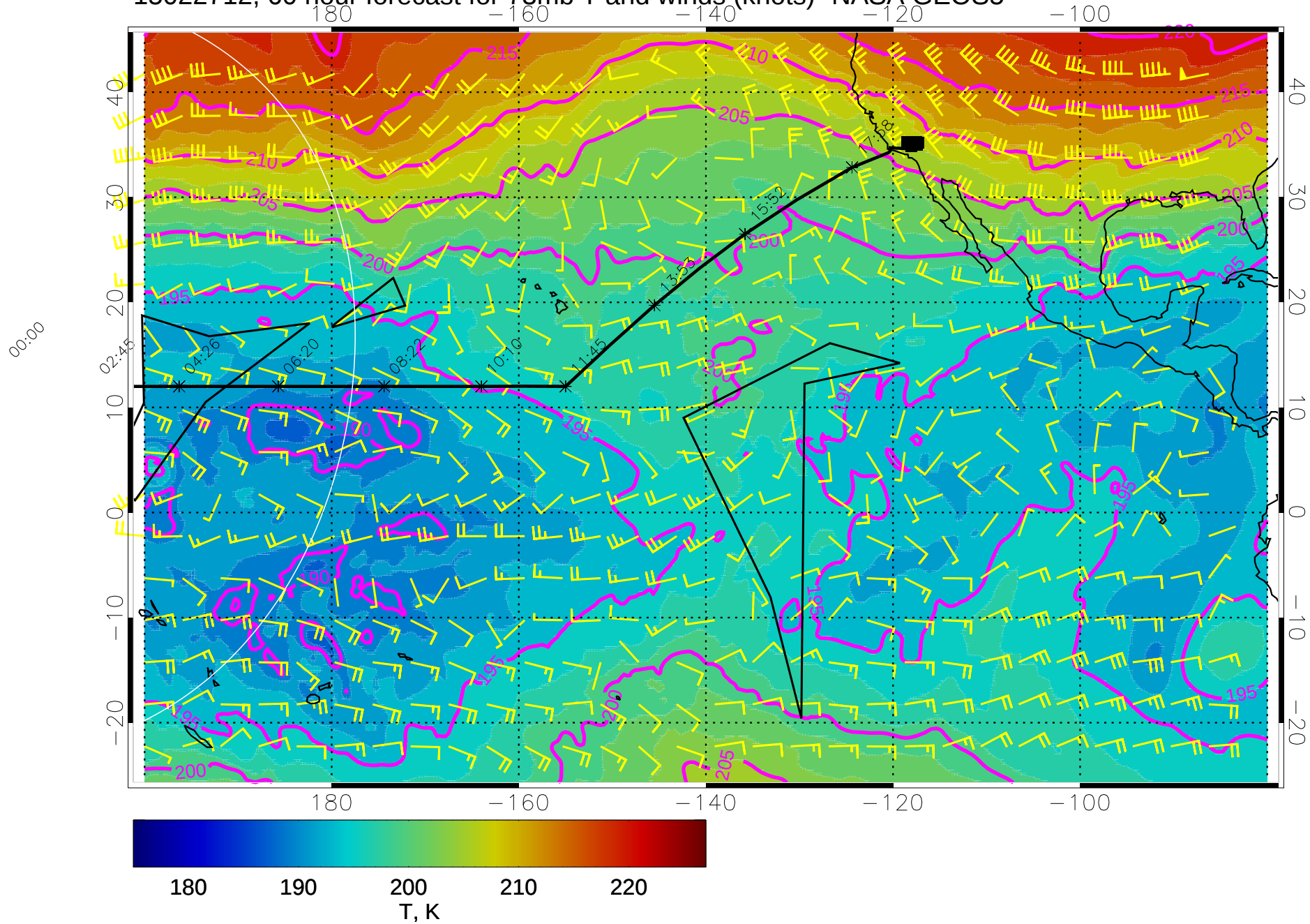
15022712, 60 hour forecast for 73mb T and winds (knots)- NASA GEOS5
