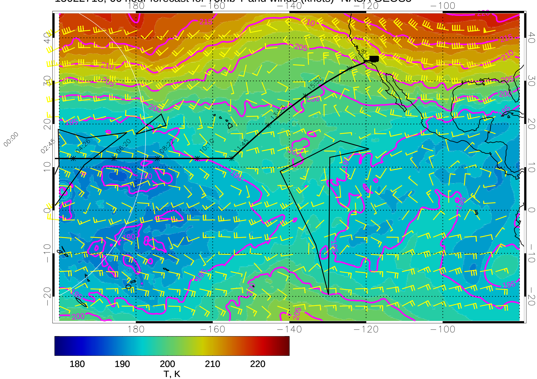
15022718, 66 hour forecast for 73mb T and winds (knots)- NASA GEOS5
