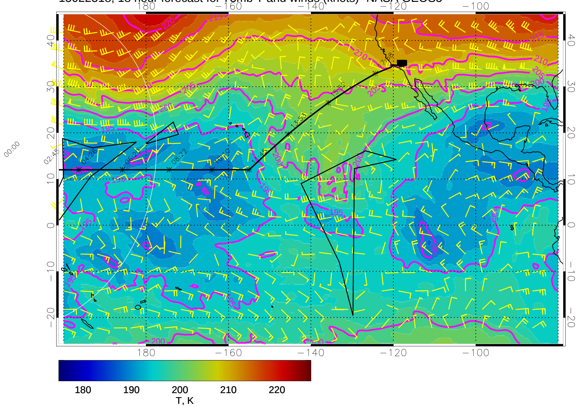
15022318, 18 hour forecast for 73mb T and winds (knots)- NASA GEOS5
