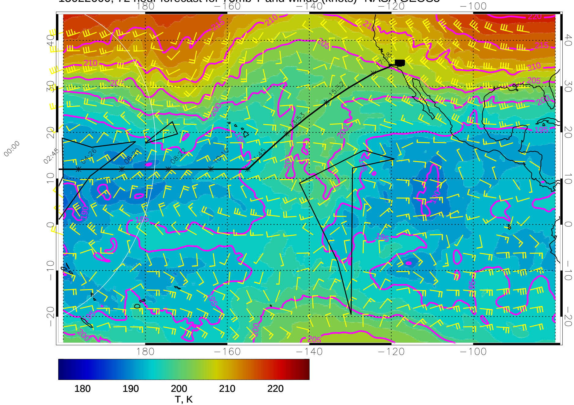
15022600, 72 hour forecast for 73mb T and winds (knots)- NASA GEOS5
