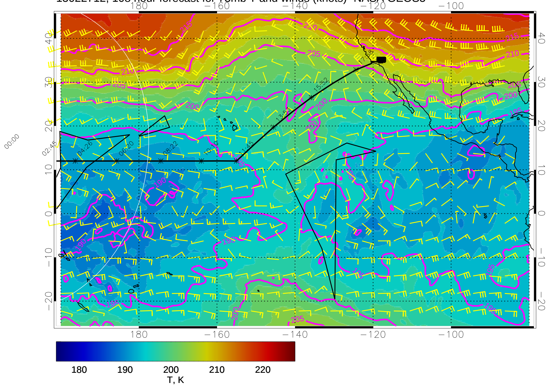
15022712, 108 hour forecast for 73mb T and winds (knots)- NASA GEOS5
