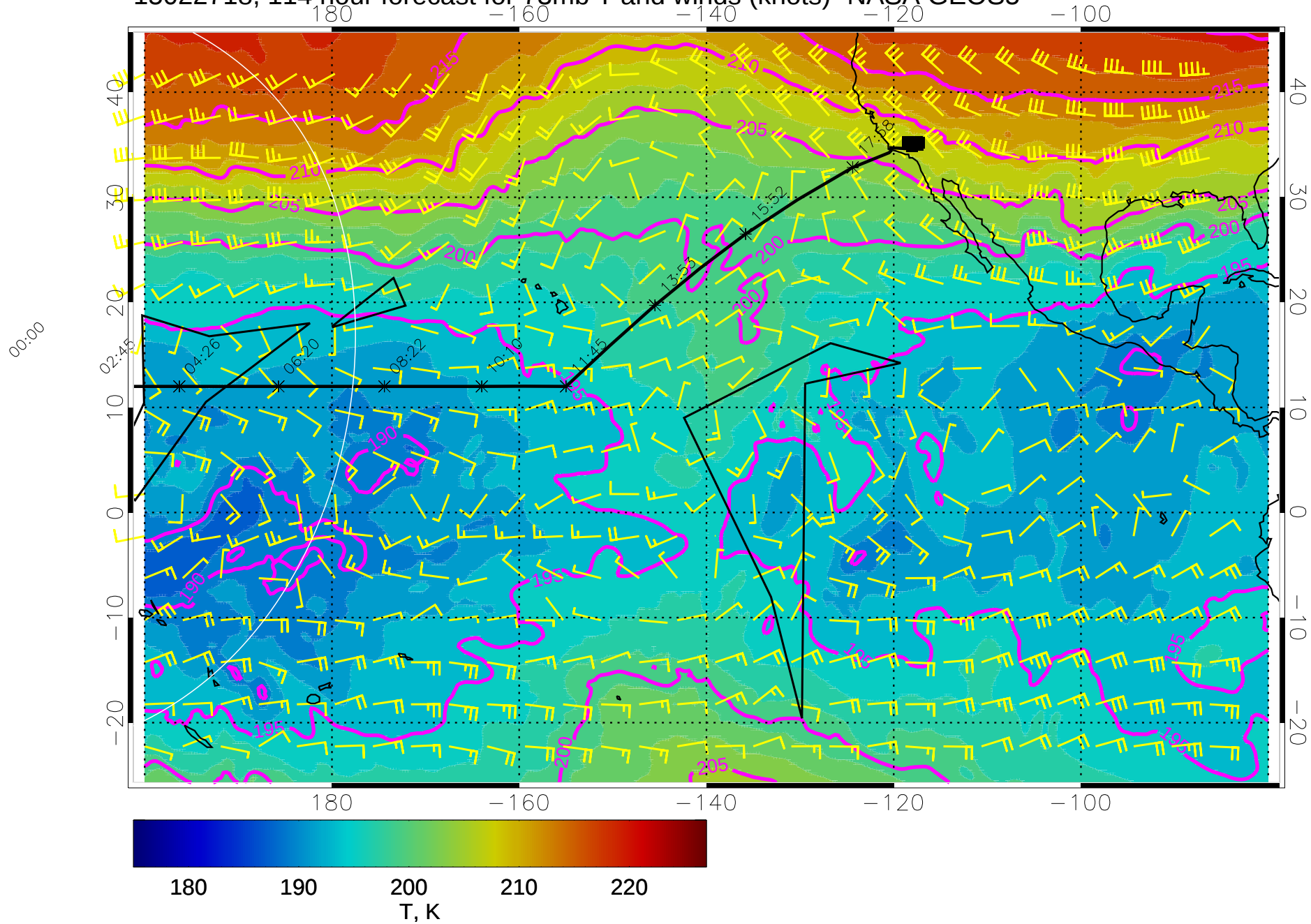
15022718, 114 hour forecast for 73mb T and winds (knots)- NASA GEOS5
