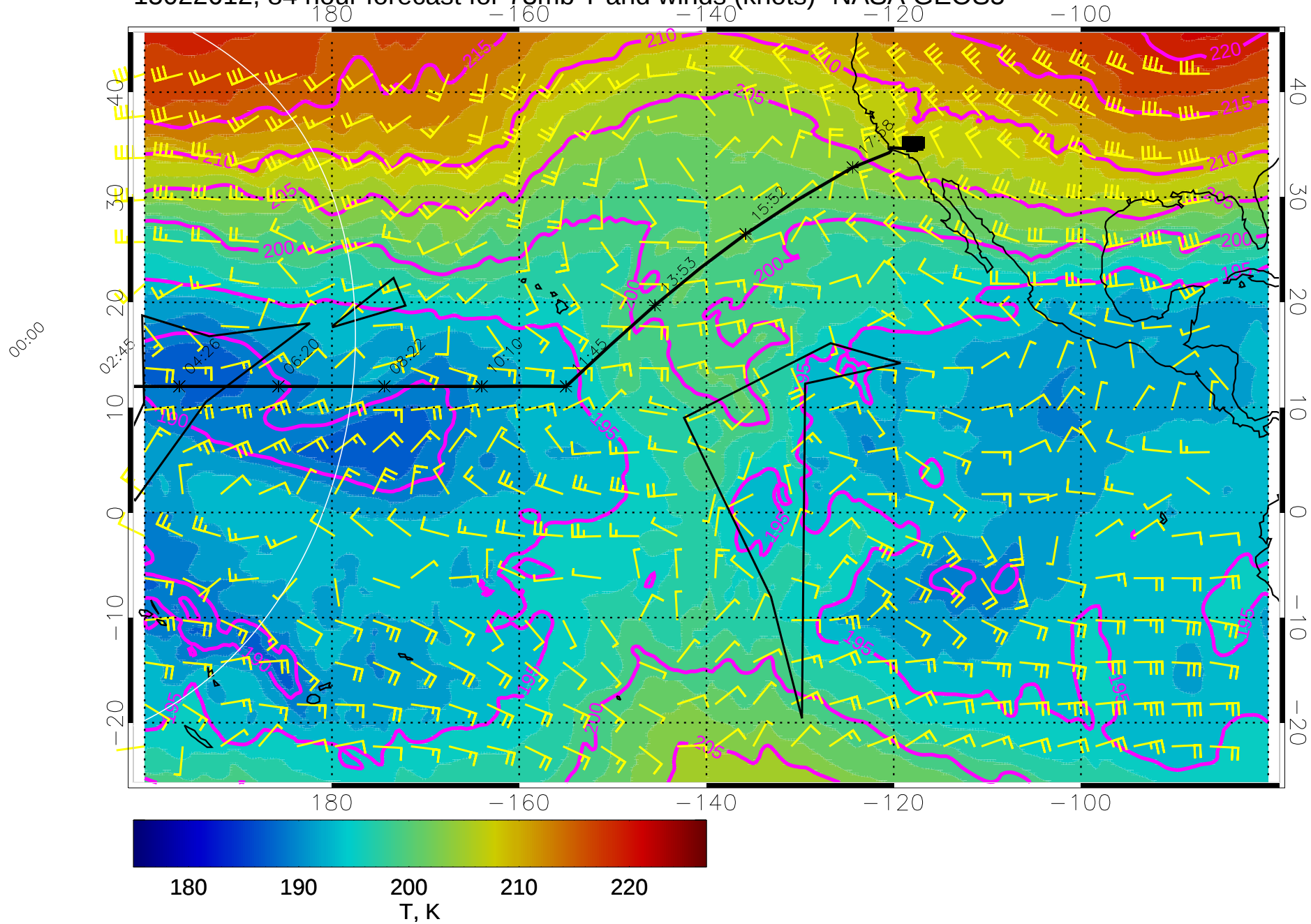
15022612, 84 hour forecast for 73mb T and winds (knots)- NASA GEOS5
