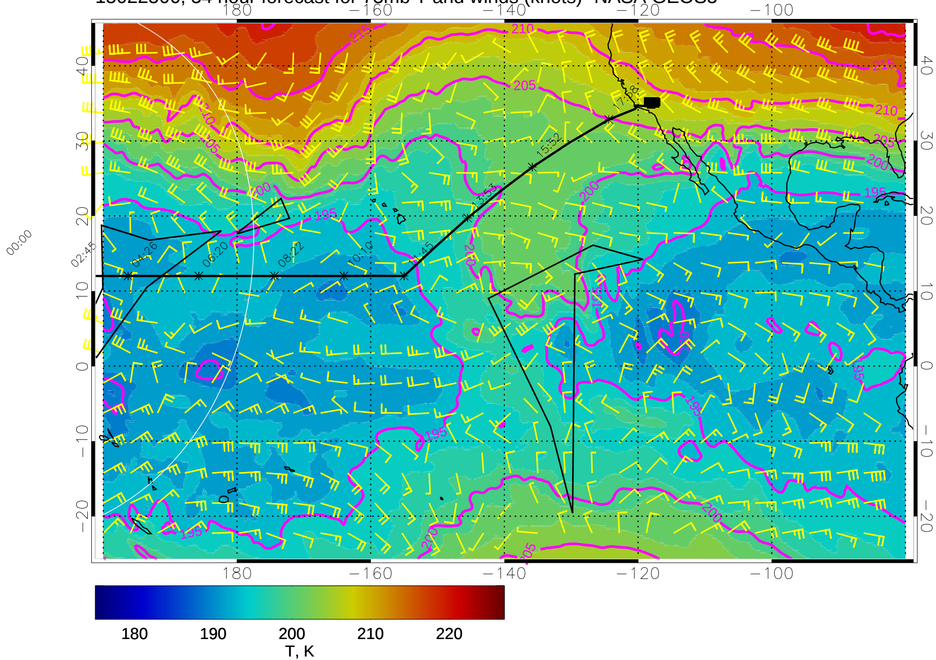
15022506, 54 hour forecast for 73mb T and winds (knots)- NASA GEOS5
