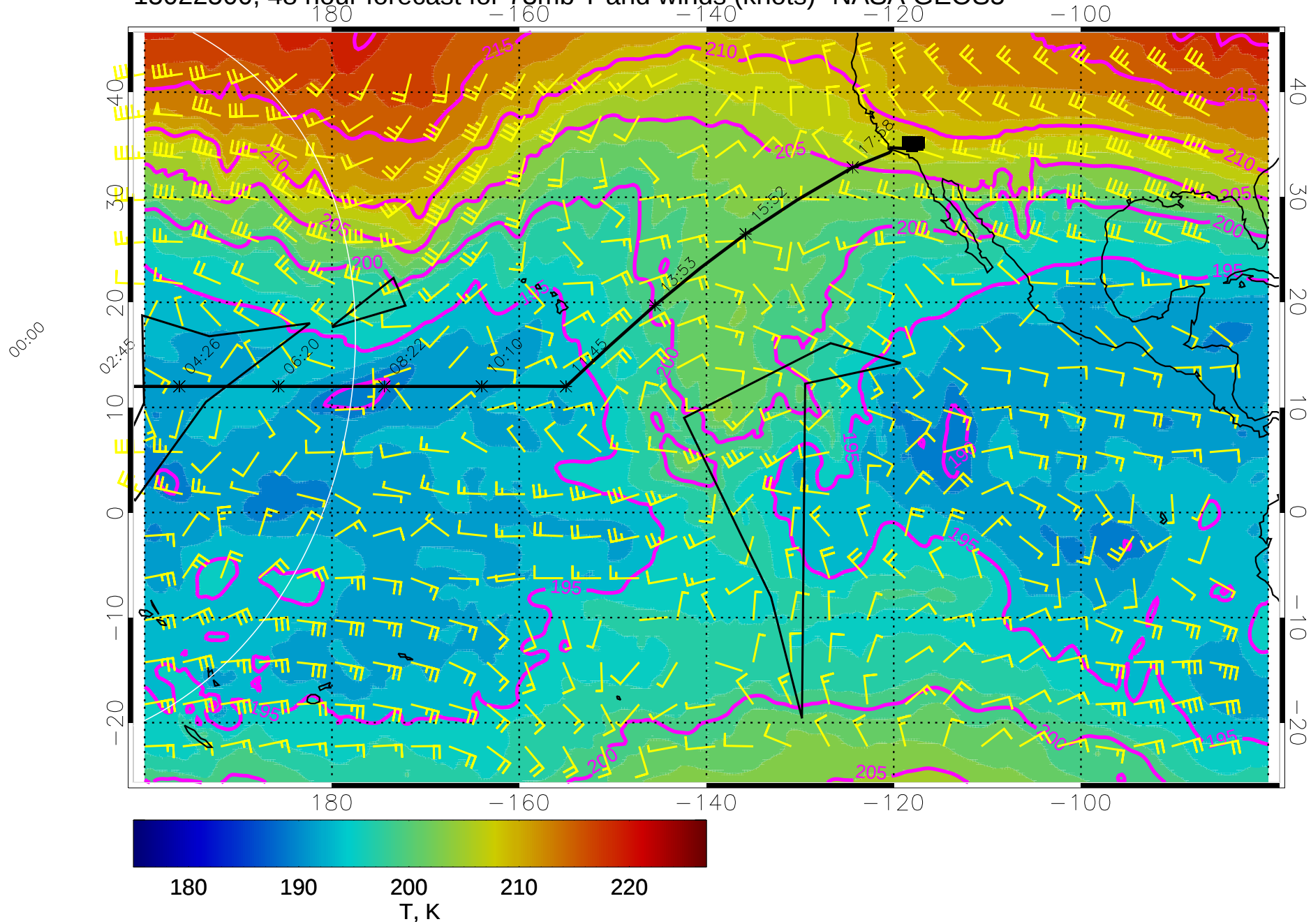
15022500, 48 hour forecast for 73mb T and winds (knots)- NASA GEOS5
