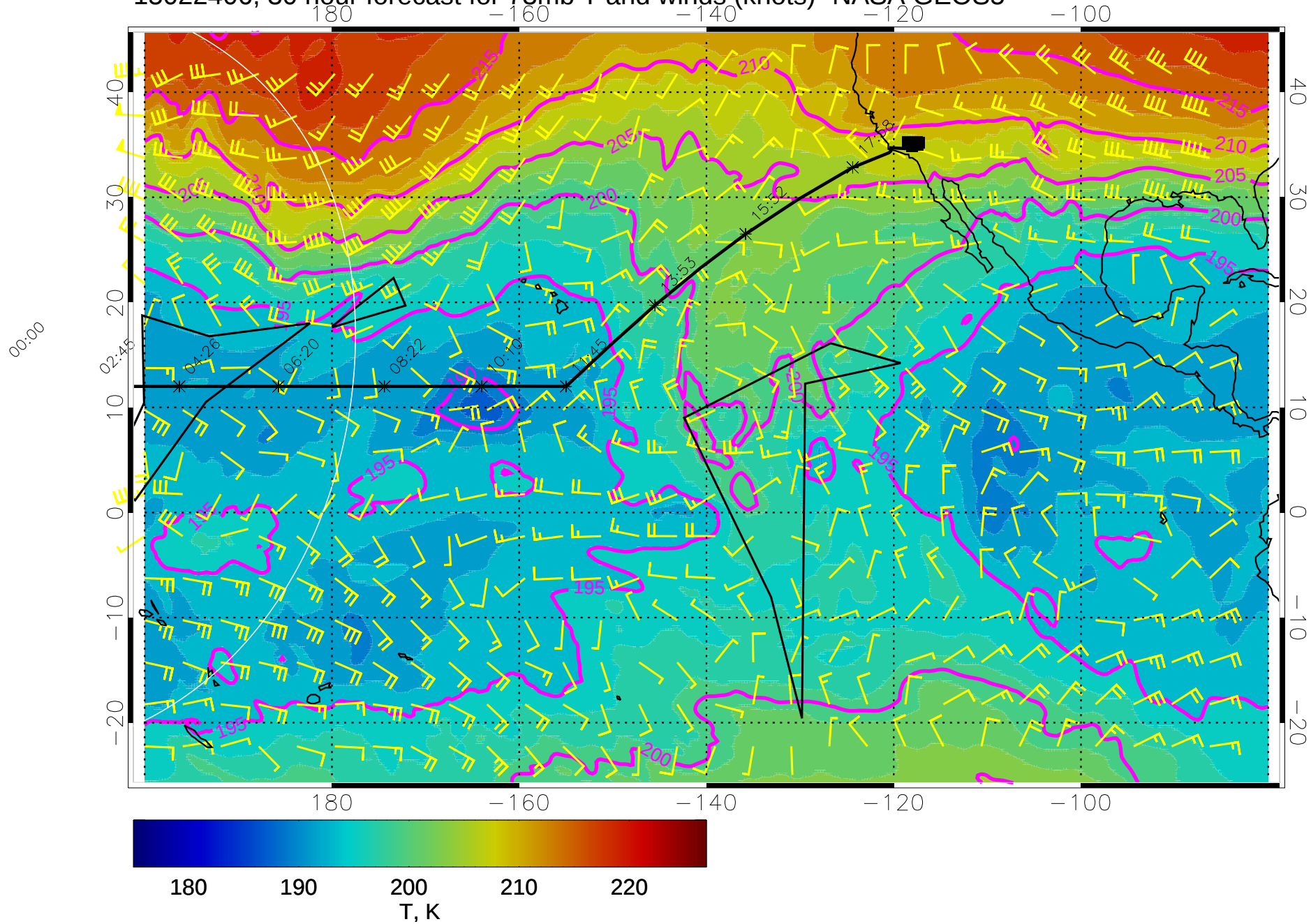
15022406, 30 hour forecast for 73mb T and winds (knots)- NASA GEOS5
