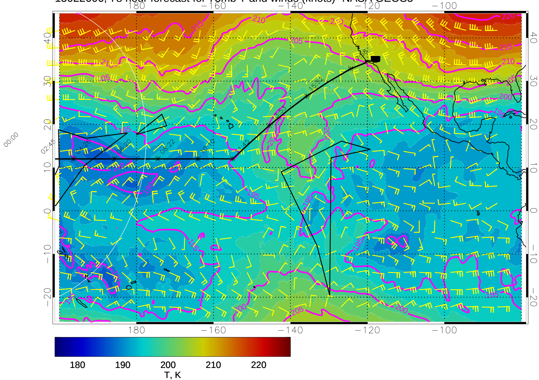
15022606, 78 hour forecast for 73mb T and winds (knots)- NASA GEOS5
