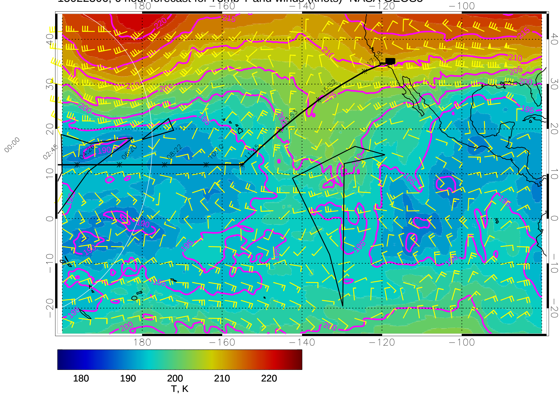
15022306, 6 hour forecast for 73mb T and winds (knots)- NASA GEOS5
