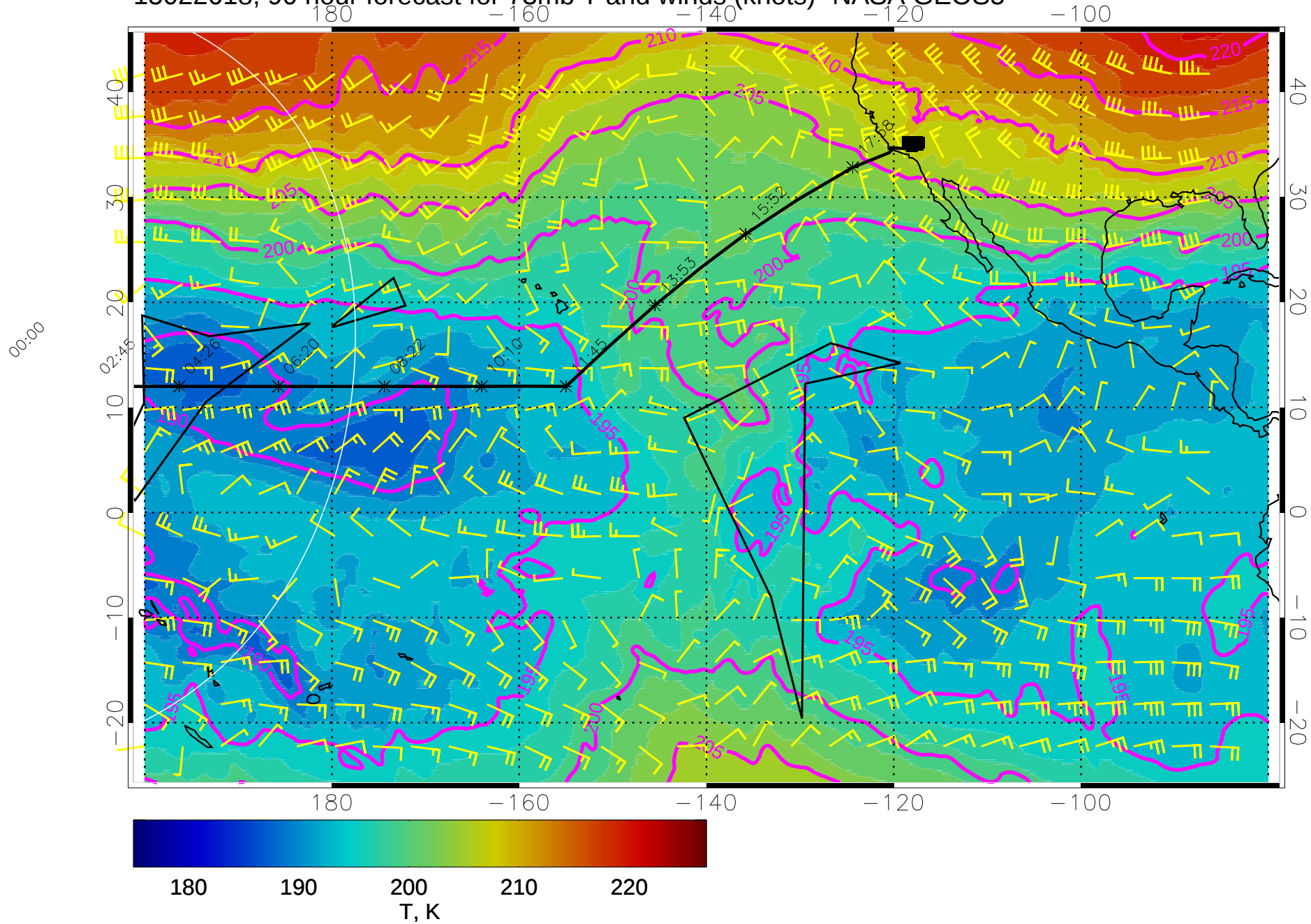
15022618, 90 hour forecast for 73mb T and winds (knots)- NASA GEOS5
