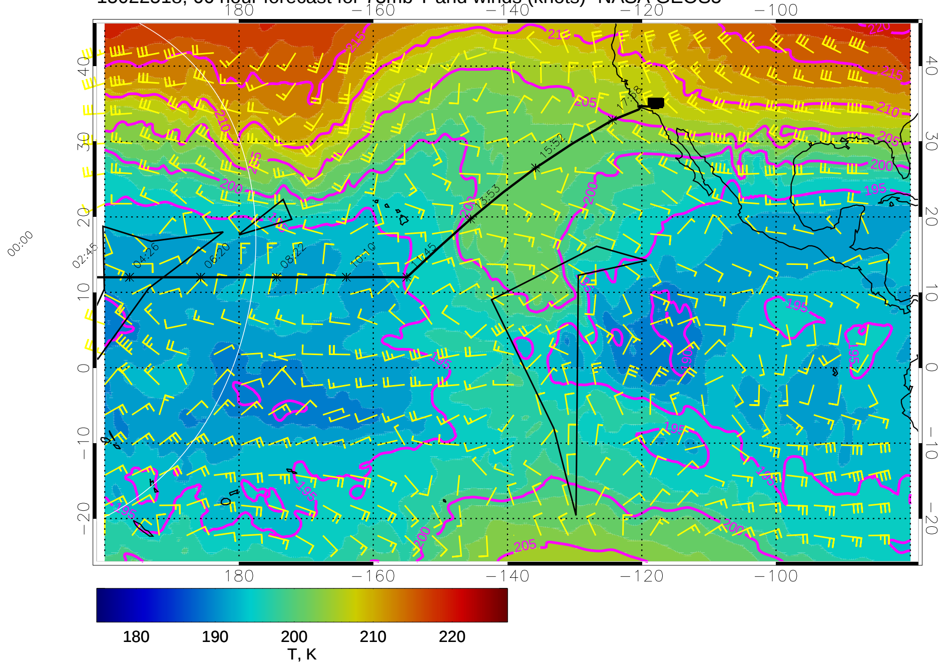
15022518, 66 hour forecast for 73mb T and winds (knots)- NASA GEOS5
