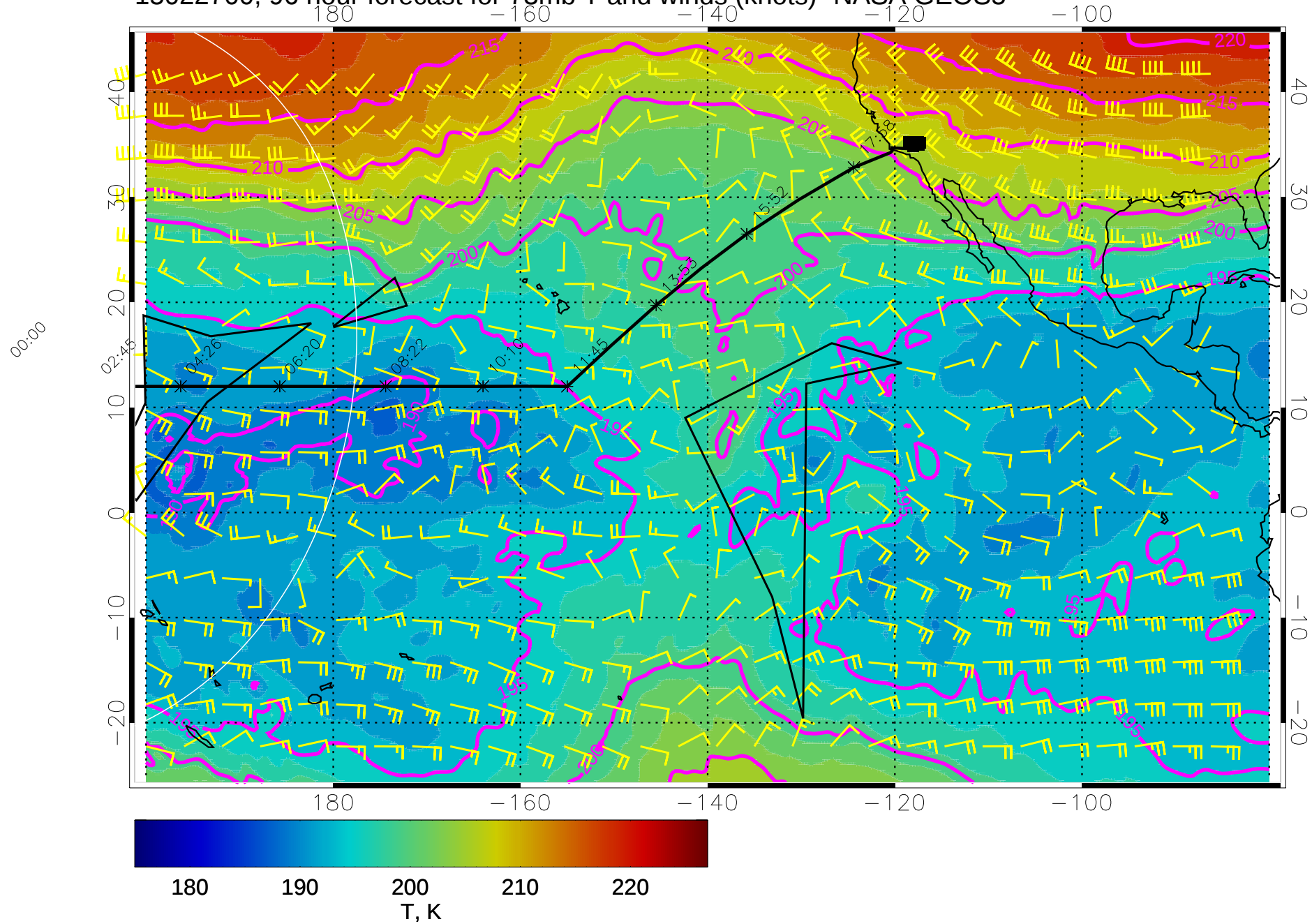
15022700, 96 hour forecast for 73mb T and winds (knots)- NASA GEOS5
