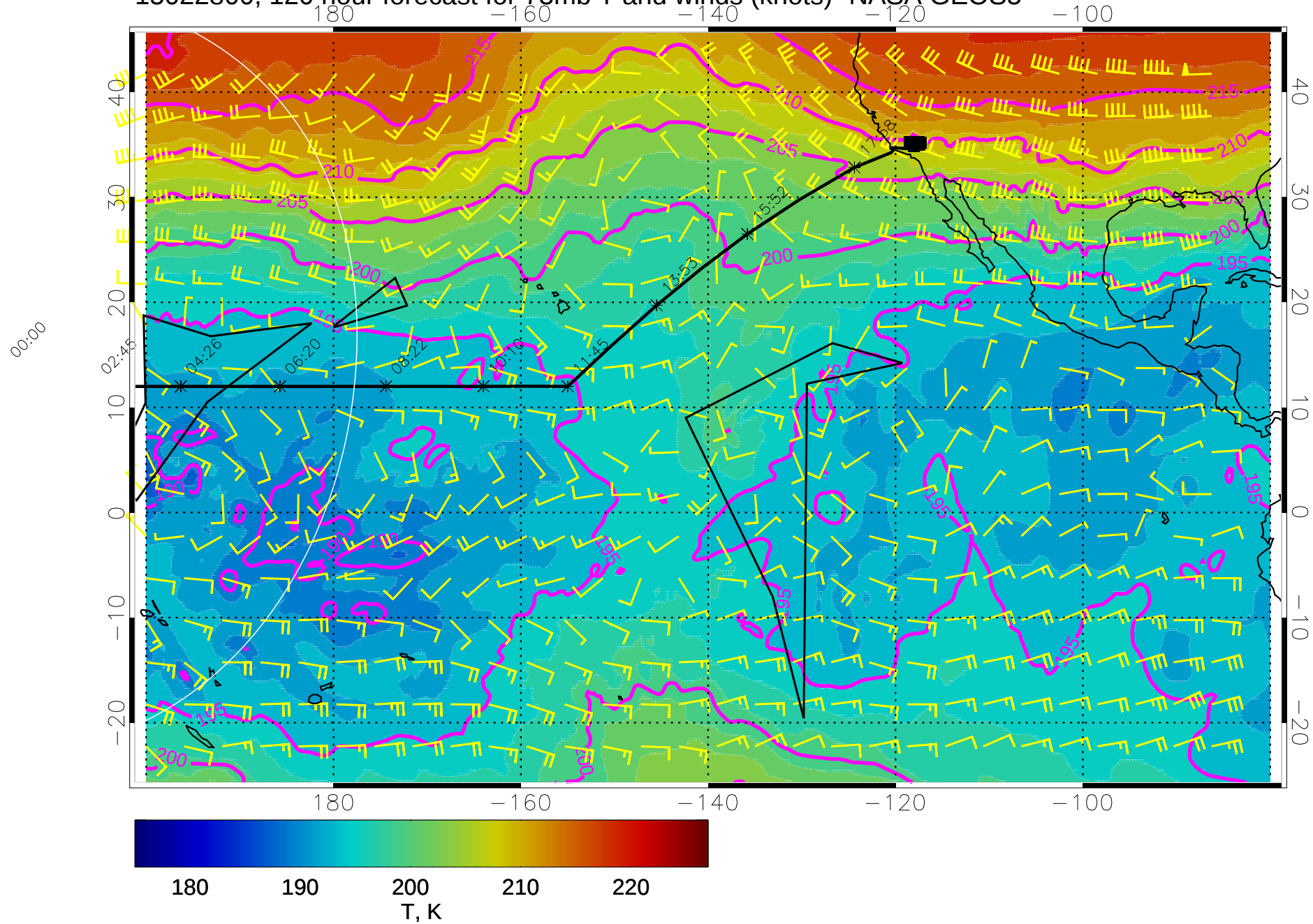
15022800, 120 hour forecast for 73mb T and winds (knots)- NASA GEOS5
