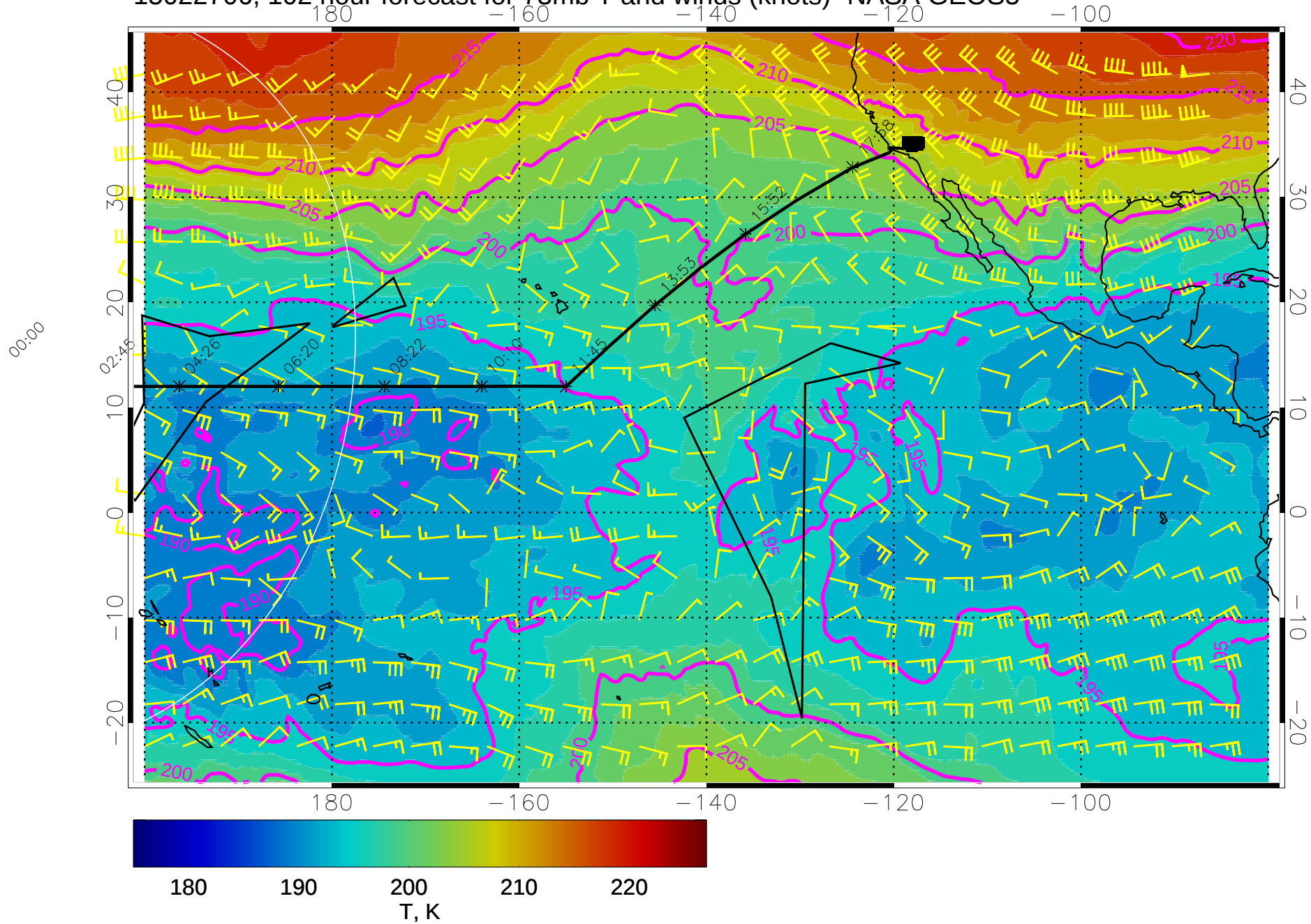
15022706, 102 hour forecast for 73mb T and winds (knots)- NASA GEOS5
