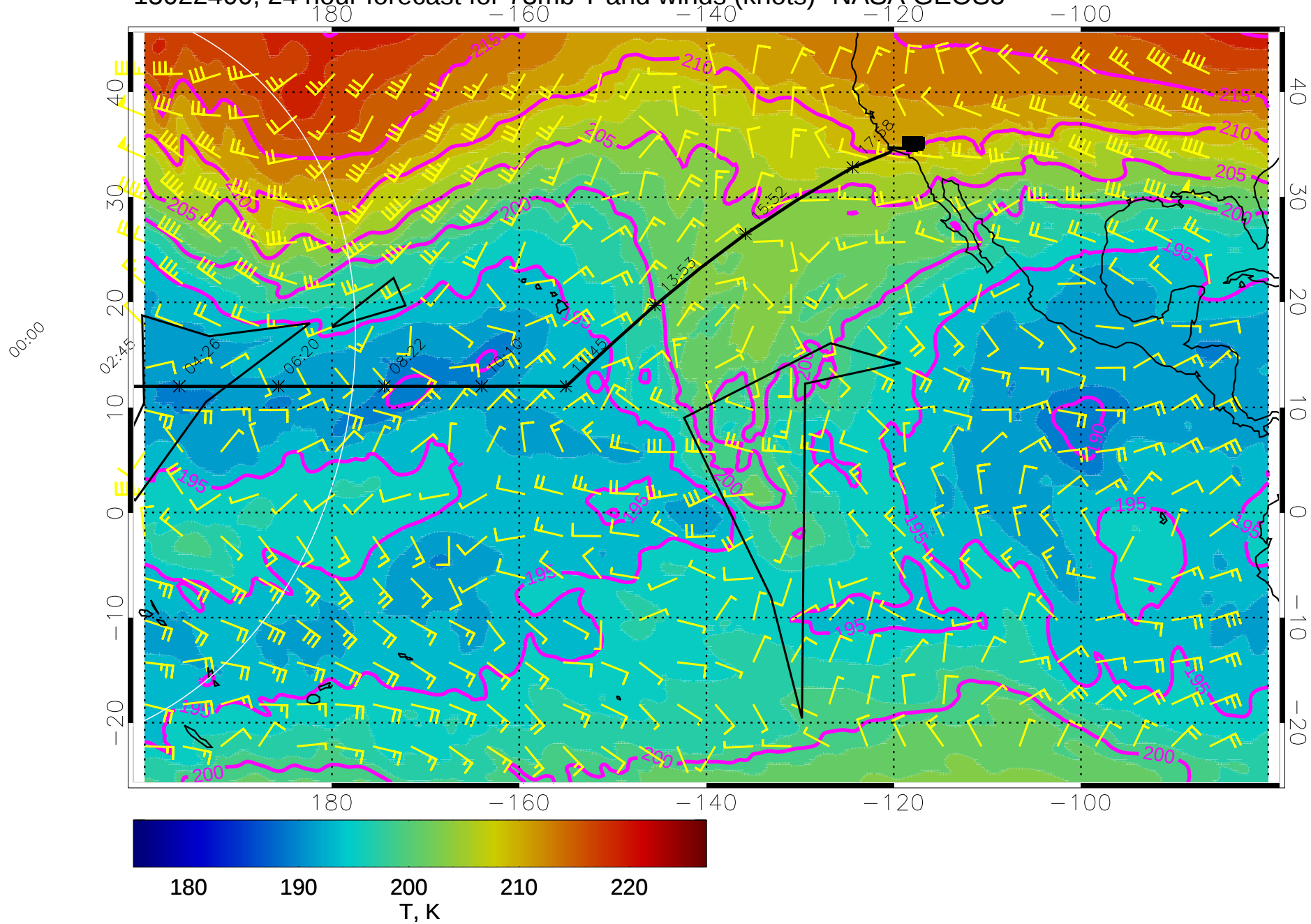
15022400, 24 hour forecast for 73mb T and winds (knots)- NASA GEOS5
