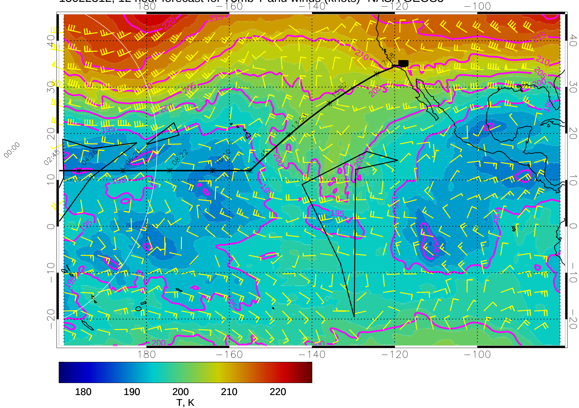
15022312, 12 hour forecast for 73mb T and winds (knots)- NASA GEOS5
