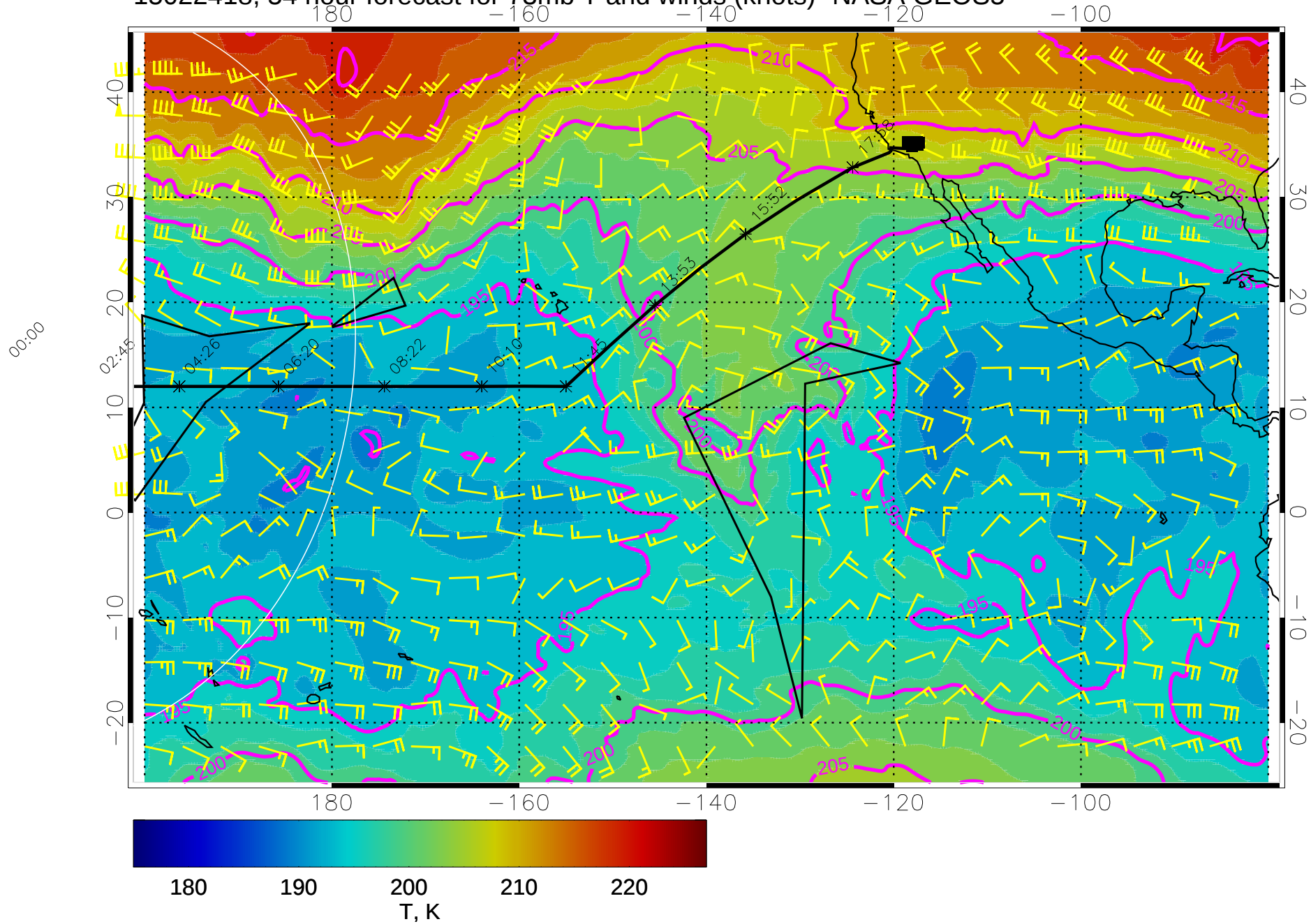
15022418, 54 hour forecast for 73mb T and winds (knots)- NASA GEOS5
