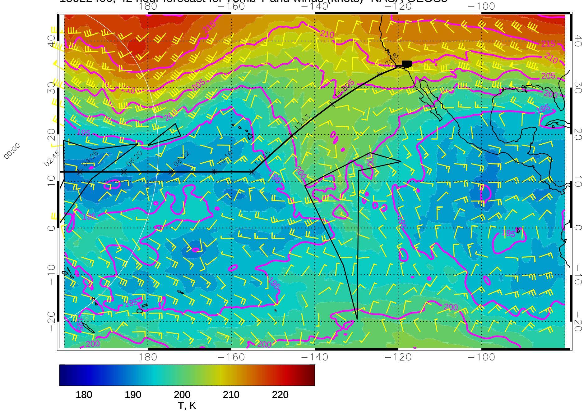
15022406, 42 hour forecast for 73mb T and winds (knots)- NASA GEOS5
