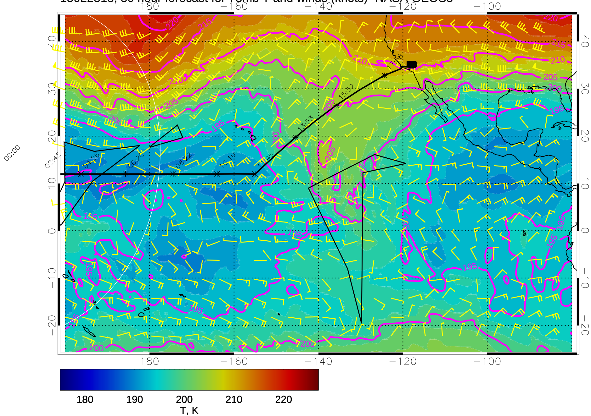
15022318, 30 hour forecast for 73mb T and winds (knots)- NASA GEOS5
