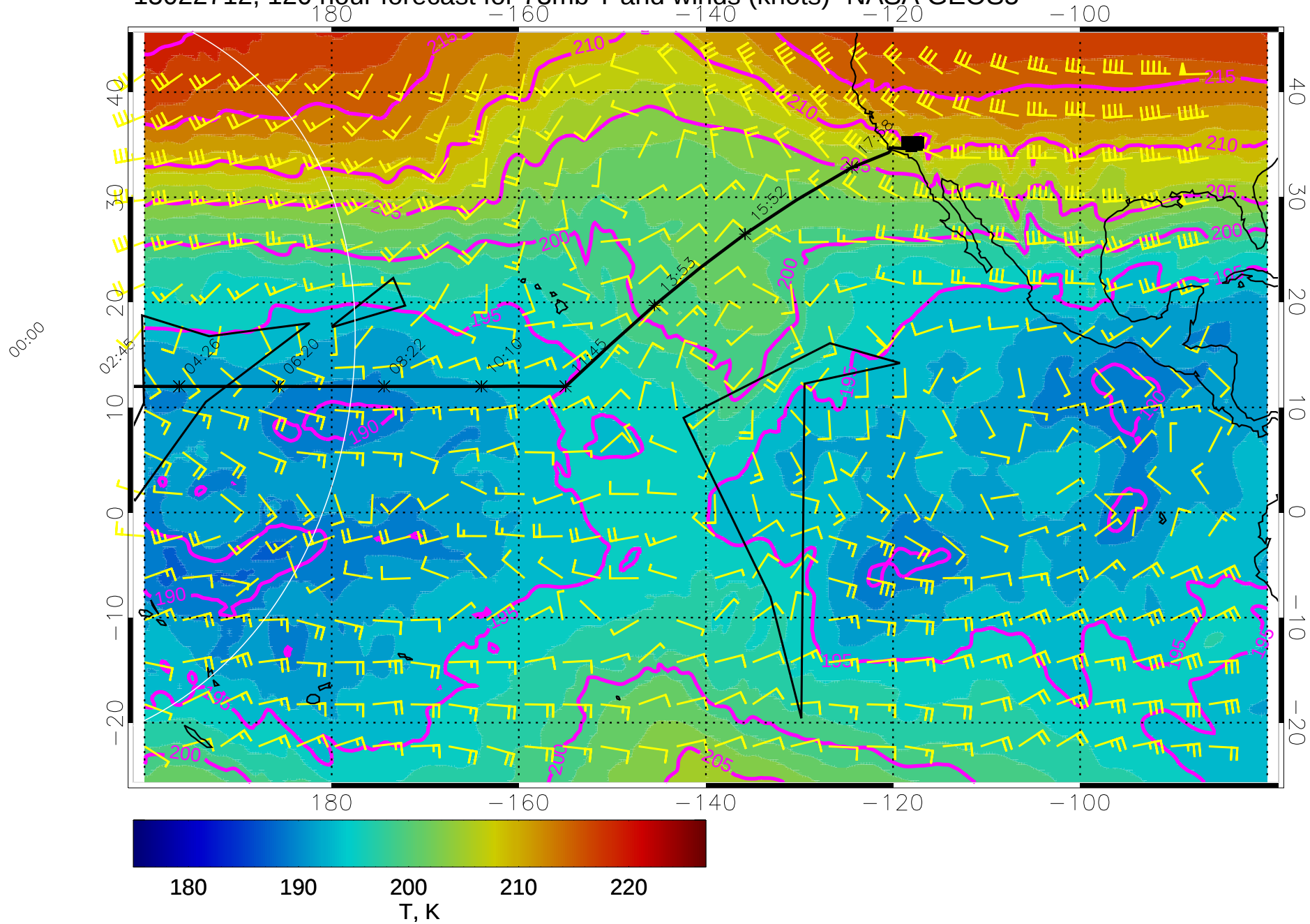
15022712, 120 hour forecast for 73mb T and winds (knots)- NASA GEOS5
