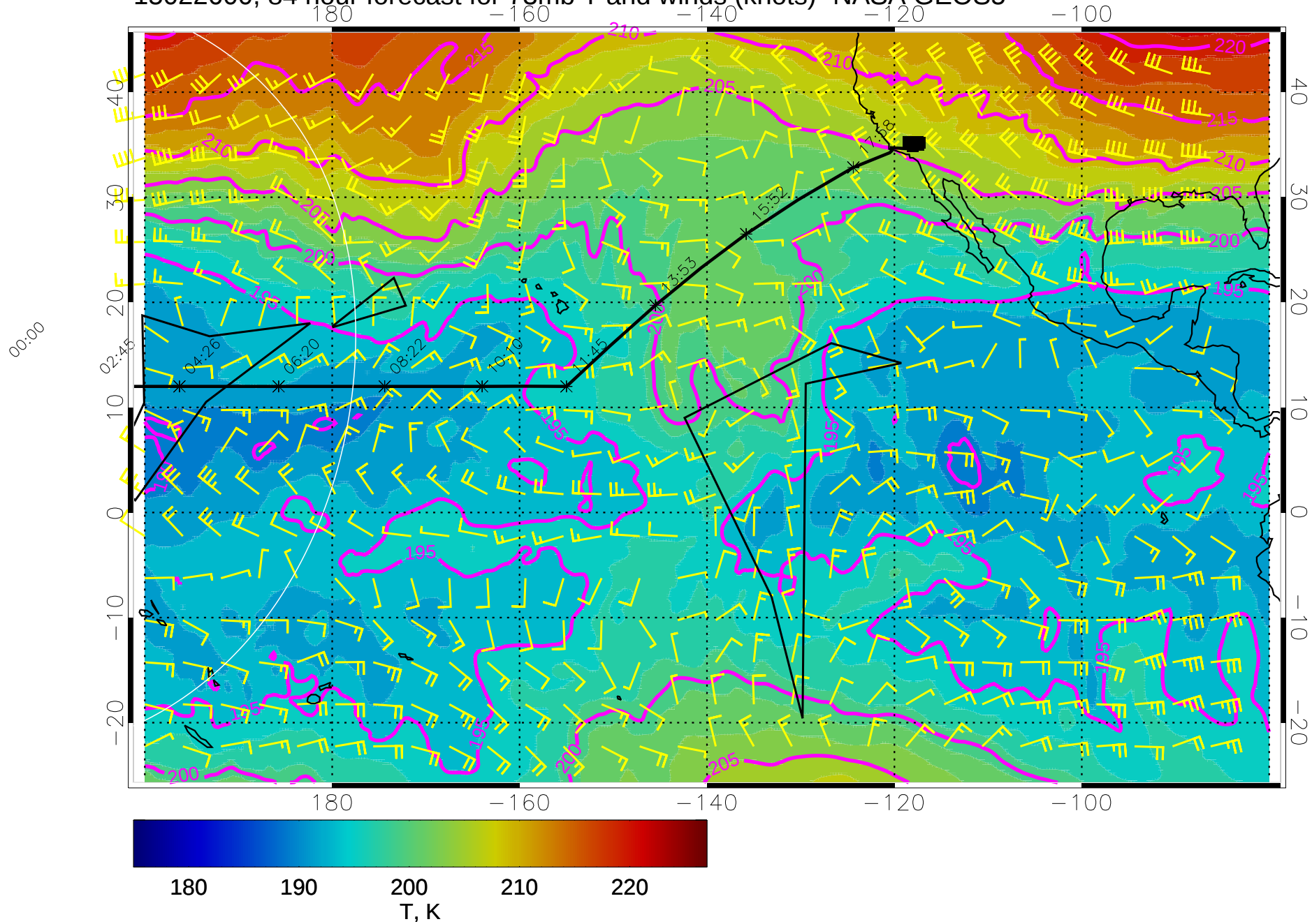
15022600, 84 hour forecast for 73mb T and winds (knots)- NASA GEOS5
