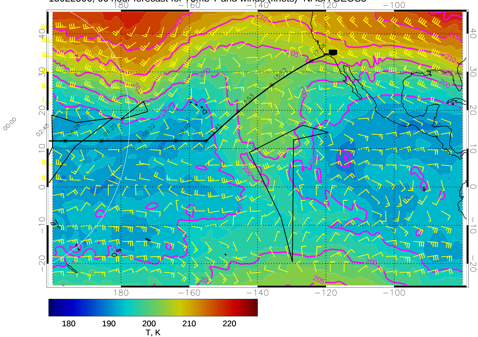
15022506, 66 hour forecast for 73mb T and winds (knots)- NASA GEOS5
