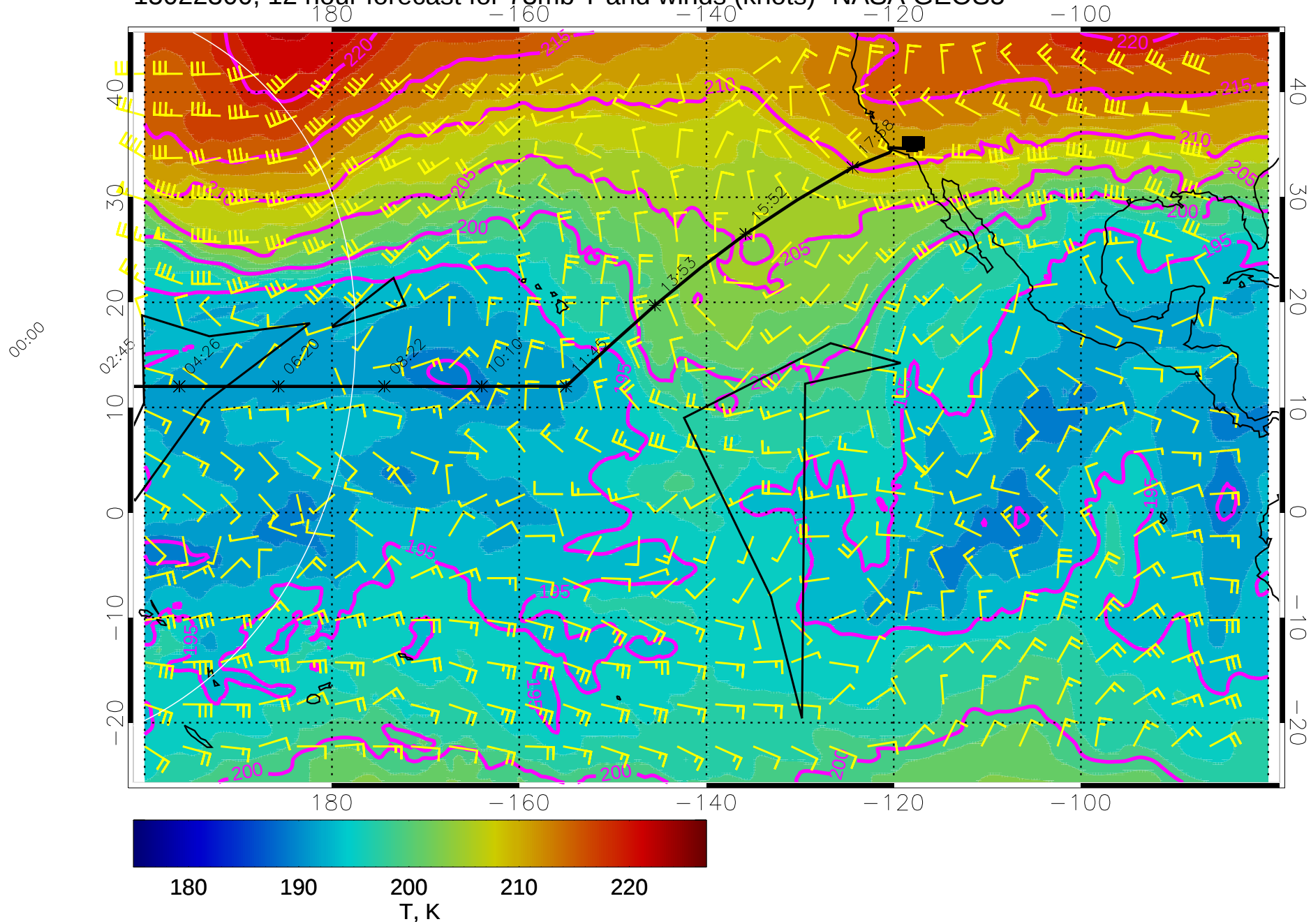
15022300, 12 hour forecast for 73mb T and winds (knots)- NASA GEOS5
