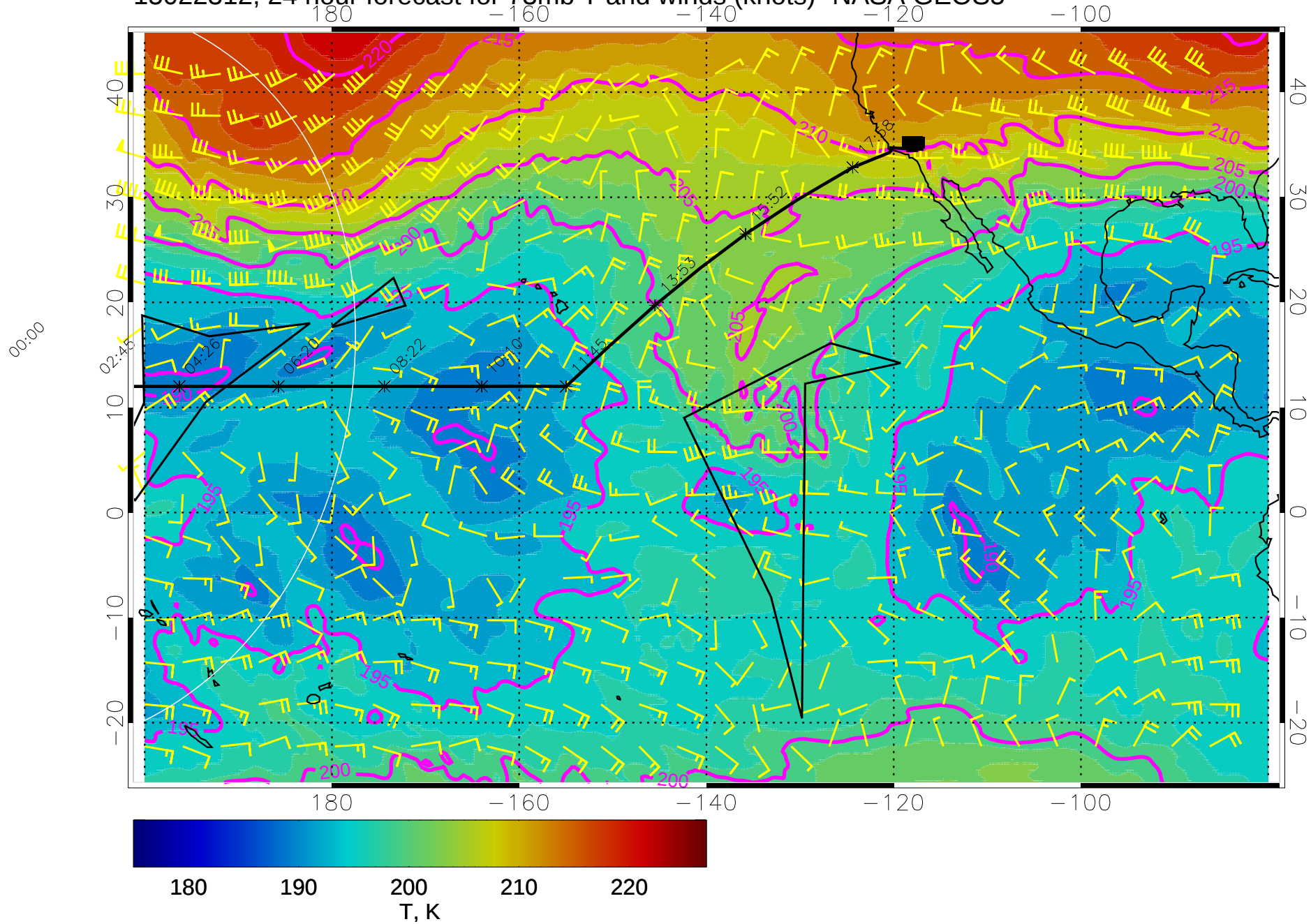
15022312, 24 hour forecast for 73mb T and winds (knots)- NASA GEOS5
