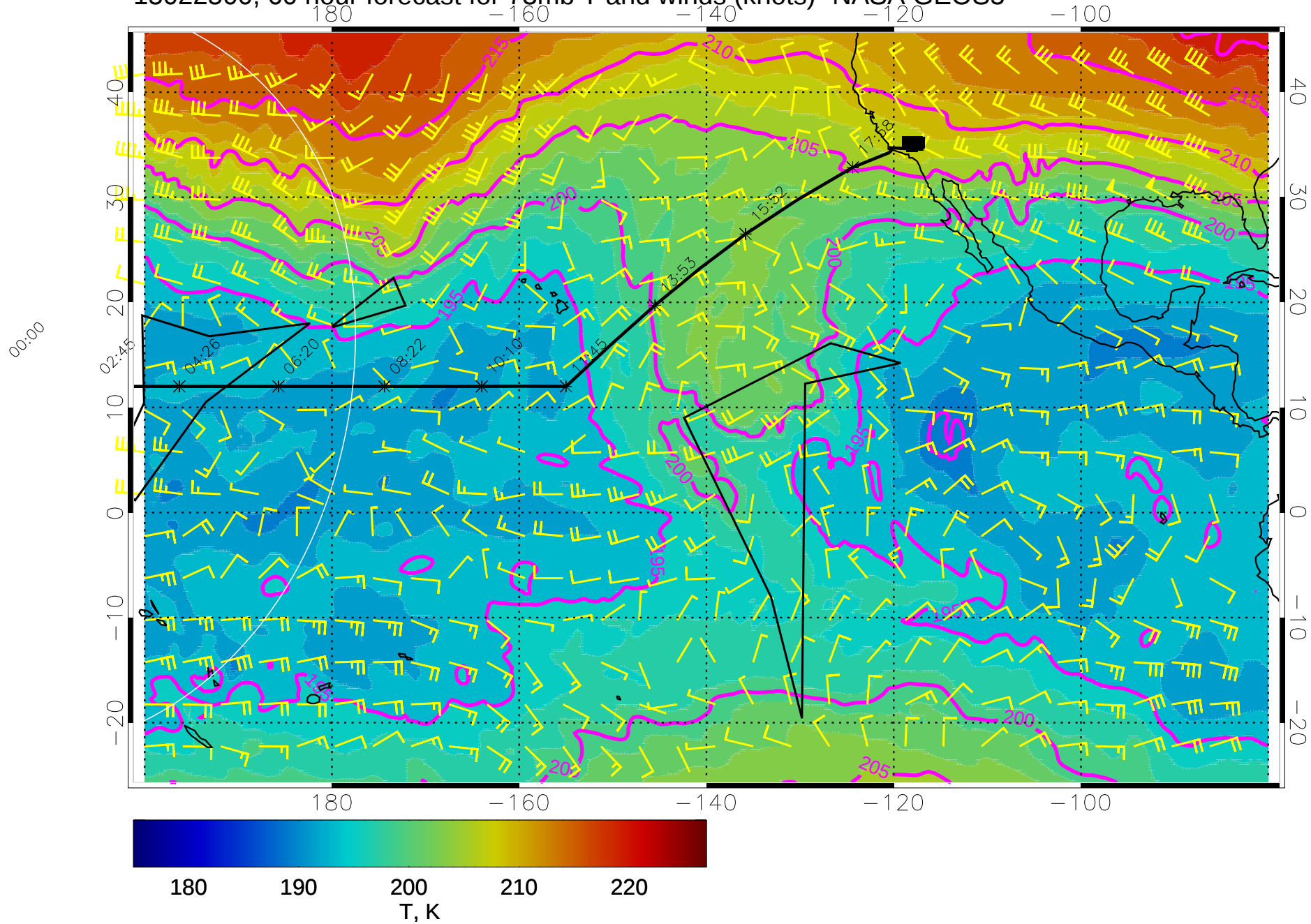
15022500, 60 hour forecast for 73mb T and winds (knots)- NASA GEOS5
