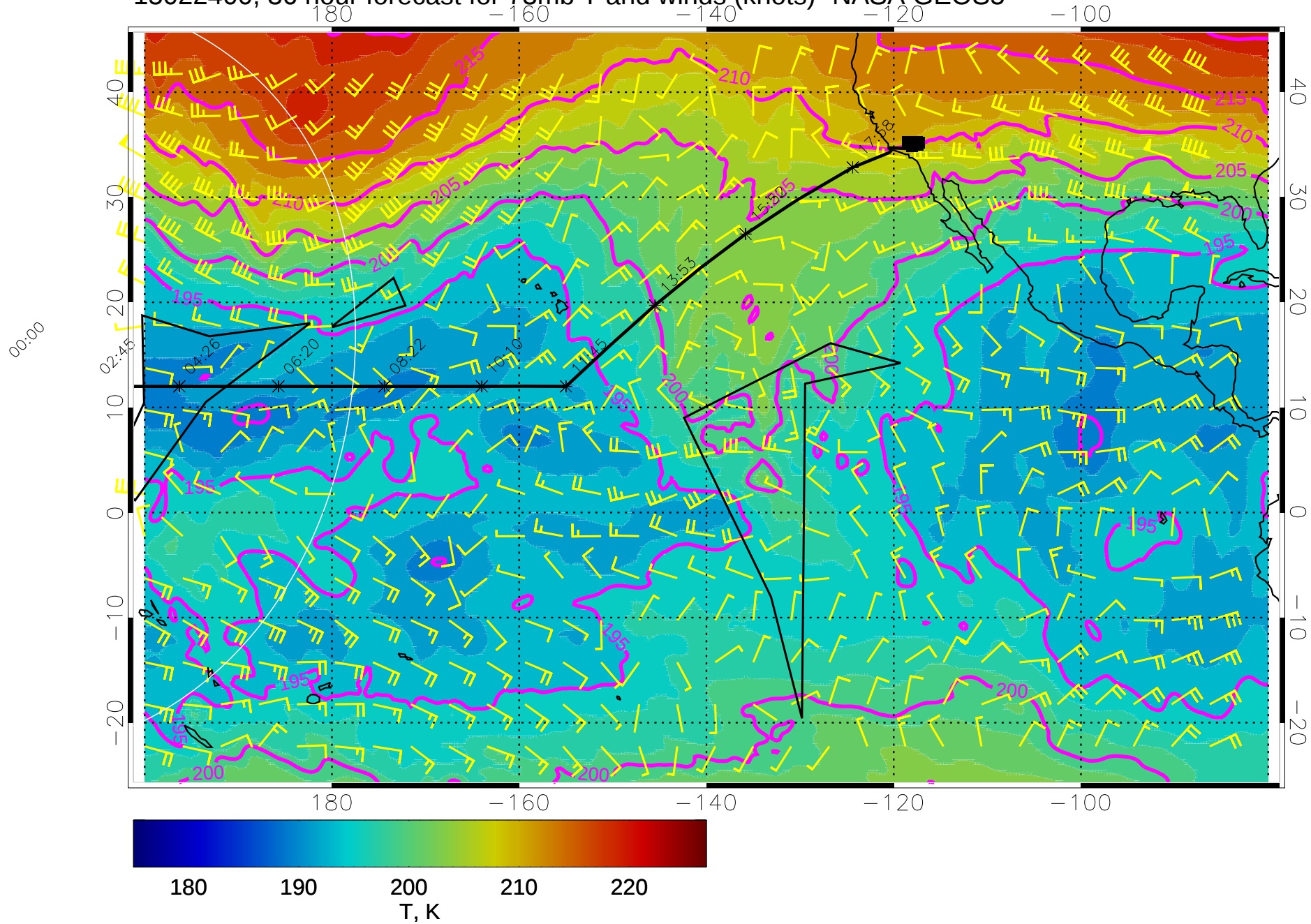
15022400, 36 hour forecast for 73mb T and winds (knots)- NASA GEOS5
