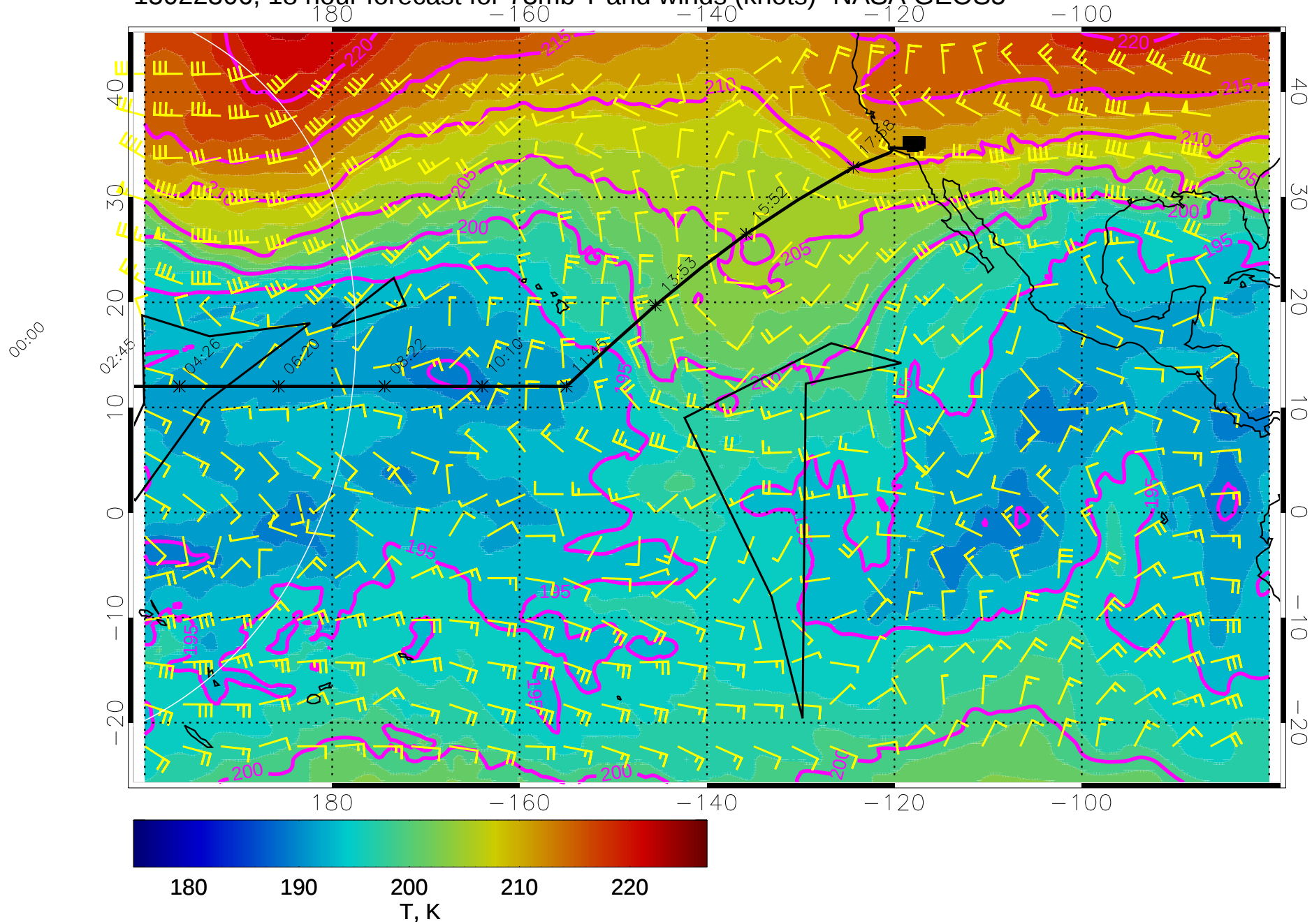
15022306, 18 hour forecast for 73mb T and winds (knots)- NASA GEOS5
