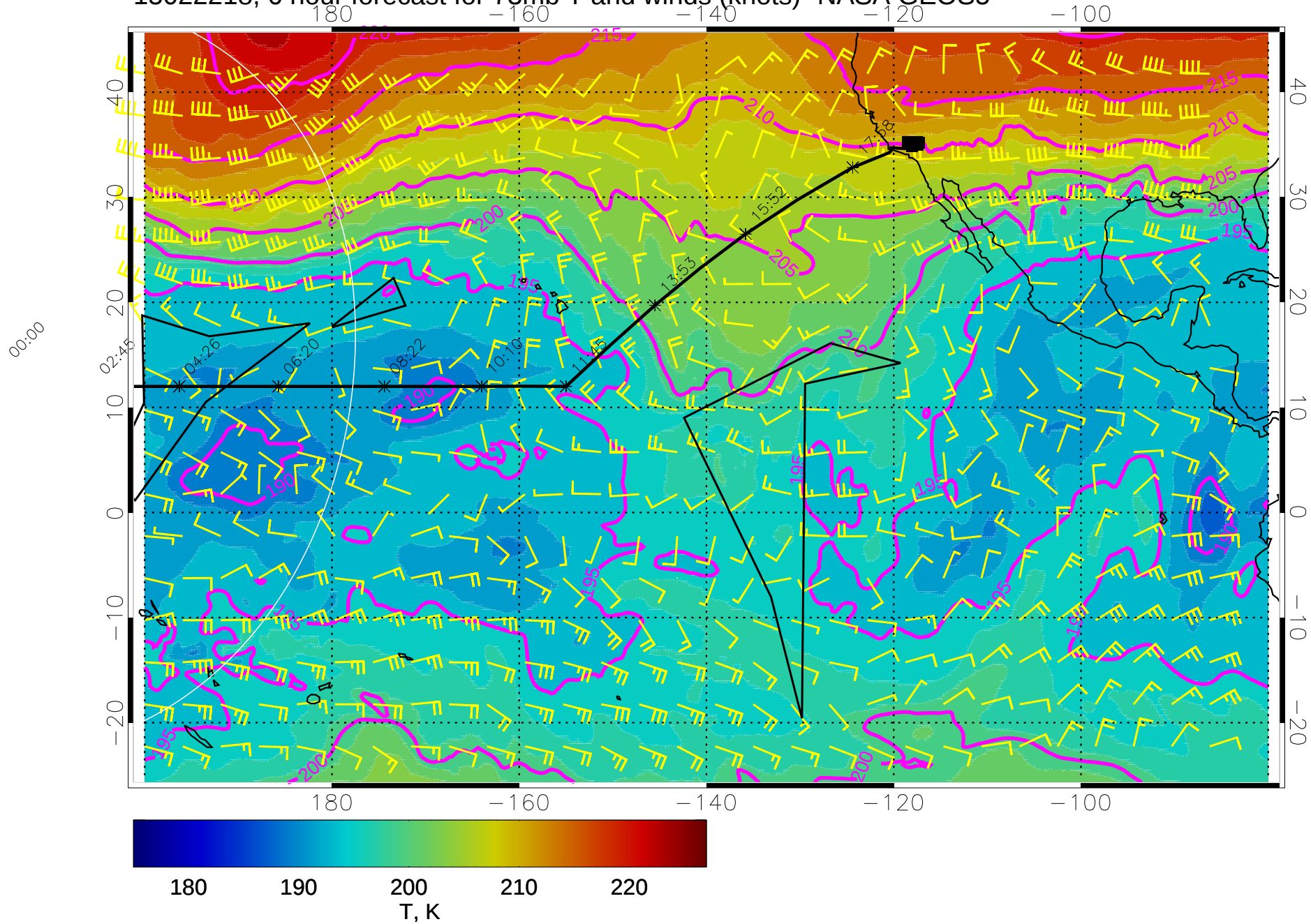
15022218, 6 hour forecast for 73mb T and winds (knots)- NASA GEOS5
