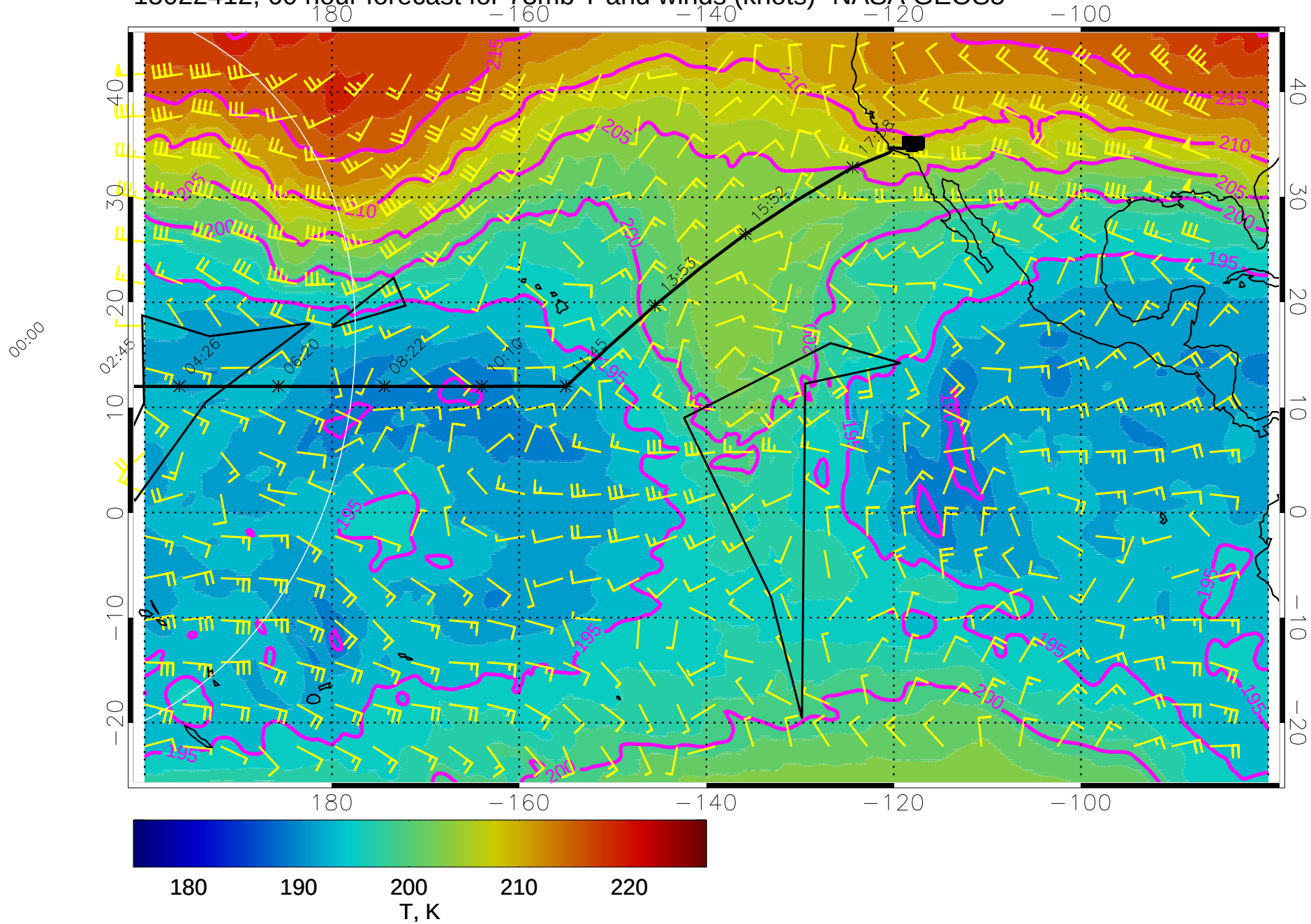
15022412, 60 hour forecast for 73mb T and winds (knots)- NASA GEOS5
