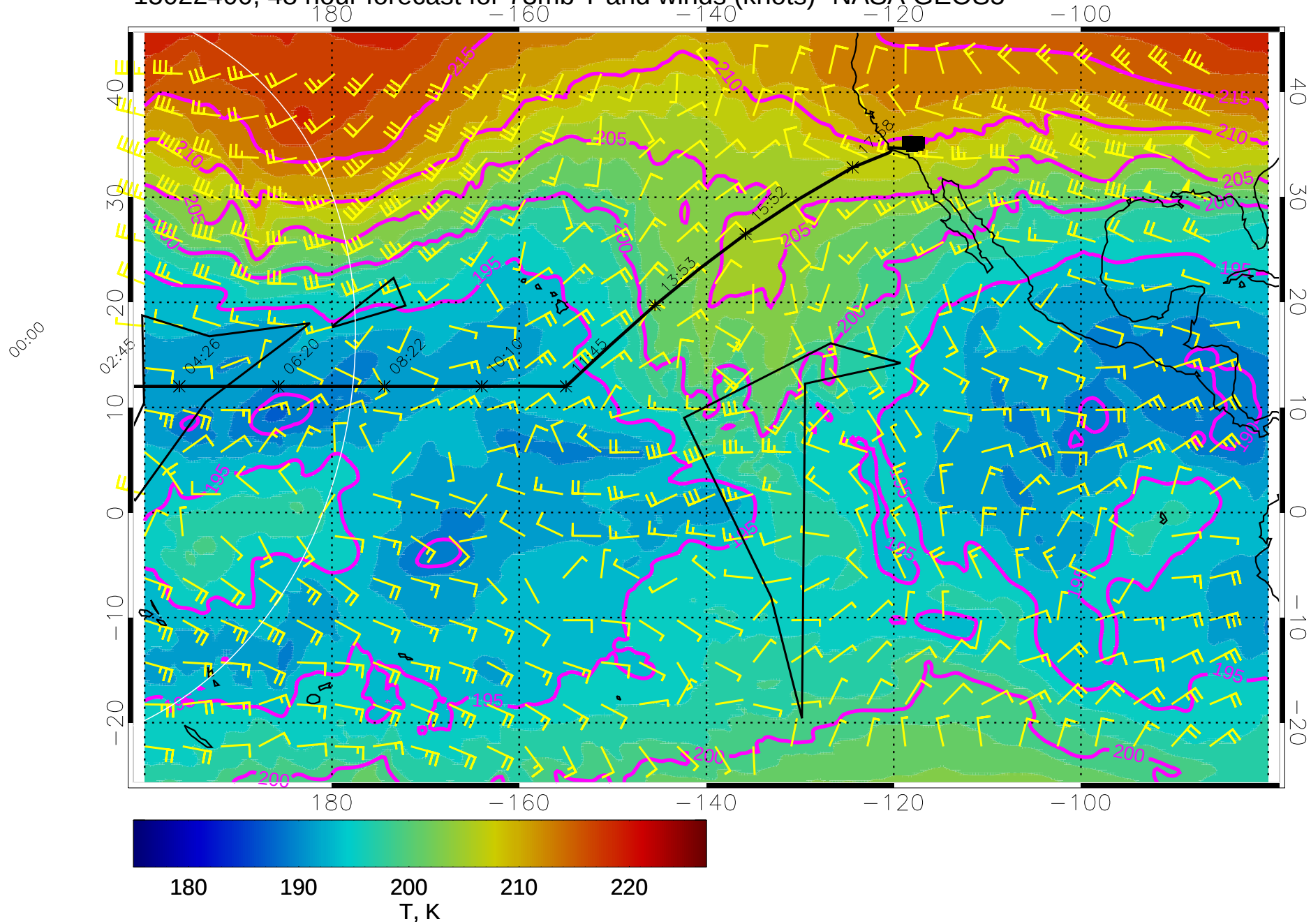
15022400, 48 hour forecast for 73mb T and winds (knots)- NASA GEOS5
