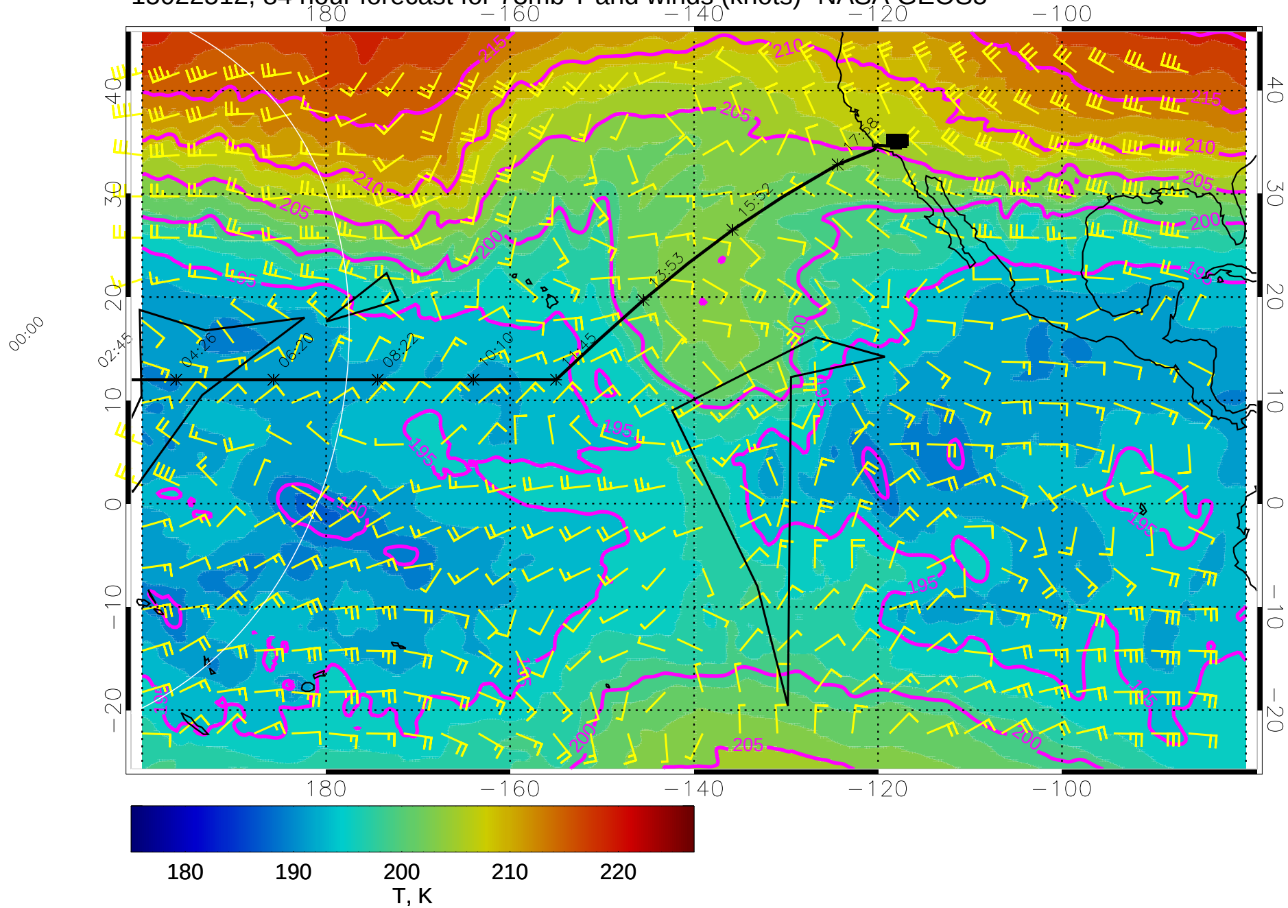
15022512, 84 hour forecast for 73mb T and winds (knots)- NASA GEOS5
