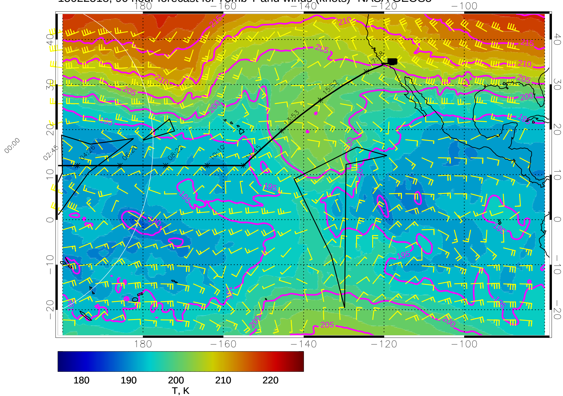
15022518, 90 hour forecast for 73mb T and winds (knots)- NASA GEOS5
