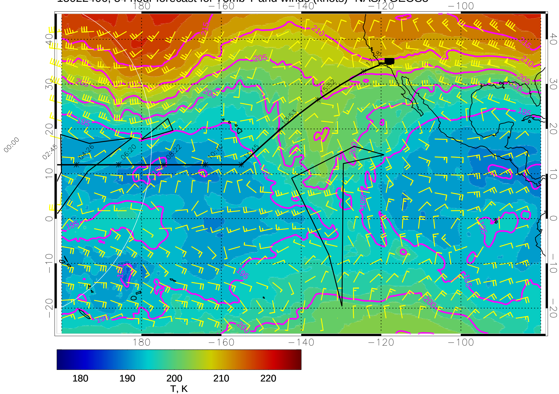
15022406, 54 hour forecast for 73mb T and winds (knots)- NASA GEOS5
