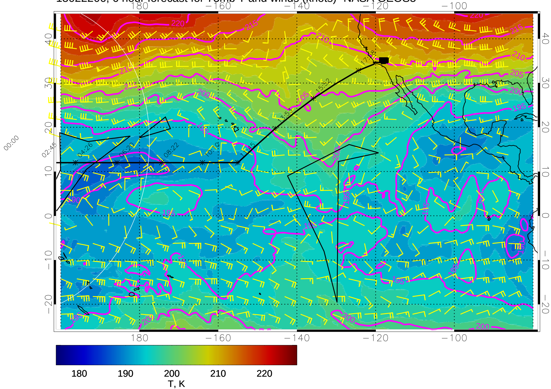
15022206, 6 hour forecast for 73mb T and winds (knots)- NASA GEOS5
