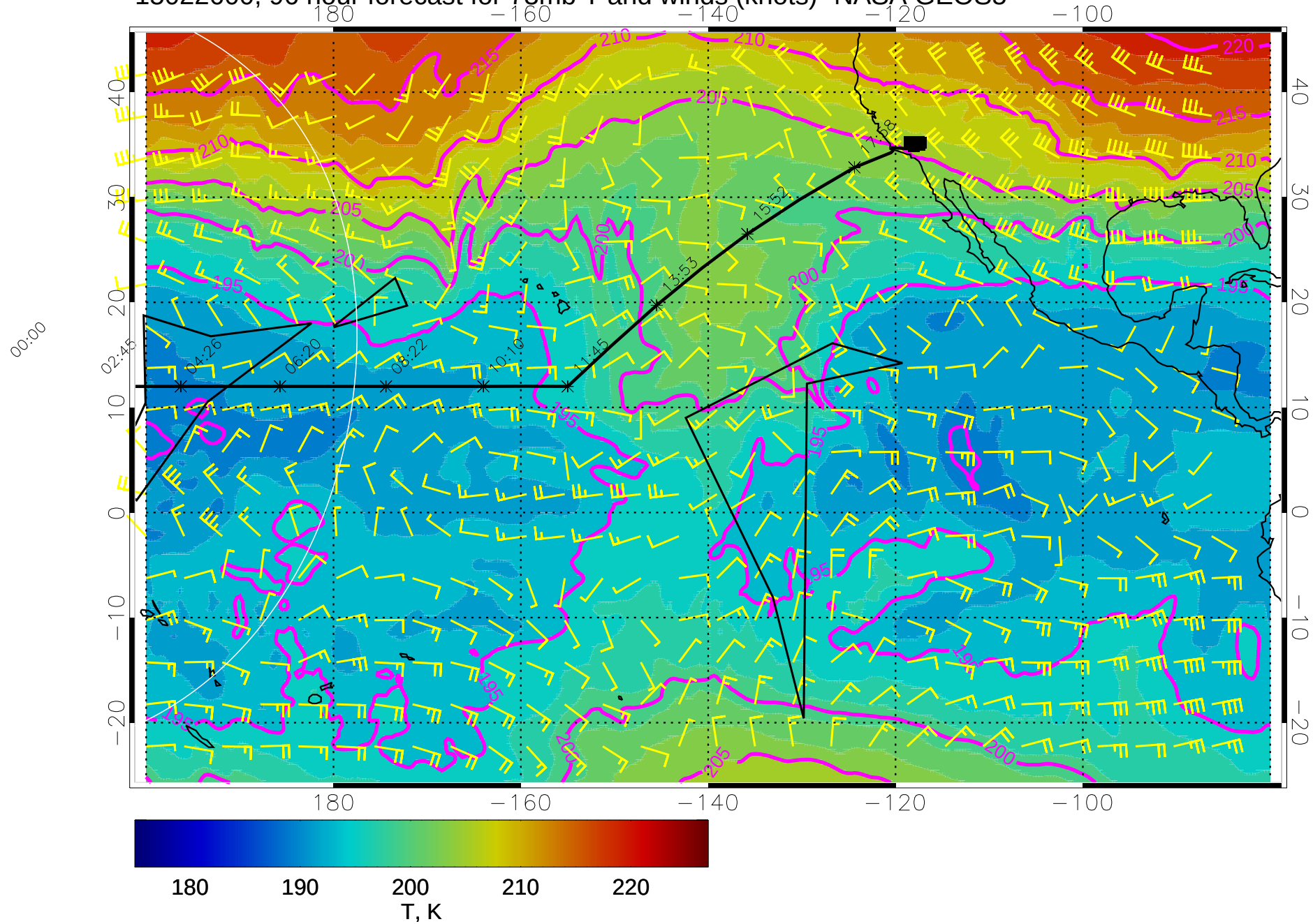
15022600, 96 hour forecast for 73mb T and winds (knots)- NASA GEOS5
