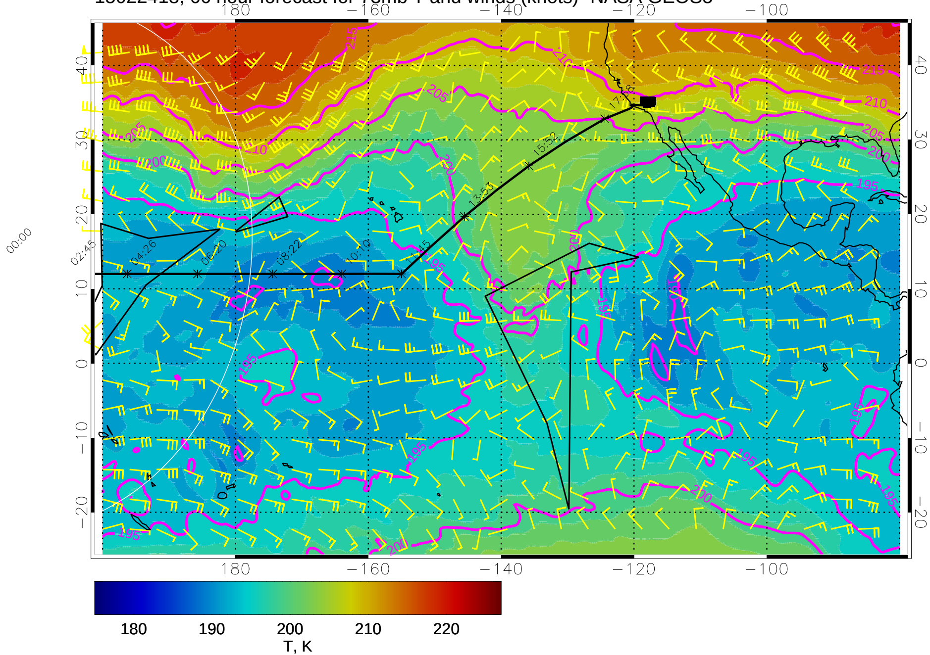
15022418, 66 hour forecast for 73mb T and winds (knots)- NASA GEOS5
