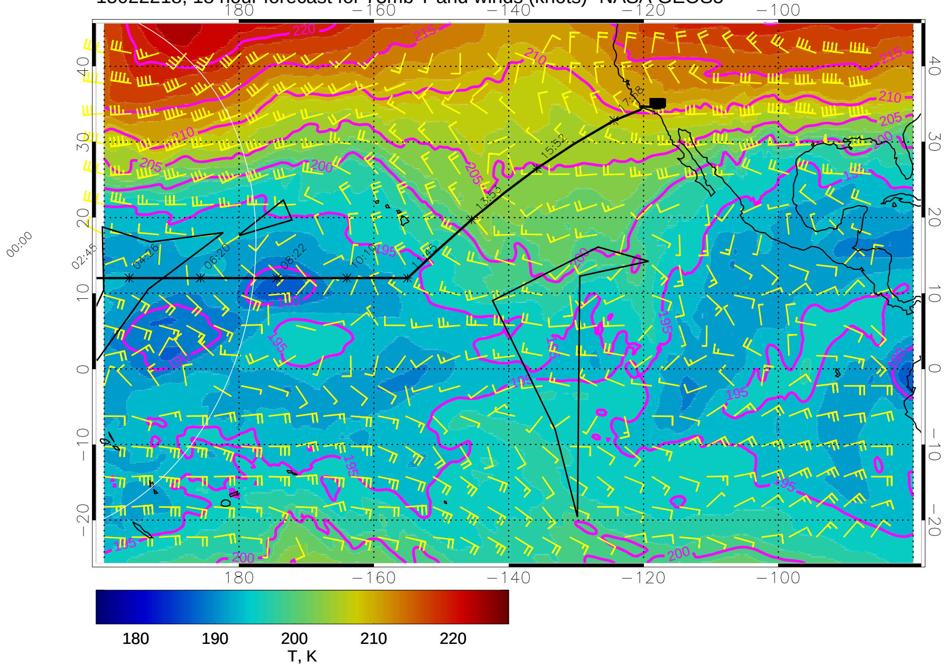
15022218, 18 hour forecast for 73mb T and winds (knots)- NASA GEOS5
