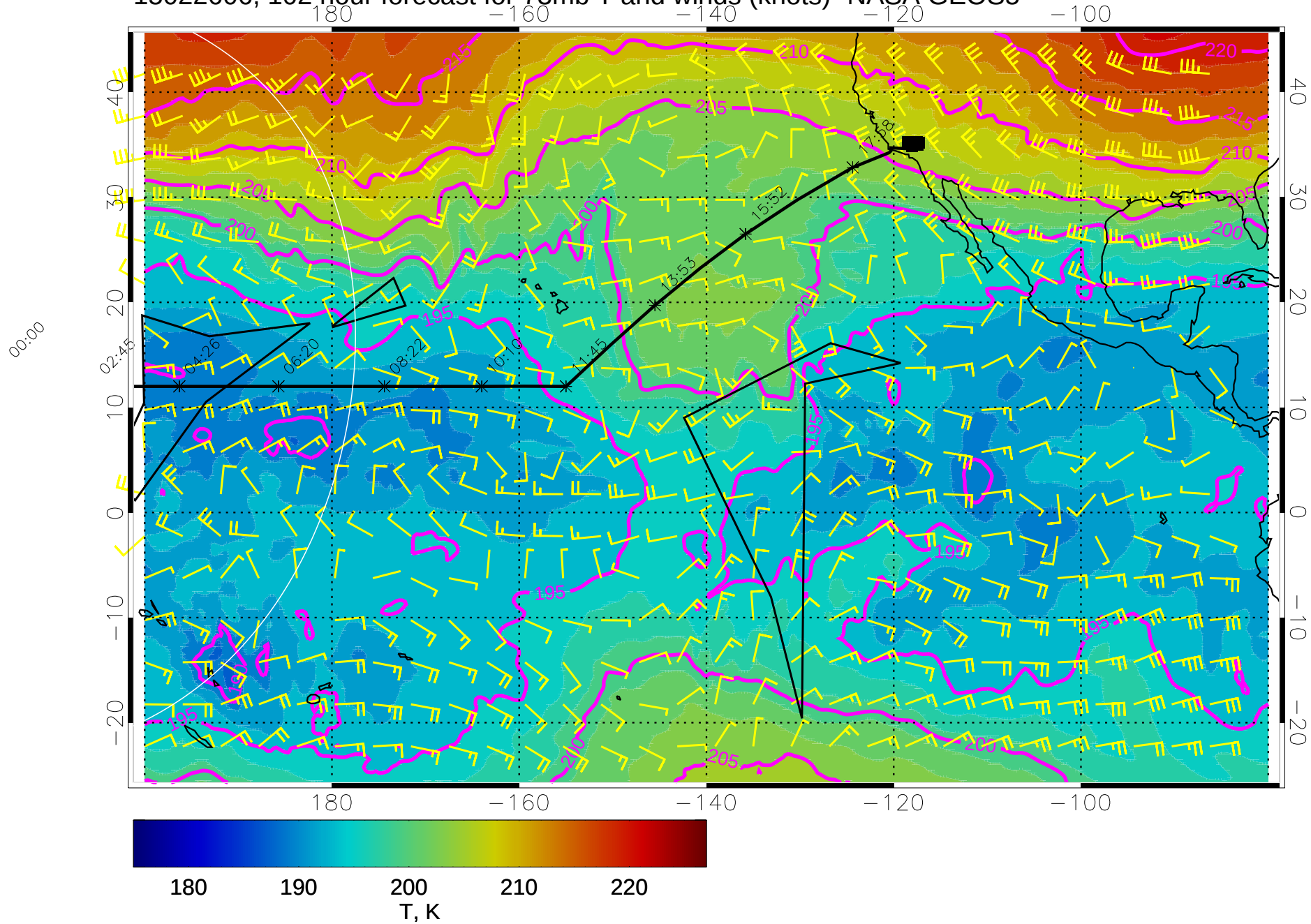
15022606, 102 hour forecast for 73mb T and winds (knots)- NASA GEOS5
