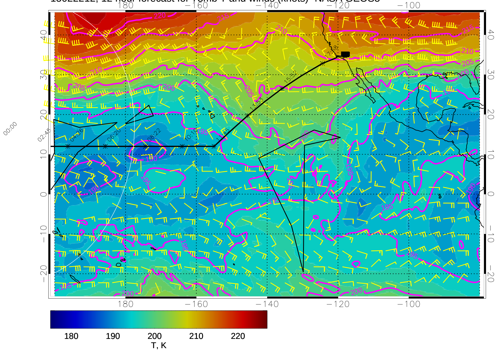
15022212, 12 hour forecast for 73mb T and winds (knots)- NASA GEOS5
