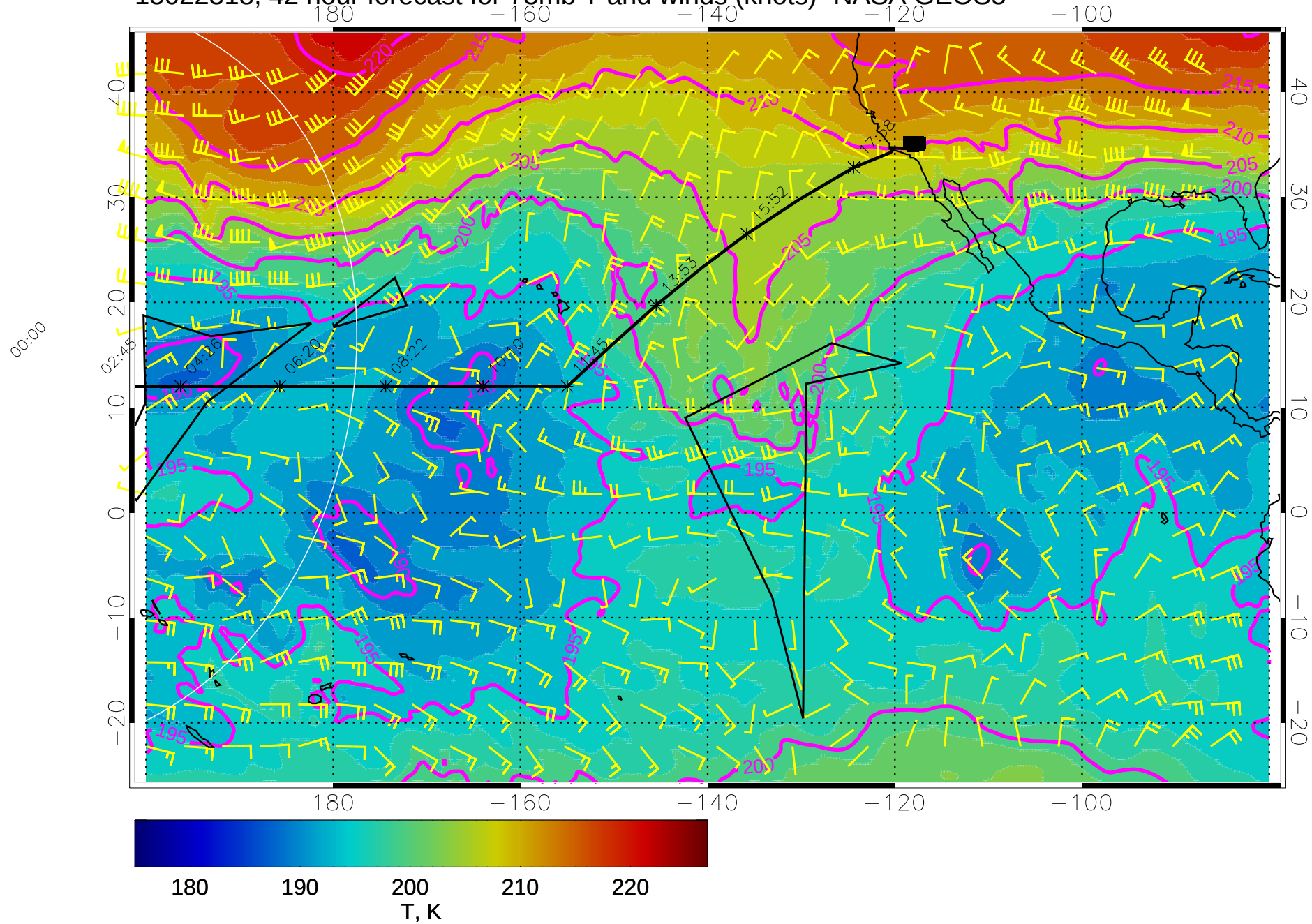
15022318, 42 hour forecast for 73mb T and winds (knots)- NASA GEOS5
