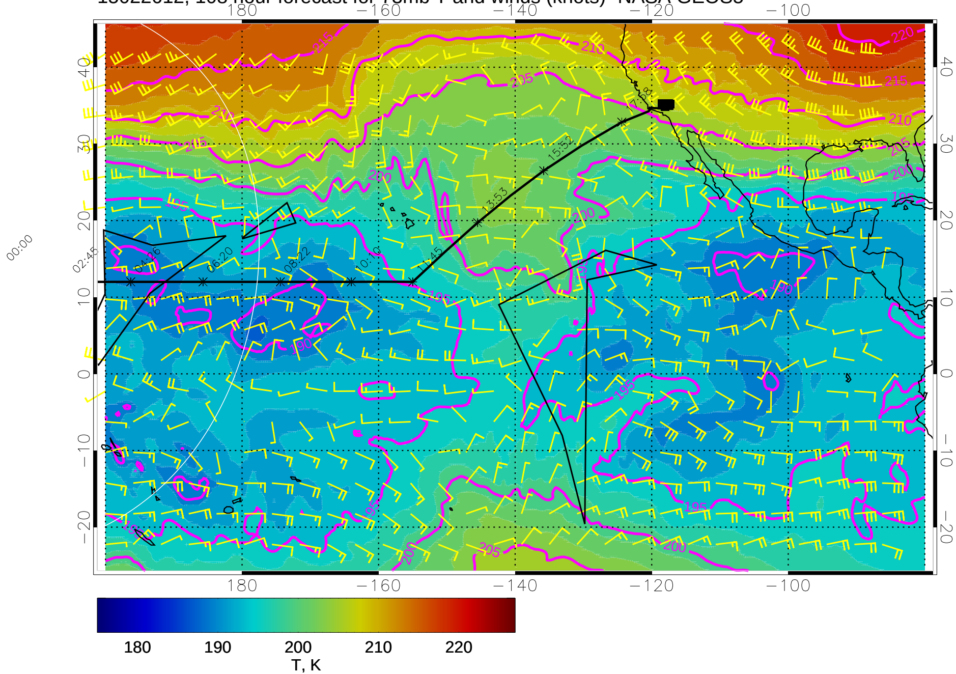
15022612, 108 hour forecast for 73mb T and winds (knots)- NASA GEOS5
