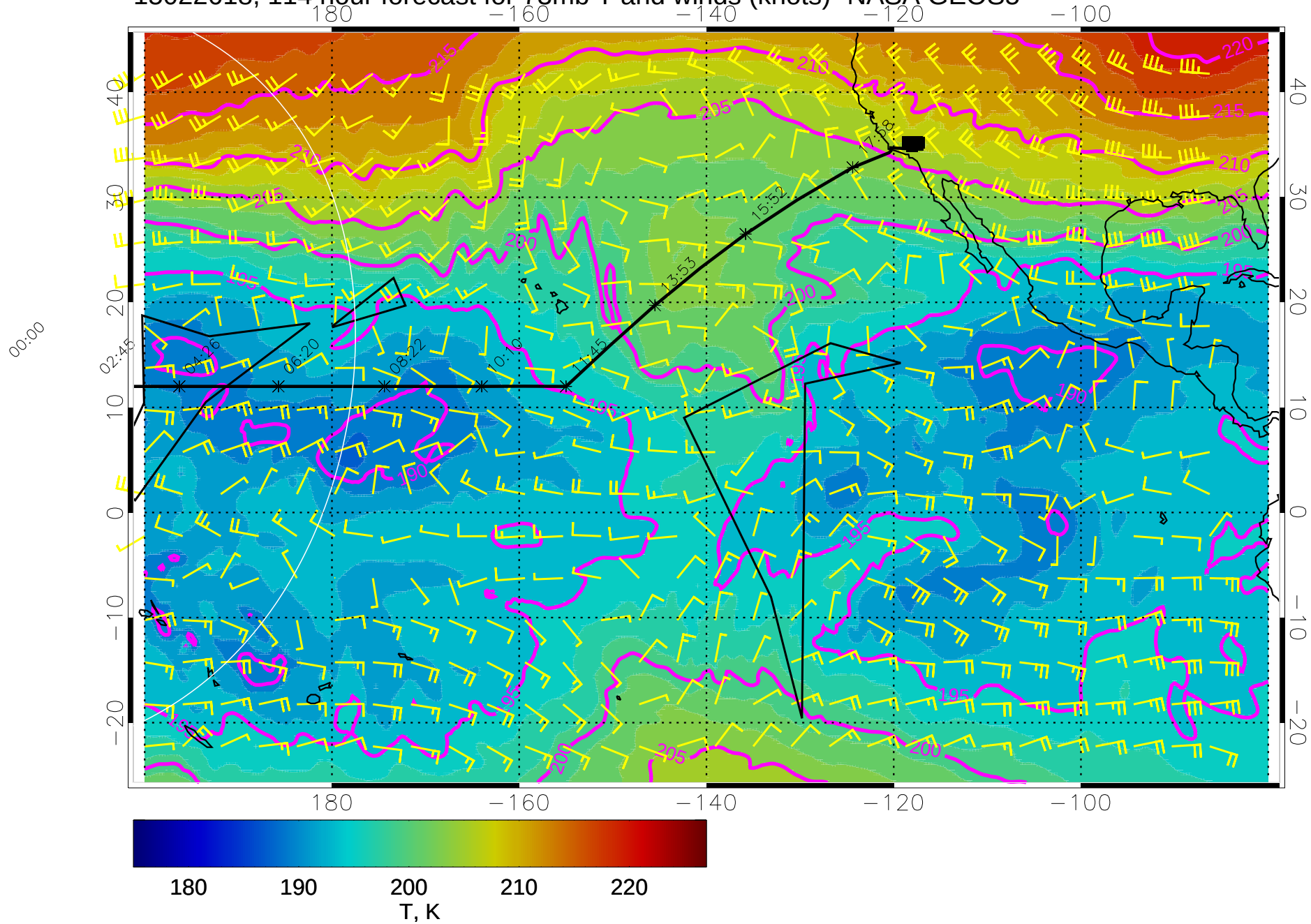
15022618, 114 hour forecast for 73mb T and winds (knots)- NASA GEOS5
