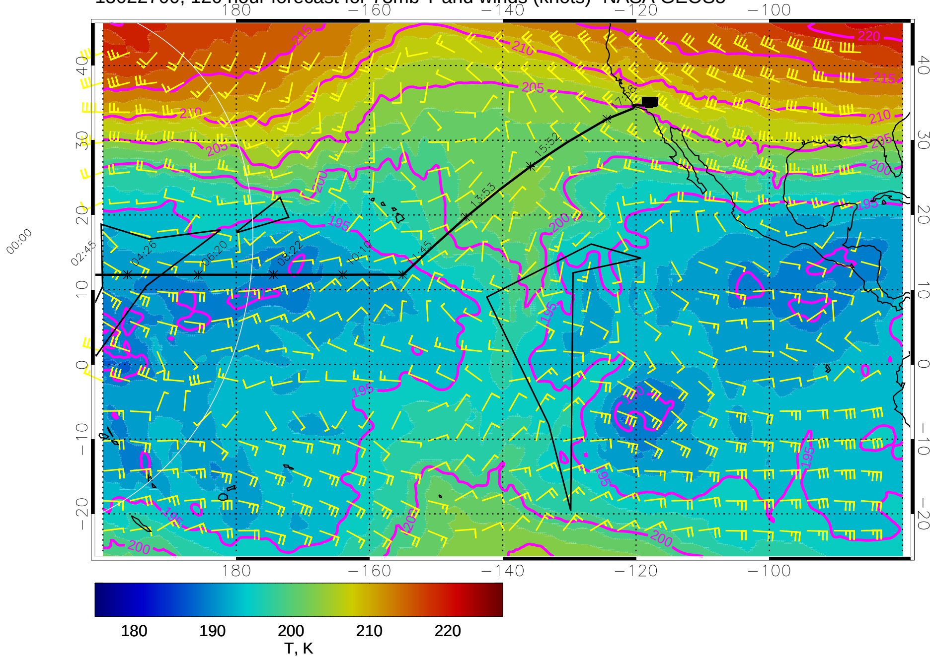
15022700, 120 hour forecast for 73mb T and winds (knots)- NASA GEOS5
