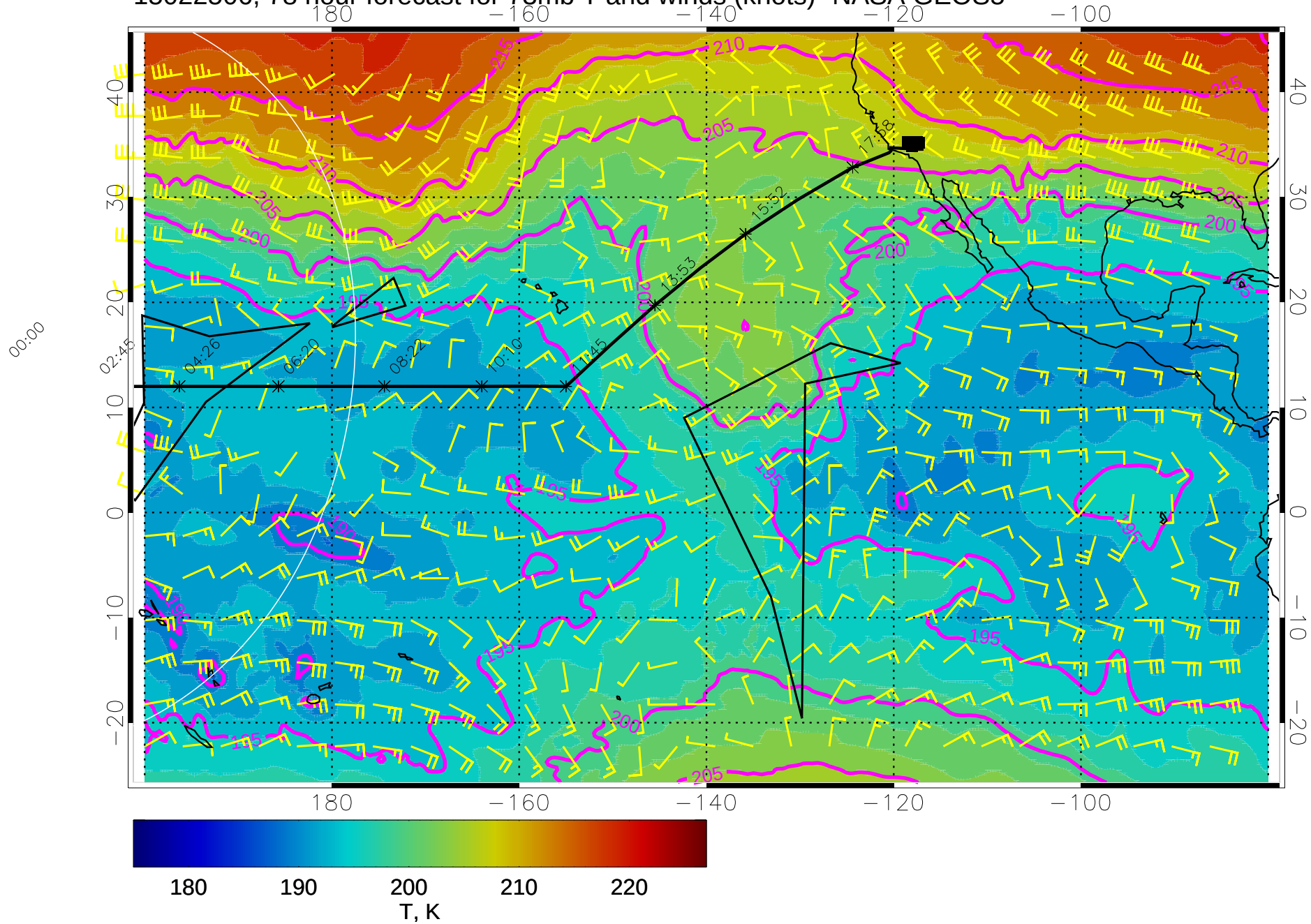
15022506, 78 hour forecast for 73mb T and winds (knots)- NASA GEOS5
