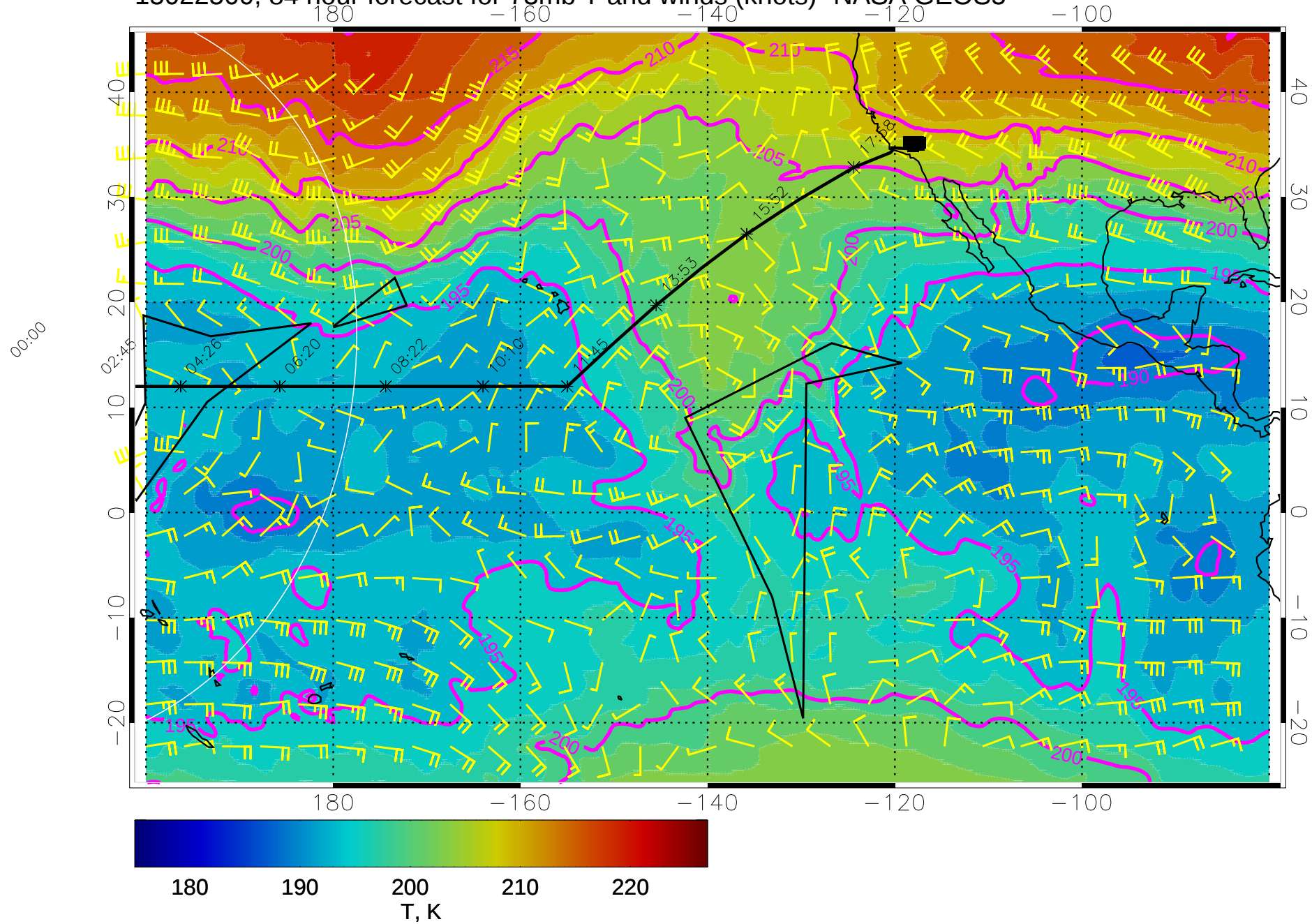
15022500, 84 hour forecast for 73mb T and winds (knots)- NASA GEOS5
