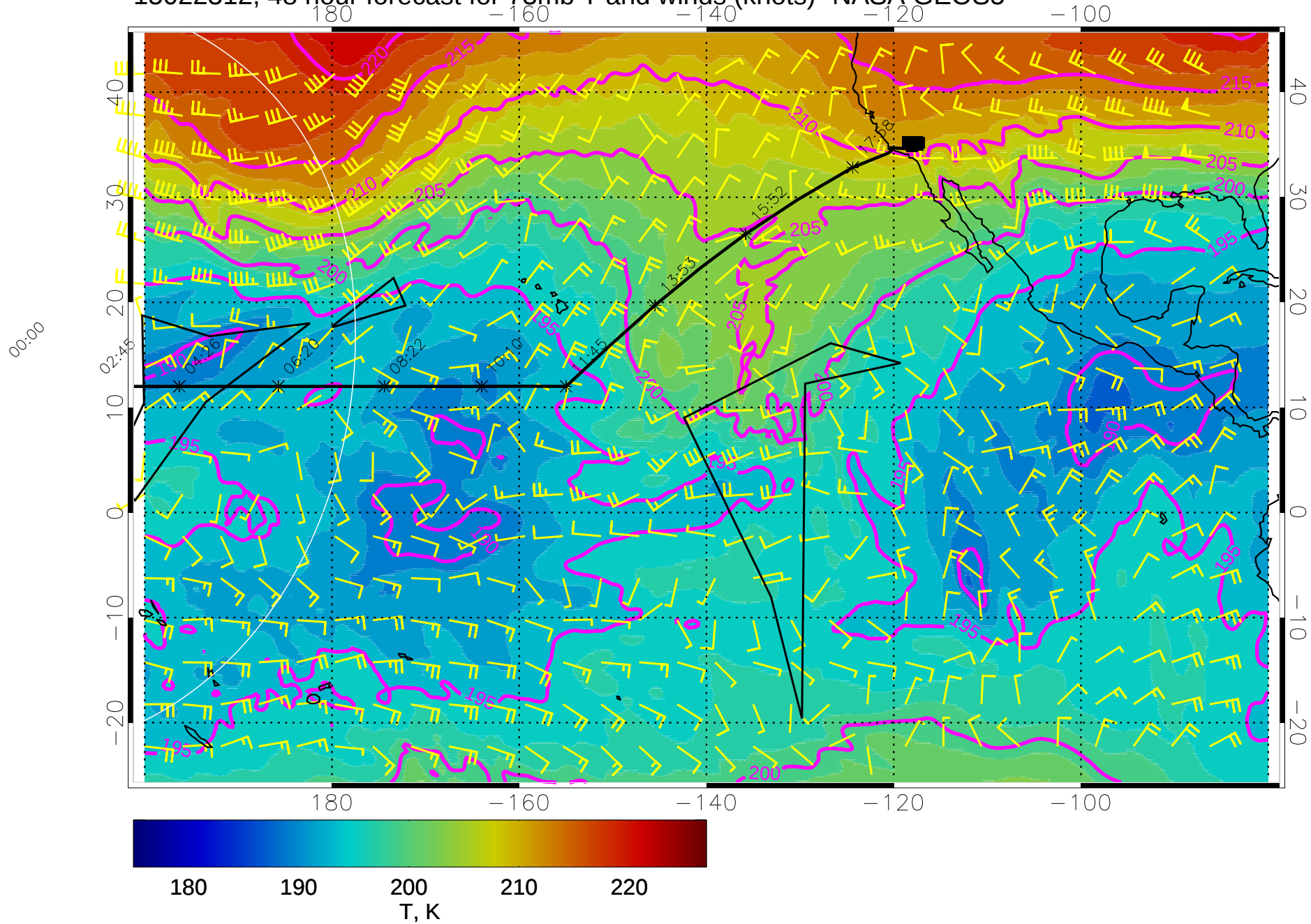
15022312, 48 hour forecast for 73mb T and winds (knots)- NASA GEOS5
