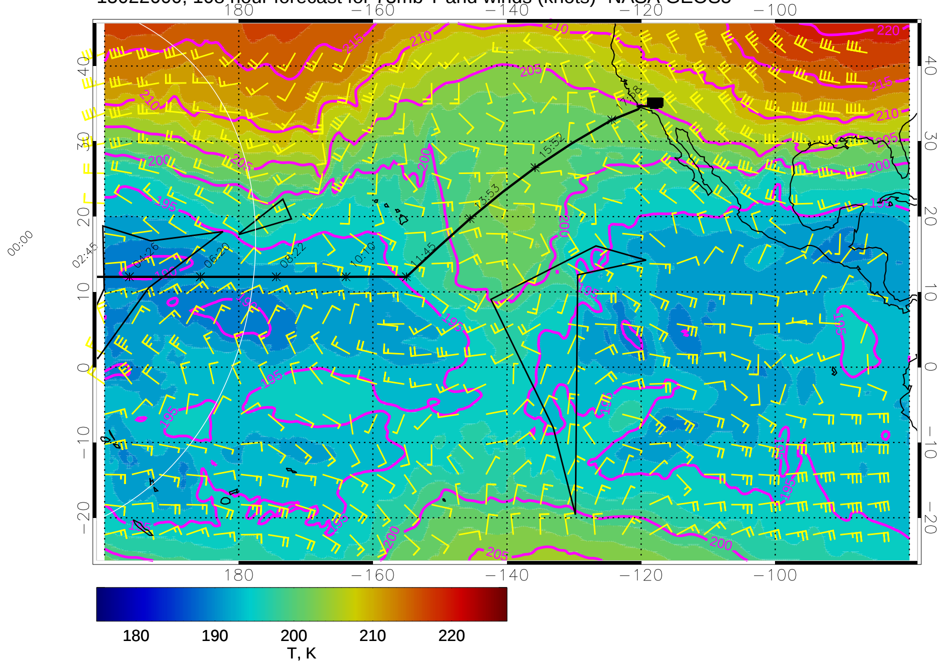
15022600, 108 hour forecast for 73mb T and winds (knots)- NASA GEOS5
