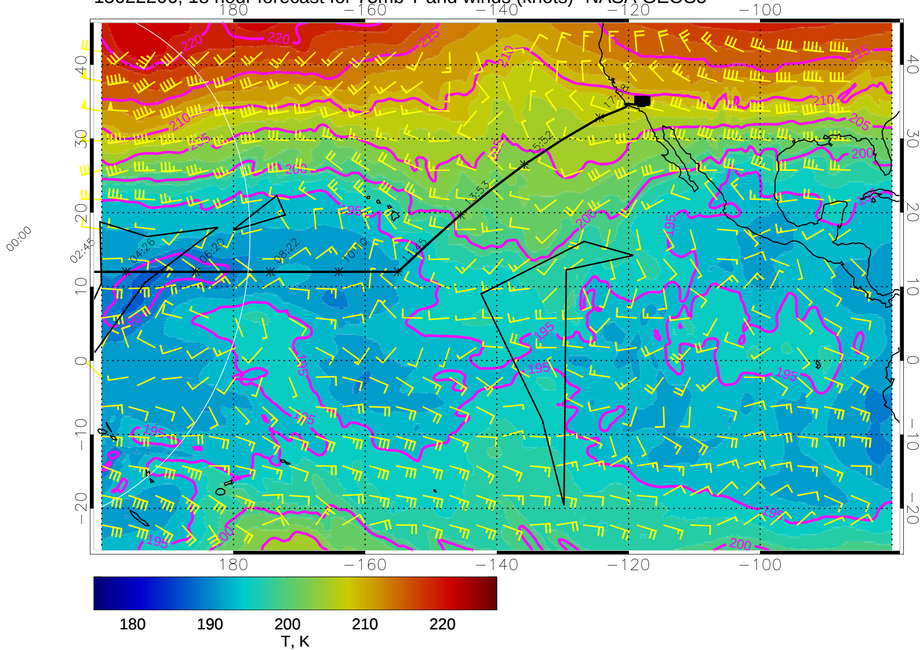
15022206, 18 hour forecast for 73mb T and winds (knots)- NASA GEOS5
