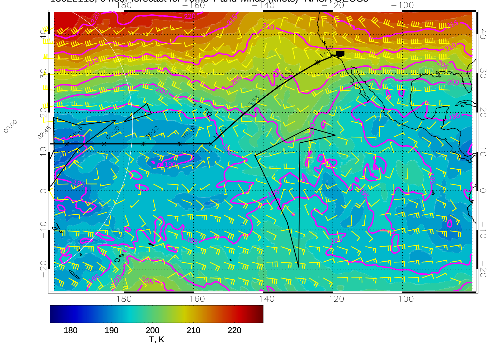
15022118, 6 hour forecast for 73mb T and winds (knots)- NASA GEOS5
