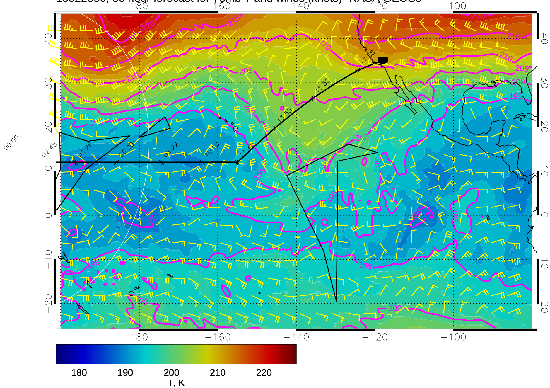
15022300, 36 hour forecast for 73mb T and winds (knots)- NASA GEOS5
