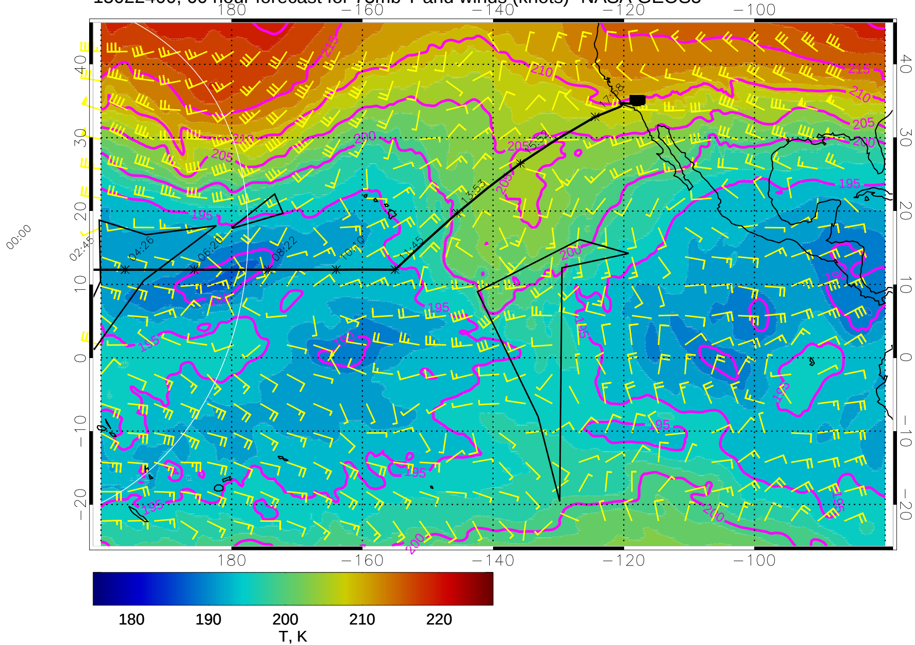
15022400, 60 hour forecast for 73mb T and winds (knots)- NASA GEOS5
