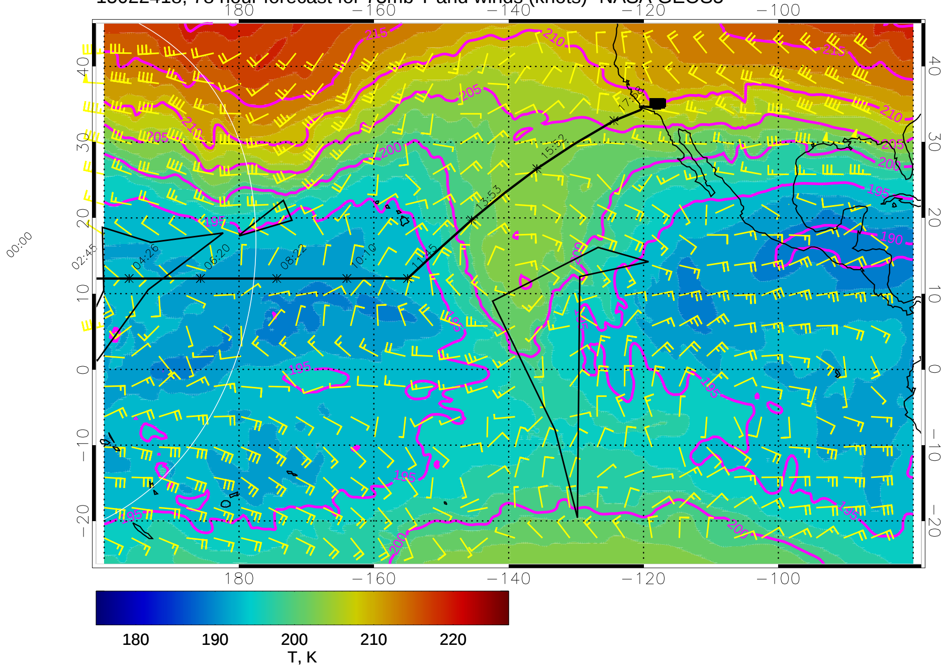
15022418, 78 hour forecast for 73mb T and winds (knots)- NASA GEOS5
