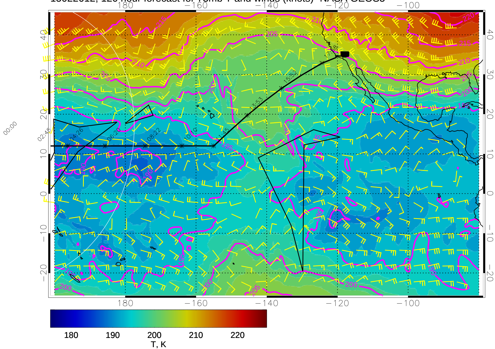
15022612, 120 hour forecast for 73mb T and winds (knots)- NASA GEOS5
