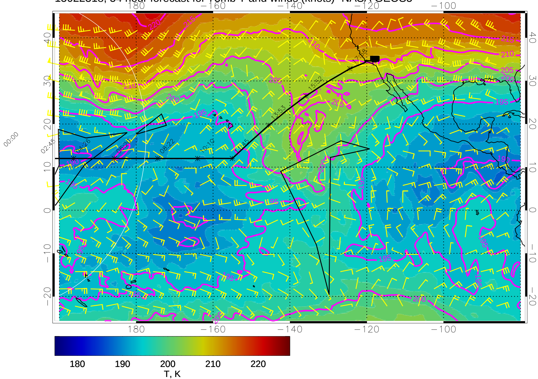
15022318, 54 hour forecast for 73mb T and winds (knots)- NASA GEOS5
