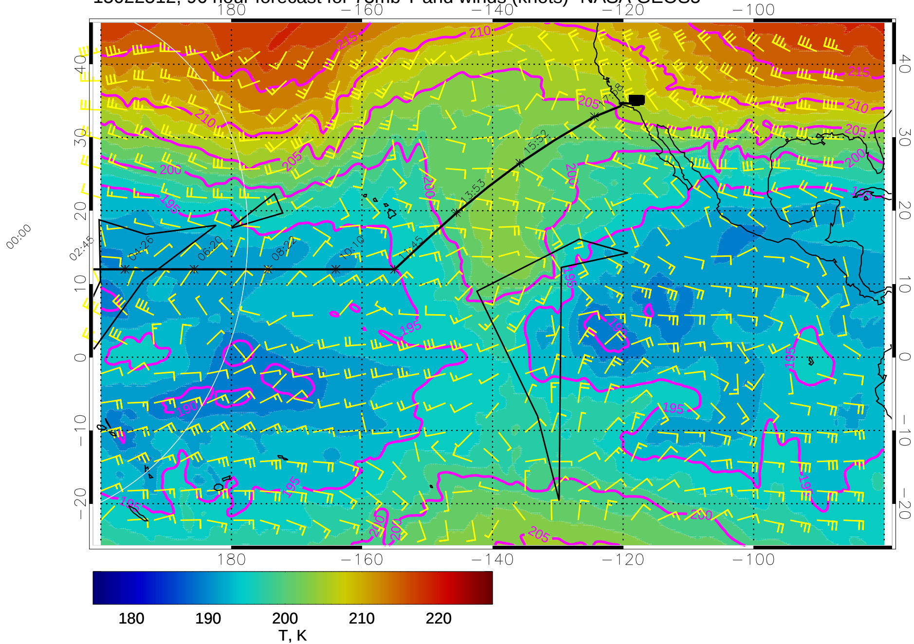
15022512, 96 hour forecast for 73mb T and winds (knots)- NASA GEOS5
