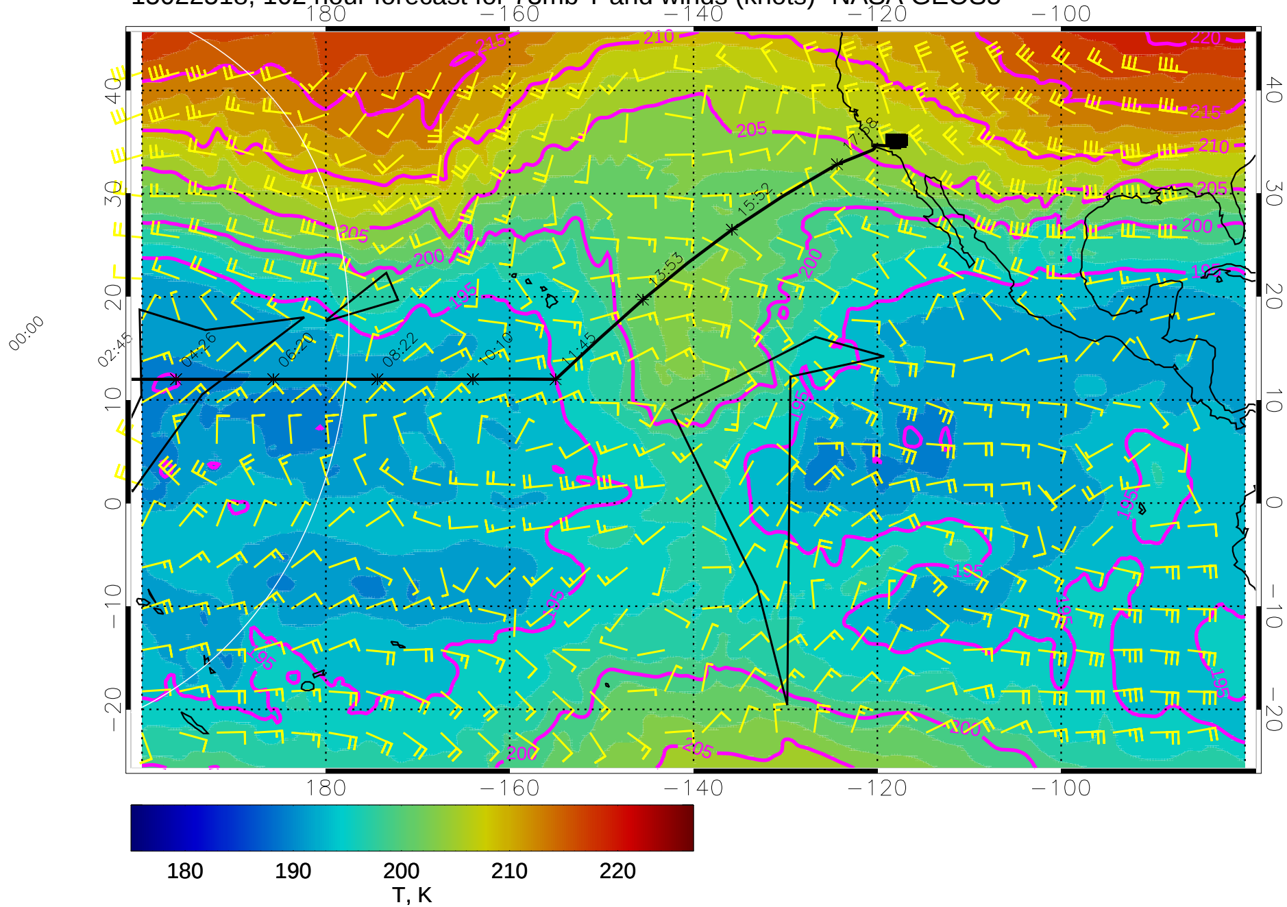
15022518, 102 hour forecast for 73mb T and winds (knots)- NASA GEOS5
