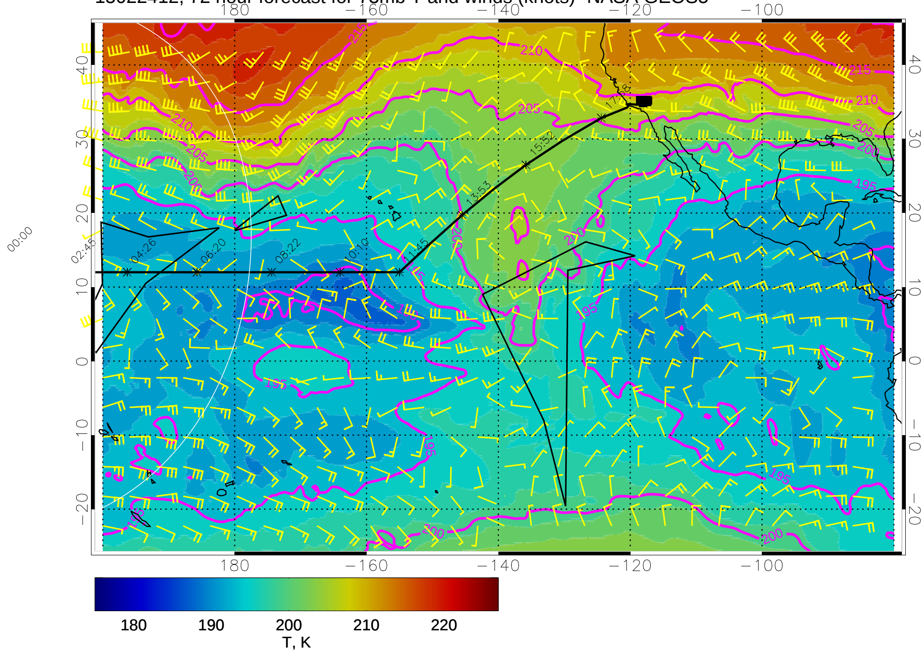
15022412, 72 hour forecast for 73mb T and winds (knots)- NASA GEOS5
