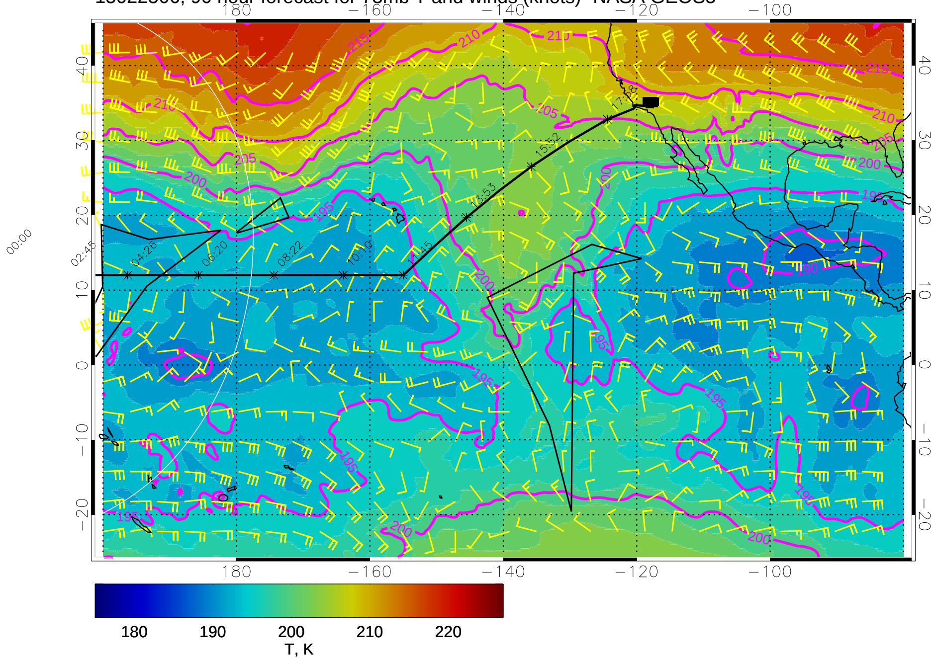
15022506, 90 hour forecast for 73mb T and winds (knots)- NASA GEOS5
