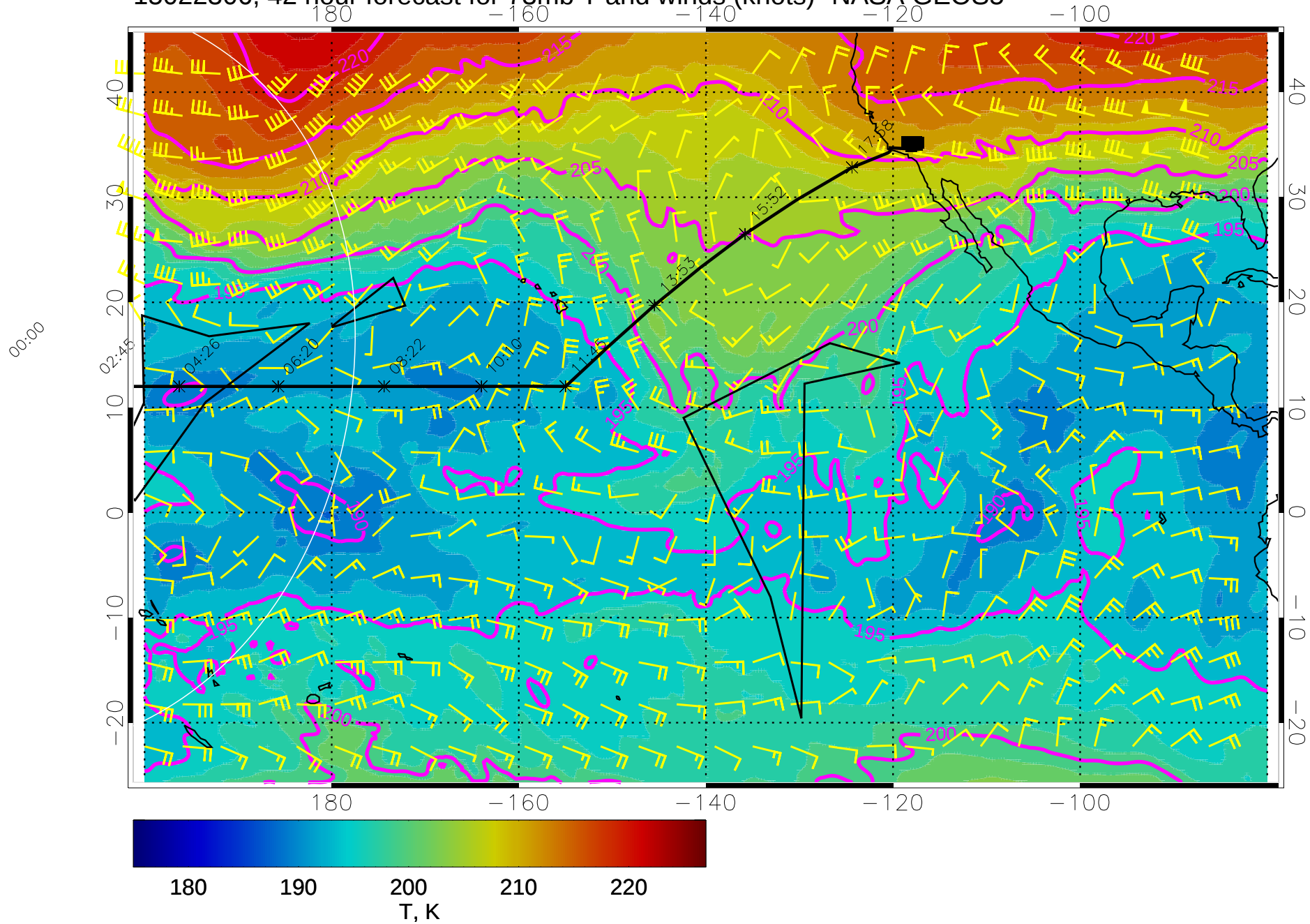
15022306, 42 hour forecast for 73mb T and winds (knots)- NASA GEOS5
