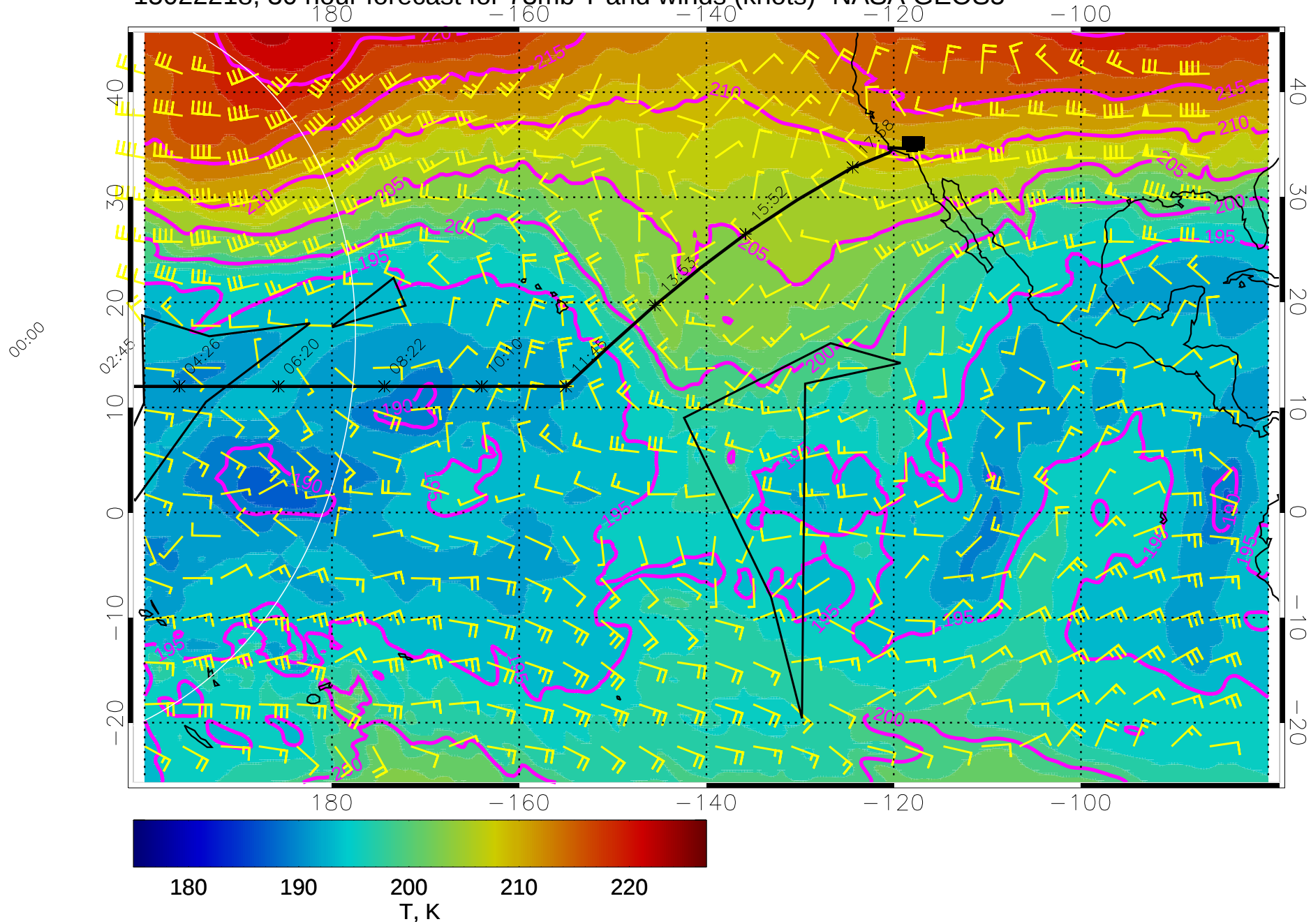
15022218, 30 hour forecast for 73mb T and winds (knots)- NASA GEOS5
