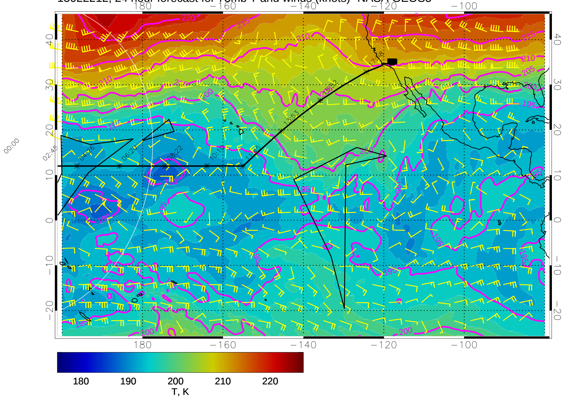
15022212, 24 hour forecast for 73mb T and winds (knots)- NASA GEOS5
