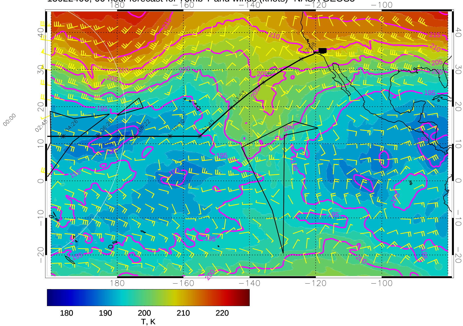
15022406, 66 hour forecast for 73mb T and winds (knots)- NASA GEOS5
