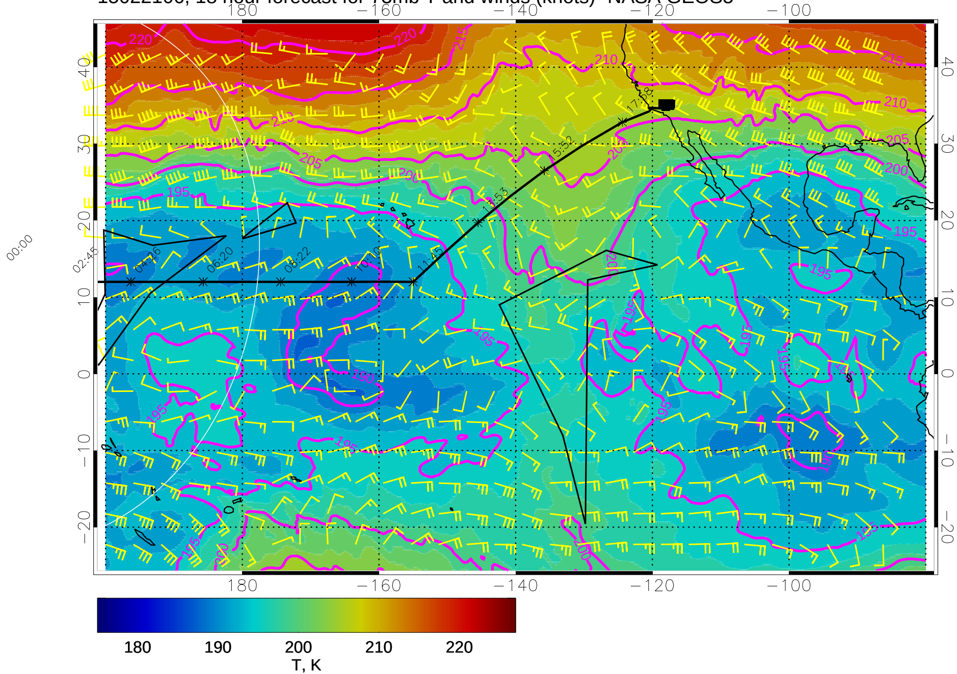
15022106, 18 hour forecast for 73mb T and winds (knots)- NASA GEOS5
