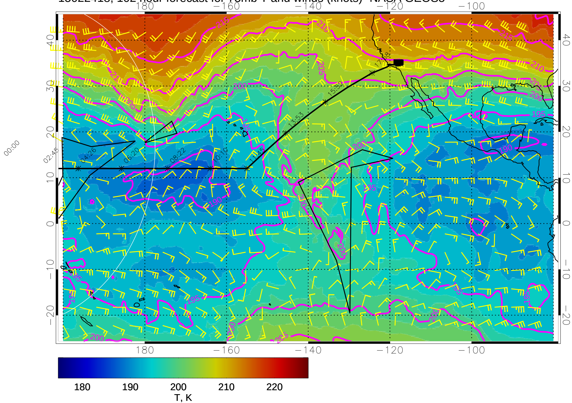
15022418, 102 hour forecast for 73mb T and winds (knots)- NASA GEOS5
