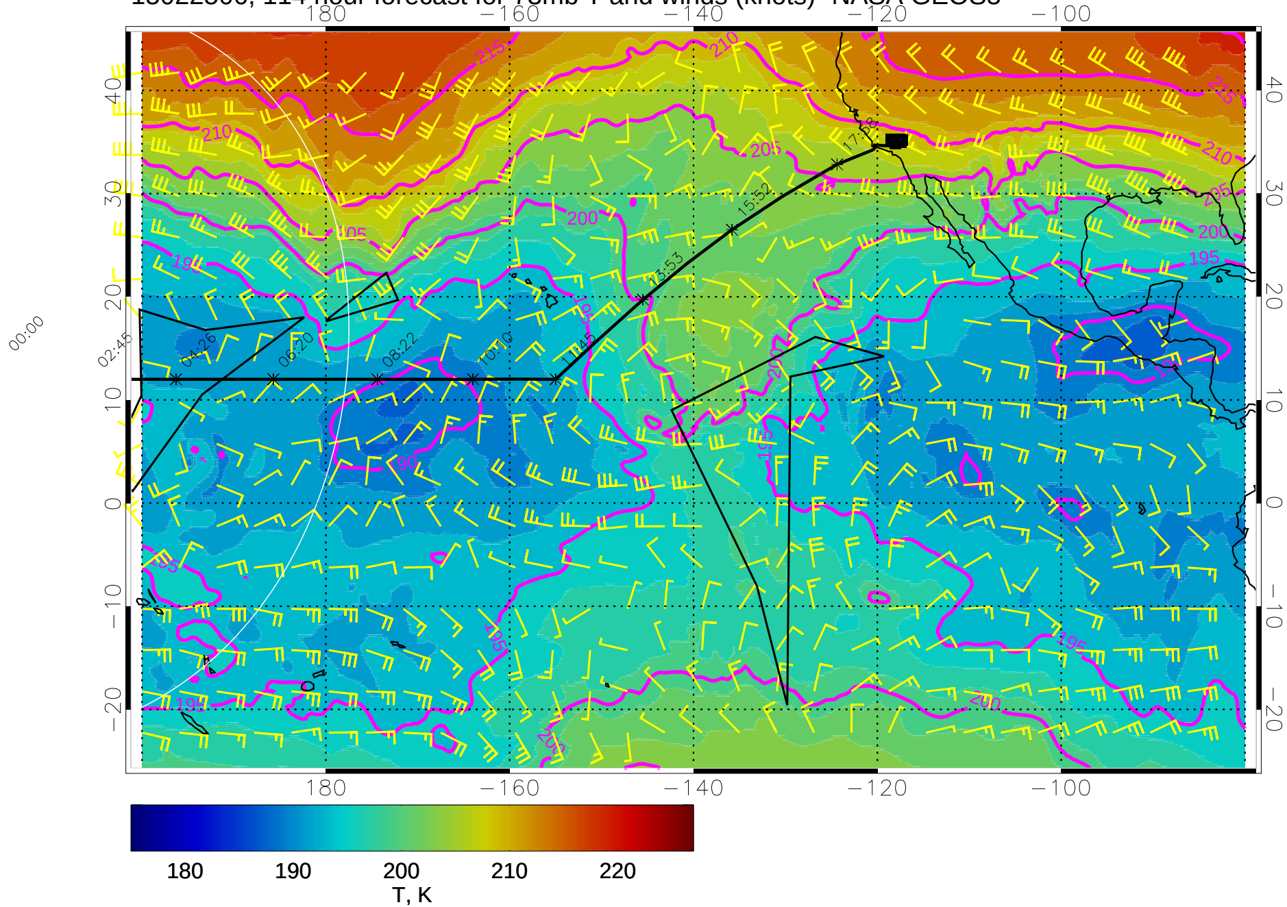
15022506, 114 hour forecast for 73mb T and winds (knots)- NASA GEOS5
