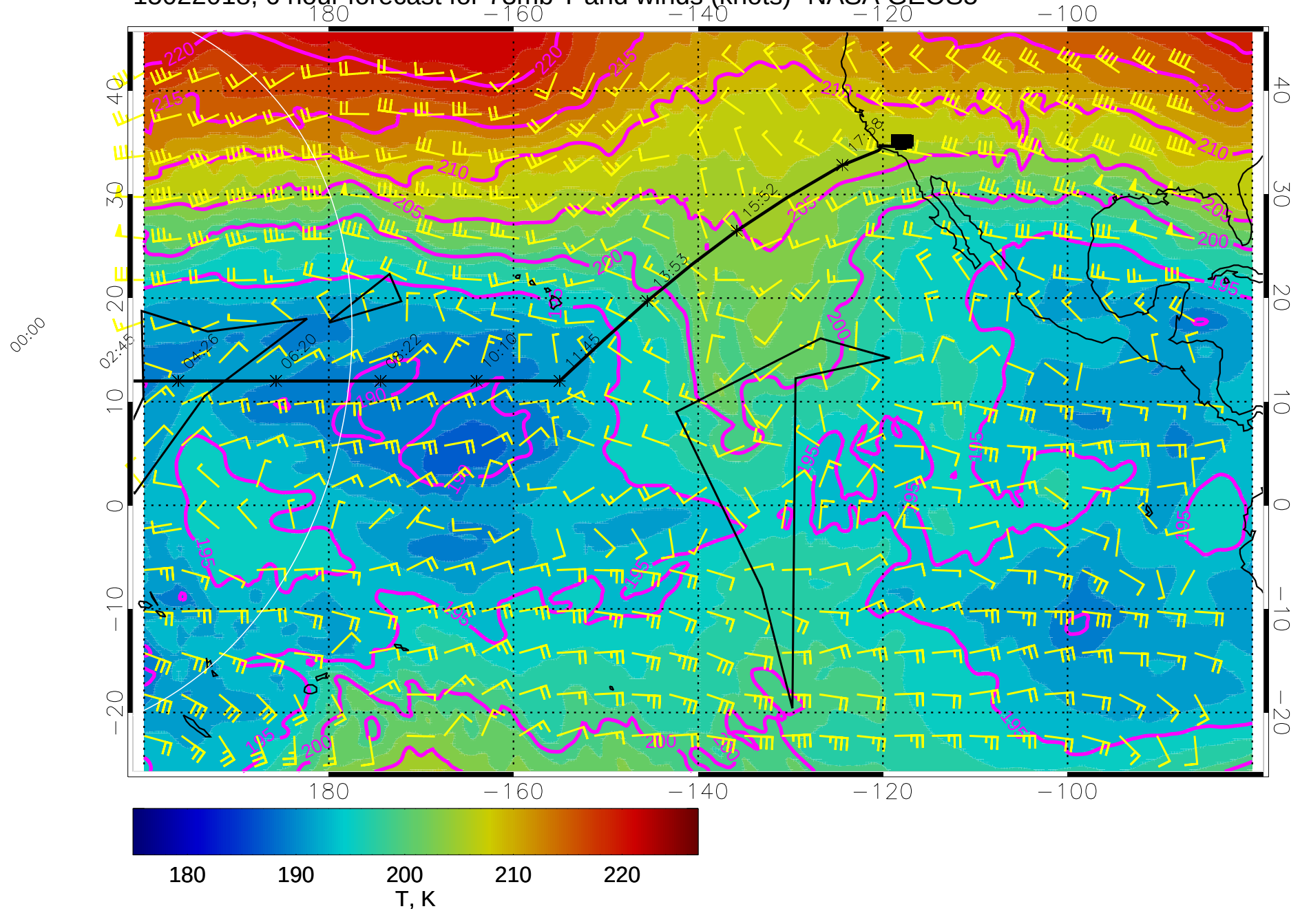
15022018, 6 hour forecast for 73mb T and winds (knots)- NASA GEOS5
