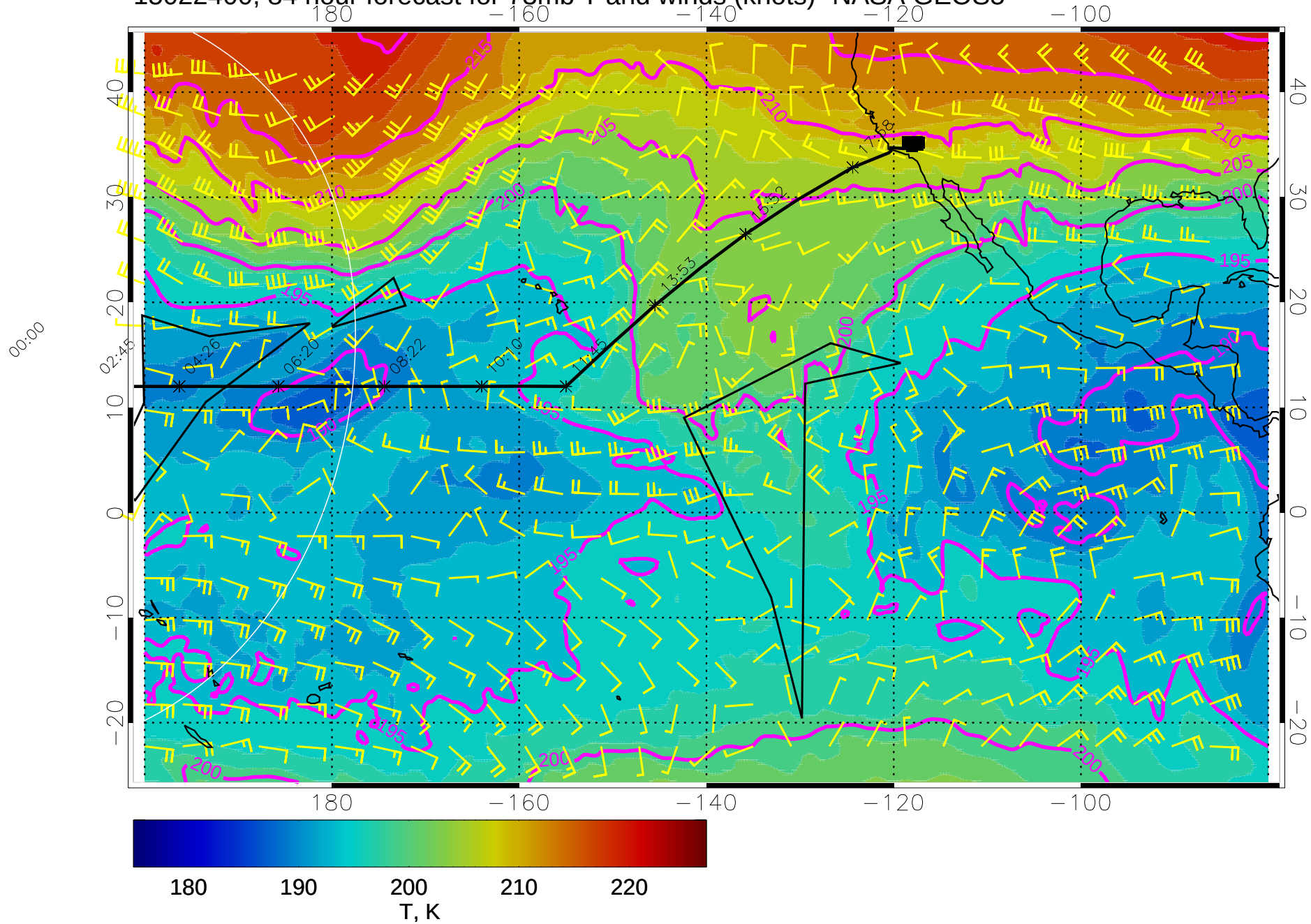
15022400, 84 hour forecast for 73mb T and winds (knots)- NASA GEOS5
