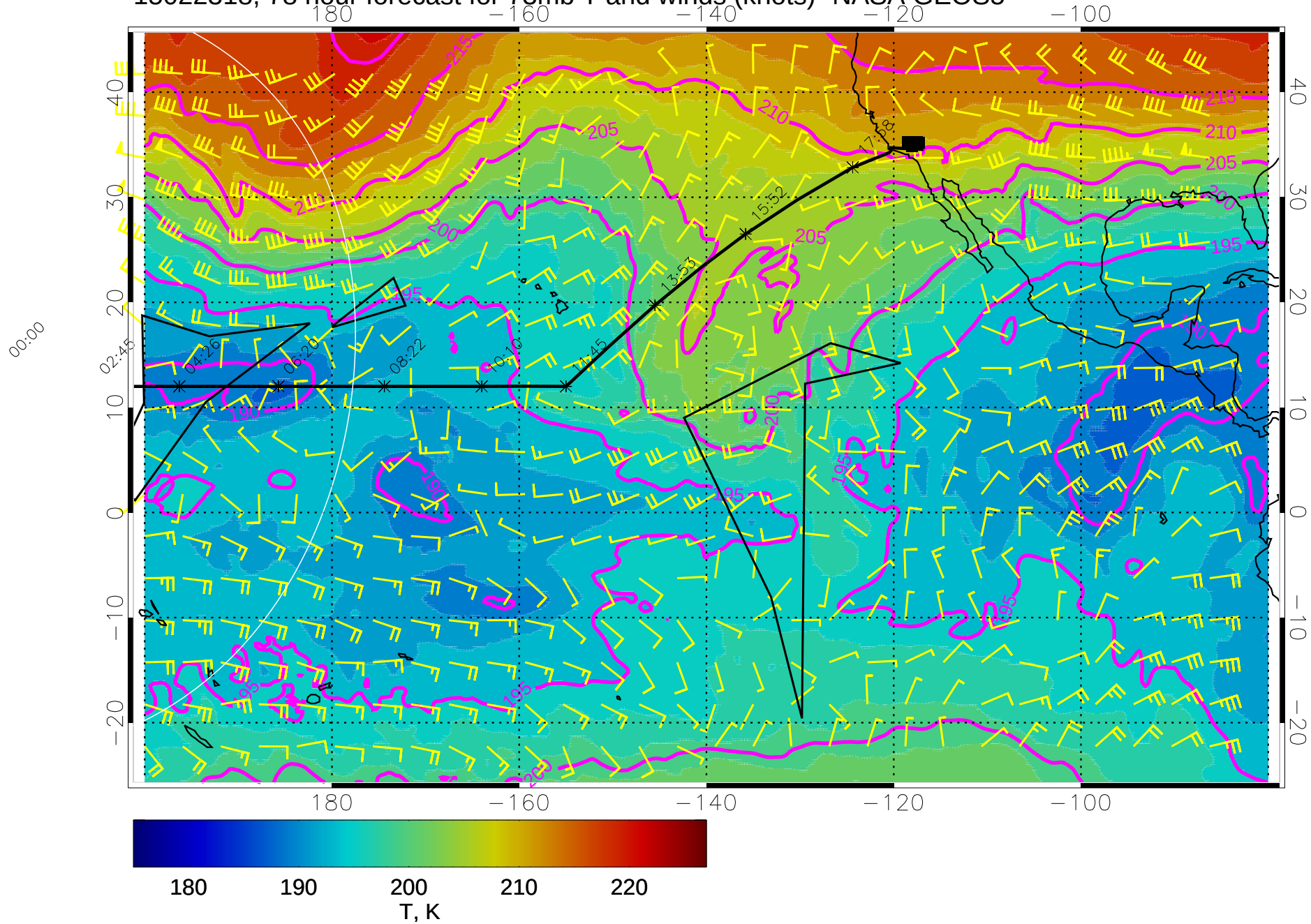
15022318, 78 hour forecast for 73mb T and winds (knots)- NASA GEOS5
