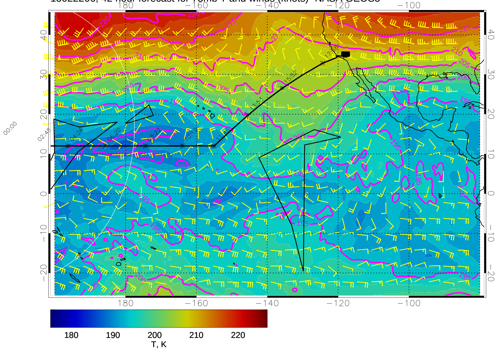
15022206, 42 hour forecast for 73mb T and winds (knots)- NASA GEOS5
