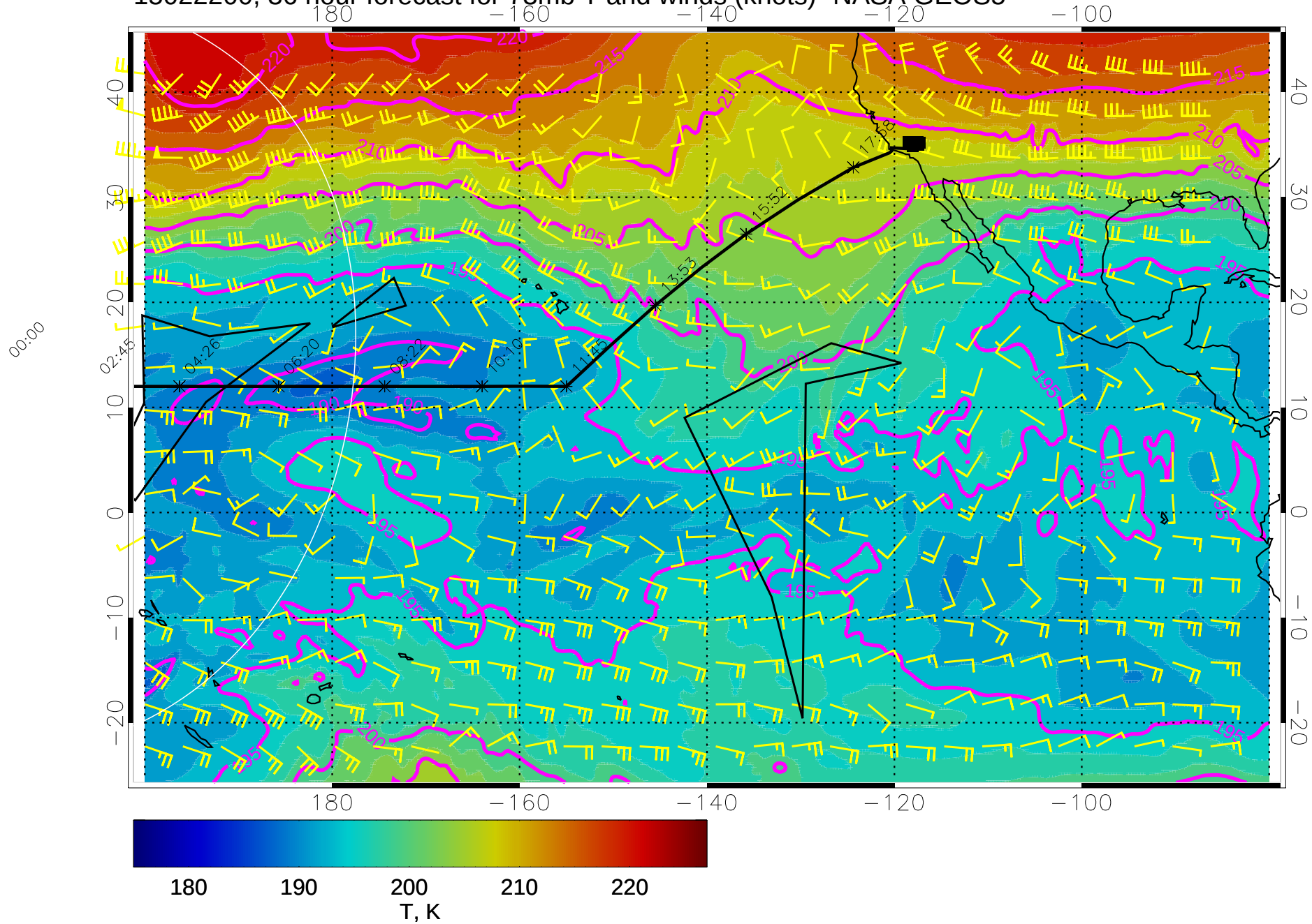
15022200, 36 hour forecast for 73mb T and winds (knots)- NASA GEOS5
