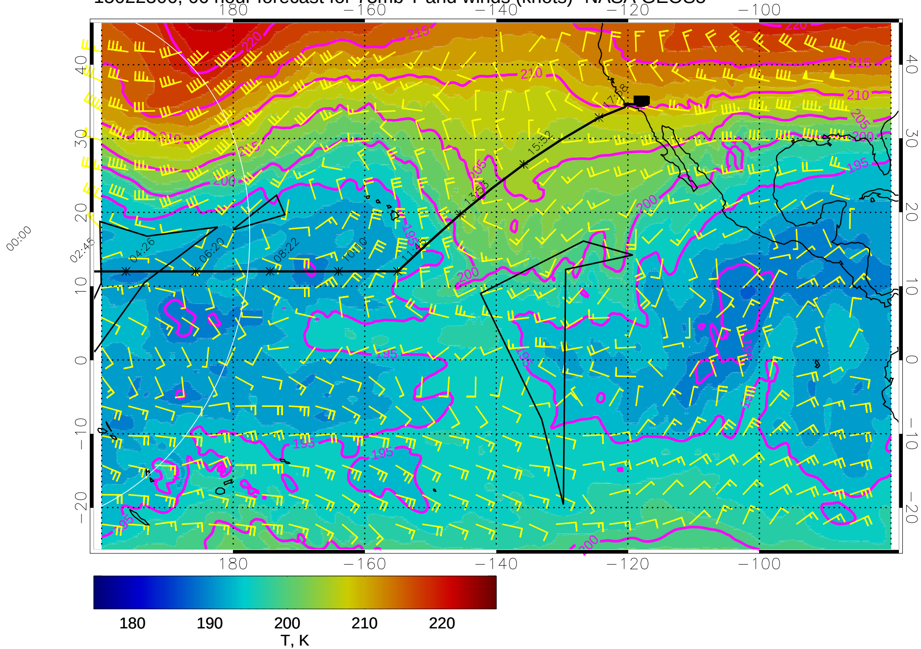
15022306, 66 hour forecast for 73mb T and winds (knots)- NASA GEOS5
