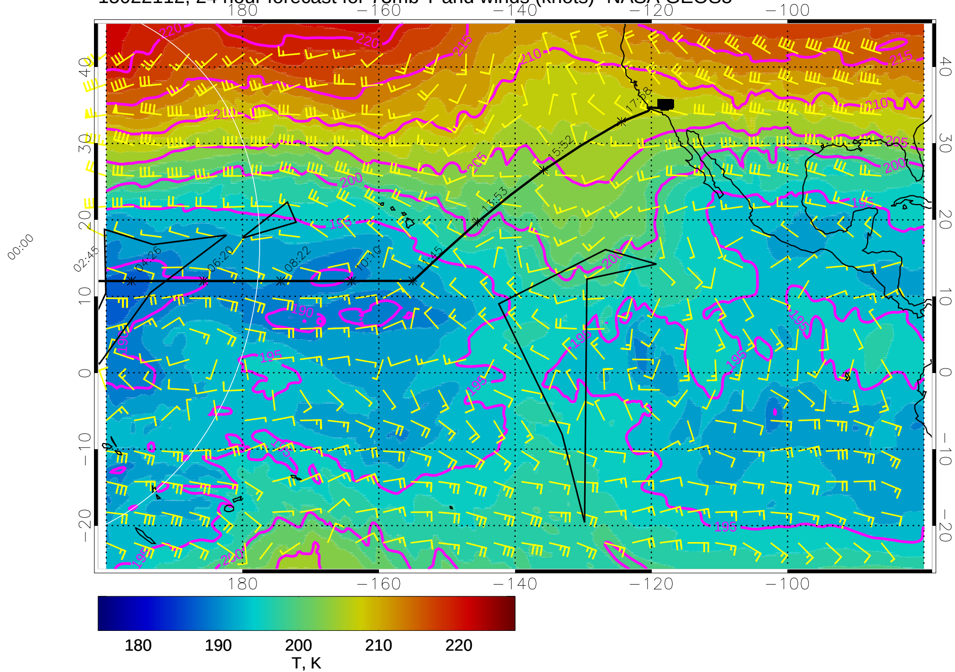
15022112, 24 hour forecast for 73mb T and winds (knots)- NASA GEOS5
