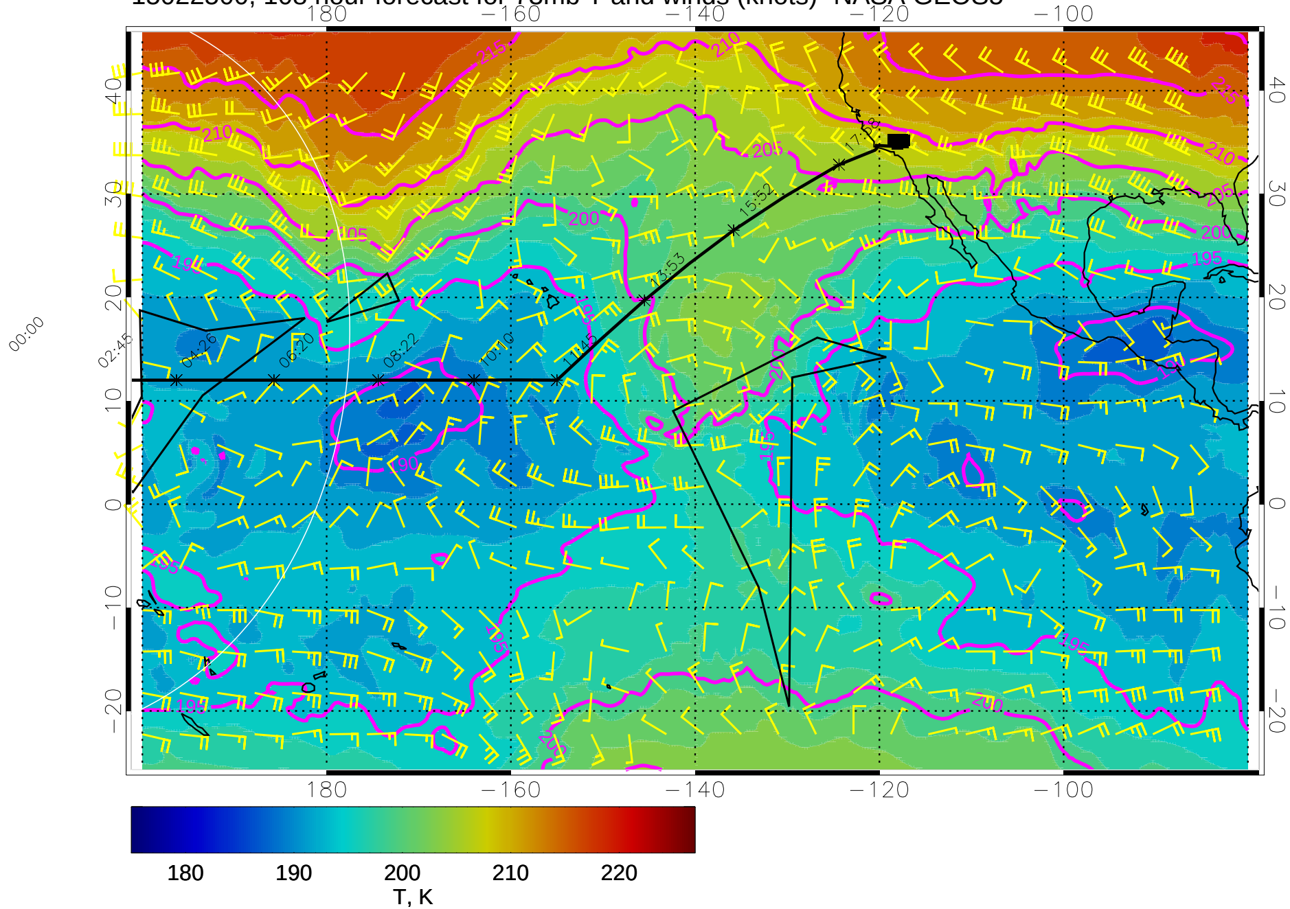
15022500, 108 hour forecast for 73mb T and winds (knots)- NASA GEOS5
