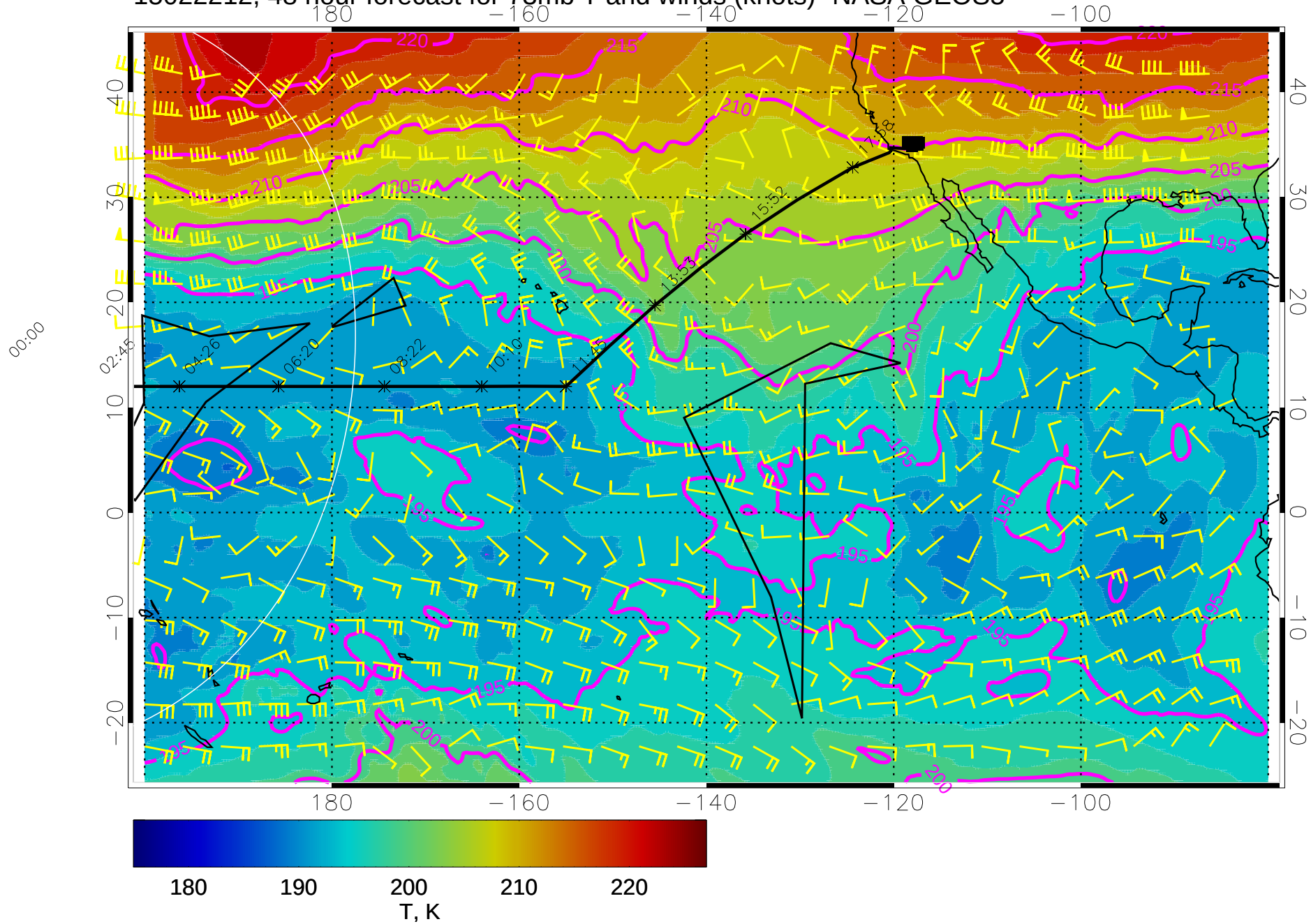
15022212, 48 hour forecast for 73mb T and winds (knots)- NASA GEOS5
