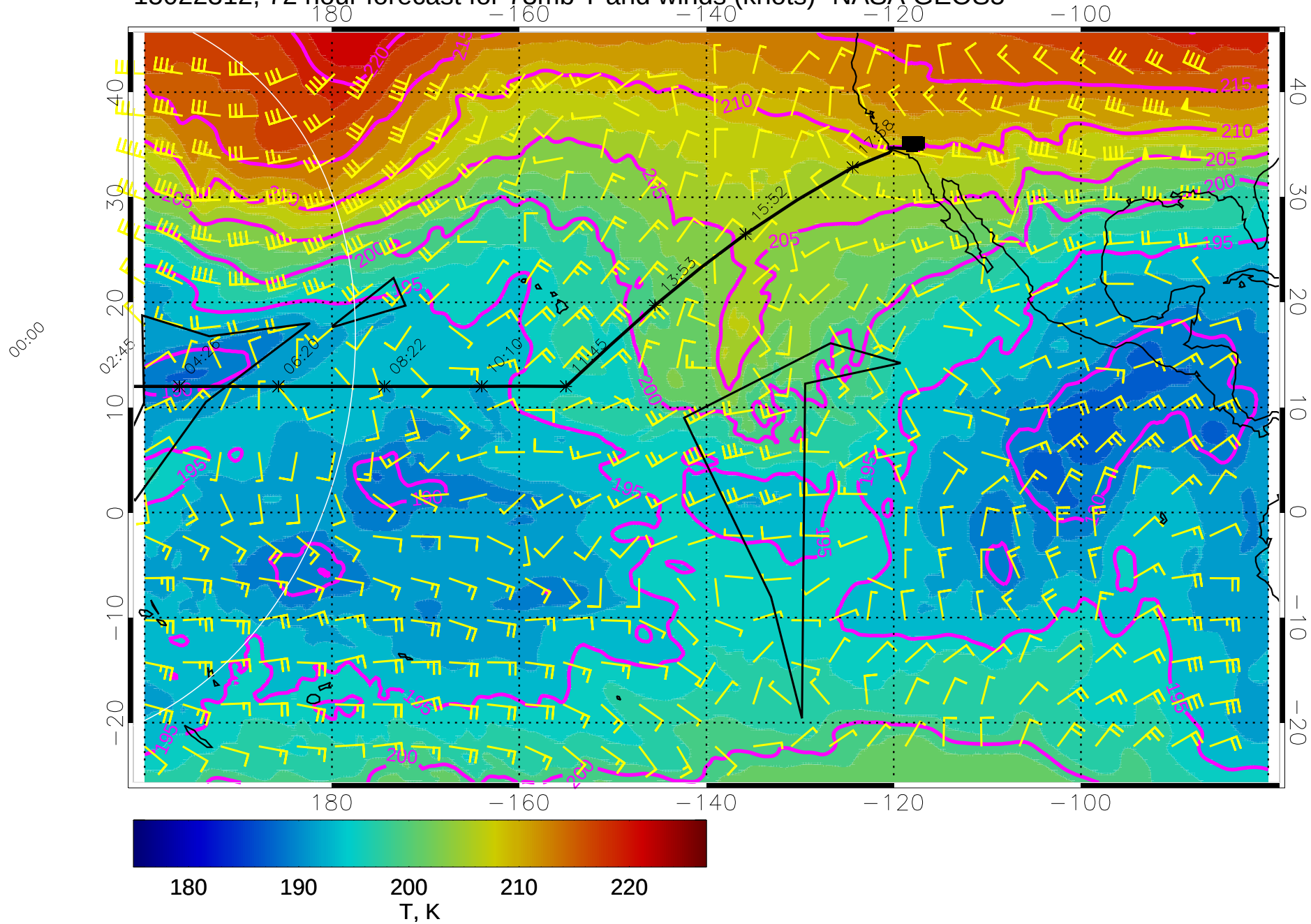
15022312, 72 hour forecast for 73mb T and winds (knots)- NASA GEOS5
