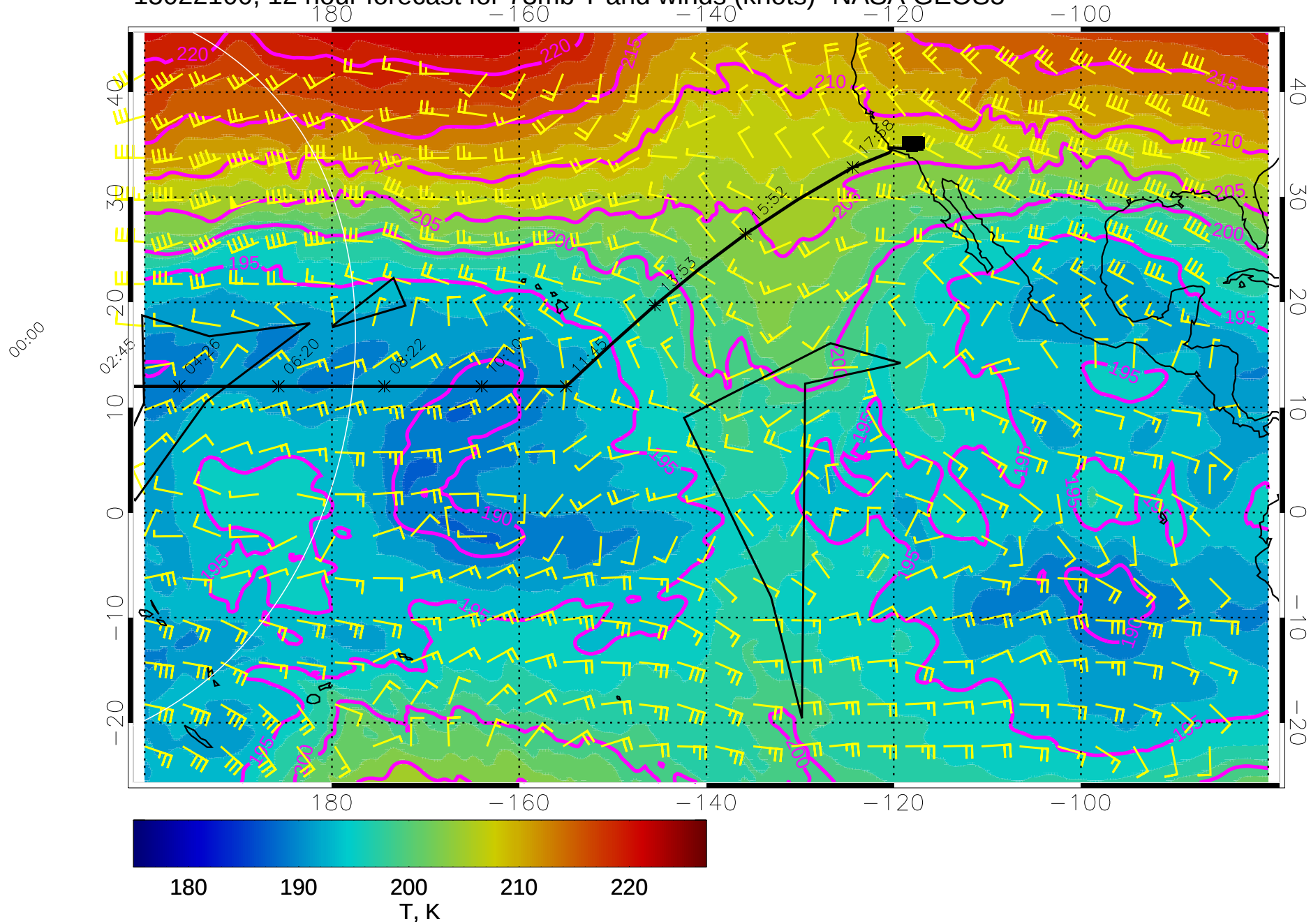
15022100, 12 hour forecast for 73mb T and winds (knots)- NASA GEOS5
