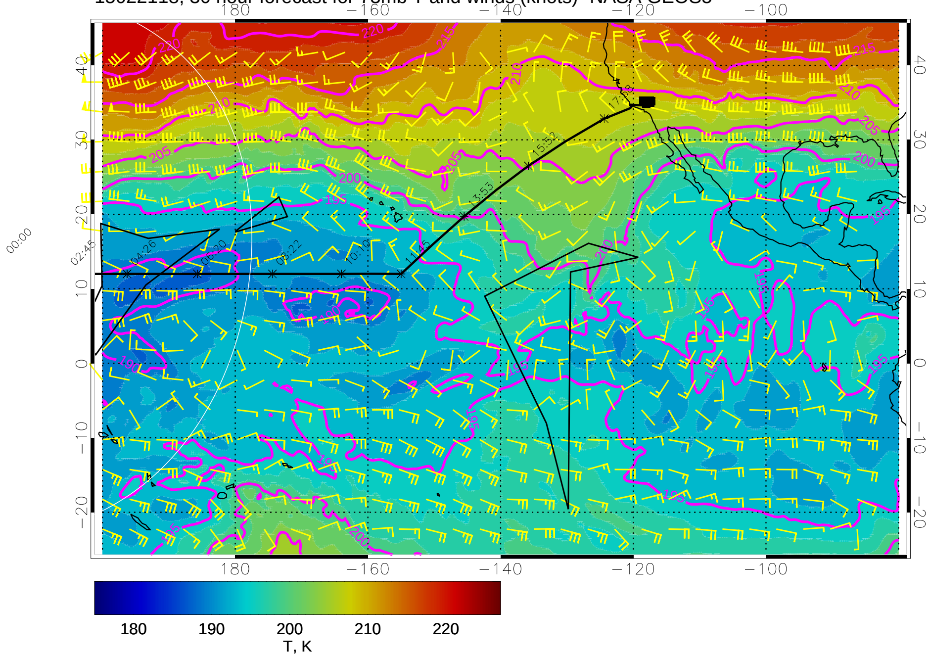
15022118, 30 hour forecast for 73mb T and winds (knots)- NASA GEOS5
