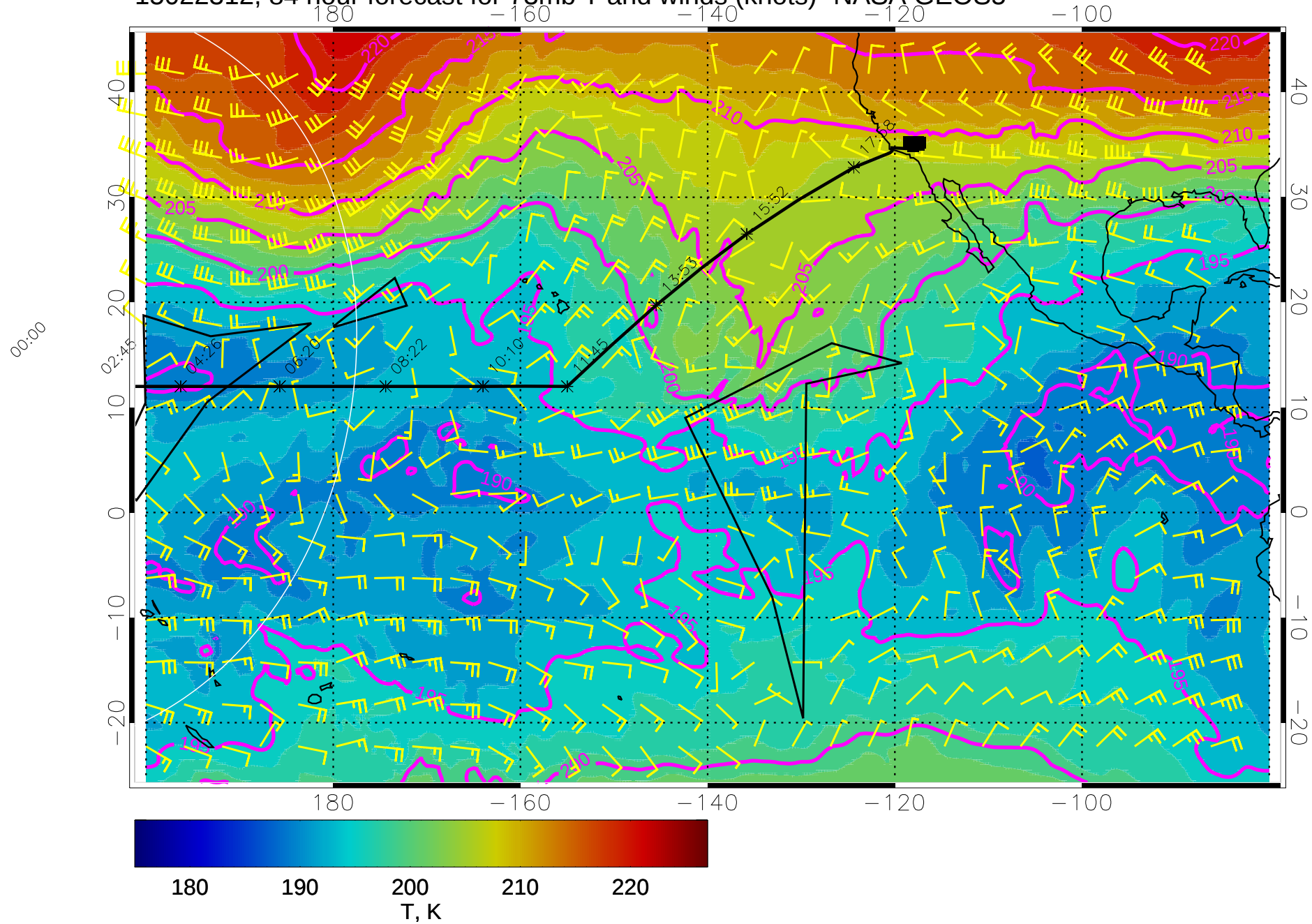
15022312, 84 hour forecast for 73mb T and winds (knots)- NASA GEOS5
