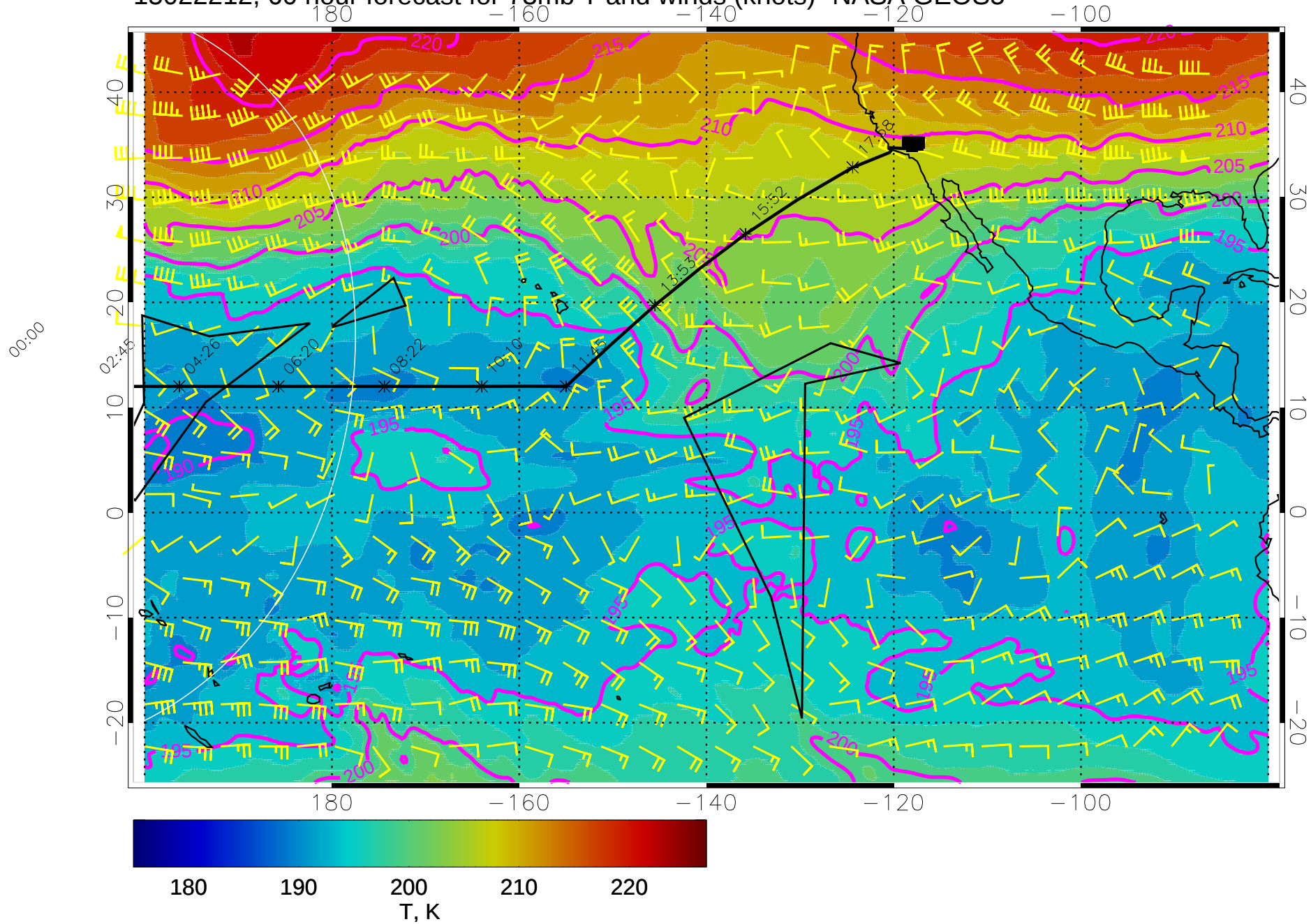
15022212, 60 hour forecast for 73mb T and winds (knots)- NASA GEOS5
