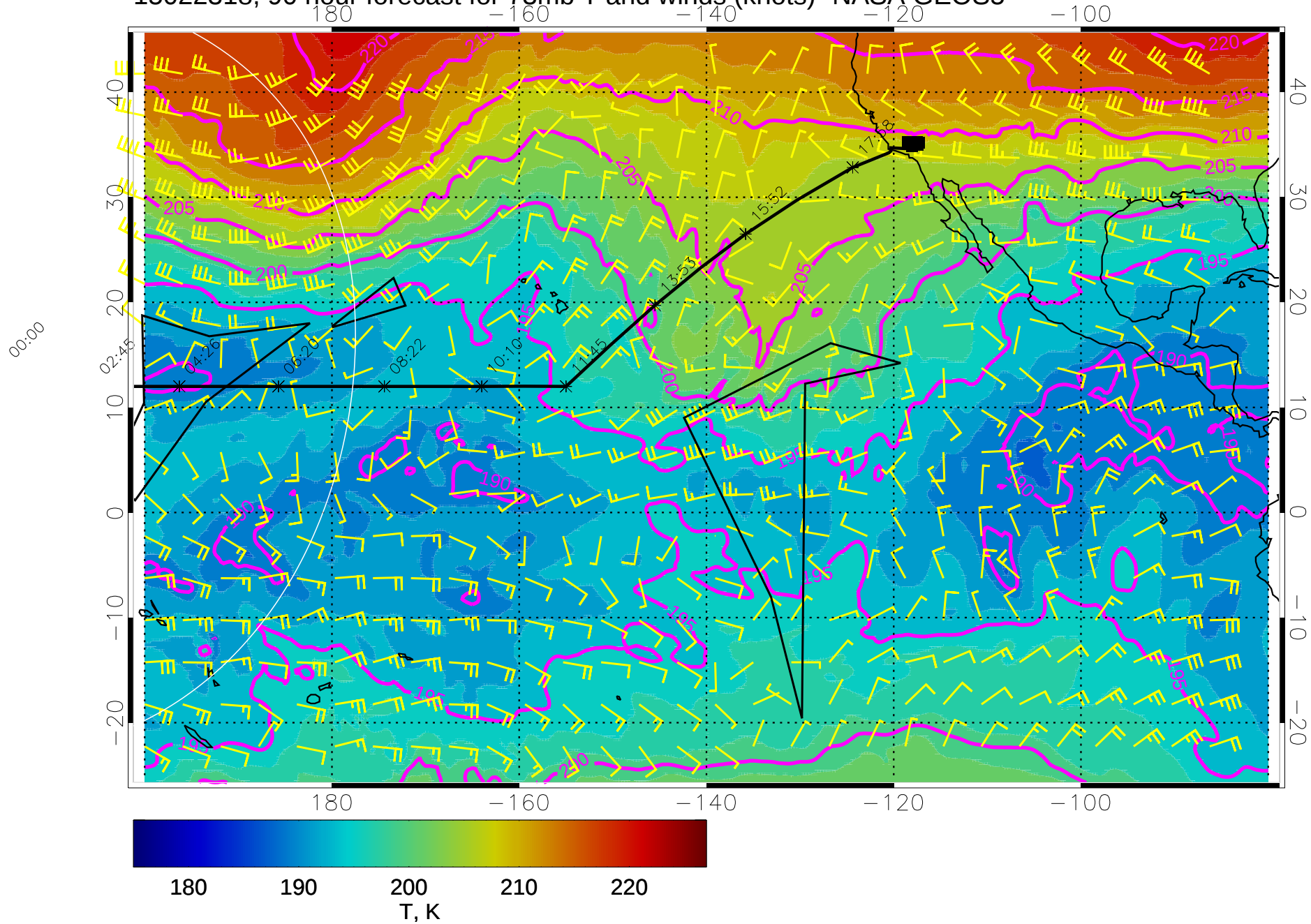
15022318, 90 hour forecast for 73mb T and winds (knots)- NASA GEOS5
