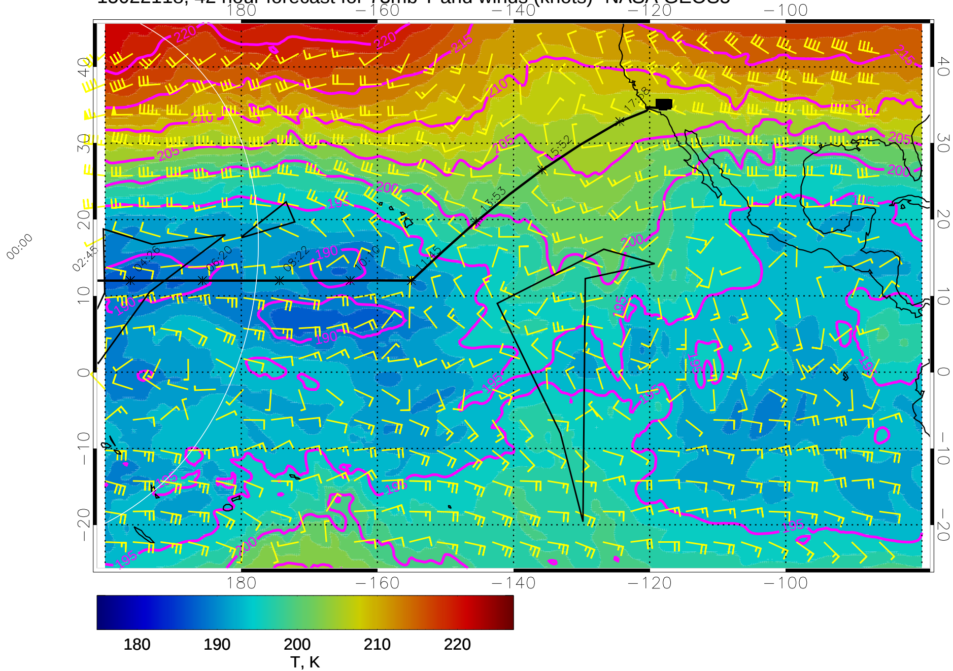
15022118, 42 hour forecast for 73mb T and winds (knots)- NASA GEOS5
