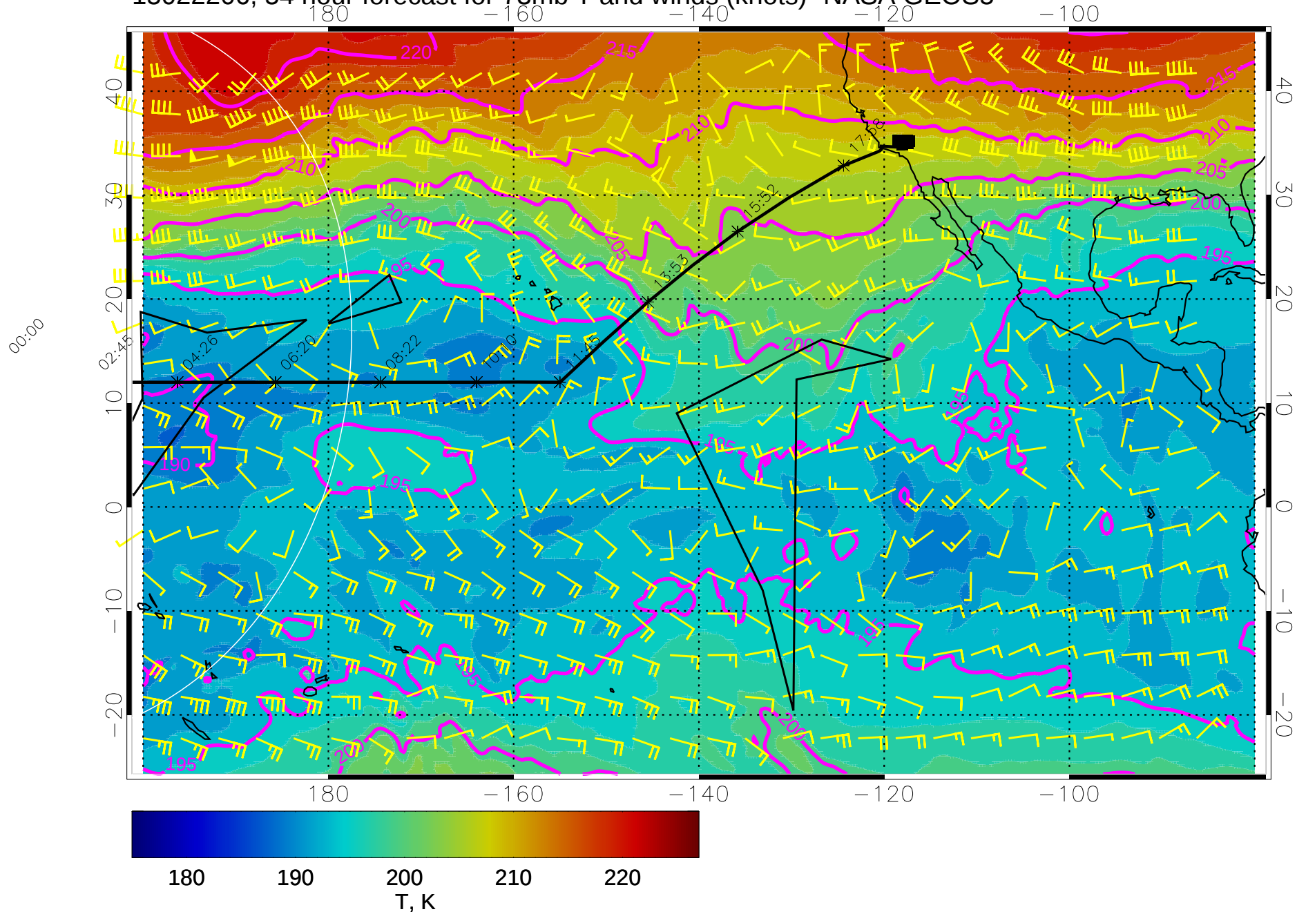
15022206, 54 hour forecast for 73mb T and winds (knots)- NASA GEOS5
