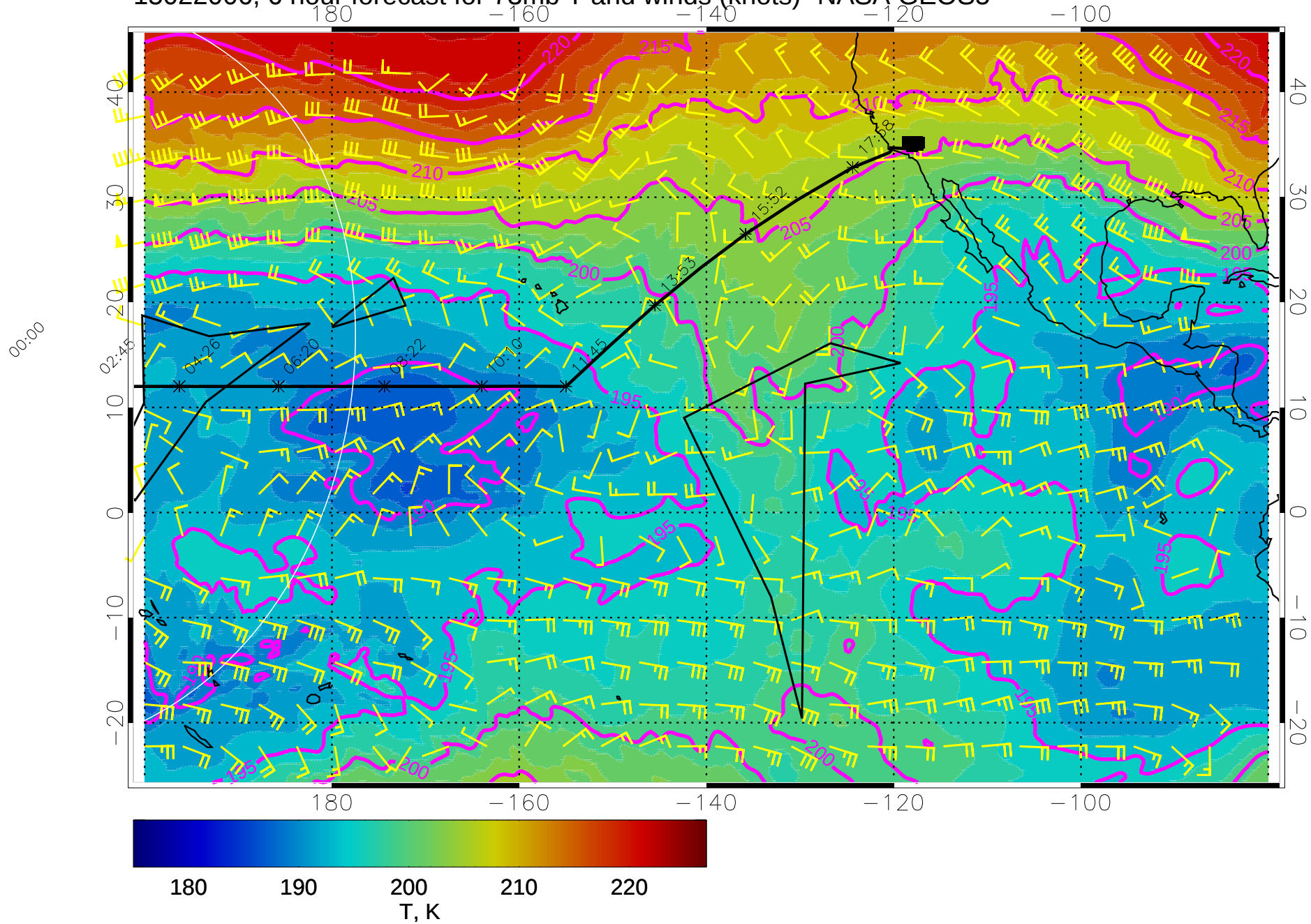
15022006, 6 hour forecast for 73mb T and winds (knots)- NASA GEOS5
