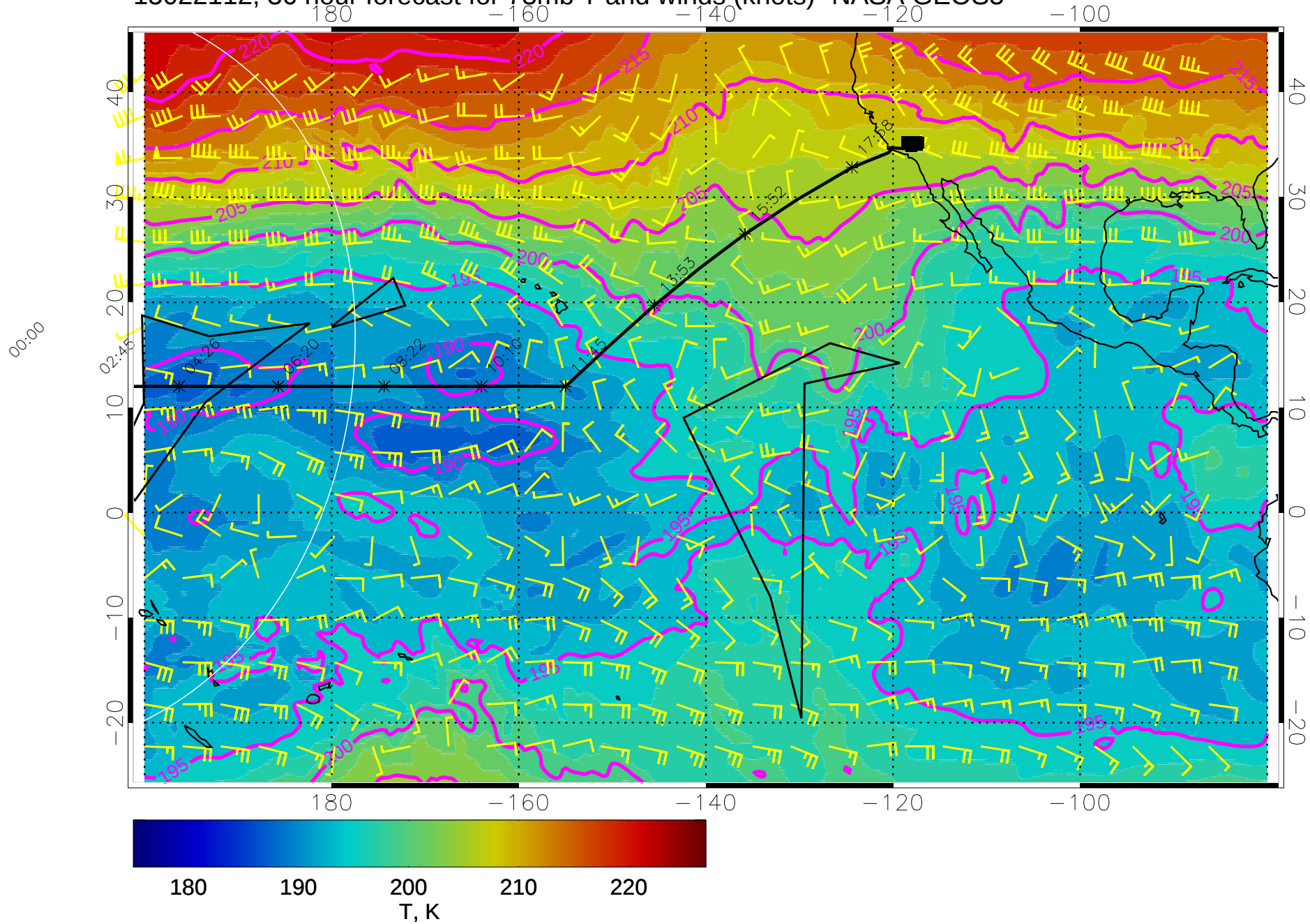
15022112, 36 hour forecast for 73mb T and winds (knots)- NASA GEOS5
