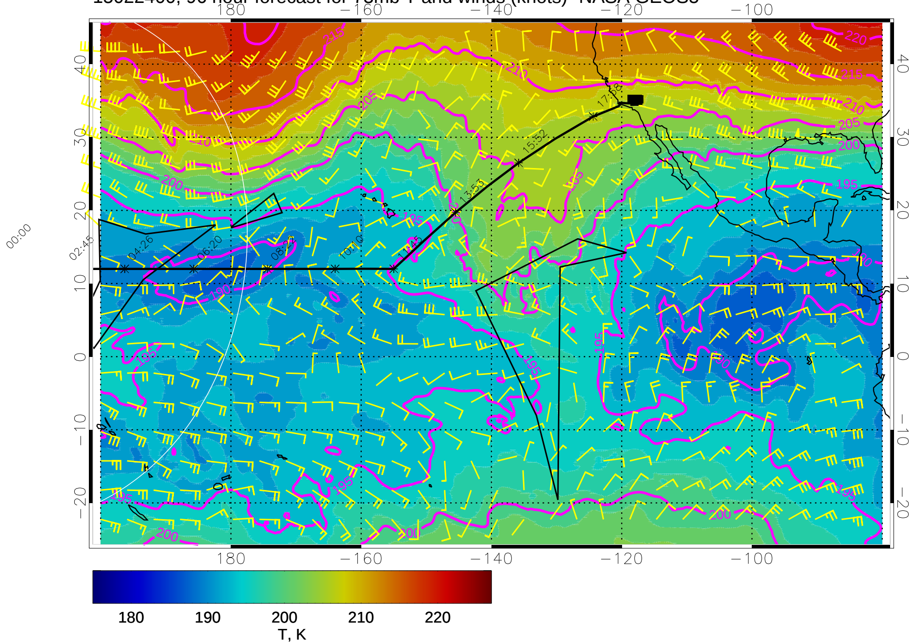
15022400, 96 hour forecast for 73mb T and winds (knots)- NASA GEOS5
