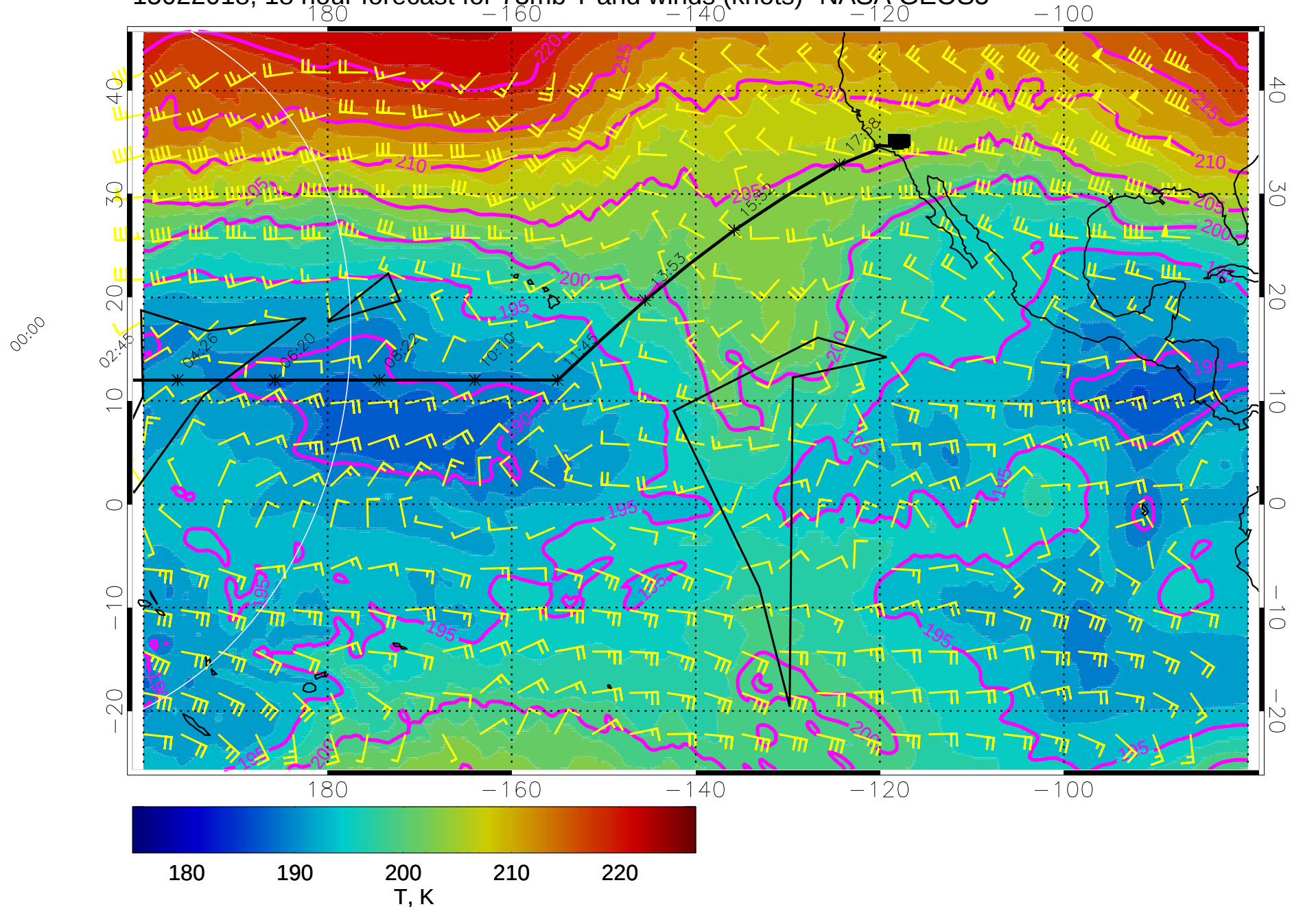
15022018, 18 hour forecast for 73mb T and winds (knots)- NASA GEOS5
