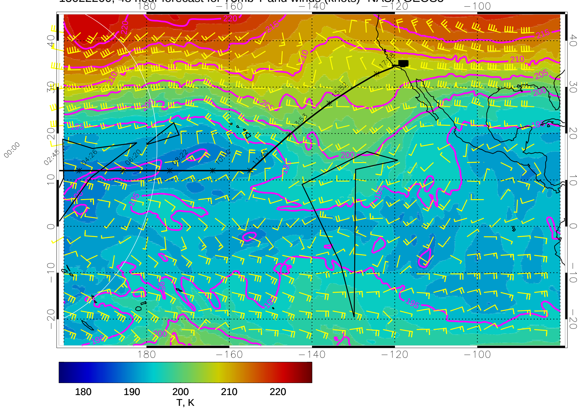
15022200, 48 hour forecast for 73mb T and winds (knots)- NASA GEOS5
