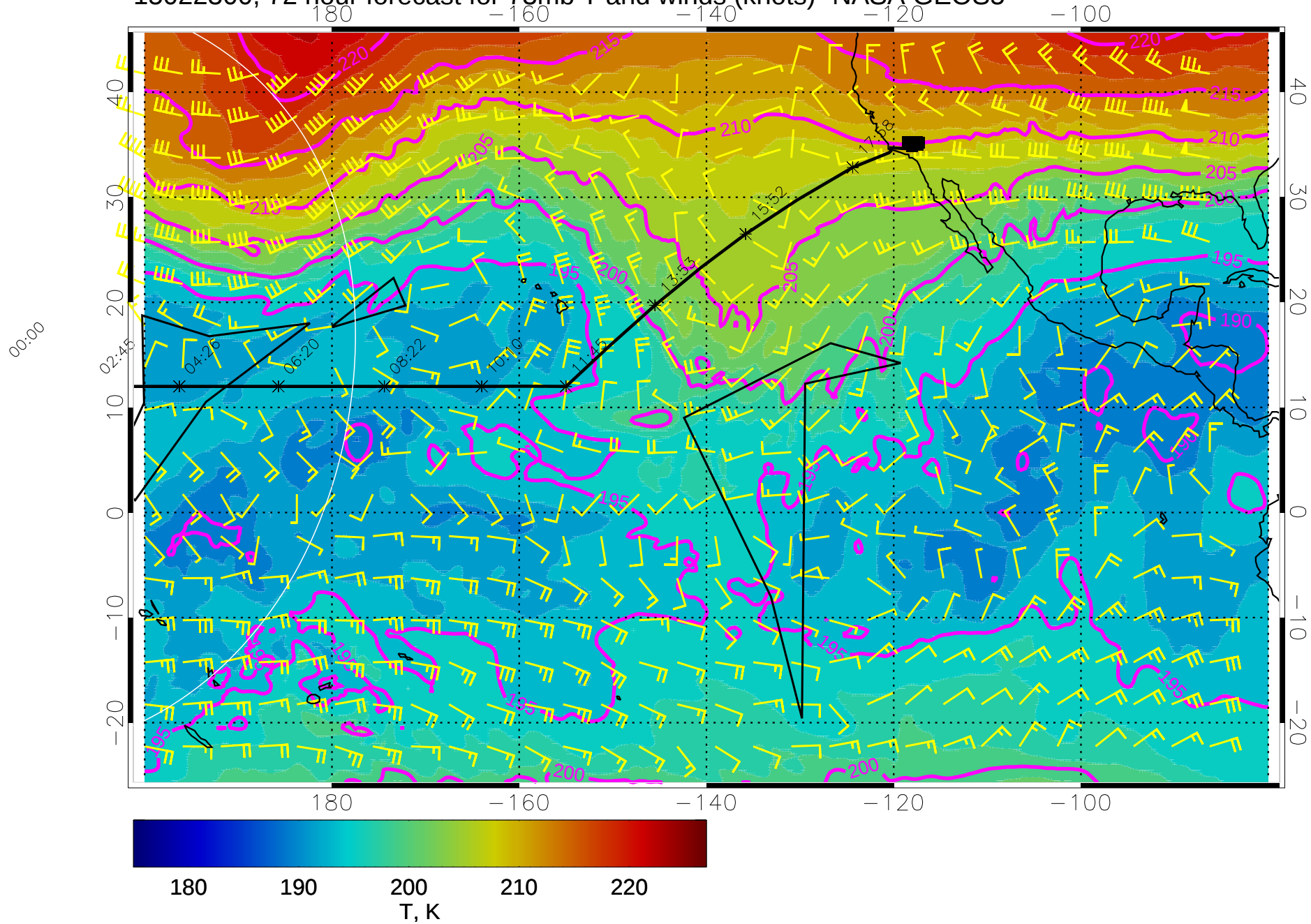
15022300, 72 hour forecast for 73mb T and winds (knots)- NASA GEOS5
