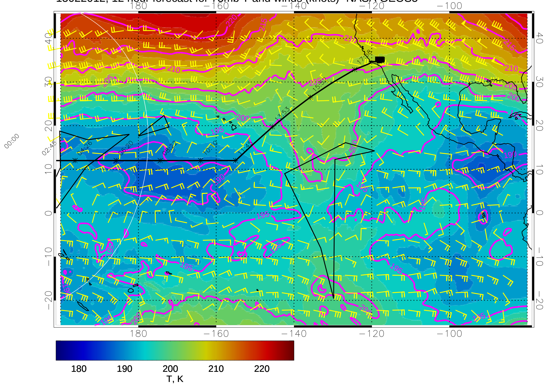
15022012, 12 hour forecast for 73mb T and winds (knots)- NASA GEOS5
