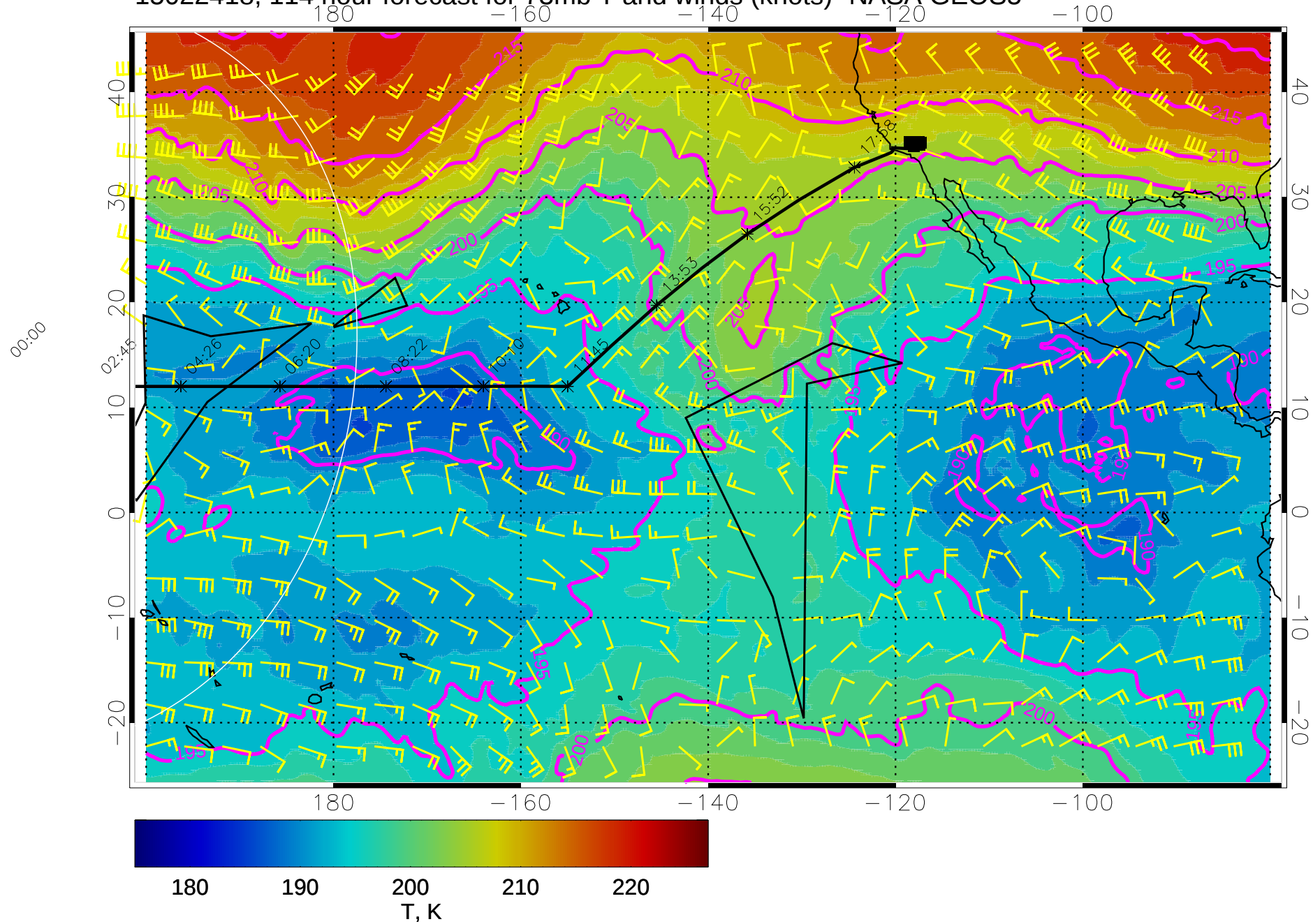
15022418, 114 hour forecast for 73mb T and winds (knots)- NASA GEOS5
