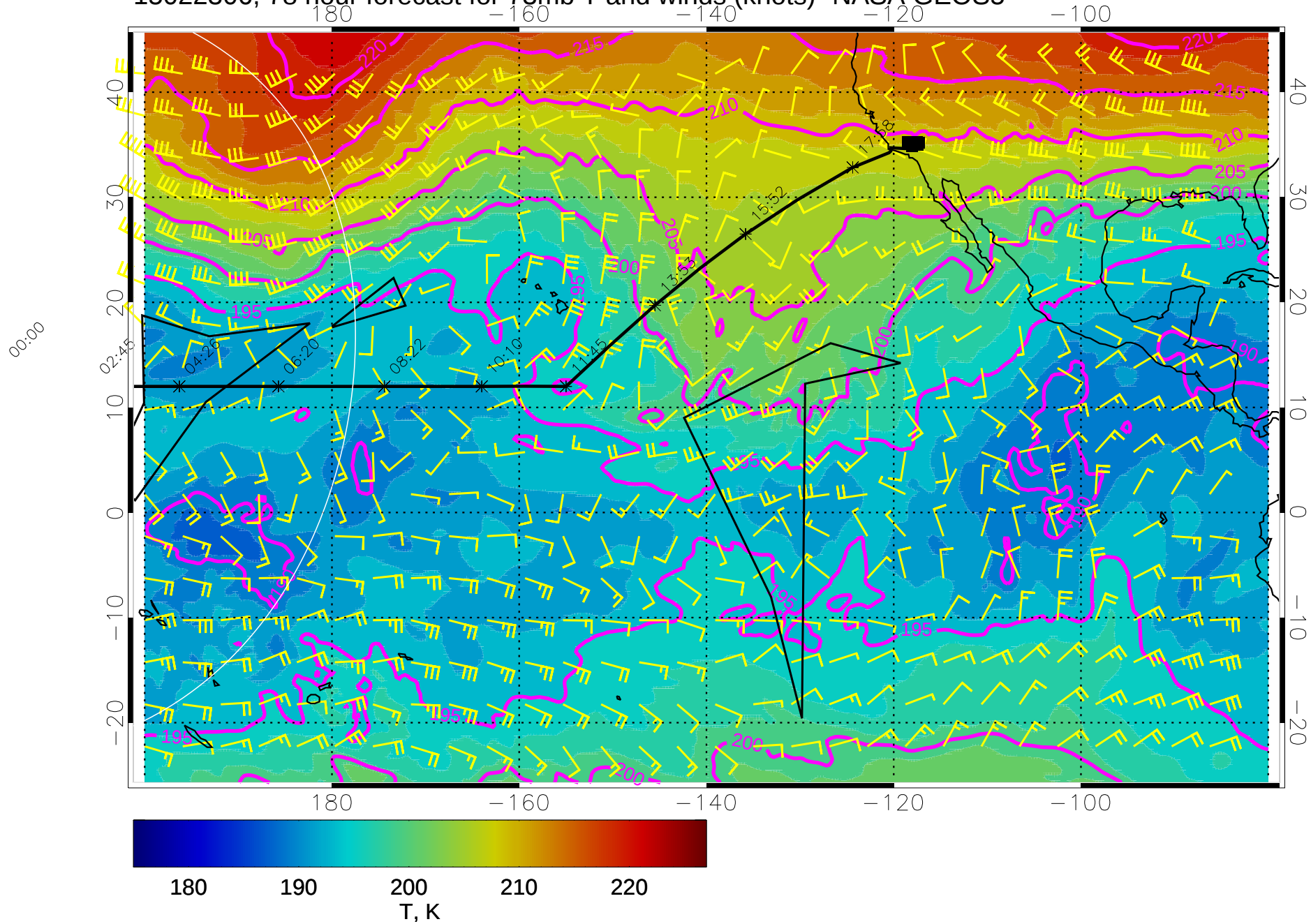
15022306, 78 hour forecast for 73mb T and winds (knots)- NASA GEOS5
