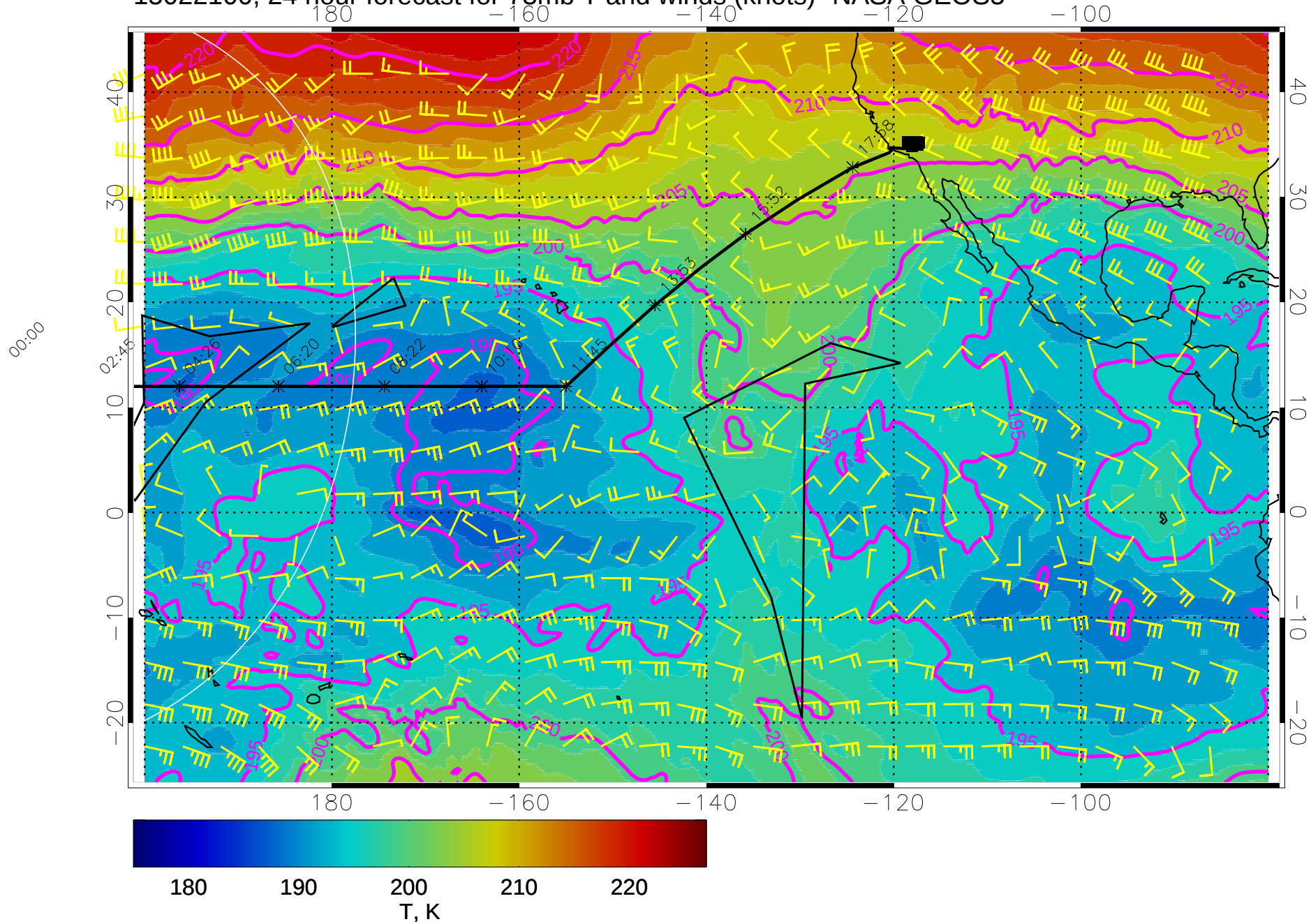
15022100, 24 hour forecast for 73mb T and winds (knots)- NASA GEOS5
