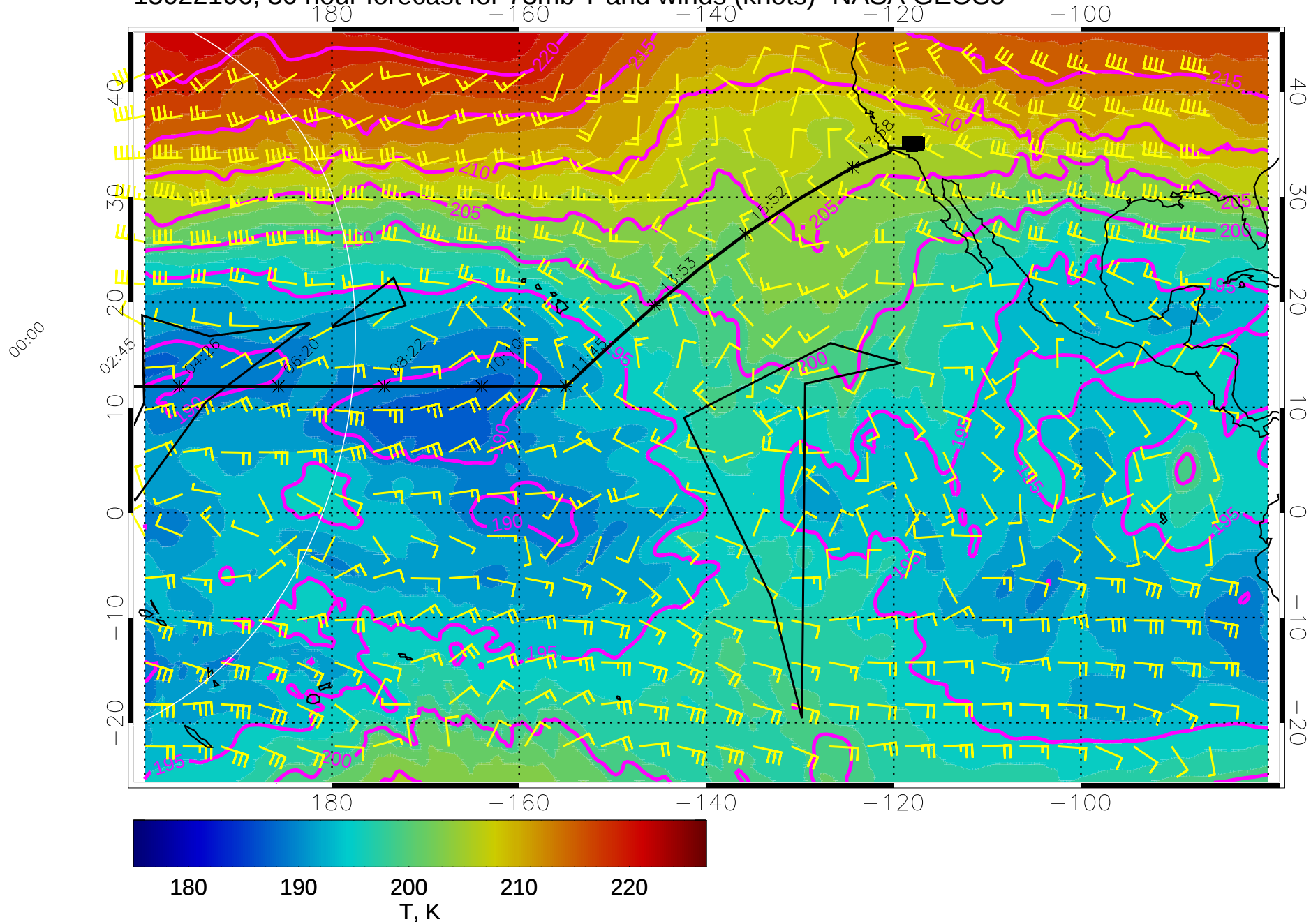
15022106, 30 hour forecast for 73mb T and winds (knots)- NASA GEOS5
